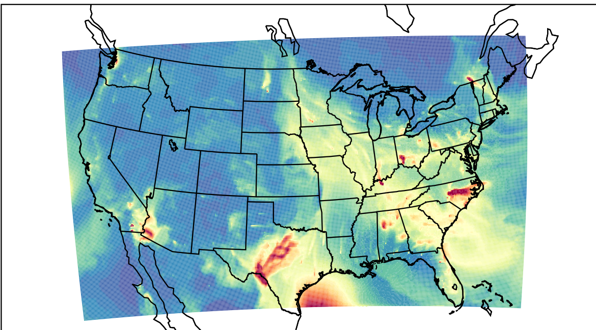
WRF 2023-02-27_07:00:00
