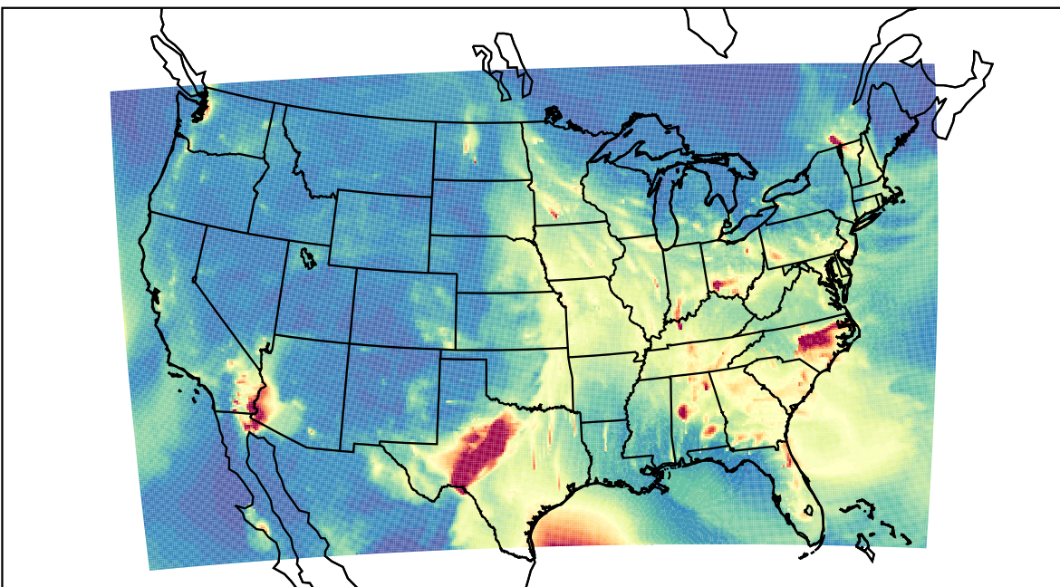
WRF 2023-02-27_05:00:00
