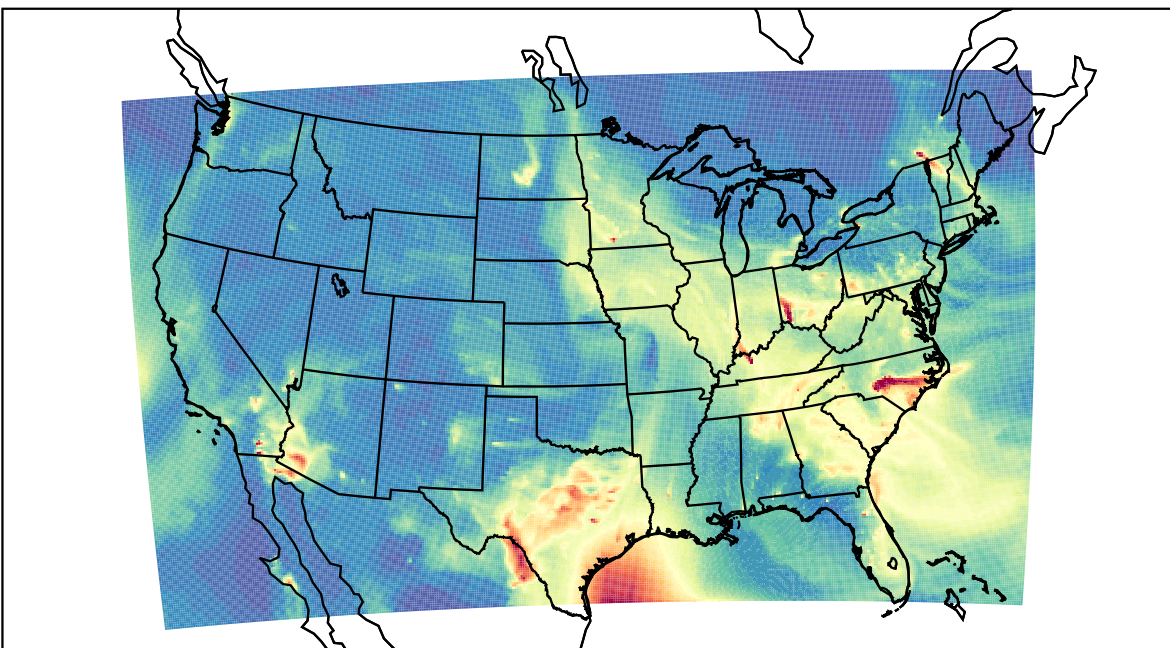
WRF 2023-02-27_09:00:00
