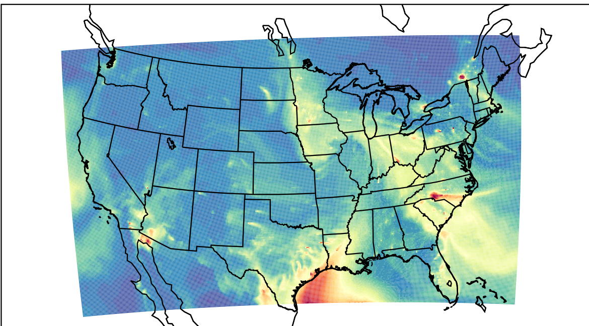
WRF 2023-02-27_14:00:00
