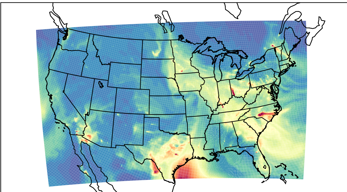
WRF 2023-02-27_10:00:00
