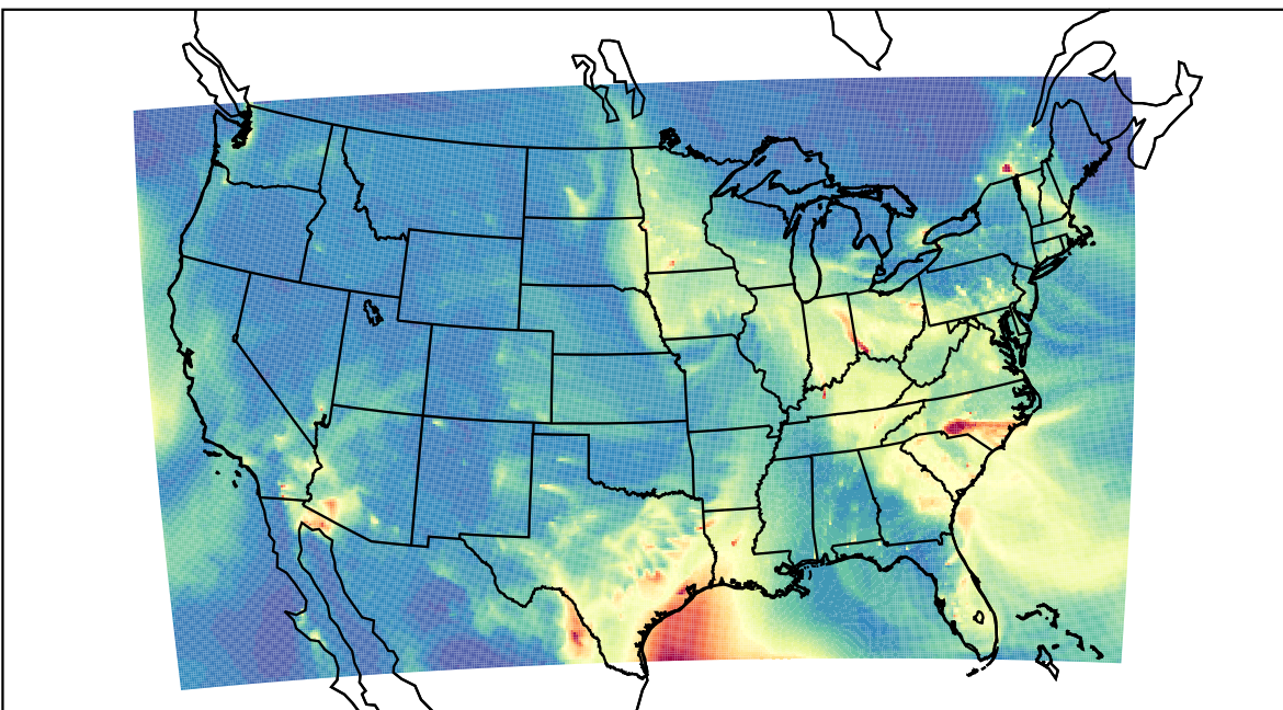
WRF 2023-02-27_12:00:00
