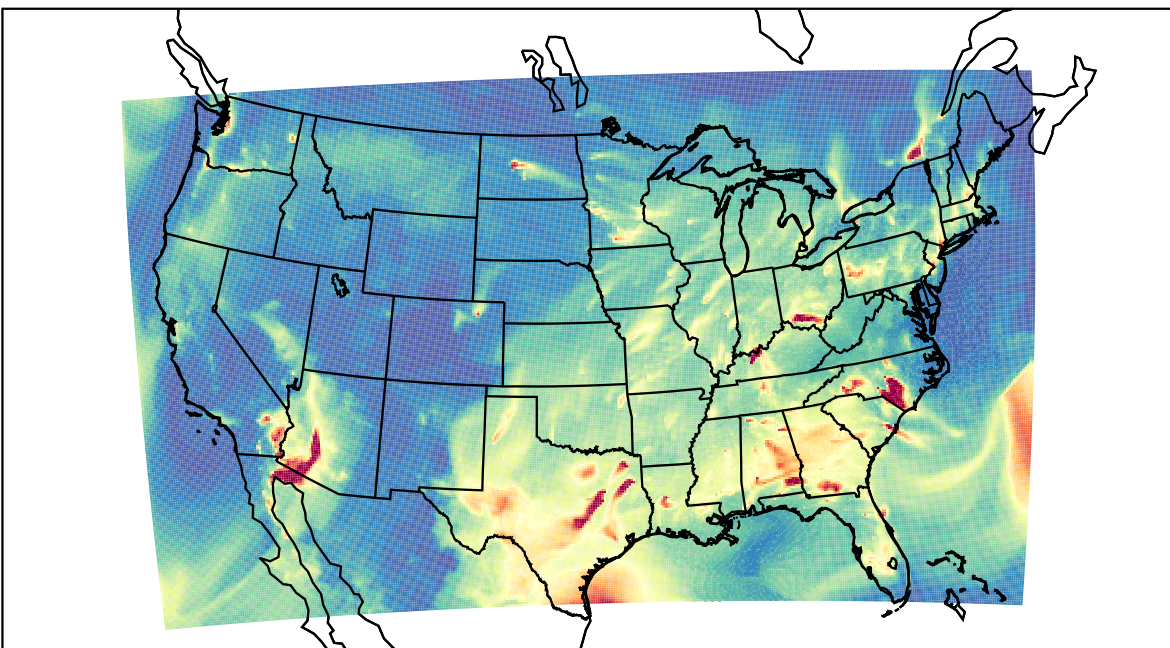
WRF 2023-02-26_06:00:00
