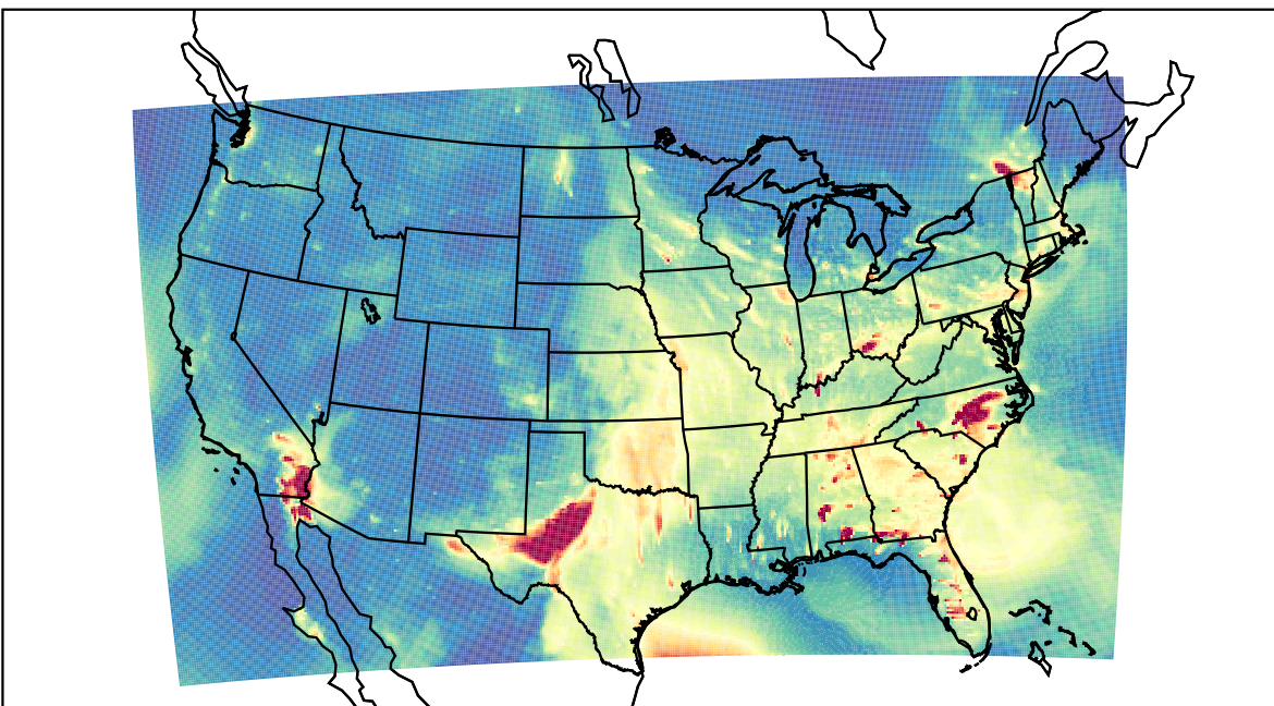
WRF 2023-02-27_02:00:00
