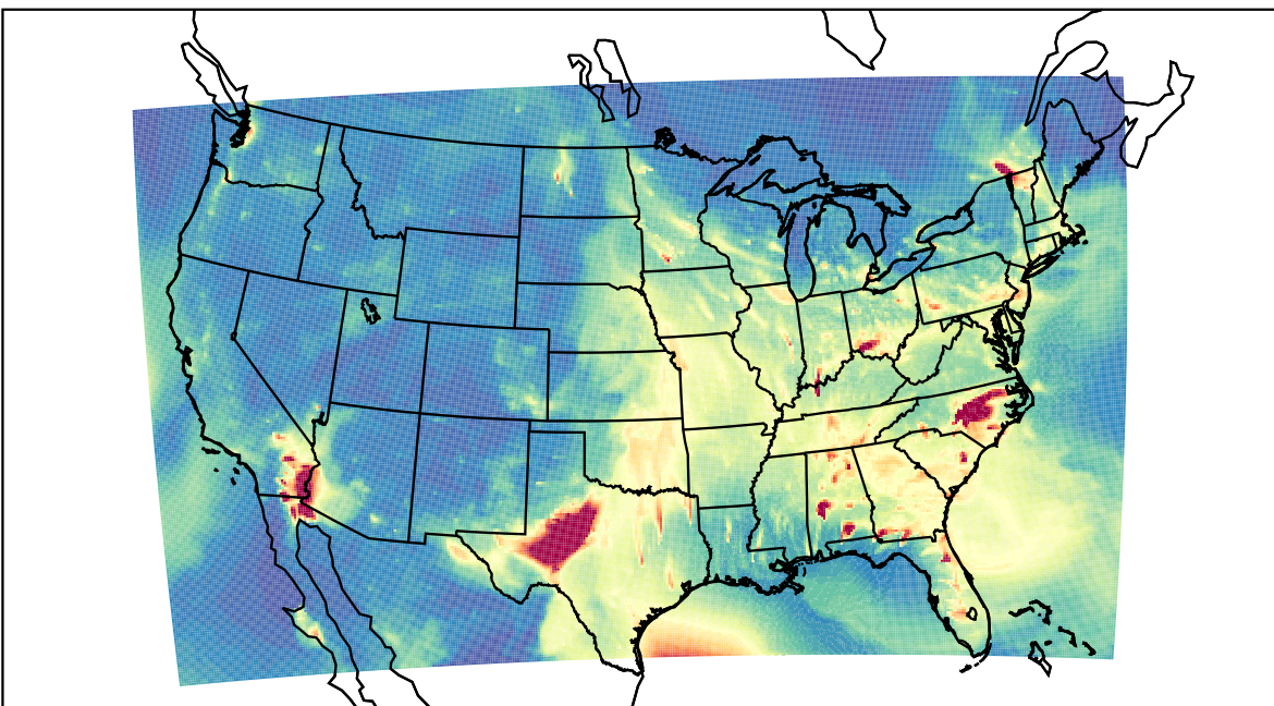
WRF 2023-02-27_03:00:00
