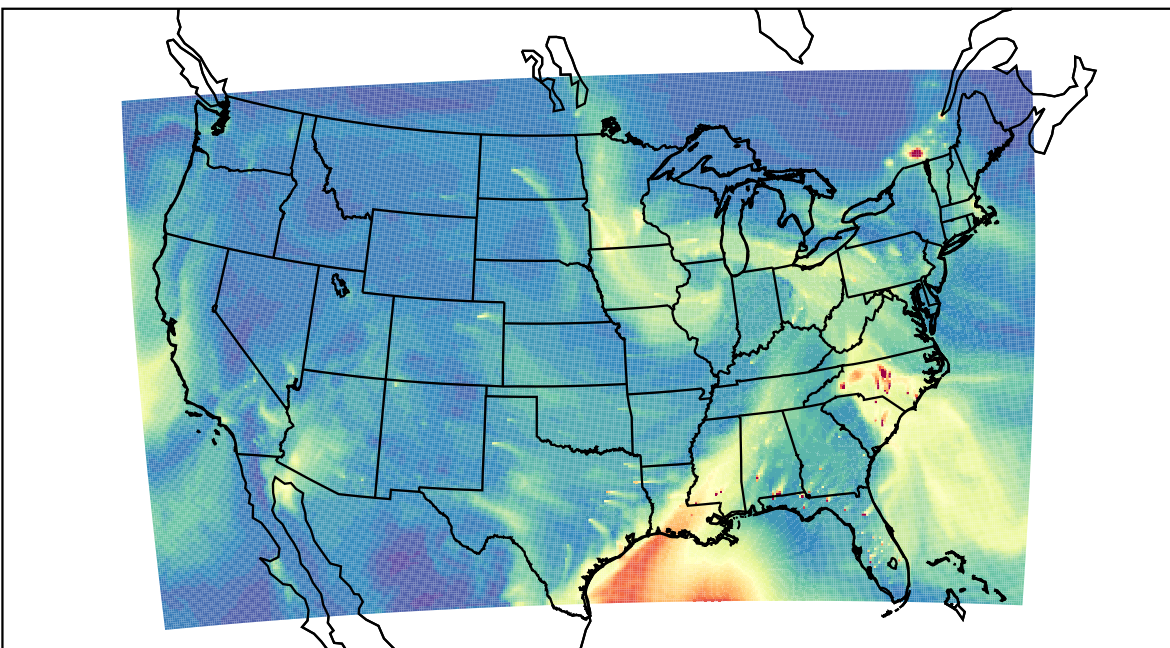
WRF 2023-02-27_19:00:00
