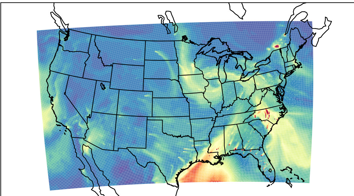
WRF 2023-02-27_20:00:00
