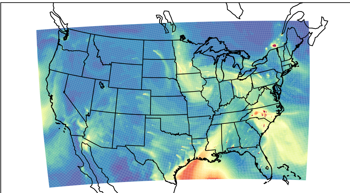
WRF 2023-02-27_18:00:00
