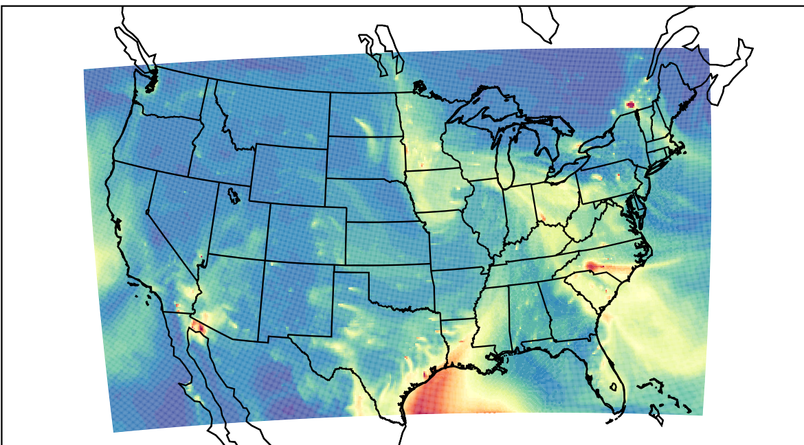
WRF 2023-02-27_15:00:00
