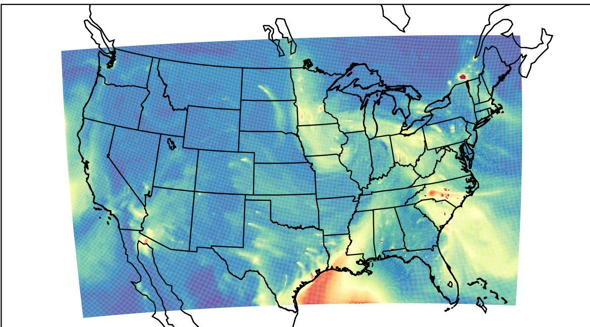
WRF 2023-02-27_17:00:00
