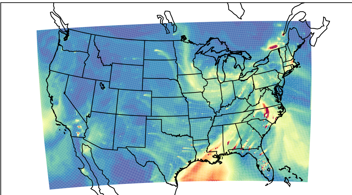
WRF 2023-02-27_23:00:00
