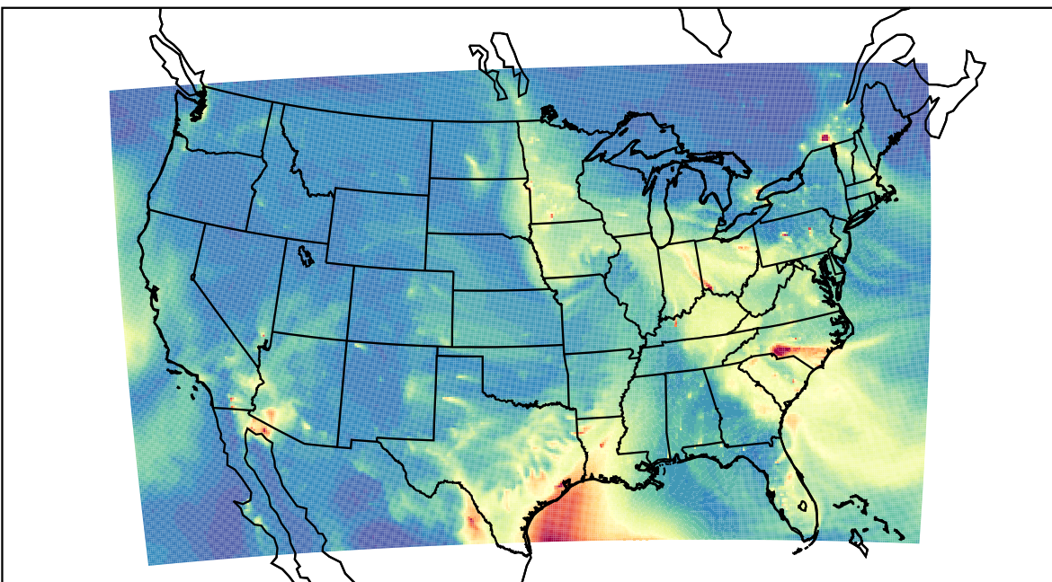
WRF 2023-02-27_13:00:00
