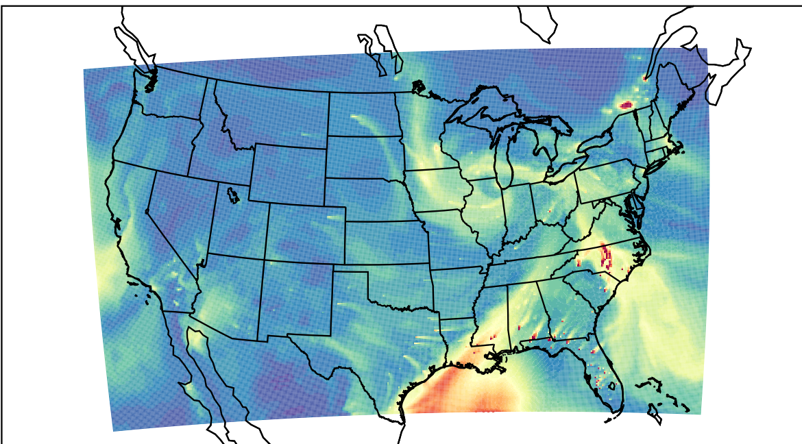
WRF 2023-02-27_21:00:00
