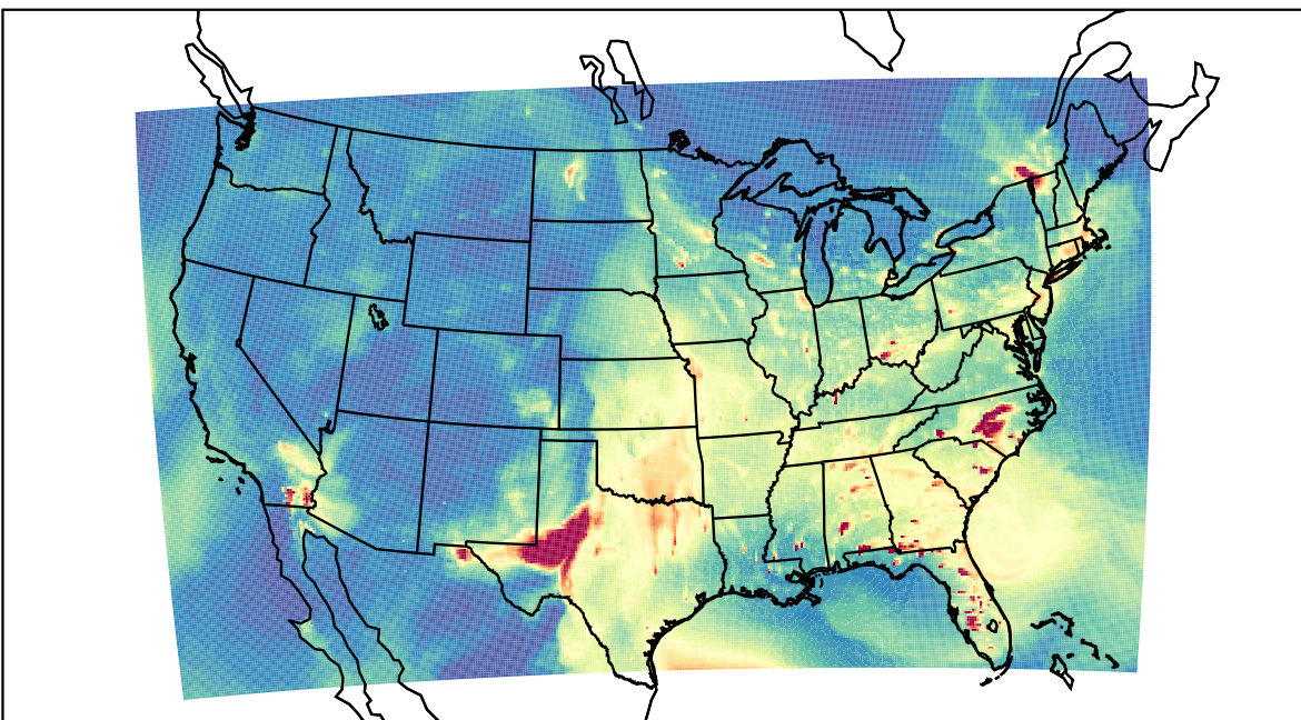
WRF 2023-02-27_00:00:00
