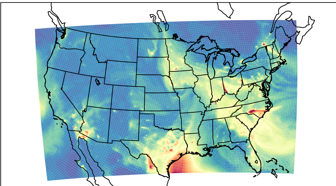
WRF 2023-02-27_11:00:00
