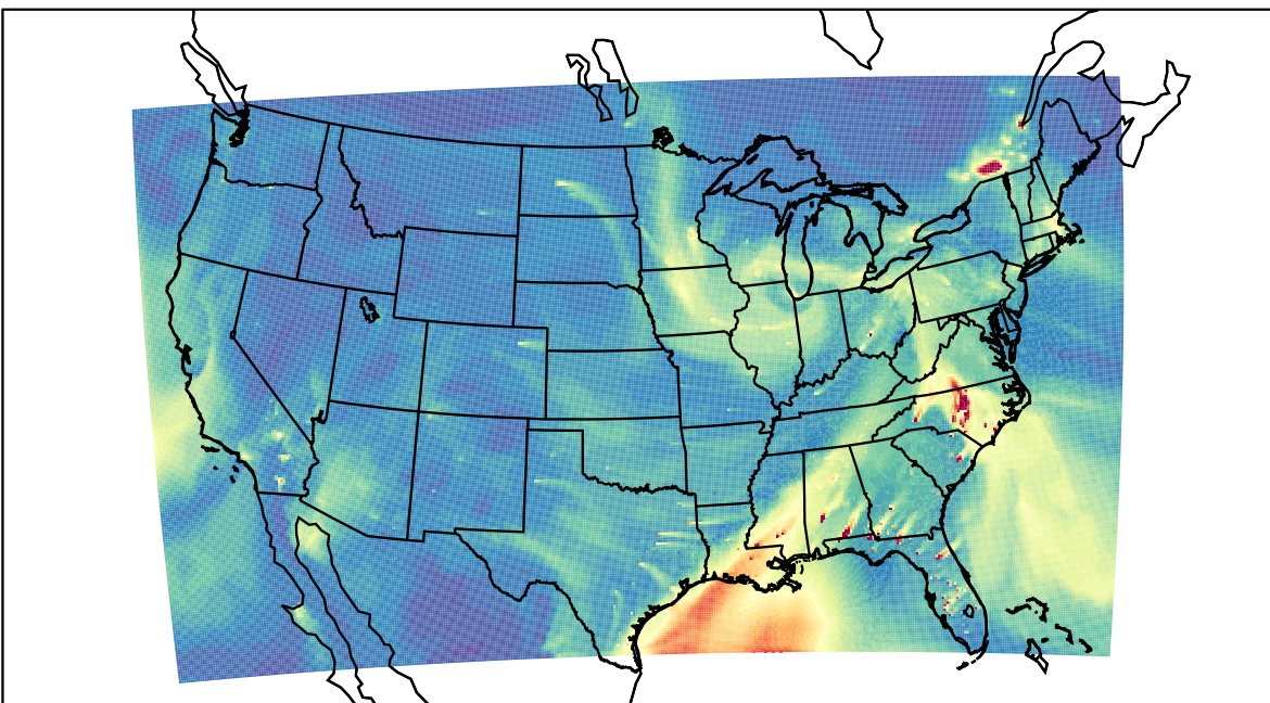
WRF 2023-02-27_22:00:00
