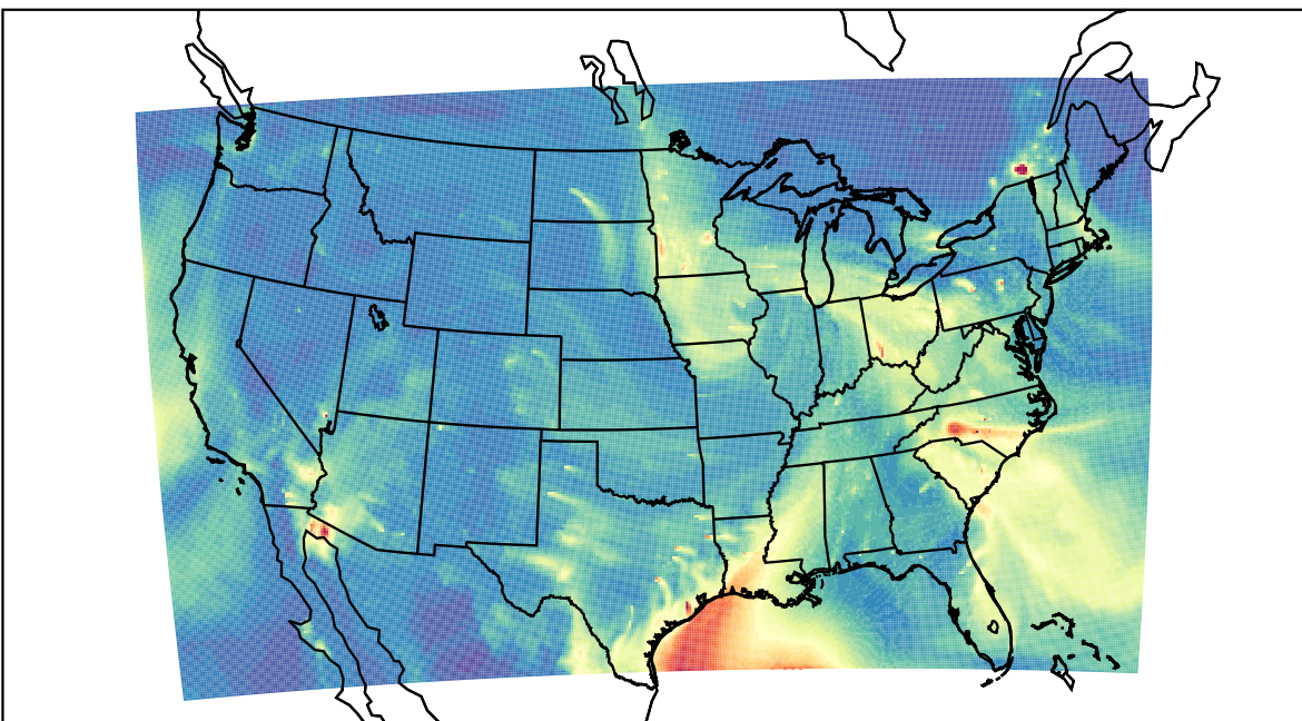
WRF 2023-02-27_16:00:00
