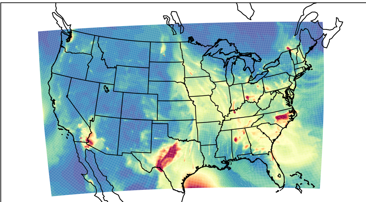
WRF 2023-02-27_06:00:00
