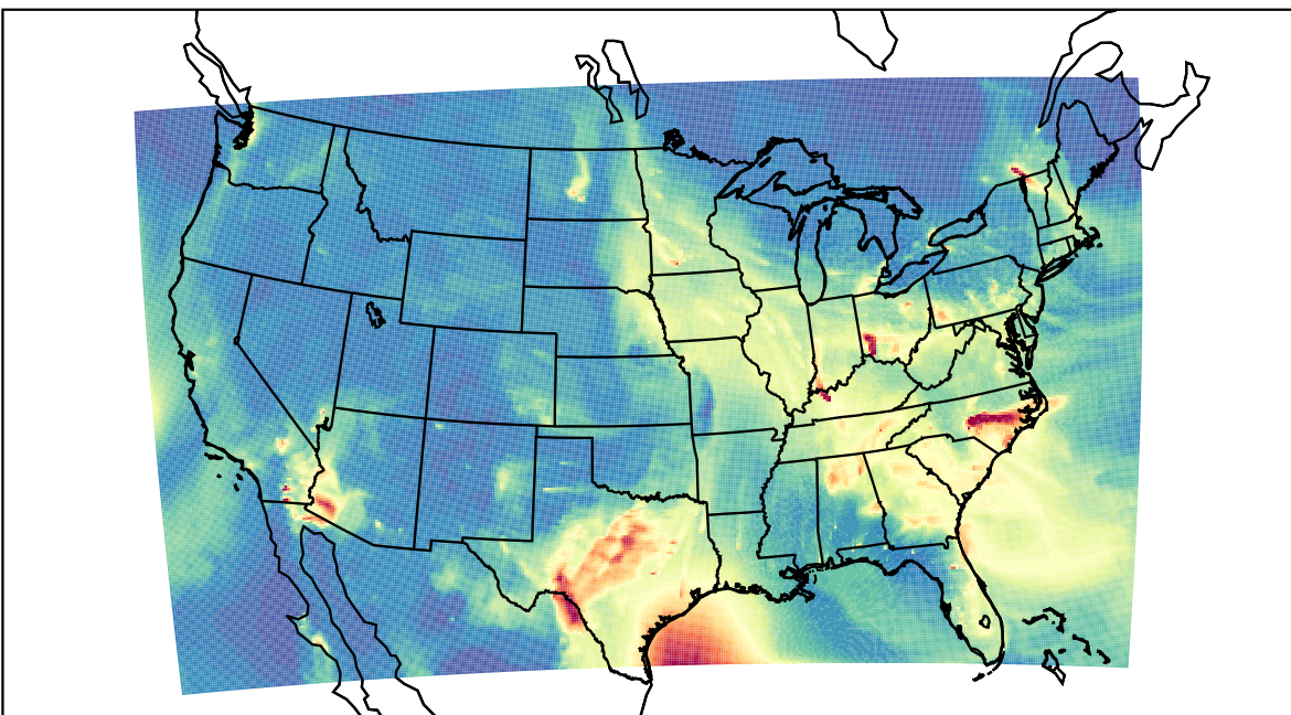
WRF 2023-02-27_08:00:00
