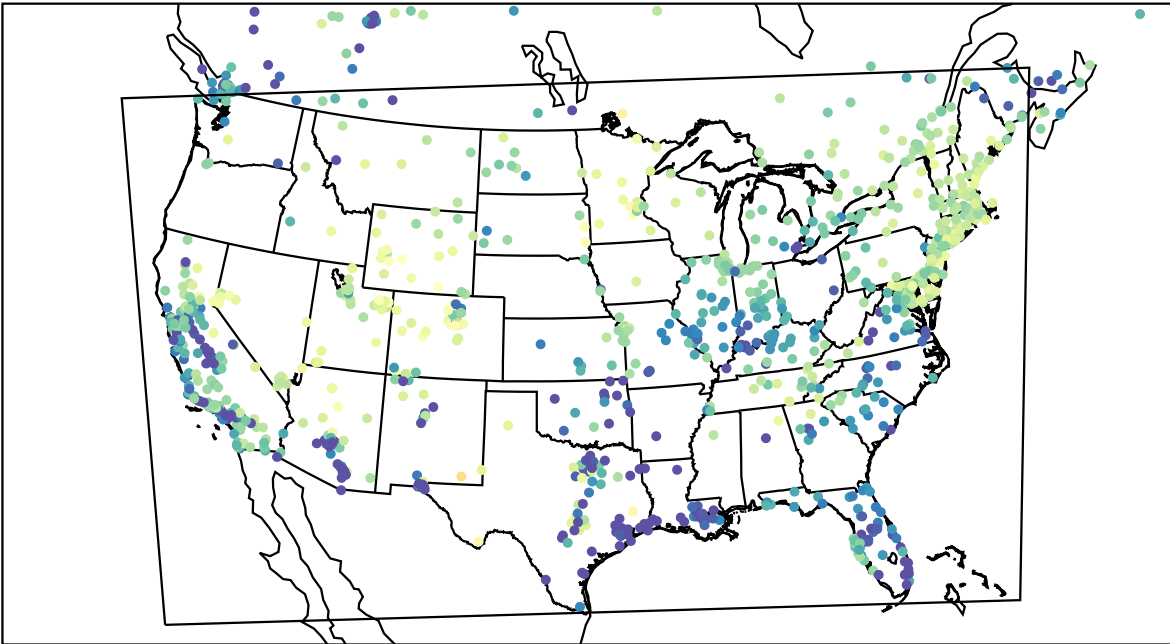
AirNOW (2023-02-28_06:00:00)
