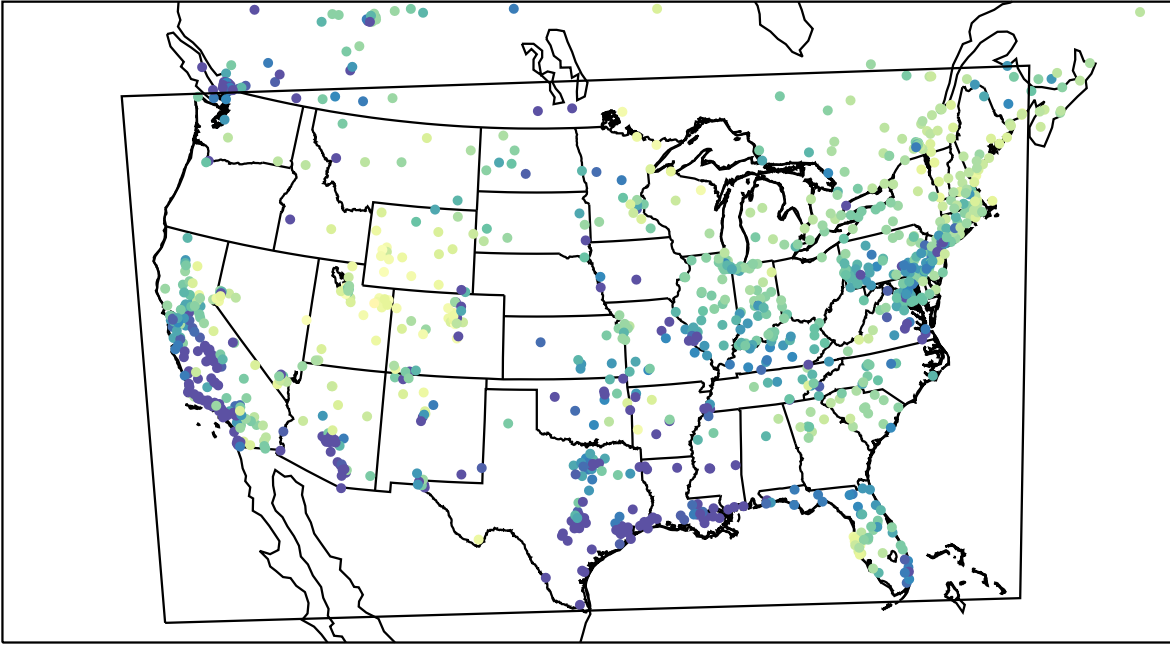
AirNOW (2023-02-28_14:00:00)
