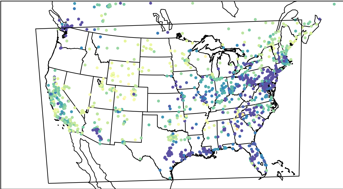
AirNOW (2023-03-01_05:00:00)
