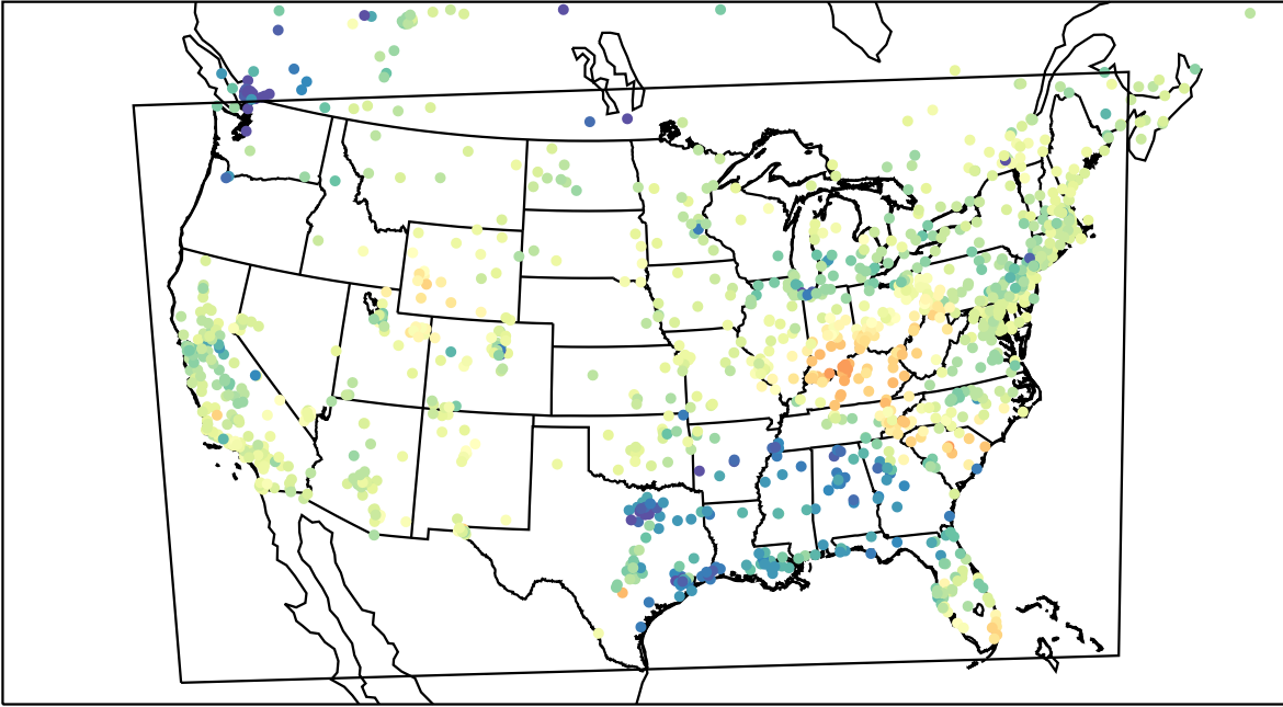
AirNOW (2023-03-01_19:00:00)
