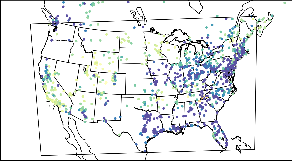
AirNOW (2023-03-01_11:00:00)
