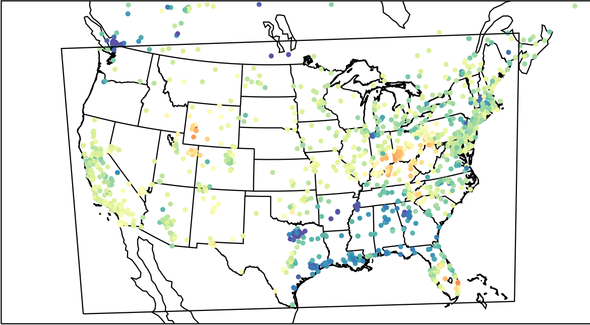
AirNOW (2023-03-01_22:00:00)
