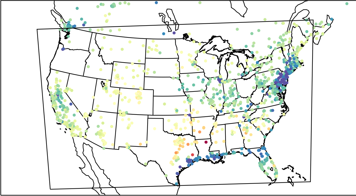
AirNOW (2023-02-28_23:00:00)
