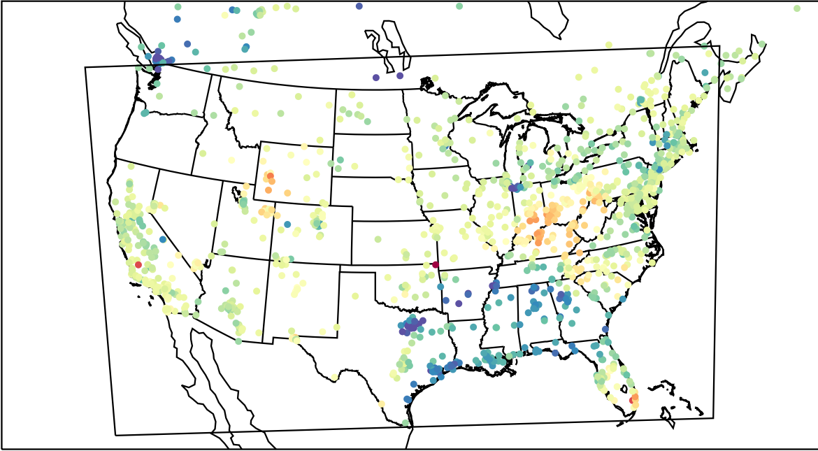
AirNOW (2023-03-01_21:00:00)
