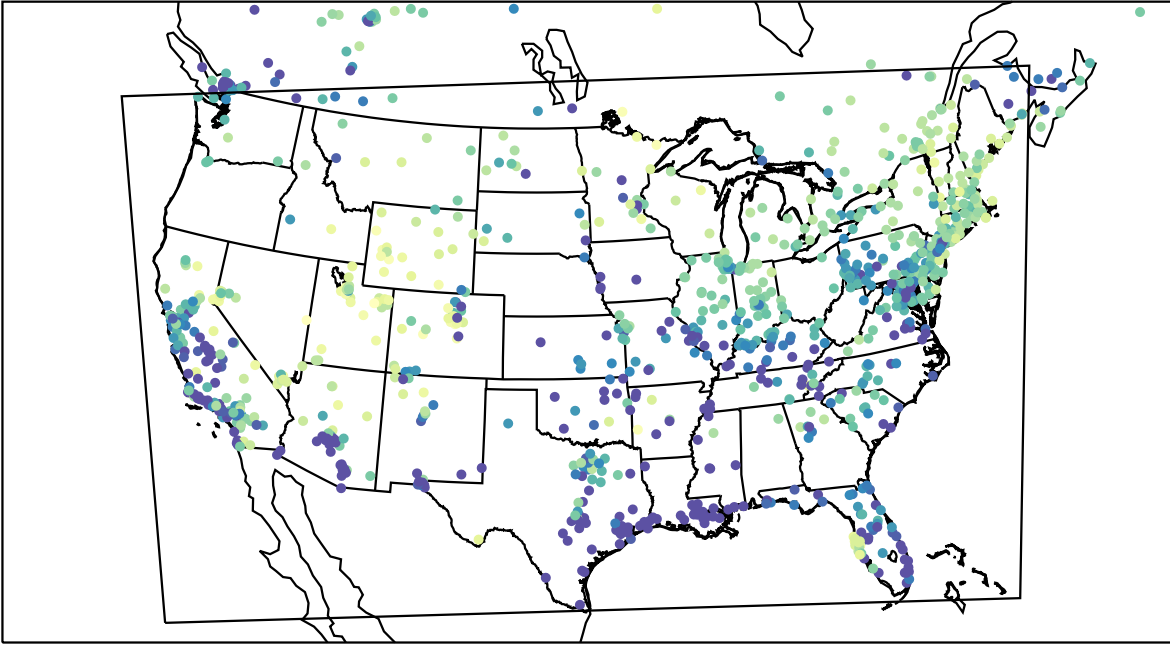
AirNOW (2023-02-28_12:00:00)
