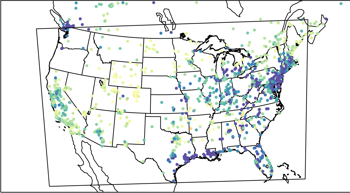
AirNOW (2023-03-01_02:00:00)
