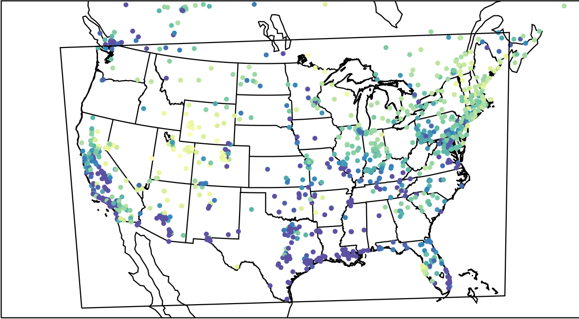
AirNOW (2023-02-28_13:00:00)
