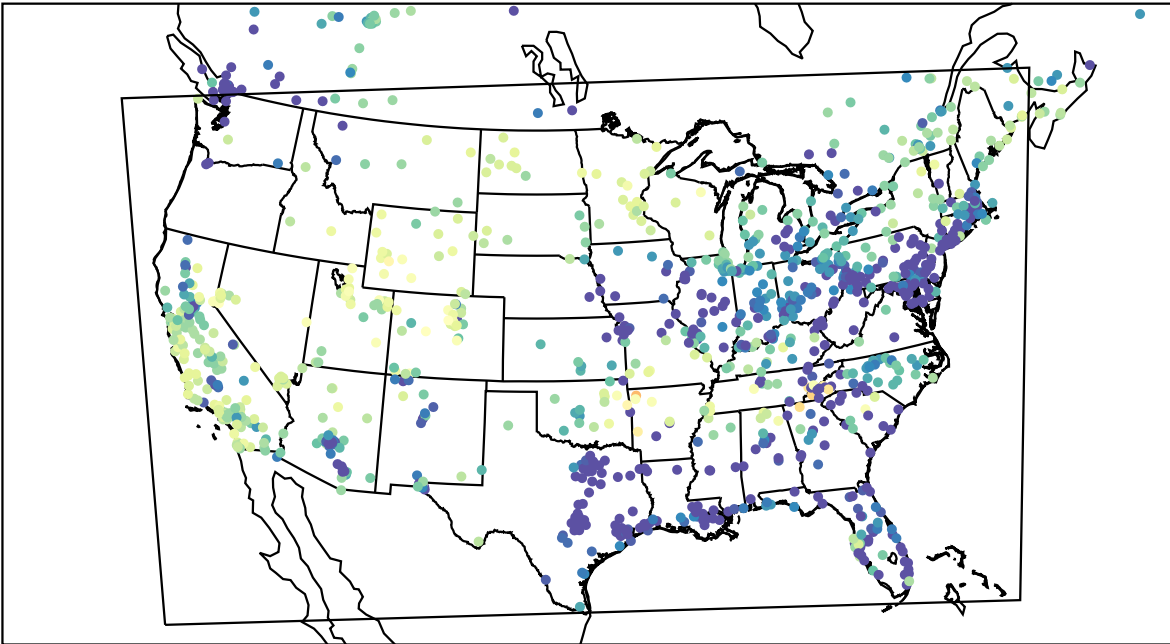
AirNOW (2023-03-01_09:00:00)
