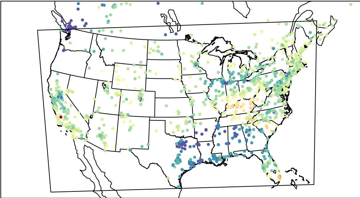
AirNOW (2023-03-01_17:00:00)
