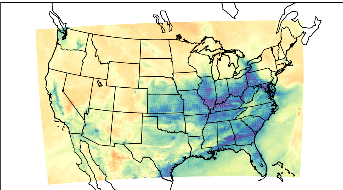
WRF (2023-02-28_12:00:00)
