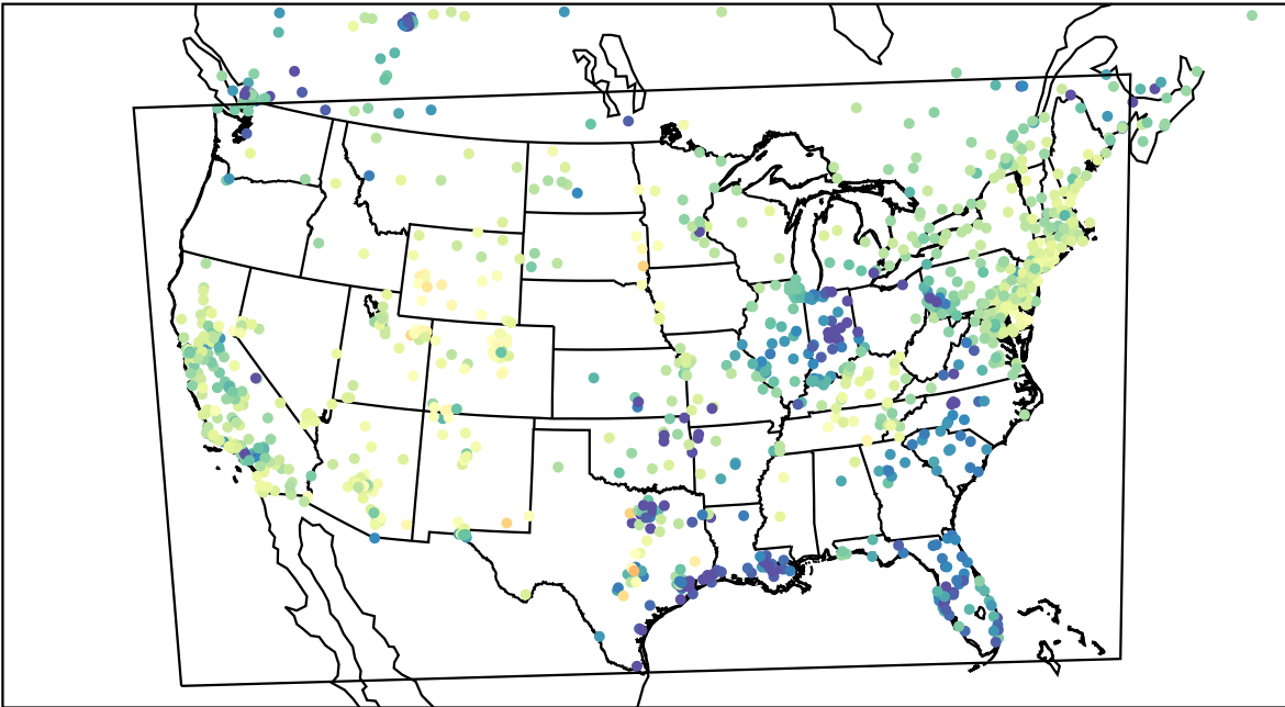
AirNOW (2023-02-28_01:00:00)
