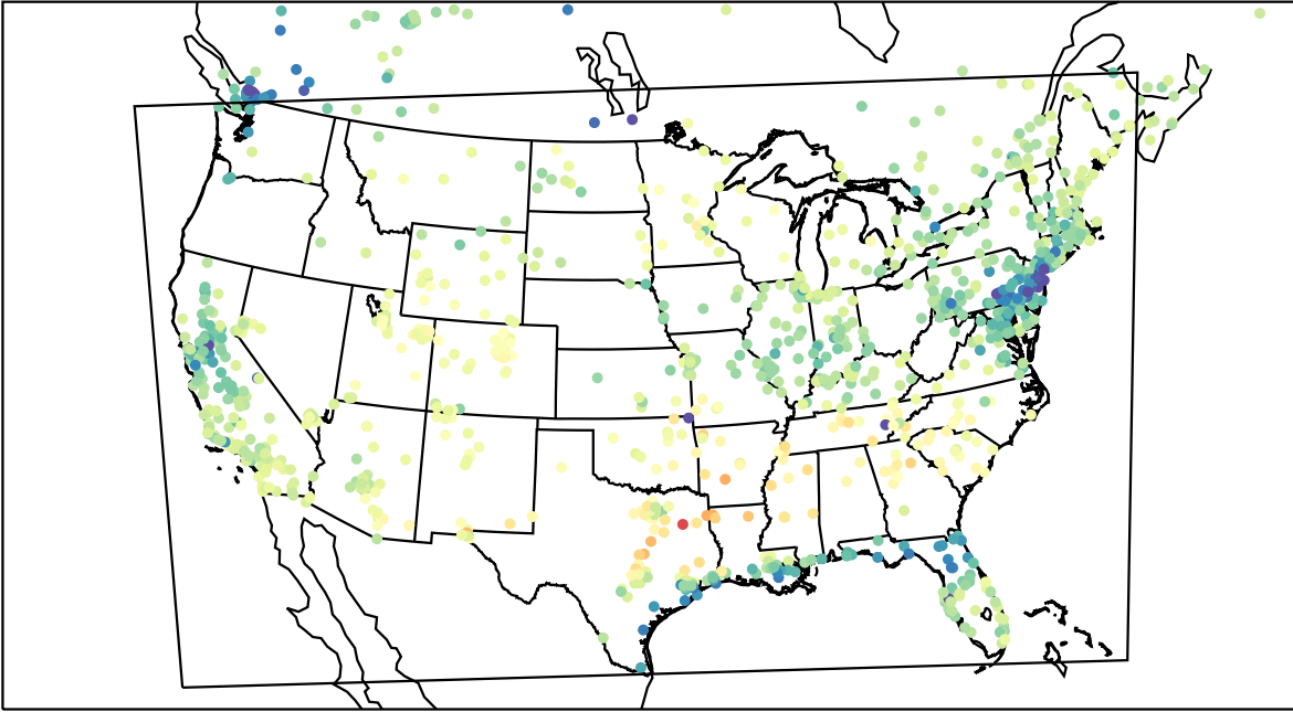
AirNOW (2023-02-28_19:00:00)
