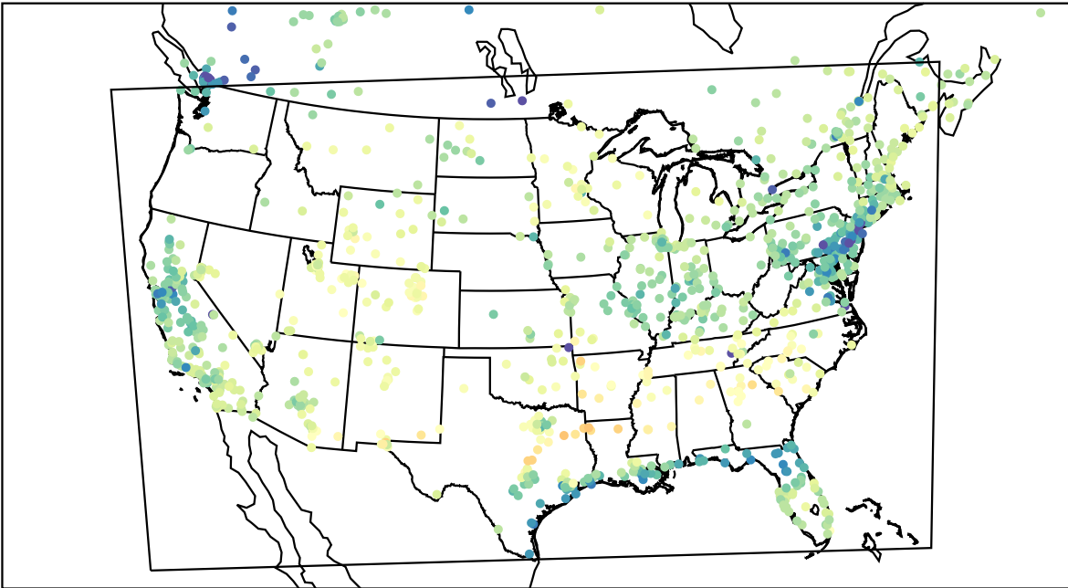
AirNOW (2023-02-28_18:00:00)
