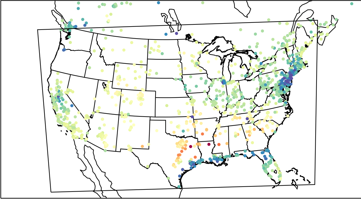
AirNOW (2023-02-28_22:00:00)
