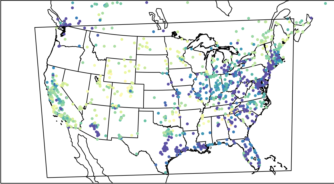
AirNOW (2023-03-01_06:00:00)
