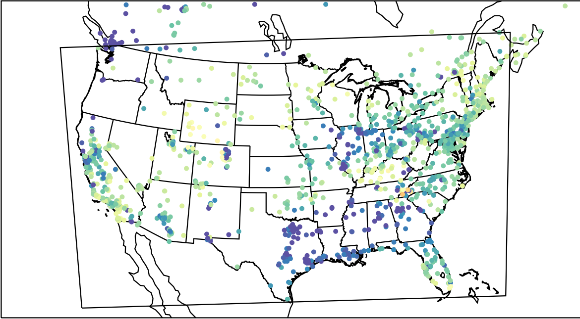
AirNOW (2023-03-01_15:00:00)
