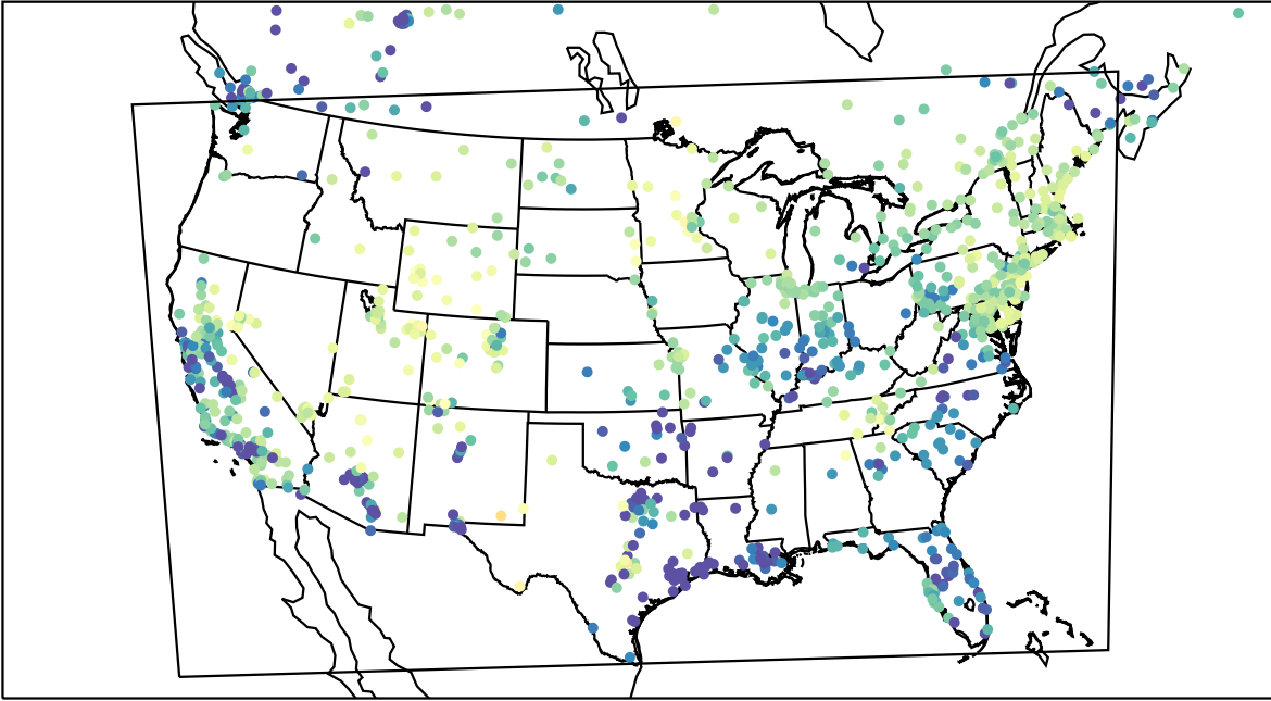
AirNOW (2023-02-28_05:00:00)
