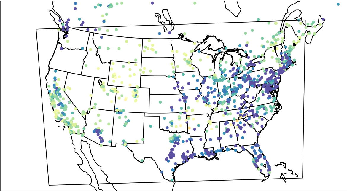
AirNOW (2023-03-01_07:00:00)
