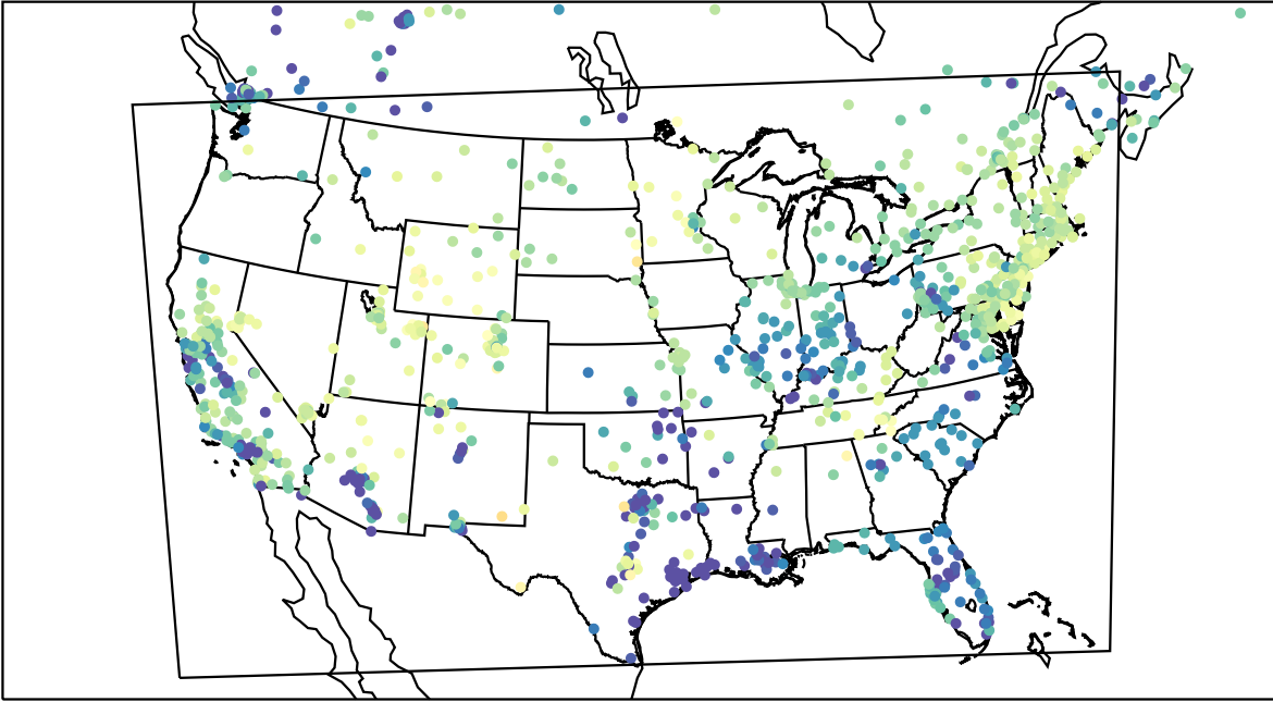
AirNOW (2023-02-28_04:00:00)
