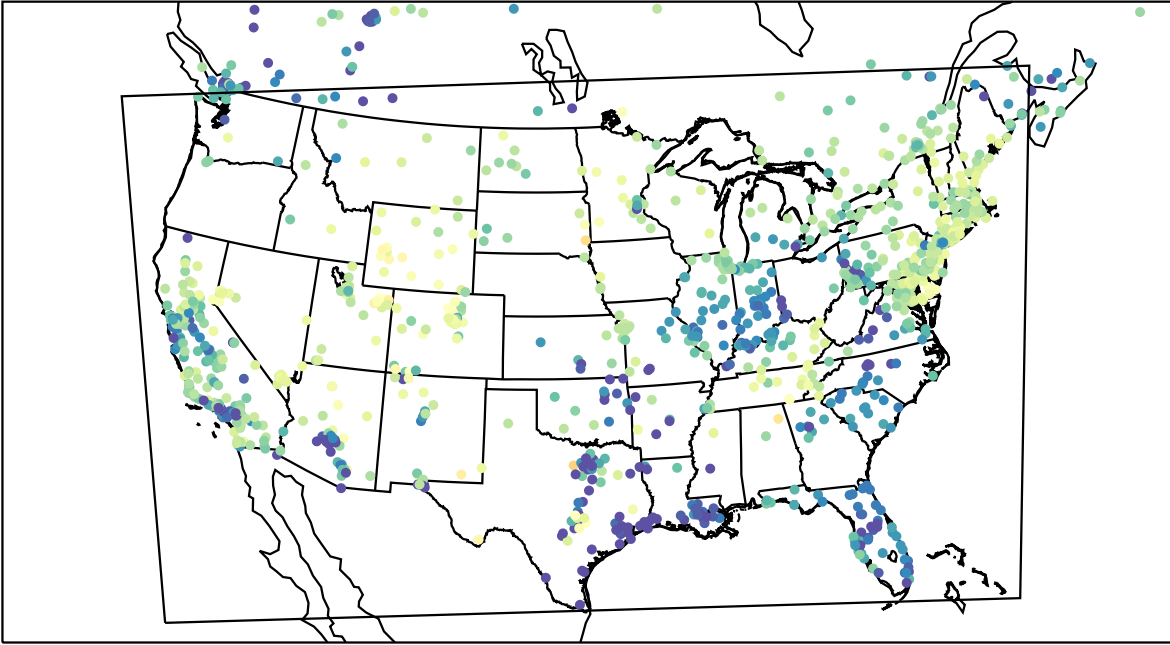
AirNOW (2023-02-28_03:00:00)
