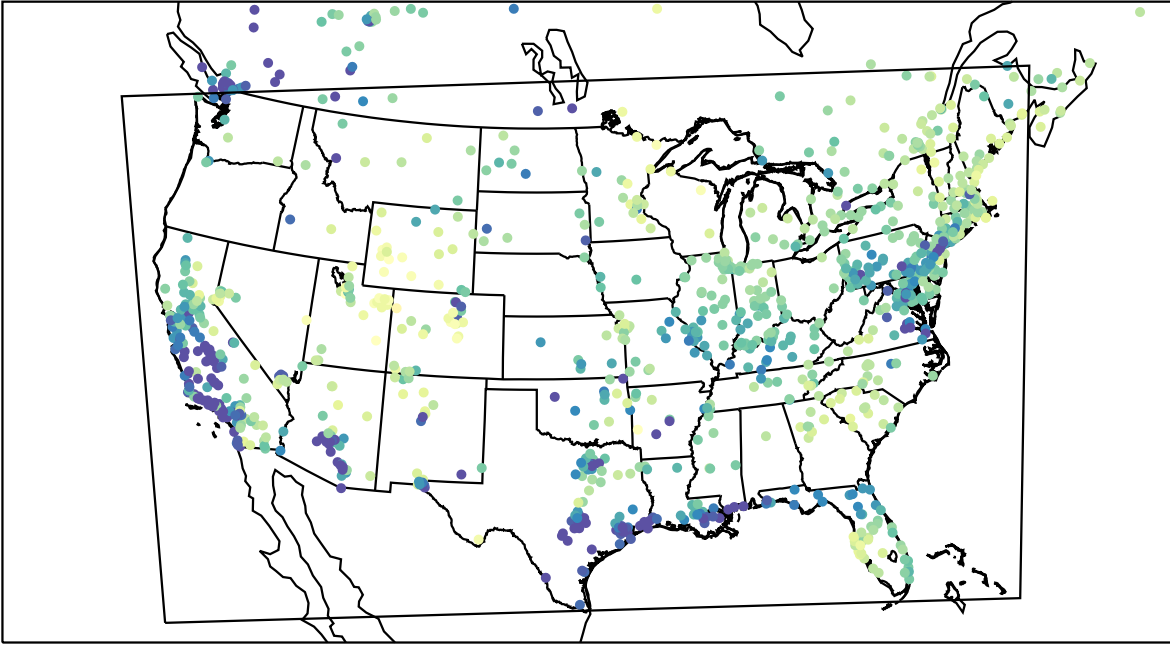
AirNOW (2023-02-28_15:00:00)
