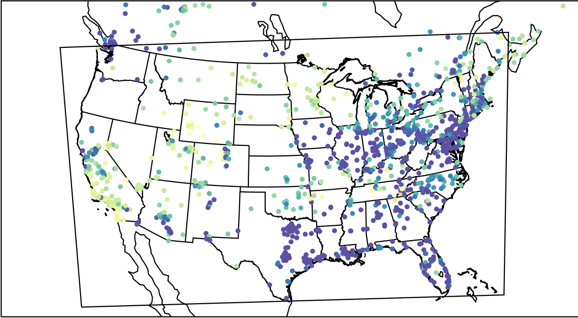
AirNOW (2023-03-01_12:00:00)
