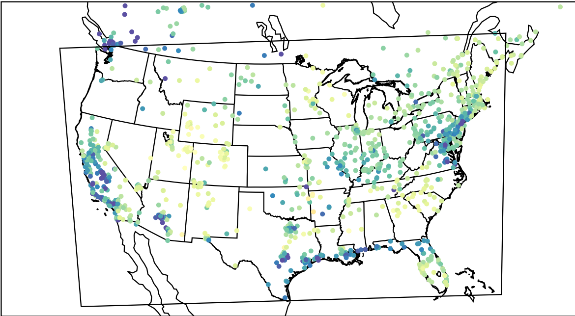
AirNOW (2023-02-28_16:00:00)
