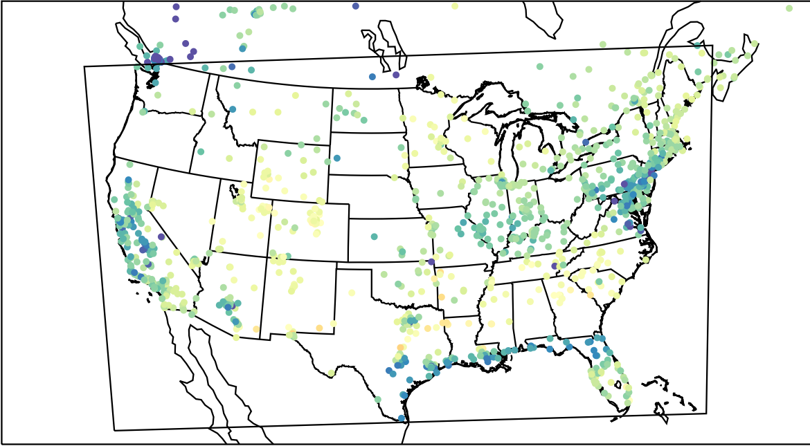
AirNOW (2023-02-28_17:00:00)
