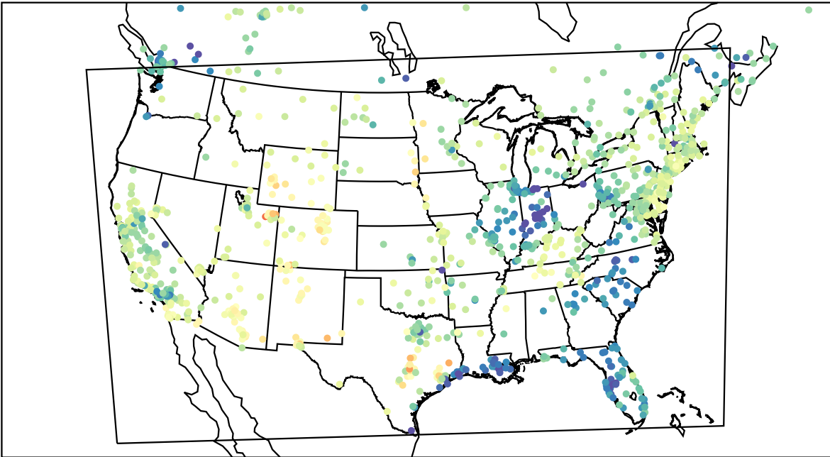
AirNOW (2023-02-28_00:00:00)
