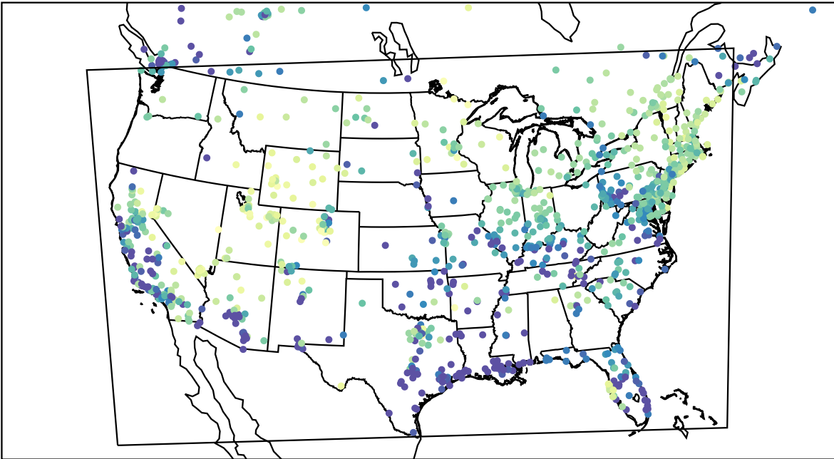
AirNOW (2023-02-28_11:00:00)
