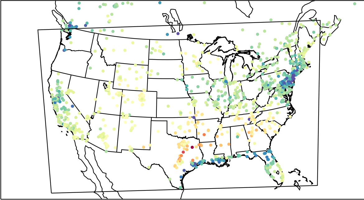
AirNOW (2023-02-28_21:00:00)
