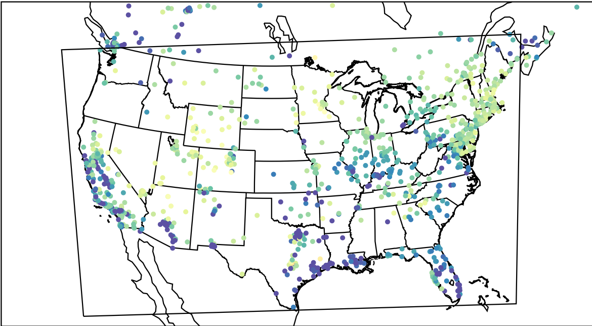
AirNOW (2023-02-28_07:00:00)
