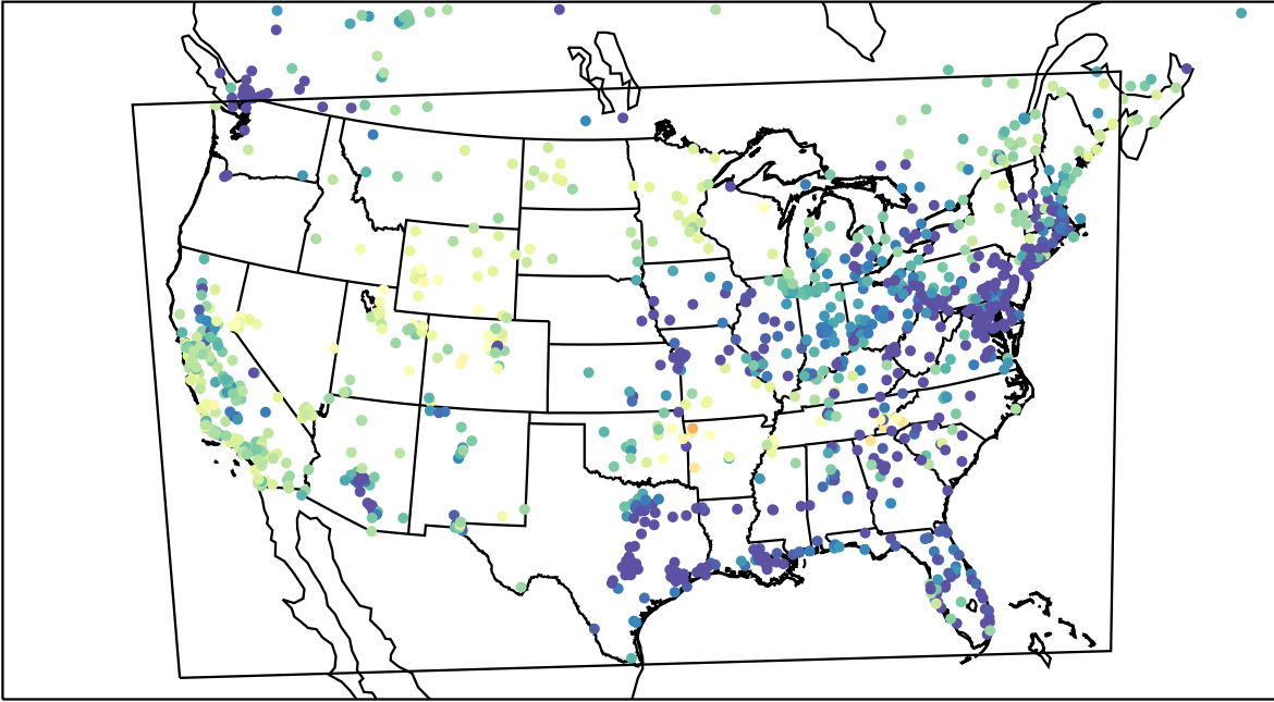
AirNOW (2023-03-01_08:00:00)
