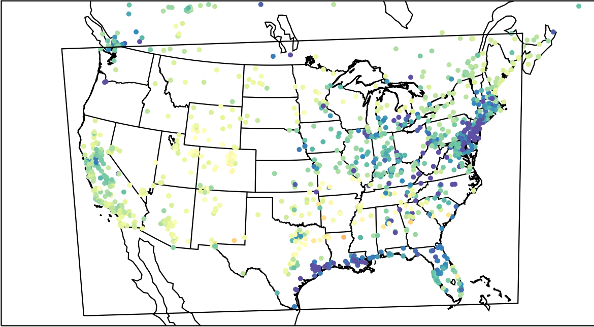
AirNOW (2023-03-01_00:00:00)
