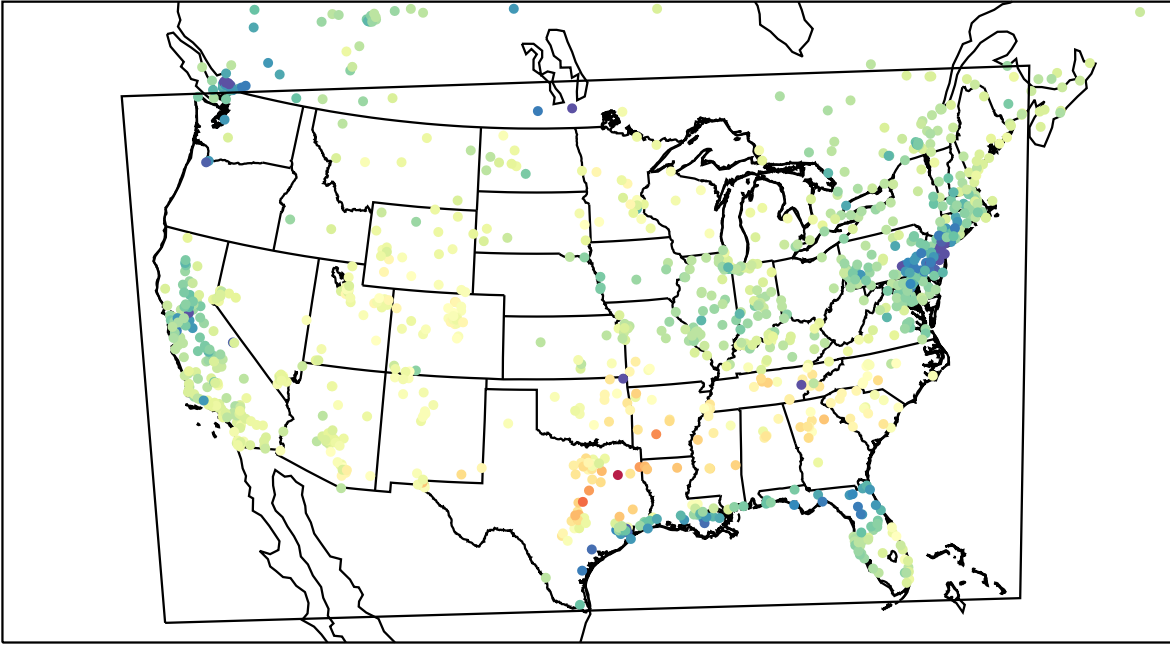
AirNOW (2023-02-28_20:00:00)
