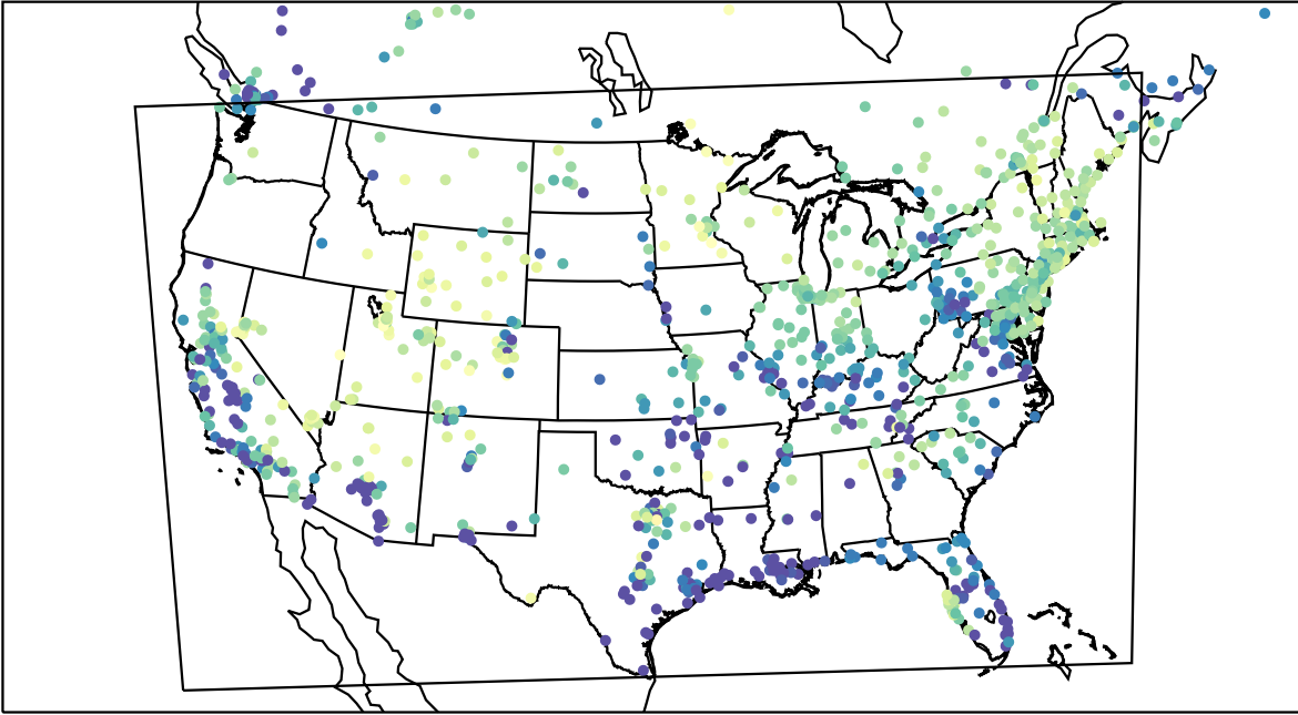
AirNOW (2023-02-28_10:00:00)
