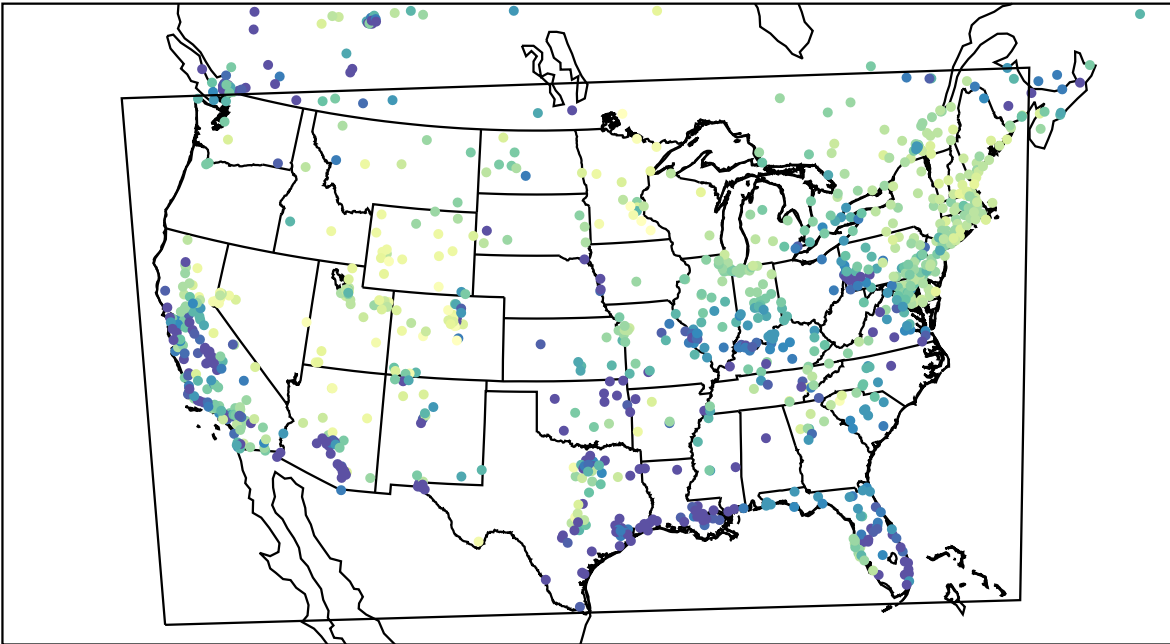
AirNOW (2023-02-28_08:00:00)
