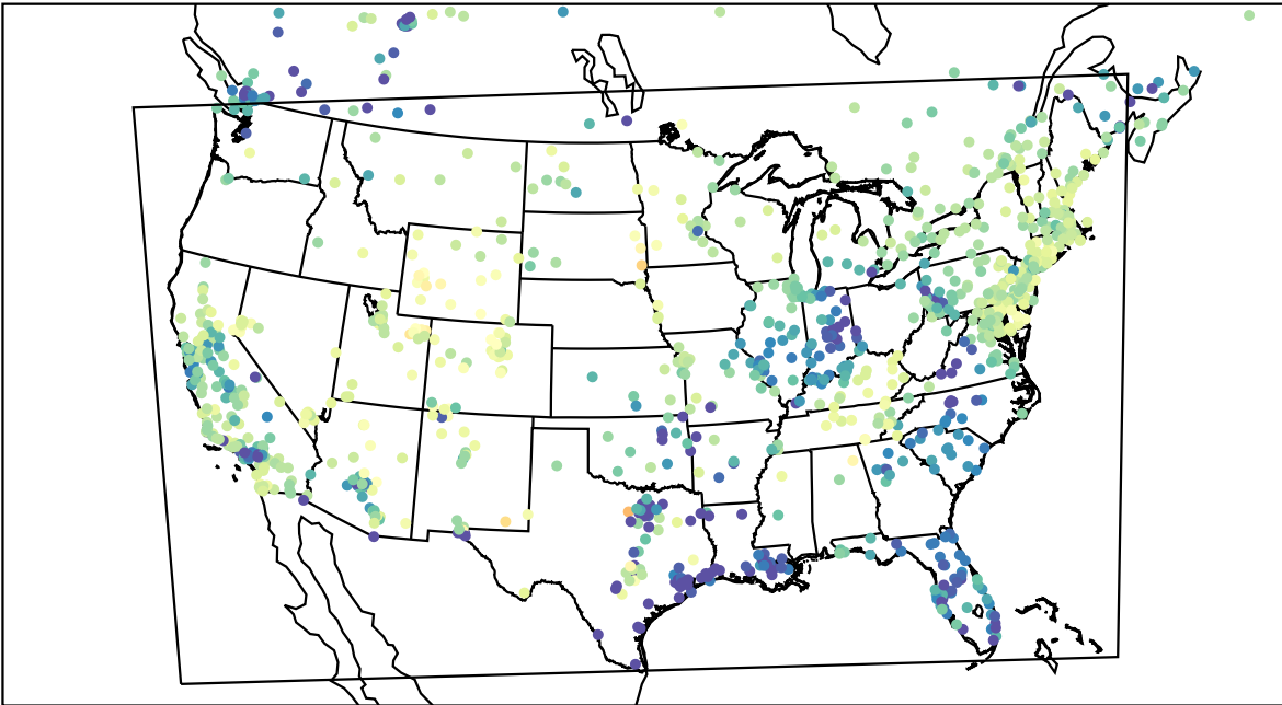
AirNOW (2023-02-28_02:00:00)
