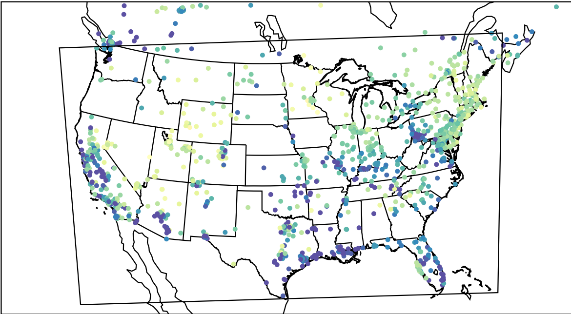
AirNOW (2023-02-28_09:00:00)
