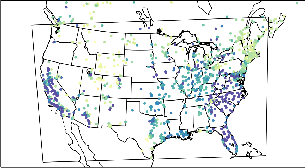
AirNOW (2023-03-03_06:00:00)
