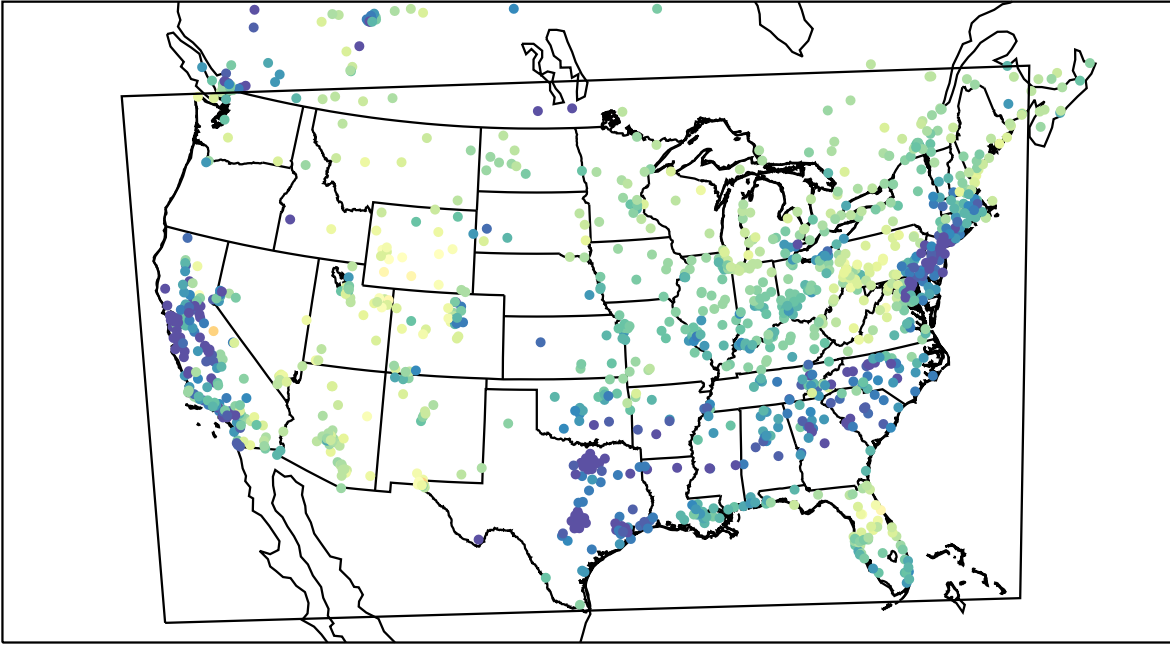
AirNOW (2023-03-02_16:00:00)
