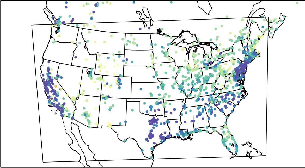
AirNOW (2023-03-02_15:00:00)
