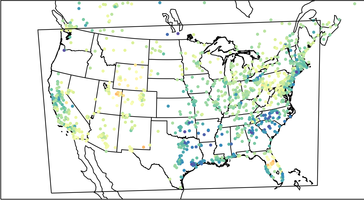
AirNOW (2023-03-02_19:00:00)
