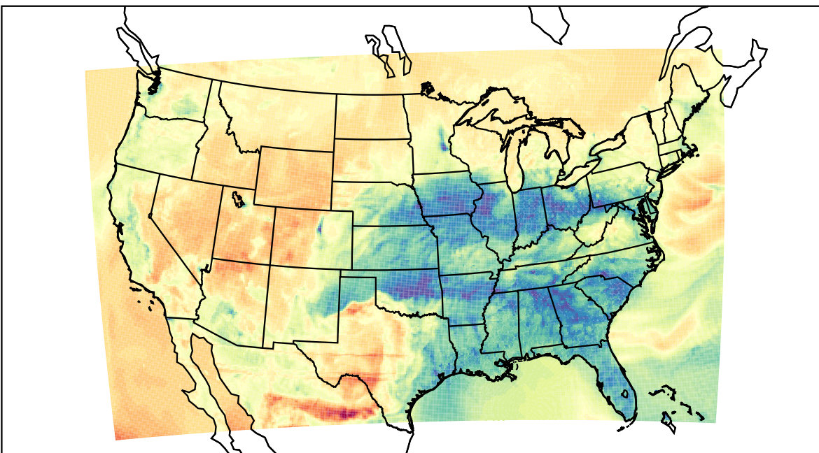
WRF (2023-03-03_02:00:00)
