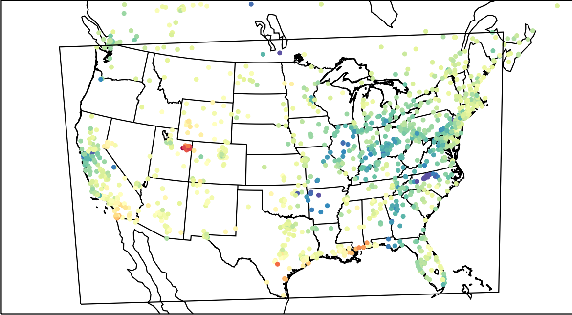
AirNOW (2023-03-03_21:00:00)
