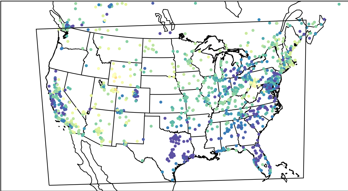
AirNOW (2023-03-02_07:00:00)
