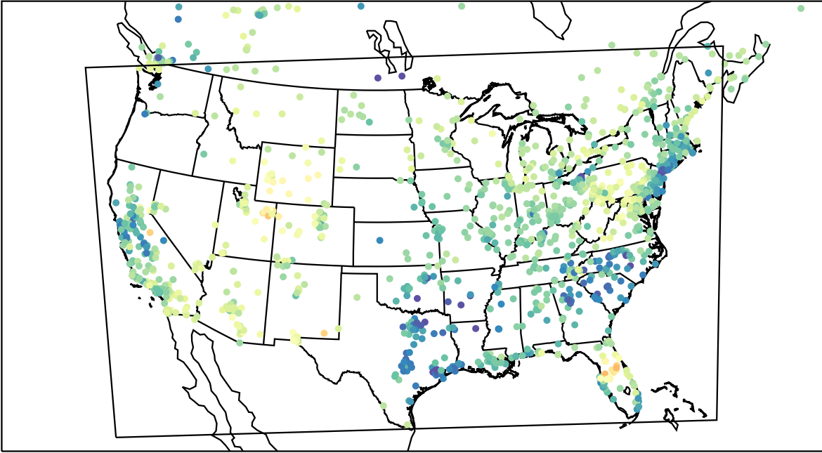
AirNOW (2023-03-02_18:00:00)
