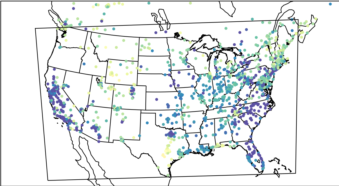
AirNOW (2023-03-03_09:00:00)
