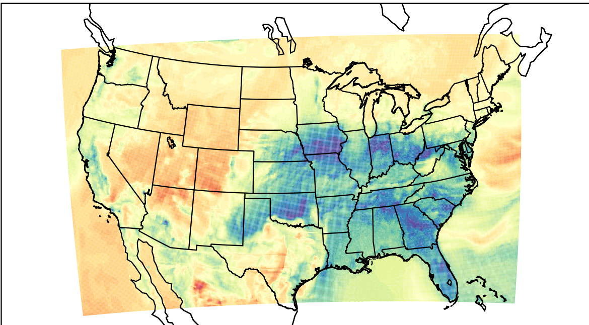
WRF (2023-03-03_05:00:00)
