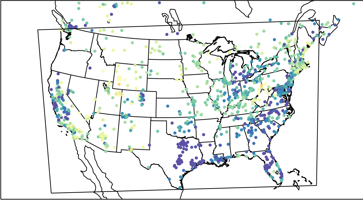
AirNOW (2023-03-02_06:00:00)
