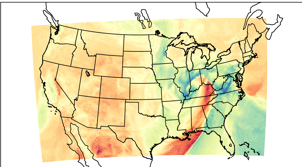
WRF (2023-03-03_21:00:00)
