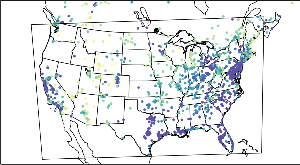
AirNOW (2023-03-02_12:00:00)
