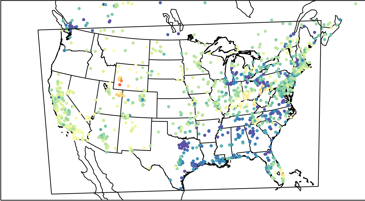
AirNOW (2023-03-02_00:00:00)
