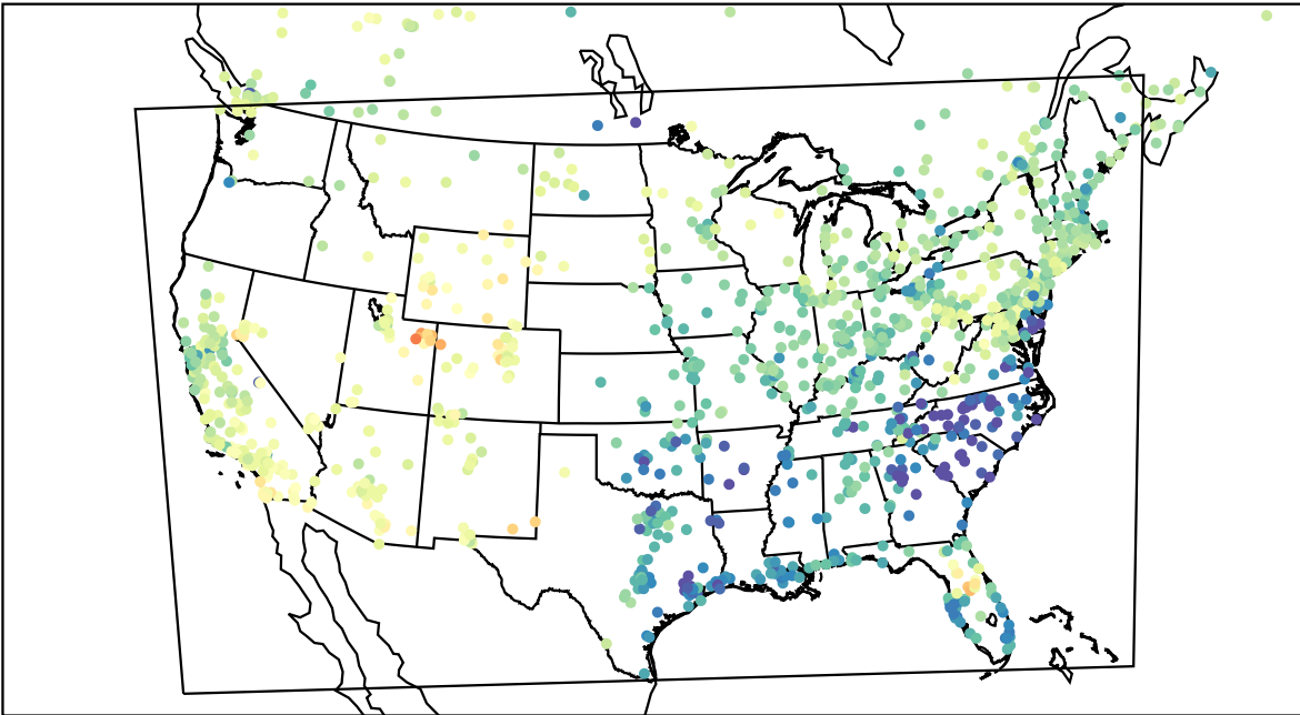
AirNOW (2023-03-02_23:00:00)
