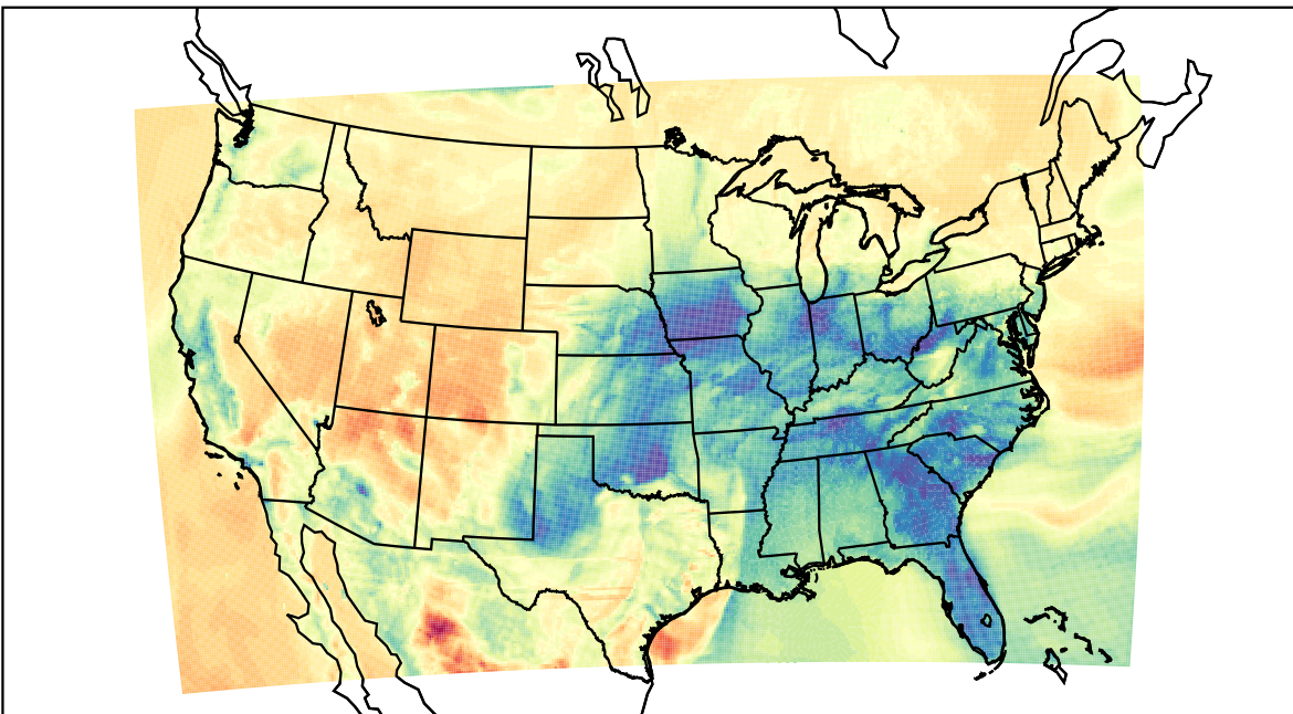
WRF (2023-03-03_07:00:00)
