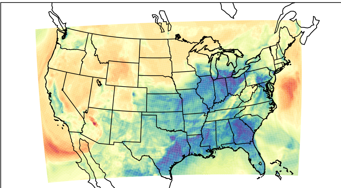
WRF (2023-03-02_05:00:00)
