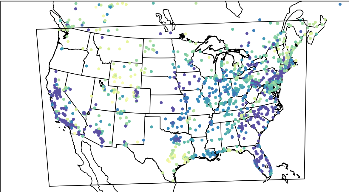
AirNOW (2023-03-03_11:00:00)
