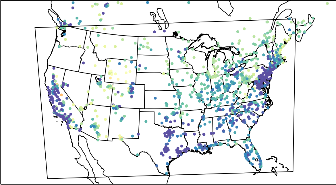
AirNOW (2023-03-02_14:00:00)
