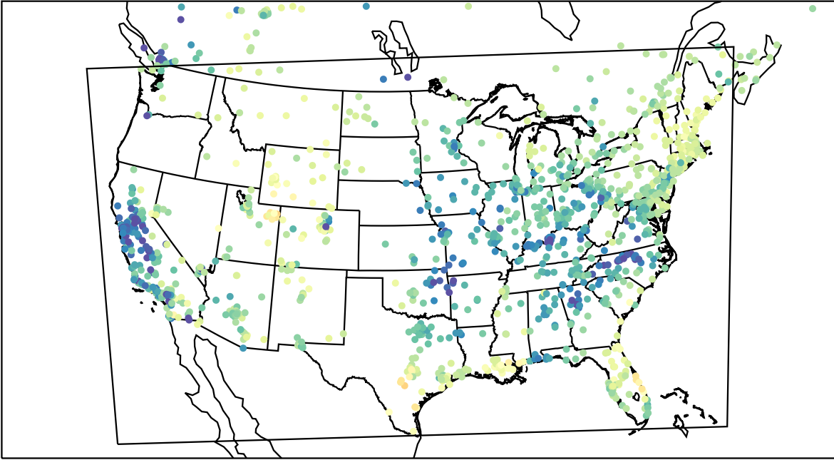
AirNOW (2023-03-03_17:00:00)
