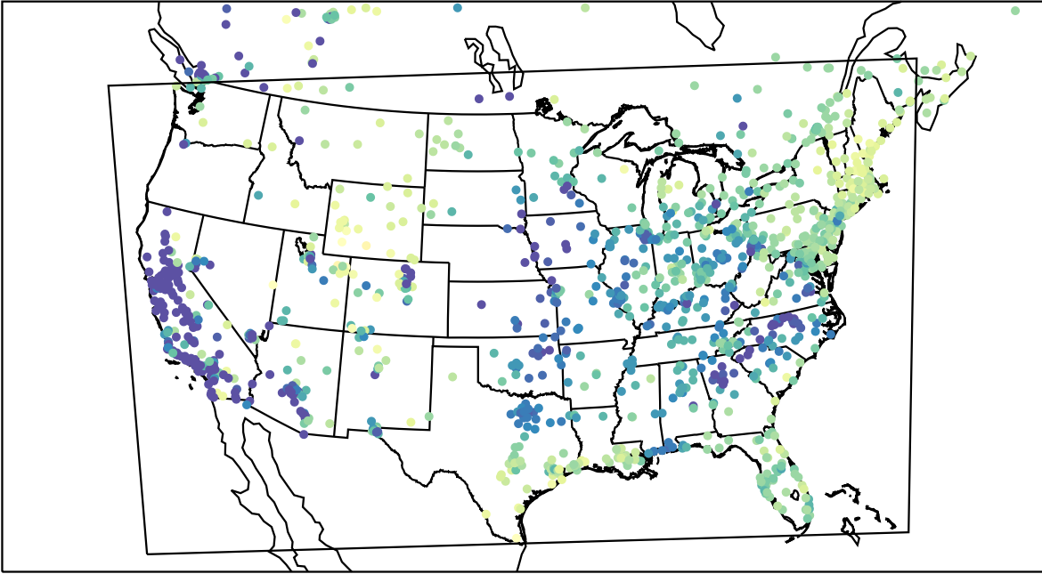
AirNOW (2023-03-03_15:00:00)
