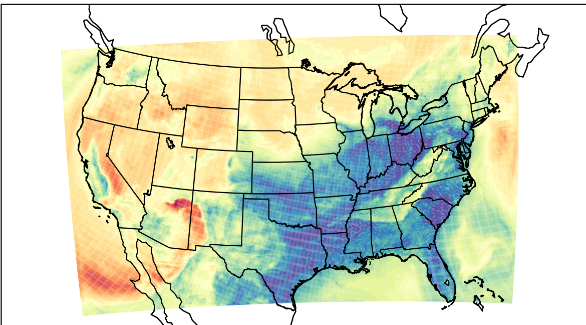
WRF (2023-03-02_11:00:00)
