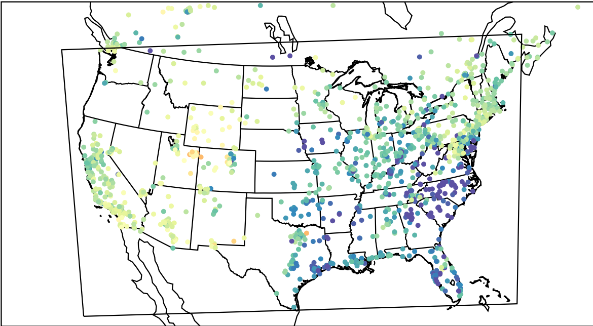
AirNOW (2023-03-03_01:00:00)
