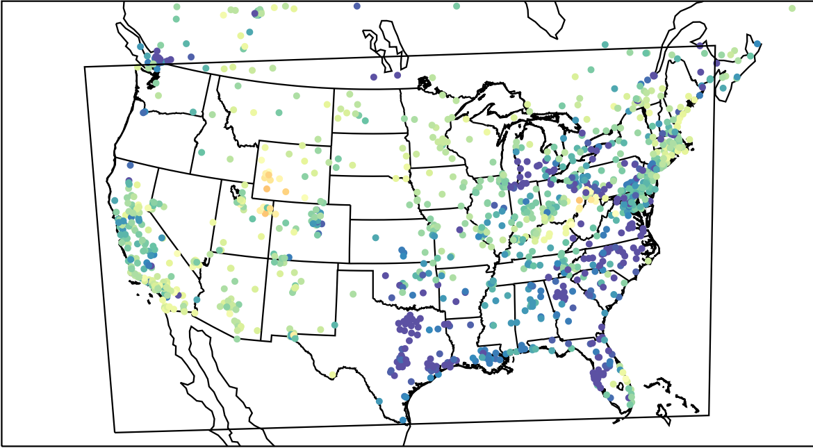
AirNOW (2023-03-02_03:00:00)
