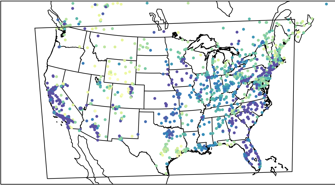
AirNOW (2023-03-03_12:00:00)
