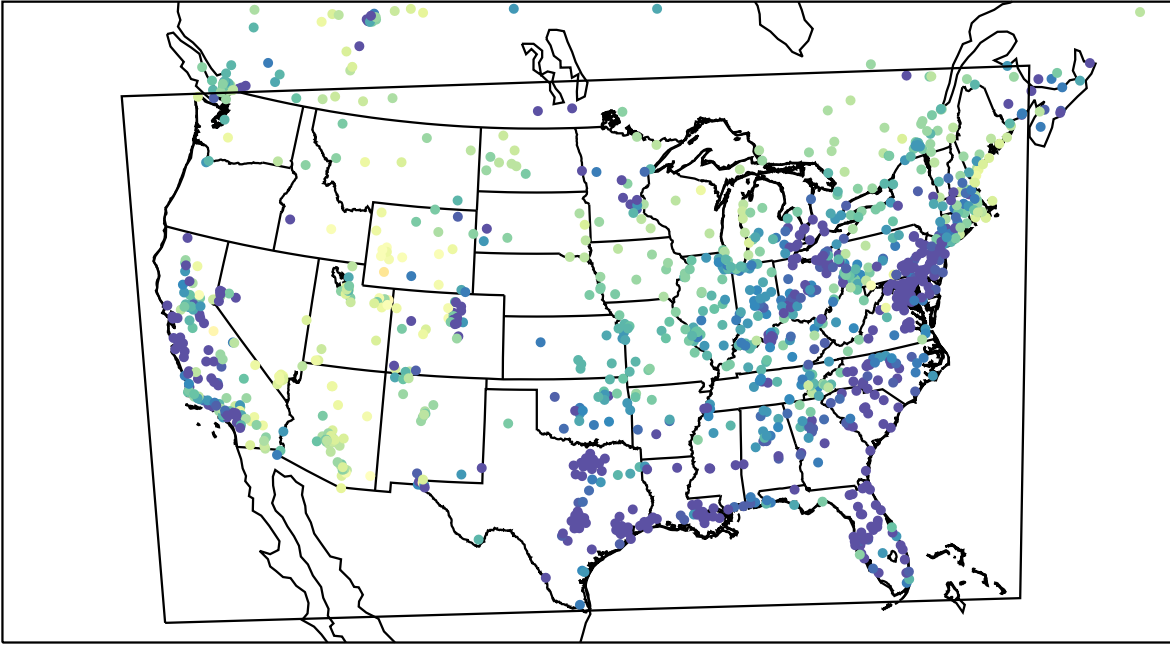
AirNOW (2023-03-02_11:00:00)
