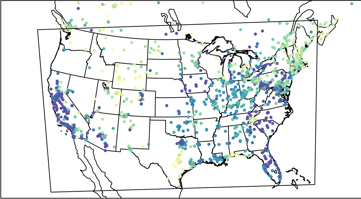
AirNOW (2023-03-03_08:00:00)
