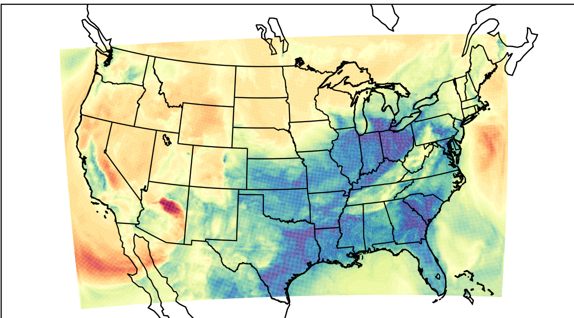
WRF (2023-03-02_08:00:00)
