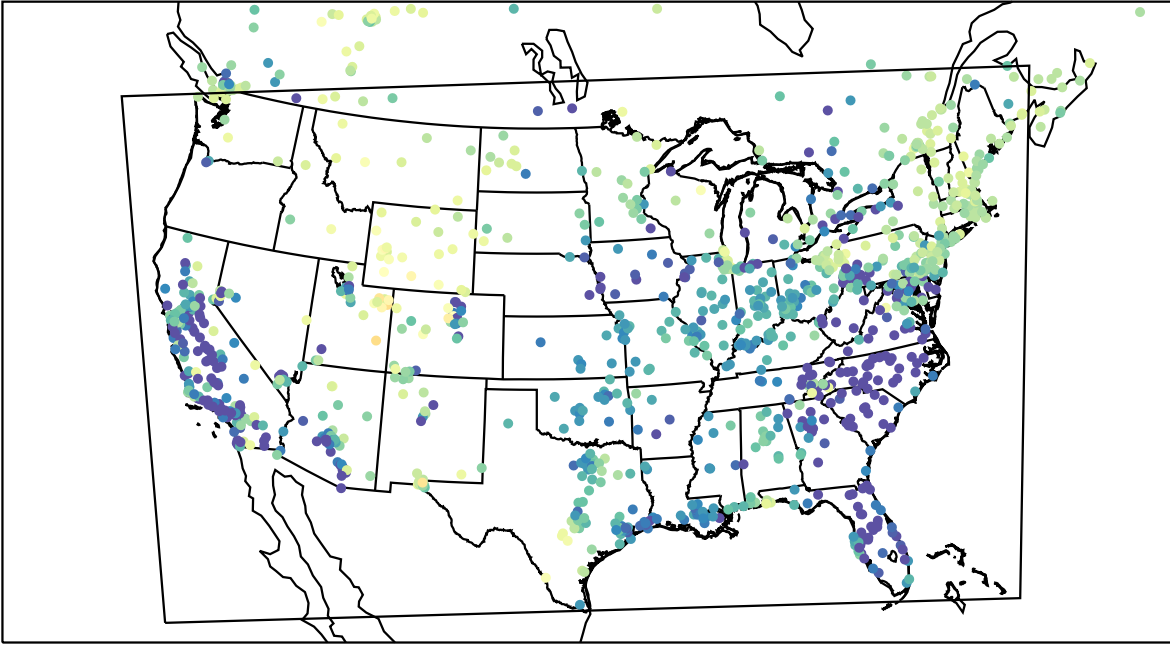
AirNOW (2023-03-03_05:00:00)
