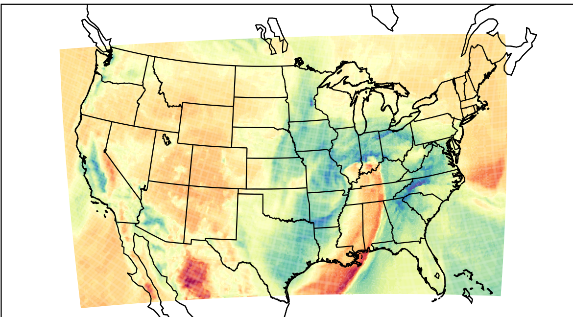
WRF (2023-03-03_17:00:00)
