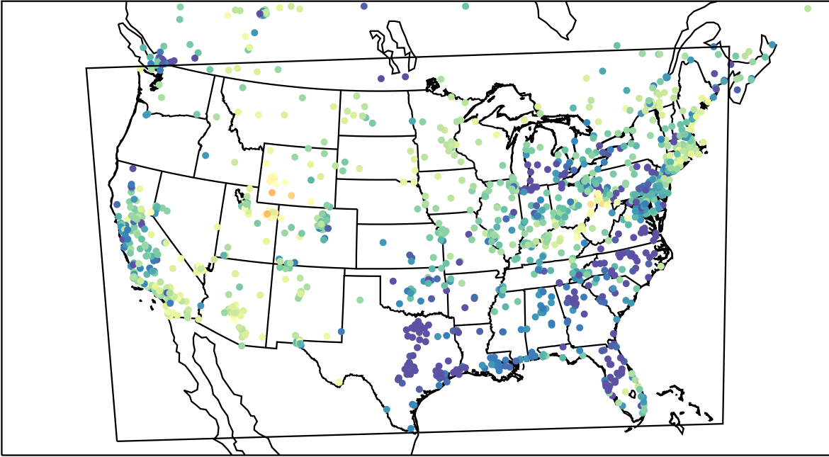
AirNOW (2023-03-02_04:00:00)
