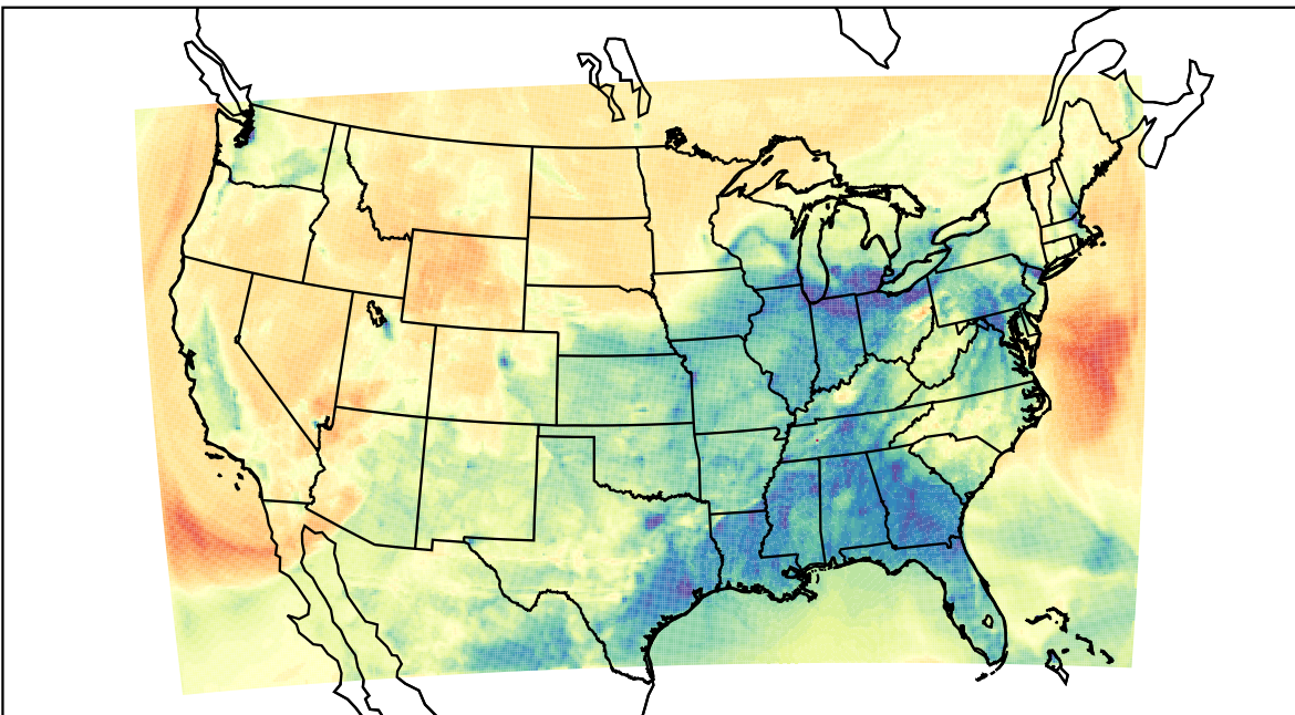
WRF (2023-03-02_02:00:00)
