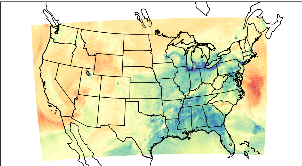
WRF (2023-03-02_00:00:00)
