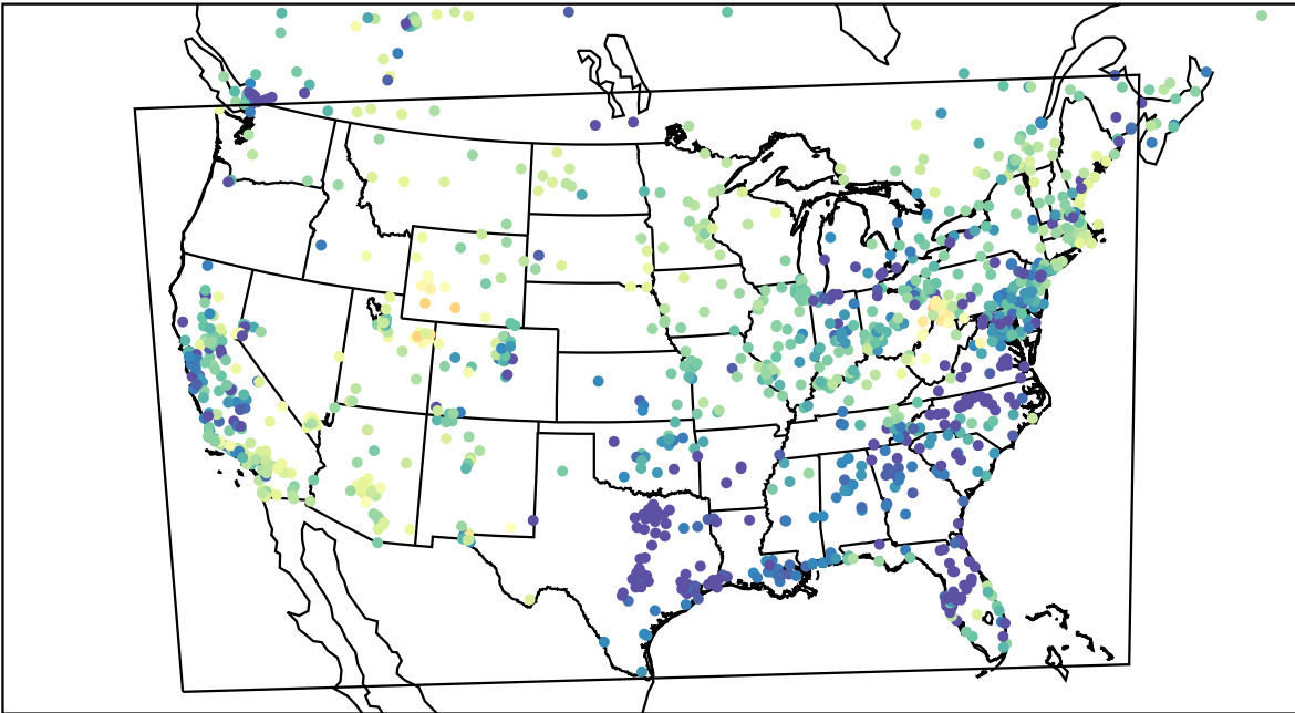
AirNOW (2023-03-02_05:00:00)
