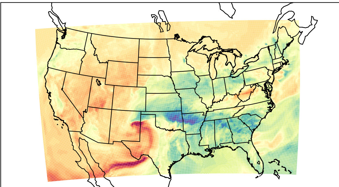
WRF (2023-03-02_22:00:00)
