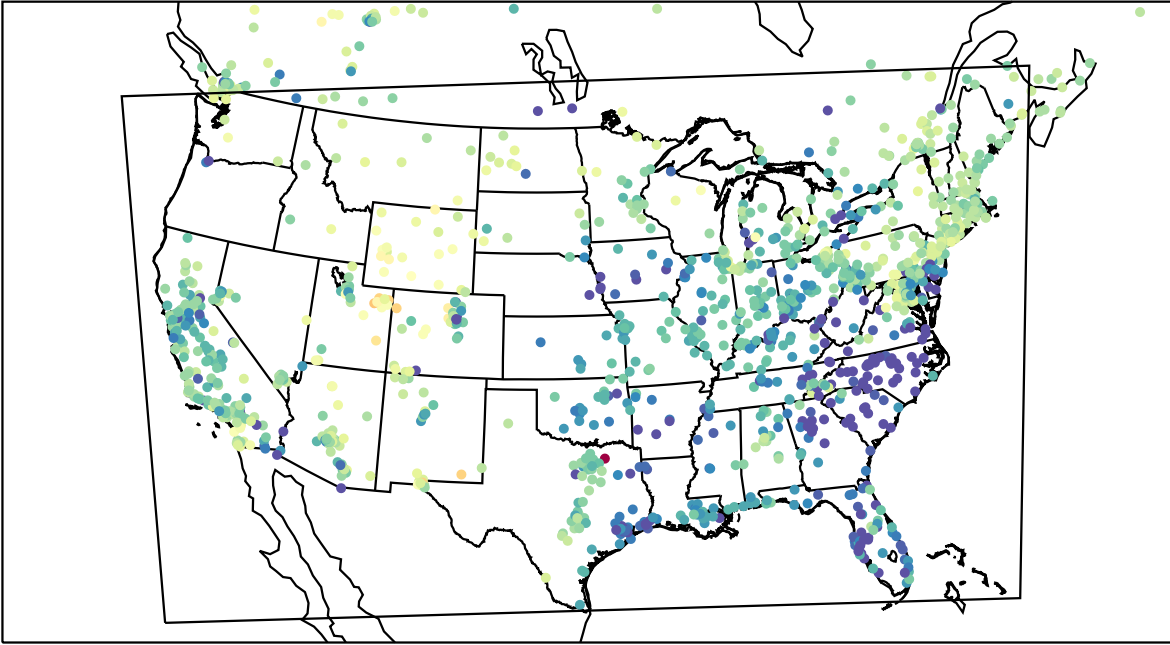
AirNOW (2023-03-03_02:00:00)
