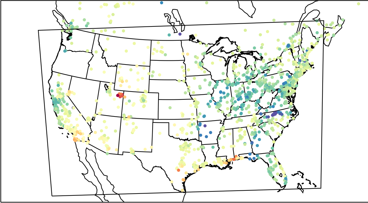
AirNOW (2023-03-03_22:00:00)
