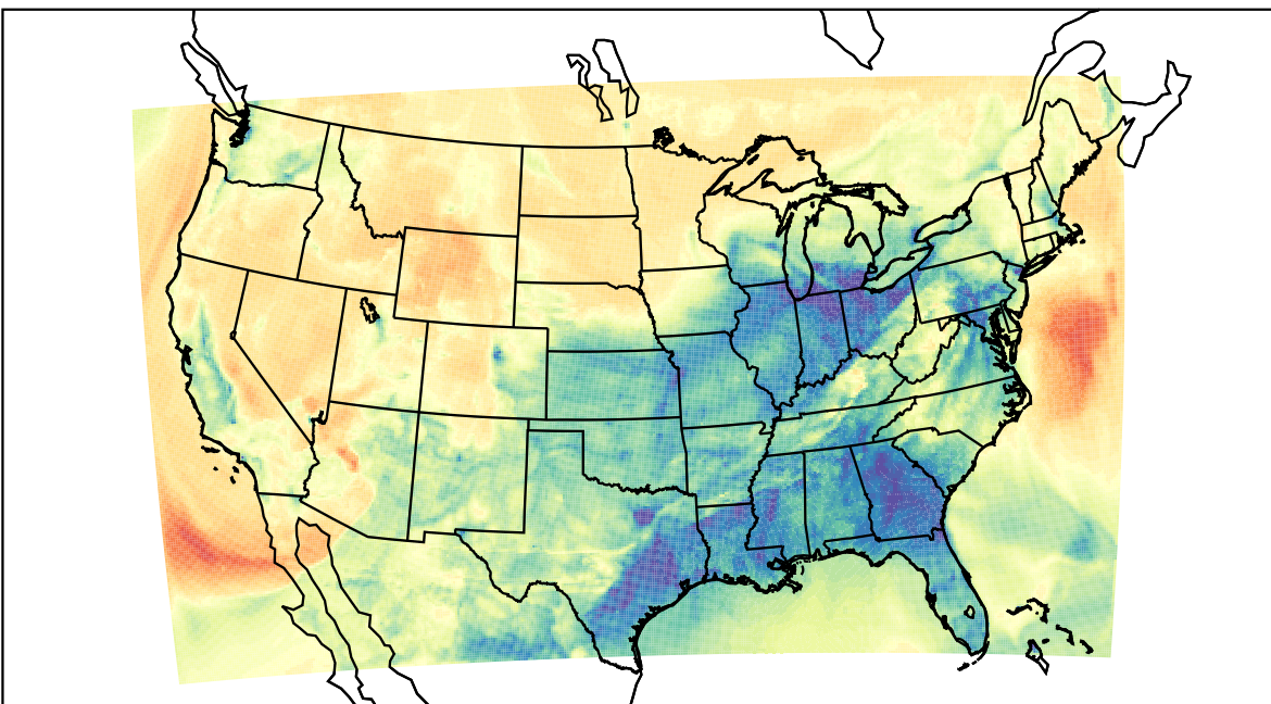
WRF (2023-03-02_04:00:00)
