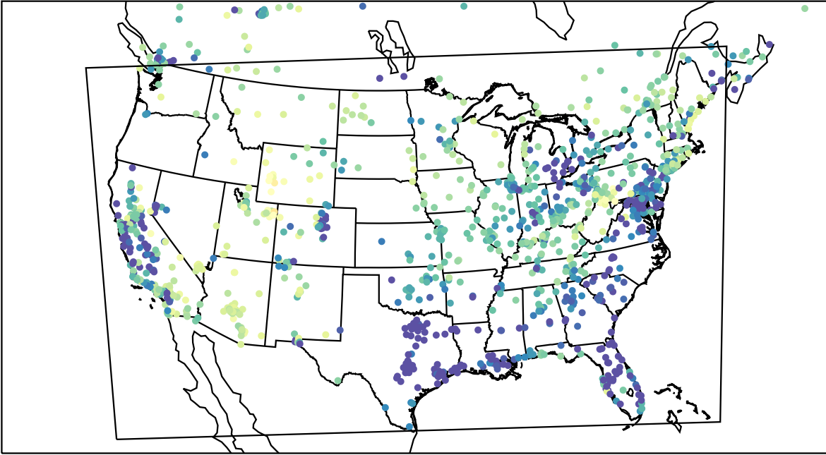
AirNOW (2023-03-02_08:00:00)
