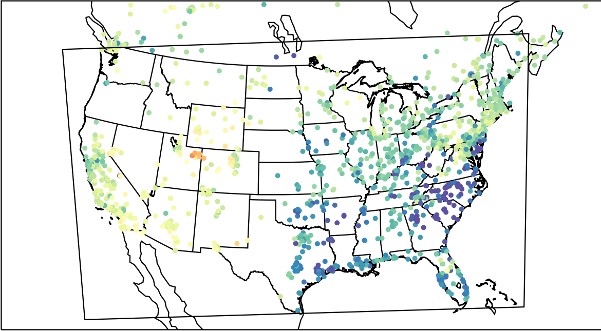
AirNOW (2023-03-03_00:00:00)
