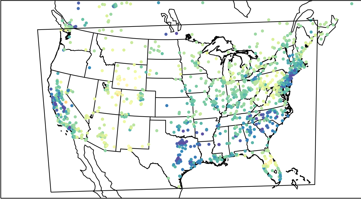
AirNOW (2023-03-02_17:00:00)
