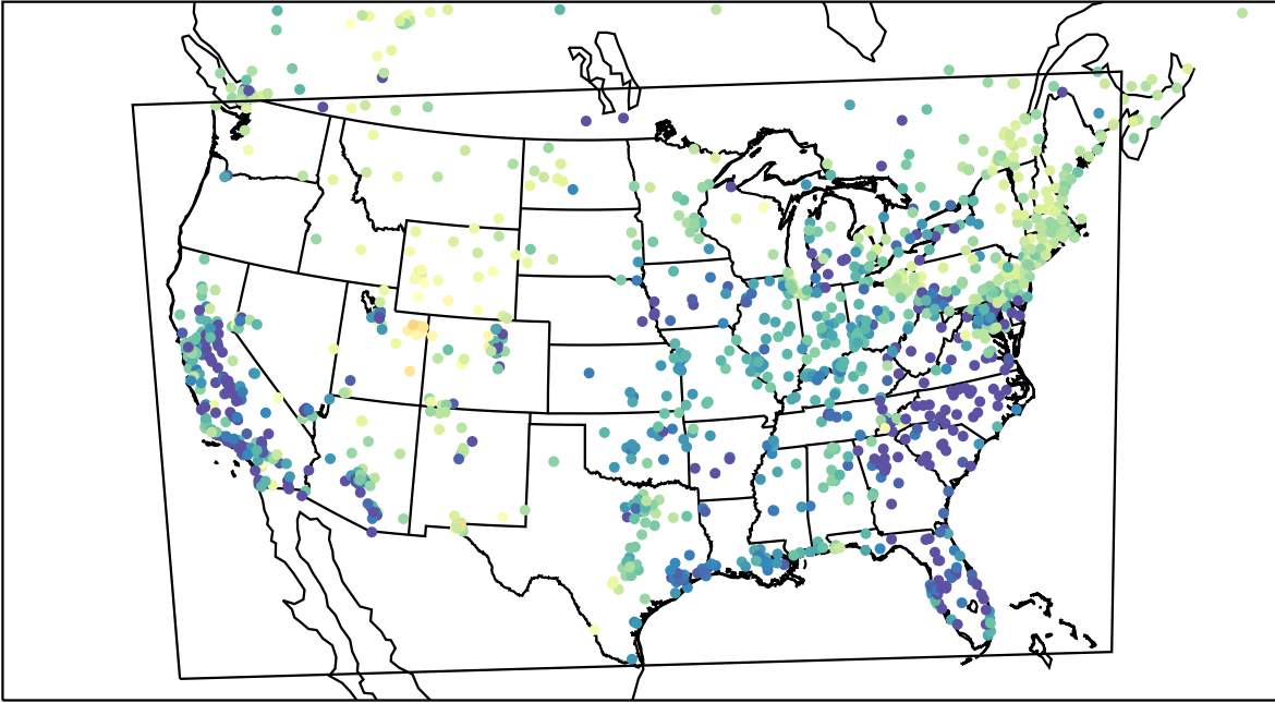
AirNOW (2023-03-03_04:00:00)
