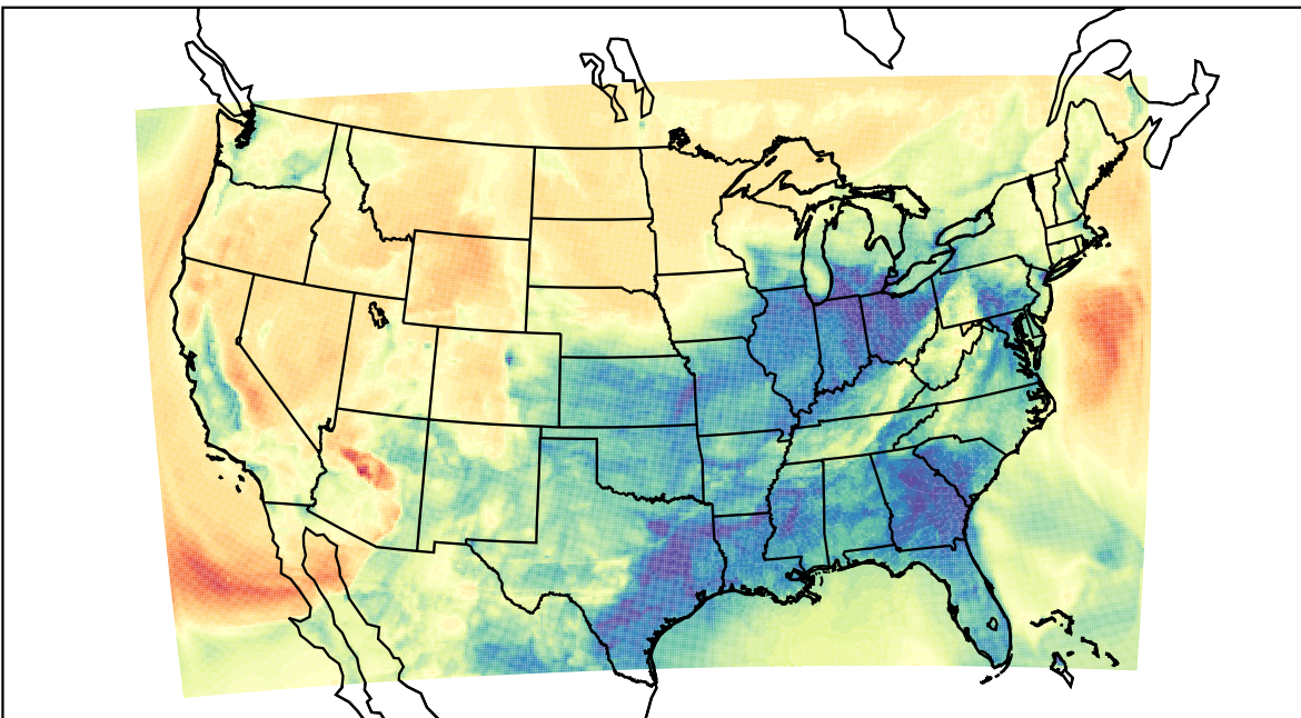
WRF (2023-03-02_06:00:00)
