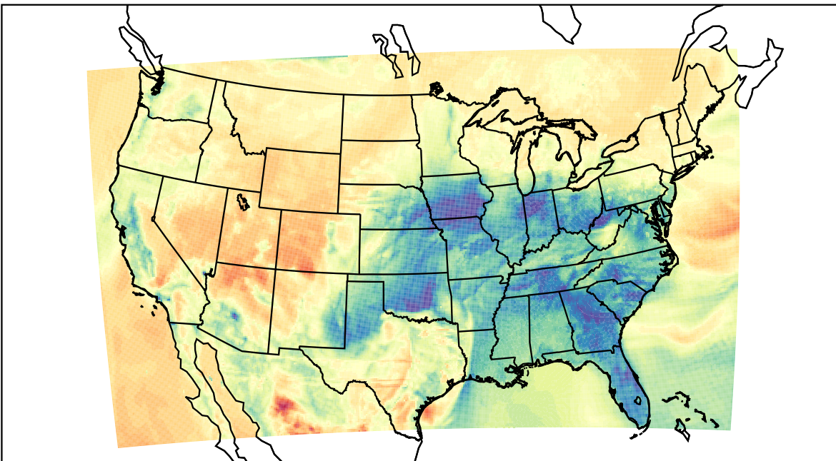
WRF (2023-03-03_06:00:00)
