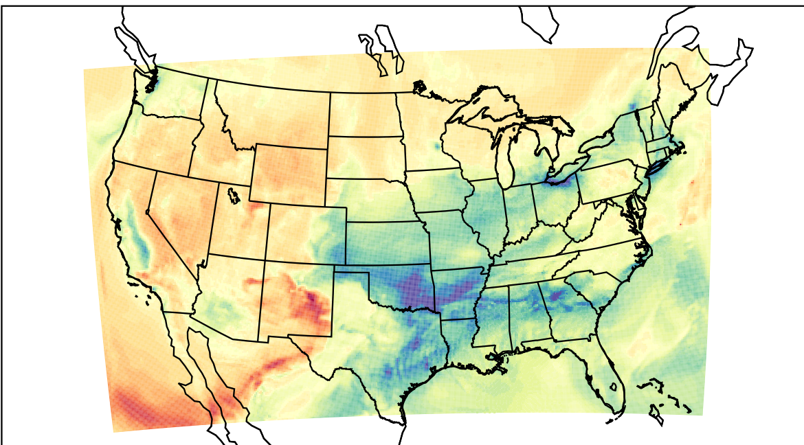
WRF (2023-03-02_17:00:00)
