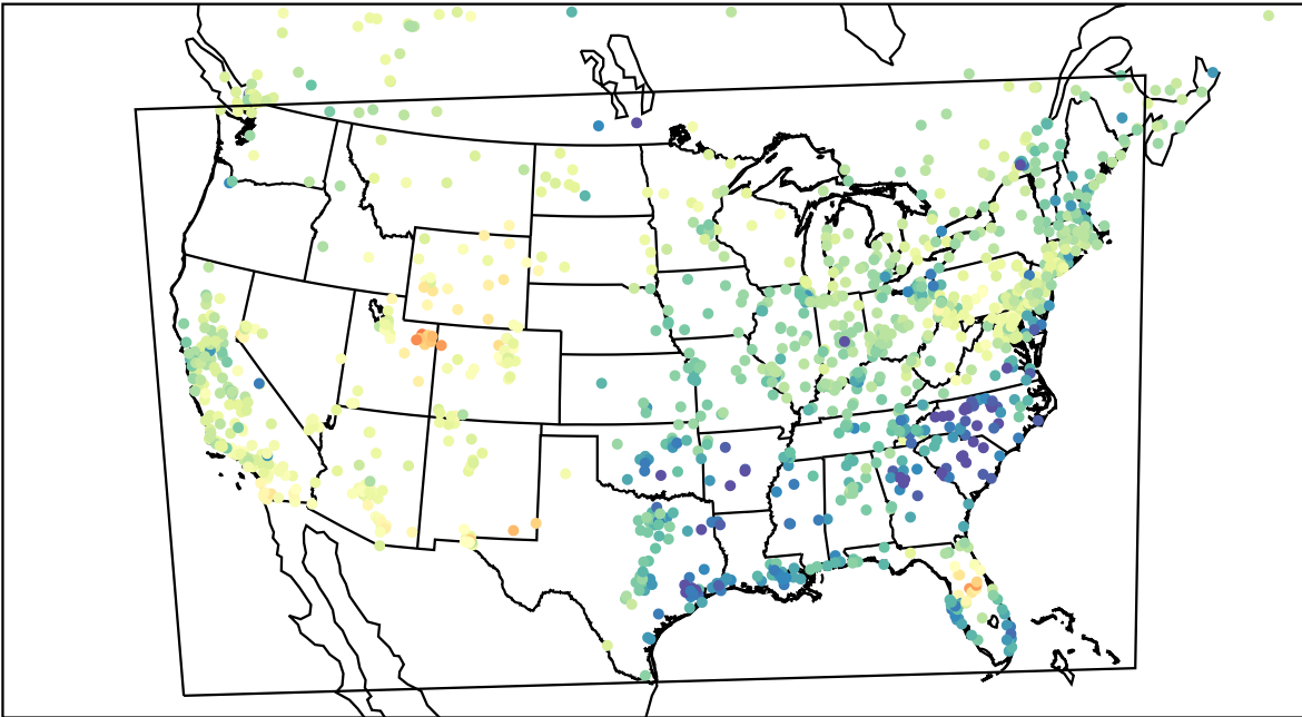
AirNOW (2023-03-02_22:00:00)
