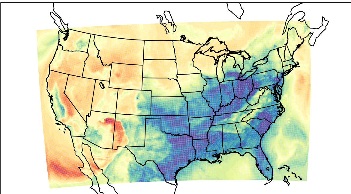
WRF (2023-03-02_12:00:00)
