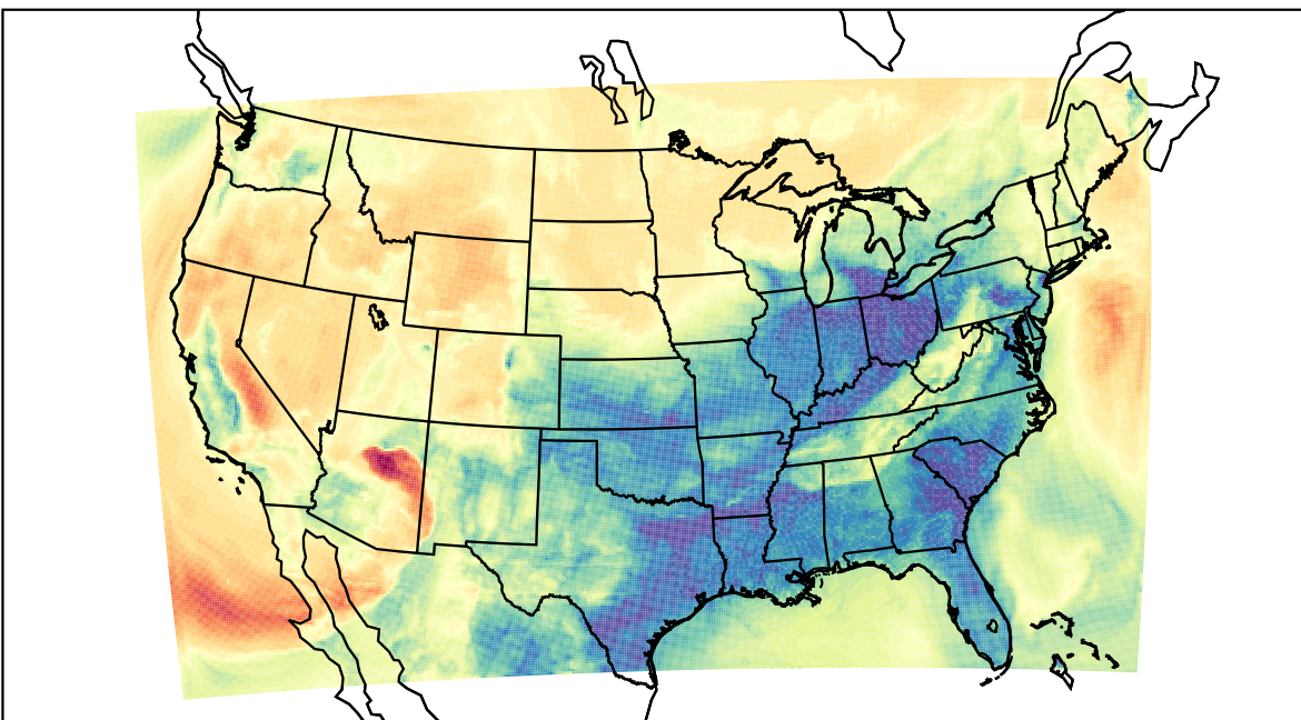
WRF (2023-03-02_09:00:00)
