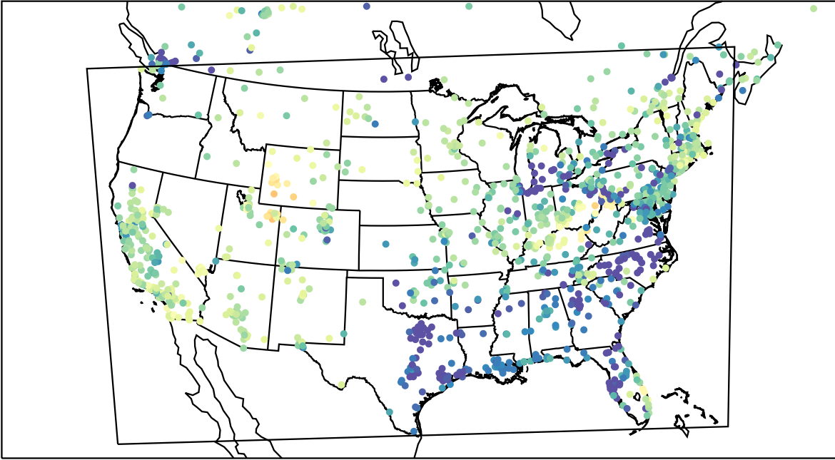
AirNOW (2023-03-02_02:00:00)
