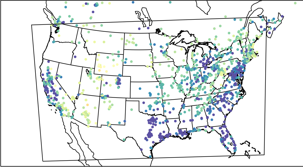
AirNOW (2023-03-02_09:00:00)
