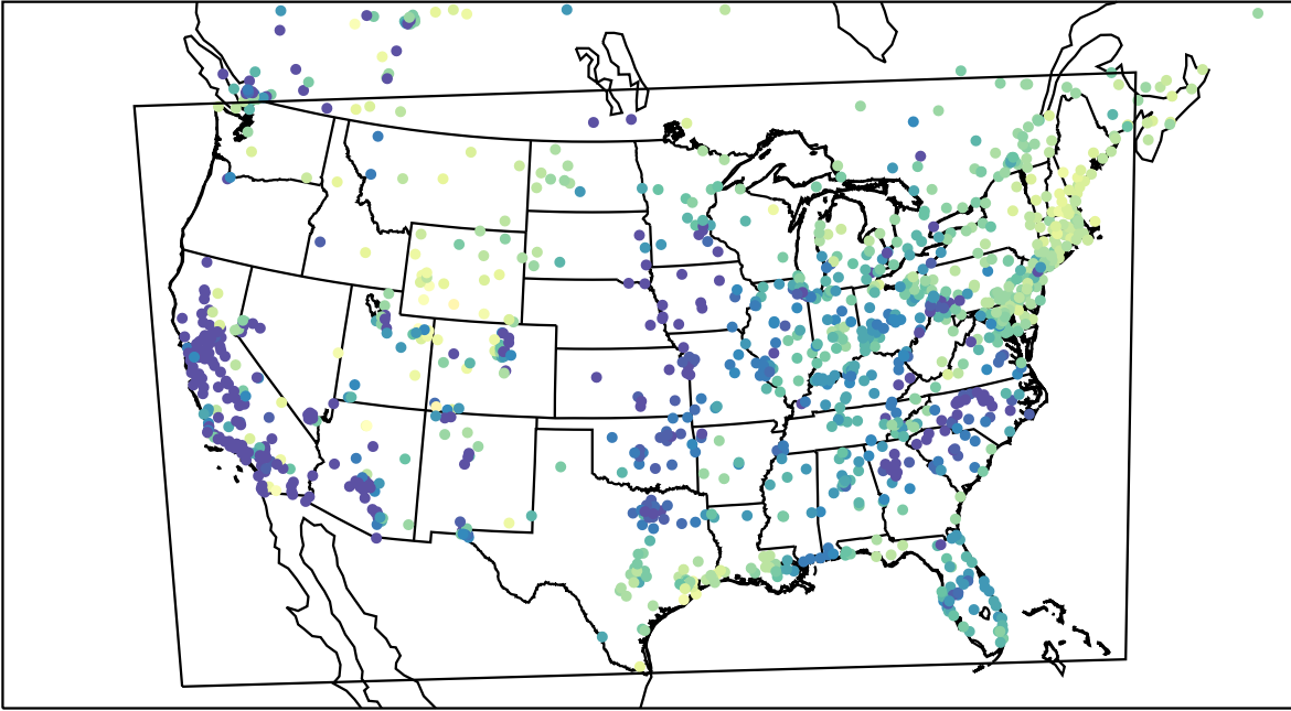
AirNOW (2023-03-03_14:00:00)
