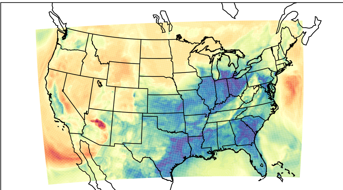
WRF (2023-03-02_07:00:00)
