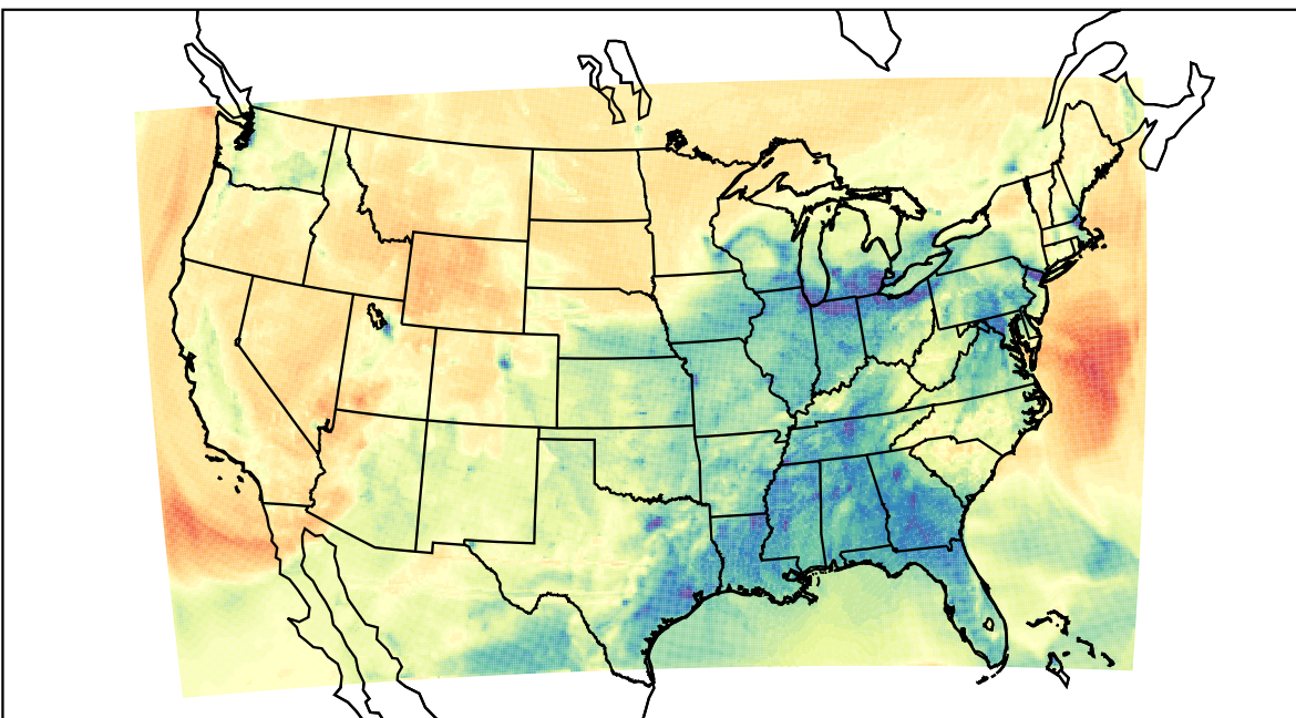
WRF (2023-03-02_01:00:00)
