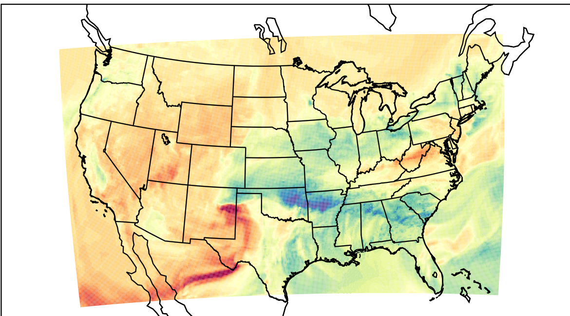
WRF (2023-03-02_21:00:00)
