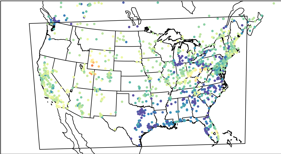
AirNOW (2023-03-02_01:00:00)
