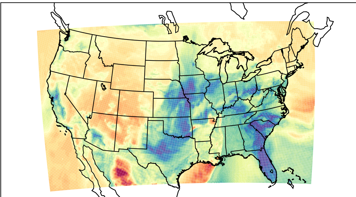
WRF (2023-03-03_12:00:00)
