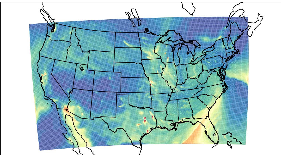
WRF 2023-03-04_06:00:00
