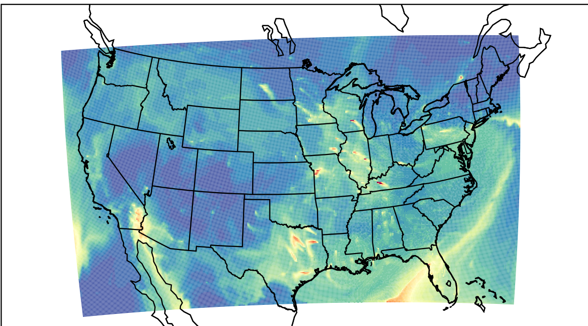
WRF 2023-03-04_13:00:00
