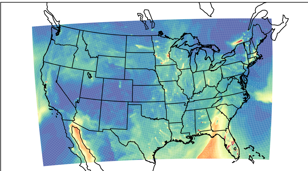
WRF 2023-03-04_00:00:00
