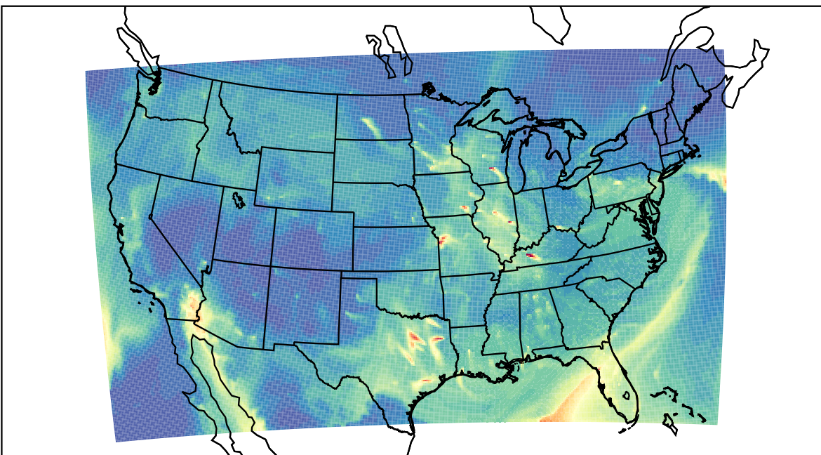
WRF 2023-03-04_12:00:00
