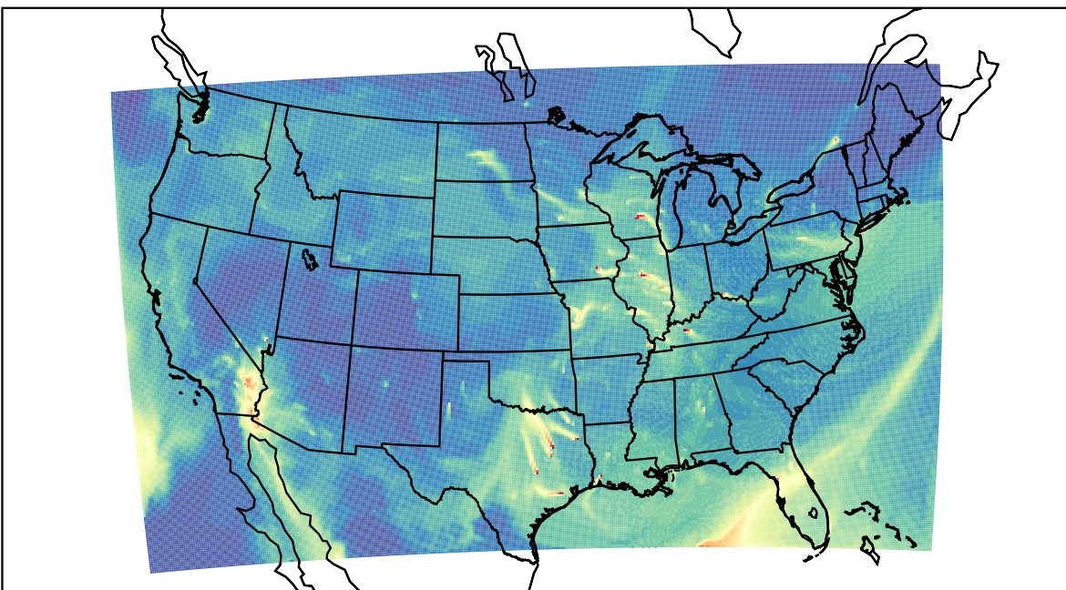
WRF 2023-03-04_16:00:00
