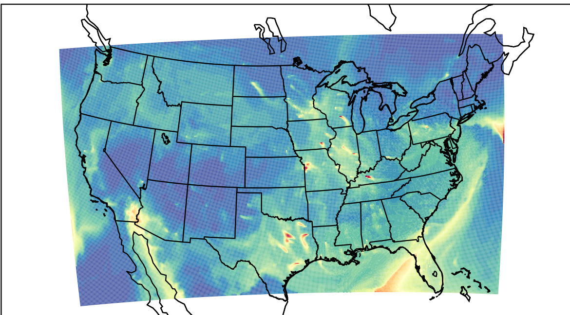
WRF 2023-03-04_11:00:00
