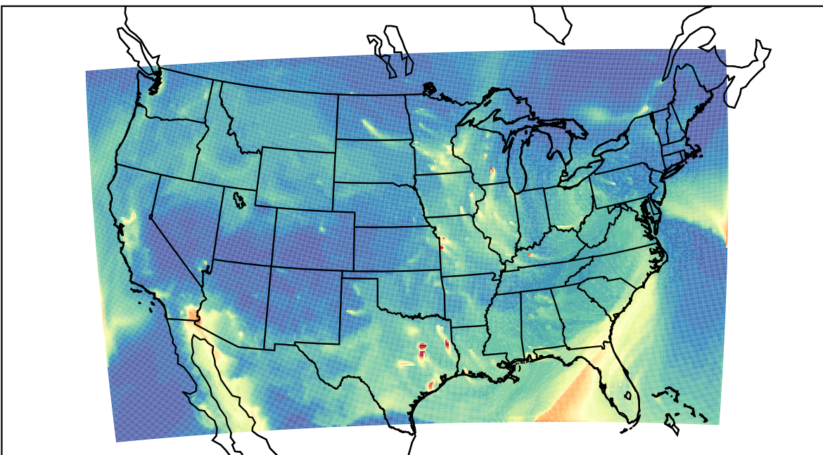
WRF 2023-03-04_07:00:00
