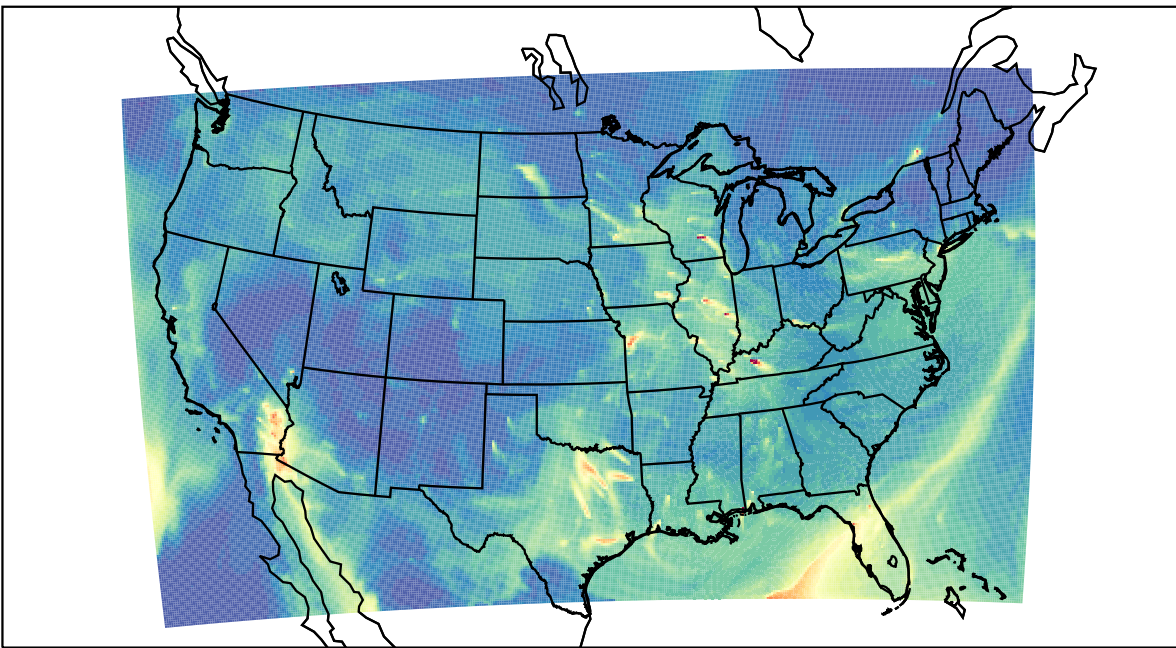
WRF 2023-03-04_14:00:00
