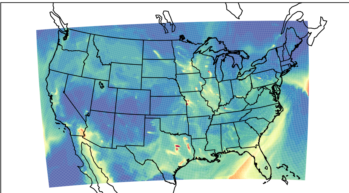
WRF 2023-03-04_09:00:00
