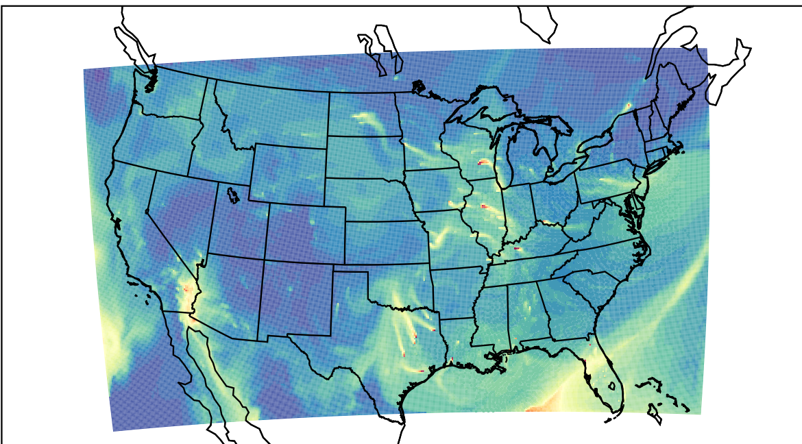
WRF 2023-03-04_17:00:00
