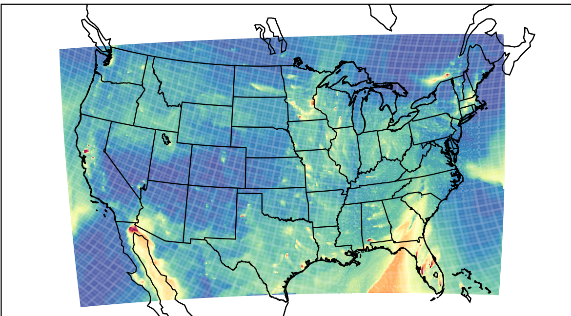
WRF 2023-03-04_02:00:00
