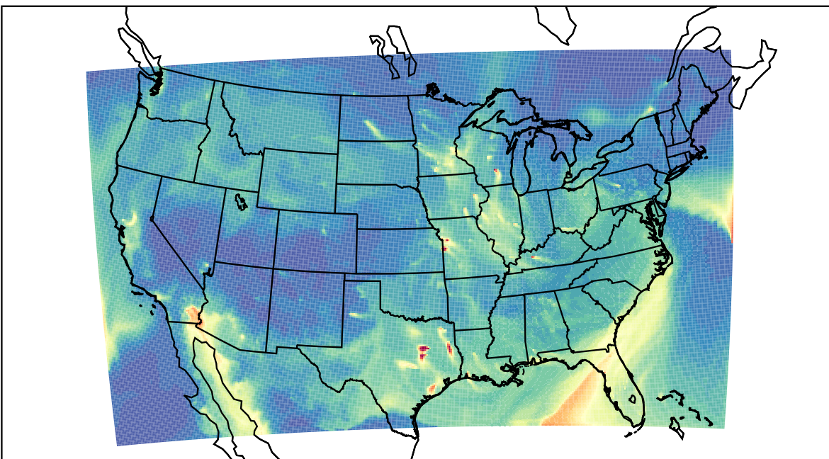
WRF 2023-03-04_08:00:00
