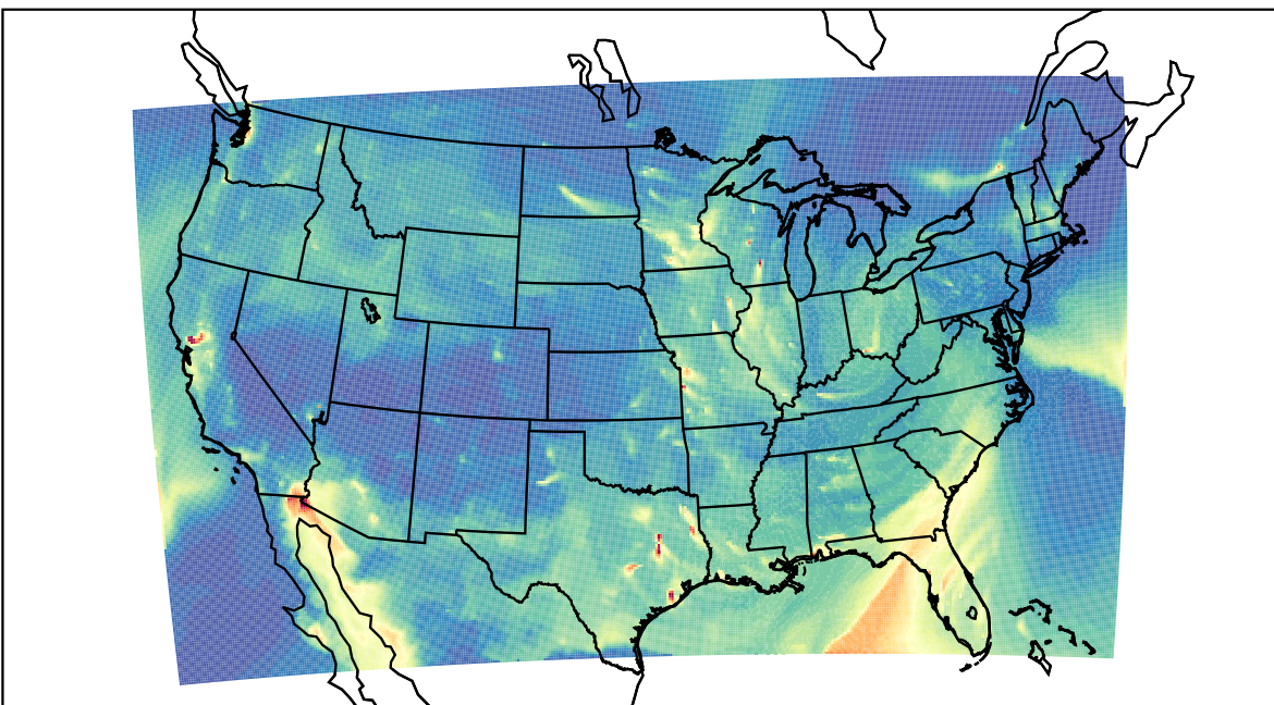
WRF 2023-03-04_05:00:00
