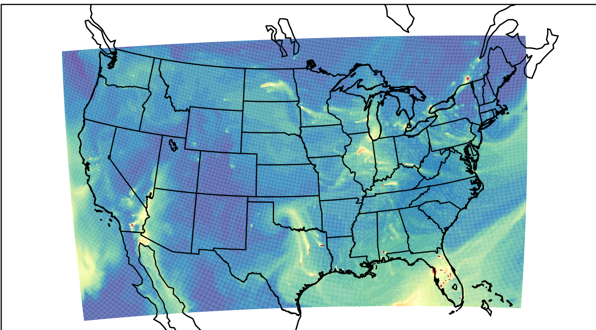
WRF 2023-03-04_22:00:00
