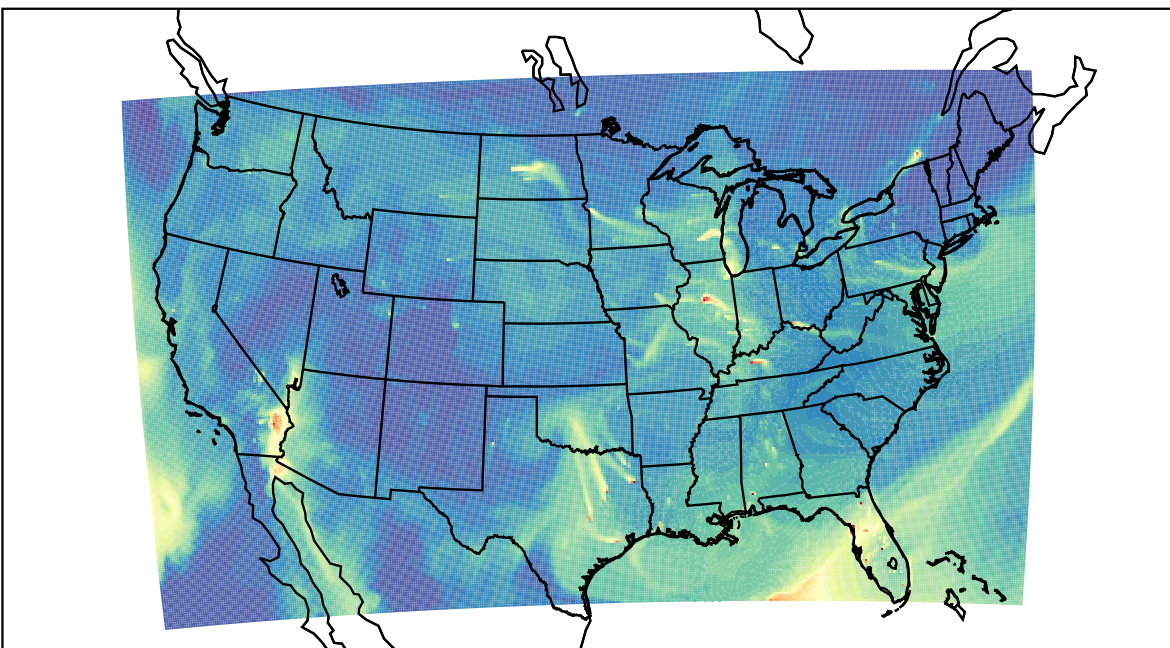
WRF 2023-03-04_19:00:00
