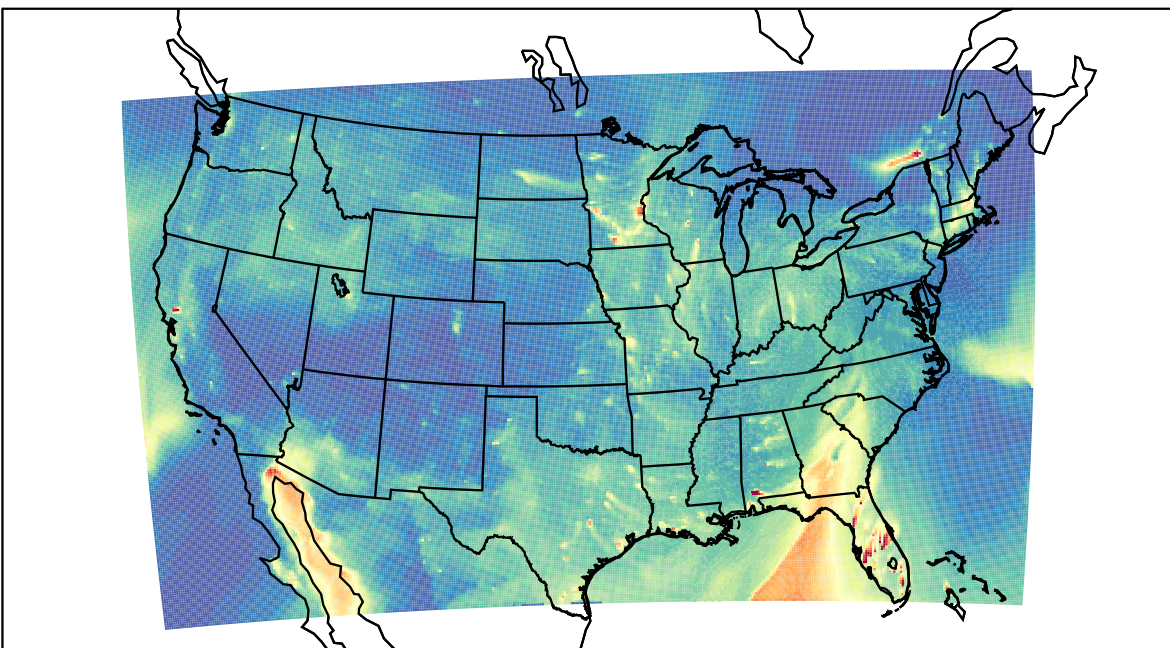
WRF 2023-03-04_01:00:00
