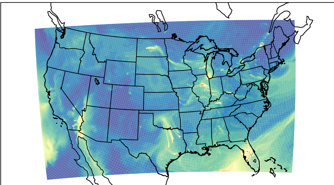
WRF 2023-03-04_21:00:00
