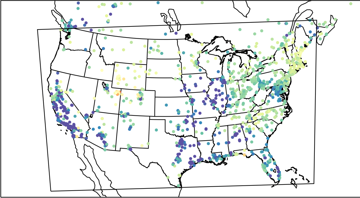
AirNOW (2023-03-04_07:00:00)
