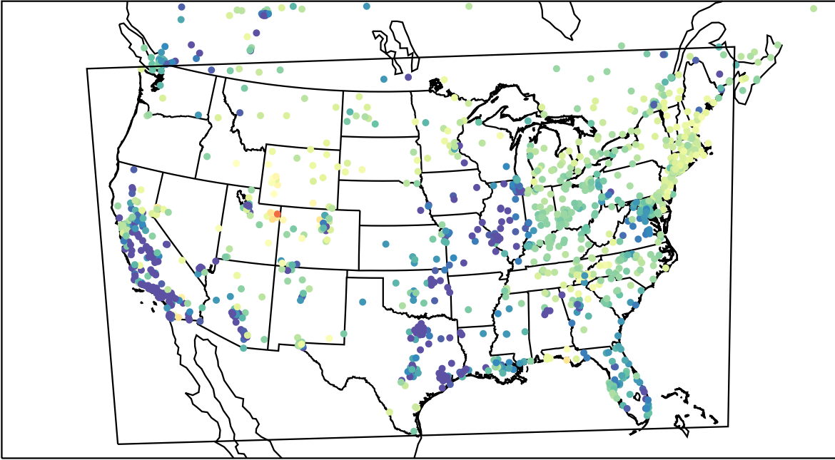
AirNOW (2023-03-04_06:00:00)
