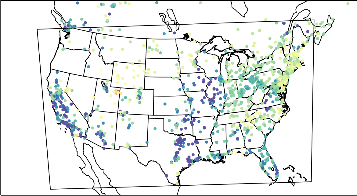
AirNOW (2023-03-04_04:00:00)
