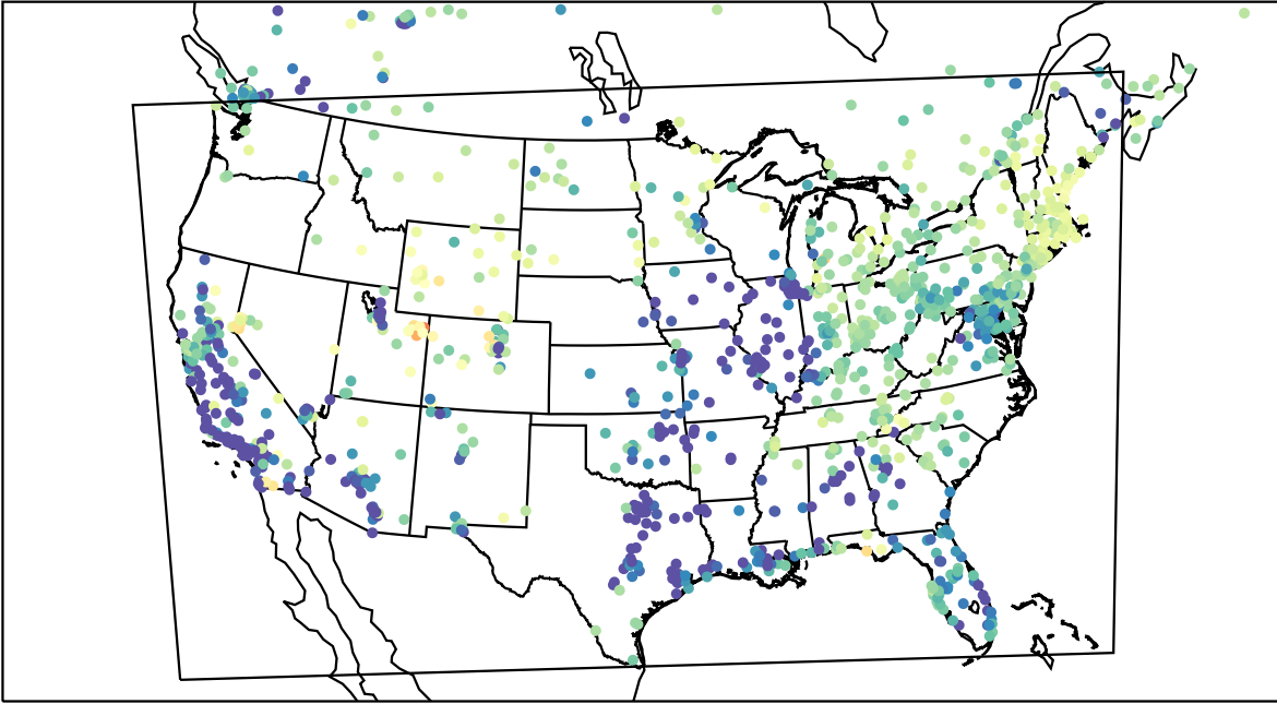
AirNOW (2023-03-04_08:00:00)
