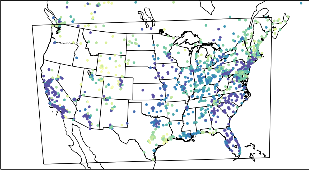
AirNOW (2023-03-03_12:00:00)
