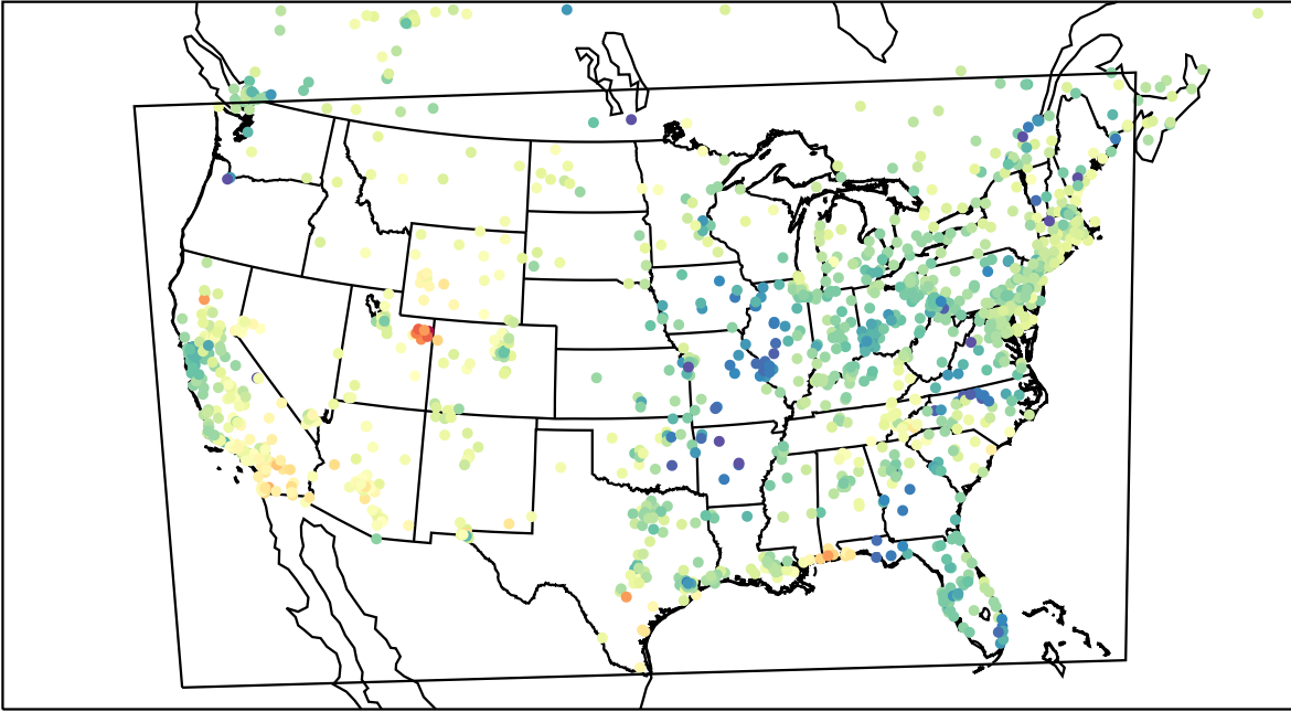
AirNOW (2023-03-04_00:00:00)
