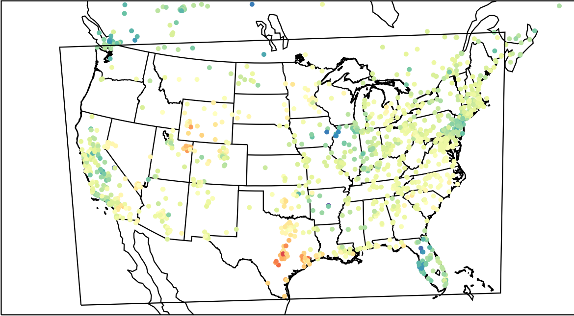
AirNOW (2023-03-04_19:00:00)
