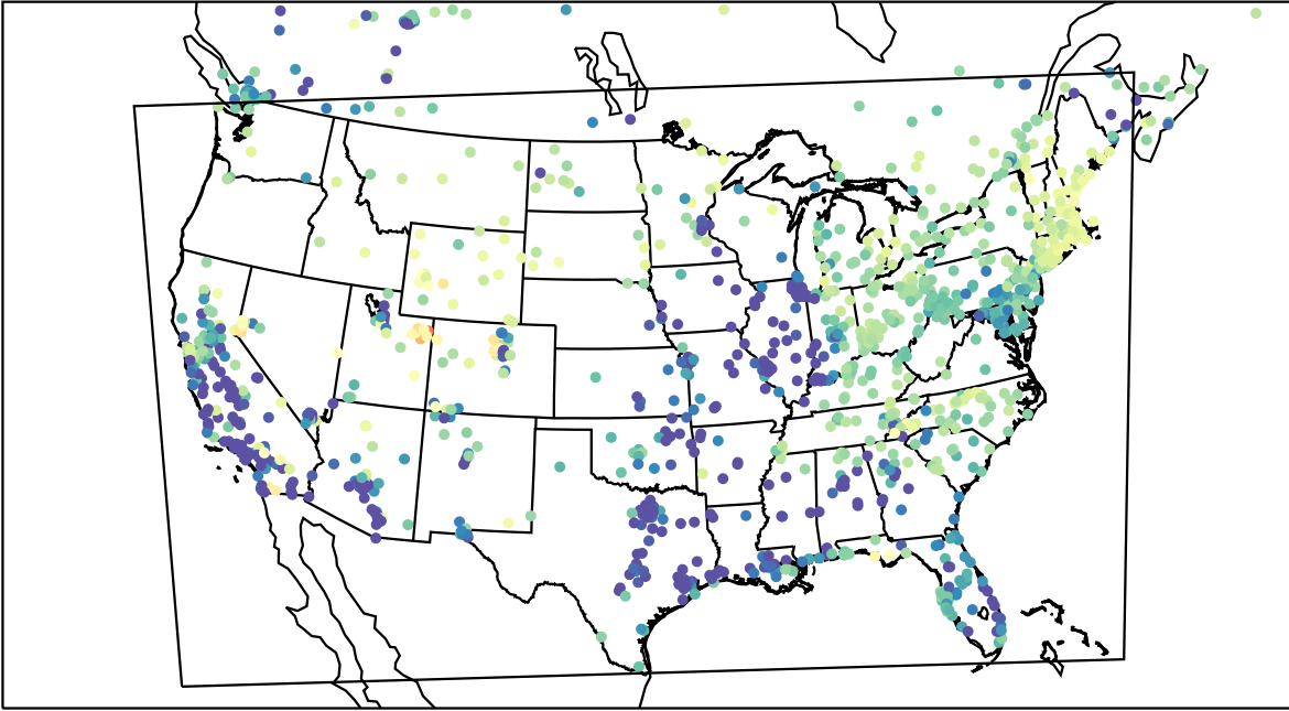
AirNOW (2023-03-04_09:00:00)
