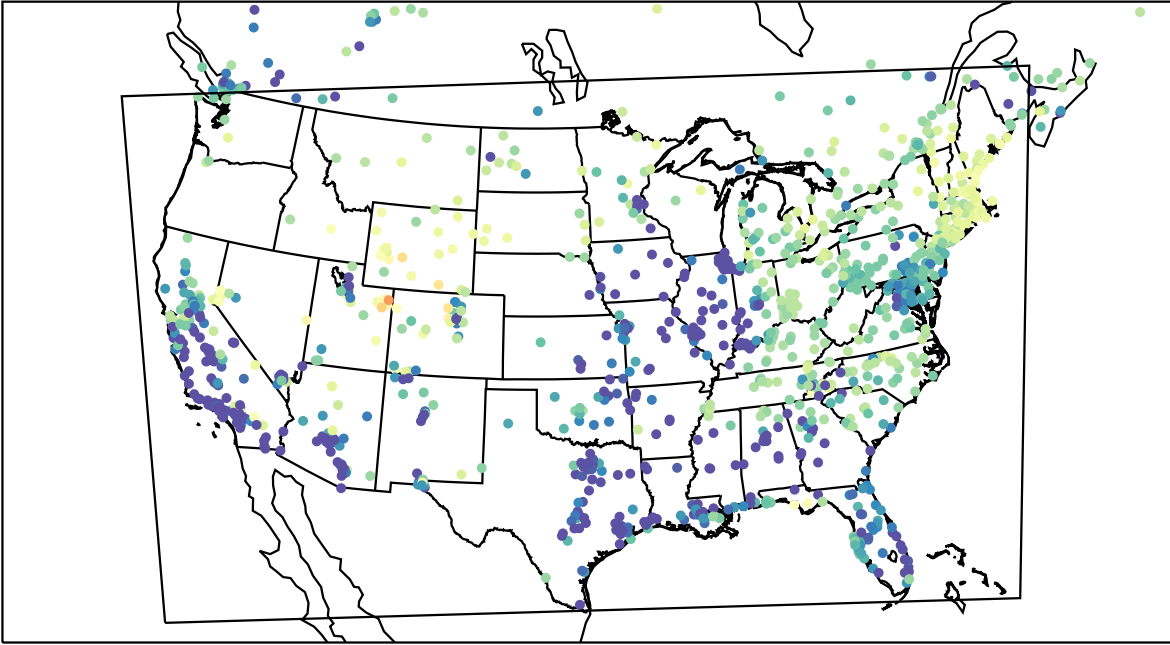
AirNOW (2023-03-04_10:00:00)
