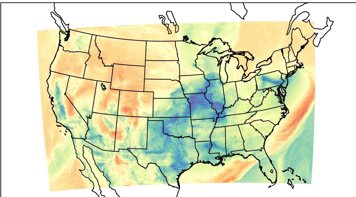
WRF (2023-03-04_15:00:00)
