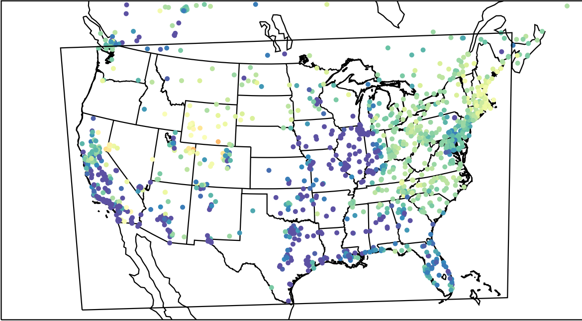
AirNOW (2023-03-04_13:00:00)
