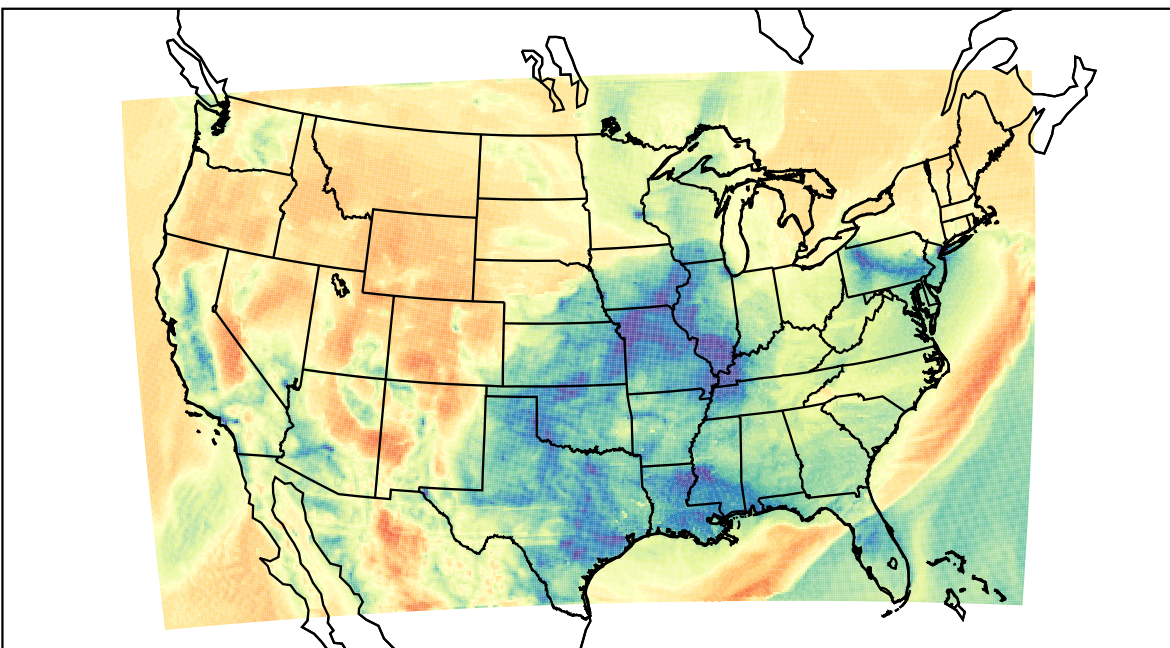
WRF (2023-03-04_14:00:00)
