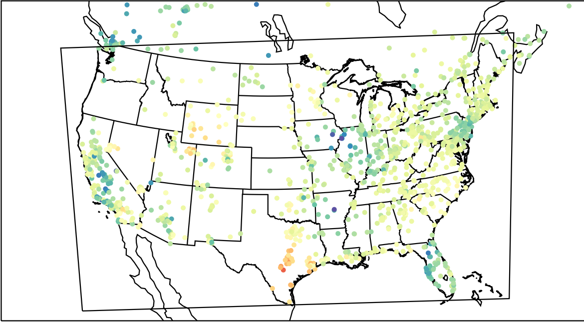
AirNOW (2023-03-04_18:00:00)
