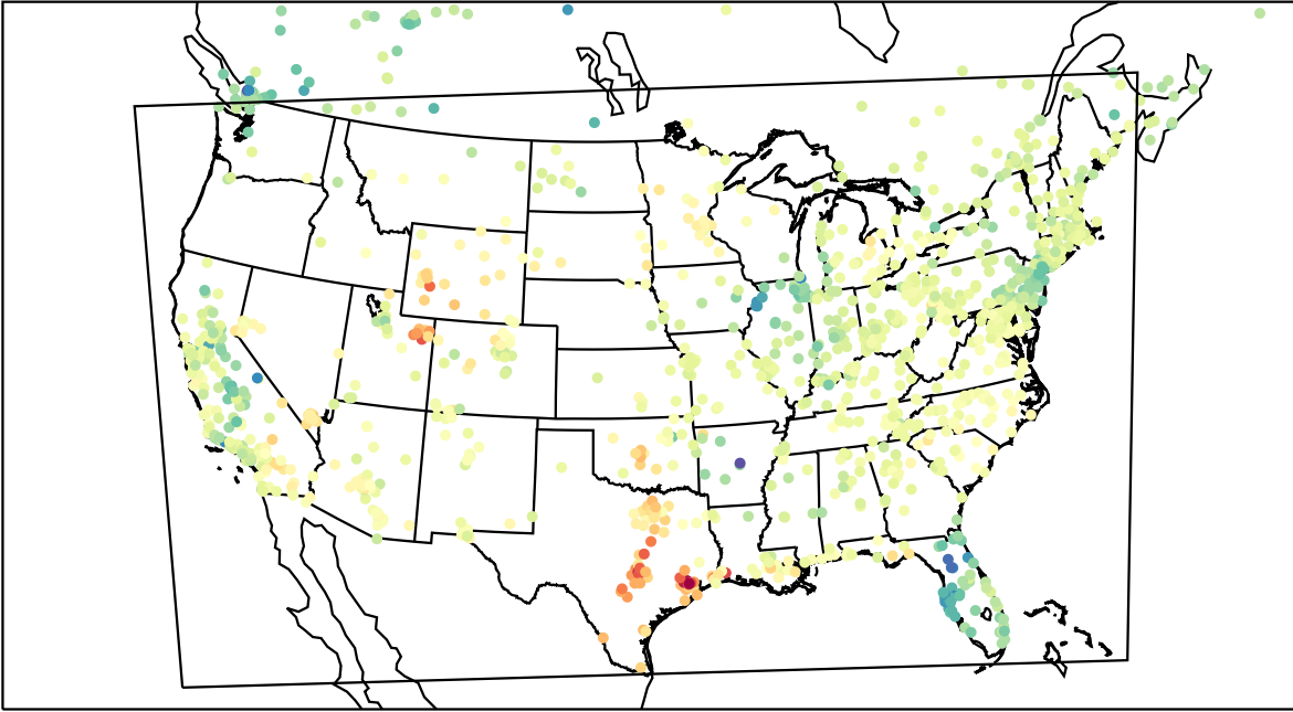
AirNOW (2023-03-04_20:00:00)
