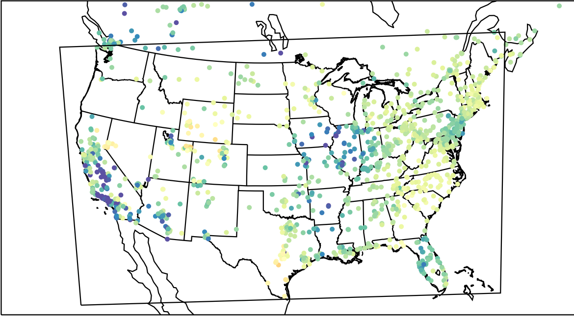
AirNOW (2023-03-04_16:00:00)
