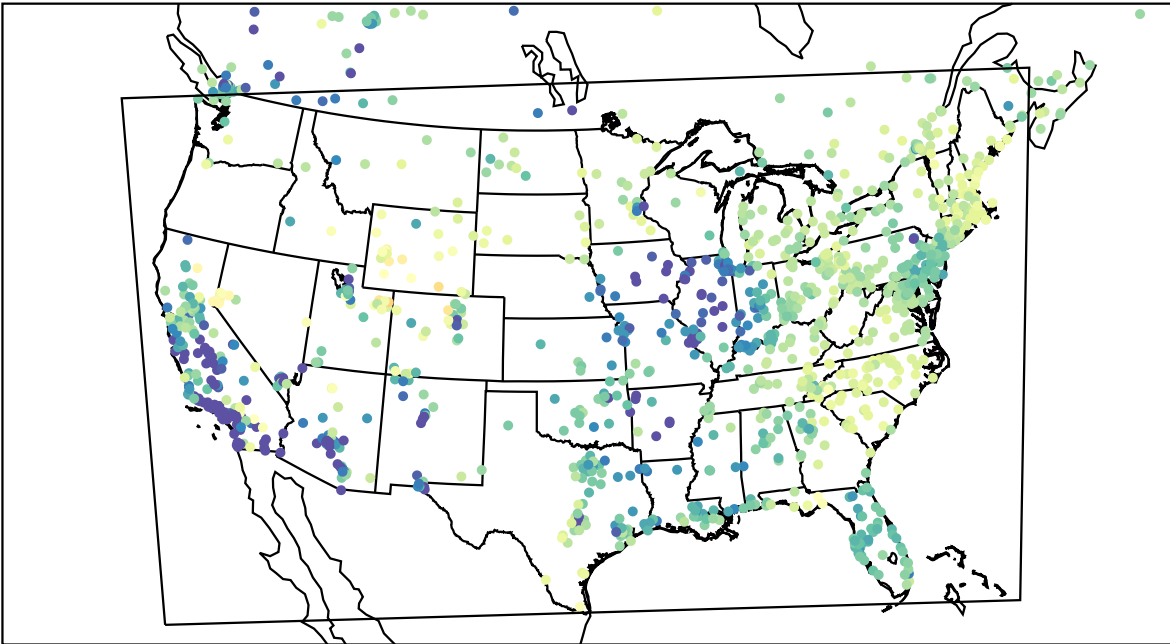
AirNOW (2023-03-04_15:00:00)
