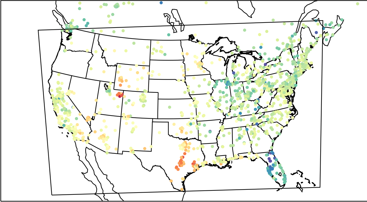
AirNOW (2023-03-04_23:00:00)
