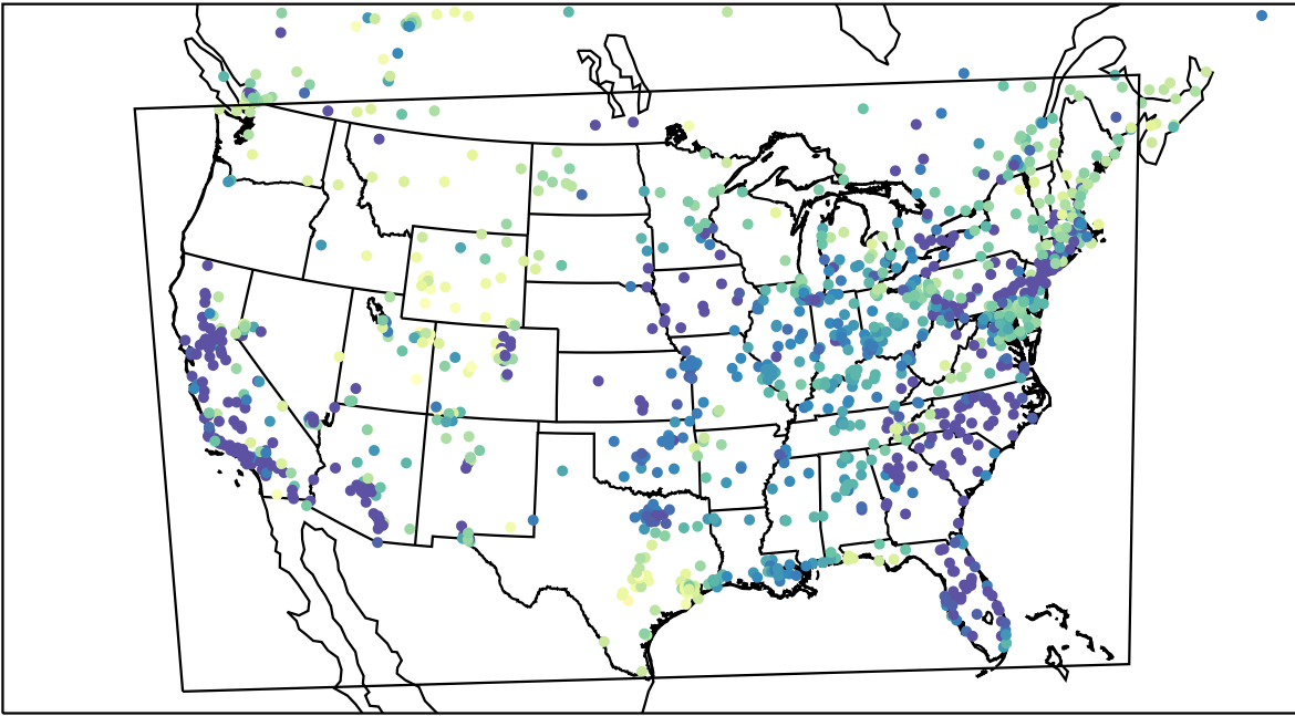
AirNOW (2023-03-03_11:00:00)
