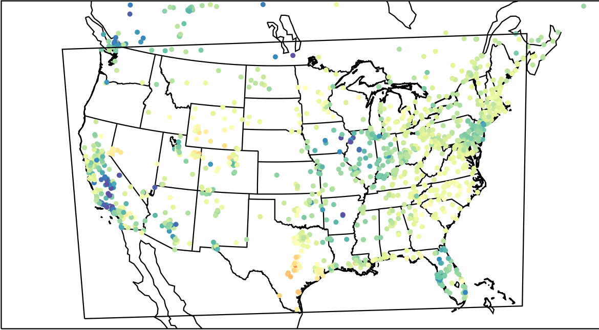
AirNOW (2023-03-04_17:00:00)
