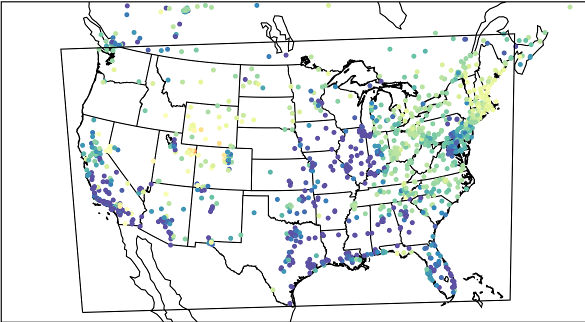
AirNOW (2023-03-04_11:00:00)
