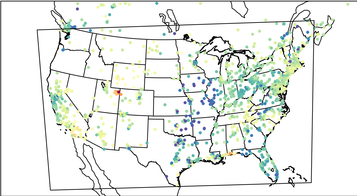
AirNOW (2023-03-04_01:00:00)
