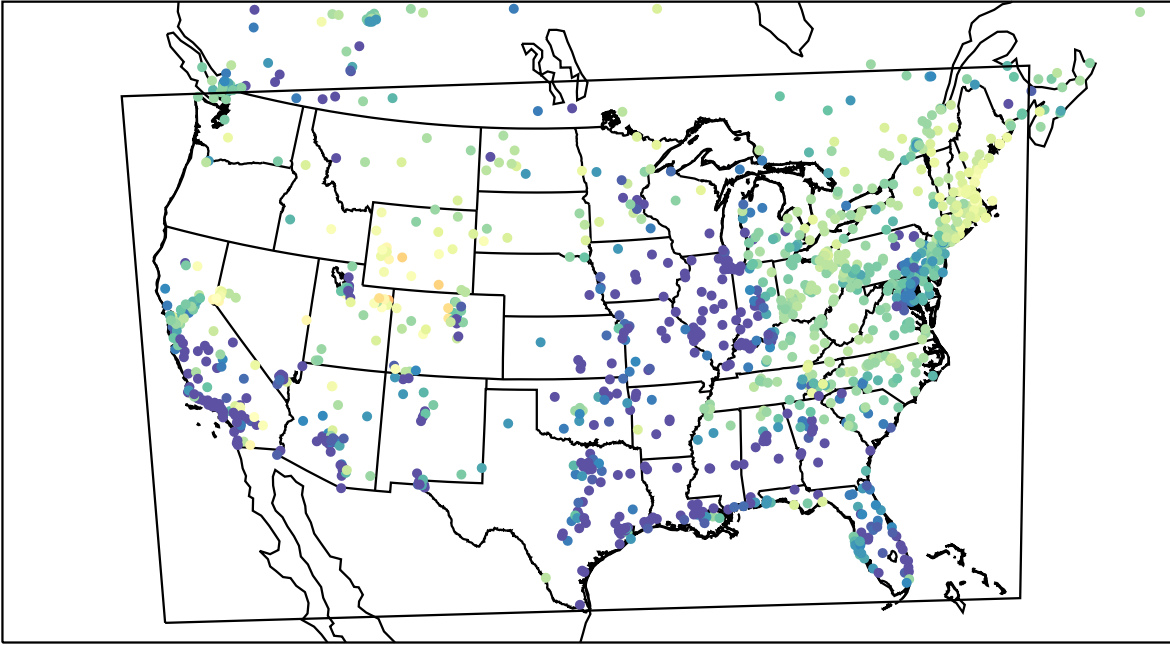
AirNOW (2023-03-04_12:00:00)
