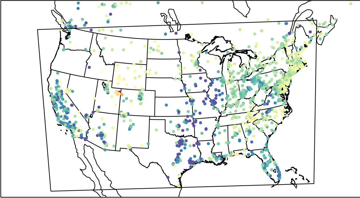
AirNOW (2023-03-04_03:00:00)
