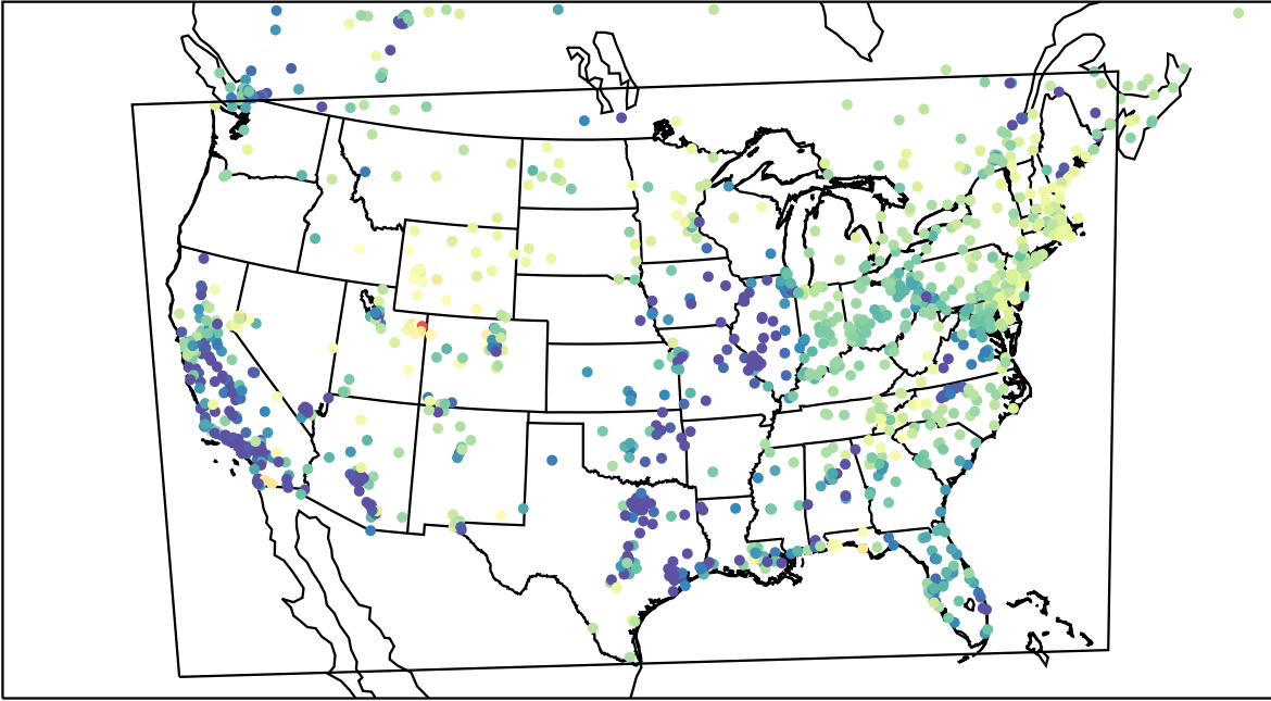
AirNOW (2023-03-04_05:00:00)
