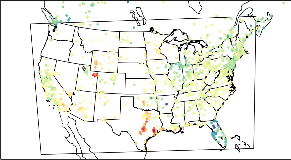
AirNOW (2023-03-04_22:00:00)
