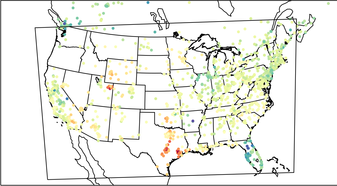
AirNOW (2023-03-04_21:00:00)
