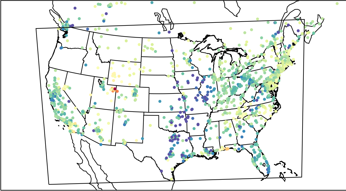
AirNOW (2023-03-04_02:00:00)
