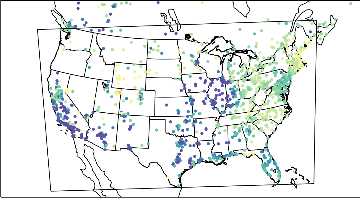
AirNOW (2023-03-04_14:00:00)
