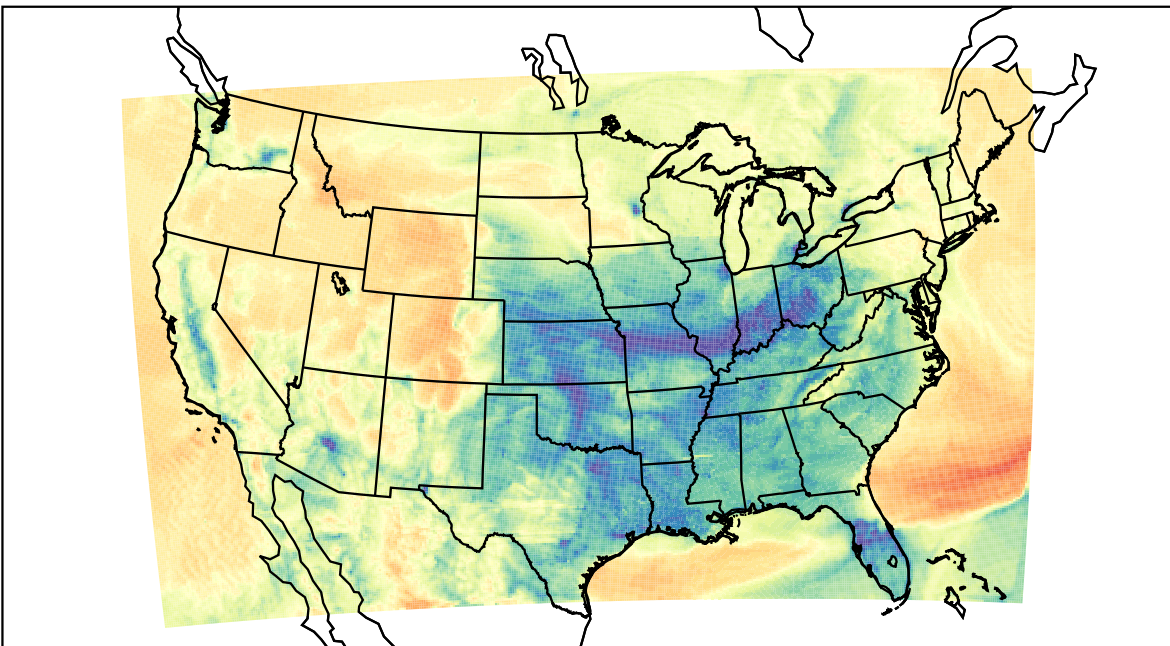
WRF (2023-03-05_14:00:00)
