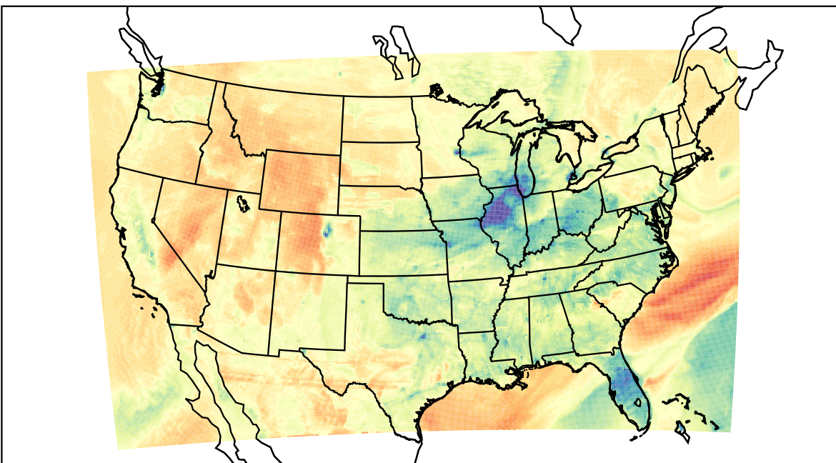
WRF (2023-03-05_01:00:00)
