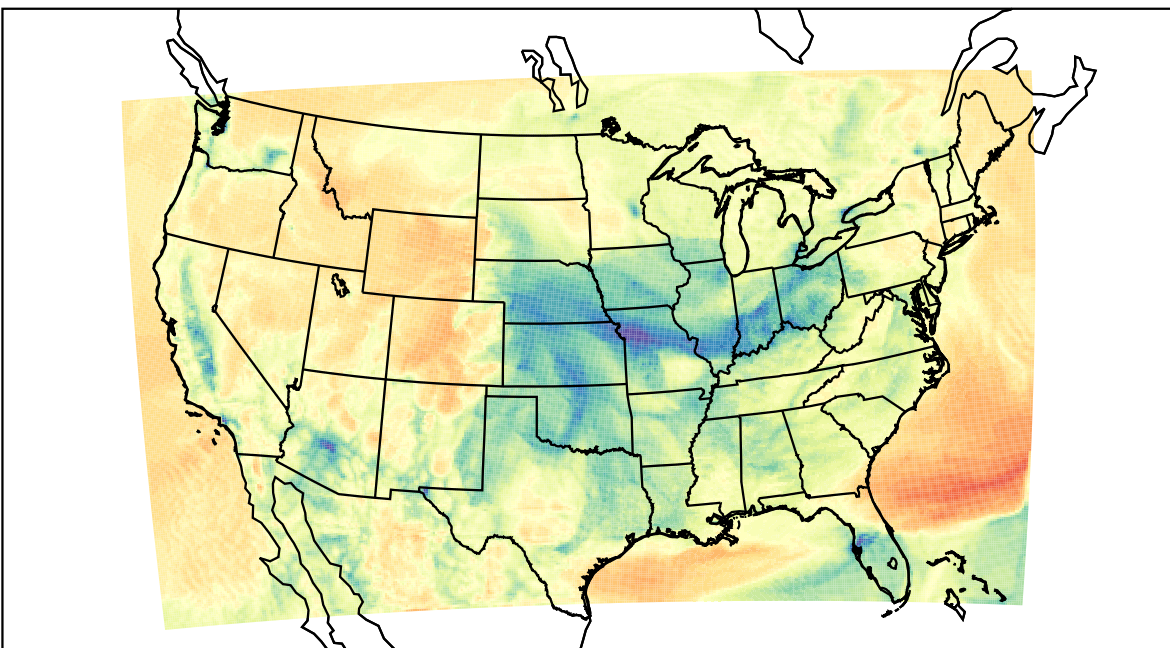
WRF (2023-03-05_16:00:00)
