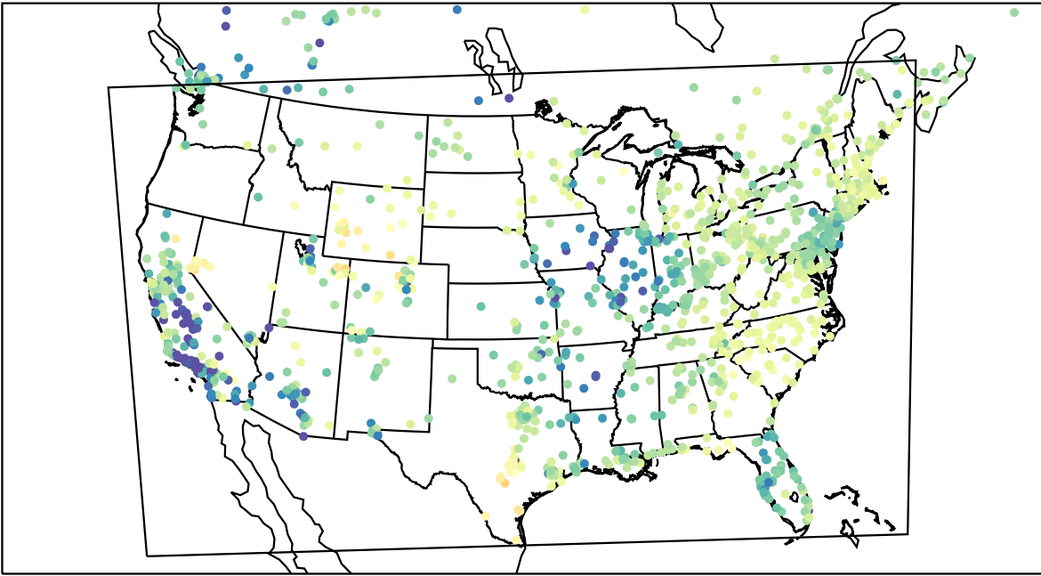
AirNOW (2023-03-04_16:00:00)
