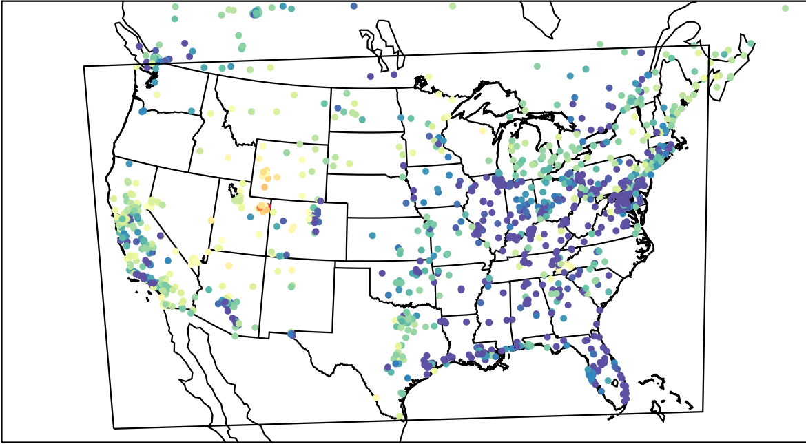
AirNOW (2023-03-05_08:00:00)
