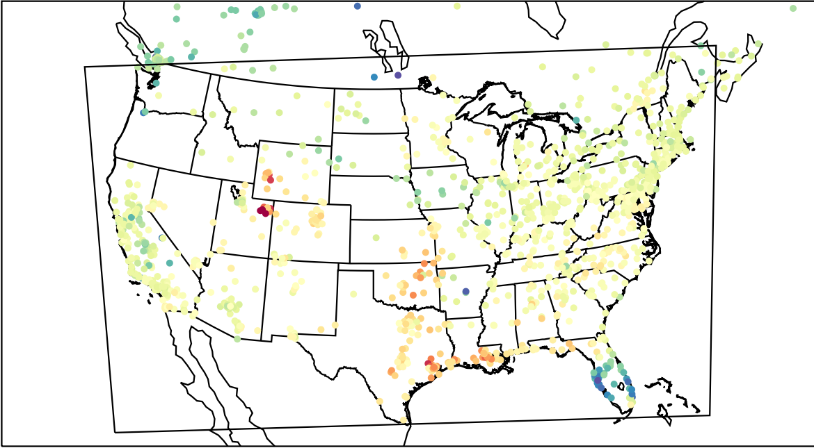
AirNOW (2023-03-05_20:00:00)
