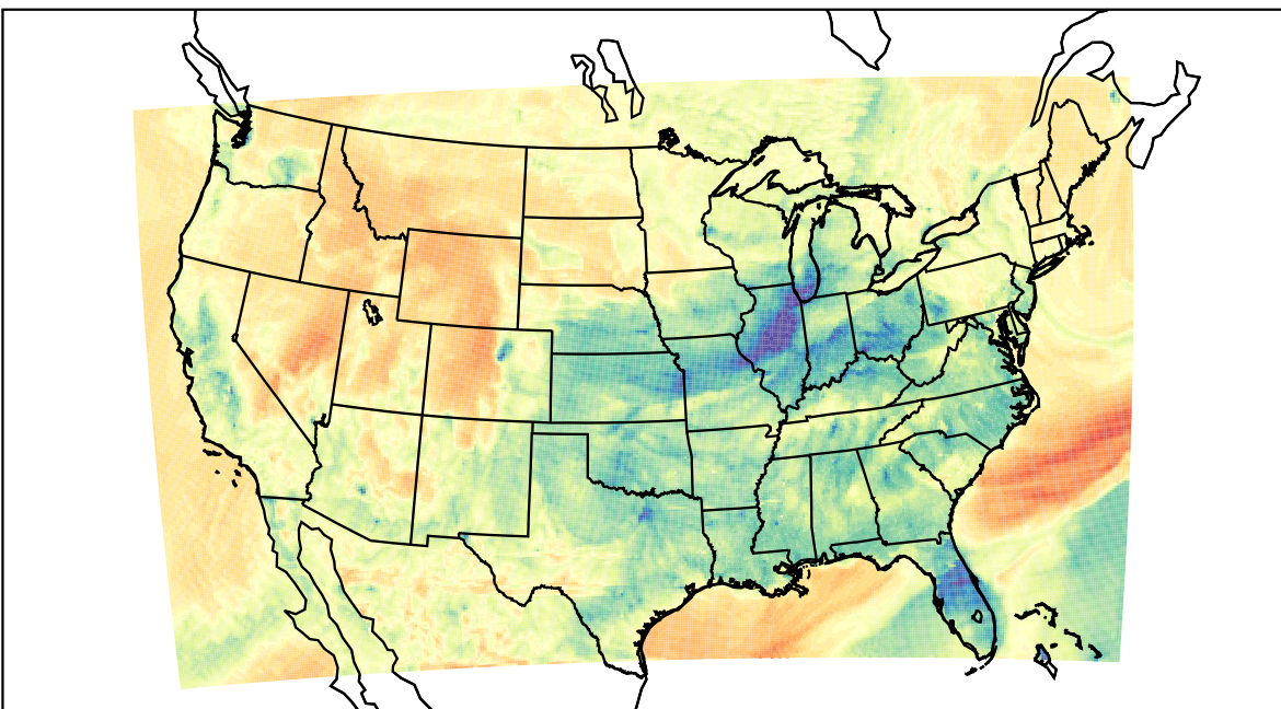
WRF (2023-03-05_04:00:00)
