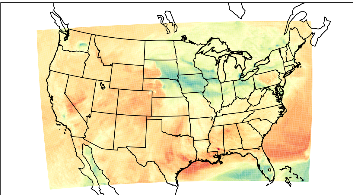
WRF (2023-03-05_22:00:00)
