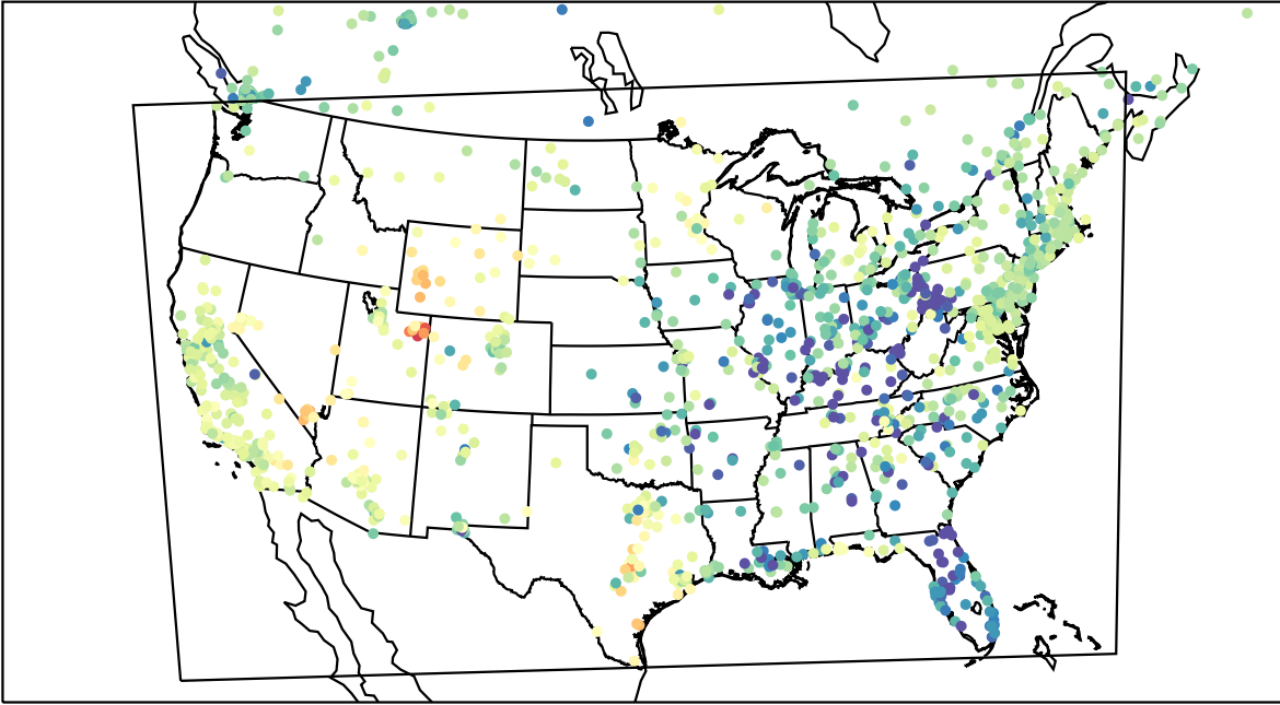
AirNOW (2023-03-05_01:00:00)
