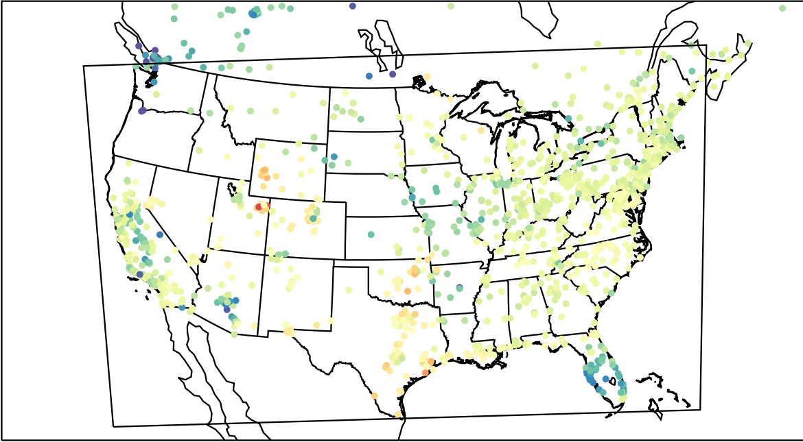
AirNOW (2023-03-05_17:00:00)
