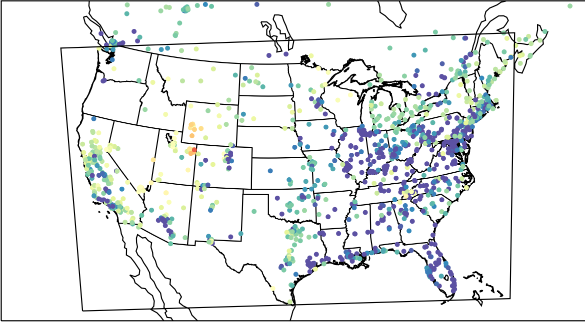
AirNOW (2023-03-05_09:00:00)
