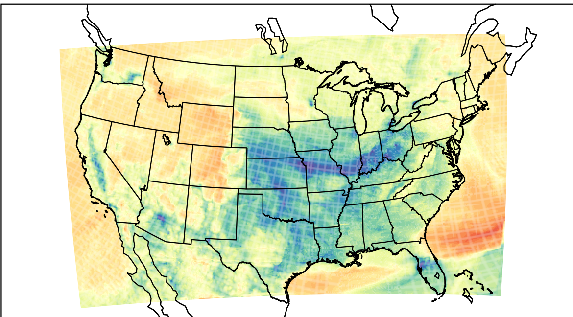
WRF (2023-03-05_15:00:00)
