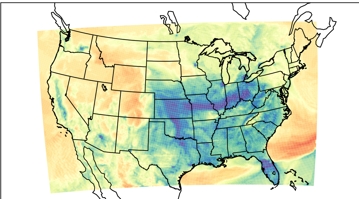
WRF (2023-03-05_13:00:00)
