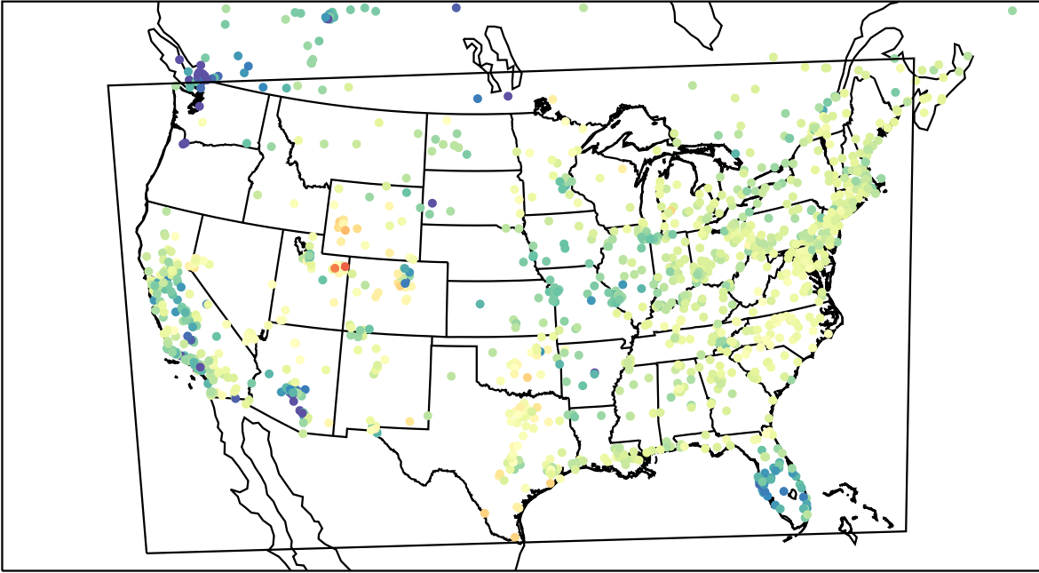
AirNOW (2023-03-05_16:00:00)
