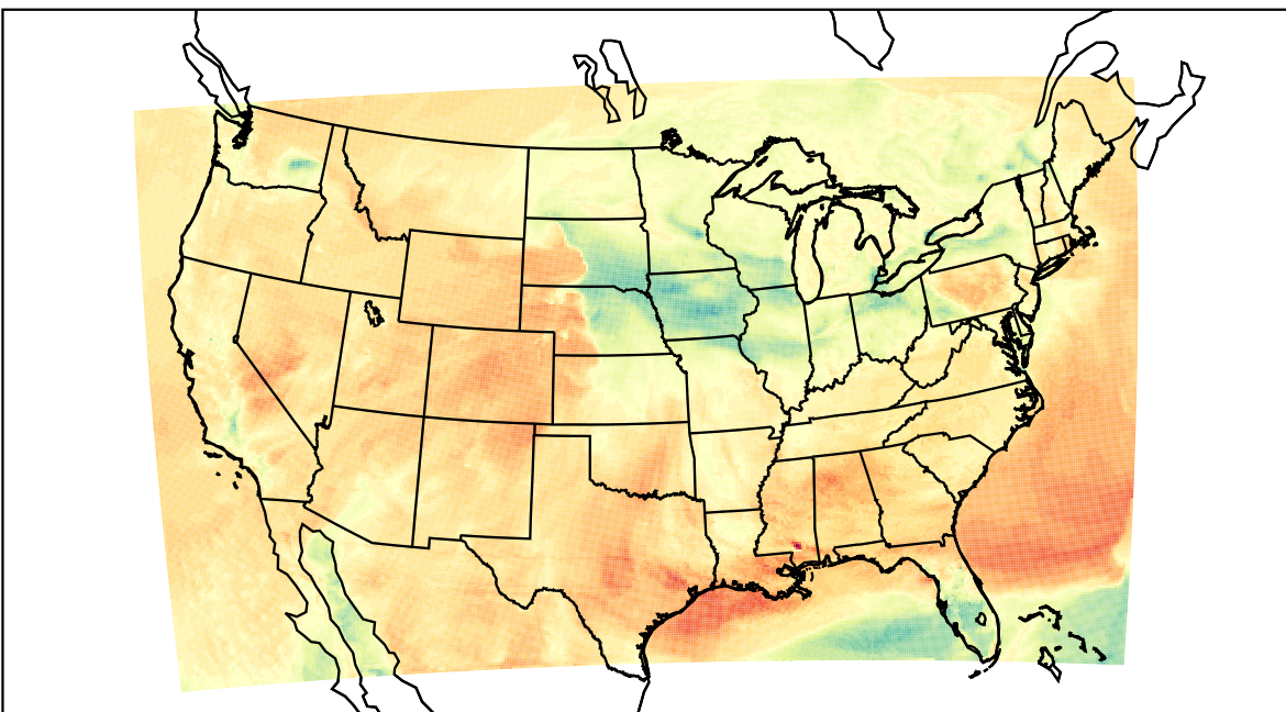
WRF (2023-03-05_21:00:00)
