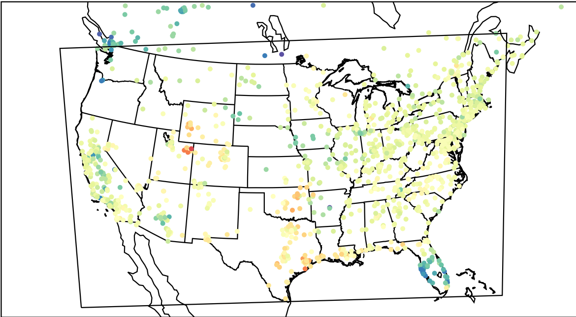
AirNOW (2023-03-05_18:00:00)
