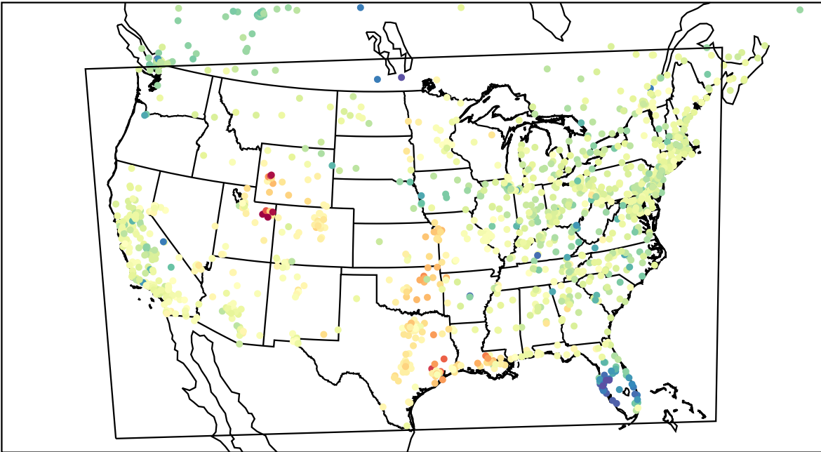
AirNOW (2023-03-05_23:00:00)
