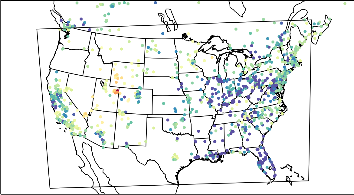
AirNOW (2023-03-05_05:00:00)
