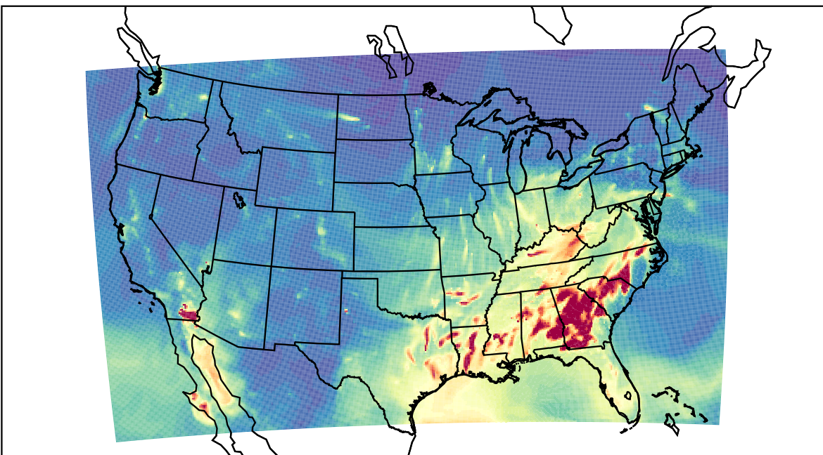
WRF 2023-03-07_05:00:00
