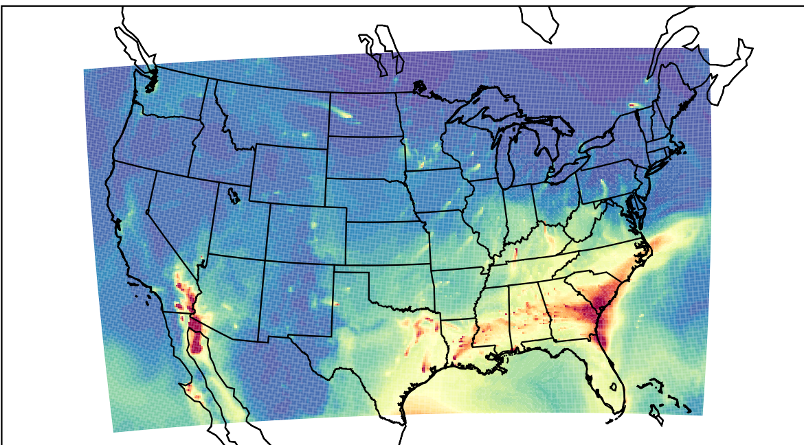
WRF 2023-03-07_14:00:00
