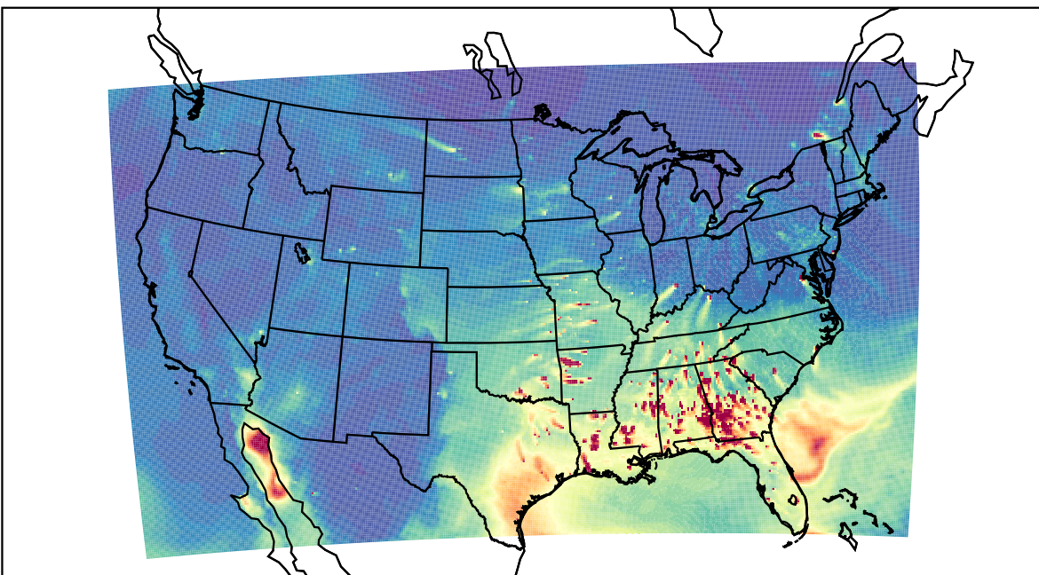
WRF 2023-03-07_23:00:00
