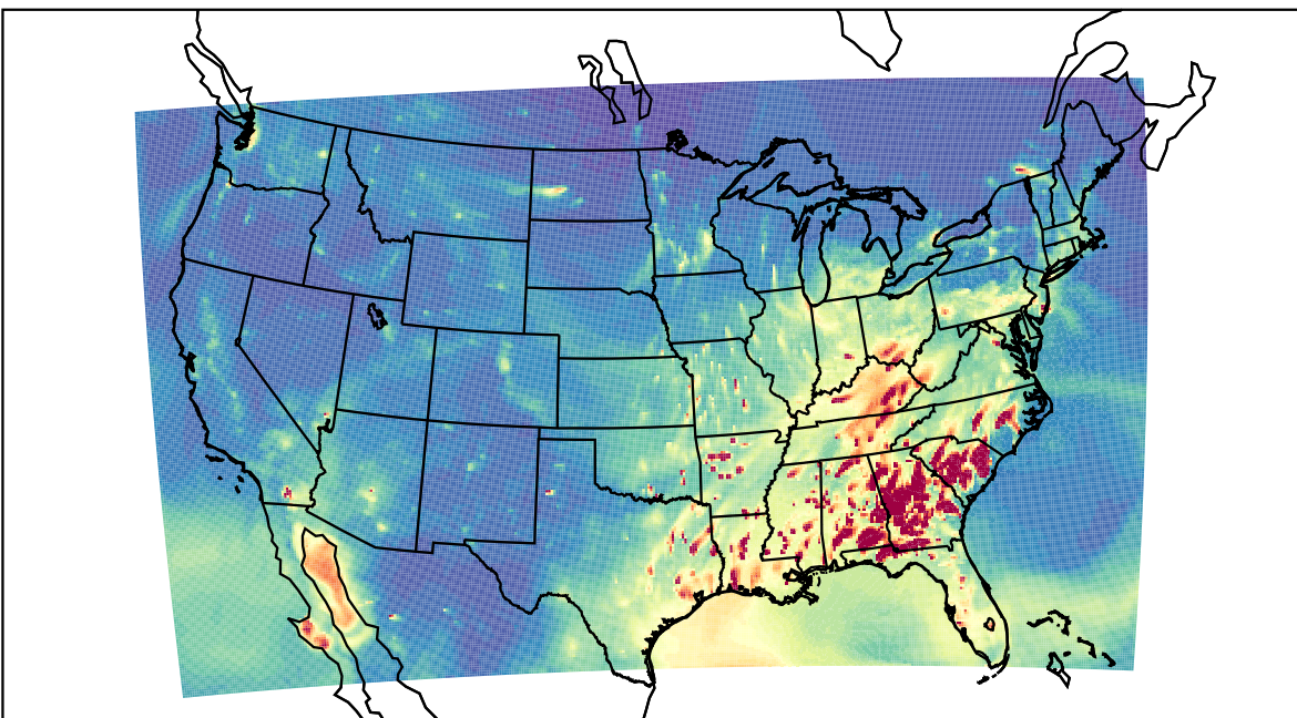
WRF 2023-03-07_02:00:00
