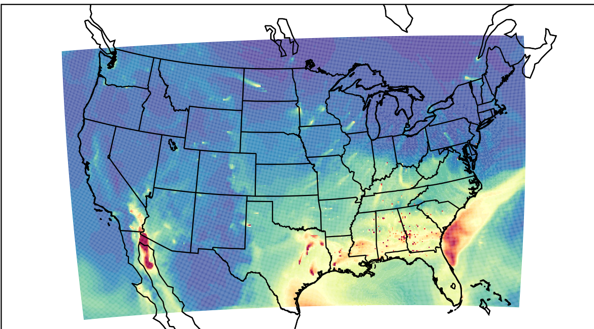
WRF 2023-03-07_17:00:00
