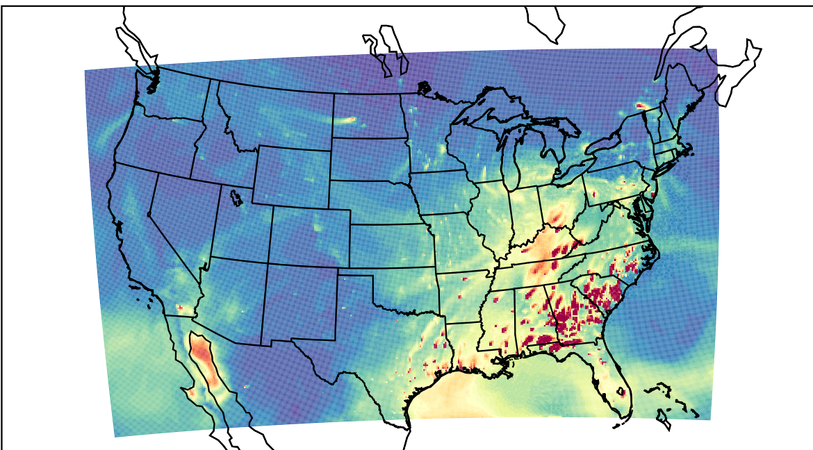
WRF 2023-03-07_00:00:00
