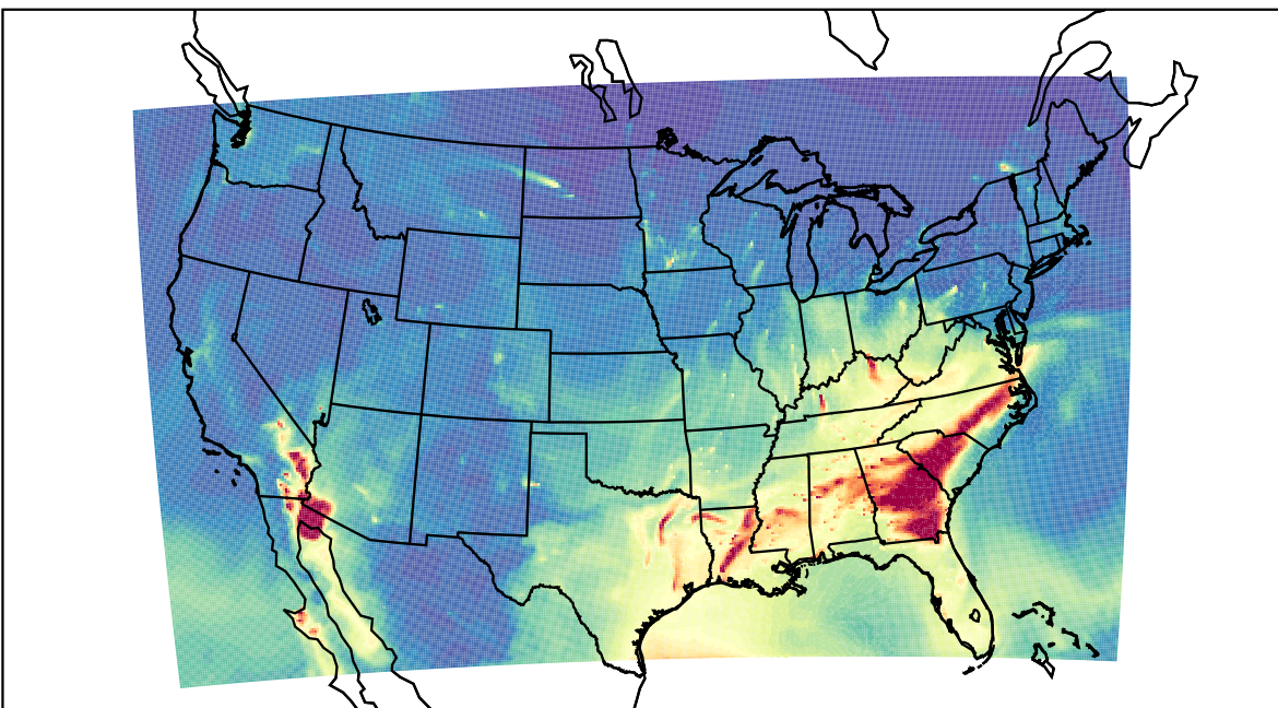
WRF 2023-03-07_10:00:00
