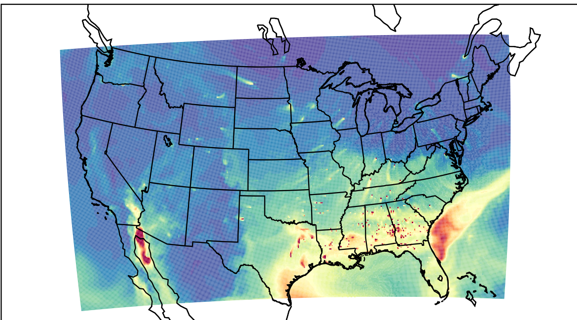
WRF 2023-03-07_18:00:00
