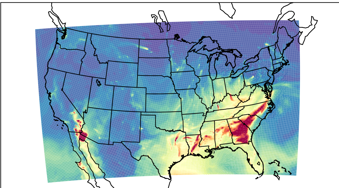
WRF 2023-03-07_09:00:00
