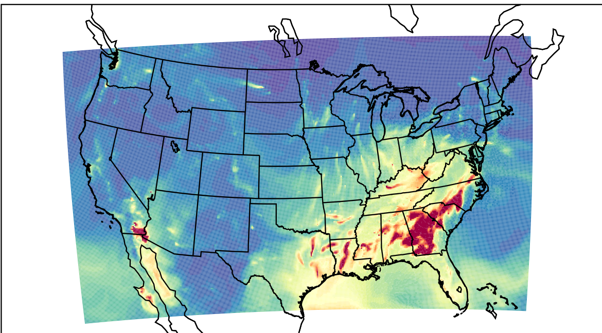
WRF 2023-03-07_06:00:00
