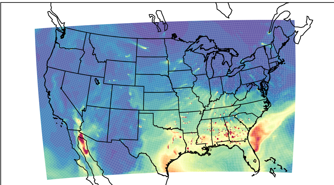
WRF 2023-03-07_19:00:00
