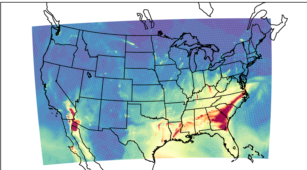
WRF 2023-03-07_11:00:00
