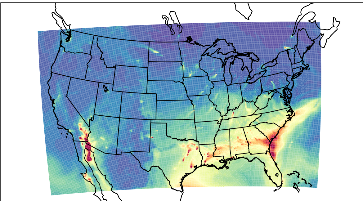
WRF 2023-03-07_15:00:00
