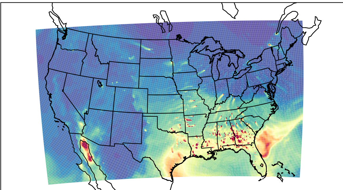
WRF 2023-03-07_21:00:00
