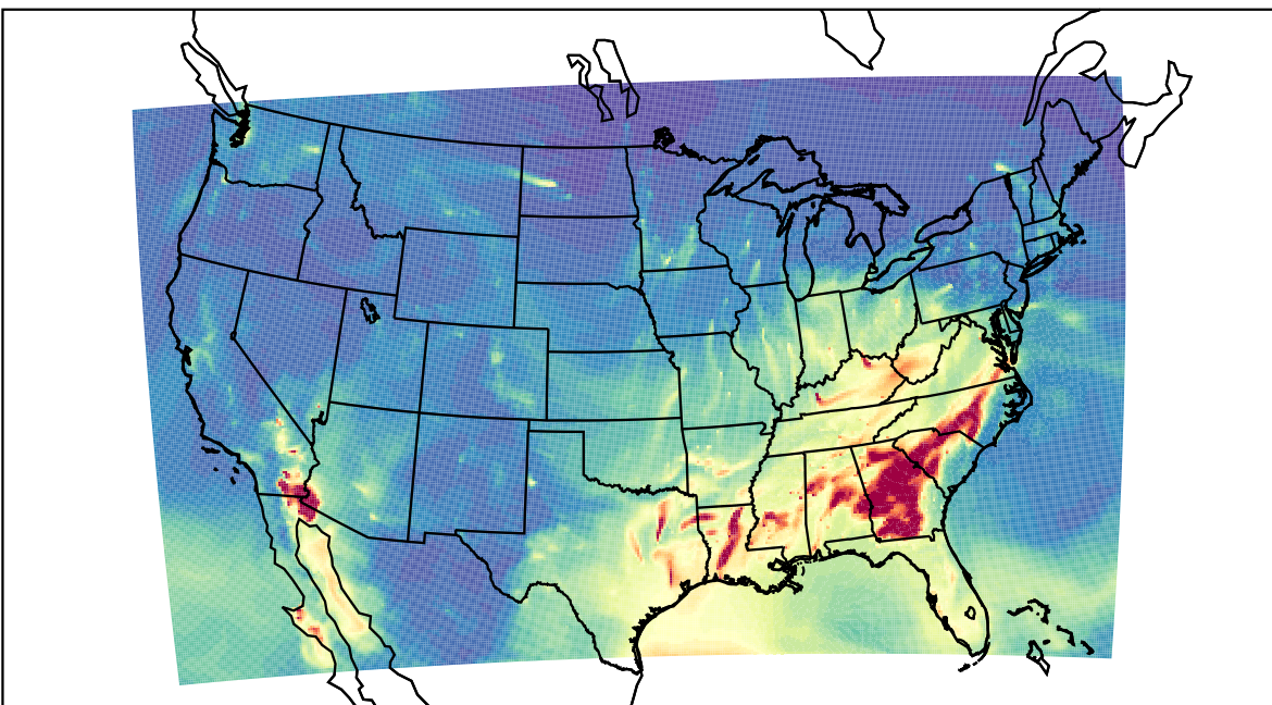
WRF 2023-03-07_07:00:00
