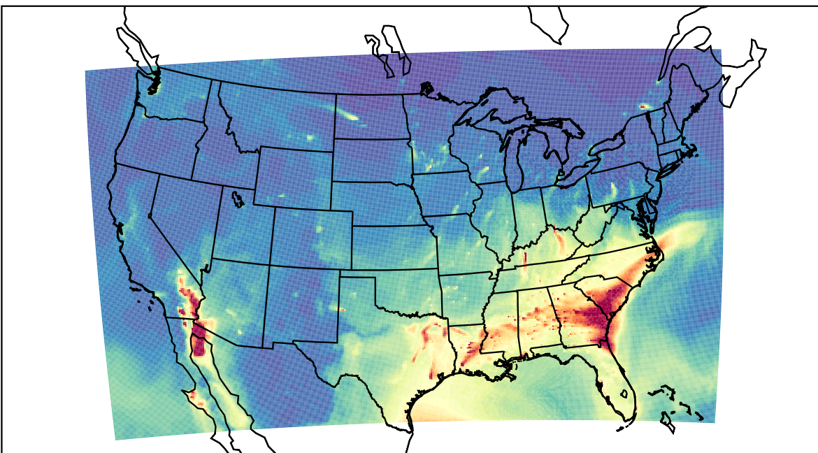
WRF 2023-03-07_13:00:00
