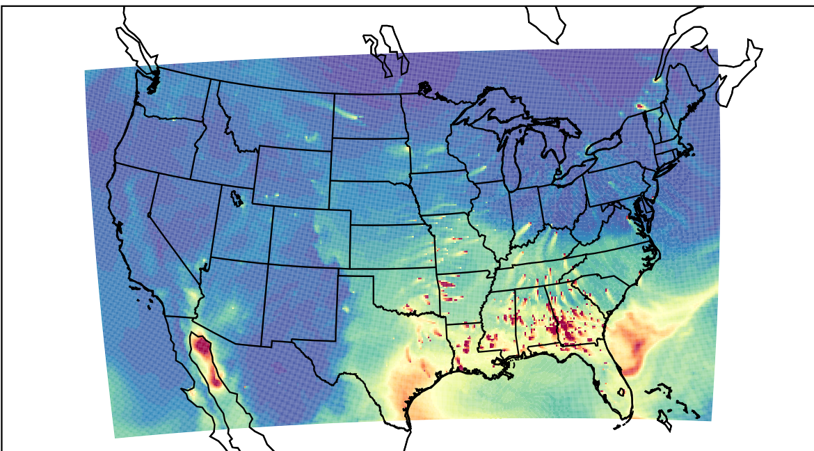
WRF 2023-03-07_22:00:00
