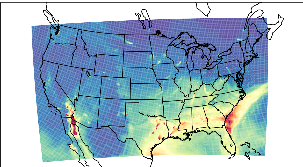
WRF 2023-03-07_16:00:00
