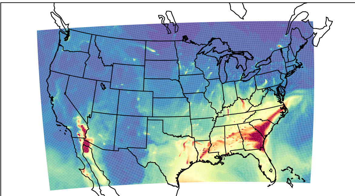
WRF 2023-03-07_12:00:00
