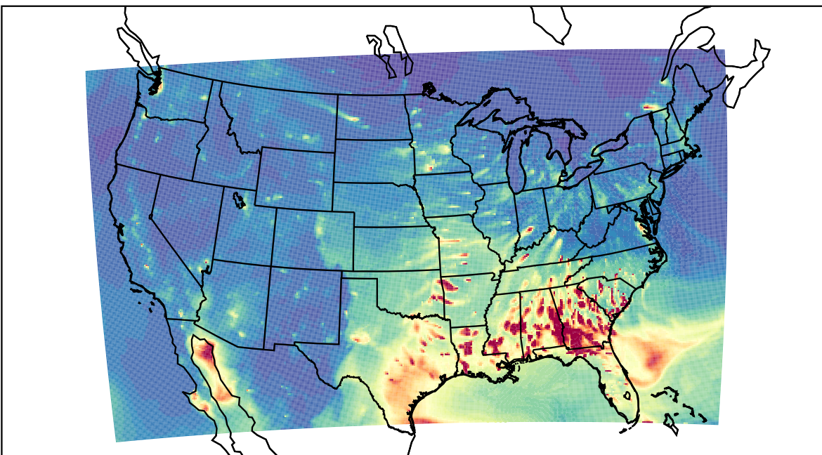
WRF 2023-03-08_02:00:00
