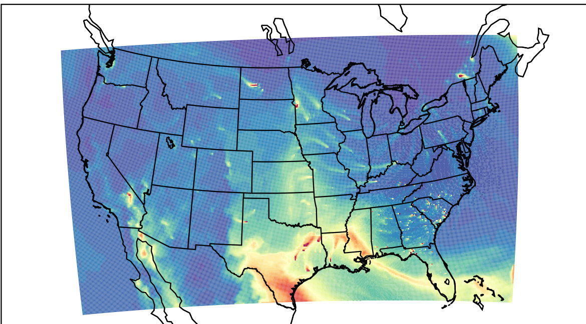
WRF 2023-03-08_17:00:00
