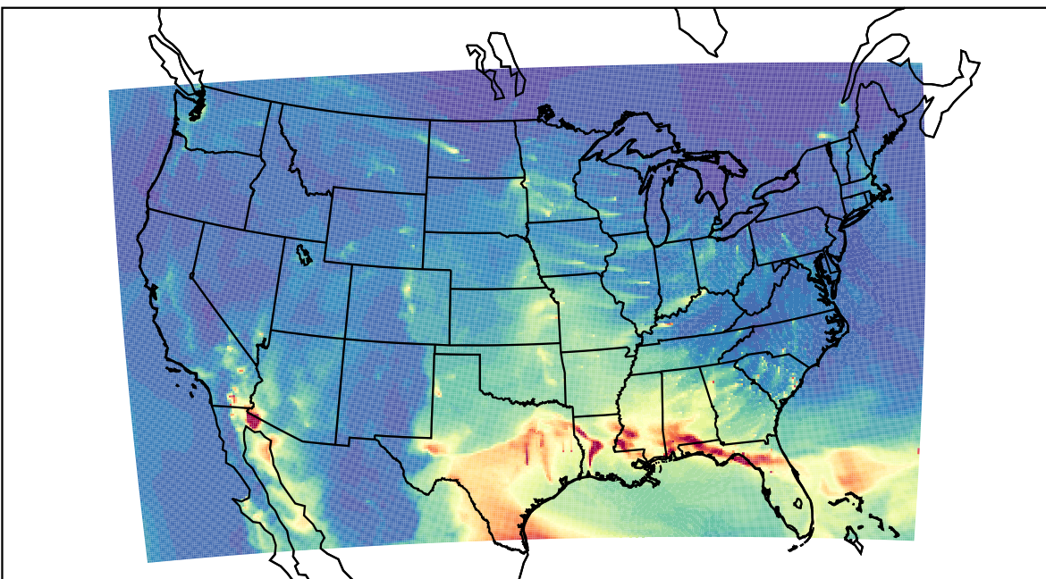
WRF 2023-03-08_09:00:00
