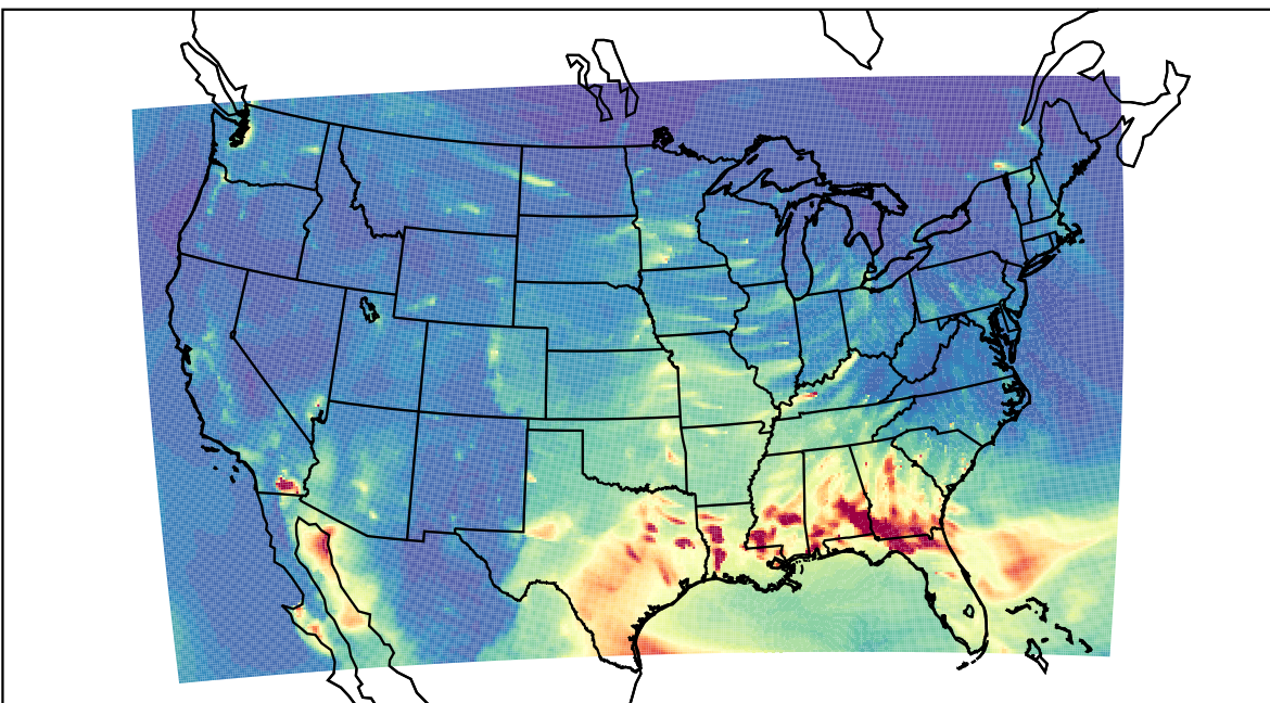
WRF 2023-03-08_05:00:00
