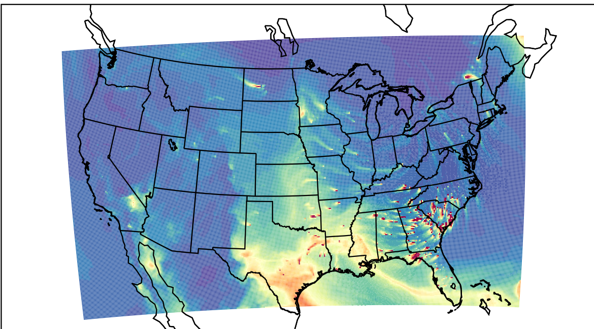
WRF 2023-03-08_21:00:00
