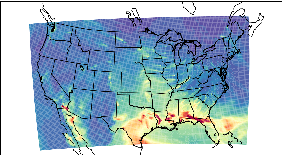
WRF 2023-03-08_07:00:00
