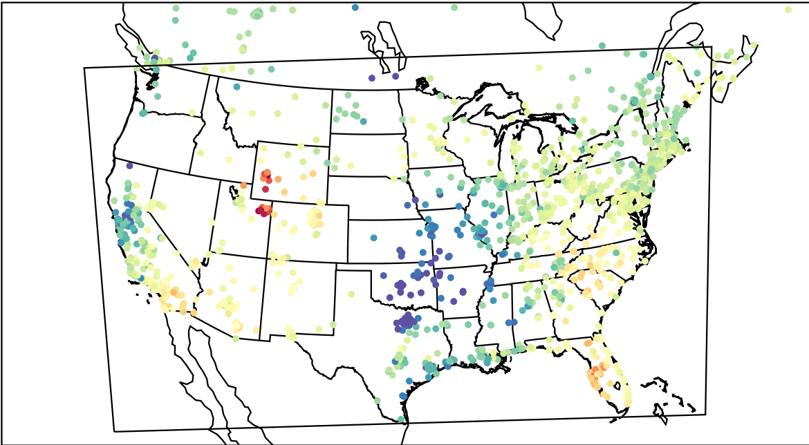
AirNOW (2023-03-09_21:00:00)
