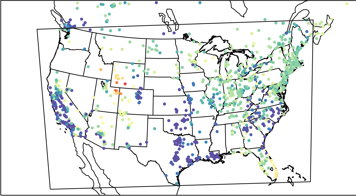
AirNOW (2023-03-09_06:00:00)
