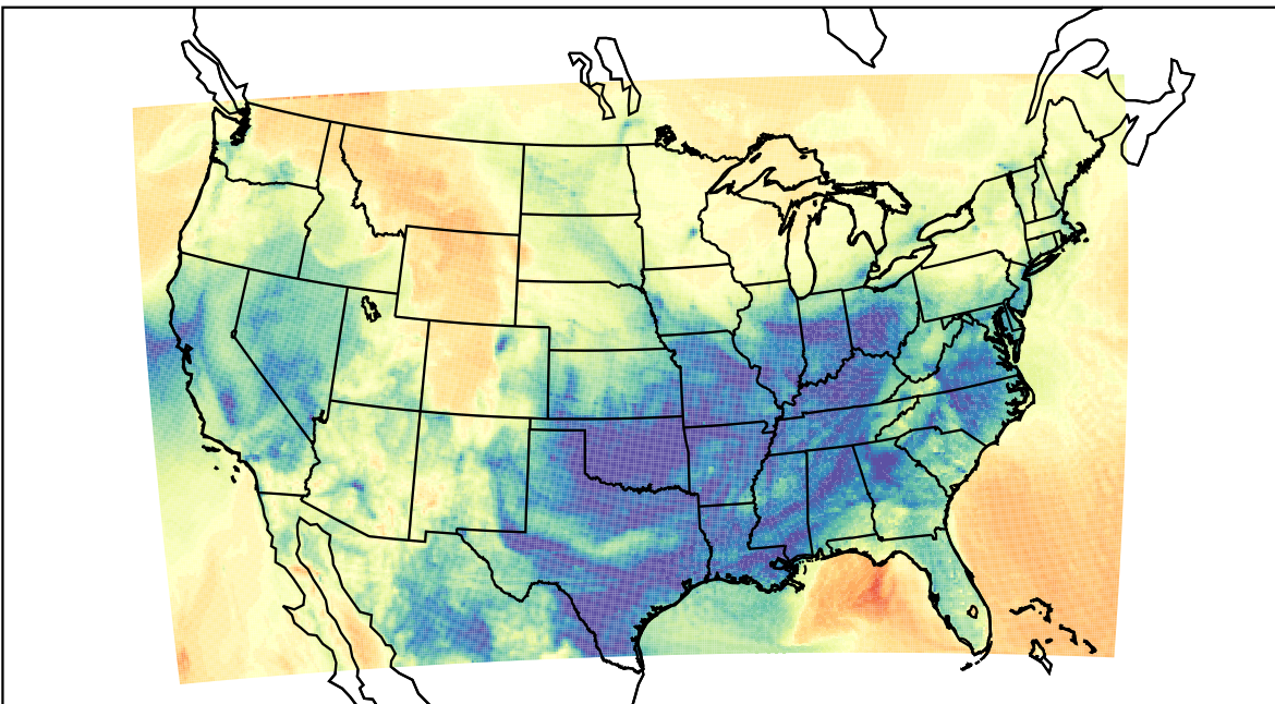
WRF (2023-03-10_13:00:00)
