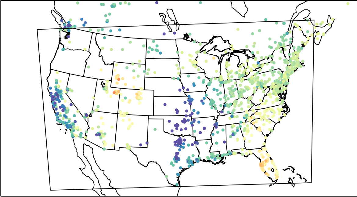
AirNOW (2023-03-09_17:00:00)
