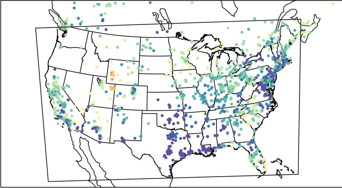
AirNOW (2023-03-10_07:00:00)
