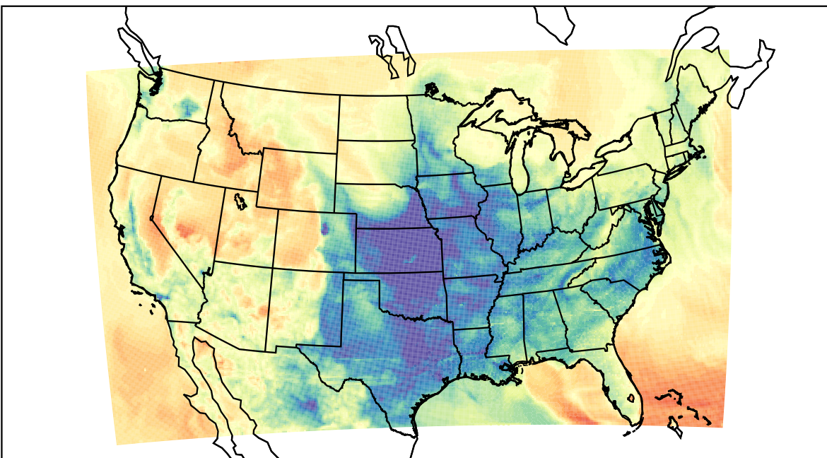
WRF (2023-03-09_07:00:00)
