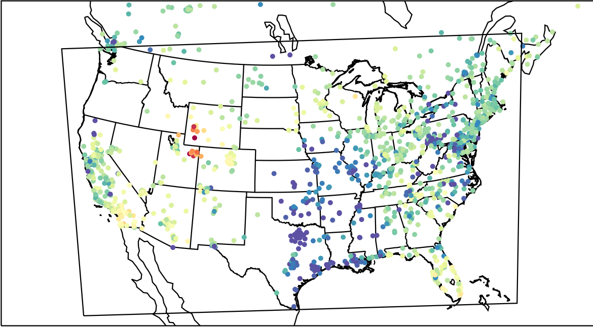
AirNOW (2023-03-10_01:00:00)
