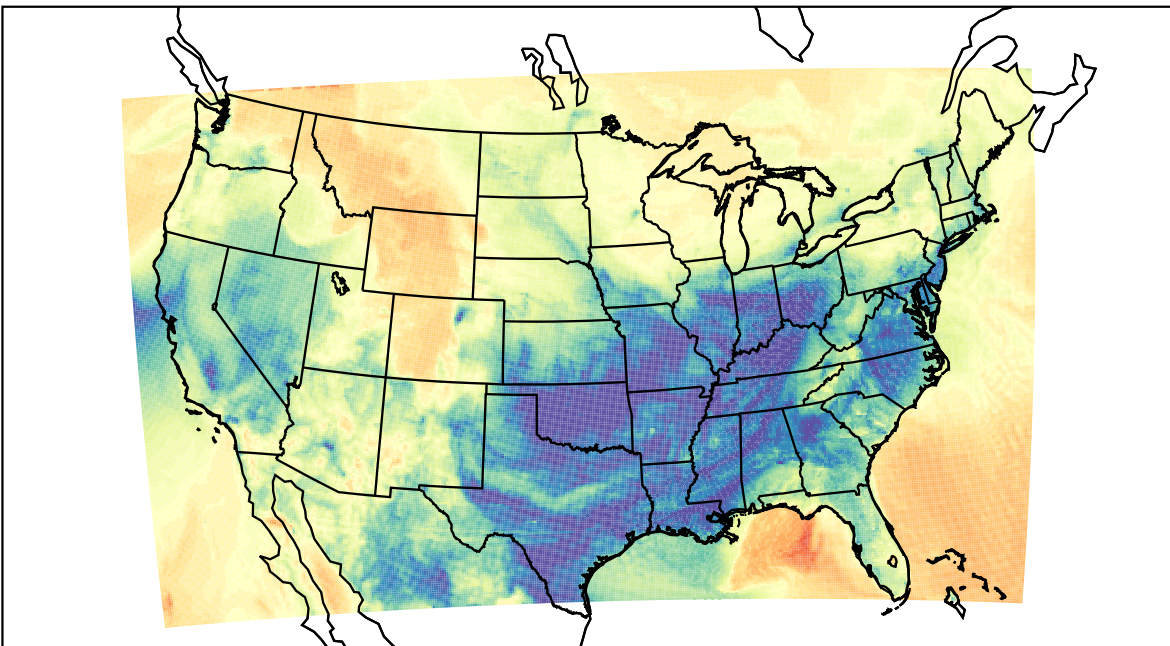
WRF (2023-03-10_12:00:00)
