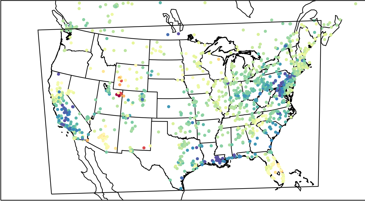
AirNOW (2023-03-10_22:00:00)
