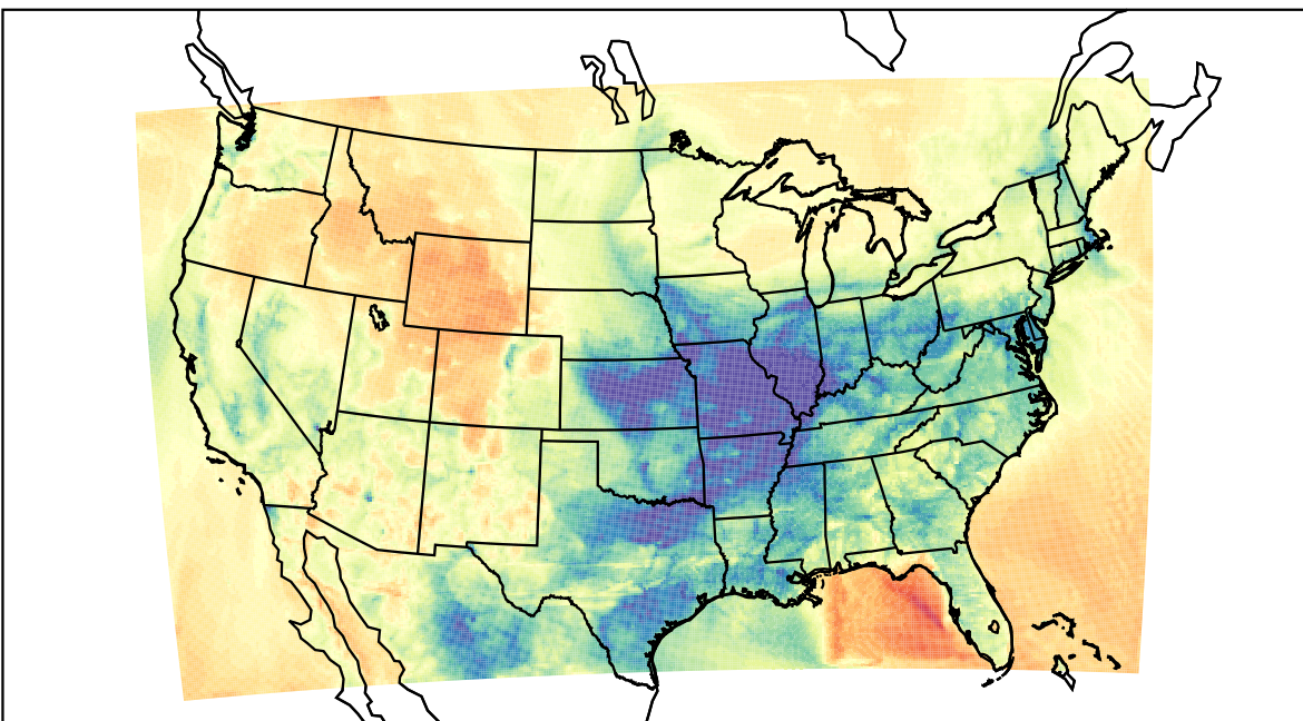
WRF (2023-03-10_03:00:00)
