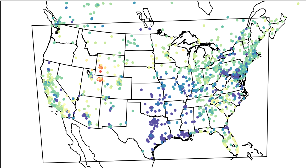
AirNOW (2023-03-10_03:00:00)
