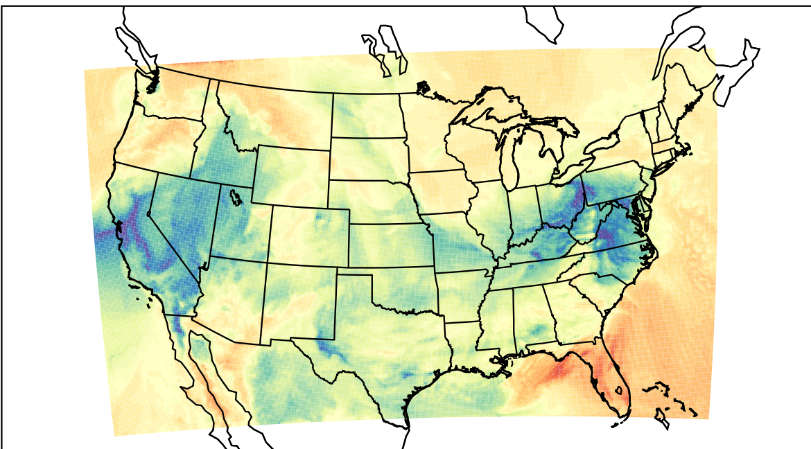
WRF (2023-03-10_19:00:00)
