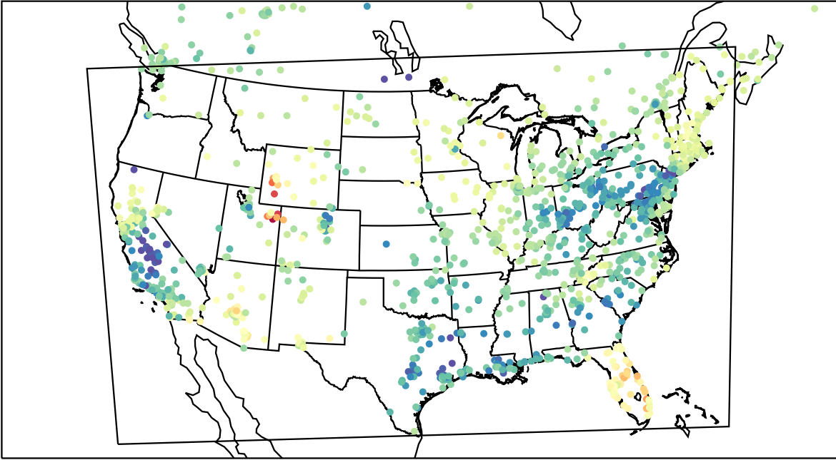
AirNOW (2023-03-10_19:00:00)
