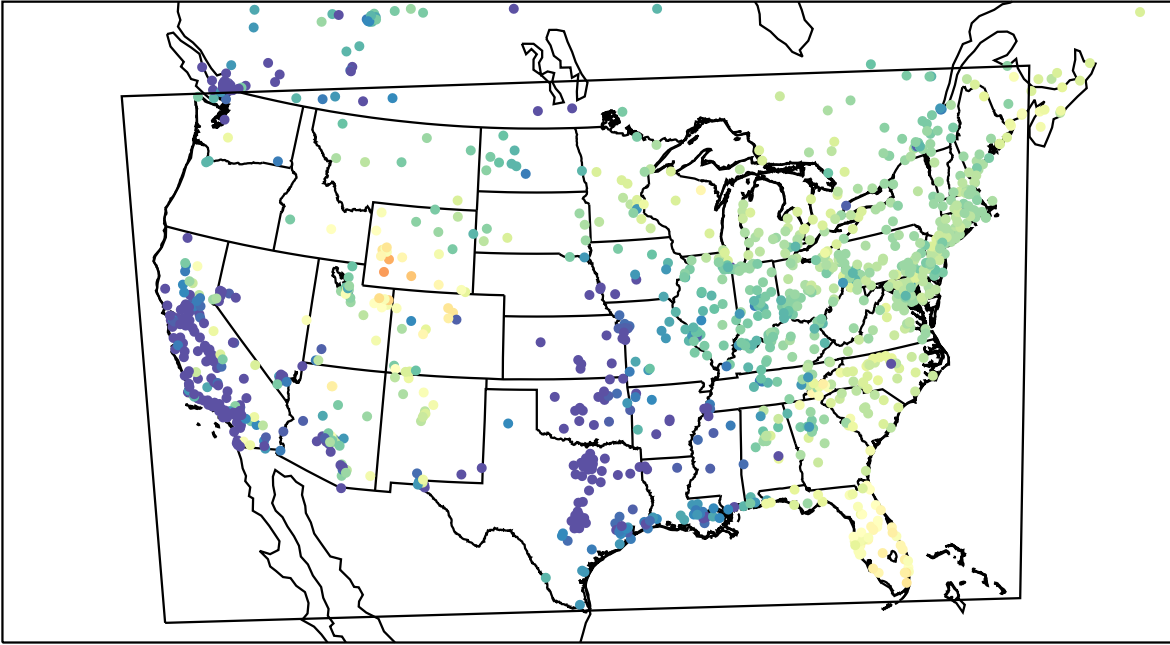
AirNOW (2023-03-09_15:00:00)
