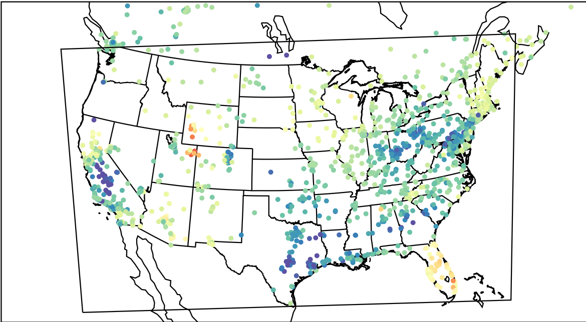
AirNOW (2023-03-10_18:00:00)
