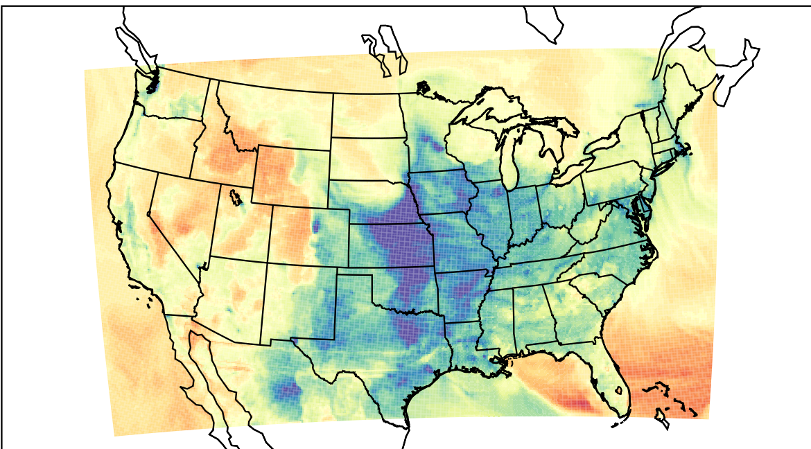
WRF (2023-03-09_02:00:00)
