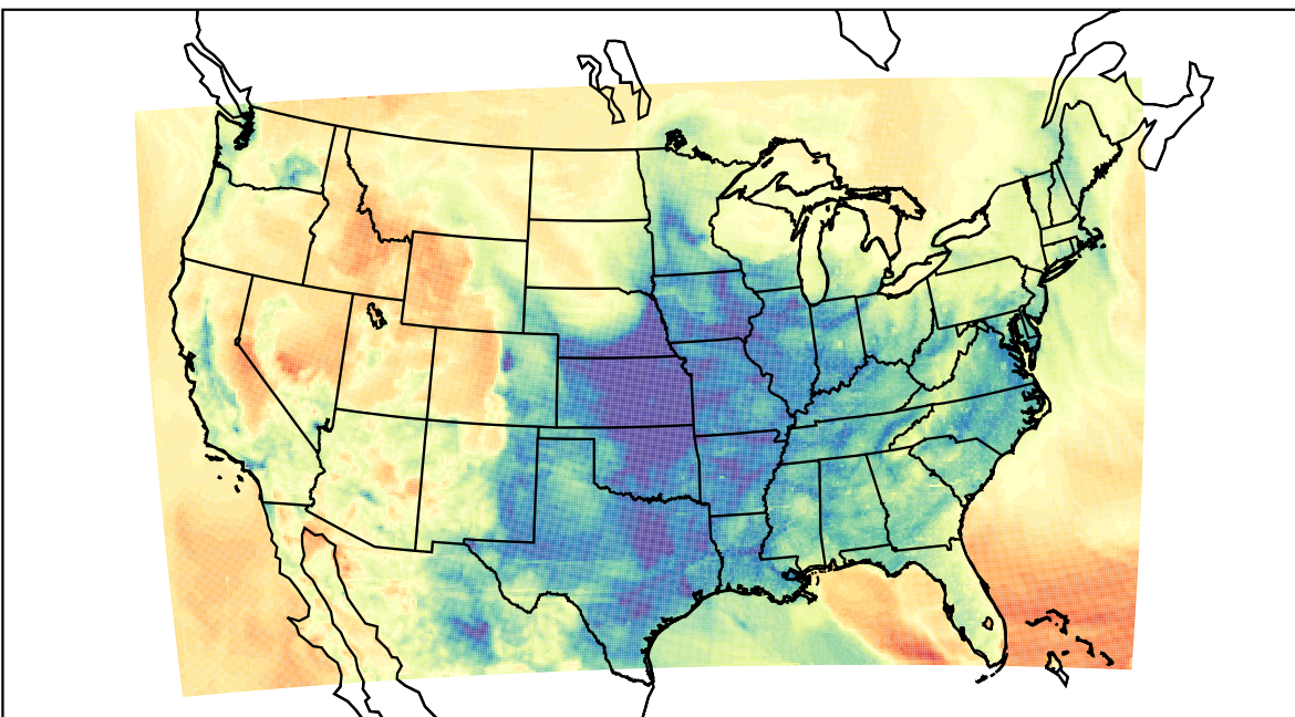
WRF (2023-03-09_05:00:00)
