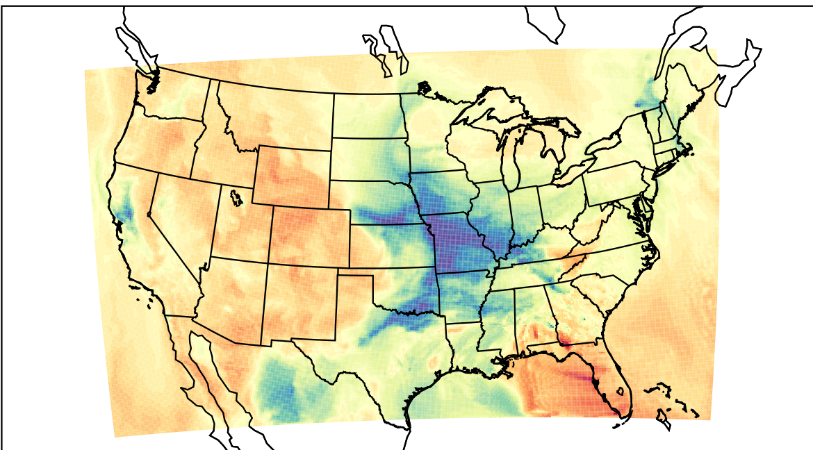
WRF (2023-03-09_21:00:00)
