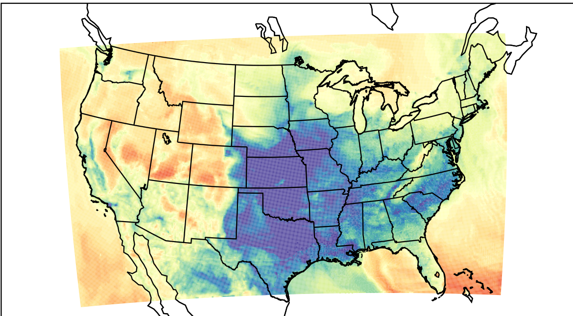
WRF (2023-03-09_12:00:00)
