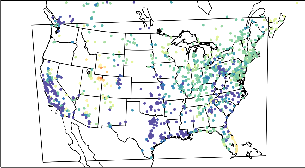
AirNOW (2023-03-09_09:00:00)
