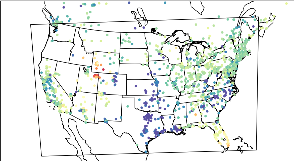
AirNOW (2023-03-09_02:00:00)
