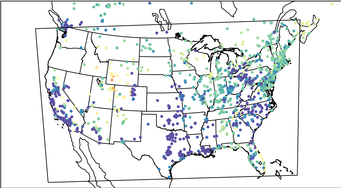
AirNOW (2023-03-09_11:00:00)
