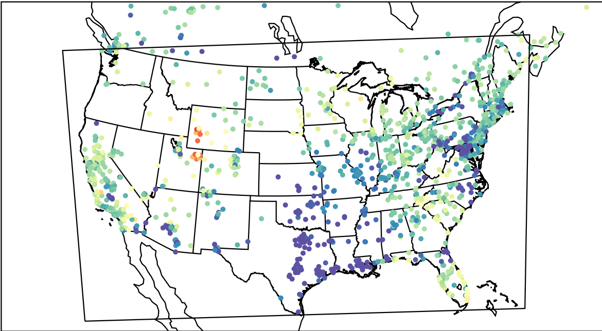
AirNOW (2023-03-10_04:00:00)
