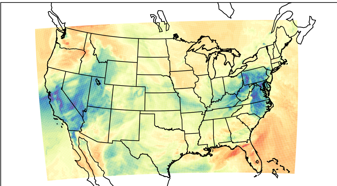
WRF (2023-03-10_22:00:00)
