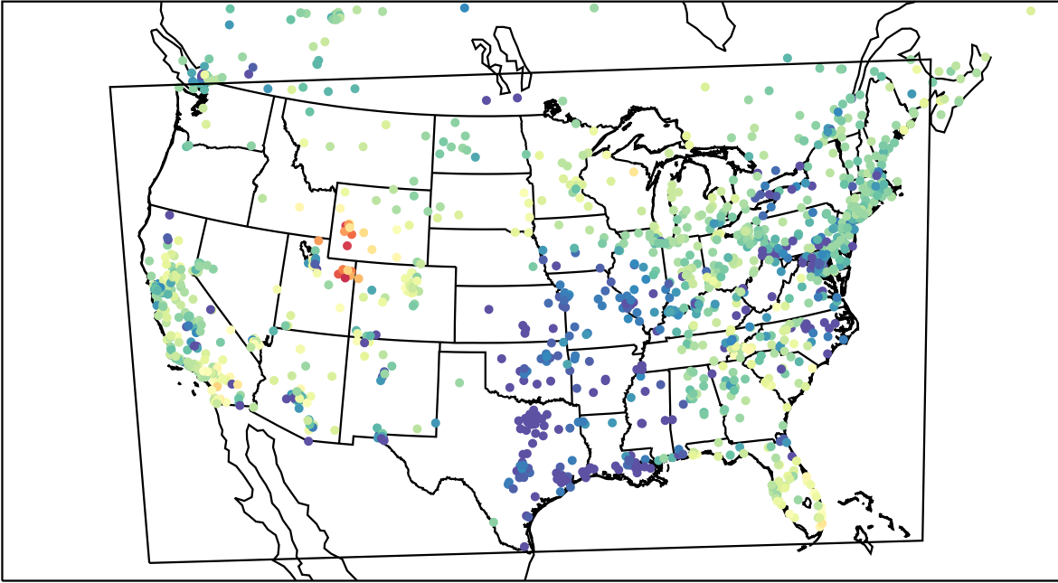
AirNOW (2023-03-10_02:00:00)
