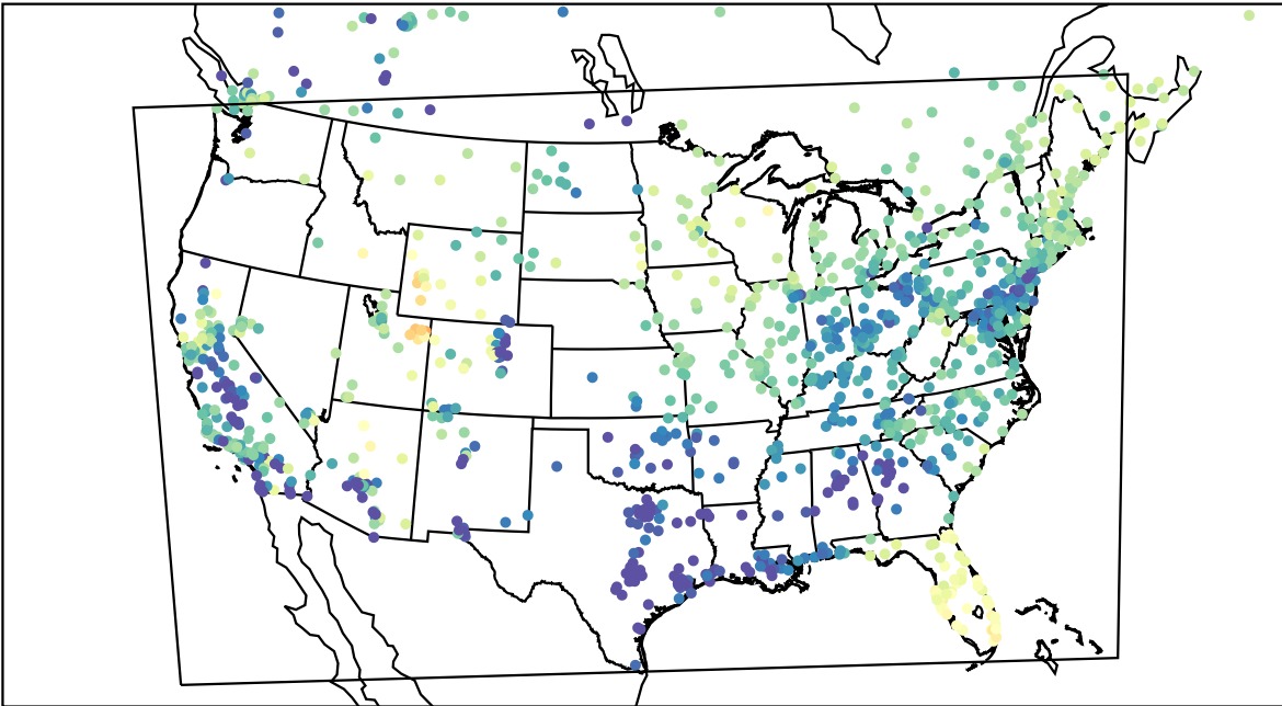
AirNOW (2023-03-10_15:00:00)
