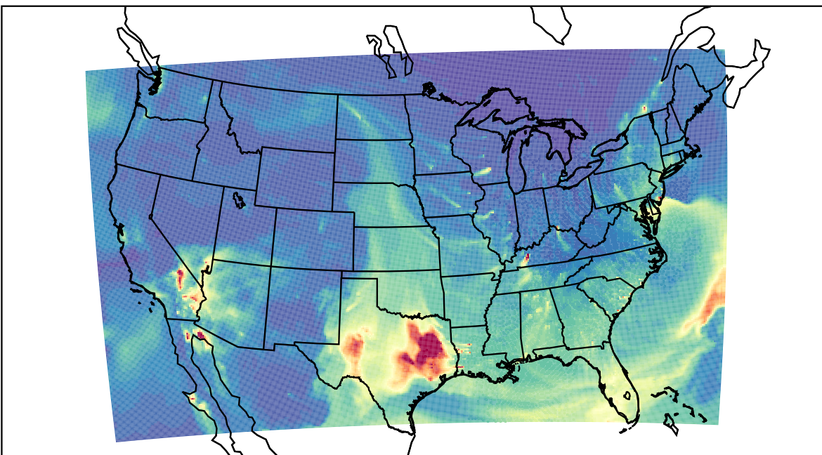
WRF 2023-03-11_12:00:00
