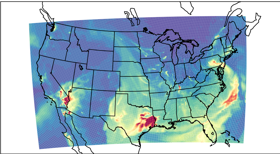
WRF 2023-03-11_07:00:00
