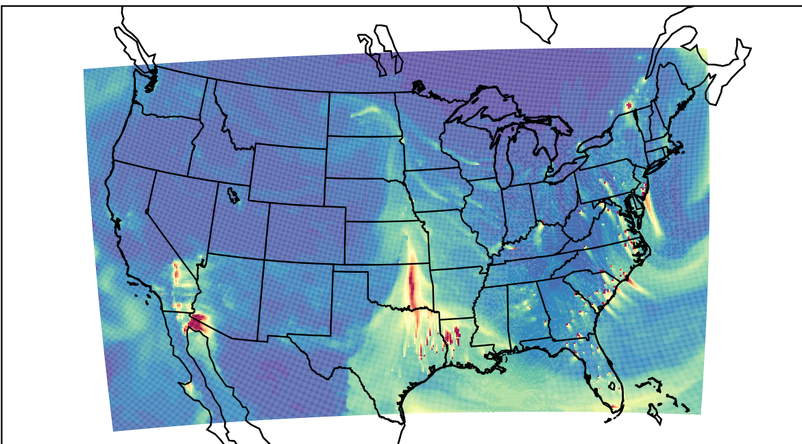
WRF 2023-03-11_22:00:00
