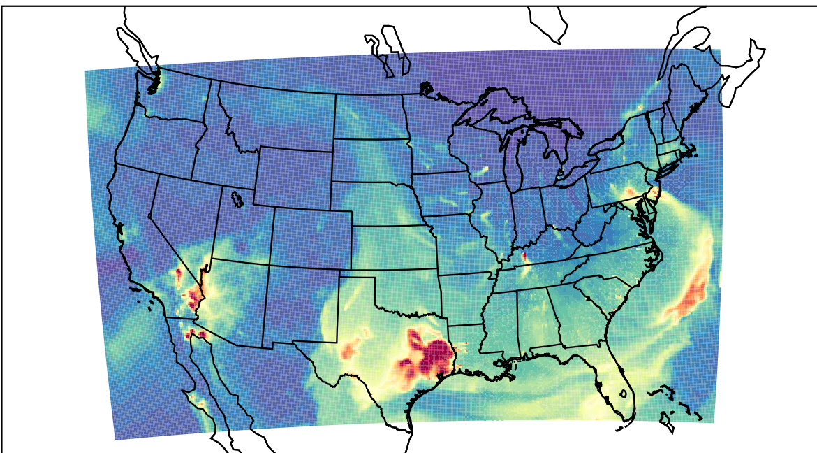
WRF 2023-03-11_09:00:00
