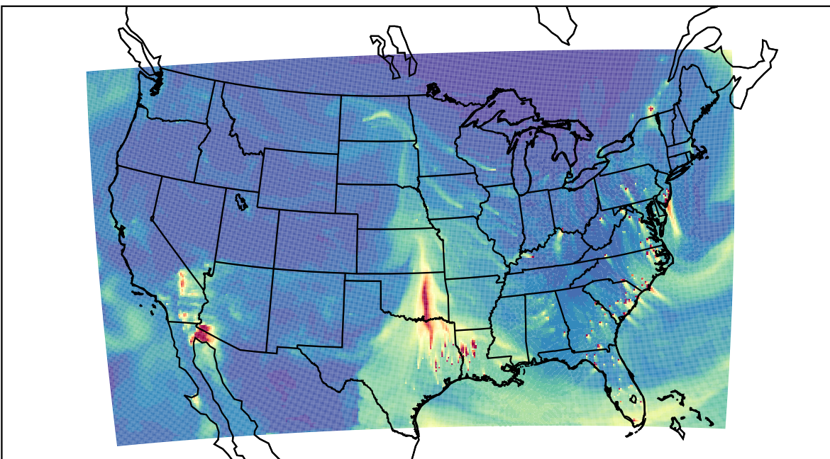
WRF 2023-03-11_21:00:00
