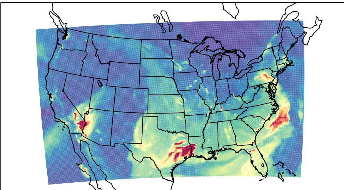
WRF 2023-03-11_05:00:00
