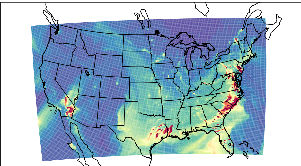
WRF 2023-03-11_00:00:00
