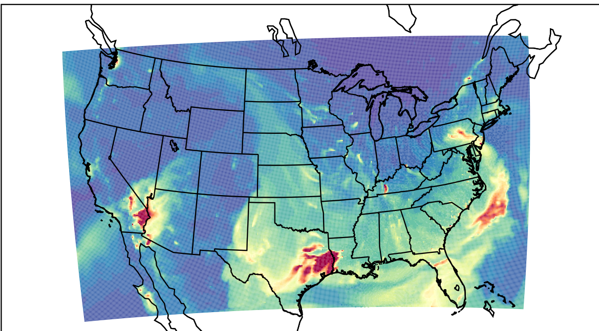
WRF 2023-03-11_06:00:00
