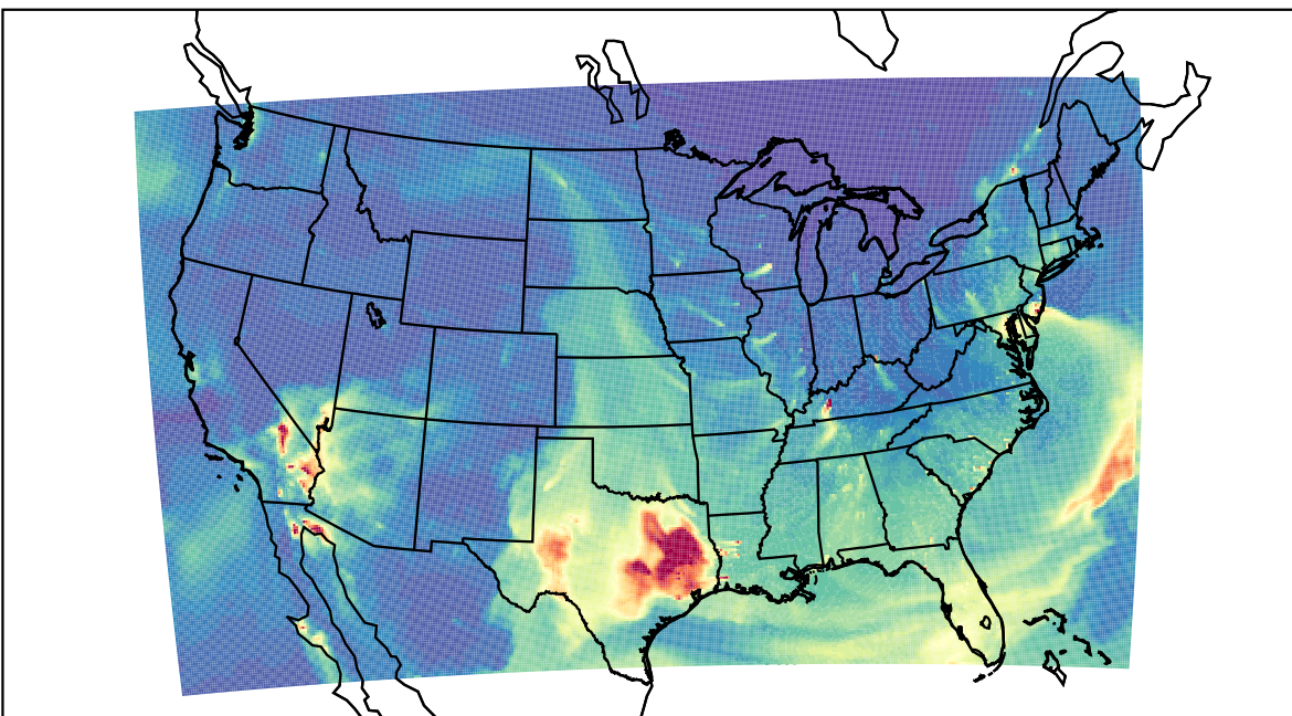
WRF 2023-03-11_11:00:00
