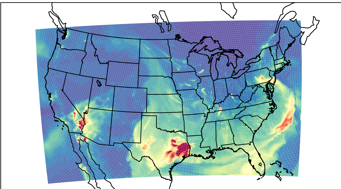
WRF 2023-03-11_08:00:00
