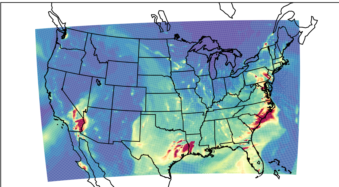
WRF 2023-03-11_02:00:00
