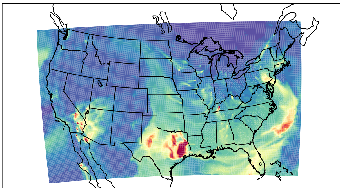
WRF 2023-03-11_09:00:00
