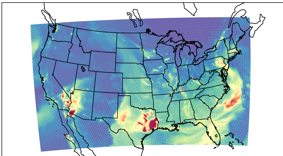
WRF 2023-03-11_07:00:00
