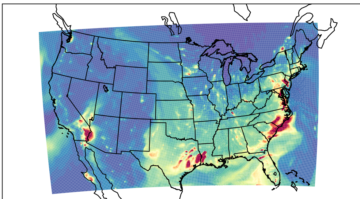
WRF 2023-03-11_02:00:00
