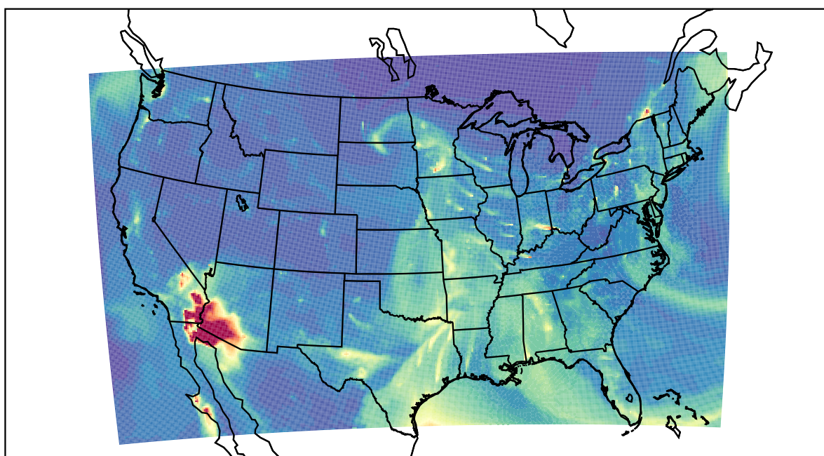
WRF 2023-03-12_06:00:00
