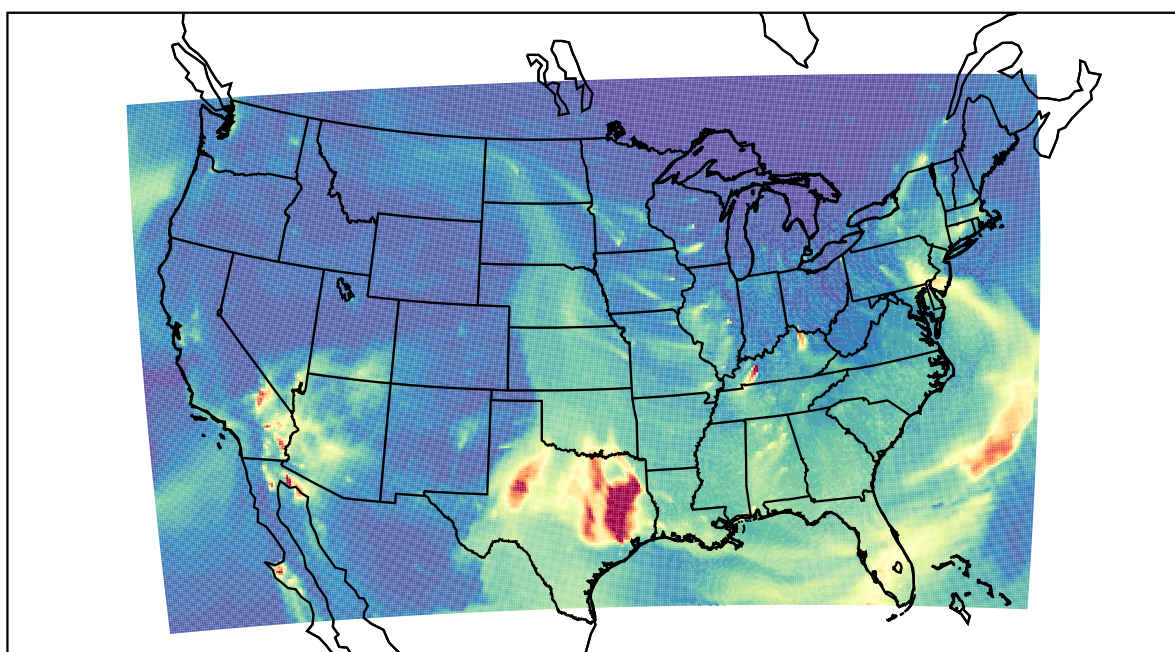
WRF 2023-03-11_11:00:00
