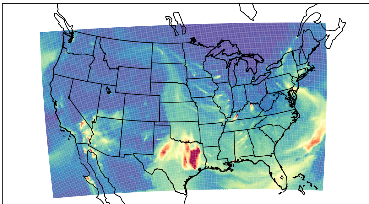
WRF 2023-03-11_12:00:00
