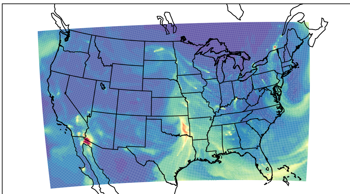
WRF 2023-03-11_21:00:00
