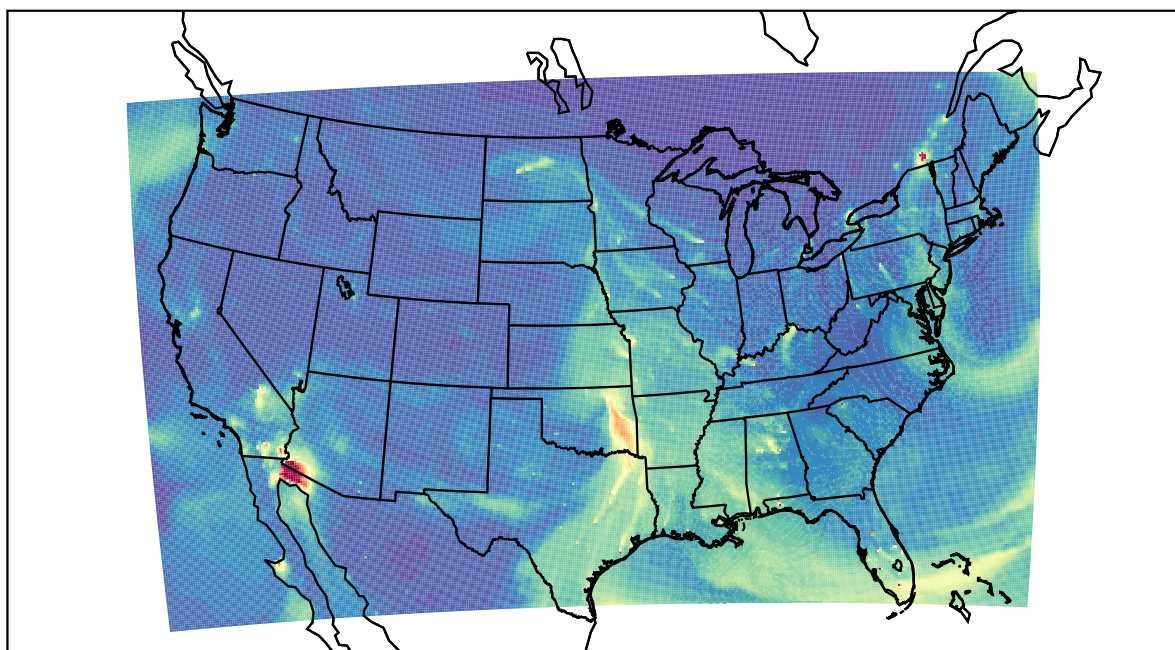
WRF 2023-03-11_22:00:00
