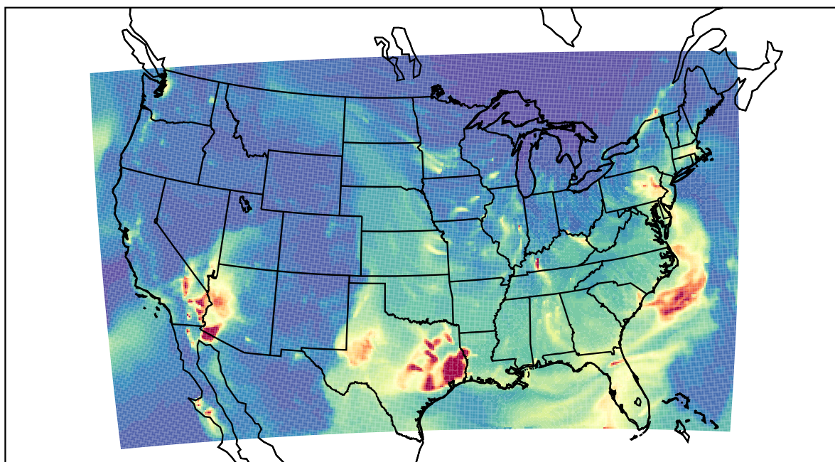
WRF 2023-03-11_06:00:00
