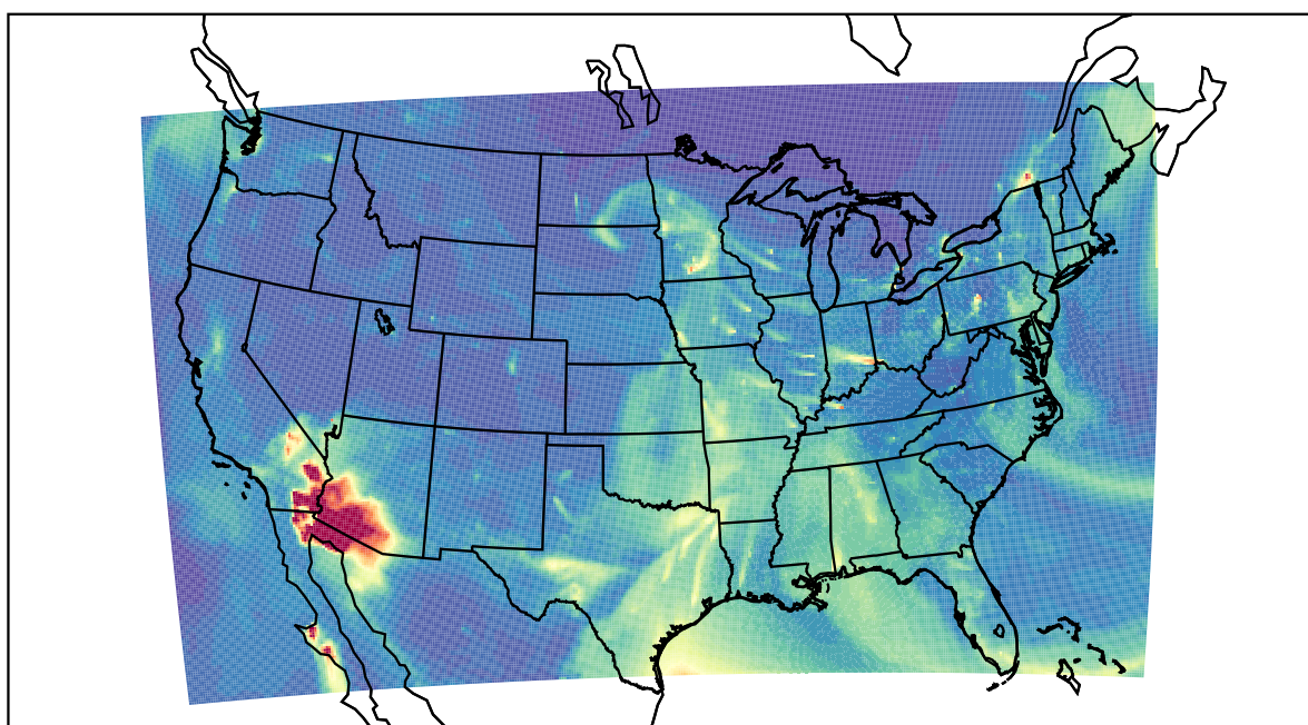
WRF 2023-03-12_07:00:00
