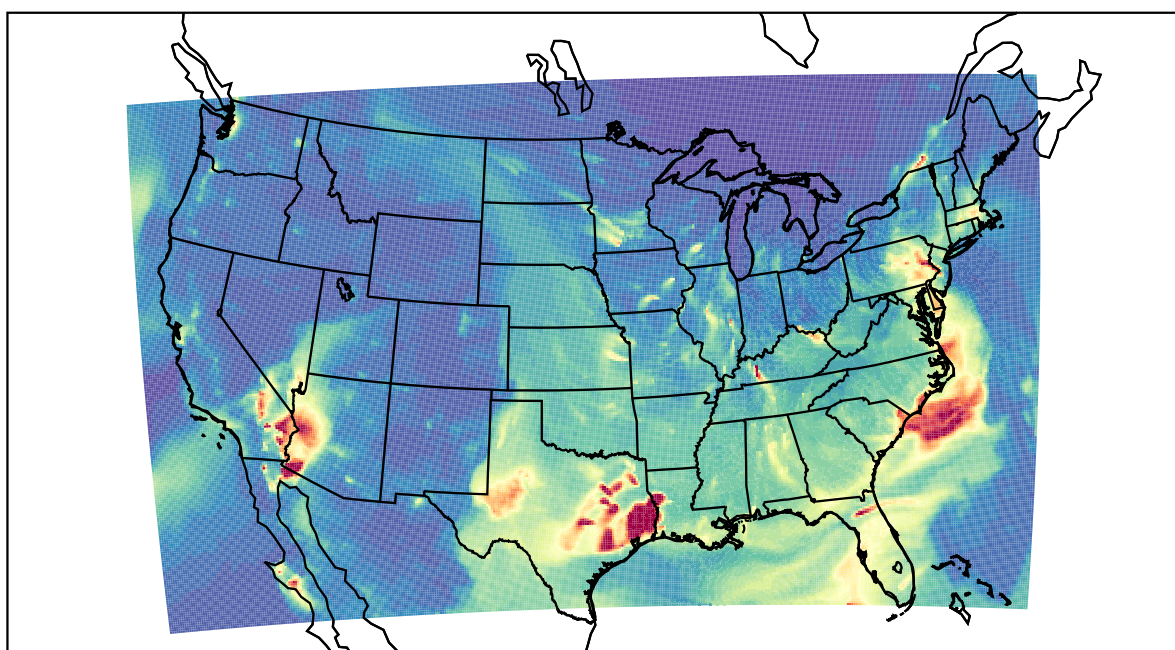
WRF 2023-03-11_05:00:00
