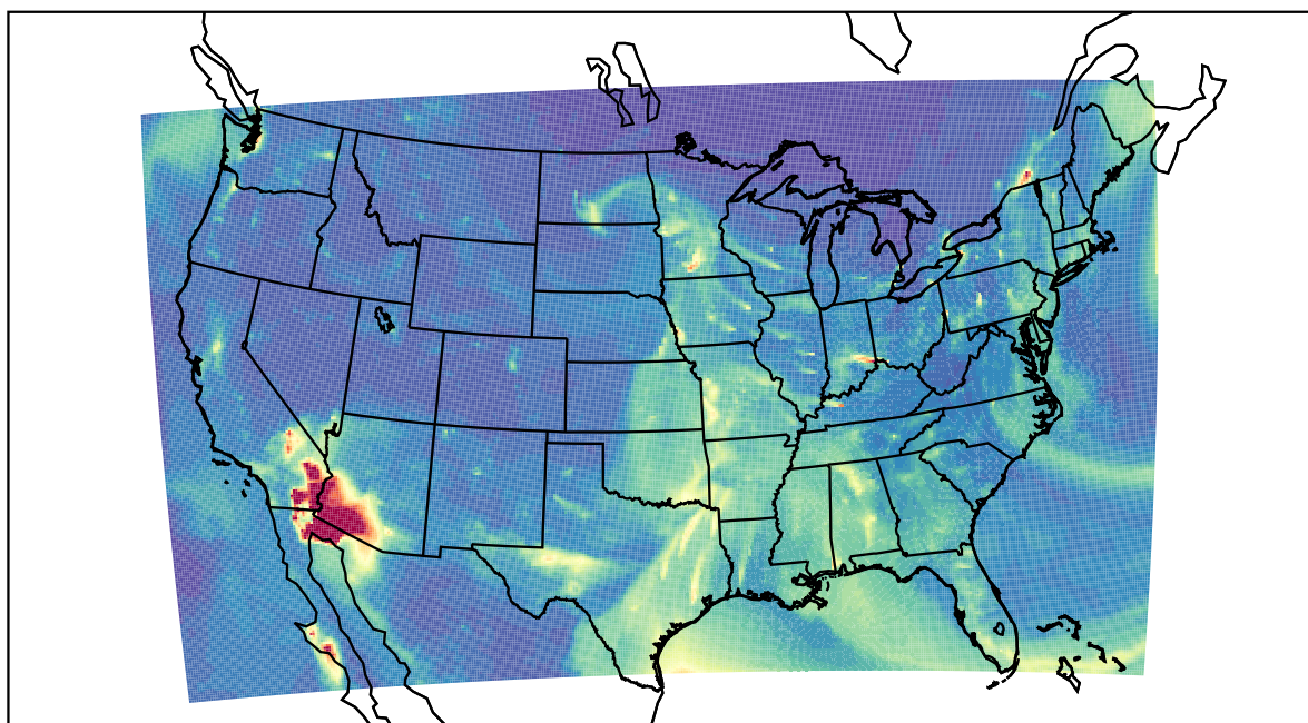
WRF 2023-03-12_05:00:00
