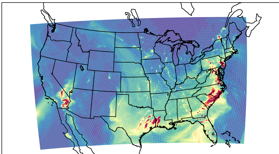
WRF 2023-03-11_00:00:00
