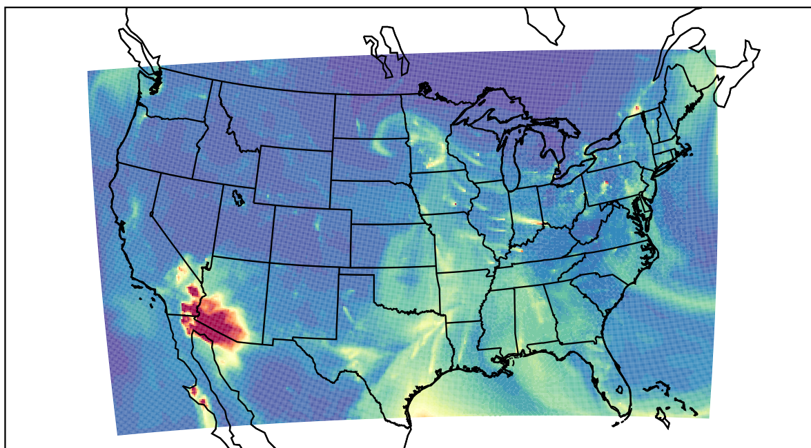
WRF 2023-03-12_08:00:00
