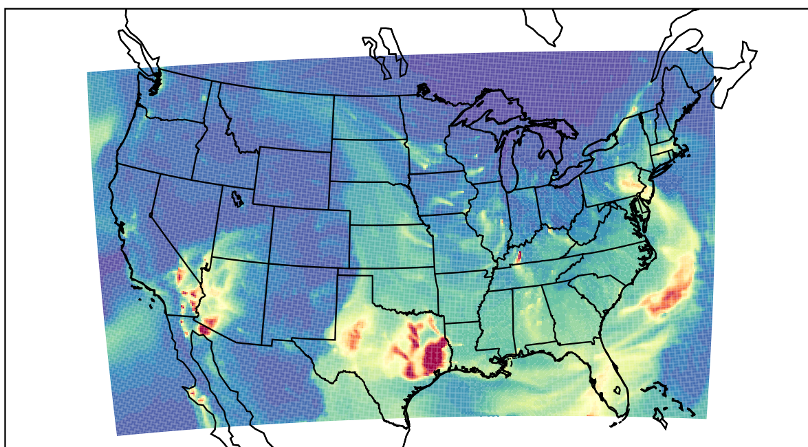
WRF 2023-03-11_08:00:00
