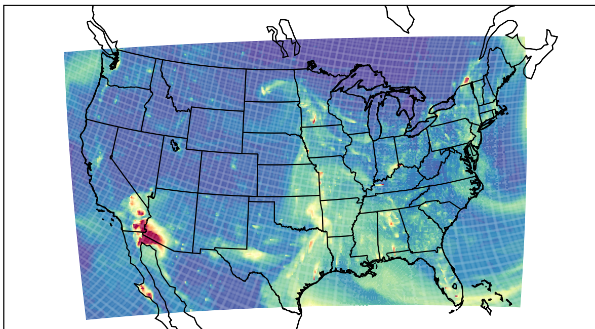
WRF 2023-03-12_02:00:00
