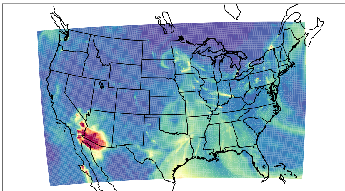
WRF 2023-03-12_09:00:00
