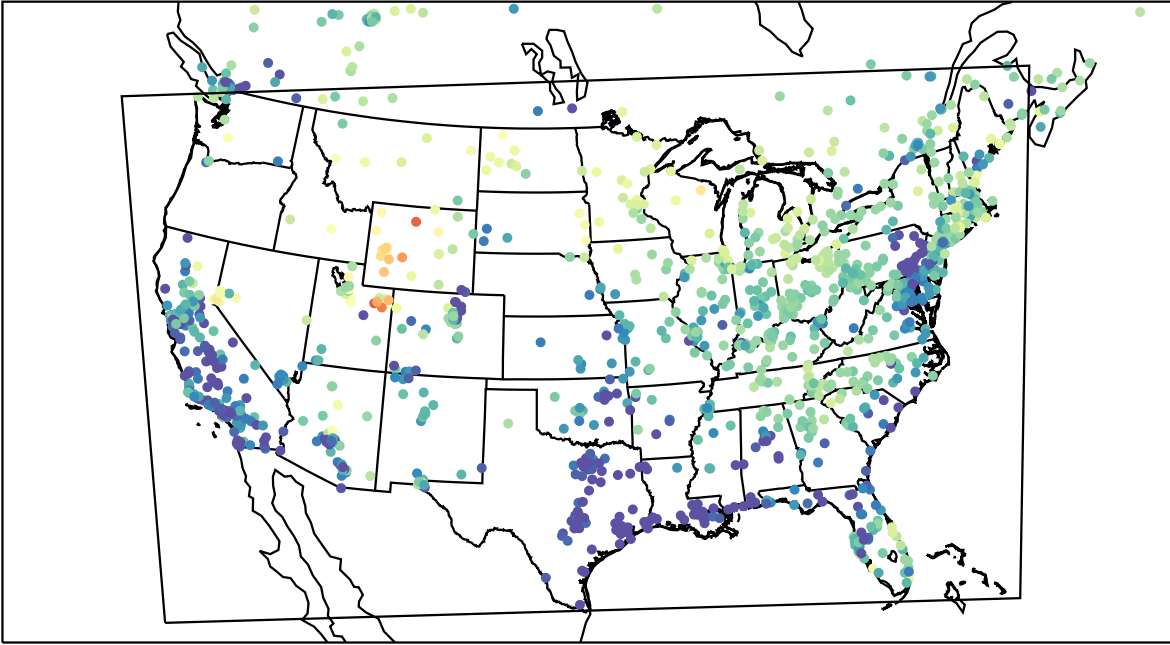
AirNOW (2023-03-11_04:00:00)
