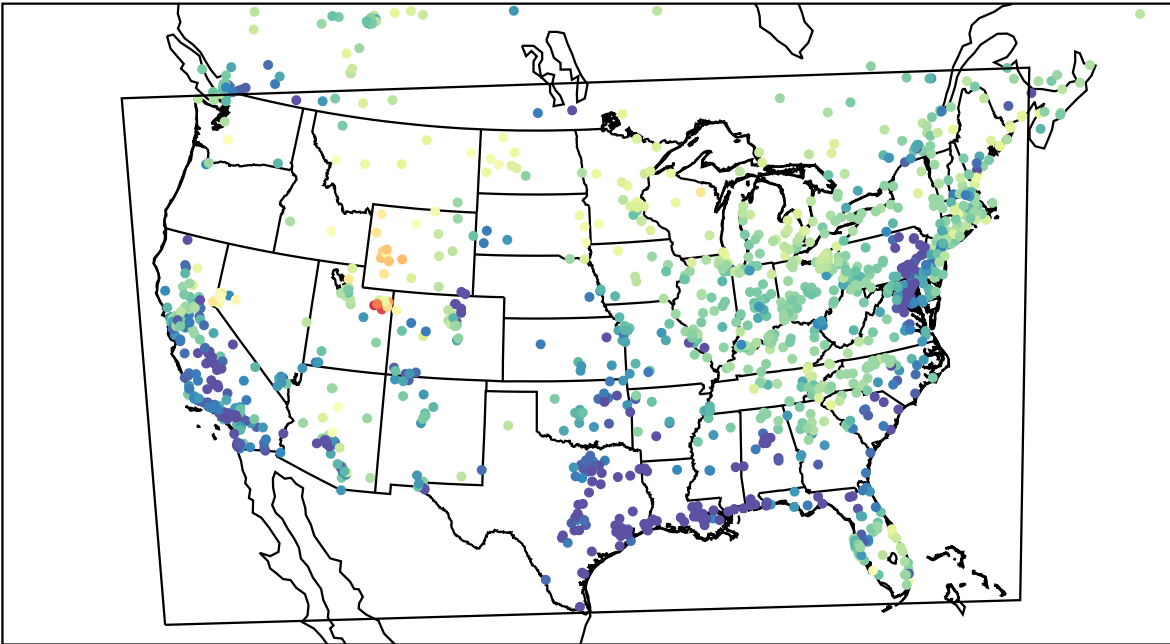
AirNOW (2023-03-11_03:00:00)
