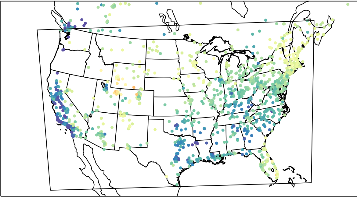
AirNOW (2023-03-12_17:00:00)
