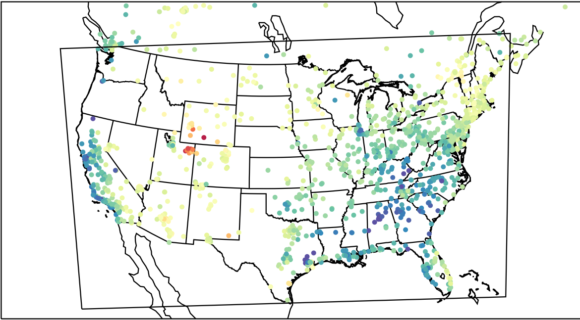
AirNOW (2023-03-12_21:00:00)
