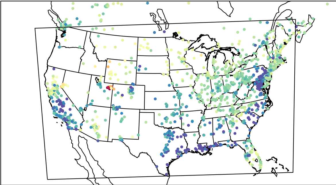
AirNOW (2023-03-11_01:00:00)
