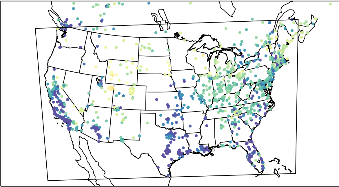
AirNOW (2023-03-12_06:00:00)
