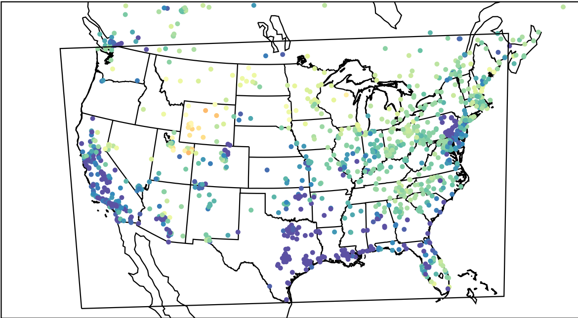
AirNOW (2023-03-11_05:00:00)
