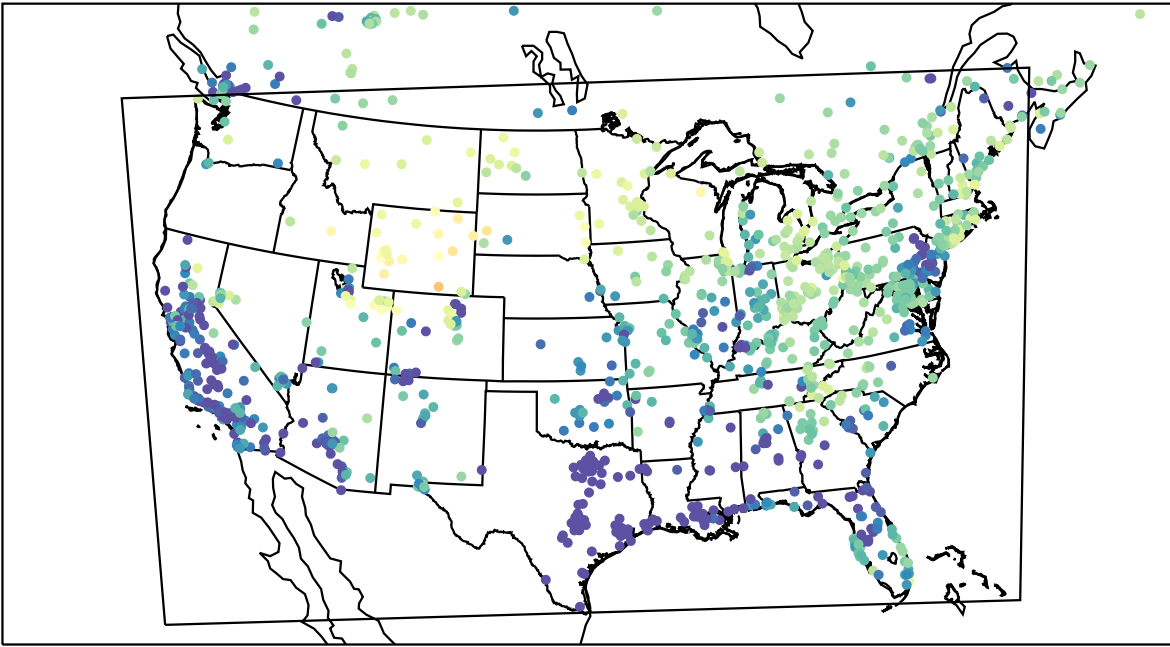
AirNOW (2023-03-11_08:00:00)
