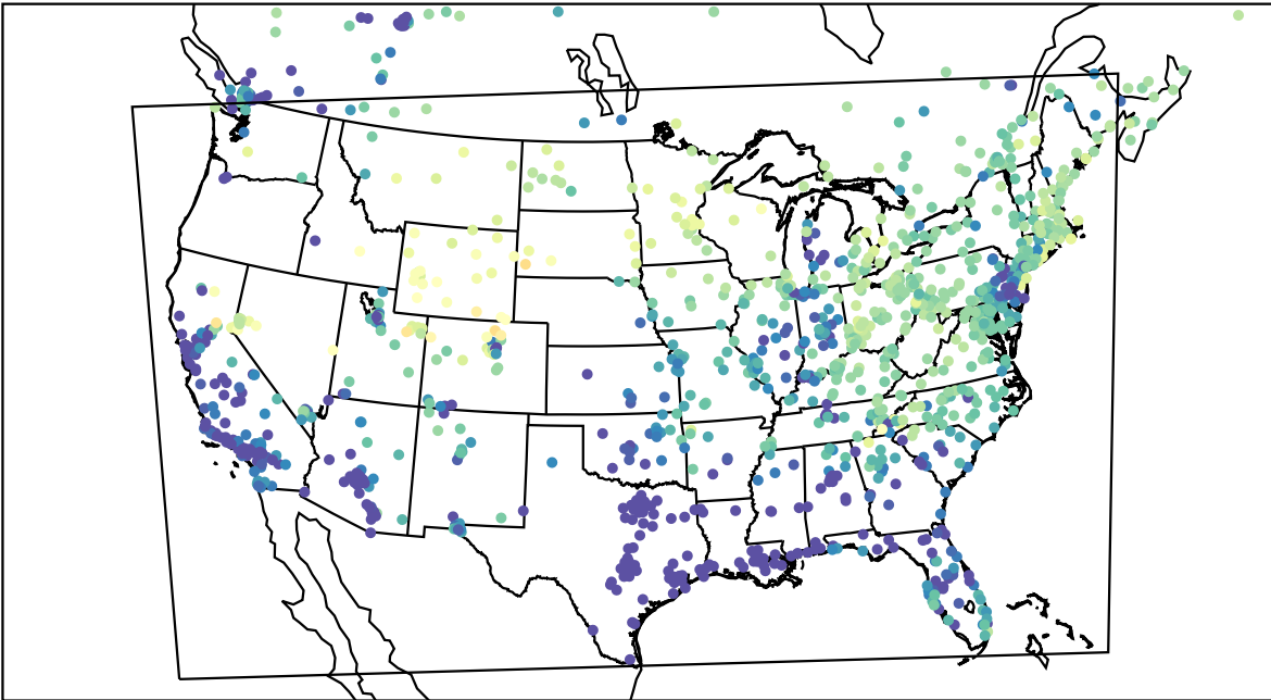
AirNOW (2023-03-11_12:00:00)
