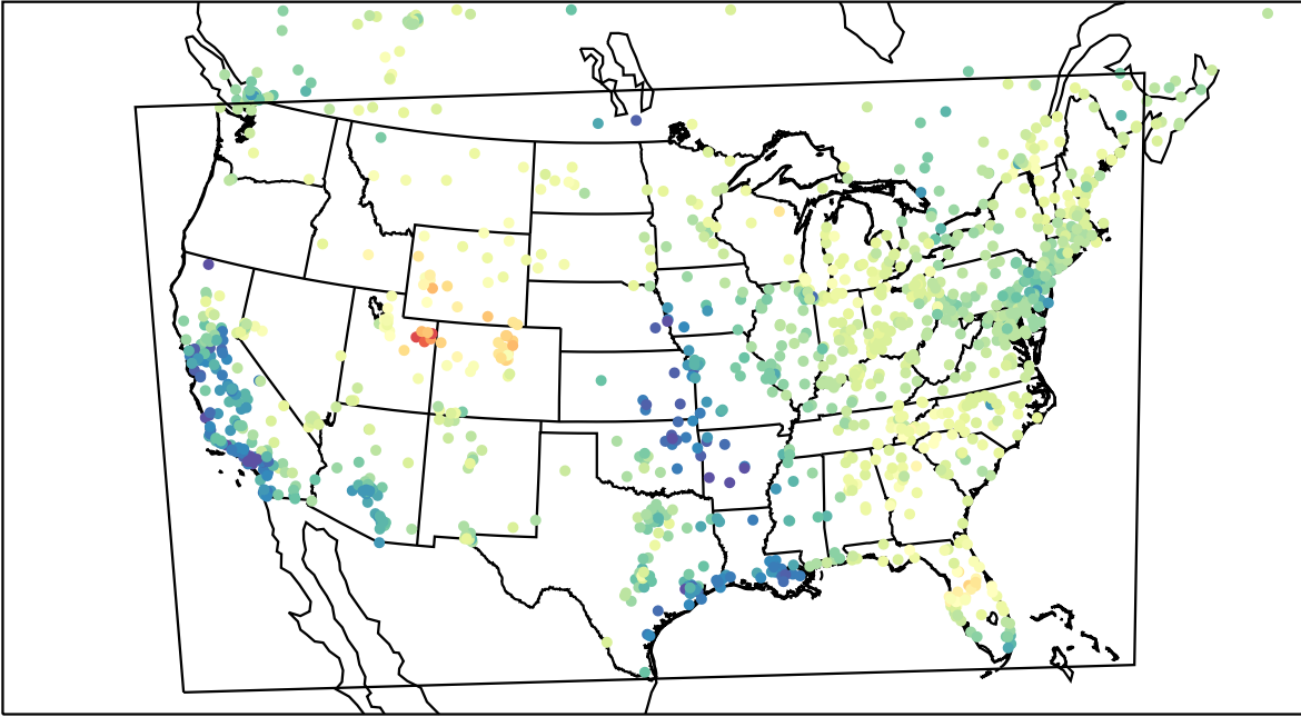
AirNOW (2023-03-11_22:00:00)
