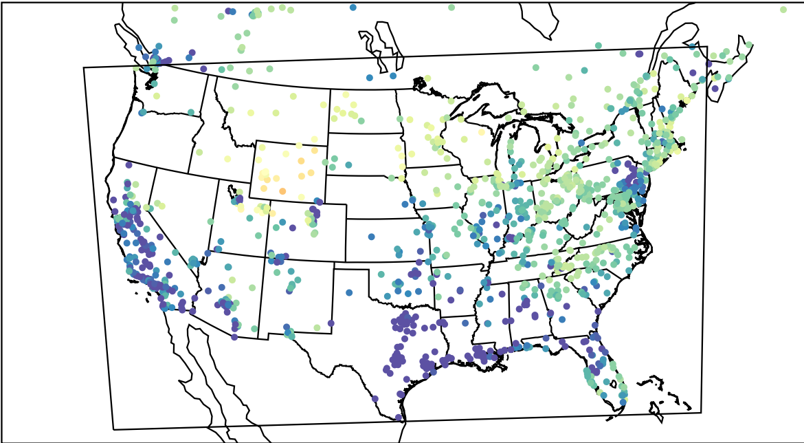
AirNOW (2023-03-11_07:00:00)
