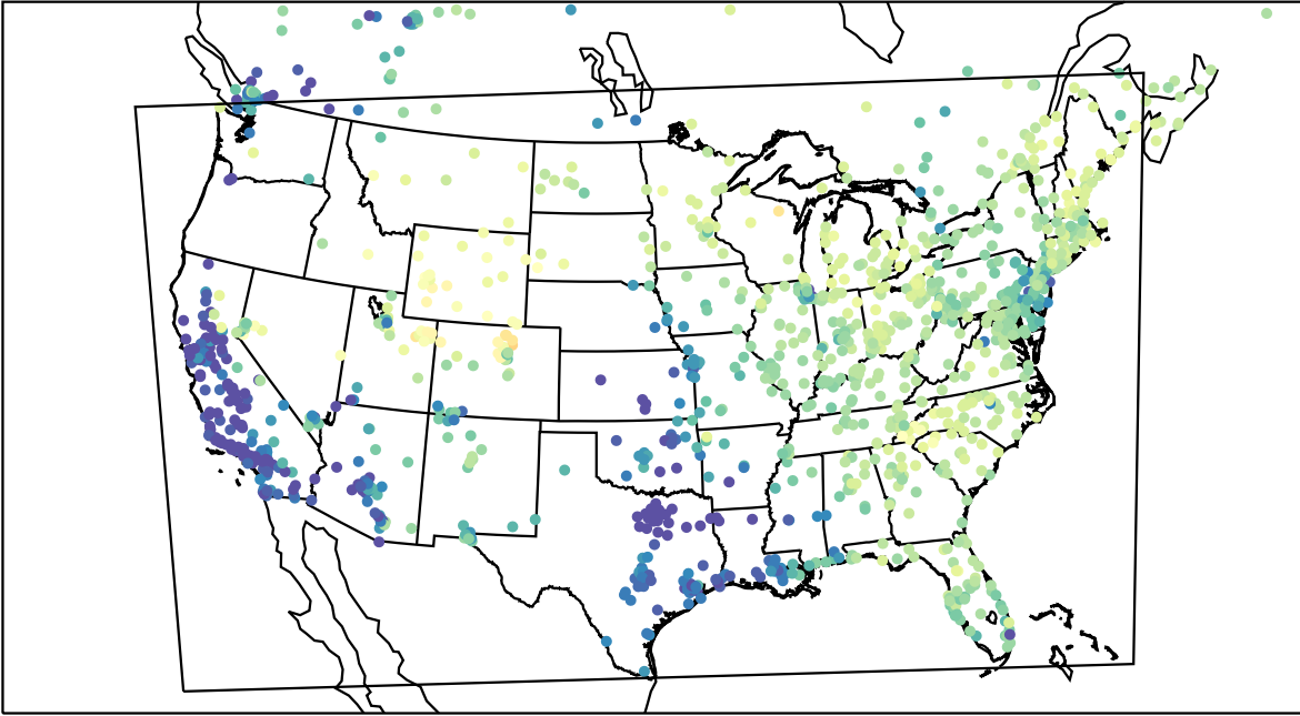
AirNOW (2023-03-11_16:00:00)
