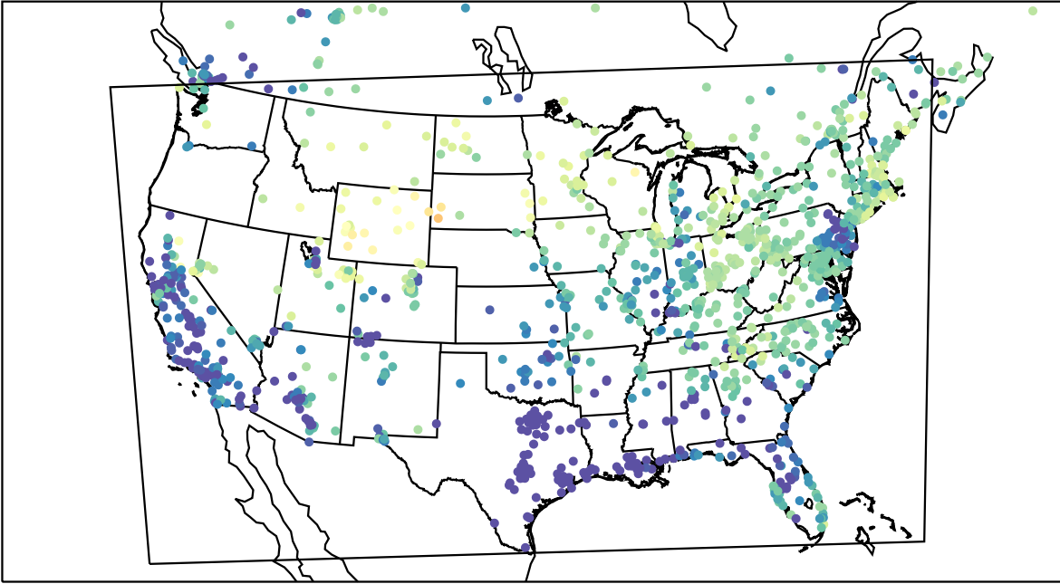
AirNOW (2023-03-11_09:00:00)
