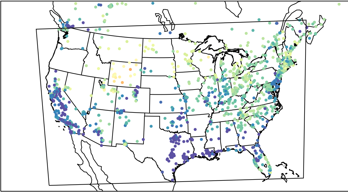
AirNOW (2023-03-11_06:00:00)
