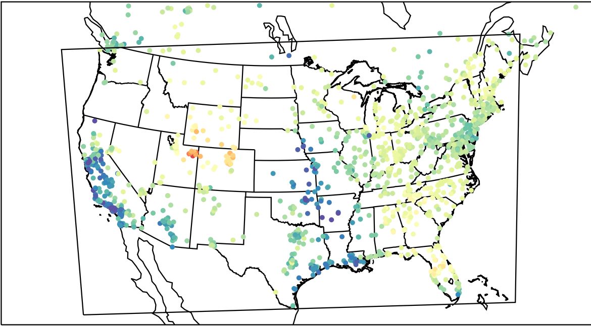
AirNOW (2023-03-11_21:00:00)
