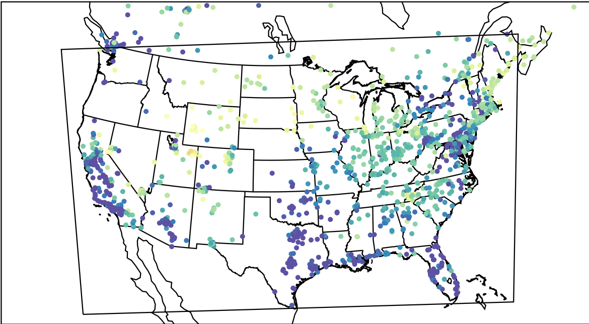
AirNOW (2023-03-12_09:00:00)
