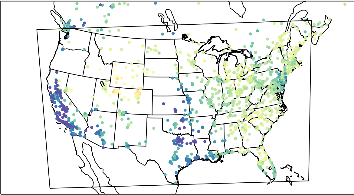
AirNOW (2023-03-11_17:00:00)
