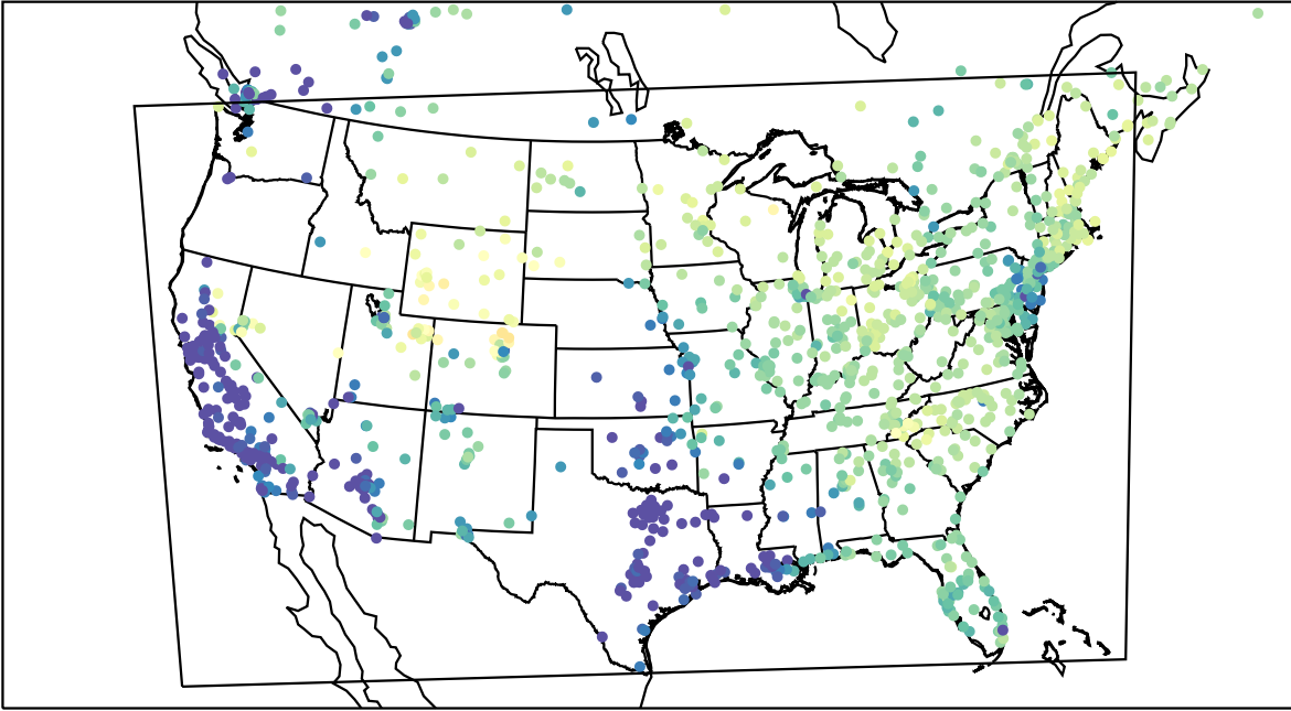
AirNOW (2023-03-11_15:00:00)
