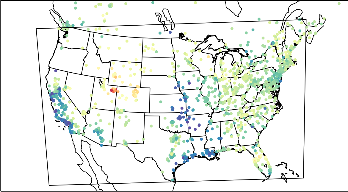
AirNOW (2023-03-11_23:00:00)
