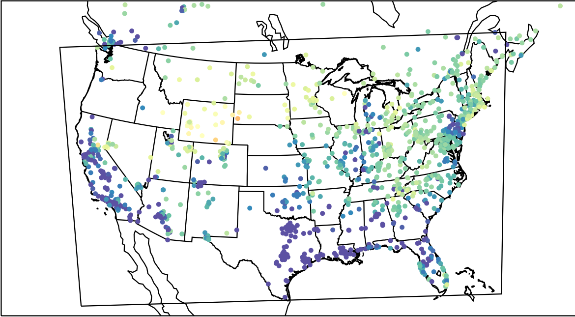
AirNOW (2023-03-11_10:00:00)
