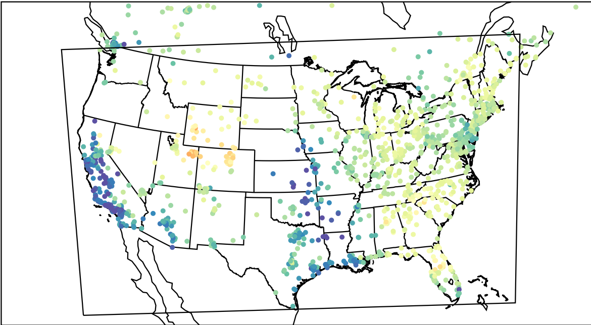
AirNOW (2023-03-11_19:00:00)
