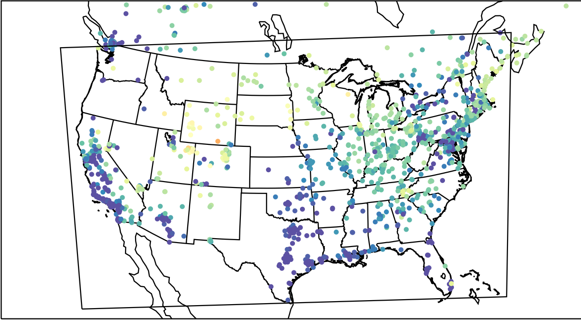
AirNOW (2023-03-12_08:00:00)
