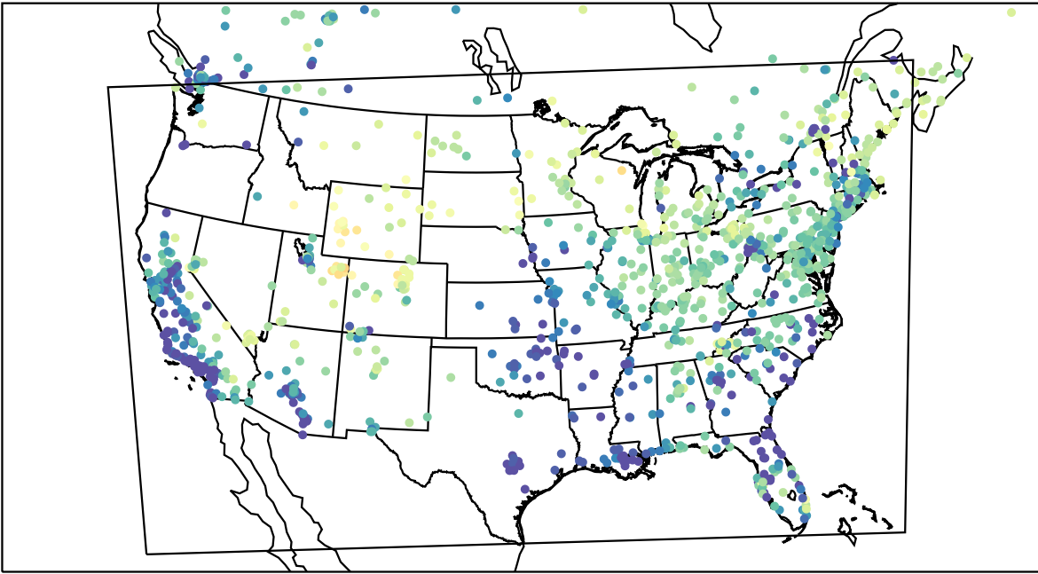
AirNOW (2023-03-12_04:00:00)
