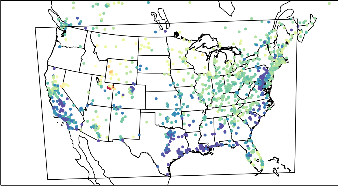
AirNOW (2023-03-11_02:00:00)
