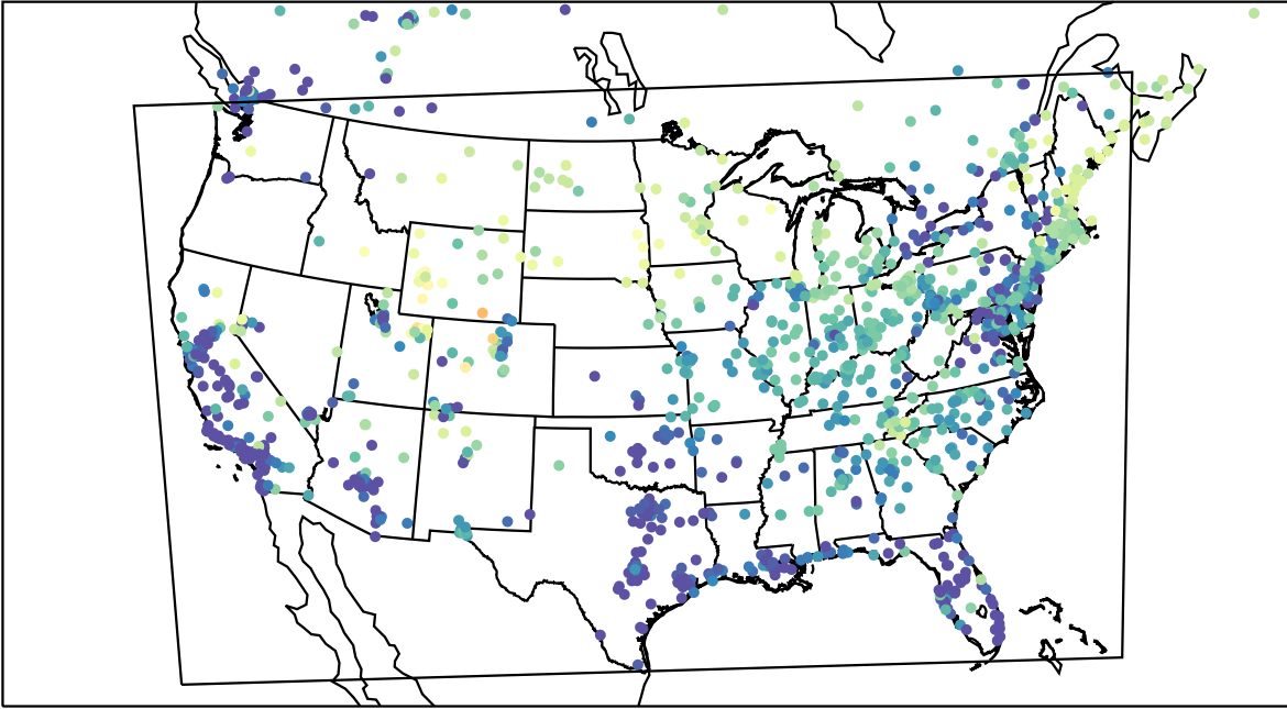
AirNOW (2023-03-12_12:00:00)
