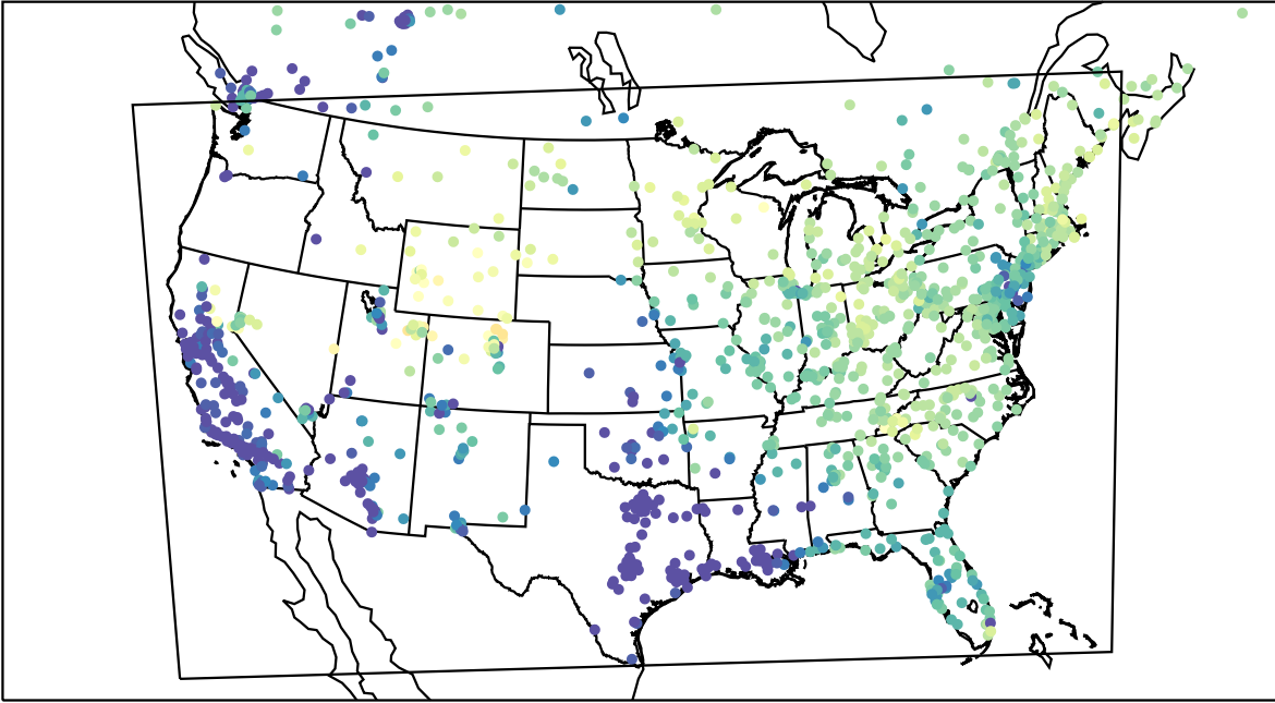
AirNOW (2023-03-11_14:00:00)
