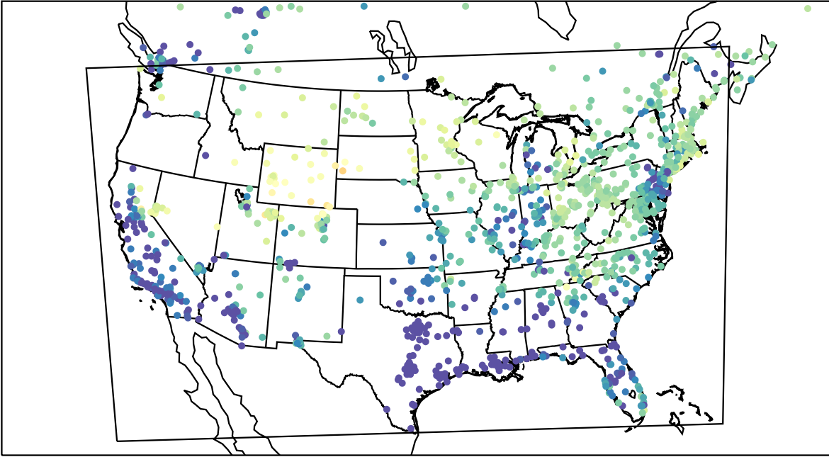
AirNOW (2023-03-11_11:00:00)
