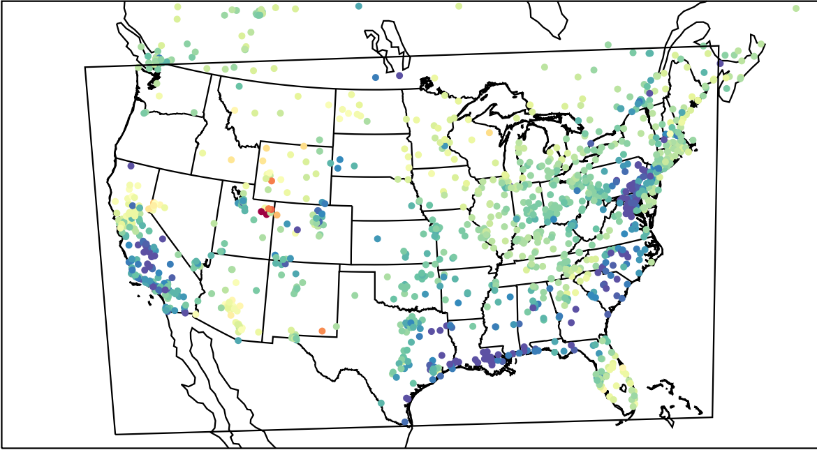
AirNOW (2023-03-11_00:00:00)
