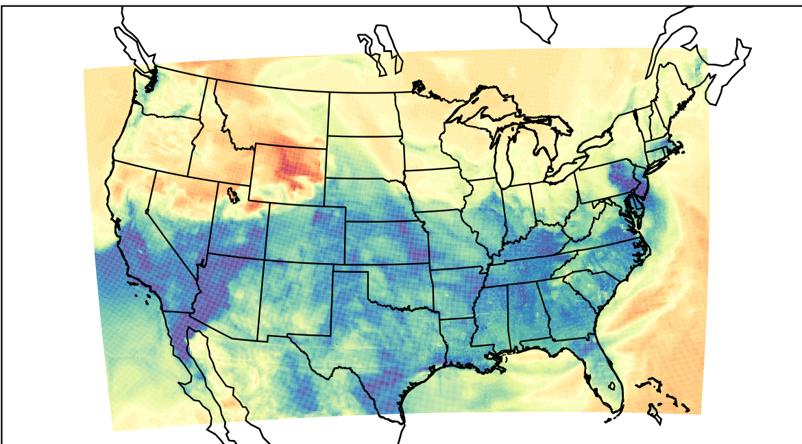
WRF (2023-03-11_07:00:00)
