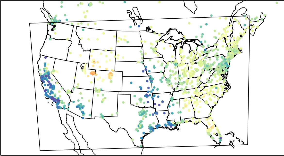
AirNOW (2023-03-11_20:00:00)
