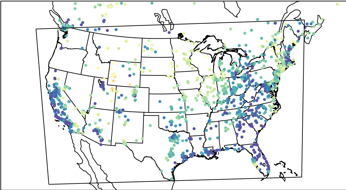
AirNOW (2023-03-13_06:00:00)
