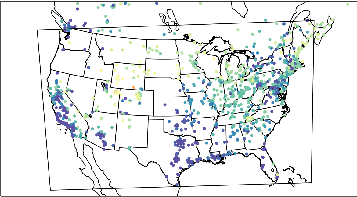
AirNOW (2023-03-12_08:00:00)
