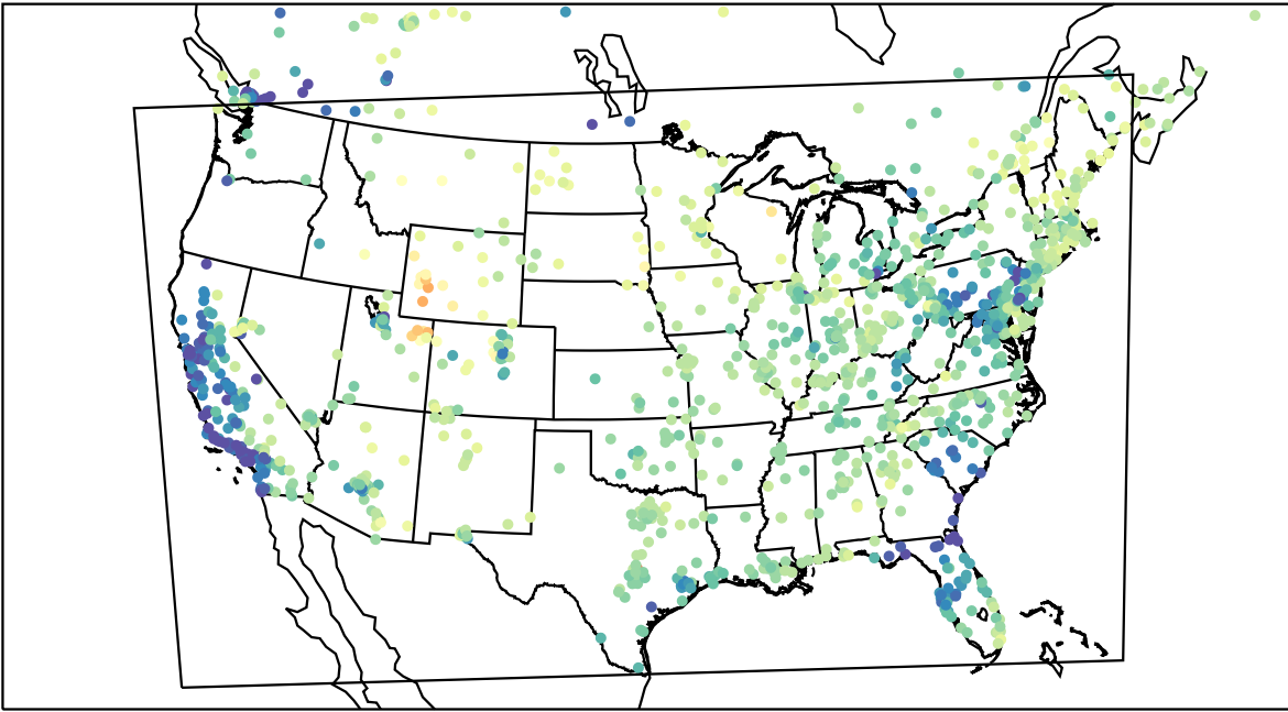
AirNOW (2023-03-13_17:00:00)
