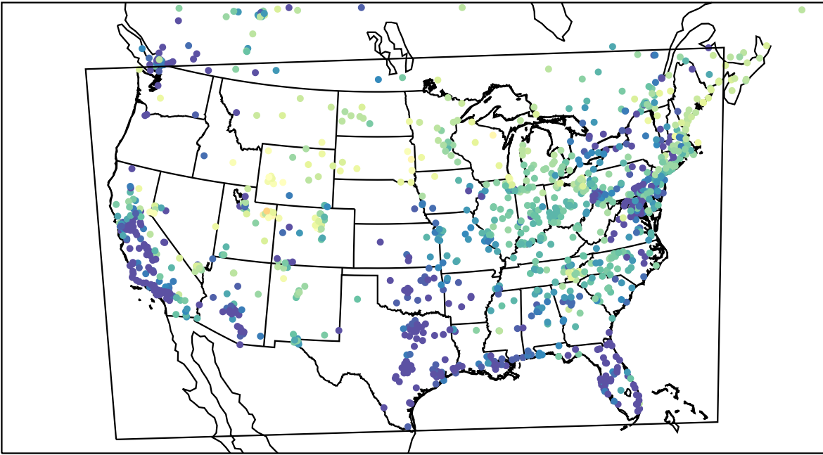
AirNOW (2023-03-12_09:00:00)
