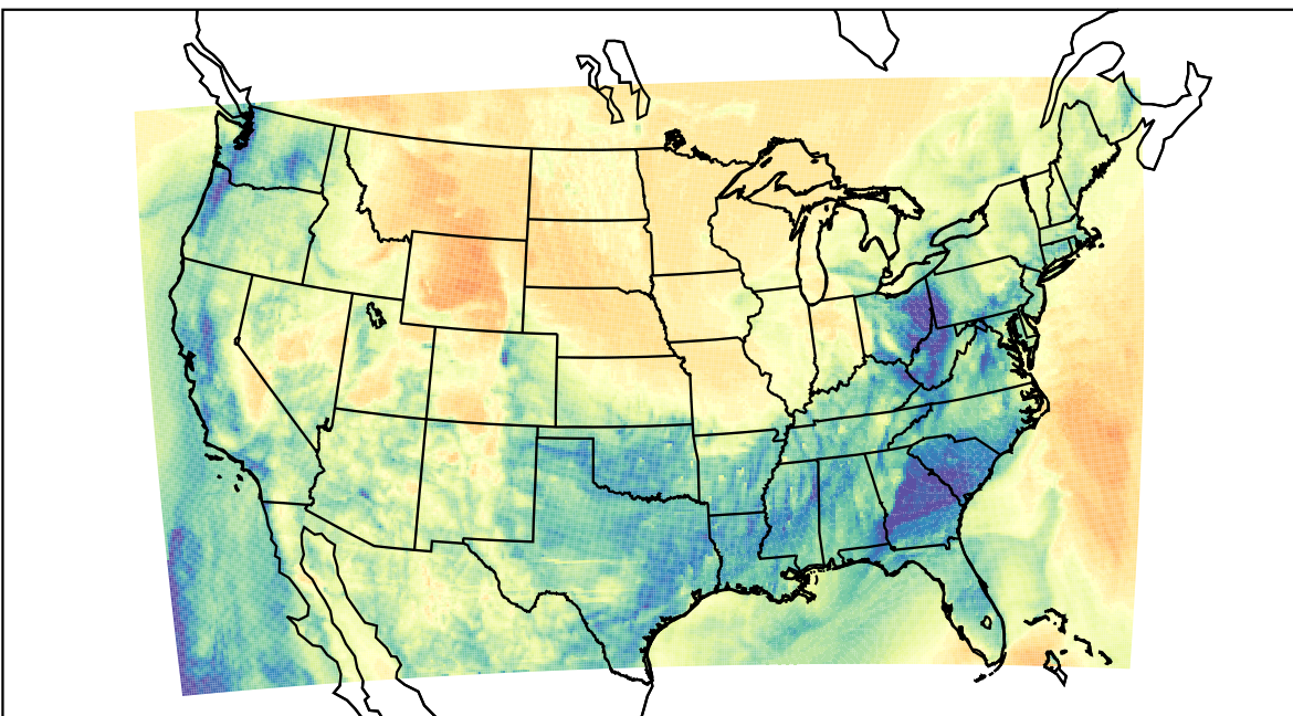
WRF (2023-03-13_09:00:00)
