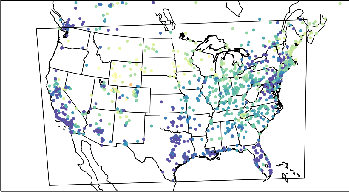
AirNOW (2023-03-12_11:00:00)
