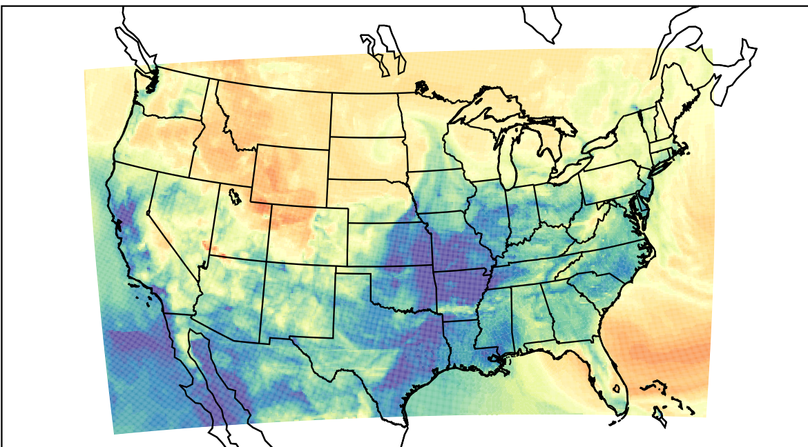
WRF (2023-03-12_07:00:00)
