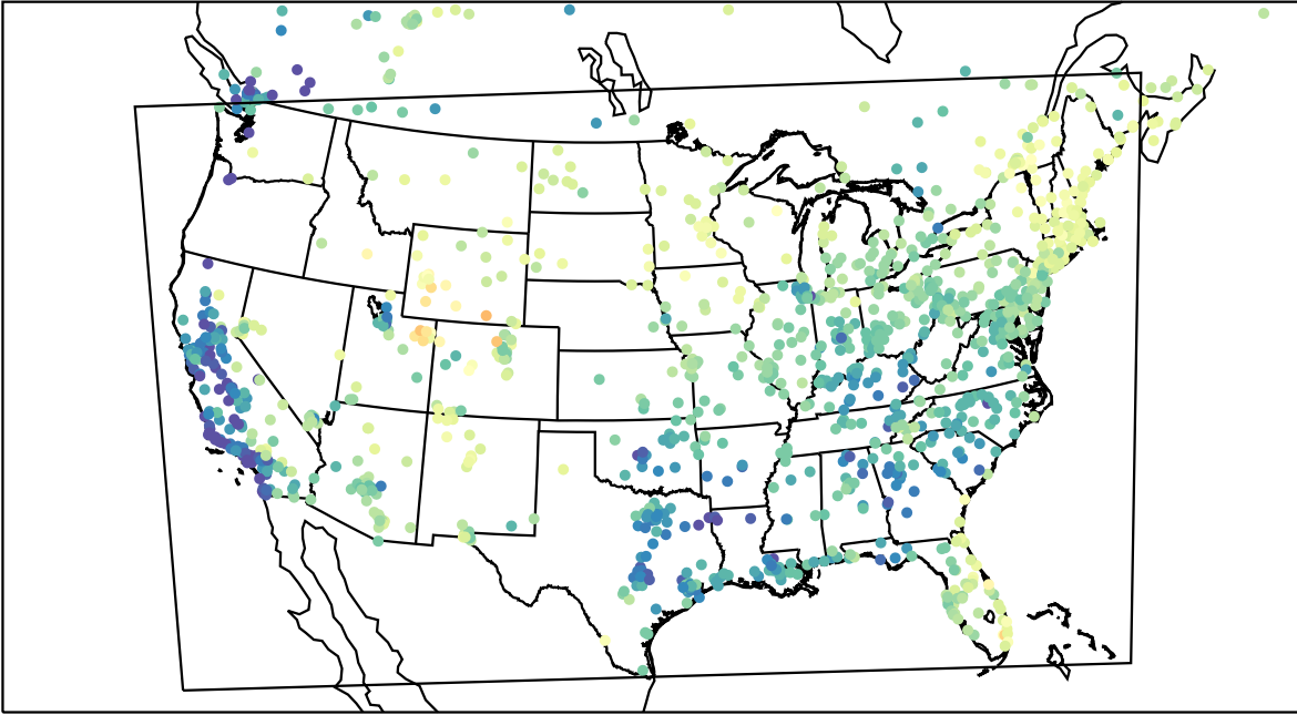
AirNOW (2023-03-12_17:00:00)
