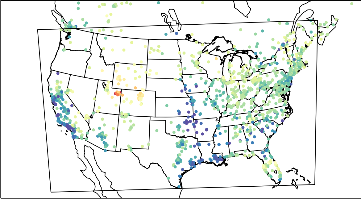
AirNOW (2023-03-12_00:00:00)
