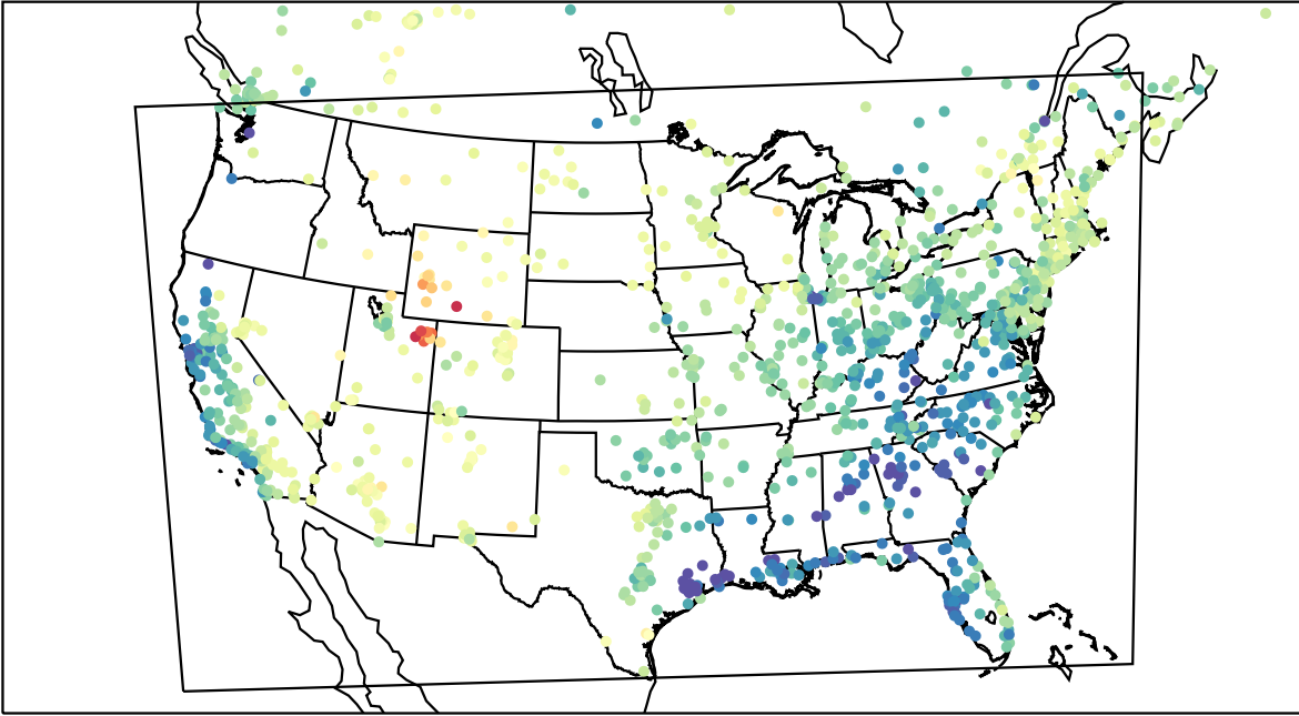
AirNOW (2023-03-12_23:00:00)
