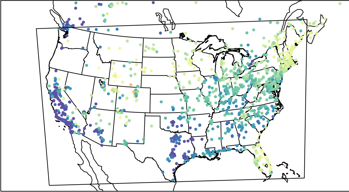
AirNOW (2023-03-12_15:00:00)
