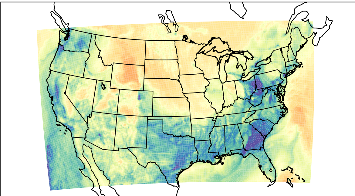
WRF (2023-03-13_12:00:00)
