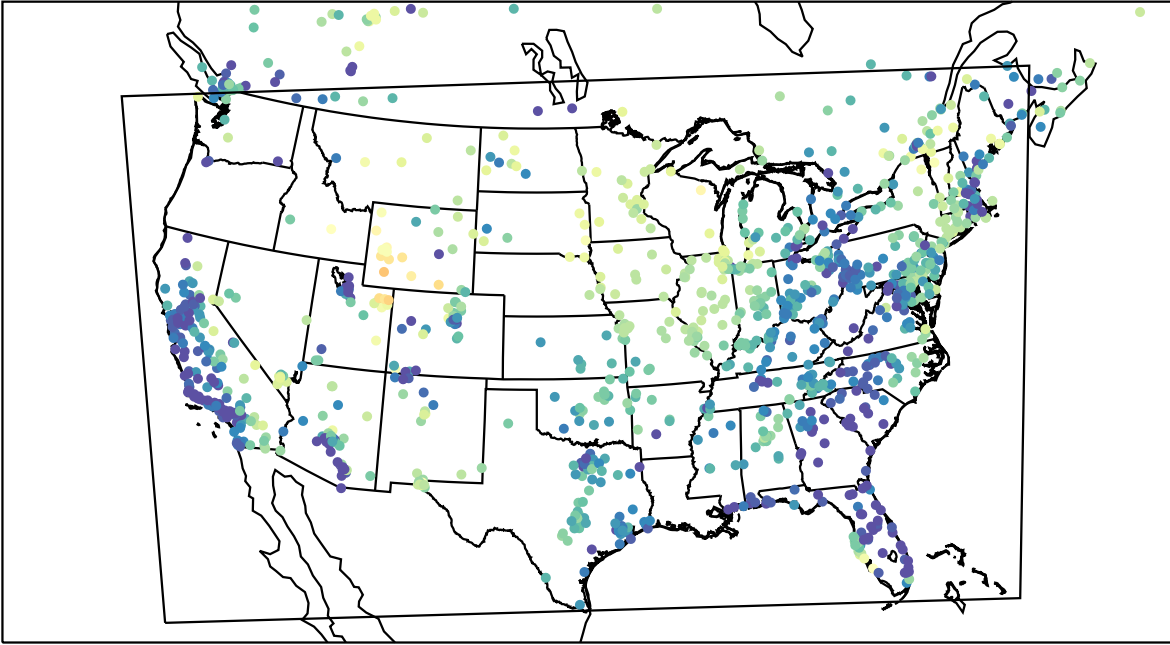
AirNOW (2023-03-13_07:00:00)
