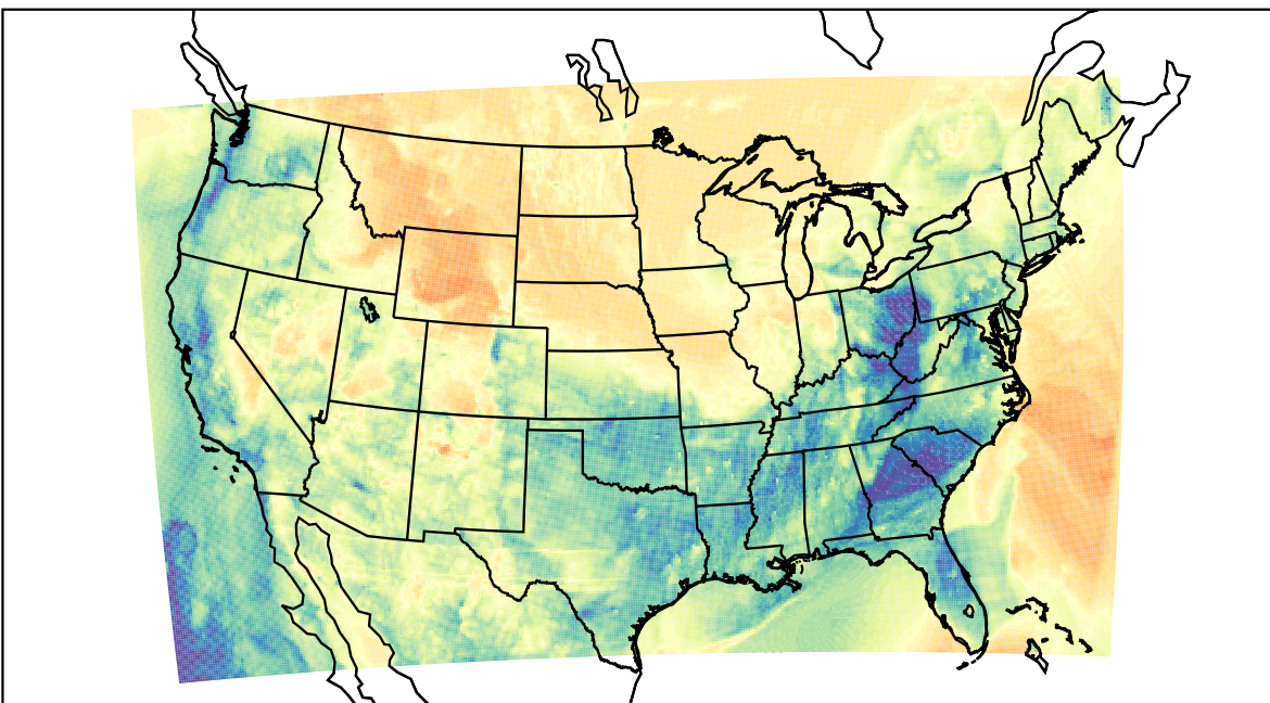
WRF (2023-03-13_06:00:00)
