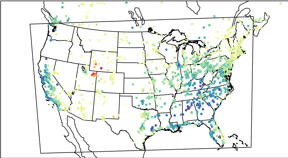
AirNOW (2023-03-12_21:00:00)
