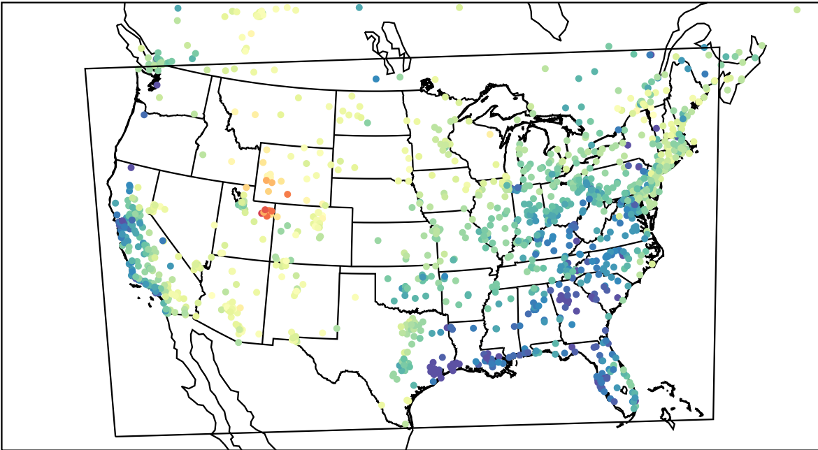
AirNOW (2023-03-13_00:00:00)
