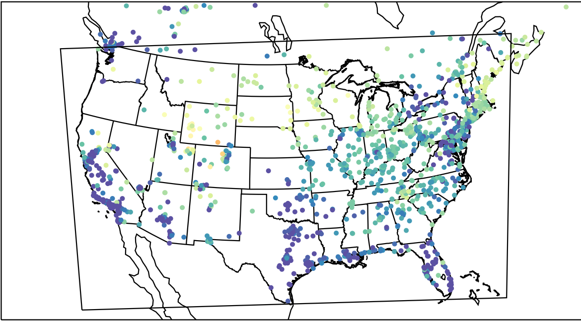
AirNOW (2023-03-12_12:00:00)
