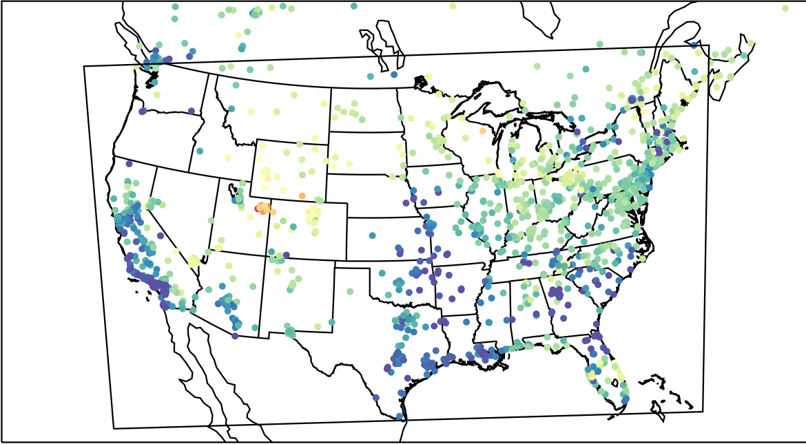
AirNOW (2023-03-12_02:00:00)
