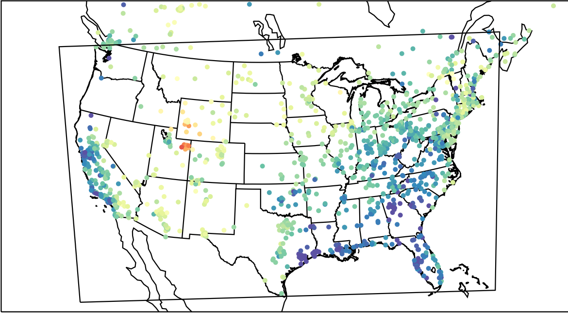
AirNOW (2023-03-13_01:00:00)
