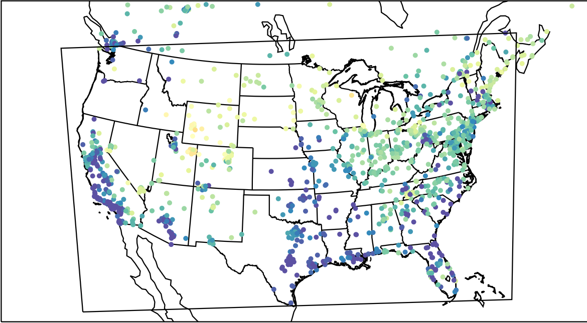
AirNOW (2023-03-12_05:00:00)
