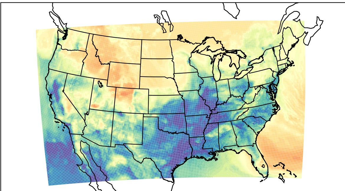
WRF (2023-03-12_12:00:00)
