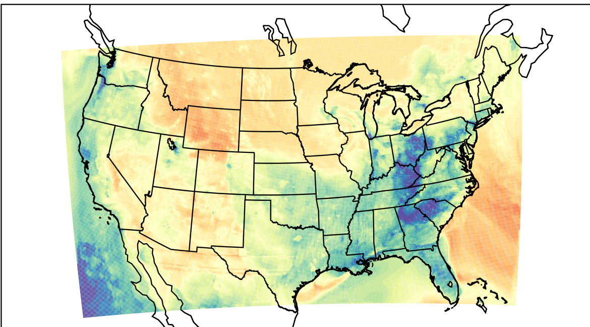
WRF (2023-03-13_01:00:00)
