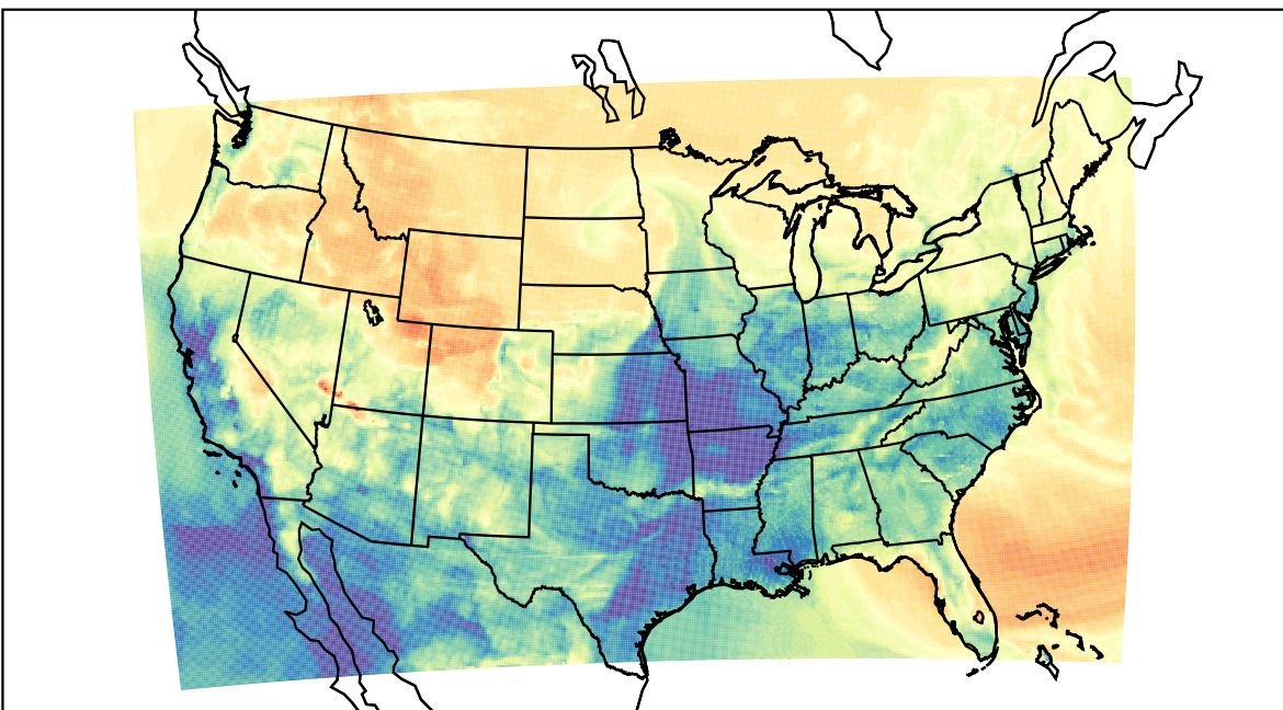
WRF (2023-03-12_06:00:00)
