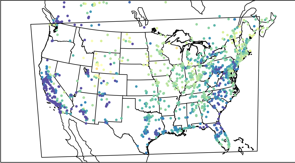
AirNOW (2023-03-13_14:00:00)
