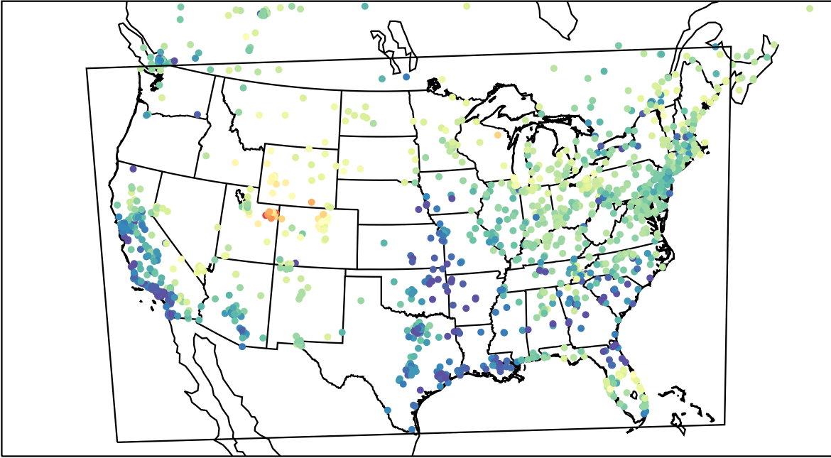
AirNOW (2023-03-12_01:00:00)
