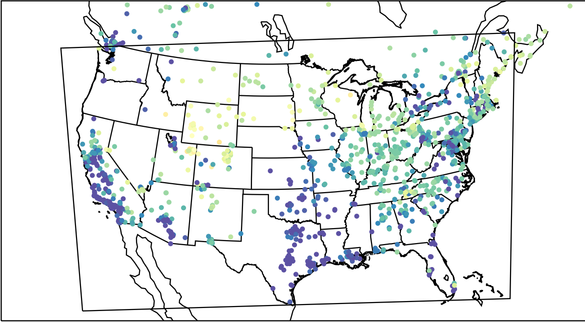
AirNOW (2023-03-12_07:00:00)
