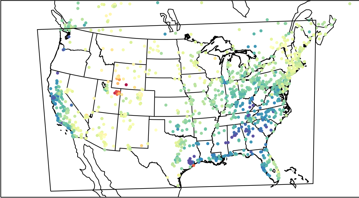
AirNOW (2023-03-12_22:00:00)
