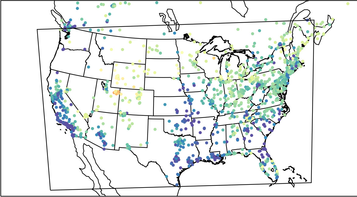
AirNOW (2023-03-12_03:00:00)
