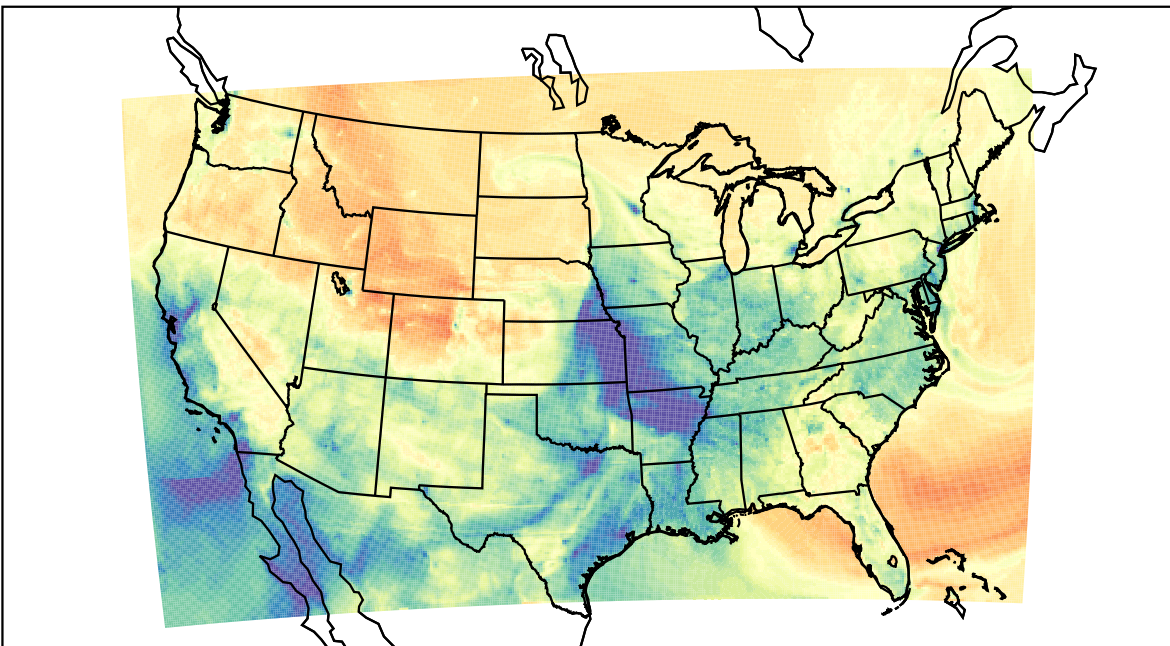
WRF (2023-03-12_01:00:00)
