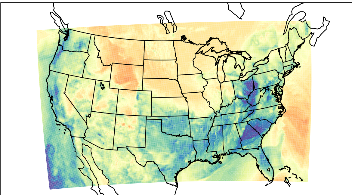
WRF (2023-03-13_07:00:00)
