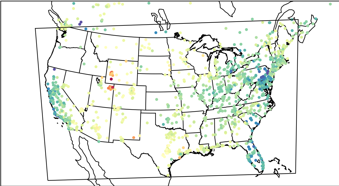
AirNOW (2023-03-13_22:00:00)
