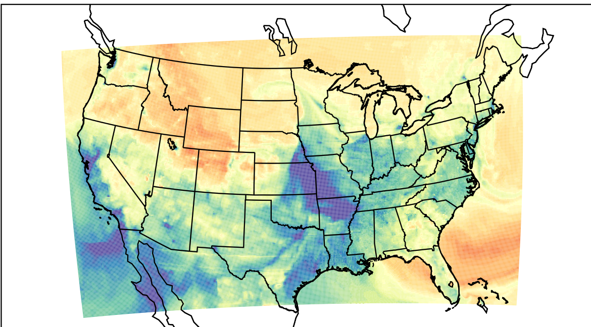
WRF (2023-03-12_02:00:00)
