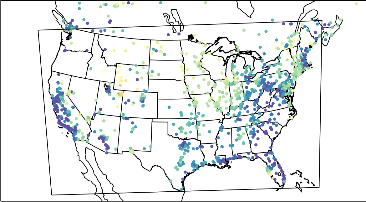
AirNOW (2023-03-13_08:00:00)
