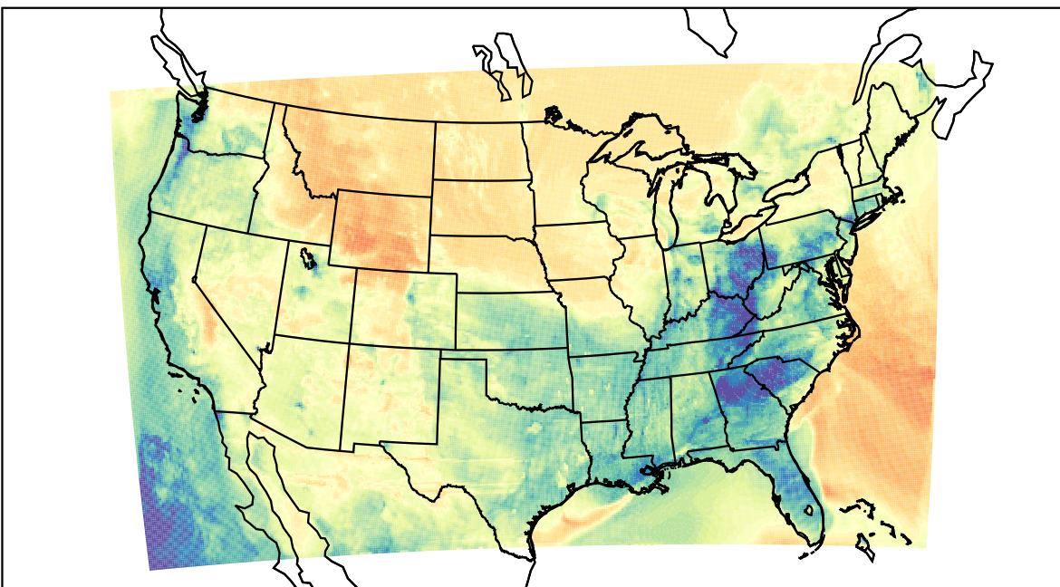
WRF (2023-03-13_02:00:00)
