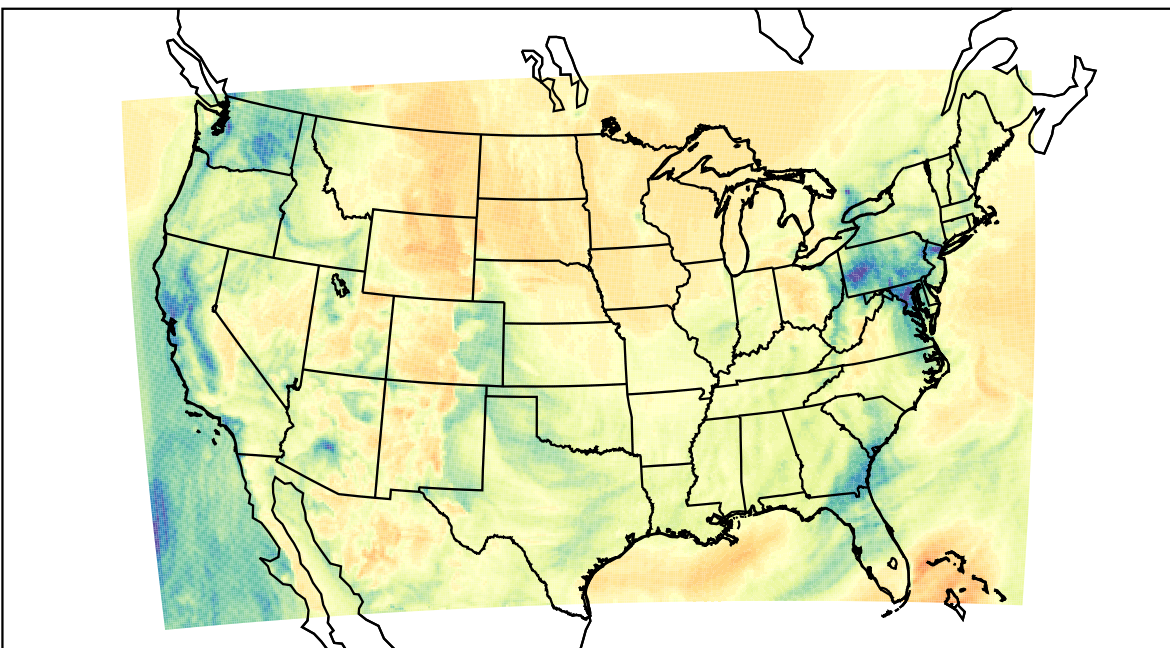
WRF (2023-03-13_17:00:00)
