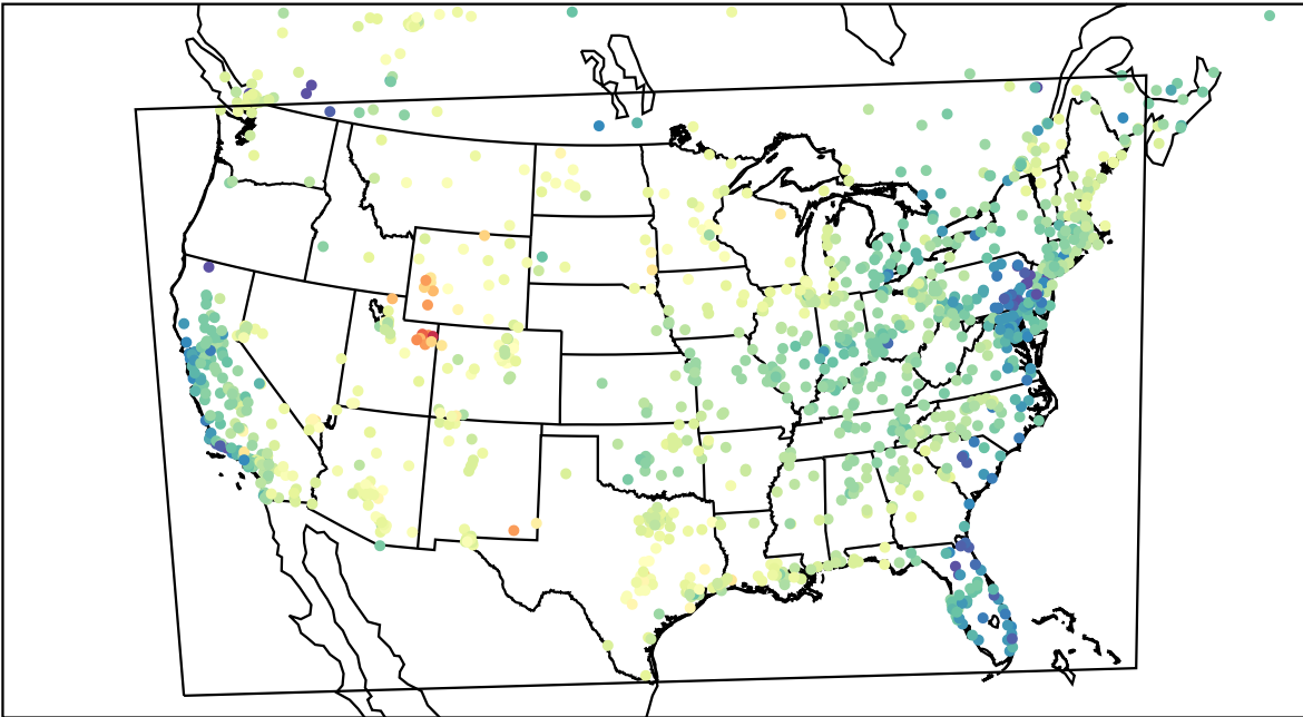
AirNOW (2023-03-13_23:00:00)
