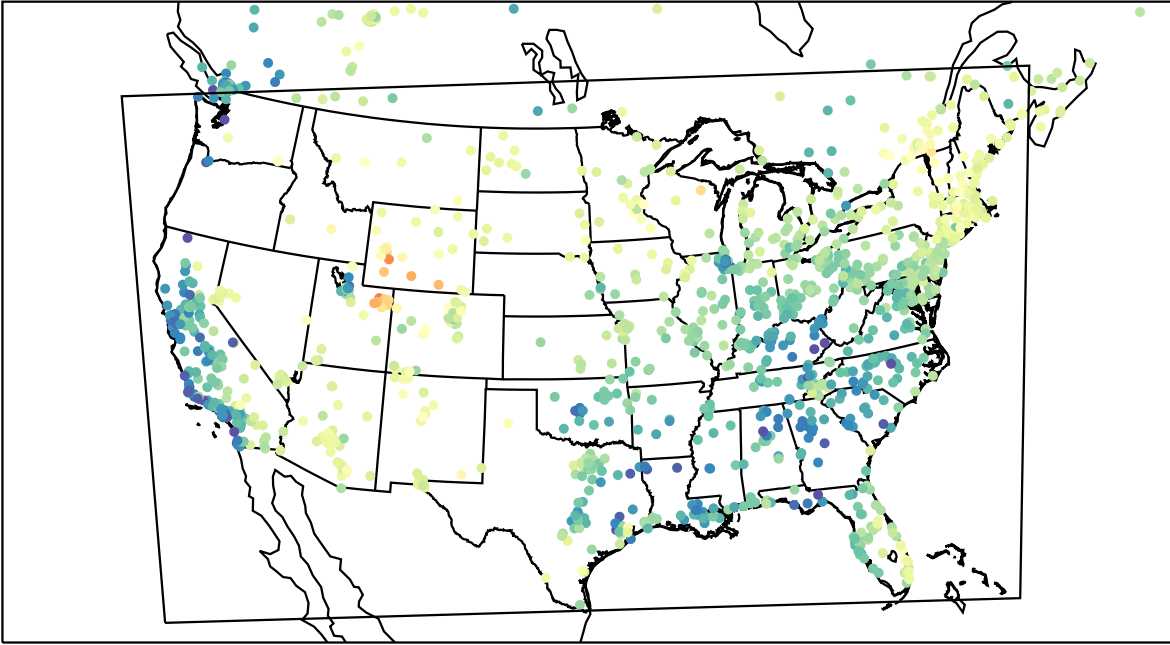
AirNOW (2023-03-12_19:00:00)
