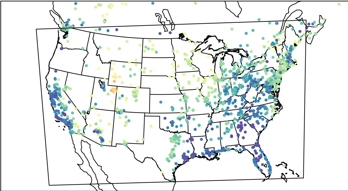
AirNOW (2023-03-13_03:00:00)
