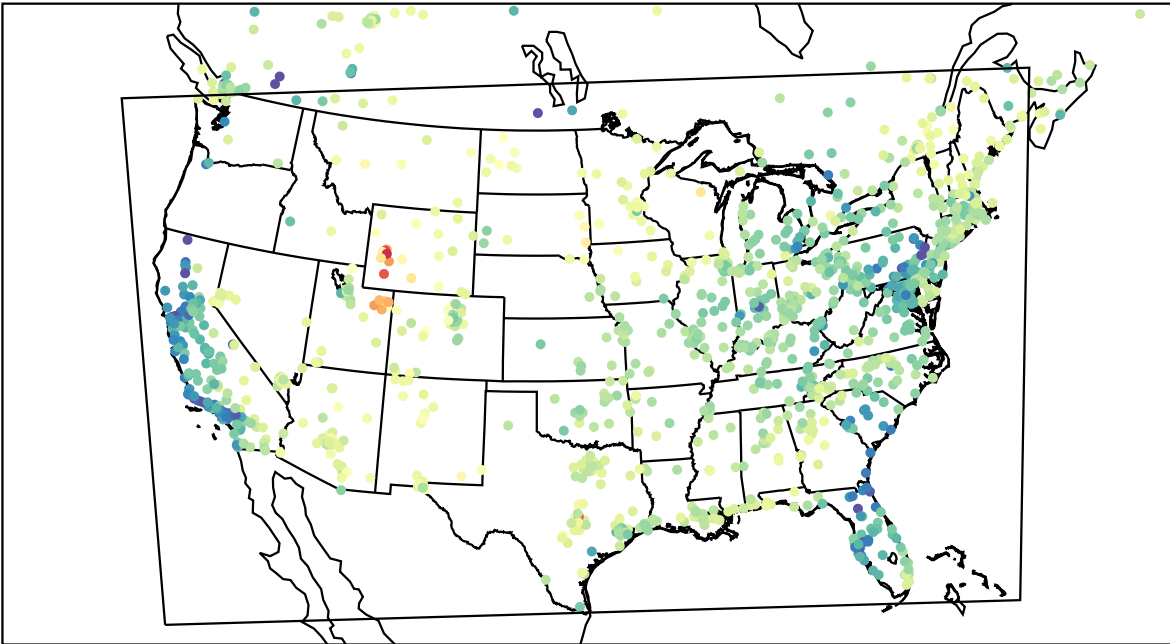
AirNOW (2023-03-13_19:00:00)
