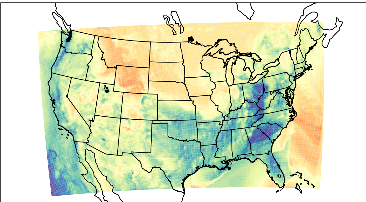
WRF (2023-03-13_05:00:00)
