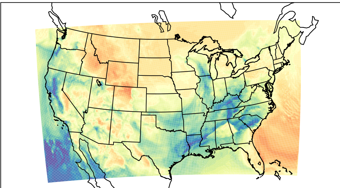
WRF (2023-03-12_17:00:00)
