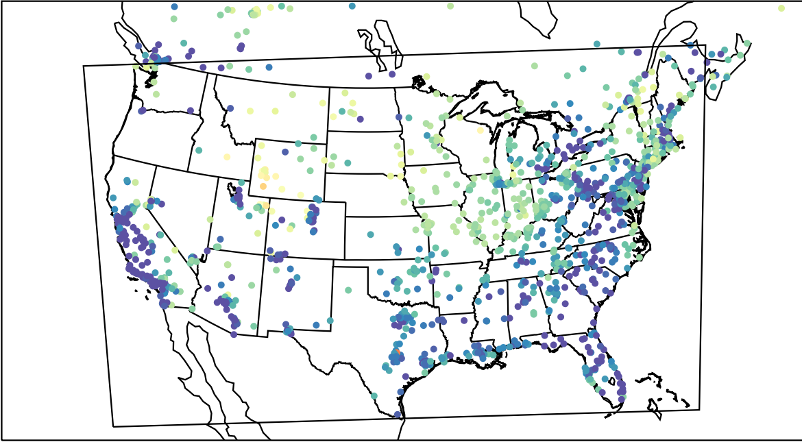
AirNOW (2023-03-13_12:00:00)
