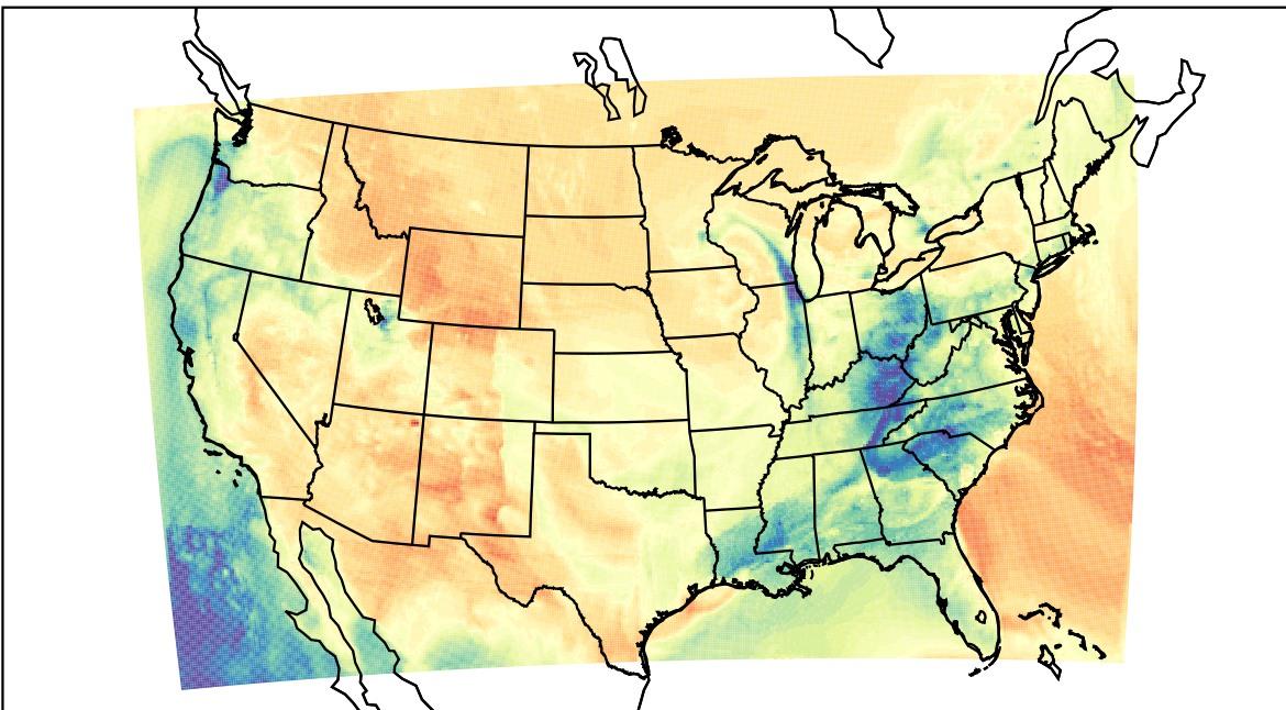
WRF (2023-03-12_22:00:00)
