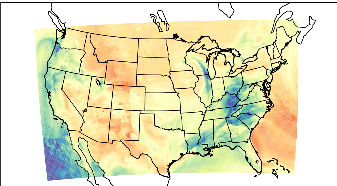
WRF (2023-03-12_21:00:00)
