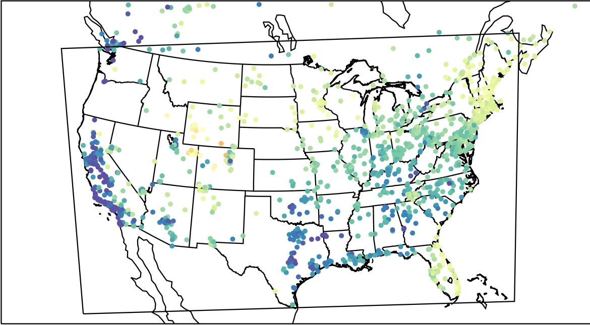
AirNOW (2023-03-12_16:00:00)
