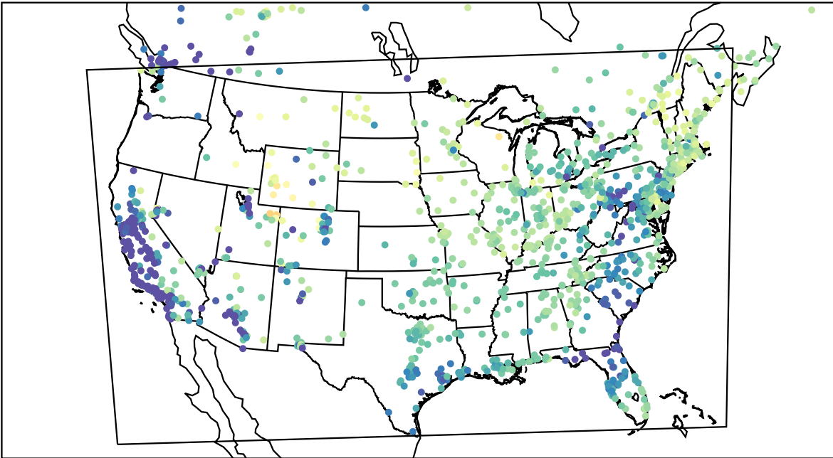
AirNOW (2023-03-13_15:00:00)
