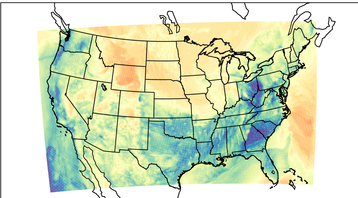
WRF (2023-03-13_08:00:00)
