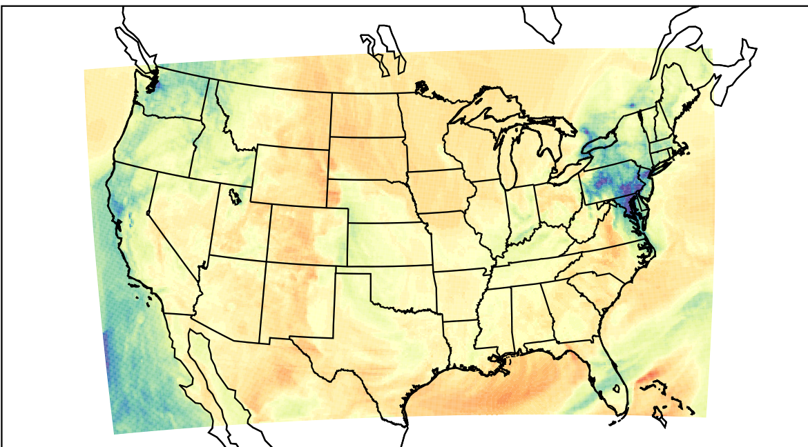
WRF (2023-03-13_21:00:00)
