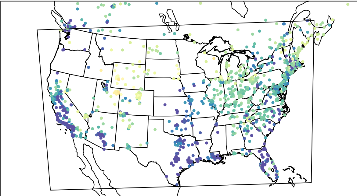
AirNOW (2023-03-12_06:00:00)
