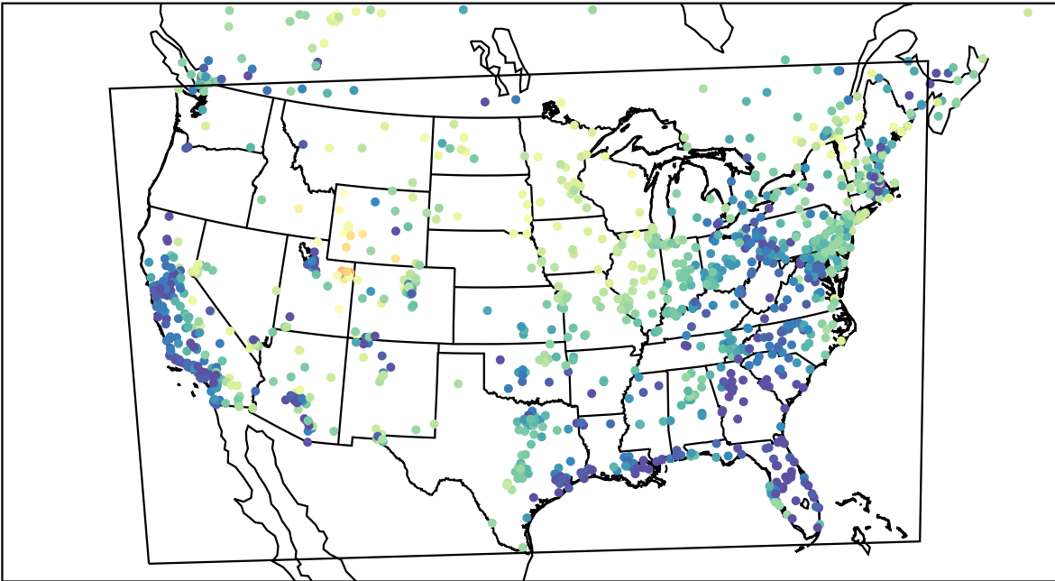
AirNOW (2023-03-13_05:00:00)
