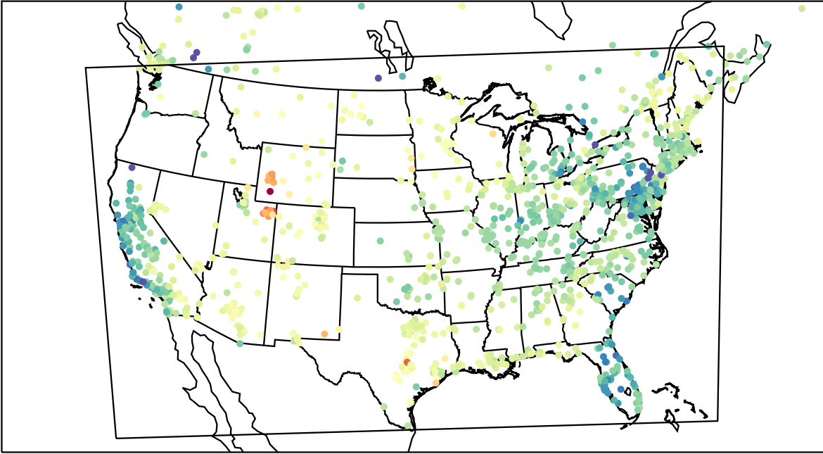
AirNOW (2023-03-13_21:00:00)
