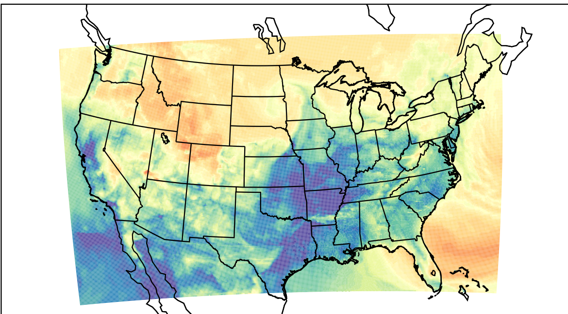
WRF (2023-03-12_08:00:00)
