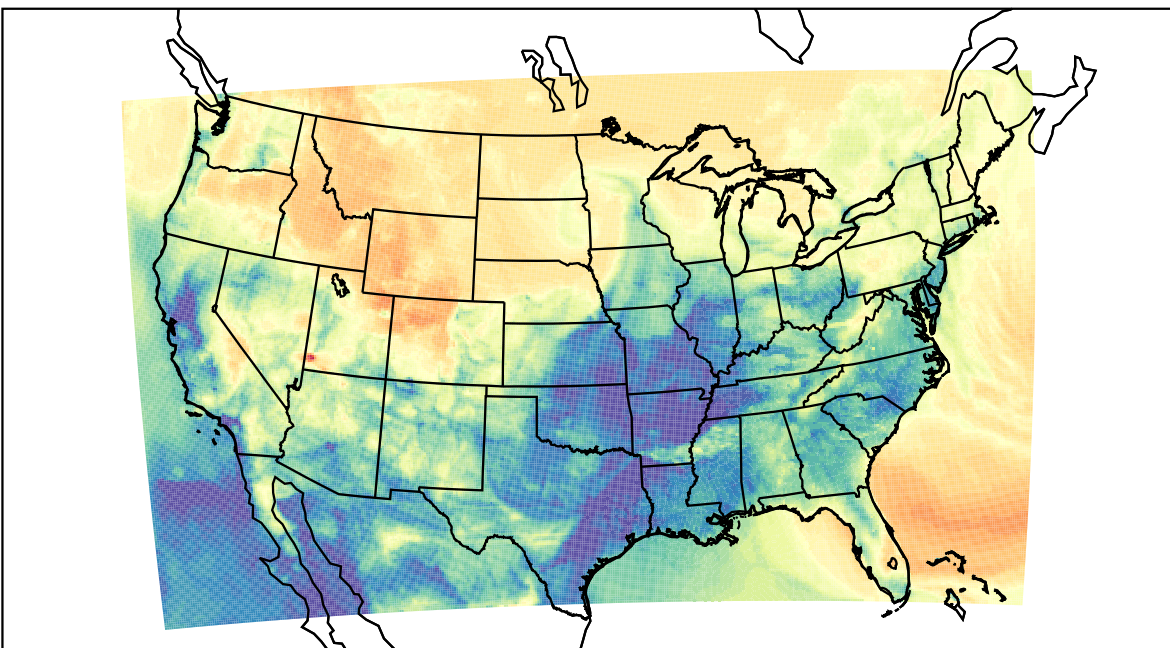
WRF (2023-03-12_09:00:00)
