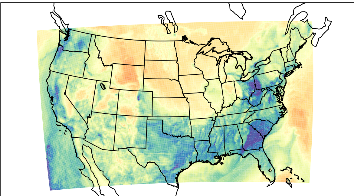
WRF (2023-03-13_11:00:00)
