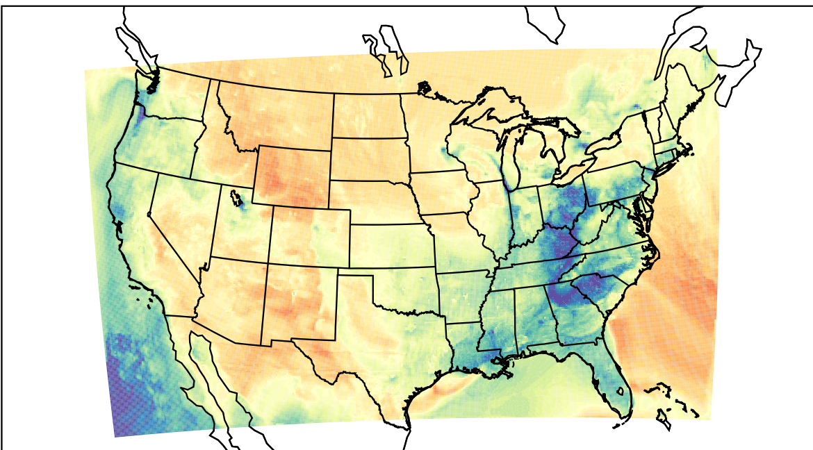
WRF (2023-03-13_00:00:00)
