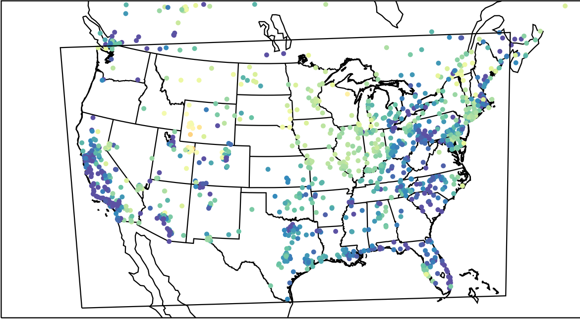
AirNOW (2023-03-13_09:00:00)
