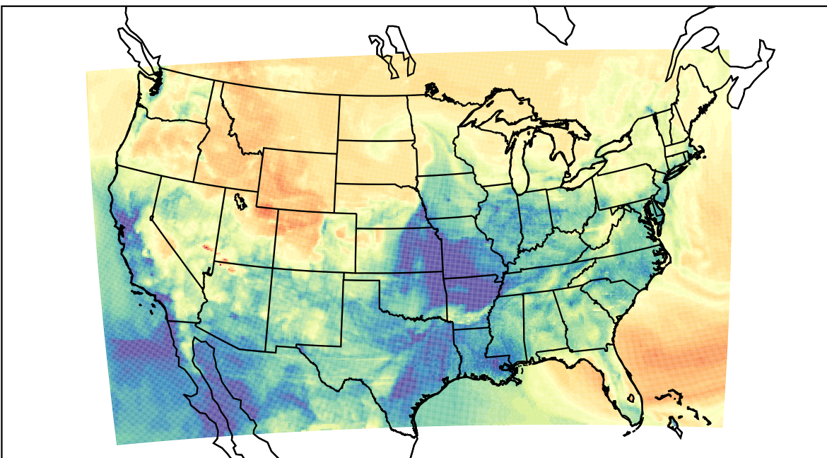
WRF (2023-03-12_05:00:00)
