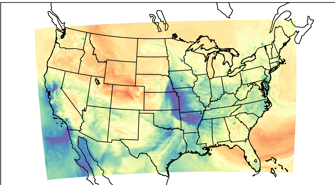
WRF (2023-03-12_00:00:00)
