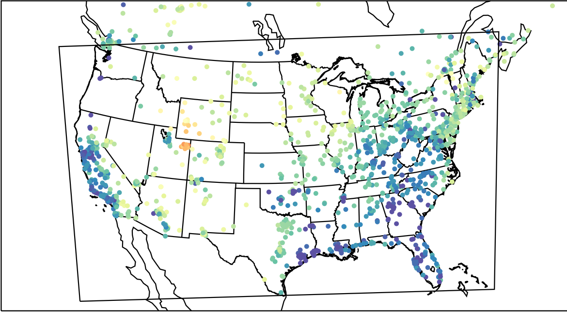
AirNOW (2023-03-13_02:00:00)
