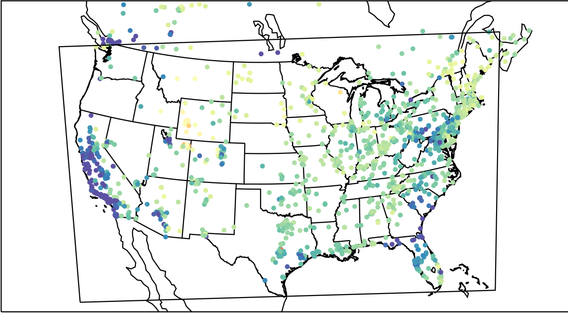
AirNOW (2023-03-13_16:00:00)
