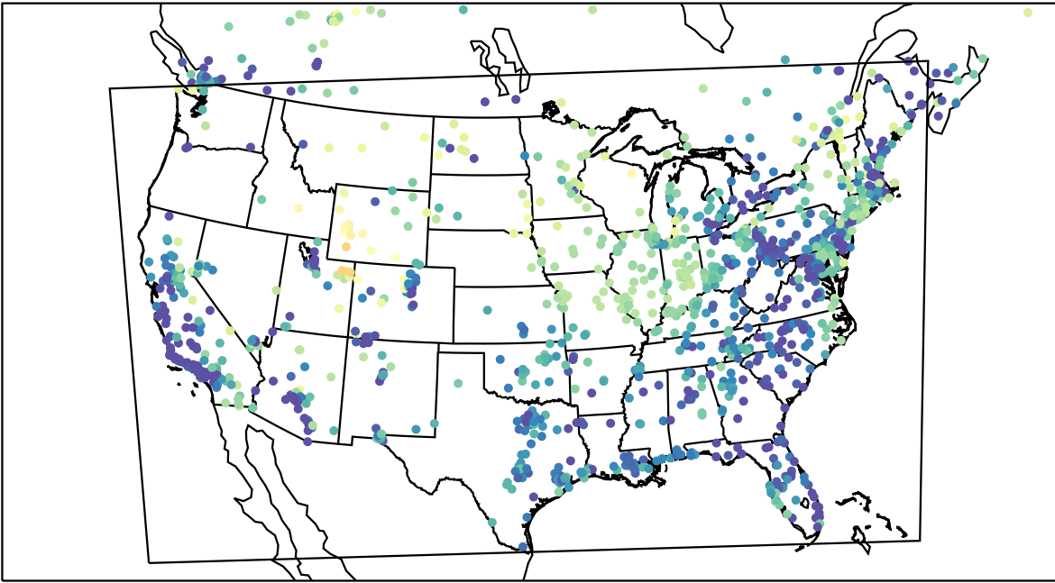
AirNOW (2023-03-13_11:00:00)
