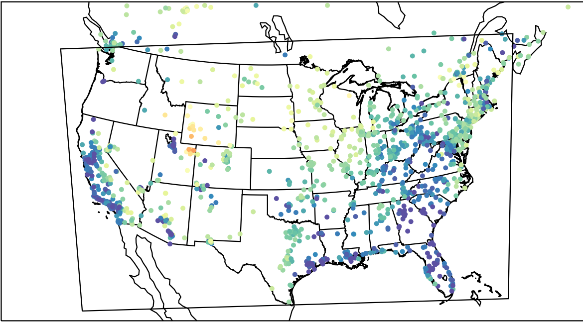
AirNOW (2023-03-13_04:00:00)
