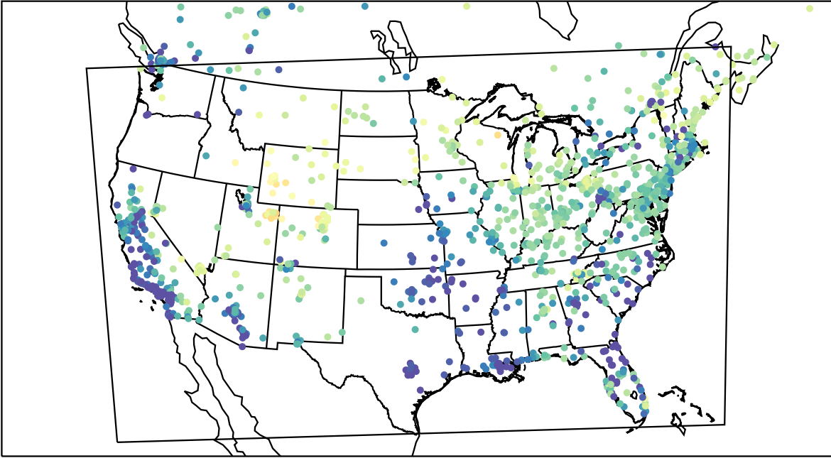
AirNOW (2023-03-12_04:00:00)
