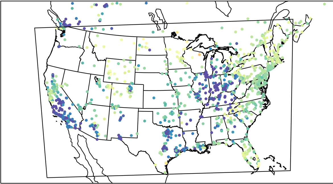
AirNOW (2023-03-15_07:00:00)
