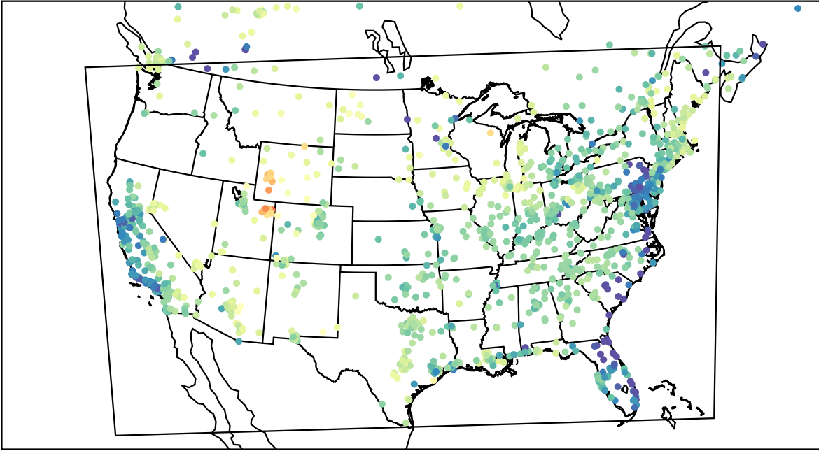
AirNOW (2023-03-14_01:00:00)
