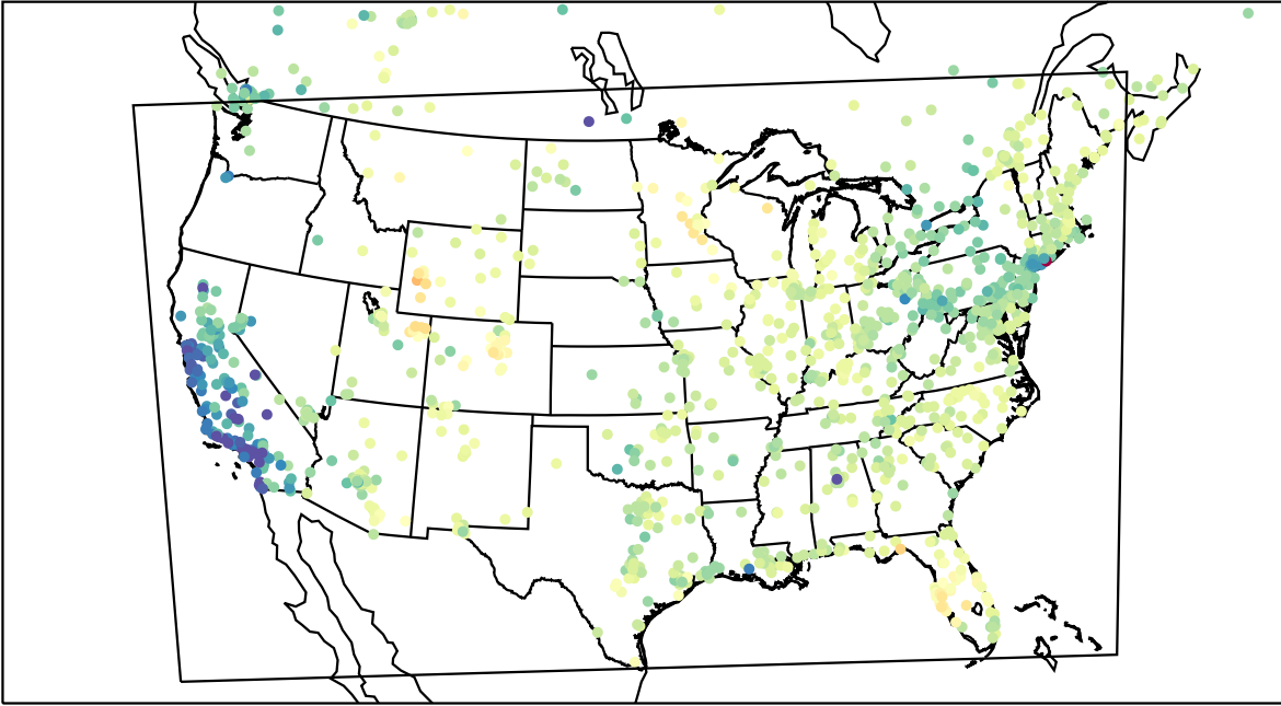
AirNOW (2023-03-14_18:00:00)
