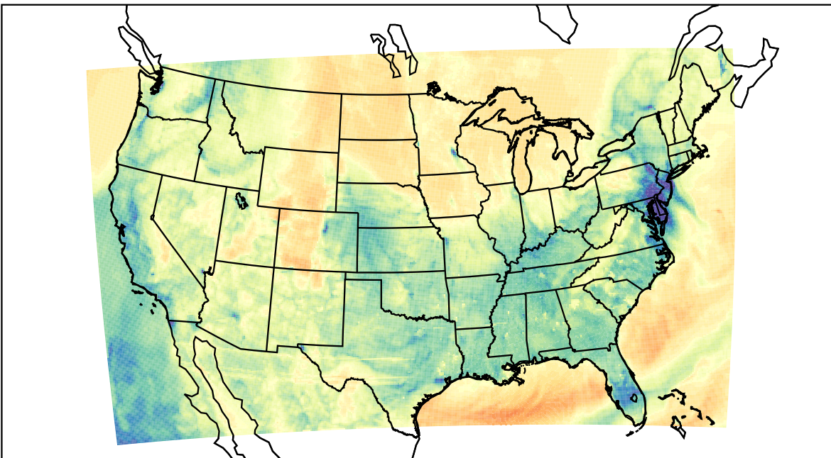
WRF (2023-03-14_03:00:00)
