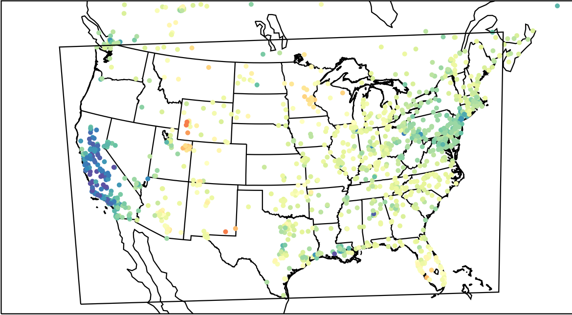
AirNOW (2023-03-14_23:00:00)
