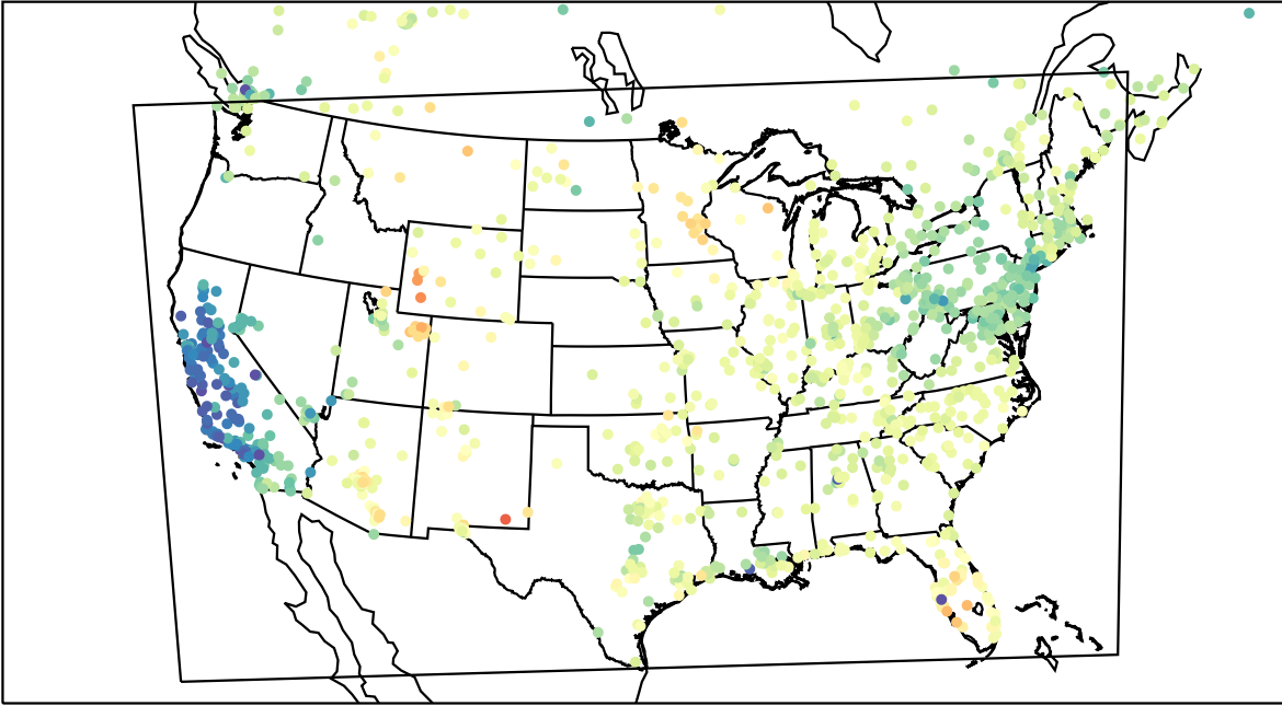
AirNOW (2023-03-14_22:00:00)
