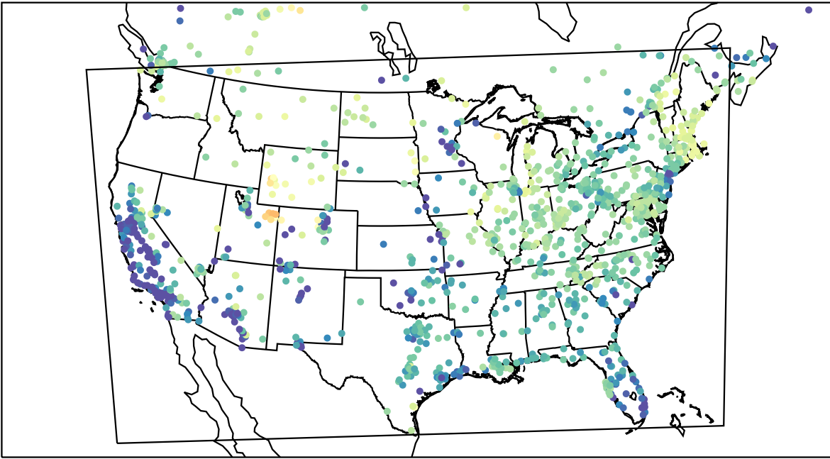
AirNOW (2023-03-14_09:00:00)
