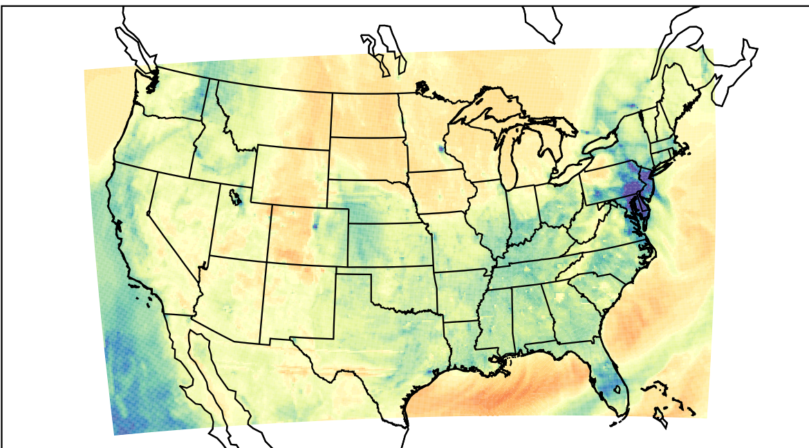
WRF (2023-03-14_01:00:00)
