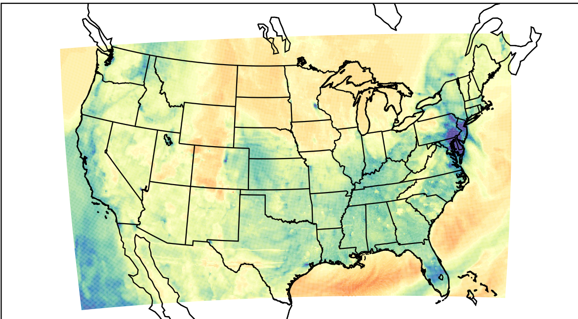
WRF (2023-03-14_02:00:00)
