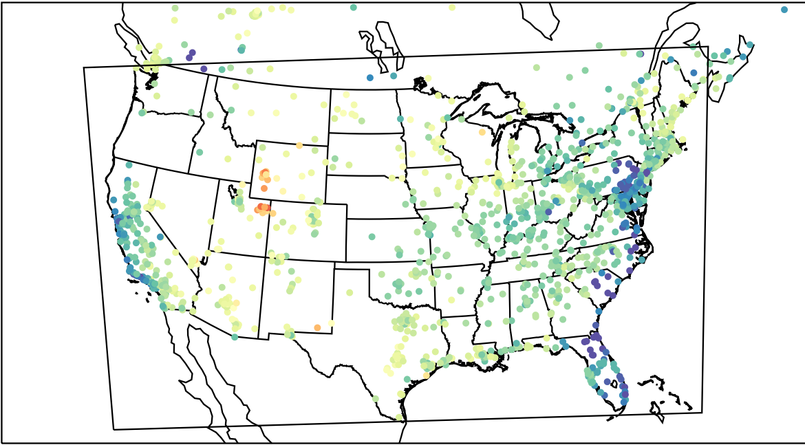
AirNOW (2023-03-14_00:00:00)
