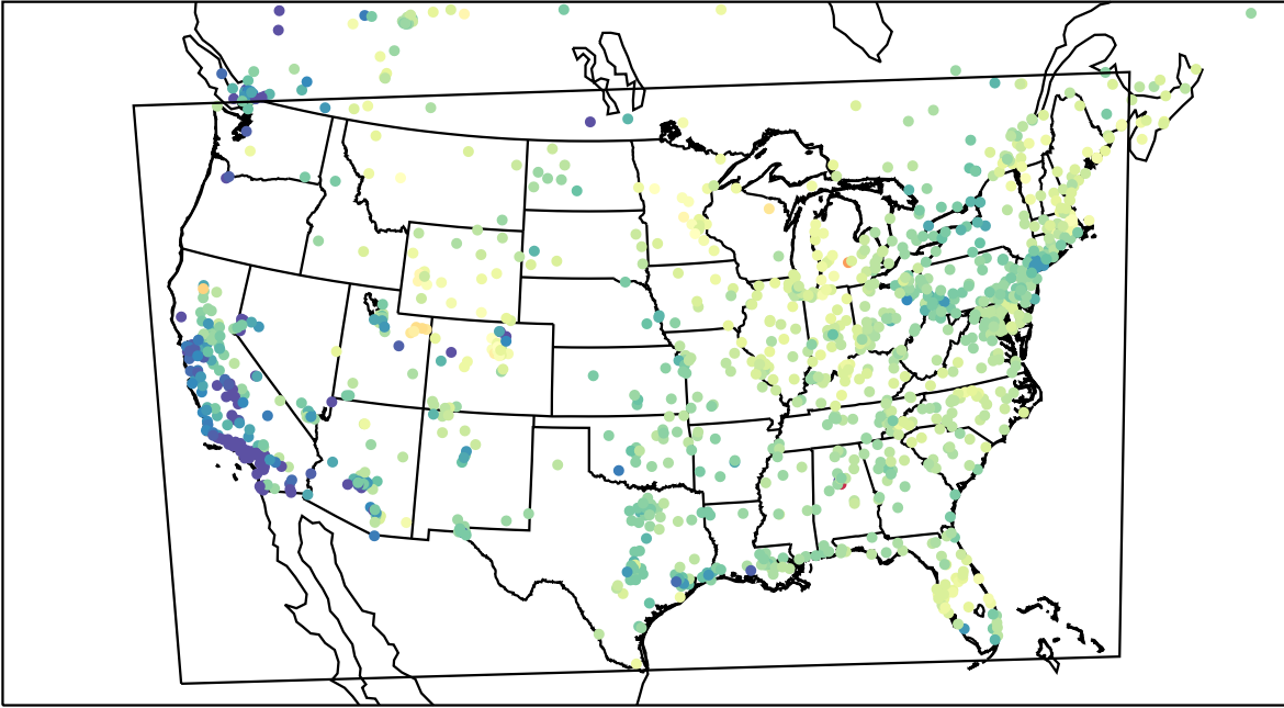
AirNOW (2023-03-14_16:00:00)
