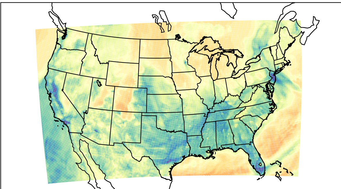
WRF (2023-03-14_08:00:00)
