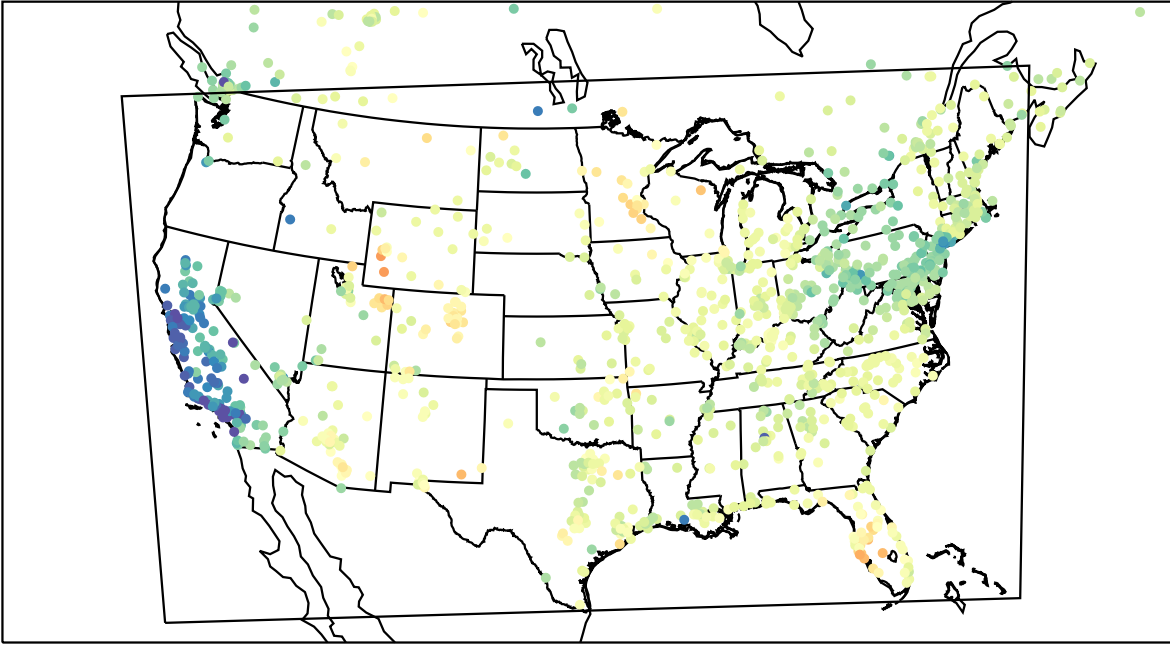
AirNOW (2023-03-14_20:00:00)
