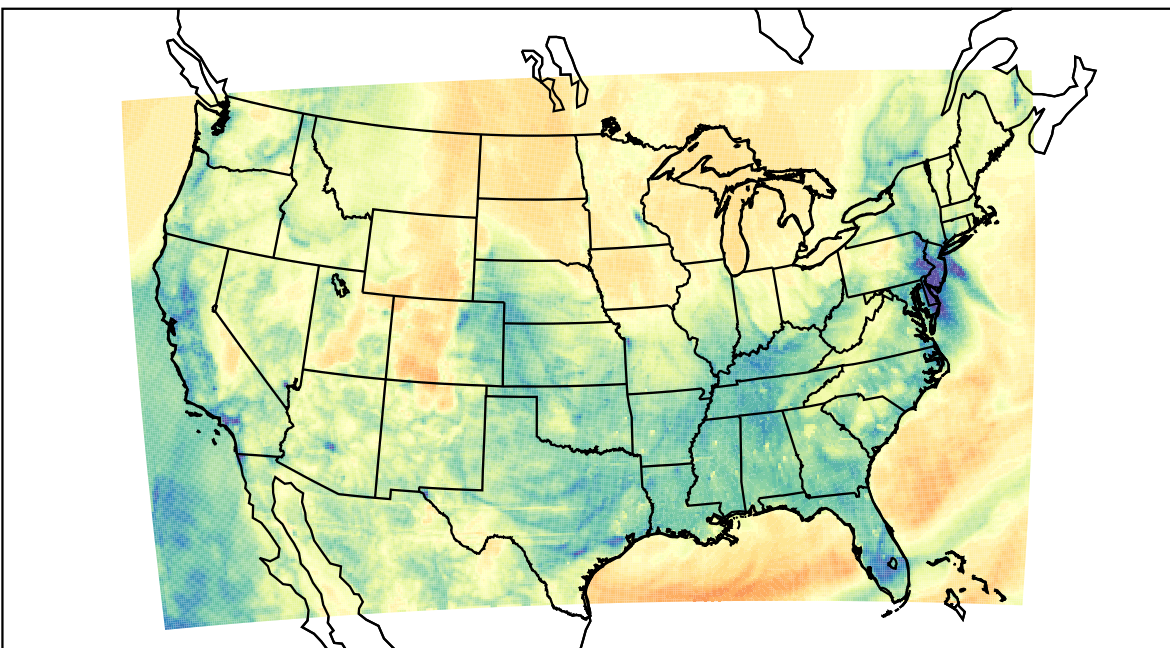
WRF (2023-03-14_05:00:00)
