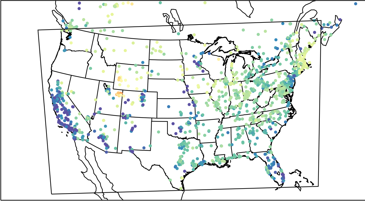
AirNOW (2023-03-14_07:00:00)
