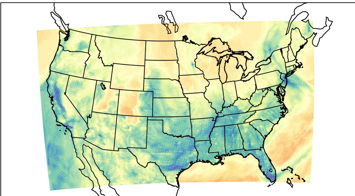
WRF (2023-03-14_09:00:00)
