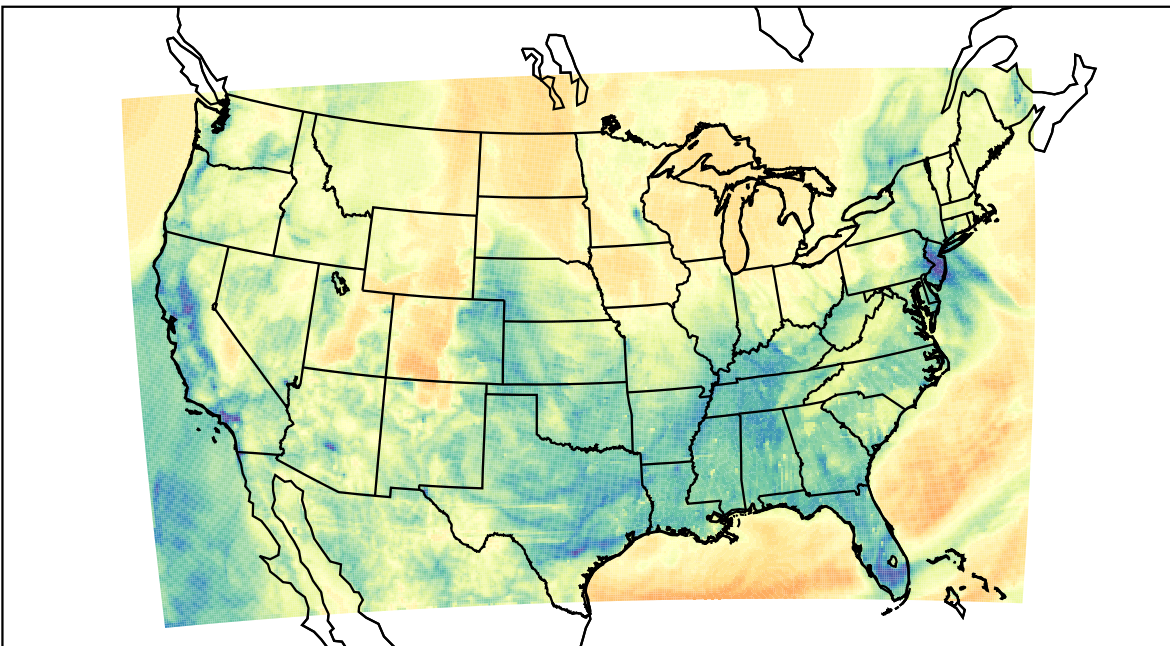
WRF (2023-03-14_07:00:00)
