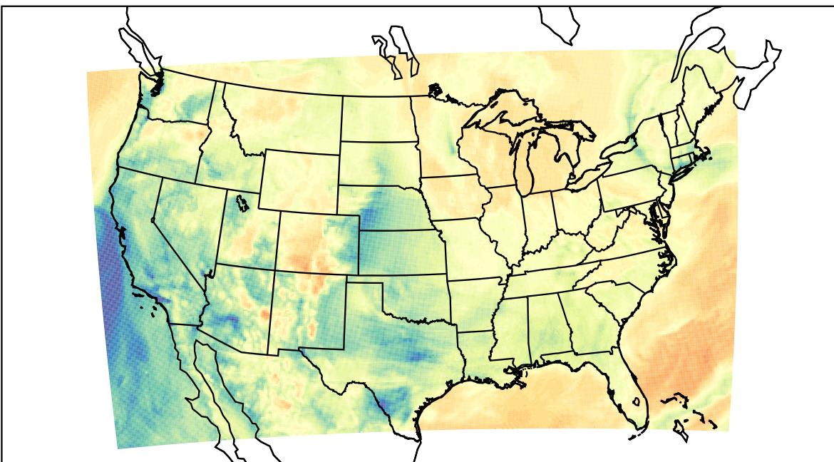
WRF (2023-03-14_16:00:00)
