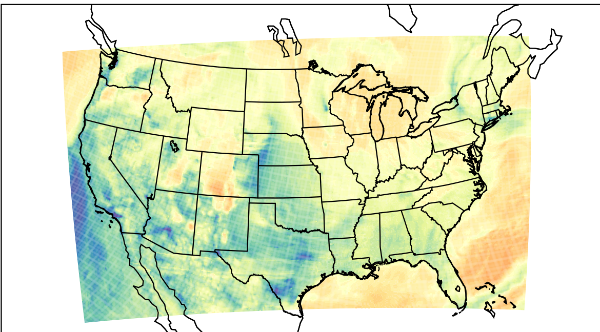
WRF (2023-03-14_15:00:00)
