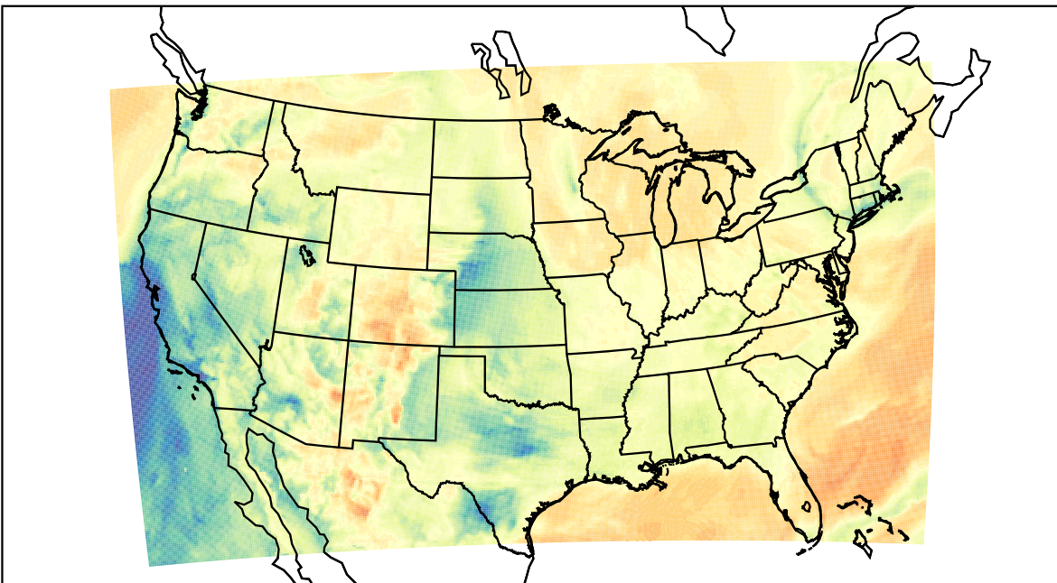
WRF (2023-03-14_17:00:00)
