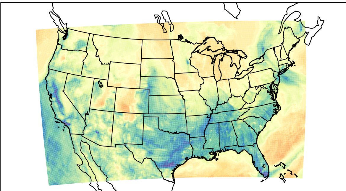
WRF (2023-03-14_11:00:00)
