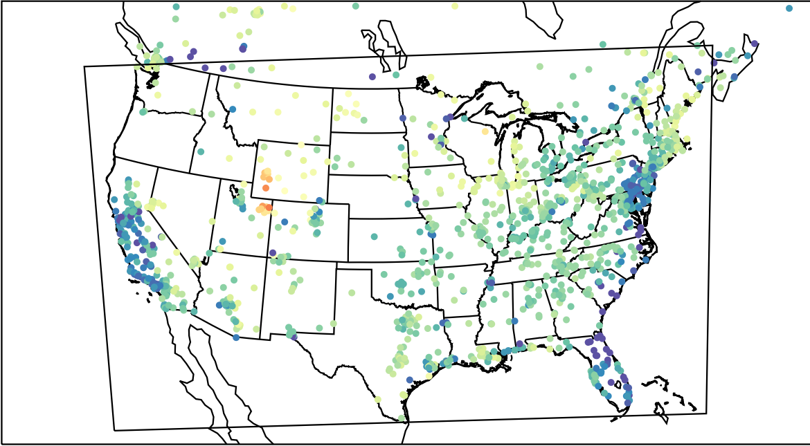
AirNOW (2023-03-14_02:00:00)
