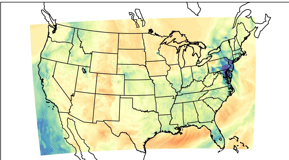
WRF (2023-03-14_00:00:00)
