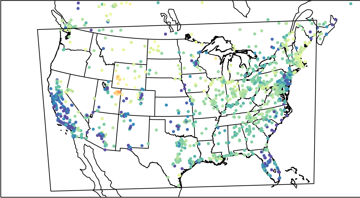
AirNOW (2023-03-14_05:00:00)
