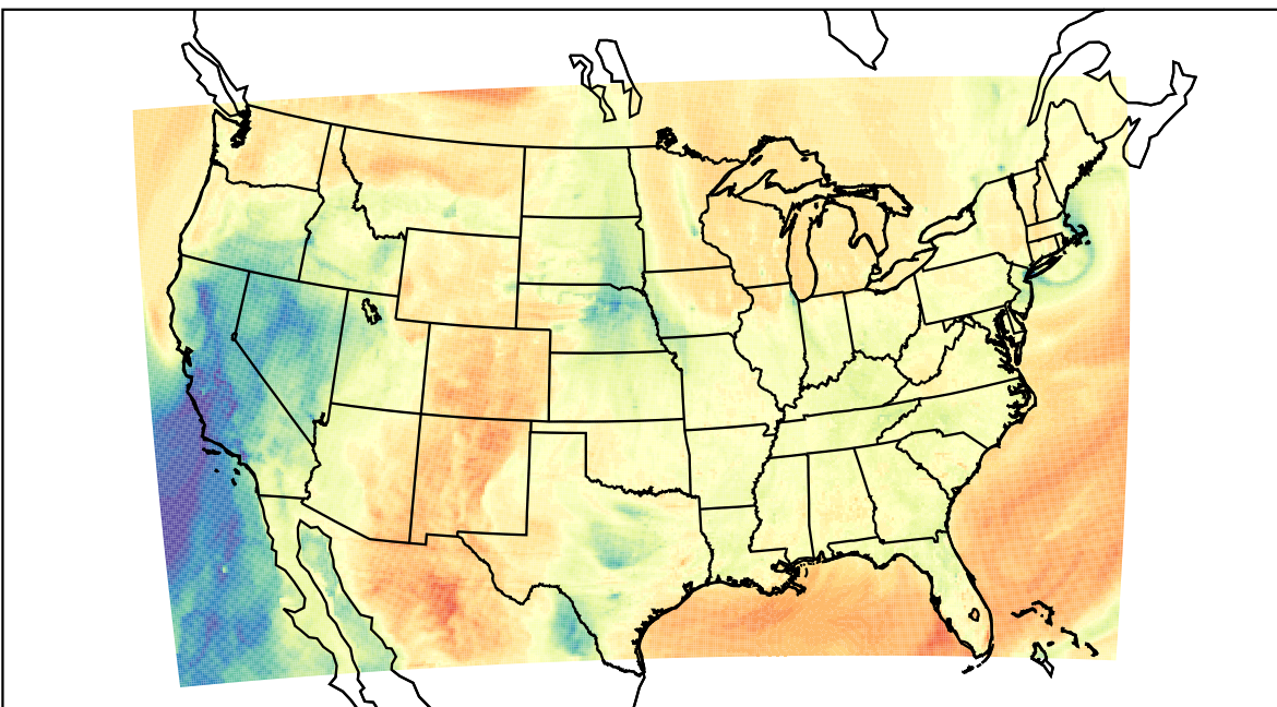
WRF (2023-03-14_23:00:00)
