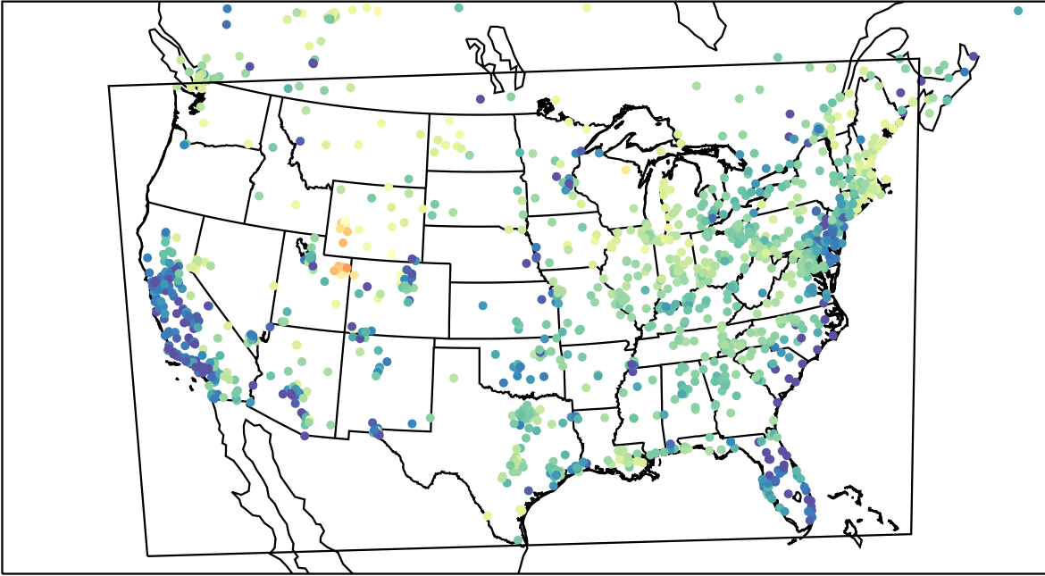
AirNOW (2023-03-14_04:00:00)
