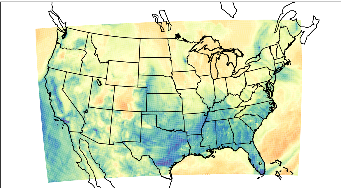
WRF (2023-03-14_12:00:00)
