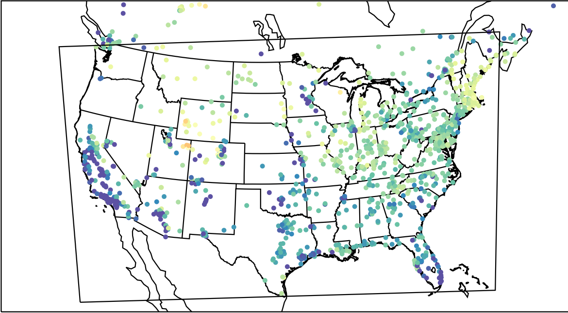
AirNOW (2023-03-14_10:00:00)
