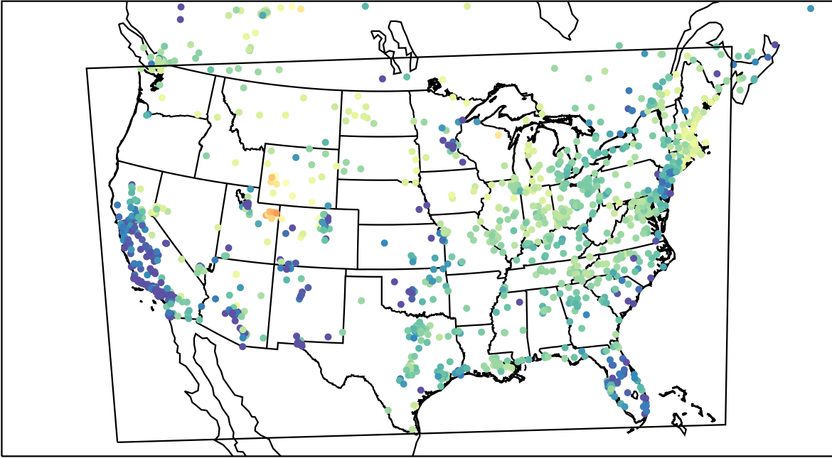
AirNOW (2023-03-14_06:00:00)
