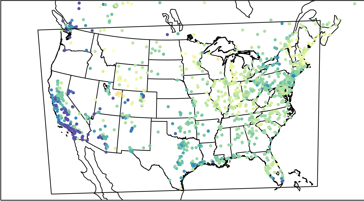
AirNOW (2023-03-14_15:00:00)
