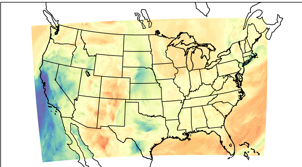
WRF (2023-03-14_19:00:00)
