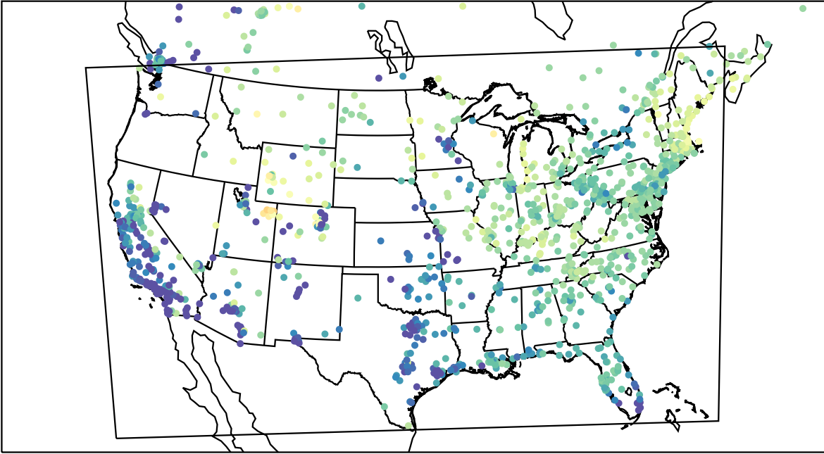
AirNOW (2023-03-14_13:00:00)
