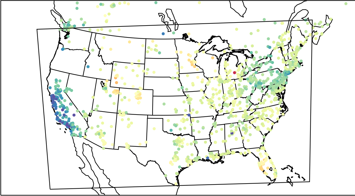
AirNOW (2023-03-14_19:00:00)
