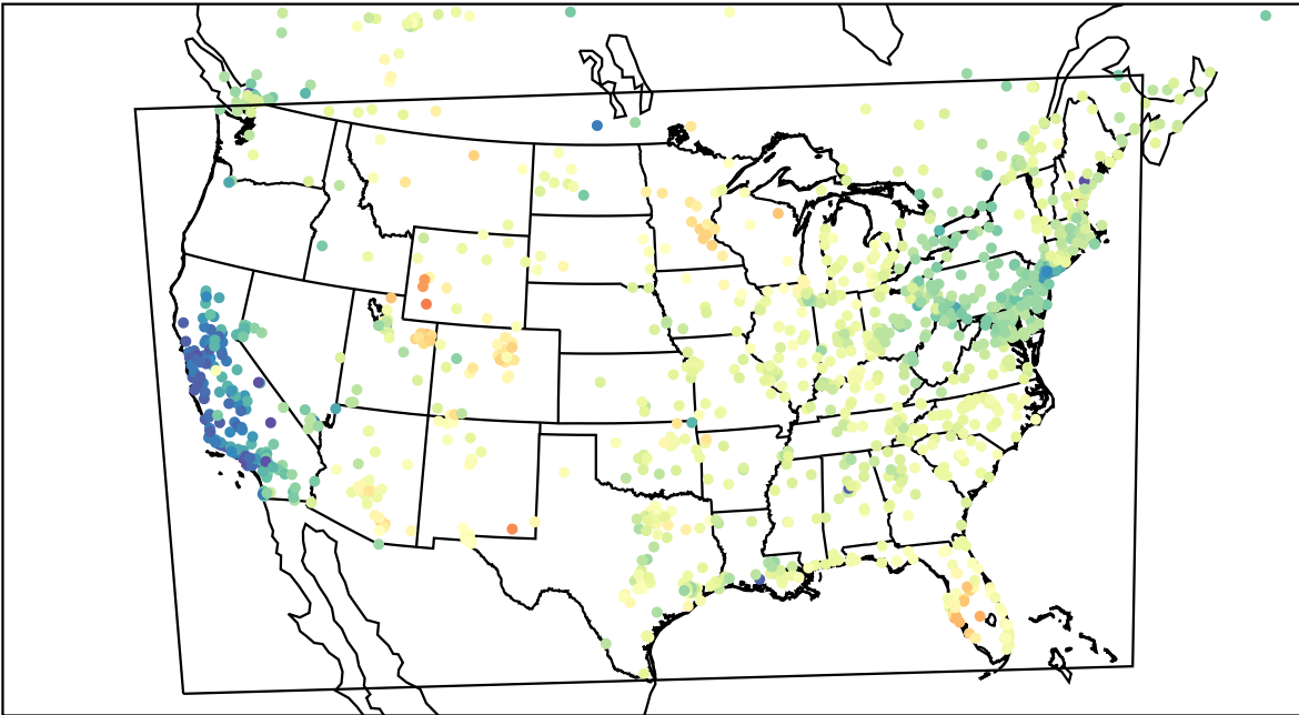
AirNOW (2023-03-14_21:00:00)
