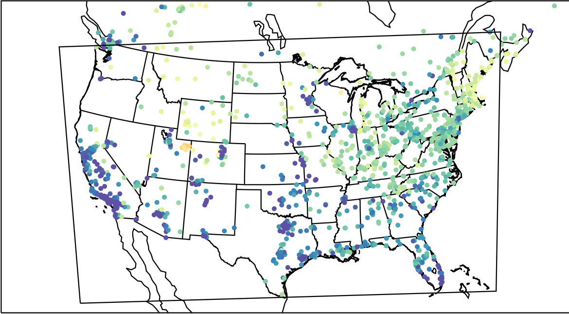
AirNOW (2023-03-14_12:00:00)
