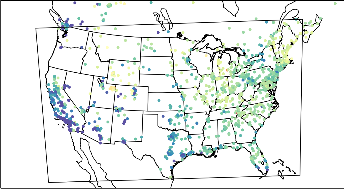
AirNOW (2023-03-14_14:00:00)
