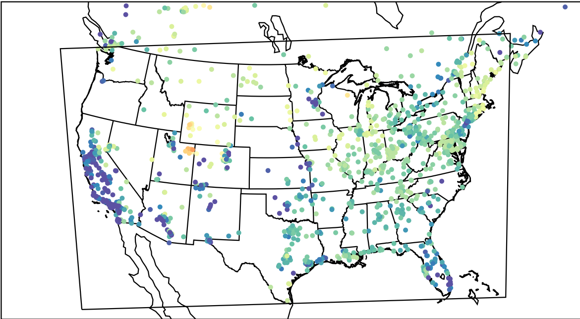
AirNOW (2023-03-14_08:00:00)
