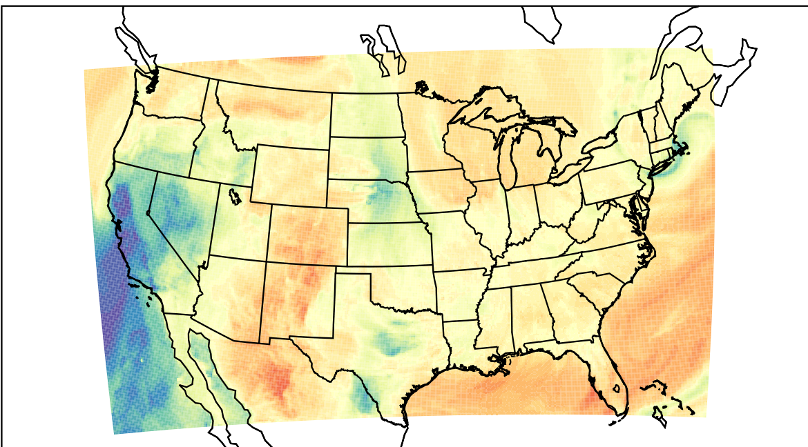
WRF (2023-03-14_21:00:00)
