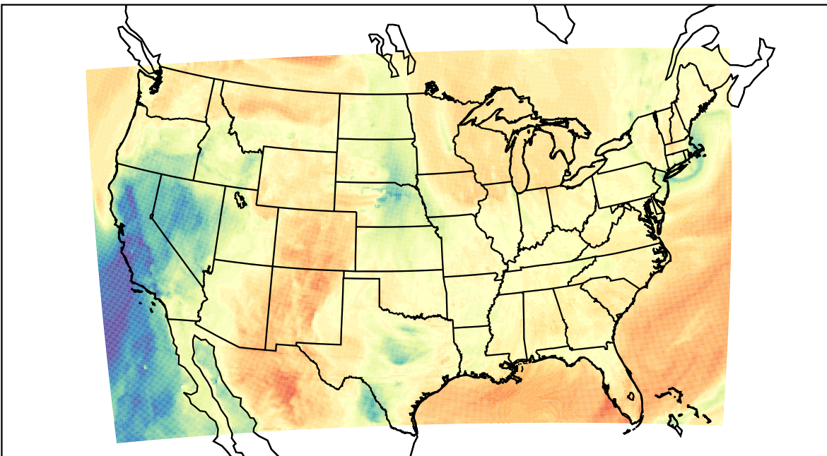
WRF (2023-03-14_22:00:00)
