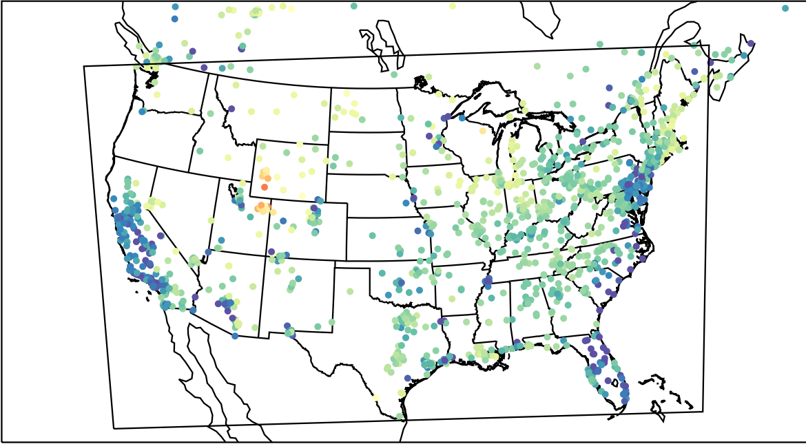
AirNOW (2023-03-14_03:00:00)
