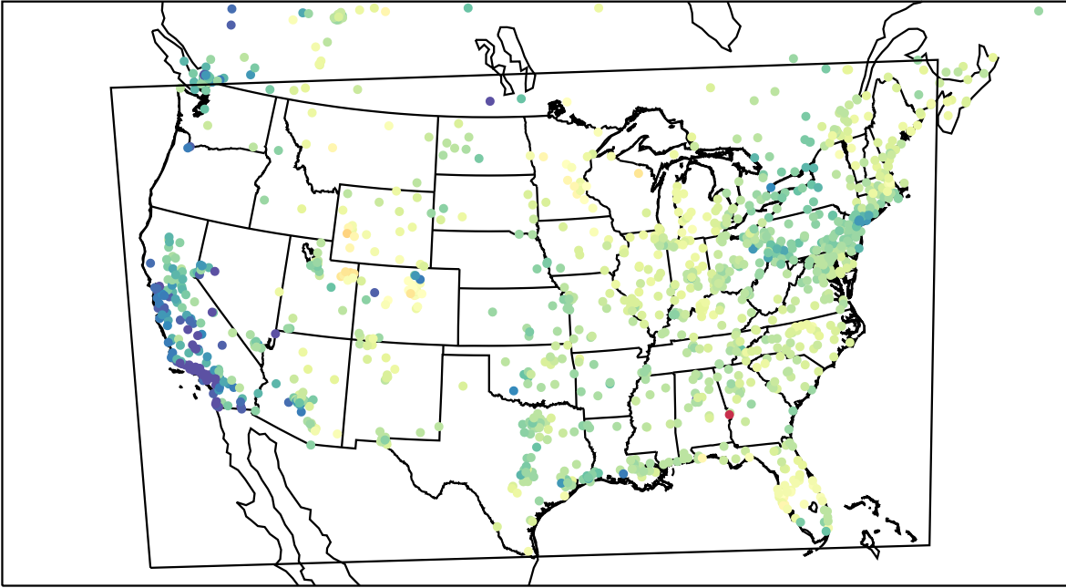
AirNOW (2023-03-14_17:00:00)
