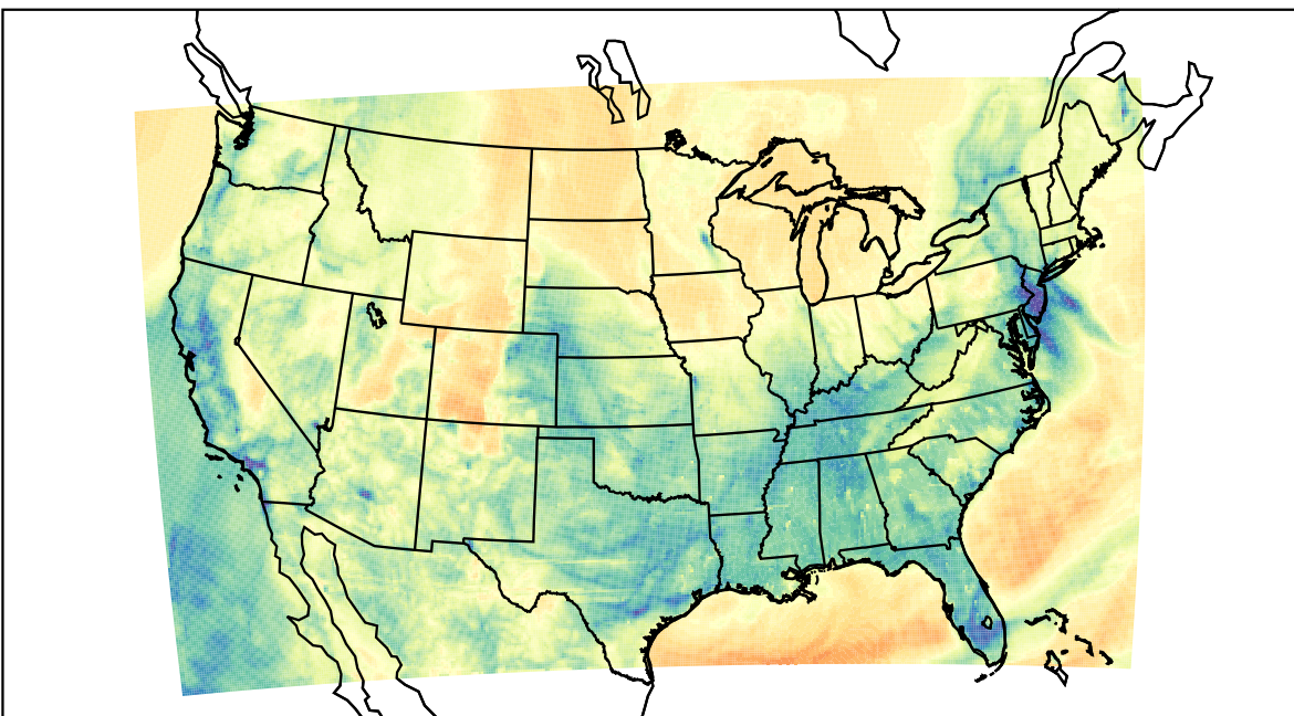
WRF (2023-03-14_06:00:00)
