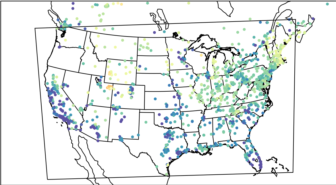
AirNOW (2023-03-14_11:00:00)
