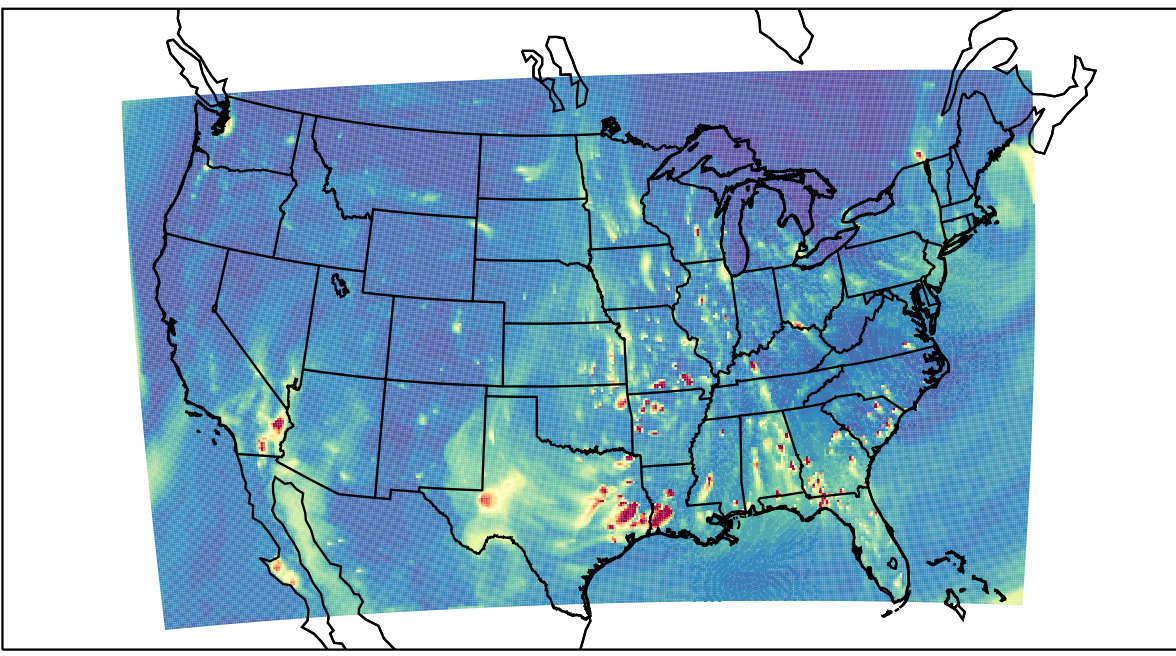
WRF 2023-03-15_02:00:00
