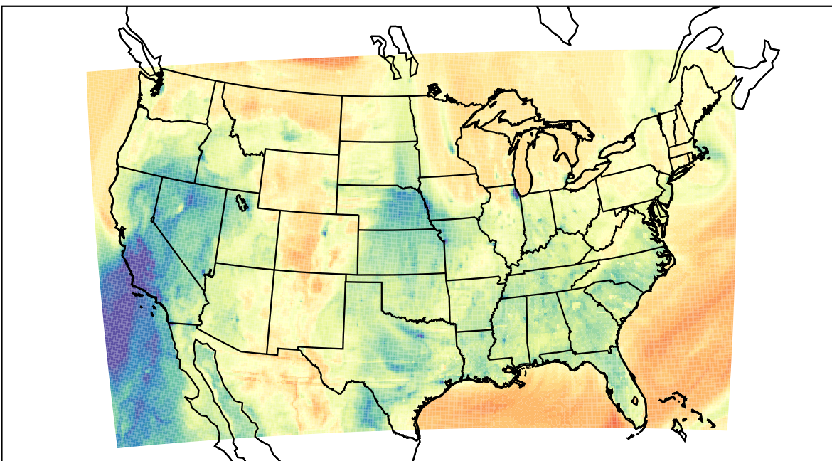
WRF (2023-03-15_01:00:00)
