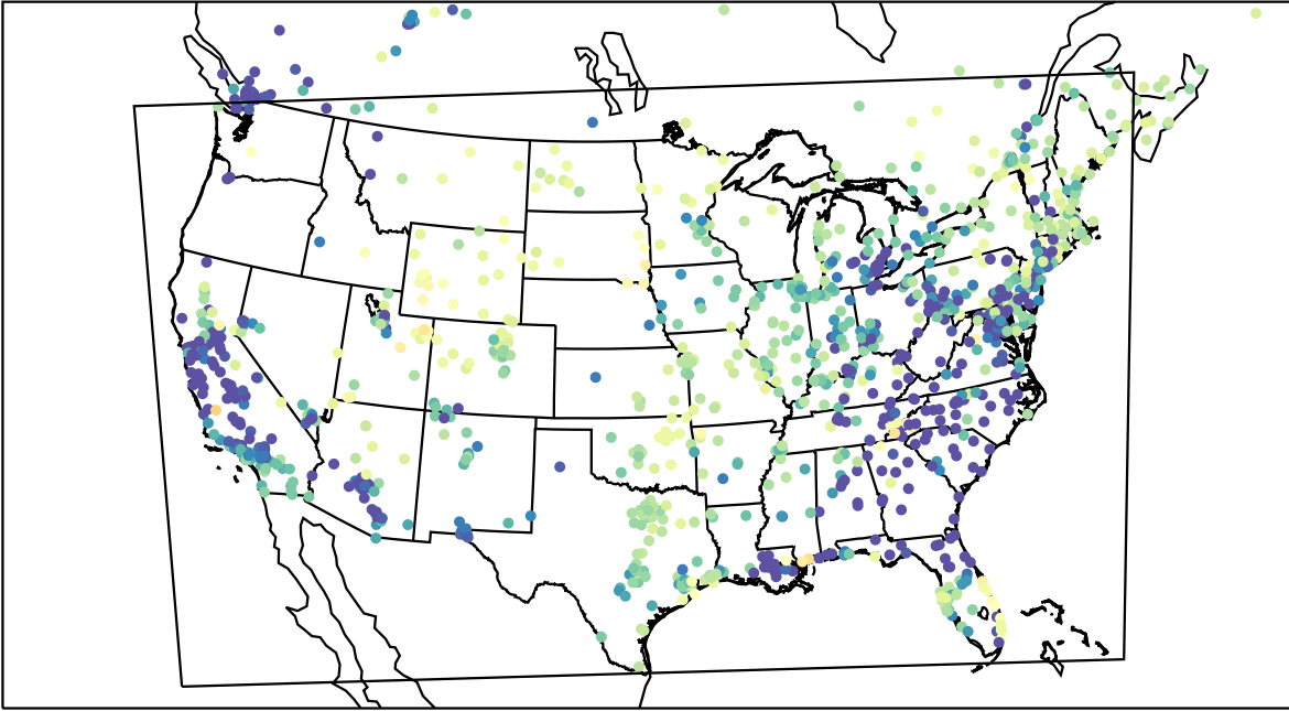
AirNOW (2023-03-16_10:00:00)
