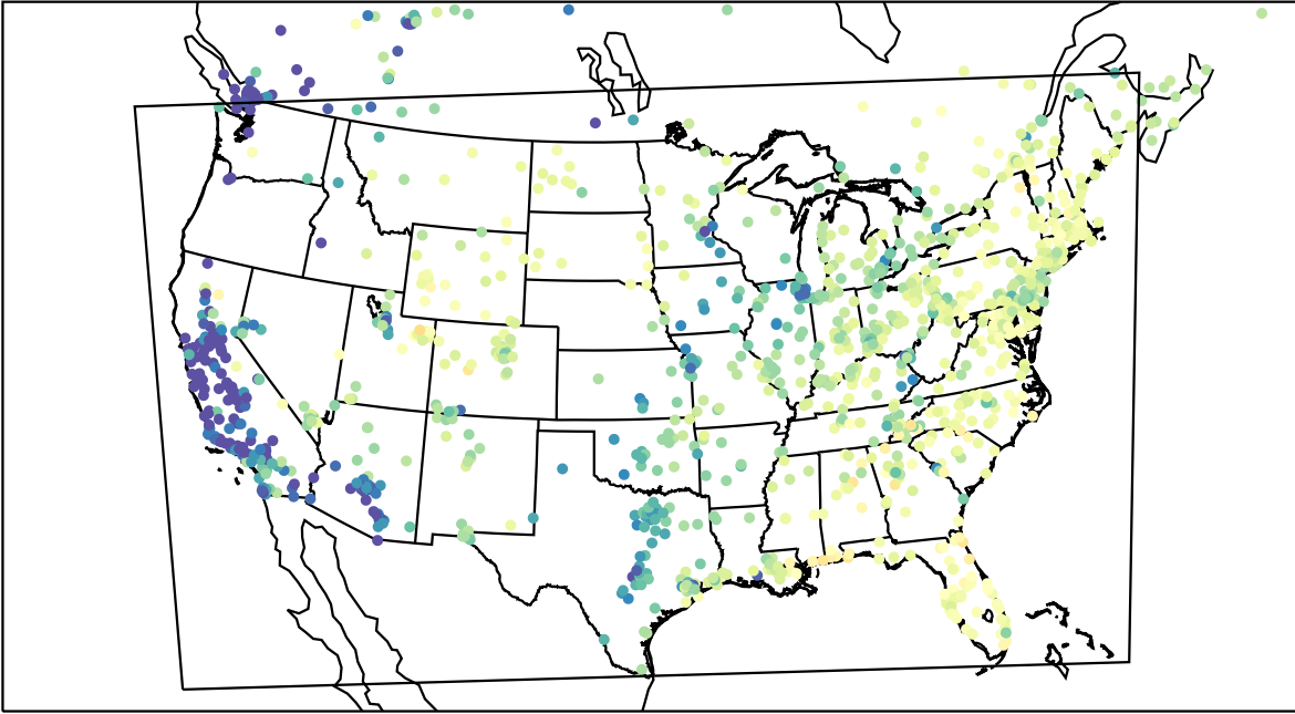
AirNOW (2023-03-16_15:00:00)
