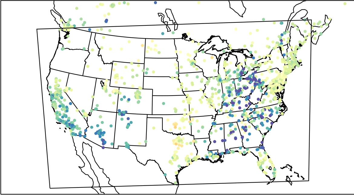
AirNOW (2023-03-16_01:00:00)
