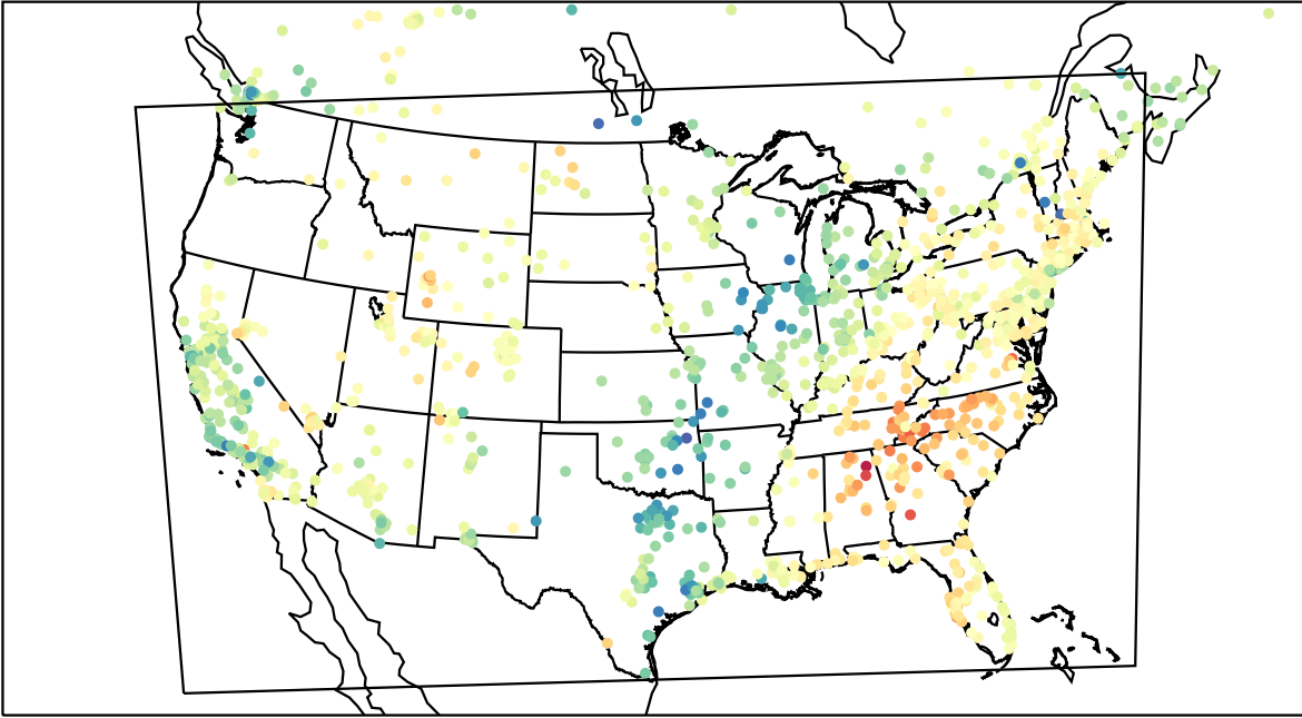
AirNOW (2023-03-16_22:00:00)
