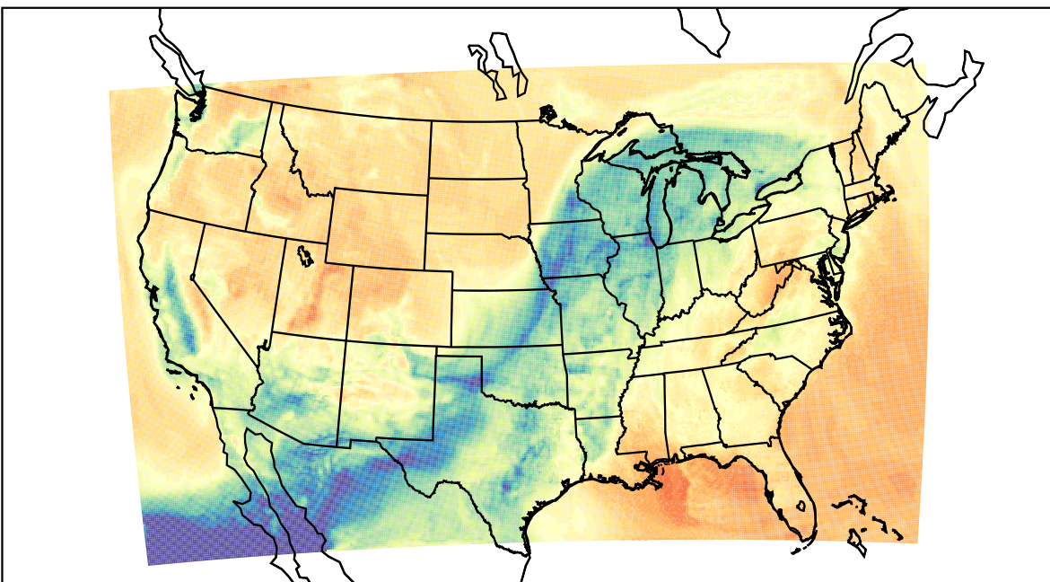
WRF (2023-03-16_17:00:00)
