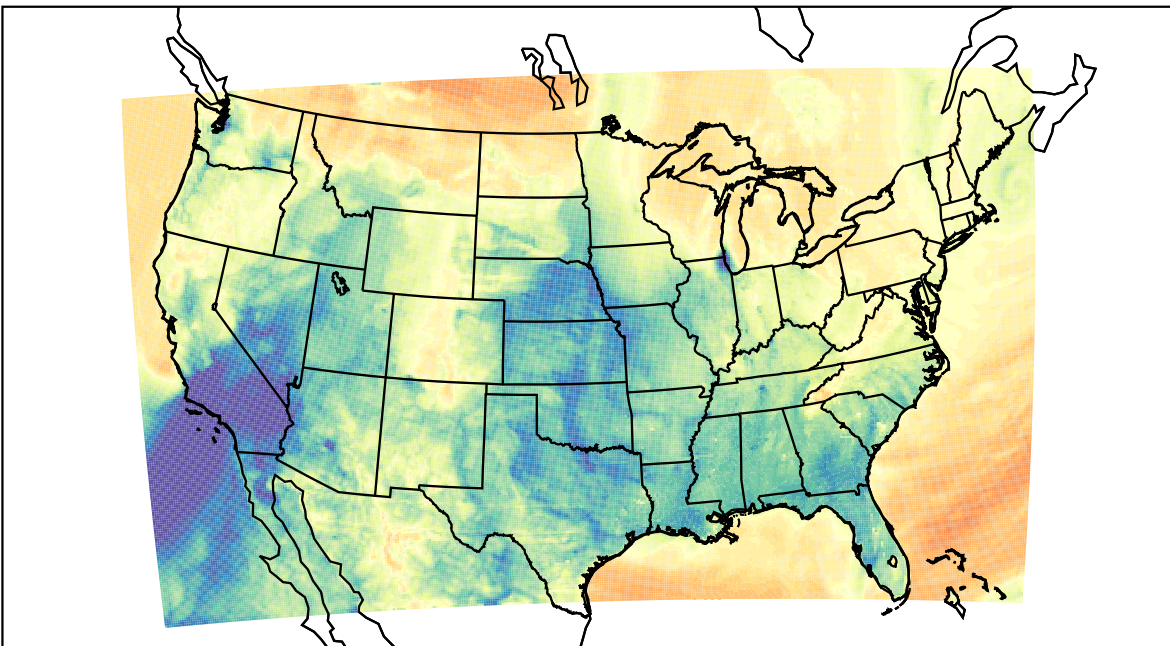
WRF (2023-03-15_09:00:00)
