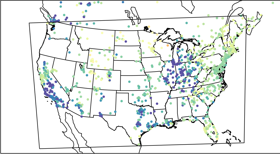
AirNOW (2023-03-15_06:00:00)
