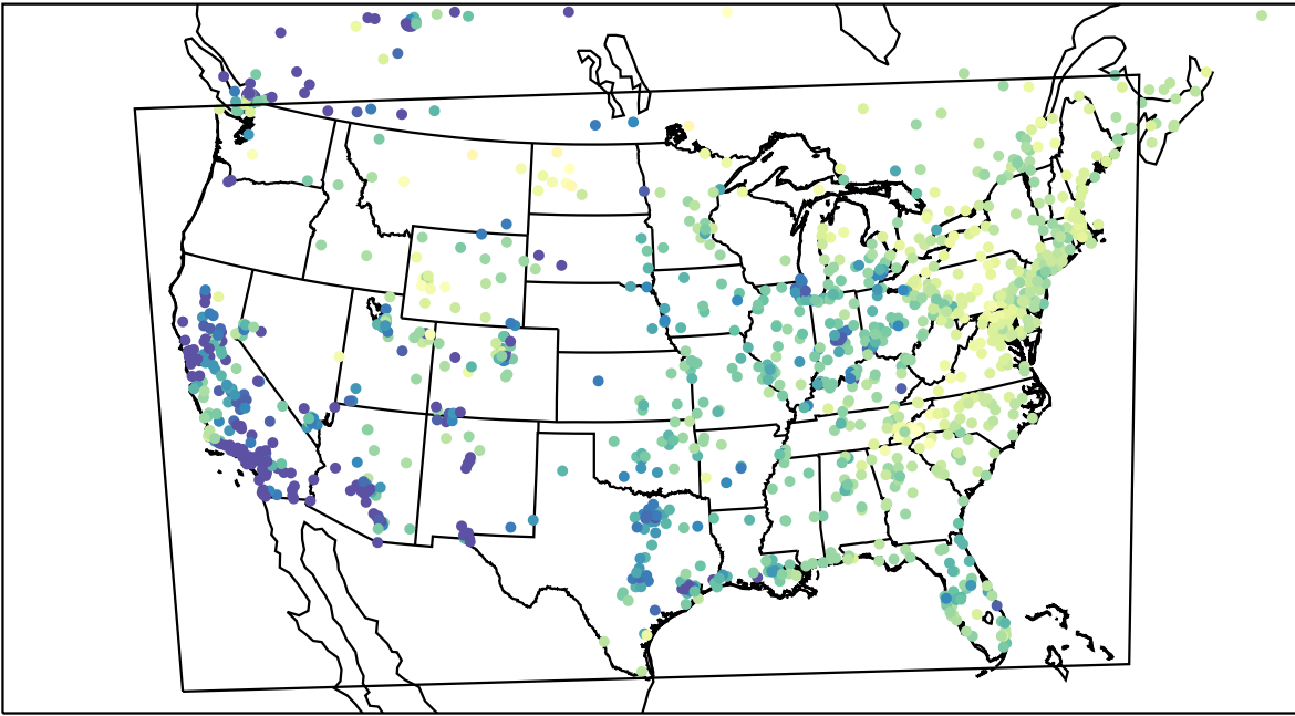
AirNOW (2023-03-15_14:00:00)
