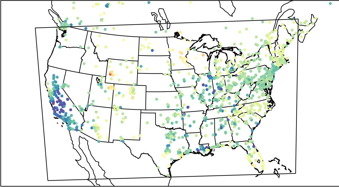
AirNOW (2023-03-15_01:00:00)
