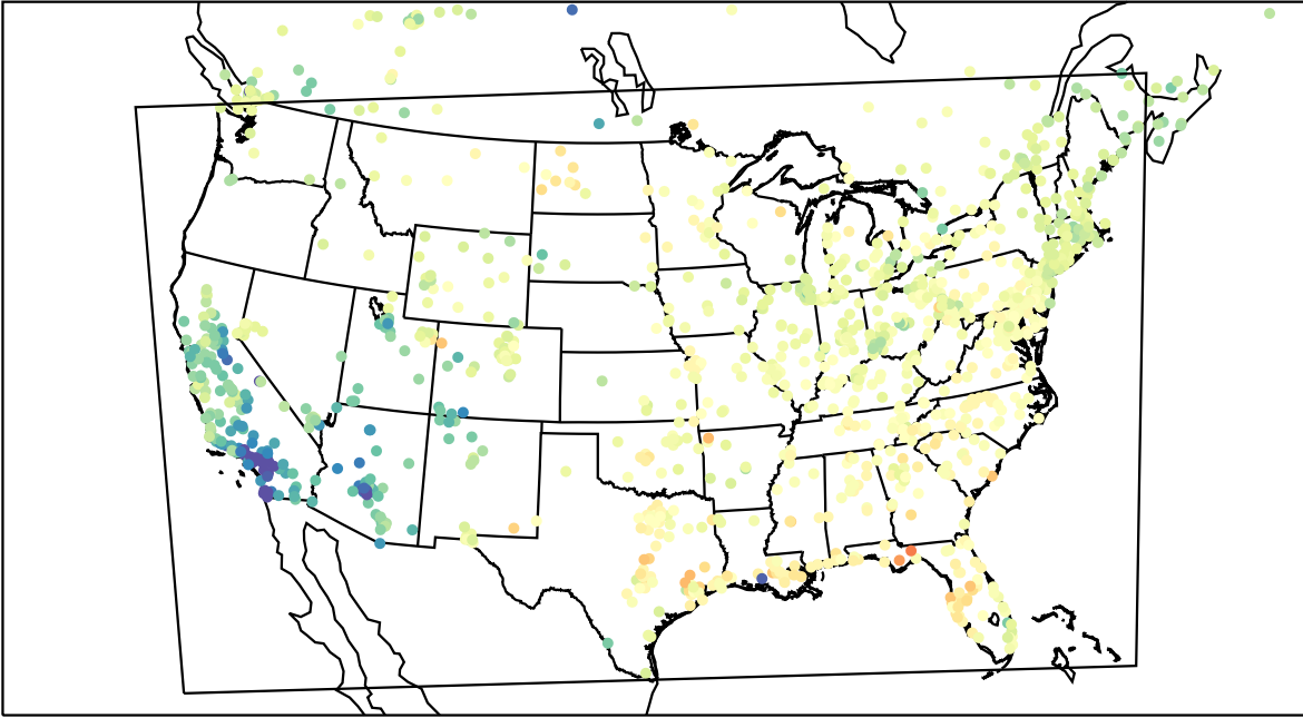
AirNOW (2023-03-15_20:00:00)
