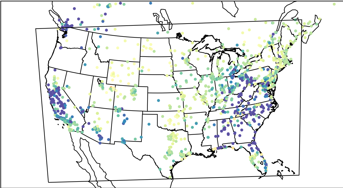
AirNOW (2023-03-16_07:00:00)
