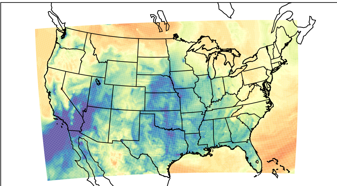
WRF (2023-03-15_13:00:00)
