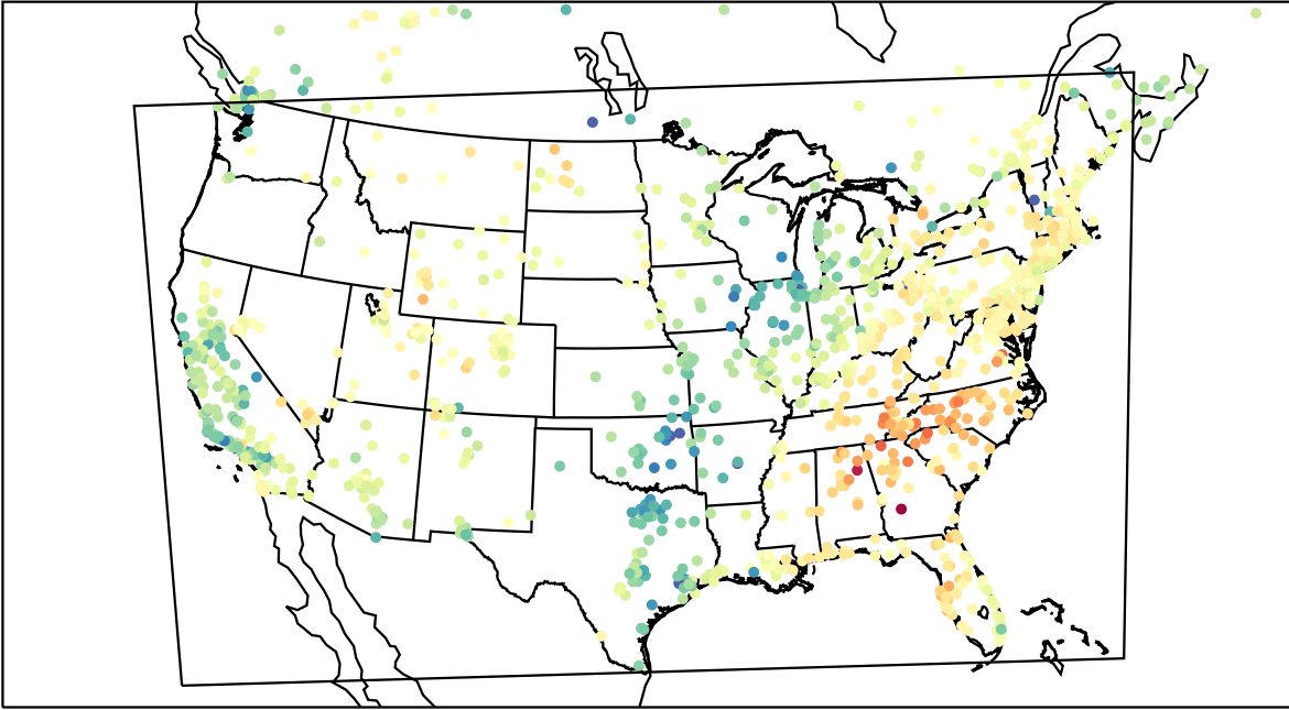
AirNOW (2023-03-16_21:00:00)
