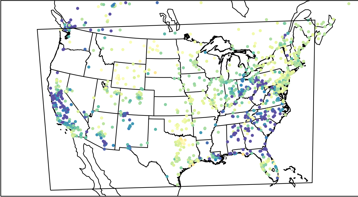
AirNOW (2023-03-16_05:00:00)
