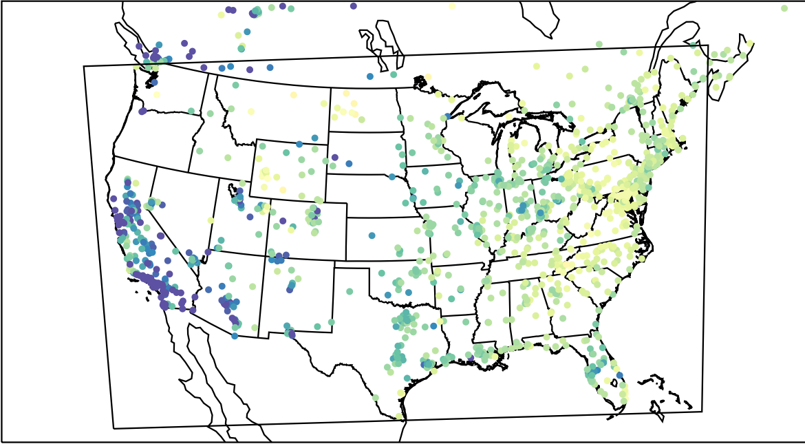
AirNOW (2023-03-15_15:00:00)
