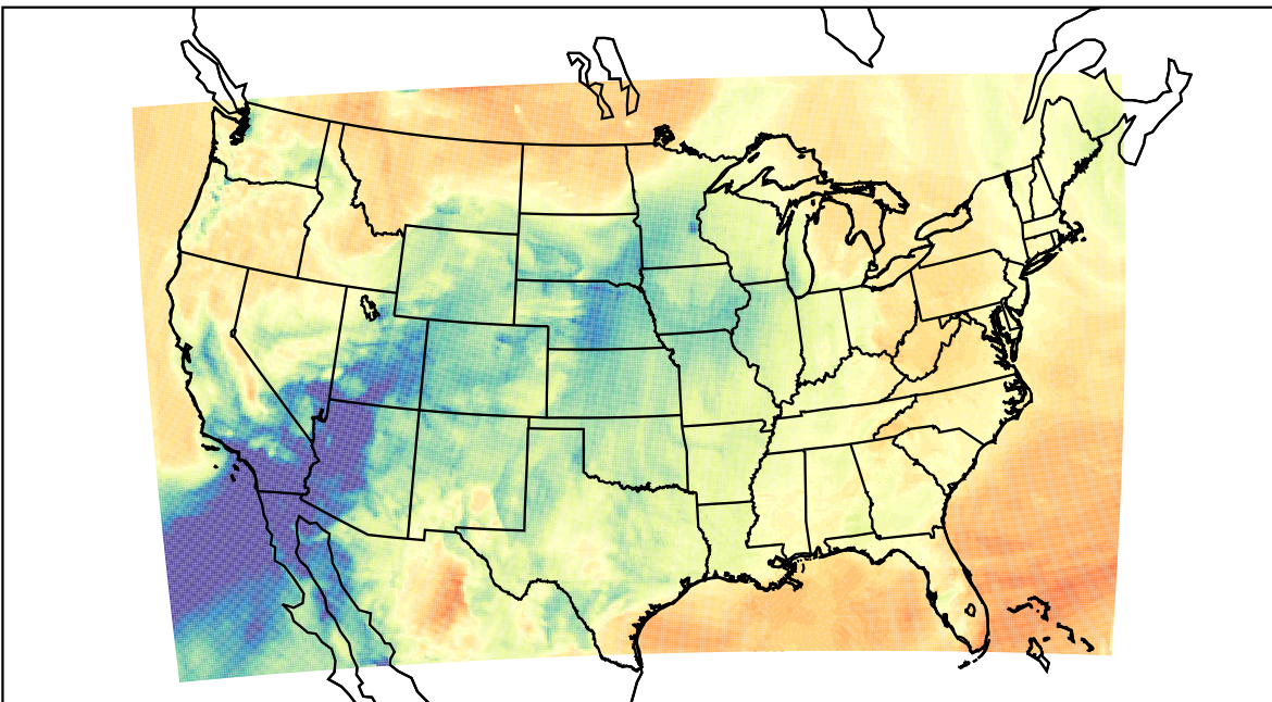
WRF (2023-03-15_17:00:00)
