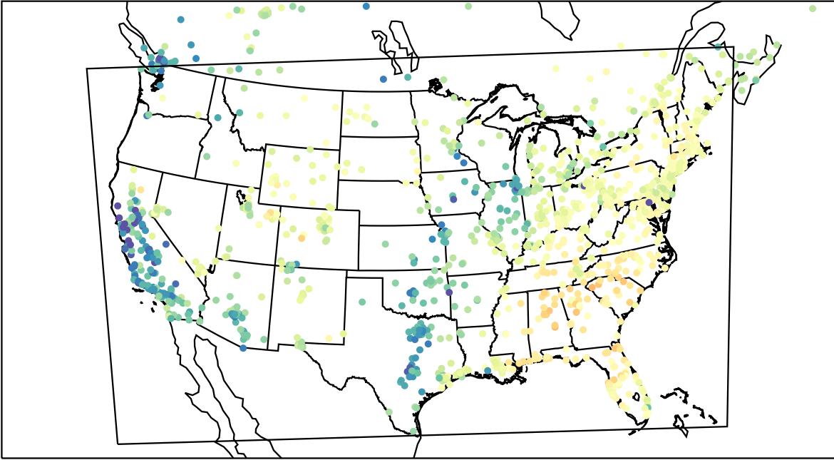
AirNOW (2023-03-16_17:00:00)
