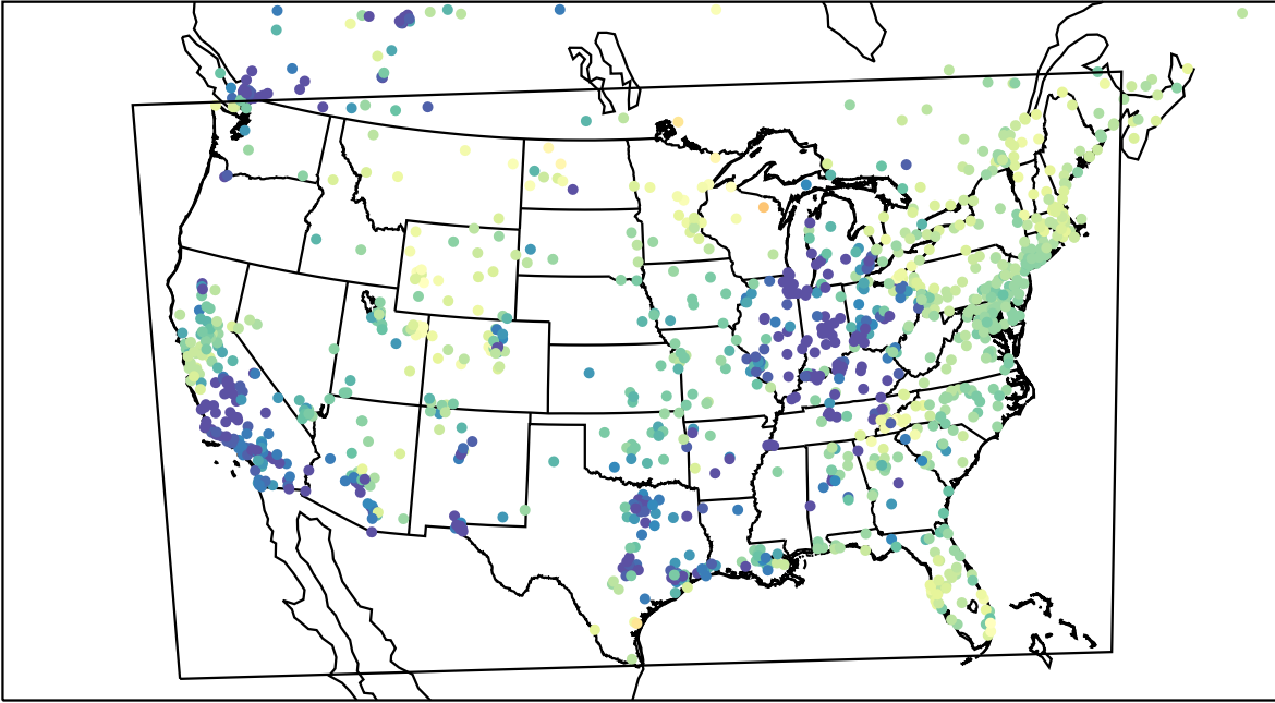
AirNOW (2023-03-15_07:00:00)
