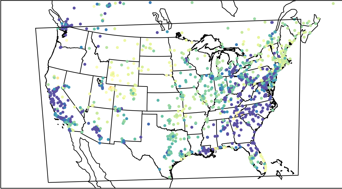
AirNOW (2023-03-16_12:00:00)
