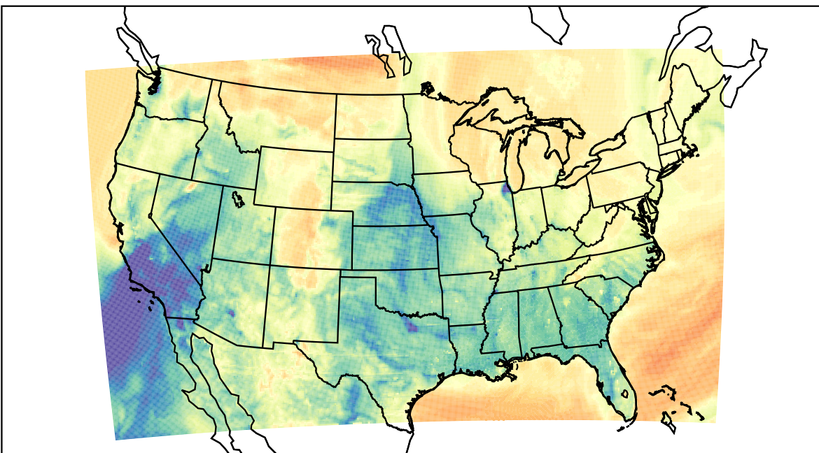
WRF (2023-03-15_06:00:00)
