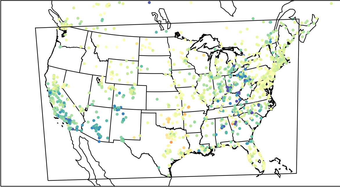
AirNOW (2023-03-16_00:00:00)
