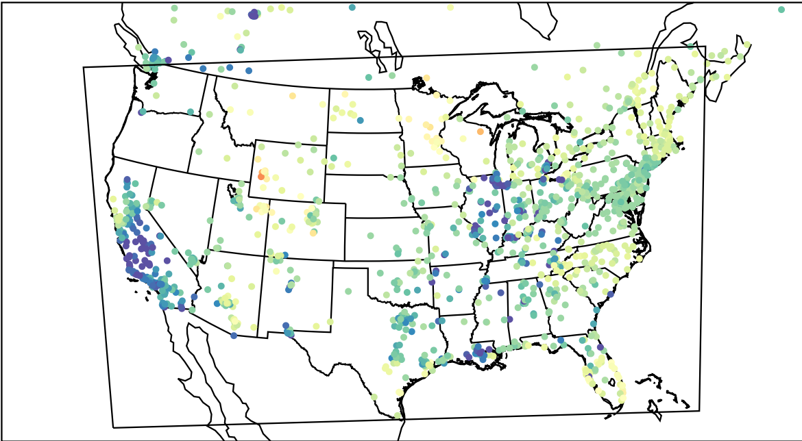
AirNOW (2023-03-15_02:00:00)
