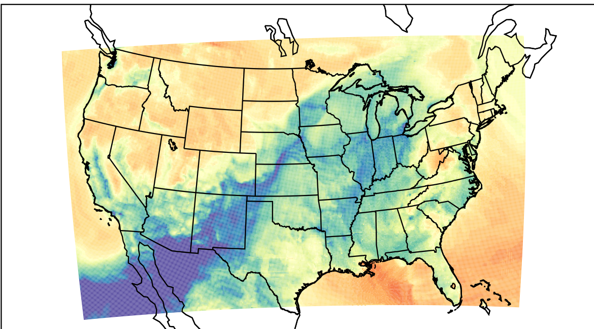
WRF (2023-03-16_09:00:00)
