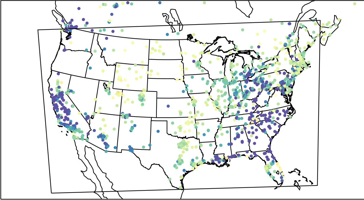
AirNOW (2023-03-16_09:00:00)
