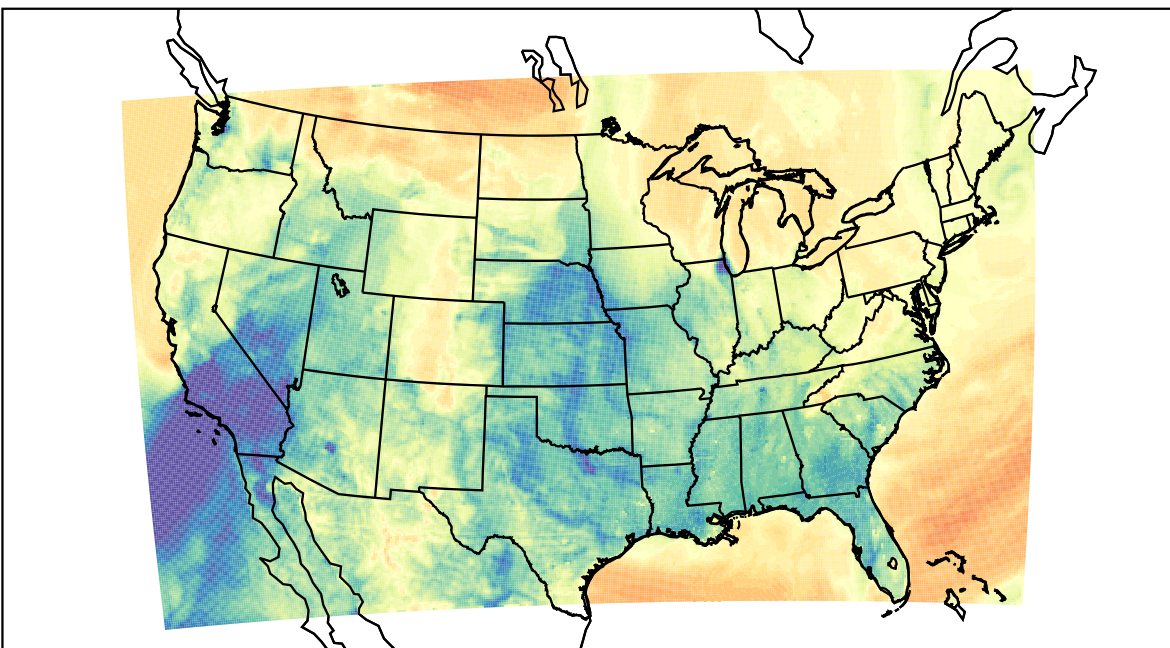
WRF (2023-03-15_08:00:00)
