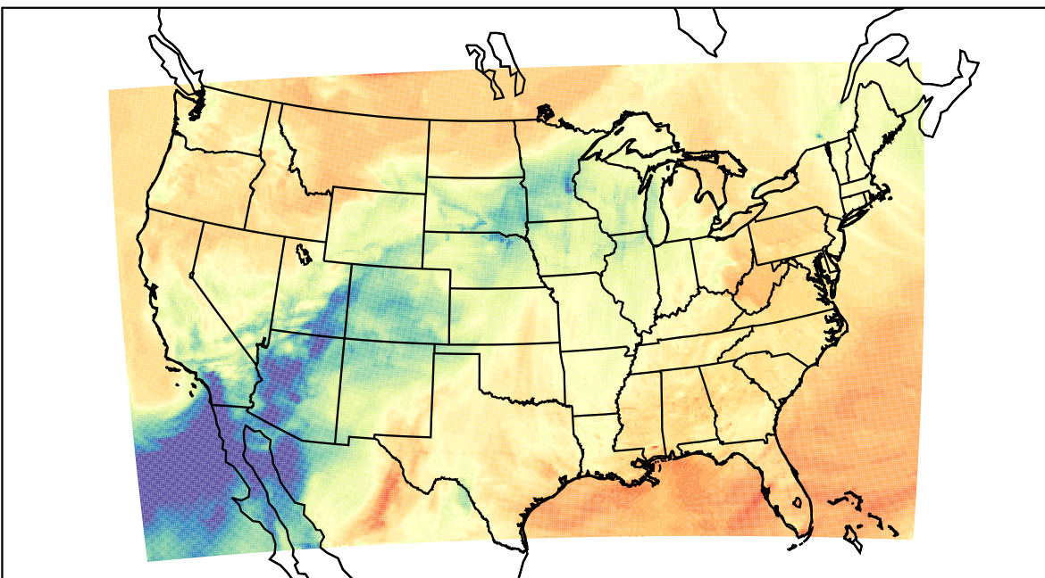
WRF (2023-03-15_21:00:00)
