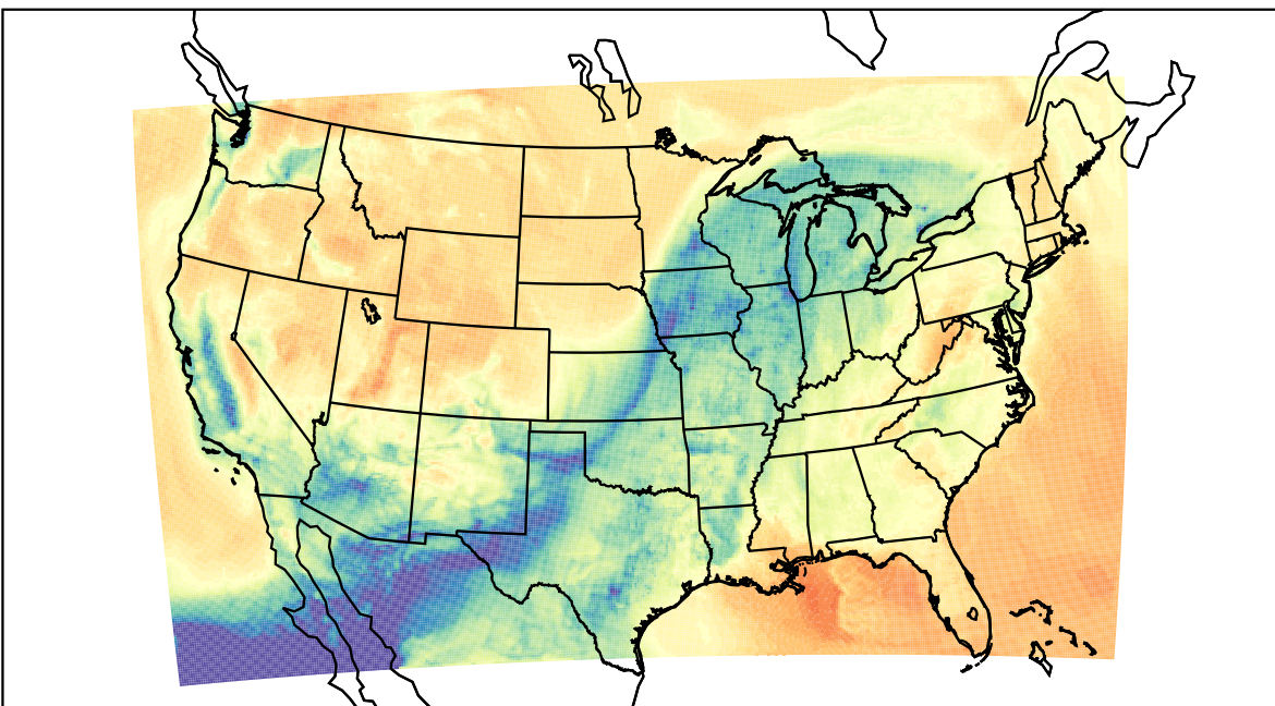
WRF (2023-03-16_16:00:00)
