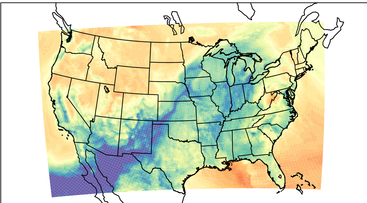
WRF (2023-03-16_11:00:00)
