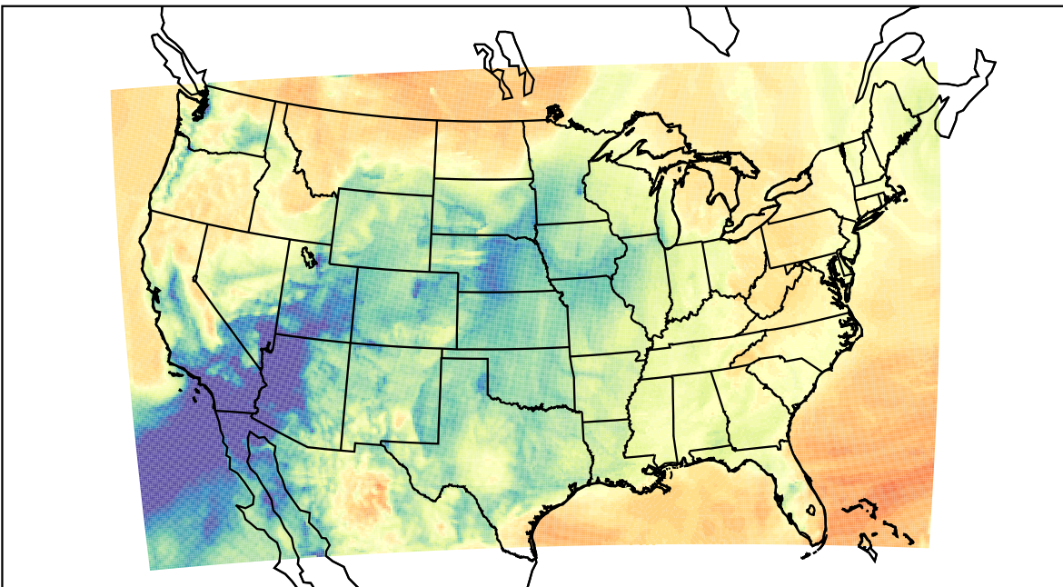
WRF (2023-03-15_16:00:00)
