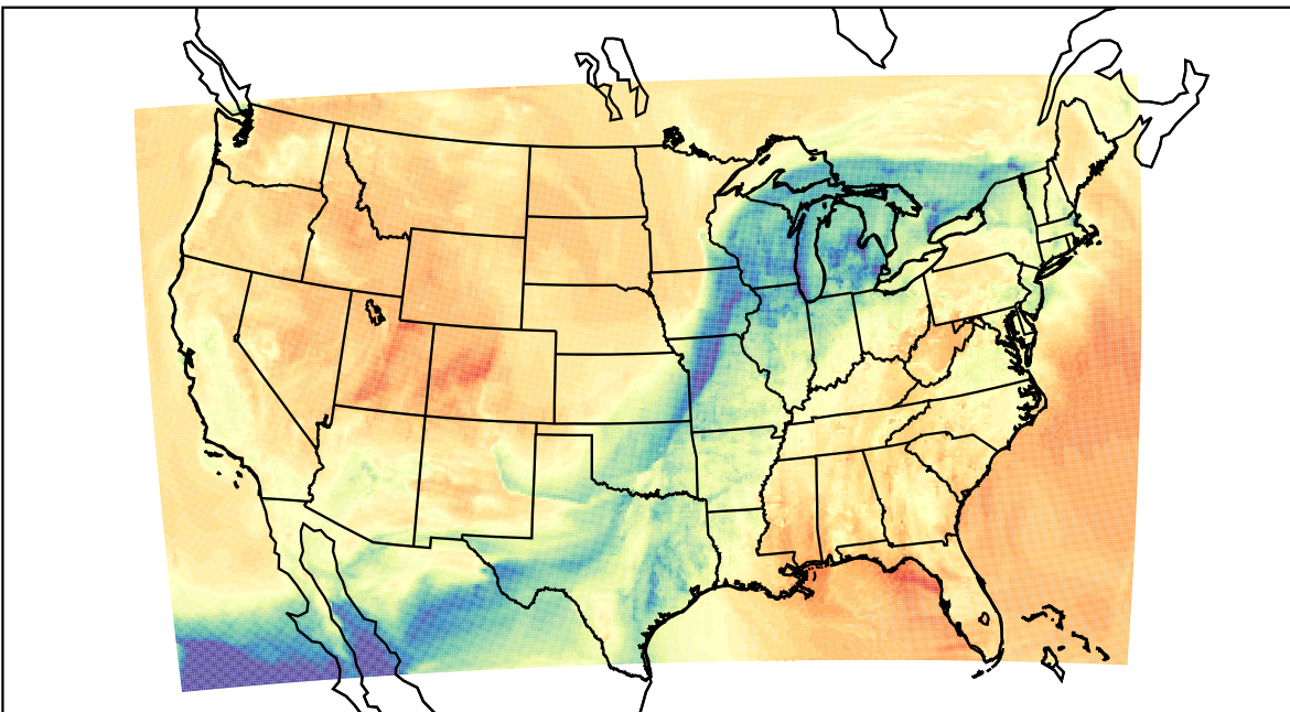
WRF (2023-03-16_22:00:00)
