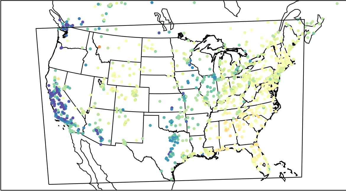
AirNOW (2023-03-16_16:00:00)
