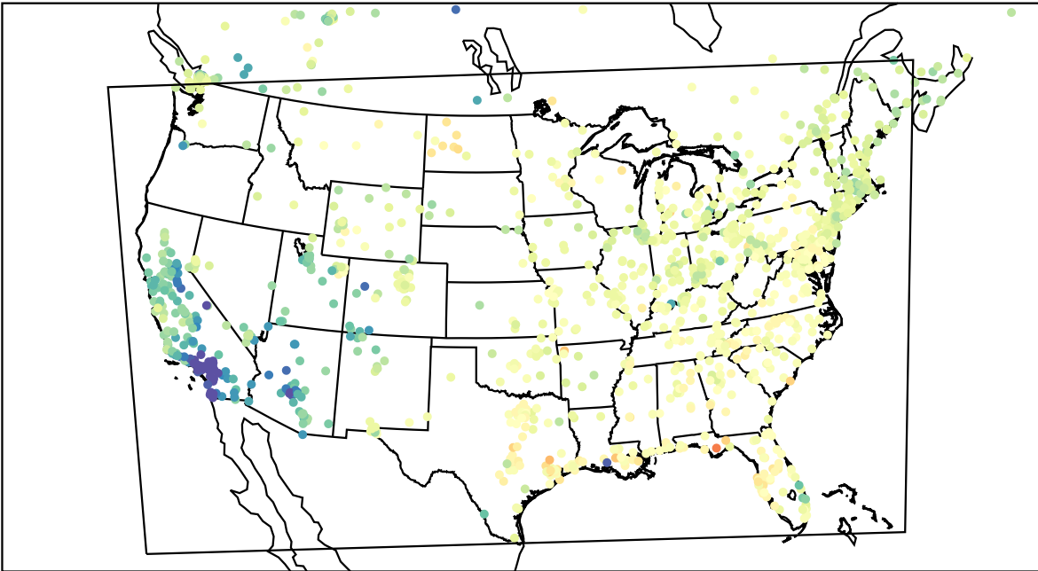
AirNOW (2023-03-15_19:00:00)
