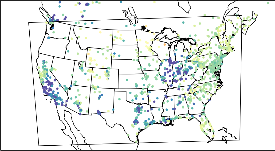
AirNOW (2023-03-15_05:00:00)
