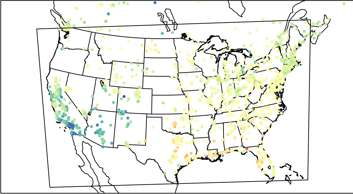
AirNOW (2023-03-15_22:00:00)
