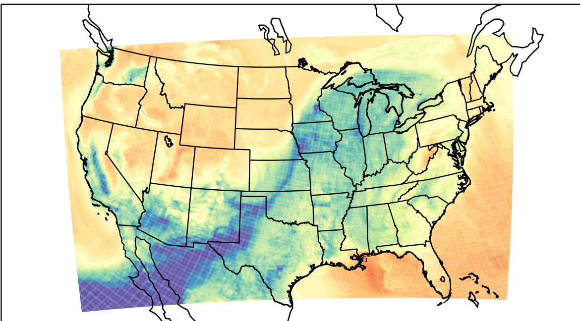
WRF (2023-03-16_15:00:00)
