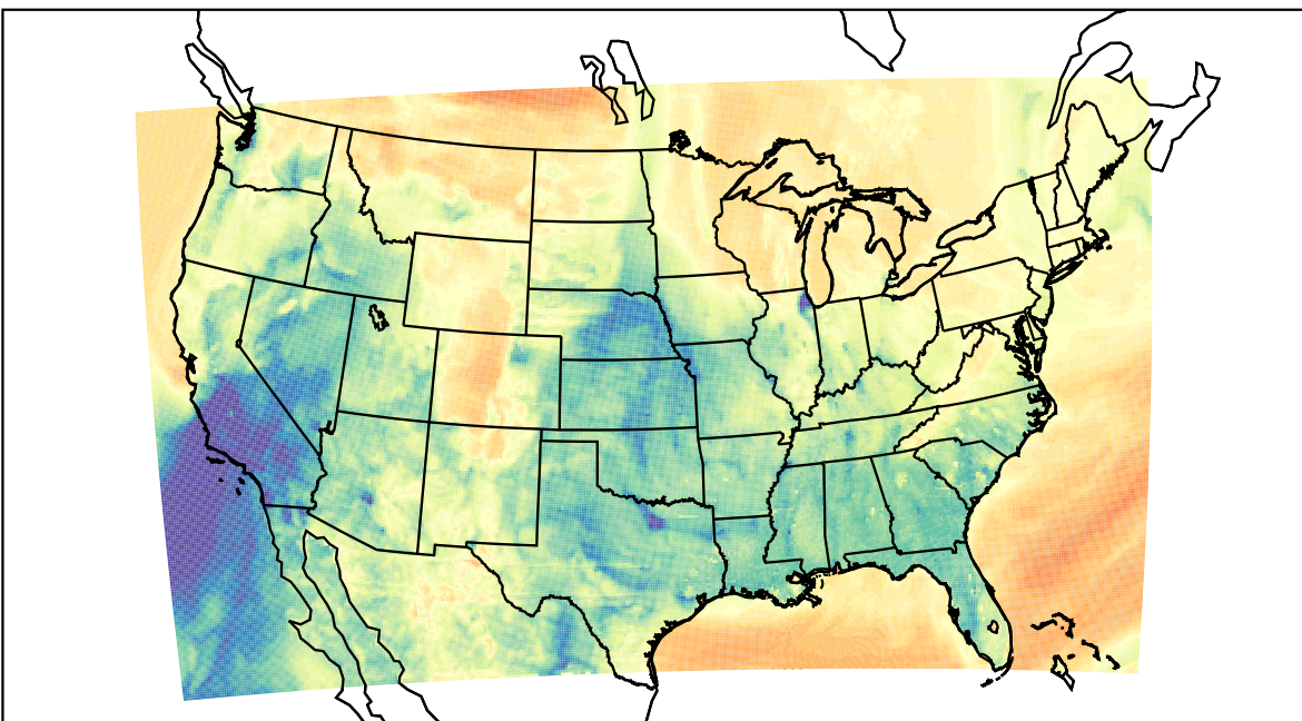
WRF (2023-03-15_05:00:00)
