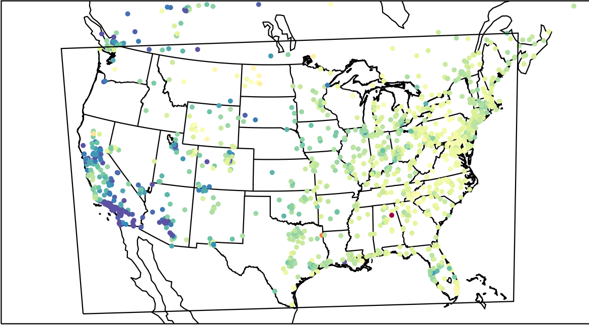
AirNOW (2023-03-15_16:00:00)
