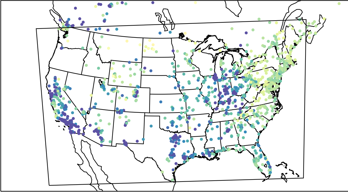
AirNOW (2023-03-15_13:00:00)
