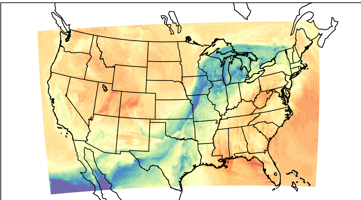
WRF (2023-03-16_21:00:00)
