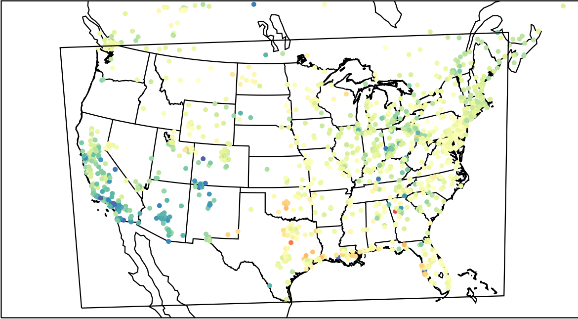
AirNOW (2023-03-15_23:00:00)
