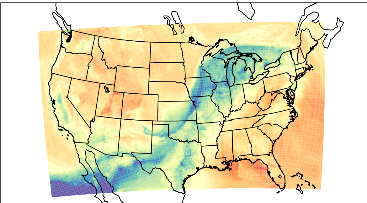
WRF (2023-03-16_19:00:00)
