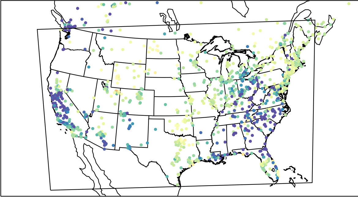
AirNOW (2023-03-16_06:00:00)
