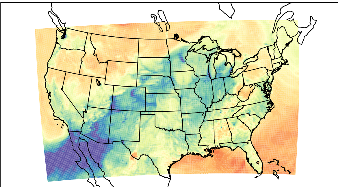
WRF (2023-03-16_02:00:00)
