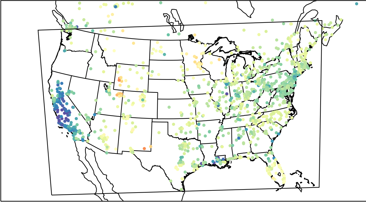
AirNOW (2023-03-15_00:00:00)
