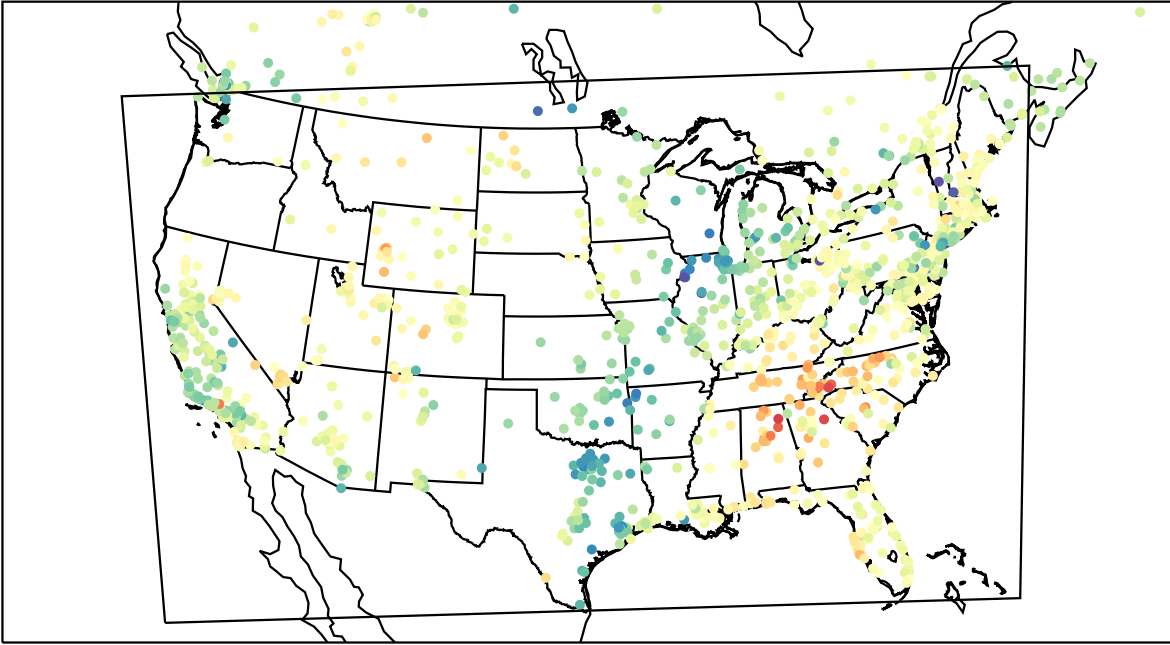
AirNOW (2023-03-16_23:00:00)
