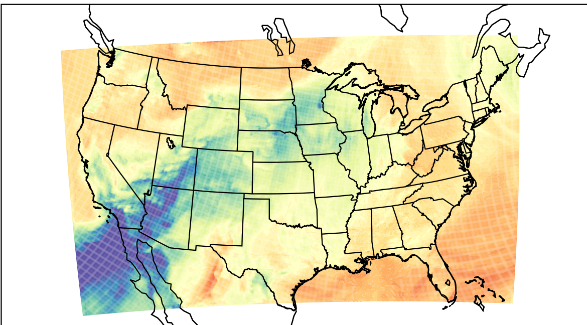
WRF (2023-03-15_19:00:00)
