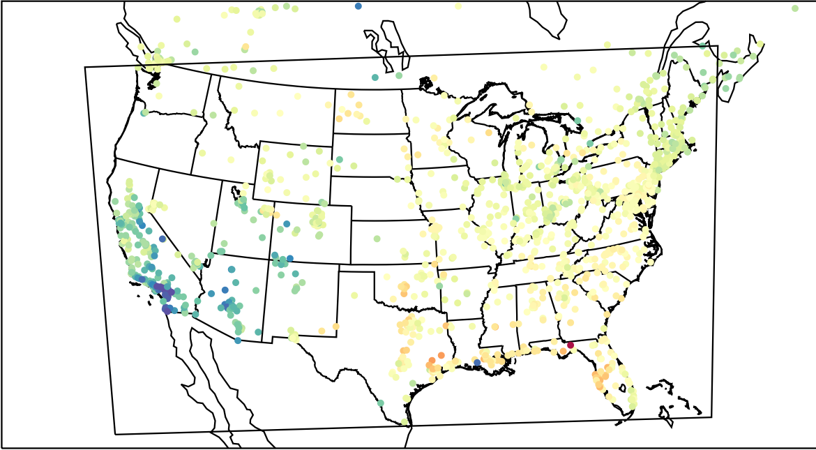
AirNOW (2023-03-15_21:00:00)
