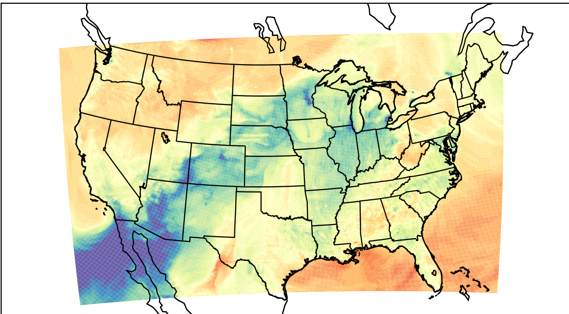
WRF (2023-03-16_00:00:00)
