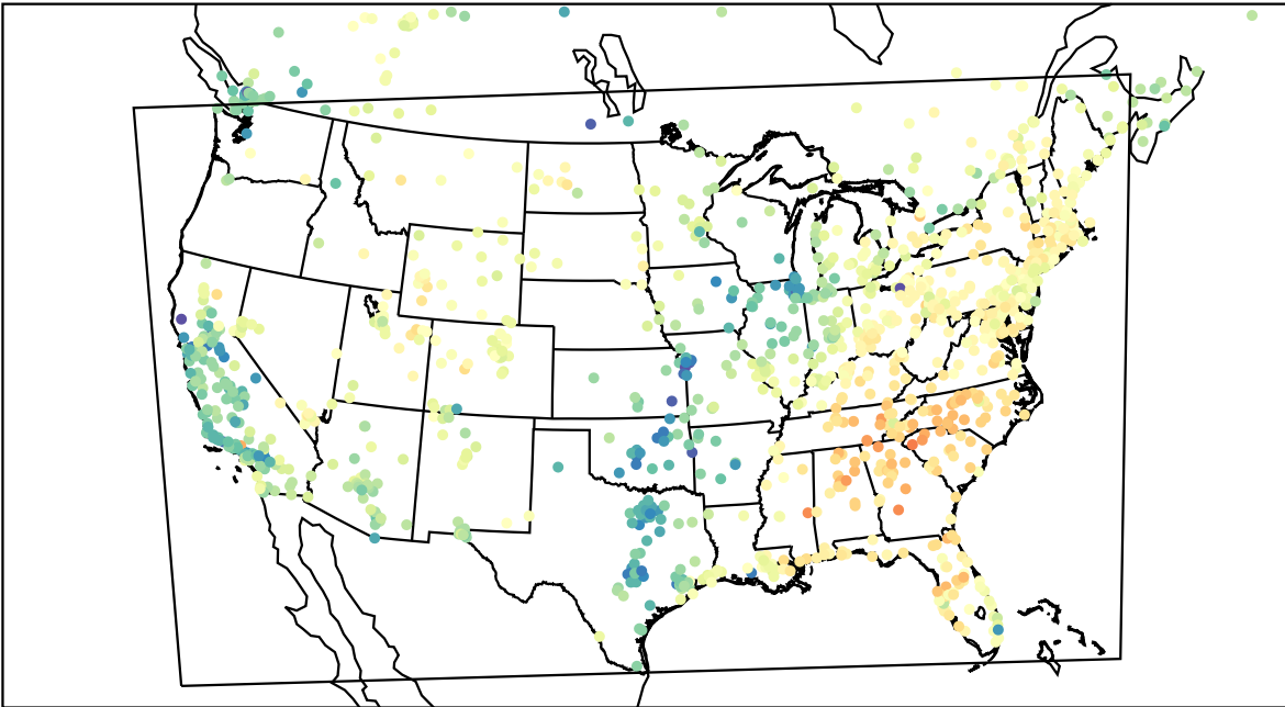
AirNOW (2023-03-16_19:00:00)
