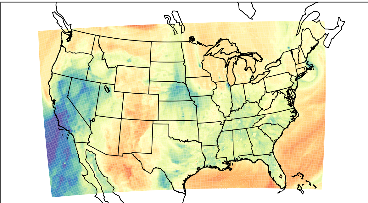
WRF (2023-03-15_00:00:00)
