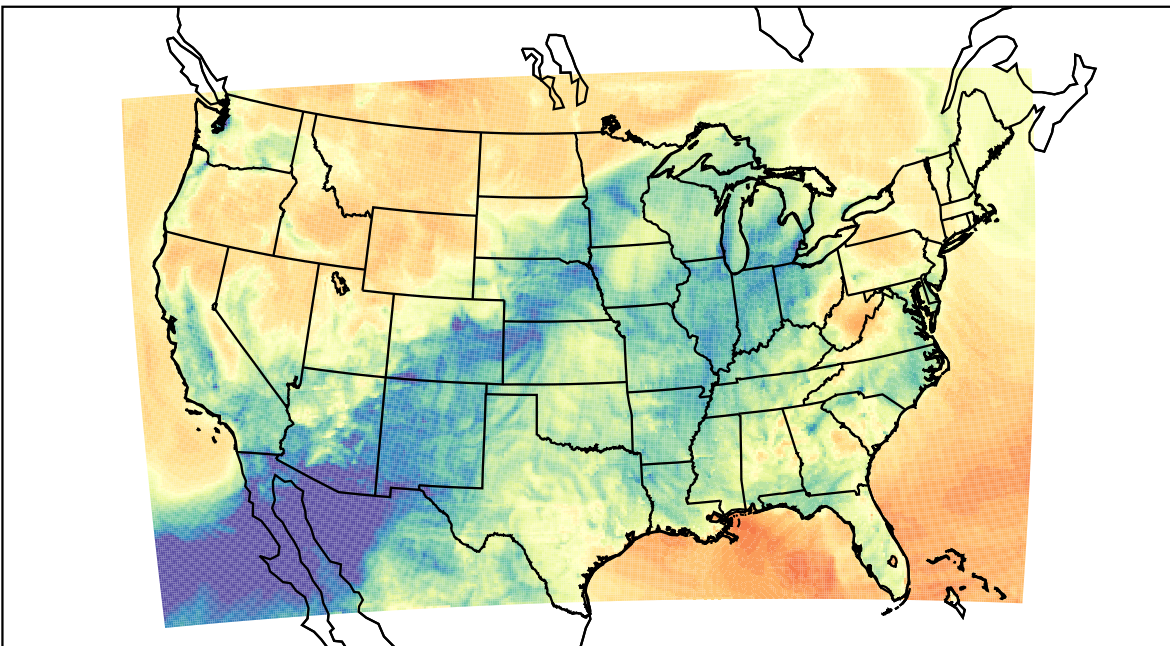
WRF (2023-03-16_05:00:00)
