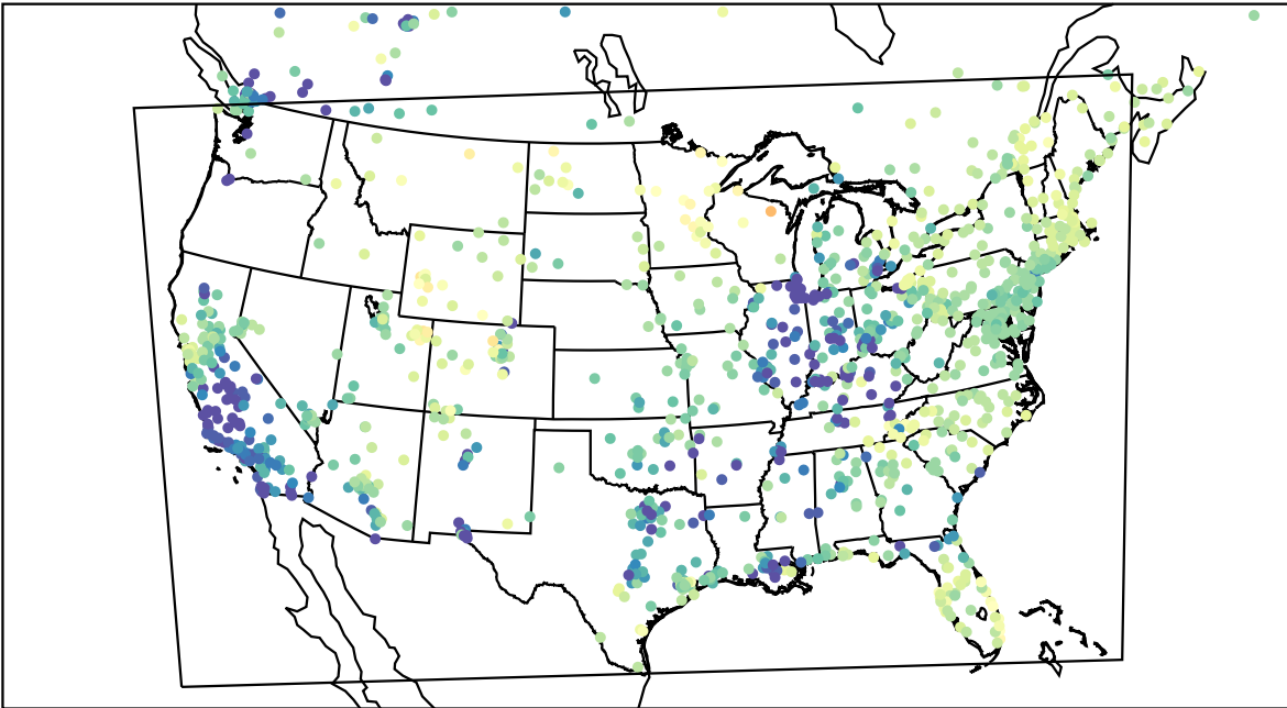
AirNOW (2023-03-15_04:00:00)
