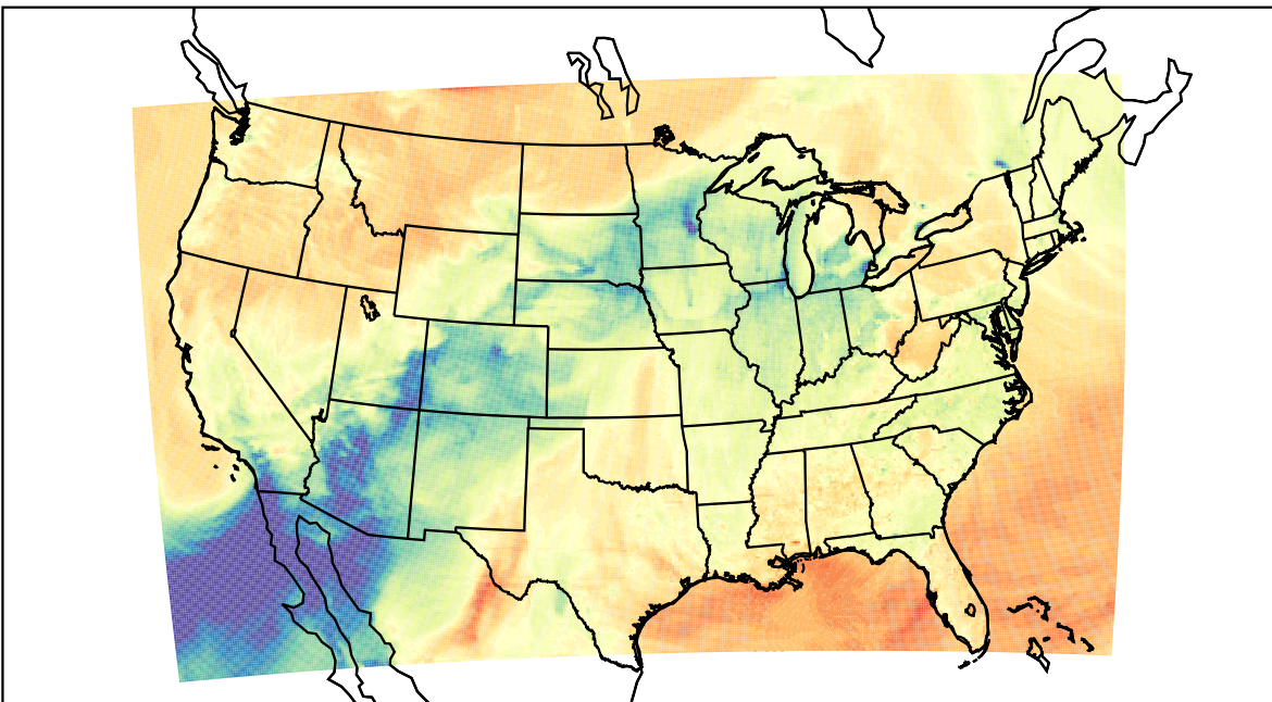
WRF (2023-03-15_23:00:00)
