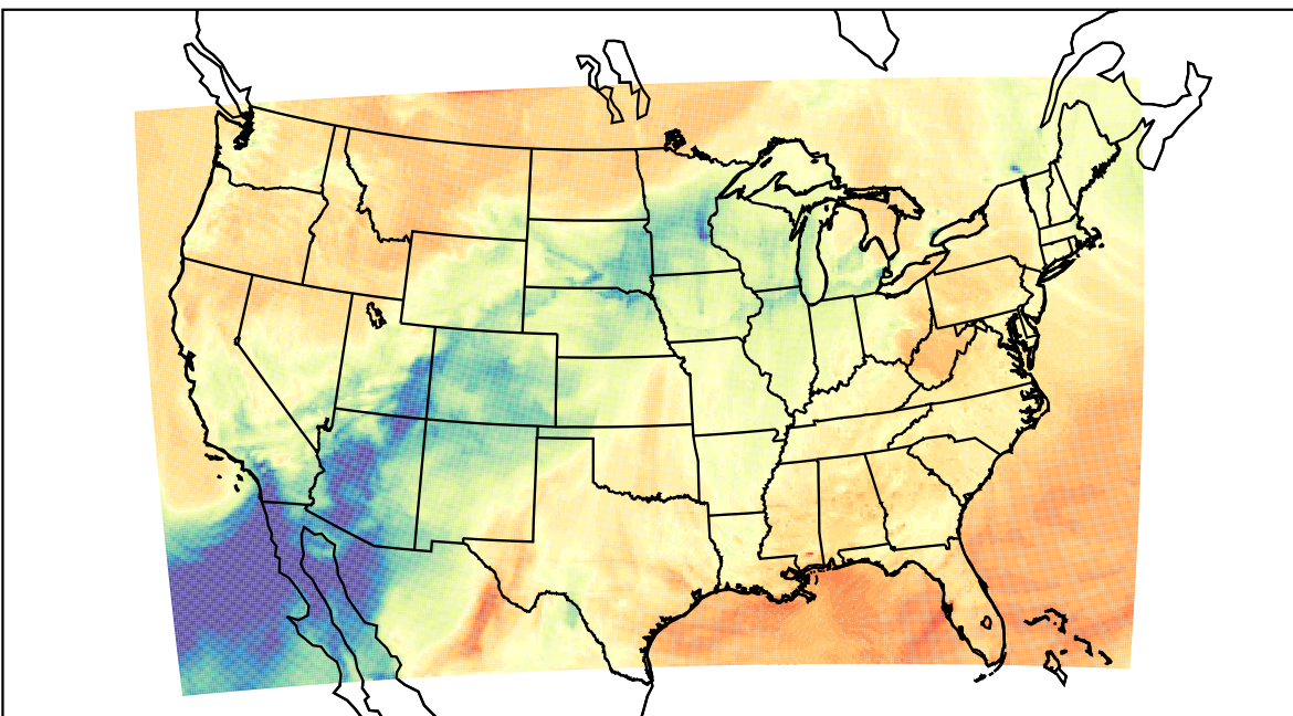
WRF (2023-03-15_22:00:00)
