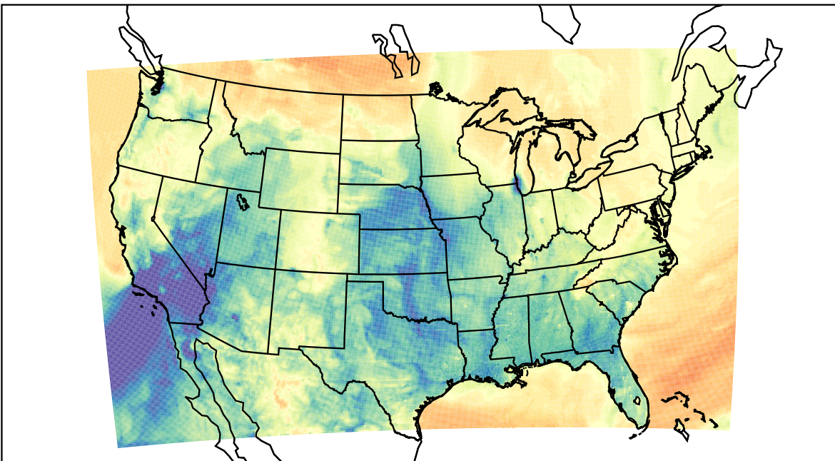
WRF (2023-03-15_10:00:00)
