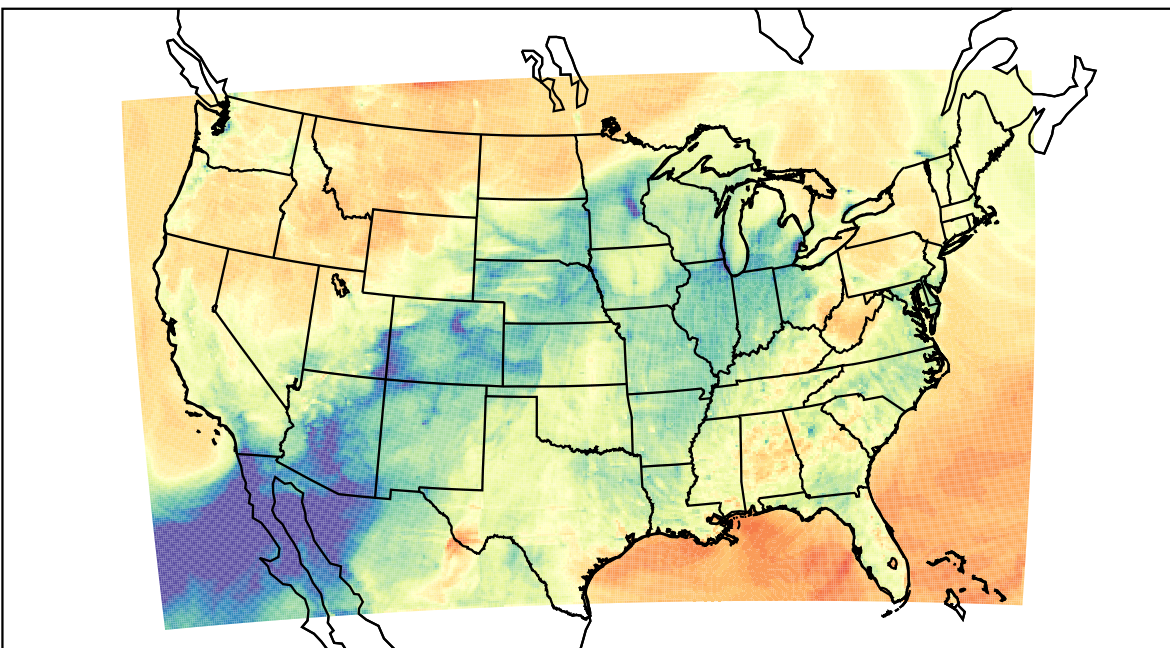
WRF (2023-03-16_01:00:00)
