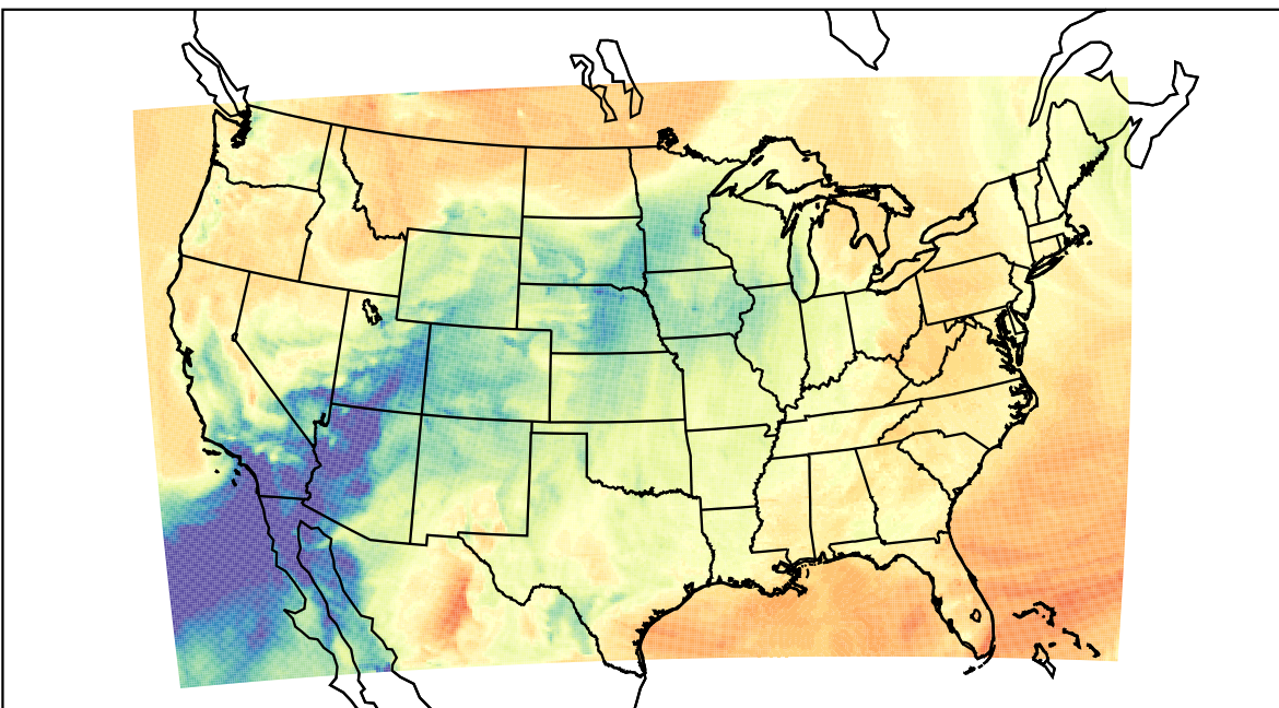
WRF (2023-03-15_18:00:00)
