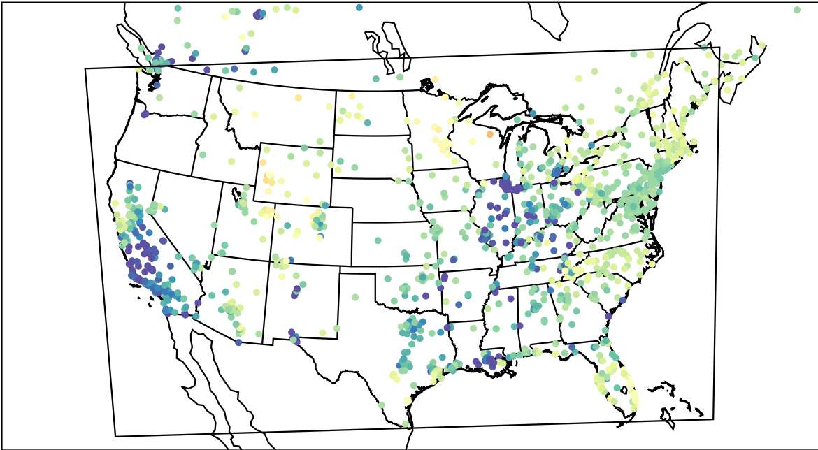
AirNOW (2023-03-15_03:00:00)
