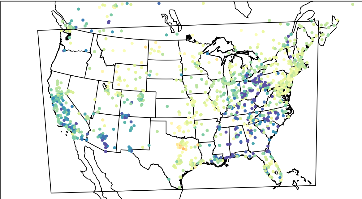
AirNOW (2023-03-16_02:00:00)
