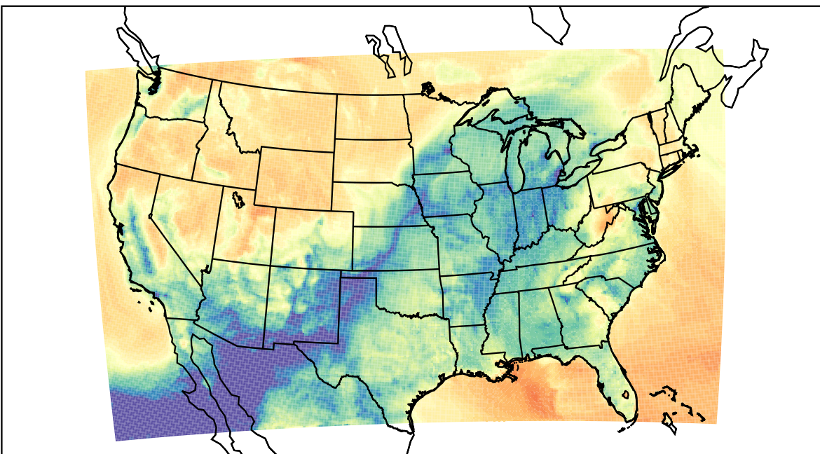
WRF (2023-03-16_12:00:00)
