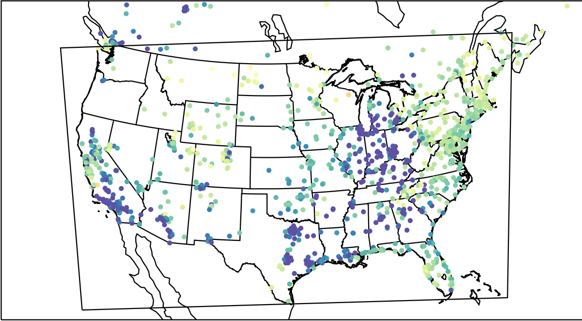
AirNOW (2023-03-15_10:00:00)
