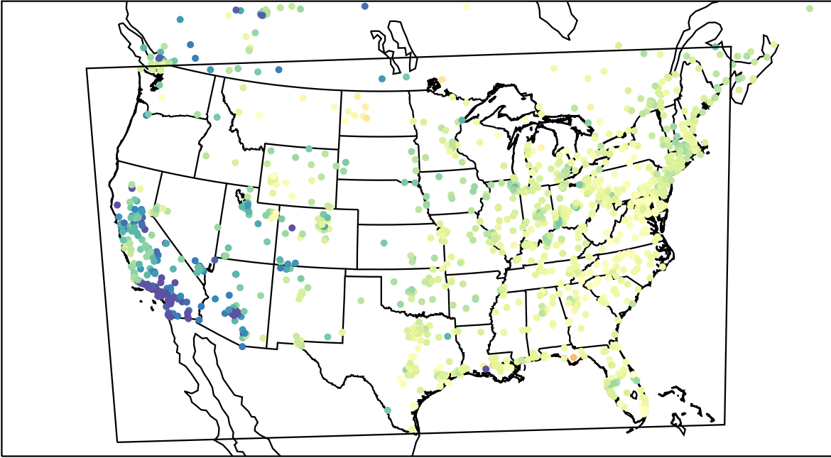
AirNOW (2023-03-15_17:00:00)
