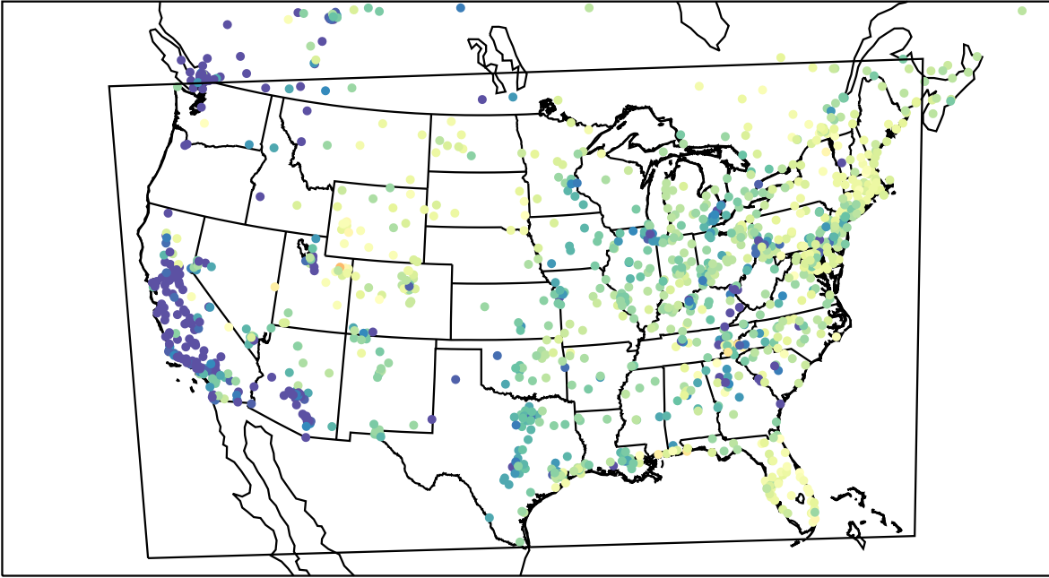
AirNOW (2023-03-16_14:00:00)
