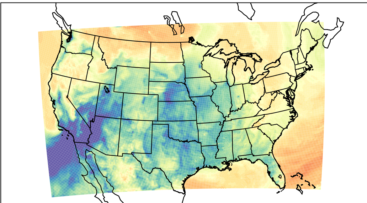
WRF (2023-03-15_14:00:00)
