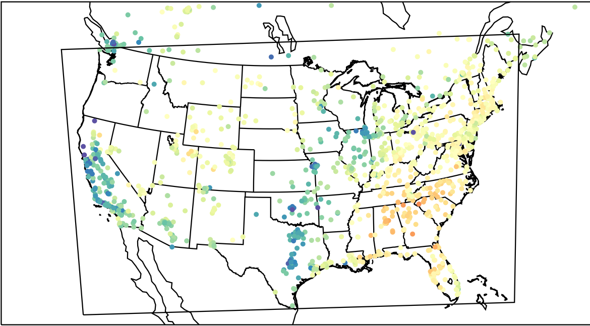
AirNOW (2023-03-16_18:00:00)
