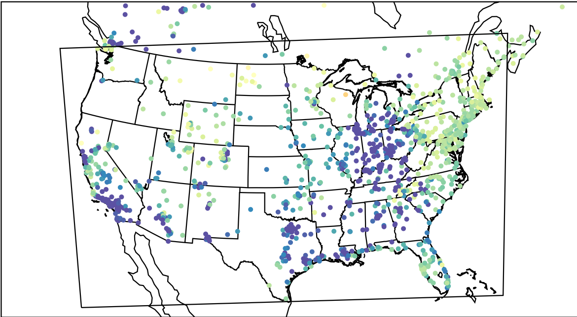
AirNOW (2023-03-15_12:00:00)
