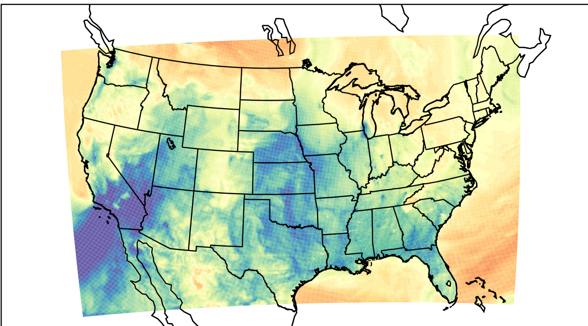
WRF (2023-03-15_11:00:00)
