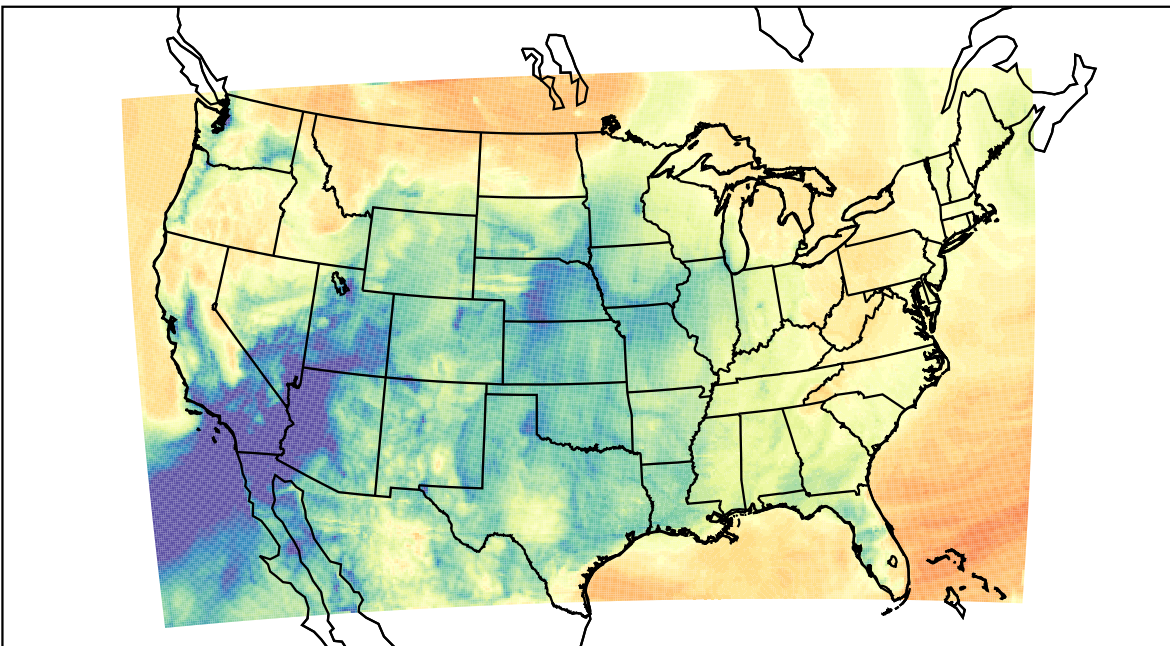
WRF (2023-03-15_15:00:00)
