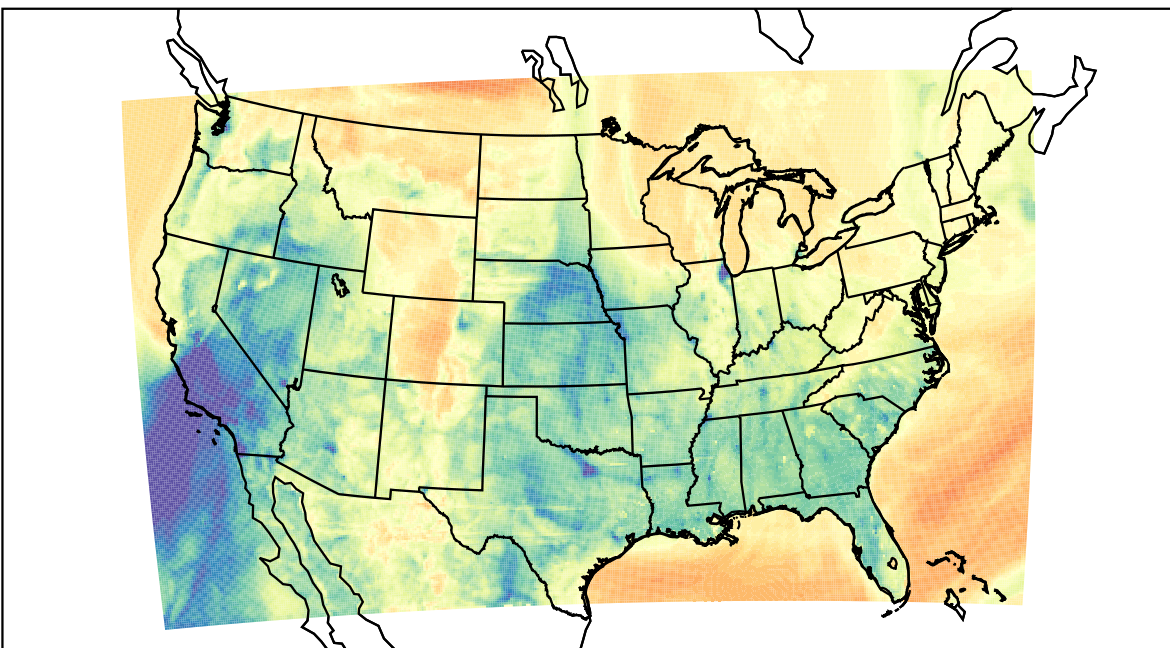
WRF (2023-03-15_04:00:00)
