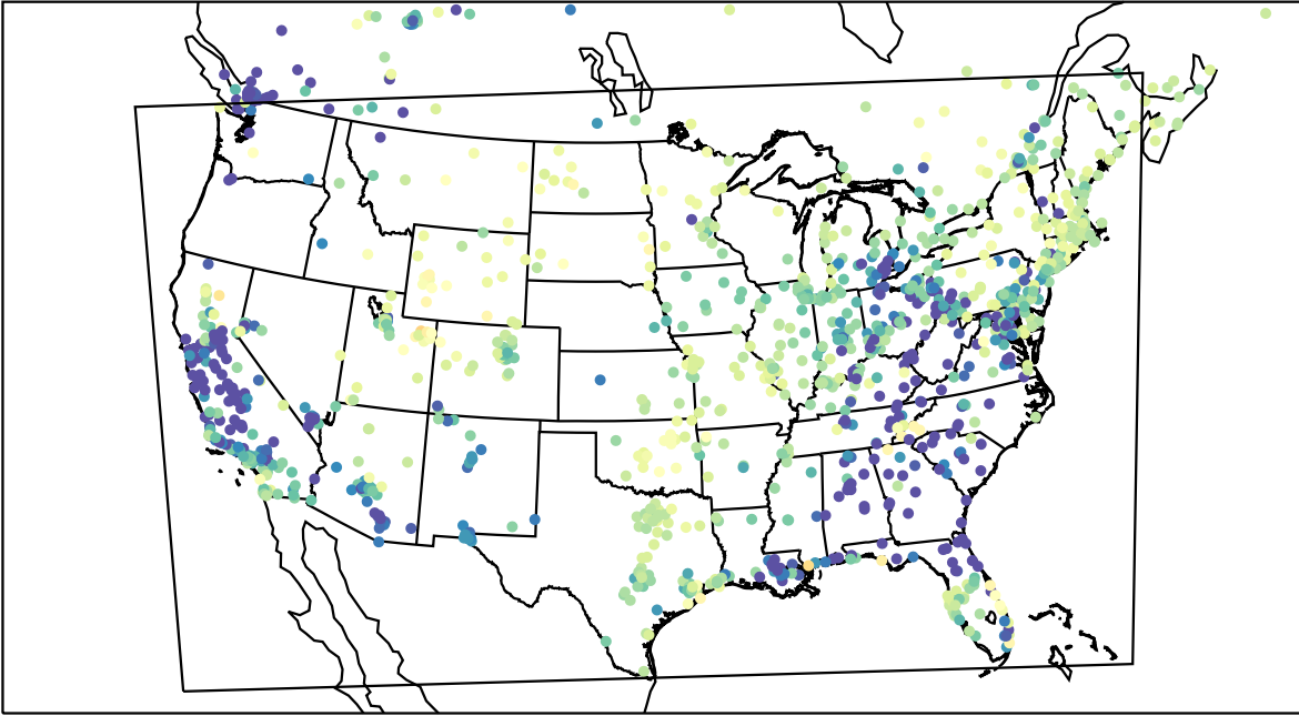
AirNOW (2023-03-16_08:00:00)
