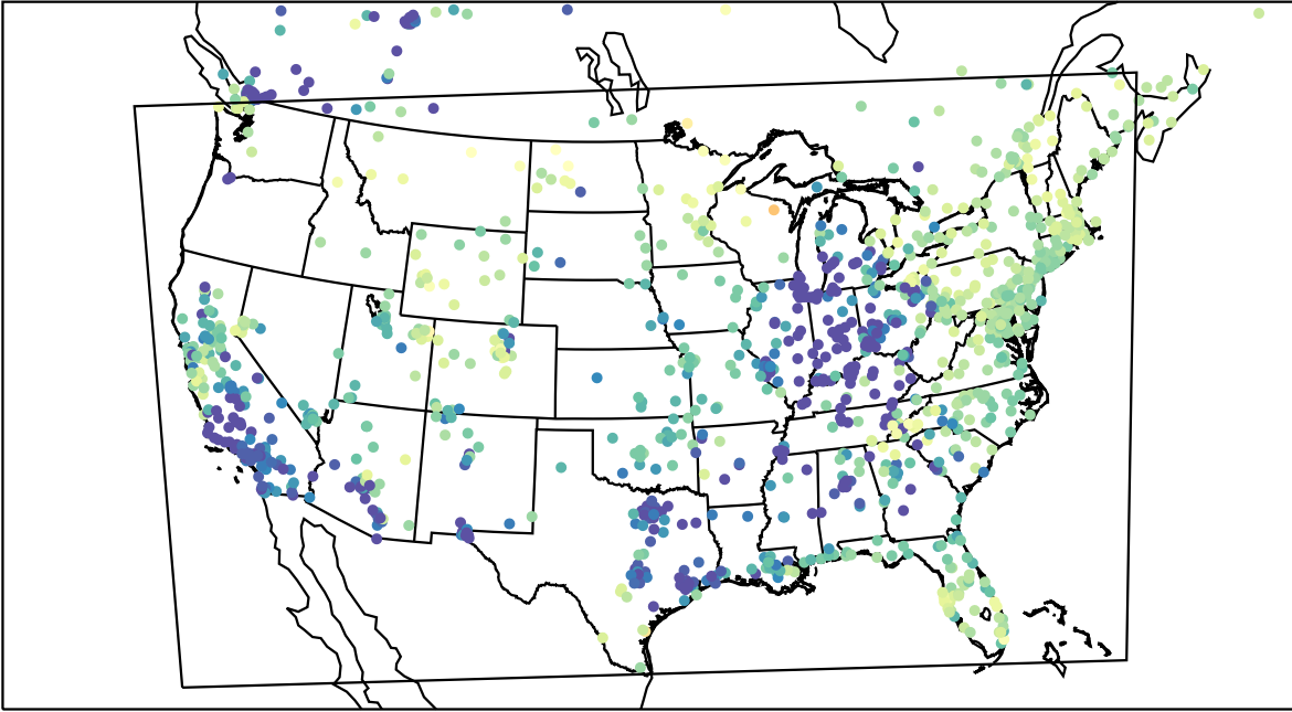
AirNOW (2023-03-15_09:00:00)
