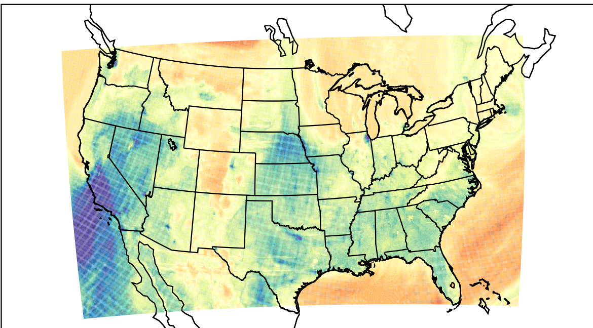
WRF (2023-03-15_02:00:00)
