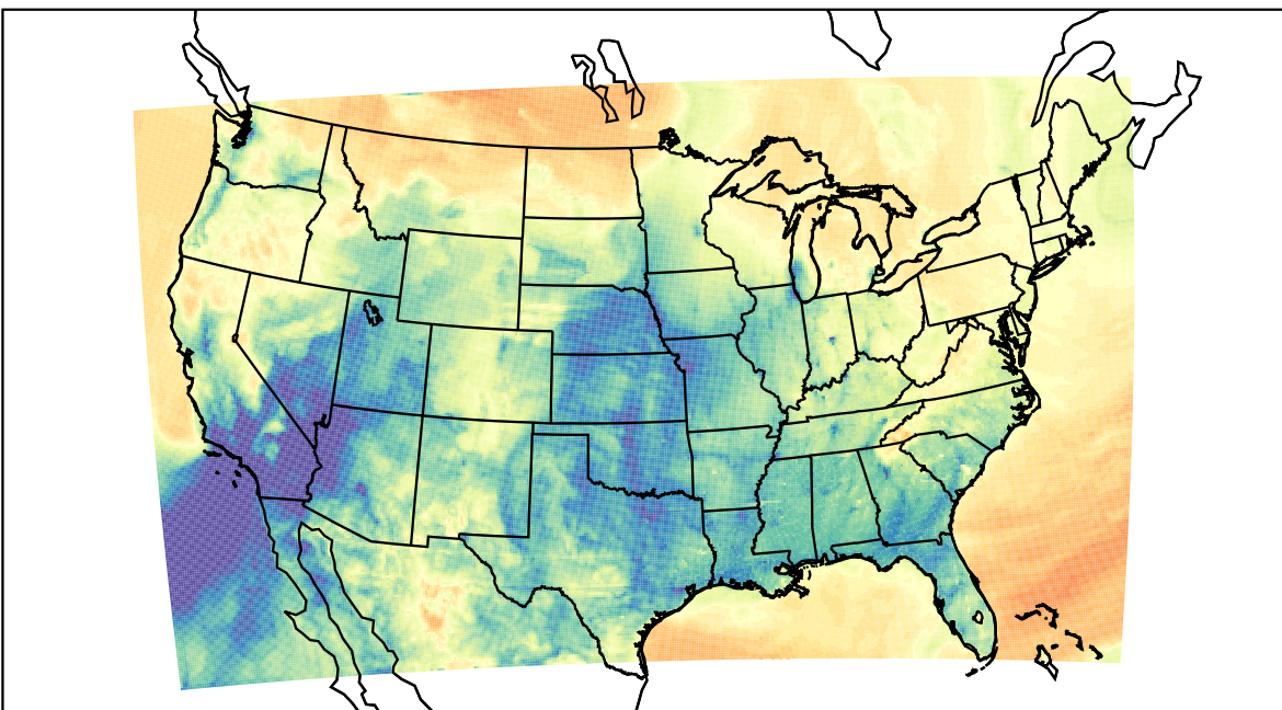
WRF (2023-03-15_12:00:00)
