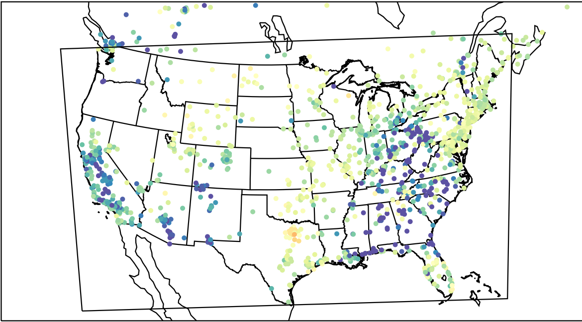
AirNOW (2023-03-16_03:00:00)
