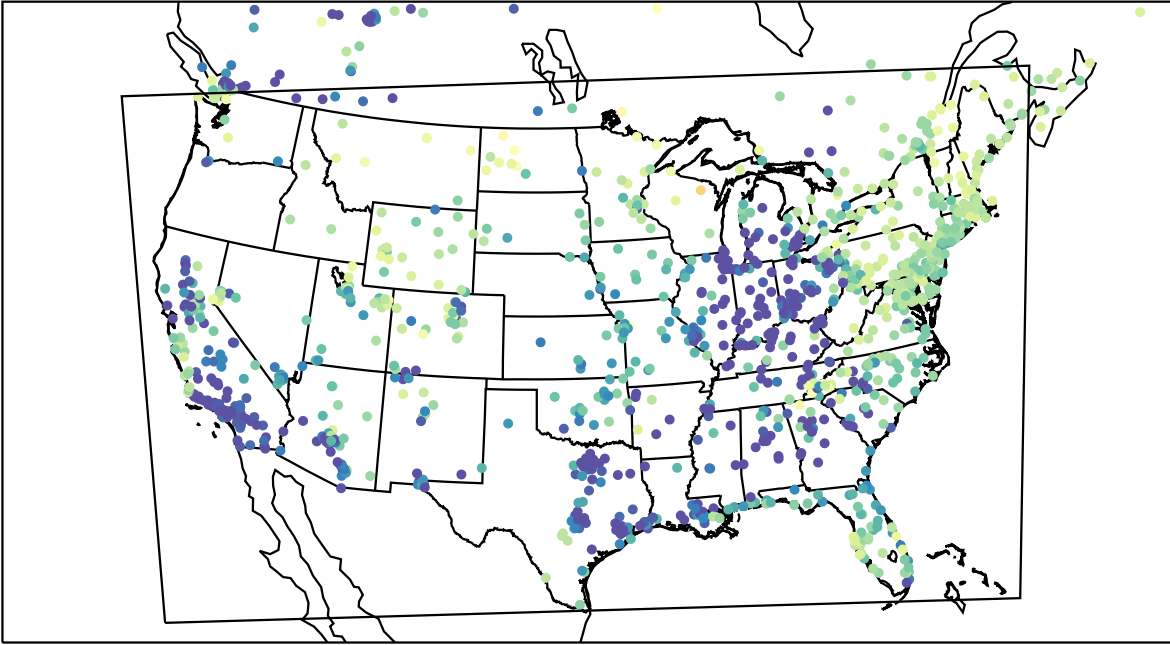
AirNOW (2023-03-15_11:00:00)
