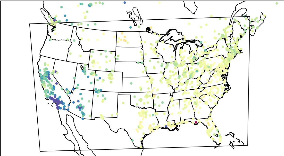
AirNOW (2023-03-15_18:00:00)
