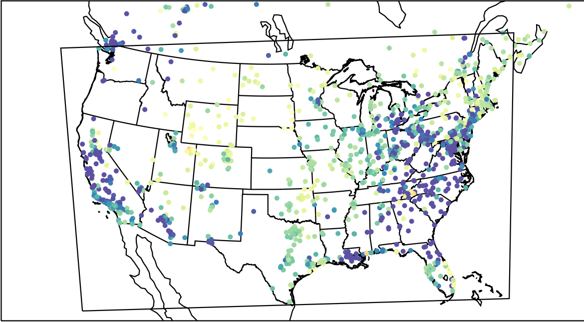
AirNOW (2023-03-16_11:00:00)
