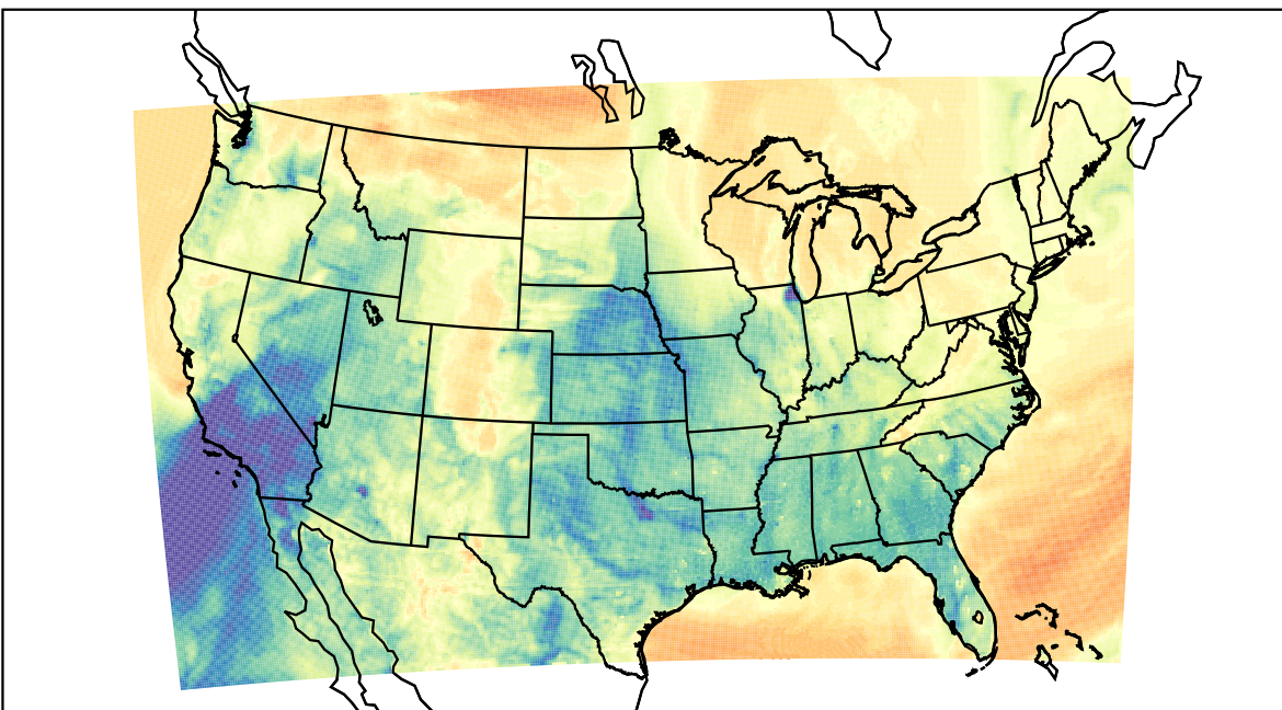
WRF (2023-03-15_07:00:00)
