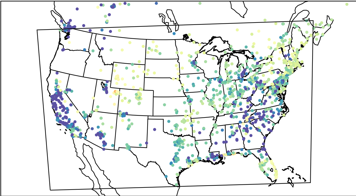
AirNOW (2023-03-16_13:00:00)
