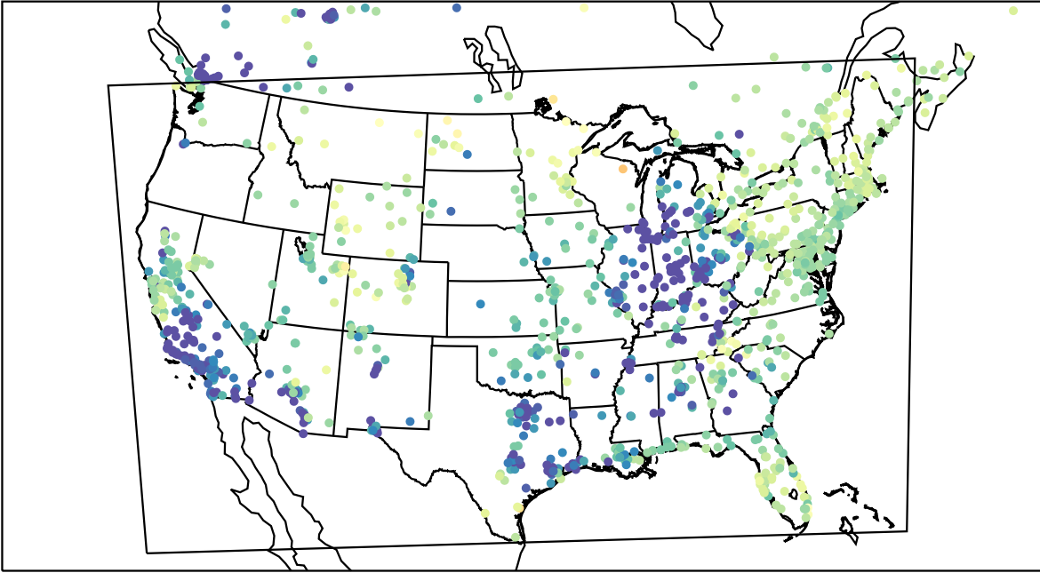
AirNOW (2023-03-15_08:00:00)
