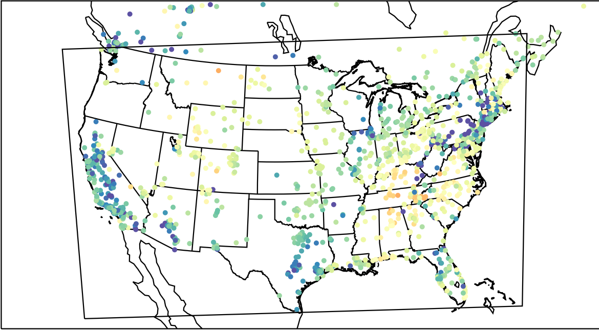
AirNOW (2023-03-17_03:00:00)
