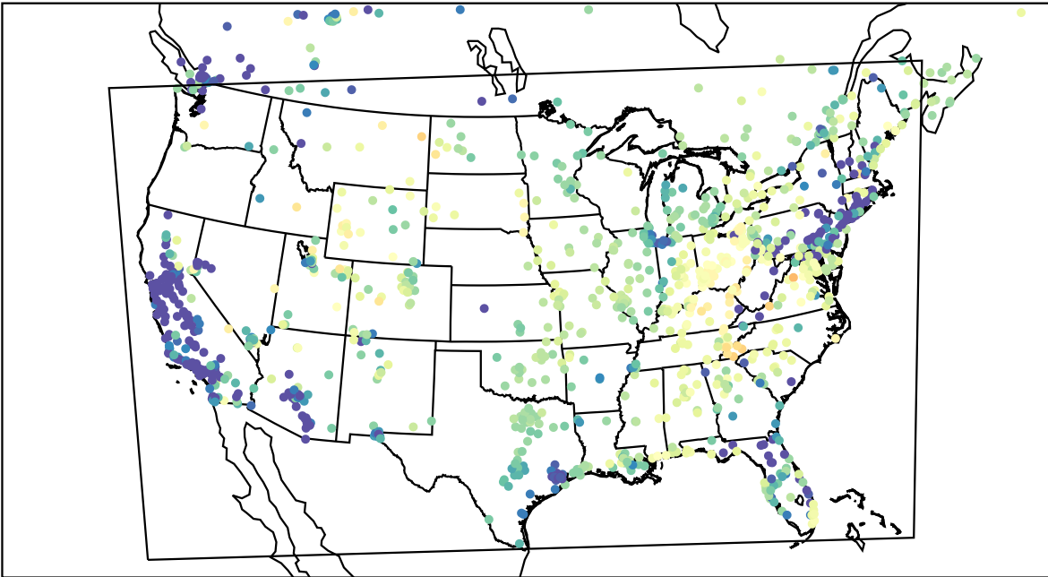
AirNOW (2023-03-17_08:00:00)
