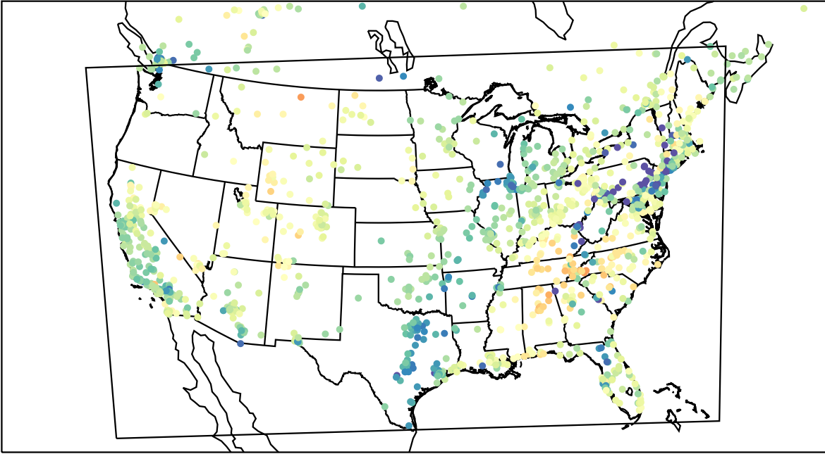
AirNOW (2023-03-17_01:00:00)
