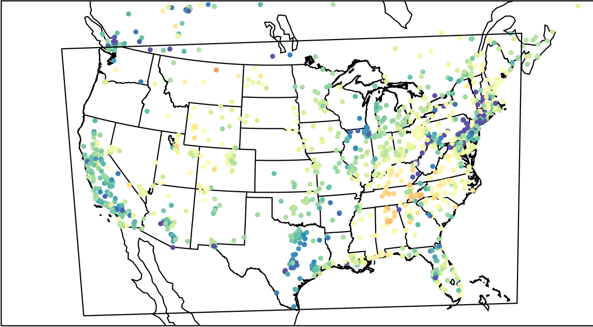
AirNOW (2023-03-17_02:00:00)
