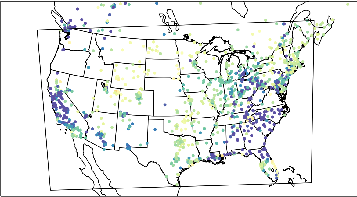
AirNOW (2023-03-16_09:00:00)
