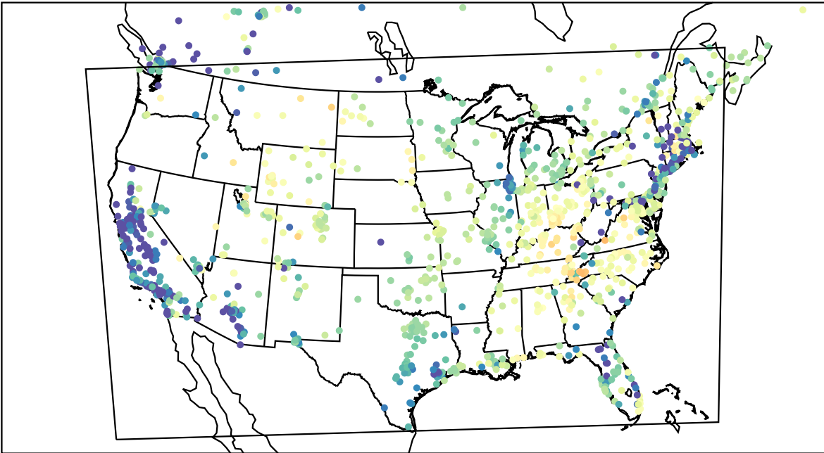
AirNOW (2023-03-17_06:00:00)
