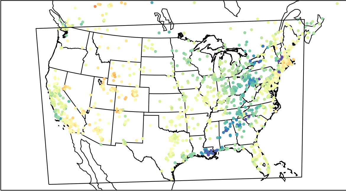
AirNOW (2023-03-17_22:00:00)
