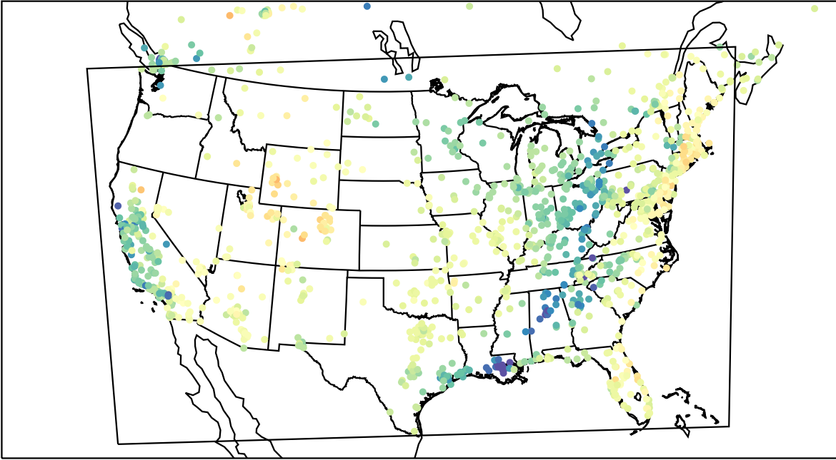
AirNOW (2023-03-17_19:00:00)
