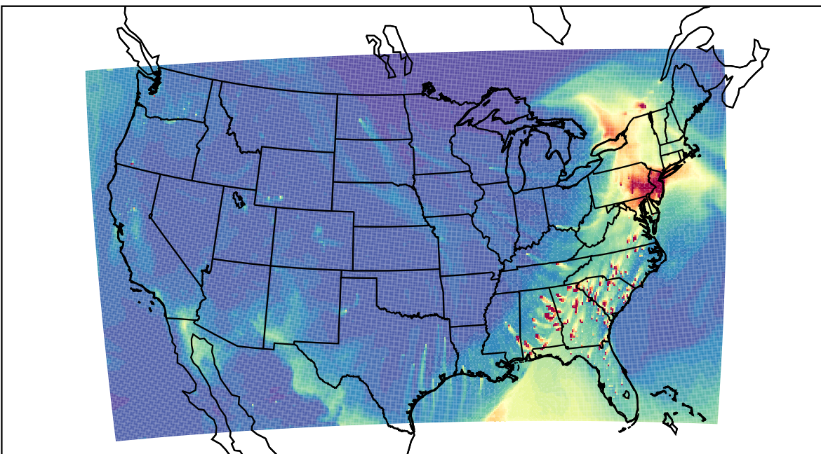
WRF 2023-03-17_21:00:00
