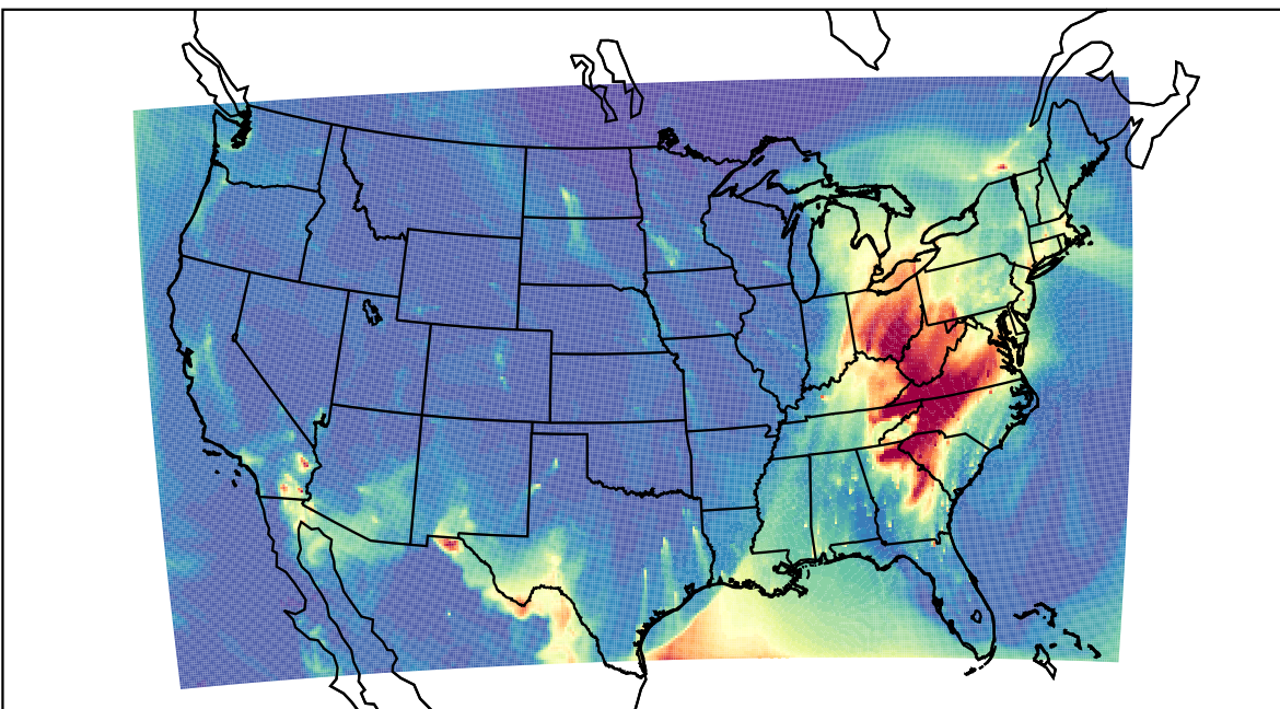
WRF 2023-03-17_11:00:00
