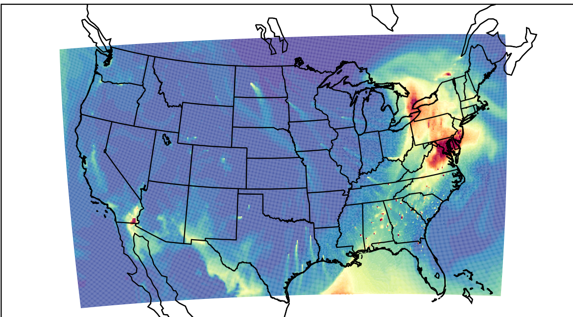
WRF 2023-03-17_17:00:00
