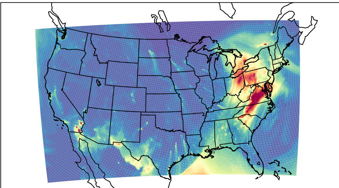
WRF 2023-03-17_14:00:00
