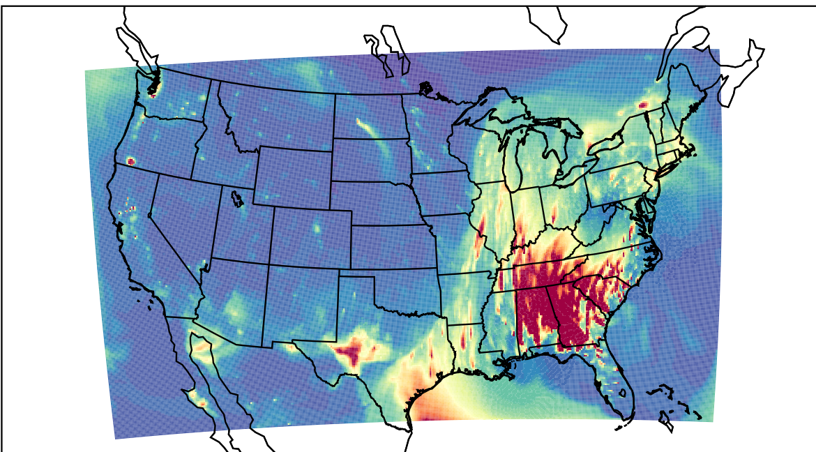
WRF 2023-03-17_02:00:00
