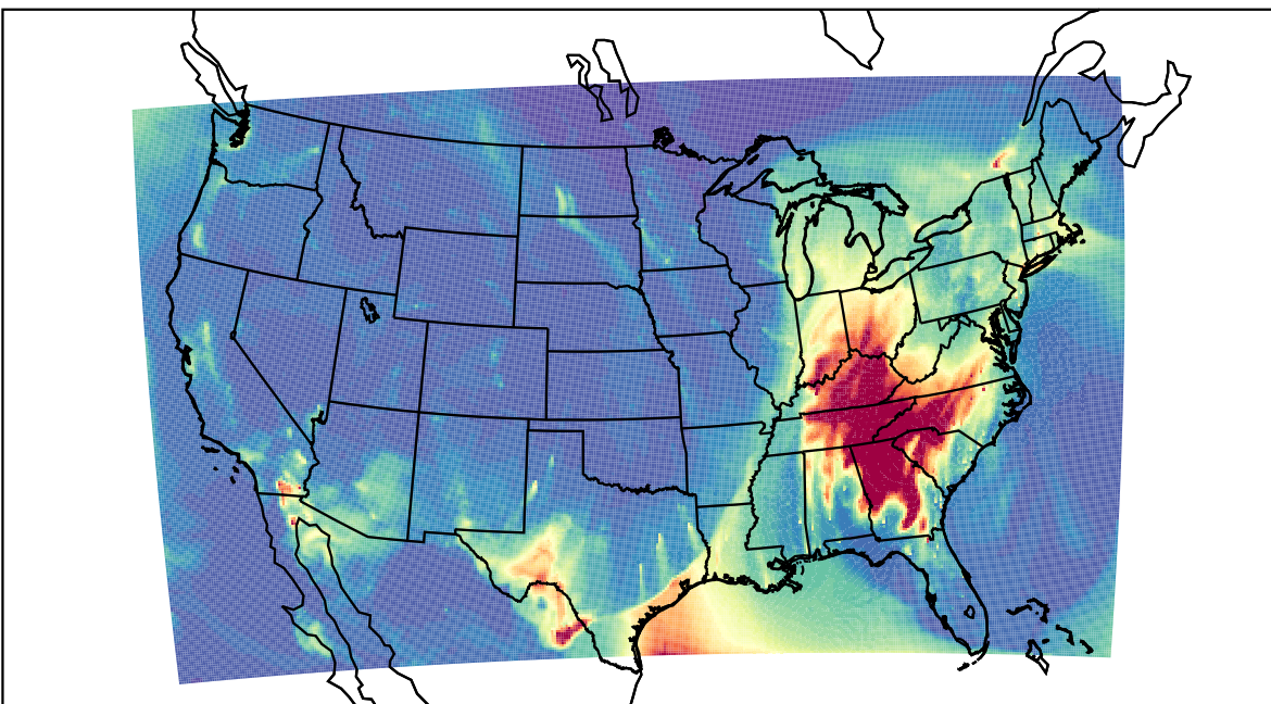
WRF 2023-03-17_07:00:00
