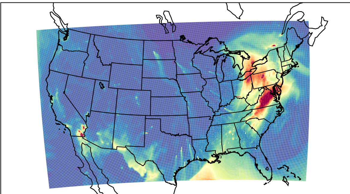
WRF 2023-03-17_15:00:00
