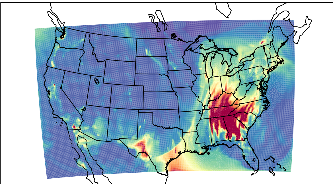
WRF 2023-03-17_05:00:00
