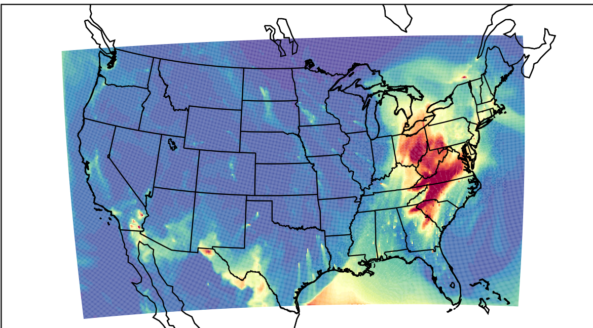
WRF 2023-03-17_12:00:00
