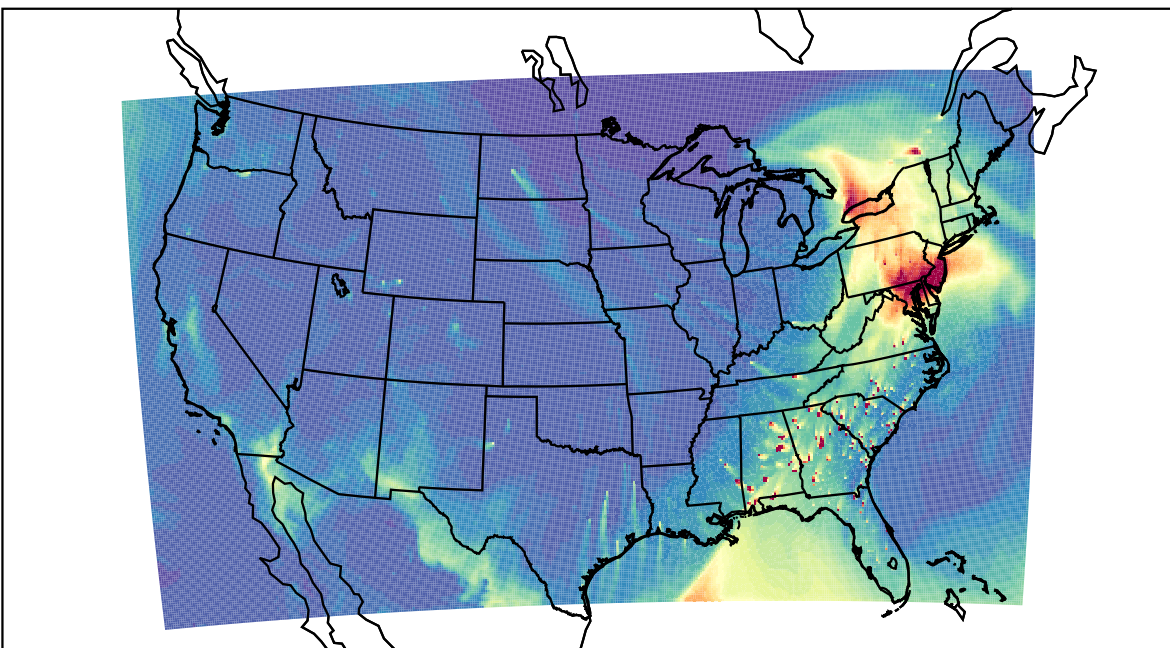
WRF 2023-03-17_19:00:00
