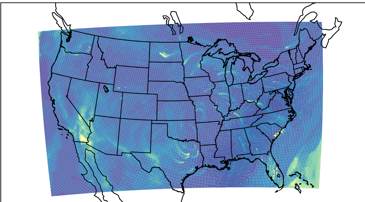
WRF 2023-03-19_21:00:00
