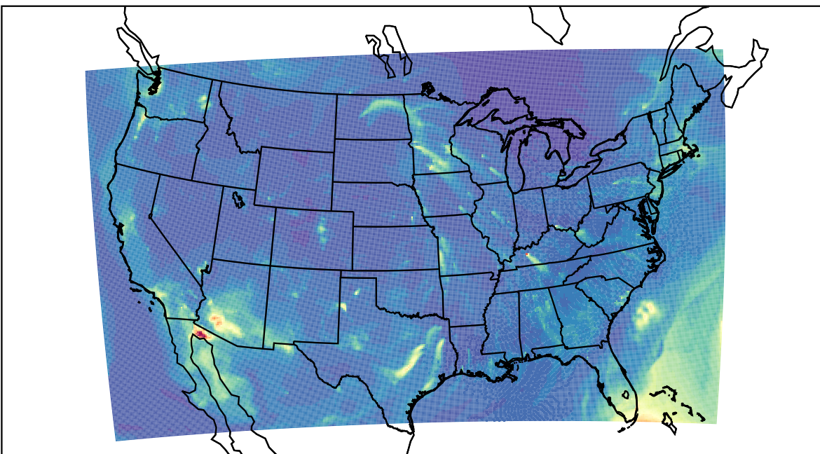
WRF 2023-03-19_06:00:00
