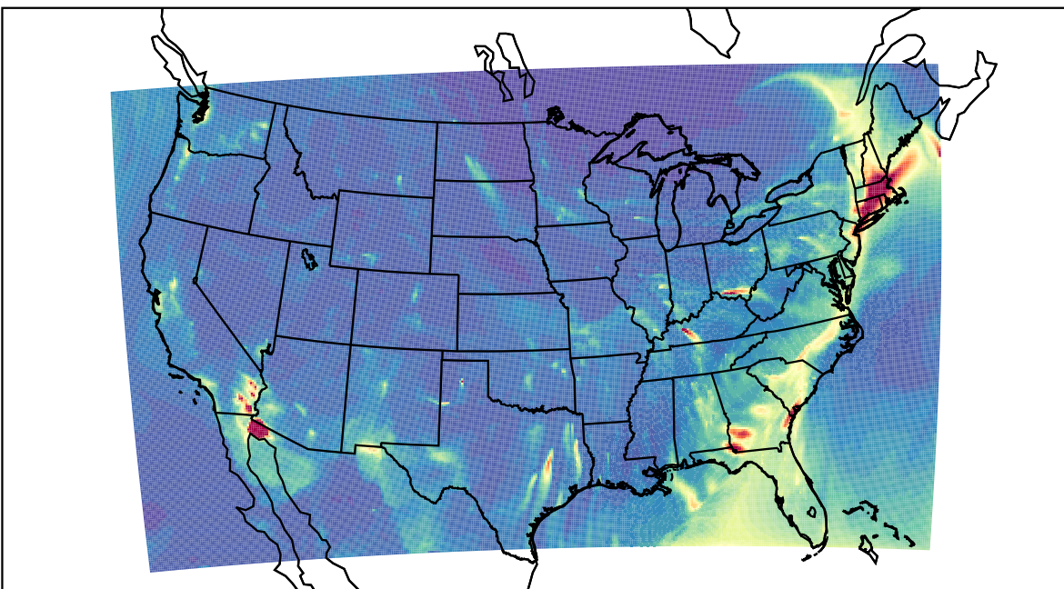
WRF 2023-03-18_06:00:00
