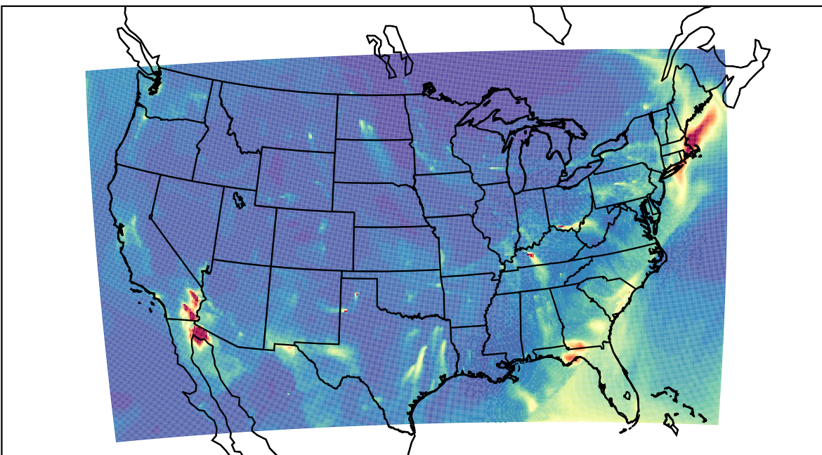
WRF 2023-03-18_09:00:00
