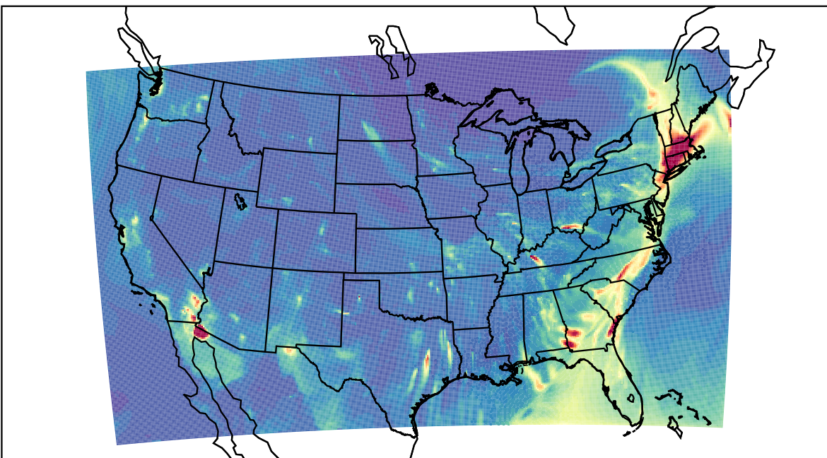
WRF 2023-03-18_05:00:00
