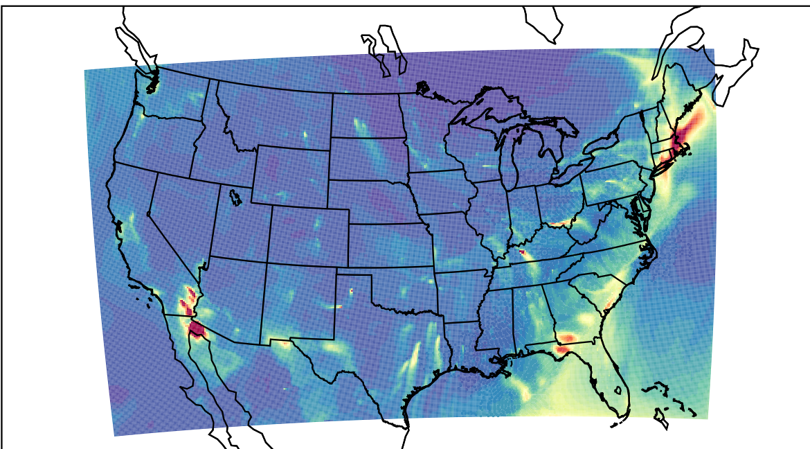
WRF 2023-03-18_08:00:00
