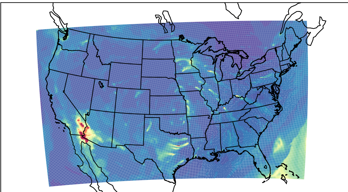
WRF 2023-03-19_13:00:00
