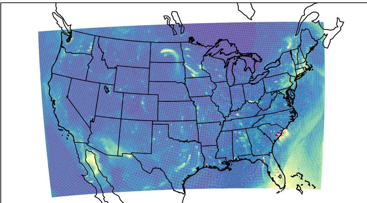
WRF 2023-03-19_01:00:00
