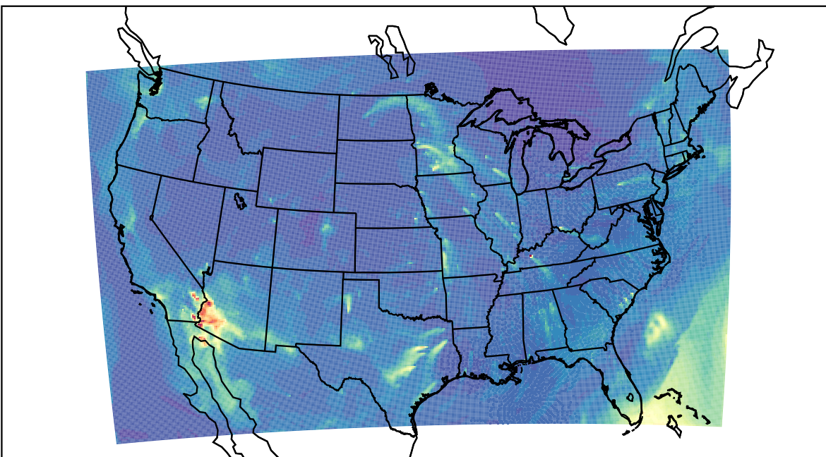
WRF 2023-03-19_09:00:00
