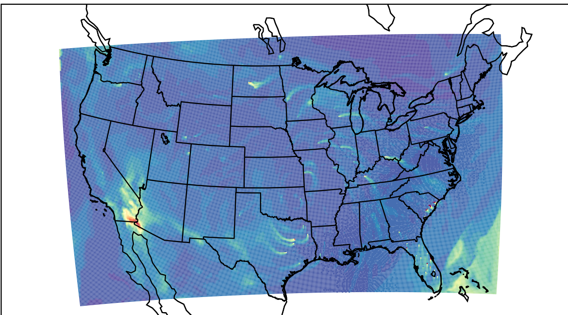
WRF 2023-03-19_19:00:00
