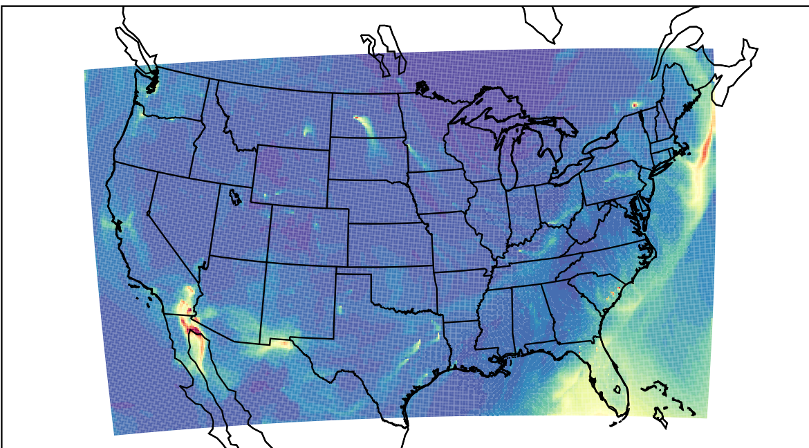
WRF 2023-03-18_17:00:00
