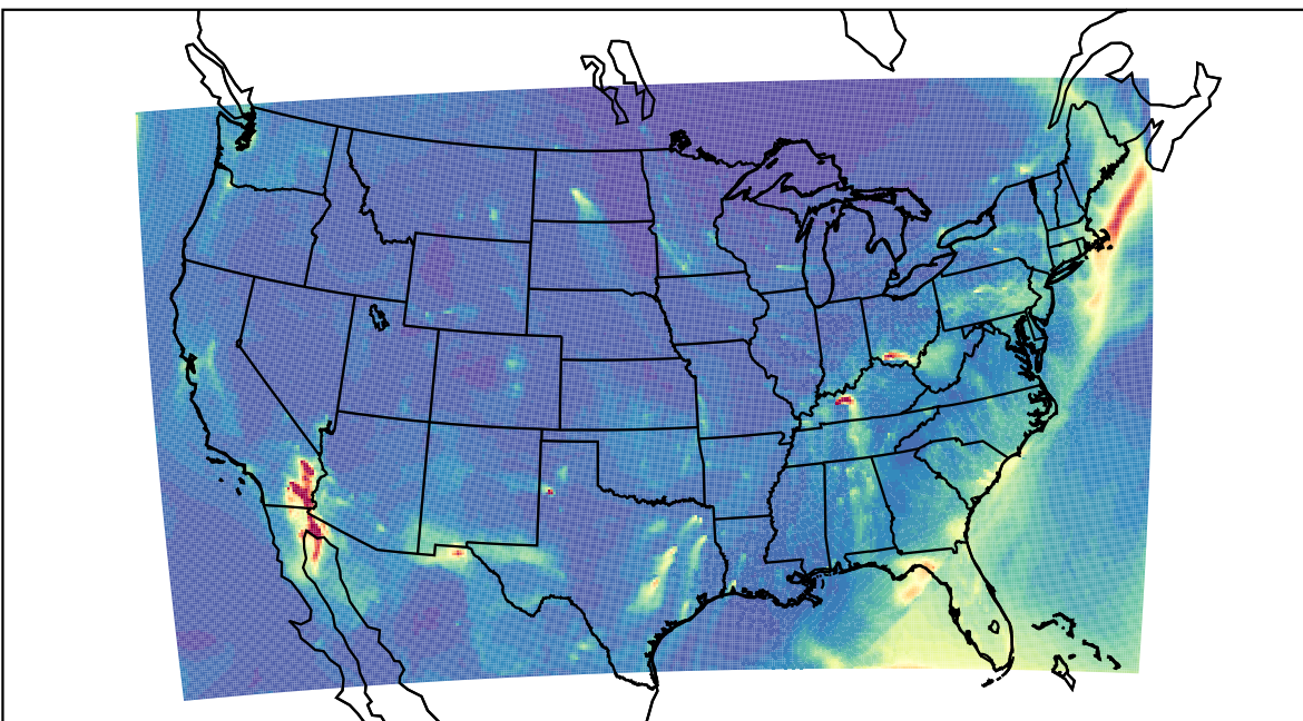
WRF 2023-03-18_12:00:00
