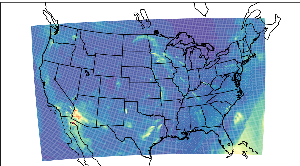
WRF 2023-03-19_08:00:00
