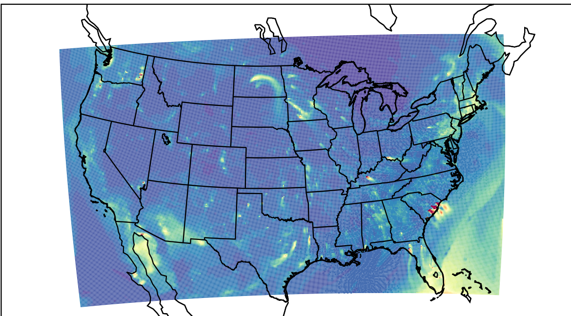
WRF 2023-03-19_02:00:00
