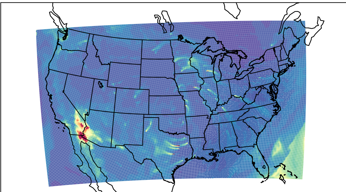
WRF 2023-03-19_15:00:00
