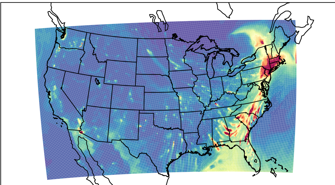
WRF 2023-03-18_02:00:00
