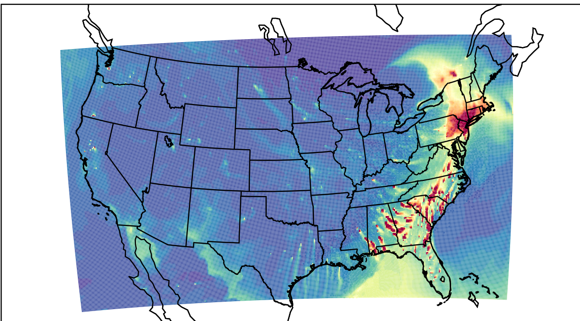
WRF 2023-03-18_00:00:00
