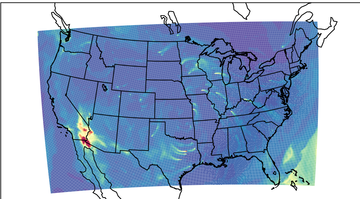
WRF 2023-03-19_16:00:00
