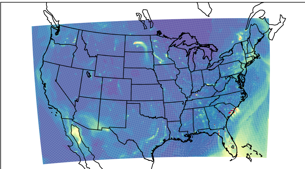
WRF 2023-03-19_00:00:00
