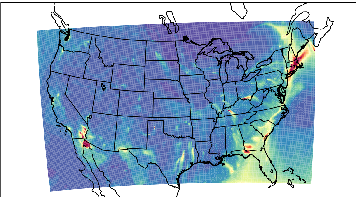
WRF 2023-03-18_07:00:00
