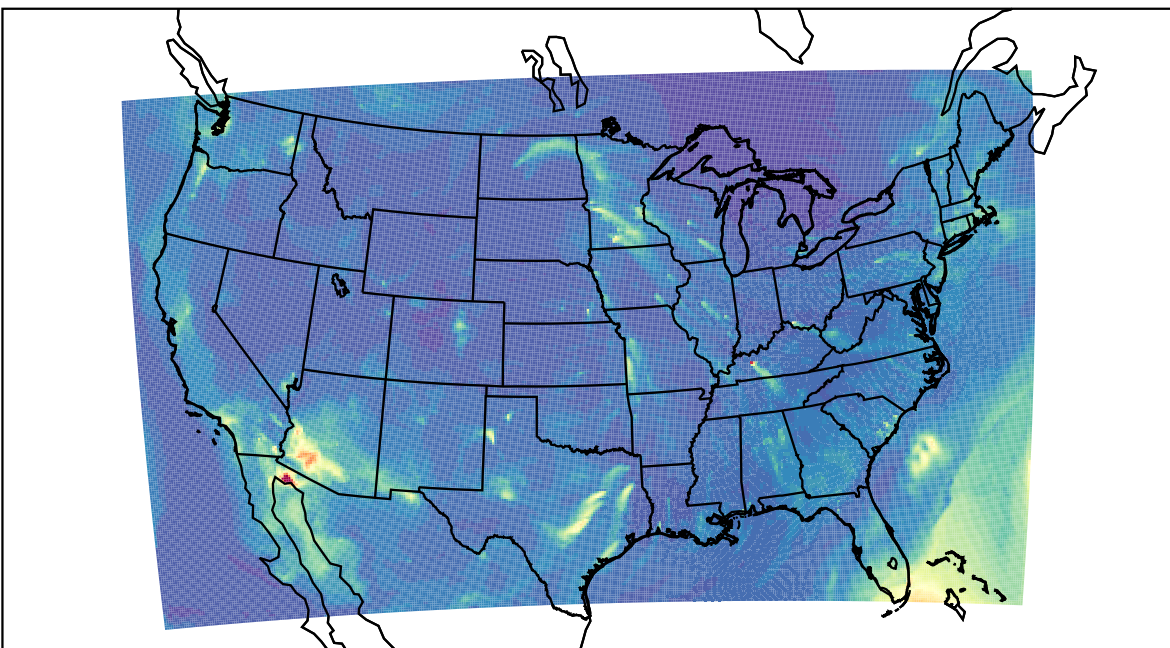
WRF 2023-03-19_07:00:00
