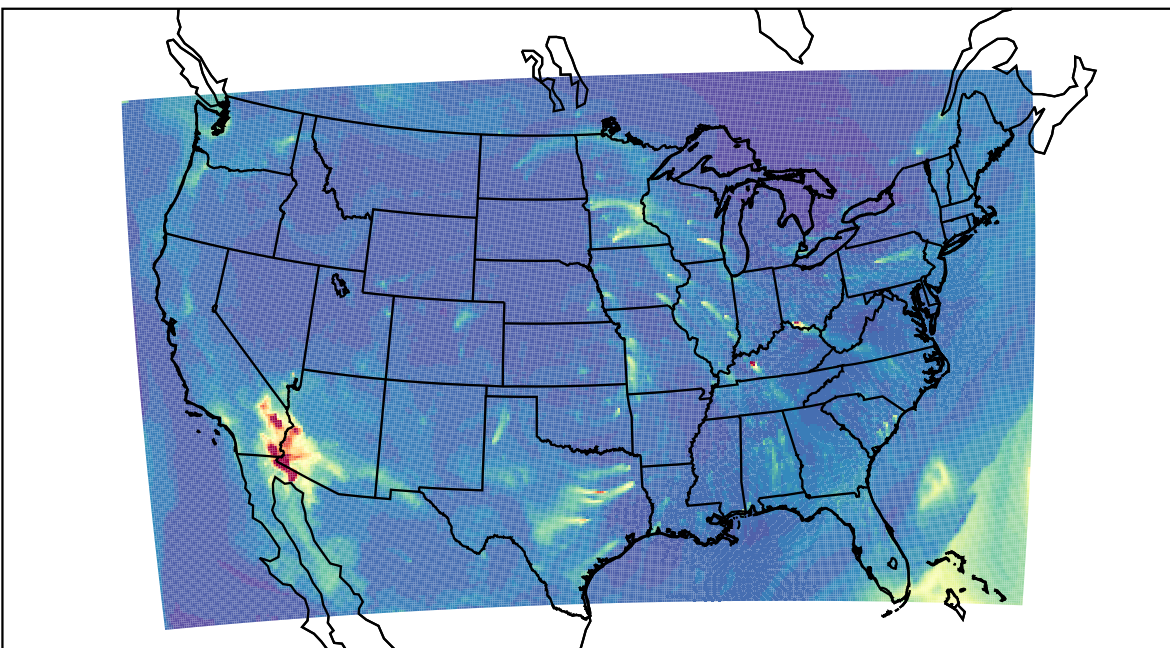
WRF 2023-03-19_12:00:00
