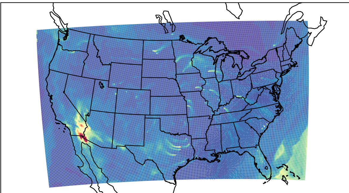
WRF 2023-03-19_17:00:00
