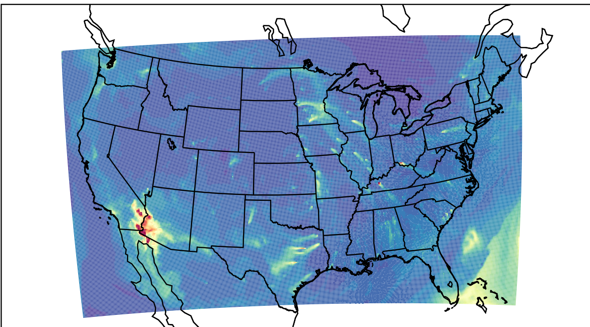
WRF 2023-03-19_11:00:00
