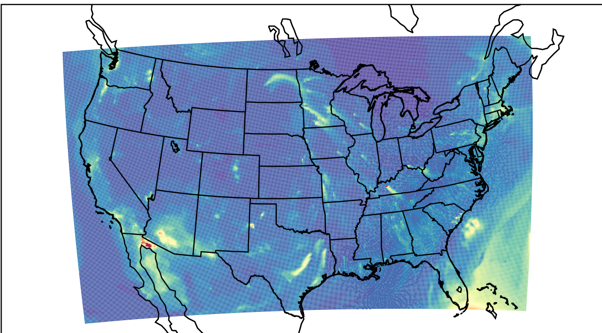
WRF 2023-03-19_05:00:00
