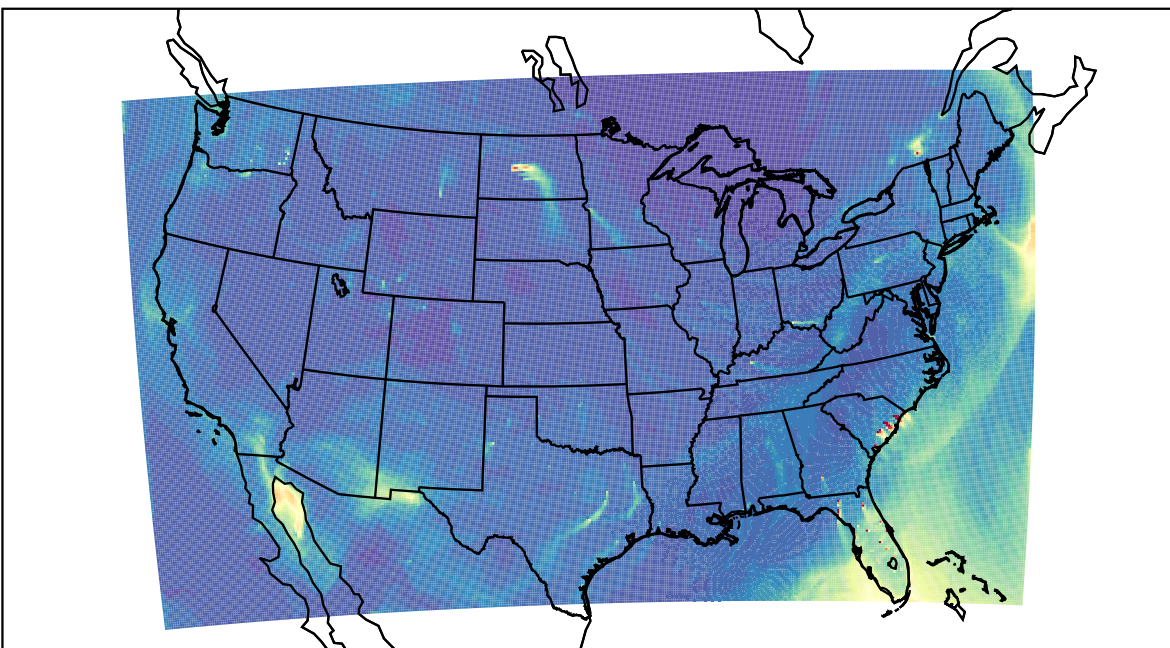
WRF 2023-03-18_21:00:00
