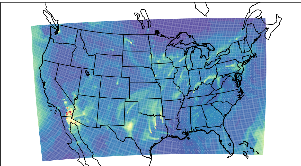
WRF 2023-03-20_15:00:00
