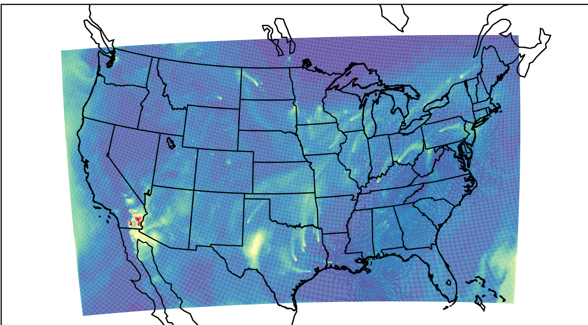
WRF 2023-03-20_17:00:00
