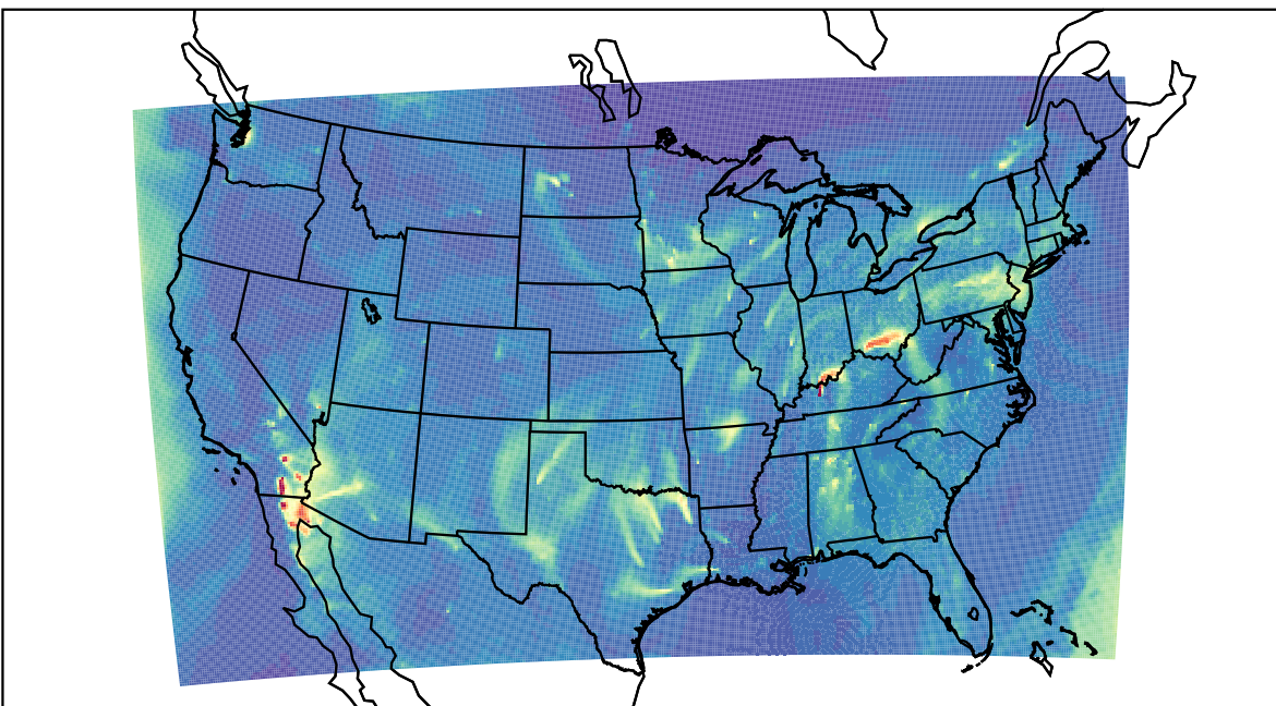
WRF 2023-03-20_12:00:00
