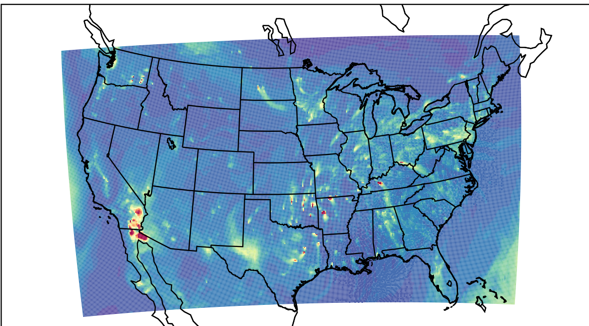
WRF 2023-03-20_02:00:00
