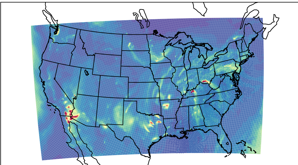
WRF 2023-03-20_07:00:00
