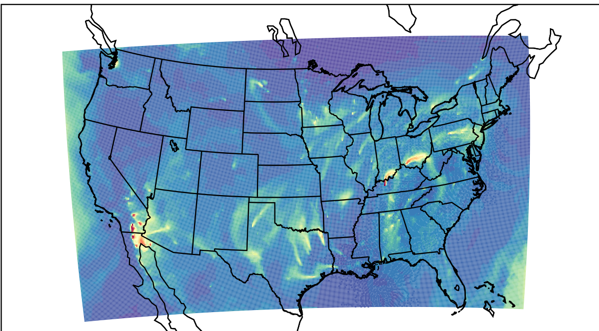
WRF 2023-03-20_13:00:00
