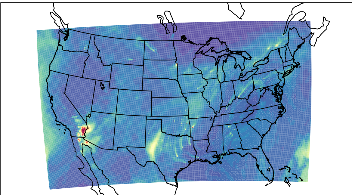
WRF 2023-03-20_21:00:00
