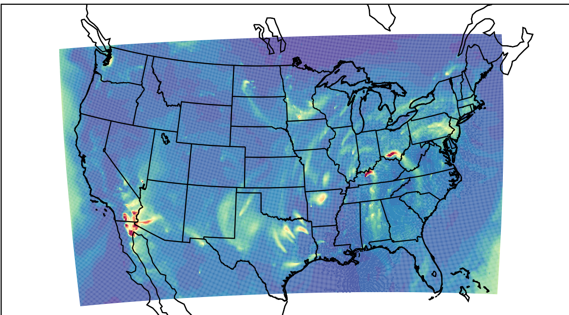
WRF 2023-03-20_09:00:00
