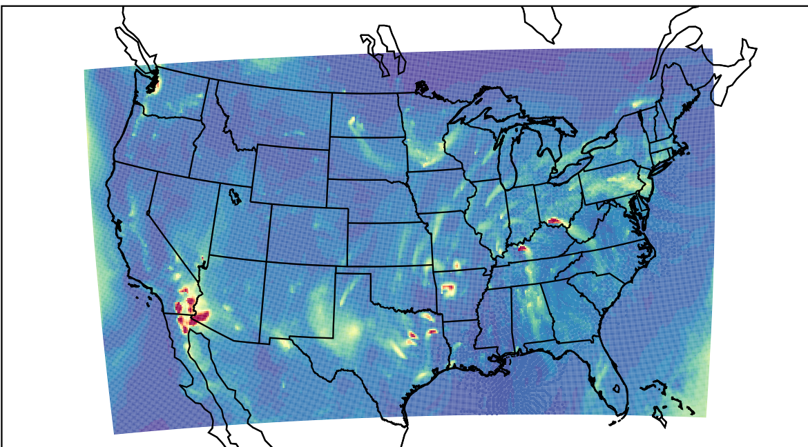
WRF 2023-03-20_06:00:00
