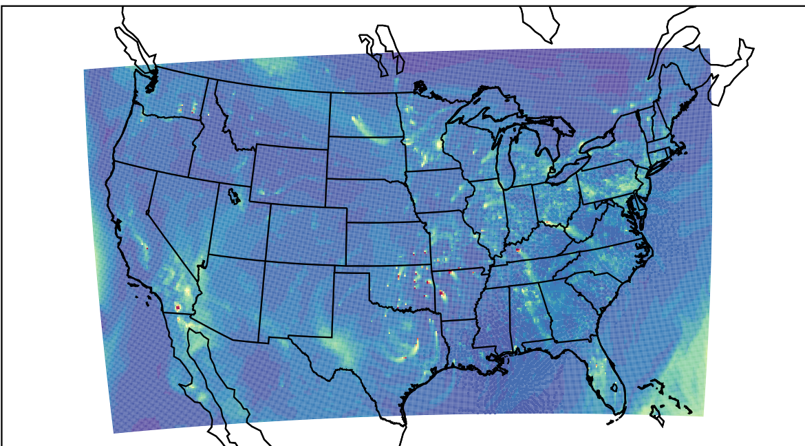
WRF 2023-03-20_00:00:00
