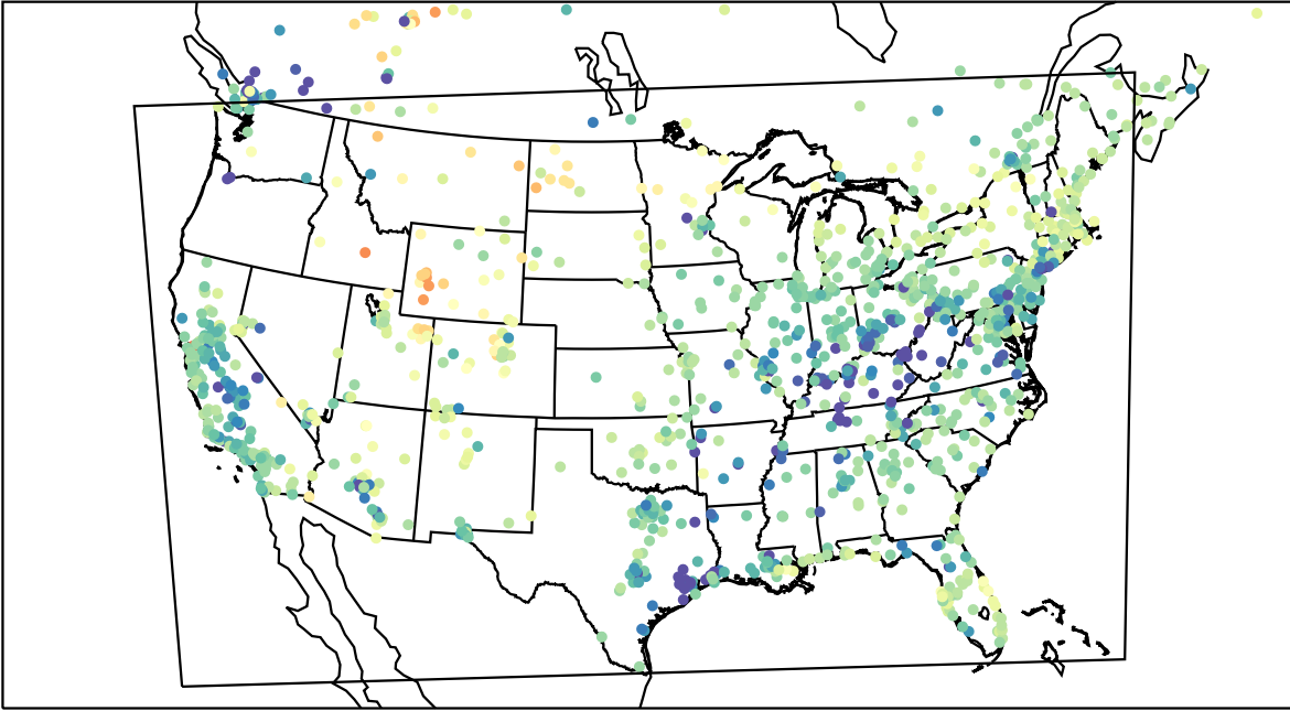
AirNOW (2023-03-20_04:00:00)
