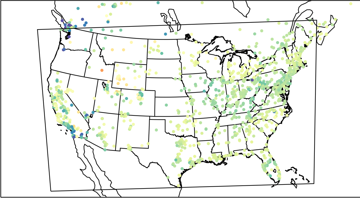
AirNOW (2023-03-19_16:00:00)
