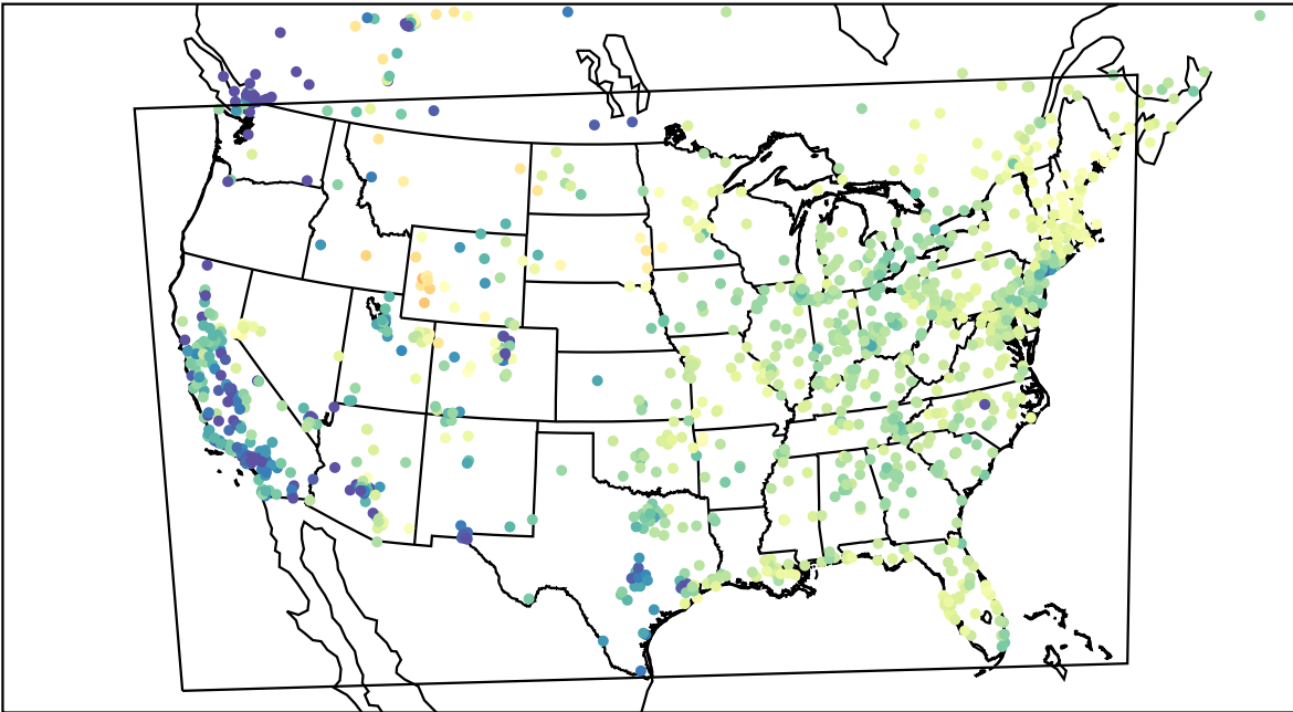
AirNOW (2023-03-20_15:00:00)
