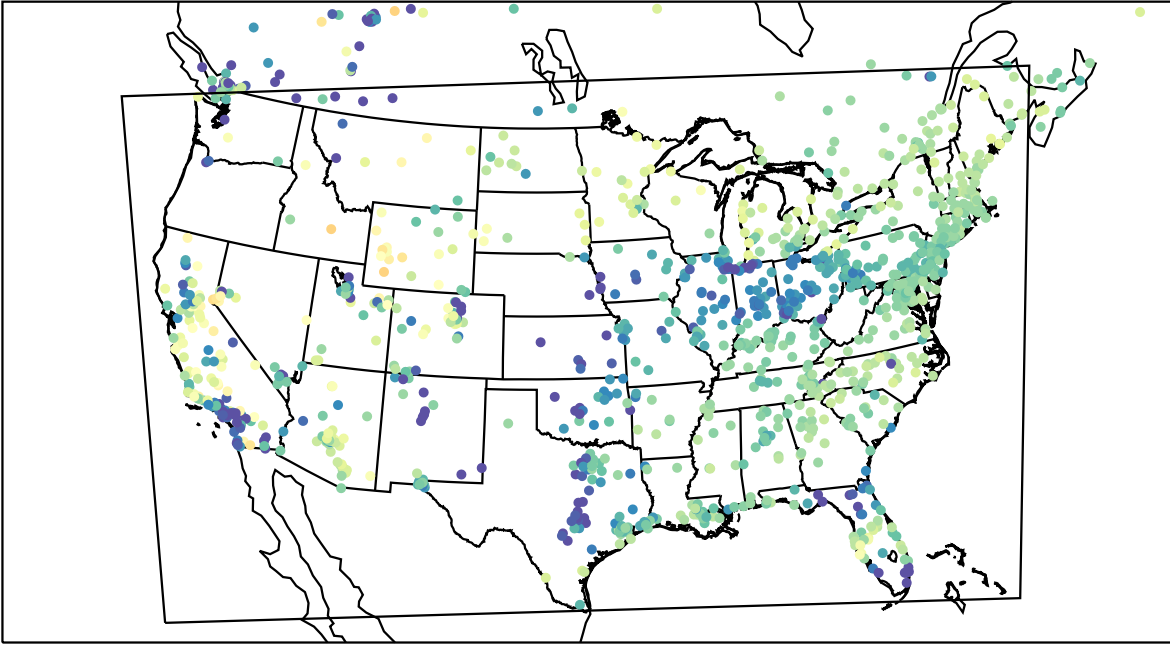
AirNOW (2023-03-19_11:00:00)
