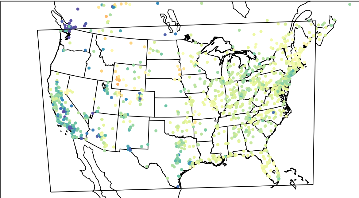
AirNOW (2023-03-20_16:00:00)
