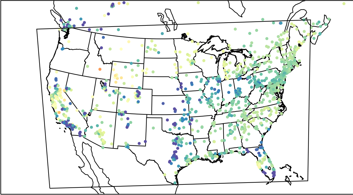
AirNOW (2023-03-19_10:00:00)
