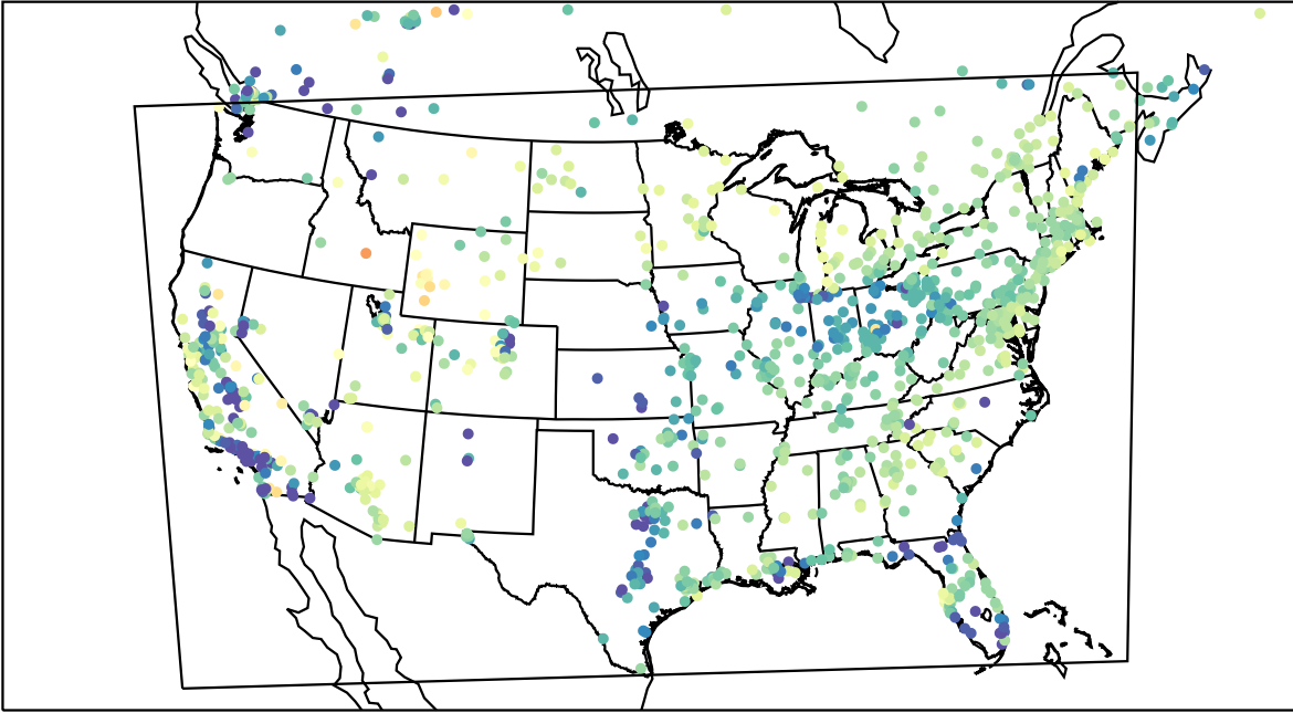
AirNOW (2023-03-19_08:00:00)
