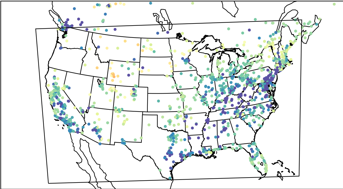
AirNOW (2023-03-20_09:00:00)
