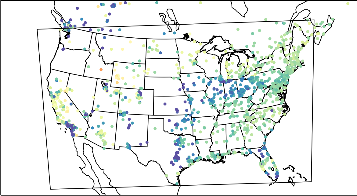
AirNOW (2023-03-19_12:00:00)
