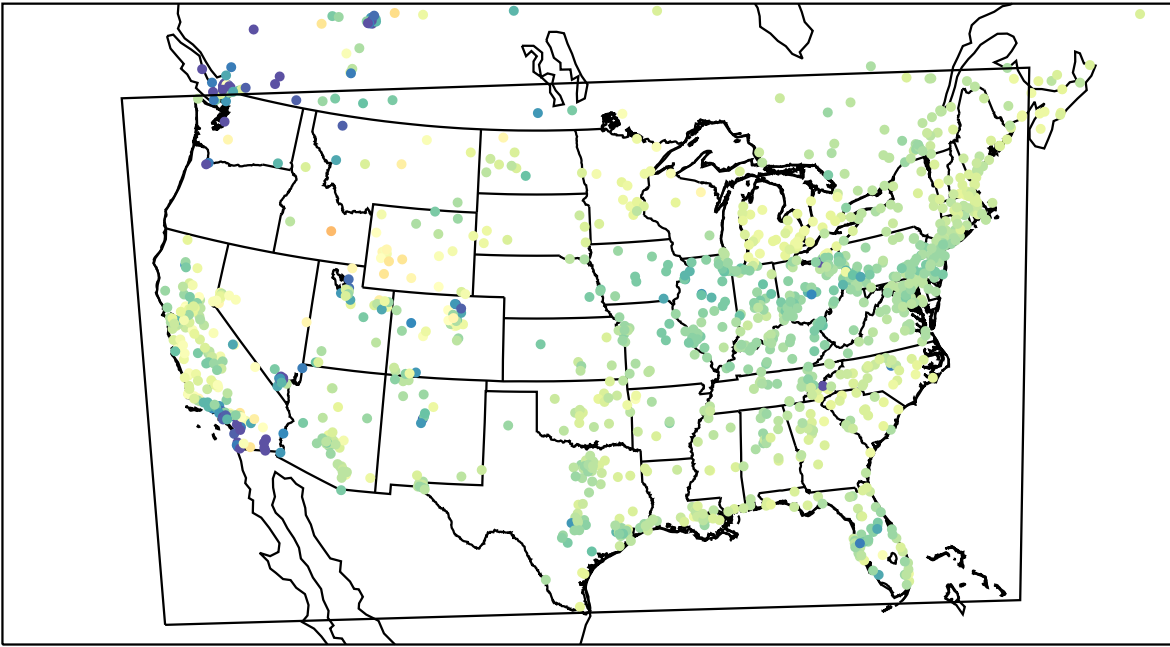
AirNOW (2023-03-19_15:00:00)
