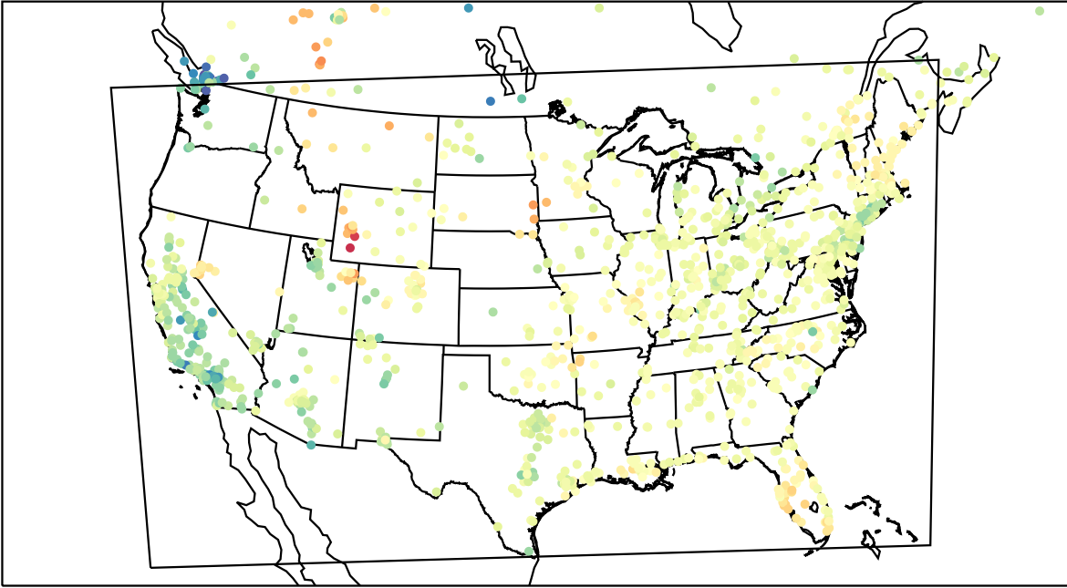
AirNOW (2023-03-20_19:00:00)
