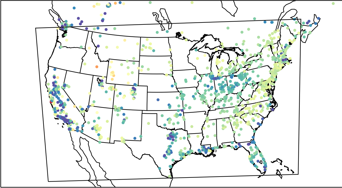
AirNOW (2023-03-19_06:00:00)
