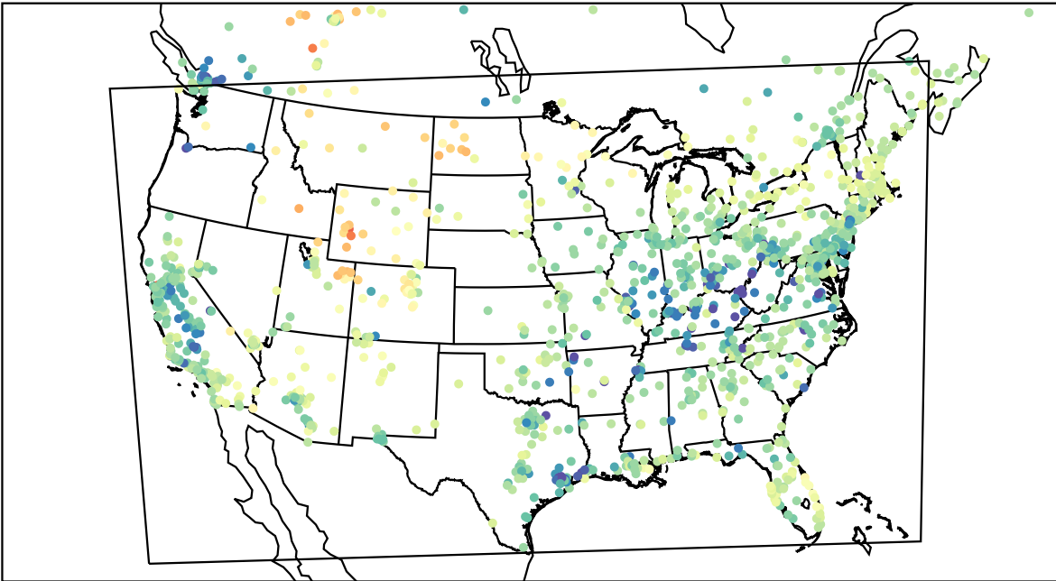
AirNOW (2023-03-20_02:00:00)
