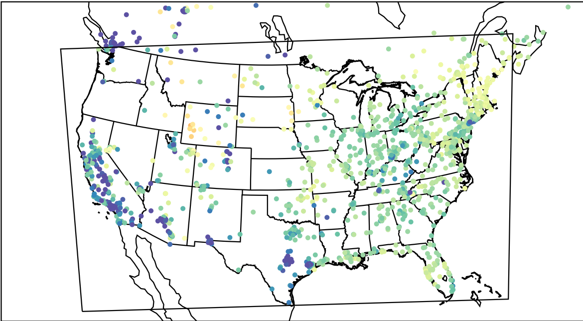
AirNOW (2023-03-20_14:00:00)
