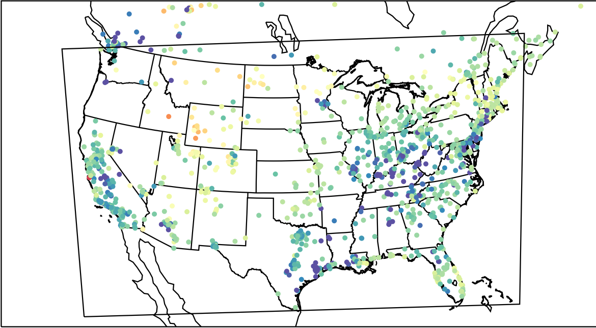
AirNOW (2023-03-20_06:00:00)
