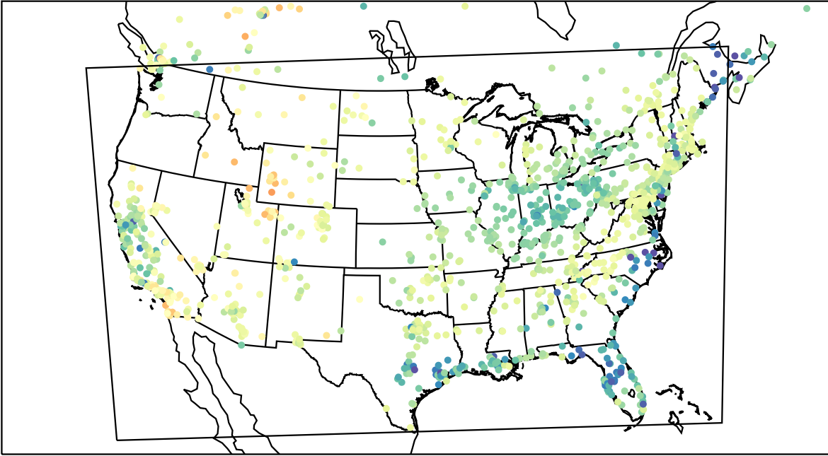
AirNOW (2023-03-19_01:00:00)
