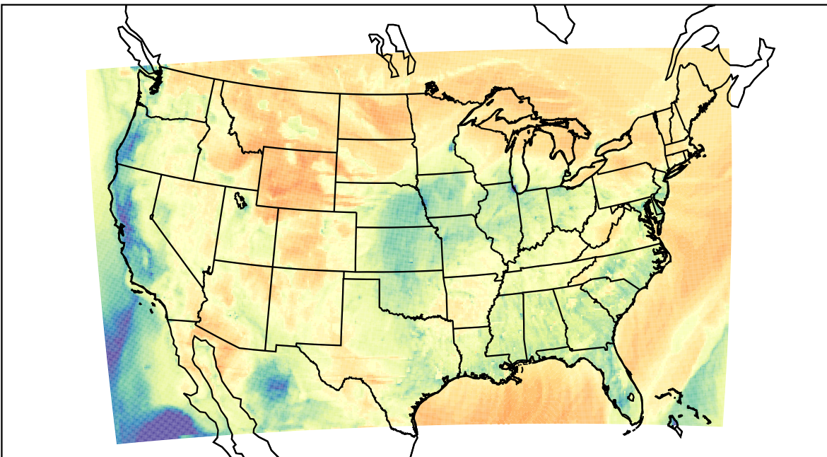
WRF (2023-03-20_01:00:00)
