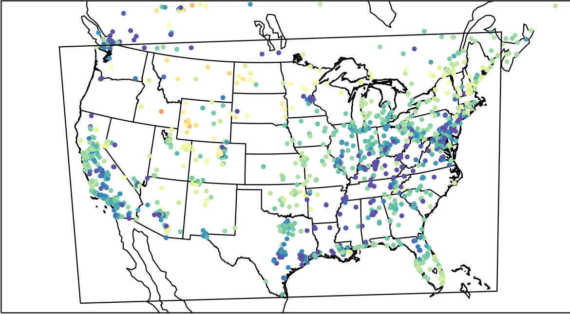
AirNOW (2023-03-20_08:00:00)
