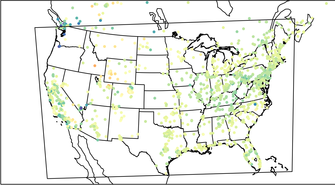
AirNOW (2023-03-19_17:00:00)
