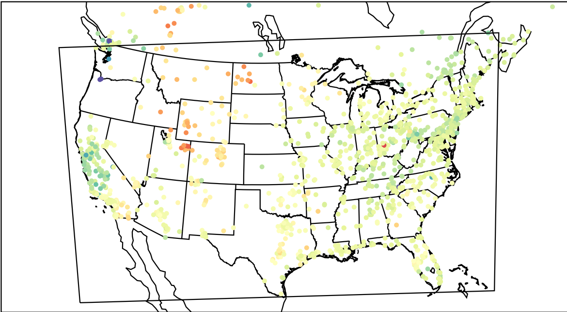
AirNOW (2023-03-19_21:00:00)
