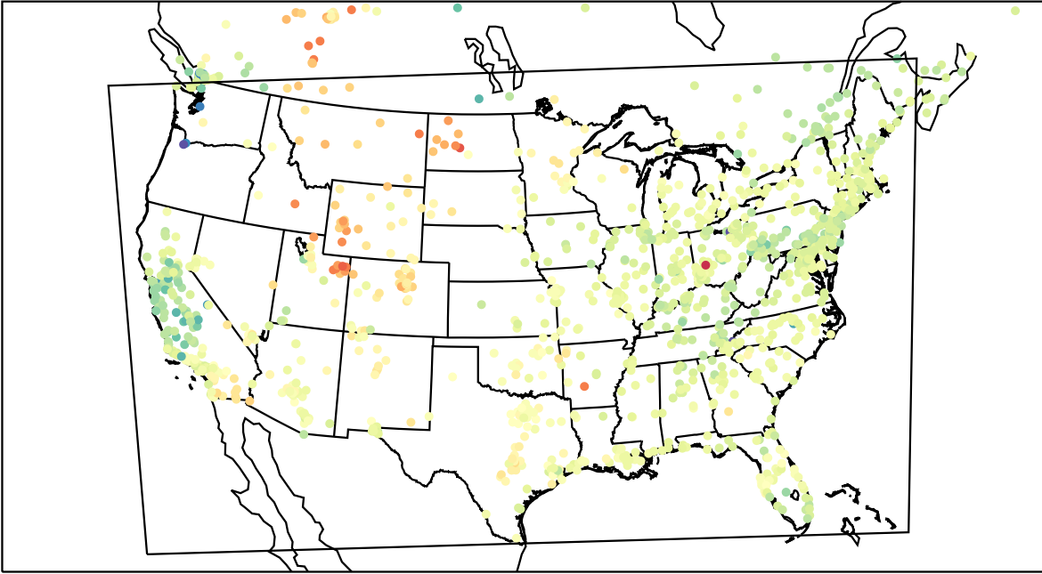
AirNOW (2023-03-19_22:00:00)
