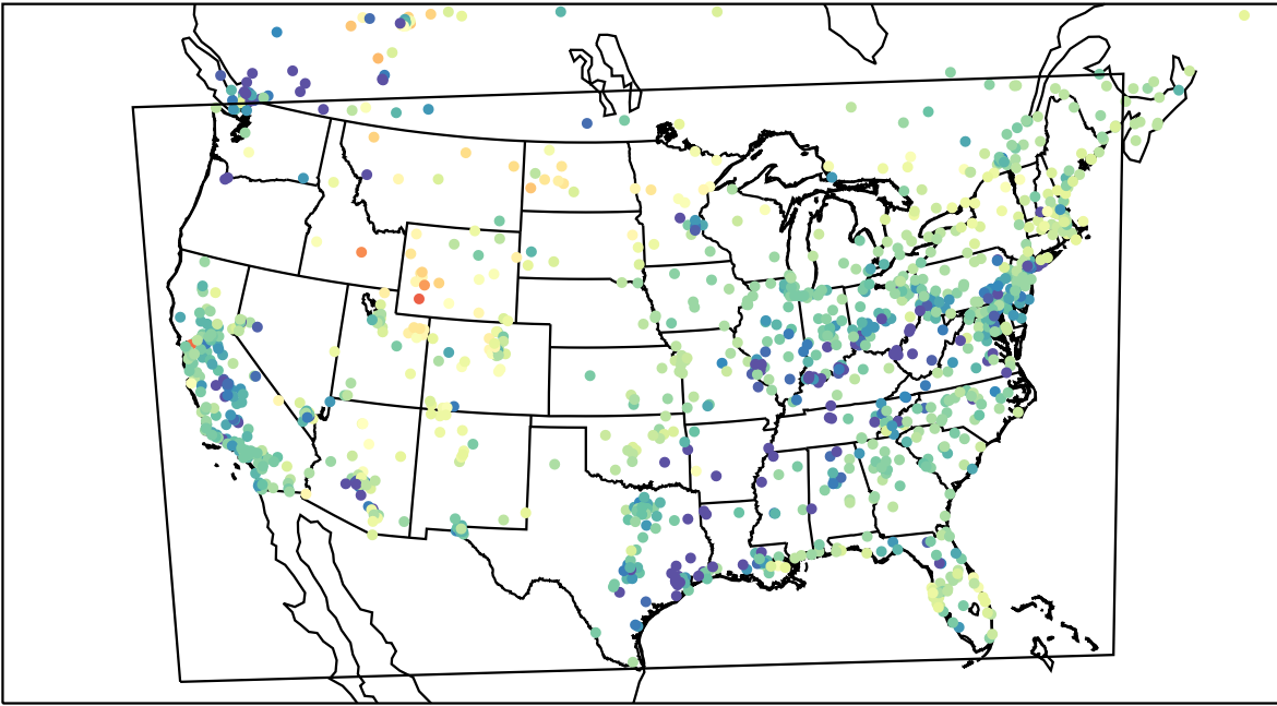
AirNOW (2023-03-20_05:00:00)
