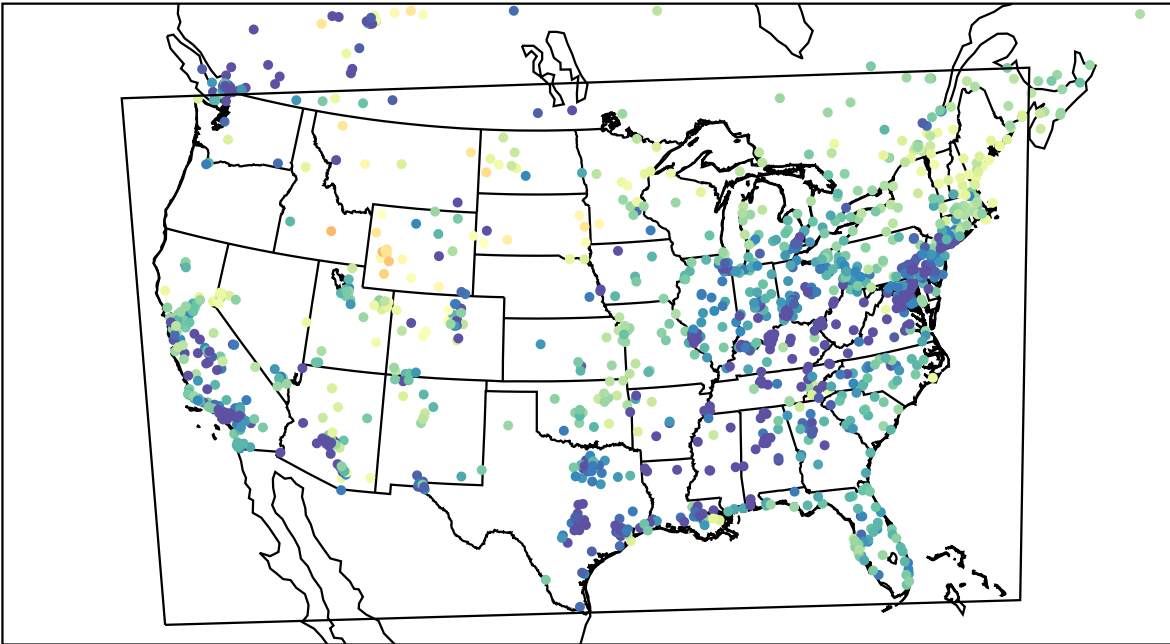
AirNOW (2023-03-20_12:00:00)
