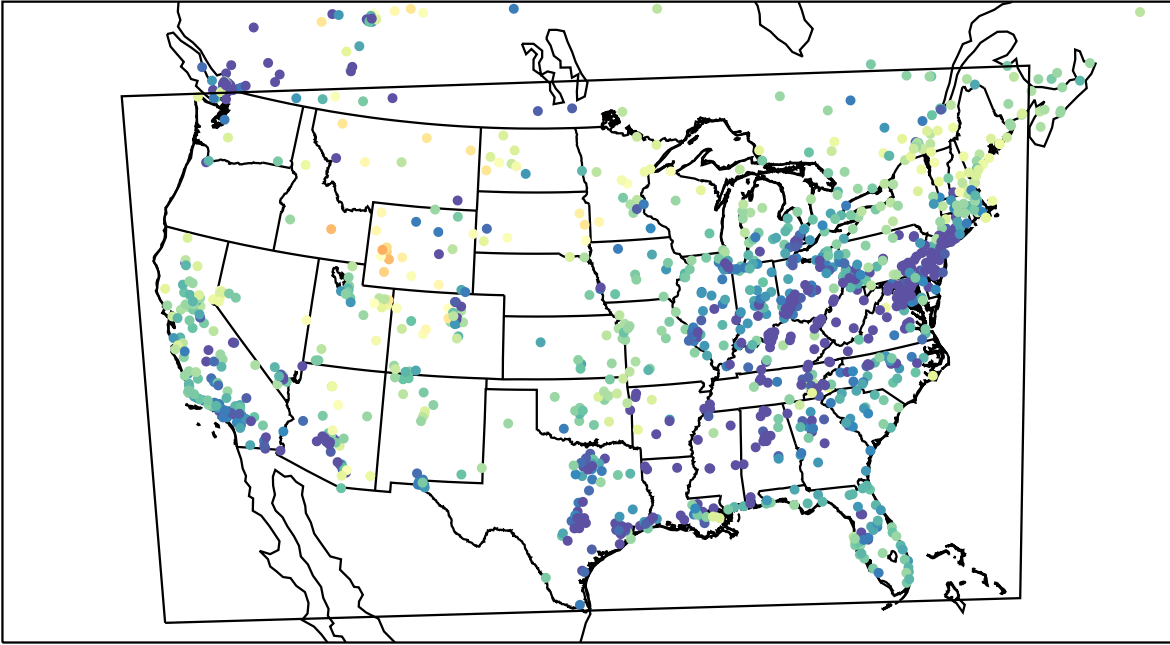
AirNOW (2023-03-20_11:00:00)
