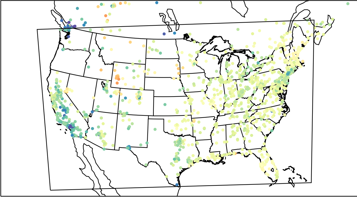
AirNOW (2023-03-20_17:00:00)
