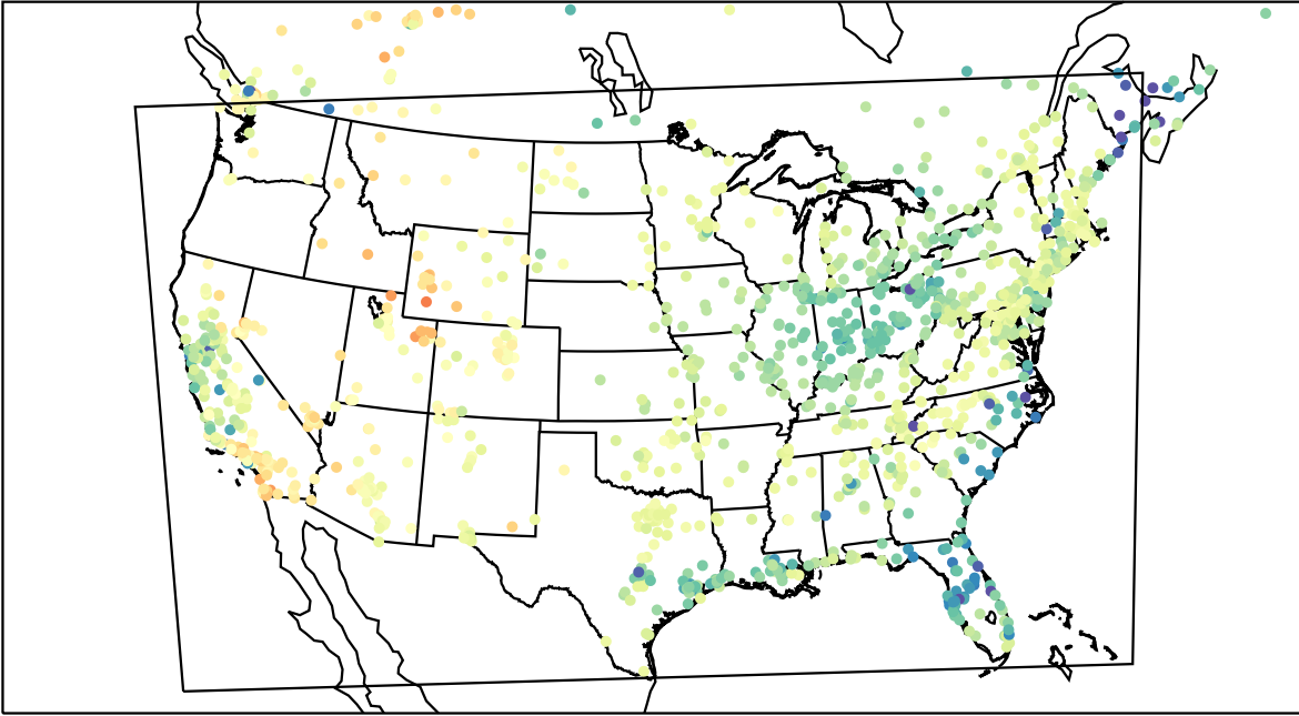
AirNOW (2023-03-19_00:00:00)
