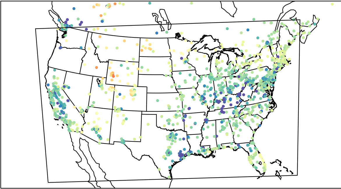
AirNOW (2023-03-20_03:00:00)
