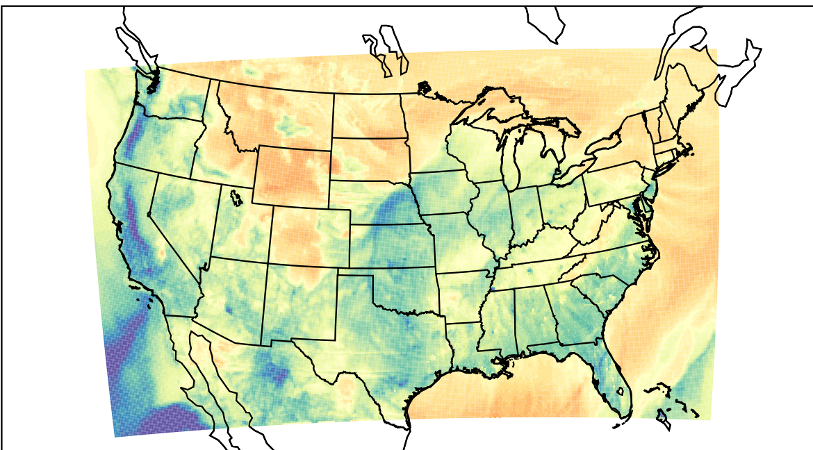
WRF (2023-03-20_05:00:00)
