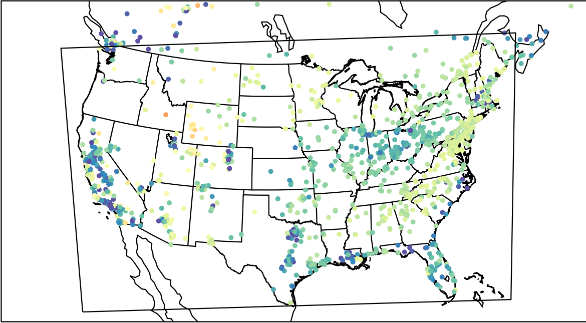
AirNOW (2023-03-19_05:00:00)
