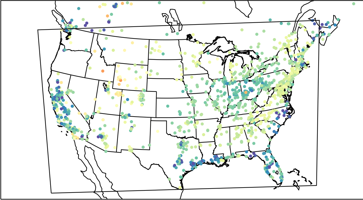
AirNOW (2023-03-19_03:00:00)
