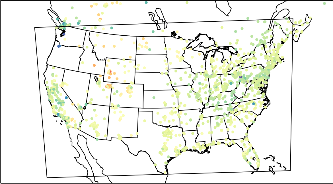
AirNOW (2023-03-19_18:00:00)
