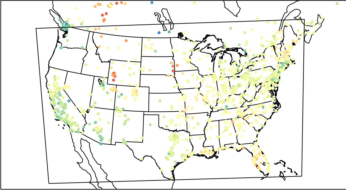
AirNOW (2023-03-20_22:00:00)
