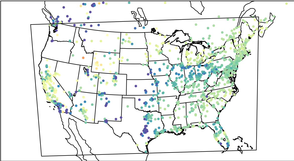
AirNOW (2023-03-19_13:00:00)
