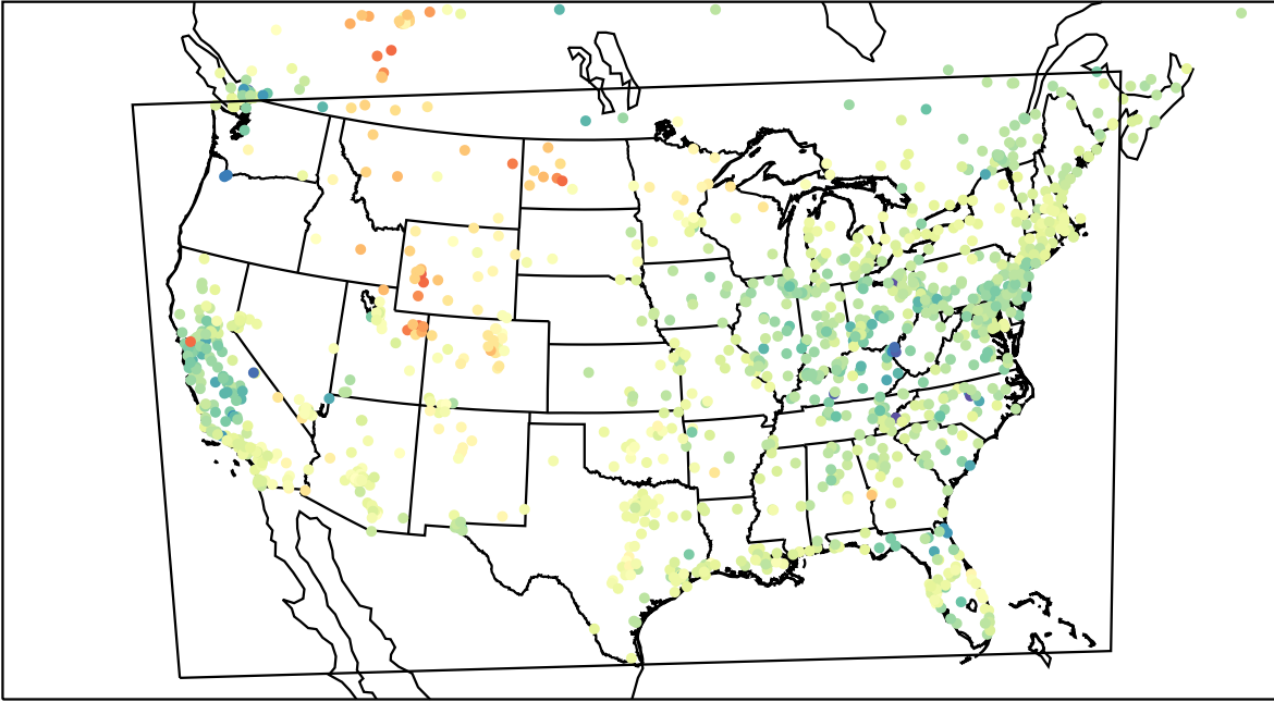
AirNOW (2023-03-20_00:00:00)
