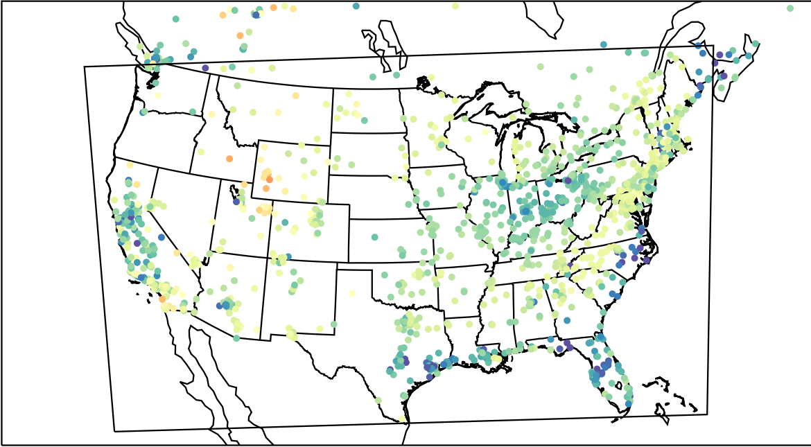
AirNOW (2023-03-19_02:00:00)
