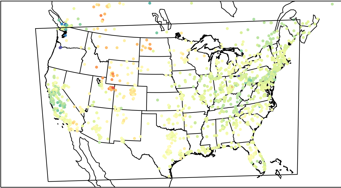
AirNOW (2023-03-19_20:00:00)
