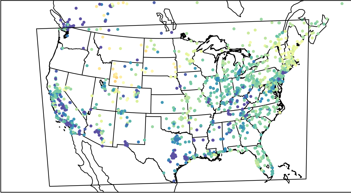
AirNOW (2023-03-20_13:00:00)
