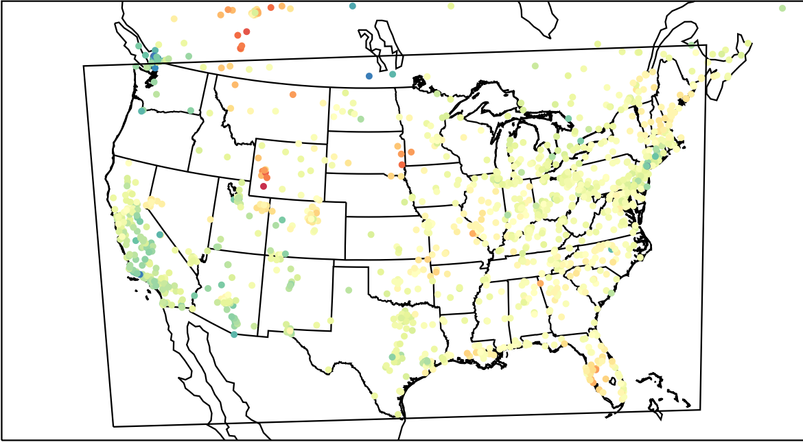
AirNOW (2023-03-20_21:00:00)
