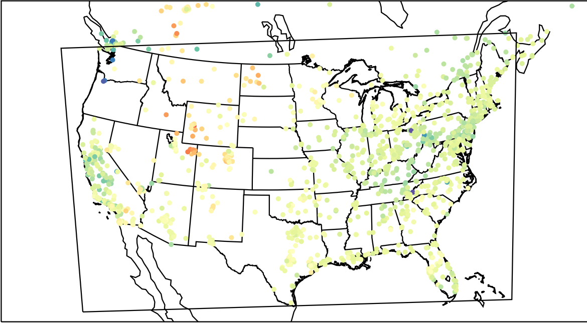
AirNOW (2023-03-19_19:00:00)
