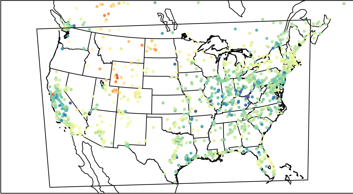
AirNOW (2023-03-20_01:00:00)
