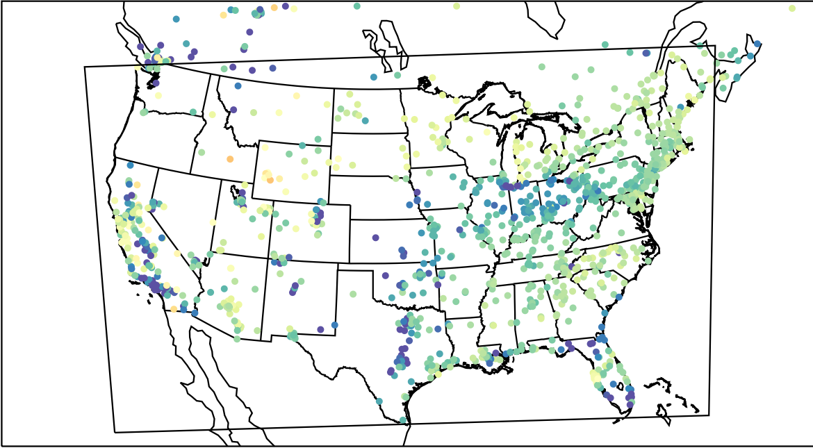
AirNOW (2023-03-19_09:00:00)
