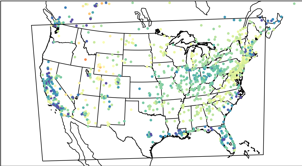
AirNOW (2023-03-19_04:00:00)
