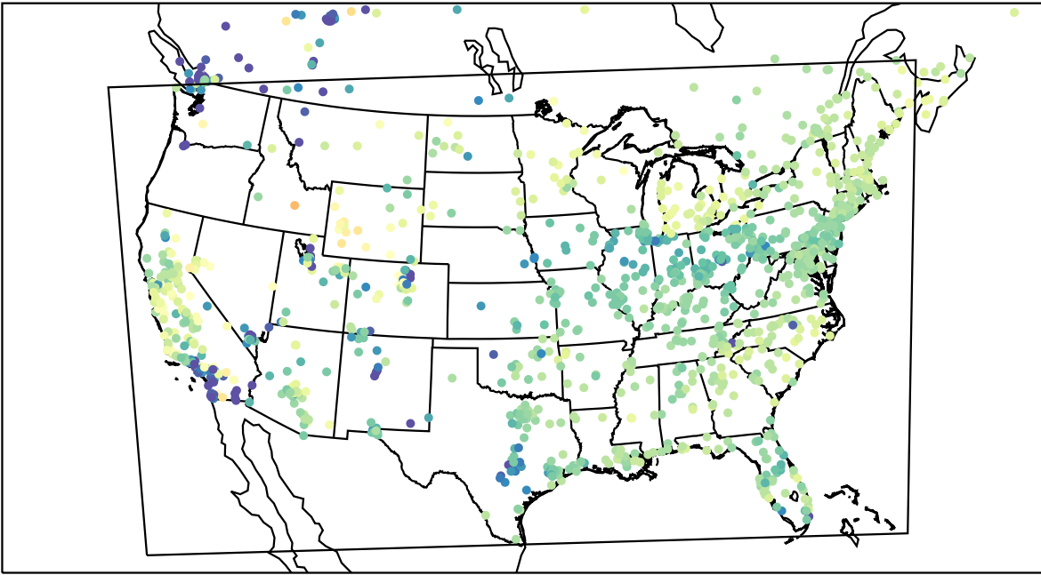
AirNOW (2023-03-19_14:00:00)
