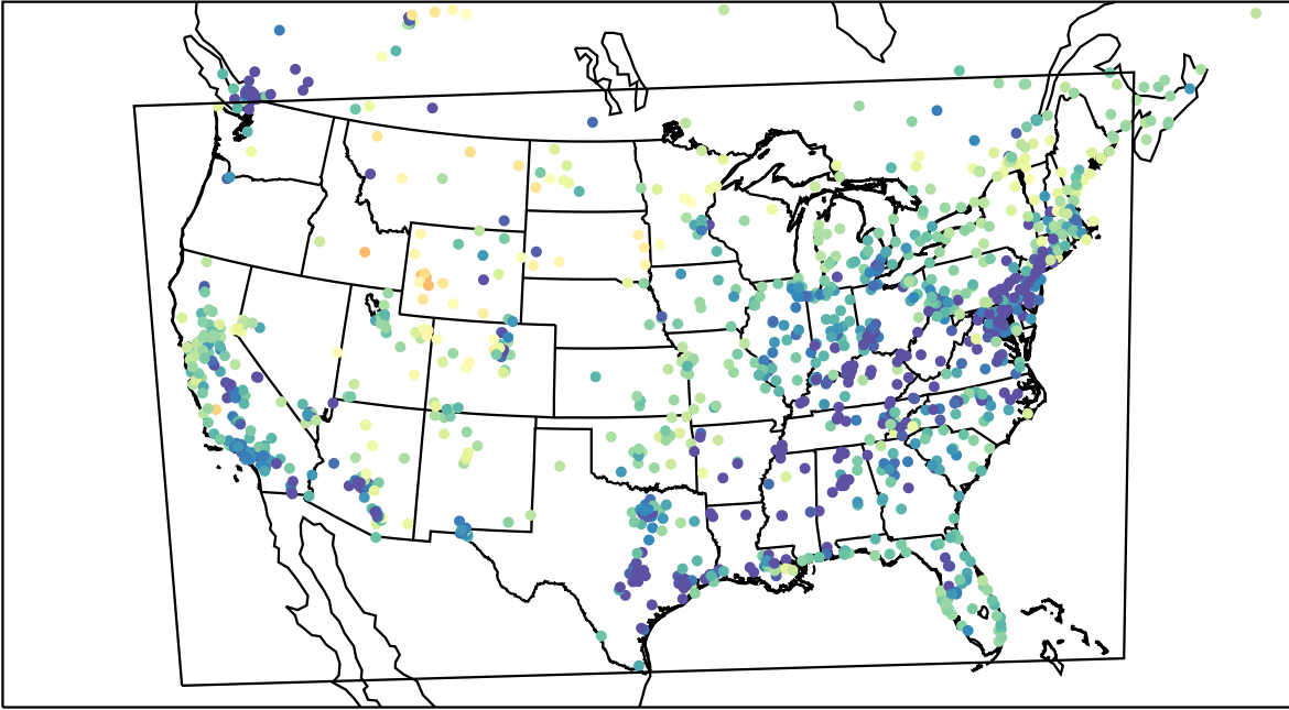
AirNOW (2023-03-20_10:00:00)
