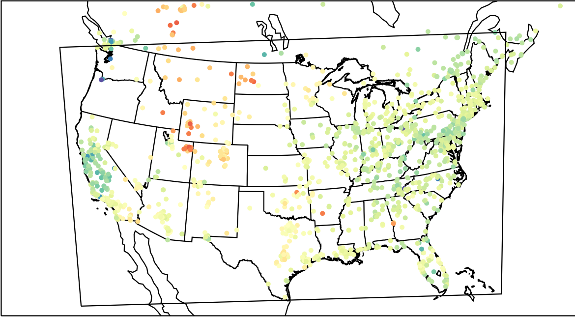
AirNOW (2023-03-19_23:00:00)
