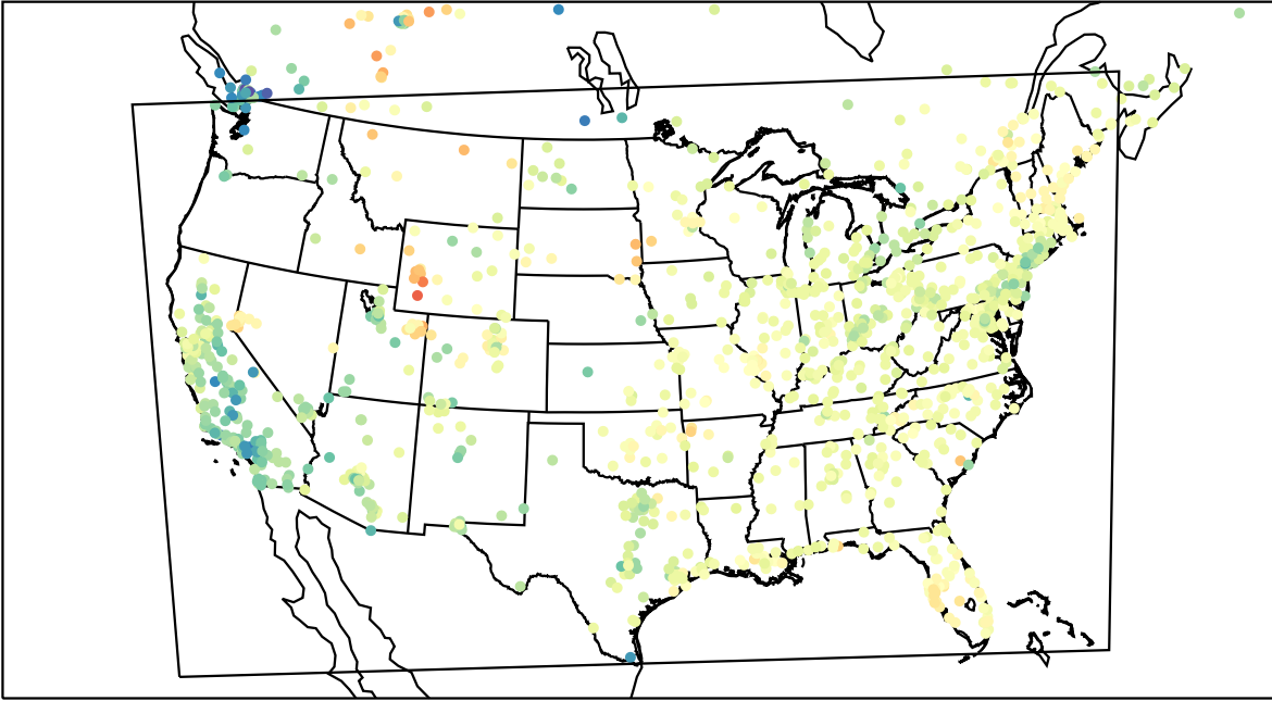
AirNOW (2023-03-20_18:00:00)
