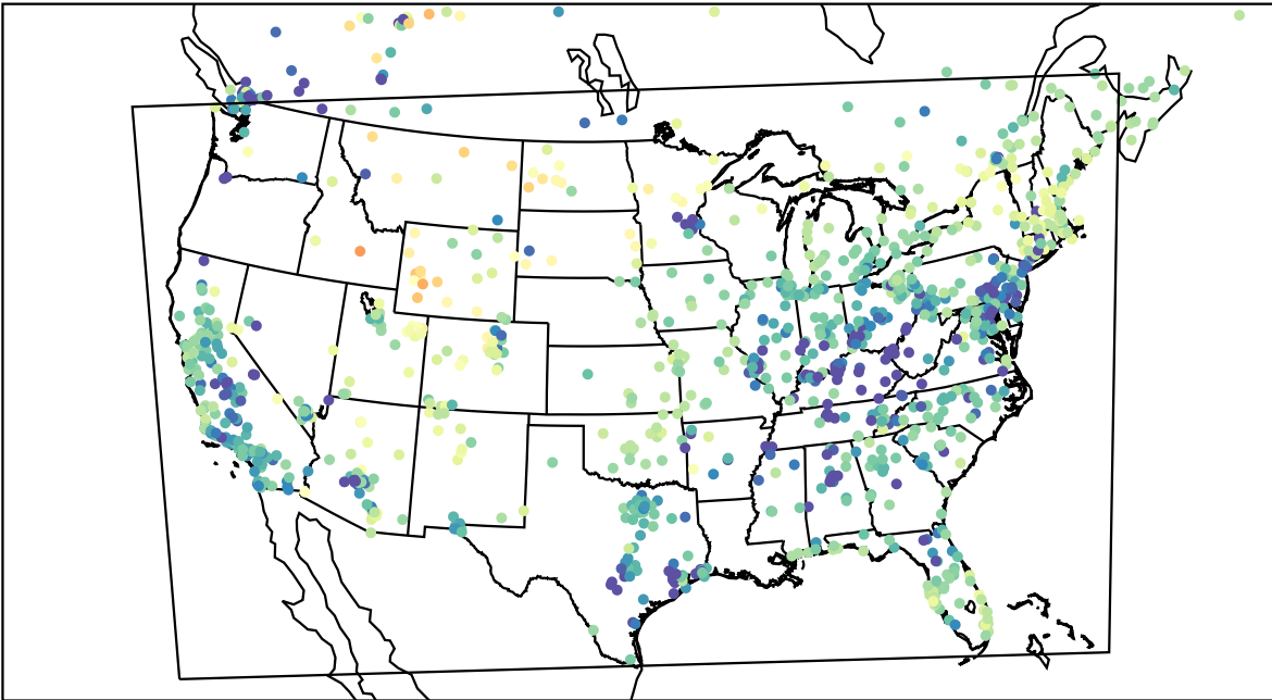
AirNOW (2023-03-20_07:00:00)
