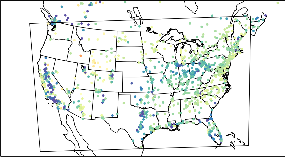
AirNOW (2023-03-19_07:00:00)
