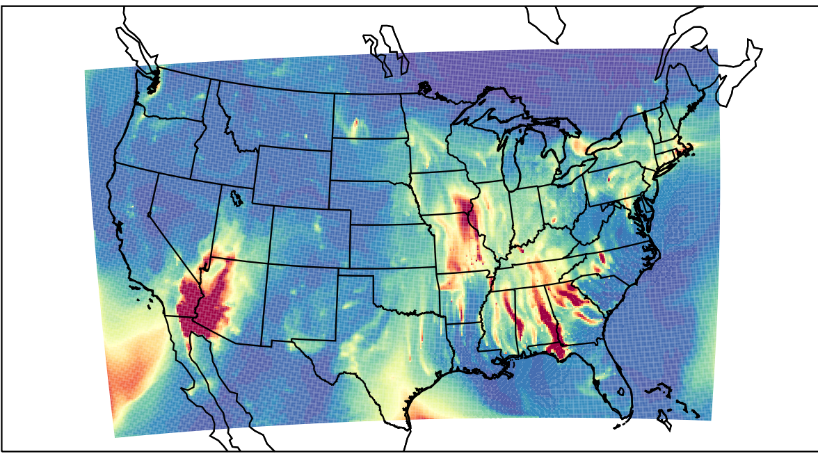
WRF 2023-03-22_05:00:00
