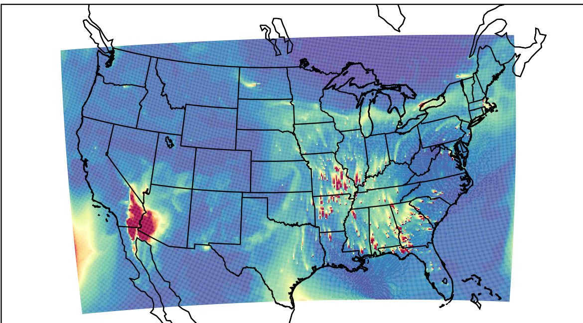
WRF 2023-03-21_21:00:00
