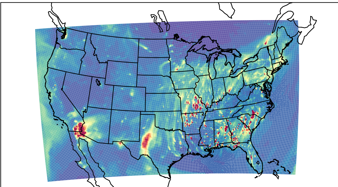
WRF 2023-03-21_02:00:00
