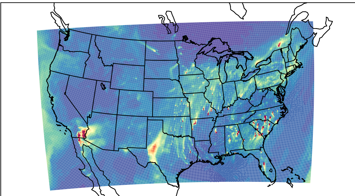
WRF 2023-03-21_00:00:00
