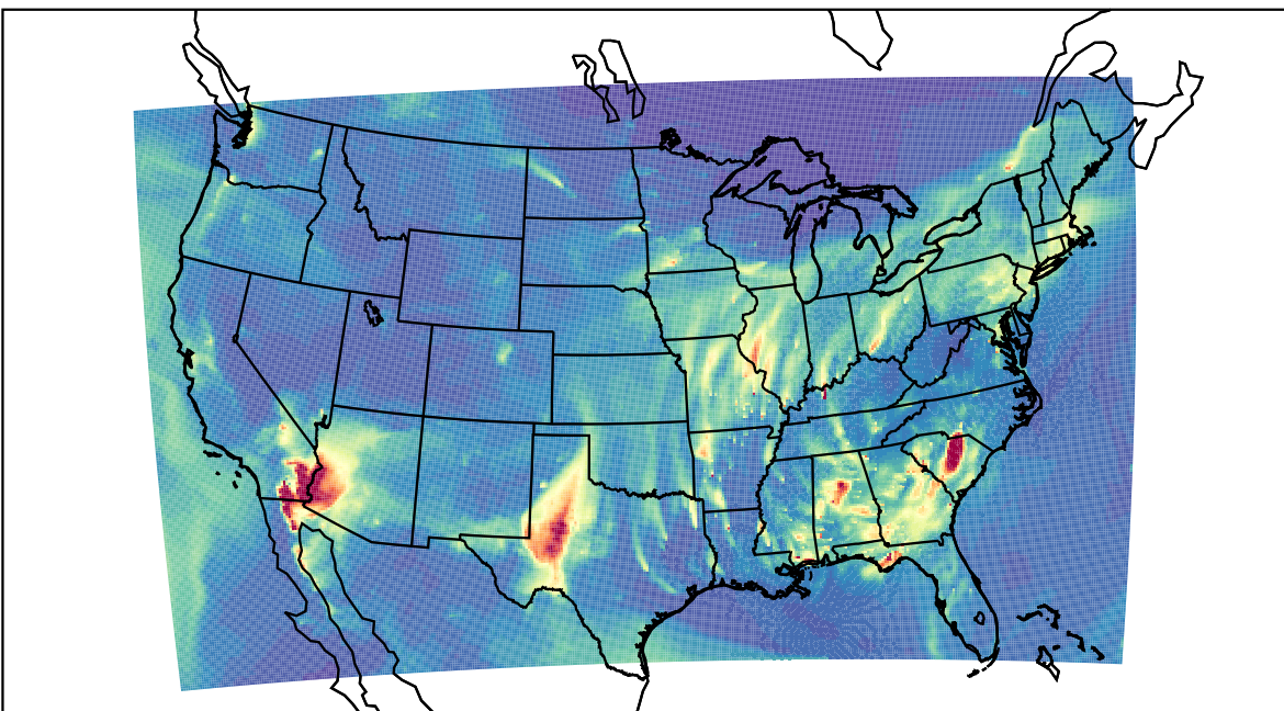
WRF 2023-03-21_07:00:00
