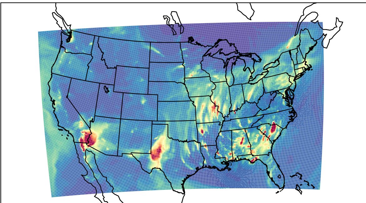
WRF 2023-03-21_05:00:00
