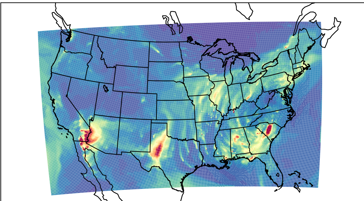
WRF 2023-03-21_09:00:00
