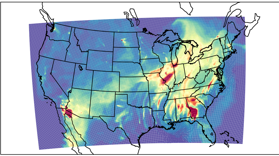
WRF 2023-03-23_07:00:00
