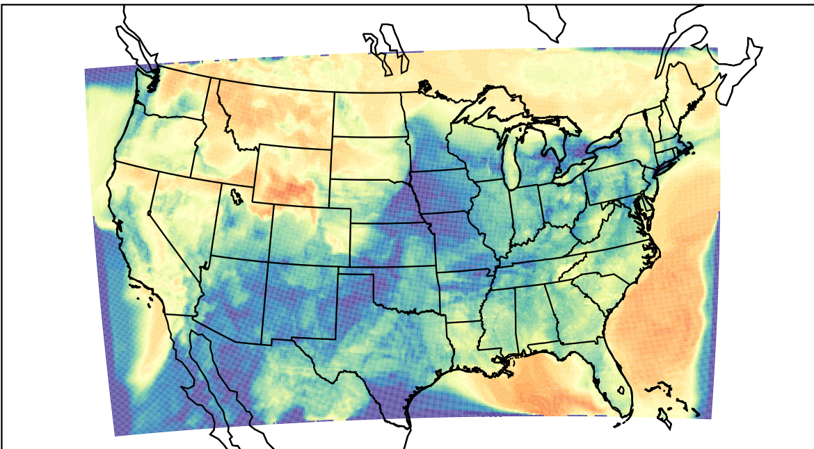
WRF (2023-03-22_07:00:00)
