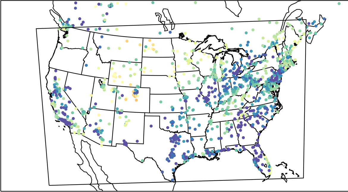
AirNOW (2023-03-23_11:00:00)
