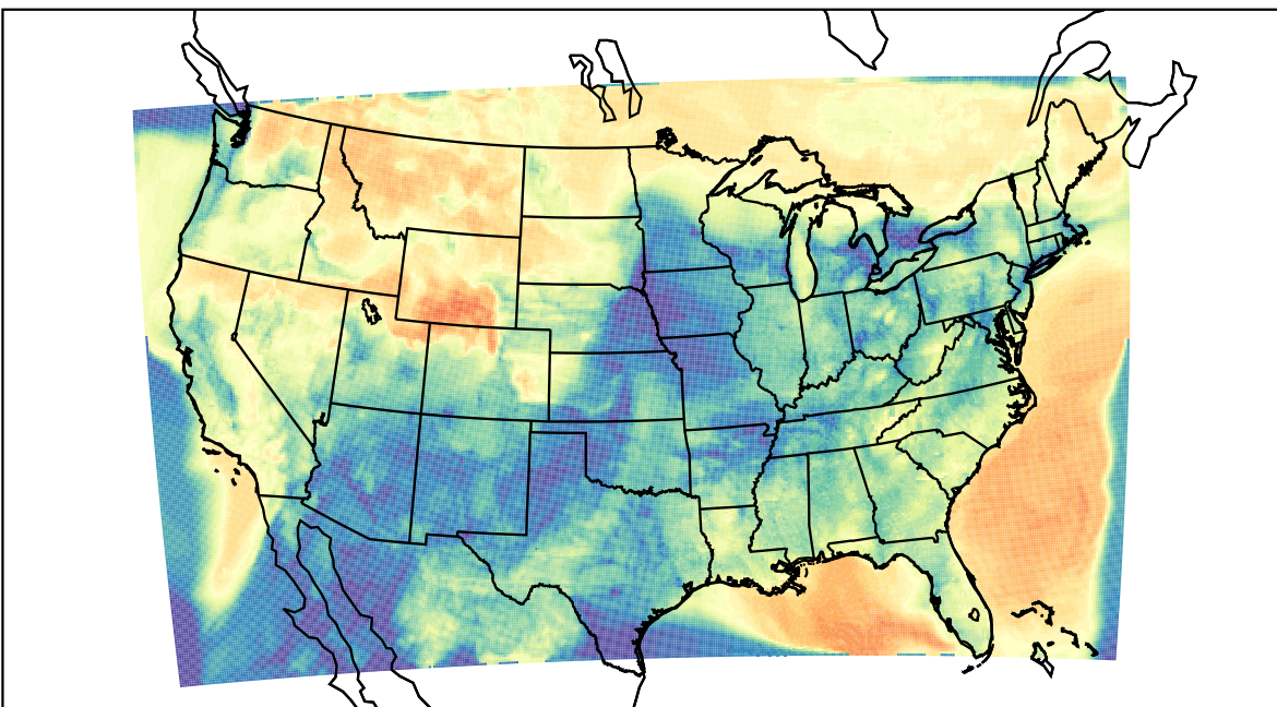
WRF (2023-03-22_06:00:00)
