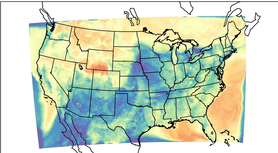
WRF (2023-03-22_05:00:00)
