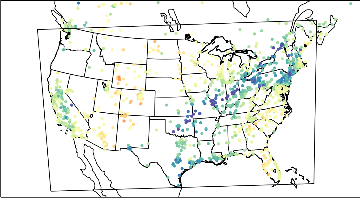
AirNOW (2023-03-23_19:00:00)
