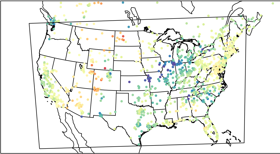
AirNOW (2023-03-22_23:00:00)
