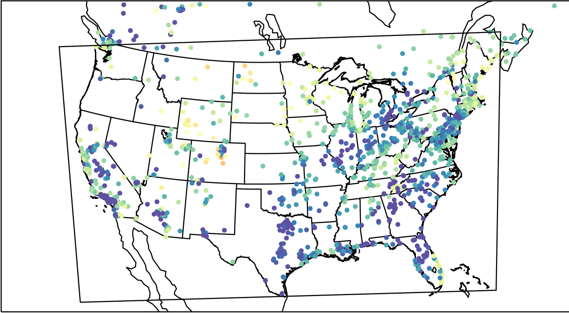
AirNOW (2023-03-23_12:00:00)
