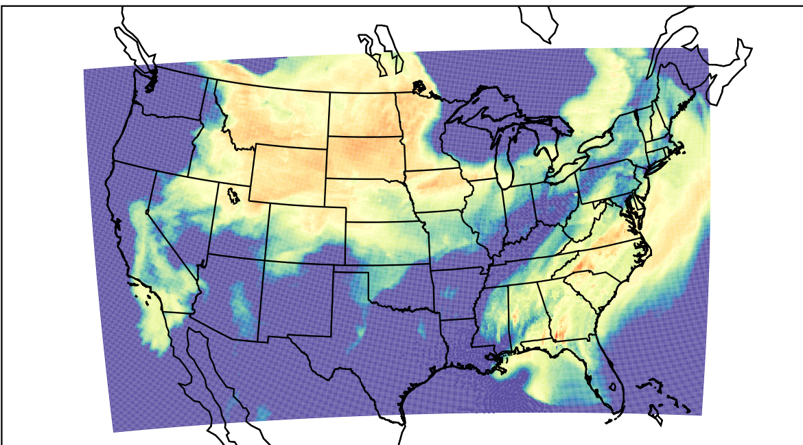
WRF (2023-03-23_23:00:00)
