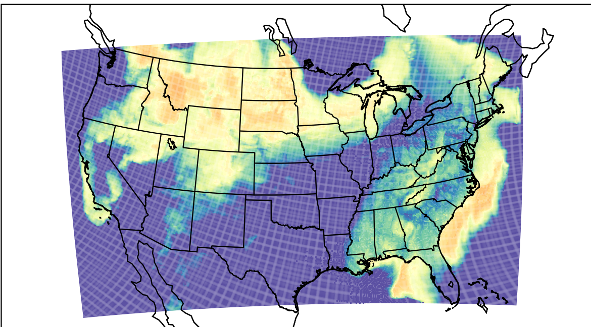
WRF (2023-03-23_11:00:00)
