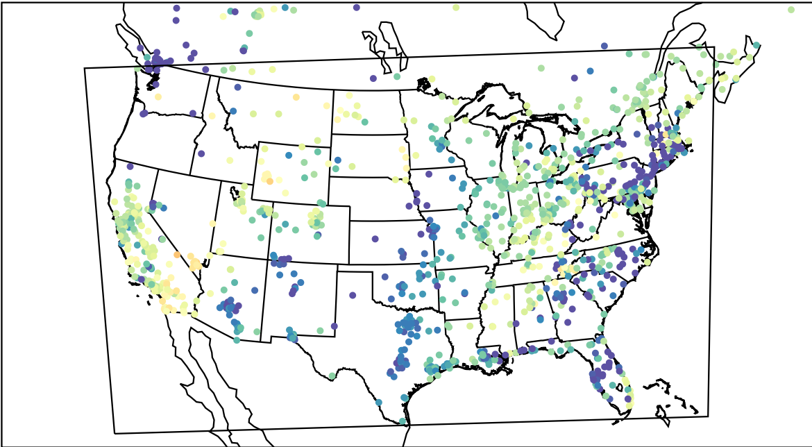
AirNOW (2023-03-22_09:00:00)
