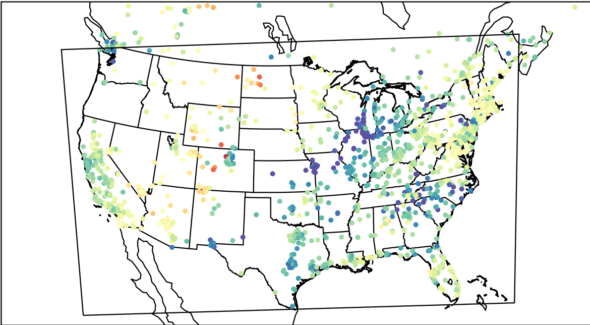
AirNOW (2023-03-23_01:00:00)
