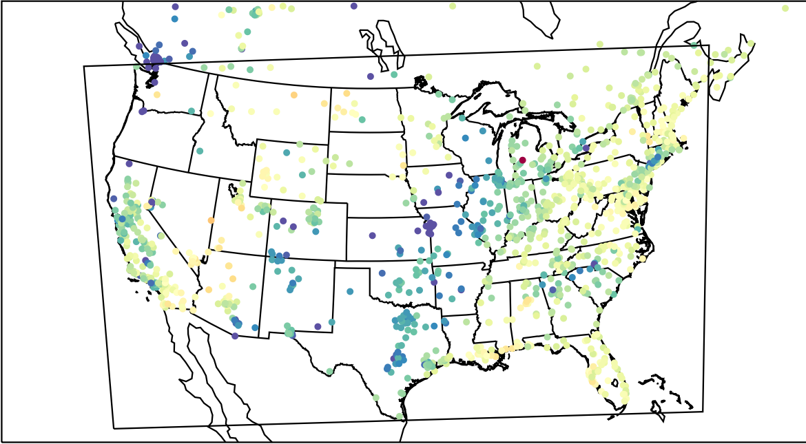
AirNOW (2023-03-22_16:00:00)
