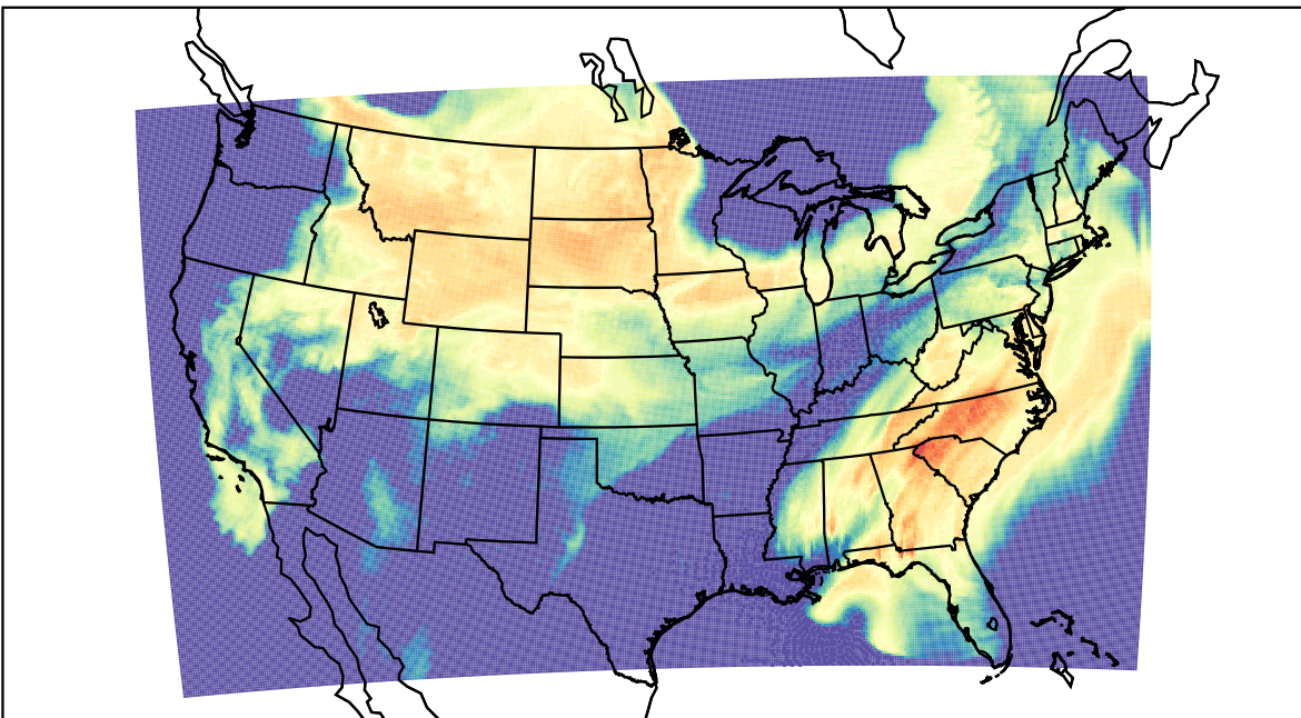
WRF (2023-03-23_20:00:00)
