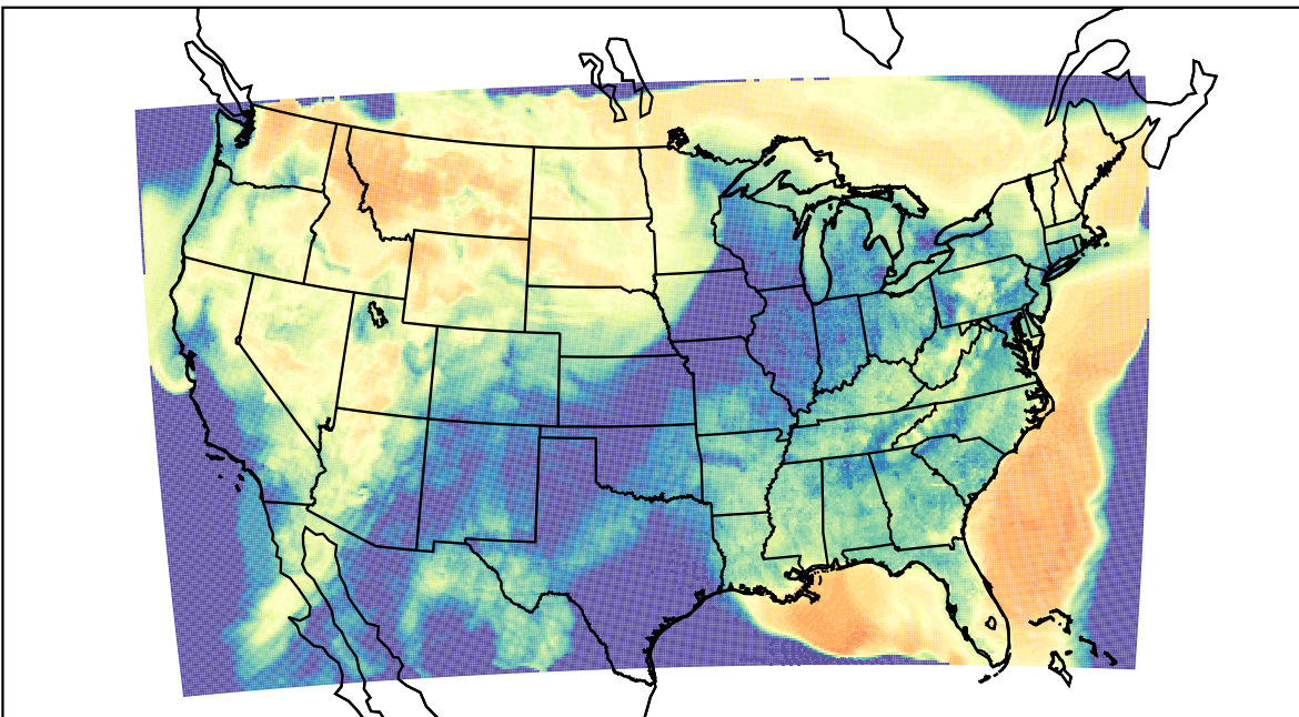
WRF (2023-03-22_14:00:00)
