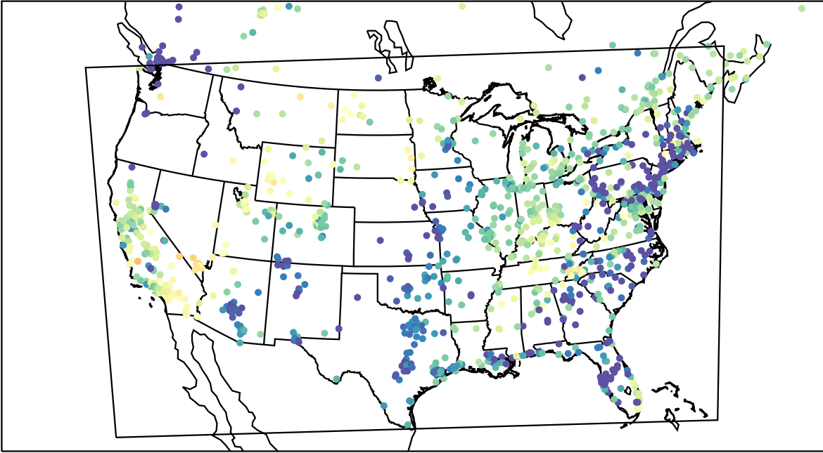
AirNOW (2023-03-22_10:00:00)
