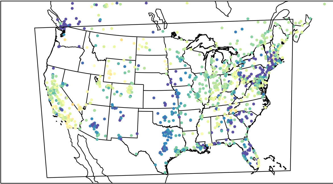
AirNOW (2023-03-22_08:00:00)
