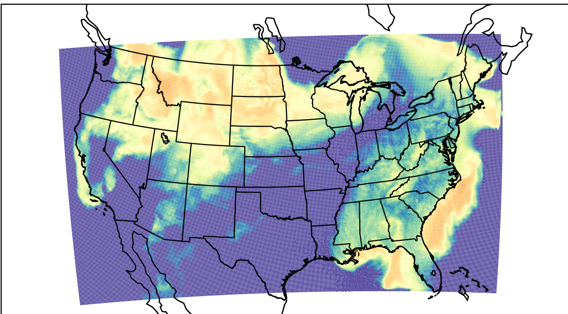
WRF (2023-03-23_08:00:00)
