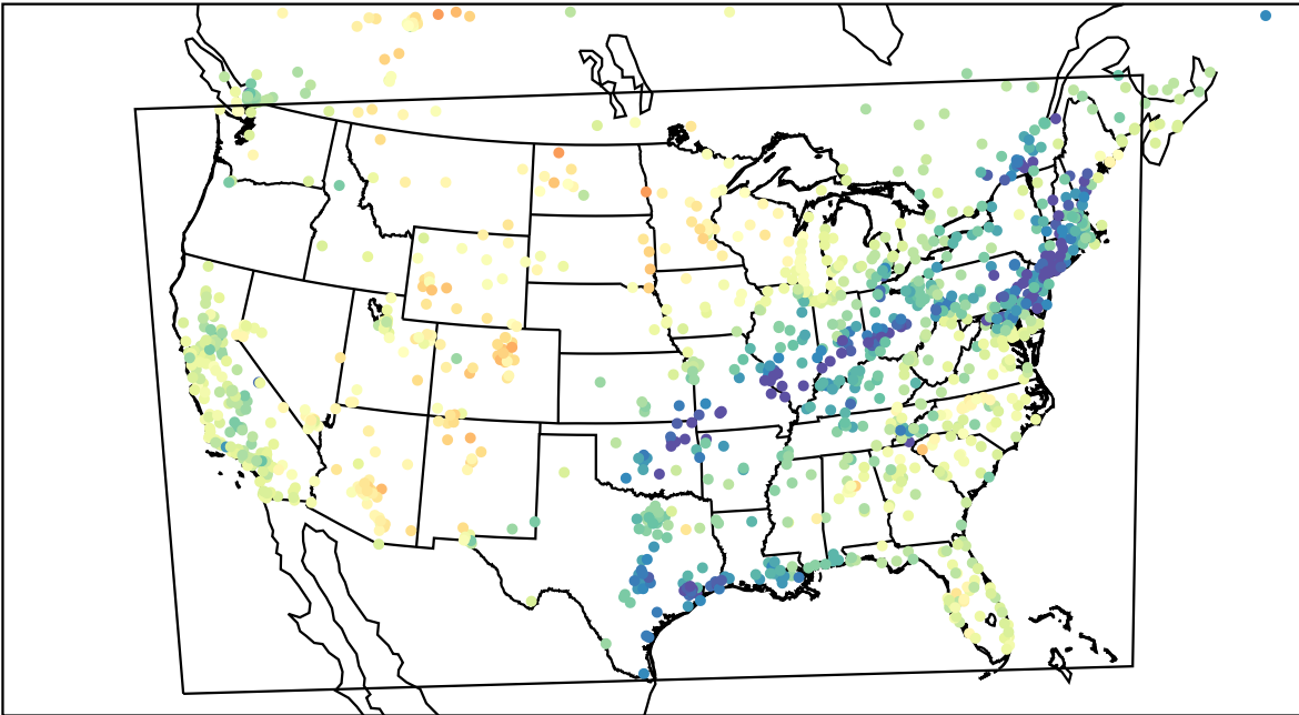
AirNOW (2023-03-23_23:00:00)
