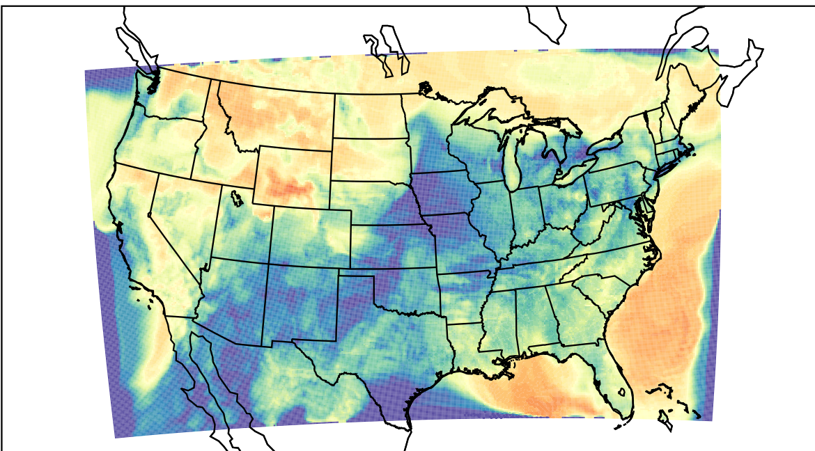
WRF (2023-03-22_08:00:00)
