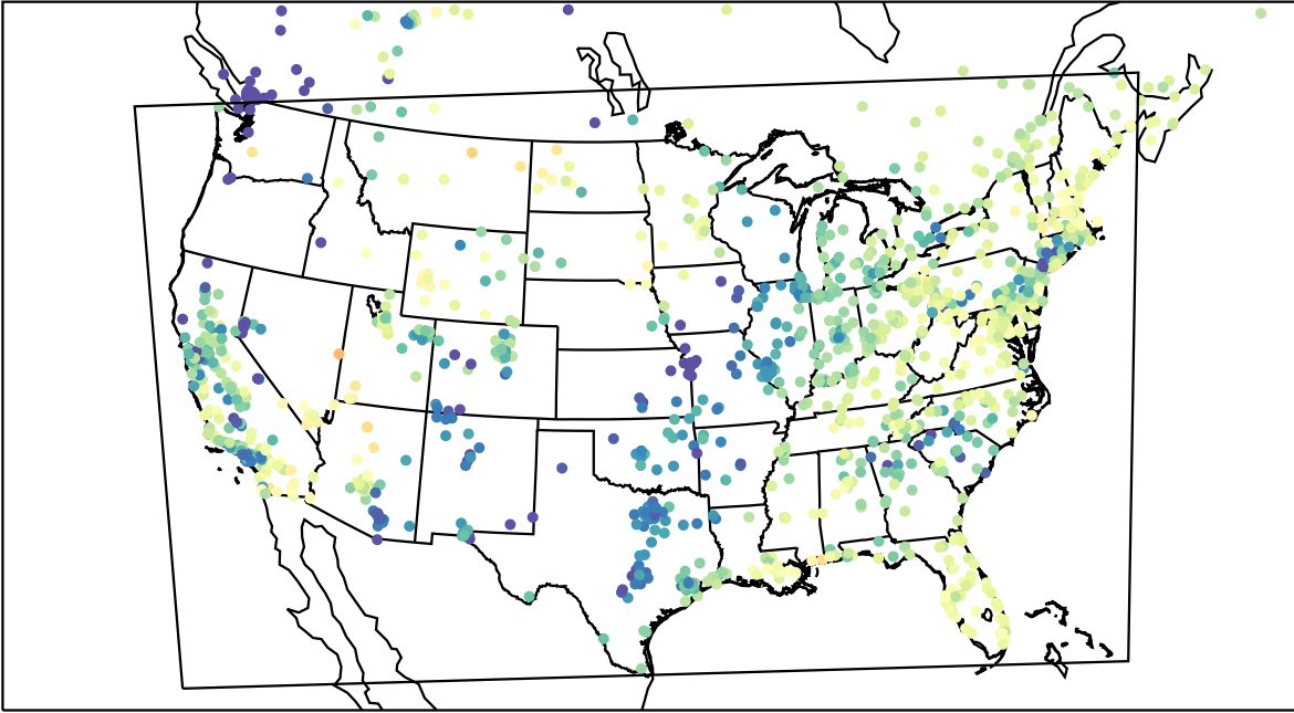
AirNOW (2023-03-22_15:00:00)
