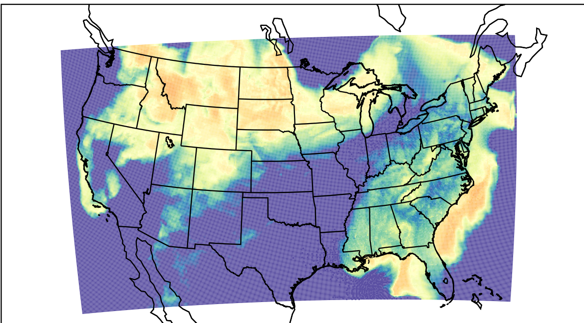
WRF (2023-03-23_09:00:00)
