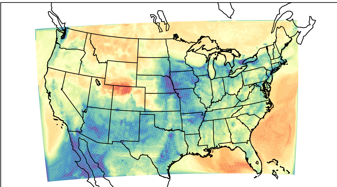
WRF (2023-03-22_02:00:00)
