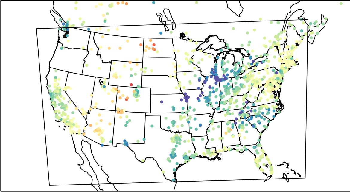
AirNOW (2023-03-23_00:00:00)
