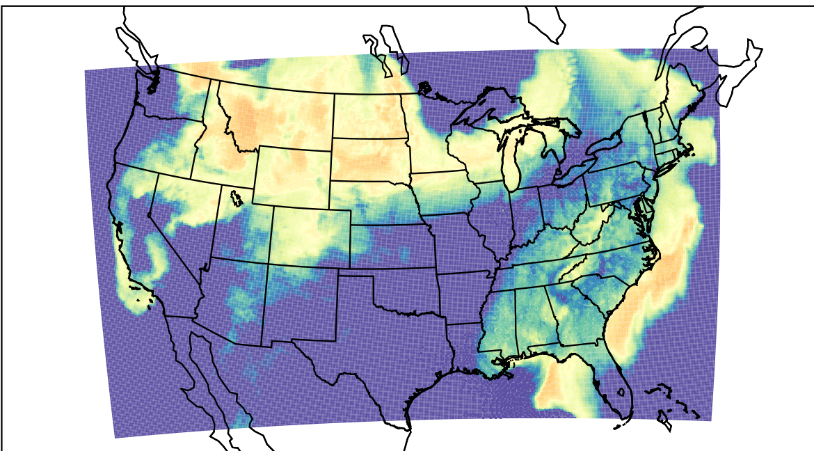
WRF (2023-03-23_12:00:00)
