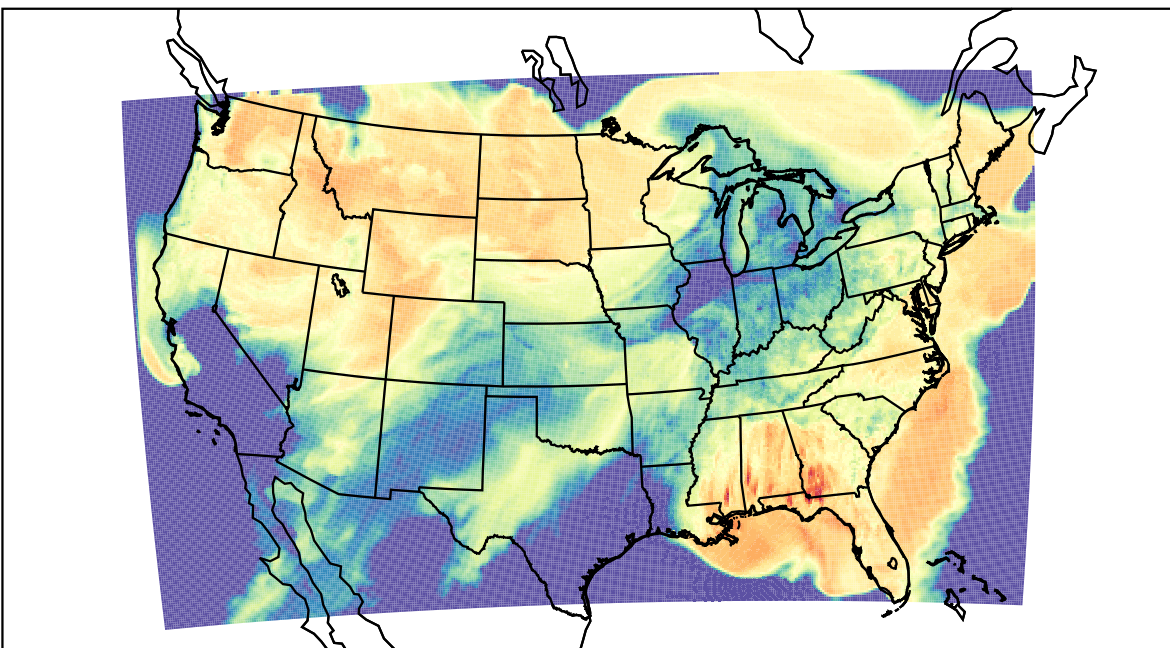
WRF (2023-03-22_22:00:00)
