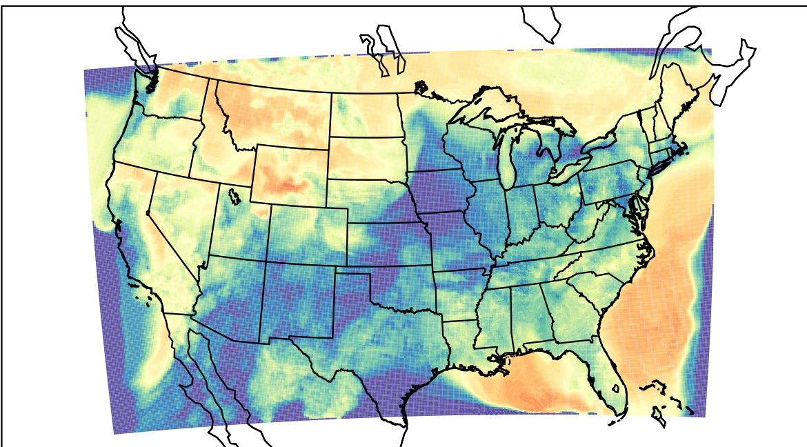
WRF (2023-03-22_09:00:00)
