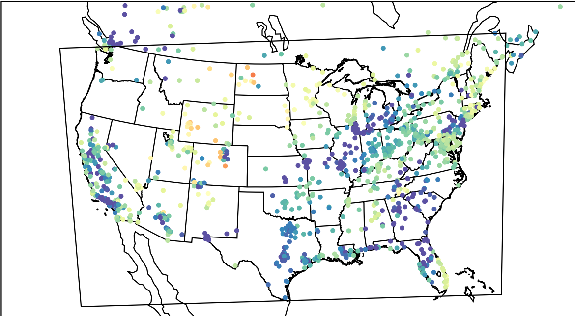
AirNOW (2023-03-23_08:00:00)
