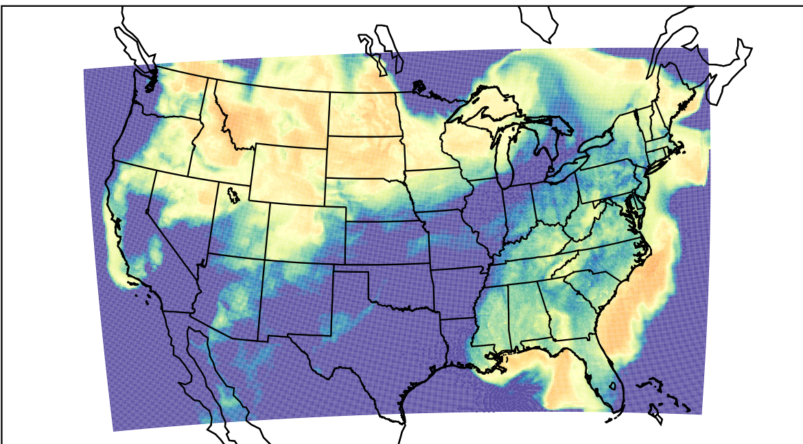
WRF (2023-03-23_07:00:00)
