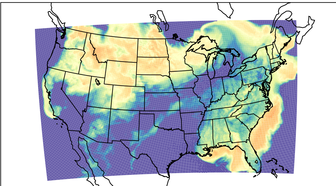
WRF (2023-03-23_05:00:00)
