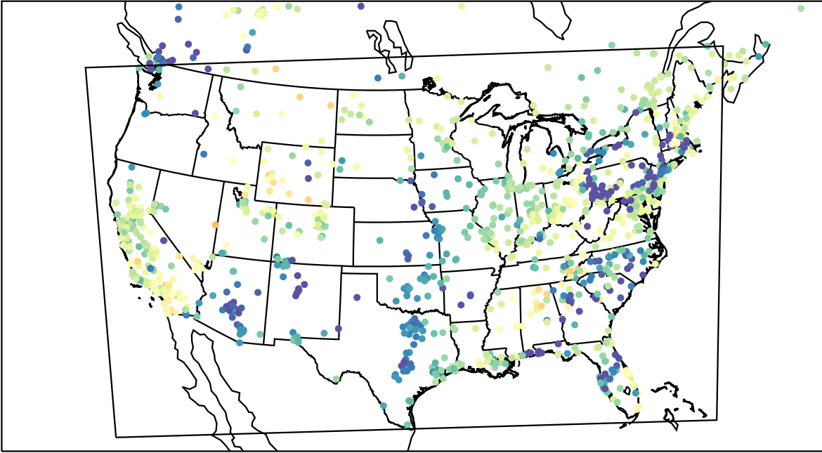
AirNOW (2023-03-22_05:00:00)
