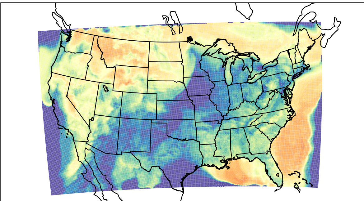
WRF (2023-03-22_11:00:00)
