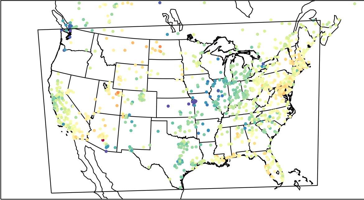
AirNOW (2023-03-22_19:00:00)
