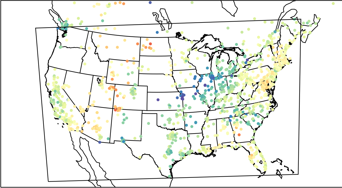
AirNOW (2023-03-22_22:00:00)
