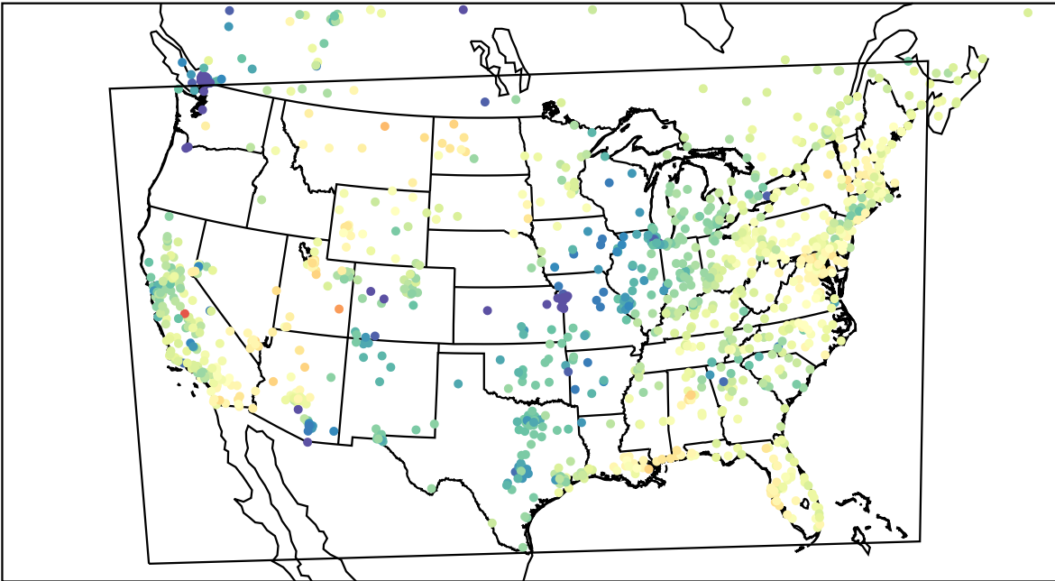
AirNOW (2023-03-22_17:00:00)
