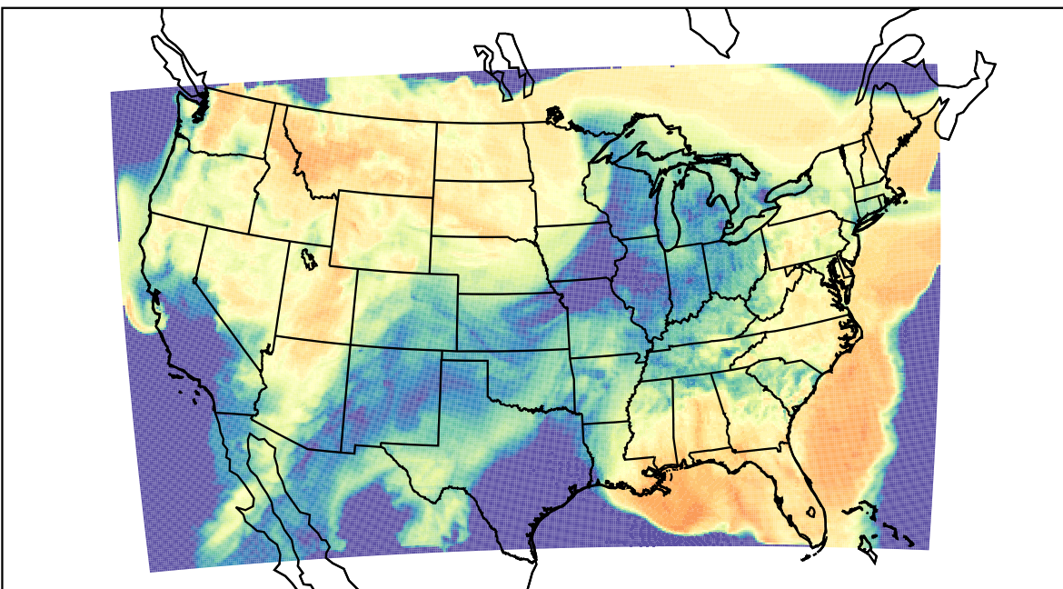
WRF (2023-03-22_17:00:00)
