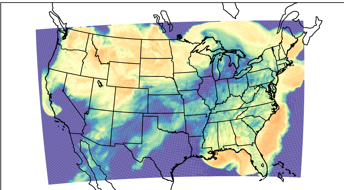
WRF (2023-03-23_01:00:00)
