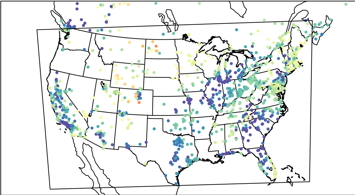
AirNOW (2023-03-23_07:00:00)
