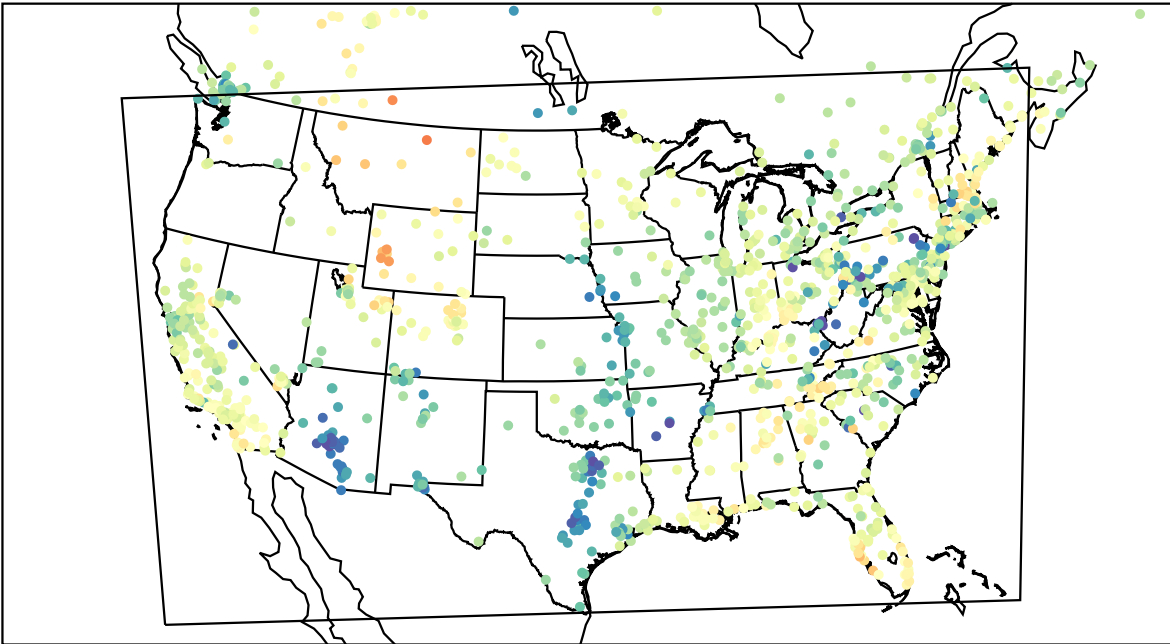
AirNOW (2023-03-22_00:00:00)
