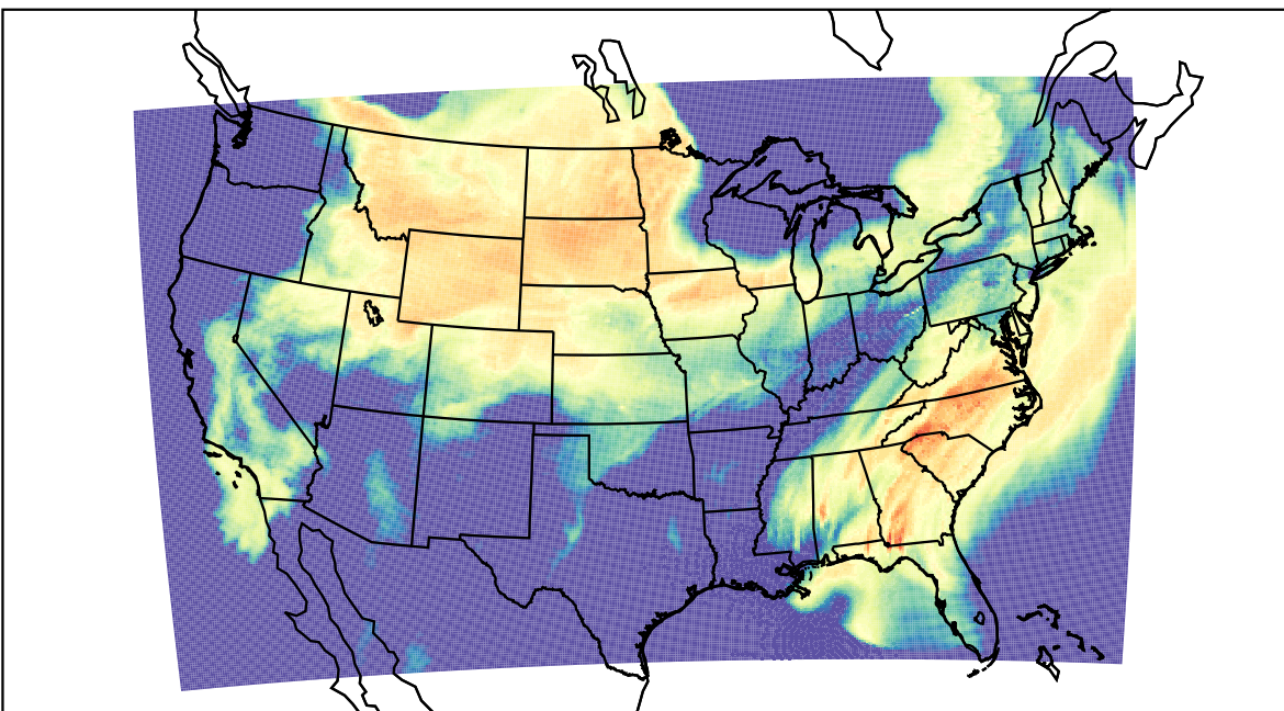
WRF (2023-03-23_22:00:00)
