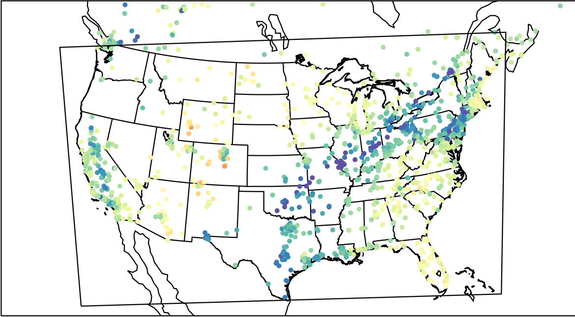
AirNOW (2023-03-23_17:00:00)
