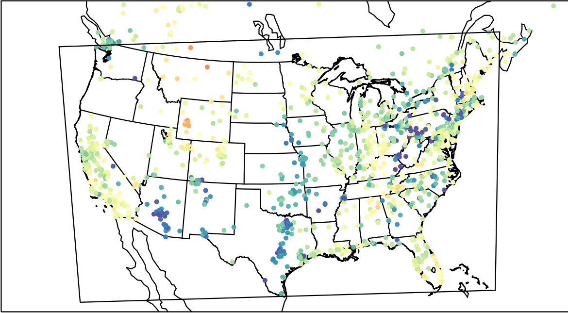
AirNOW (2023-03-22_01:00:00)
