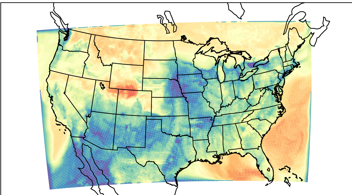
WRF (2023-03-22_03:00:00)
