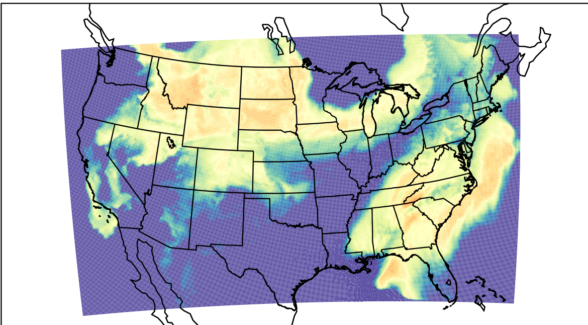
WRF (2023-03-23_16:00:00)
