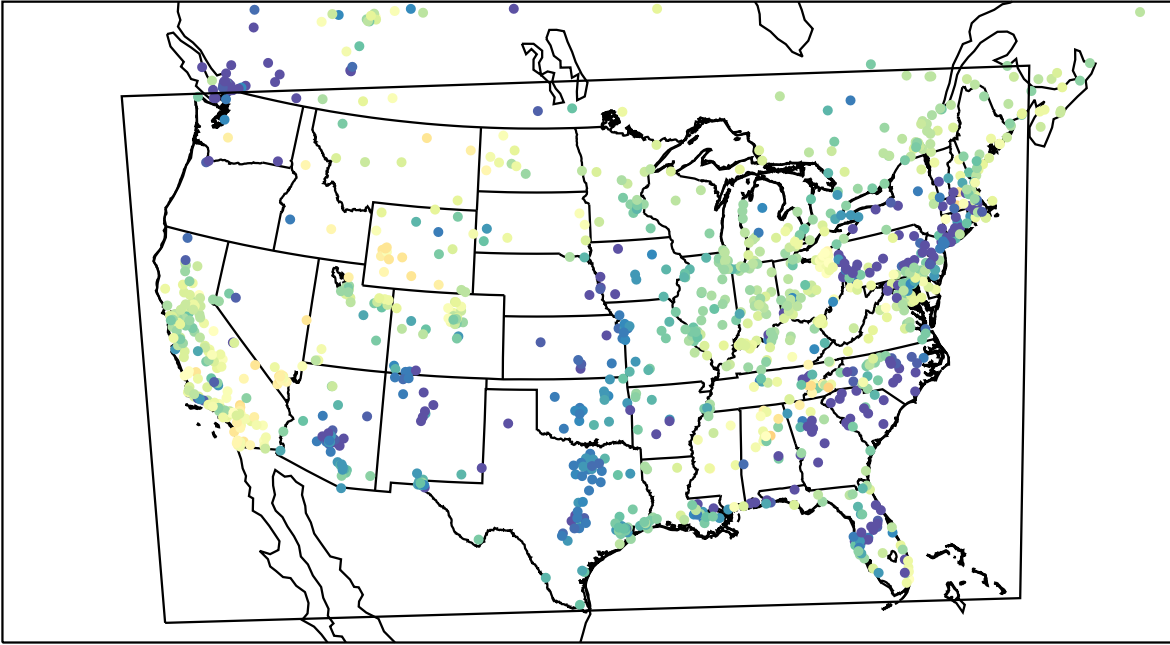
AirNOW (2023-03-22_07:00:00)
