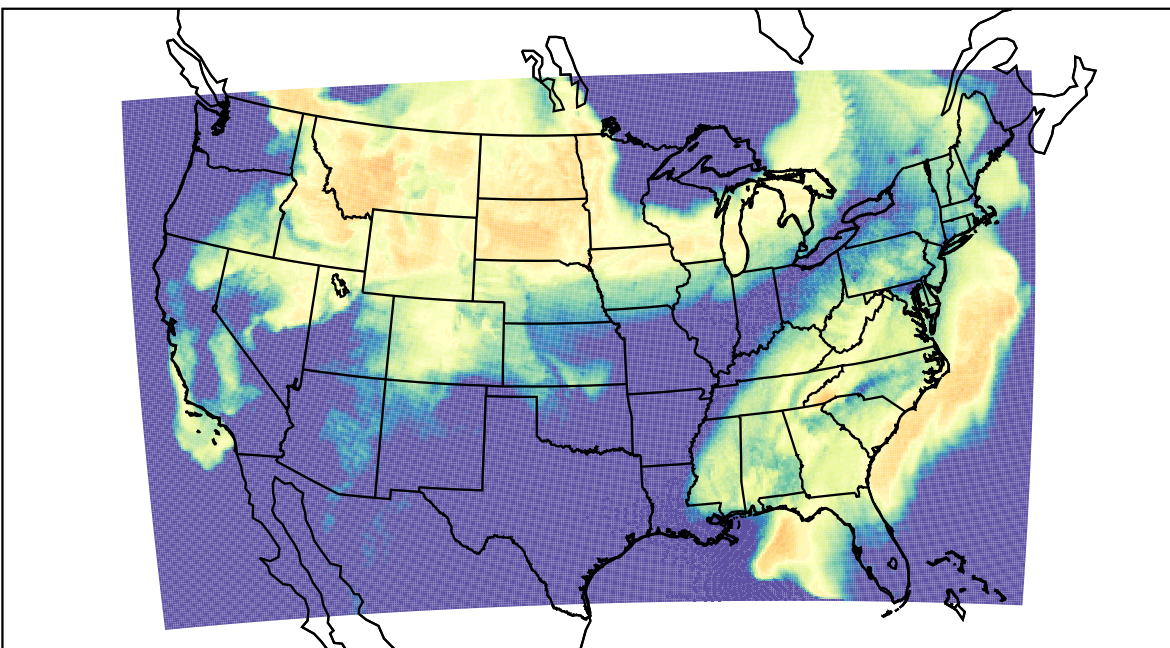
WRF (2023-03-23_15:00:00)
