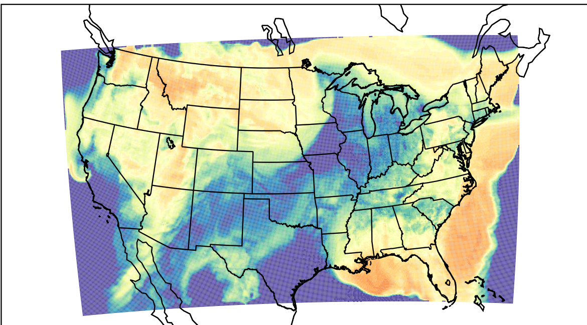
WRF (2023-03-22_16:00:00)
