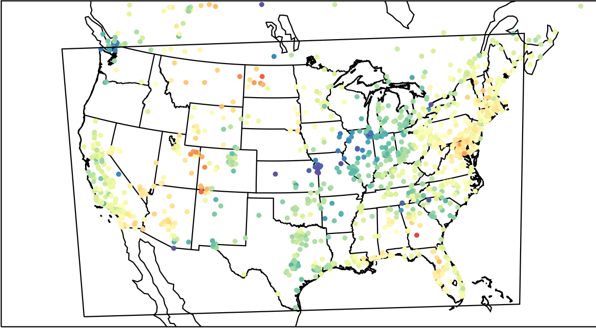
AirNOW (2023-03-22_21:00:00)
