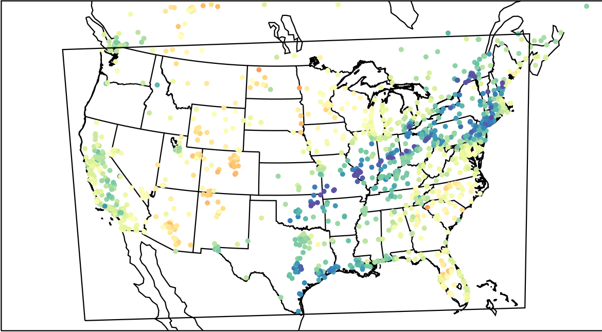
AirNOW (2023-03-23_21:00:00)
