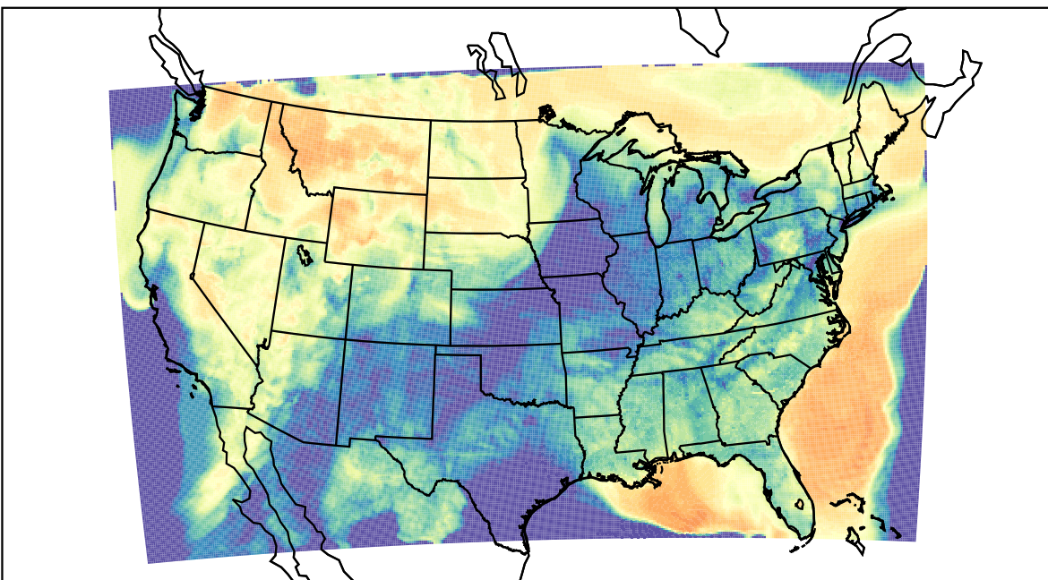
WRF (2023-03-22_12:00:00)
