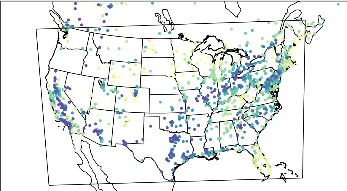
AirNOW (2023-03-23_14:00:00)
