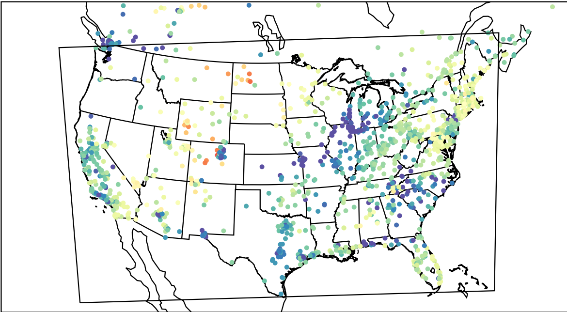
AirNOW (2023-03-23_03:00:00)
