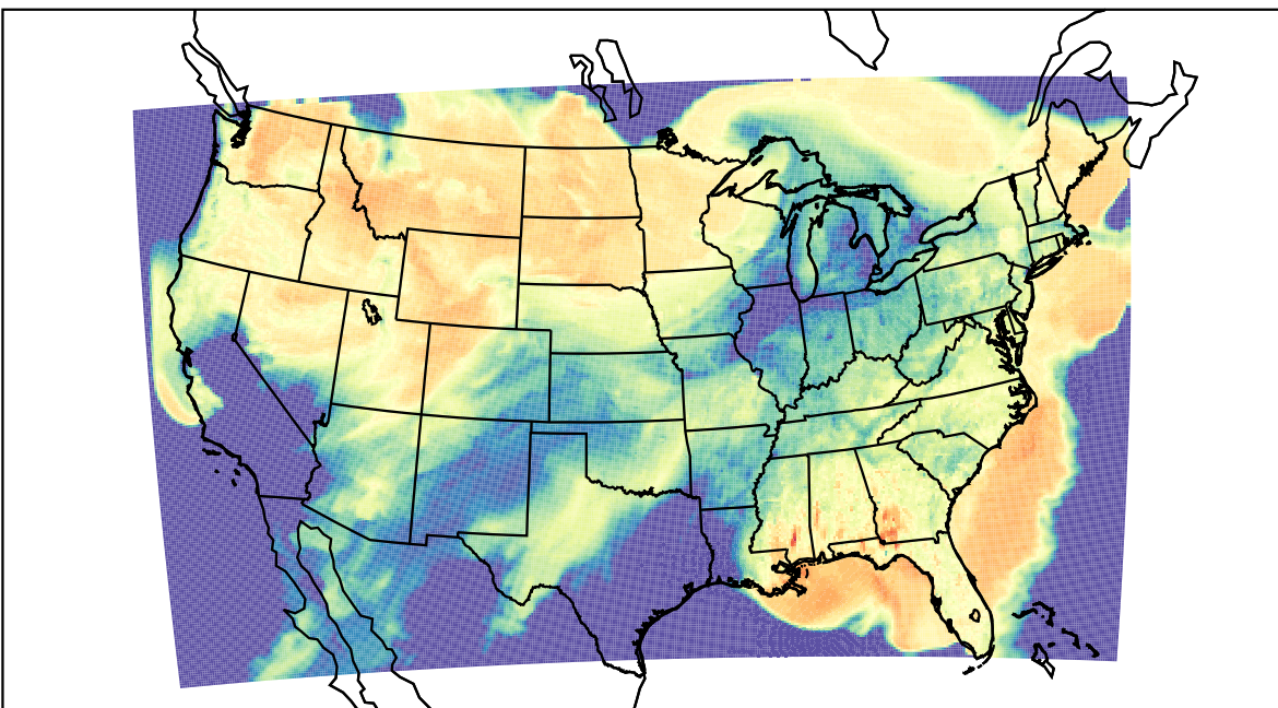
WRF (2023-03-22_23:00:00)
