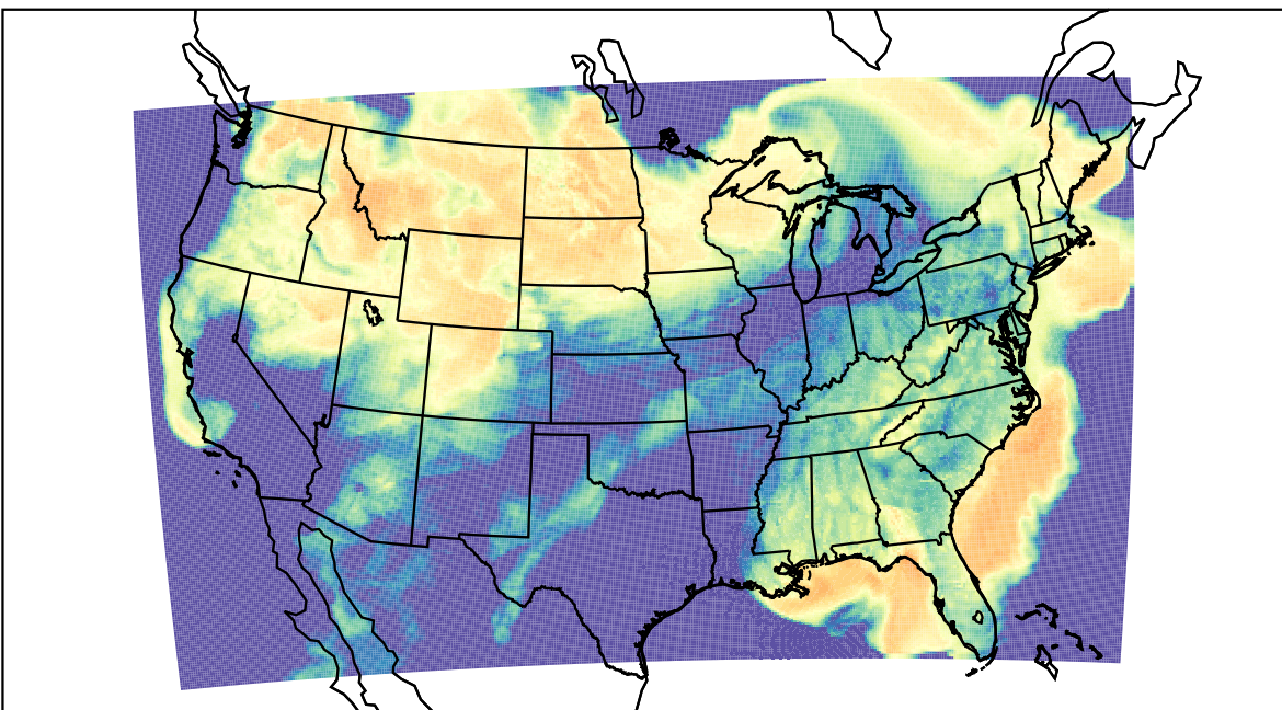
WRF (2023-03-23_04:00:00)
