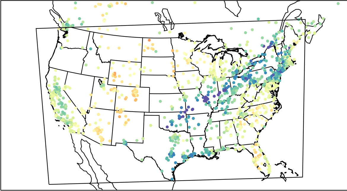
AirNOW (2023-03-23_20:00:00)
