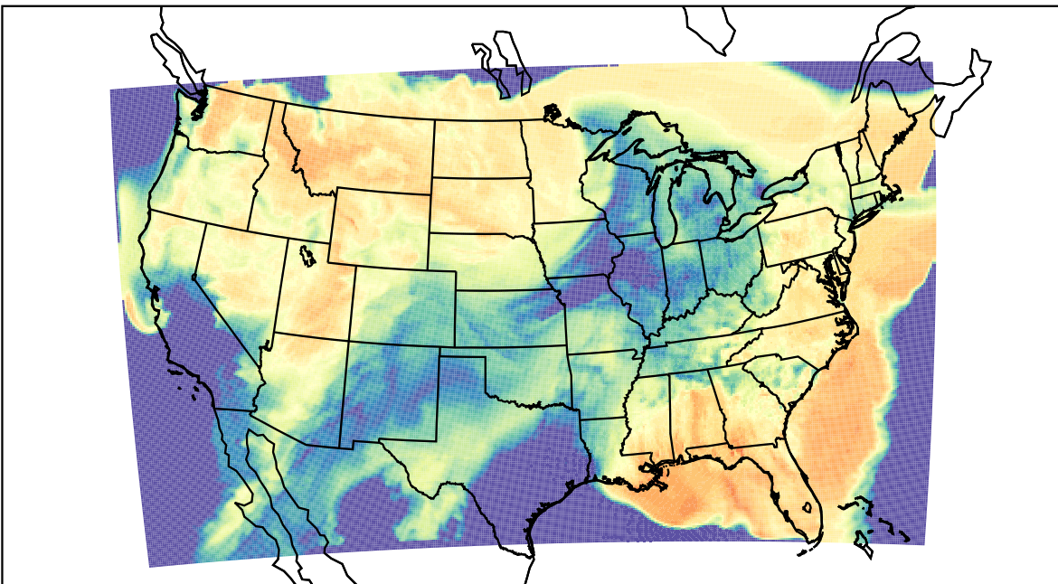
WRF (2023-03-22_18:00:00)
