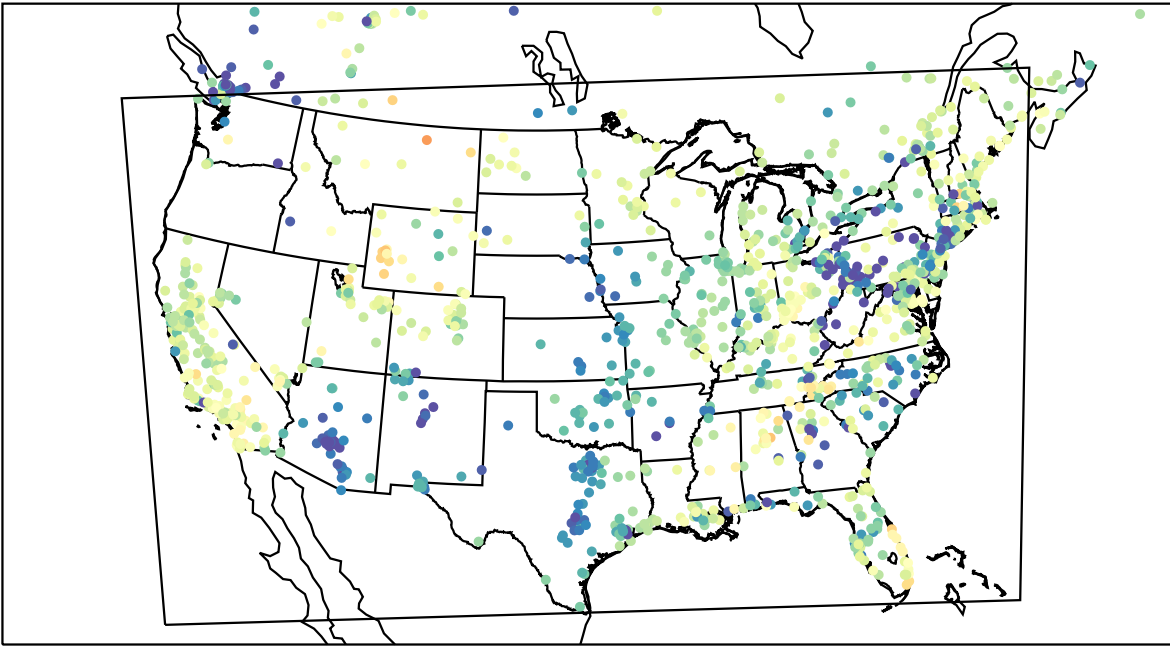
AirNOW (2023-03-22_03:00:00)
