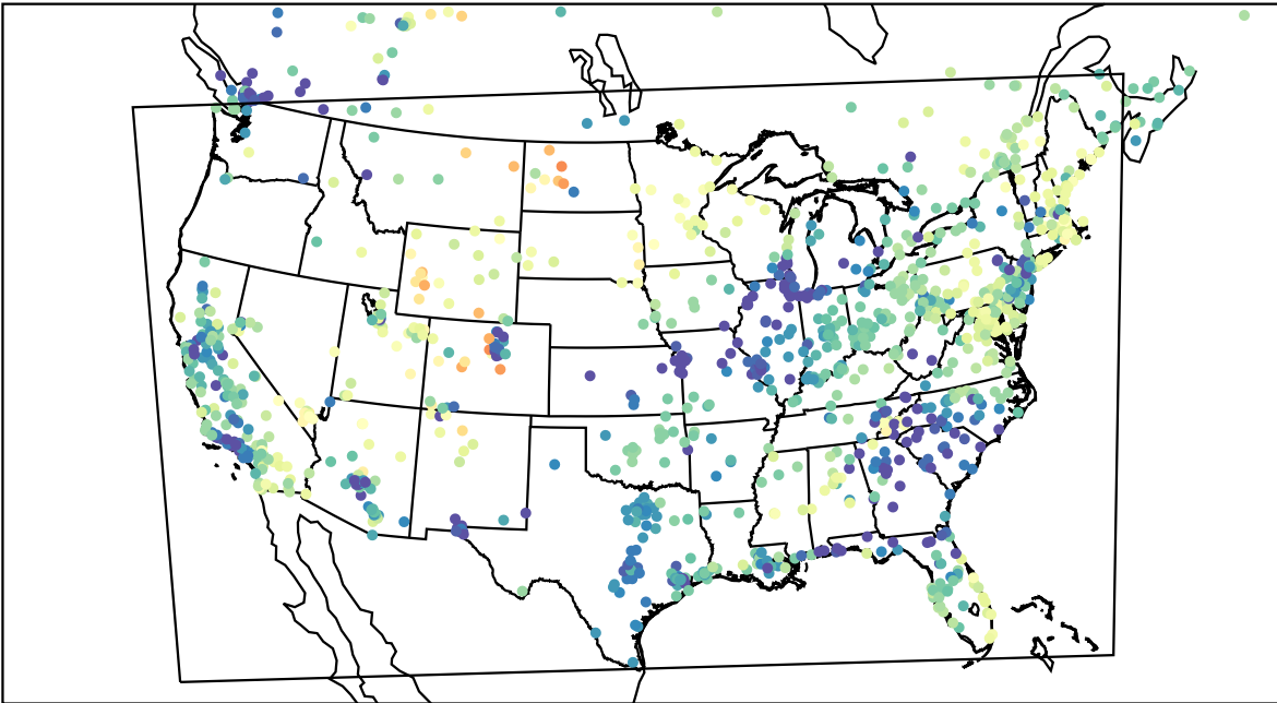
AirNOW (2023-03-23_05:00:00)
