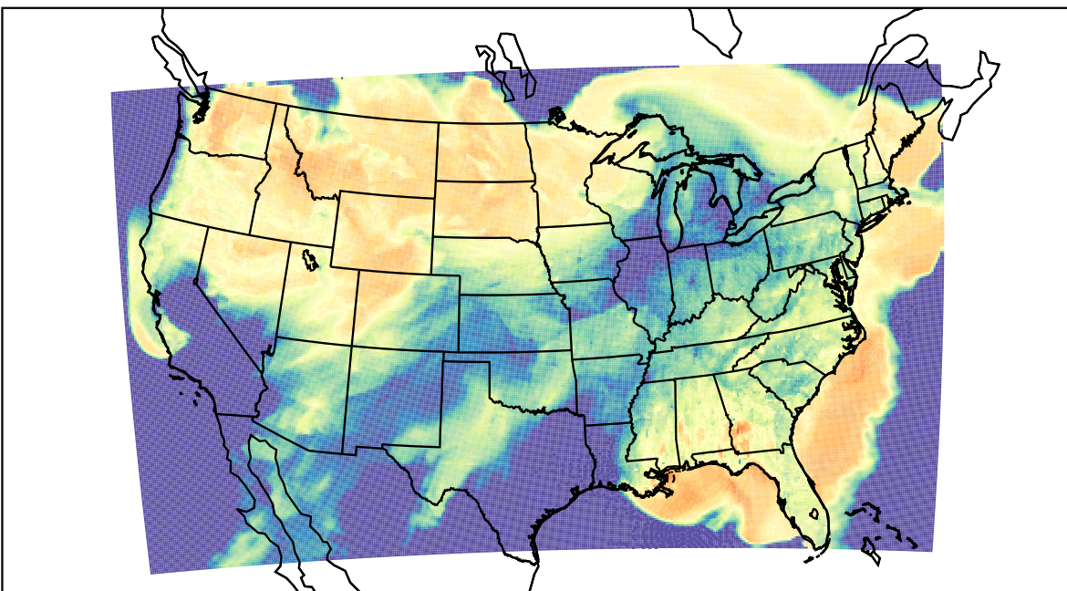
WRF (2023-03-23_00:00:00)
