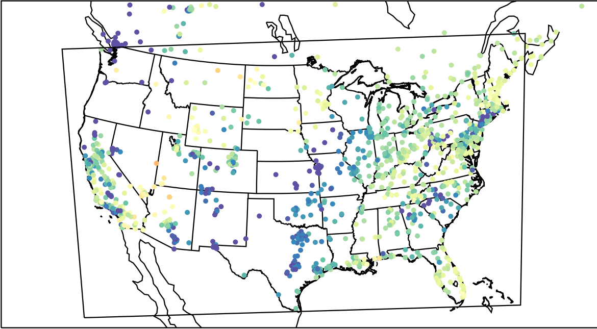
AirNOW (2023-03-22_14:00:00)
