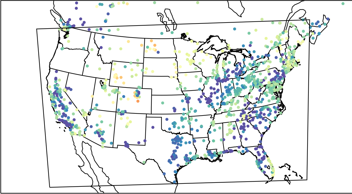
AirNOW (2023-03-23_09:00:00)
