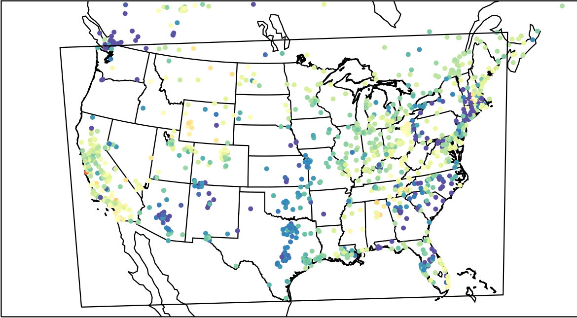
AirNOW (2023-03-22_06:00:00)
