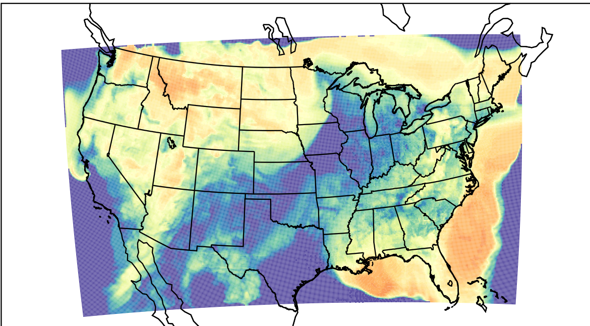
WRF (2023-03-22_15:00:00)
