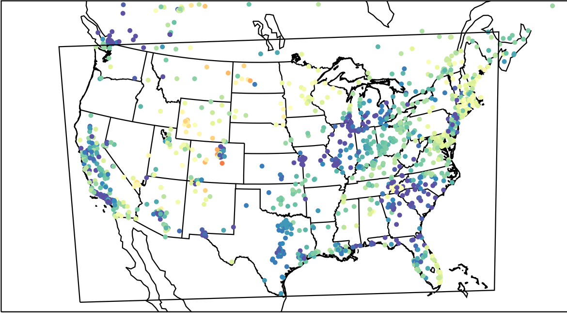
AirNOW (2023-03-23_06:00:00)
