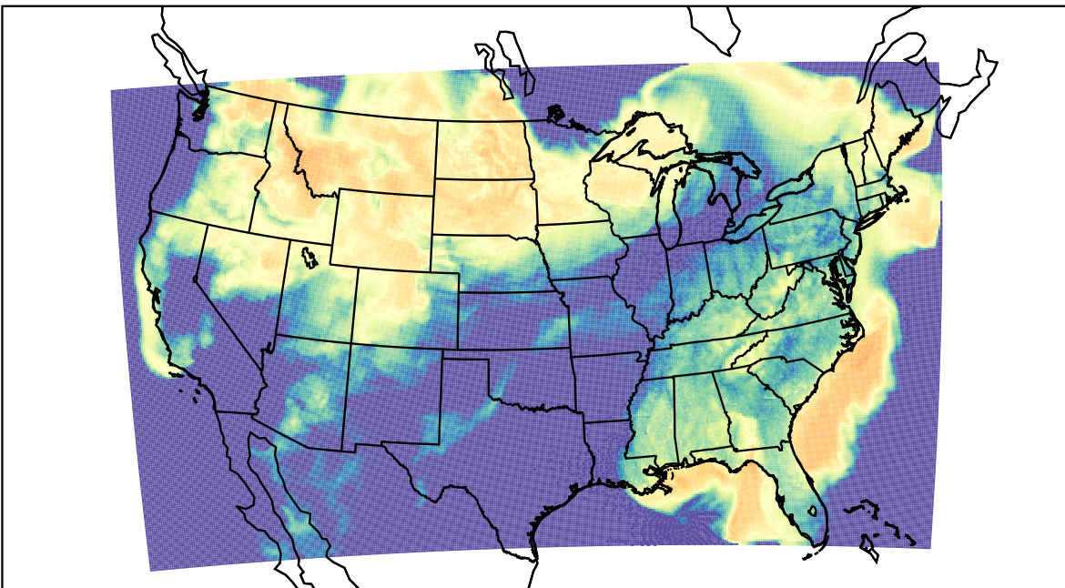
WRF (2023-03-23_06:00:00)
