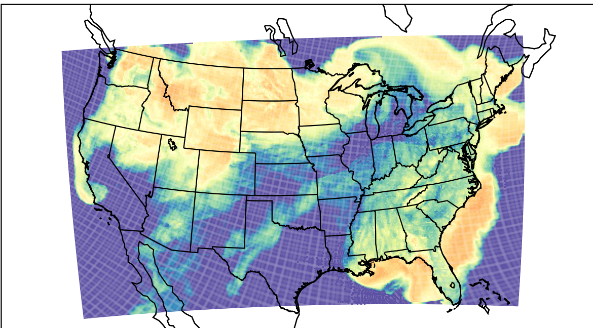
WRF (2023-03-23_03:00:00)
