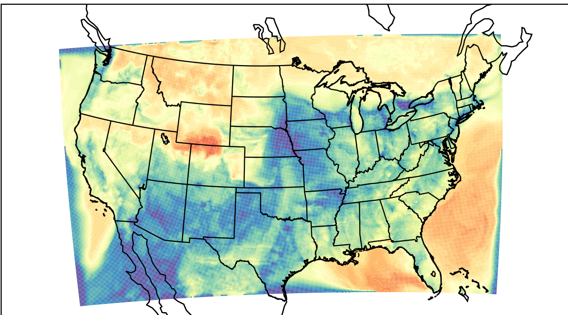
WRF (2023-03-22_04:00:00)
