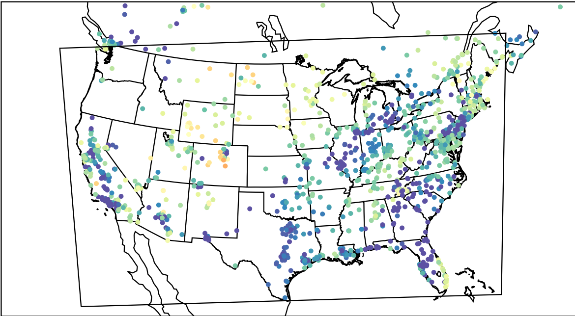
AirNOW (2023-03-23_10:00:00)
