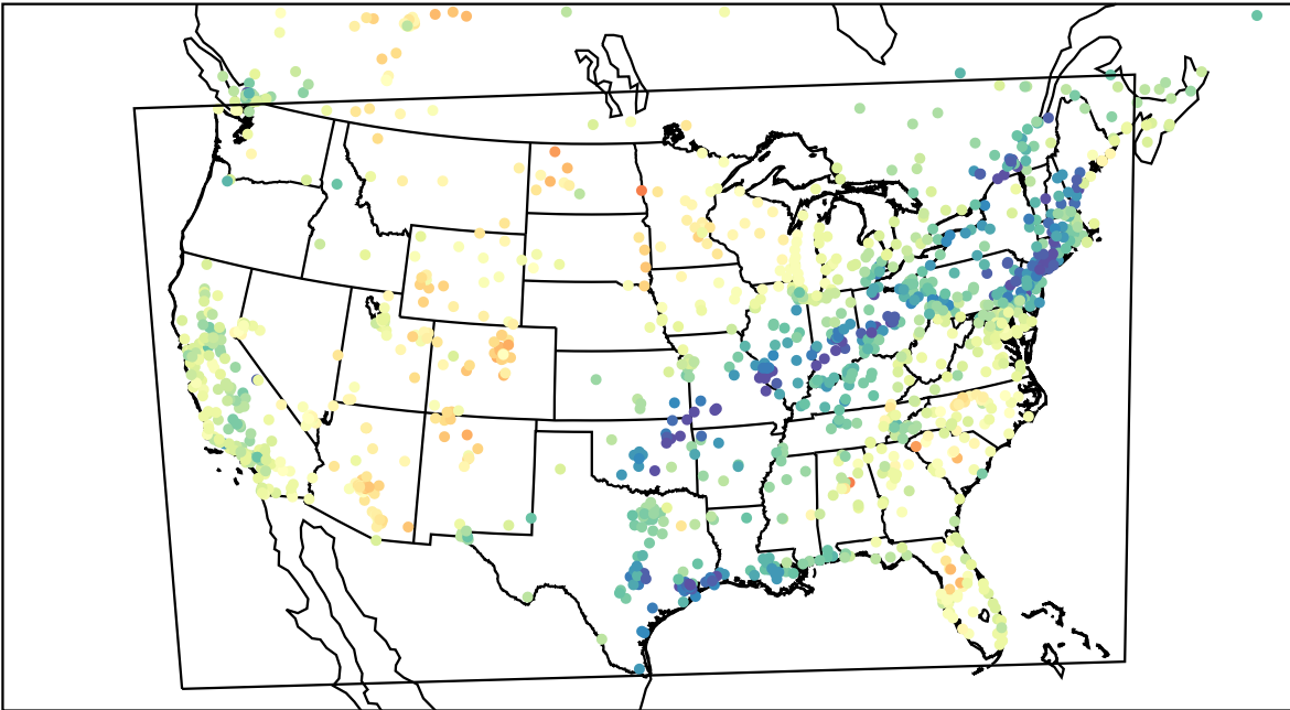
AirNOW (2023-03-23_22:00:00)
