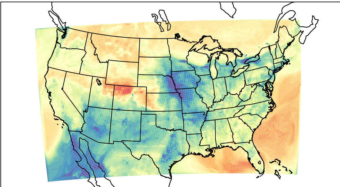
WRF (2023-03-22_01:00:00)
