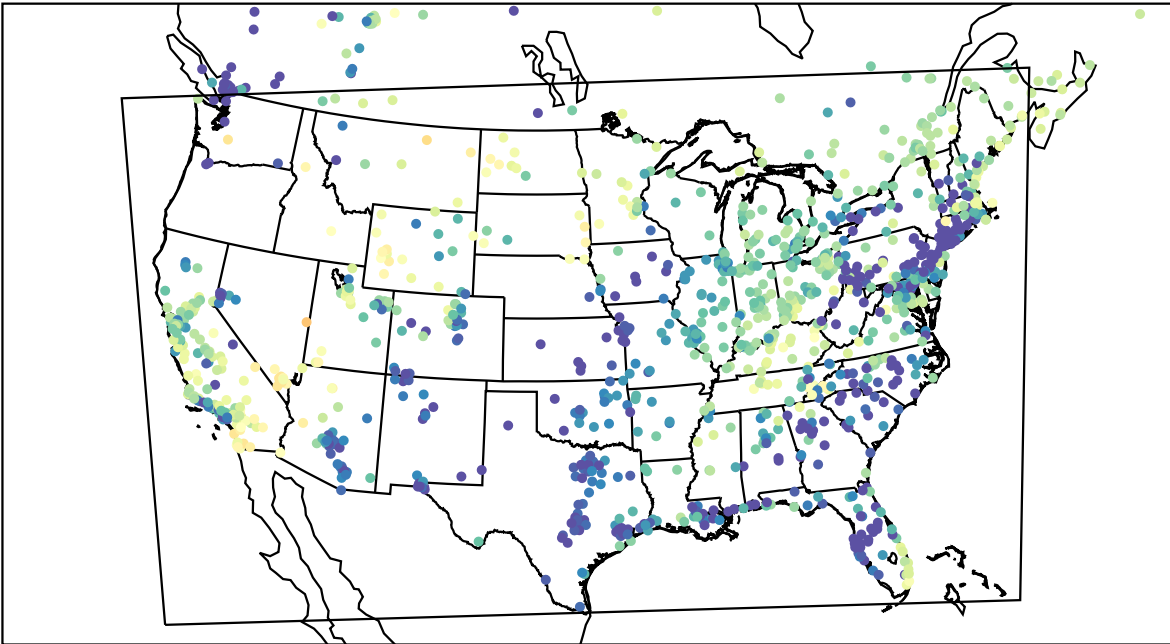
AirNOW (2023-03-22_12:00:00)
