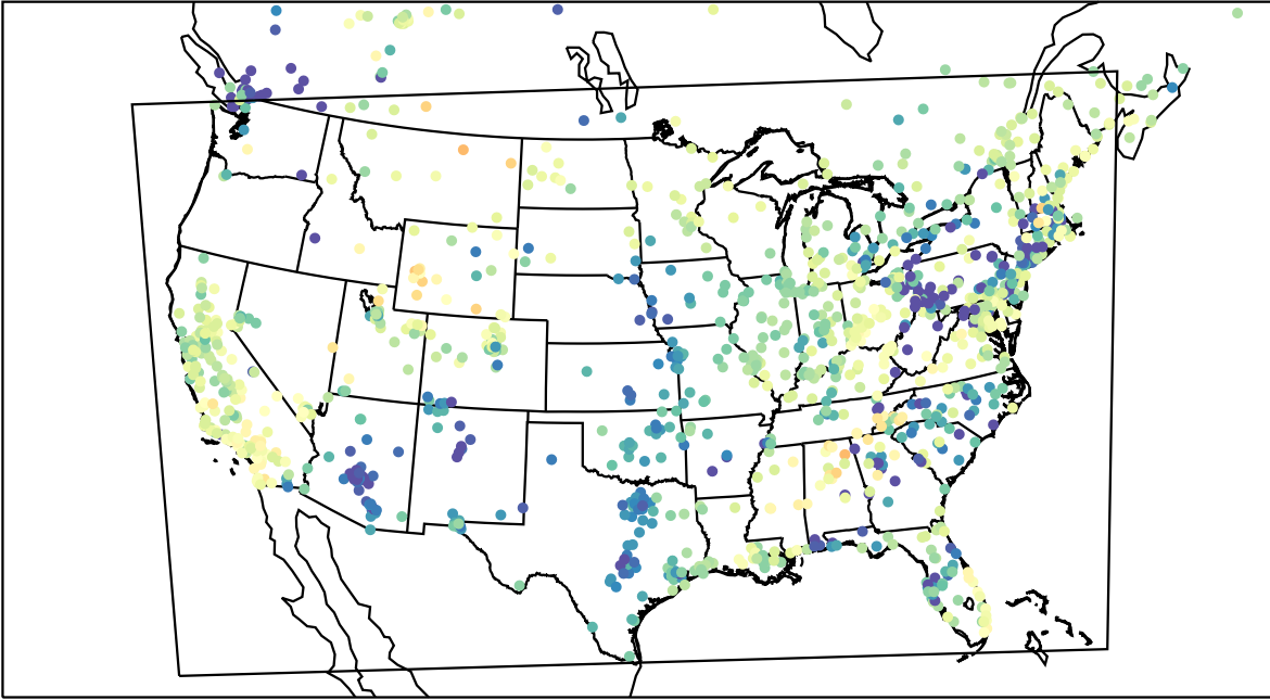
AirNOW (2023-03-22_04:00:00)
