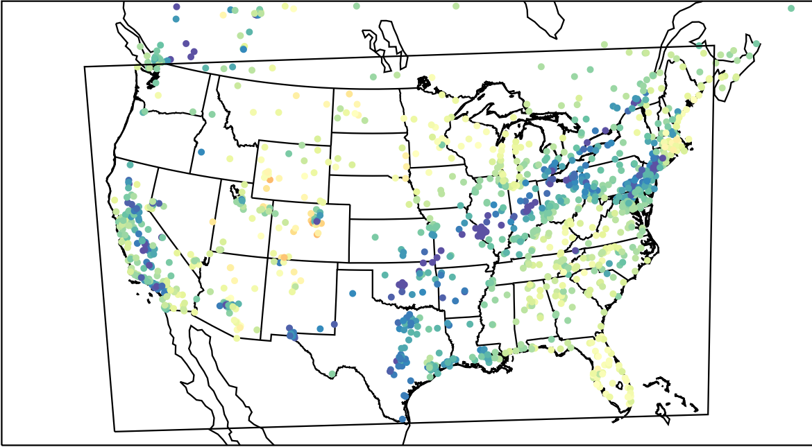
AirNOW (2023-03-23_16:00:00)
