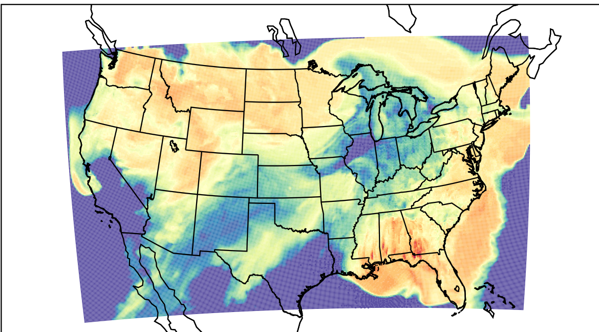
WRF (2023-03-22_21:00:00)
