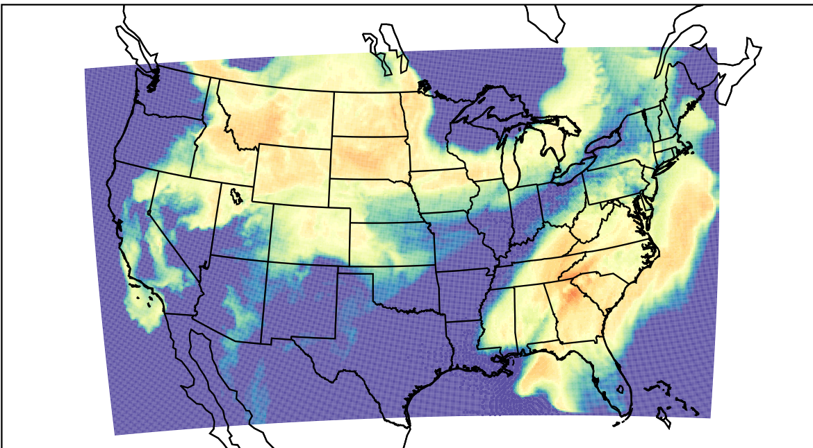
WRF (2023-03-23_17:00:00)
