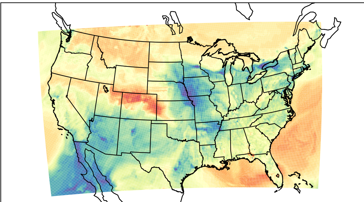
WRF (2023-03-22_00:00:00)
