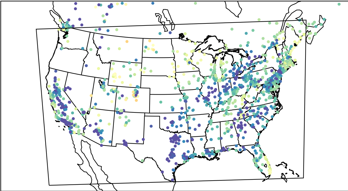
AirNOW (2023-03-23_13:00:00)
