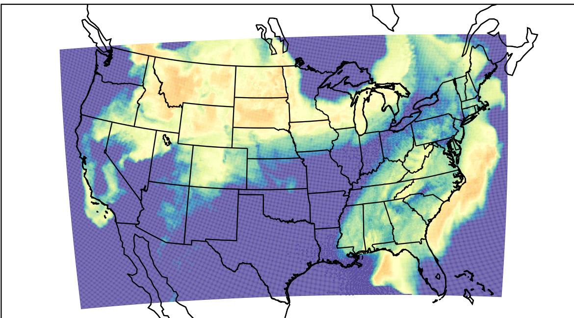
WRF (2023-03-23_14:00:00)
