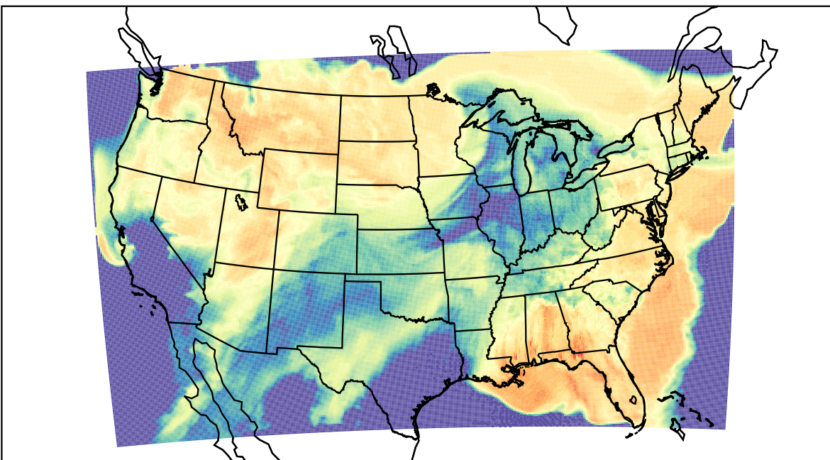
WRF (2023-03-22_19:00:00)
