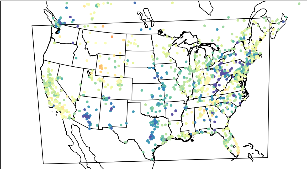
AirNOW (2023-03-22_02:00:00)
