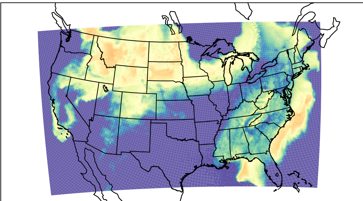
WRF (2023-03-23_13:00:00)
