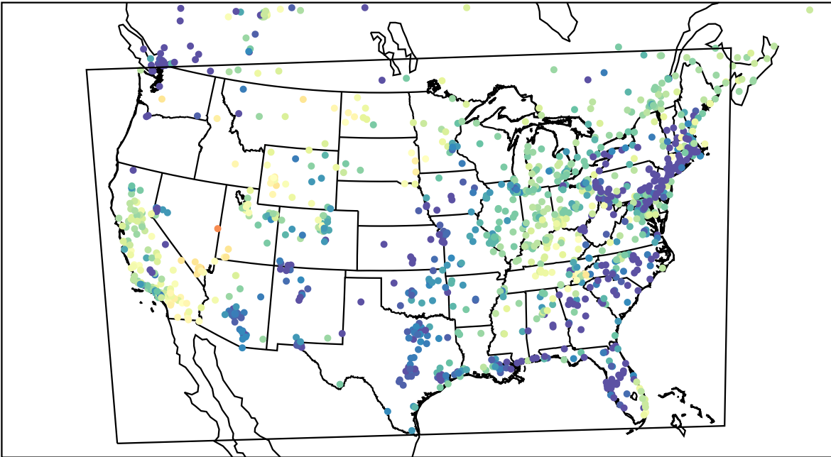
AirNOW (2023-03-22_11:00:00)
