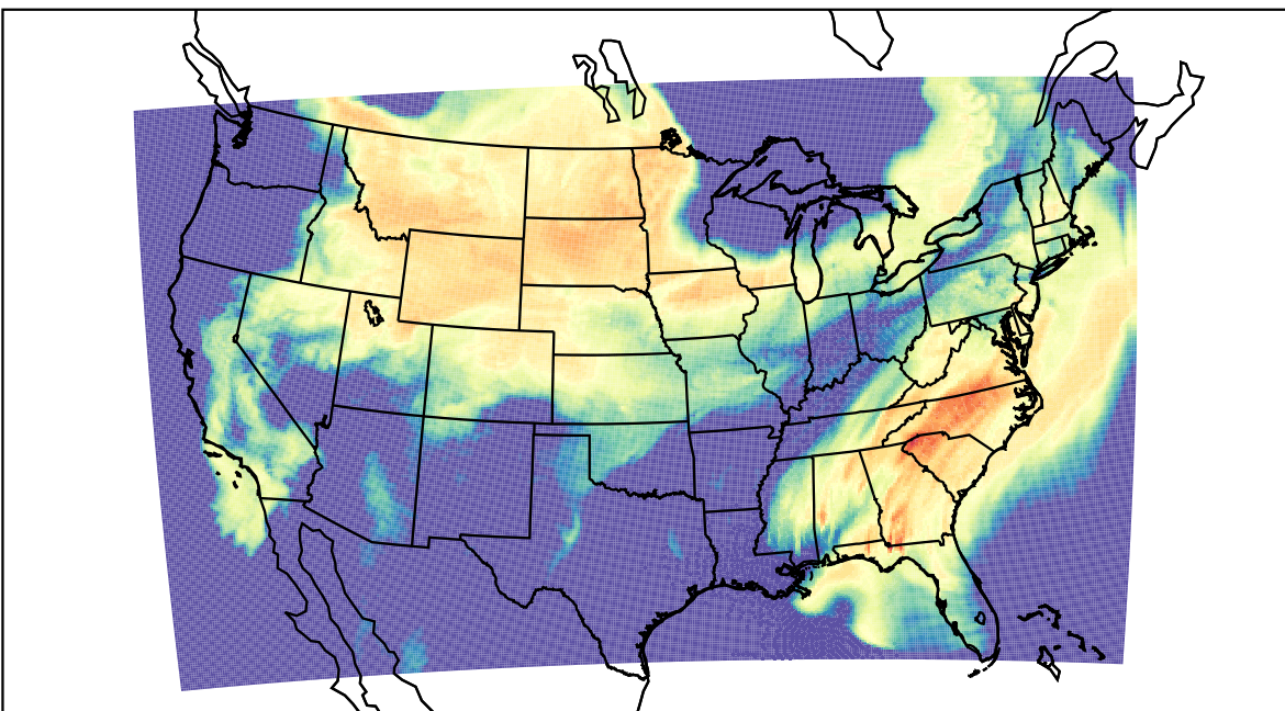
WRF (2023-03-23_21:00:00)
