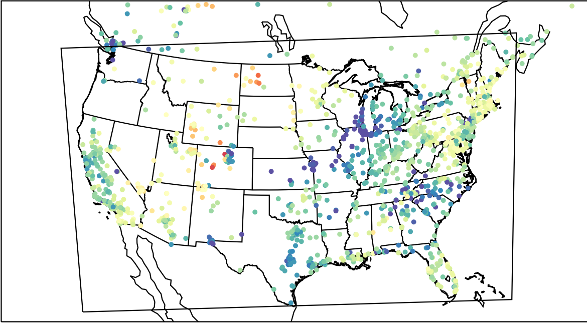
AirNOW (2023-03-23_02:00:00)
