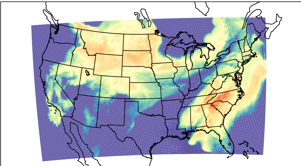
WRF (2023-03-23_19:00:00)
