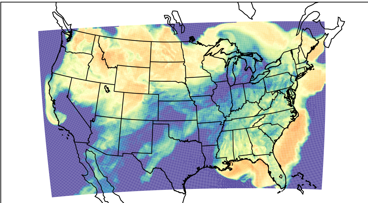
WRF (2023-03-23_02:00:00)
