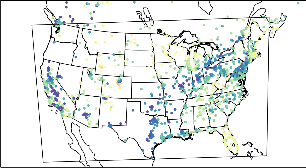
AirNOW (2023-03-23_15:00:00)
