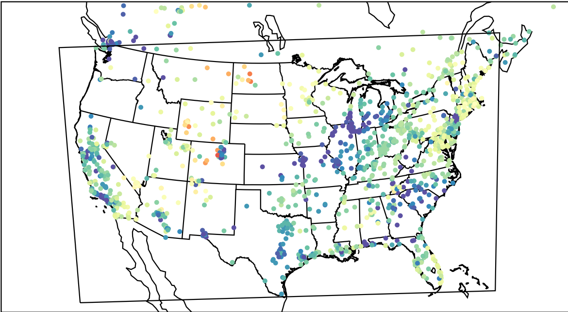
AirNOW (2023-03-23_04:00:00)
