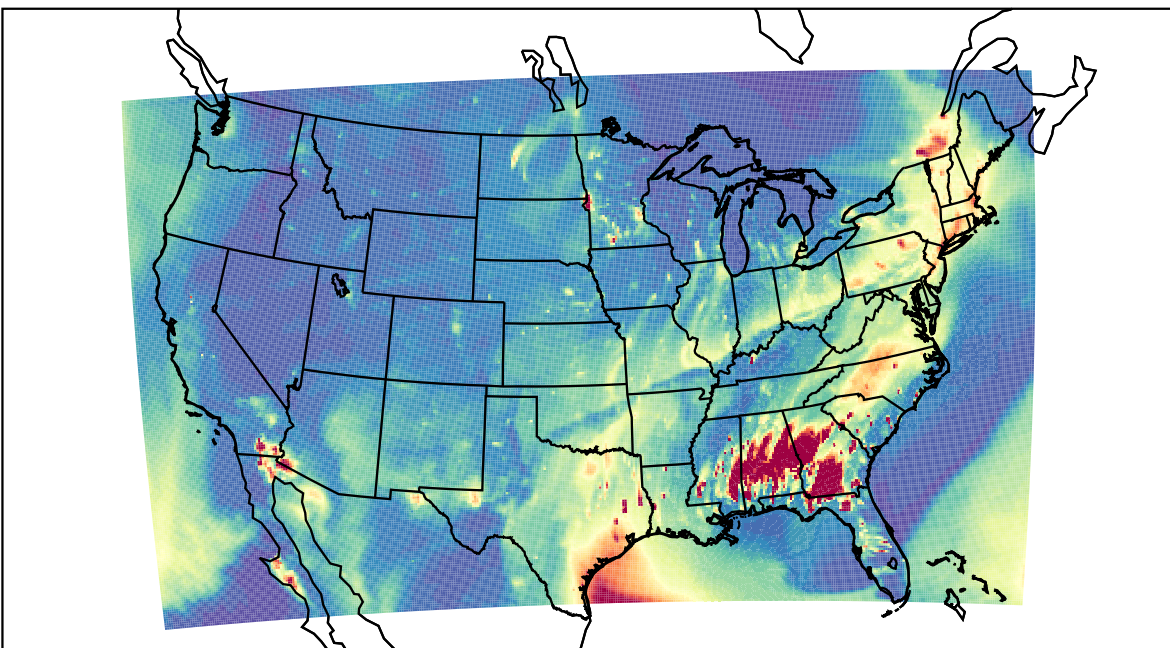
WRF 2023-03-24_01:00:00
