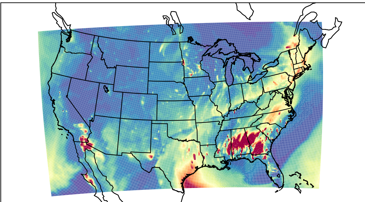
WRF 2023-03-24_02:00:00
