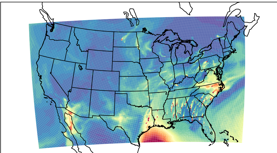
WRF 2023-03-24_21:00:00
