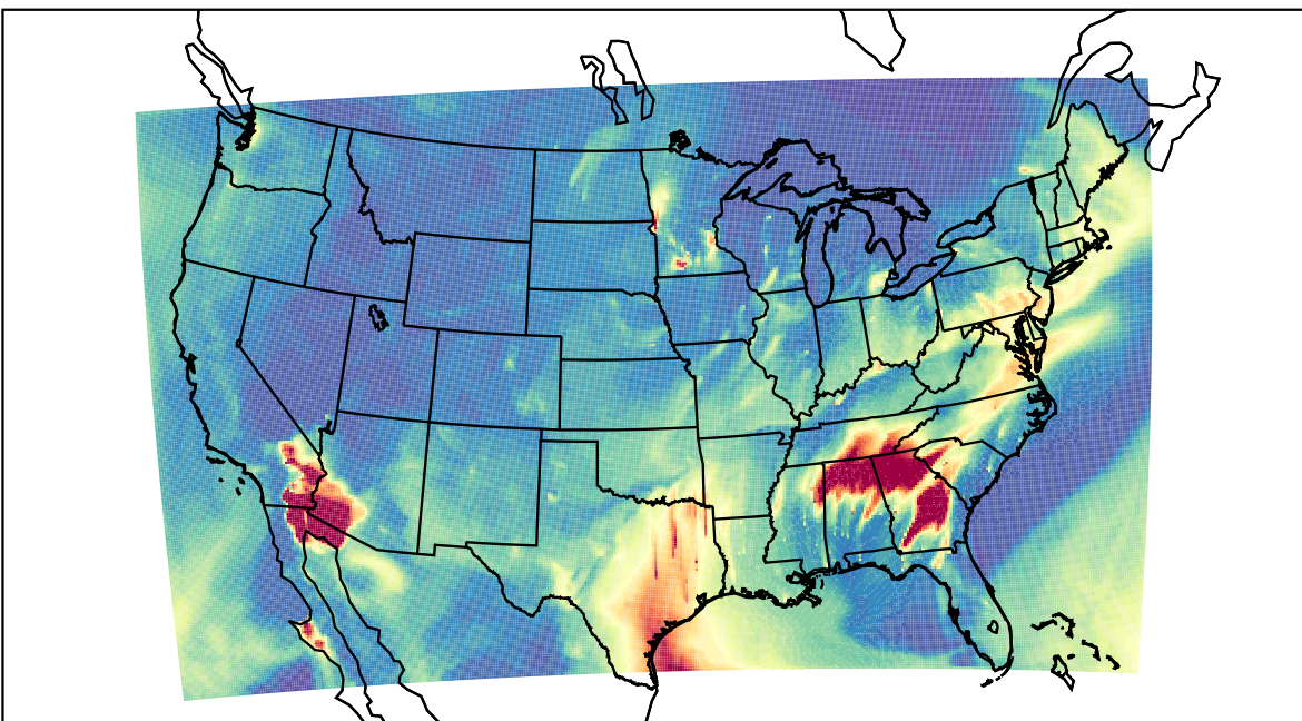
WRF 2023-03-24_07:00:00
