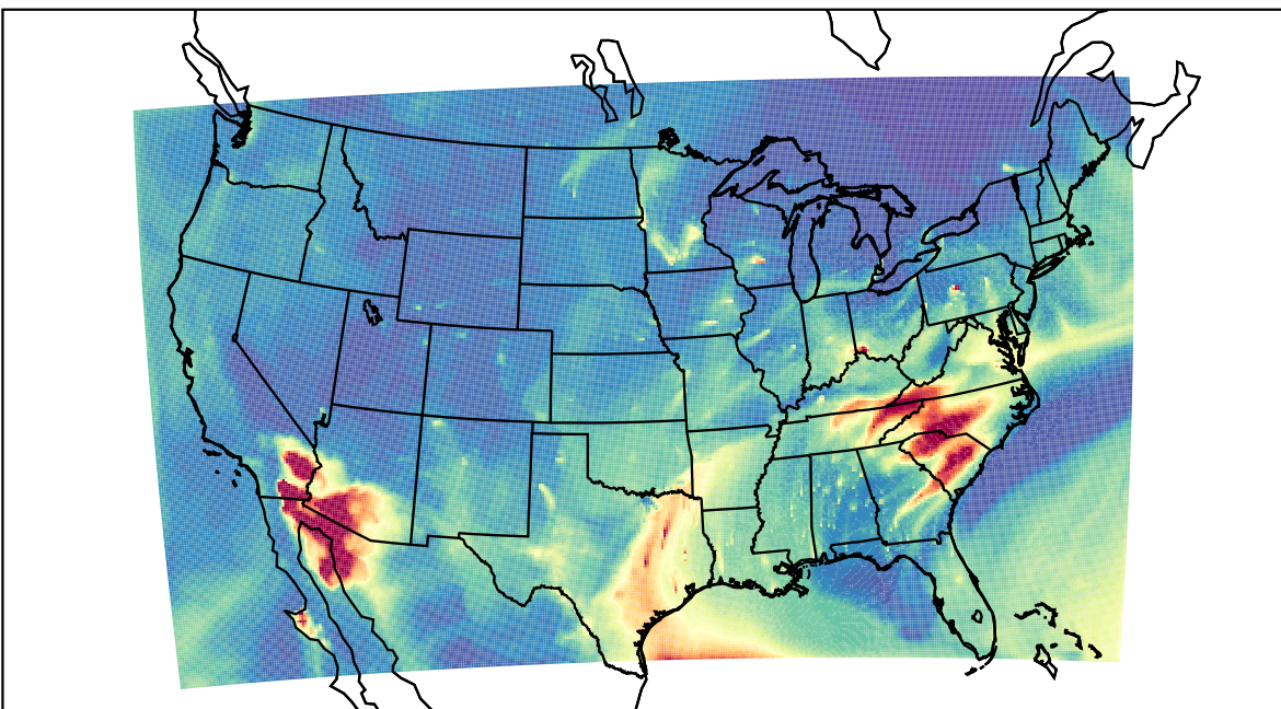
WRF 2023-03-24_14:00:00
