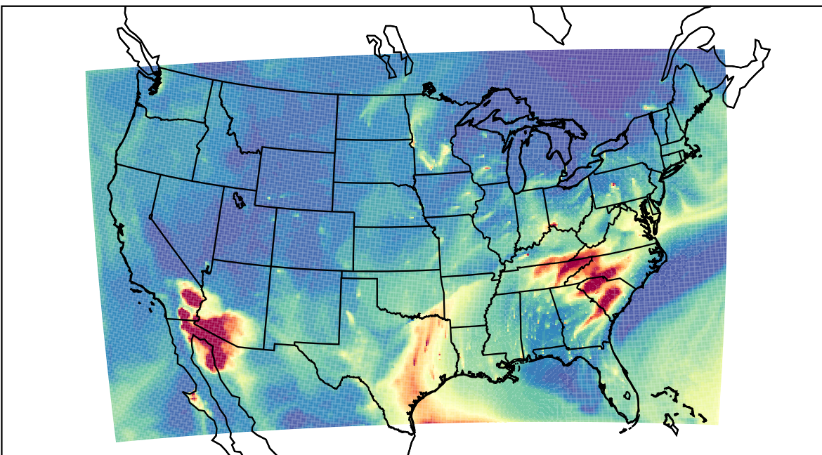
WRF 2023-03-24_13:00:00
