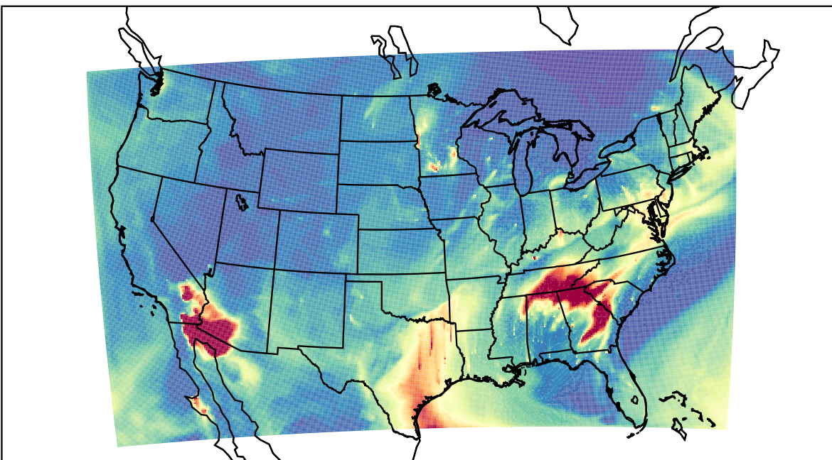
WRF 2023-03-24_09:00:00
