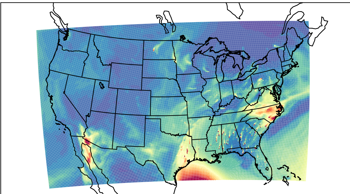
WRF 2023-03-24_19:00:00
