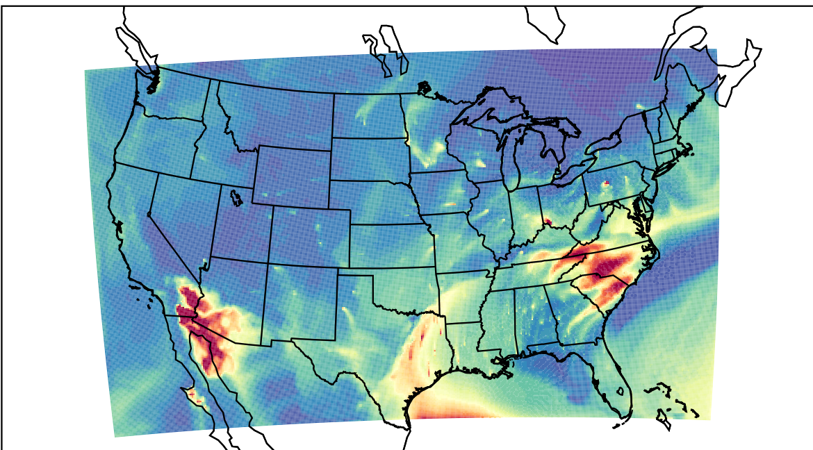
WRF 2023-03-24_15:00:00
