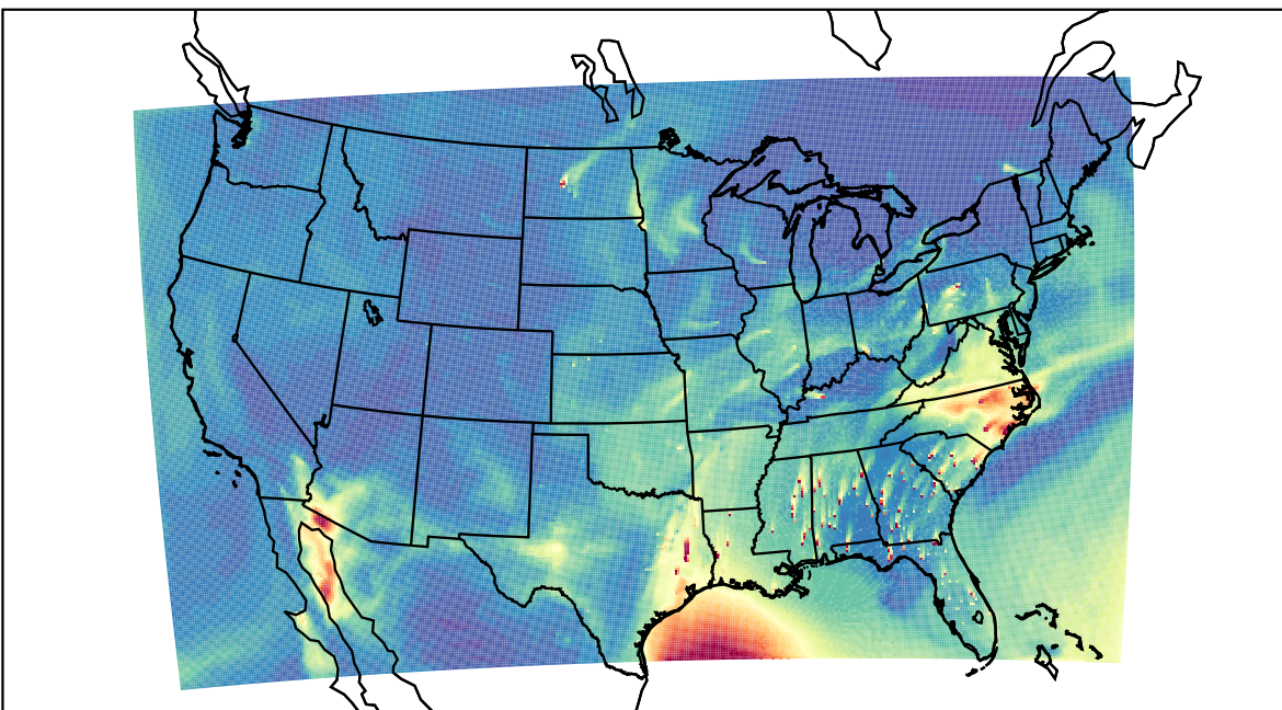
WRF 2023-03-24_20:00:00
