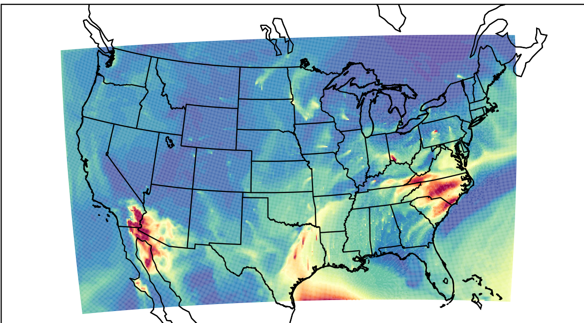
WRF 2023-03-24_16:00:00
