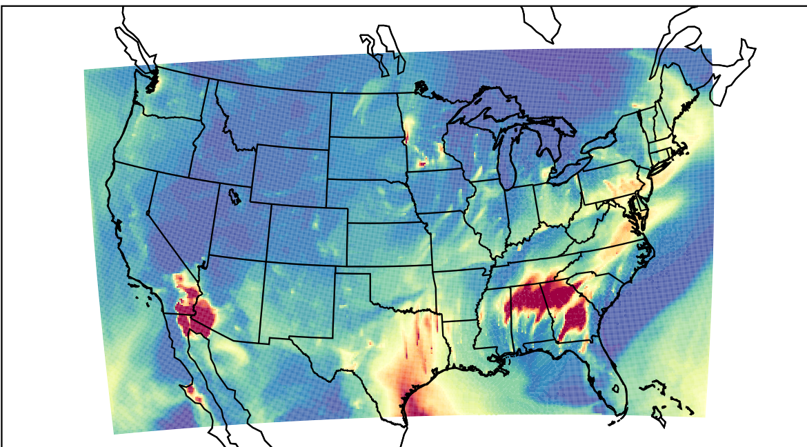
WRF 2023-03-24_06:00:00
