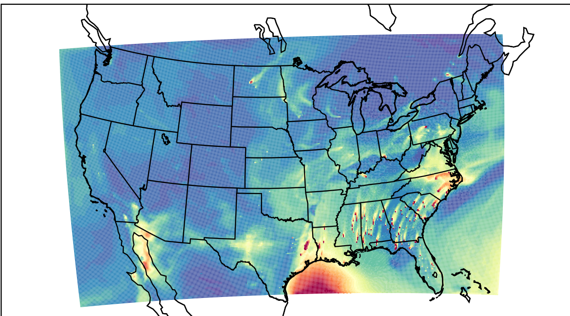
WRF 2023-03-24_22:00:00
