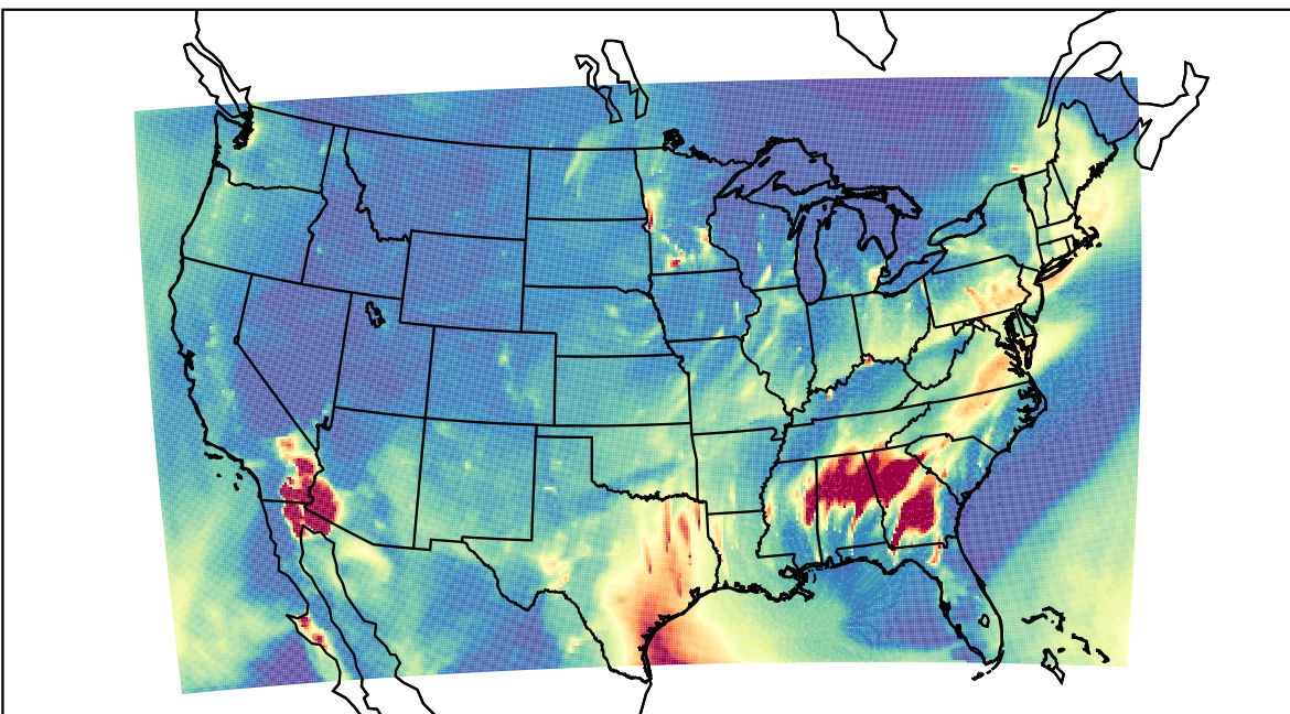
WRF 2023-03-24_05:00:00
