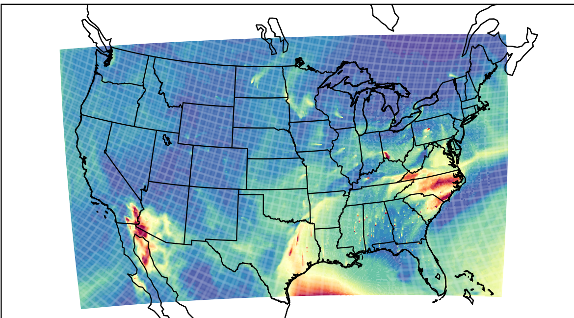
WRF 2023-03-24_17:00:00
