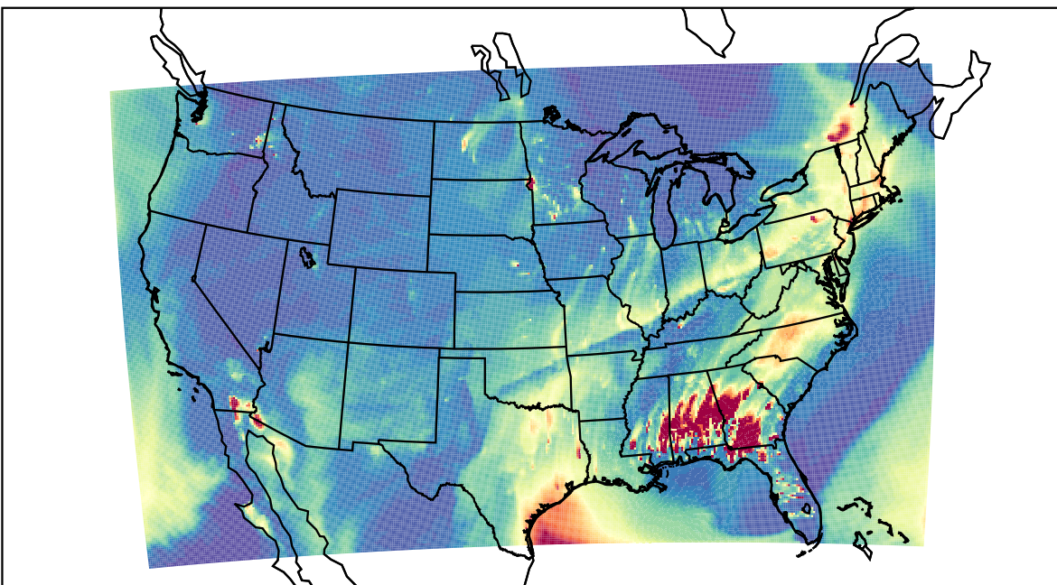
WRF 2023-03-24_00:00:00
