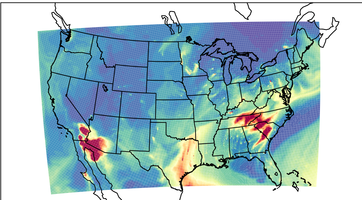
WRF 2023-03-24_12:00:00
