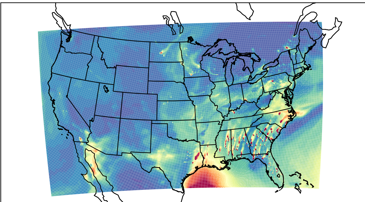
WRF 2023-03-24_23:00:00
