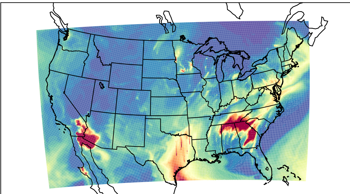
WRF 2023-03-24_08:00:00
