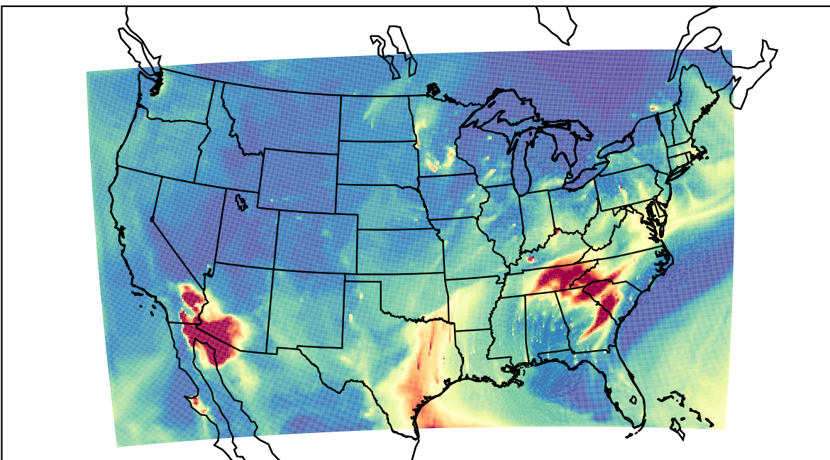
WRF 2023-03-24_11:00:00
