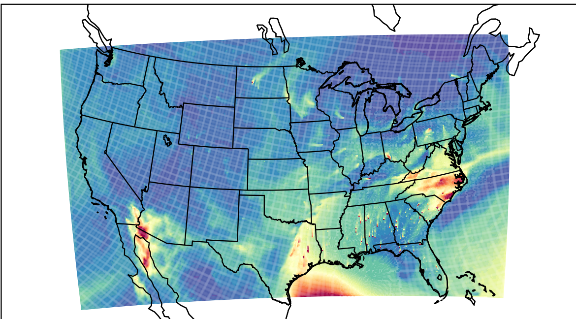
WRF 2023-03-24_18:00:00
