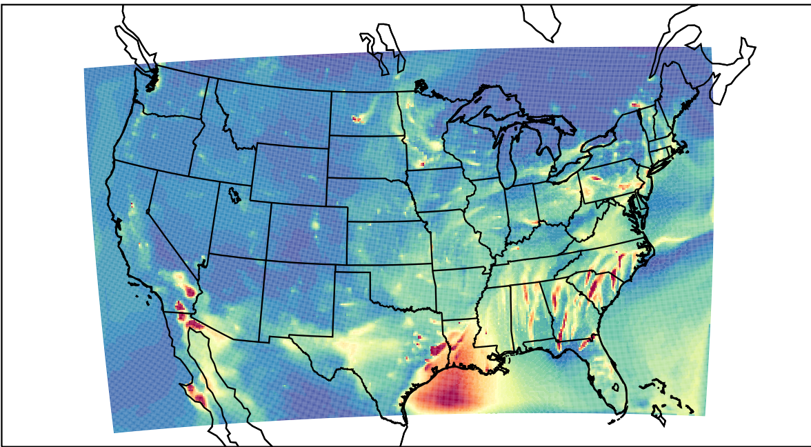
WRF 2023-03-25_03:00:00
