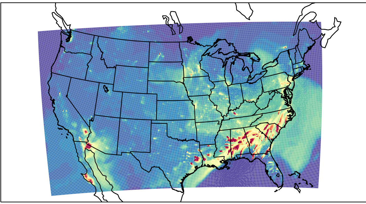
WRF 2023-03-26_02:00:00
