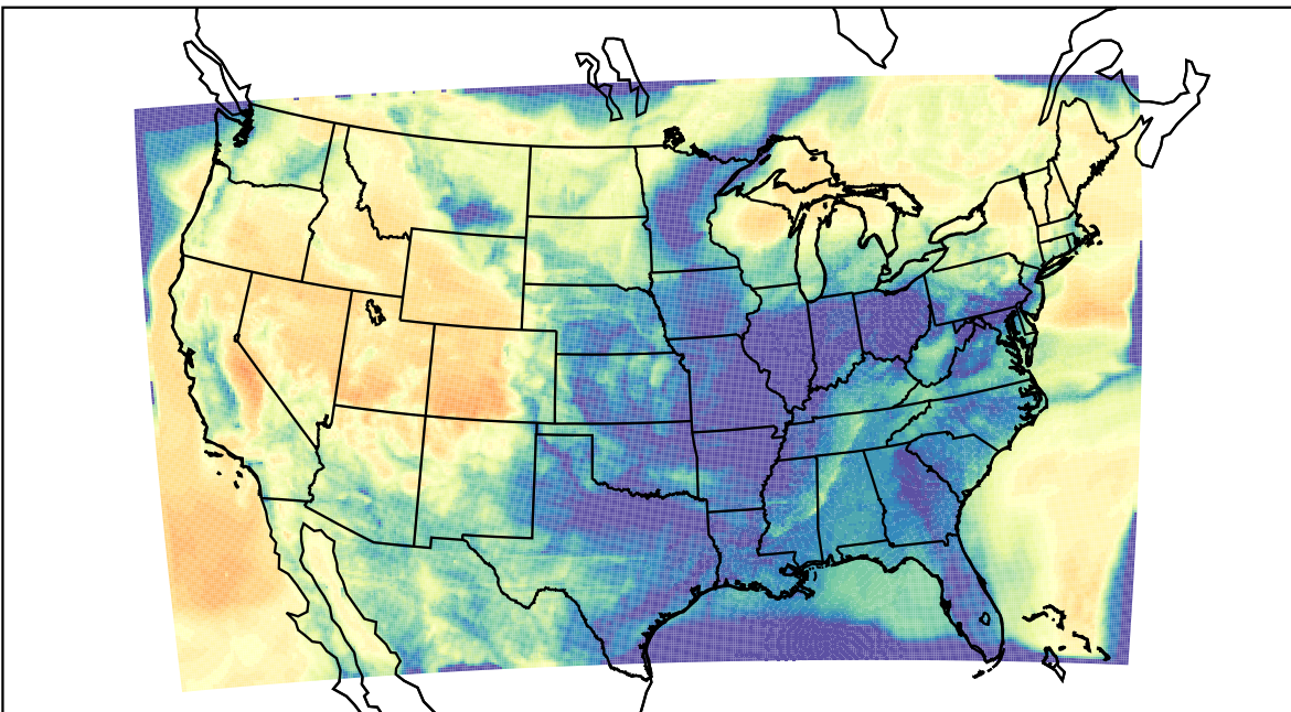
WRF (2023-03-25_08:00:00)
