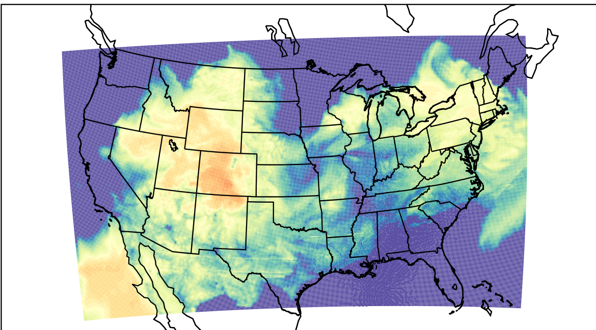
WRF (2023-03-26_14:00:00)
