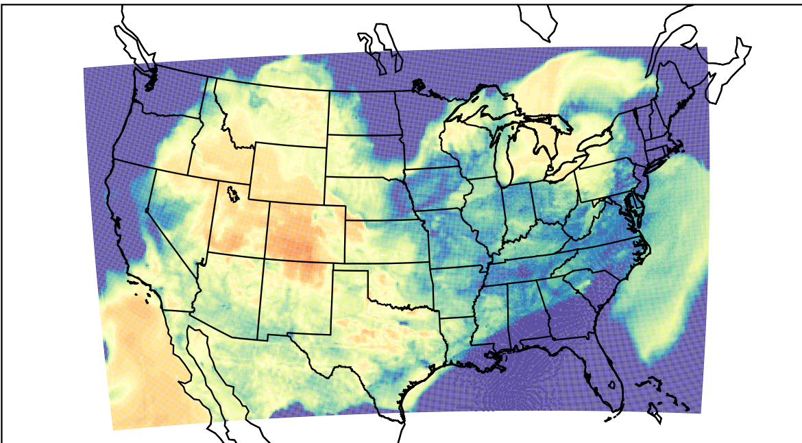
WRF (2023-03-26_06:00:00)
