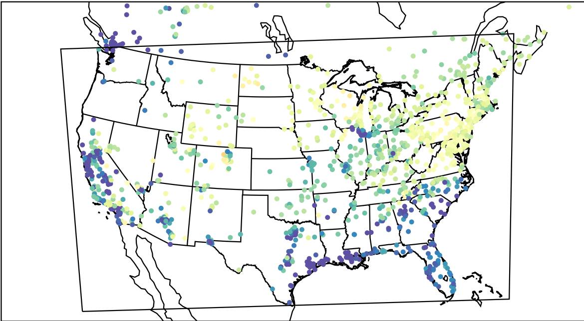
AirNOW (2023-03-26_14:00:00)
