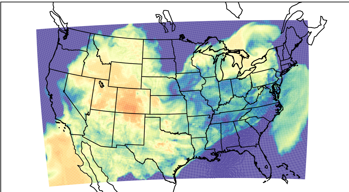
WRF (2023-03-26_08:00:00)
