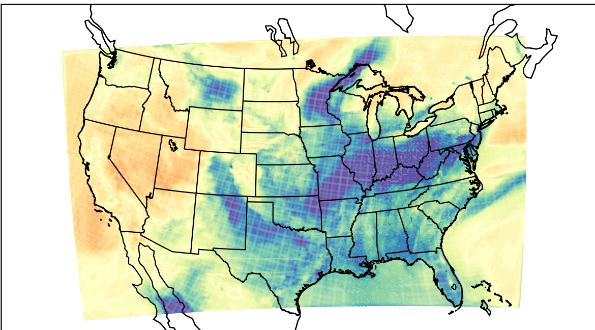
WRF (2023-03-25_01:00:00)
