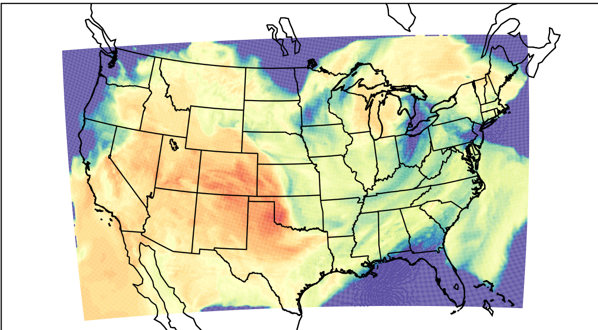
WRF (2023-03-25_21:00:00)
