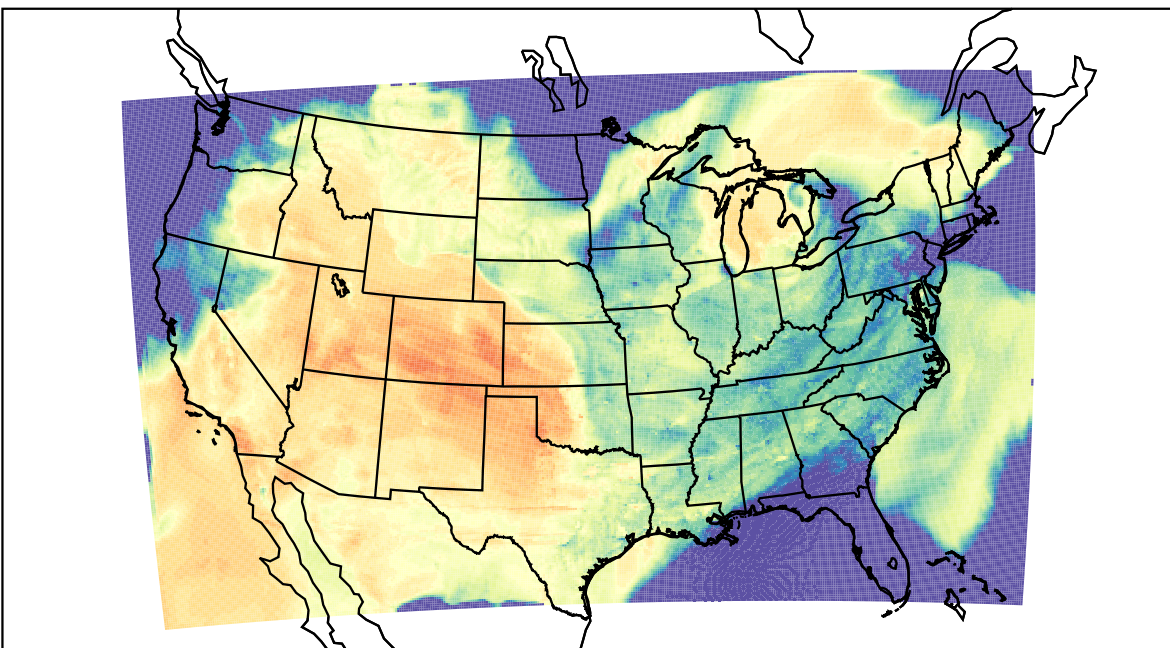
WRF (2023-03-26_00:00:00)
