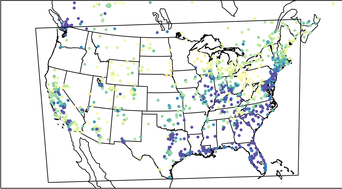
AirNOW (2023-03-26_06:00:00)
