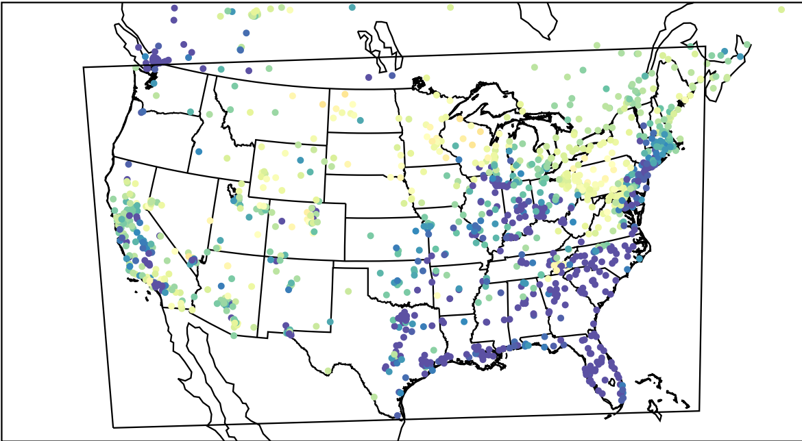
AirNOW (2023-03-26_09:00:00)
