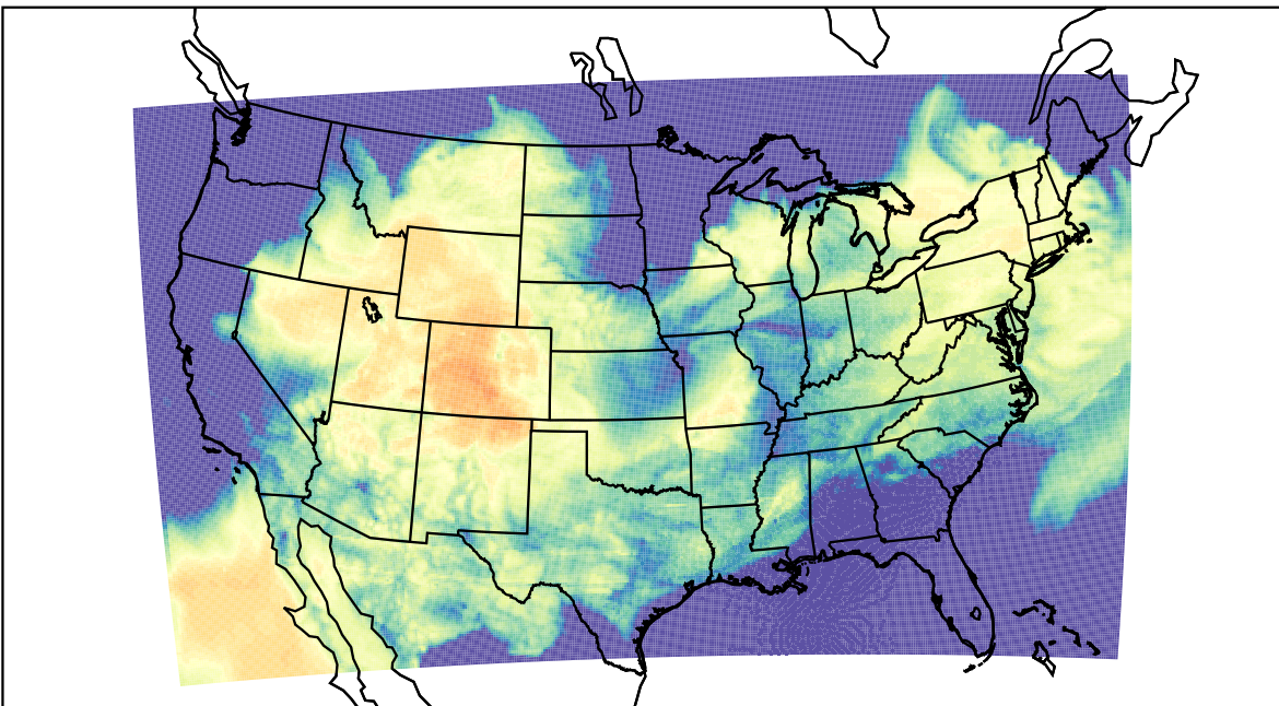
WRF (2023-03-26_15:00:00)
