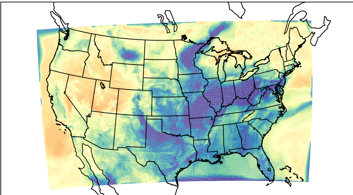
WRF (2023-03-25_04:00:00)
