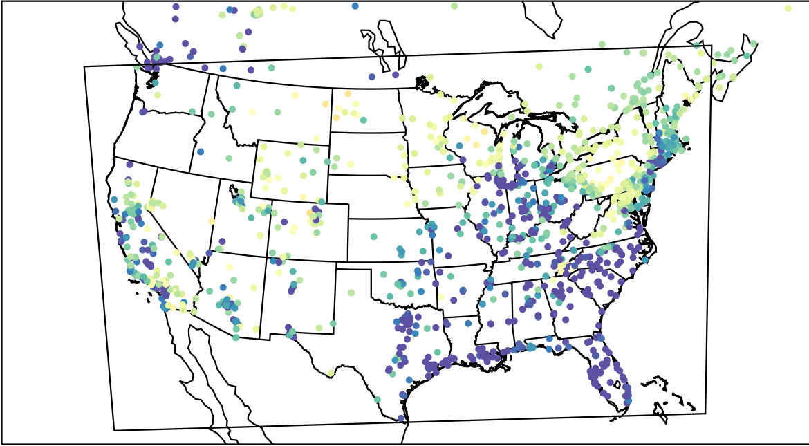
AirNOW (2023-03-26_11:00:00)
