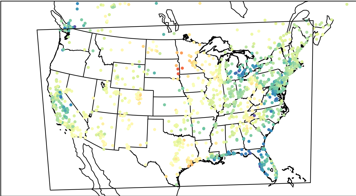
AirNOW (2023-03-25_18:00:00)
