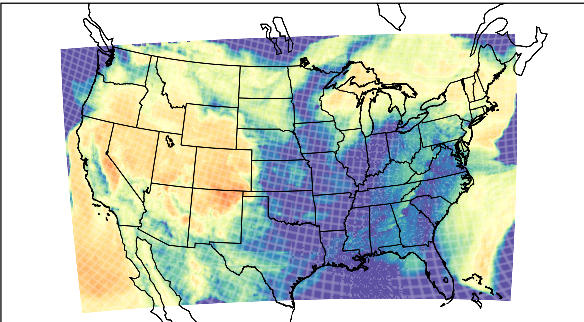
WRF (2023-03-25_13:00:00)
