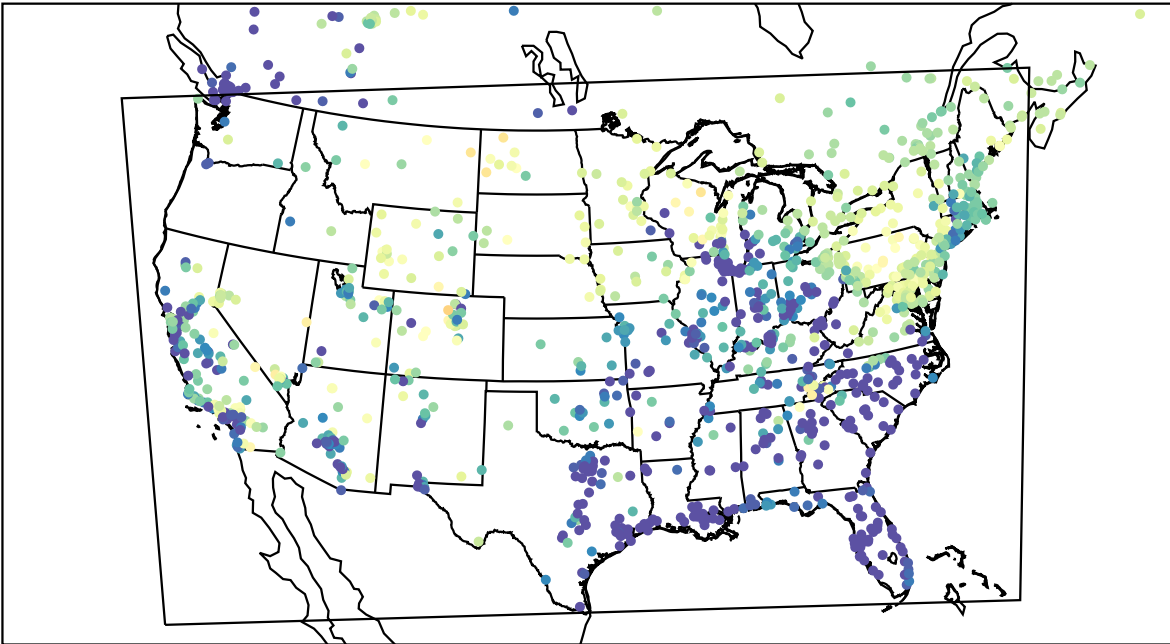
AirNOW (2023-03-26_12:00:00)
