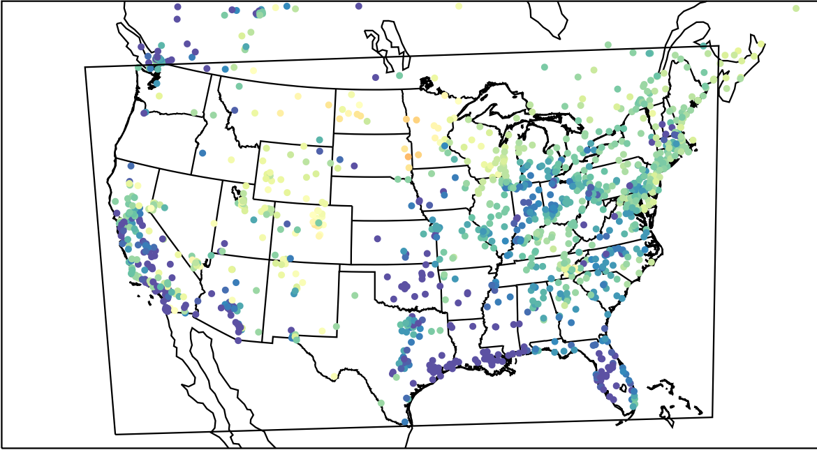
AirNOW (2023-03-25_13:00:00)
