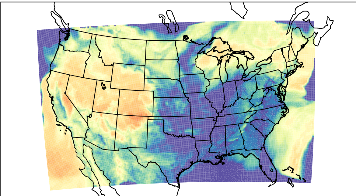
WRF (2023-03-25_12:00:00)
