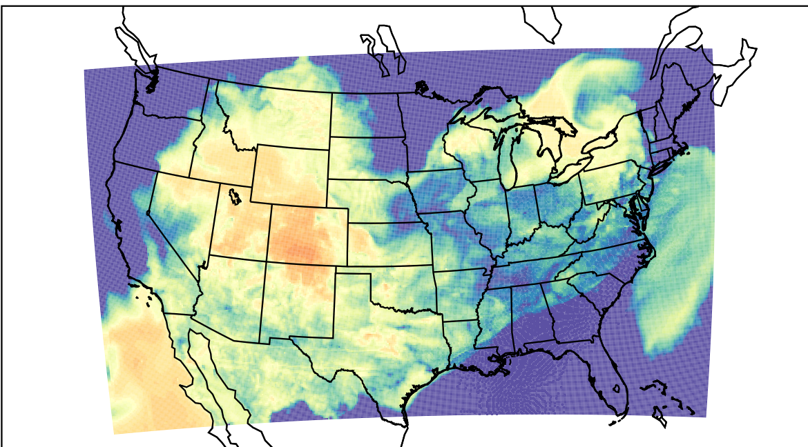
WRF (2023-03-26_09:00:00)
