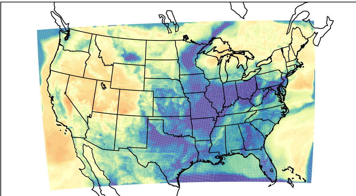
WRF (2023-03-25_06:00:00)
