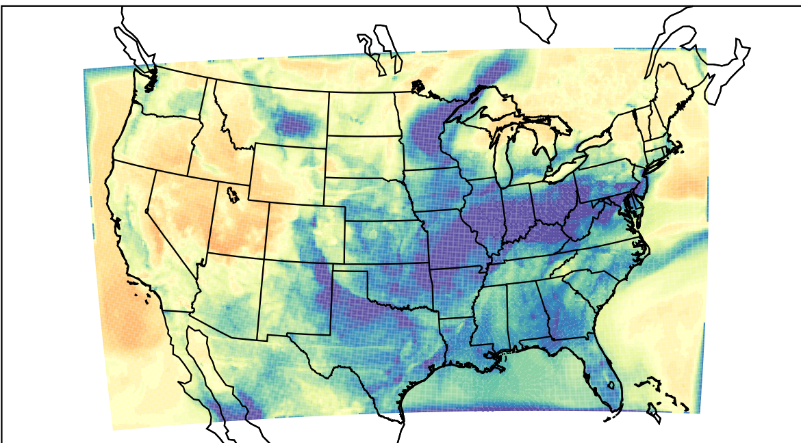
WRF (2023-03-25_03:00:00)
