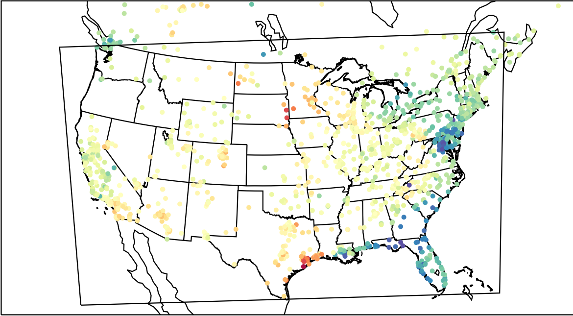
AirNOW (2023-03-25_22:00:00)
