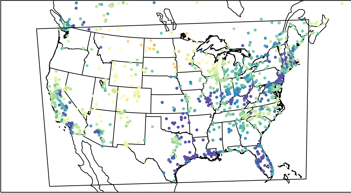
AirNOW (2023-03-25_06:00:00)
