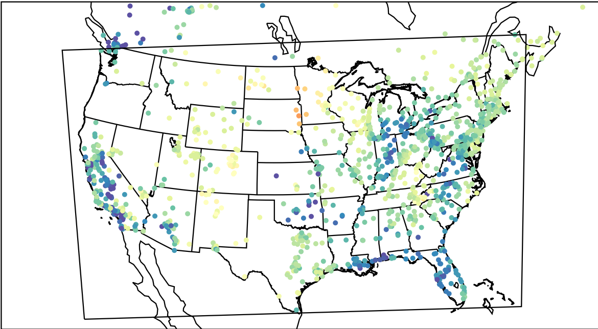
AirNOW (2023-03-25_15:00:00)
