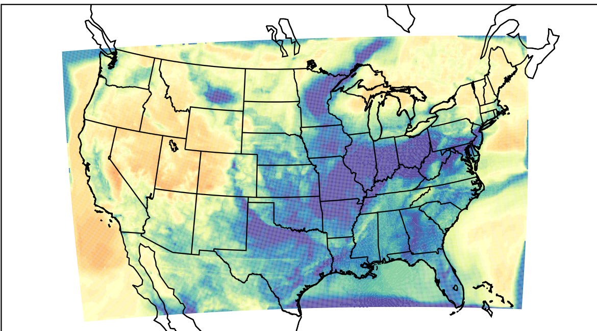
WRF (2023-03-25_05:00:00)
