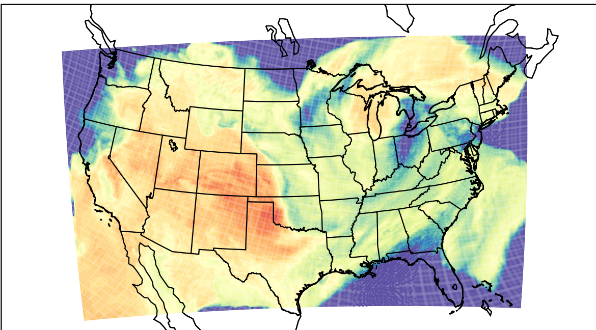
WRF (2023-03-25_20:00:00)
