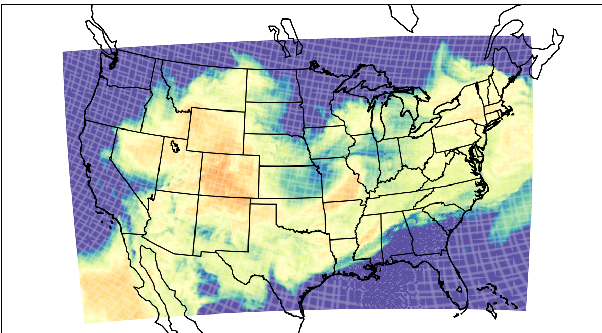
WRF (2023-03-26_17:00:00)
