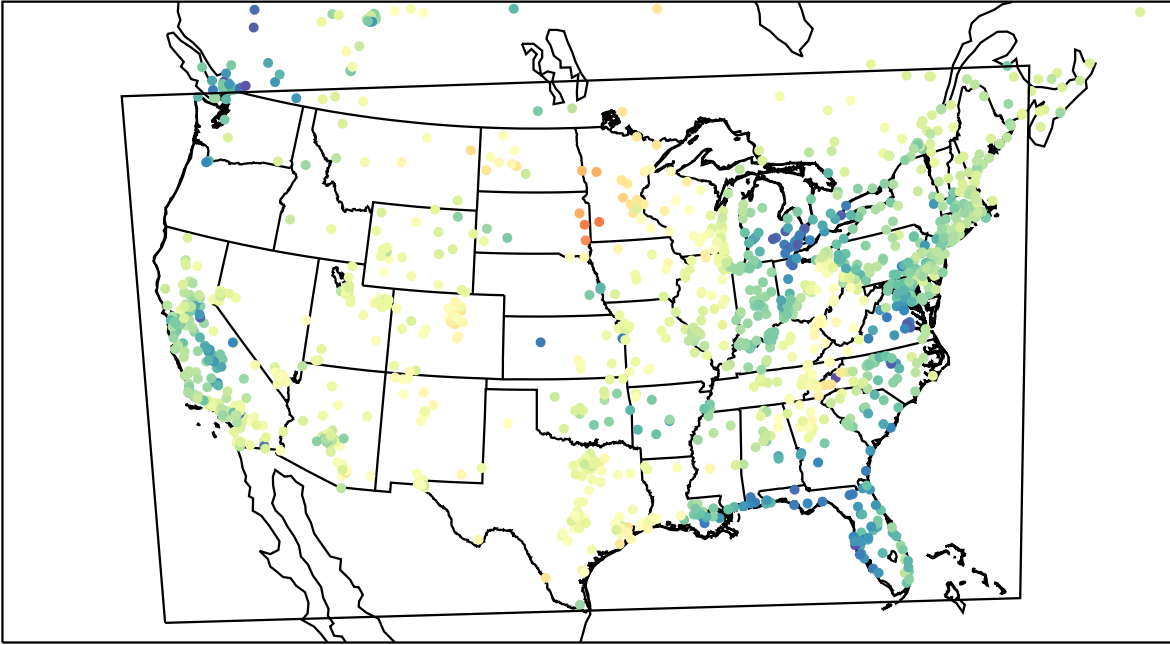
AirNOW (2023-03-25_17:00:00)
