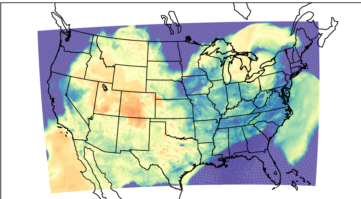
WRF (2023-03-26_05:00:00)
