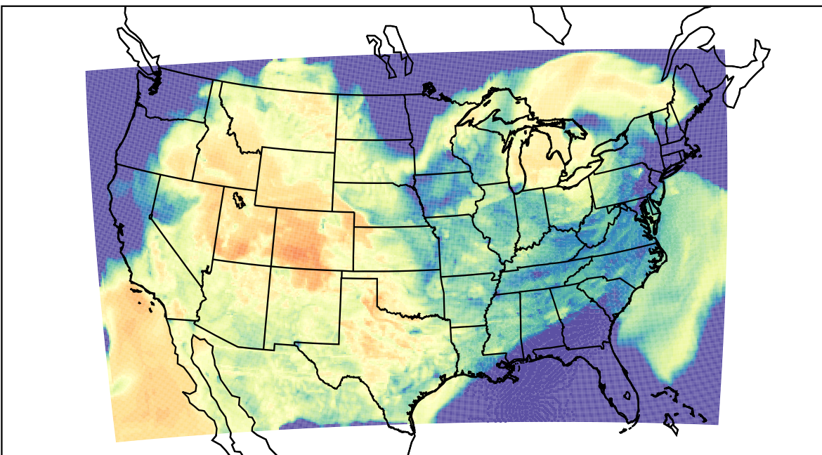
WRF (2023-03-26_03:00:00)
