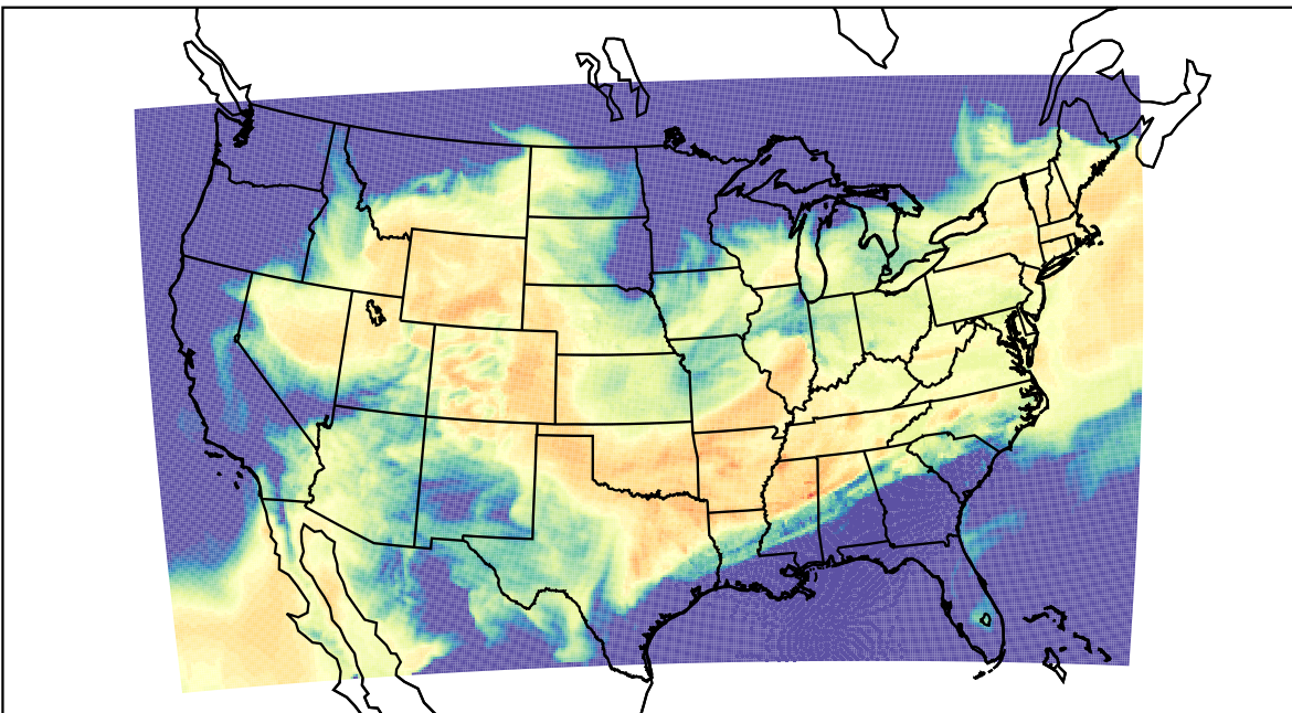
WRF (2023-03-26_21:00:00)
