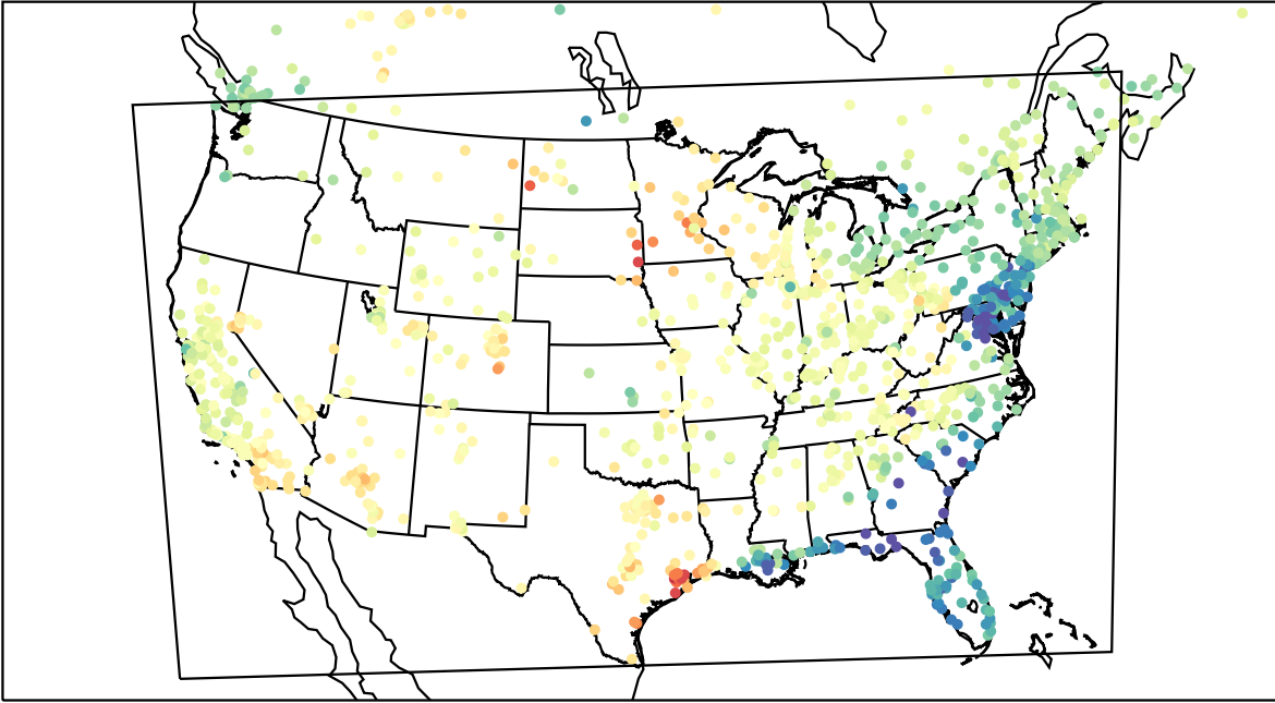
AirNOW (2023-03-25_23:00:00)
