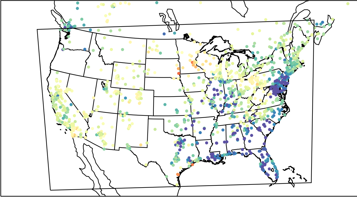
AirNOW (2023-03-26_02:00:00)
