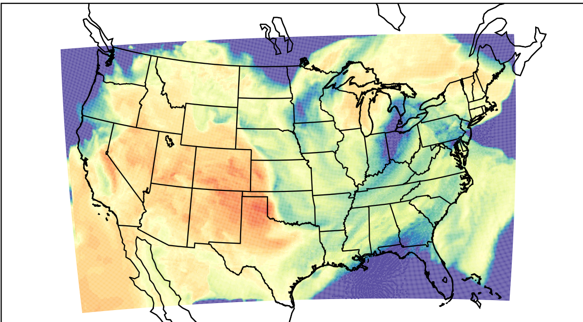
WRF (2023-03-25_19:00:00)
