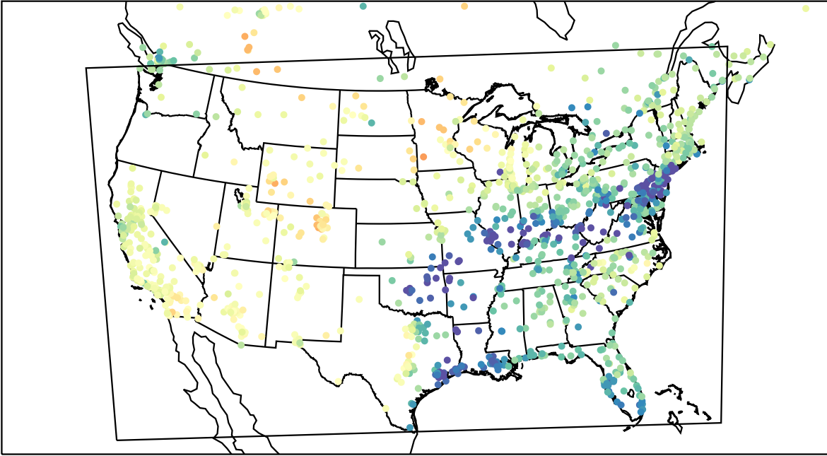
AirNOW (2023-03-25_00:00:00)
