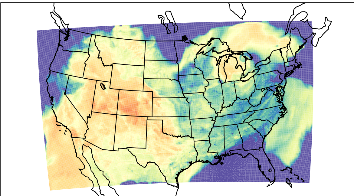
WRF (2023-03-26_01:00:00)
