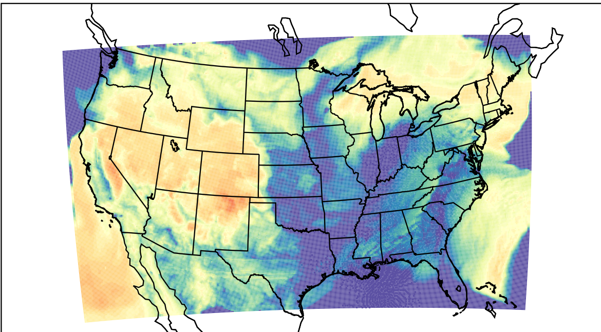
WRF (2023-03-25_14:00:00)
