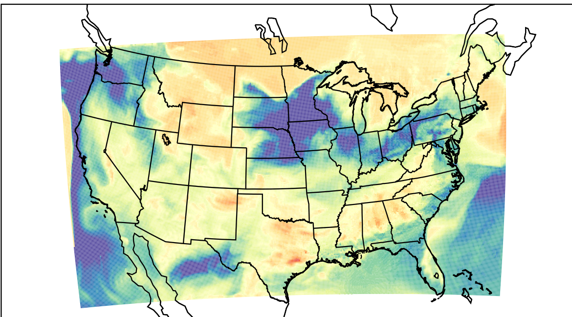
WRF (2023-03-27_22:00:00)
