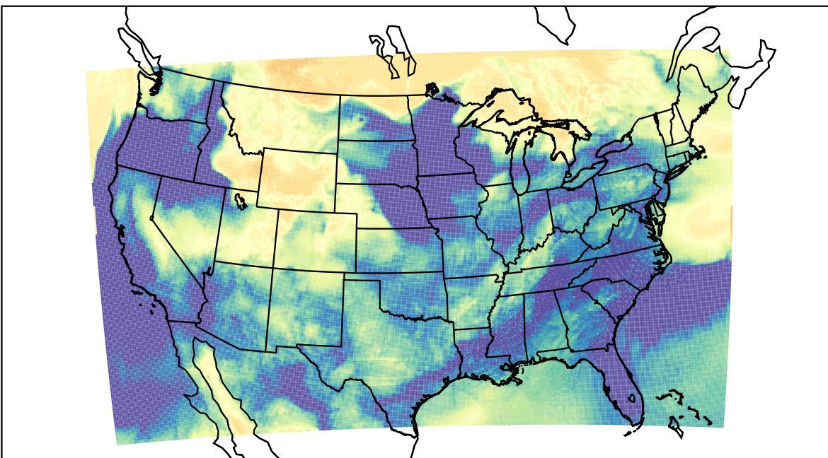
WRF (2023-03-27_10:00:00)
