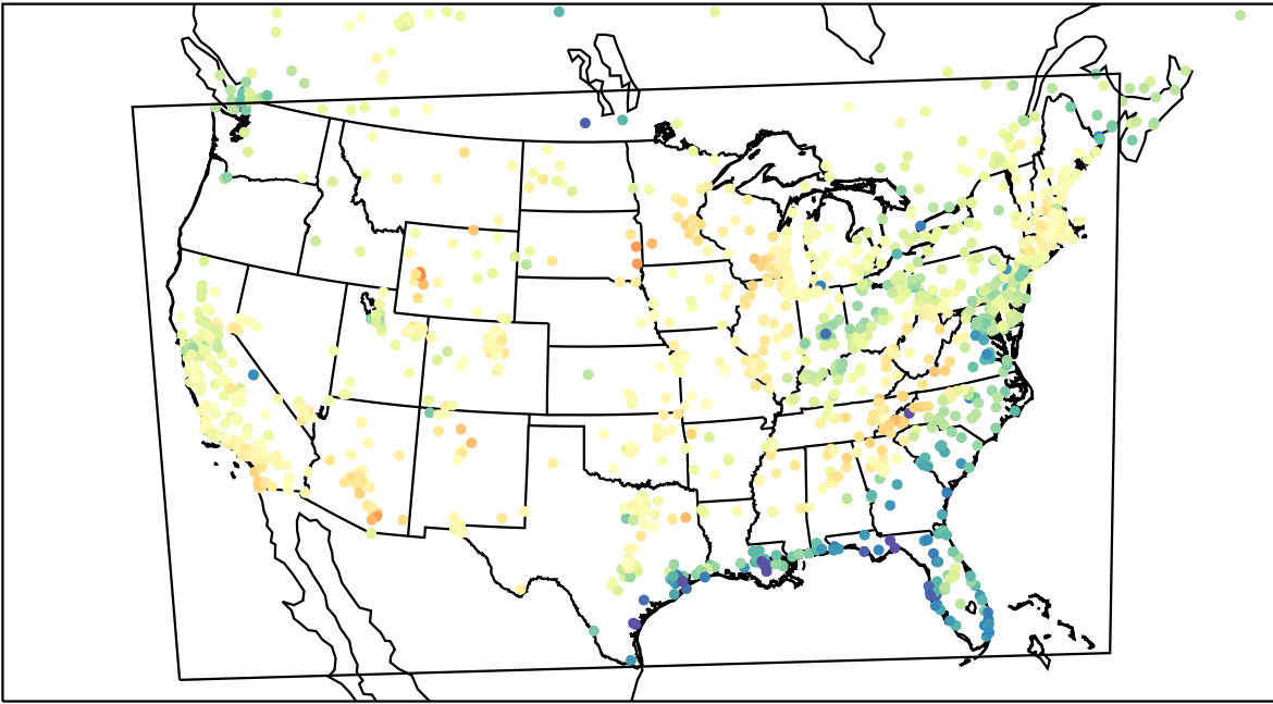
AirNOW (2023-03-27_22:00:00)
