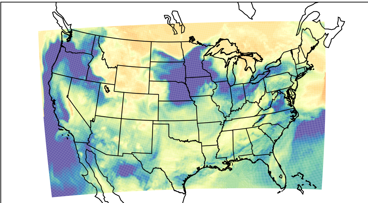
WRF (2023-03-27_17:00:00)
