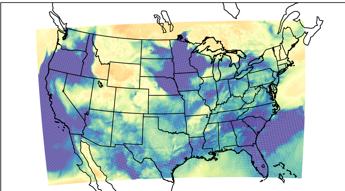
WRF (2023-03-27_06:00:00)
