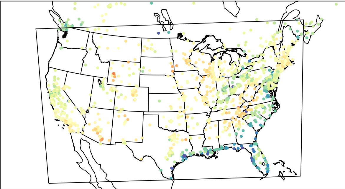
AirNOW (2023-03-27_21:00:00)
