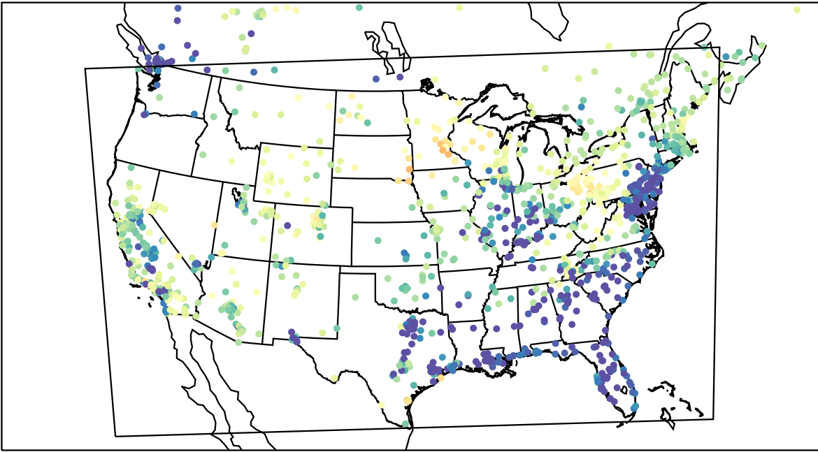
AirNOW (2023-03-26_05:00:00)
