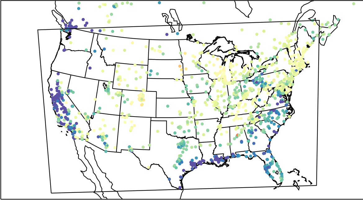
AirNOW (2023-03-27_15:00:00)
