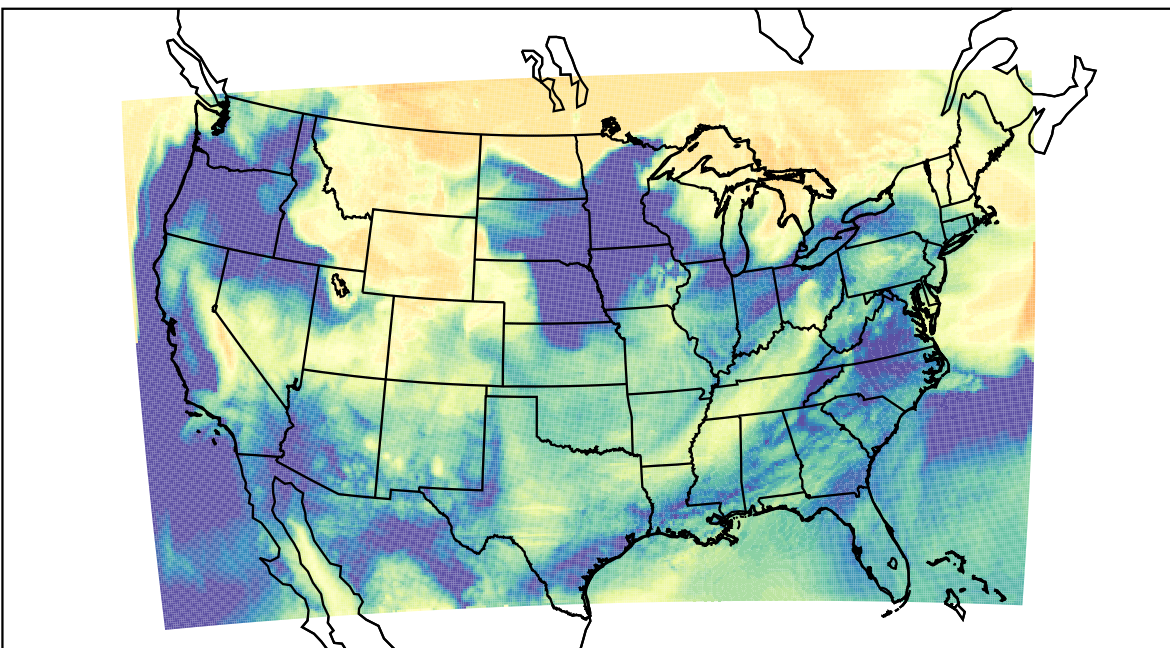
WRF (2023-03-27_15:00:00)
