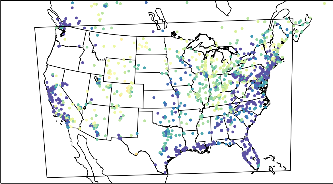
AirNOW (2023-03-27_12:00:00)
