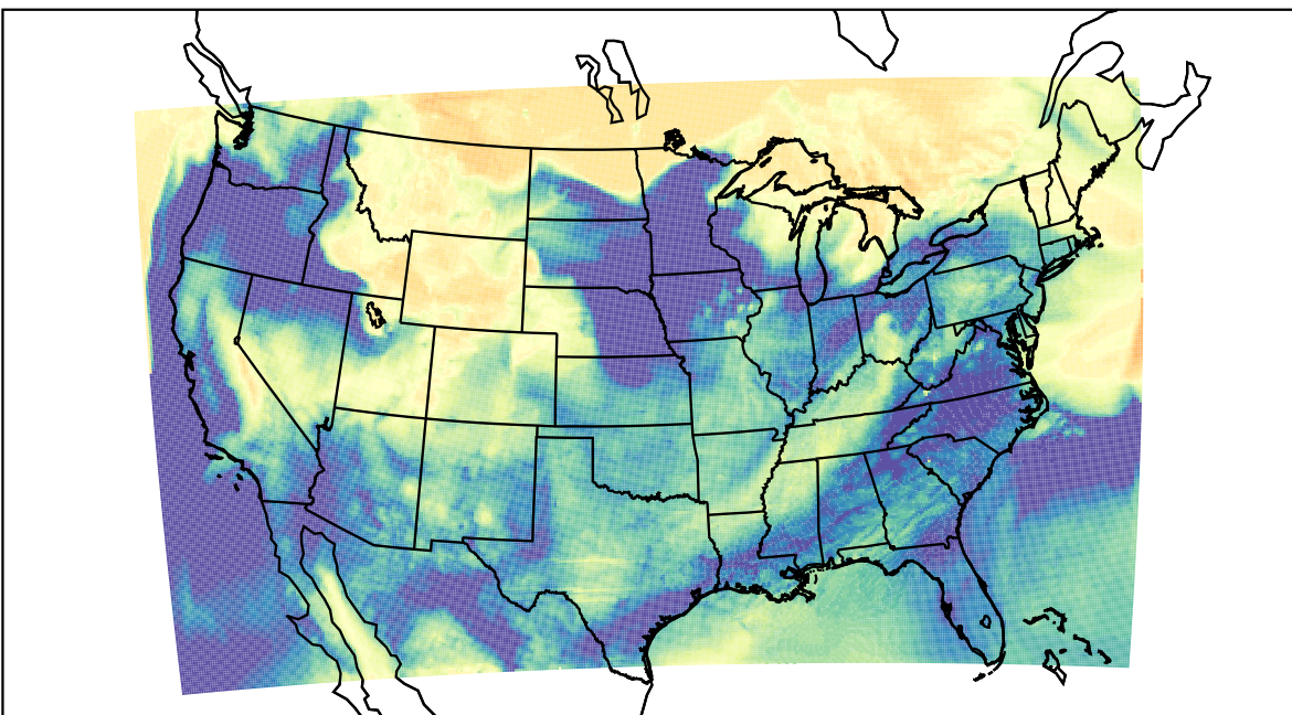
WRF (2023-03-27_14:00:00)
