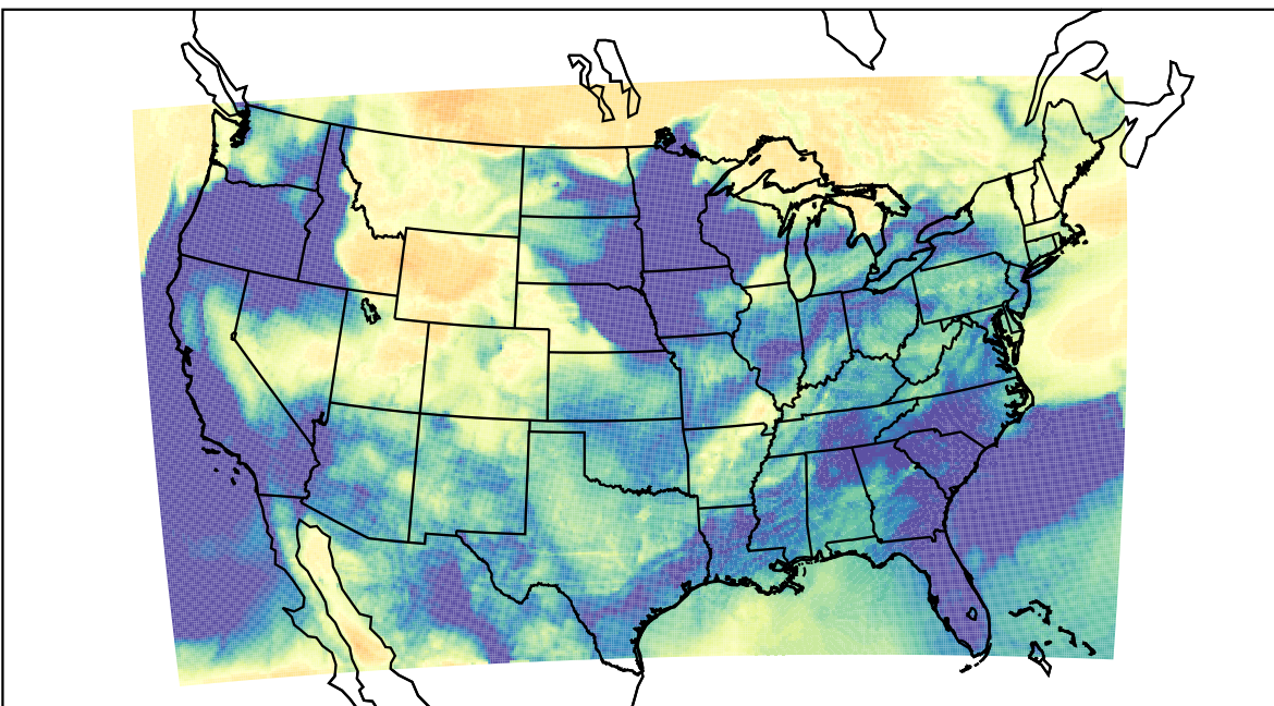
WRF (2023-03-27_07:00:00)
