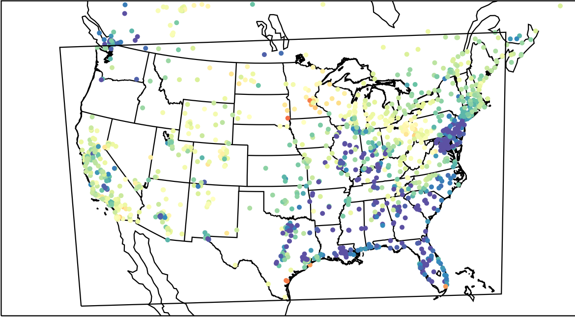
AirNOW (2023-03-26_03:00:00)
