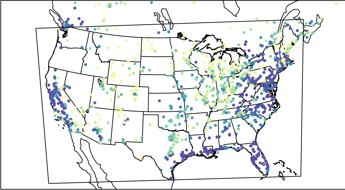
AirNOW (2023-03-27_09:00:00)
