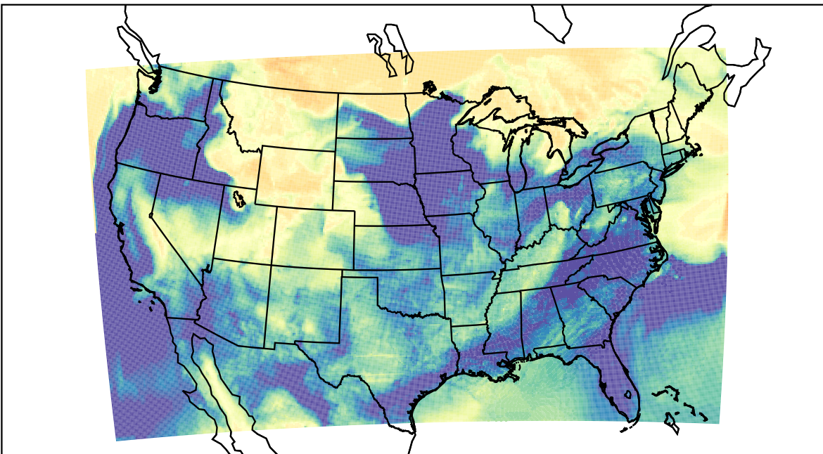
WRF (2023-03-27_13:00:00)
