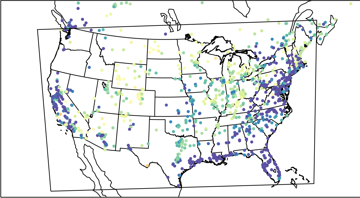
AirNOW (2023-03-27_10:00:00)
