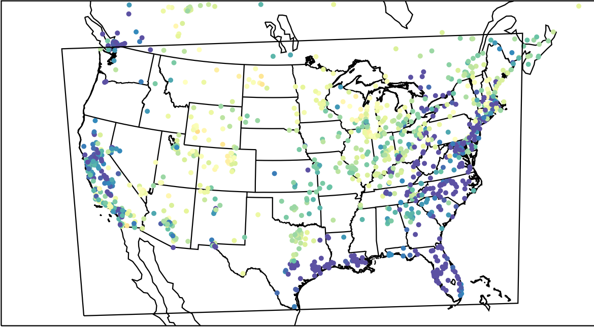
AirNOW (2023-03-27_06:00:00)
