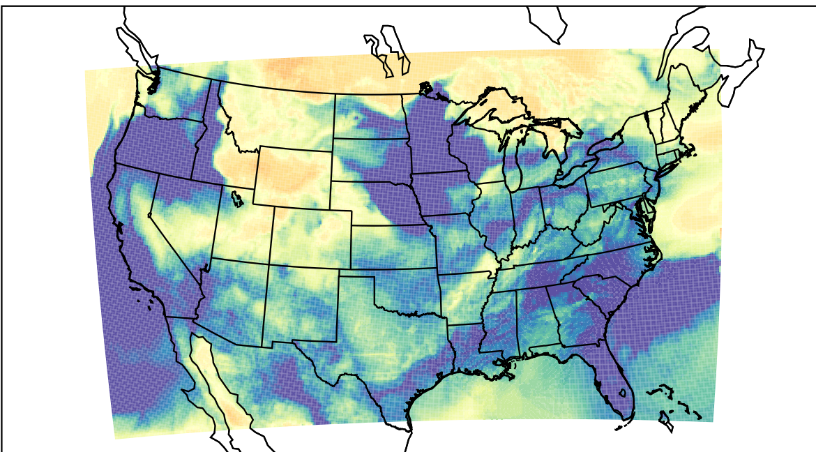
WRF (2023-03-27_08:00:00)
