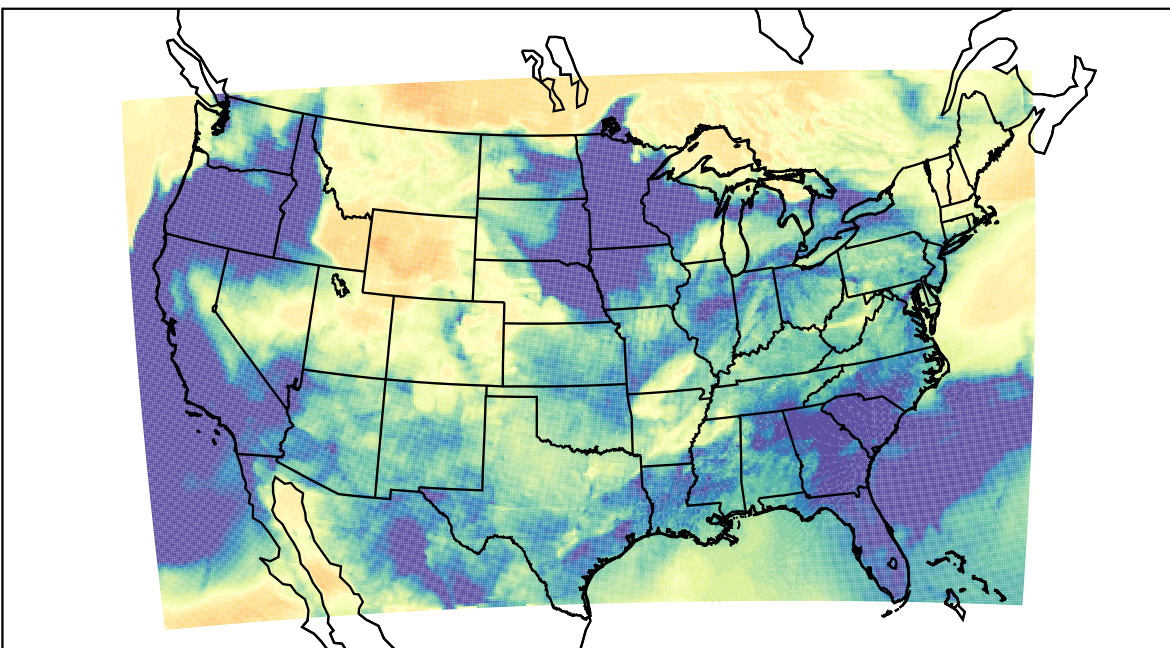
WRF (2023-03-27_04:00:00)
