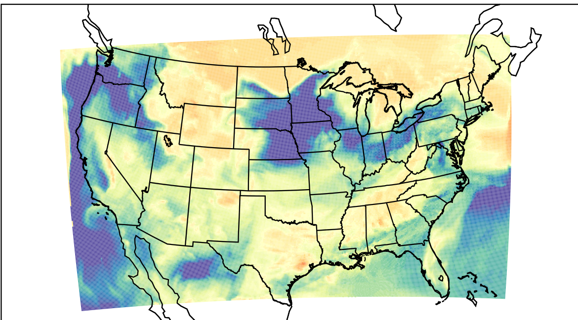
WRF (2023-03-27_19:00:00)
