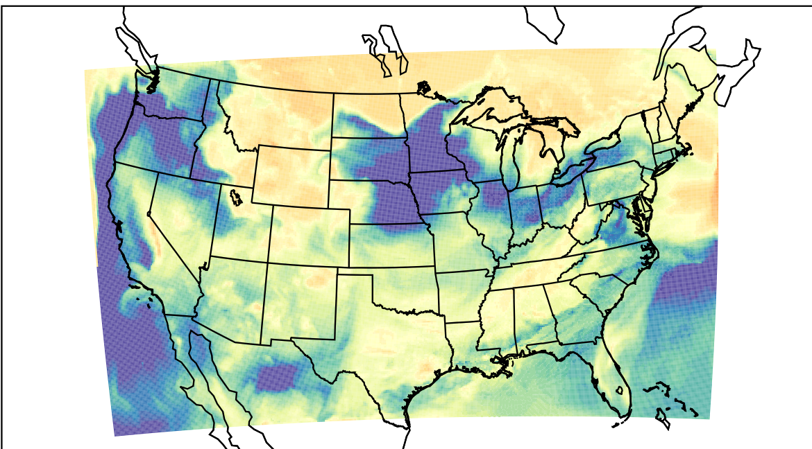
WRF (2023-03-27_18:00:00)
