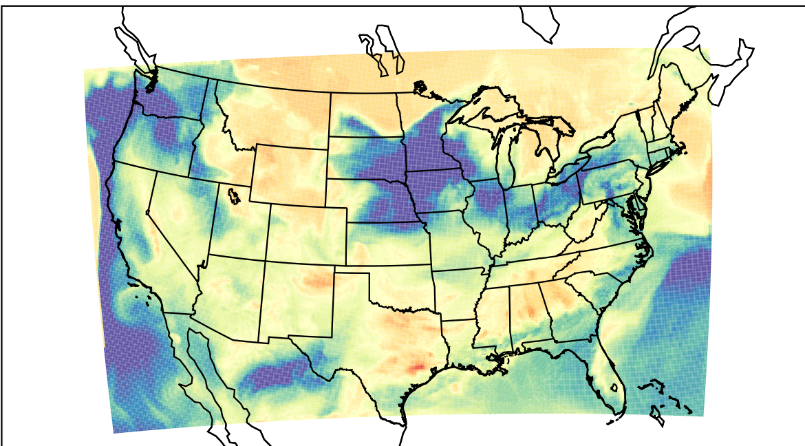
WRF (2023-03-27_21:00:00)
