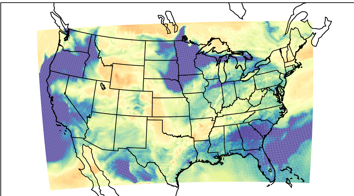
WRF (2023-03-27_00:00:00)
