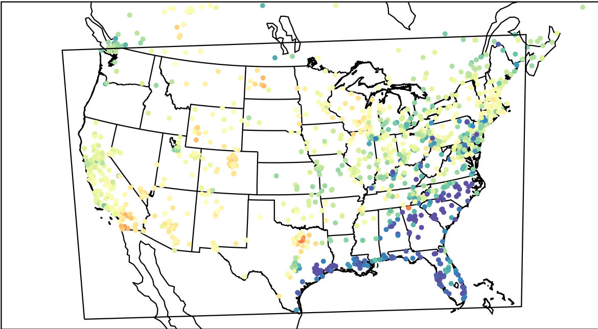
AirNOW (2023-03-27_00:00:00)
