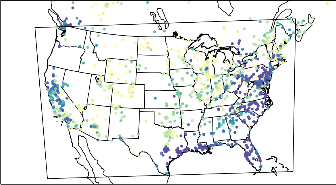
AirNOW (2023-03-27_05:00:00)
