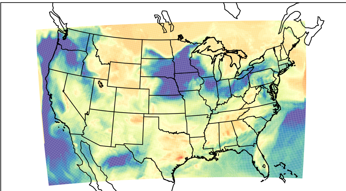
WRF (2023-03-27_20:00:00)
