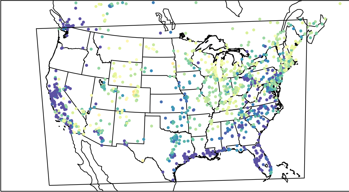
AirNOW (2023-03-27_13:00:00)
