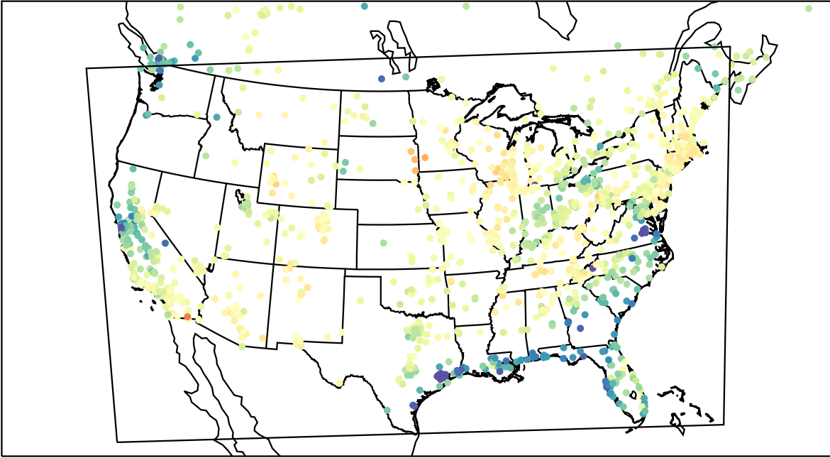
AirNOW (2023-03-27_18:00:00)
