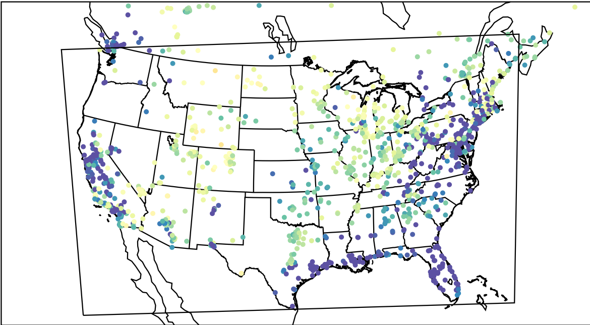
AirNOW (2023-03-27_08:00:00)
