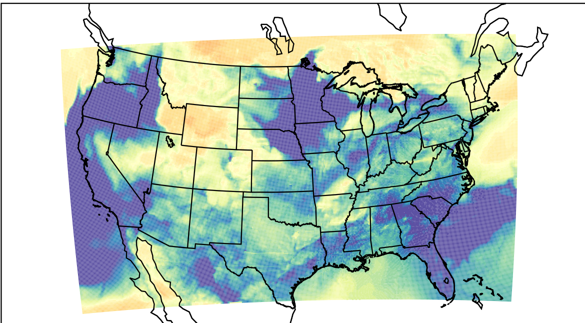
WRF (2023-03-27_05:00:00)
