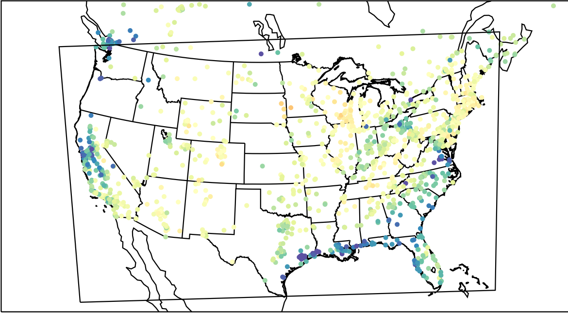
AirNOW (2023-03-27_17:00:00)
