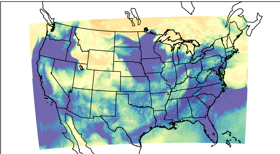
WRF (2023-03-27_11:00:00)
