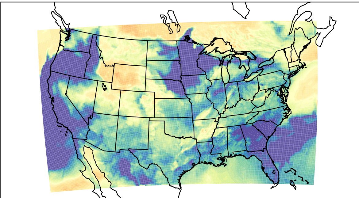
WRF (2023-03-27_03:00:00)
