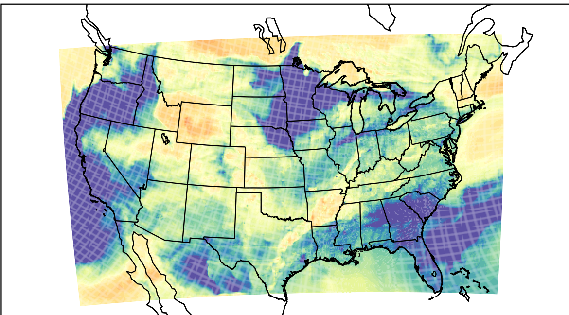
WRF (2023-03-27_01:00:00)
