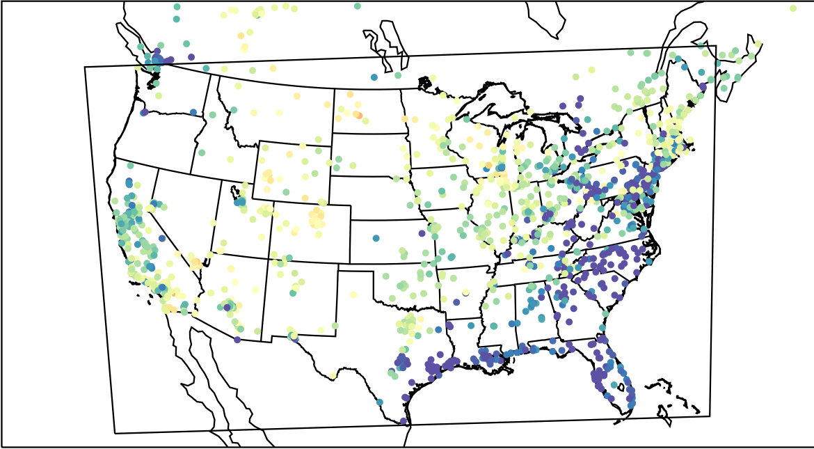
AirNOW (2023-03-27_03:00:00)
