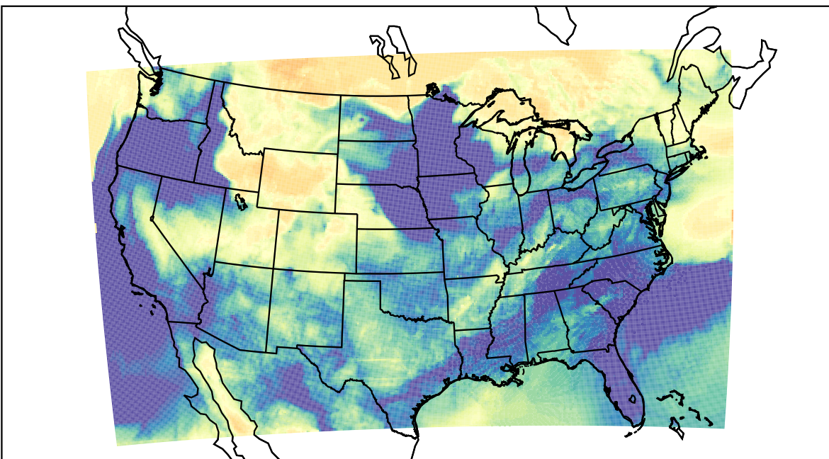
WRF (2023-03-27_09:00:00)
