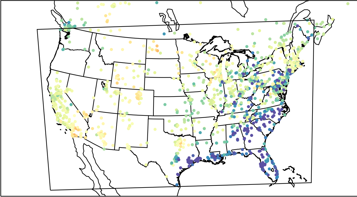
AirNOW (2023-03-27_01:00:00)
