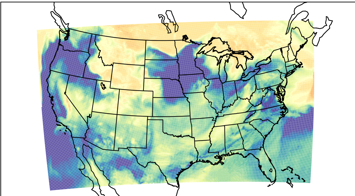
WRF (2023-03-27_16:00:00)
