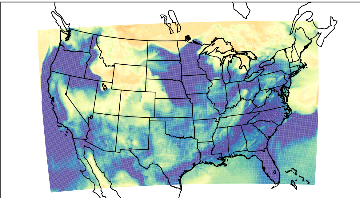
WRF (2023-03-27_12:00:00)
