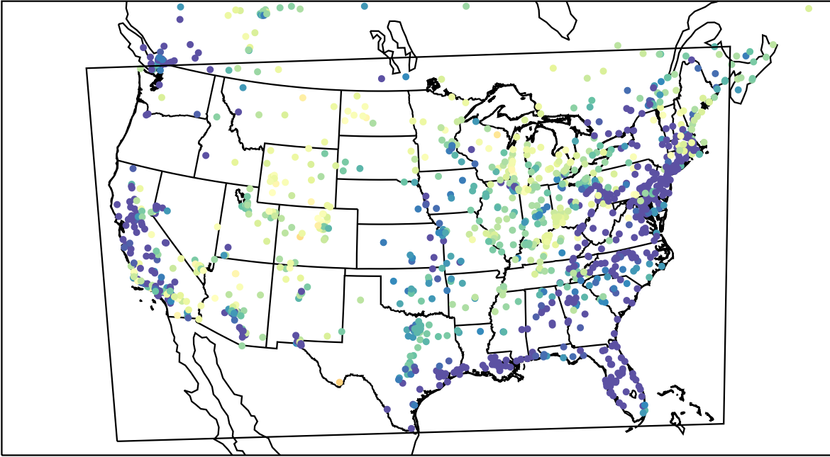
AirNOW (2023-03-27_11:00:00)
