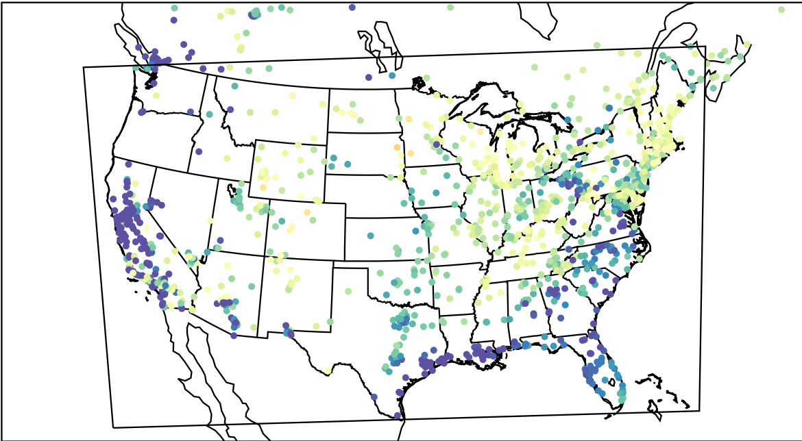
AirNOW (2023-03-27_14:00:00)
