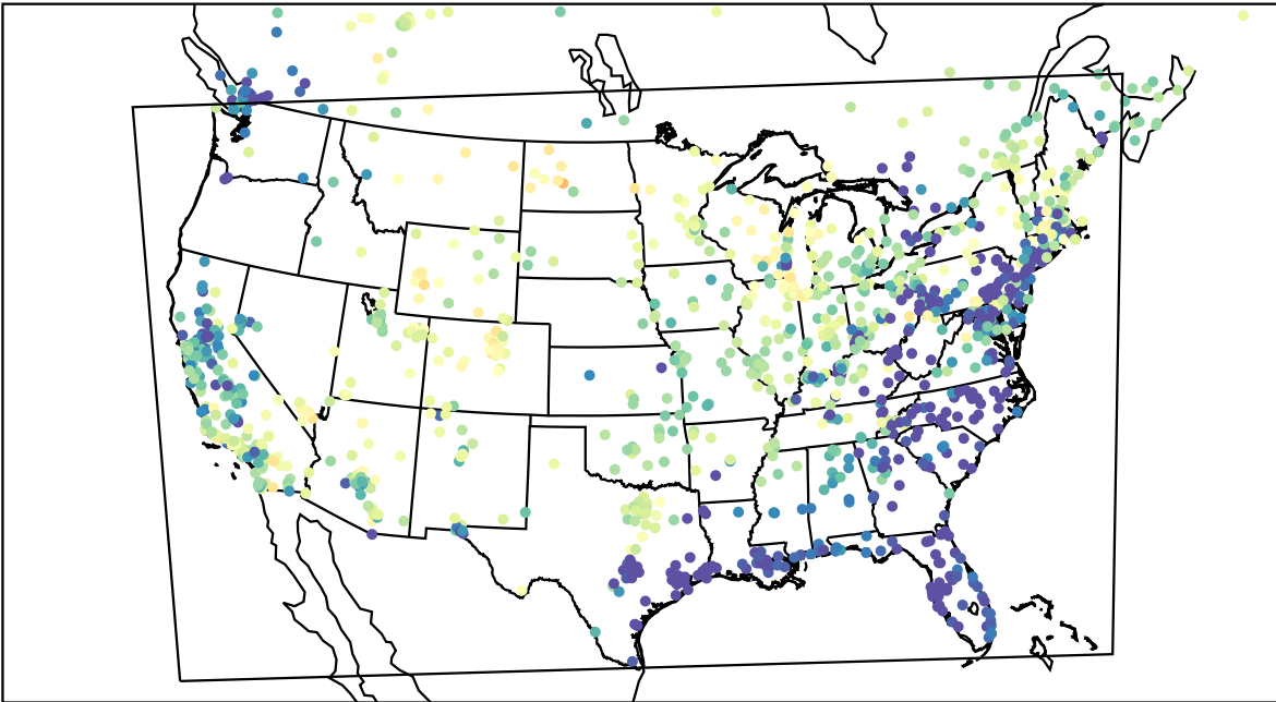
AirNOW (2023-03-27_04:00:00)
