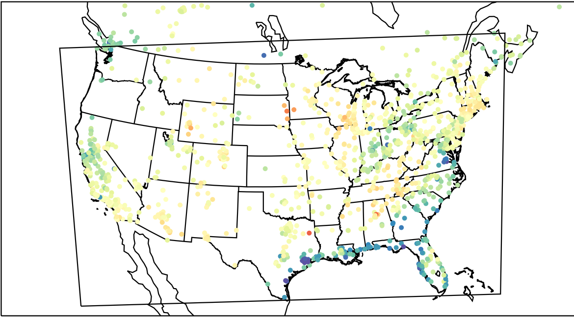
AirNOW (2023-03-27_19:00:00)
