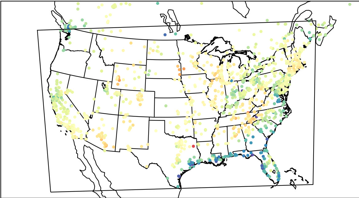
AirNOW (2023-03-27_20:00:00)
