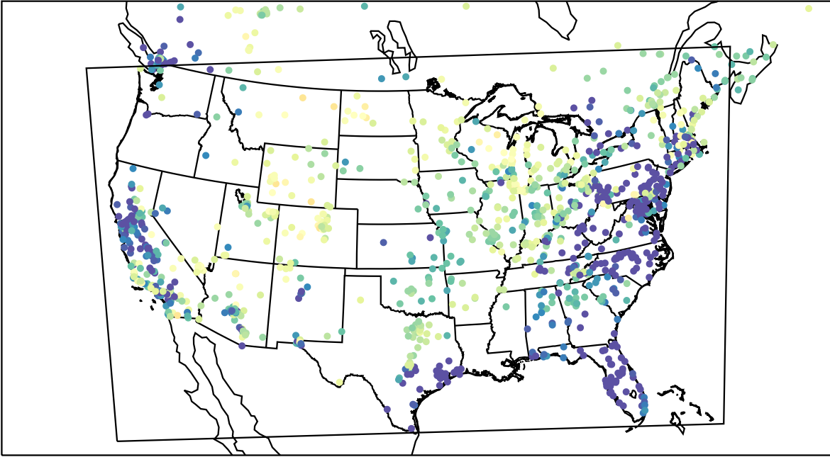
AirNOW (2023-03-27_07:00:00)
