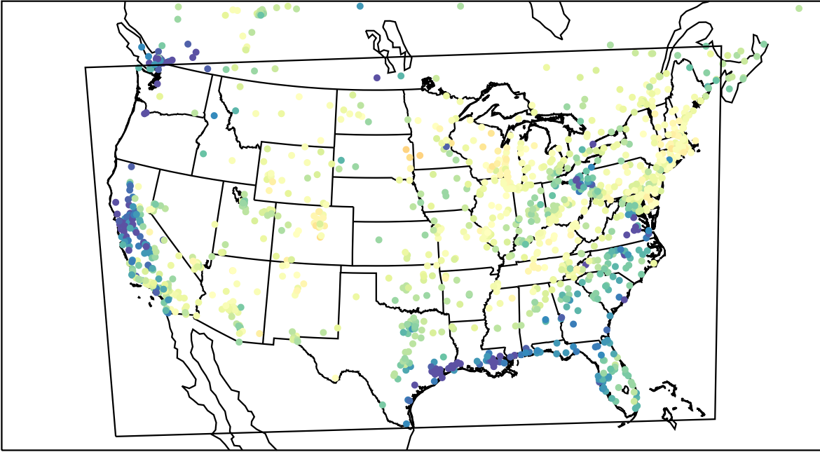
AirNOW (2023-03-27_16:00:00)
