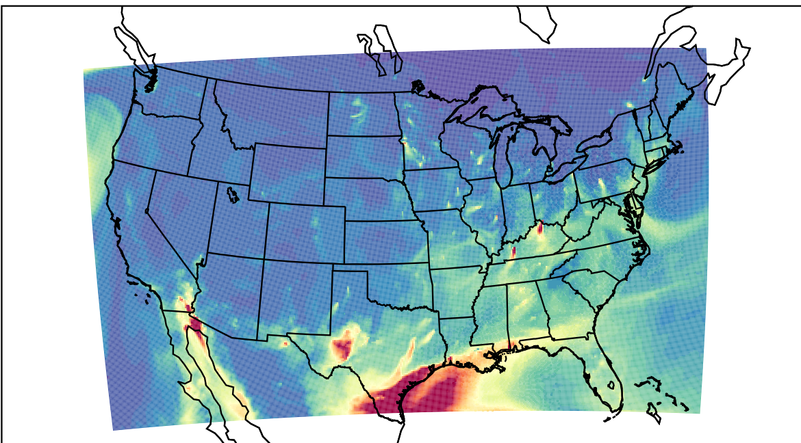
WRF 2023-03-28_11:00:00
