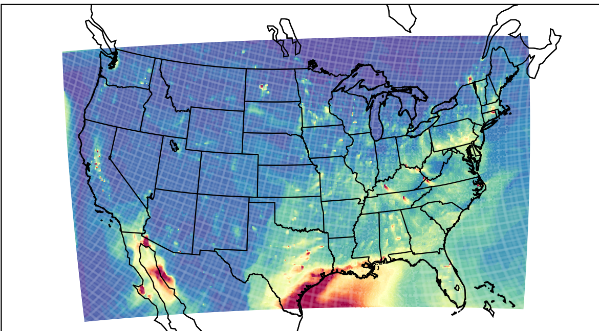
WRF 2023-03-28_02:00:00
