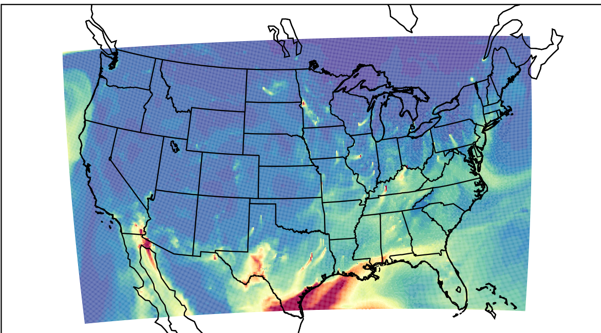
WRF 2023-03-28_14:00:00
