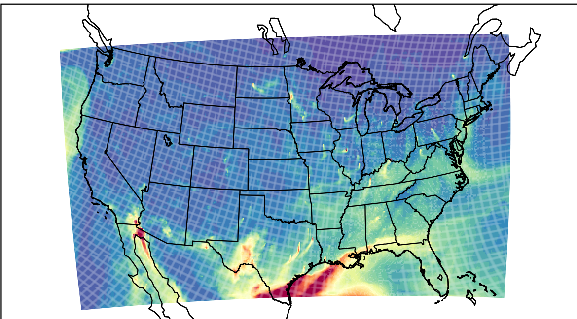
WRF 2023-03-28_15:00:00
