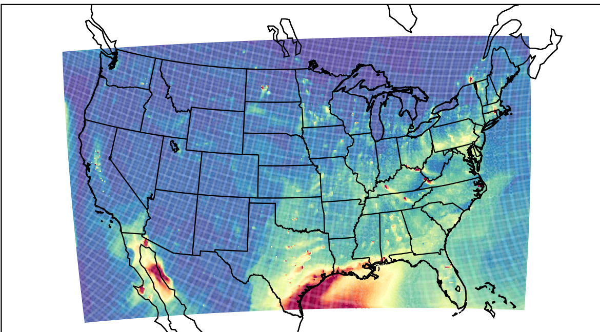
WRF 2023-03-28_01:00:00
