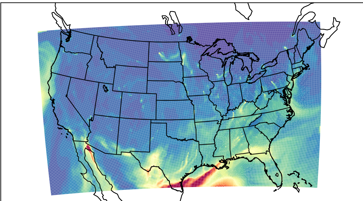
WRF 2023-03-28_17:00:00
