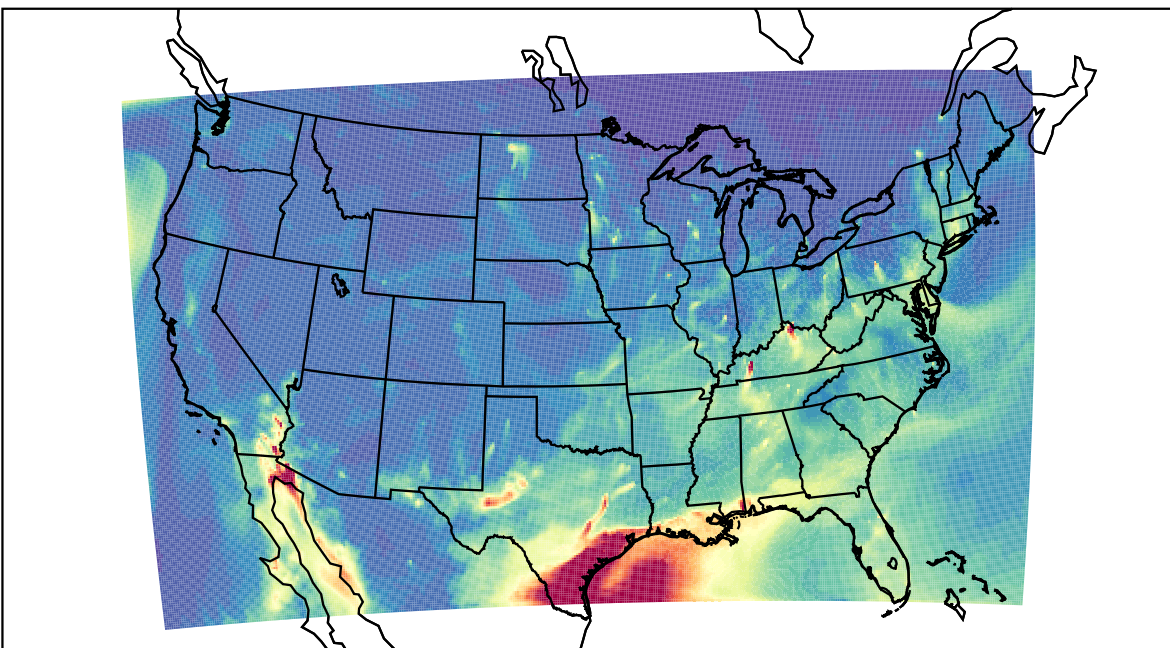
WRF 2023-03-28_08:00:00
