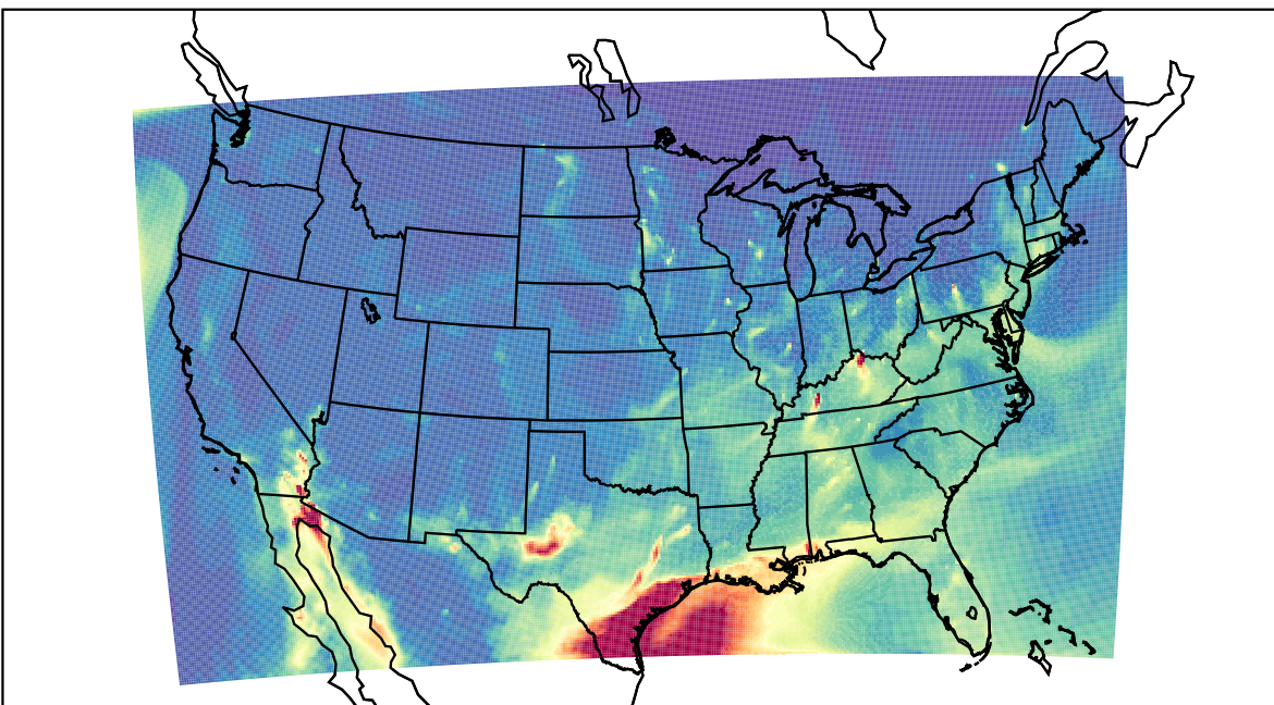
WRF 2023-03-28_09:00:00
