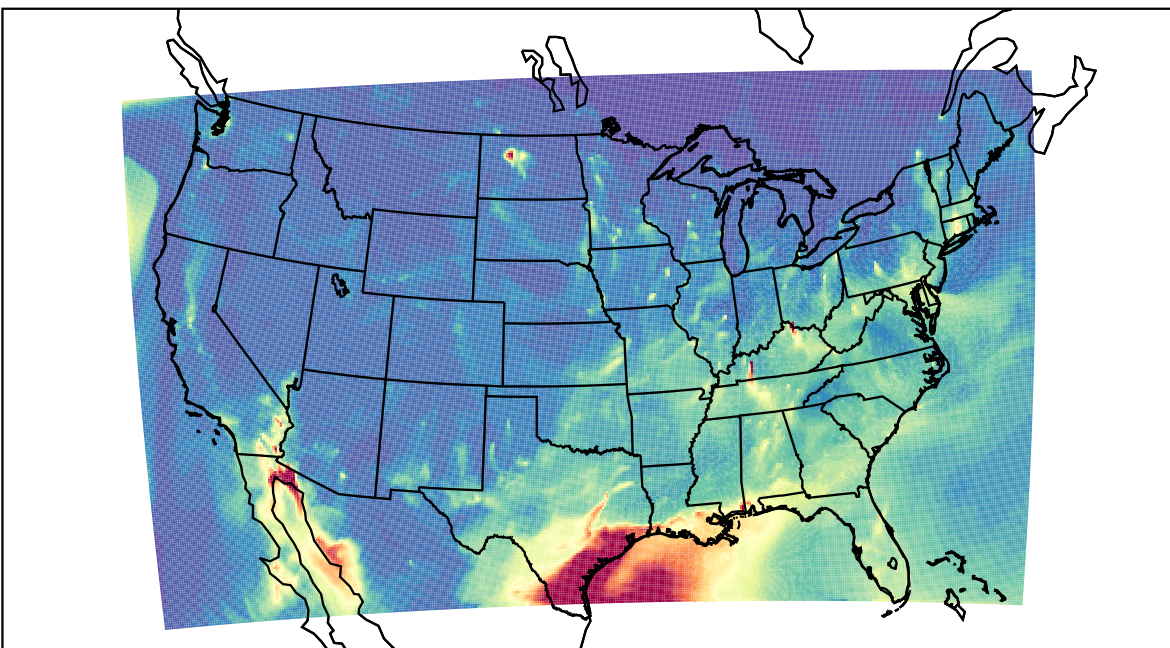
WRF 2023-03-28_06:00:00
