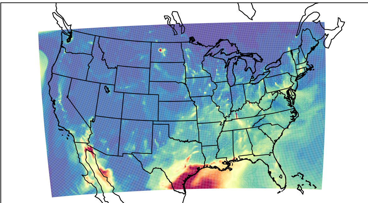
WRF 2023-03-28_05:00:00
