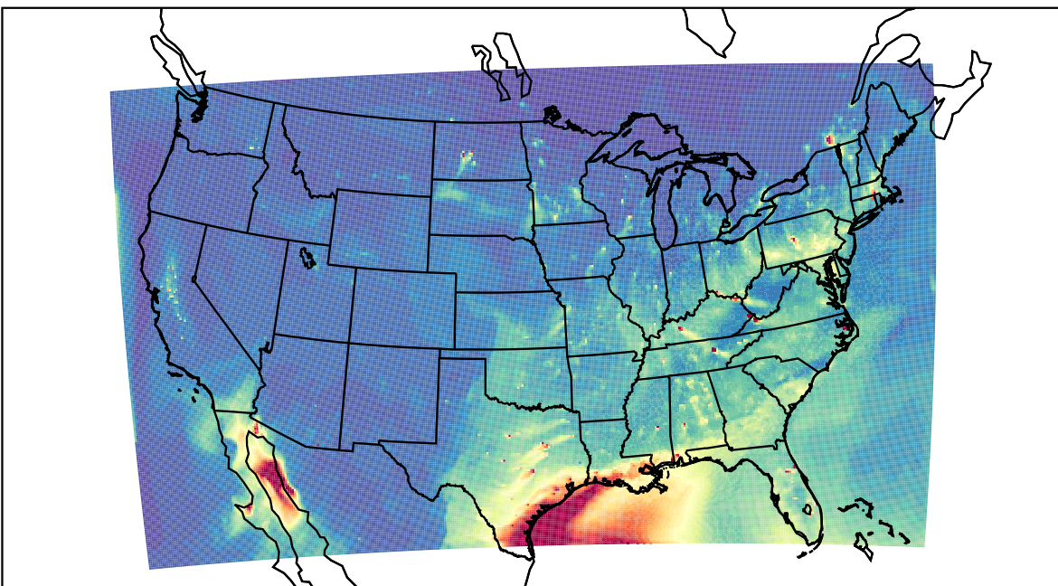
WRF 2023-03-28_00:00:00
