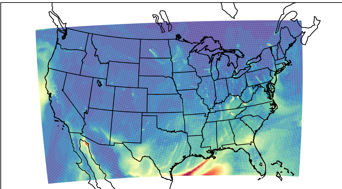
WRF 2023-03-28_21:00:00
