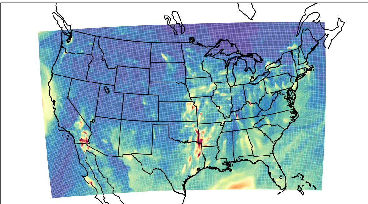
WRF 2023-03-29_05:00:00
