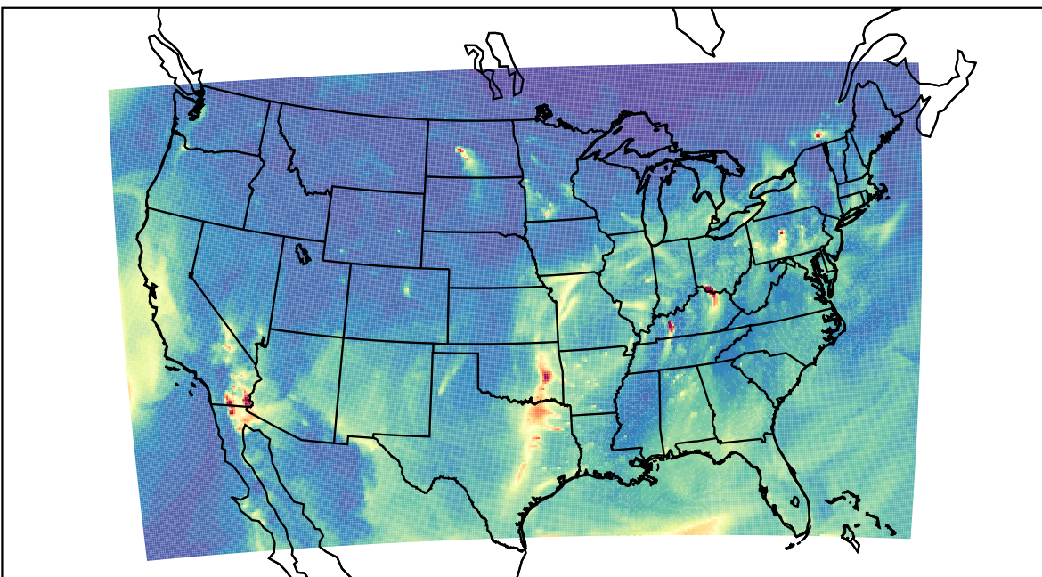
WRF 2023-03-29_12:00:00
