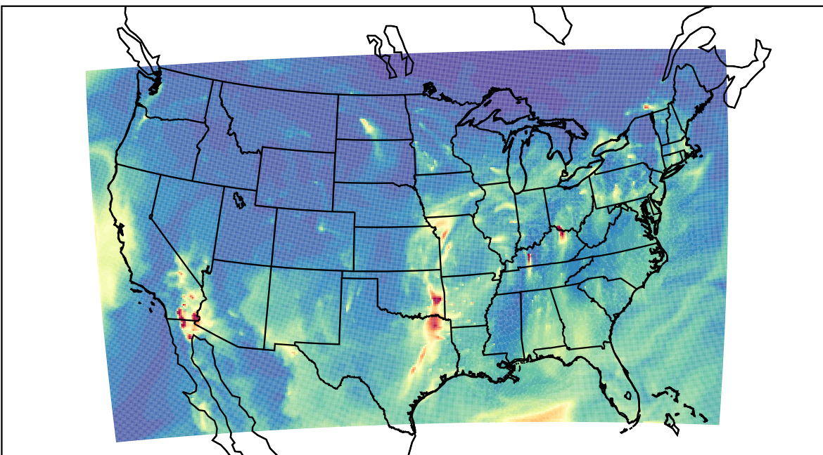
WRF 2023-03-29_09:00:00
