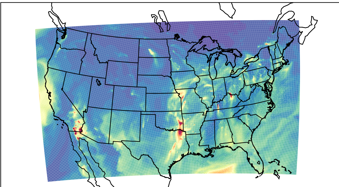
WRF 2023-03-29_08:00:00
