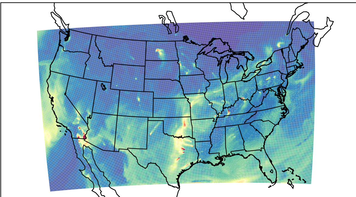
WRF 2023-03-29_15:00:00
