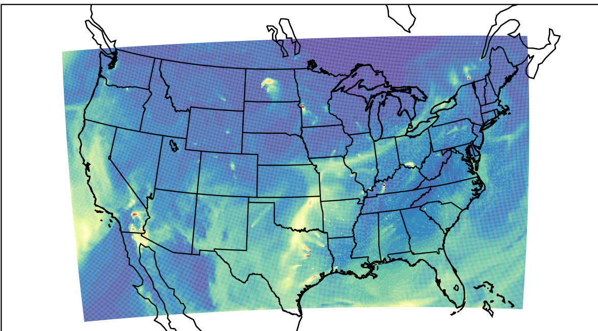
WRF 2023-03-29_17:00:00
