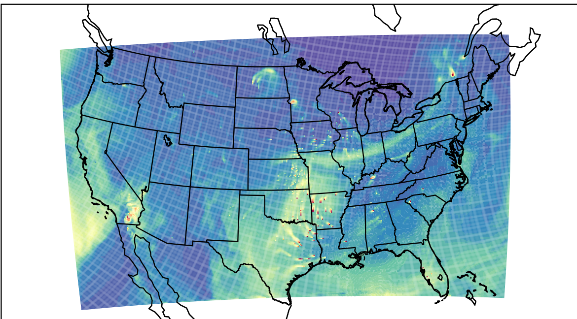
WRF 2023-03-29_21:00:00
