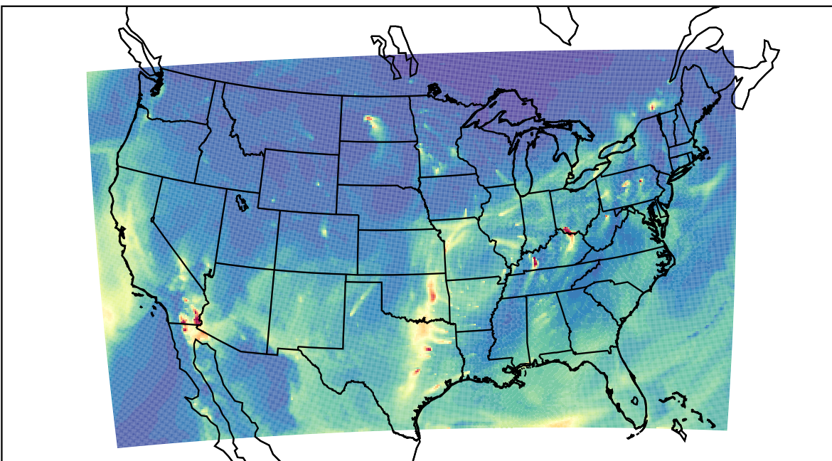
WRF 2023-03-29_14:00:00
