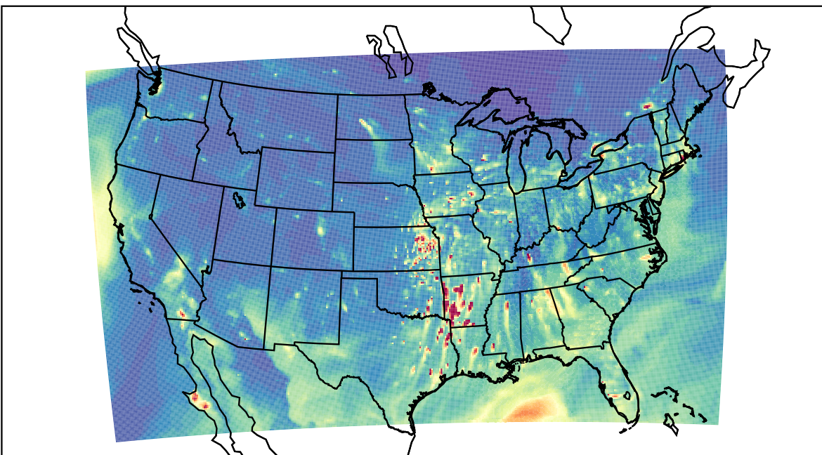
WRF 2023-03-29_02:00:00
