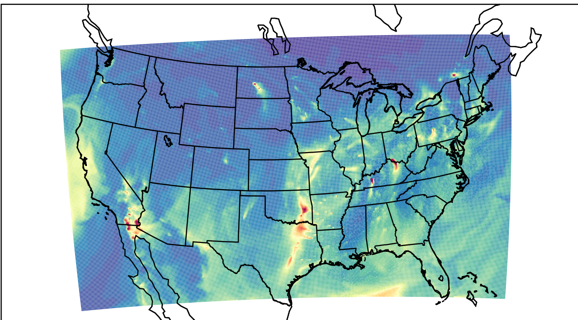
WRF 2023-03-29_11:00:00
