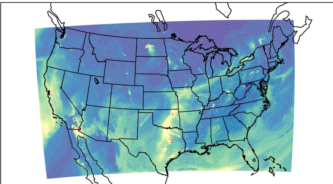
WRF 2023-03-29_16:00:00
