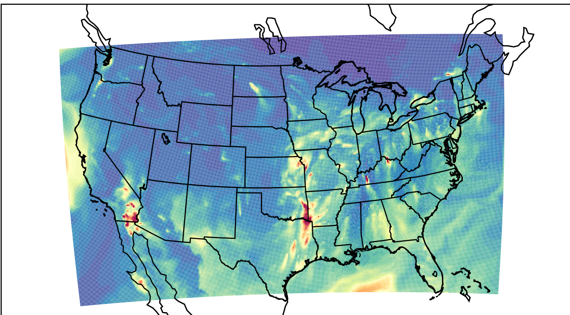
WRF 2023-03-29_06:00:00
