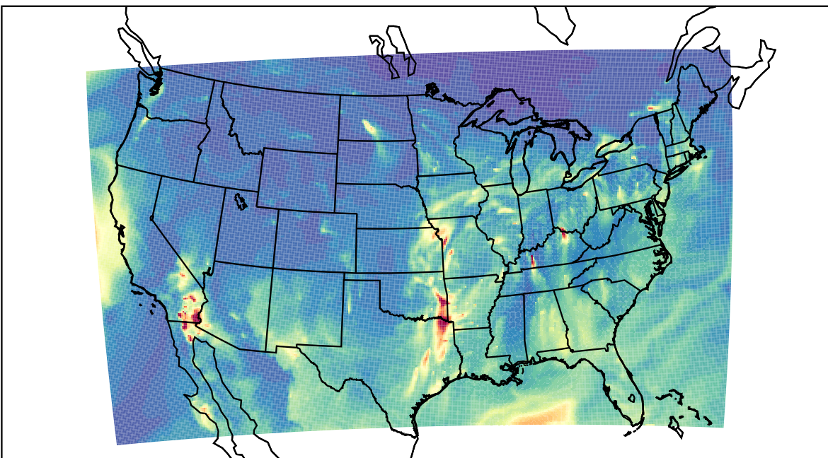
WRF 2023-03-29_07:00:00
