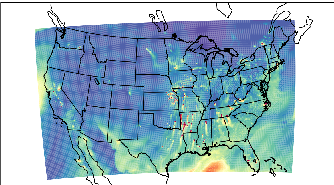
WRF 2023-03-29_00:00:00
