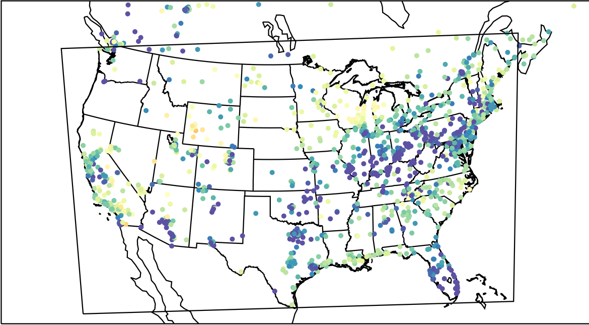
AirNOW (2023-03-29_12:00:00)
