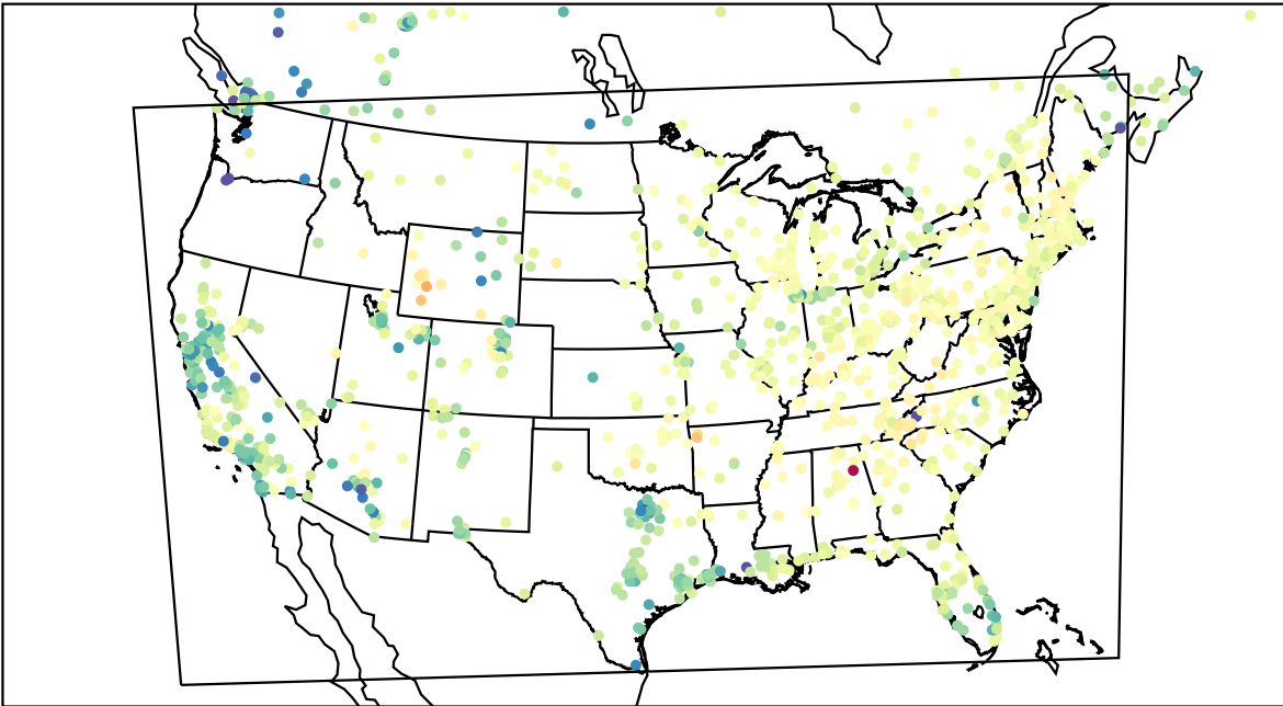
AirNOW (2023-03-29_16:00:00)
