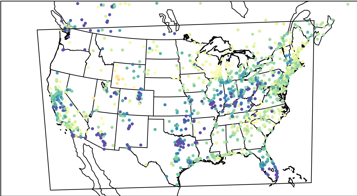
AirNOW (2023-03-29_13:00:00)
