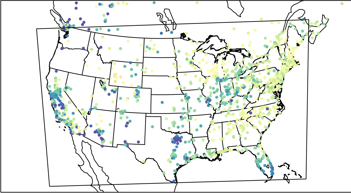
AirNOW (2023-03-29_14:00:00)
