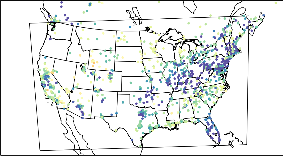
AirNOW (2023-03-29_10:00:00)
