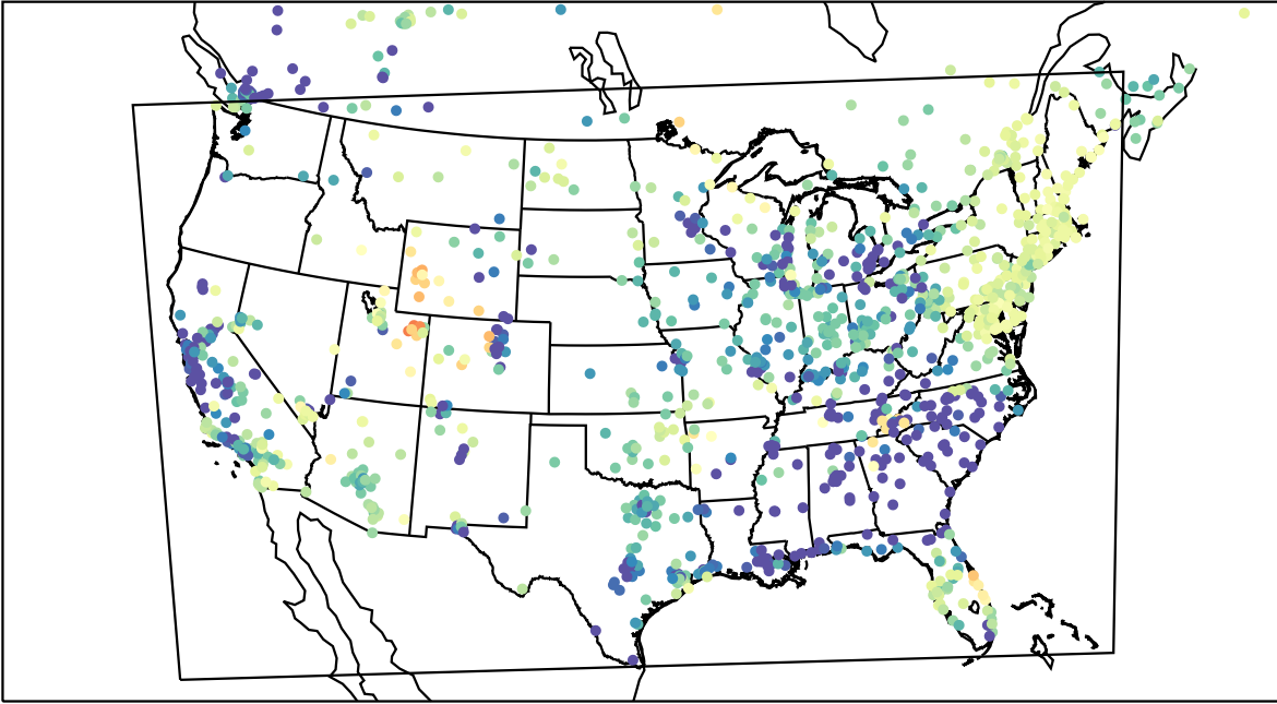
AirNOW (2023-03-30_12:00:00)
