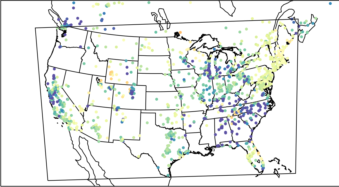
AirNOW (2023-03-30_07:00:00)
