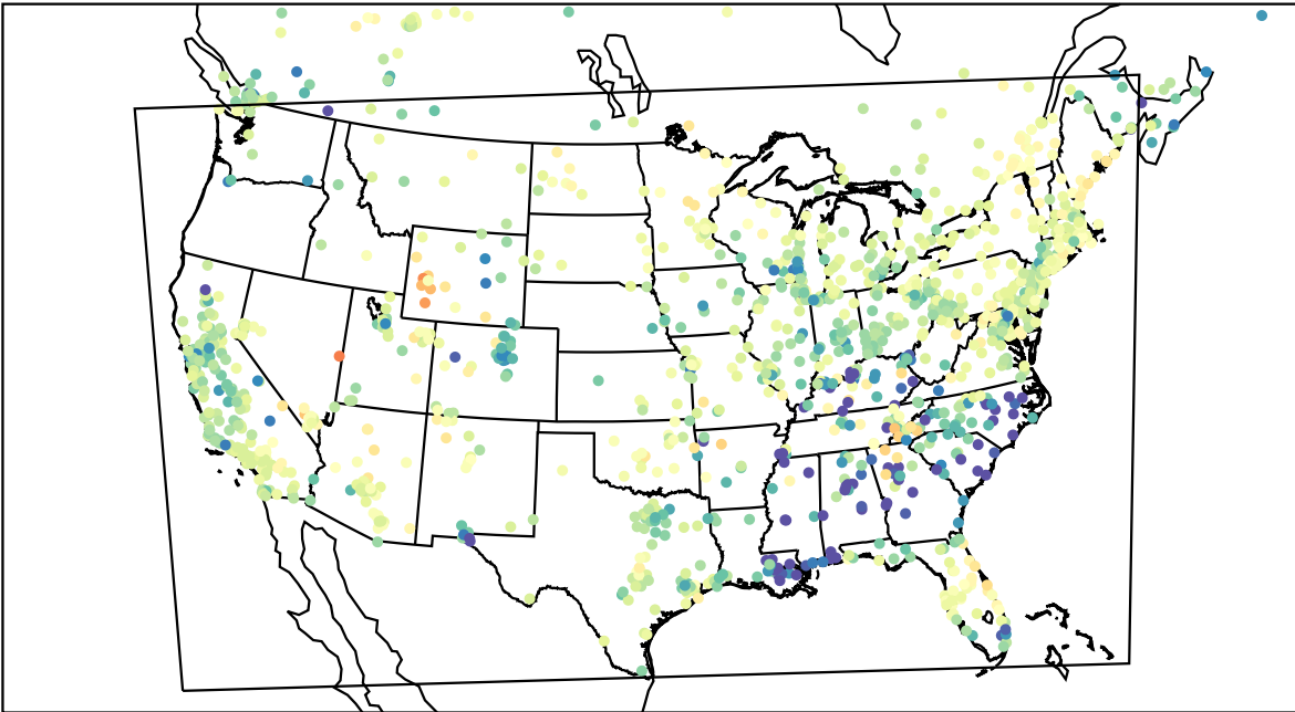
AirNOW (2023-03-30_02:00:00)
