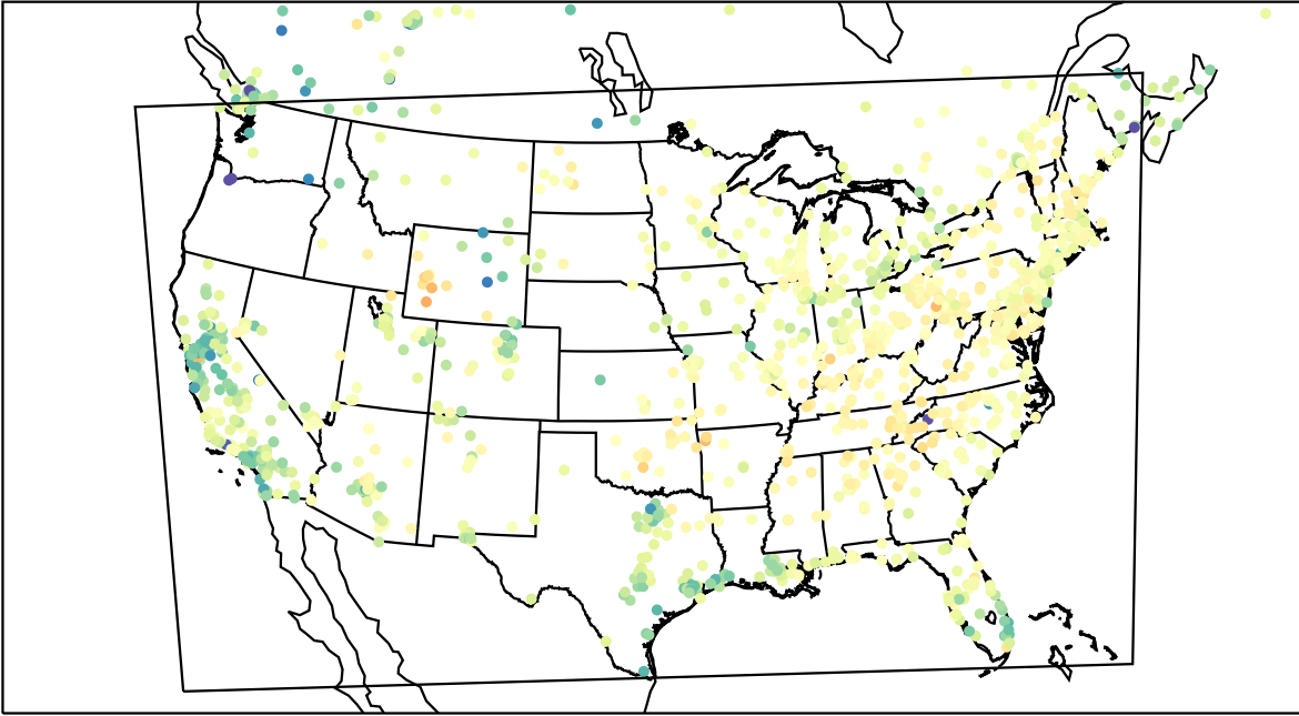
AirNOW (2023-03-29_17:00:00)
