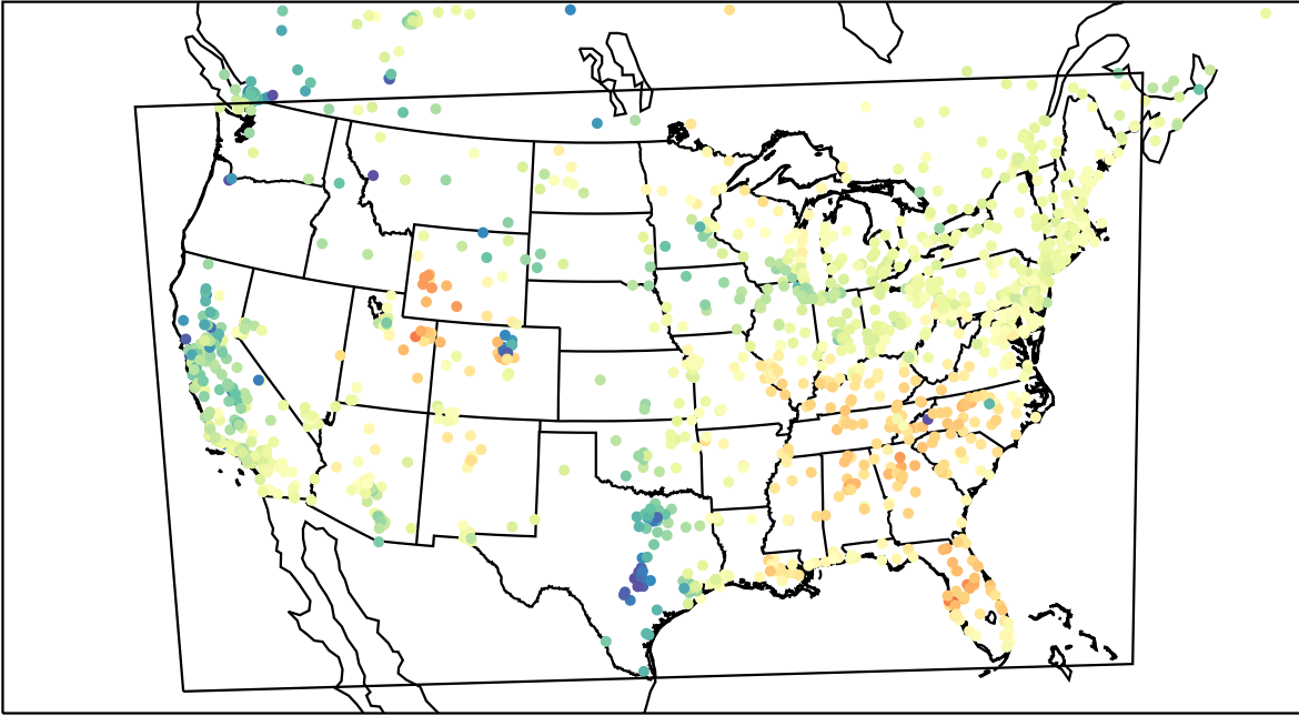
AirNOW (2023-03-30_17:00:00)
