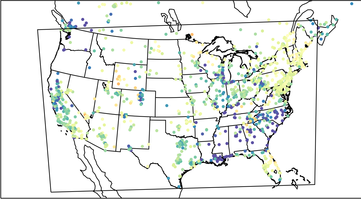
AirNOW (2023-03-30_05:00:00)
