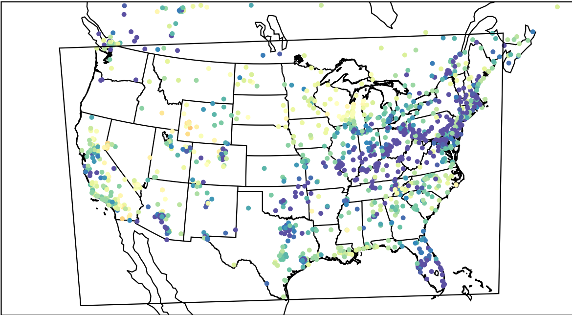
AirNOW (2023-03-29_11:00:00)
