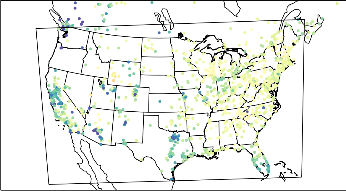
AirNOW (2023-03-29_15:00:00)
