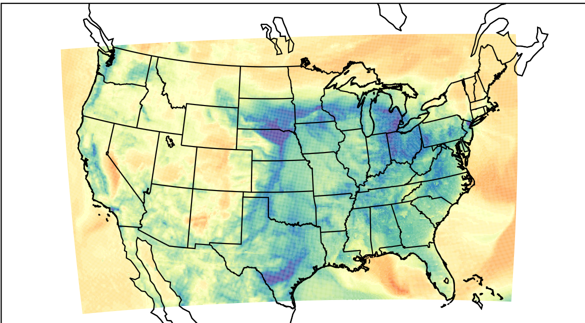
WRF (2023-03-31_08:00:00)
