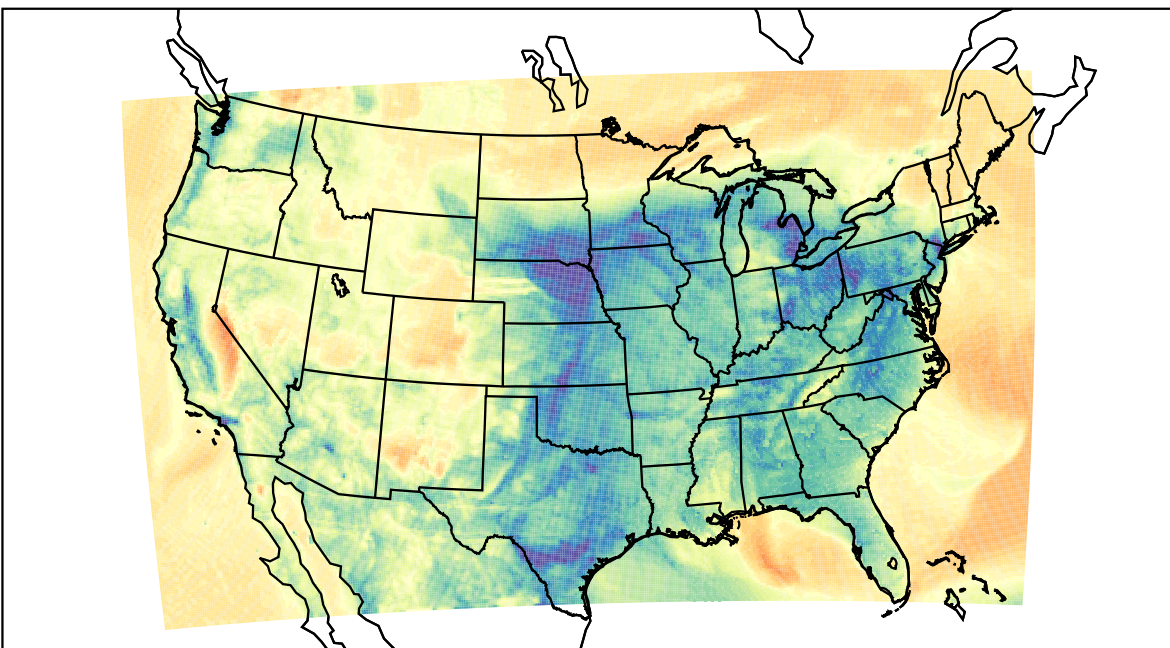
WRF (2023-03-31_11:00:00)
