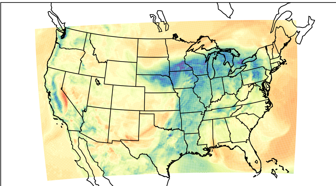
WRF (2023-03-31_16:00:00)
