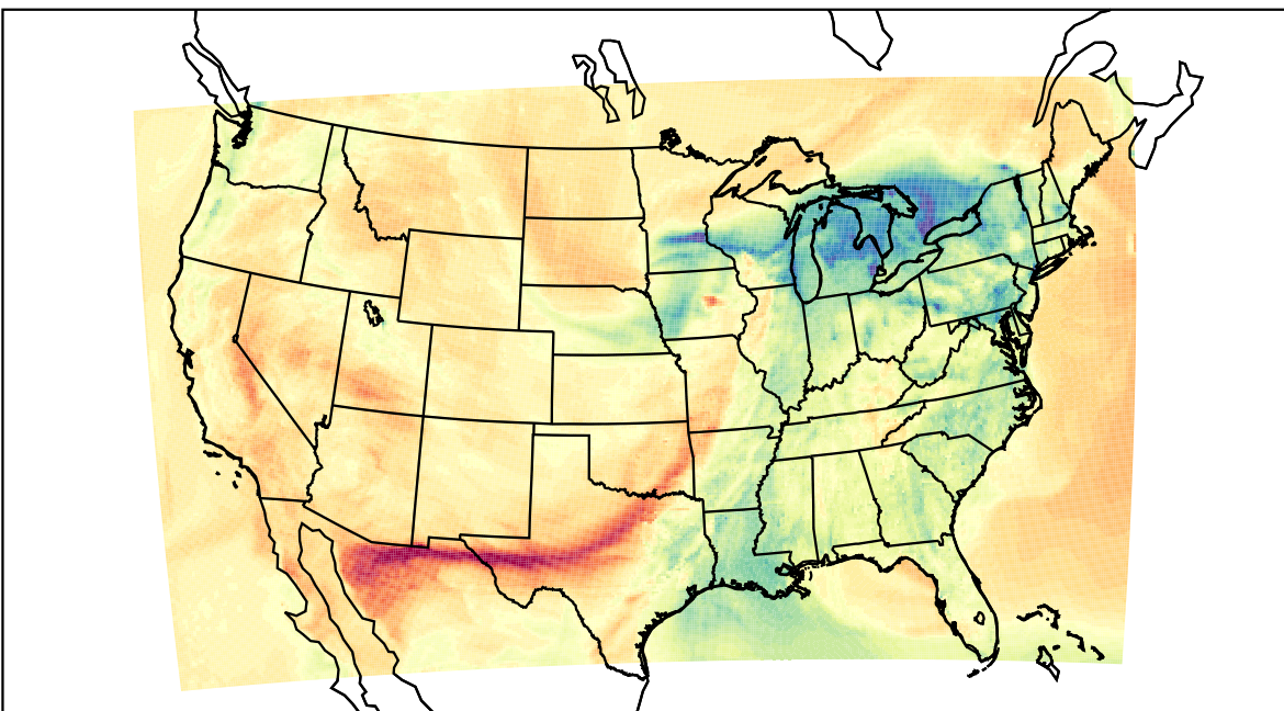
WRF (2023-03-31_23:00:00)
