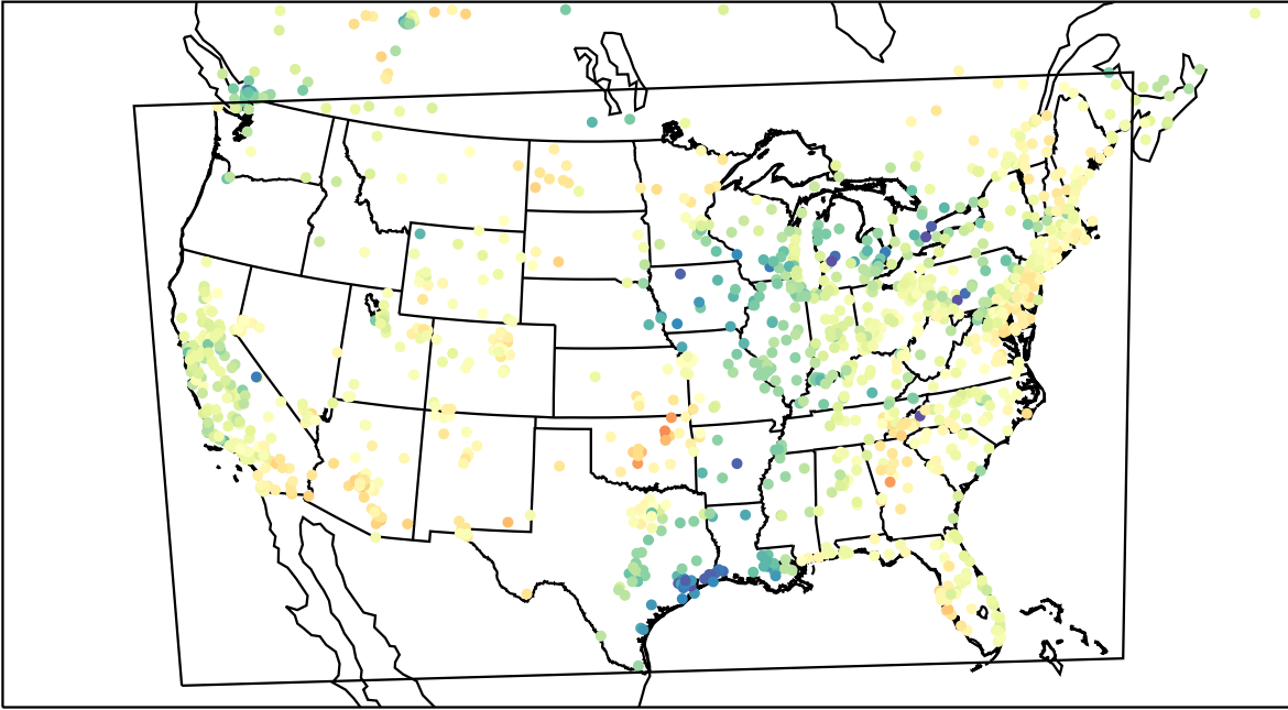
AirNOW (2023-03-31_20:00:00)
