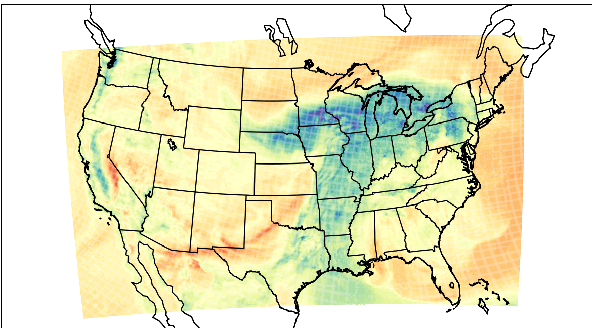
WRF (2023-03-31_17:00:00)
