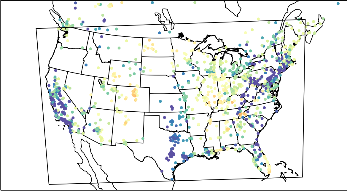
AirNOW (2023-03-31_08:00:00)
