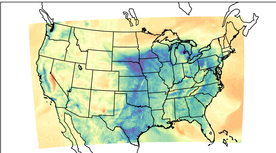
WRF (2023-03-31_13:00:00)
