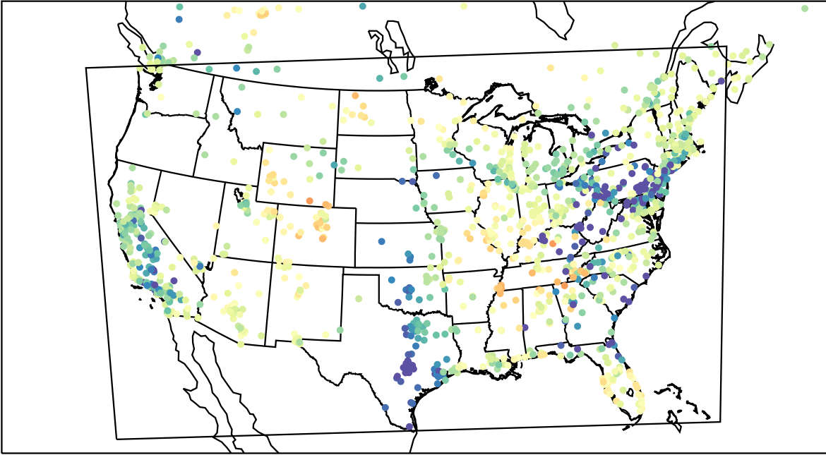
AirNOW (2023-03-31_03:00:00)
