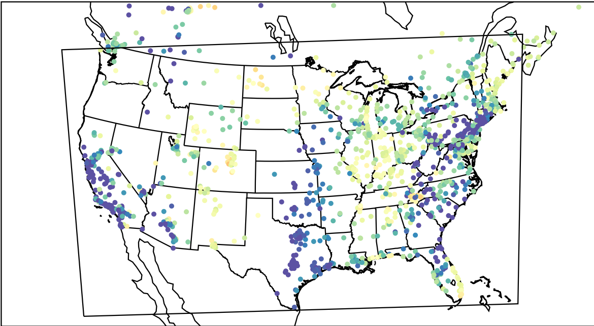
AirNOW (2023-03-31_12:00:00)
