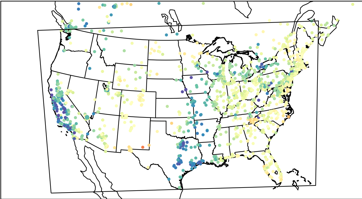
AirNOW (2023-03-31_16:00:00)
