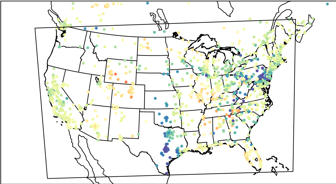
AirNOW (2023-03-31_01:00:00)
