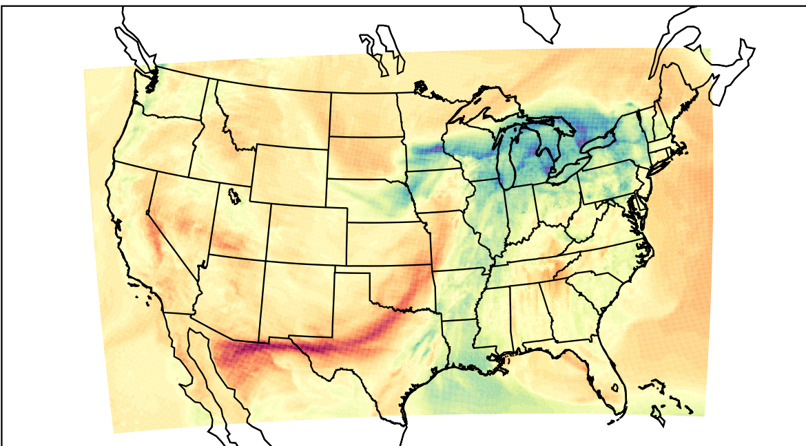
WRF (2023-03-31_21:00:00)
