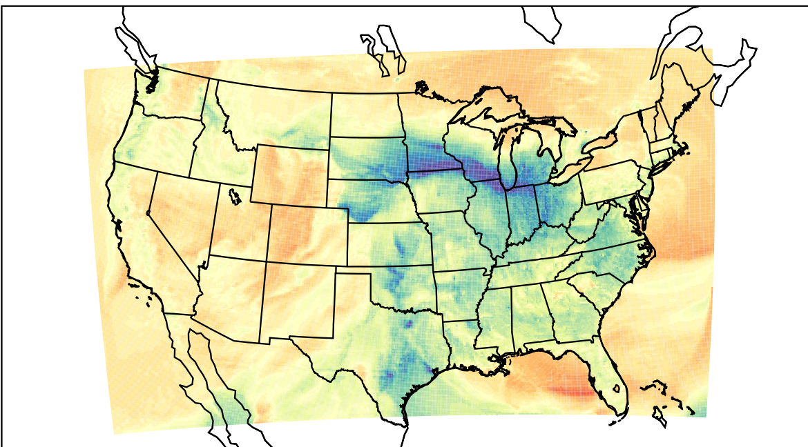
WRF (2023-03-31_00:00:00)
