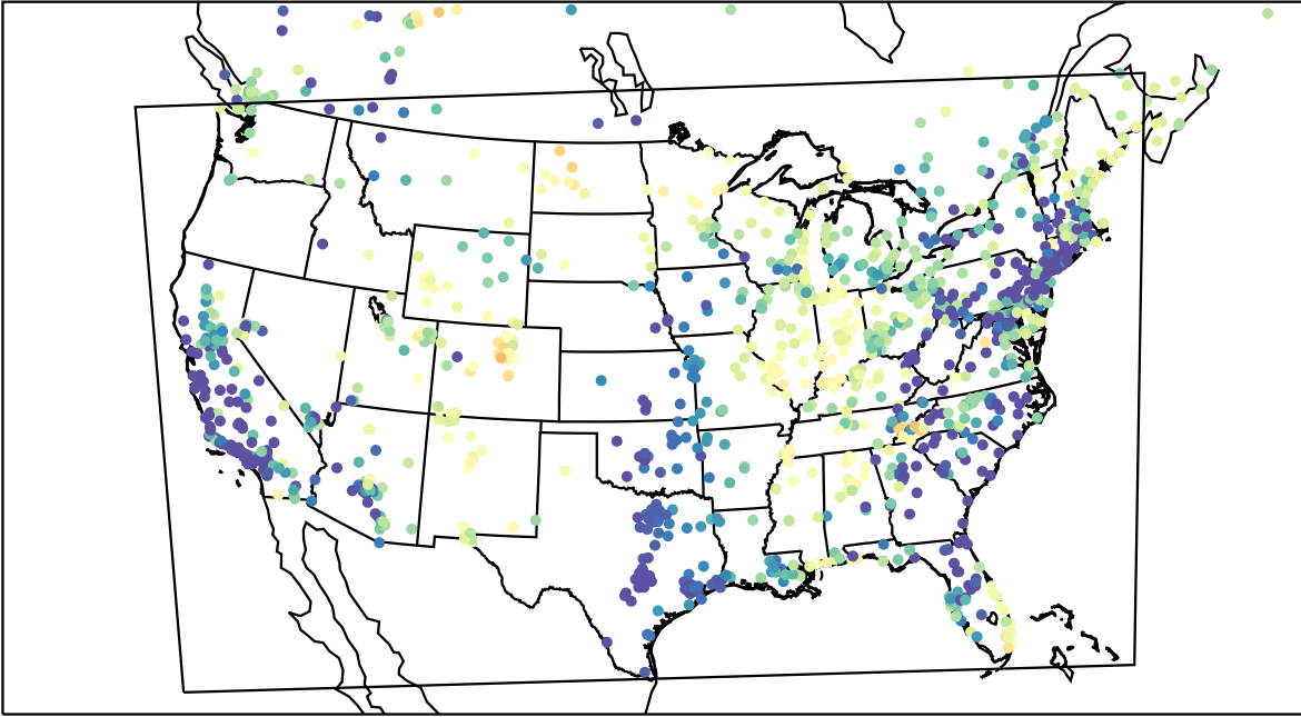
AirNOW (2023-03-31_11:00:00)
