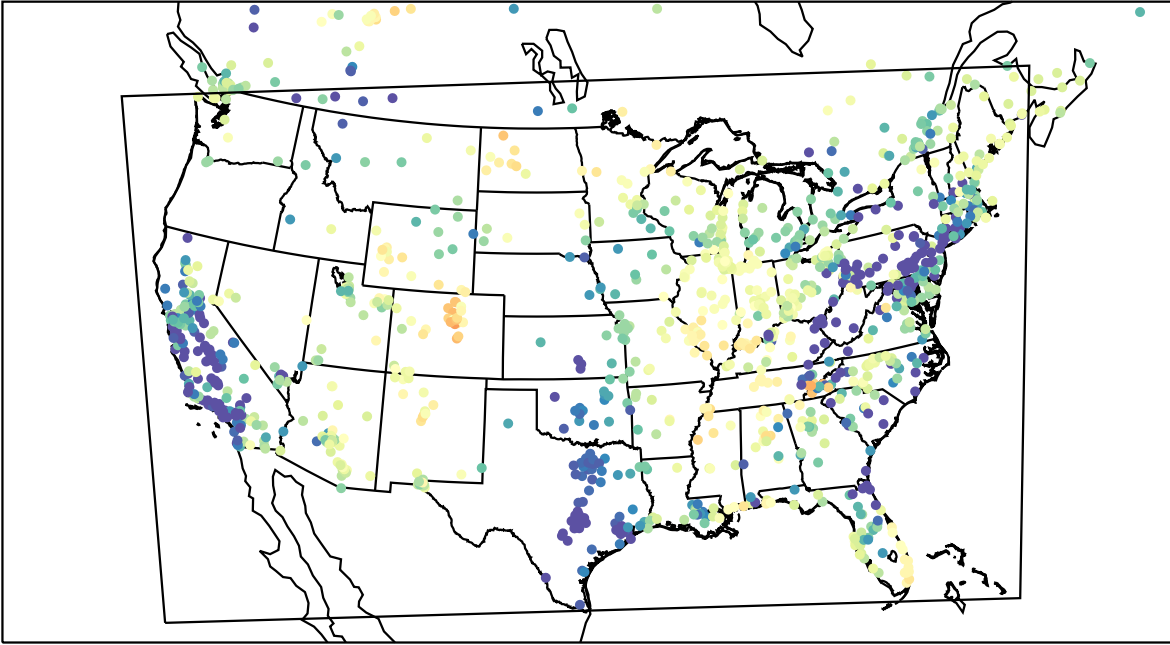
AirNOW (2023-03-31_07:00:00)
