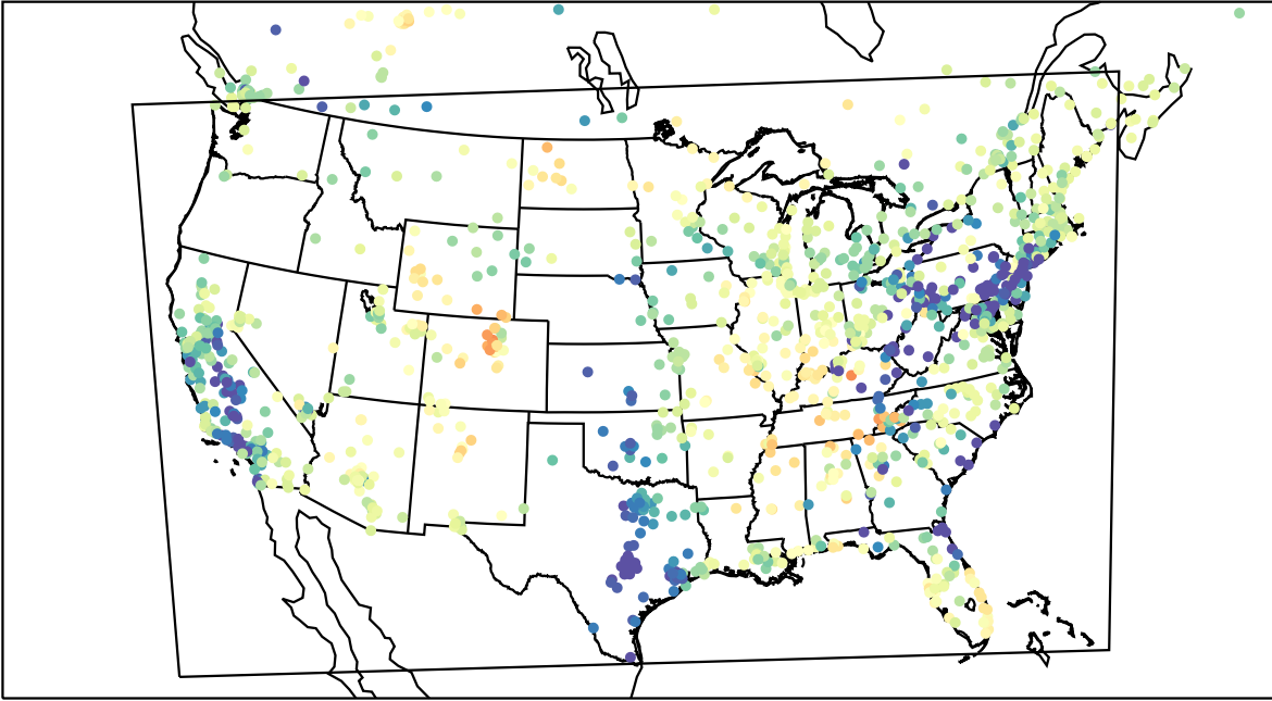
AirNOW (2023-03-31_04:00:00)
