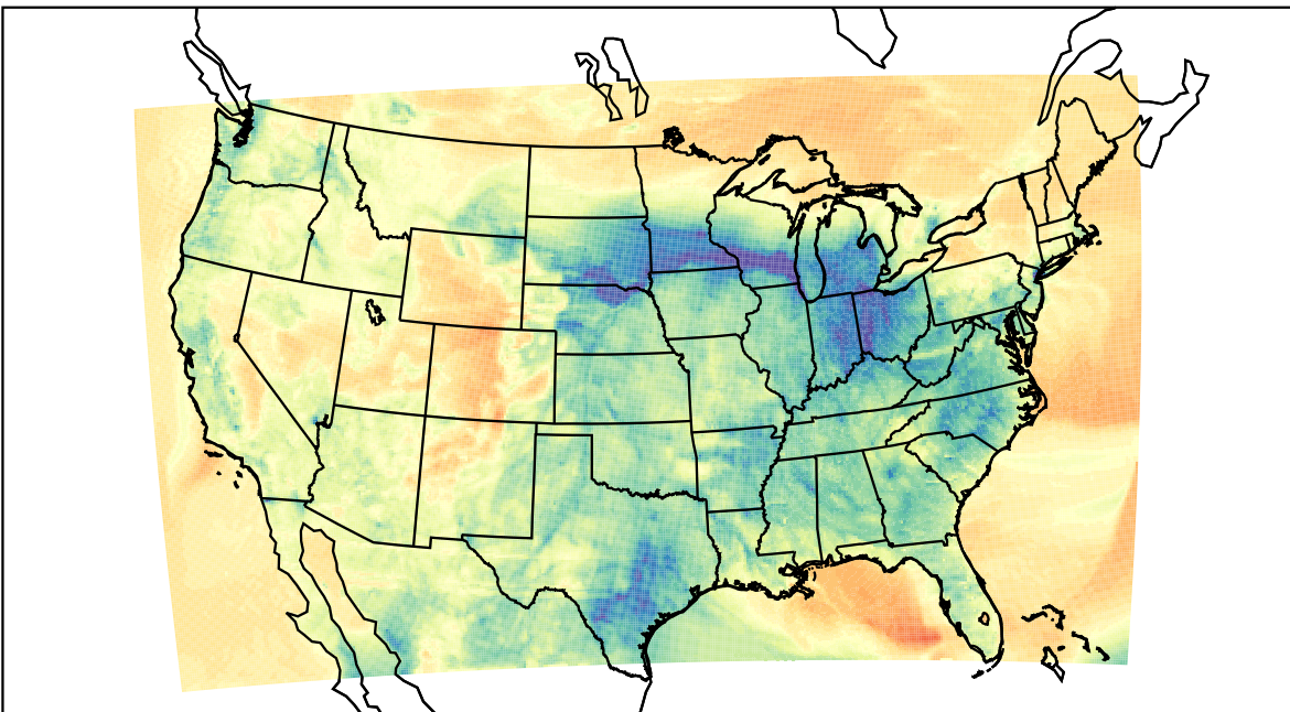
WRF (2023-03-31_03:00:00)
