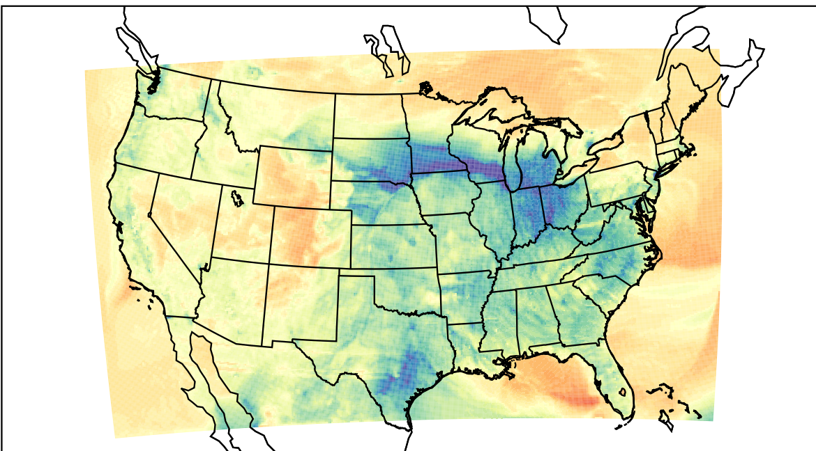
WRF (2023-03-31_02:00:00)
