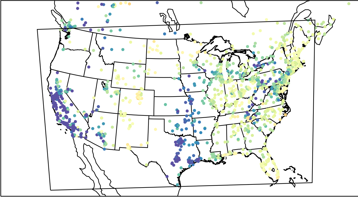
AirNOW (2023-03-31_14:00:00)
