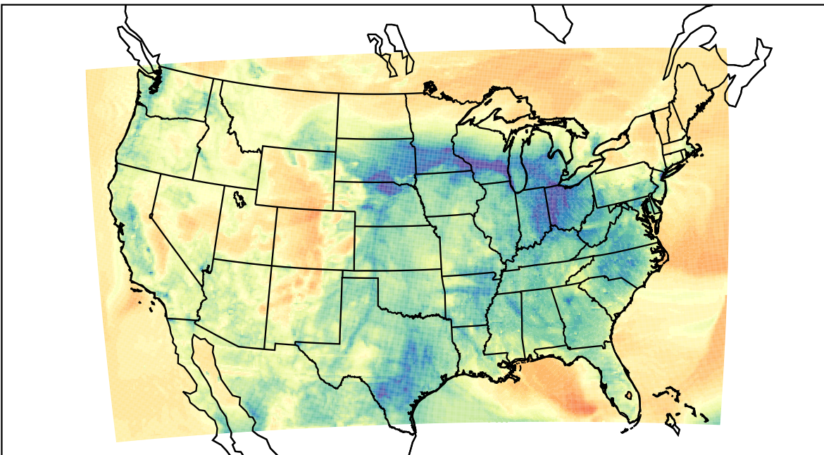
WRF (2023-03-31_04:00:00)
