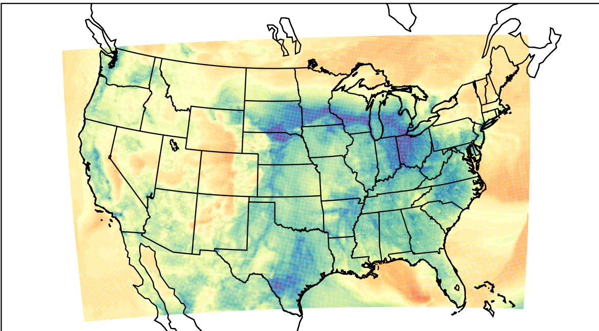
WRF (2023-03-31_05:00:00)
