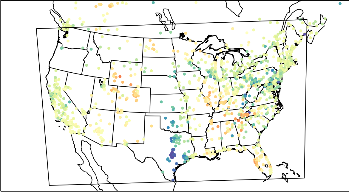
AirNOW (2023-03-31_00:00:00)
