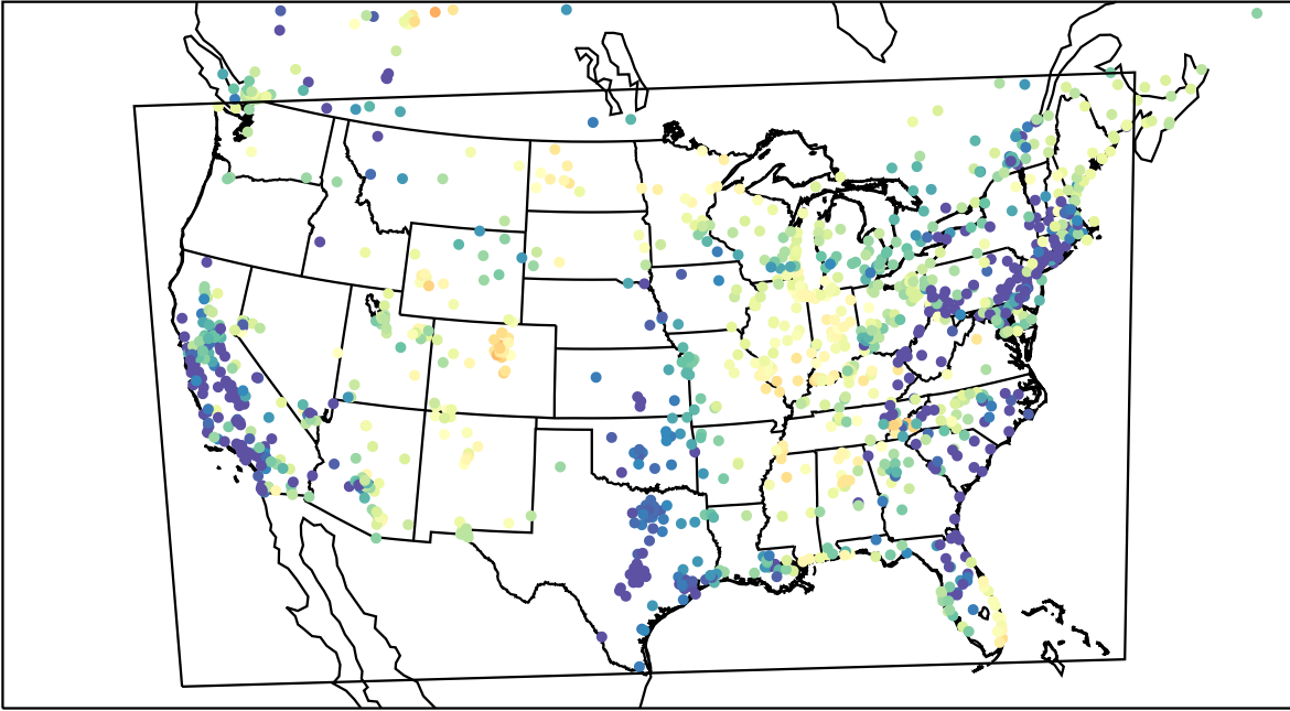
AirNOW (2023-03-31_09:00:00)
