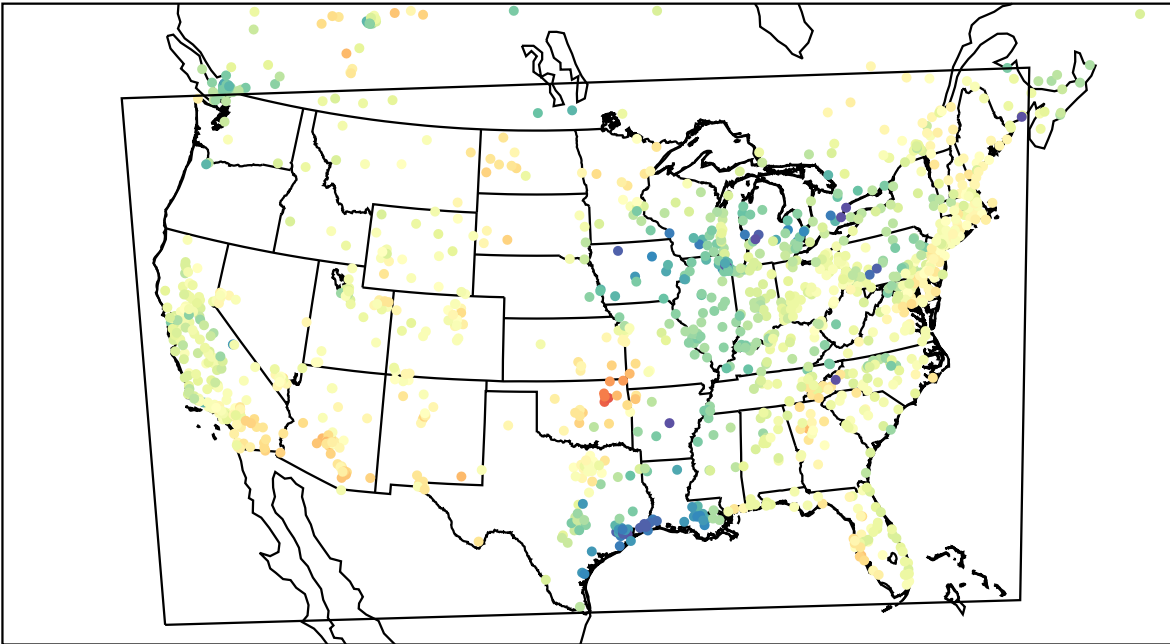
AirNOW (2023-03-31_21:00:00)
