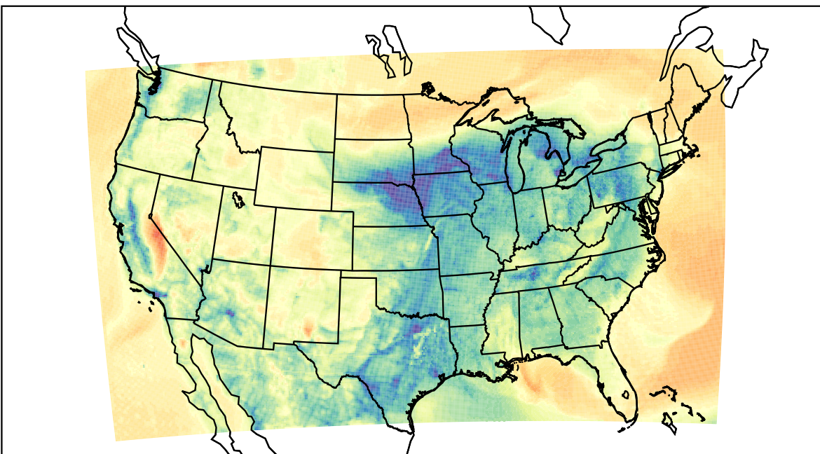
WRF (2023-03-31_14:00:00)
