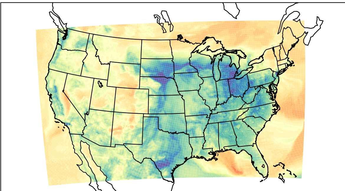
WRF (2023-03-31_07:00:00)
