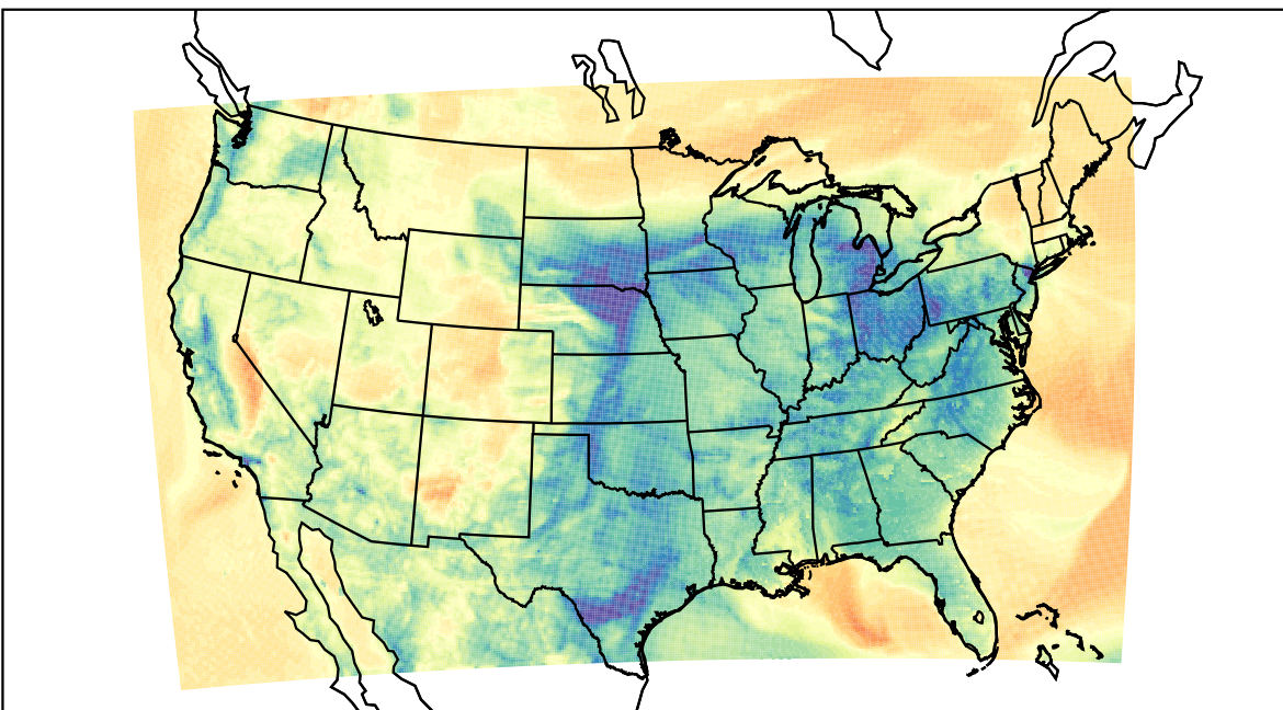
WRF (2023-03-31_09:00:00)
