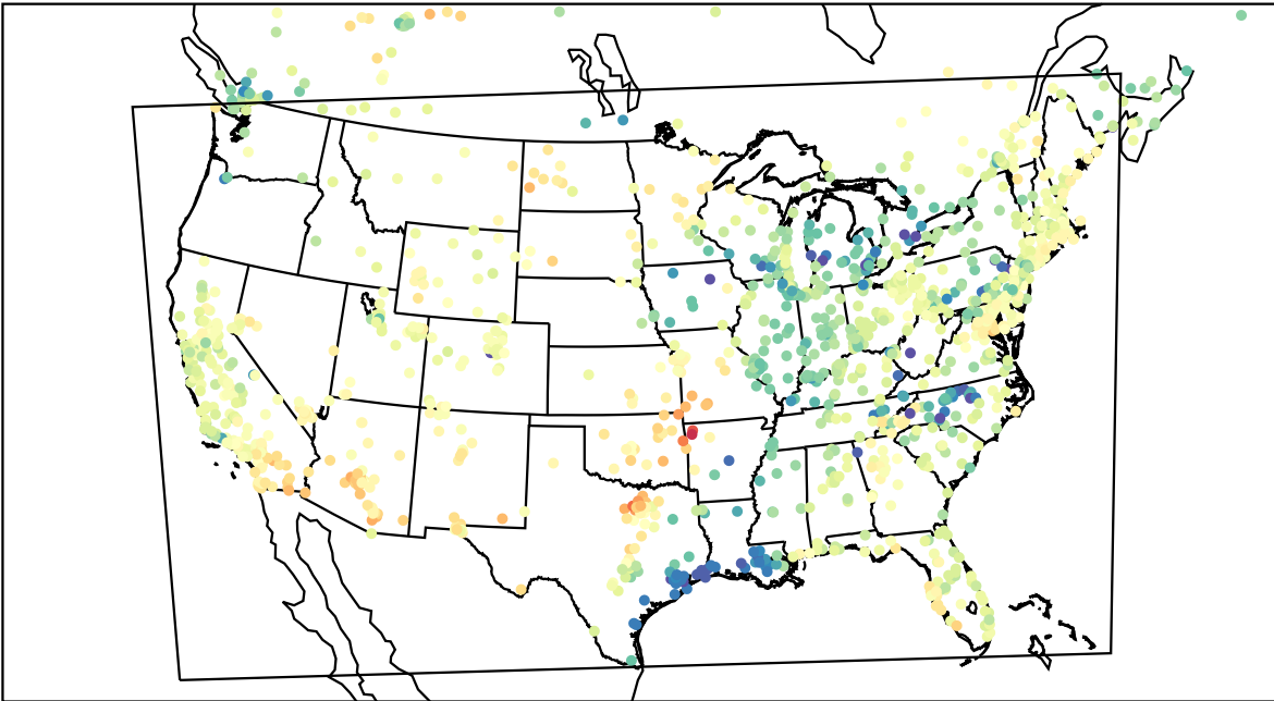
AirNOW (2023-03-31_23:00:00)
