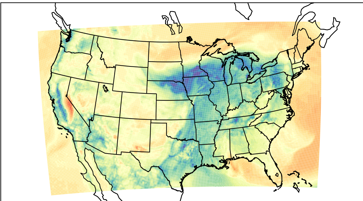
WRF (2023-03-31_15:00:00)
