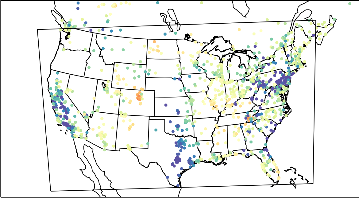
AirNOW (2023-03-31_05:00:00)
