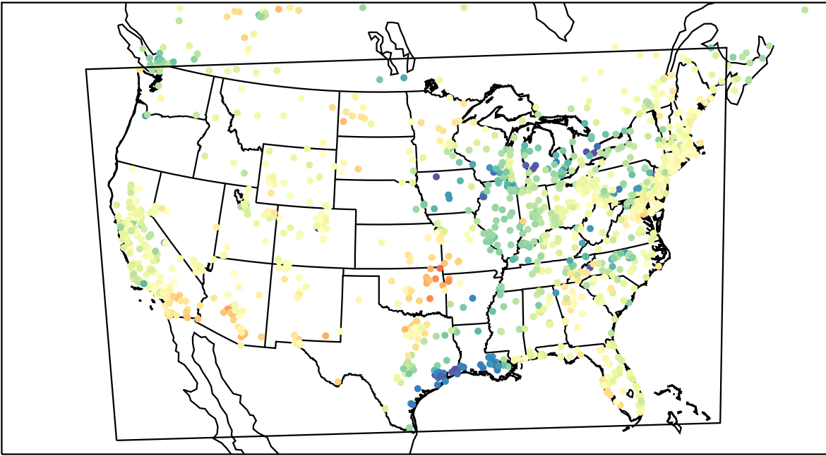
AirNOW (2023-03-31_22:00:00)
