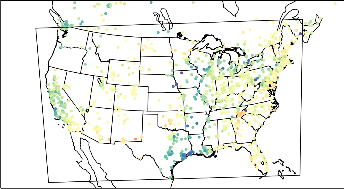
AirNOW (2023-03-31_18:00:00)
