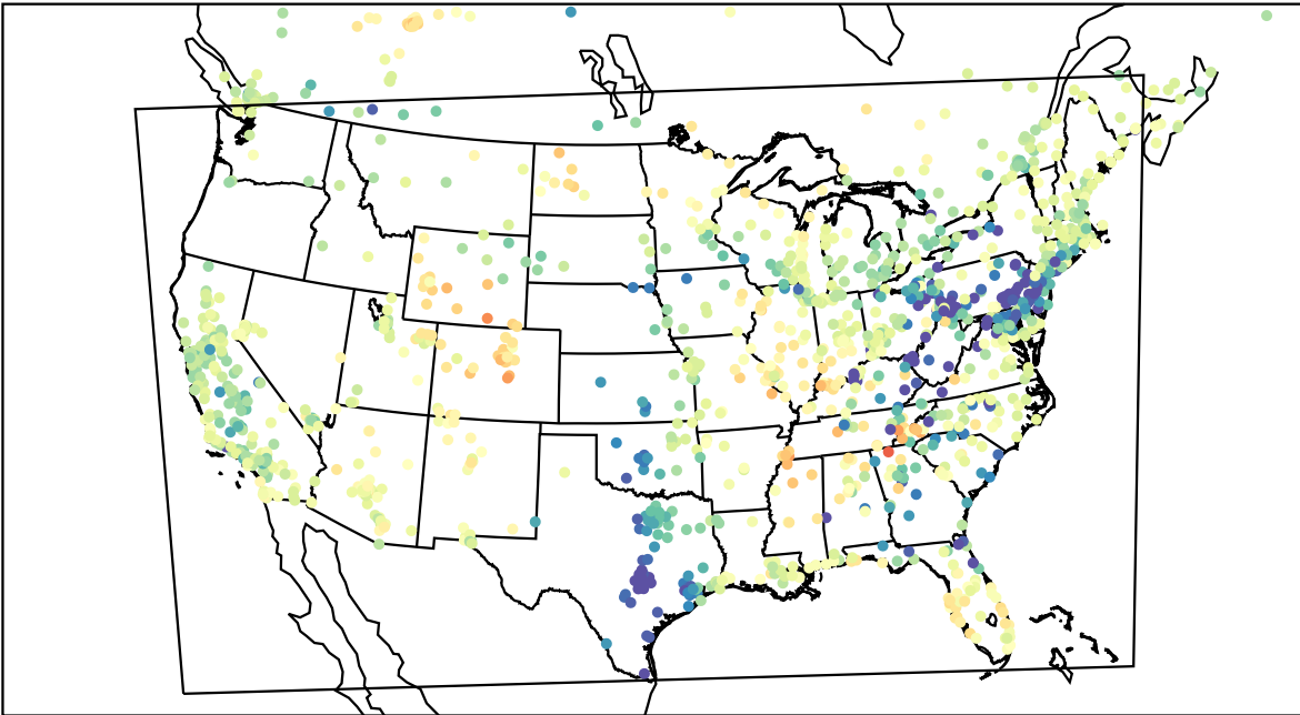
AirNOW (2023-03-31_02:00:00)
