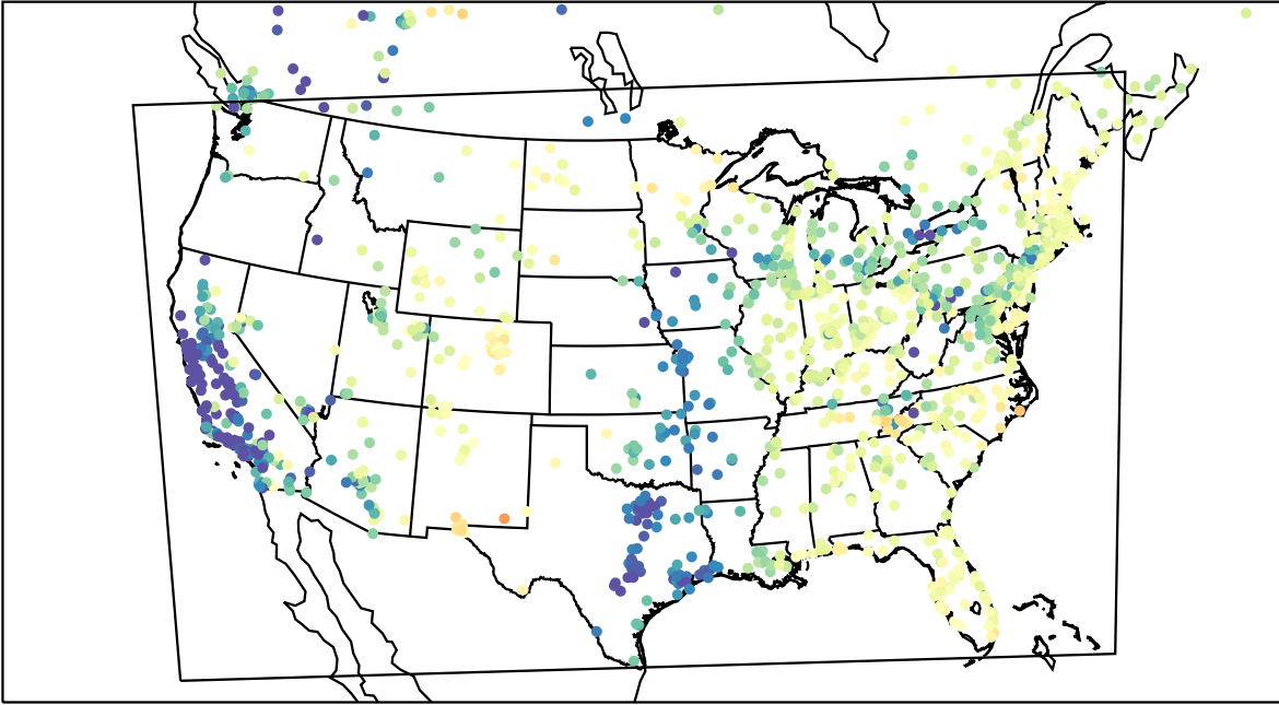
AirNOW (2023-03-31_15:00:00)
