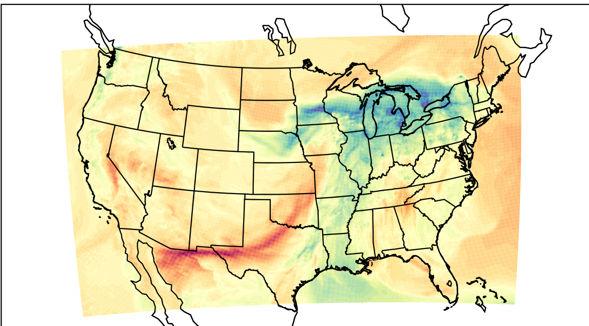
WRF (2023-03-31_20:00:00)
