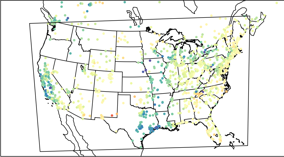
AirNOW (2023-03-31_17:00:00)
