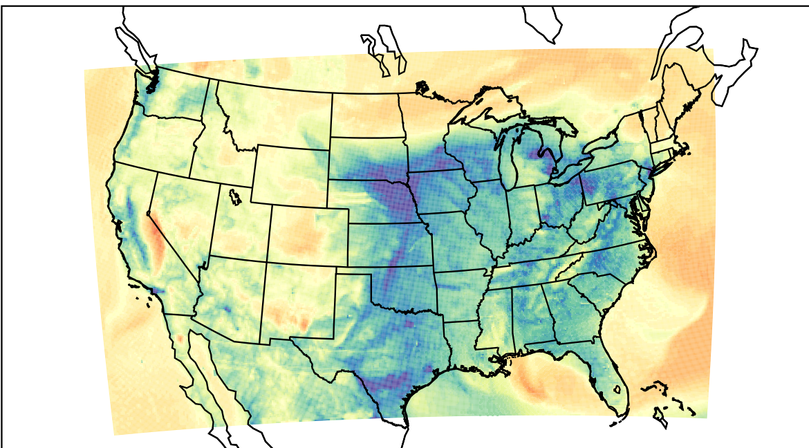
WRF (2023-03-31_12:00:00)
