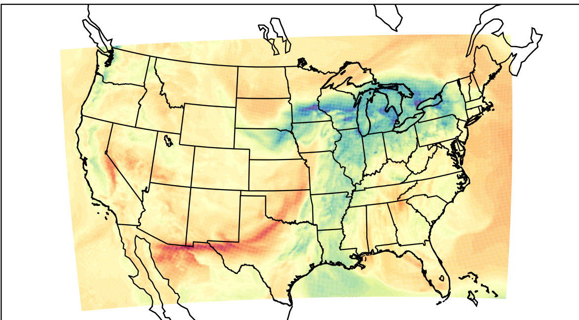
WRF (2023-03-31_19:00:00)
