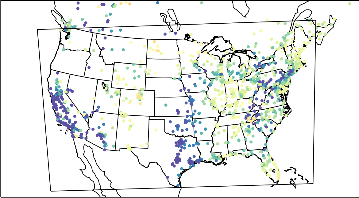
AirNOW (2023-03-31_13:00:00)
