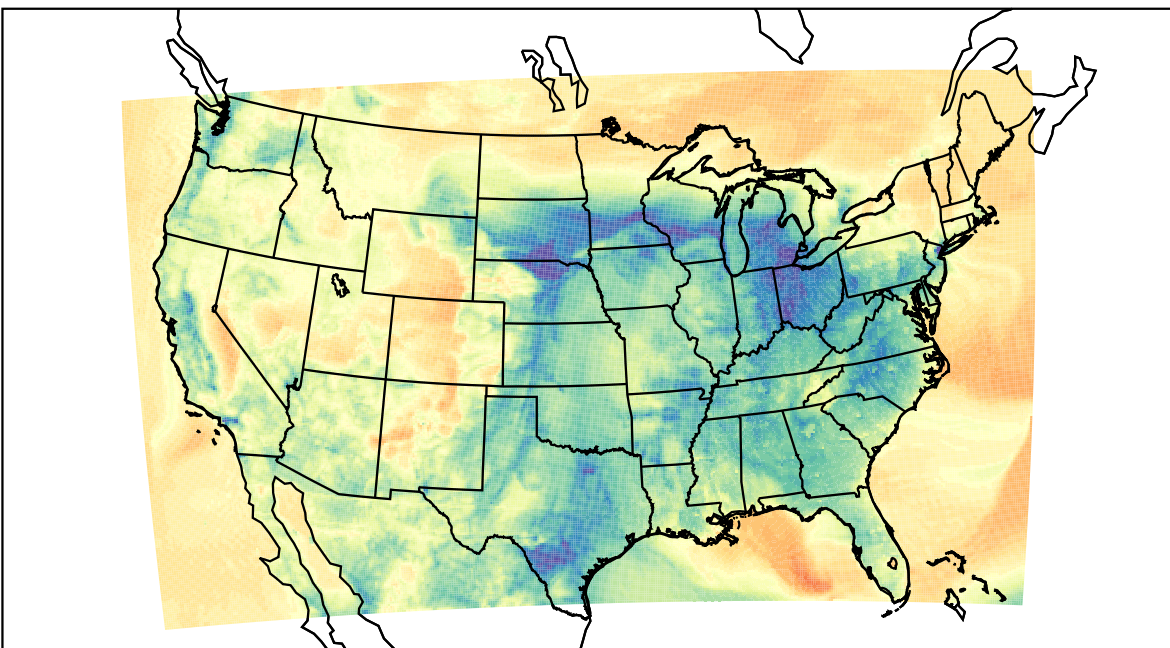
WRF (2023-03-31_06:00:00)
