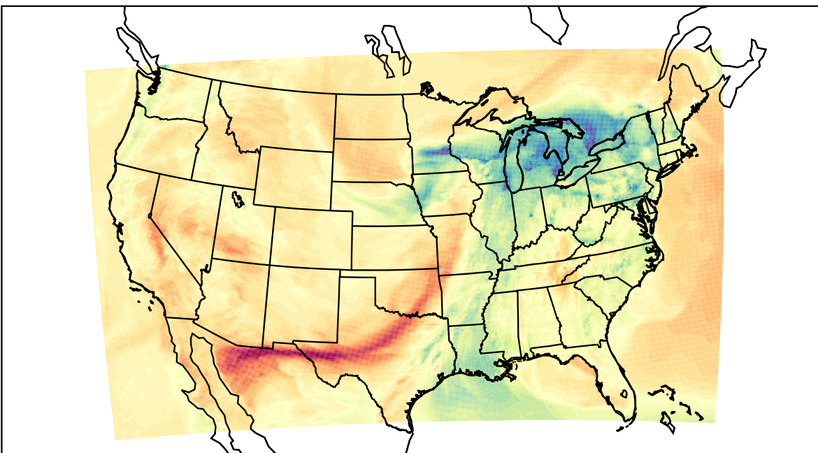
WRF (2023-03-31_22:00:00)
