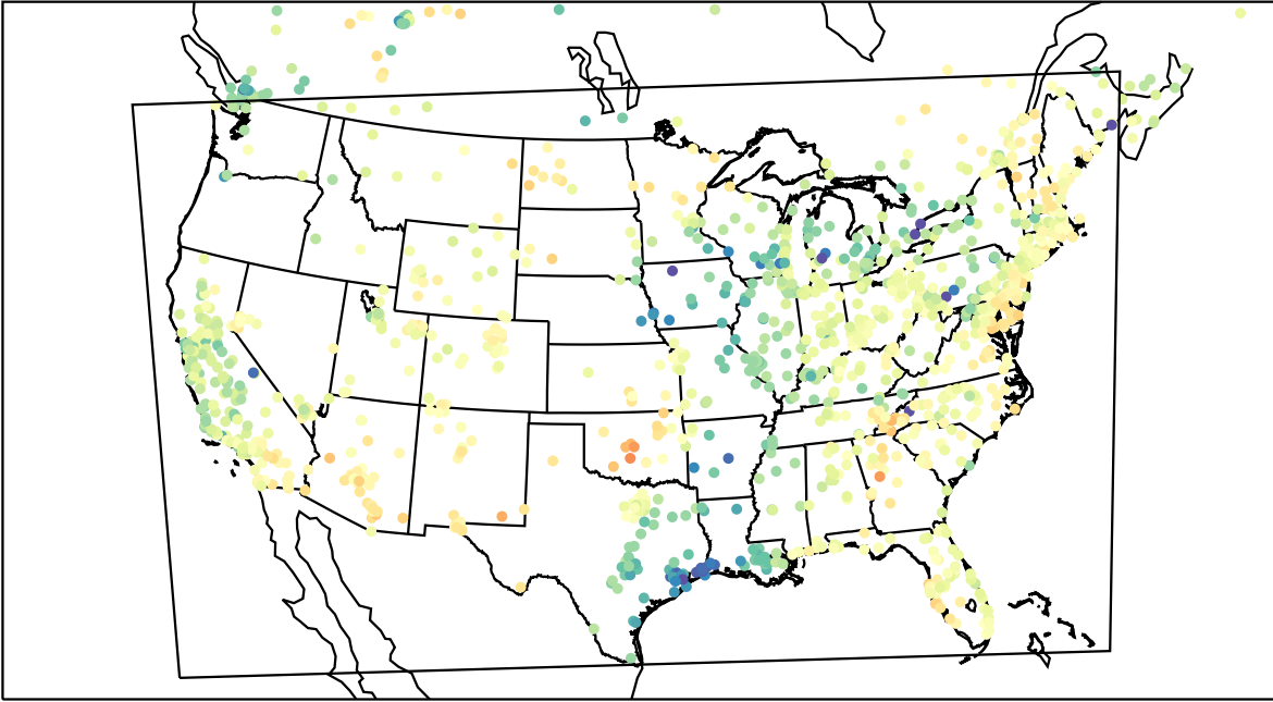
AirNOW (2023-03-31_19:00:00)
