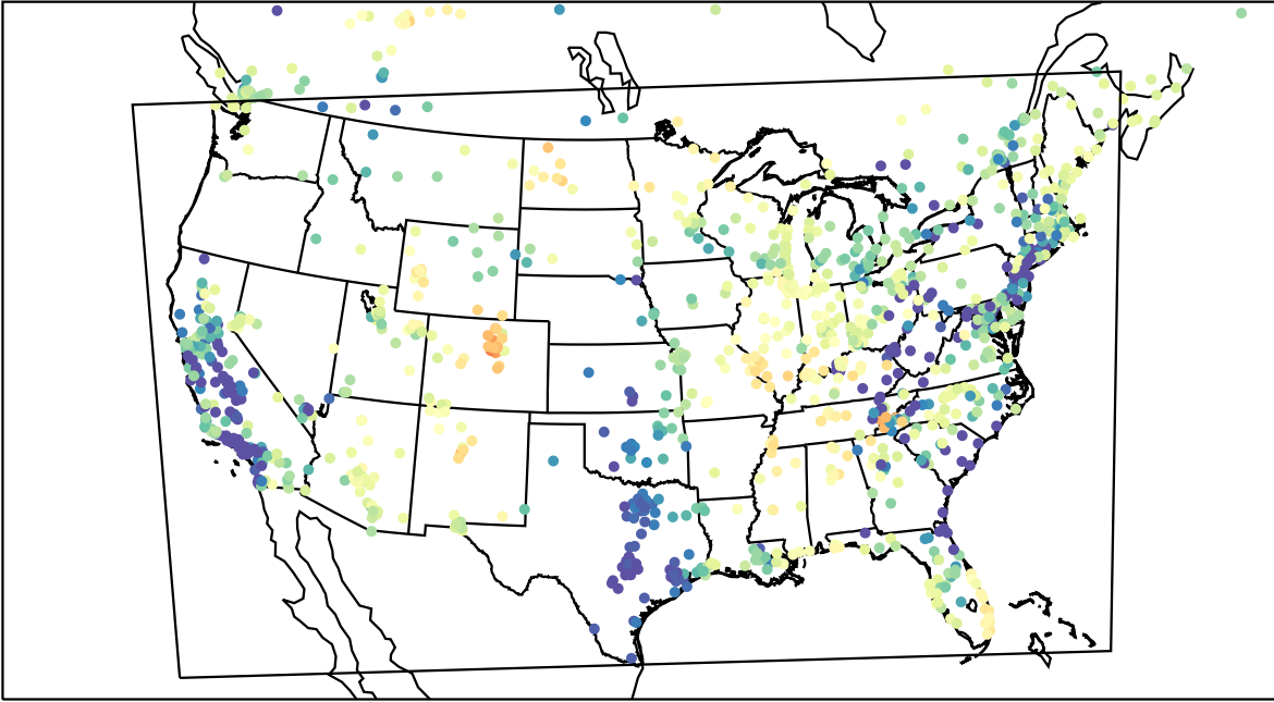
AirNOW (2023-03-31_06:00:00)
