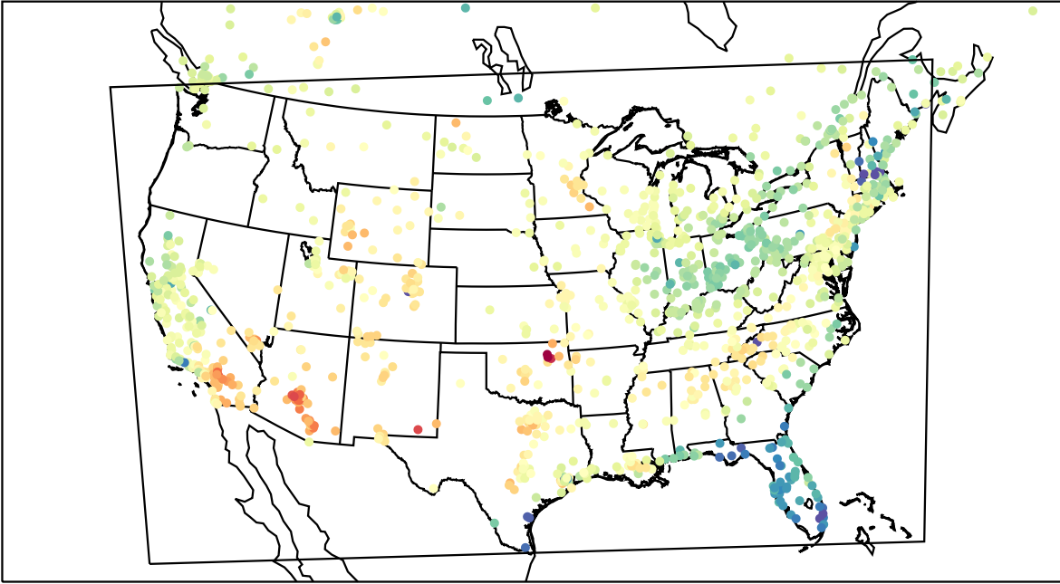
AirNOW (2023-04-01_23:00:00)
