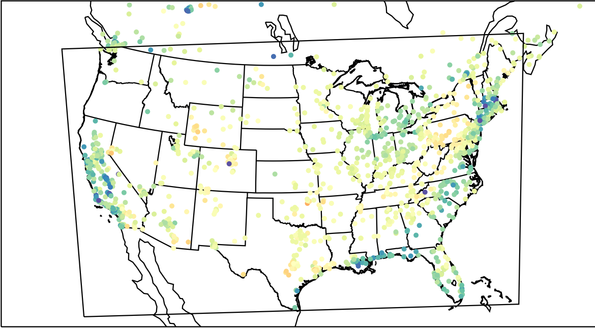
AirNOW (2023-04-01_17:00:00)
