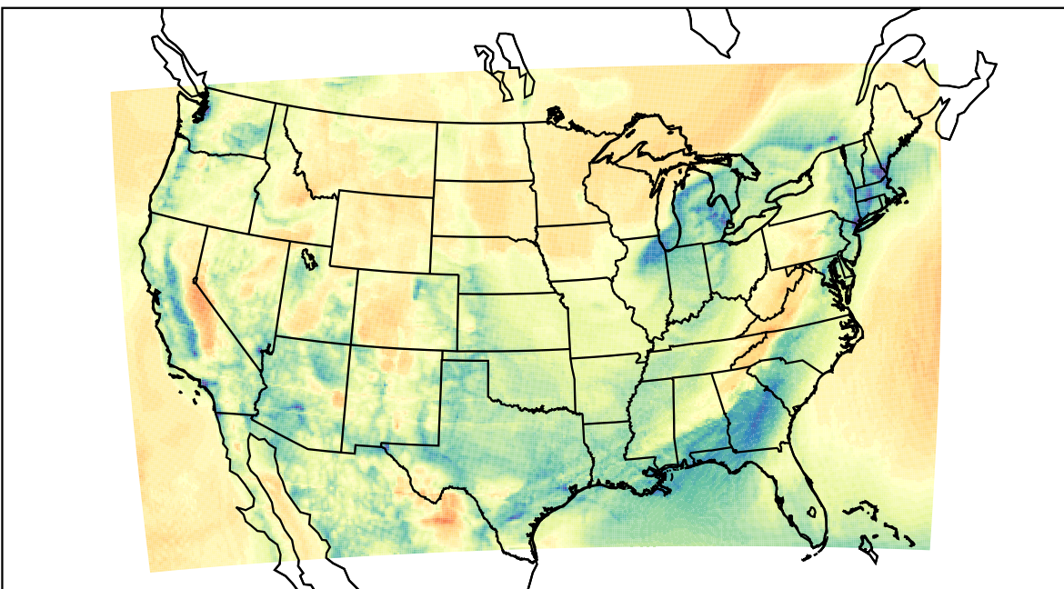
WRF (2023-04-01_15:00:00)
