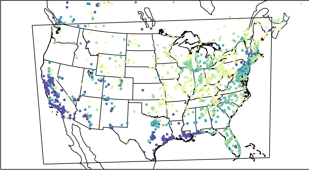
AirNOW (2023-04-01_13:00:00)
