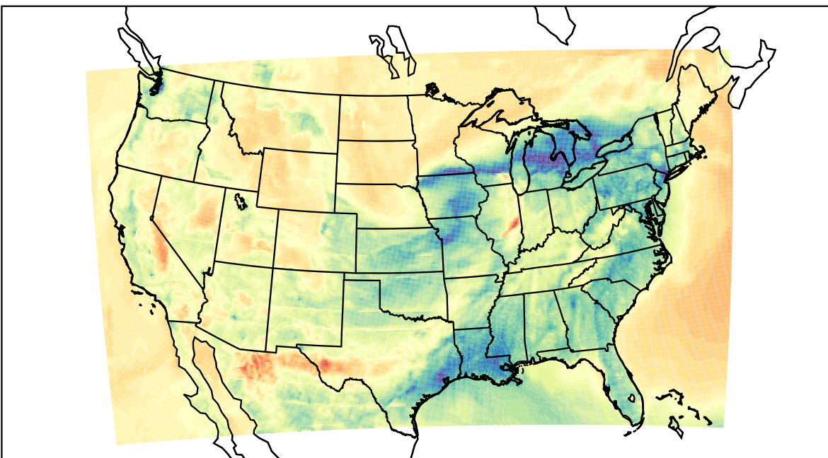
WRF (2023-04-01_03:00:00)
