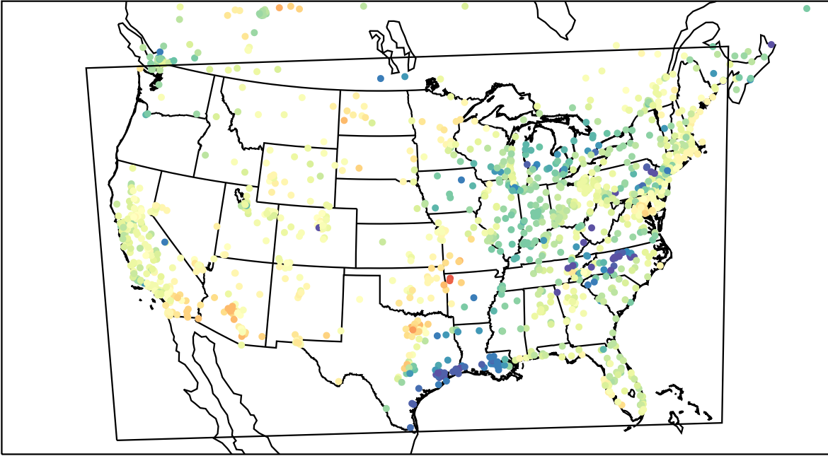
AirNOW (2023-04-01_00:00:00)
