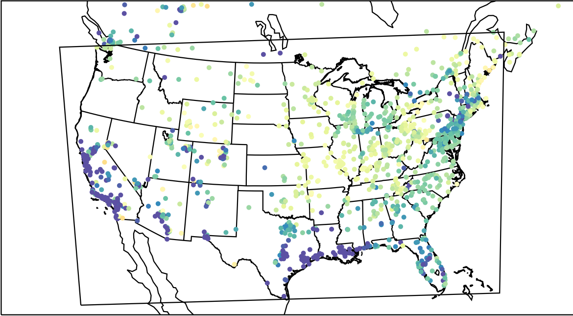
AirNOW (2023-04-01_12:00:00)
