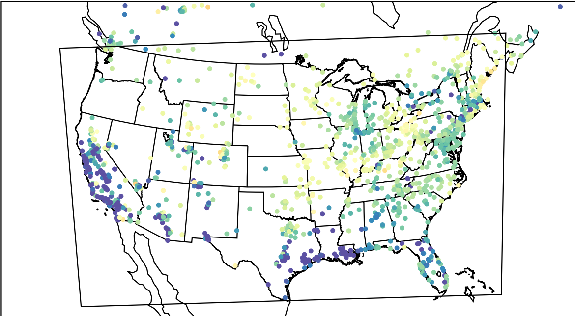
AirNOW (2023-04-01_09:00:00)
