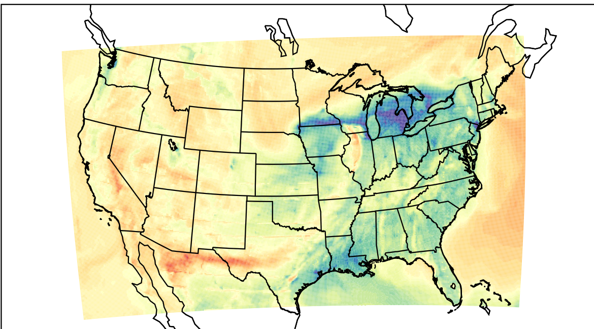
WRF (2023-04-01_01:00:00)
