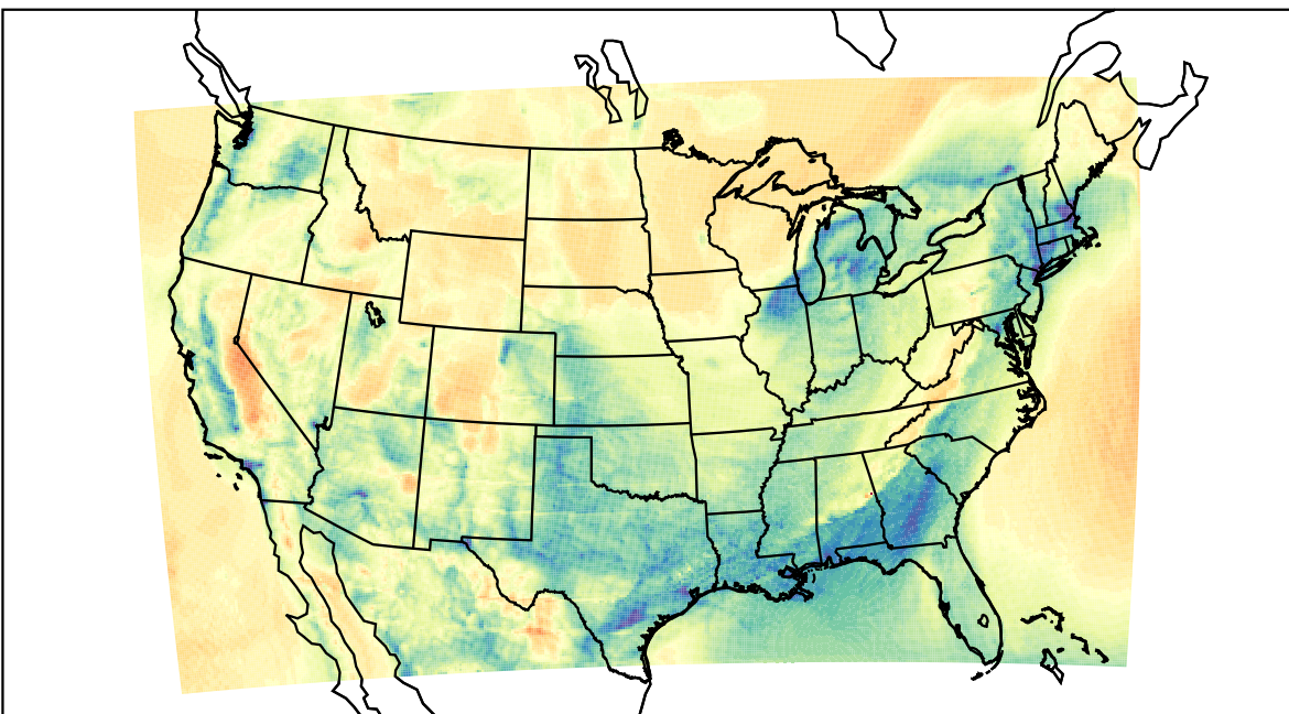
WRF (2023-04-01_14:00:00)
