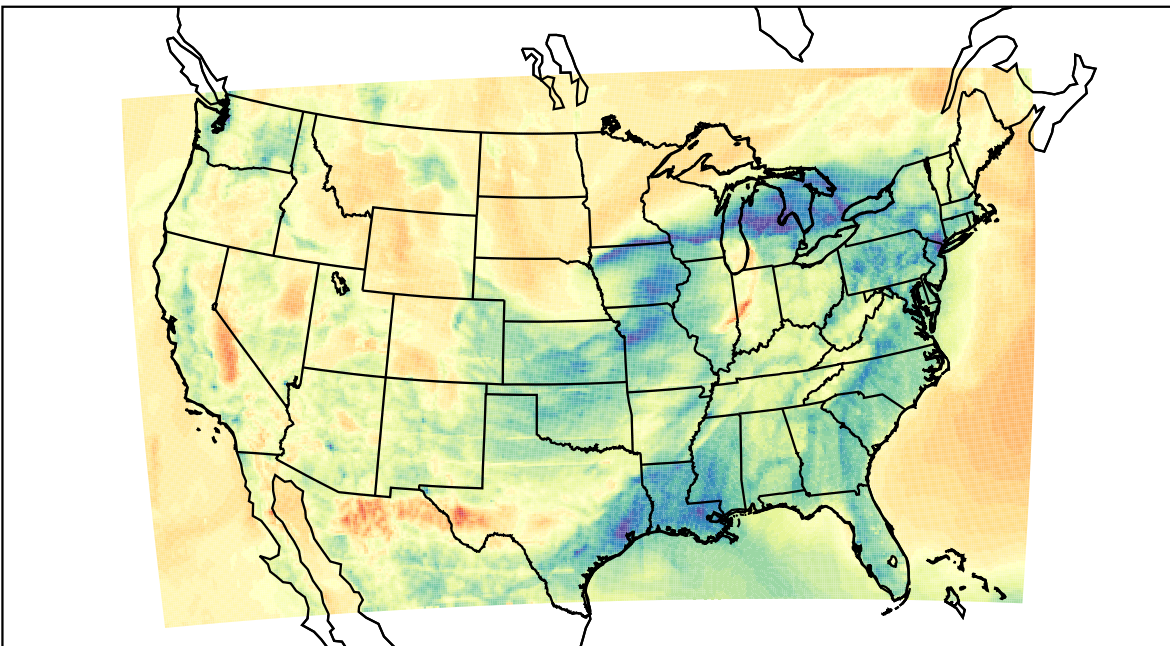
WRF (2023-04-01_04:00:00)
