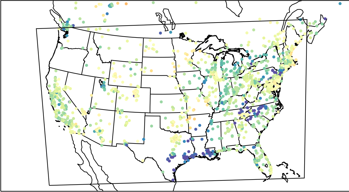
AirNOW (2023-04-01_02:00:00)
