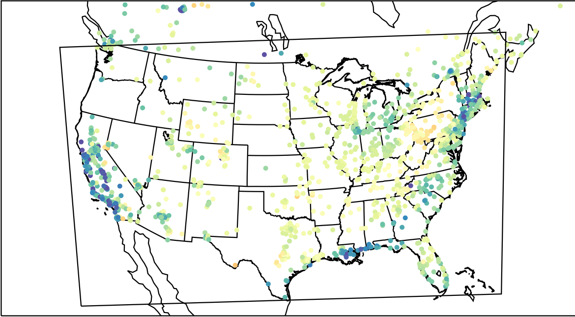
AirNOW (2023-04-01_16:00:00)
