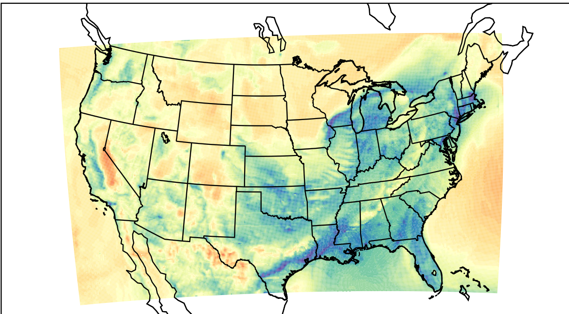
WRF (2023-04-01_11:00:00)
