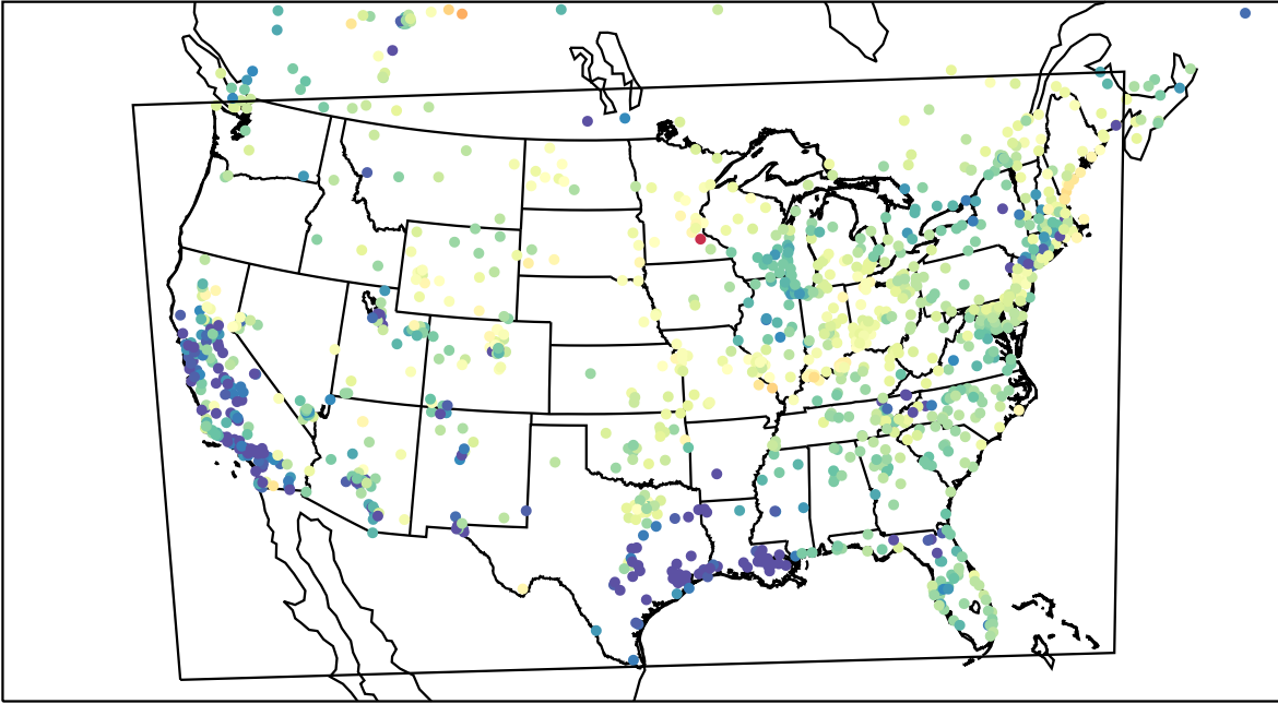
AirNOW (2023-04-01_06:00:00)
