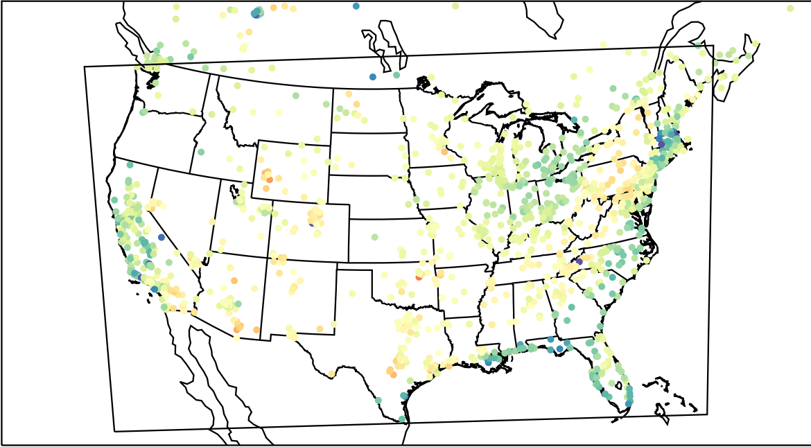
AirNOW (2023-04-01_18:00:00)
