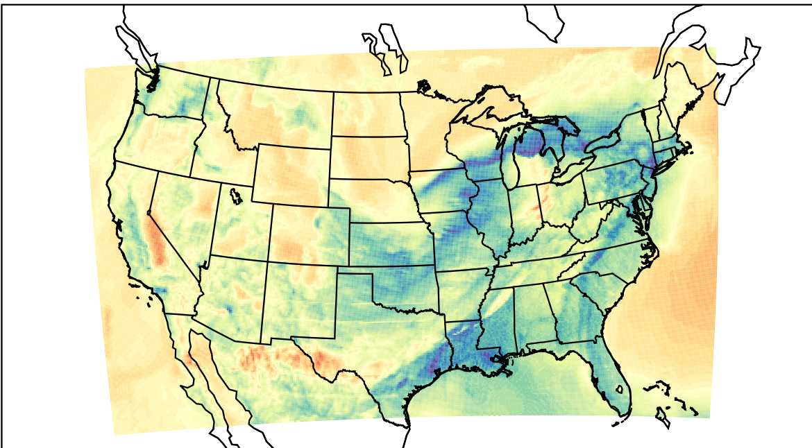
WRF (2023-04-01_06:00:00)
