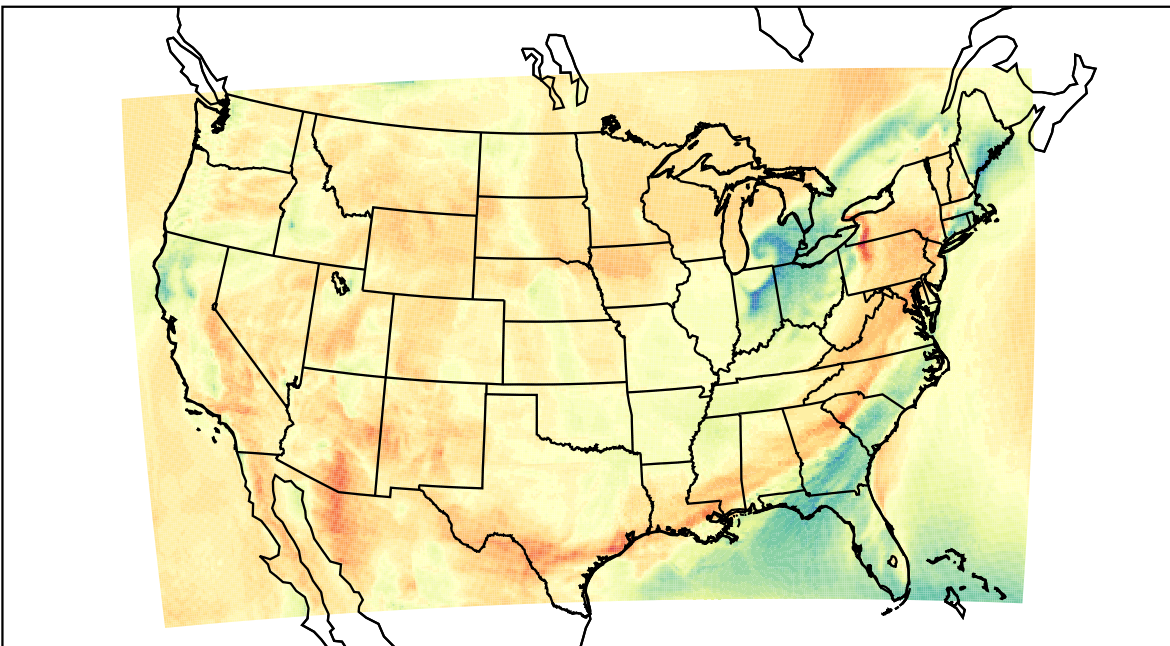
WRF (2023-04-01_19:00:00)
