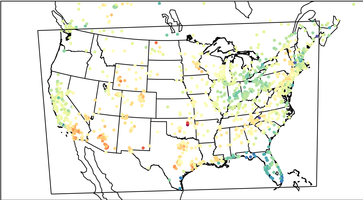
AirNOW (2023-04-01_21:00:00)
