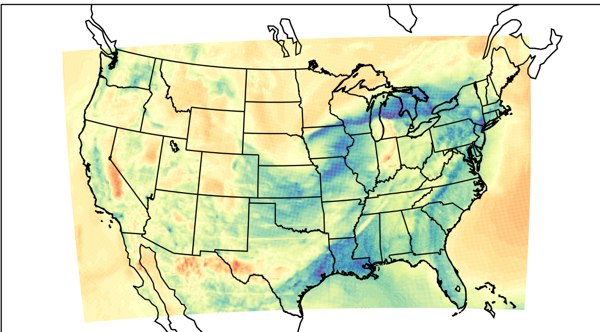
WRF (2023-04-01_05:00:00)
