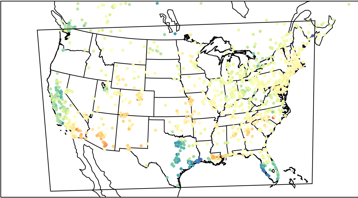
AirNOW (2023-04-02_19:00:00)
