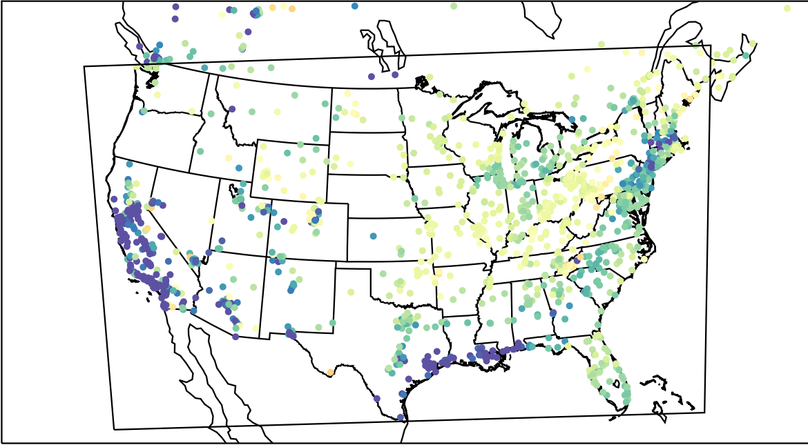
AirNOW (2023-04-01_14:00:00)
