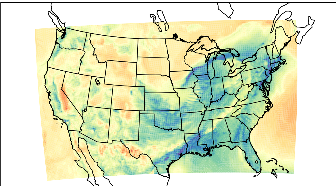
WRF (2023-04-01_09:00:00)
