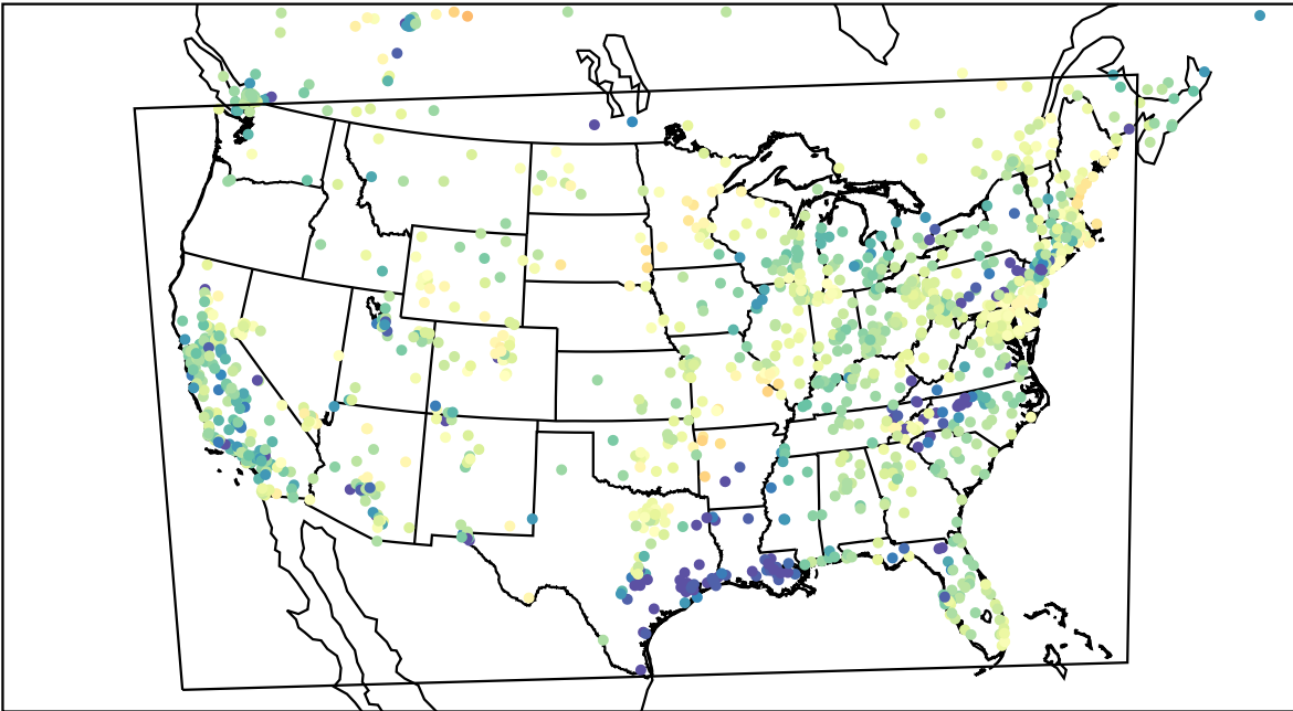
AirNOW (2023-04-01_03:00:00)
