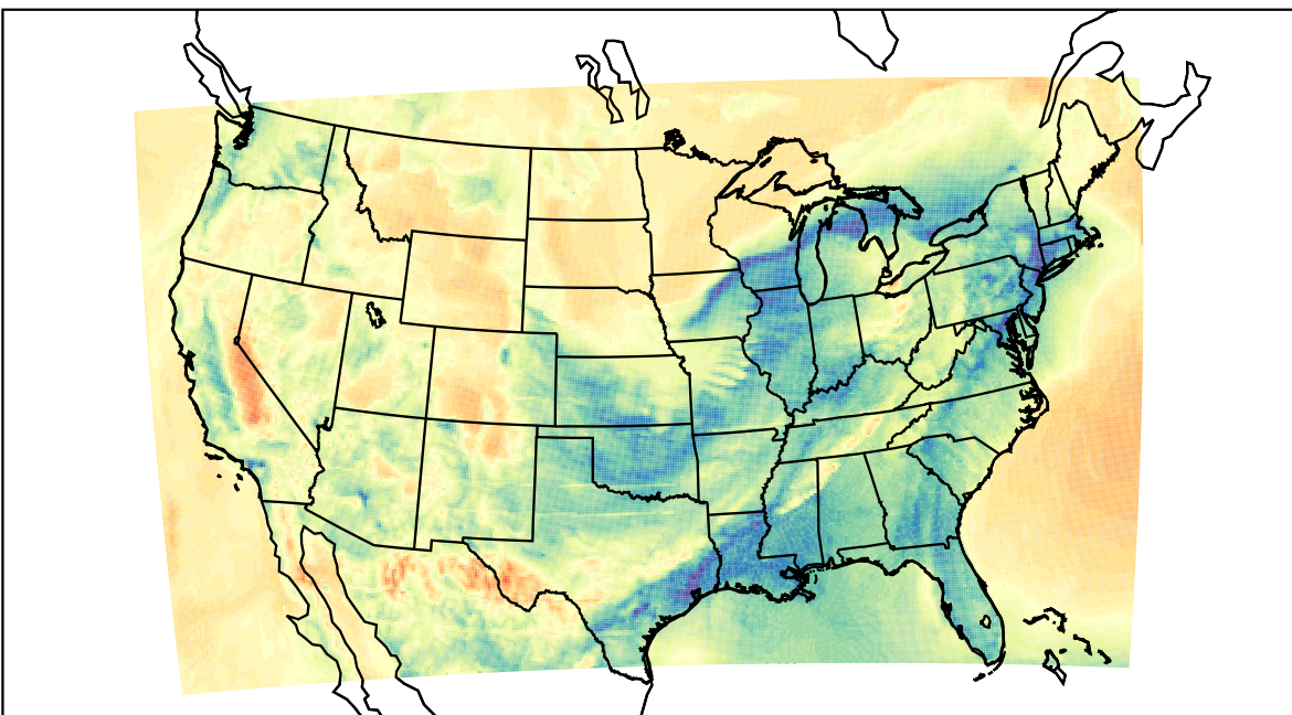
WRF (2023-04-01_08:00:00)
