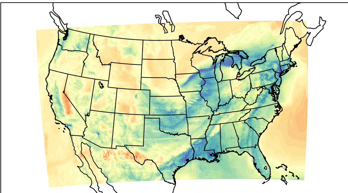
WRF (2023-04-01_07:00:00)
