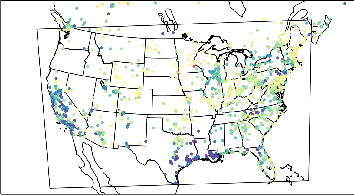
AirNOW (2023-04-01_05:00:00)
