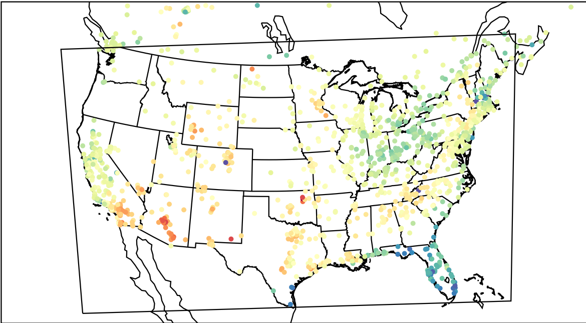
AirNOW (2023-04-01_22:00:00)
