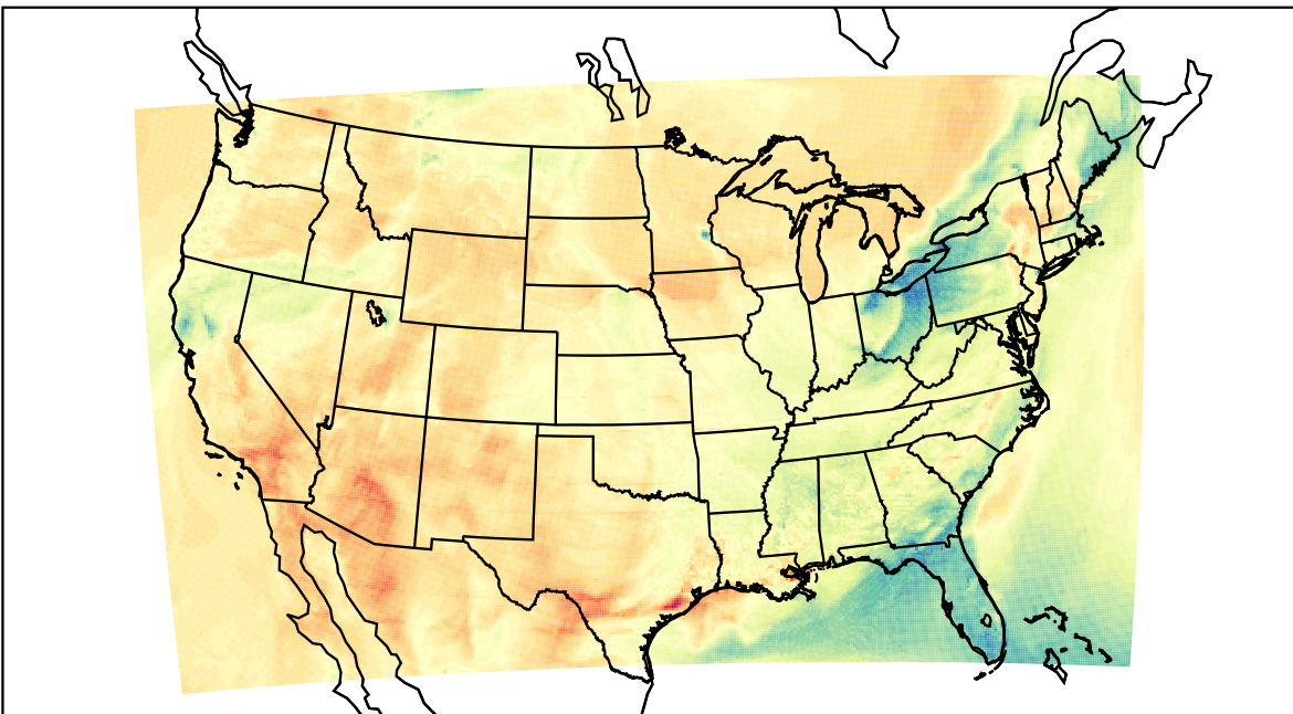
WRF (2023-04-01_23:00:00)
