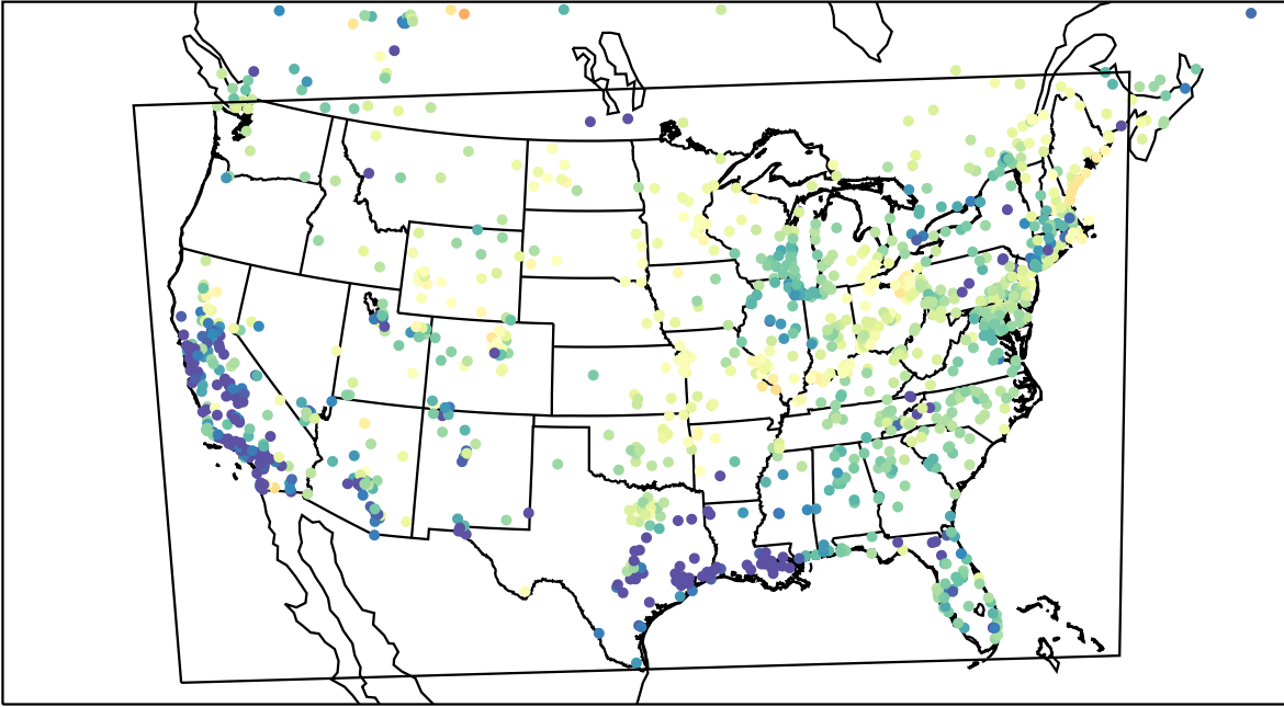
AirNOW (2023-04-01_07:00:00)
