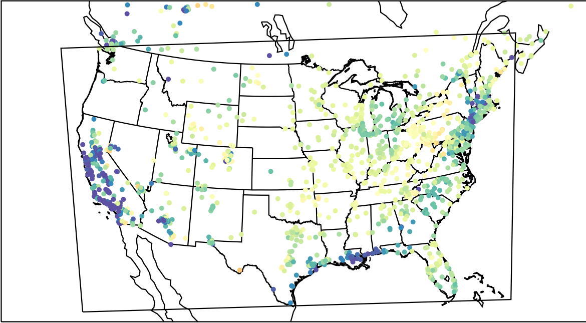
AirNOW (2023-04-01_15:00:00)
