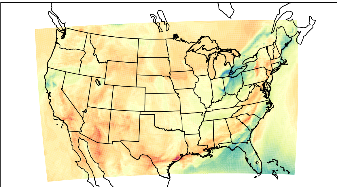
WRF (2023-04-01_21:00:00)
