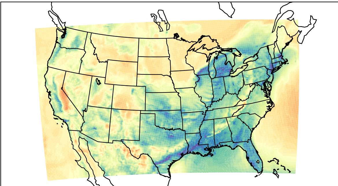
WRF (2023-04-01_12:00:00)
