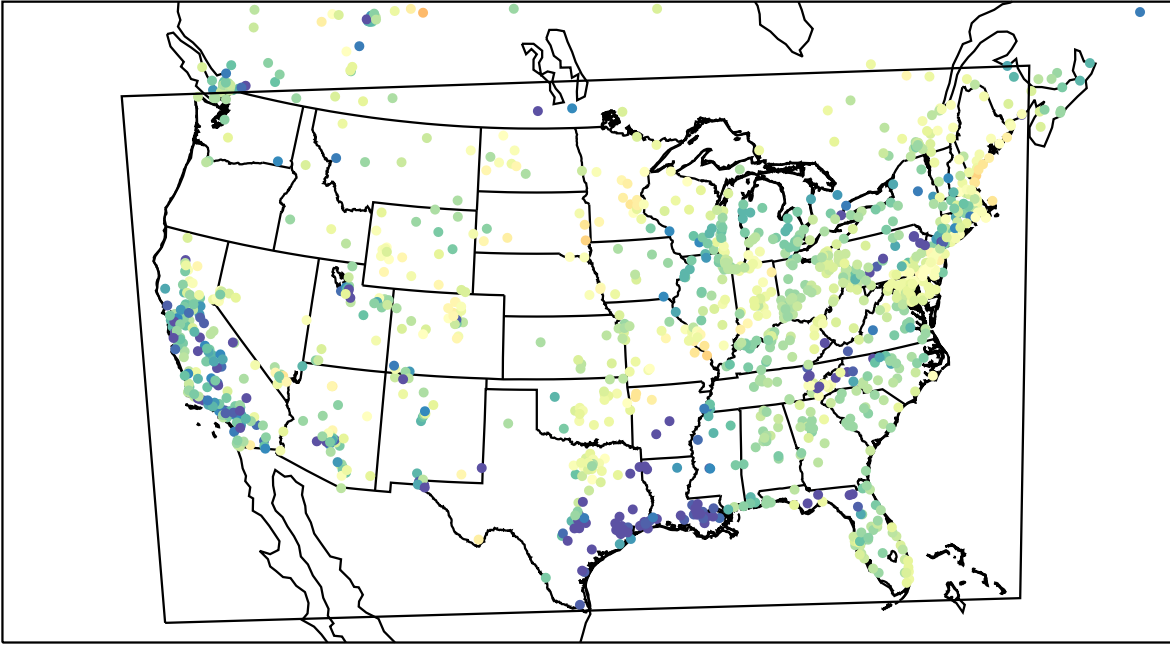
AirNOW (2023-04-01_04:00:00)
