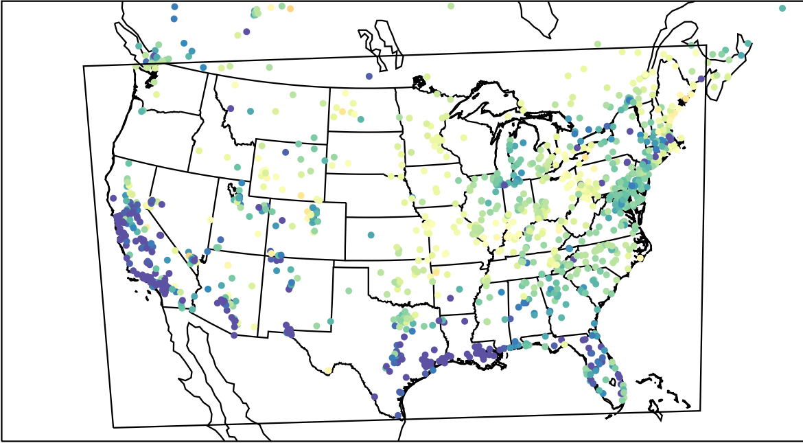
AirNOW (2023-04-01_10:00:00)
