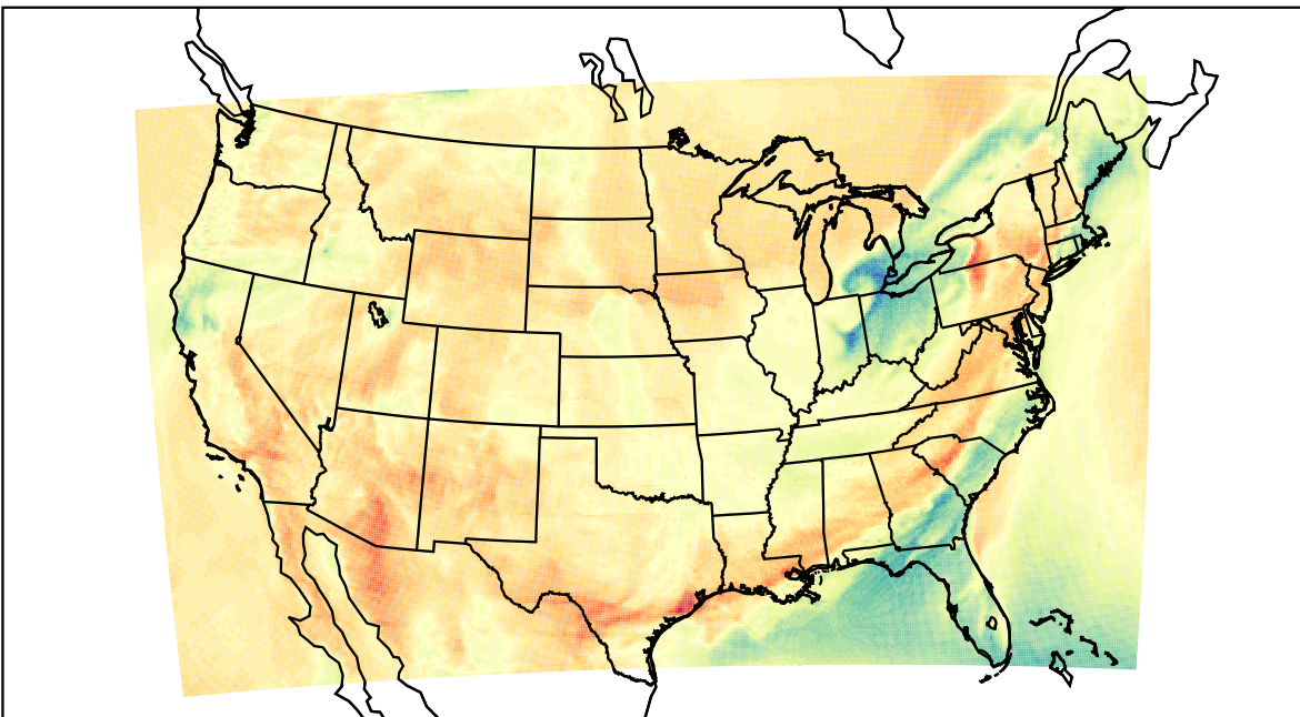
WRF (2023-04-01_20:00:00)
