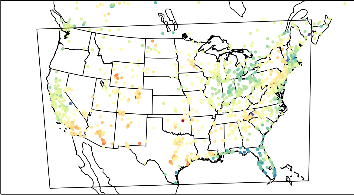
AirNOW (2023-04-01_20:00:00)
