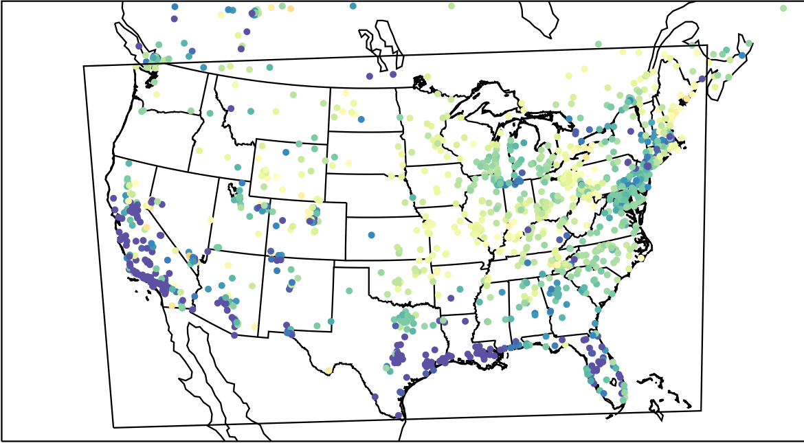
AirNOW (2023-04-01_11:00:00)
