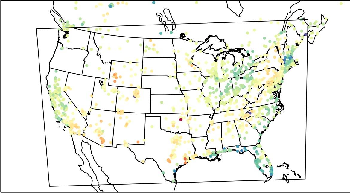
AirNOW (2023-04-01_19:00:00)
