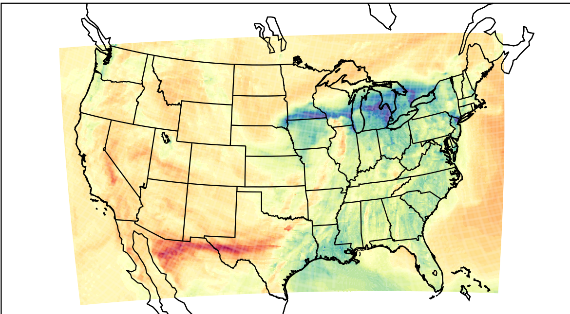
WRF (2023-04-01_00:00:00)
