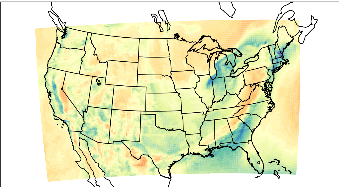
WRF (2023-04-01_16:00:00)
