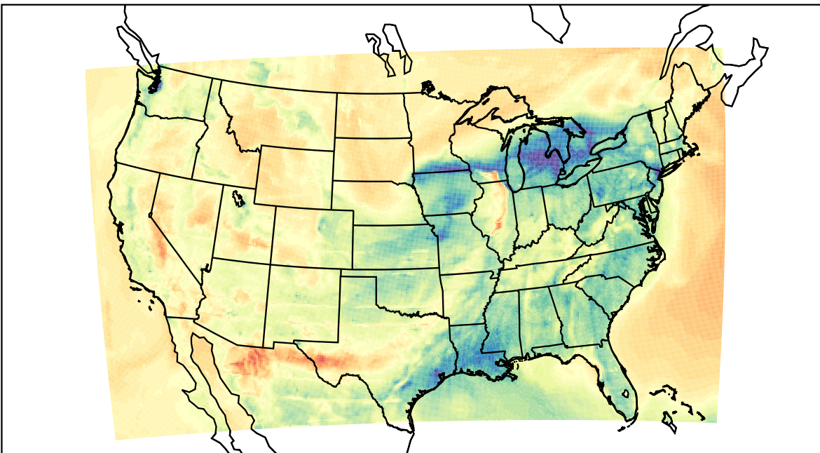
WRF (2023-04-01_02:00:00)
