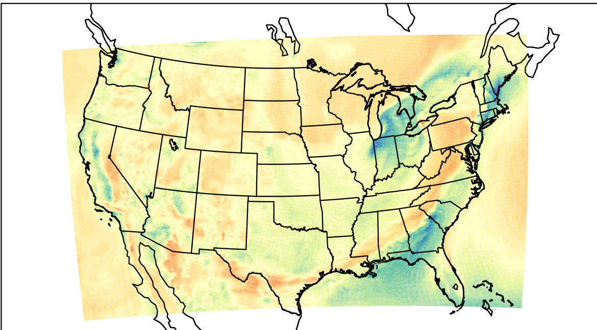
WRF (2023-04-01_17:00:00)
