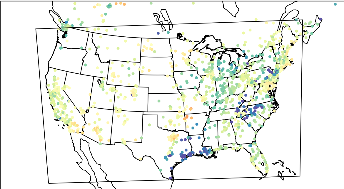
AirNOW (2023-04-01_01:00:00)
