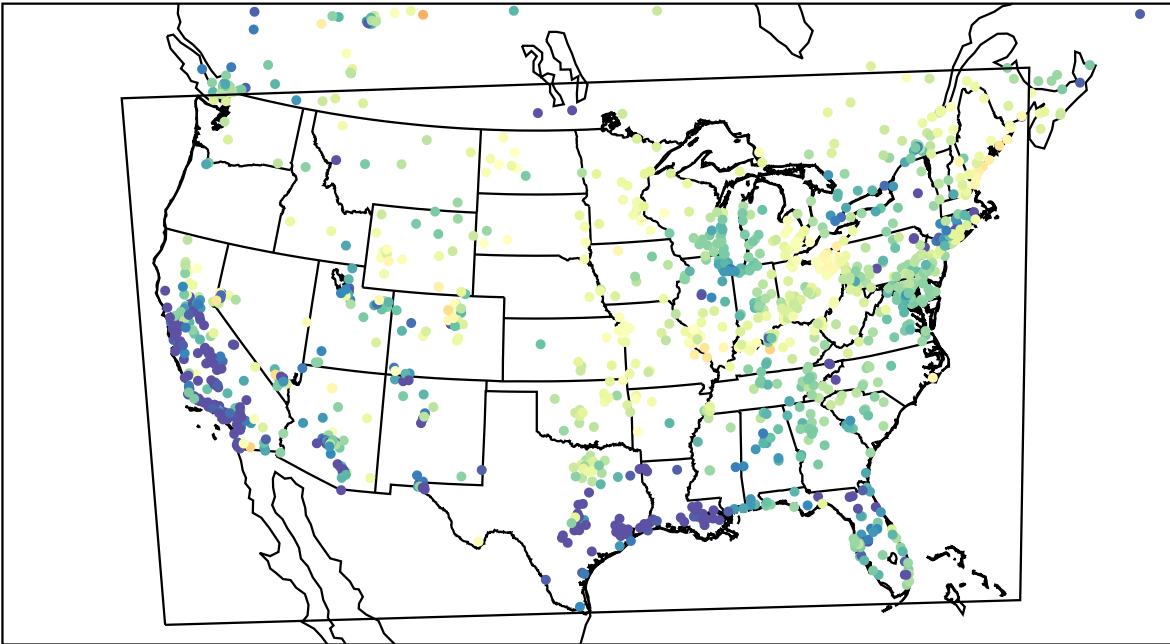
AirNOW (2023-04-01_08:00:00)
