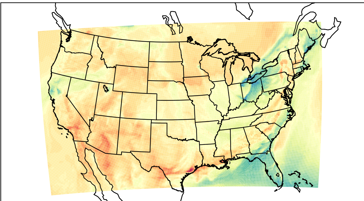
WRF (2023-04-01_22:00:00)
