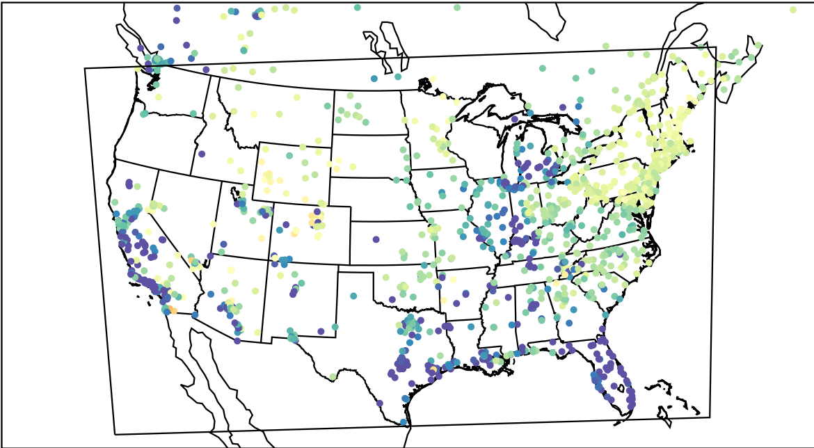
AirNOW (2023-04-02_12:00:00)
