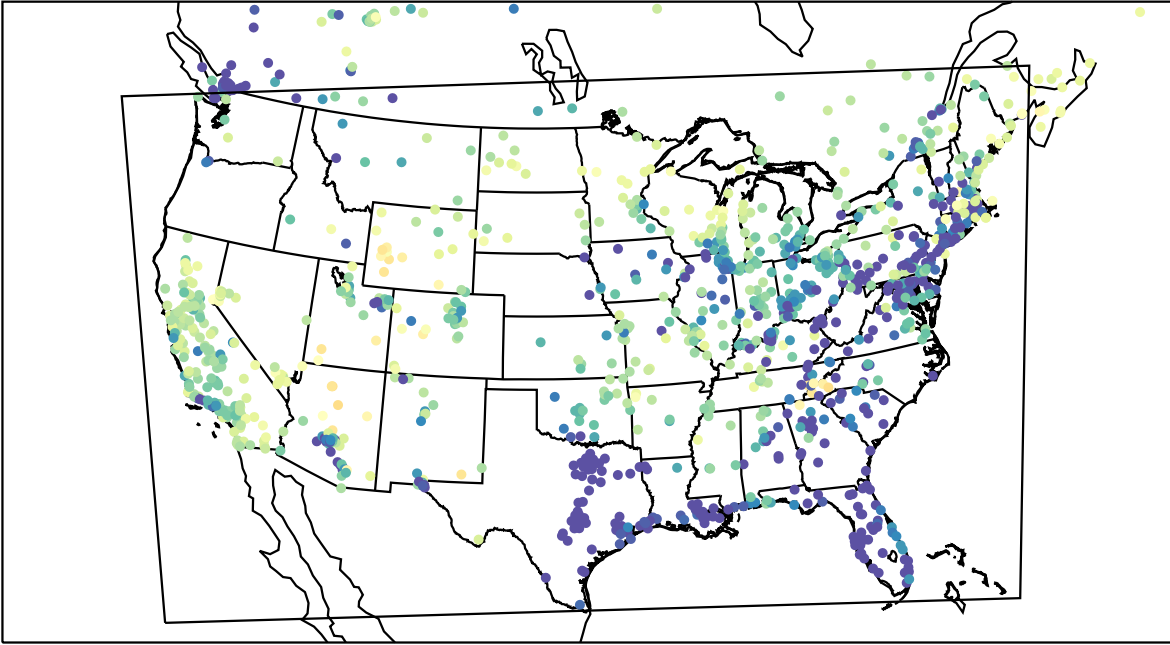
AirNOW (2023-04-03_08:00:00)
