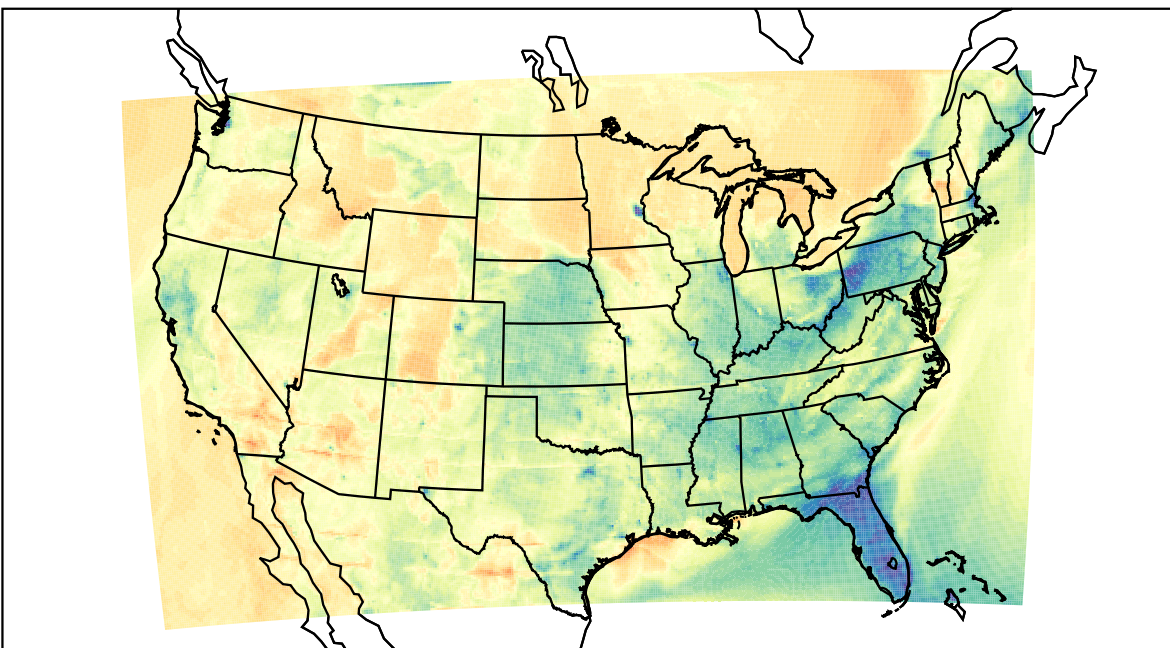
WRF (2023-04-02_02:00:00)
