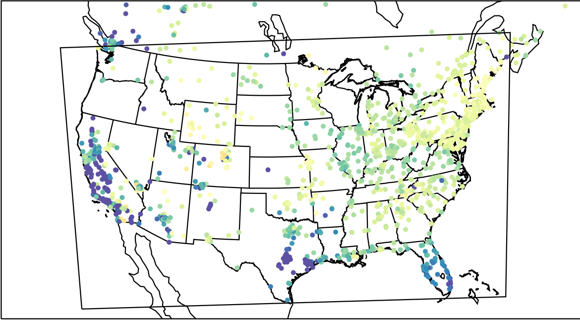
AirNOW (2023-04-02_14:00:00)
