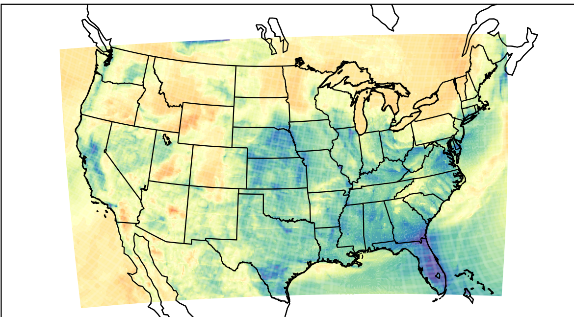
WRF (2023-04-02_08:00:00)
