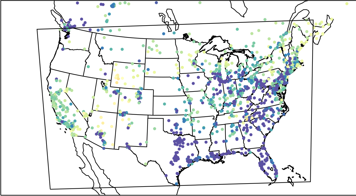
AirNOW (2023-04-03_12:00:00)
