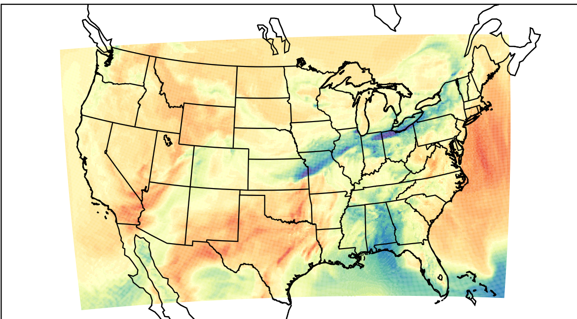
WRF (2023-04-03_22:00:00)
