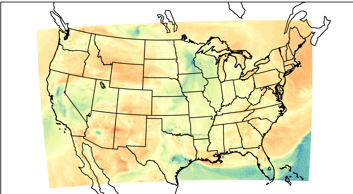
WRF (2023-04-02_18:00:00)
