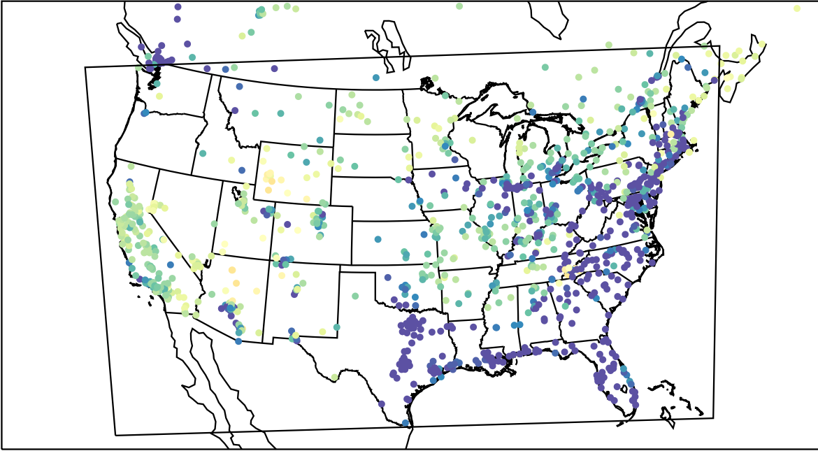
AirNOW (2023-04-03_10:00:00)
