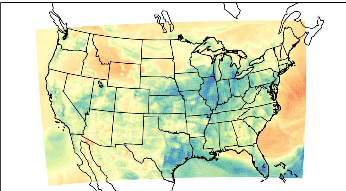
WRF (2023-04-03_04:00:00)
