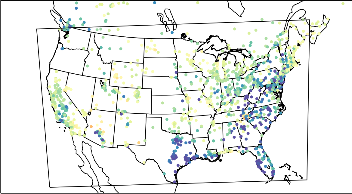
AirNOW (2023-04-03_03:00:00)
