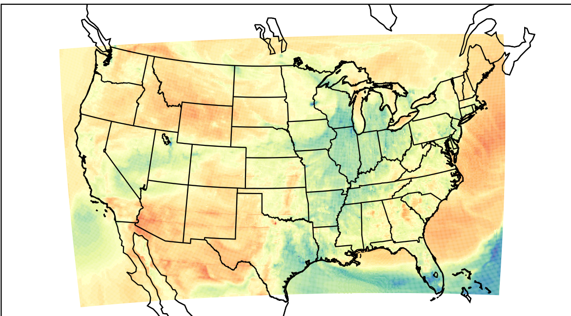
WRF (2023-04-03_00:00:00)
