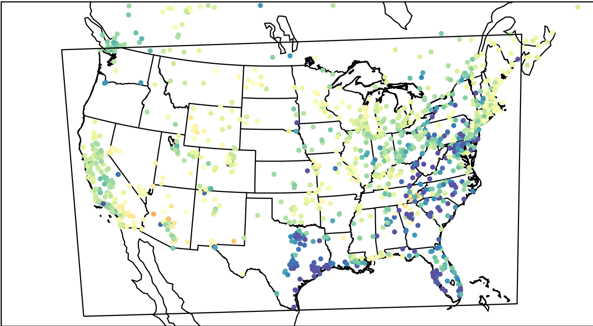
AirNOW (2023-04-03_02:00:00)
