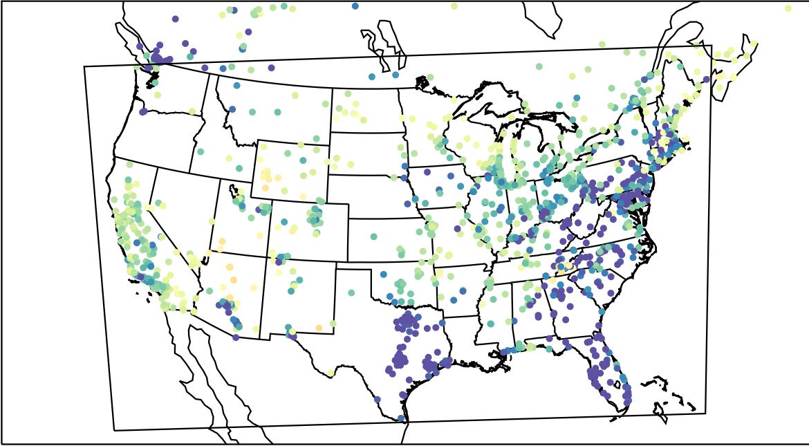
AirNOW (2023-04-03_07:00:00)
