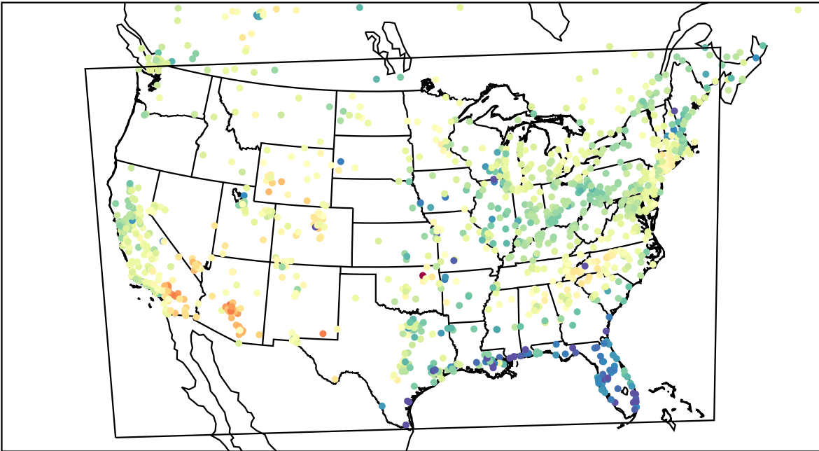
AirNOW (2023-04-02_01:00:00)
