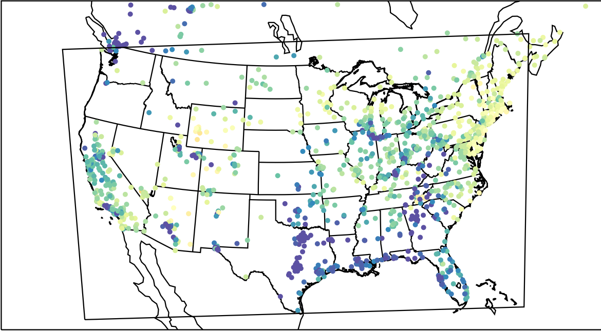
AirNOW (2023-04-03_14:00:00)
