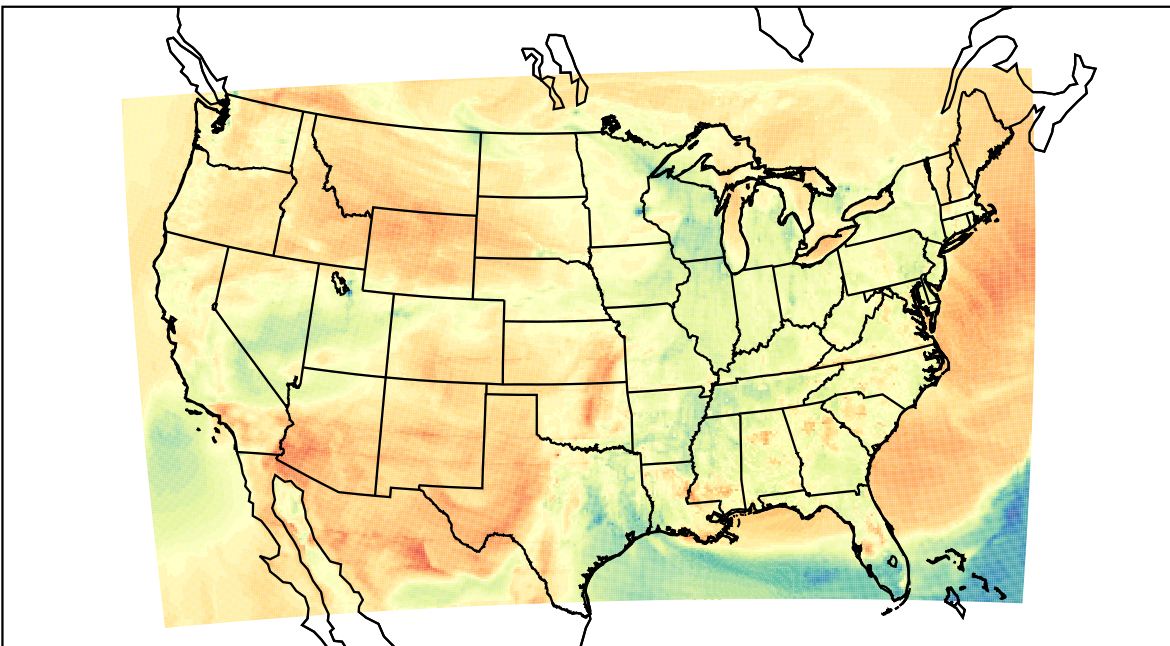
WRF (2023-04-02_23:00:00)
