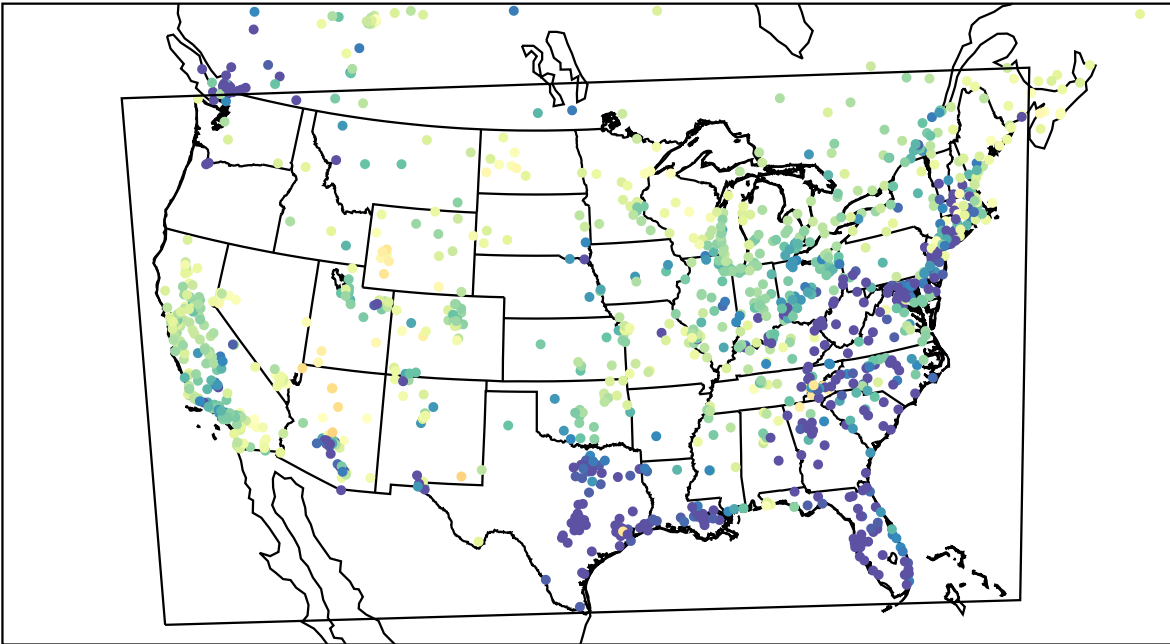
AirNOW (2023-04-03_06:00:00)
