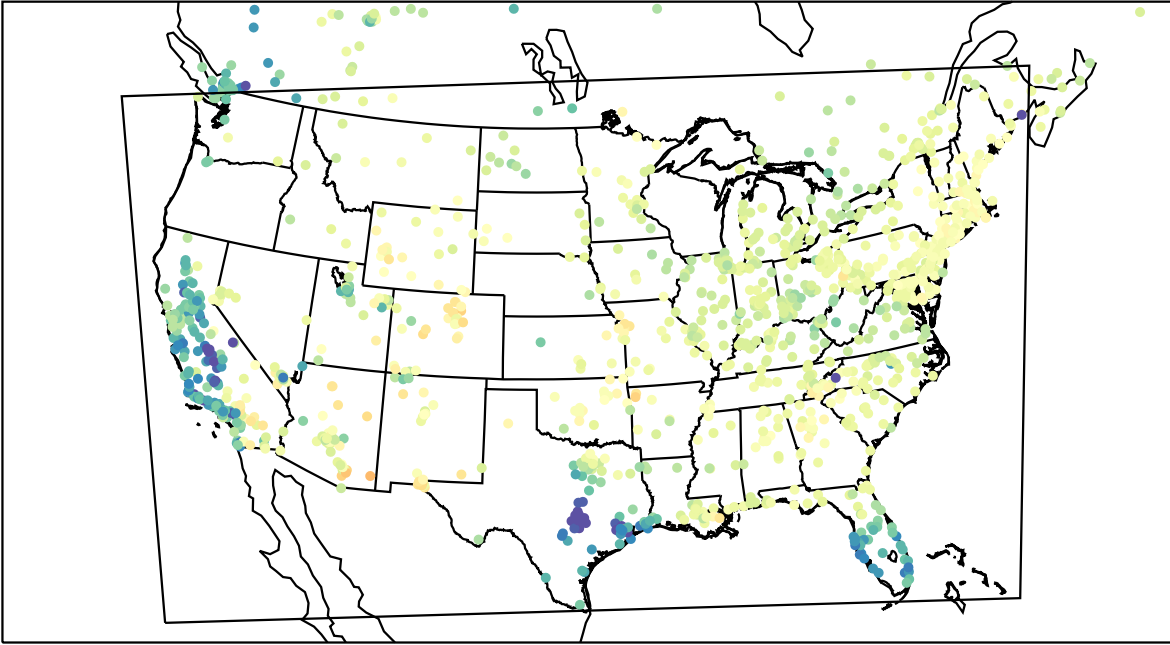
AirNOW (2023-04-02_16:00:00)
