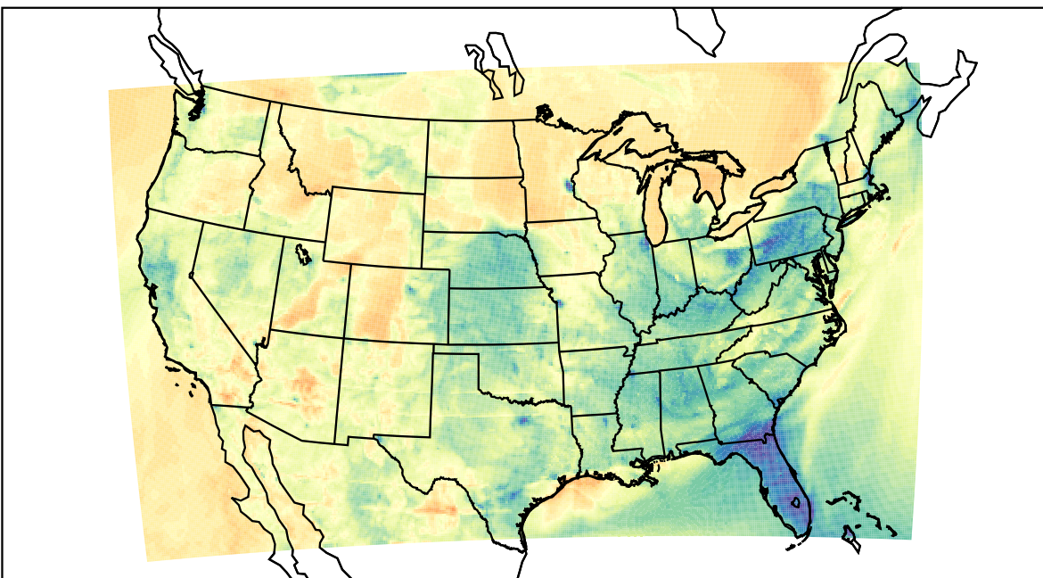
WRF (2023-04-02_03:00:00)
