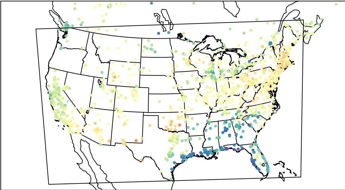
AirNOW (2023-04-03_21:00:00)
