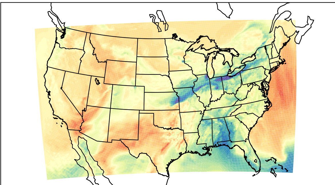
WRF (2023-04-03_23:00:00)
