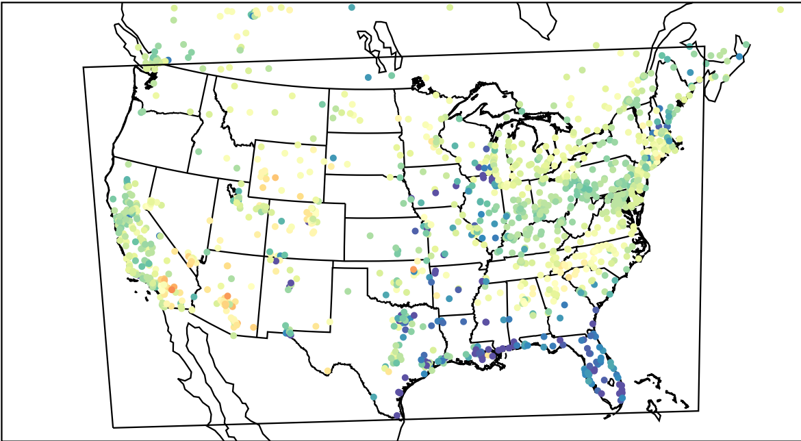
AirNOW (2023-04-02_02:00:00)
