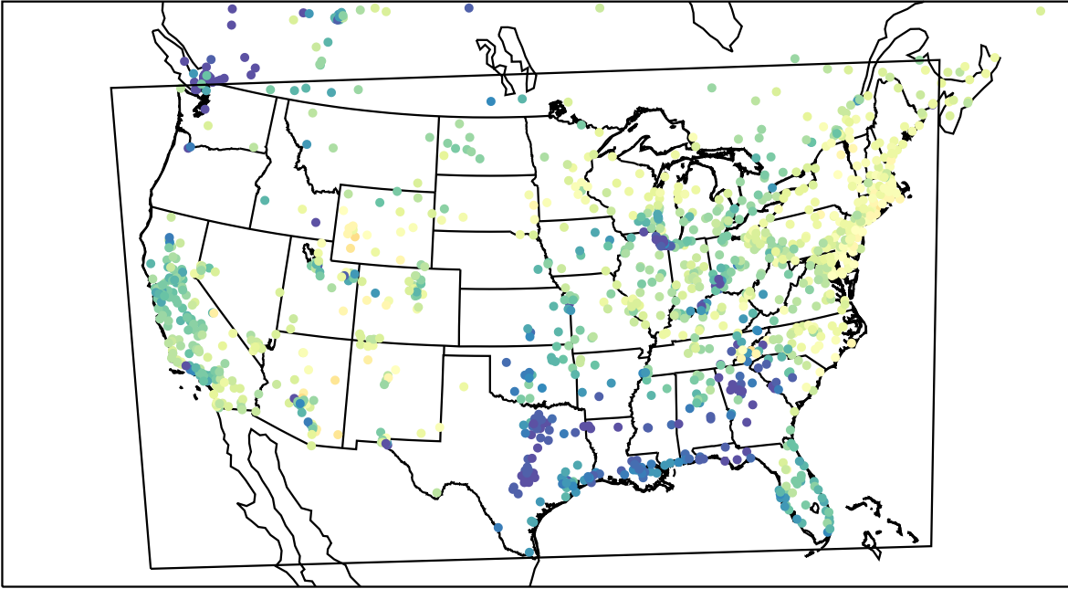
AirNOW (2023-04-03_15:00:00)
