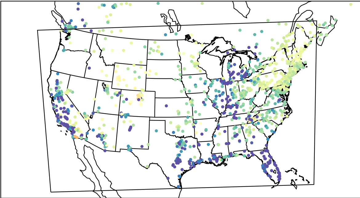
AirNOW (2023-04-02_11:00:00)
