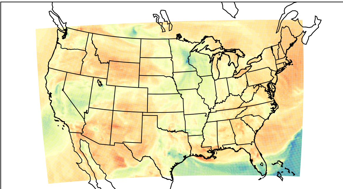
WRF (2023-04-02_19:00:00)
