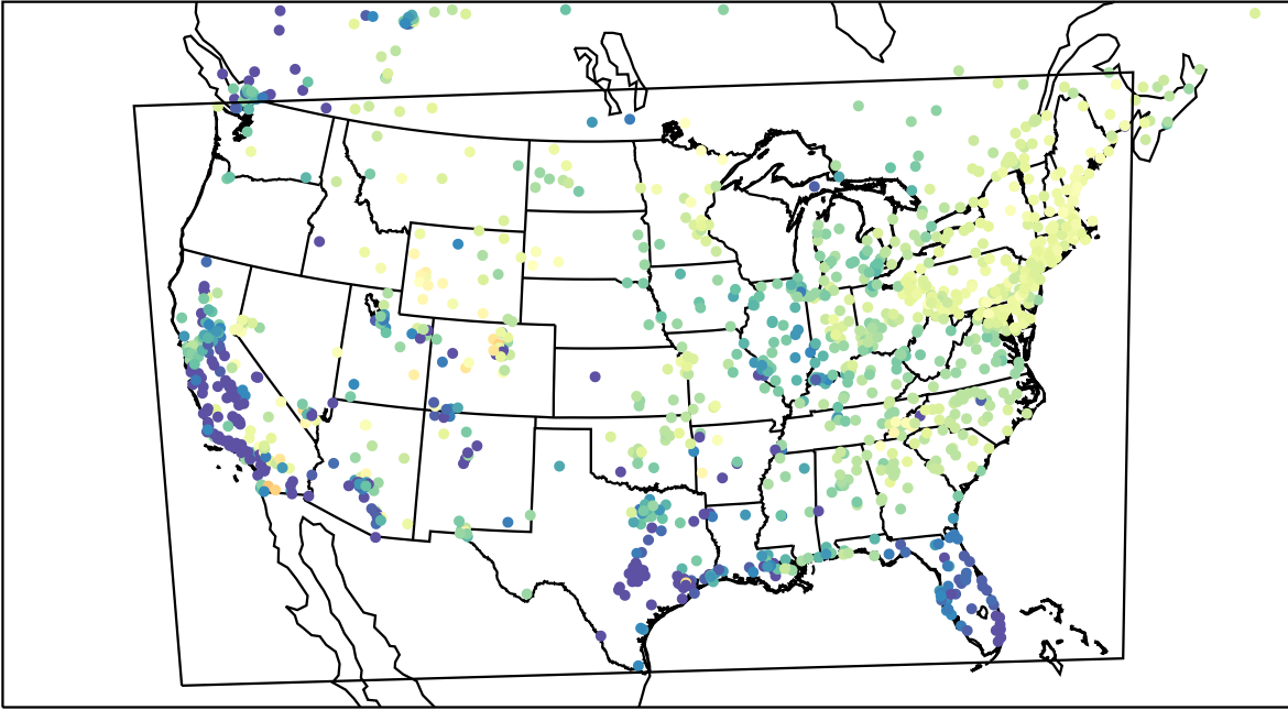
AirNOW (2023-04-02_13:00:00)
