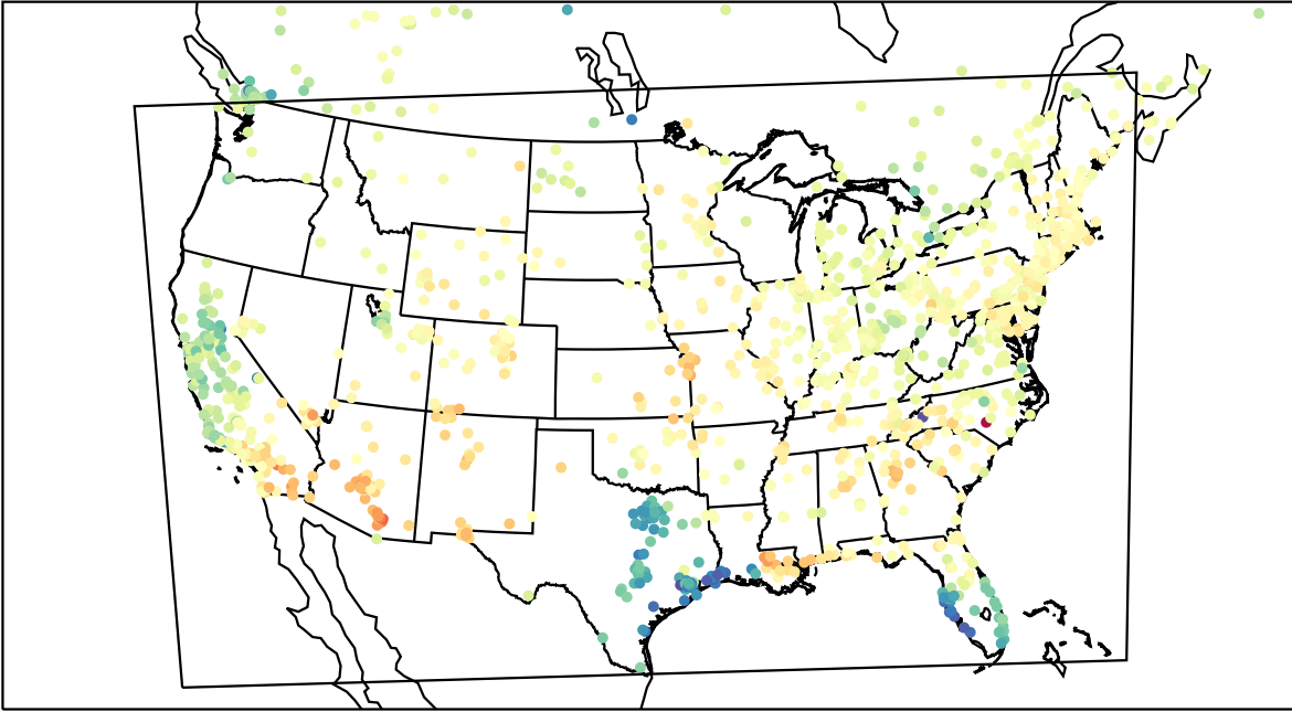
AirNOW (2023-04-02_20:00:00)
