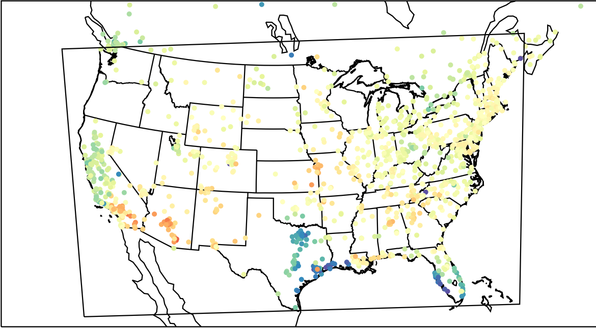
AirNOW (2023-04-02_22:00:00)
