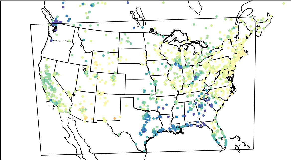
AirNOW (2023-04-03_16:00:00)
