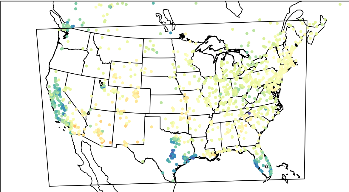
AirNOW (2023-04-02_17:00:00)
