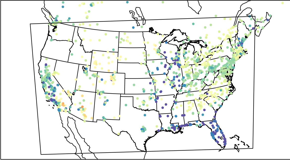
AirNOW (2023-04-02_04:00:00)
