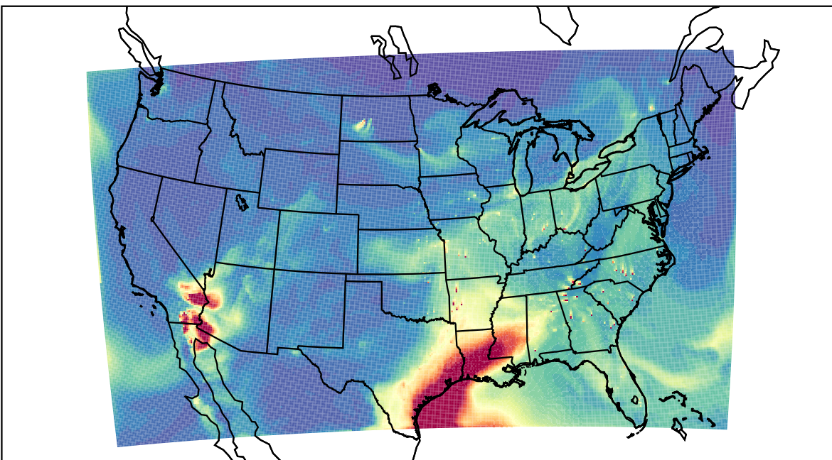
WRF 2023-04-03_19:00:00
