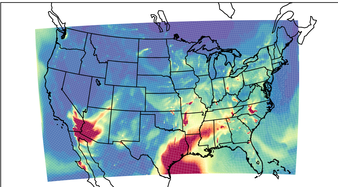
WRF 2023-04-04_02:00:00
