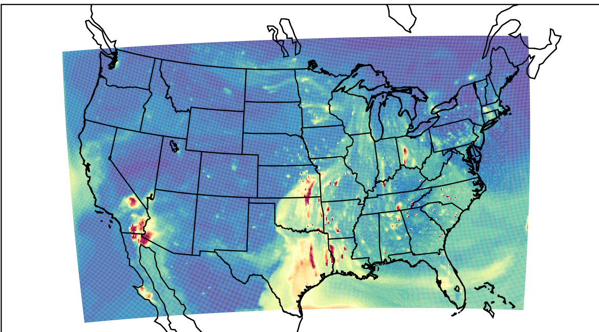
WRF 2023-04-03_01:00:00
