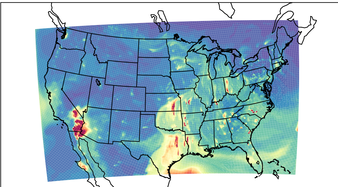
WRF 2023-04-03_03:00:00
