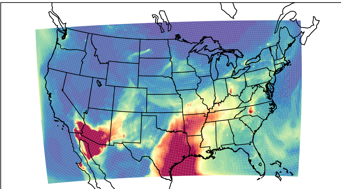
WRF 2023-04-04_09:00:00
