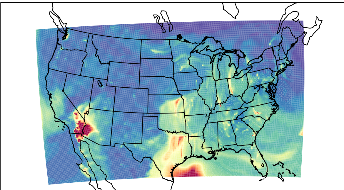
WRF 2023-04-03_06:00:00
