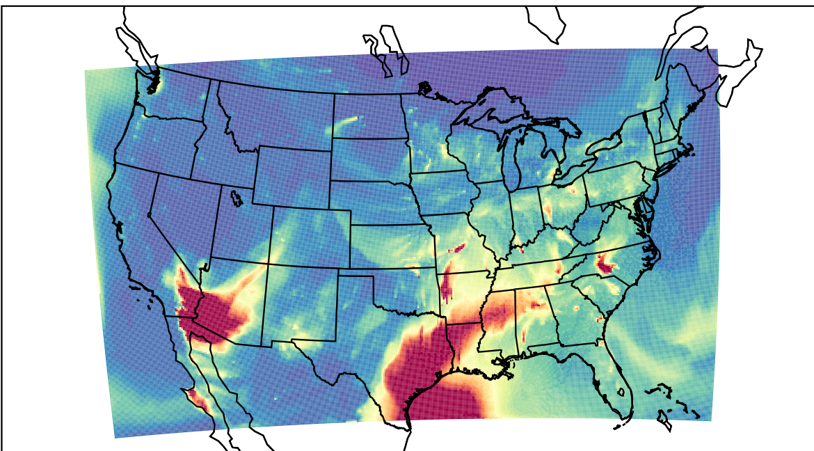
WRF 2023-04-04_03:00:00
