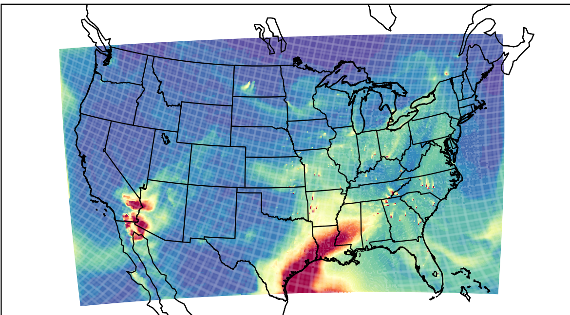
WRF 2023-04-03_20:00:00
