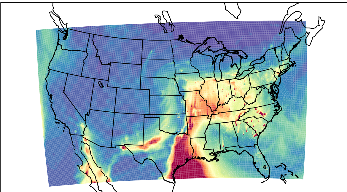
WRF 2023-04-04_23:00:00
