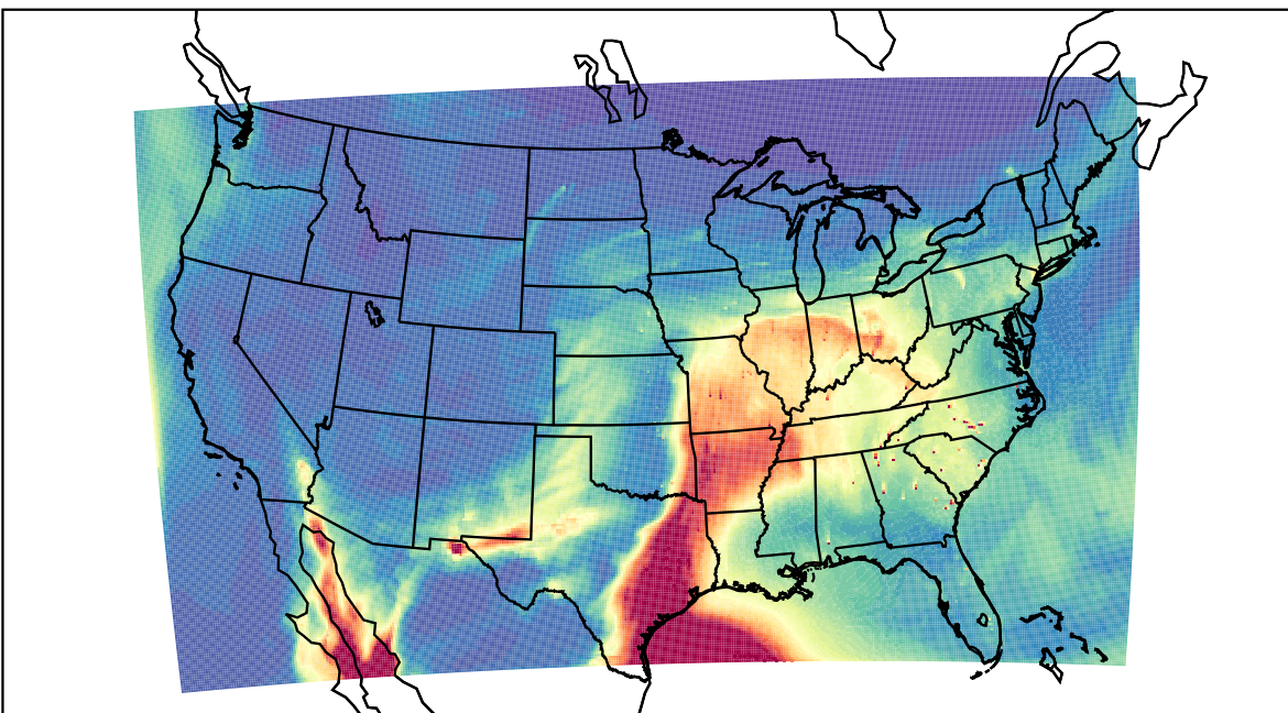
WRF 2023-04-04_19:00:00
