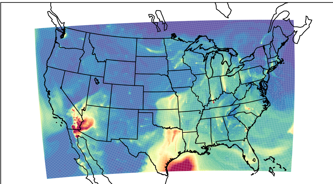
WRF 2023-04-03_08:00:00
