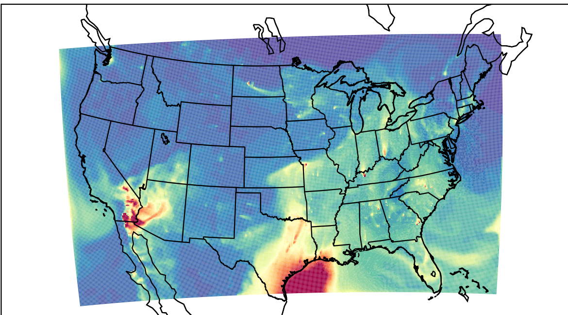
WRF 2023-04-03_11:00:00
