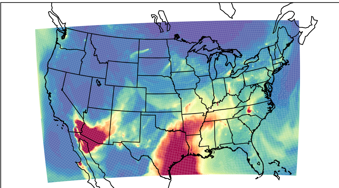
WRF 2023-04-04_07:00:00
