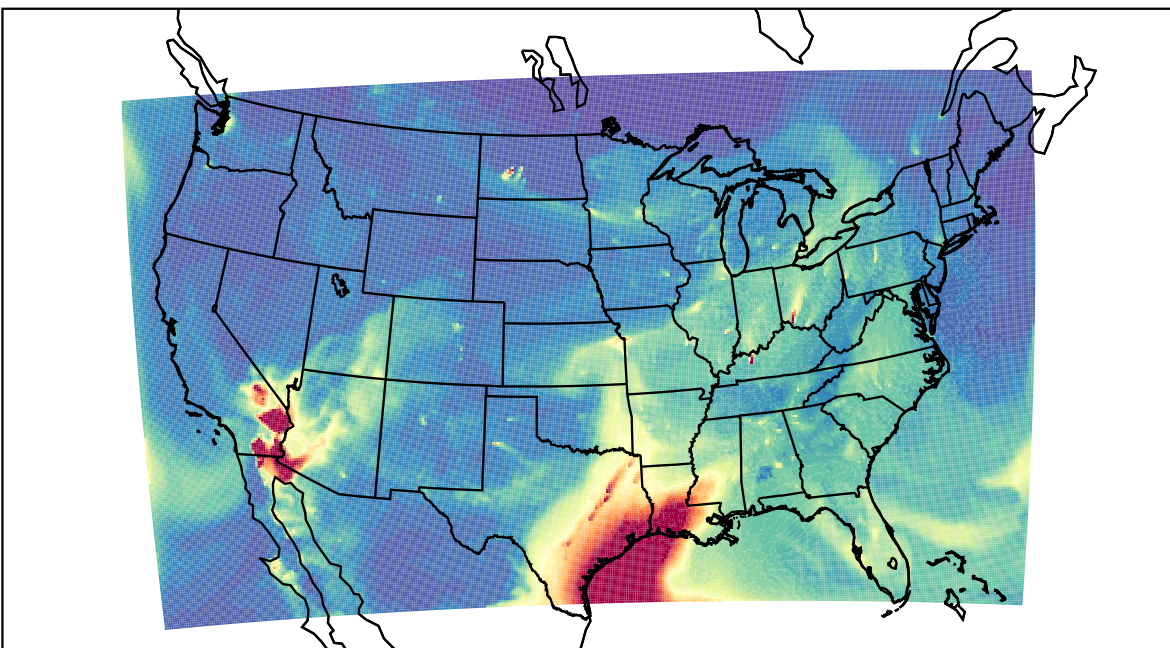
WRF 2023-04-03_15:00:00
