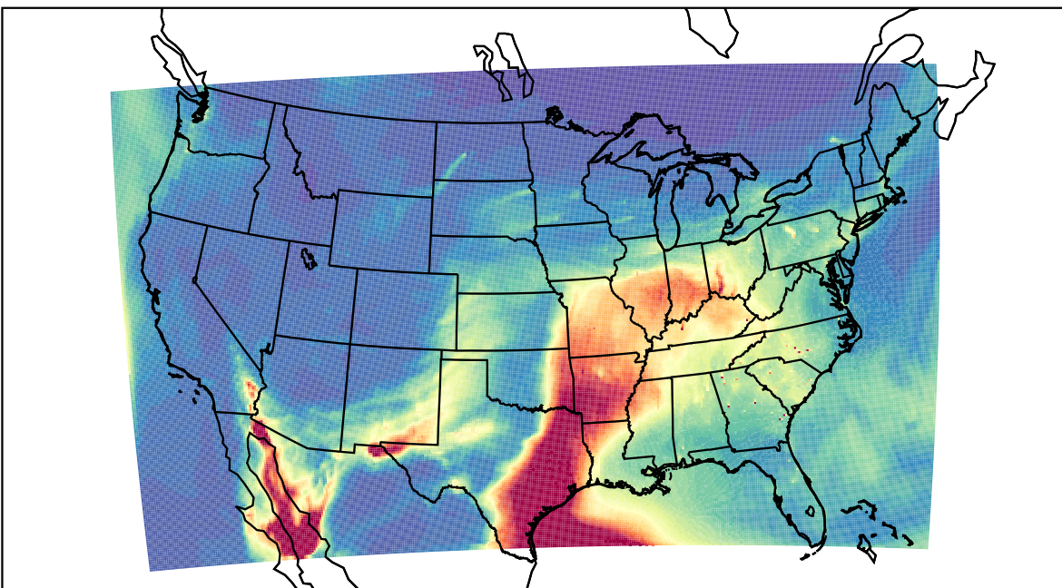
WRF 2023-04-04_17:00:00
