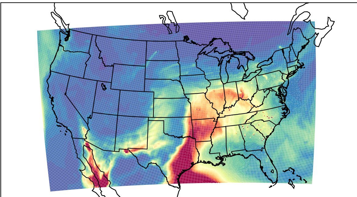
WRF 2023-04-04_18:00:00
