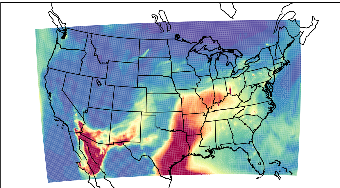
WRF 2023-04-04_15:00:00
