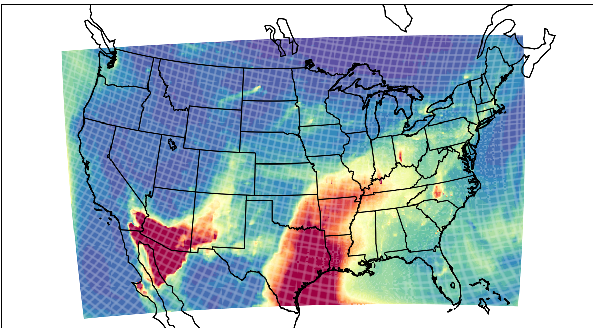
WRF 2023-04-04_11:00:00
