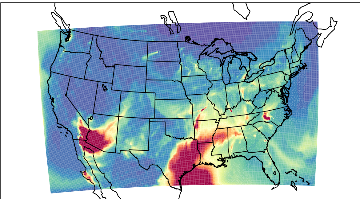
WRF 2023-04-04_04:00:00
