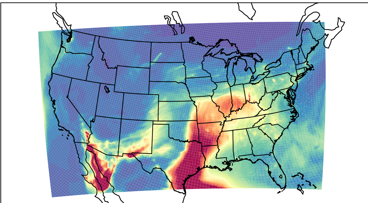
WRF 2023-04-04_16:00:00
