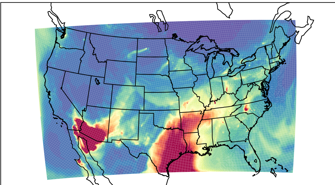
WRF 2023-04-04_08:00:00
