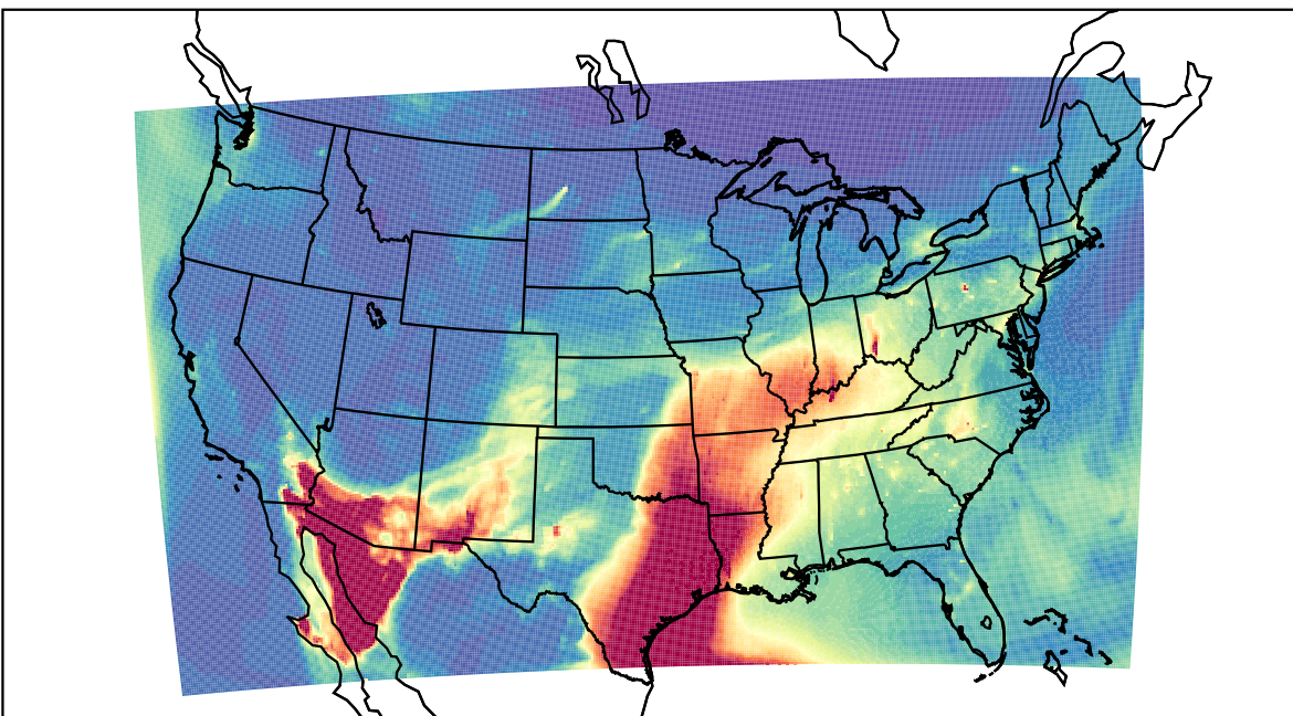
WRF 2023-04-04_14:00:00
