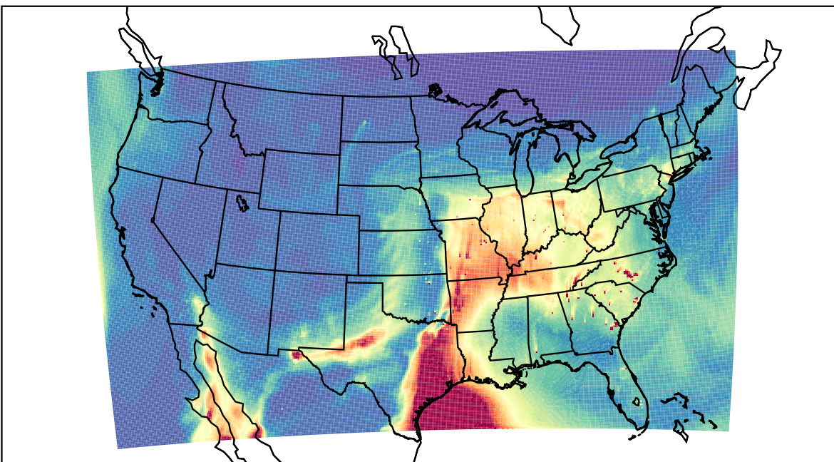
WRF 2023-04-04_22:00:00
