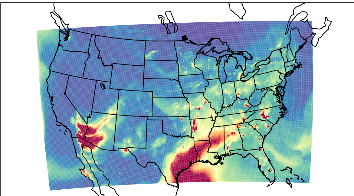
WRF 2023-04-04_01:00:00
