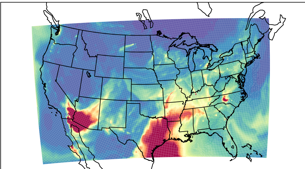
WRF 2023-04-04_05:00:00
