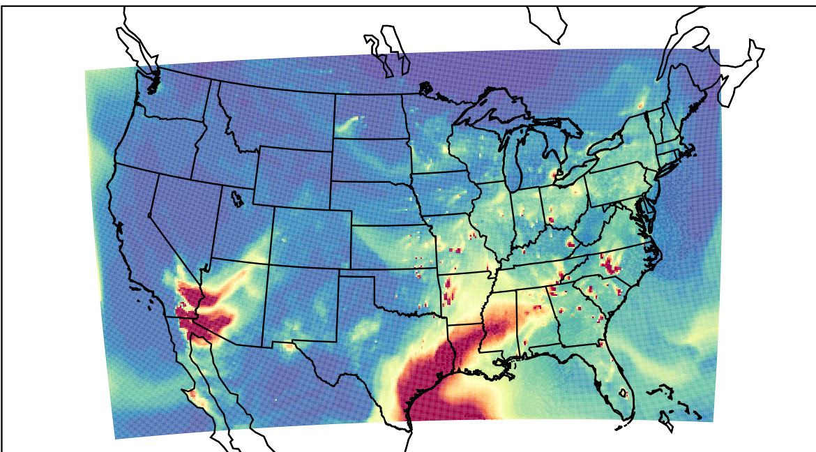
WRF 2023-04-04_00:00:00
