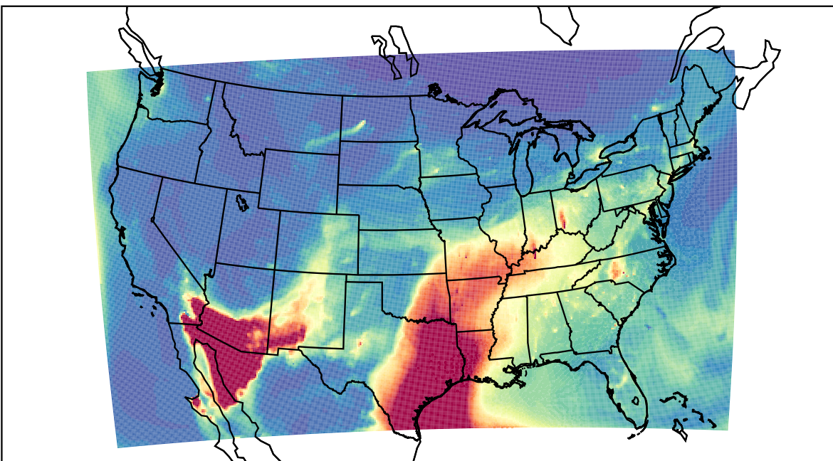
WRF 2023-04-04_12:00:00
