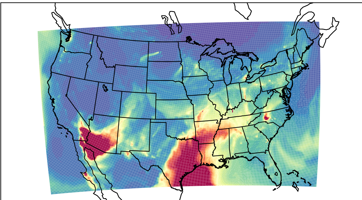
WRF 2023-04-04_06:00:00
