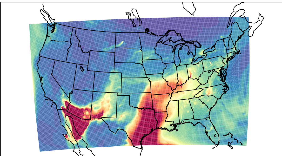
WRF 2023-04-04_13:00:00
