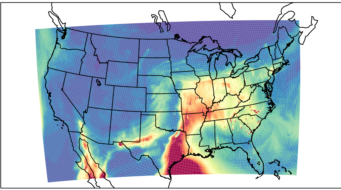
WRF 2023-04-04_21:00:00
