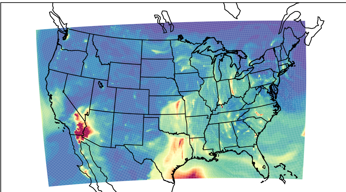
WRF 2023-04-03_05:00:00
