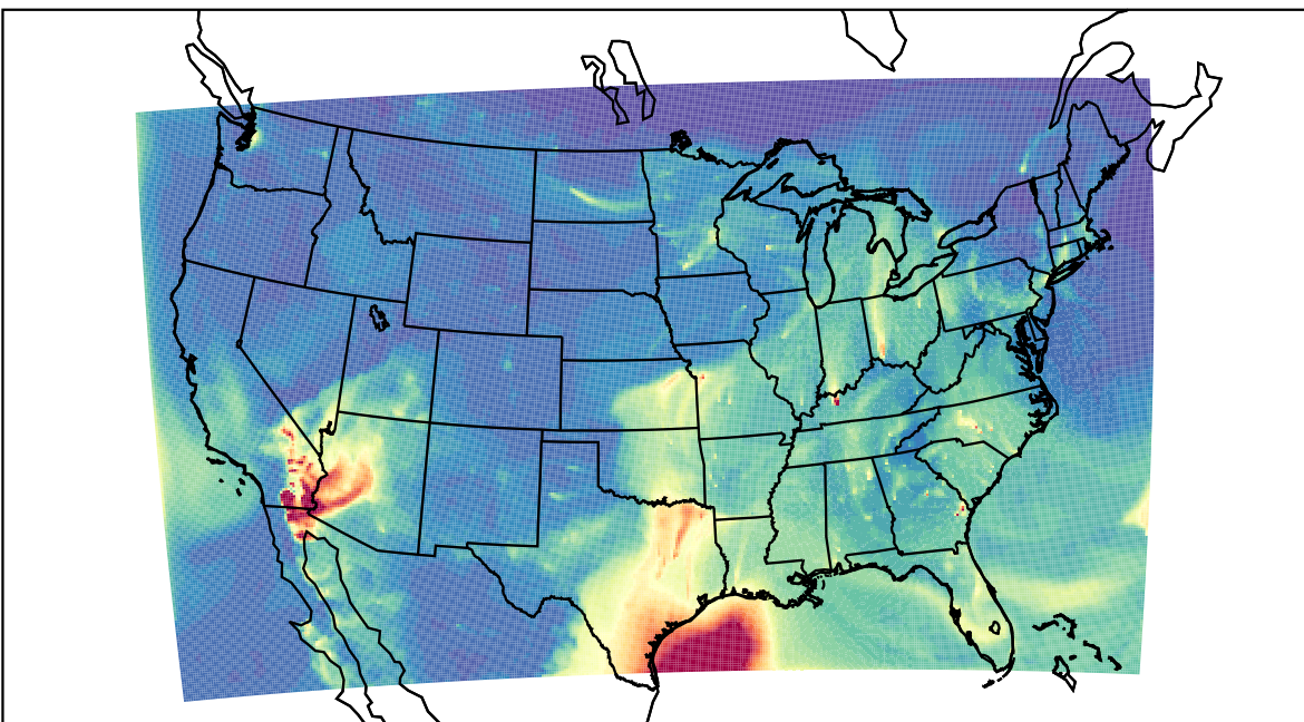
WRF 2023-04-03_09:00:00
