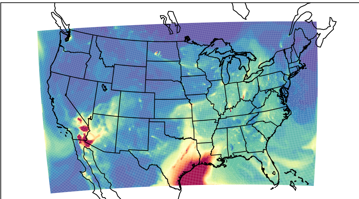
WRF 2023-04-03_14:00:00
