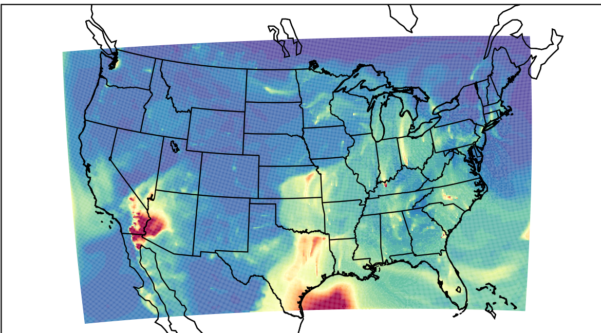
WRF 2023-04-03_07:00:00
