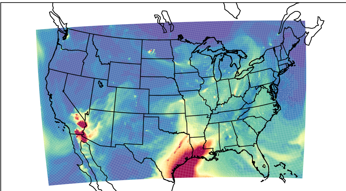
WRF 2023-04-03_16:00:00
