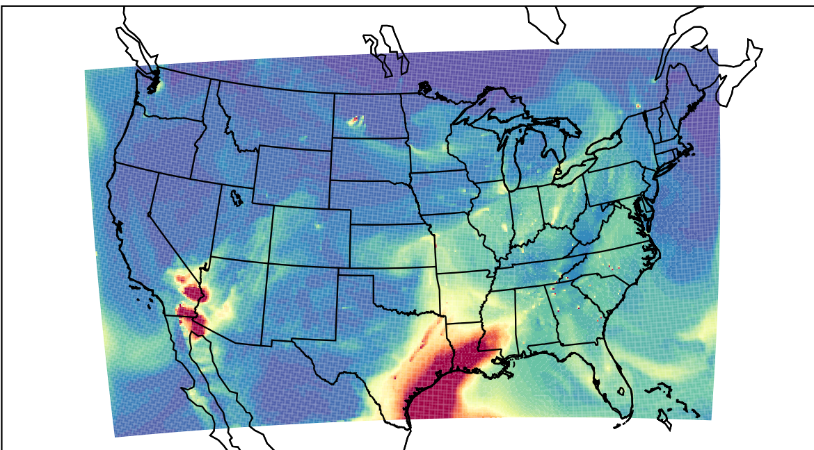
WRF 2023-04-03_17:00:00
