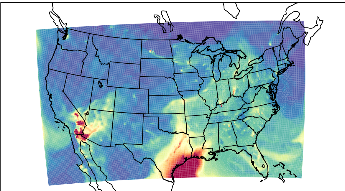
WRF 2023-04-03_13:00:00
