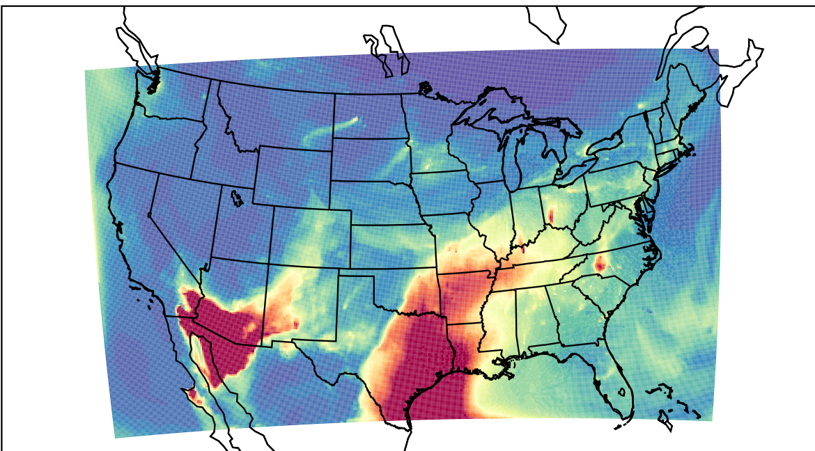
WRF 2023-04-04_10:00:00
