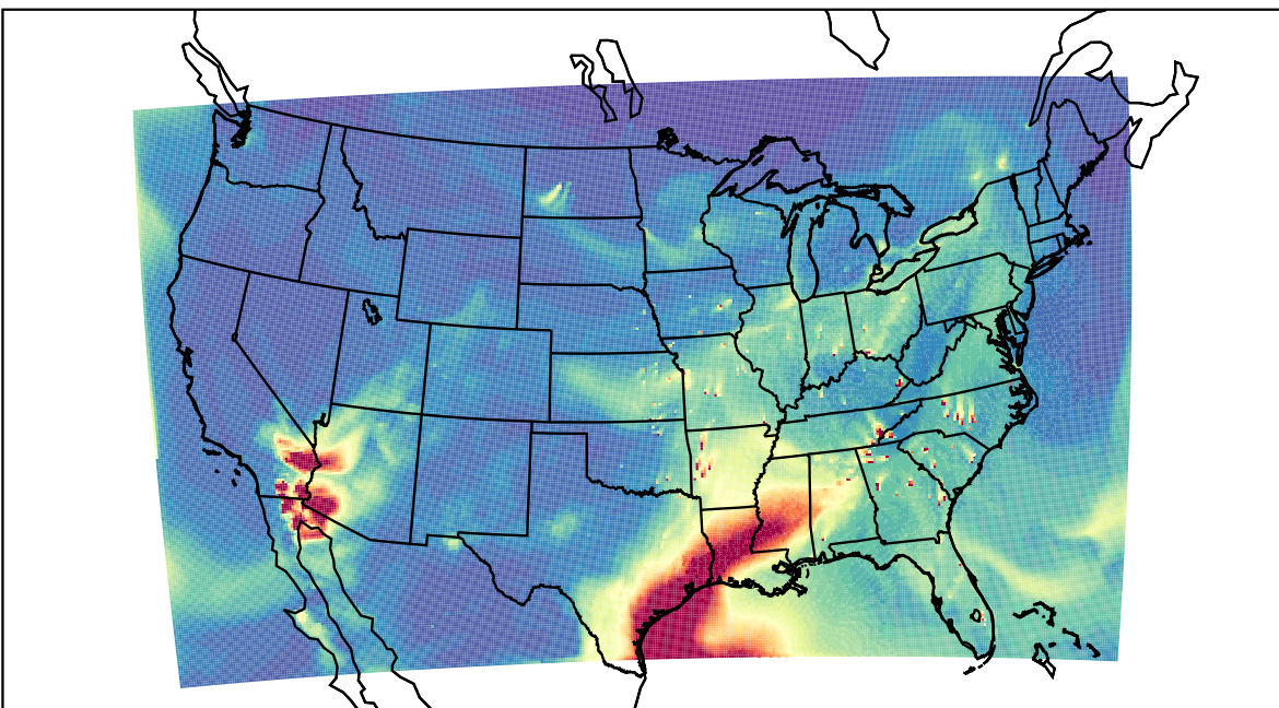
WRF 2023-04-03_21:00:00
