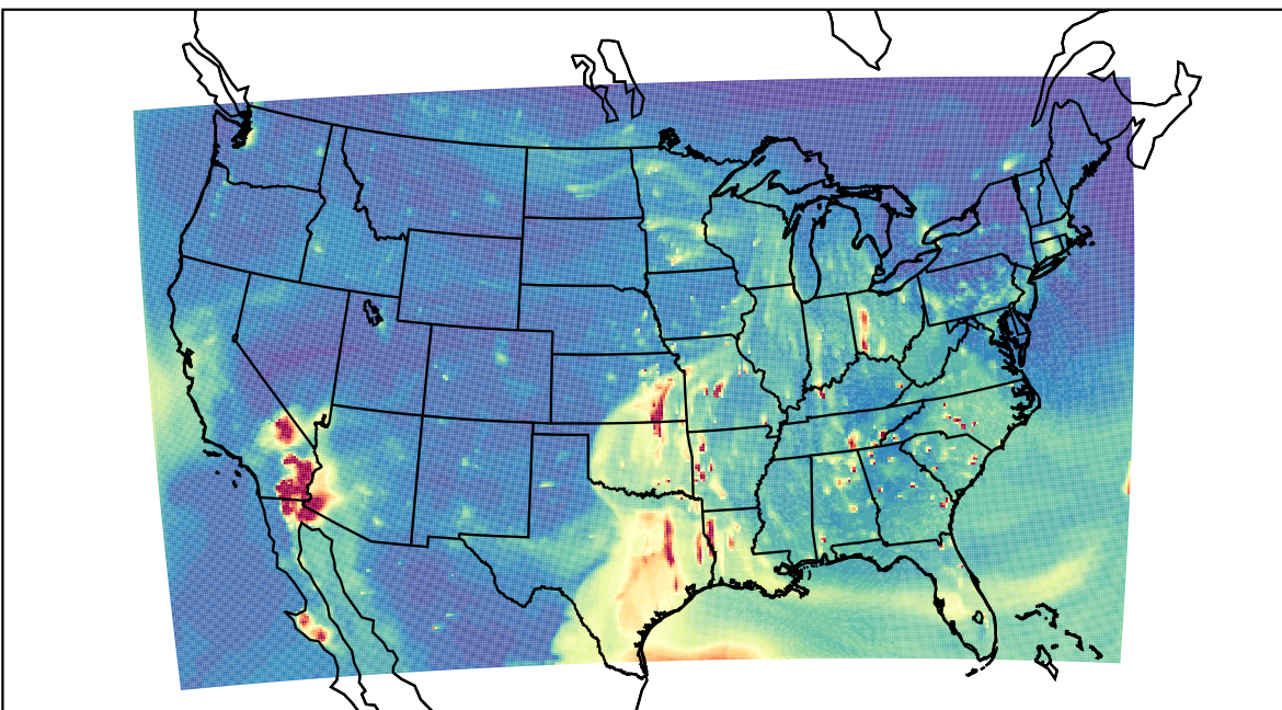
WRF 2023-04-03_02:00:00
