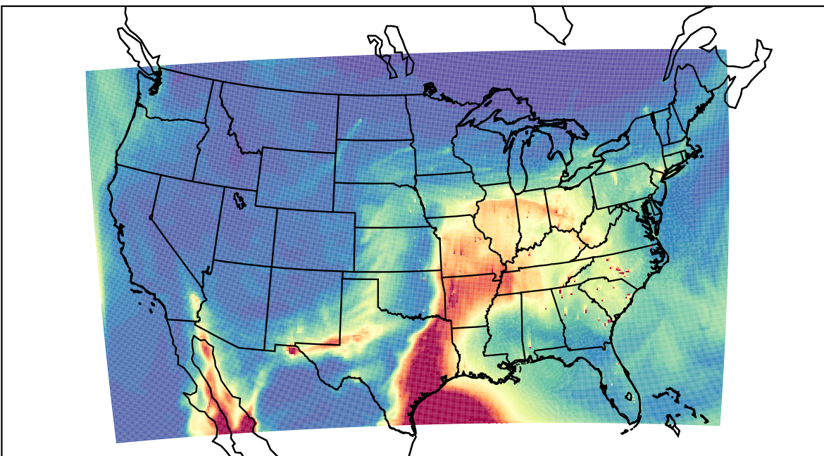
WRF 2023-04-04_20:00:00
