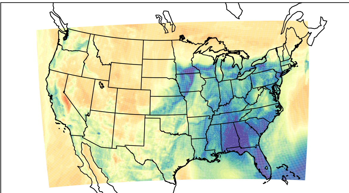
WRF (2023-04-05_07:00:00)
