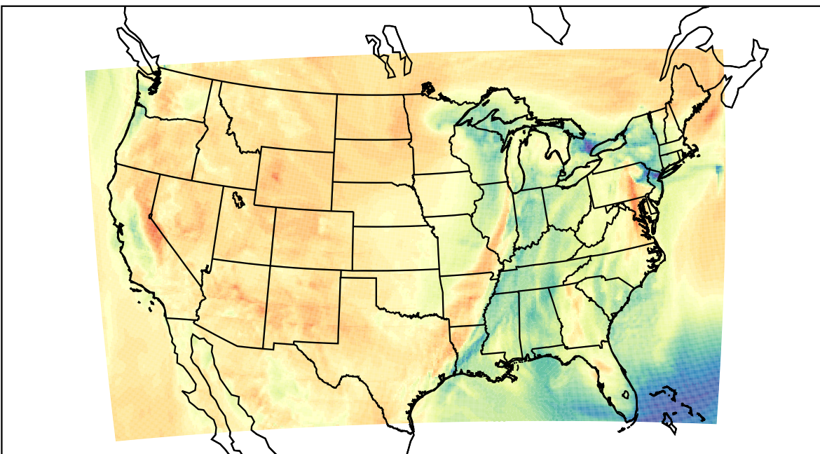
WRF (2023-04-05_18:00:00)
