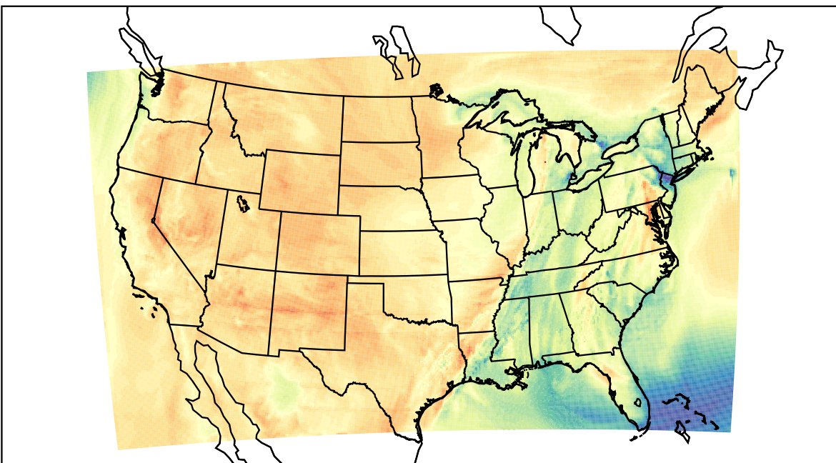
WRF (2023-04-05_21:00:00)
