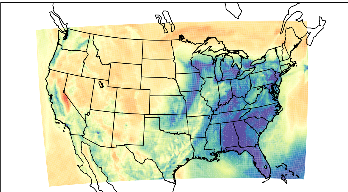
WRF (2023-04-05_12:00:00)
