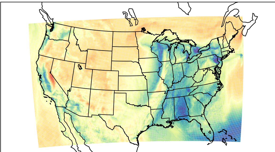
WRF (2023-04-05_15:00:00)
