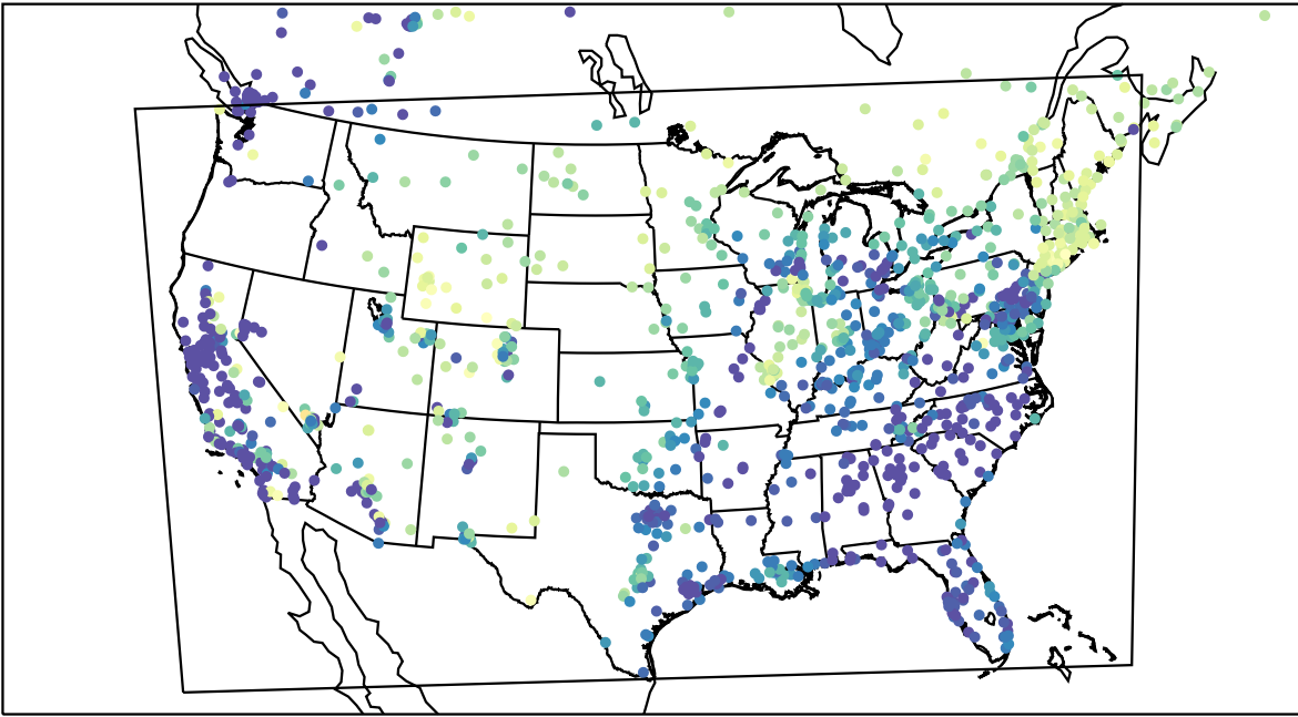
AirNOW (2023-04-05_13:00:00)
