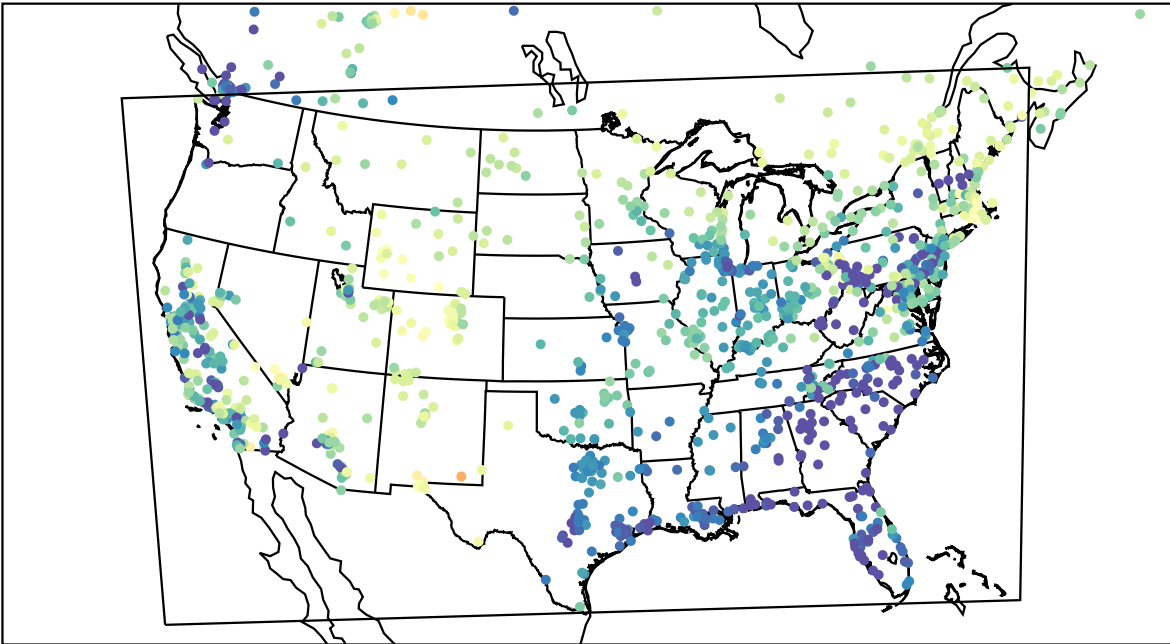
AirNOW (2023-04-05_05:00:00)
