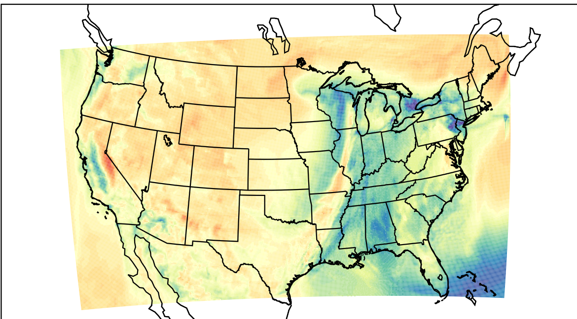
WRF (2023-04-05_16:00:00)
