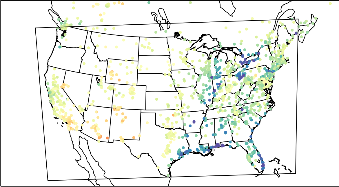
AirNOW (2023-04-05_22:00:00)
