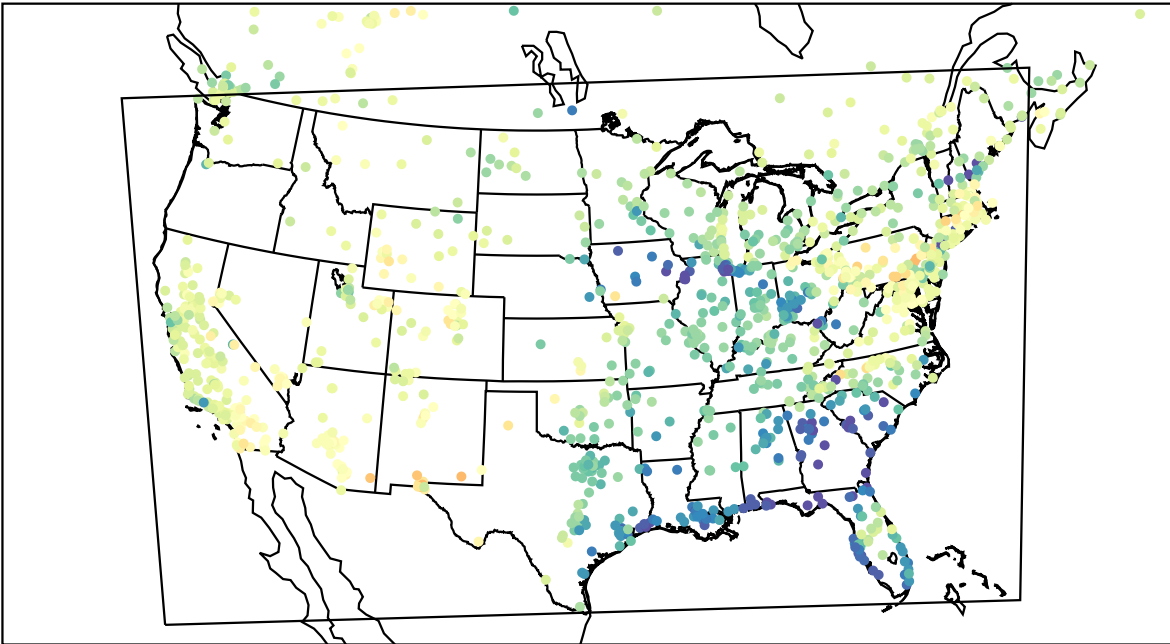
AirNOW (2023-04-04_23:00:00)
