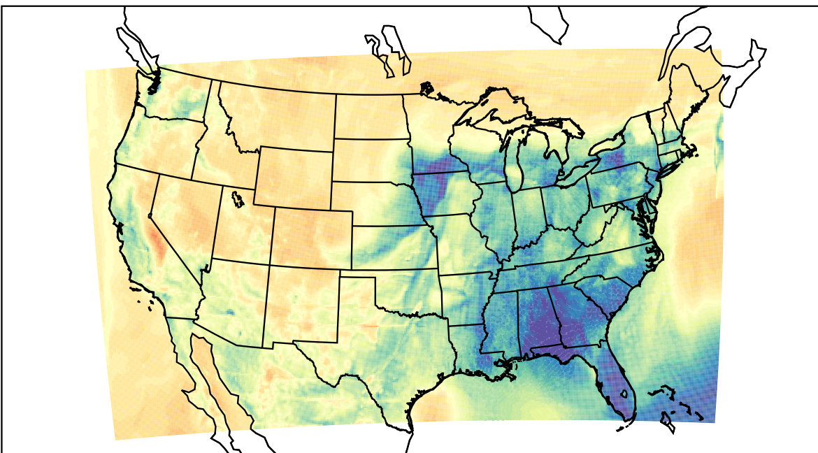
WRF (2023-04-05_05:00:00)
