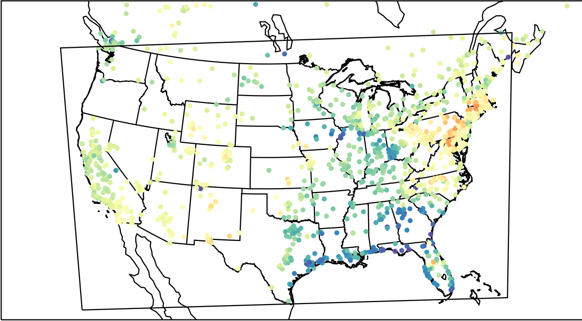
AirNOW (2023-04-04_20:00:00)
