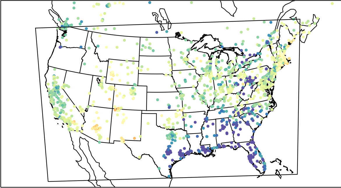
AirNOW (2023-04-04_03:00:00)
