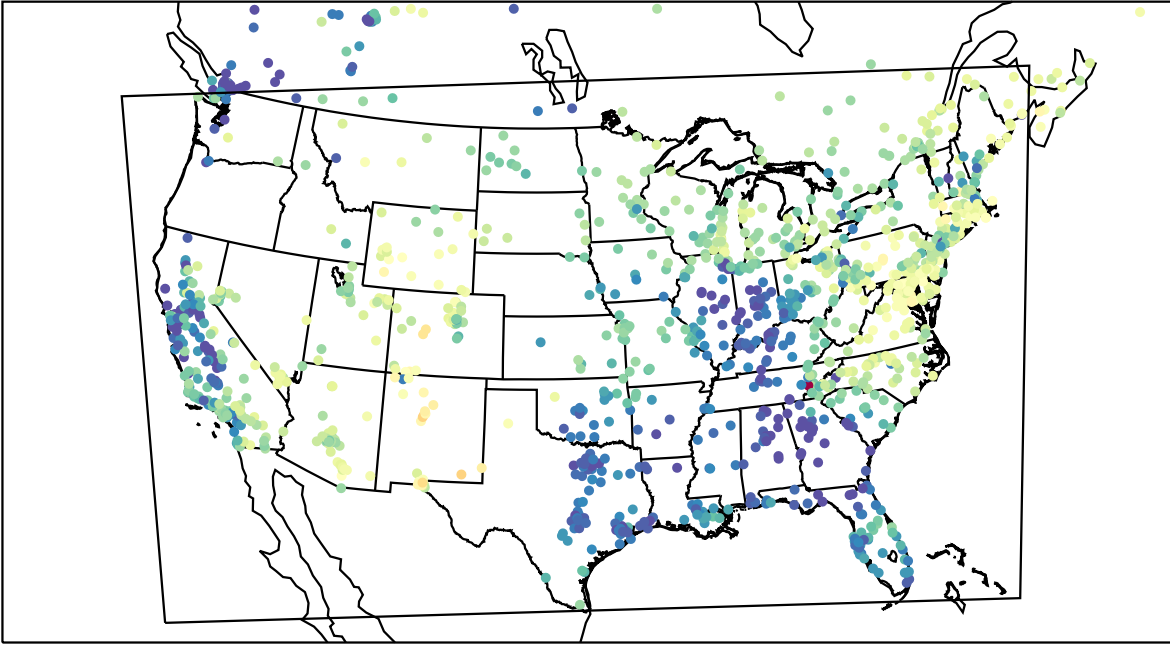
AirNOW (2023-04-04_15:00:00)
