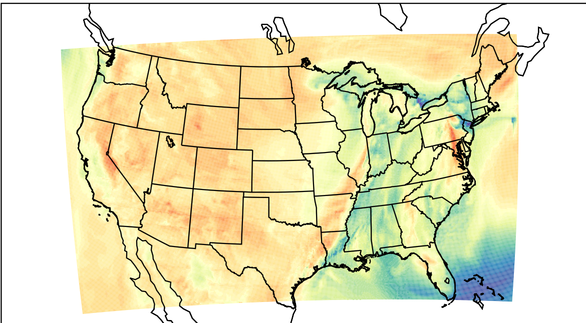
WRF (2023-04-05_19:00:00)
