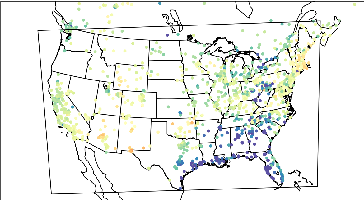
AirNOW (2023-04-04_01:00:00)
