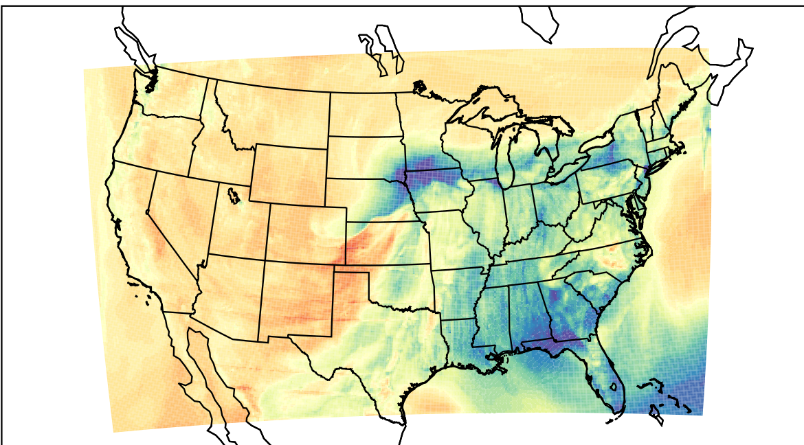
WRF (2023-04-05_01:00:00)
