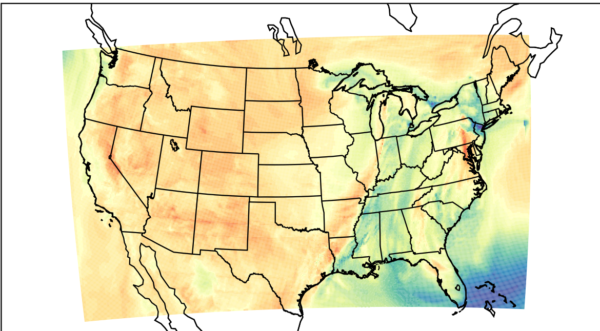
WRF (2023-04-05_20:00:00)
