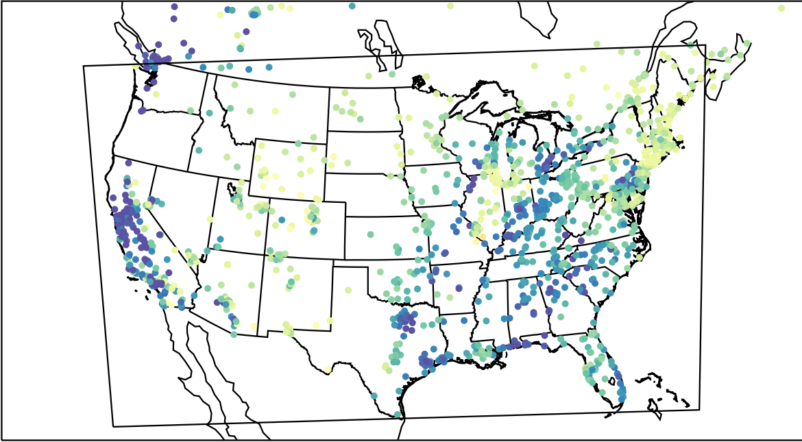
AirNOW (2023-04-05_15:00:00)
