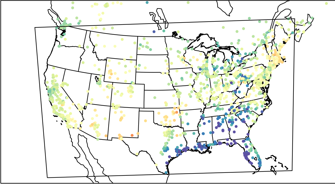
AirNOW (2023-04-04_00:00:00)
