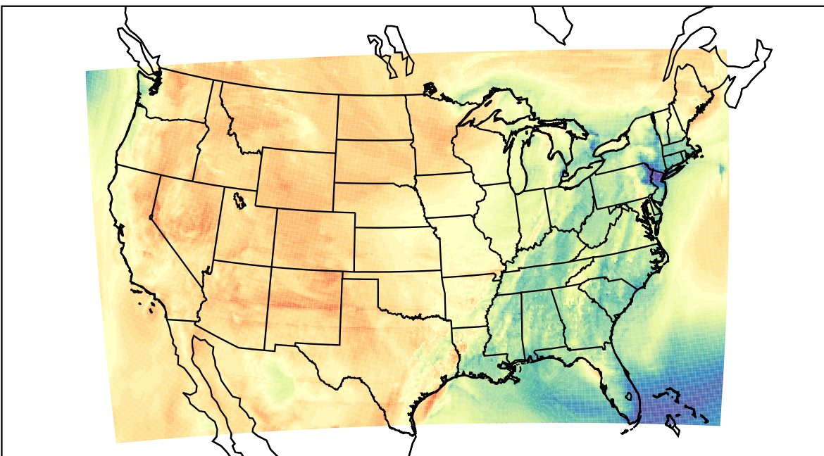
WRF (2023-04-05_23:00:00)
