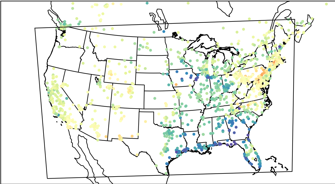
AirNOW (2023-04-04_22:00:00)
