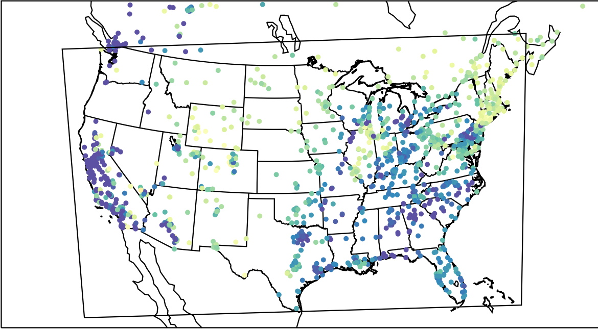
AirNOW (2023-04-05_14:00:00)
