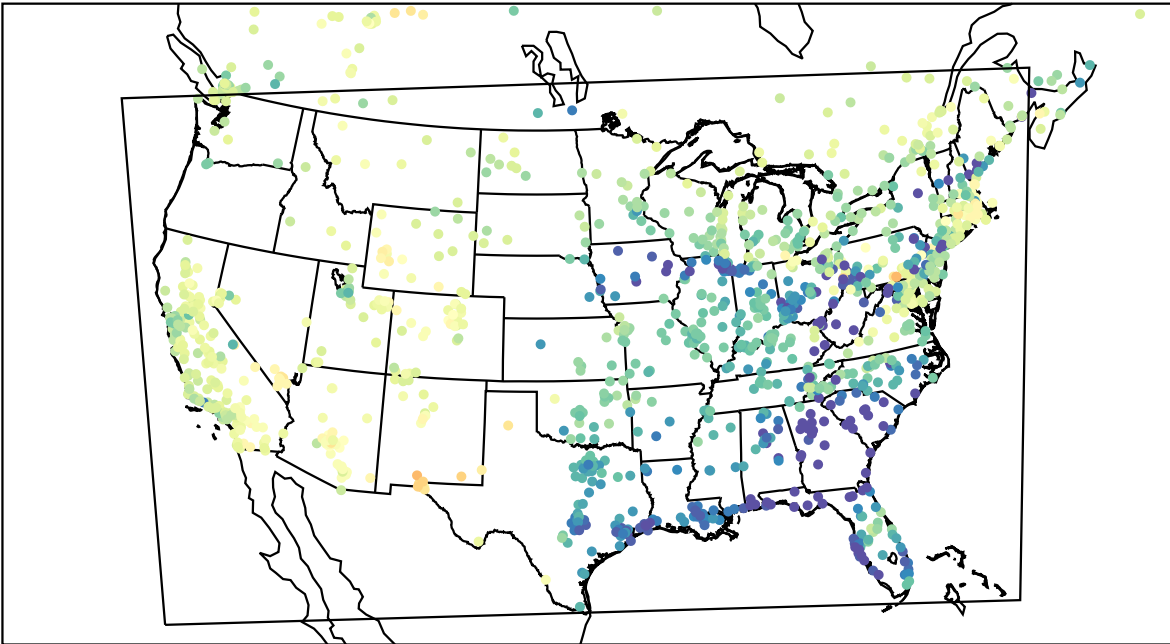
AirNOW (2023-04-05_01:00:00)
