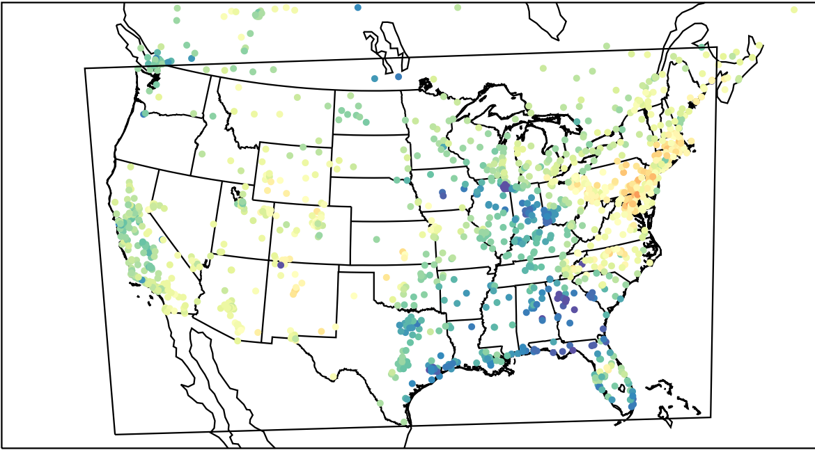
AirNOW (2023-04-04_18:00:00)
