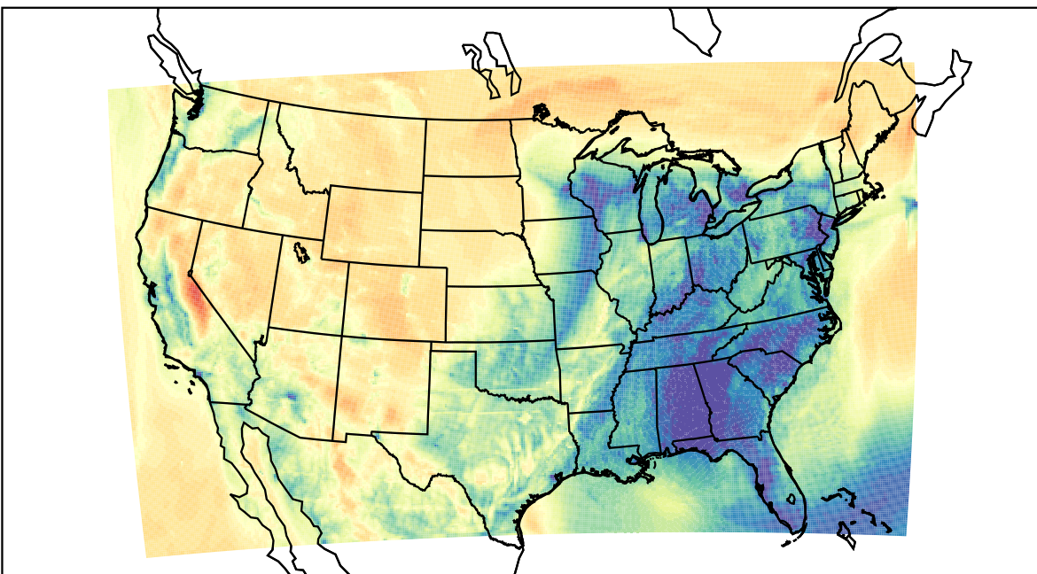
WRF (2023-04-05_13:00:00)
