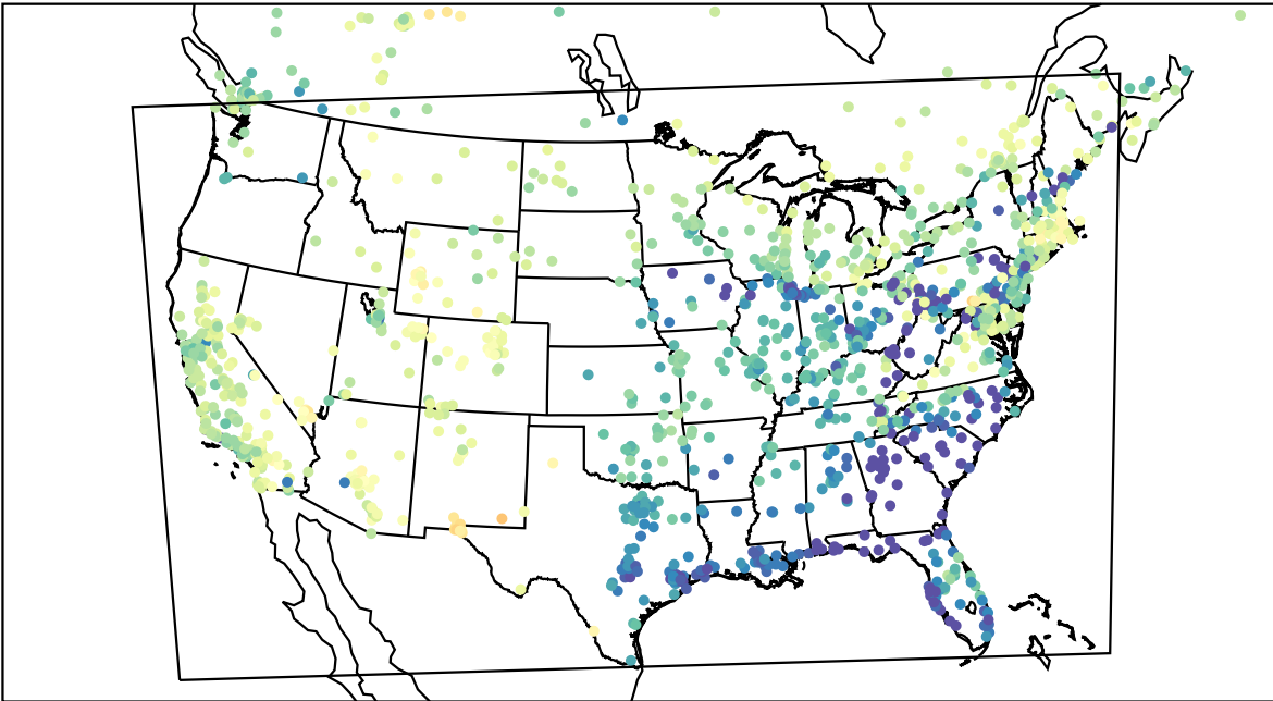
AirNOW (2023-04-05_02:00:00)
