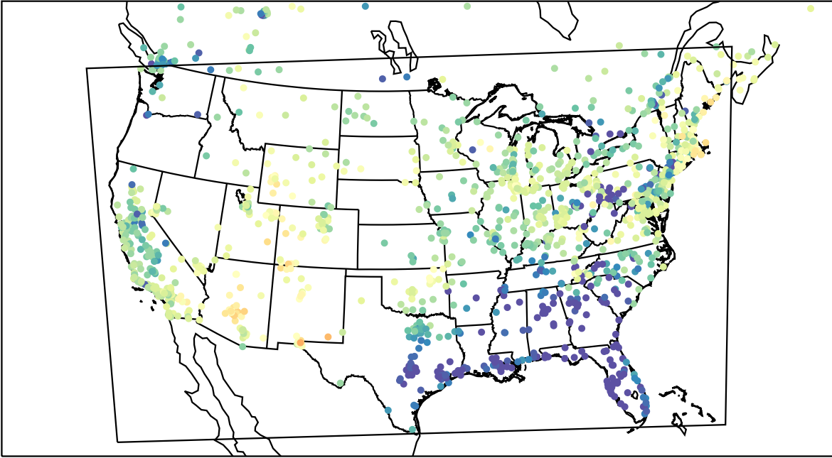
AirNOW (2023-04-04_04:00:00)
