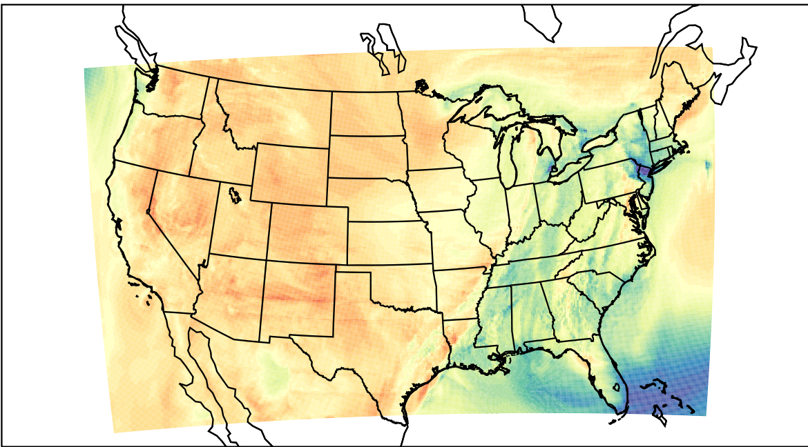
WRF (2023-04-05_22:00:00)
