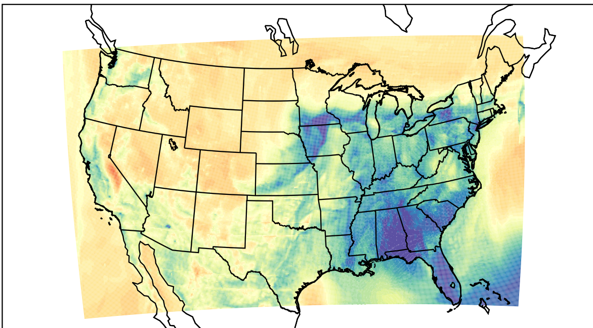
WRF (2023-04-05_06:00:00)
