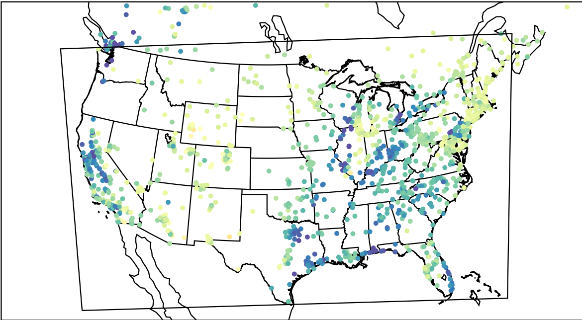
AirNOW (2023-04-05_16:00:00)
