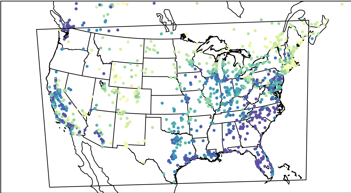
AirNOW (2023-04-05_07:00:00)
