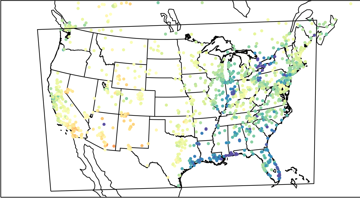
AirNOW (2023-04-05_23:00:00)
