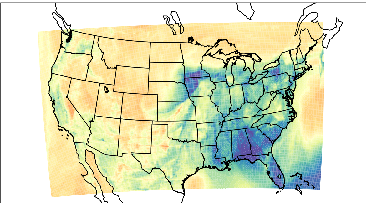
WRF (2023-04-05_04:00:00)
