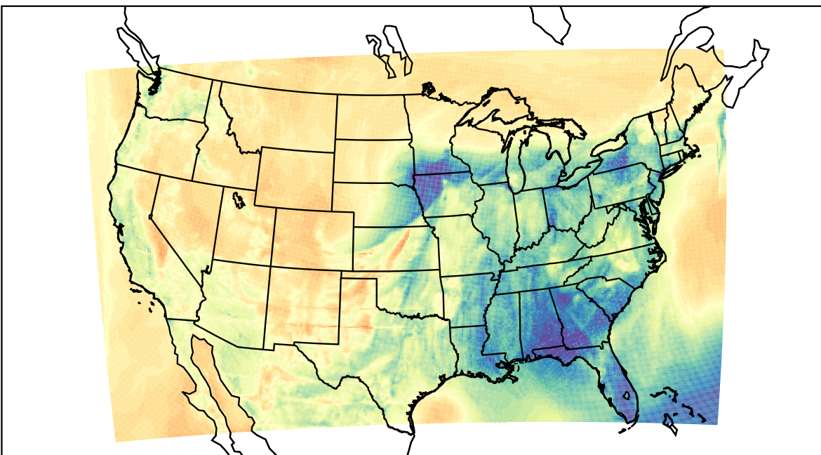
WRF (2023-04-05_03:00:00)
