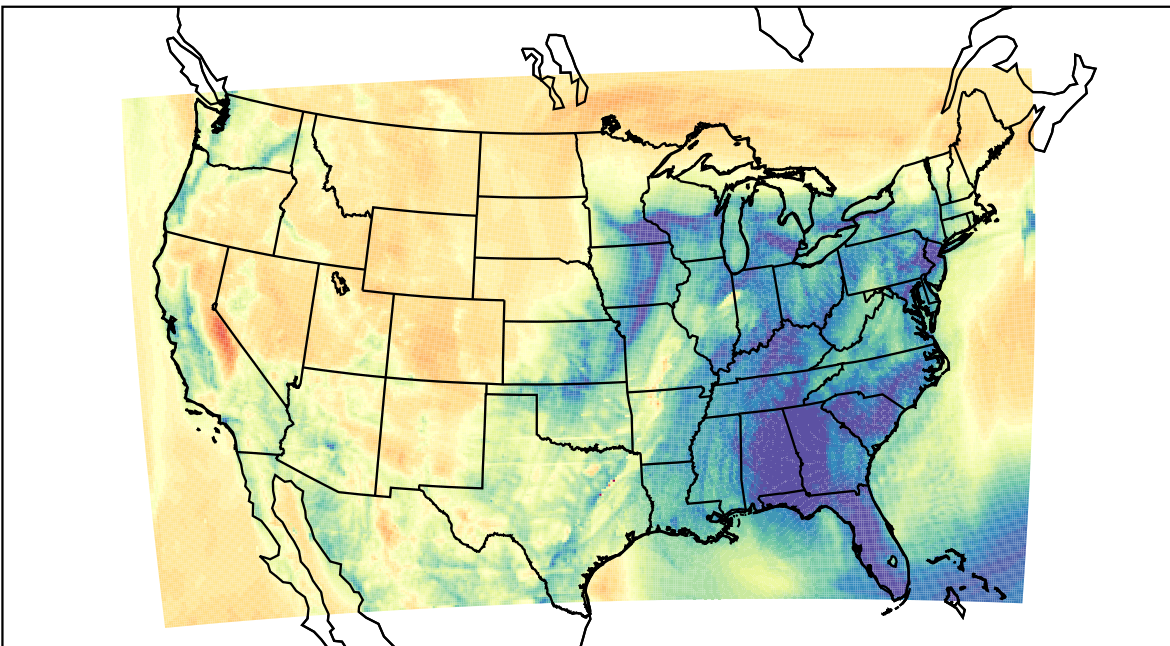
WRF (2023-04-05_10:00:00)
