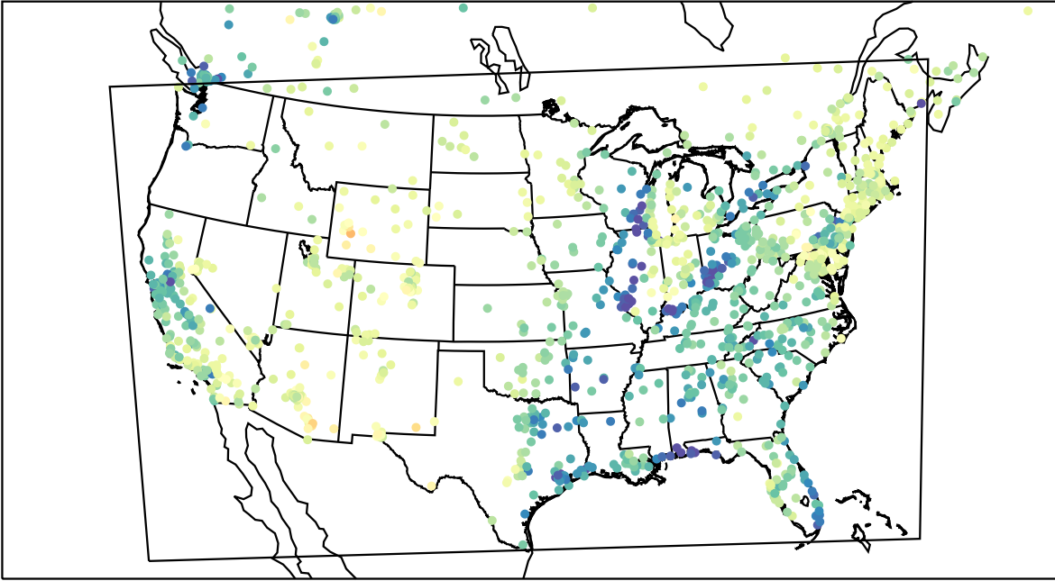
AirNOW (2023-04-05_17:00:00)
