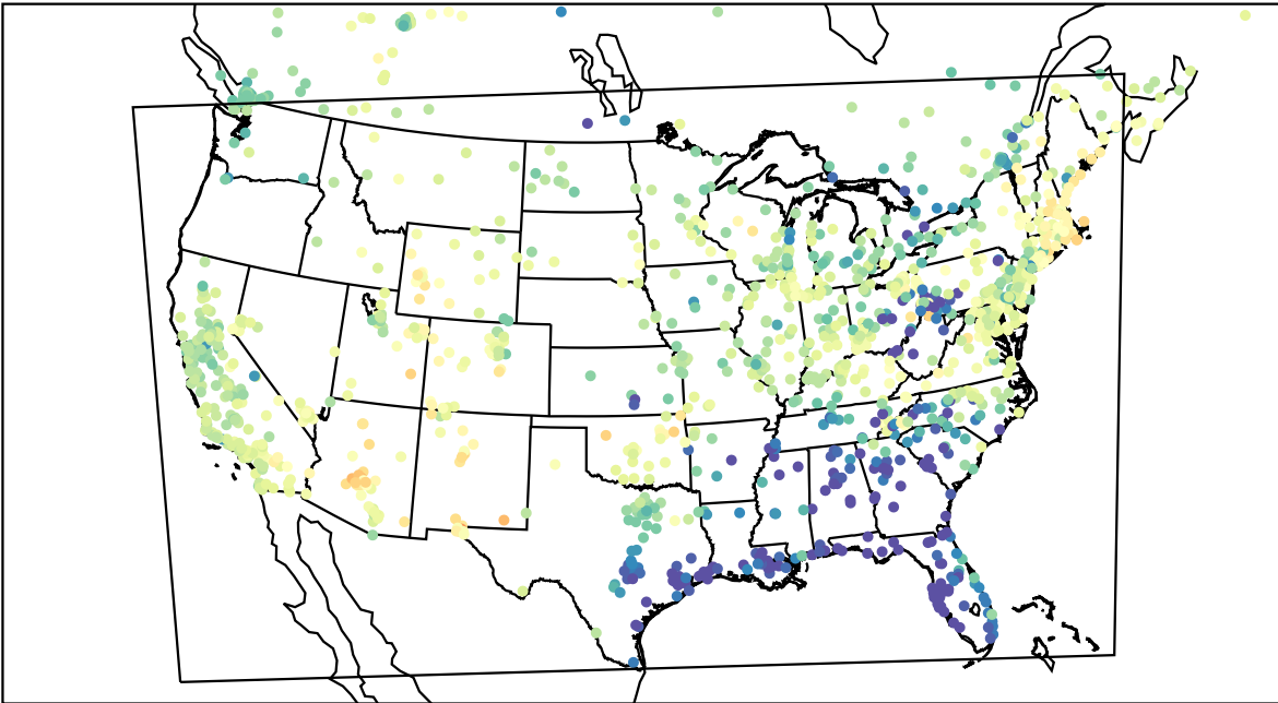
AirNOW (2023-04-04_02:00:00)
