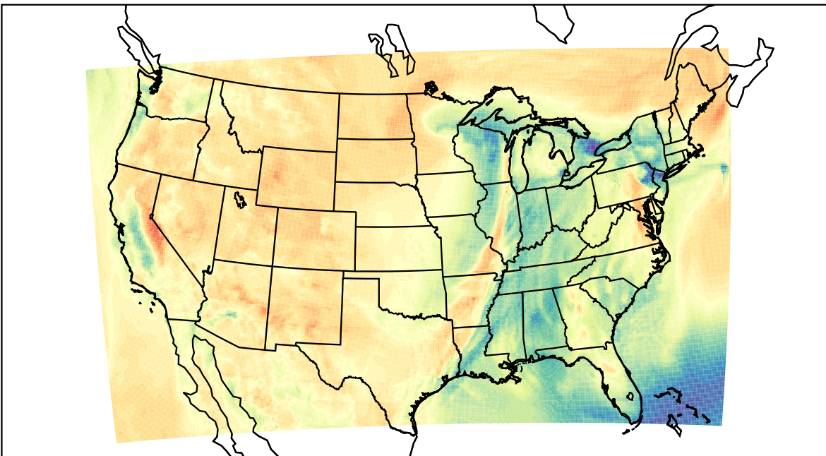
WRF (2023-04-05_17:00:00)
