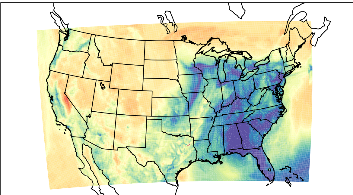
WRF (2023-04-05_11:00:00)
