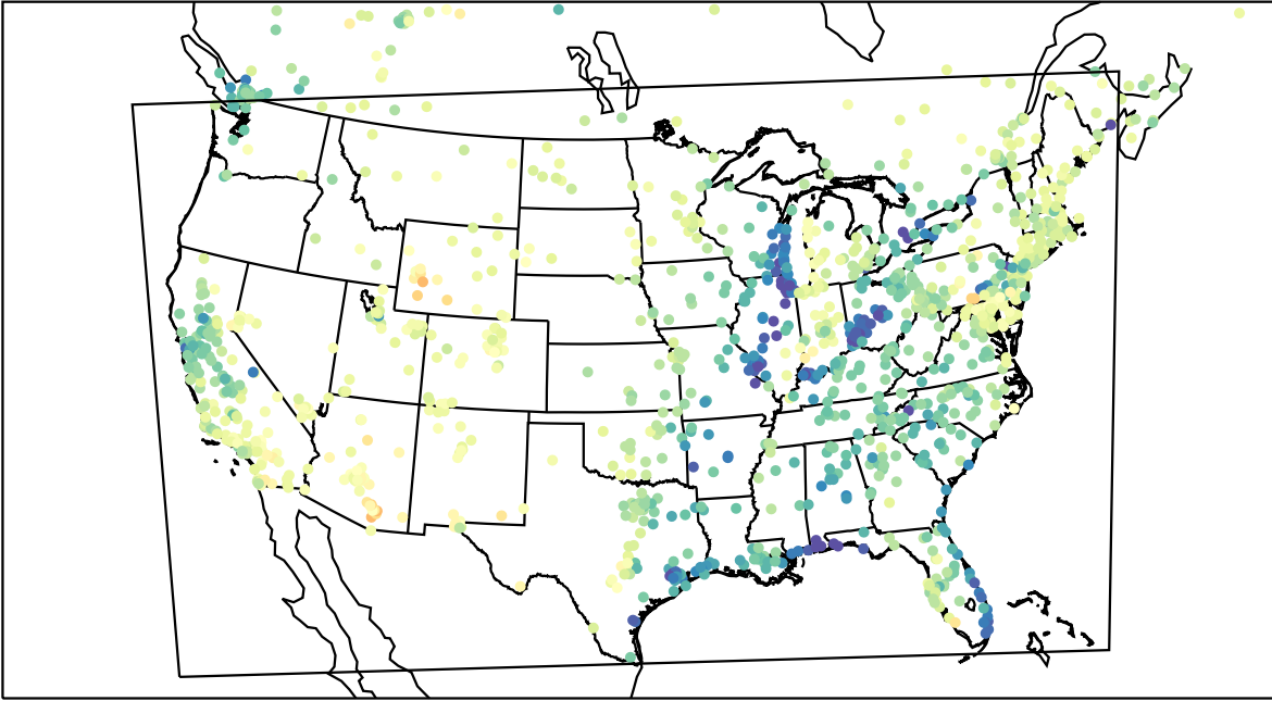
AirNOW (2023-04-05_18:00:00)
