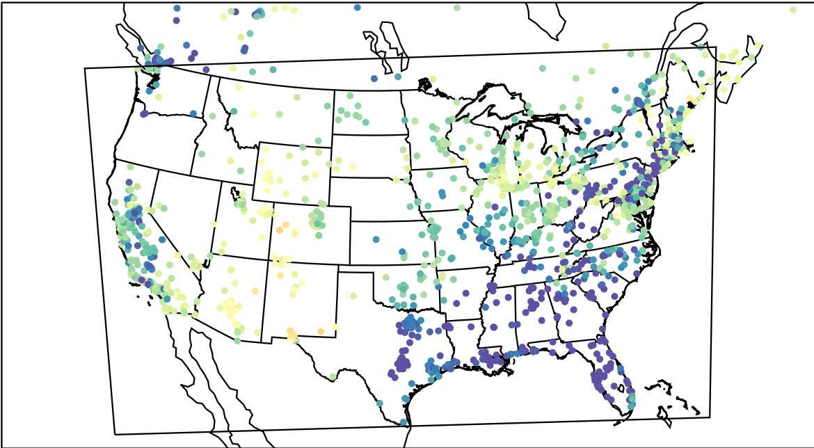
AirNOW (2023-04-04_07:00:00)
