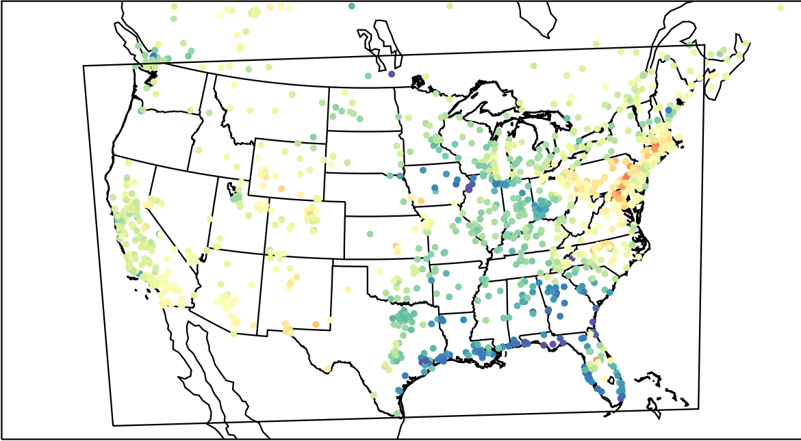
AirNOW (2023-04-04_21:00:00)
