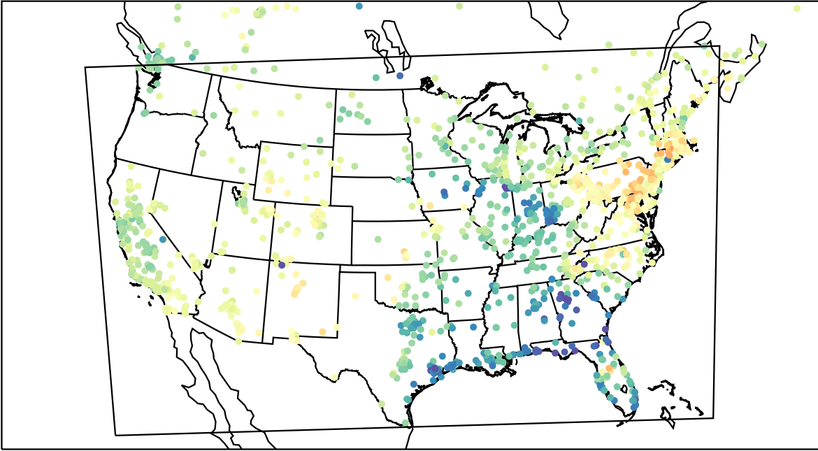
AirNOW (2023-04-04_19:00:00)
