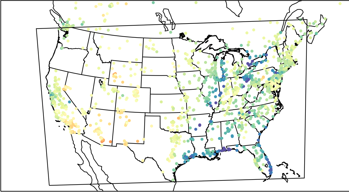
AirNOW (2023-04-05_21:00:00)
