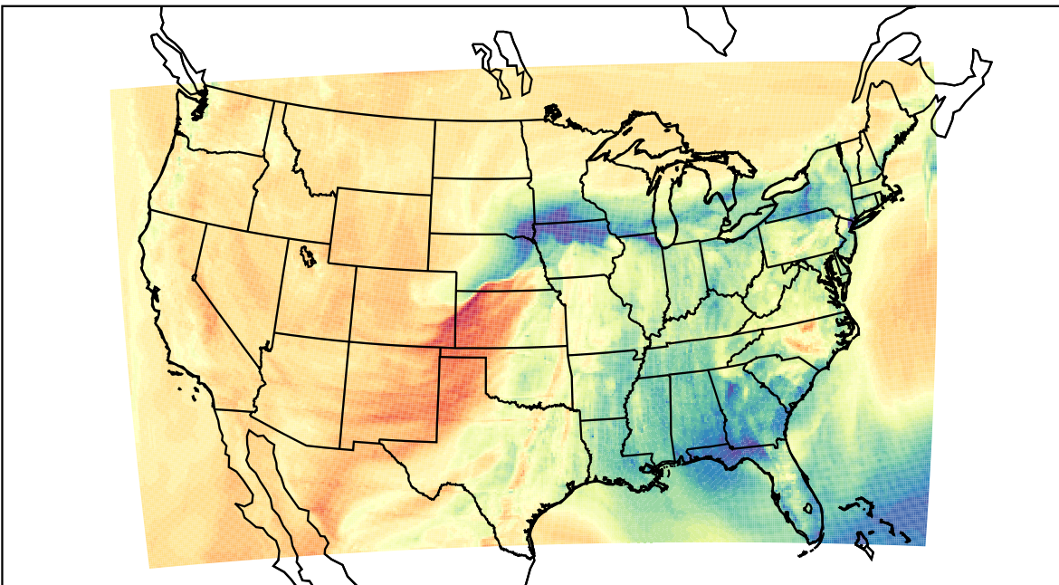
WRF (2023-04-05_00:00:00)
