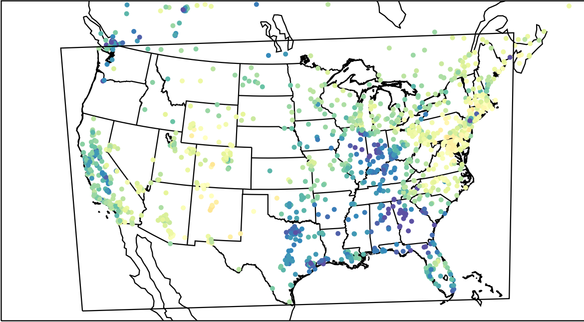
AirNOW (2023-04-04_16:00:00)
