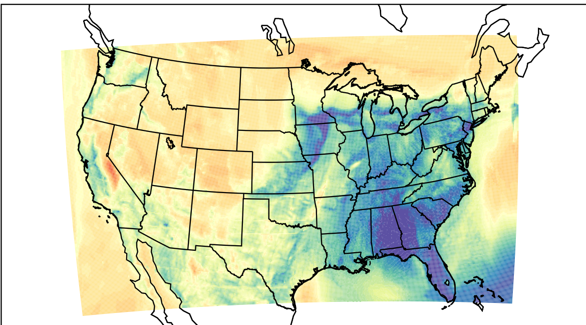
WRF (2023-04-05_08:00:00)
