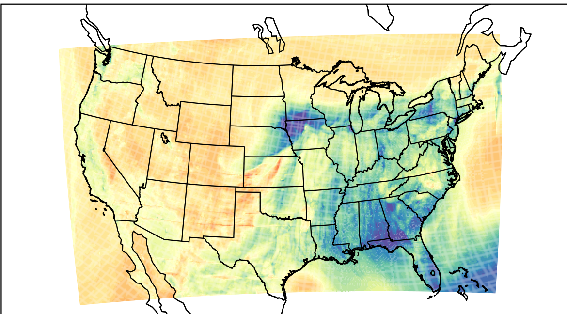
WRF (2023-04-05_02:00:00)
