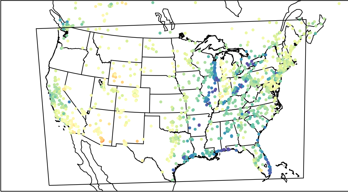
AirNOW (2023-04-05_19:00:00)
