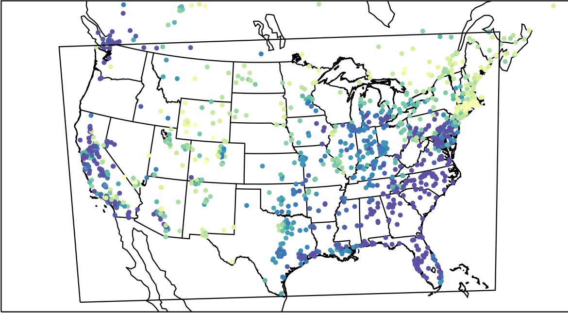
AirNOW (2023-04-05_10:00:00)
