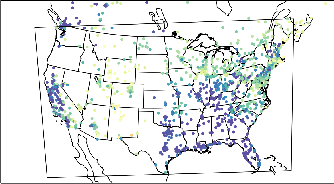
AirNOW (2023-04-04_13:00:00)
