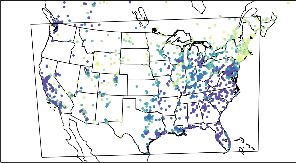
AirNOW (2023-04-05_12:00:00)
