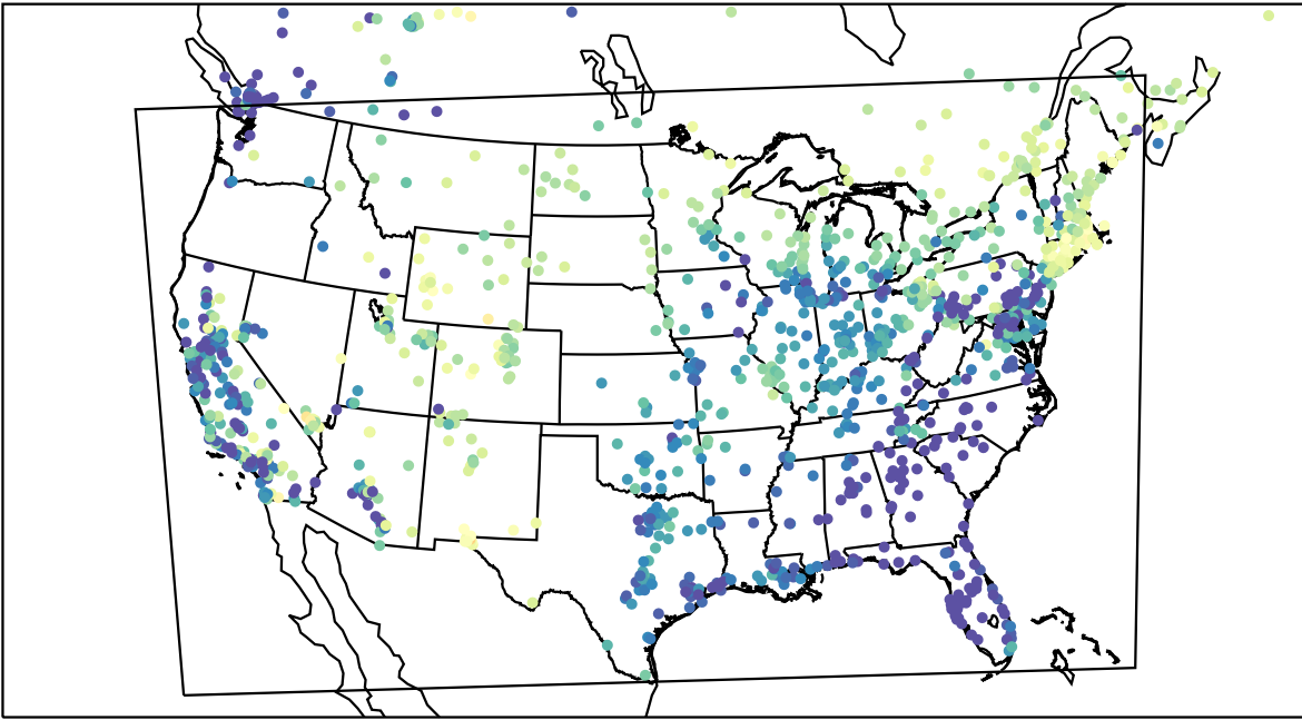
AirNOW (2023-04-05_08:00:00)
