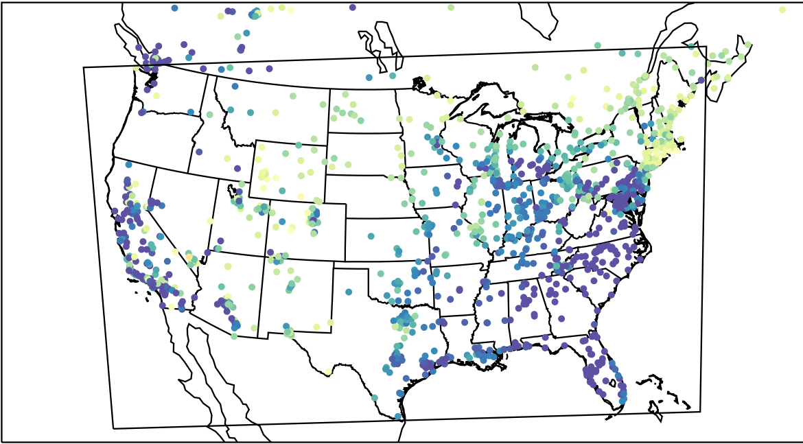
AirNOW (2023-04-05_11:00:00)
