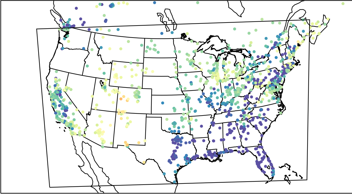
AirNOW (2023-04-04_08:00:00)
