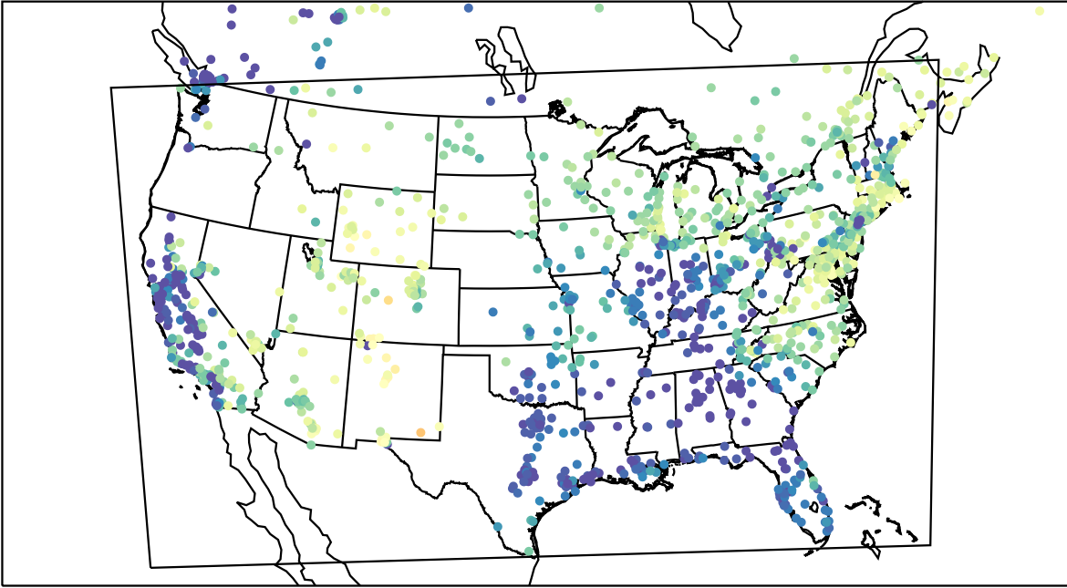
AirNOW (2023-04-04_14:00:00)
