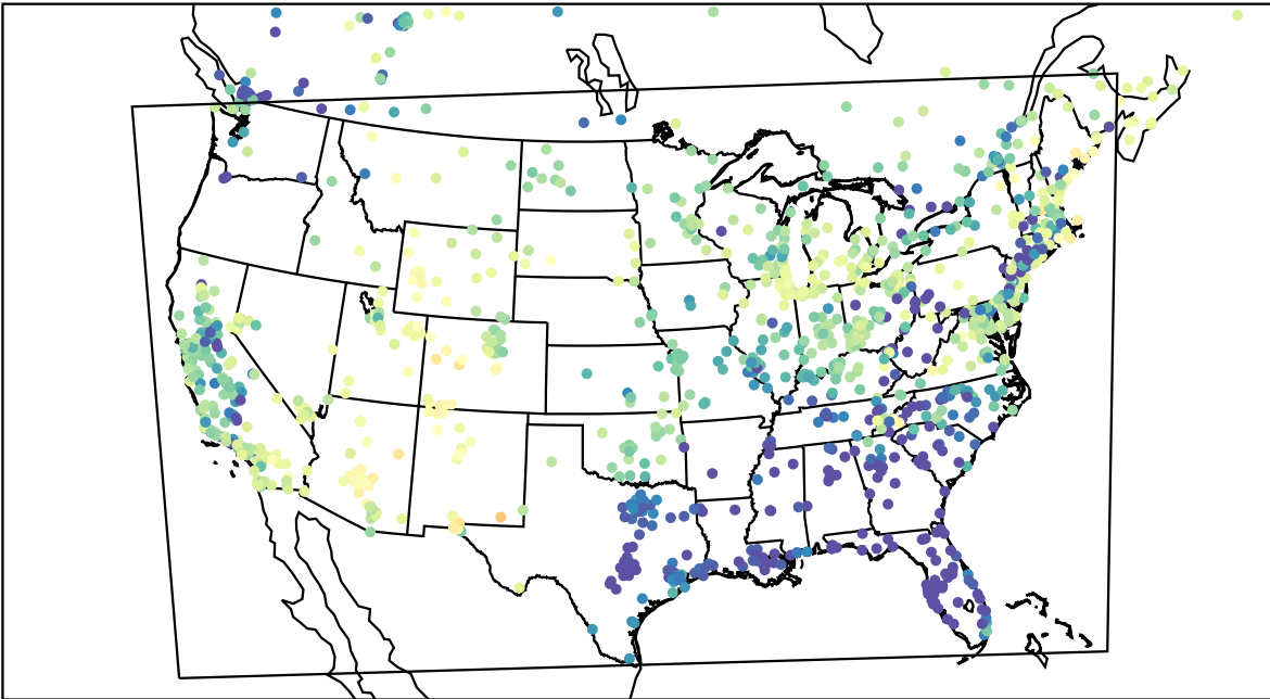
AirNOW (2023-04-04_06:00:00)
