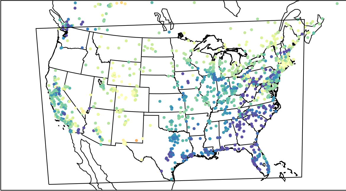
AirNOW (2023-04-05_04:00:00)
