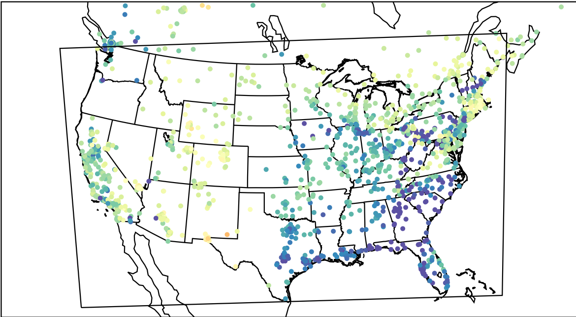
AirNOW (2023-04-05_03:00:00)
