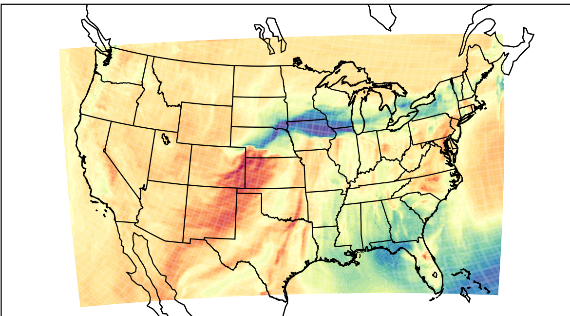
WRF (2023-04-04_21:00:00)
