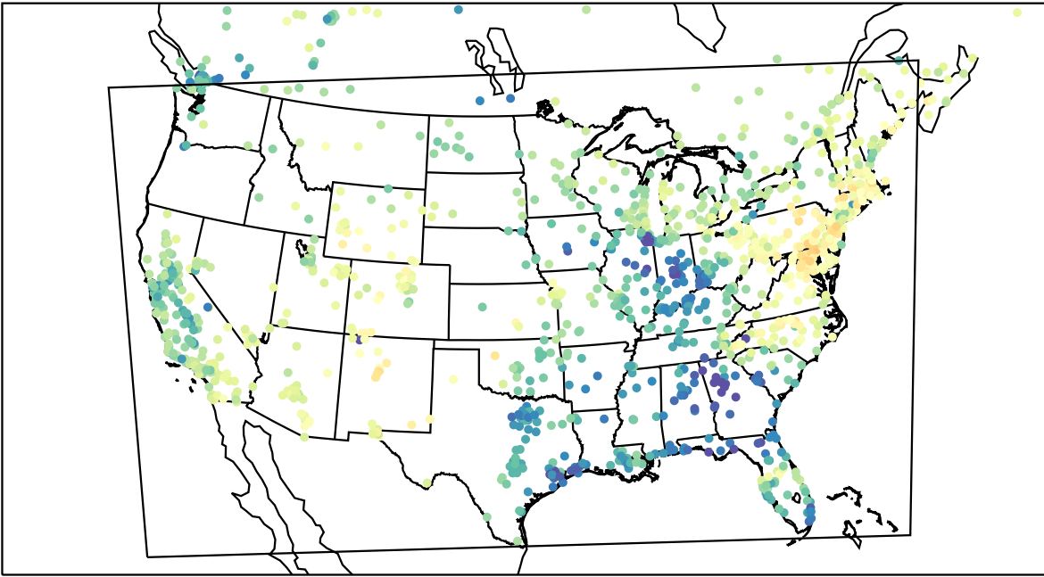
AirNOW (2023-04-04_17:00:00)
