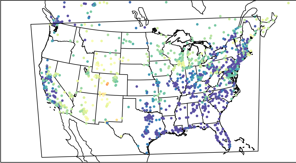
AirNOW (2023-04-04_11:00:00)
