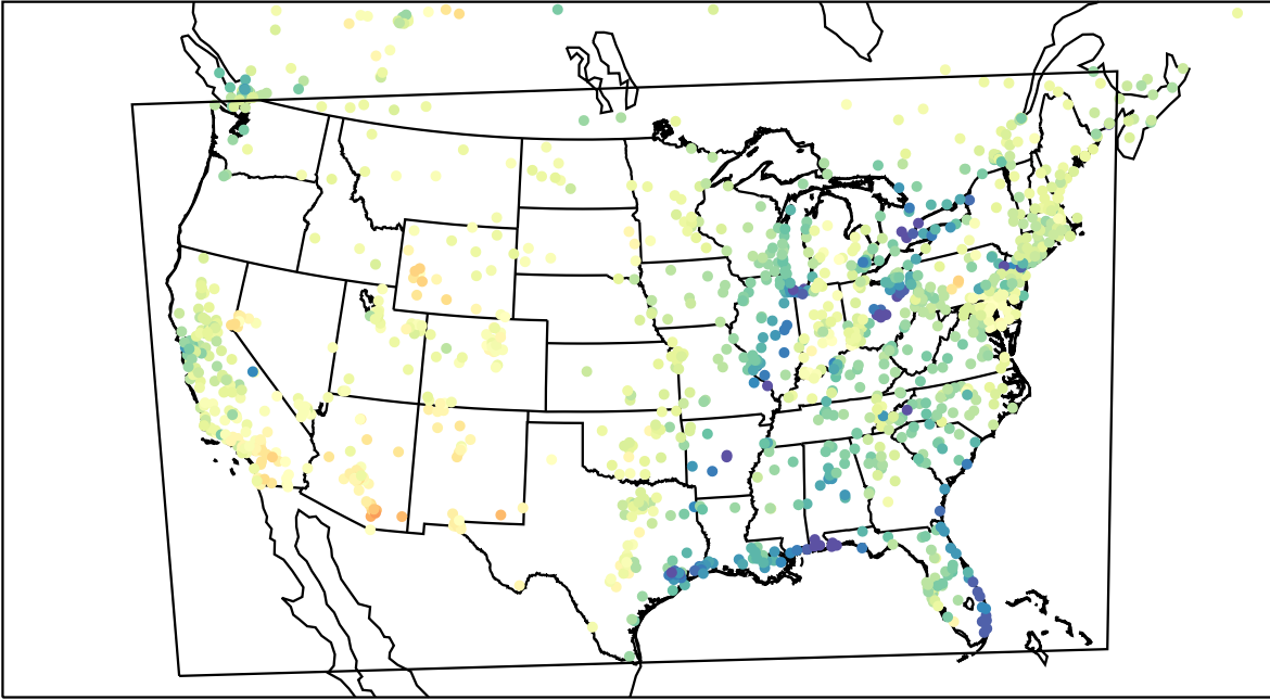
AirNOW (2023-04-05_20:00:00)
