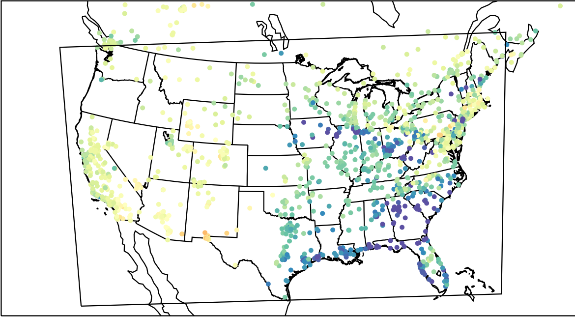
AirNOW (2023-04-05_00:00:00)
