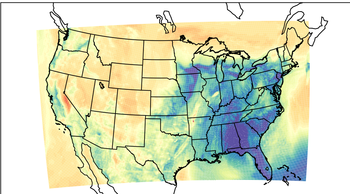
WRF (2023-04-05_09:00:00)
