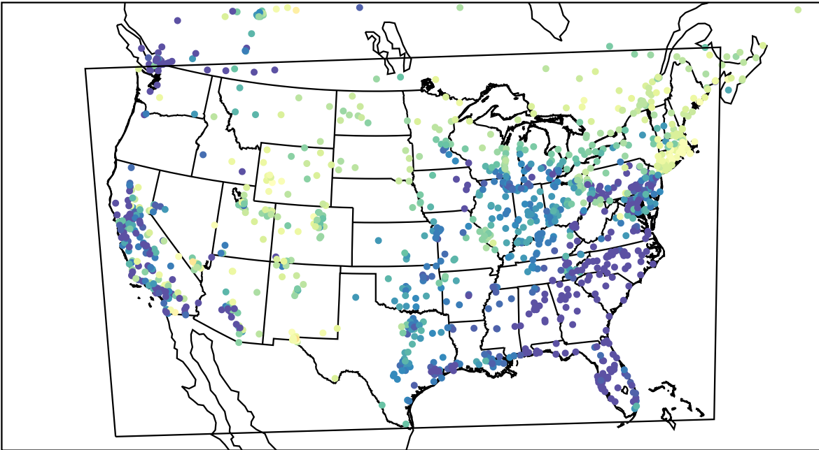
AirNOW (2023-04-05_09:00:00)
