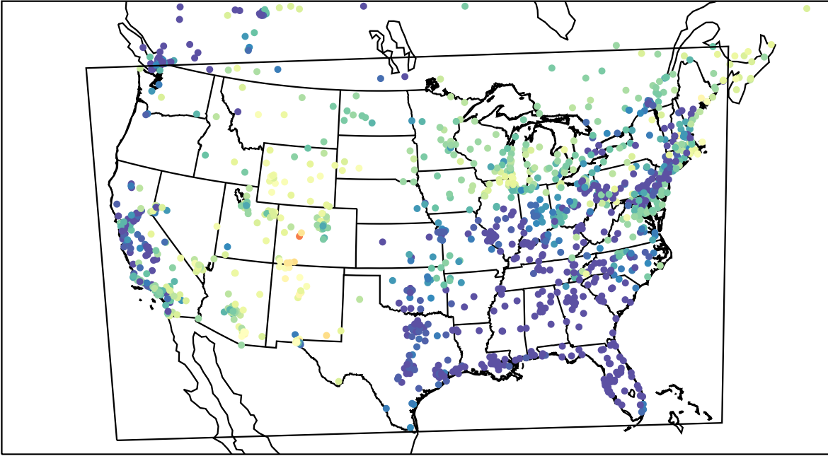
AirNOW (2023-04-04_12:00:00)
