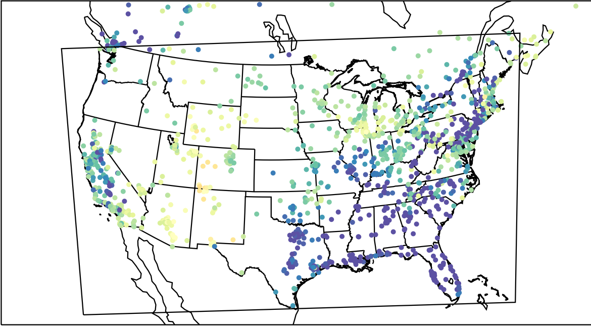
AirNOW (2023-04-04_09:00:00)
