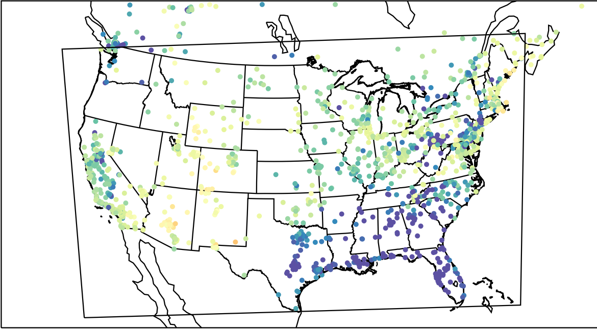
AirNOW (2023-04-04_05:00:00)
