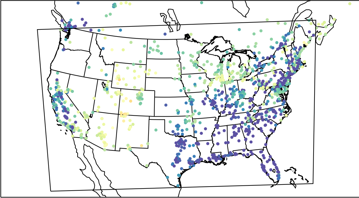
AirNOW (2023-04-04_10:00:00)
