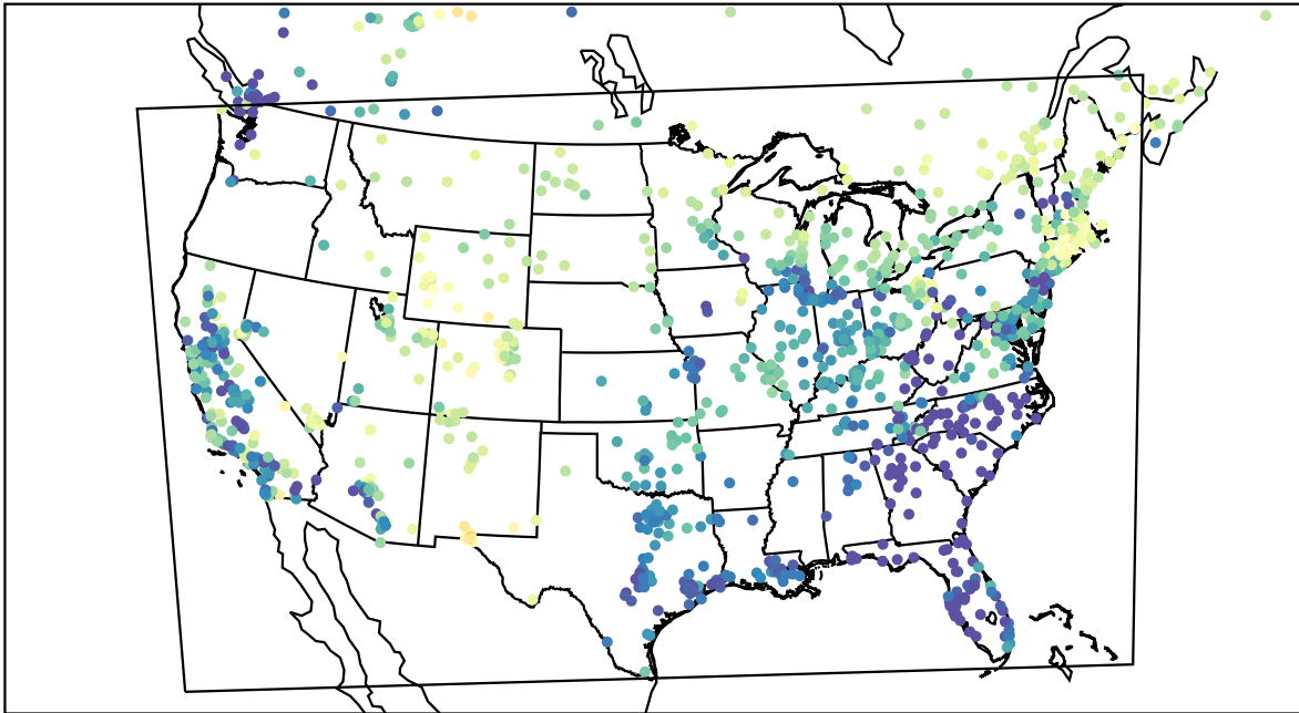
AirNOW (2023-04-05_06:00:00)
