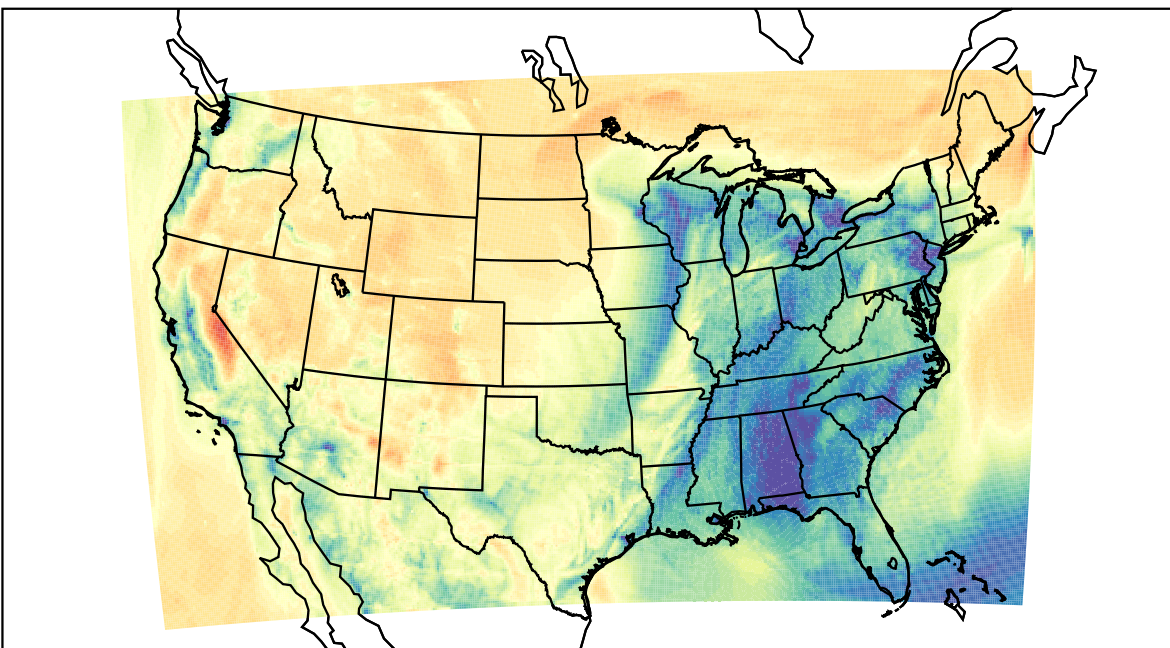
WRF (2023-04-05_14:00:00)
