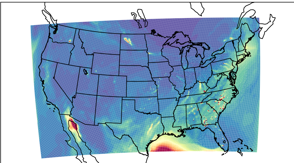
WRF 2023-04-06_21:00:00
