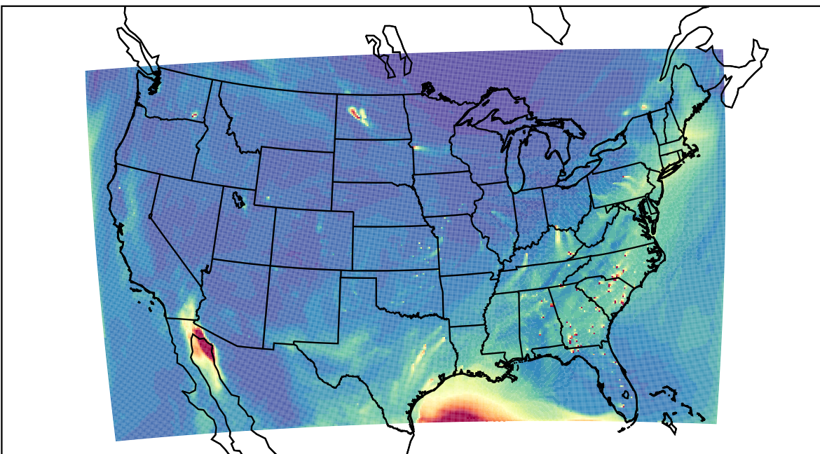
WRF 2023-04-06_20:00:00
