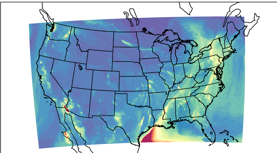
WRF 2023-04-06_06:00:00
