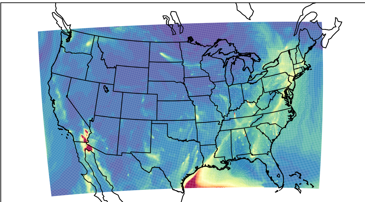
WRF 2023-04-06_09:00:00
