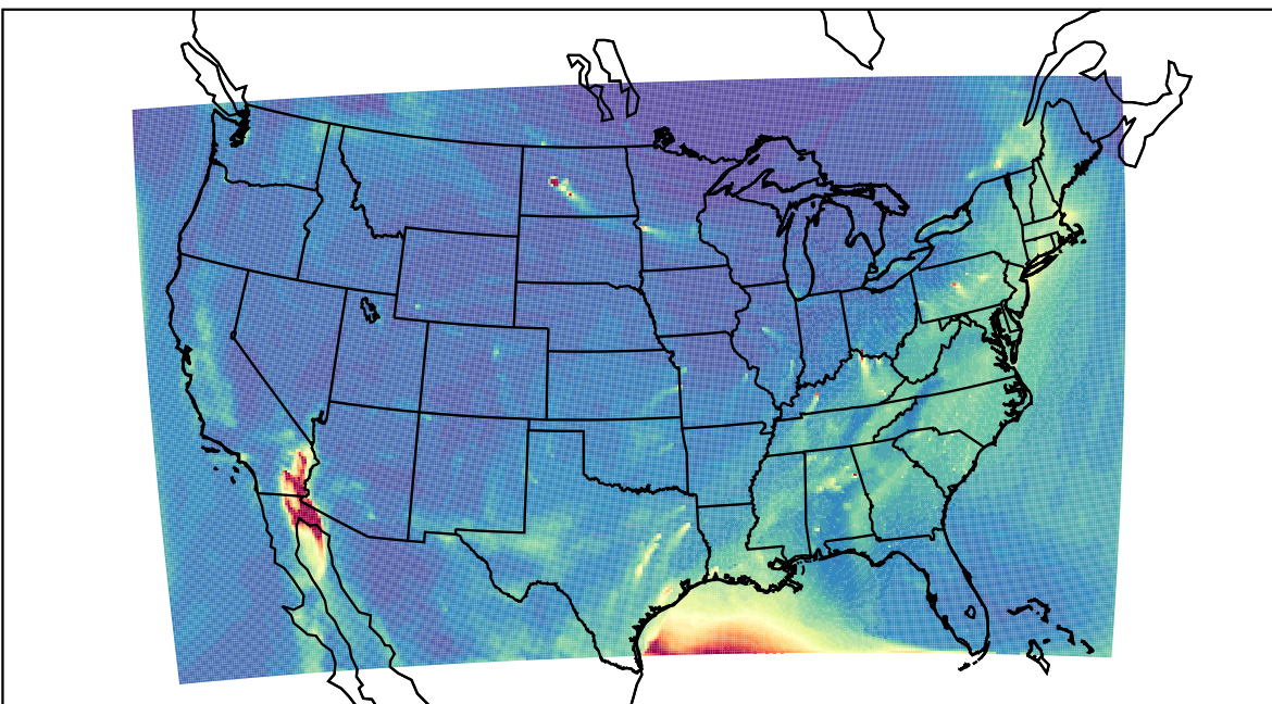
WRF 2023-04-06_16:00:00
