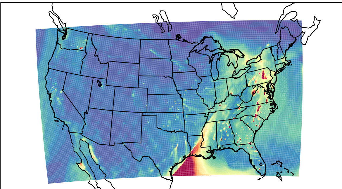
WRF 2023-04-06_01:00:00
