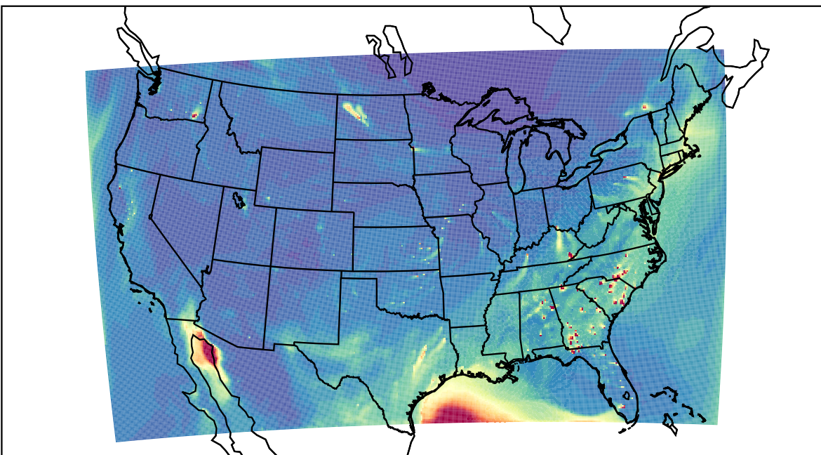
WRF 2023-04-06_22:00:00
