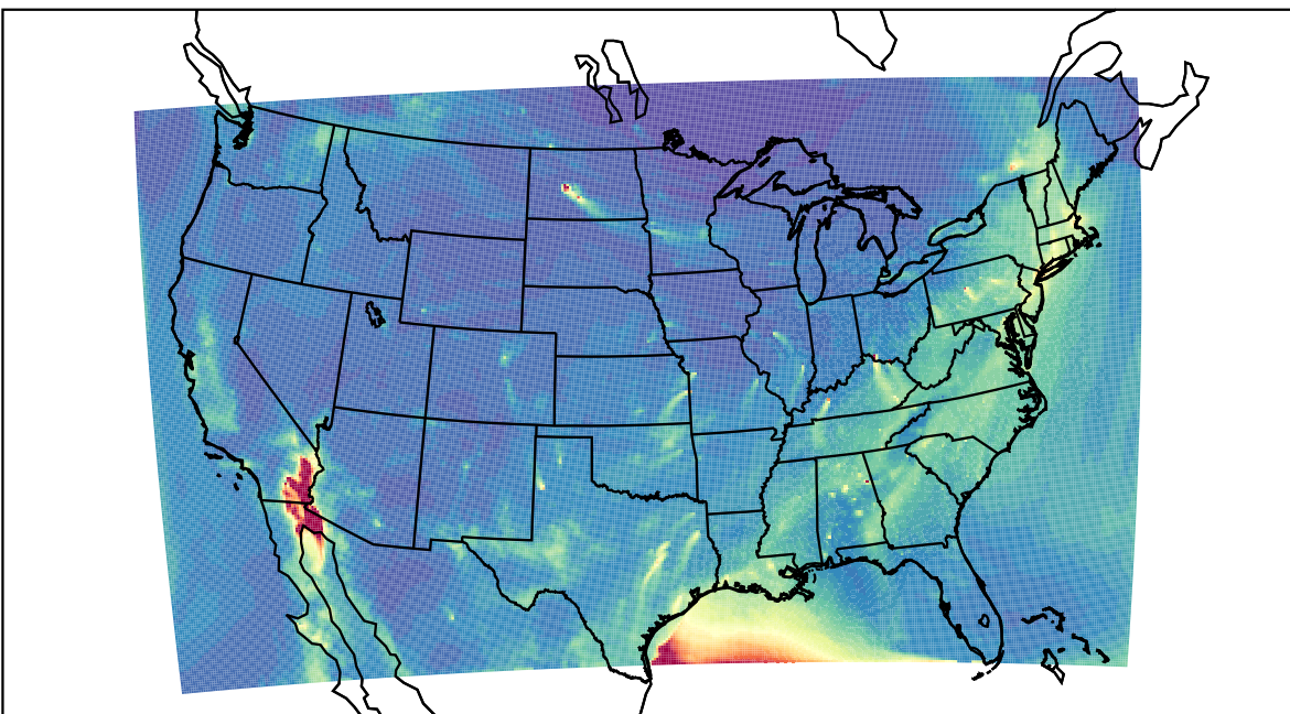
WRF 2023-04-06_14:00:00
