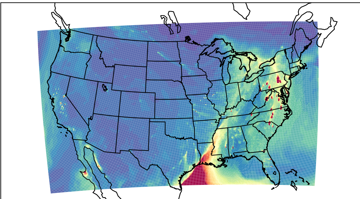
WRF 2023-04-06_00:00:00
