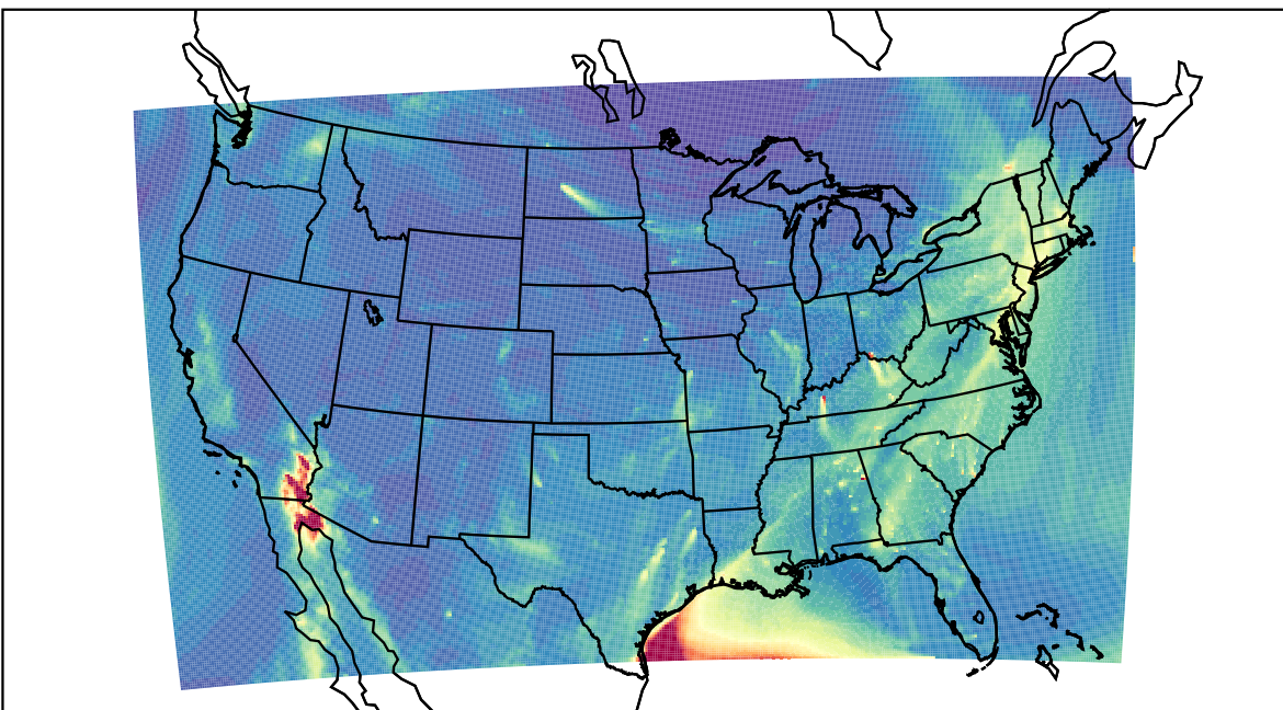
WRF 2023-04-06_11:00:00
