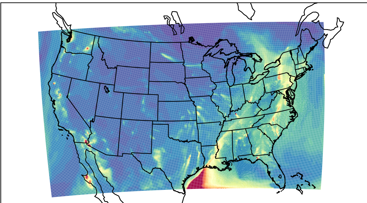
WRF 2023-04-06_05:00:00
