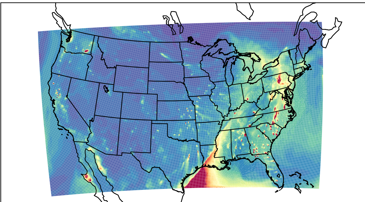
WRF 2023-04-06_02:00:00
