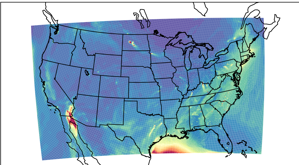
WRF 2023-04-06_17:00:00
