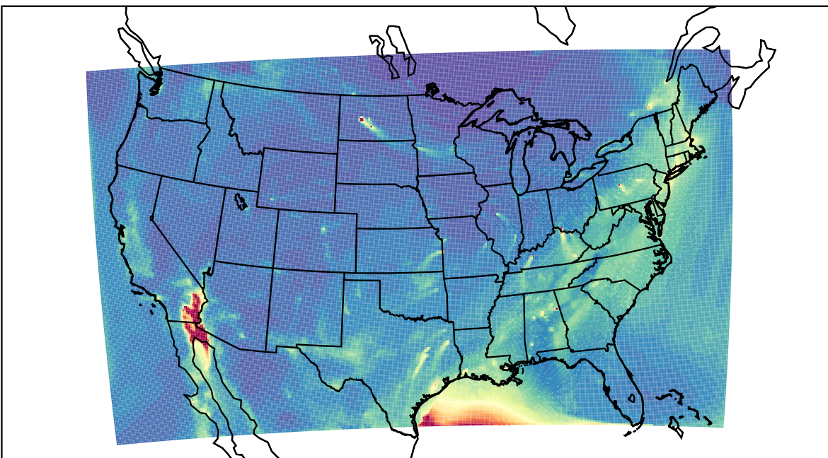
WRF 2023-04-06_15:00:00
