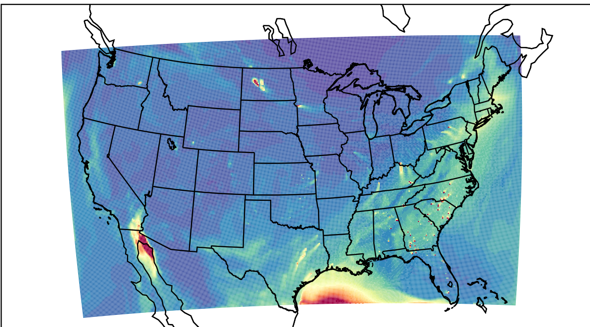
WRF 2023-04-06_19:00:00
