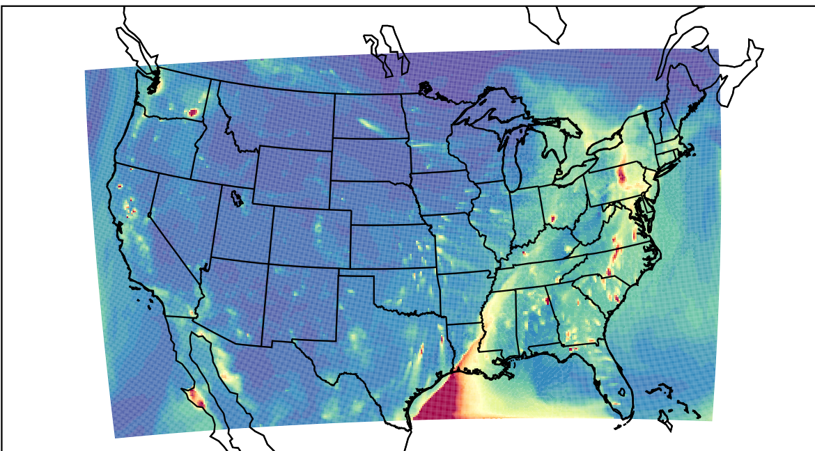
WRF 2023-04-06_03:00:00
