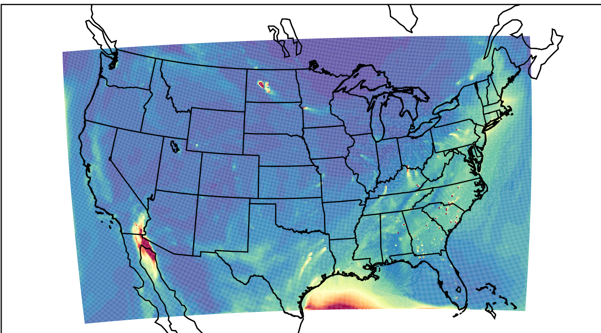
WRF 2023-04-06_18:00:00
