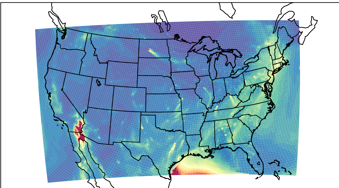
WRF 2023-04-06_13:00:00
