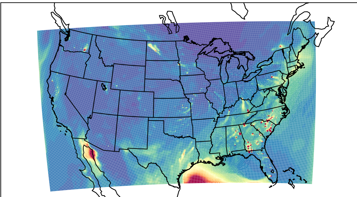
WRF 2023-04-06_23:00:00
