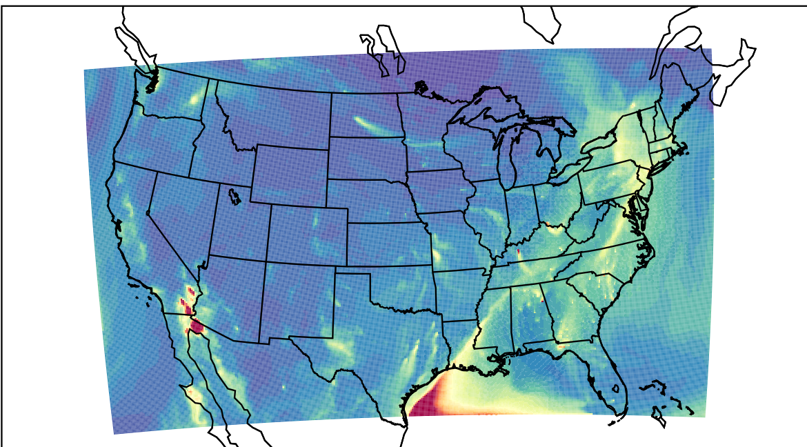
WRF 2023-04-06_08:00:00
