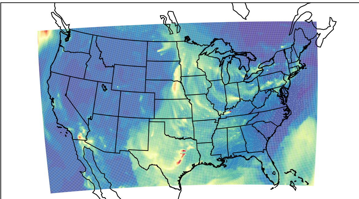
WRF 2023-04-09_10:00:00
