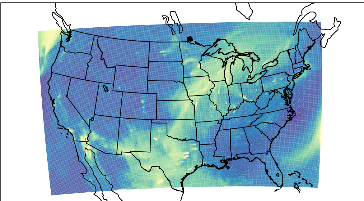
WRF 2023-04-10_16:00:00
