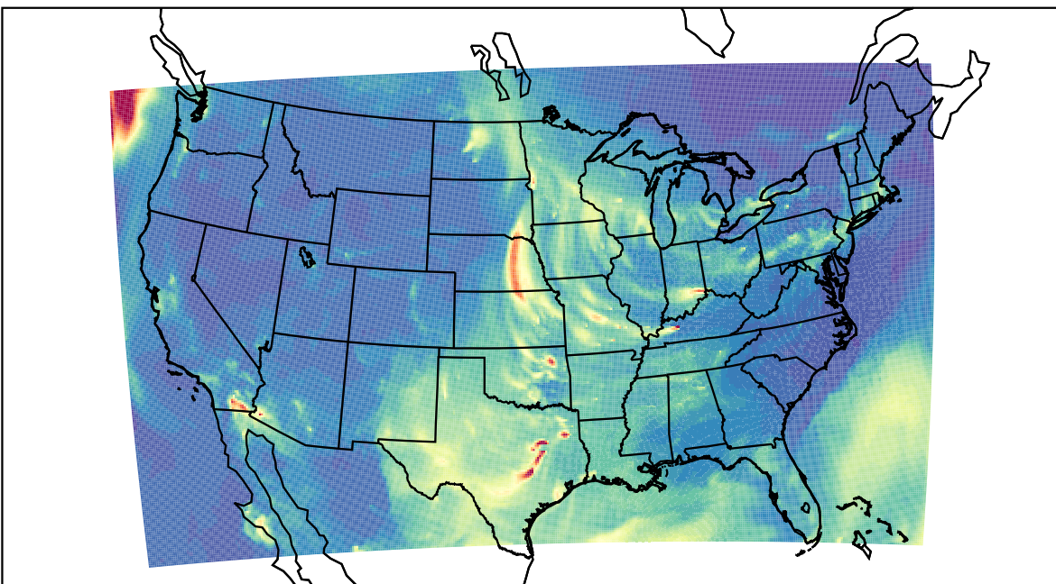
WRF 2023-04-09_07:00:00
