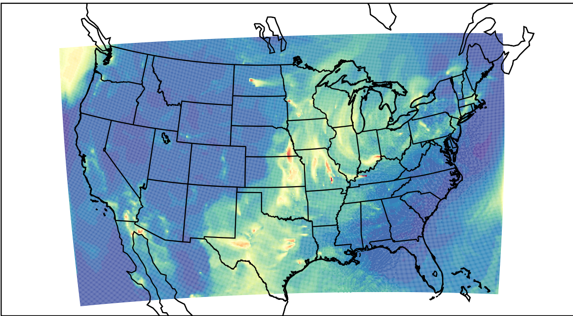
WRF 2023-04-10_07:00:00
