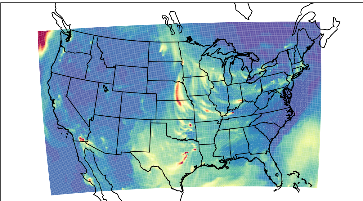
WRF 2023-04-09_06:00:00
