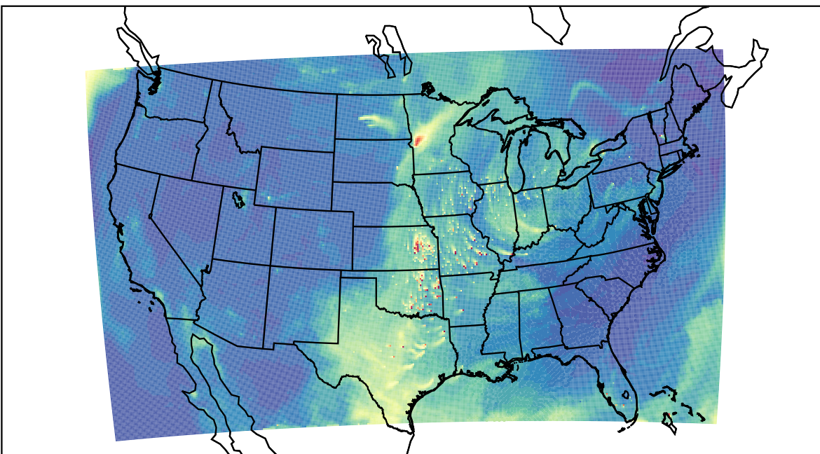
WRF 2023-04-09_21:00:00
