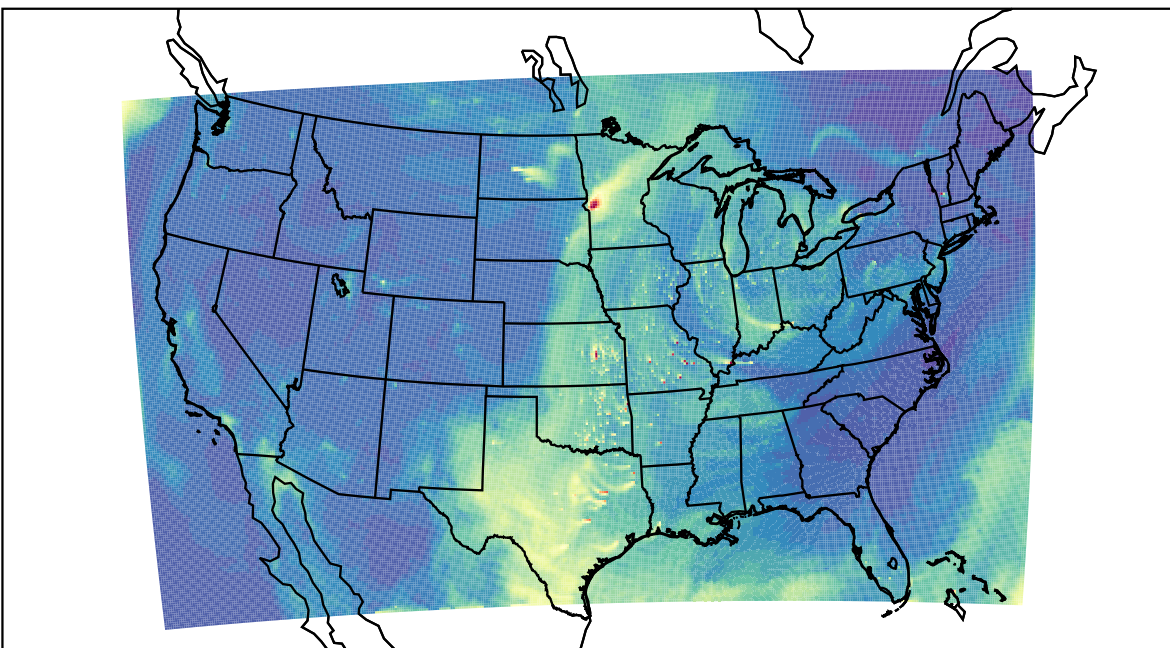
WRF 2023-04-09_19:00:00
