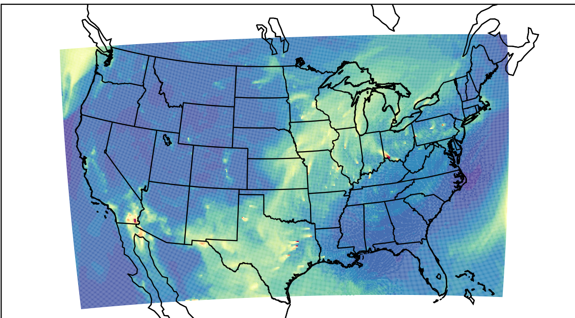
WRF 2023-04-10_15:00:00
