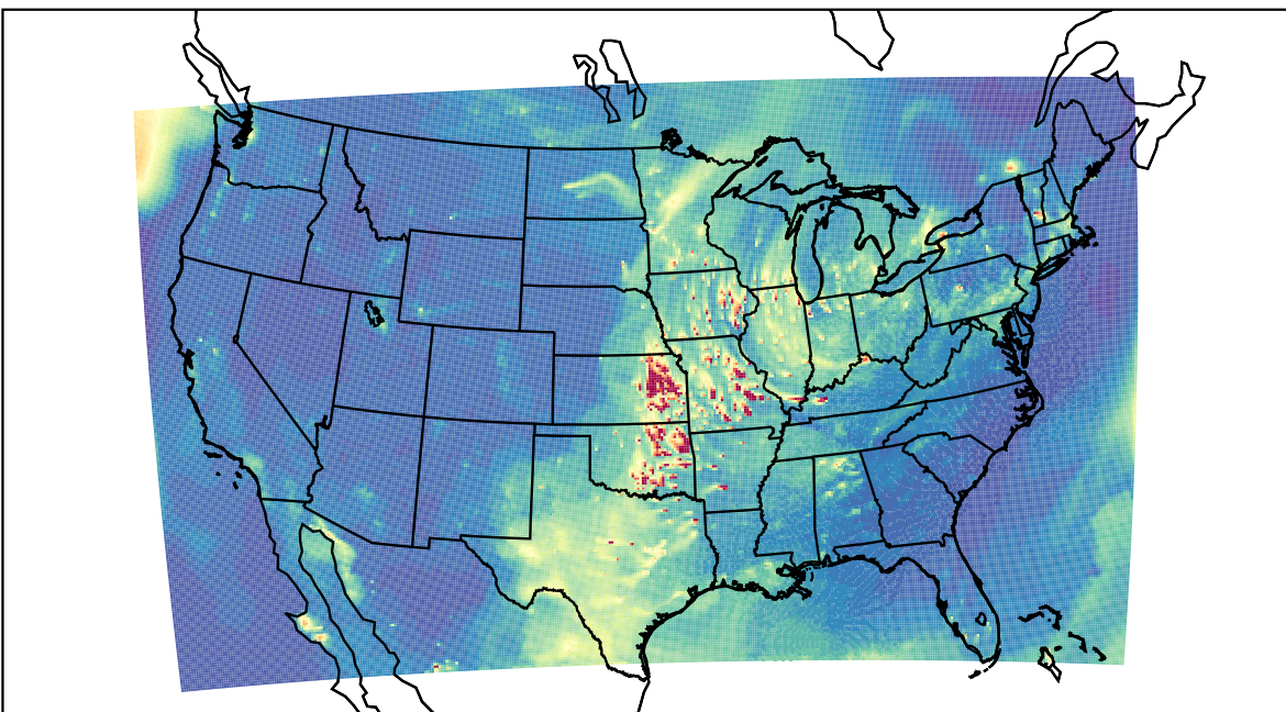
WRF 2023-04-10_01:00:00
