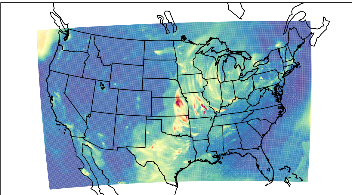
WRF 2023-04-10_04:00:00
