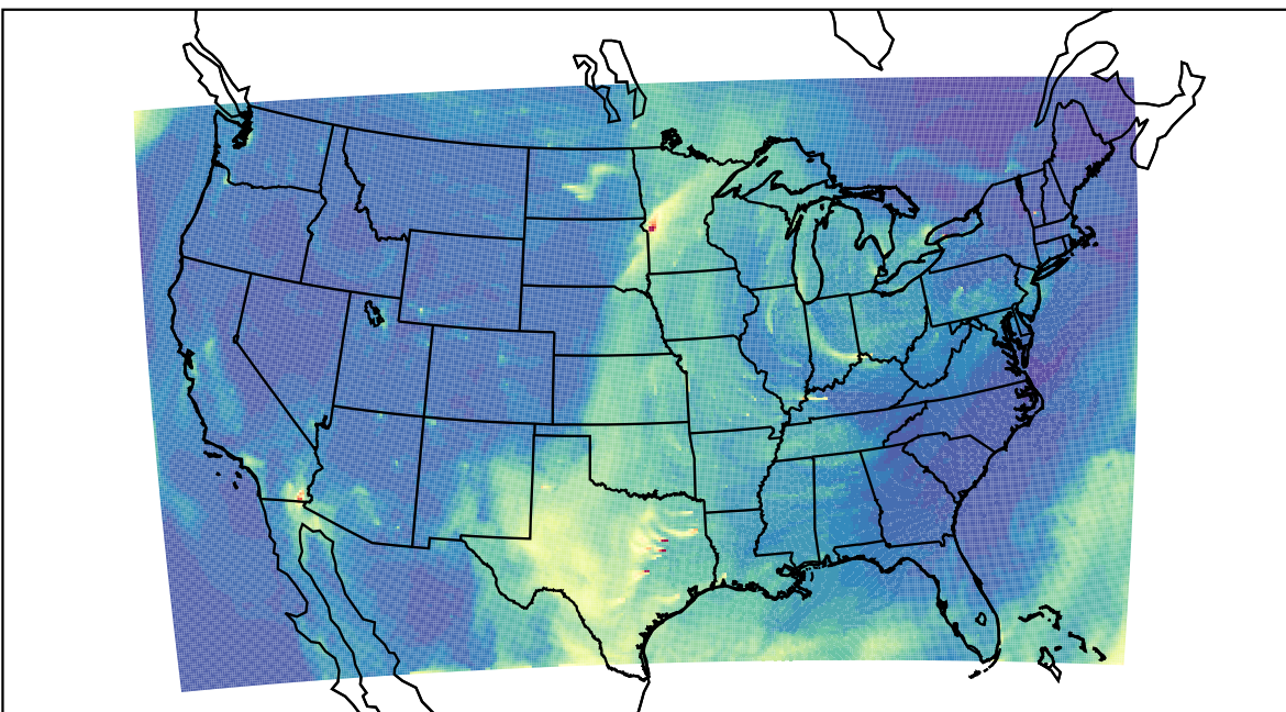
WRF 2023-04-09_17:00:00
