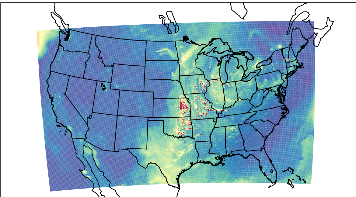
WRF 2023-04-10_00:00:00
