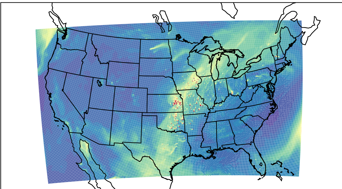
WRF 2023-04-10_21:00:00
