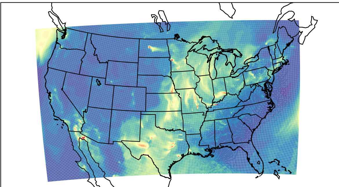
WRF 2023-04-10_08:00:00
