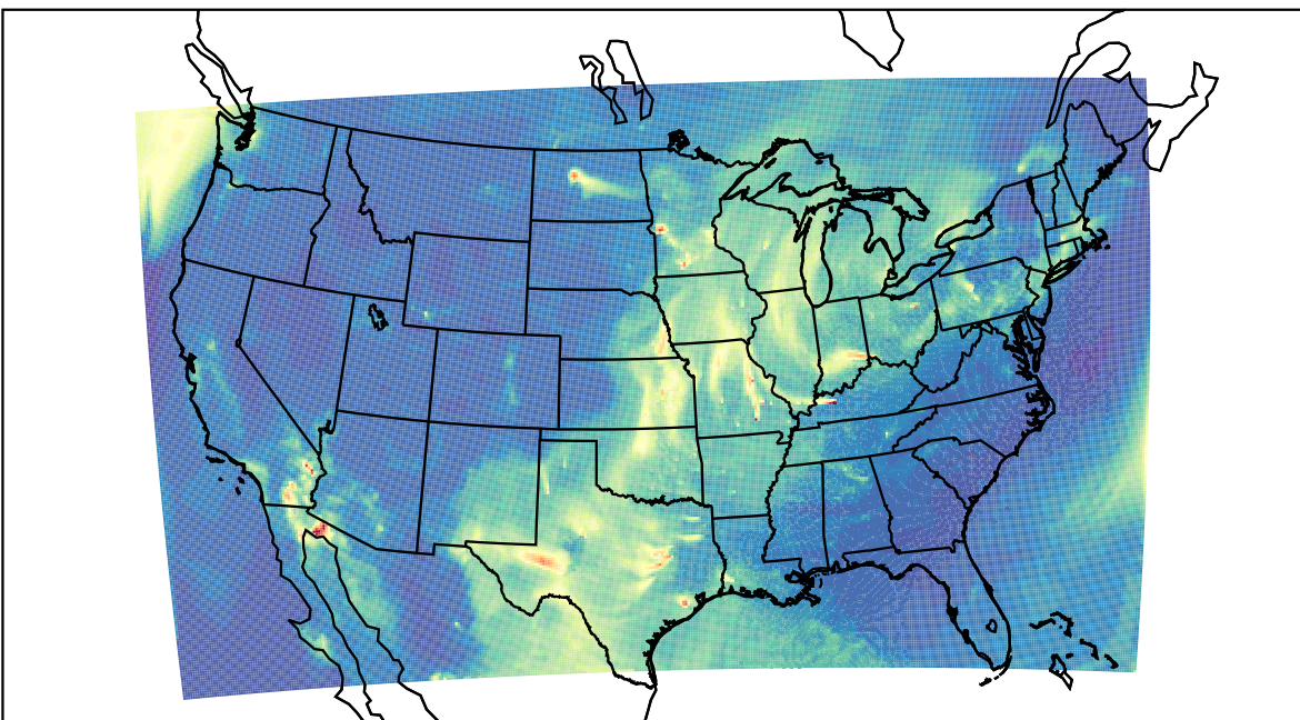
WRF 2023-04-10_09:00:00
