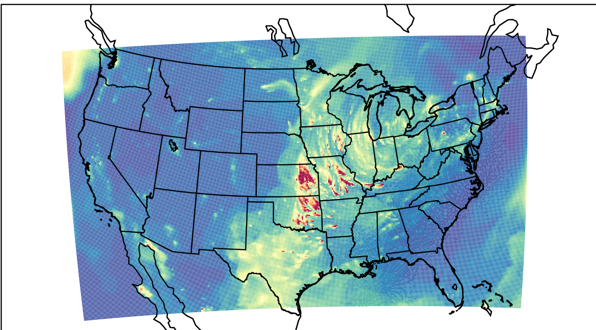
WRF 2023-04-10_02:00:00
