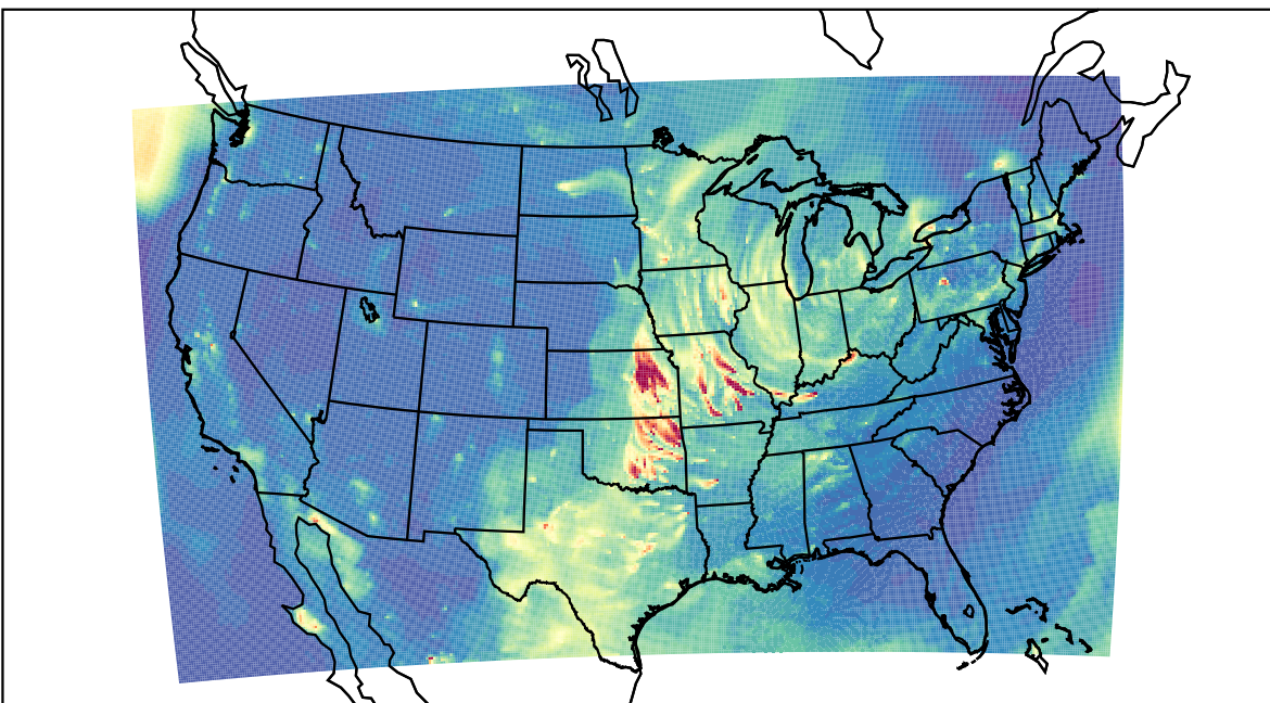
WRF 2023-04-10_03:00:00
