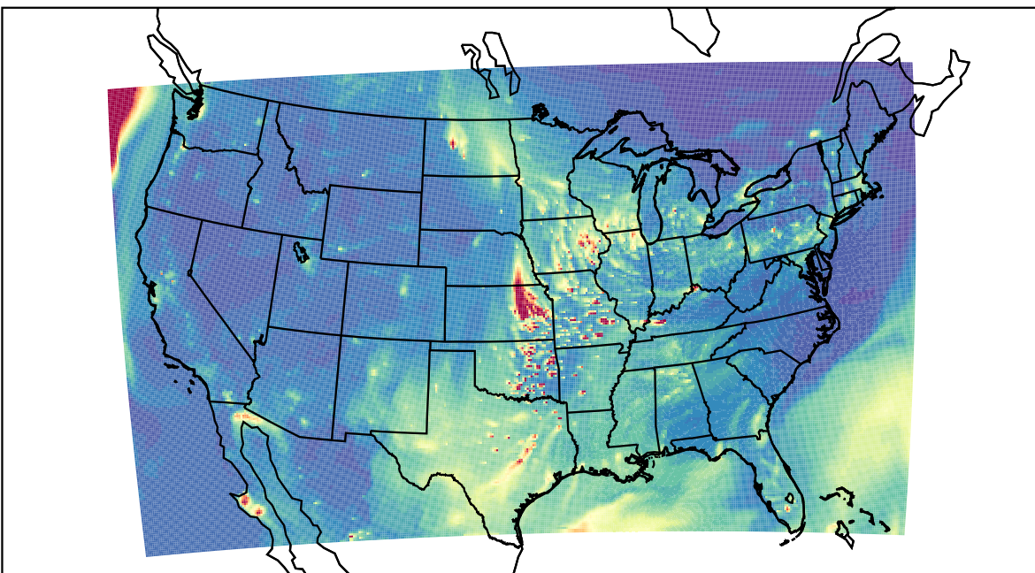
WRF 2023-04-09_02:00:00
