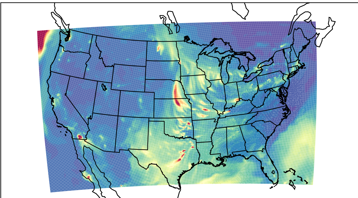
WRF 2023-04-09_05:00:00
