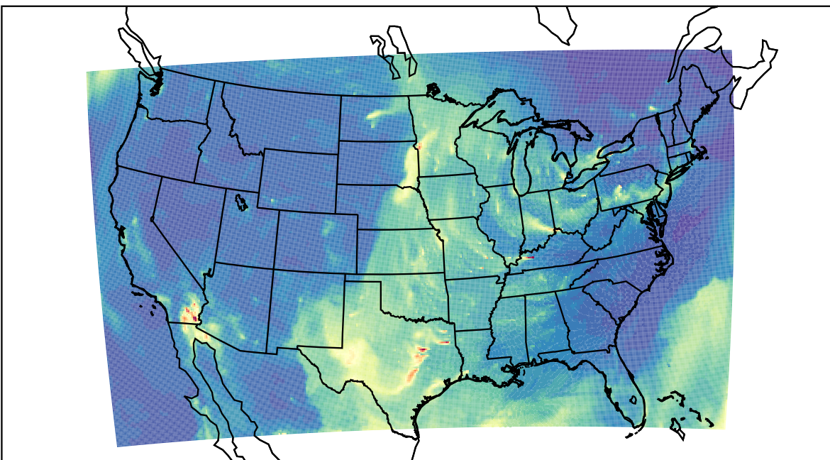
WRF 2023-04-09_13:00:00
