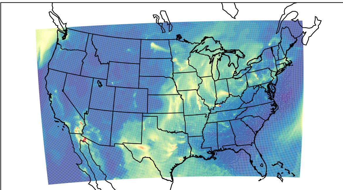
WRF 2023-04-10_10:00:00
