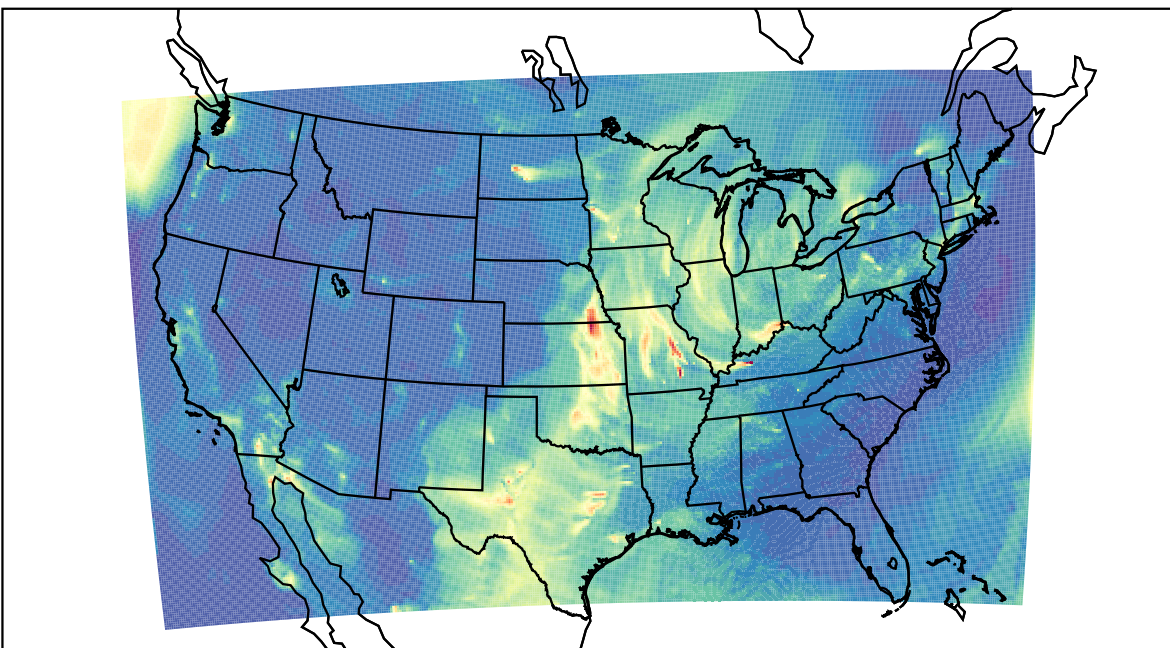
WRF 2023-04-10_06:00:00
