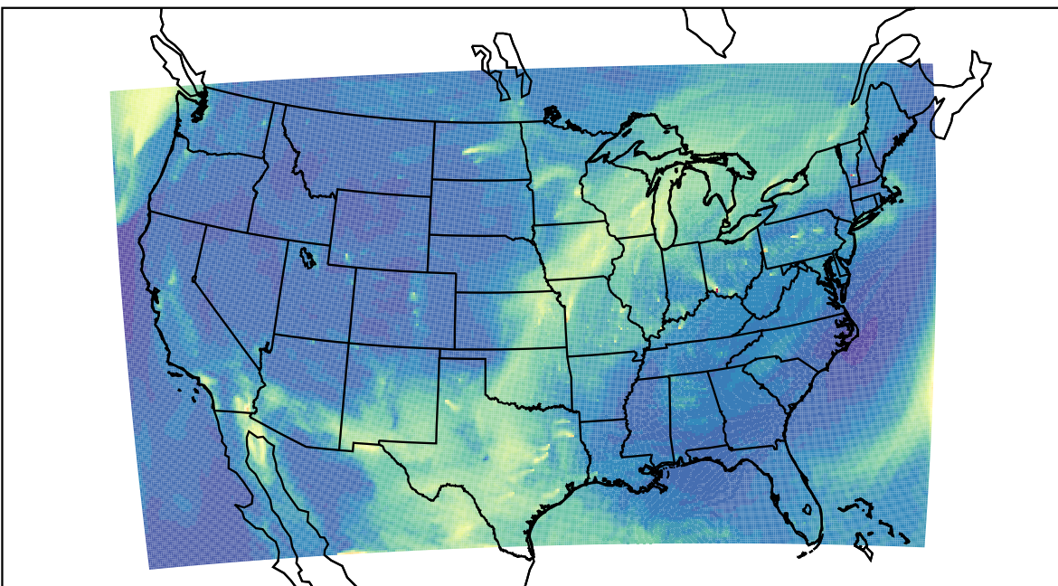
WRF 2023-04-10_17:00:00
