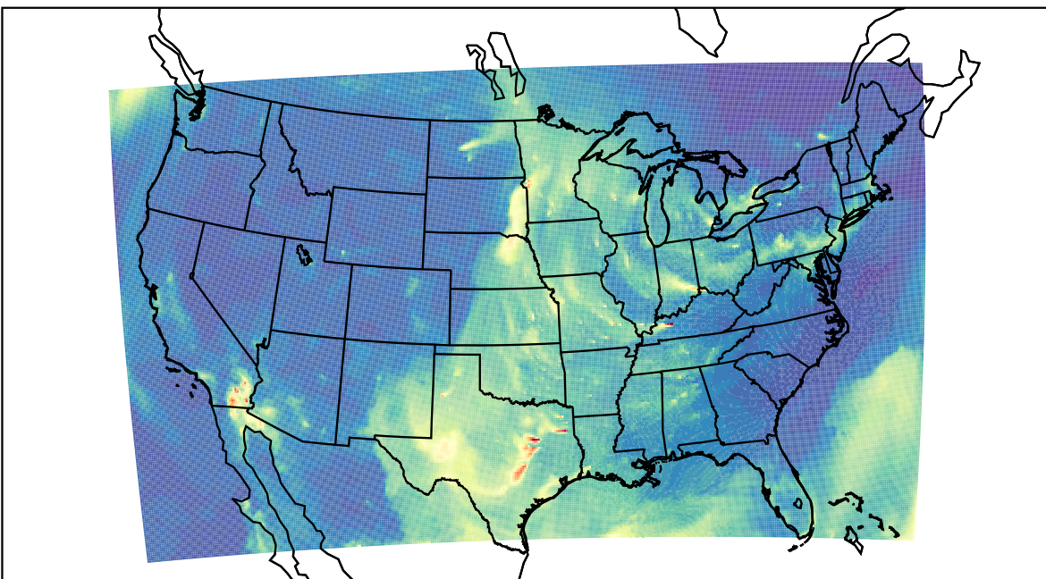
WRF 2023-04-09_12:00:00
