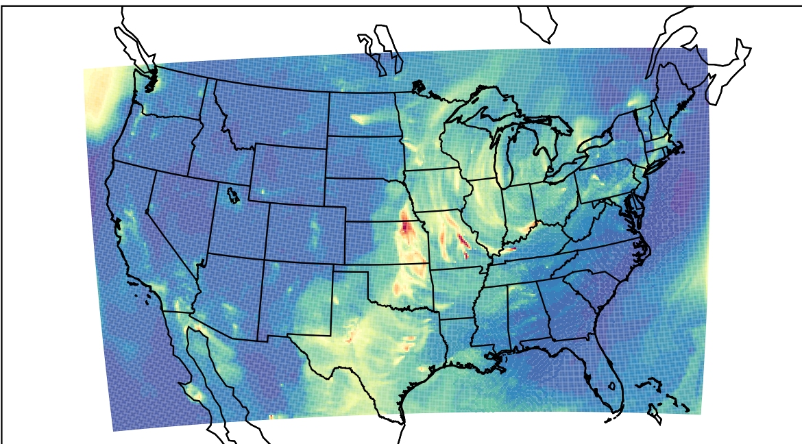
WRF 2023-04-10_05:00:00
