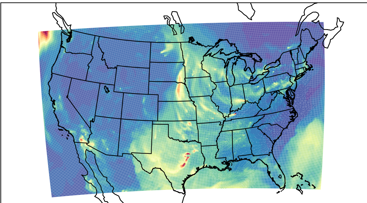
WRF 2023-04-09_09:00:00
