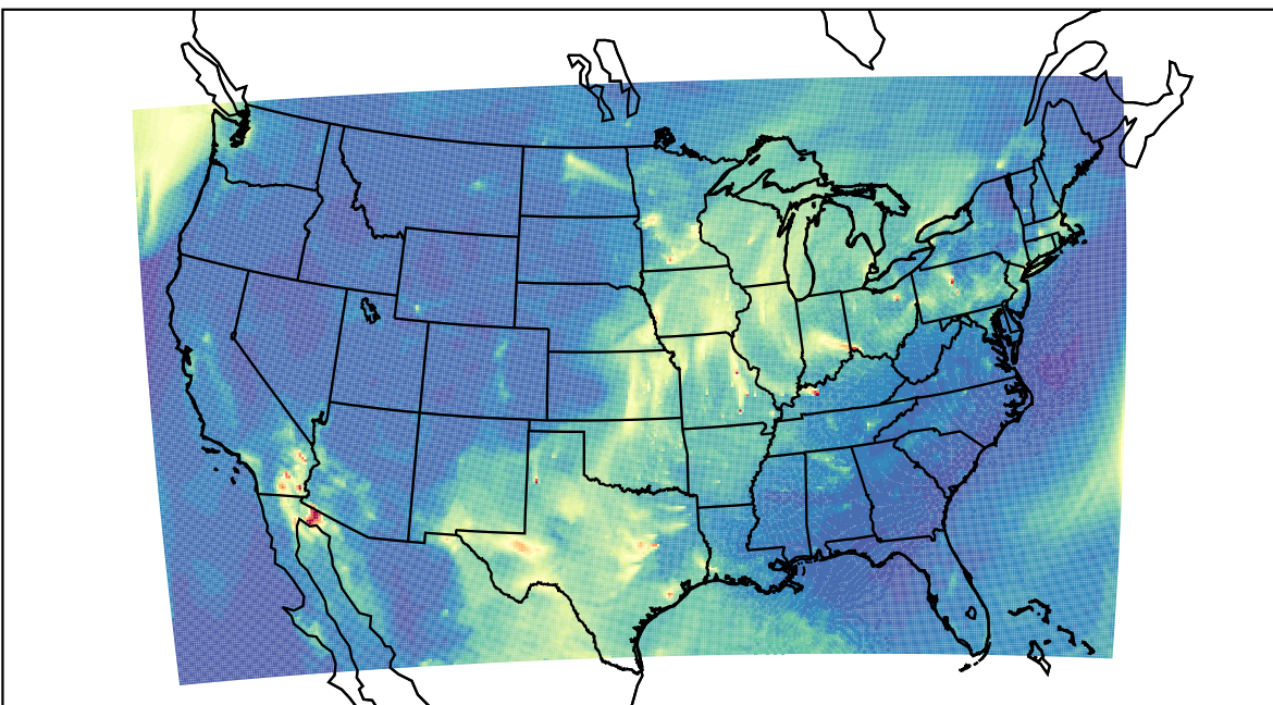
WRF 2023-04-10_11:00:00
