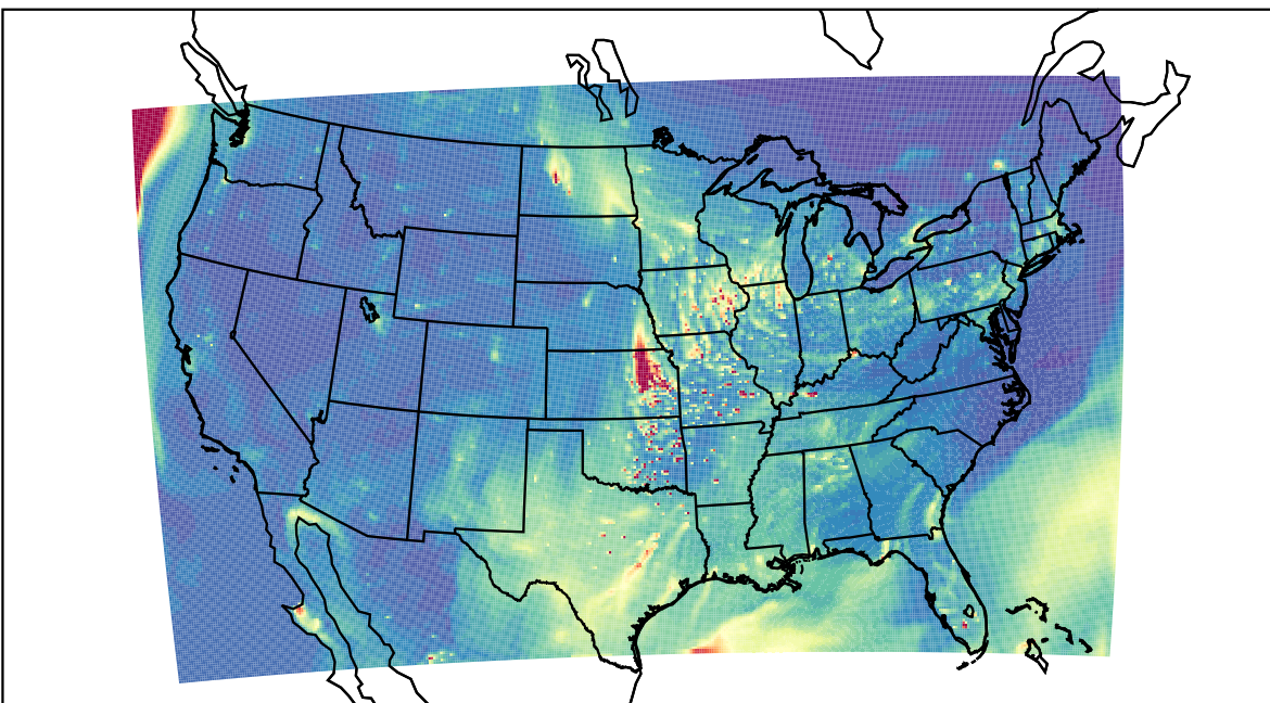
WRF 2023-04-09_01:00:00
