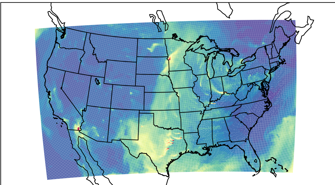
WRF 2023-04-09_16:00:00
