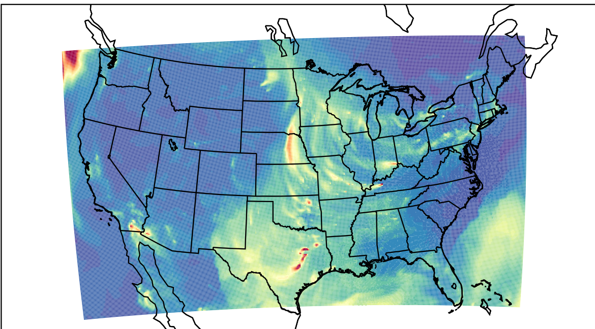
WRF 2023-04-09_08:00:00
