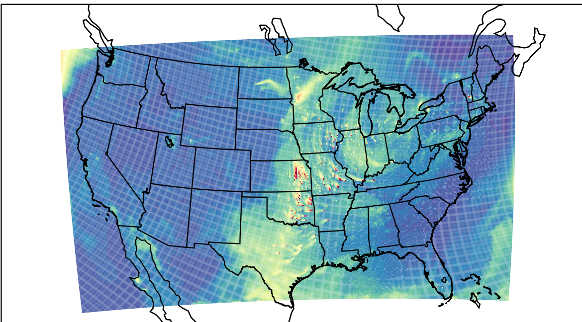
WRF 2023-04-09_23:00:00
