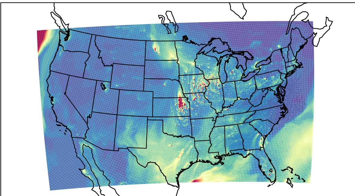
WRF 2023-04-09_00:00:00
