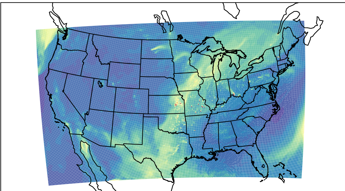
WRF 2023-04-10_19:00:00
