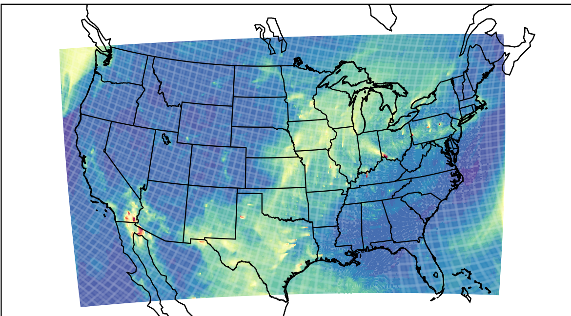
WRF 2023-04-10_14:00:00
