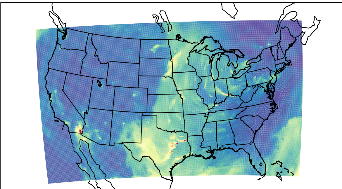
WRF 2023-04-09_15:00:00
