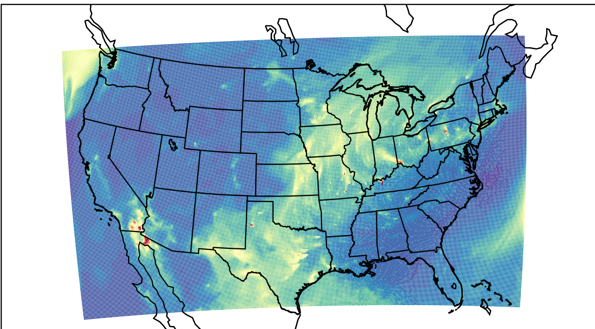
WRF 2023-04-10_13:00:00
