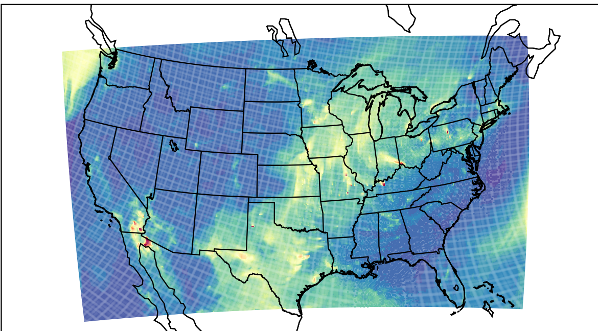
WRF 2023-04-10_12:00:00
