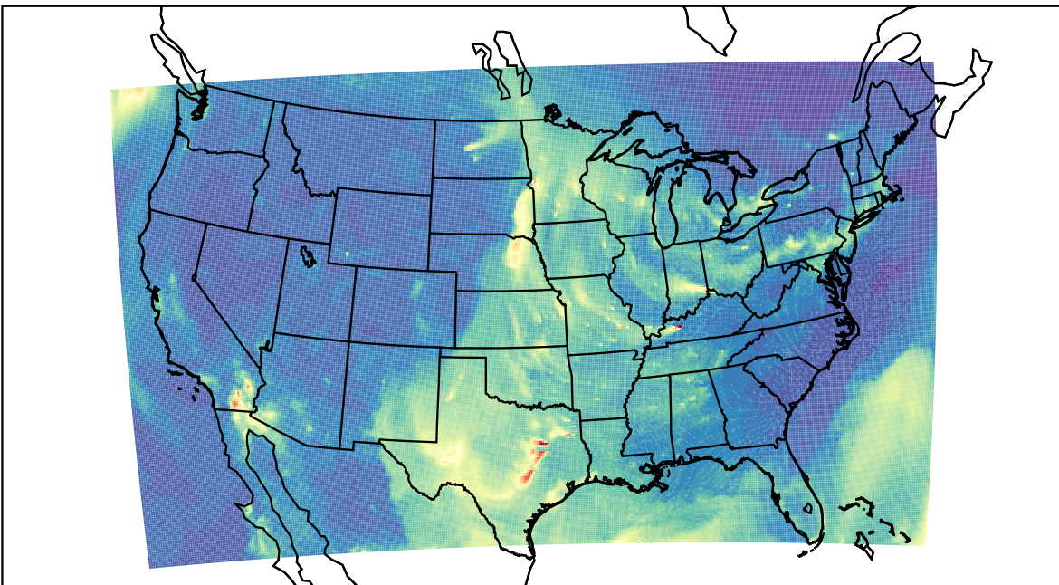
WRF 2023-04-09_11:00:00
