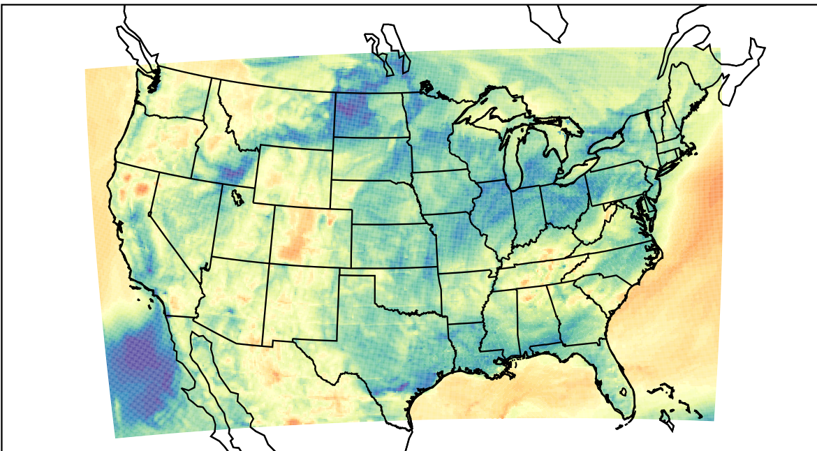
WRF (2023-04-12_07:00:00)
