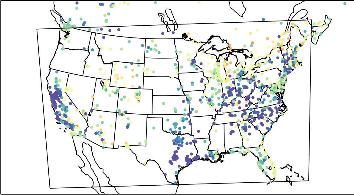
AirNOW (2023-04-11_06:00:00)
