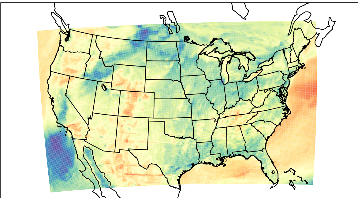
WRF (2023-04-12_02:00:00)
