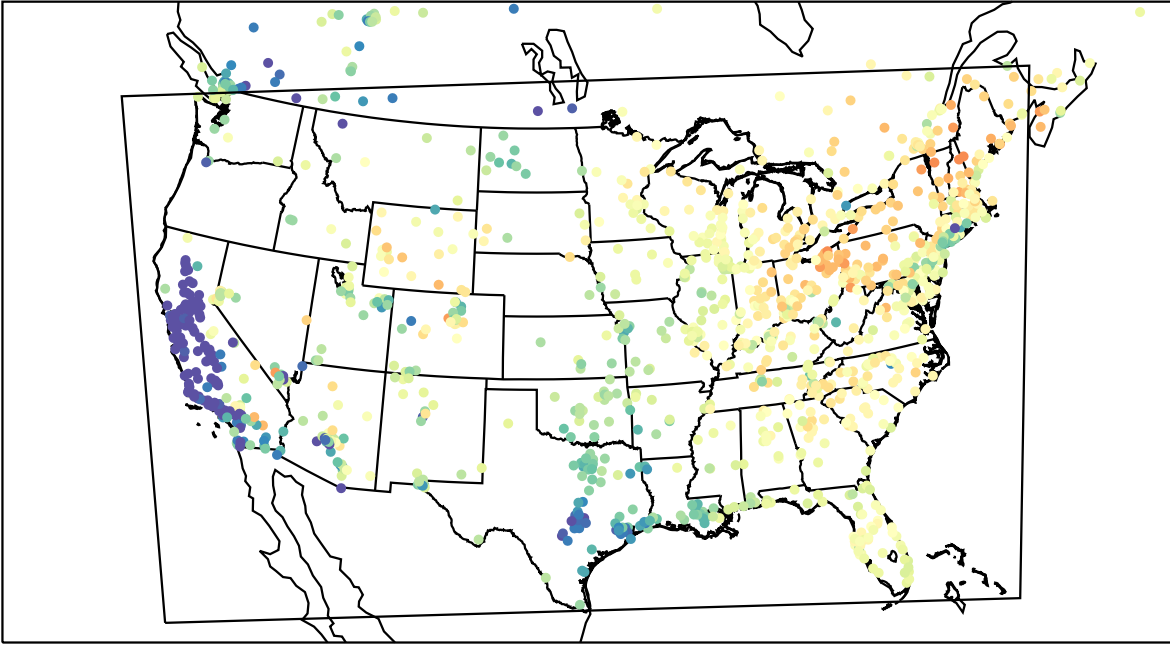
AirNOW (2023-04-11_15:00:00)
