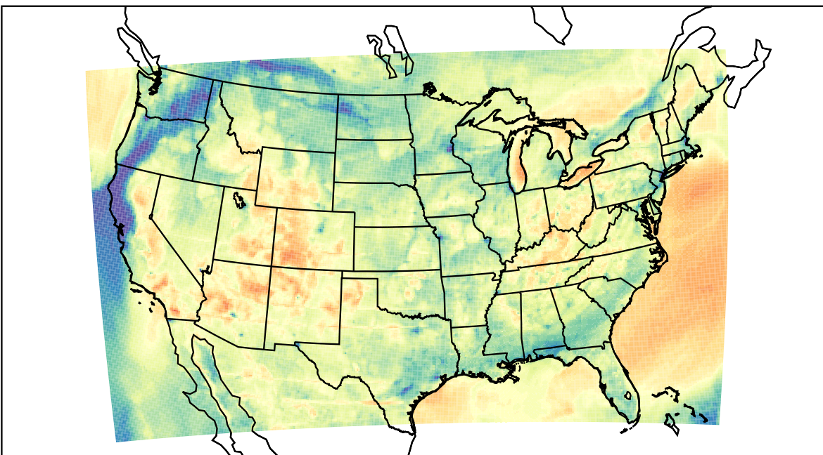
WRF (2023-04-11_02:00:00)
