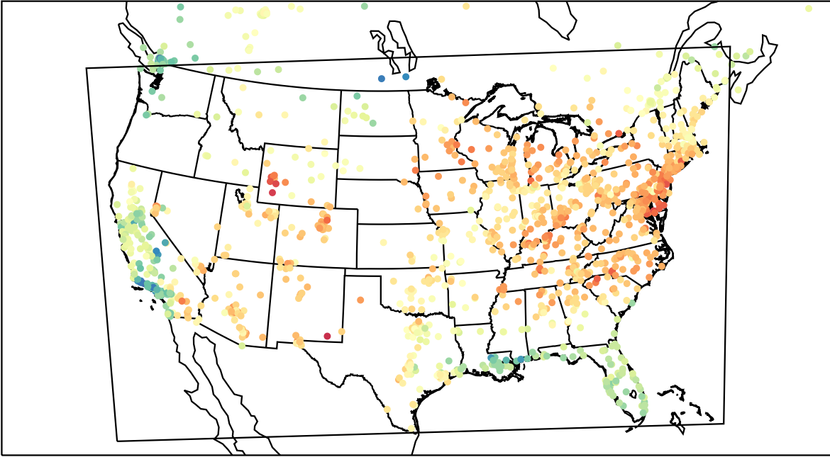
AirNOW (2023-04-12_19:00:00)
