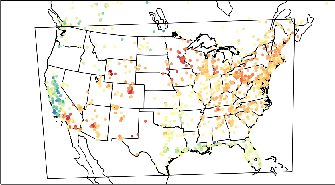
AirNOW (2023-04-11_22:00:00)
