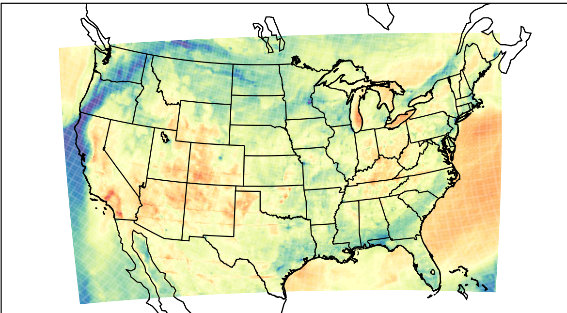
WRF (2023-04-11_01:00:00)
