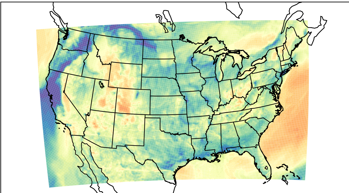
WRF (2023-04-11_06:00:00)
