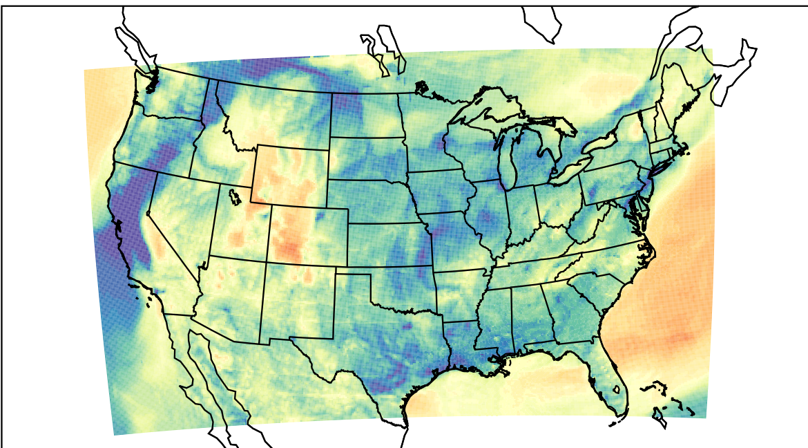
WRF (2023-04-11_11:00:00)
