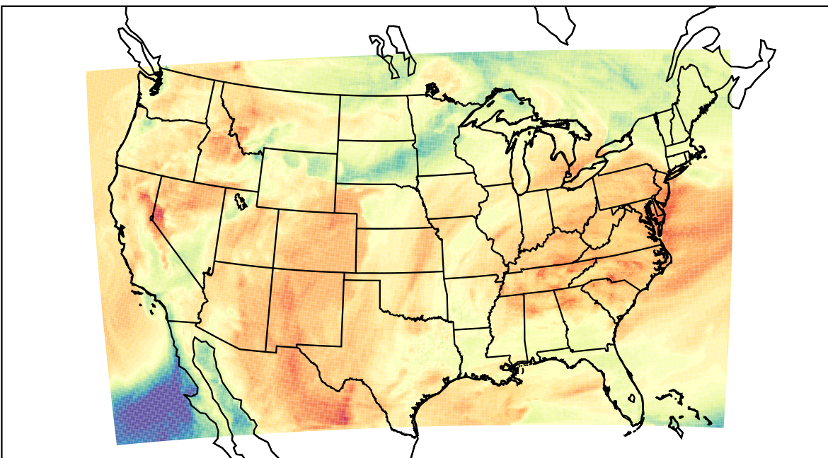
WRF (2023-04-12_19:00:00)
