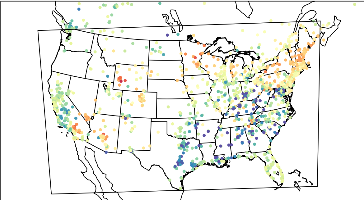
AirNOW (2023-04-12_02:00:00)
