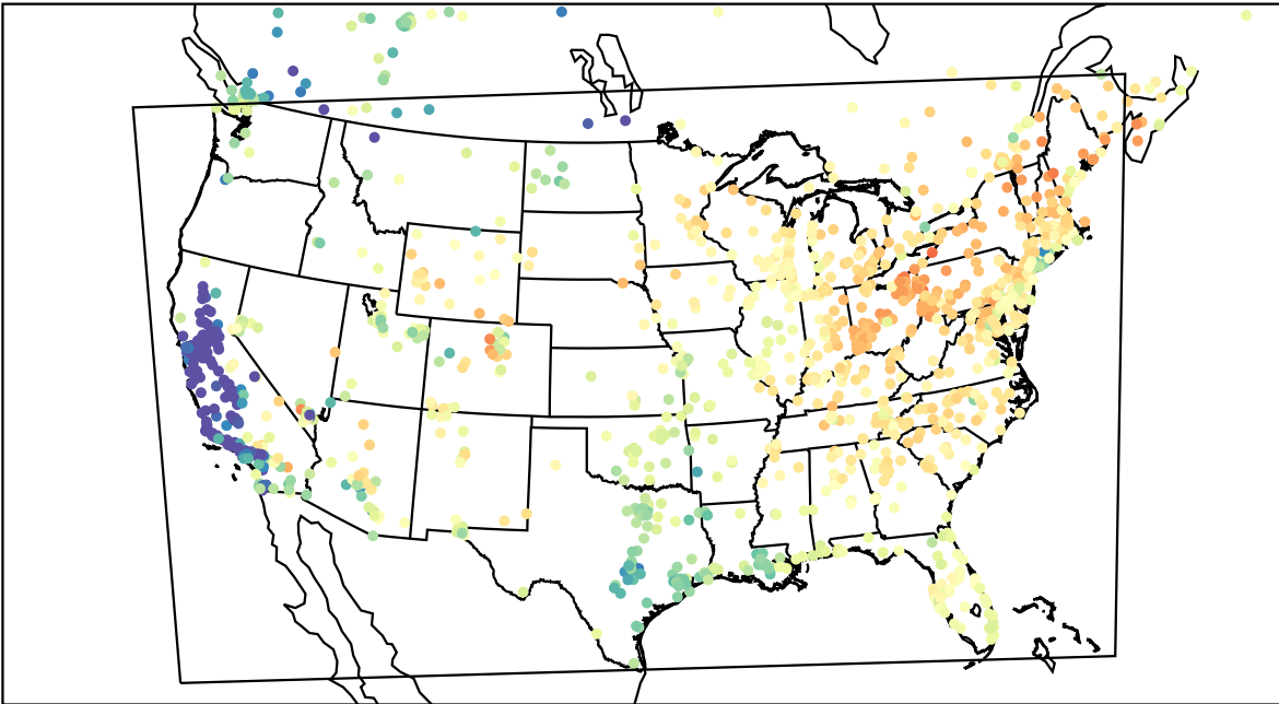
AirNOW (2023-04-11_16:00:00)
