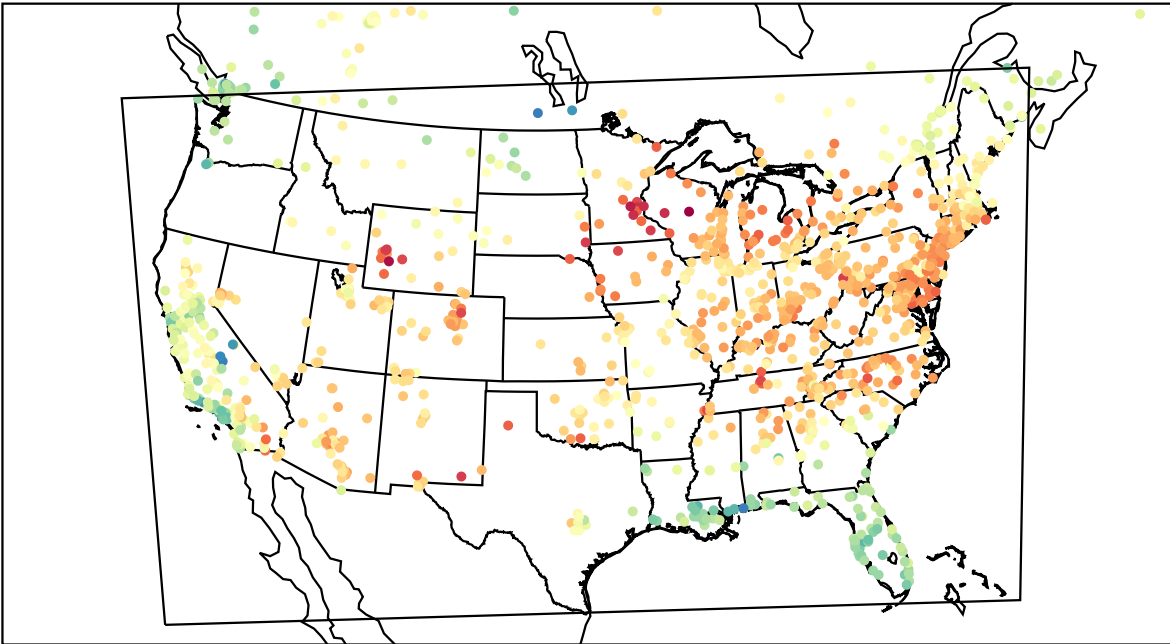
AirNOW (2023-04-12_22:00:00)
