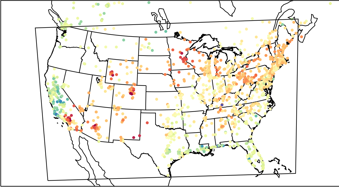
AirNOW (2023-04-11_23:00:00)
