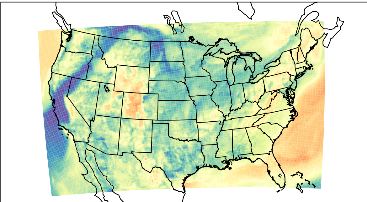
WRF (2023-04-11_15:00:00)
