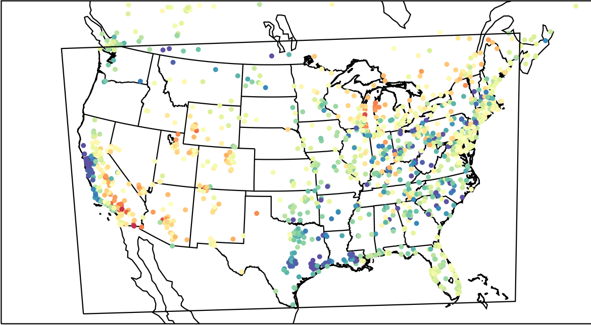
AirNOW (2023-04-11_01:00:00)
