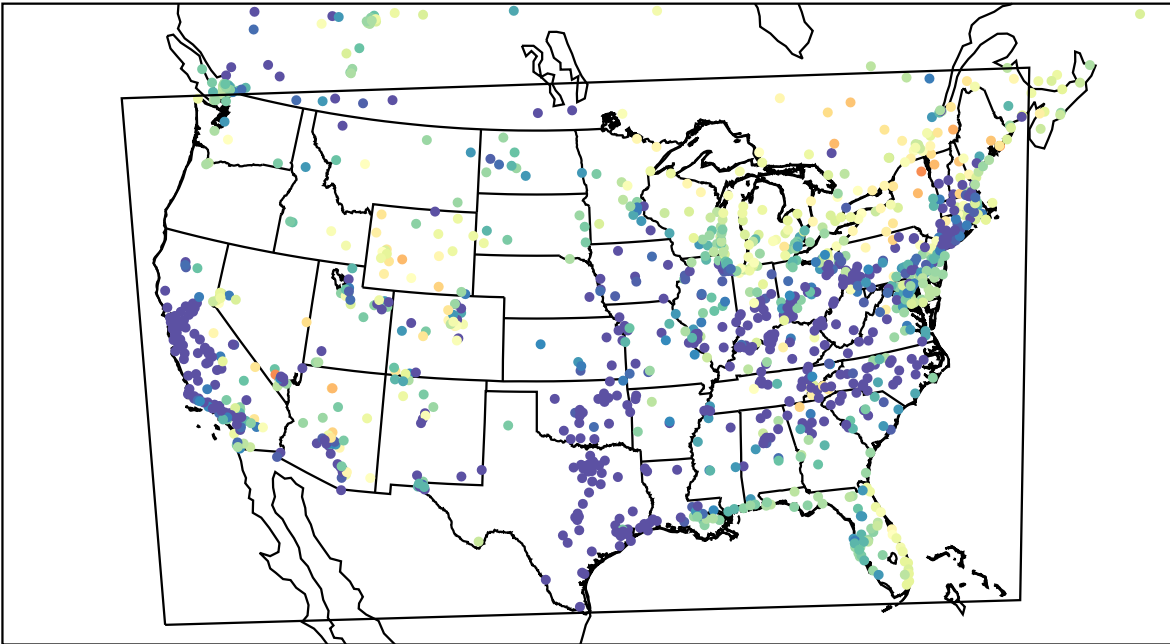
AirNOW (2023-04-11_12:00:00)
