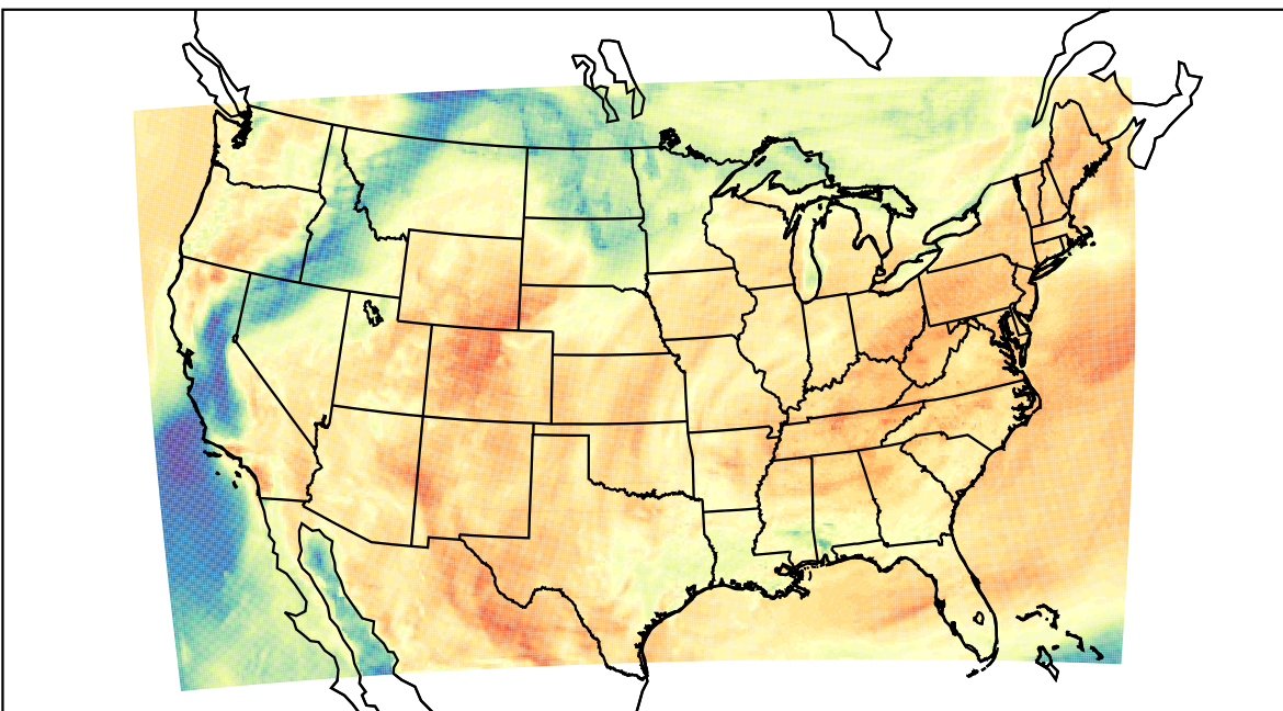
WRF (2023-04-11_19:00:00)
