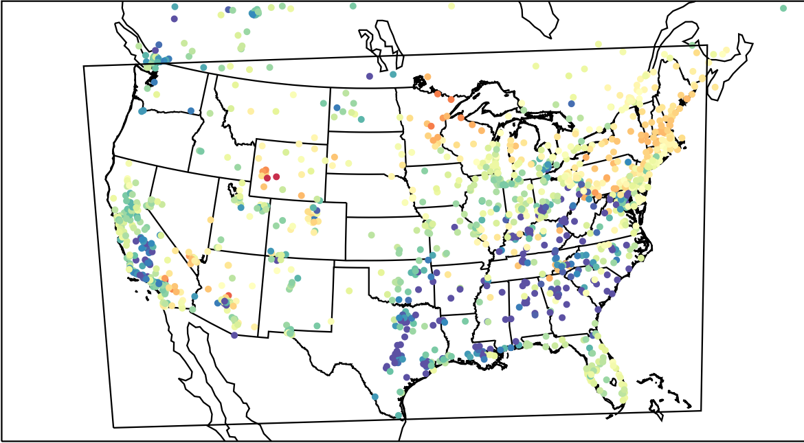
AirNOW (2023-04-12_04:00:00)
