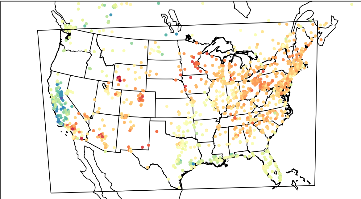
AirNOW (2023-04-11_21:00:00)
