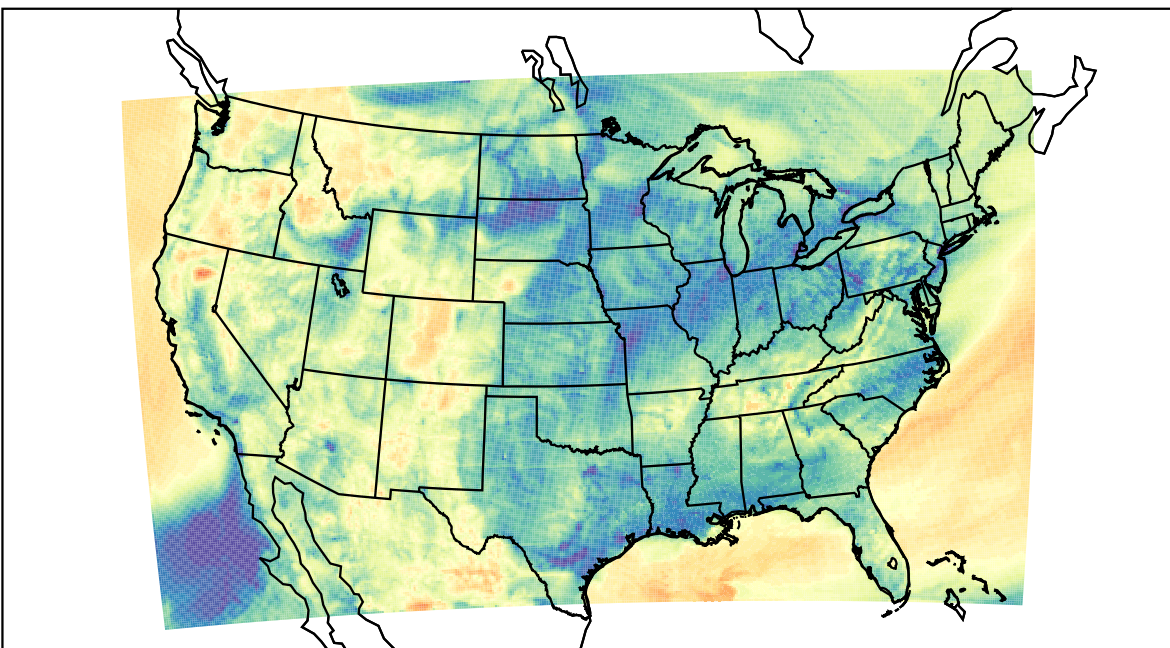
WRF (2023-04-12_12:00:00)
