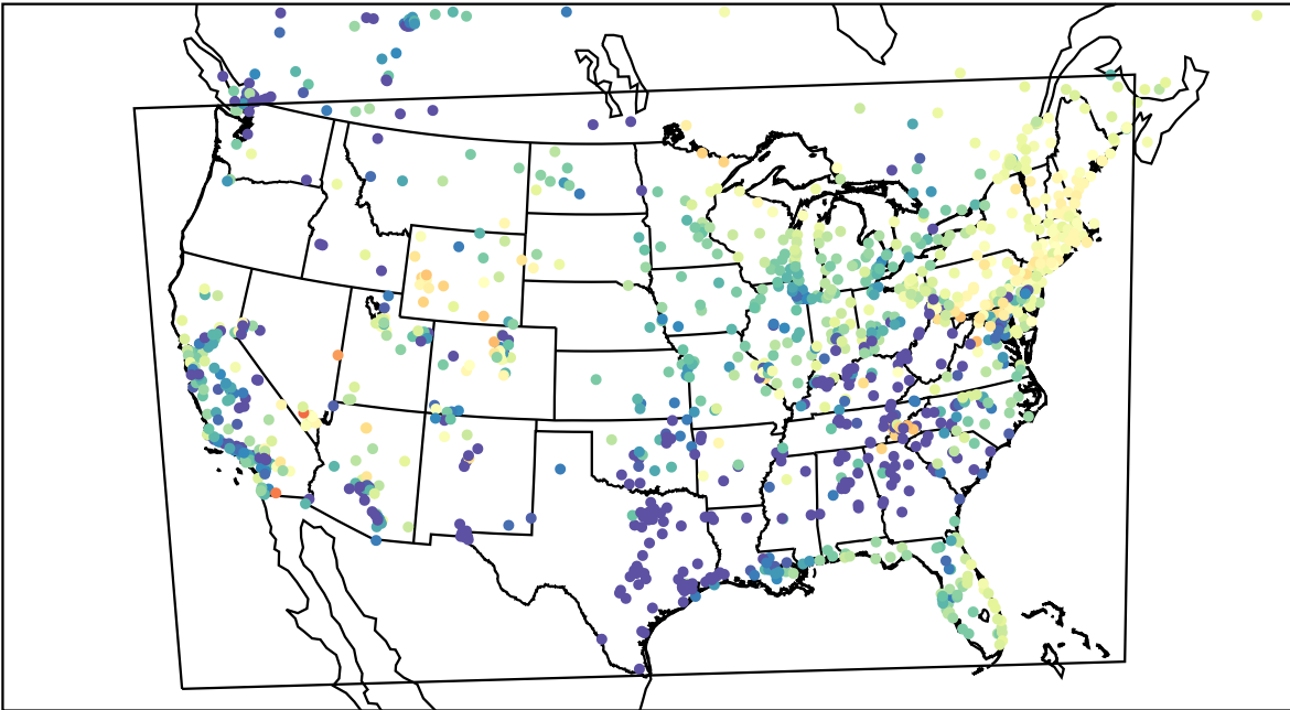
AirNOW (2023-04-12_12:00:00)
