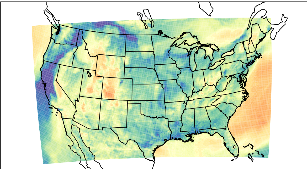
WRF (2023-04-11_08:00:00)
