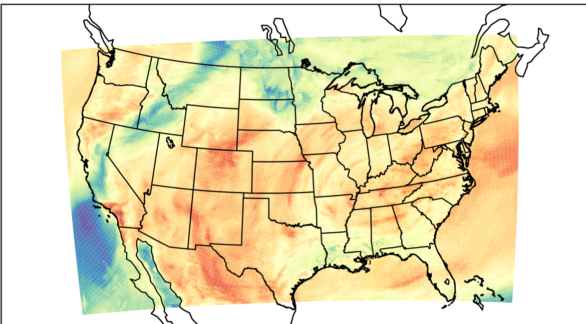
WRF (2023-04-11_22:00:00)
