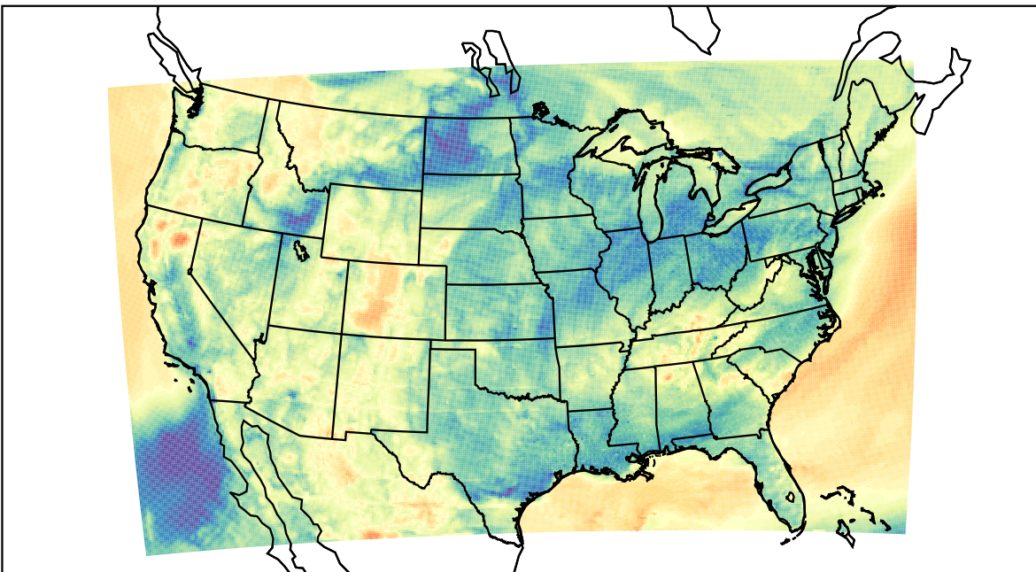
WRF (2023-04-12_08:00:00)
