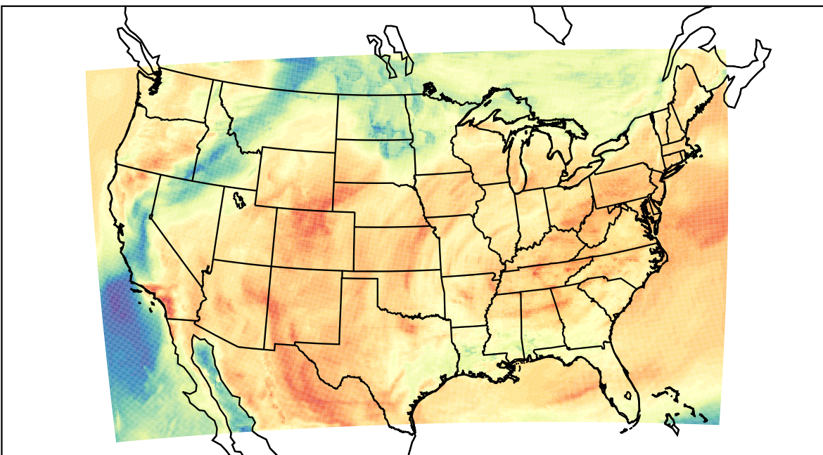
WRF (2023-04-11_21:00:00)
