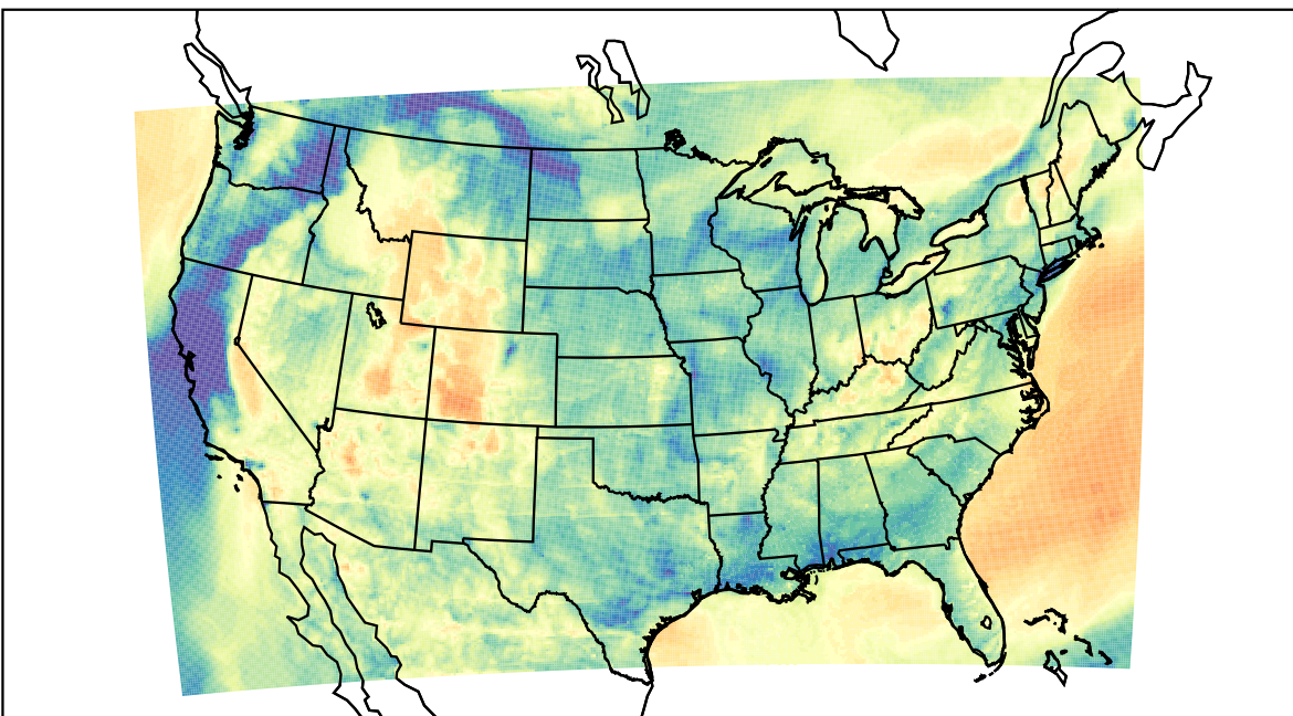
WRF (2023-04-11_07:00:00)
