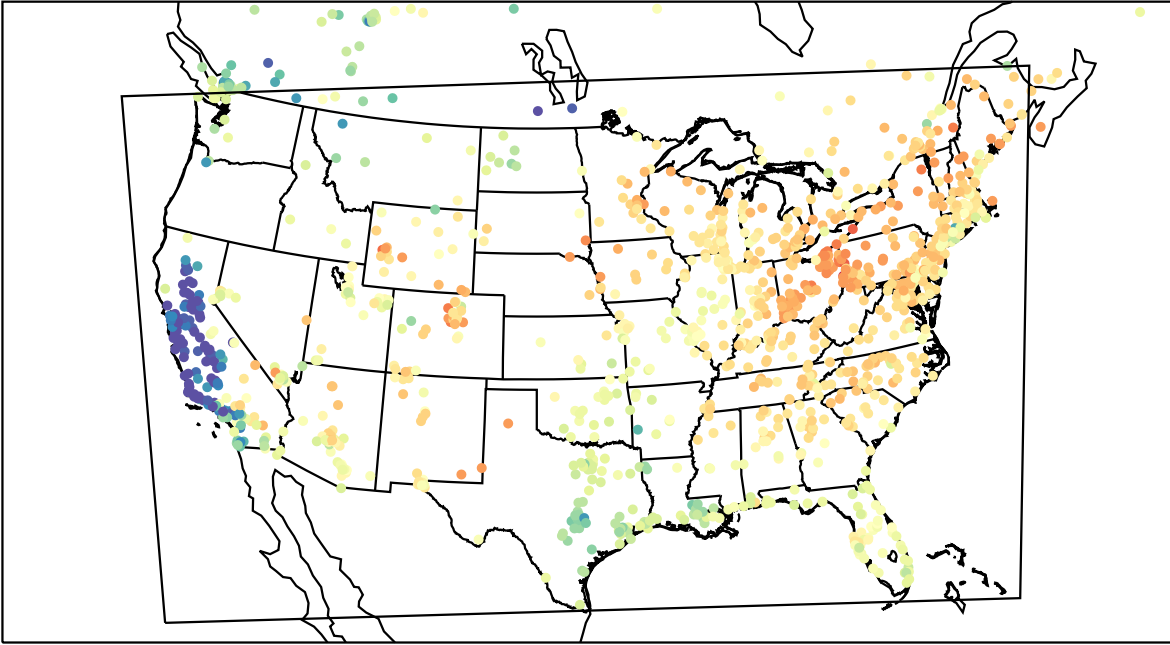
AirNOW (2023-04-11_17:00:00)
