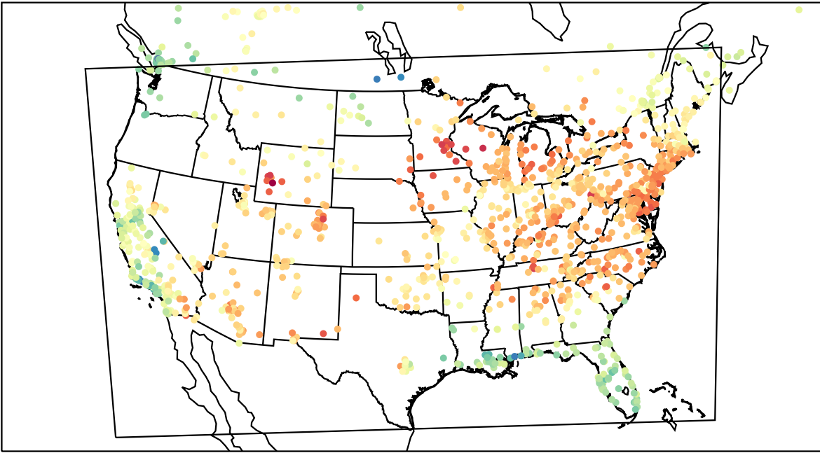
AirNOW (2023-04-12_21:00:00)
