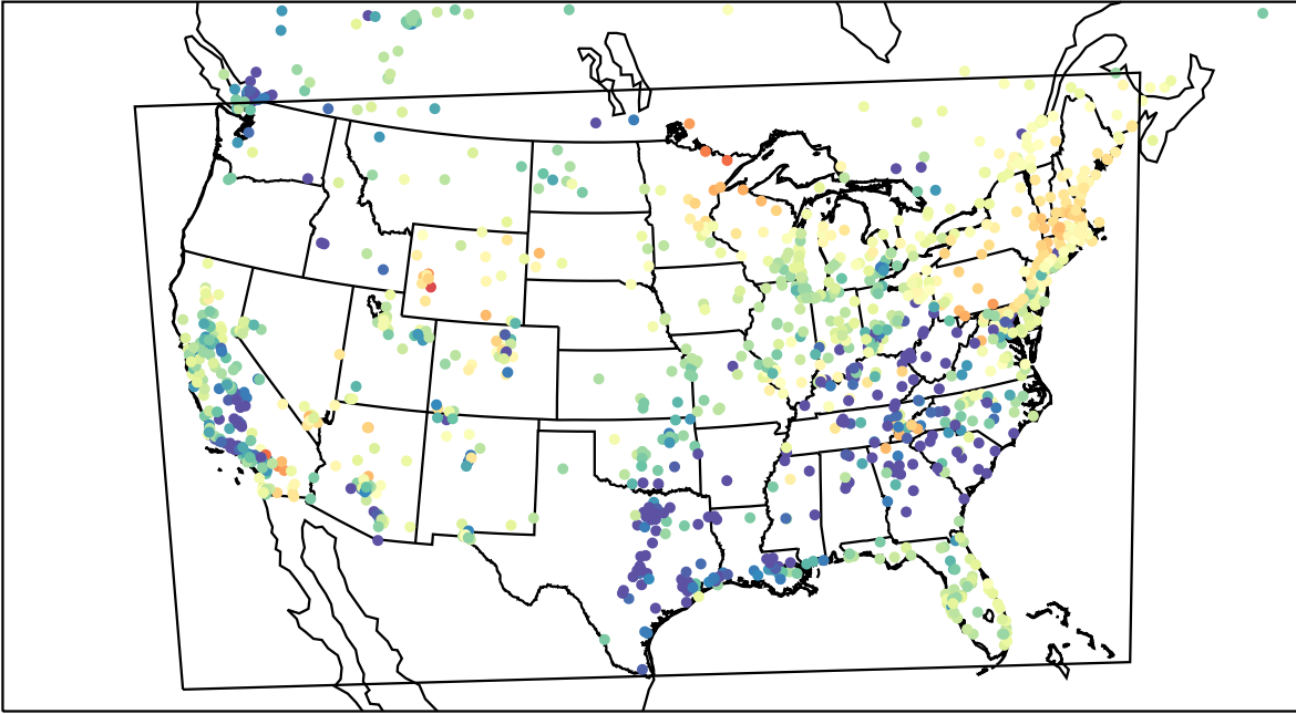
AirNOW (2023-04-12_06:00:00)
