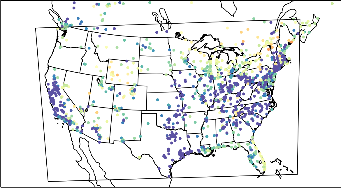
AirNOW (2023-04-11_11:00:00)
