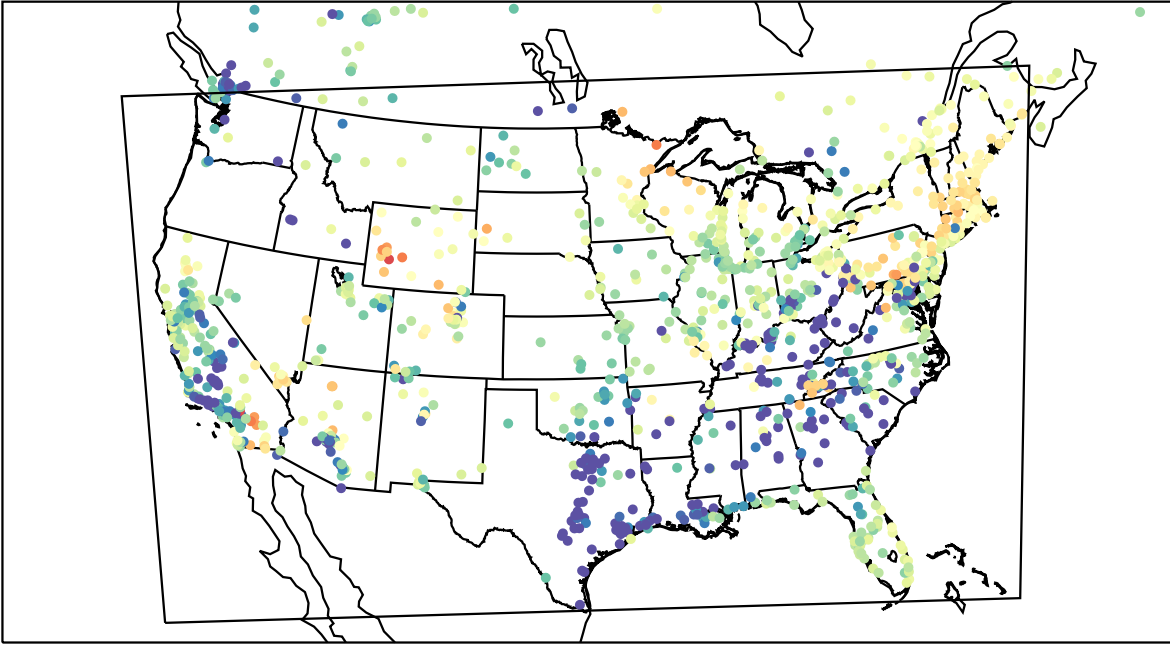
AirNOW (2023-04-12_07:00:00)
