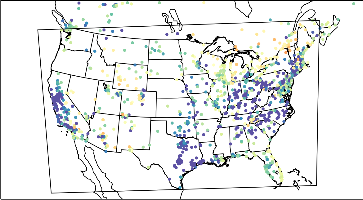
AirNOW (2023-04-11_07:00:00)
