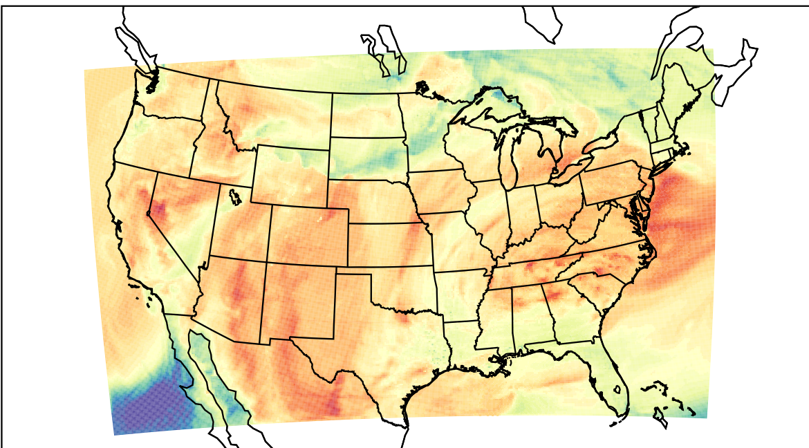
WRF (2023-04-12_21:00:00)
