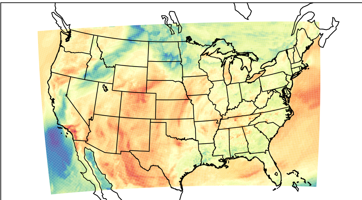
WRF (2023-04-11_23:00:00)
