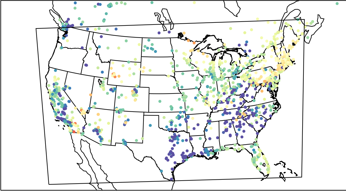
AirNOW (2023-04-12_09:00:00)
