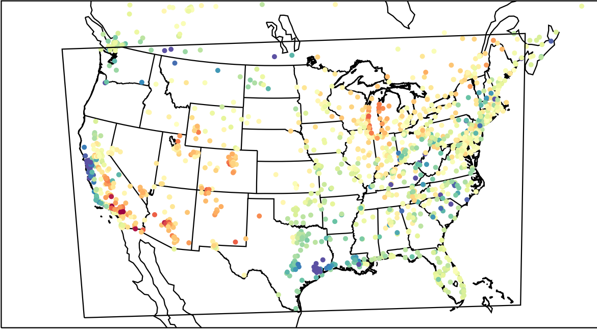
AirNOW (2023-04-11_00:00:00)
