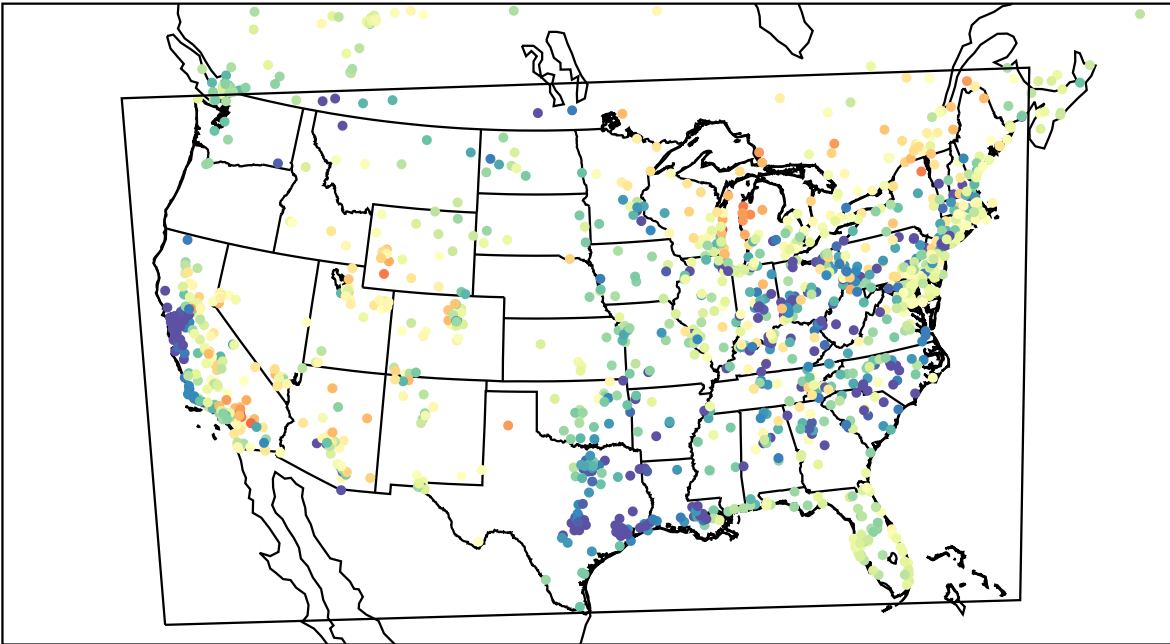
AirNOW (2023-04-11_02:00:00)
