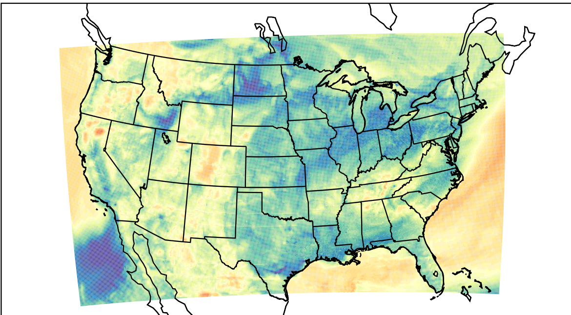
WRF (2023-04-12_09:00:00)
