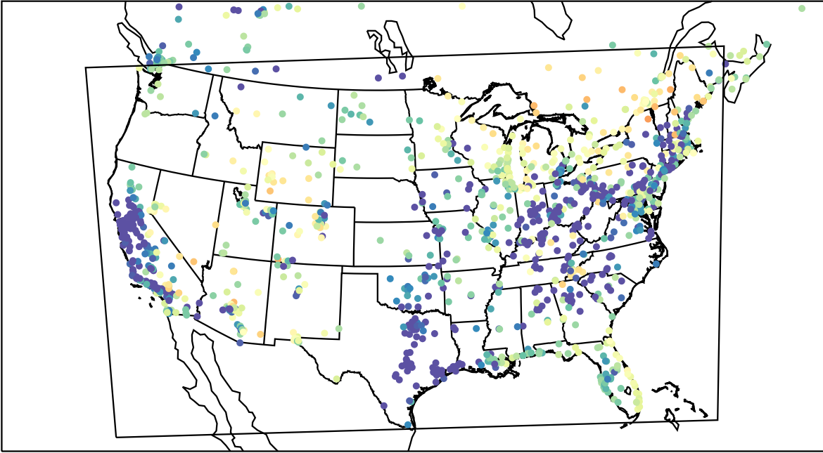
AirNOW (2023-04-11_08:00:00)
