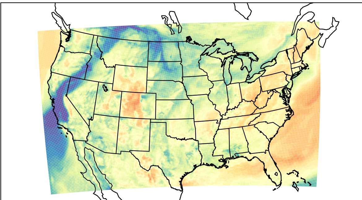
WRF (2023-04-11_16:00:00)
