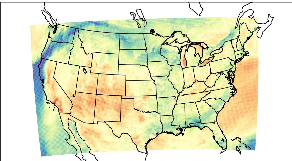
WRF (2023-04-11_00:00:00)
