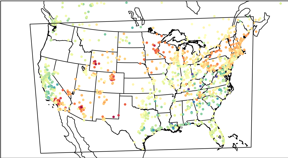
AirNOW (2023-04-12_00:00:00)
