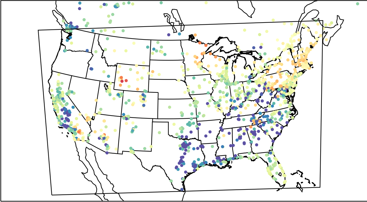
AirNOW (2023-04-12_05:00:00)
