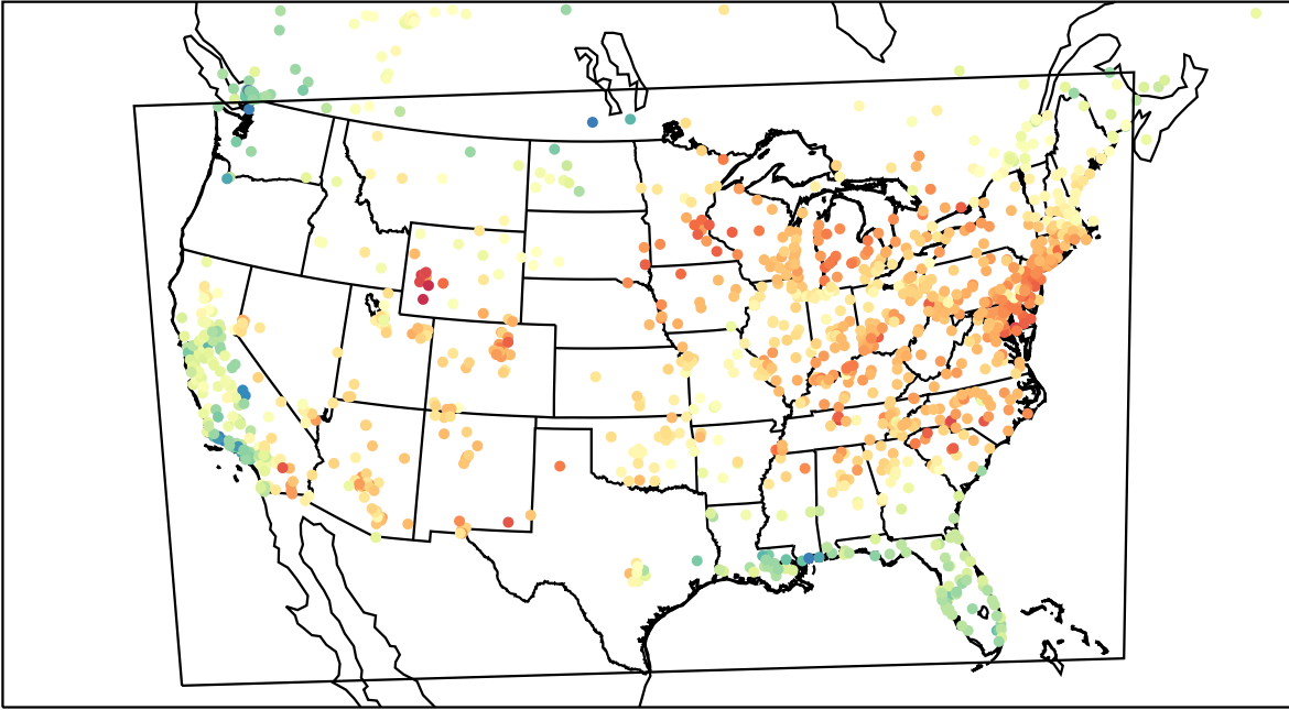
AirNOW (2023-04-12_20:00:00)
