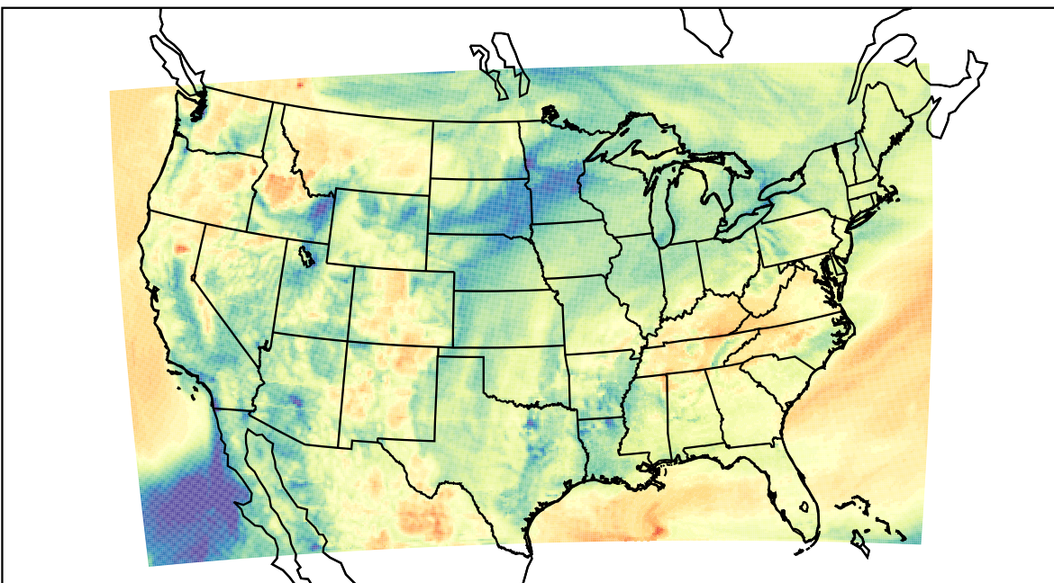
WRF (2023-04-12_15:00:00)
