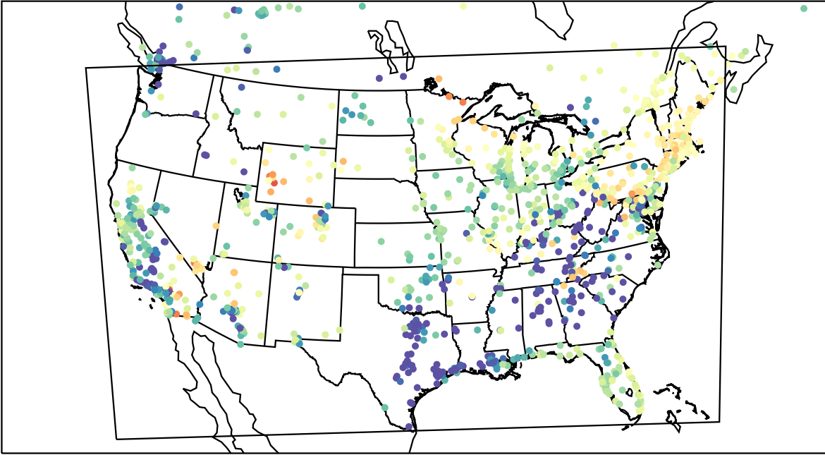
AirNOW (2023-04-12_08:00:00)
