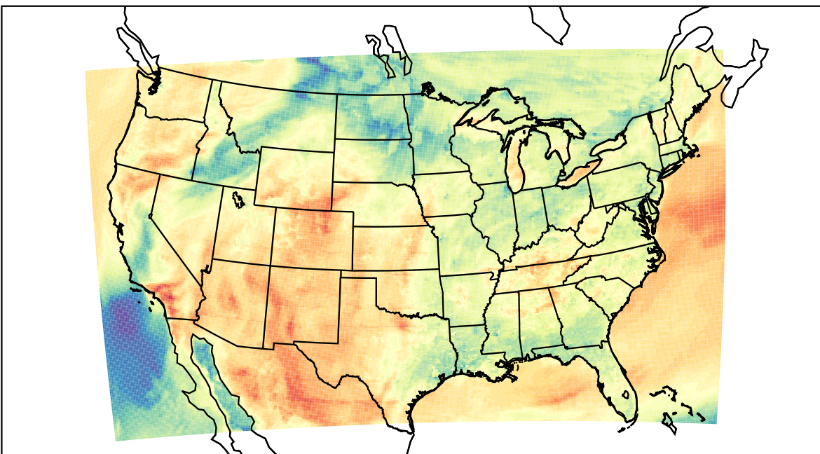
WRF (2023-04-12_00:00:00)
