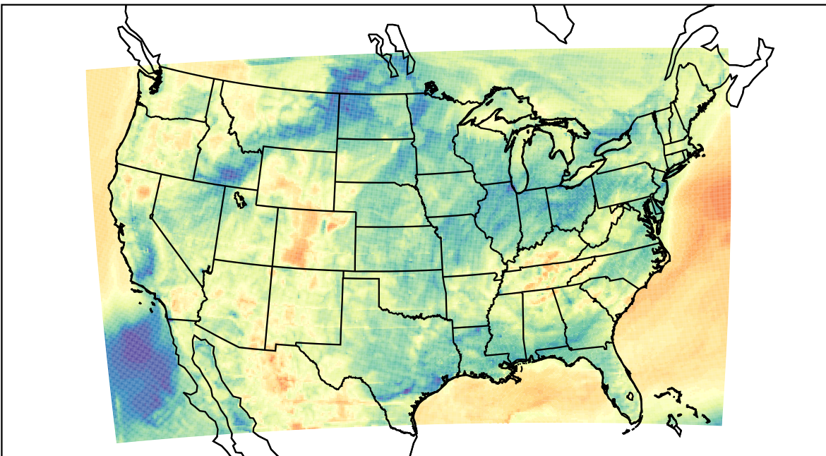
WRF (2023-04-12_05:00:00)
