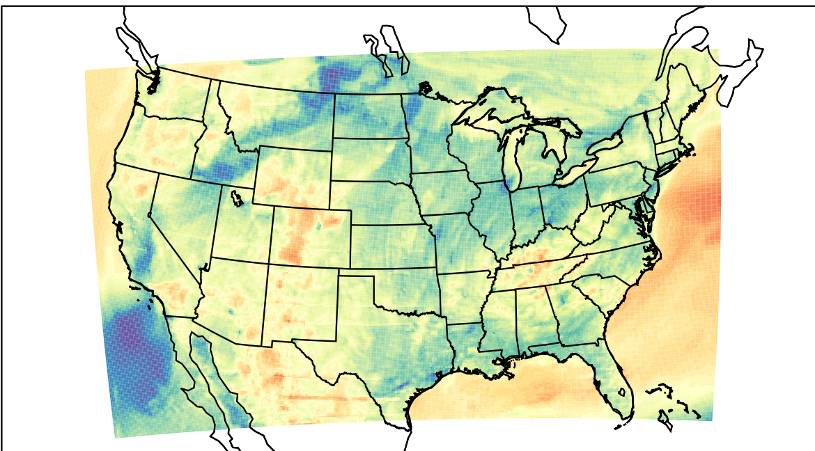
WRF (2023-04-12_03:00:00)
