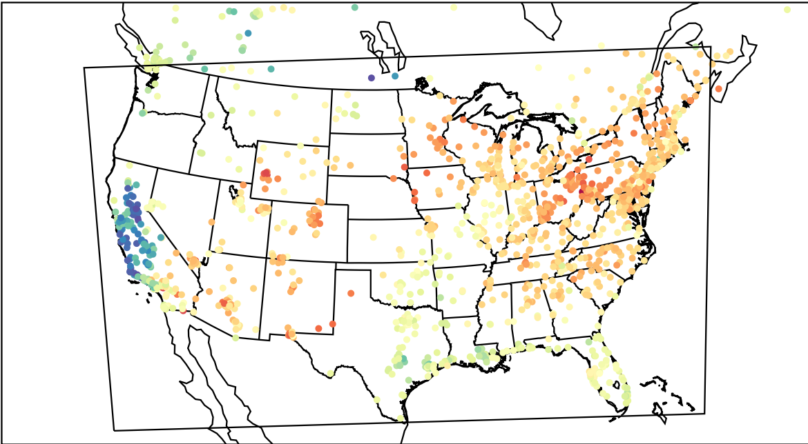
AirNOW (2023-04-11_19:00:00)
