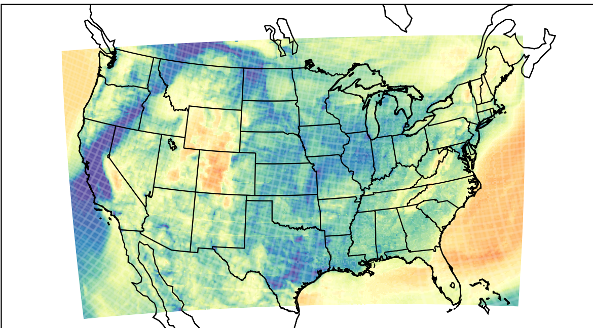
WRF (2023-04-11_14:00:00)
