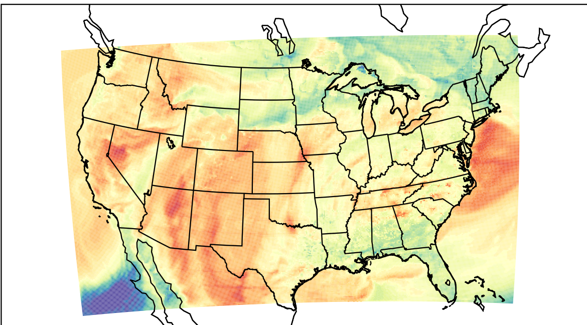
WRF (2023-04-12_23:00:00)
