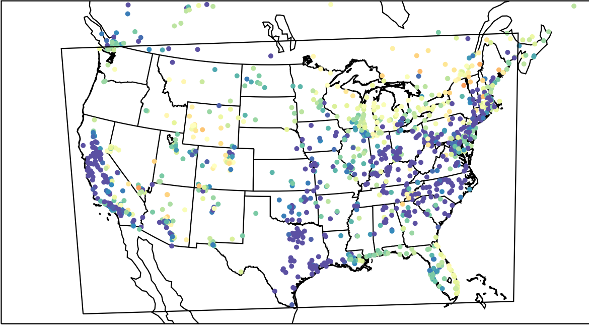
AirNOW (2023-04-11_10:00:00)
