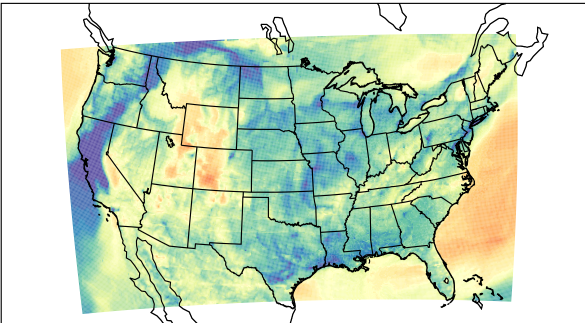
WRF (2023-04-11_10:00:00)
