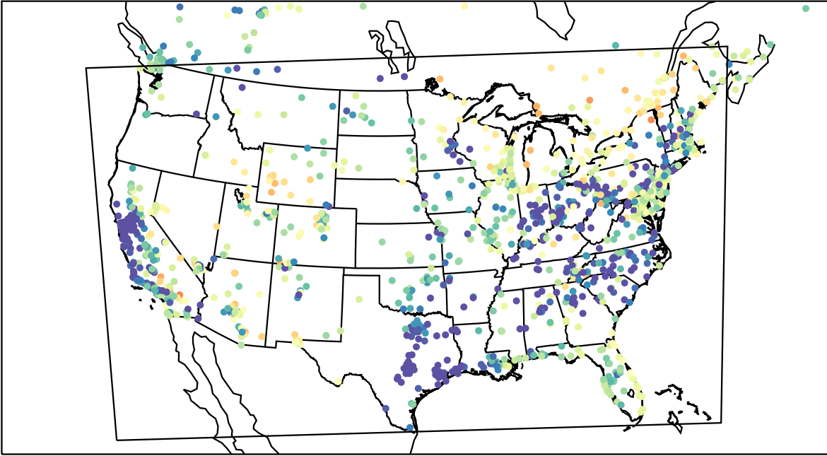
AirNOW (2023-04-11_05:00:00)
