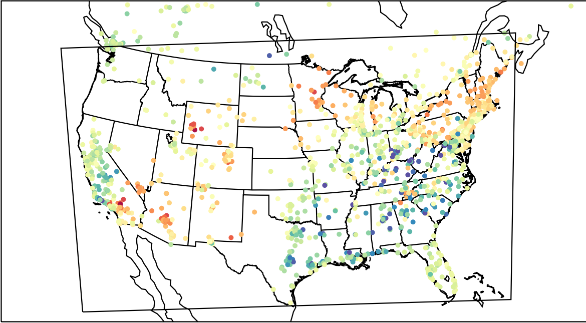
AirNOW (2023-04-12_01:00:00)
