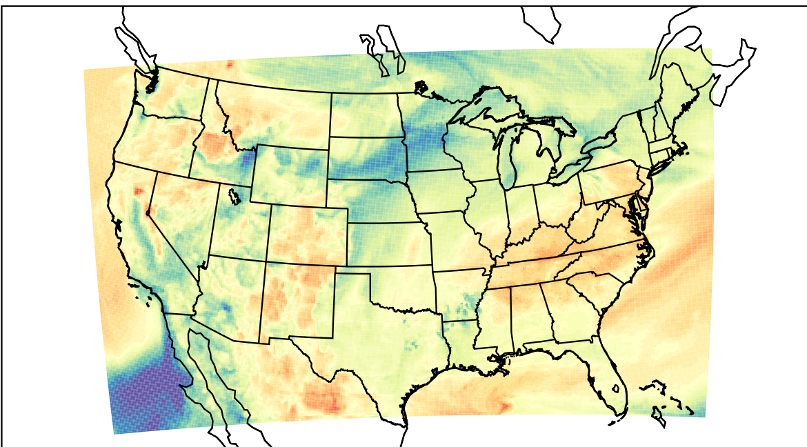
WRF (2023-04-12_16:00:00)
