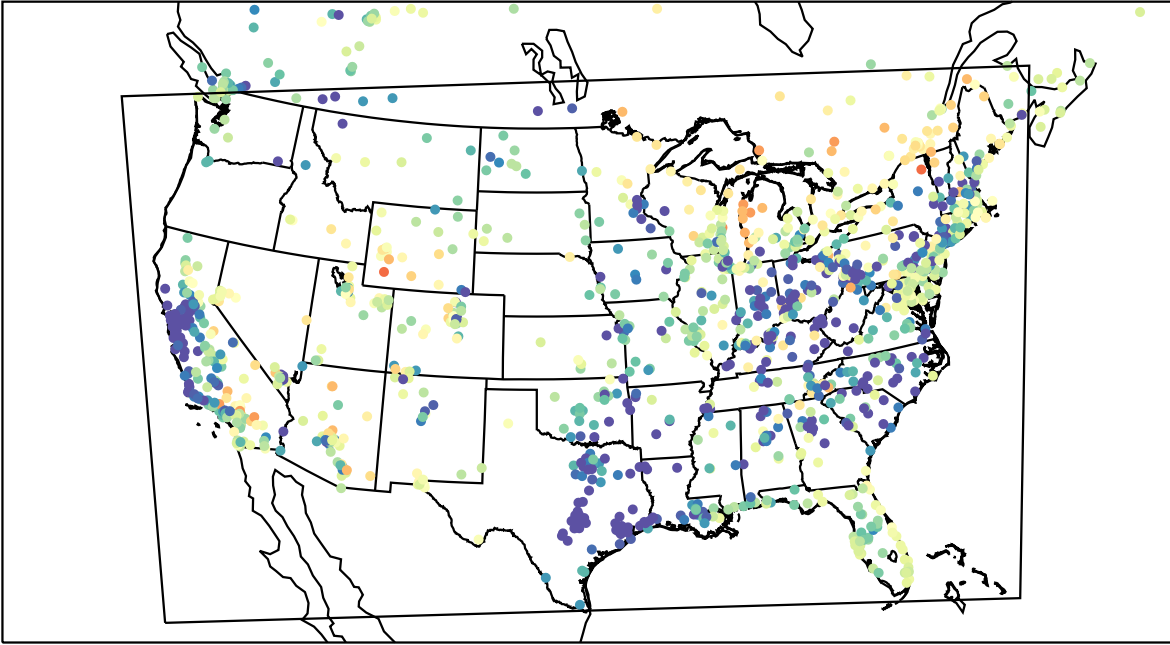
AirNOW (2023-04-11_04:00:00)
