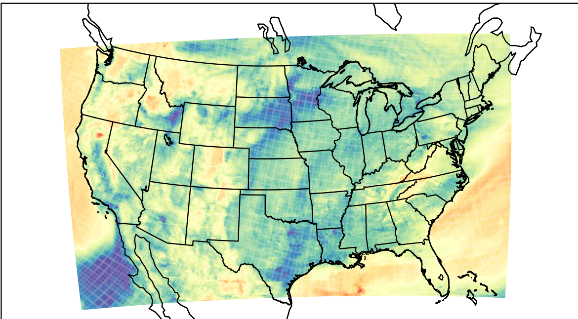
WRF (2023-04-12_14:00:00)
