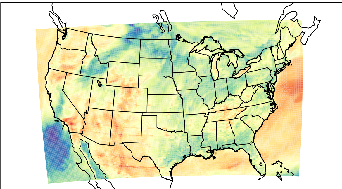
WRF (2023-04-12_01:00:00)
