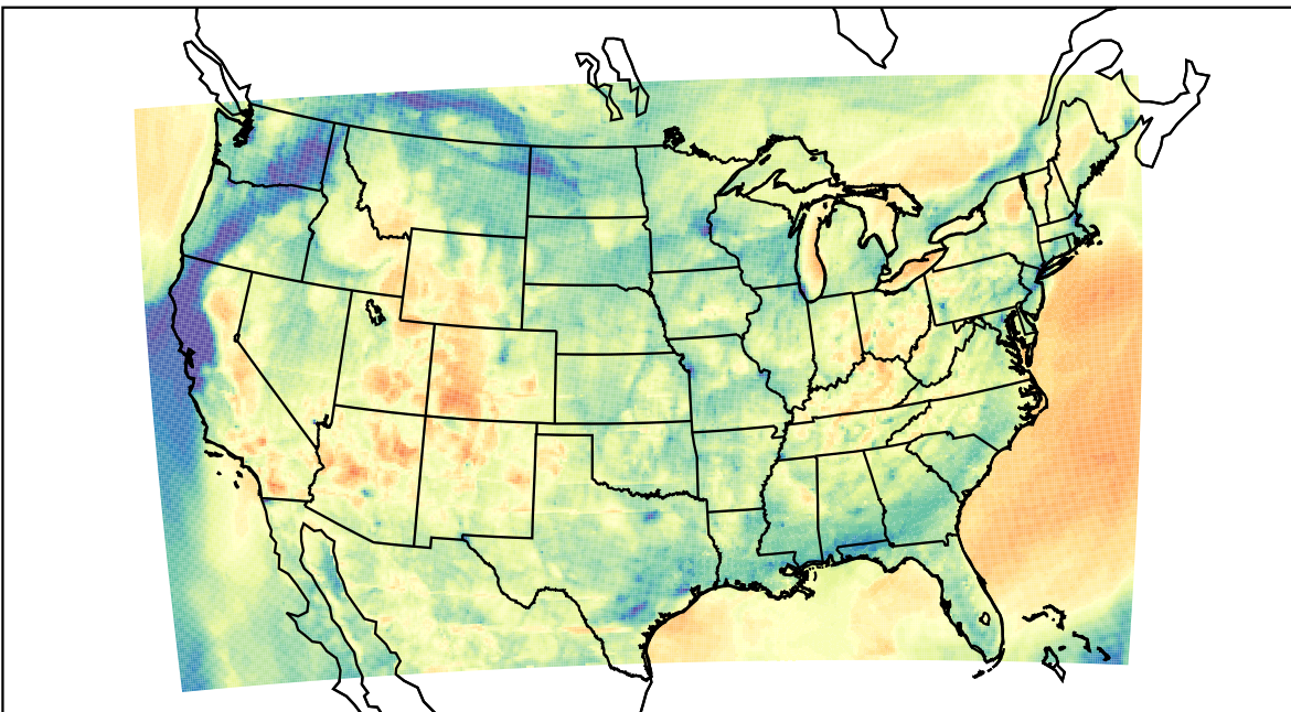
WRF (2023-04-11_03:00:00)
