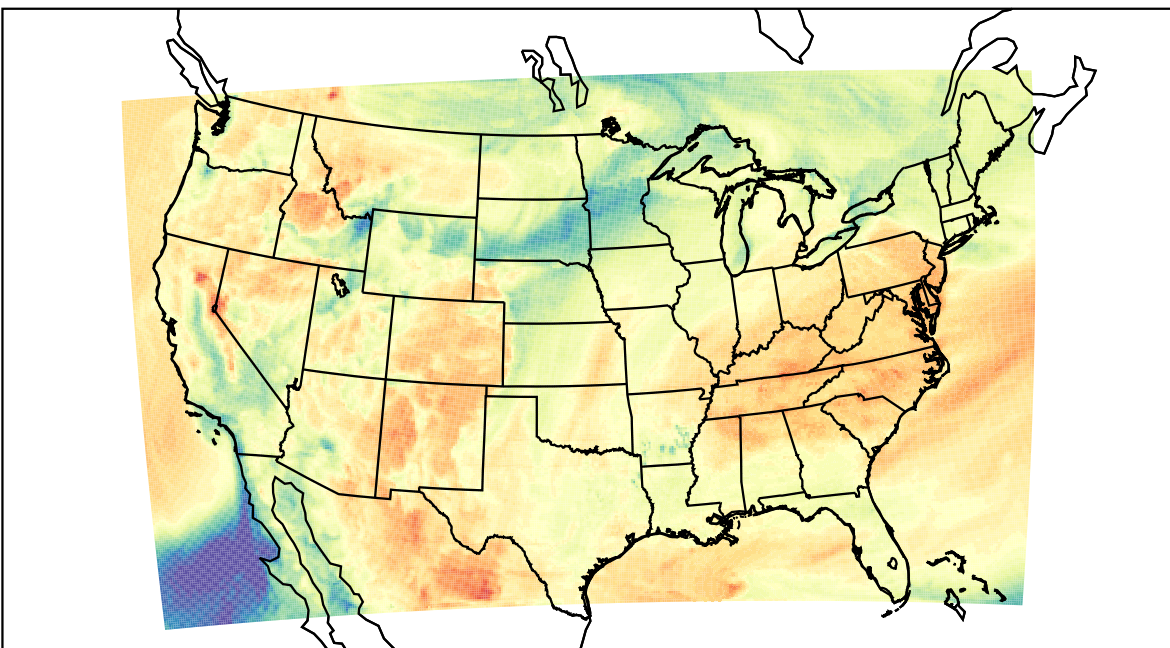
WRF (2023-04-12_17:00:00)
