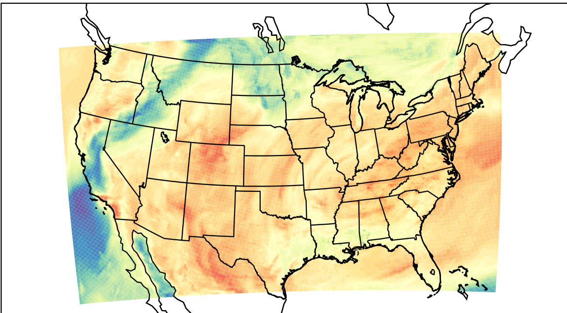
WRF (2023-04-11_20:00:00)
