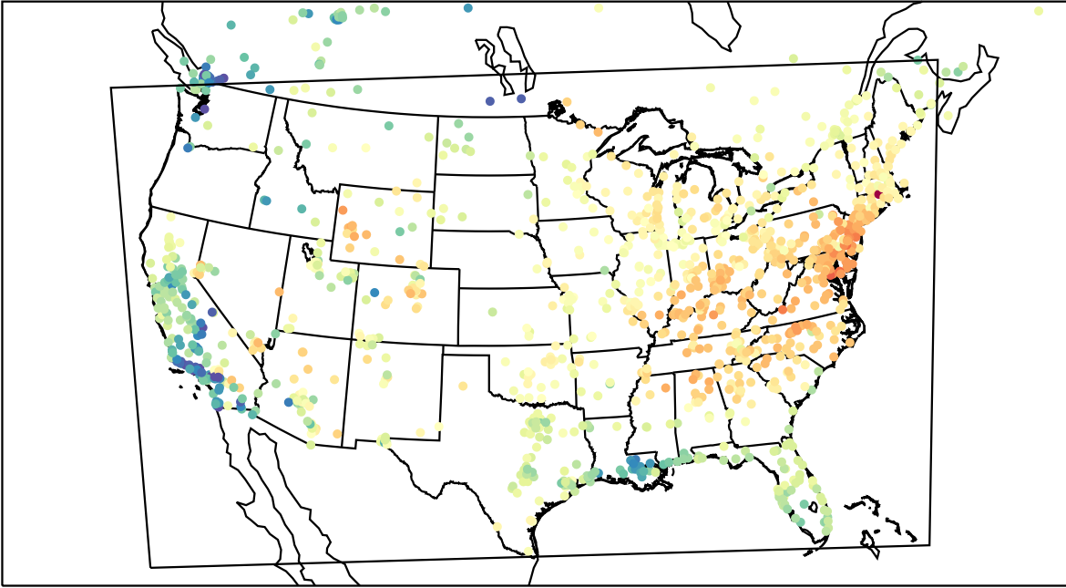
AirNOW (2023-04-12_16:00:00)
