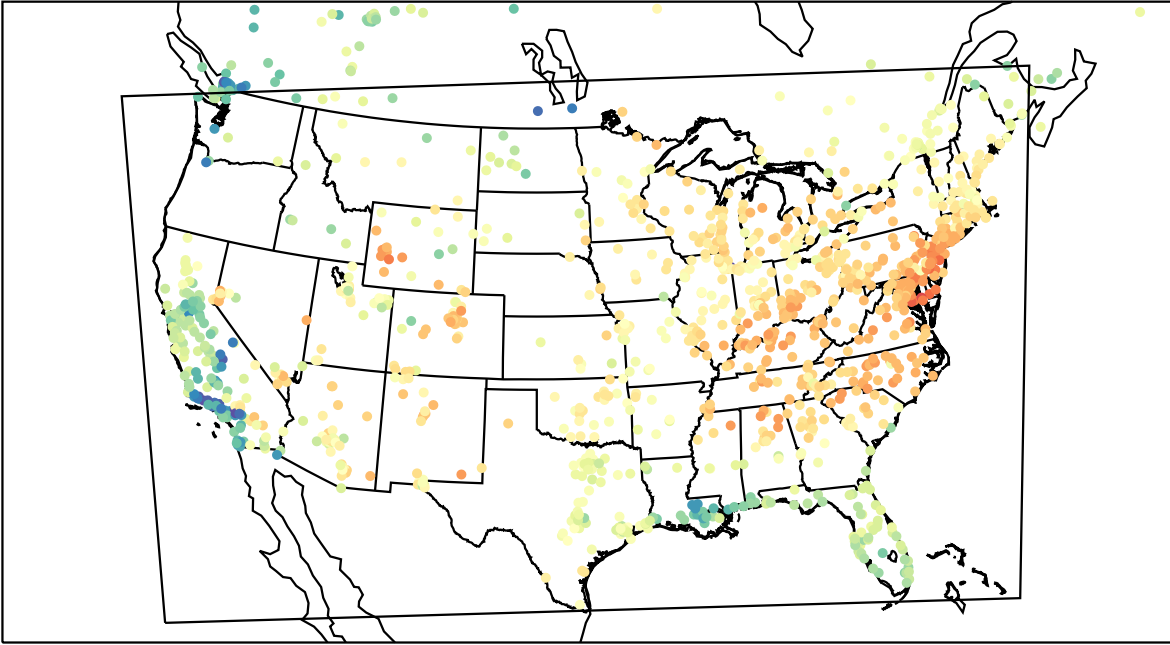
AirNOW (2023-04-12_17:00:00)
