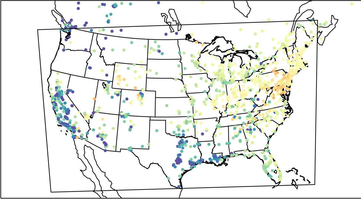
AirNOW (2023-04-12_14:00:00)
