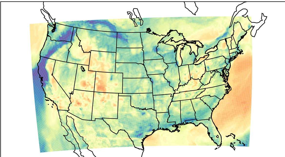
WRF (2023-04-11_04:00:00)
