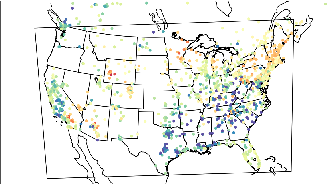
AirNOW (2023-04-12_03:00:00)
