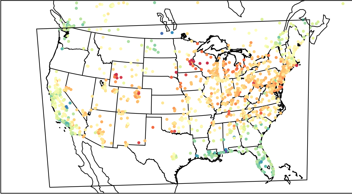
AirNOW (2023-04-12_23:00:00)
