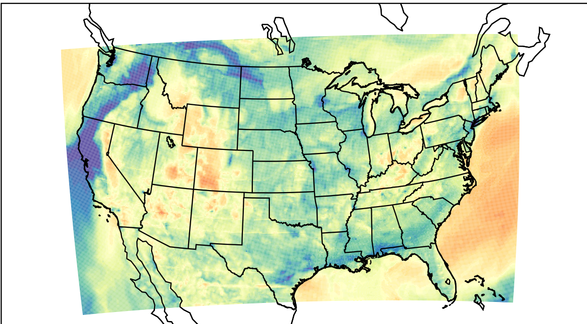
WRF (2023-04-11_05:00:00)
