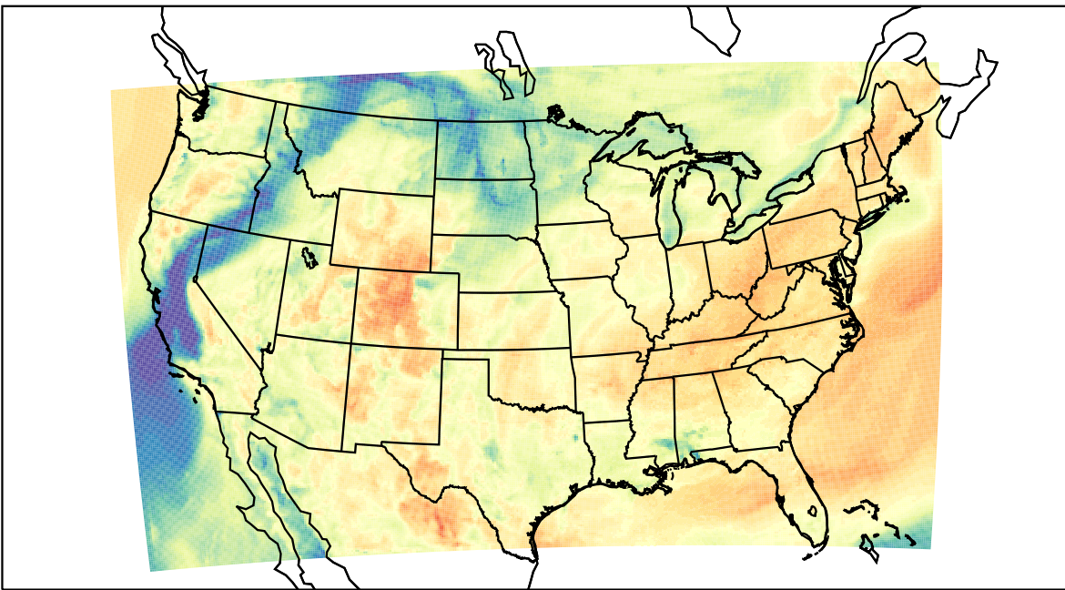
WRF (2023-04-11_17:00:00)
