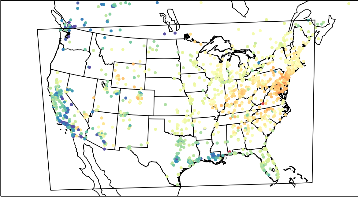
AirNOW (2023-04-12_15:00:00)
