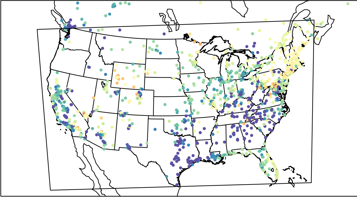
AirNOW (2023-04-12_10:00:00)
