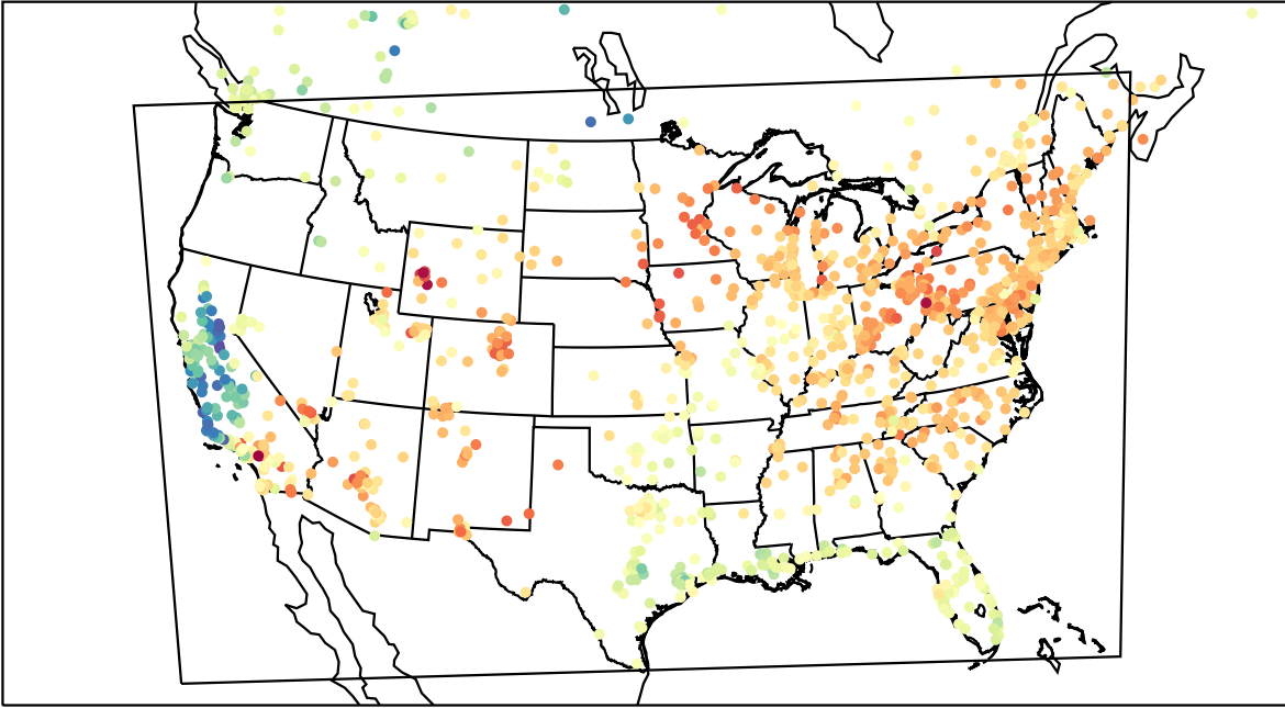
AirNOW (2023-04-11_20:00:00)
