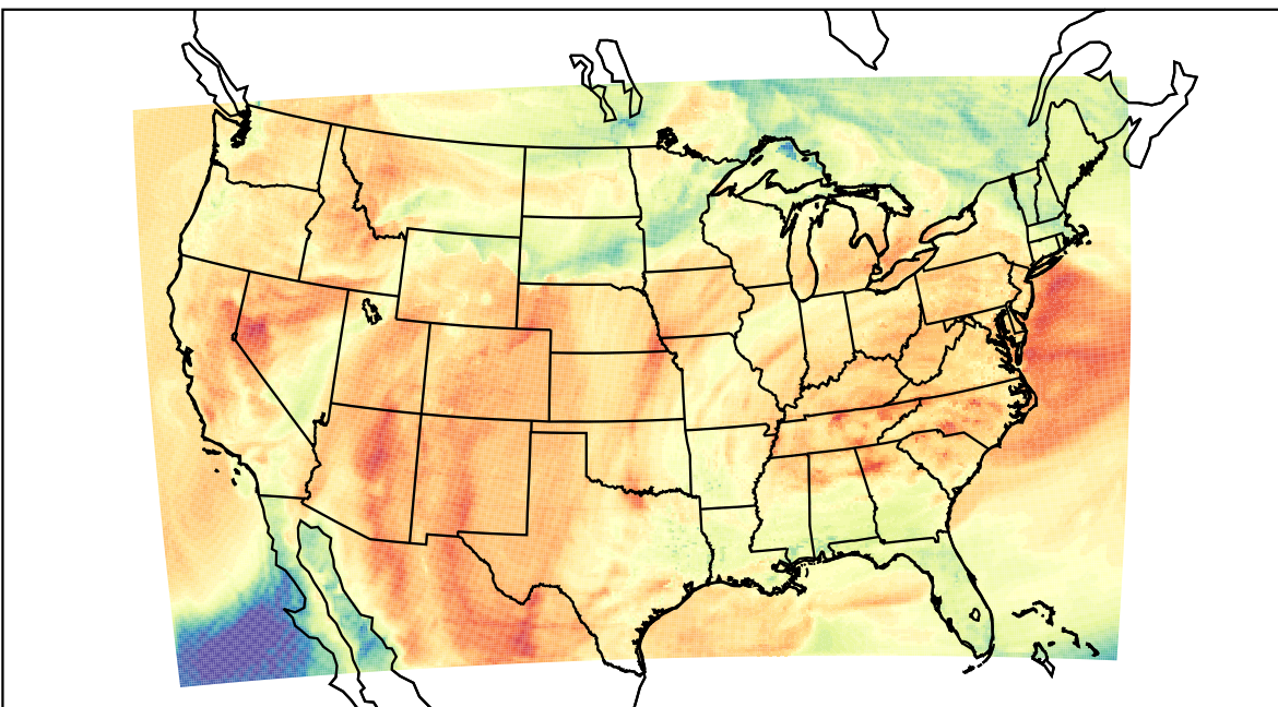
WRF (2023-04-12_22:00:00)
