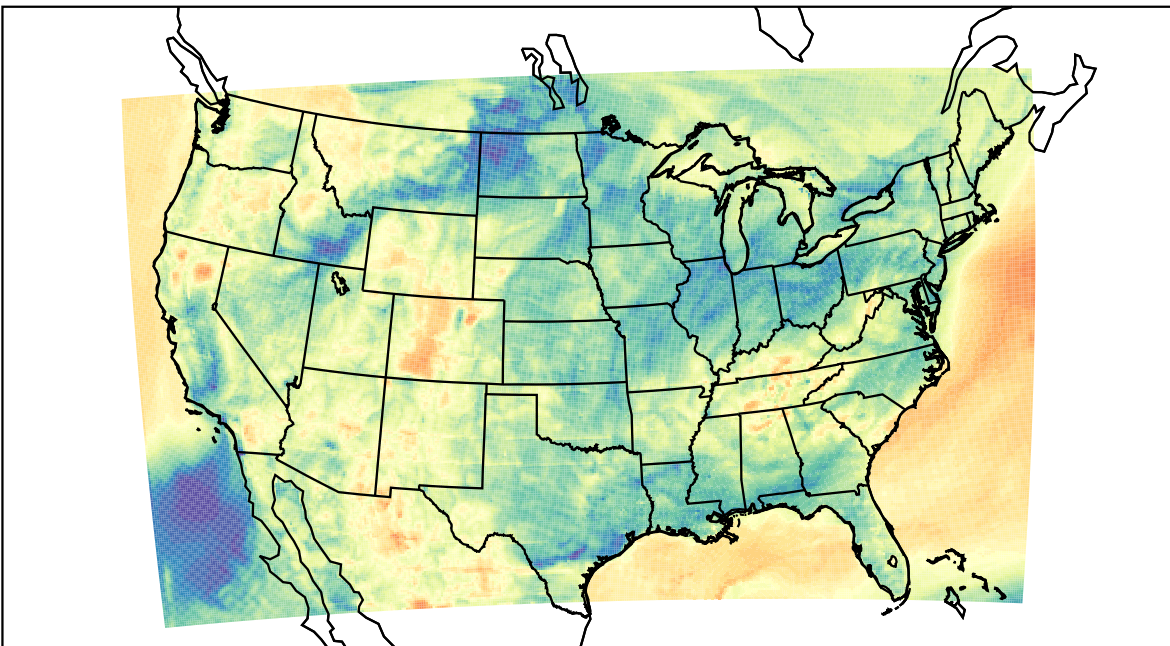
WRF (2023-04-12_06:00:00)
