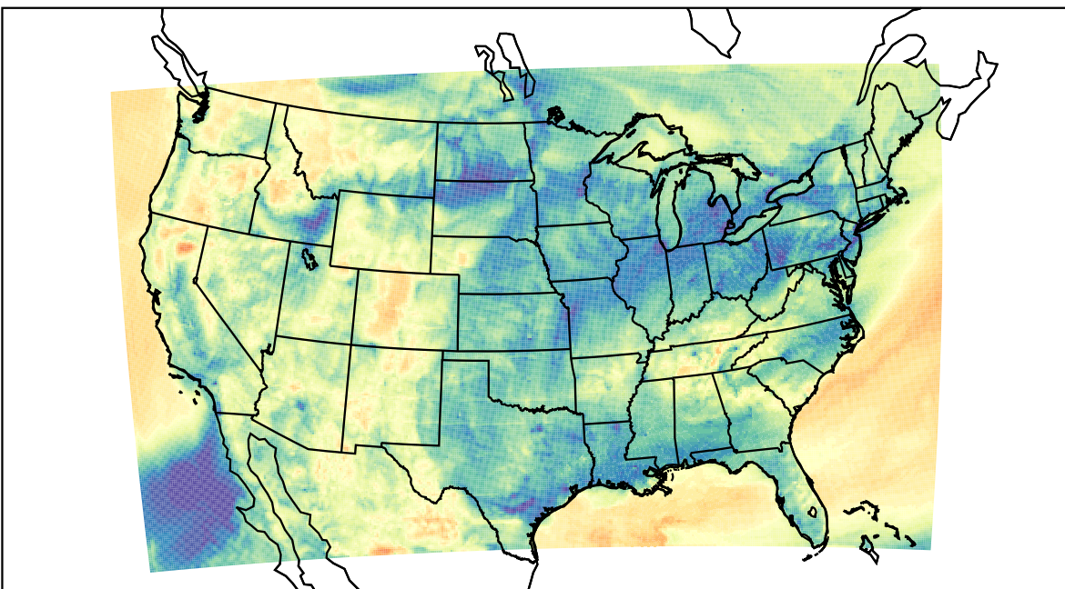
WRF (2023-04-12_11:00:00)
