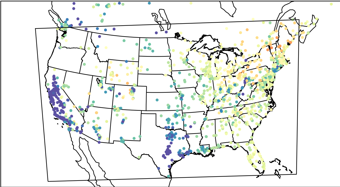
AirNOW (2023-04-11_14:00:00)
