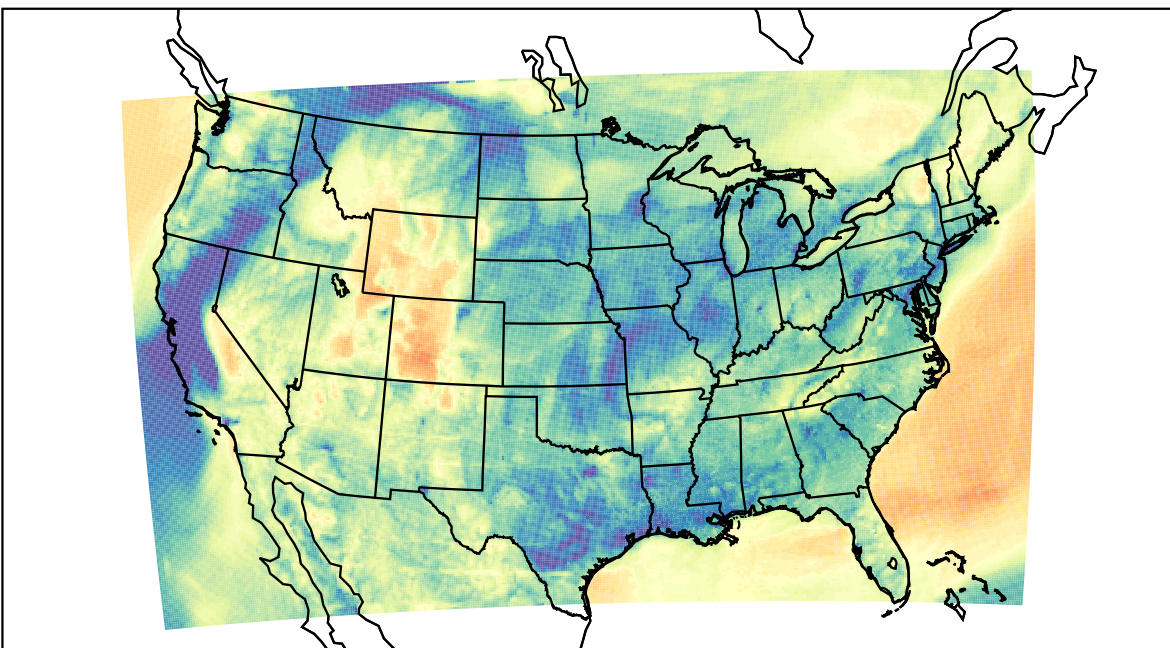
WRF (2023-04-11_12:00:00)
