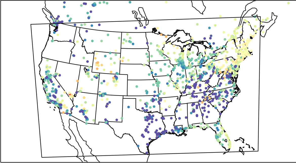
AirNOW (2023-04-12_11:00:00)
