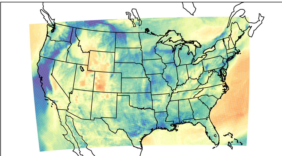
WRF (2023-04-11_09:00:00)
