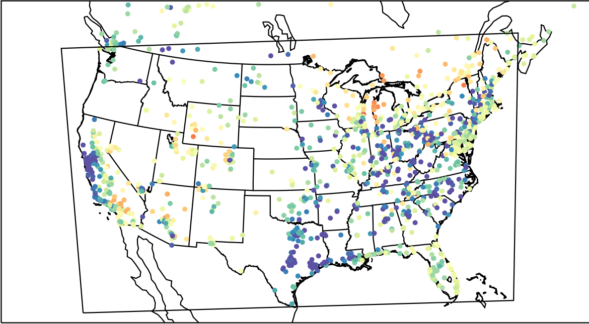
AirNOW (2023-04-11_03:00:00)
