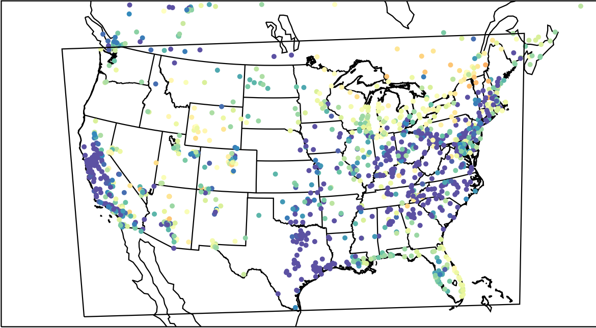
AirNOW (2023-04-11_09:00:00)
