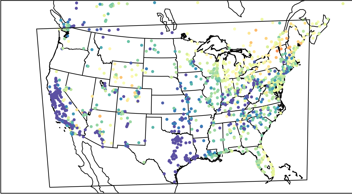
AirNOW (2023-04-11_13:00:00)
