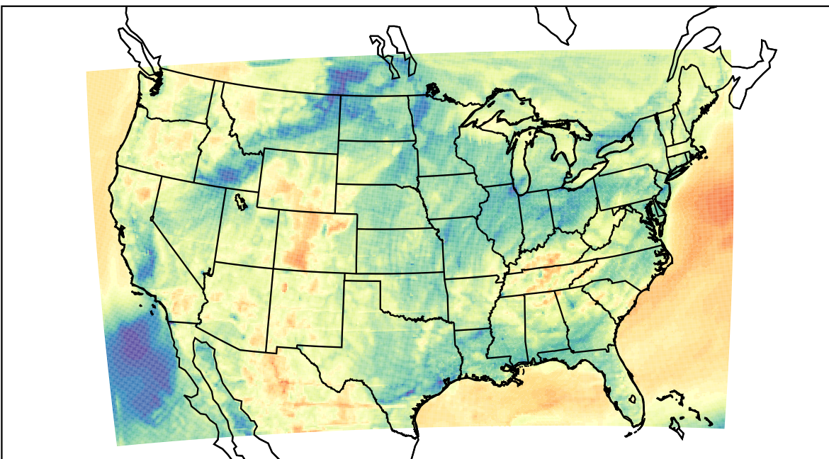
WRF (2023-04-12_04:00:00)
