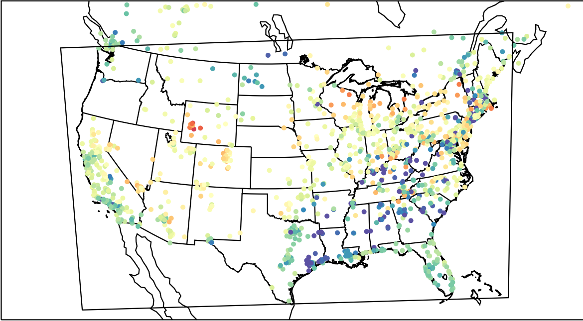
AirNOW (2023-04-13_02:00:00)
