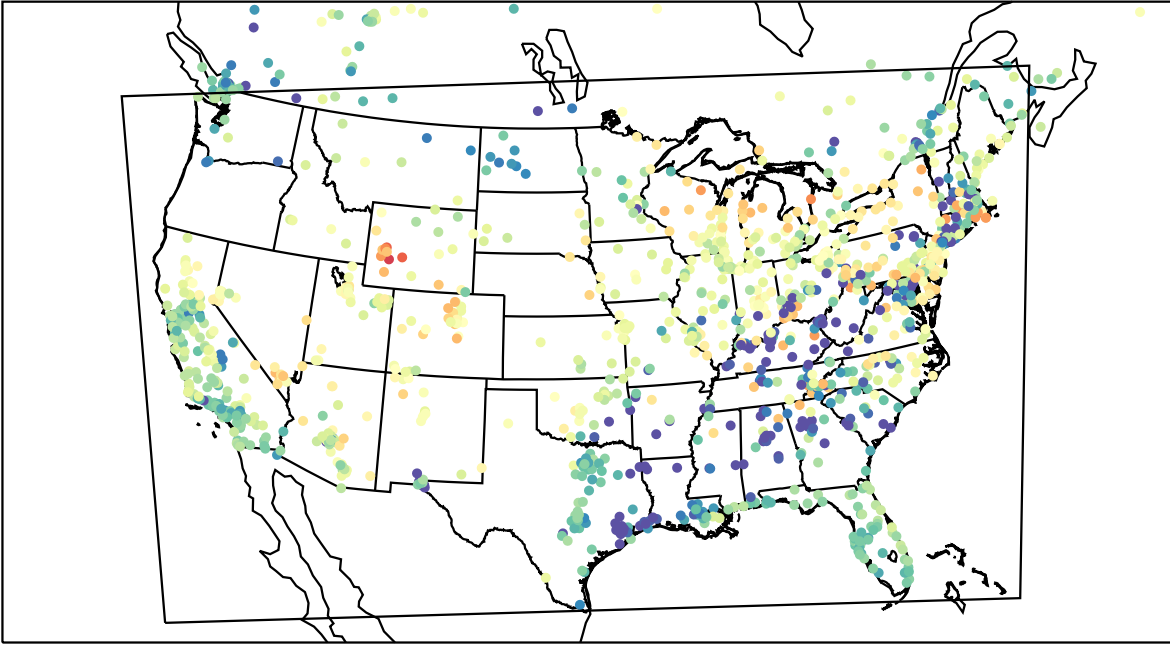
AirNOW (2023-04-13_03:00:00)
