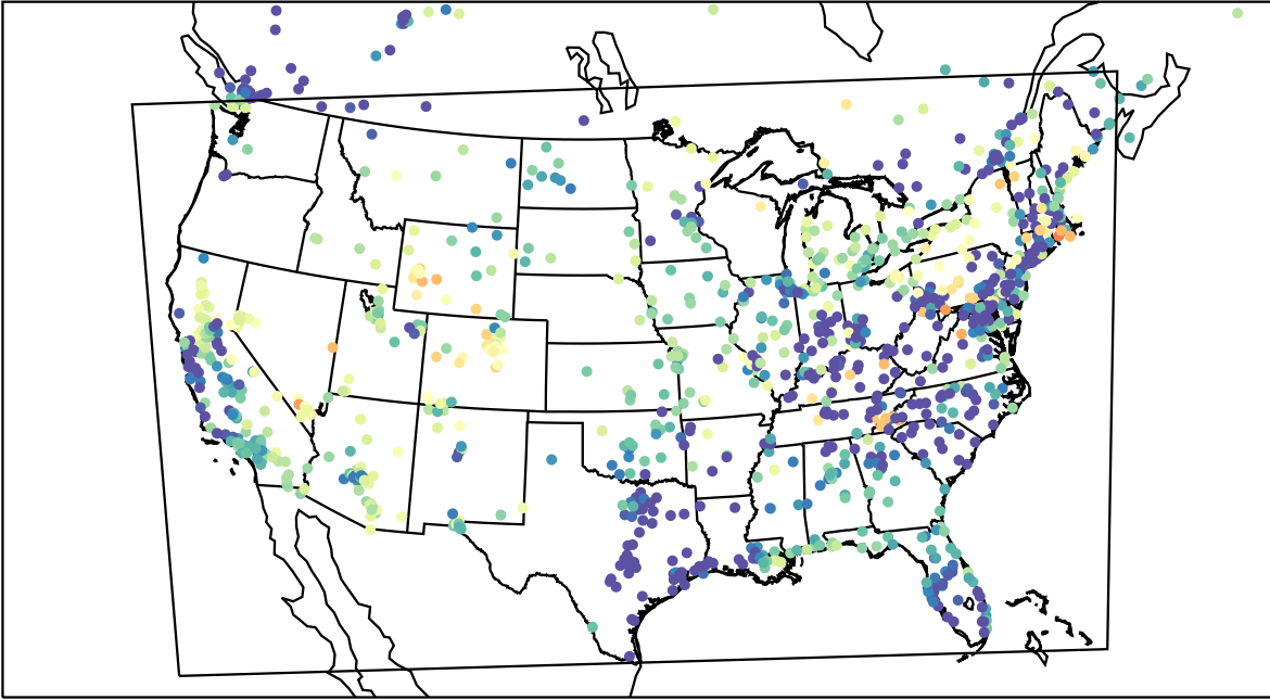
AirNOW (2023-04-13_10:00:00)
