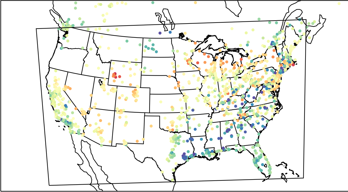
AirNOW (2023-04-13_01:00:00)
