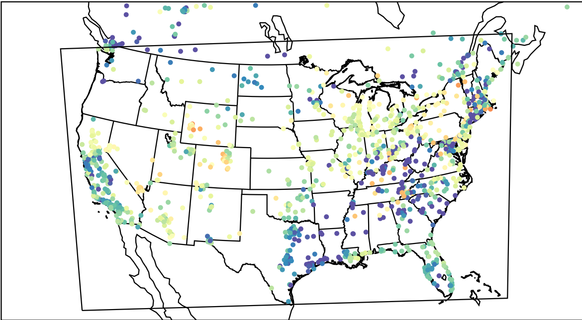
AirNOW (2023-04-13_06:00:00)
