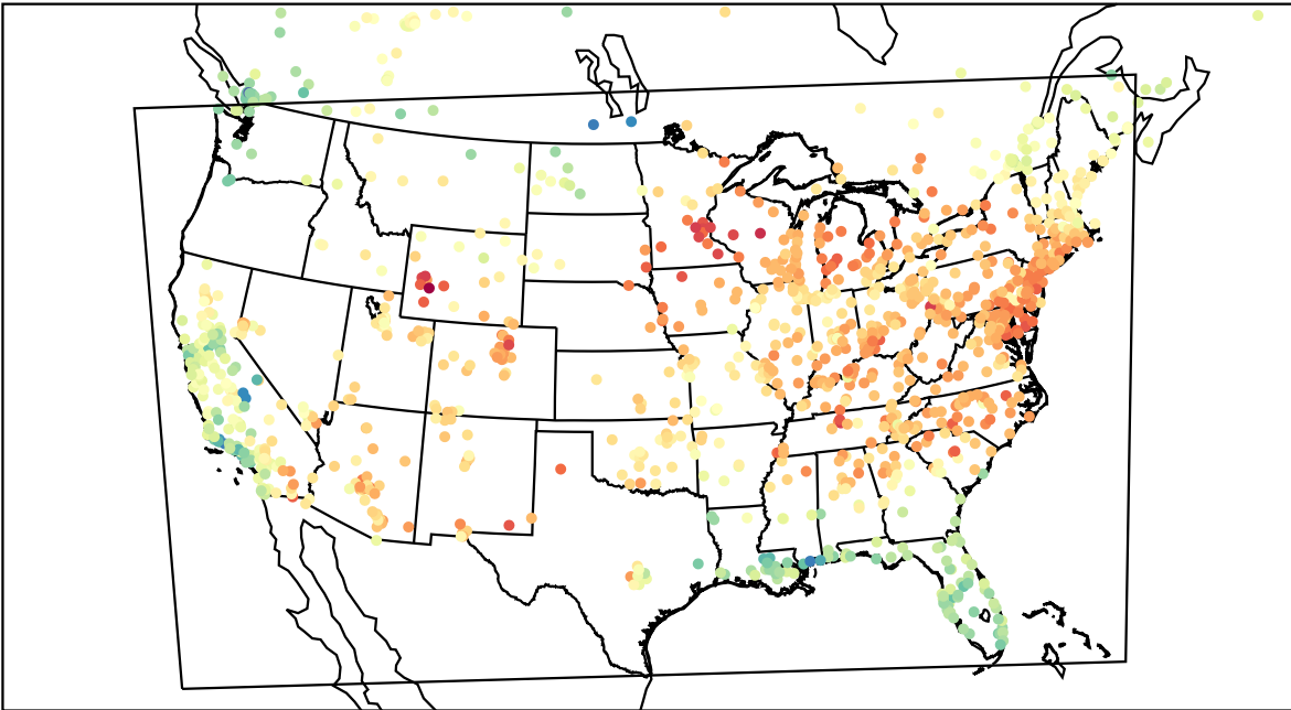
AirNOW (2023-04-12_21:00:00)
