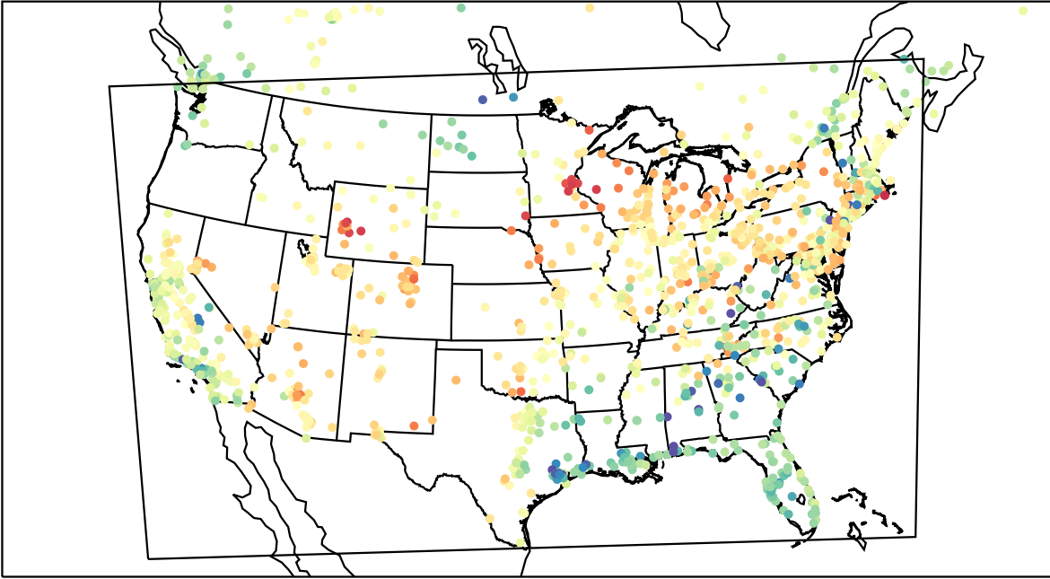
AirNOW (2023-04-13_00:00:00)
