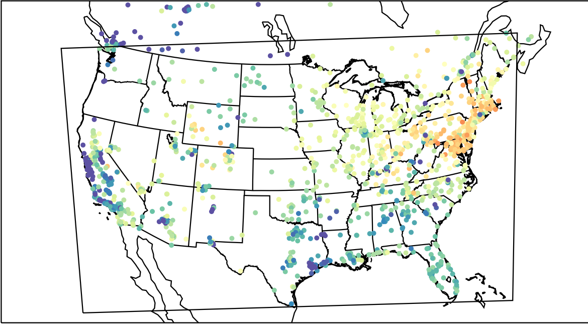
AirNOW (2023-04-13_14:00:00)
