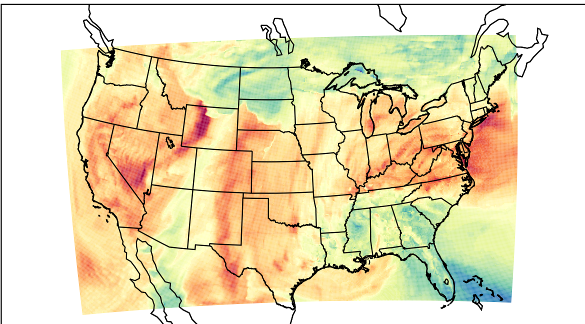
WRF (2023-04-13_22:00:00)
