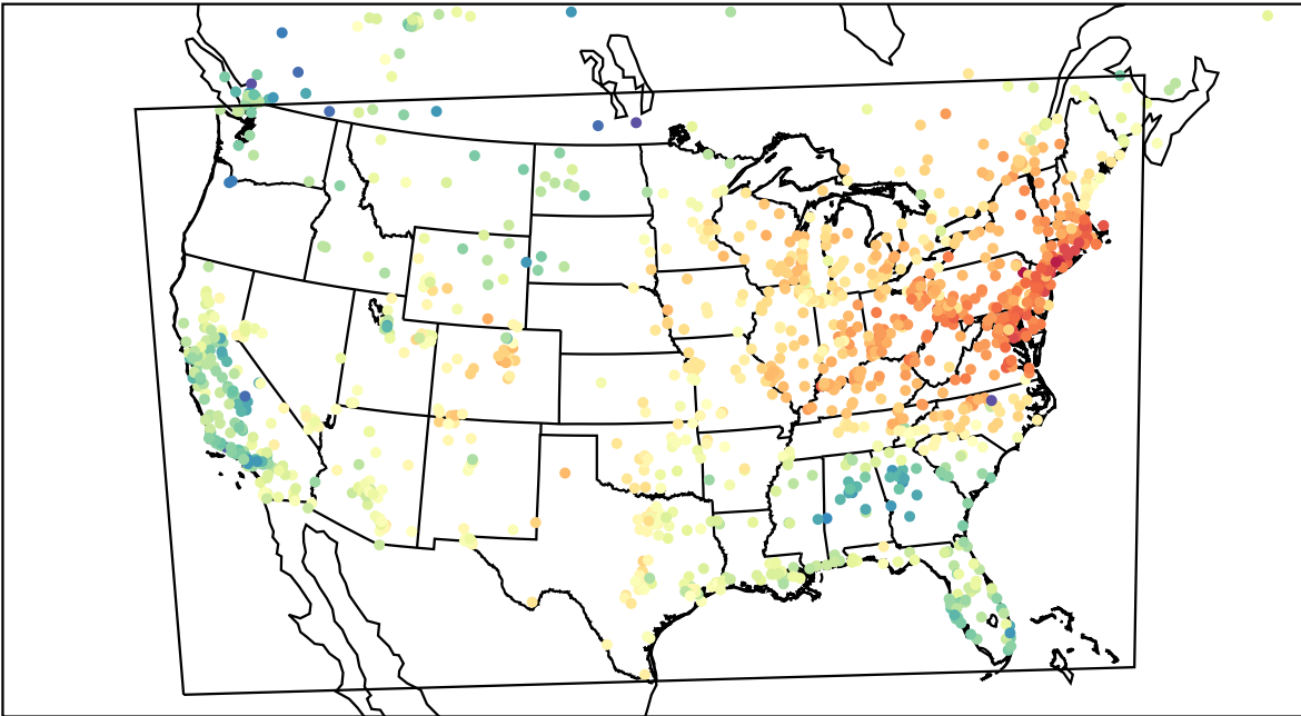
AirNOW (2023-04-13_17:00:00)
