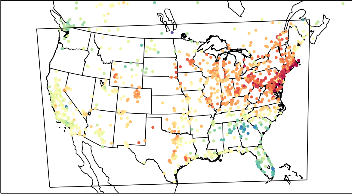
AirNOW (2023-04-13_21:00:00)
