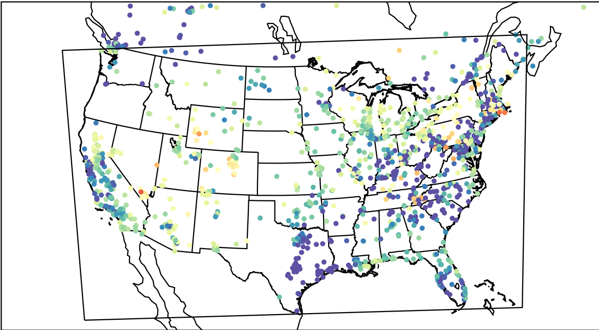
AirNOW (2023-04-13_09:00:00)
