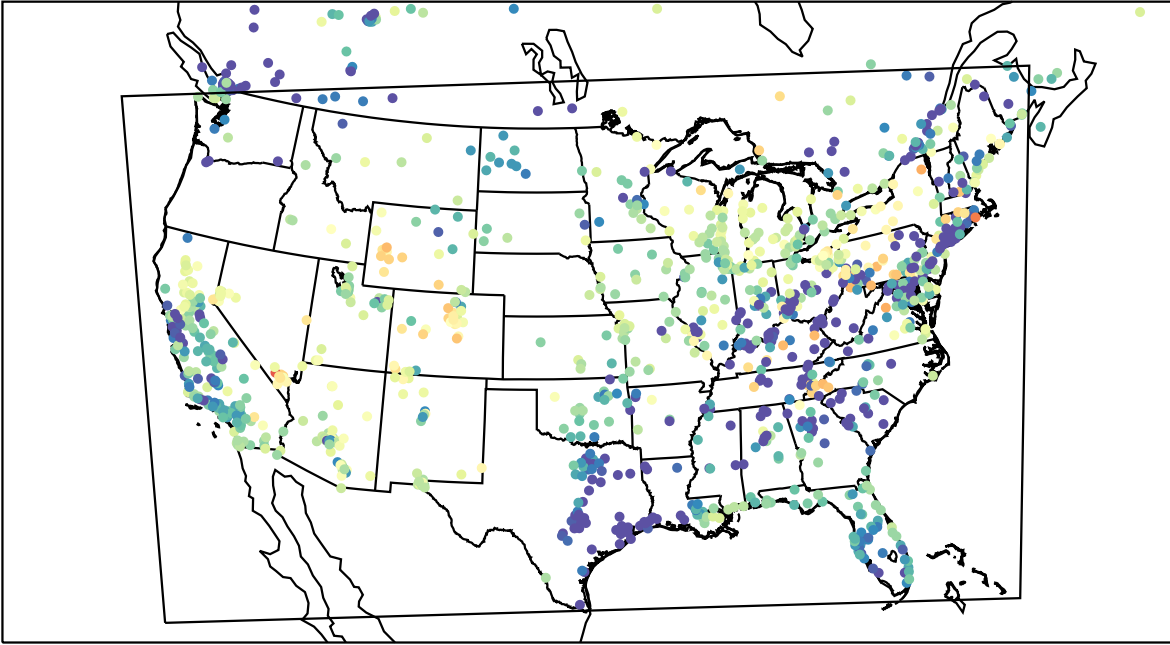
AirNOW (2023-04-13_08:00:00)
