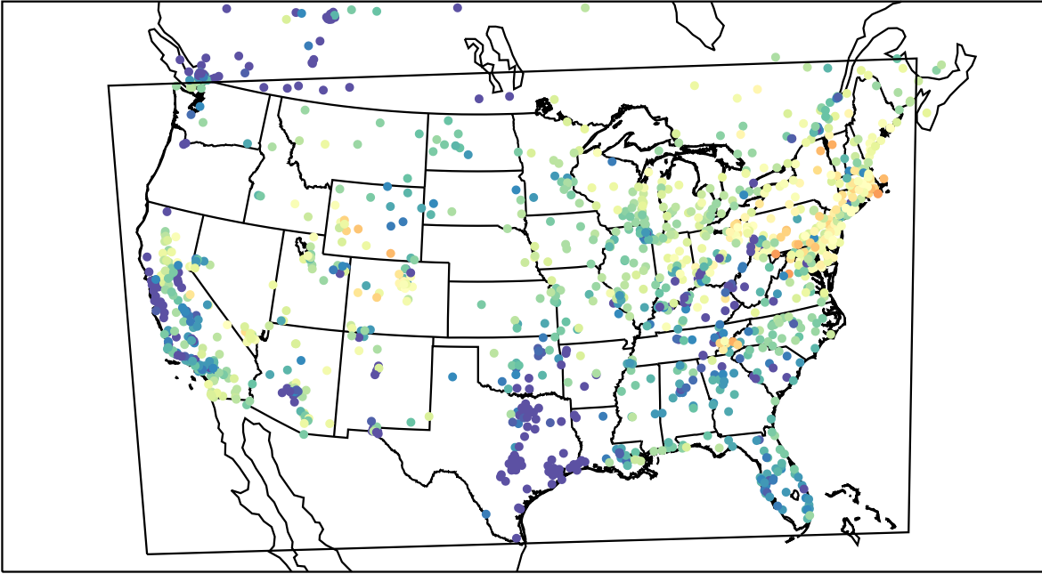
AirNOW (2023-04-13_13:00:00)
