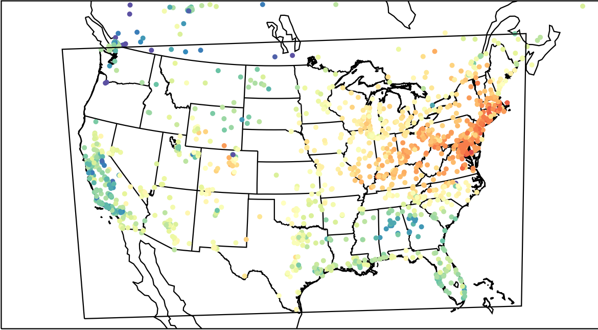
AirNOW (2023-04-13_16:00:00)
