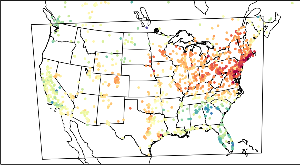
AirNOW (2023-04-13_20:00:00)
