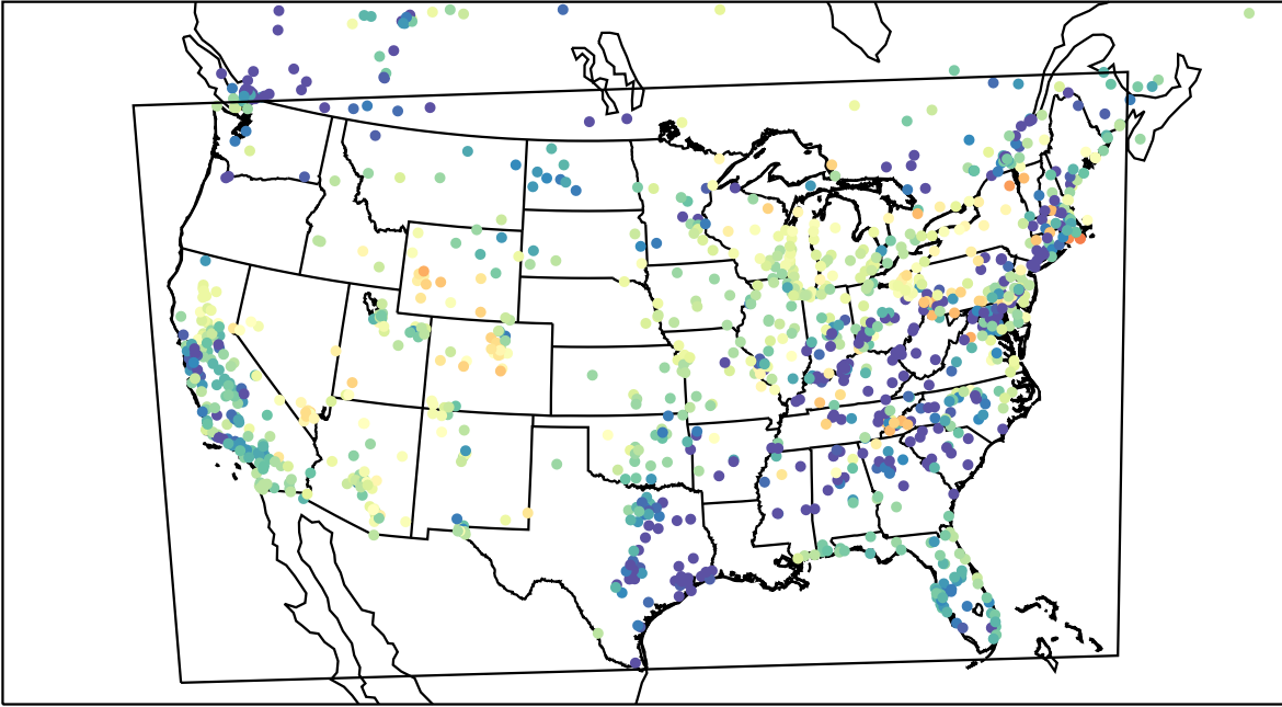
AirNOW (2023-04-13_07:00:00)
