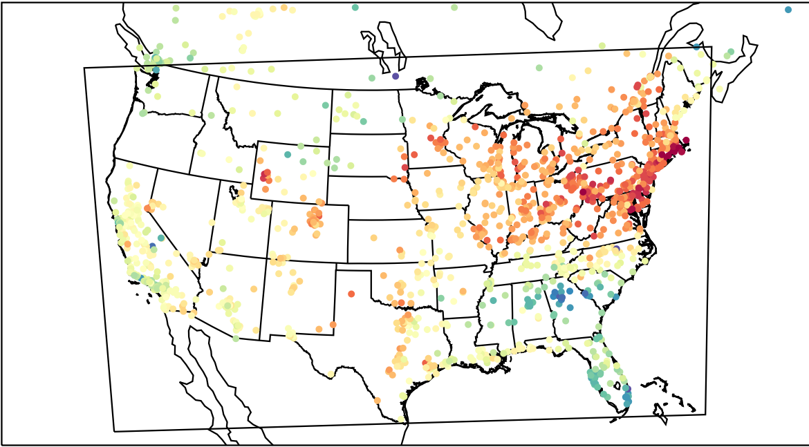
AirNOW (2023-04-13_22:00:00)
