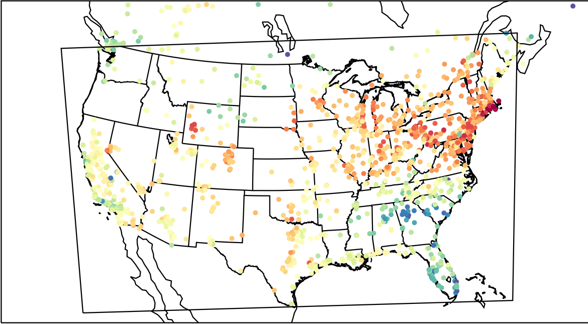
AirNOW (2023-04-13_23:00:00)
