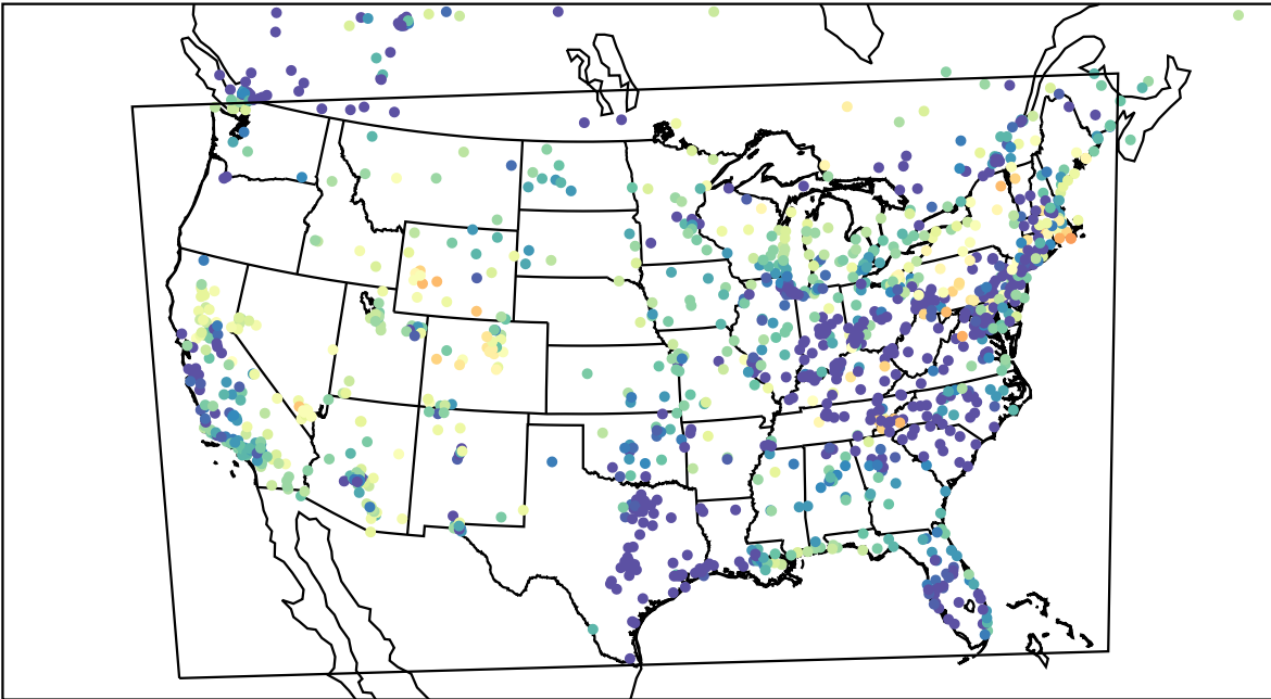
AirNOW (2023-04-13_11:00:00)
