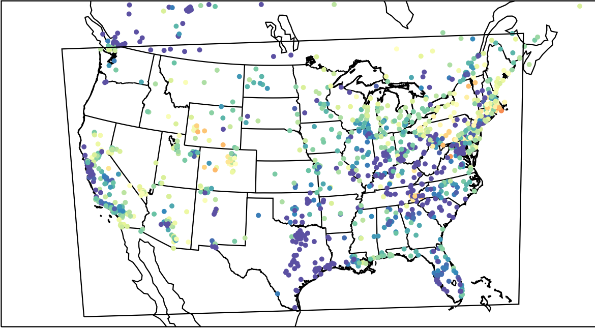
AirNOW (2023-04-13_12:00:00)
