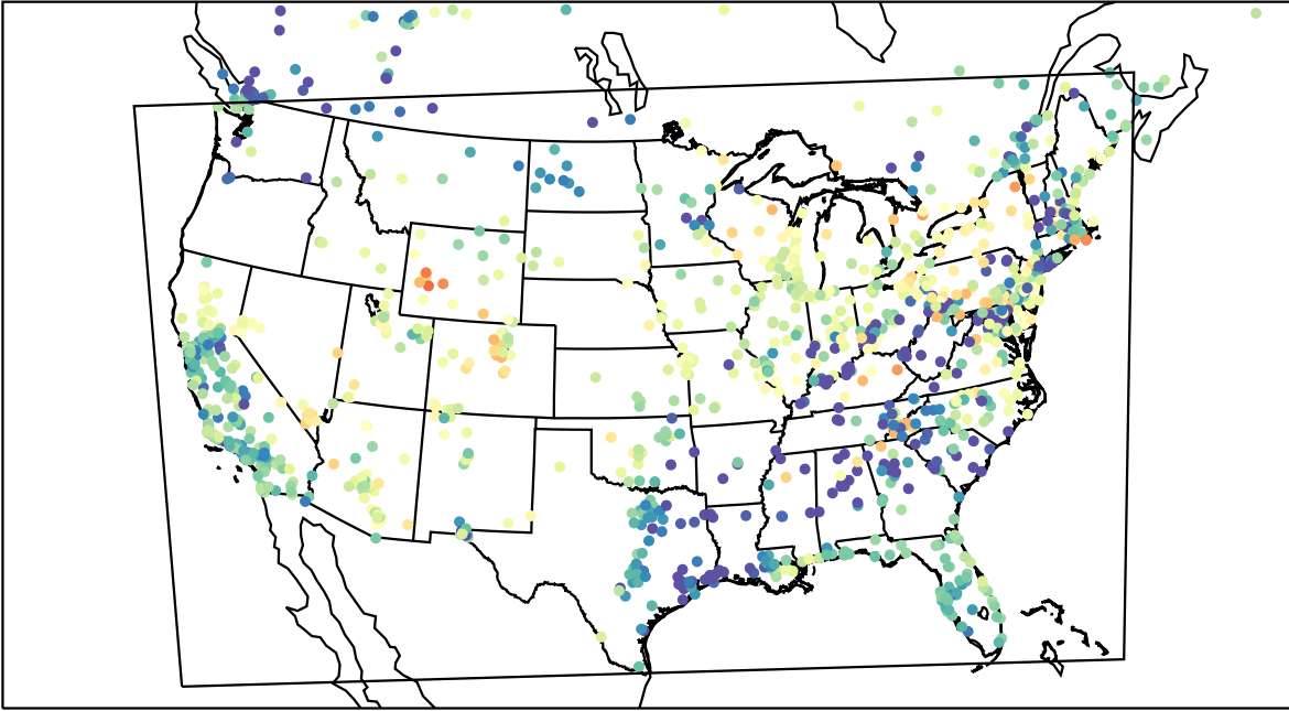
AirNOW (2023-04-13_05:00:00)
