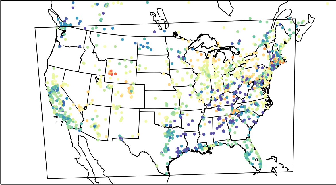
AirNOW (2023-04-13_04:00:00)
