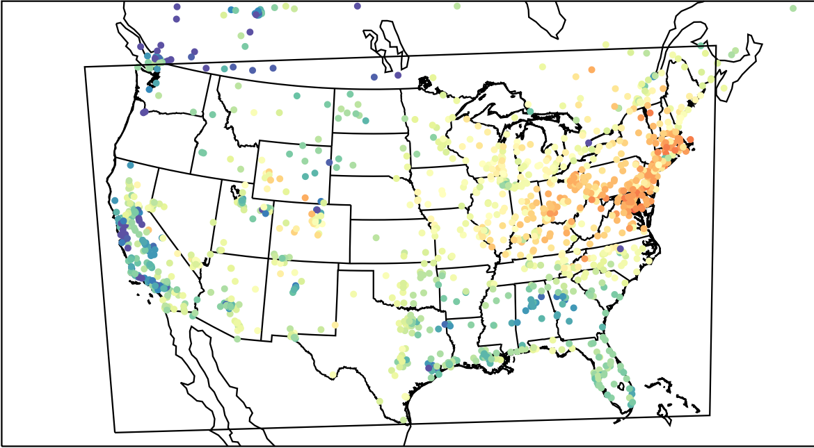
AirNOW (2023-04-13_15:00:00)
