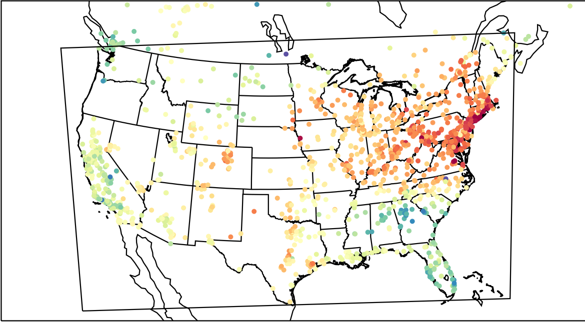
AirNOW (2023-04-13_19:00:00)
