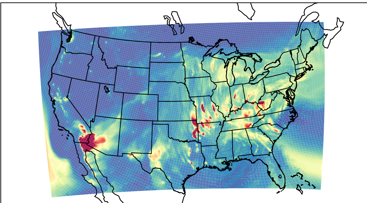
WRF 2023-04-14_04:00:00
