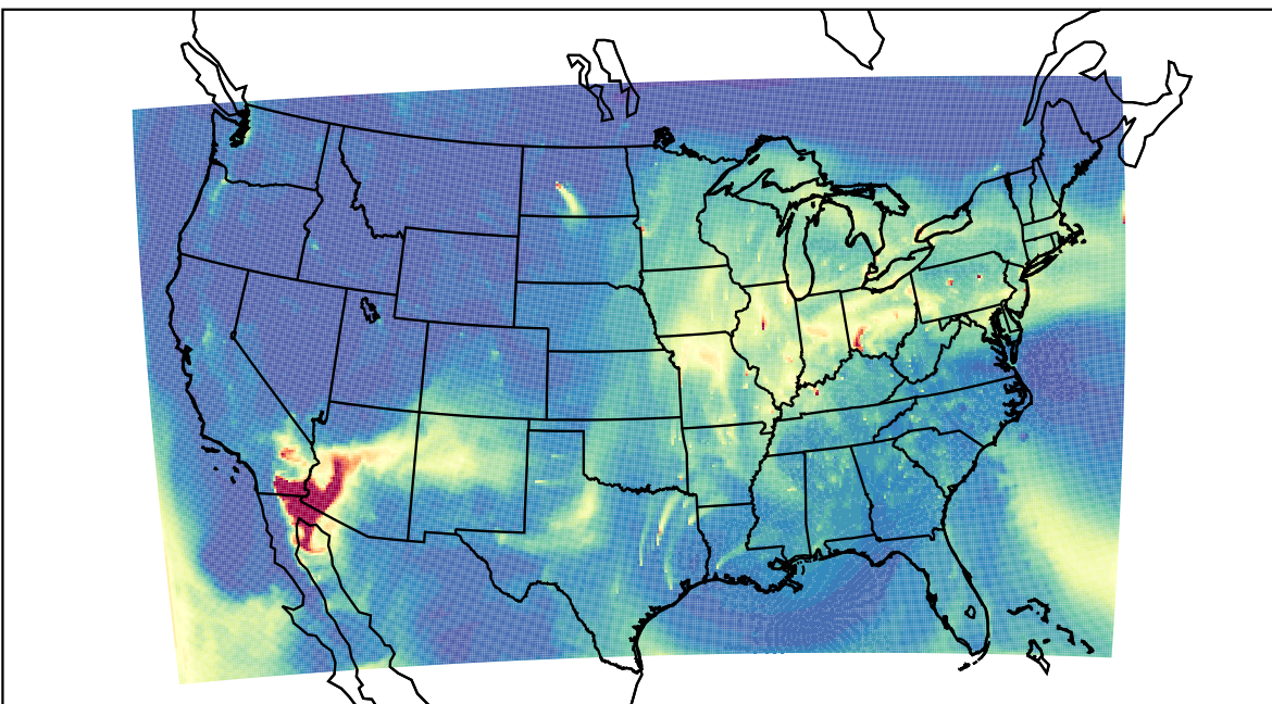
WRF 2023-04-14_15:00:00
