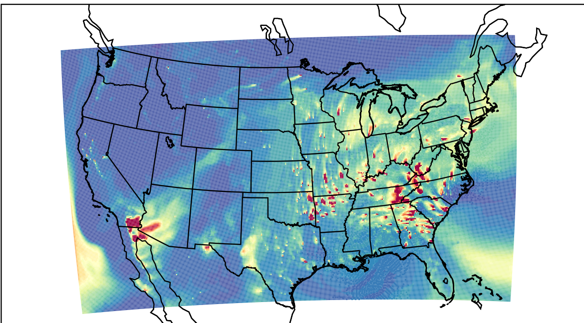
WRF 2023-04-14_01:00:00
