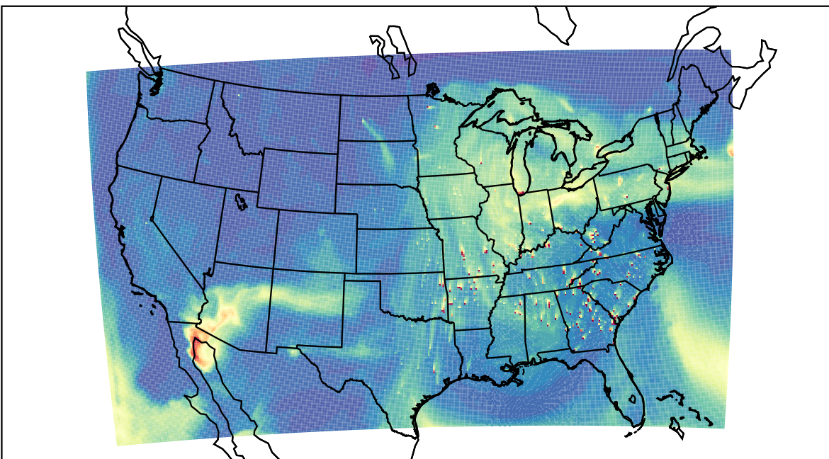
WRF 2023-04-14_20:00:00
