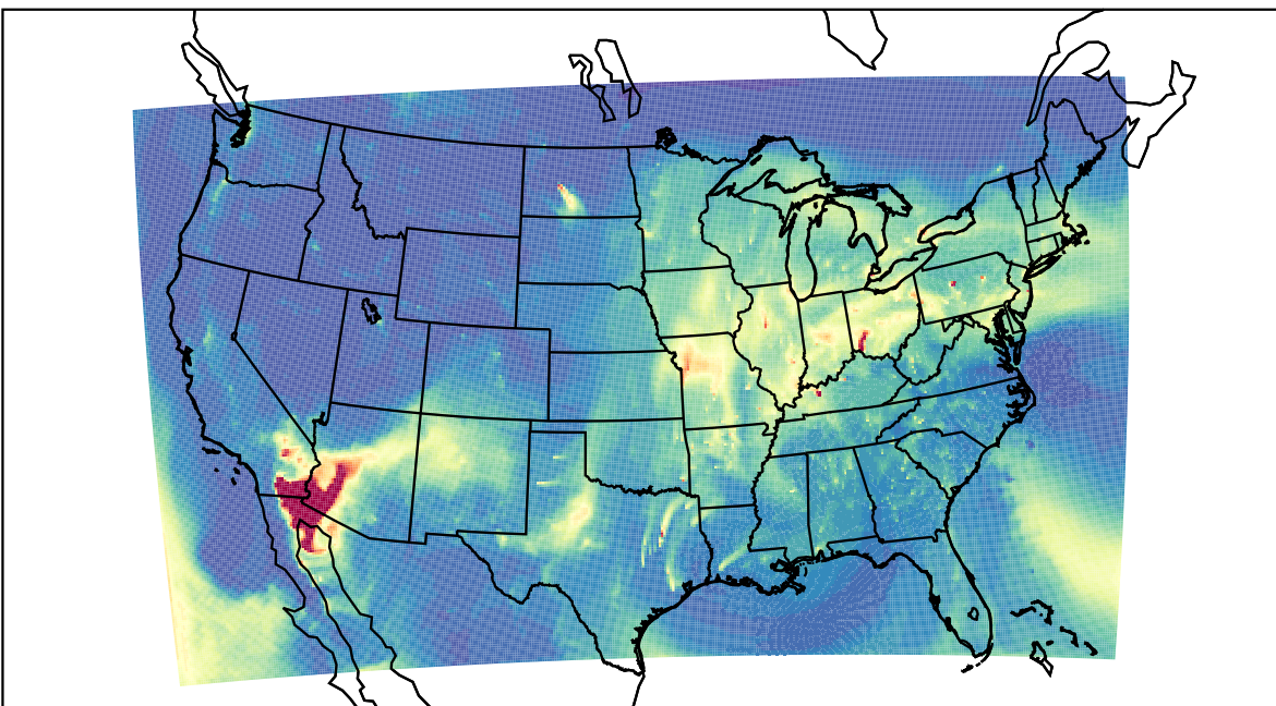
WRF 2023-04-14_14:00:00
