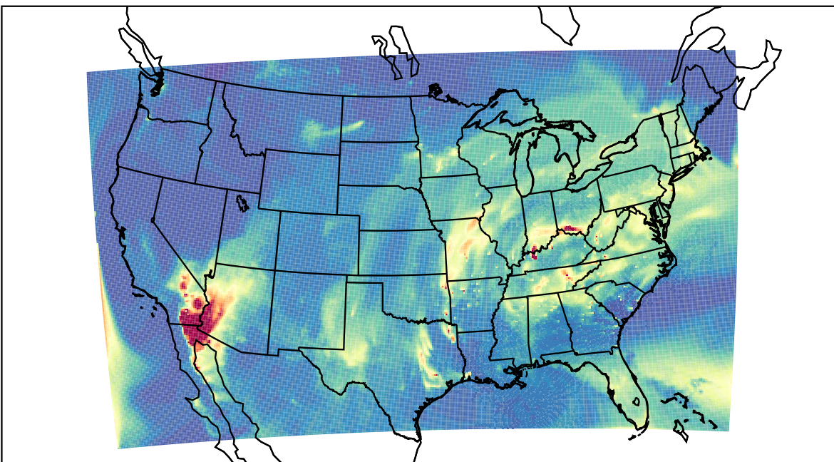
WRF 2023-04-13_11:00:00
