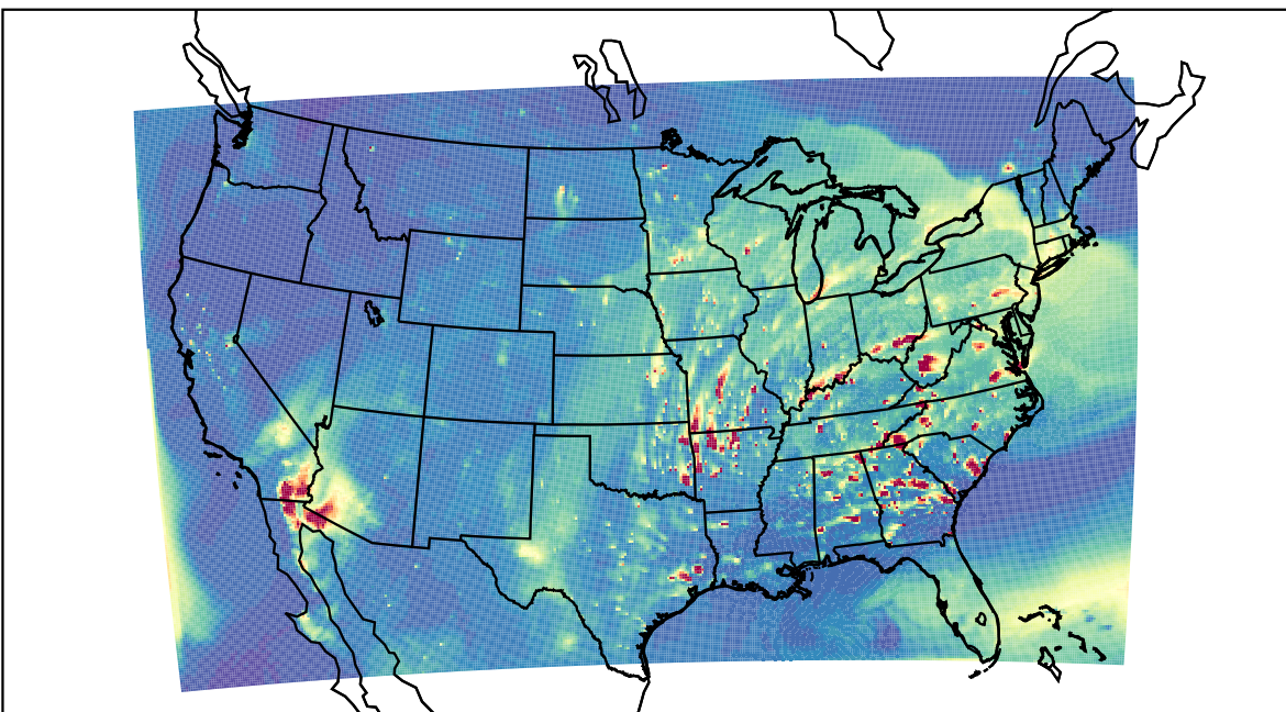
WRF 2023-04-13_01:00:00
