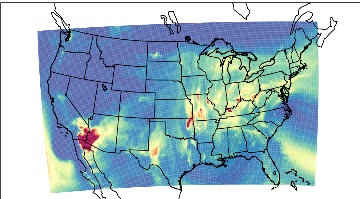
WRF 2023-04-14_08:00:00
