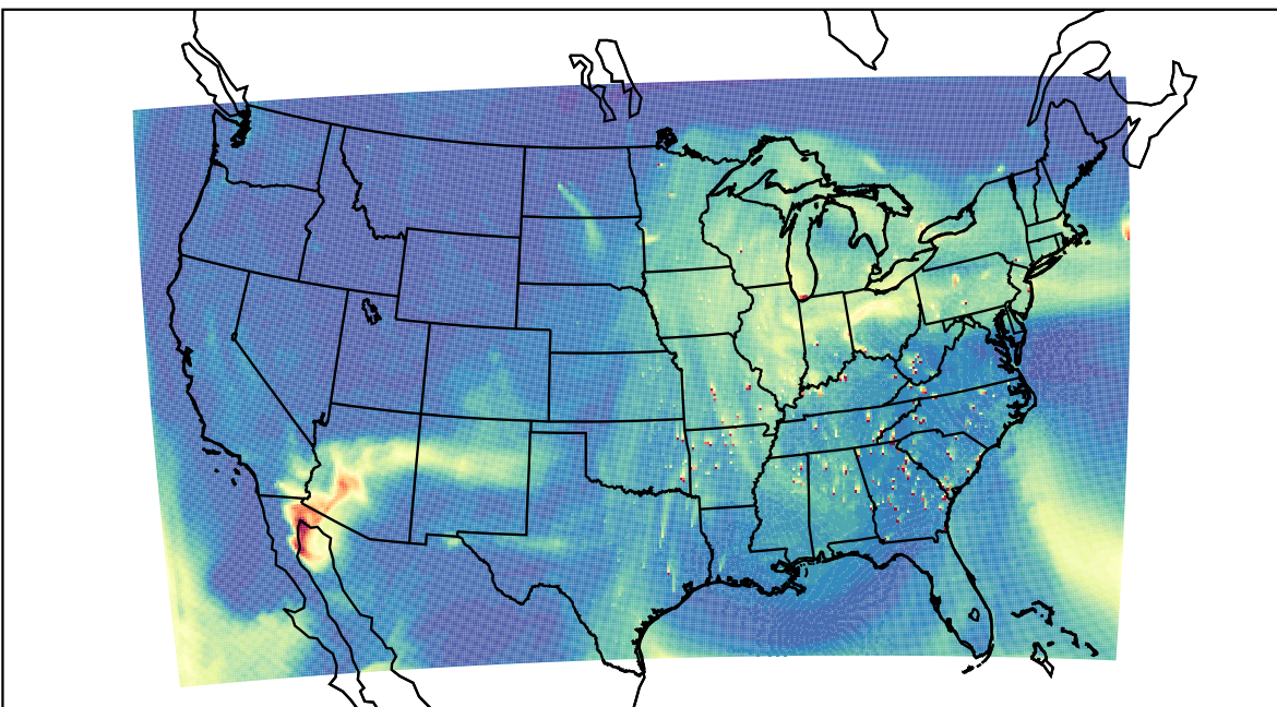
WRF 2023-04-14_19:00:00
