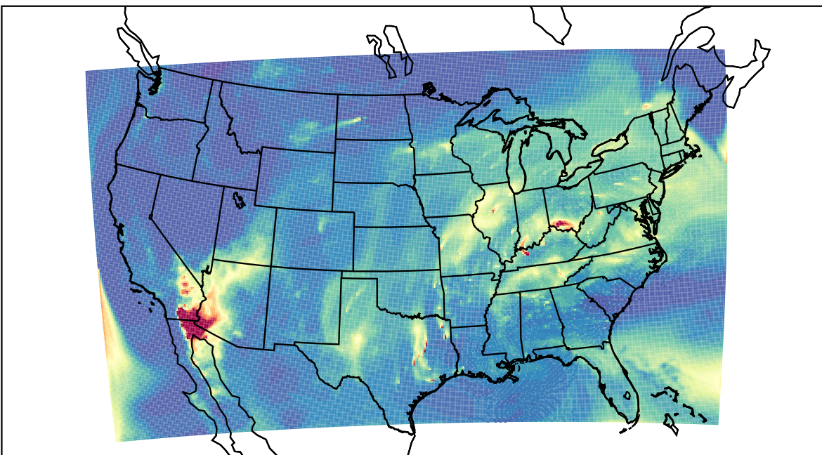
WRF 2023-04-13_15:00:00
