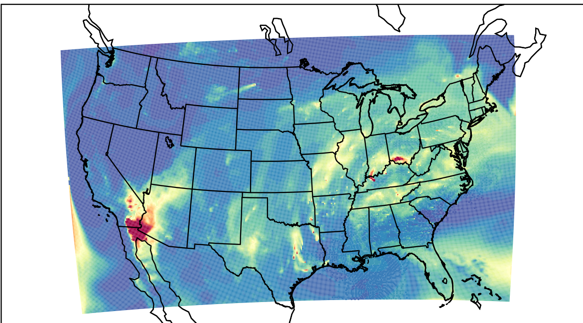
WRF 2023-04-13_14:00:00
