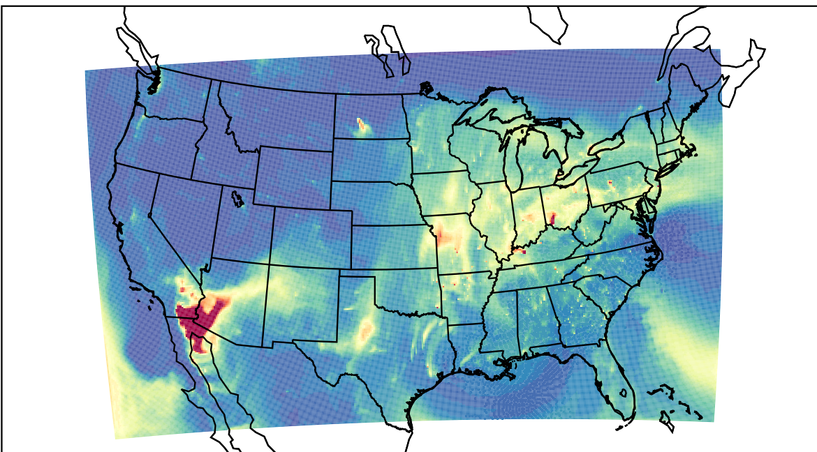
WRF 2023-04-14_13:00:00
