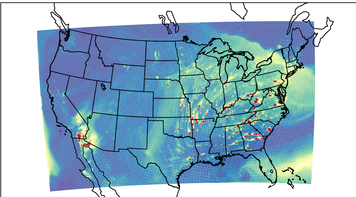
WRF 2023-04-13_00:00:00
