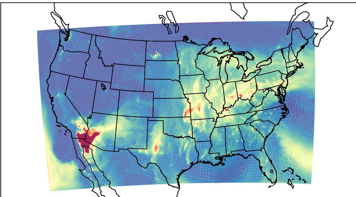
WRF 2023-04-14_11:00:00
