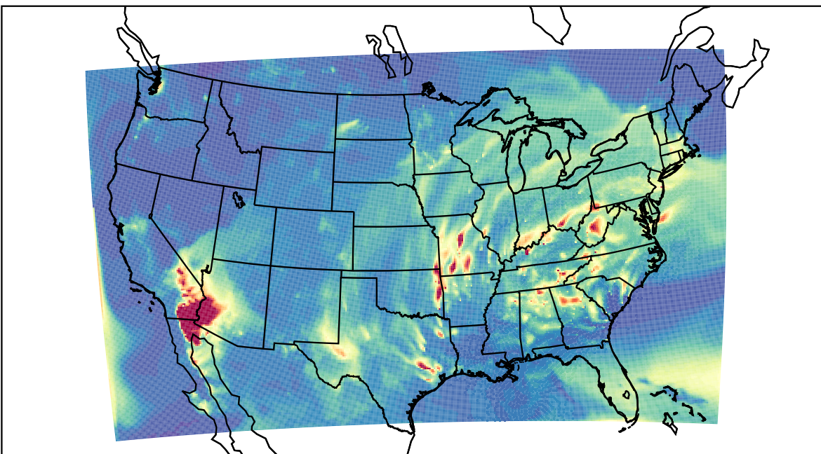
WRF 2023-04-13_06:00:00
