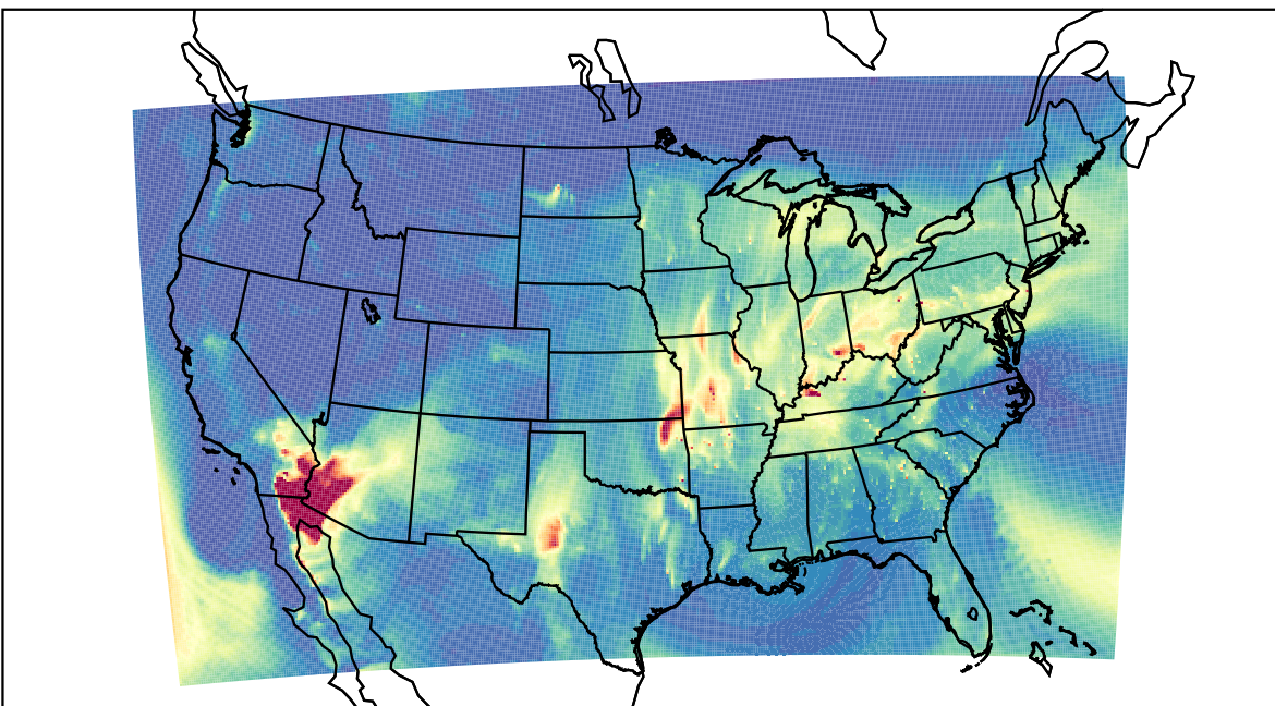
WRF 2023-04-14_09:00:00
