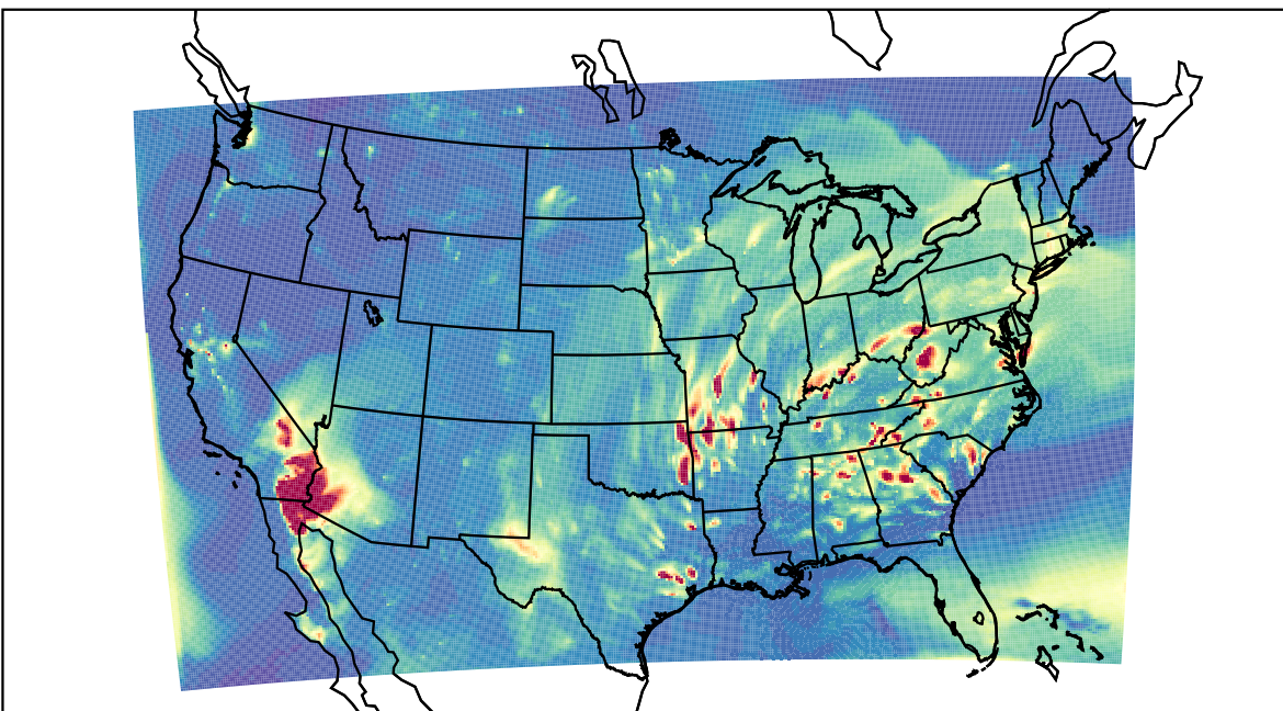
WRF 2023-04-13_04:00:00
