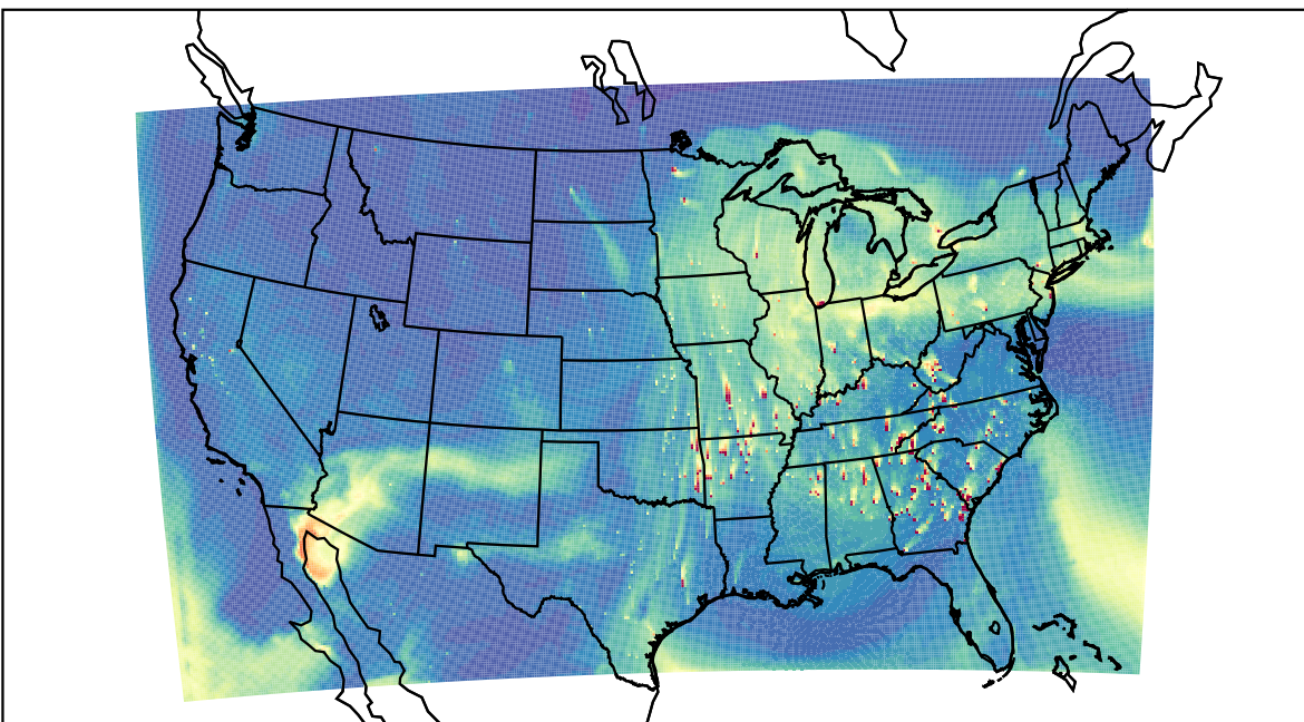
WRF 2023-04-14_22:00:00
