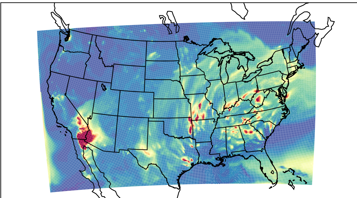
WRF 2023-04-13_05:00:00
