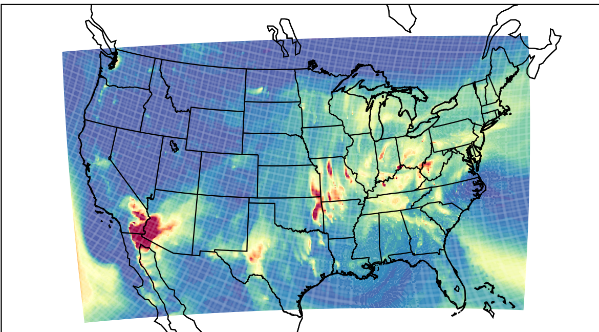
WRF 2023-04-14_06:00:00
