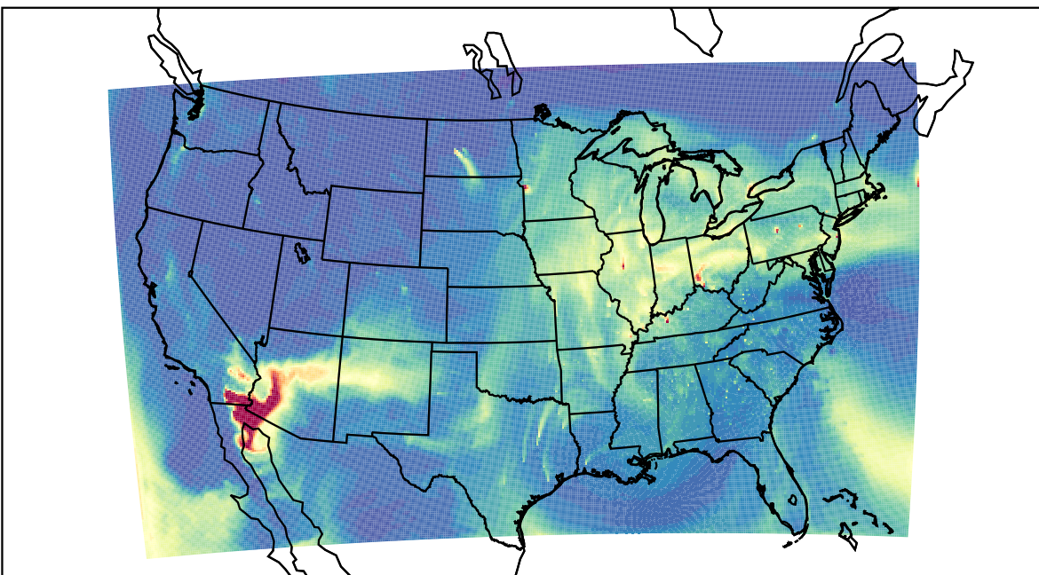
WRF 2023-04-14_16:00:00
