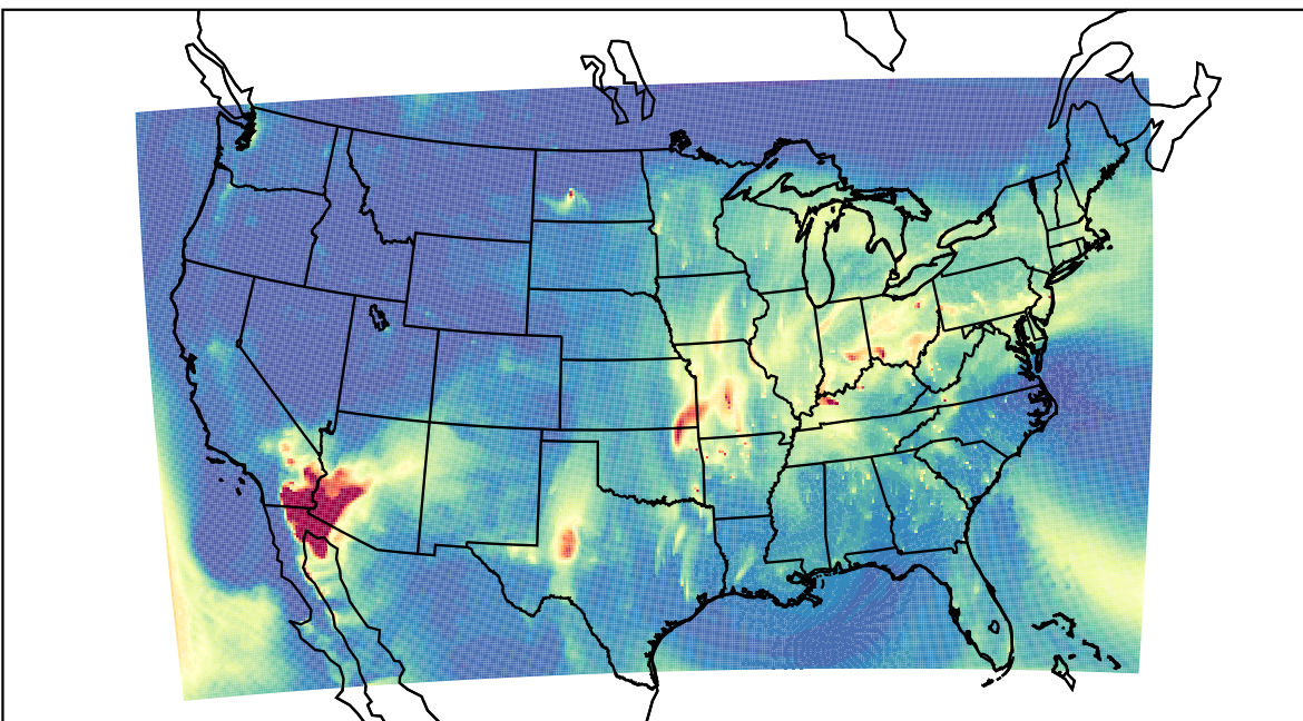
WRF 2023-04-14_10:00:00
