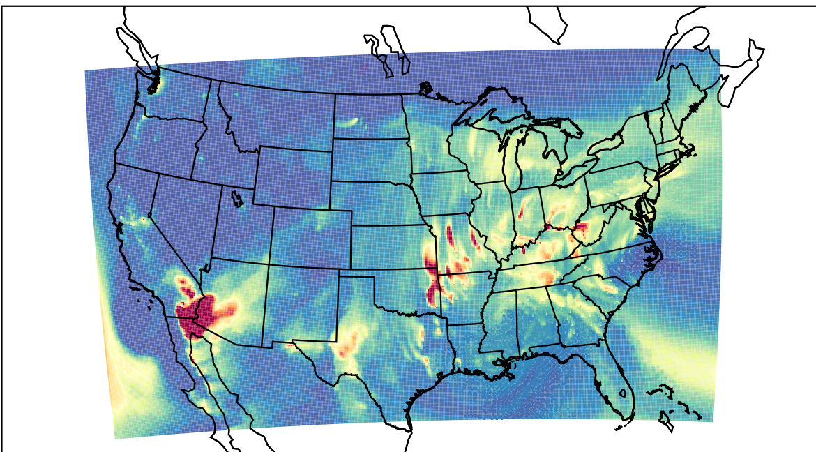
WRF 2023-04-14_05:00:00
