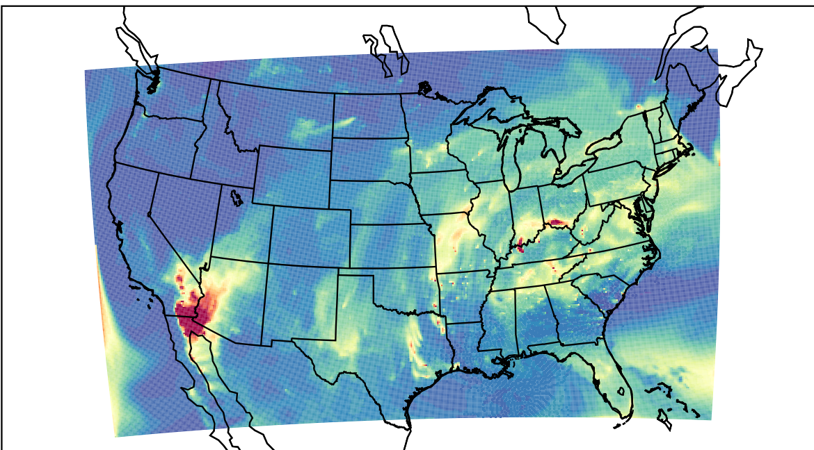
WRF 2023-04-13_12:00:00
