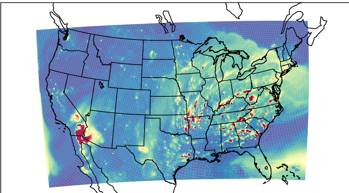
WRF 2023-04-13_02:00:00
