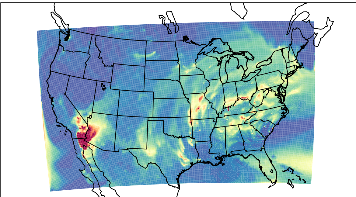
WRF 2023-04-13_09:00:00
