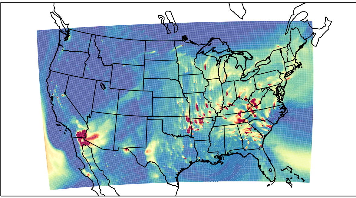
WRF 2023-04-14_02:00:00
