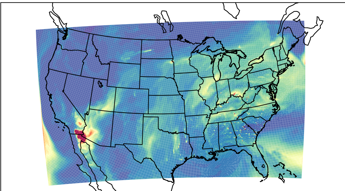
WRF 2023-04-13_17:00:00
