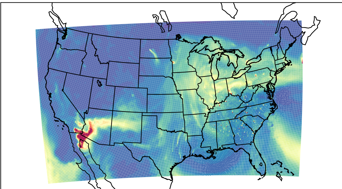
WRF 2023-04-14_17:00:00
