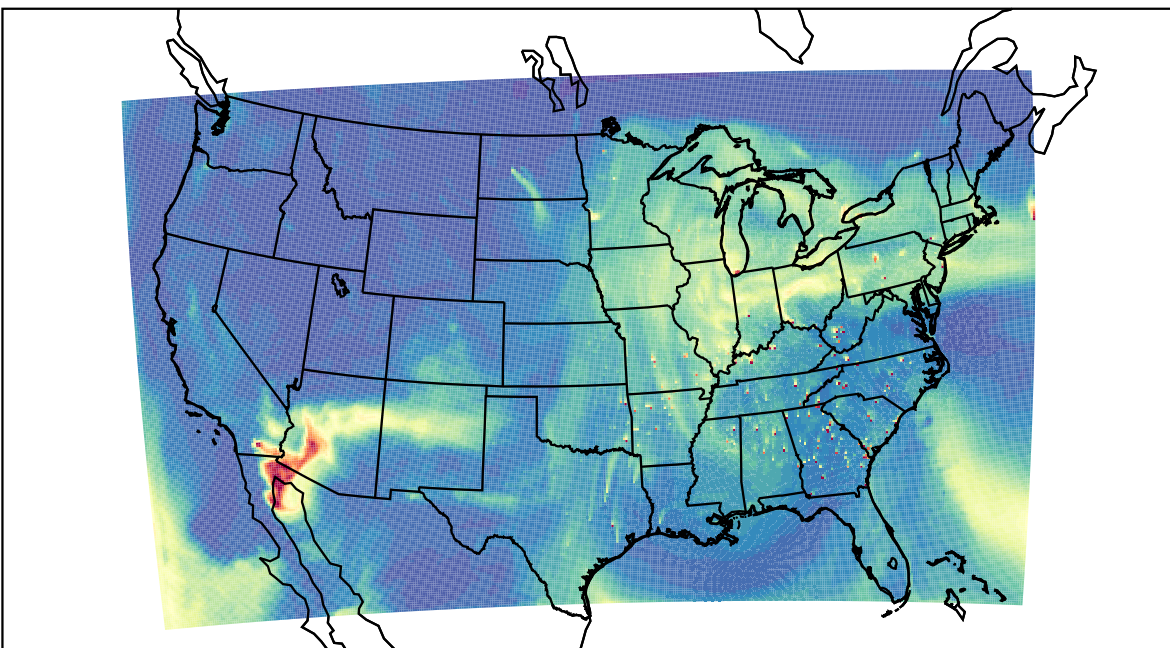
WRF 2023-04-14_18:00:00
