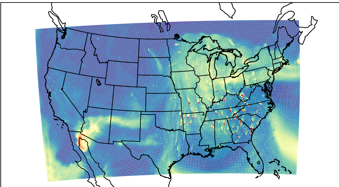
WRF 2023-04-14_21:00:00
