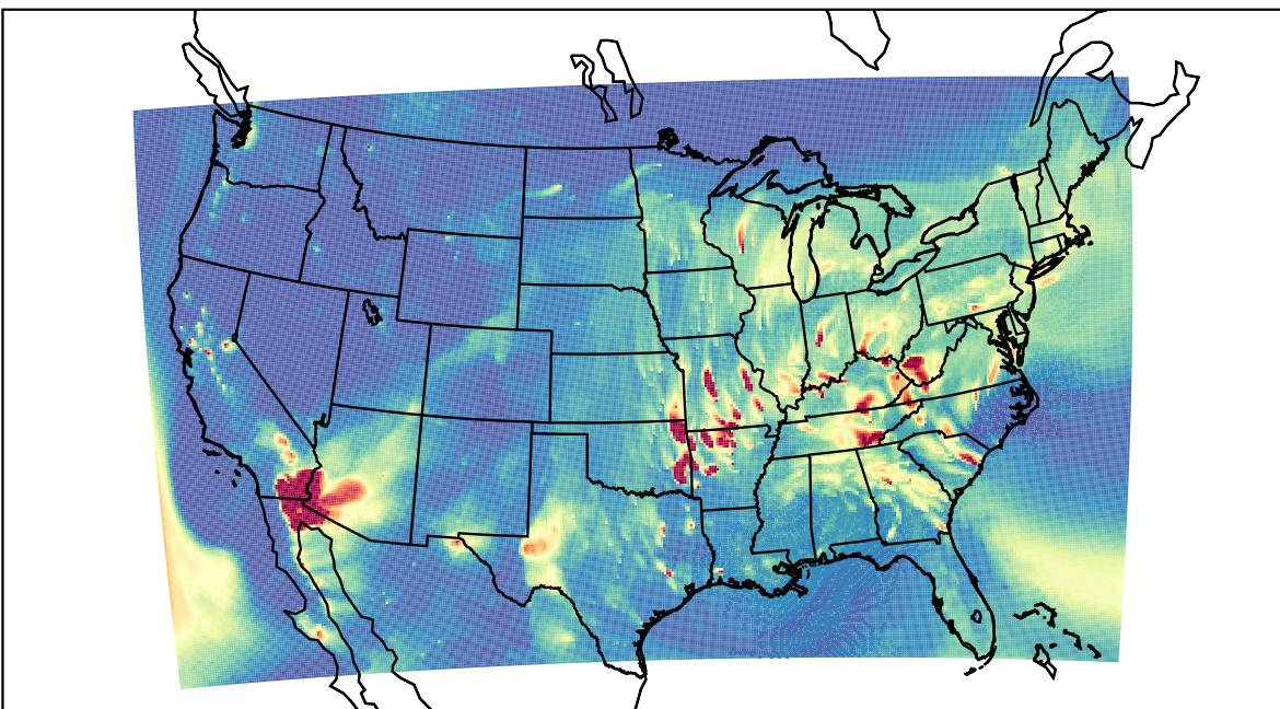
WRF 2023-04-14_03:00:00
