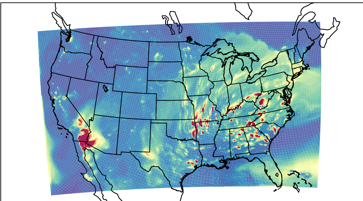
WRF 2023-04-13_03:00:00
