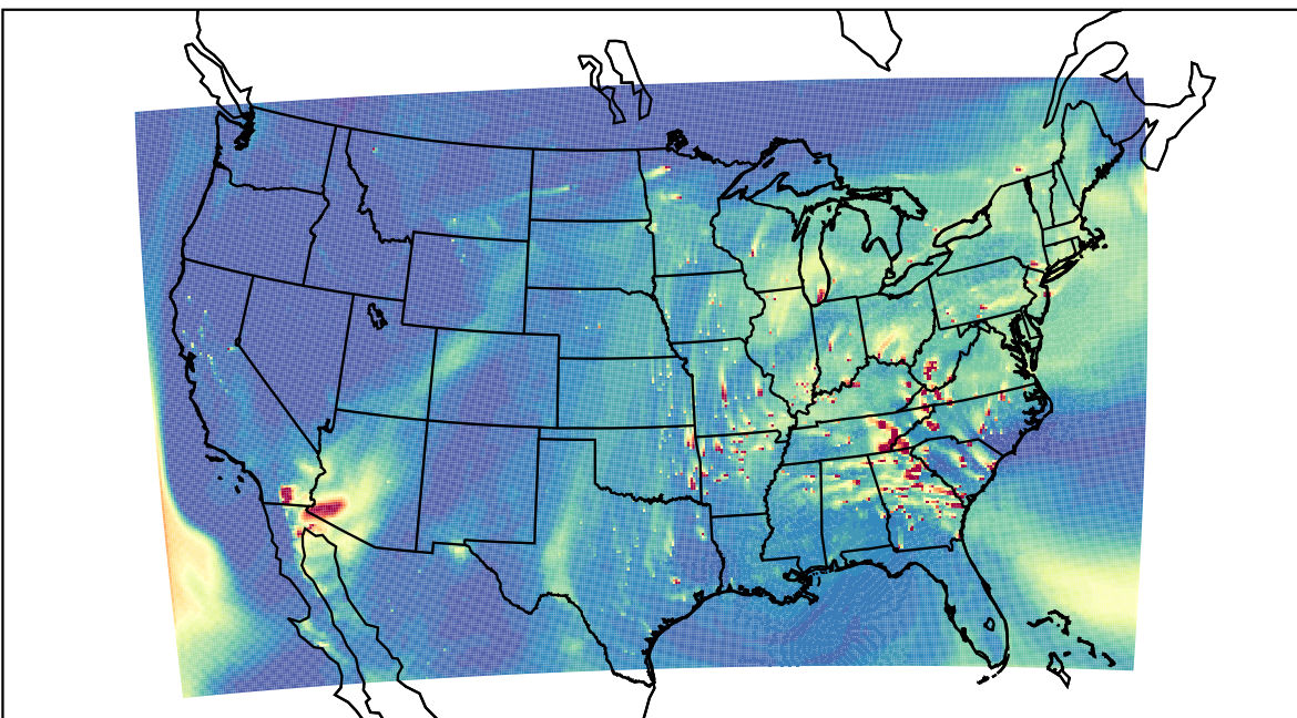
WRF 2023-04-13_23:00:00
