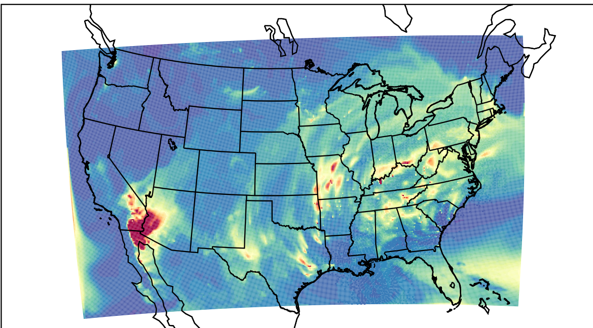
WRF 2023-04-13_08:00:00
