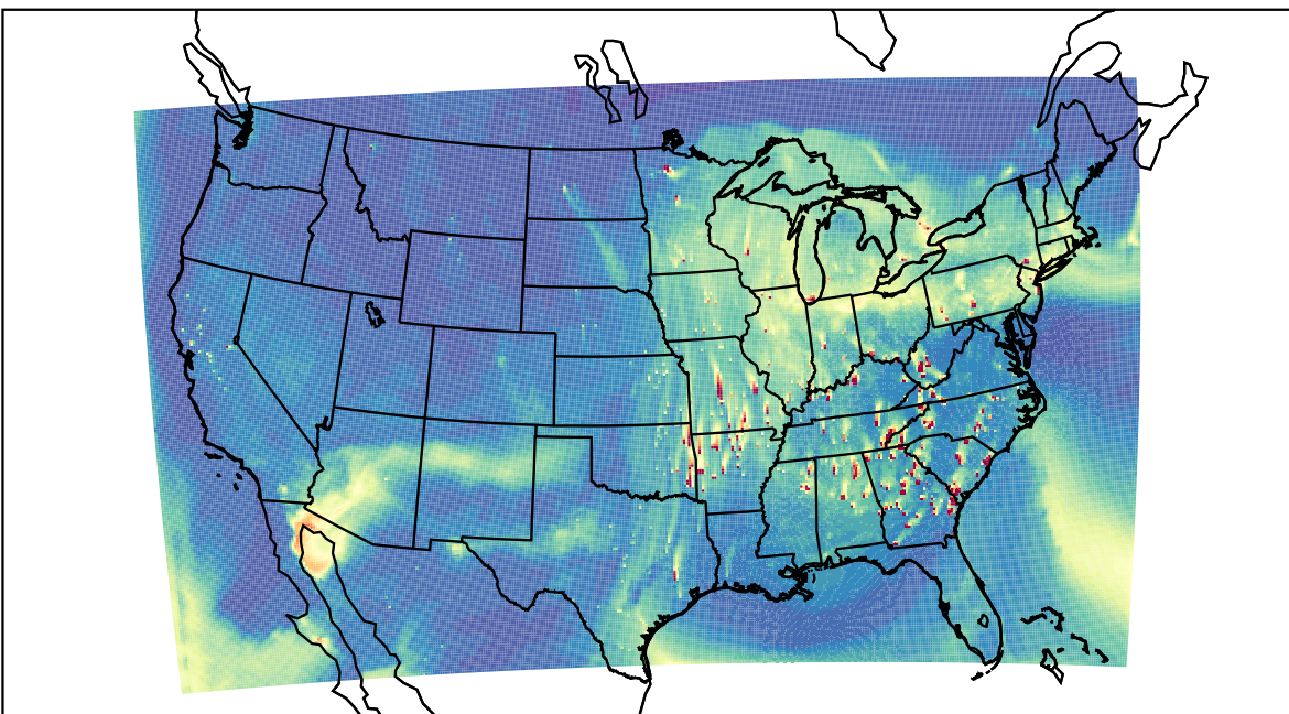
WRF 2023-04-14_23:00:00
