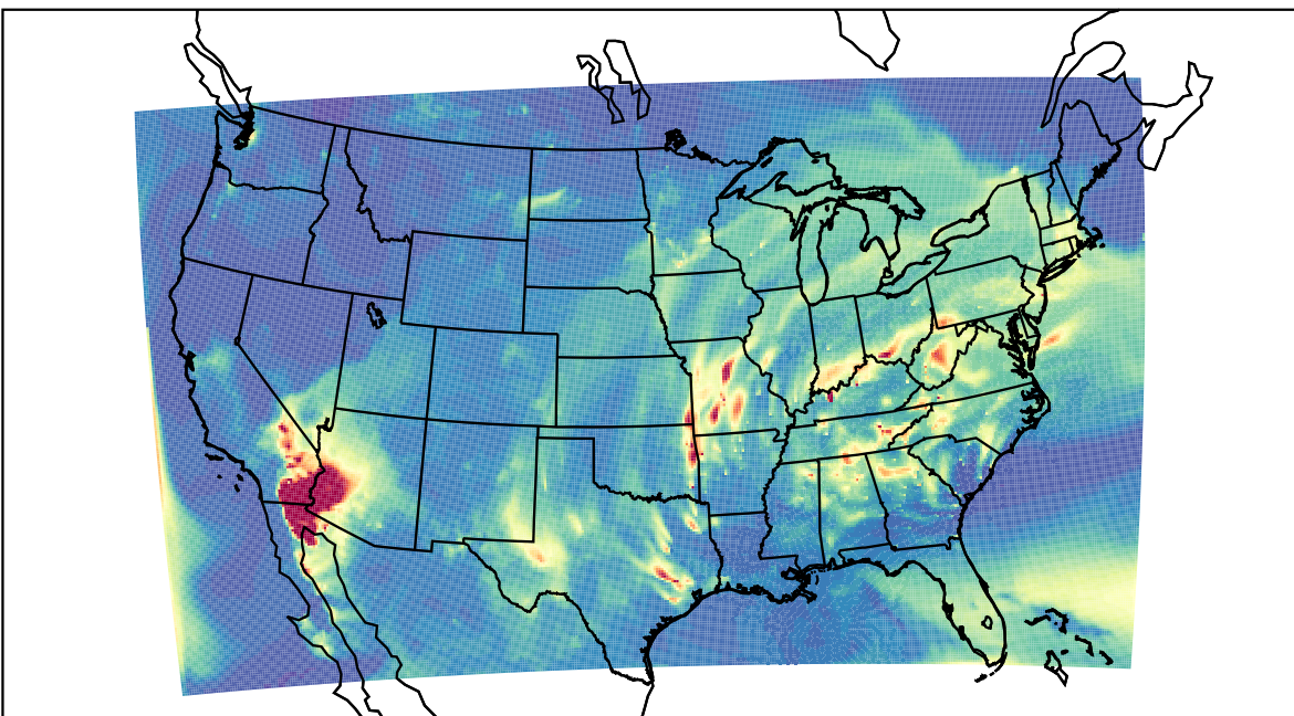
WRF 2023-04-13_07:00:00
