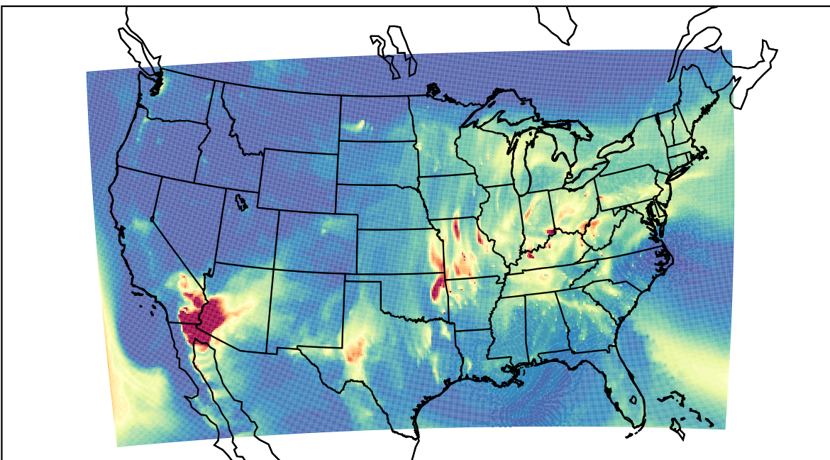
WRF 2023-04-14_07:00:00
