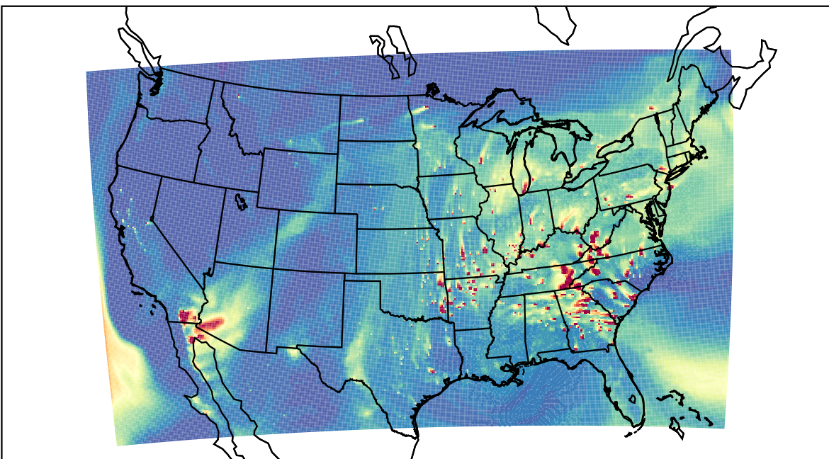
WRF 2023-04-14_00:00:00
