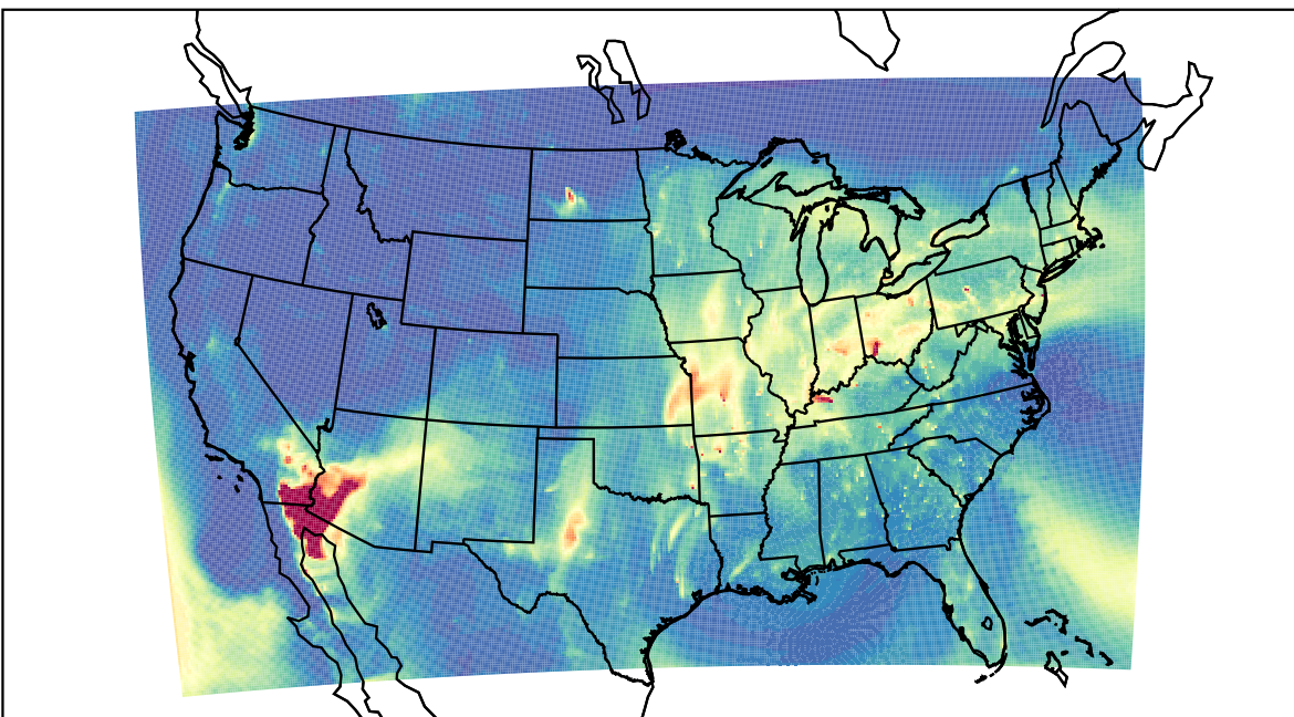
WRF 2023-04-14_12:00:00
