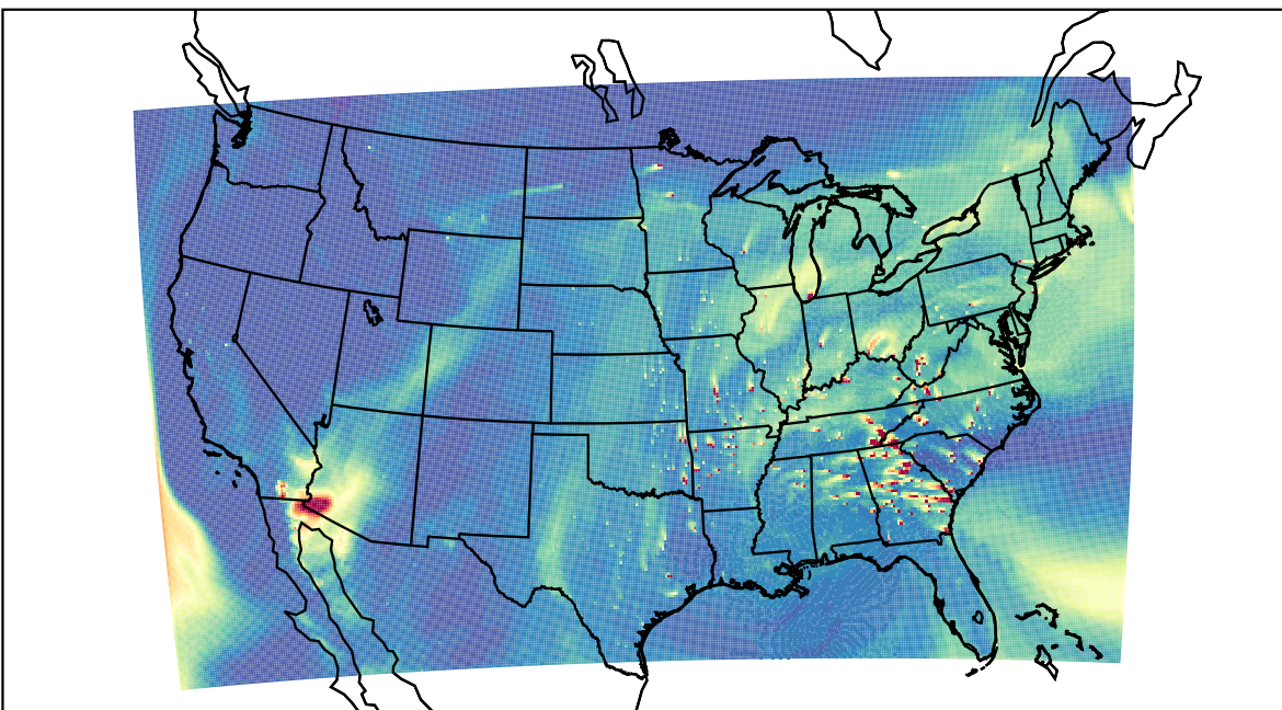
WRF 2023-04-13_21:00:00
