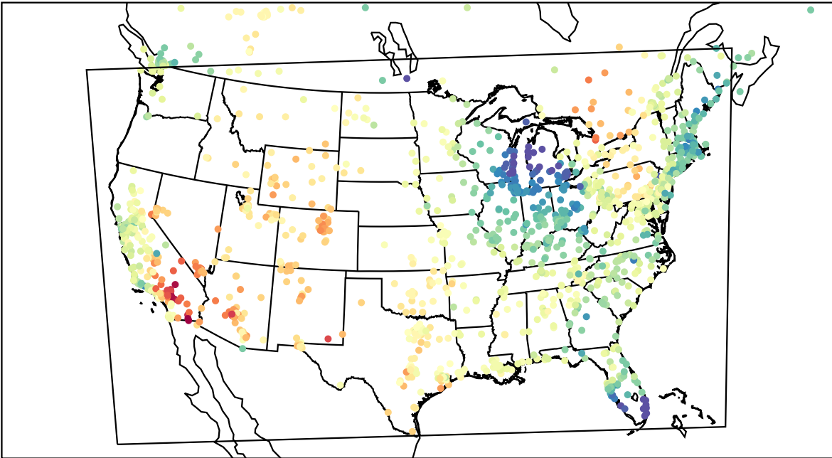
AirNOW (2023-04-16_22:00:00)
