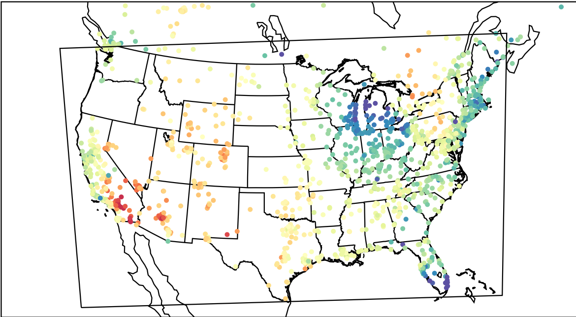
AirNOW (2023-04-16_23:00:00)
