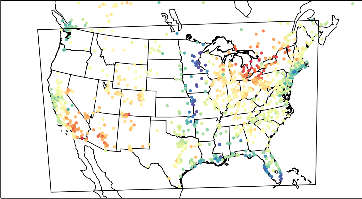
AirNOW (2023-04-15_21:00:00)
