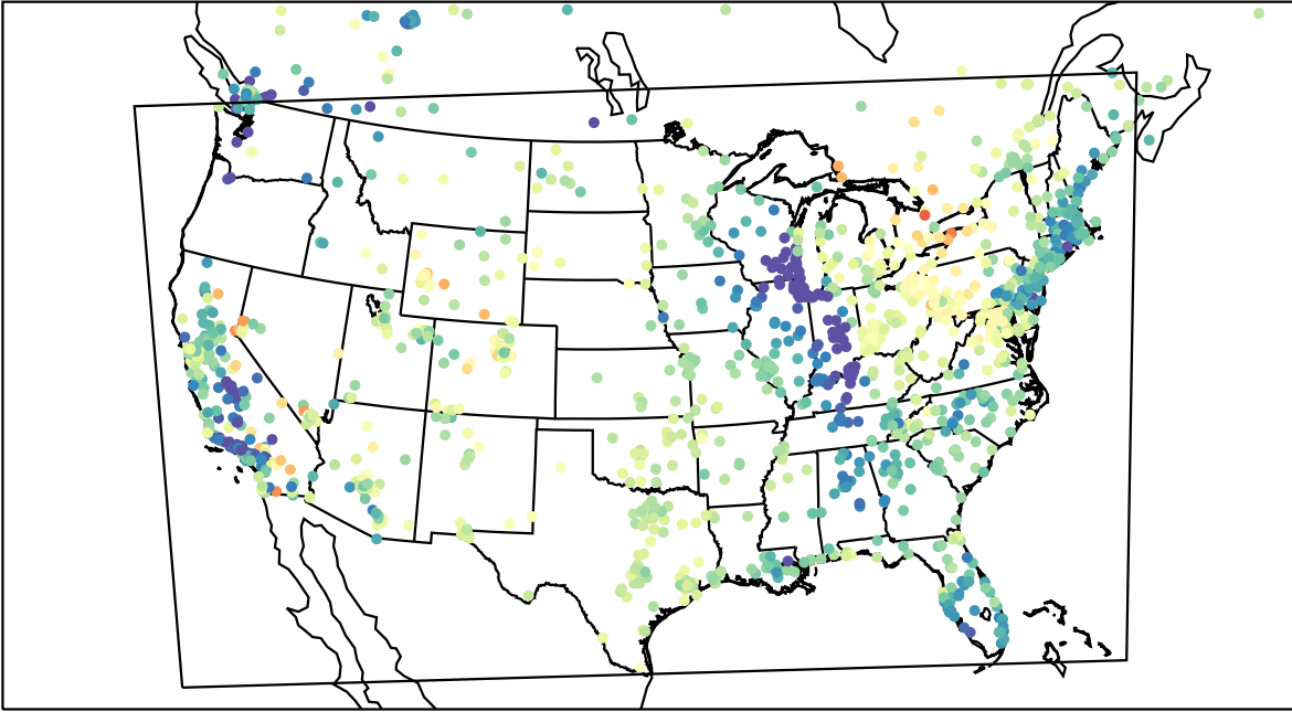
AirNOW (2023-04-16_15:00:00)
