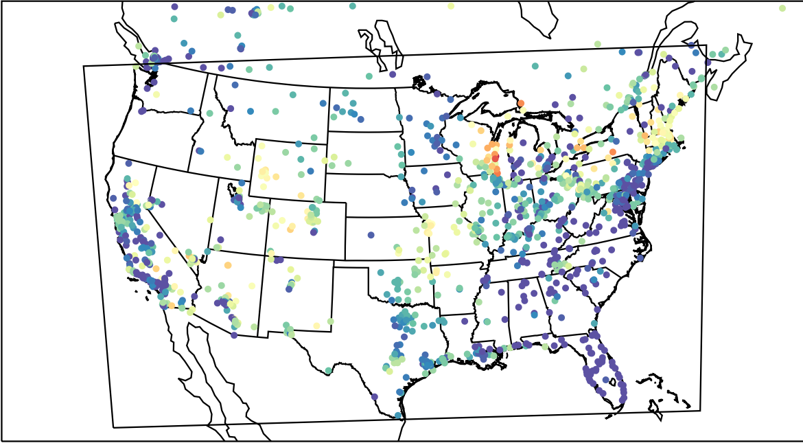
AirNOW (2023-04-15_08:00:00)
