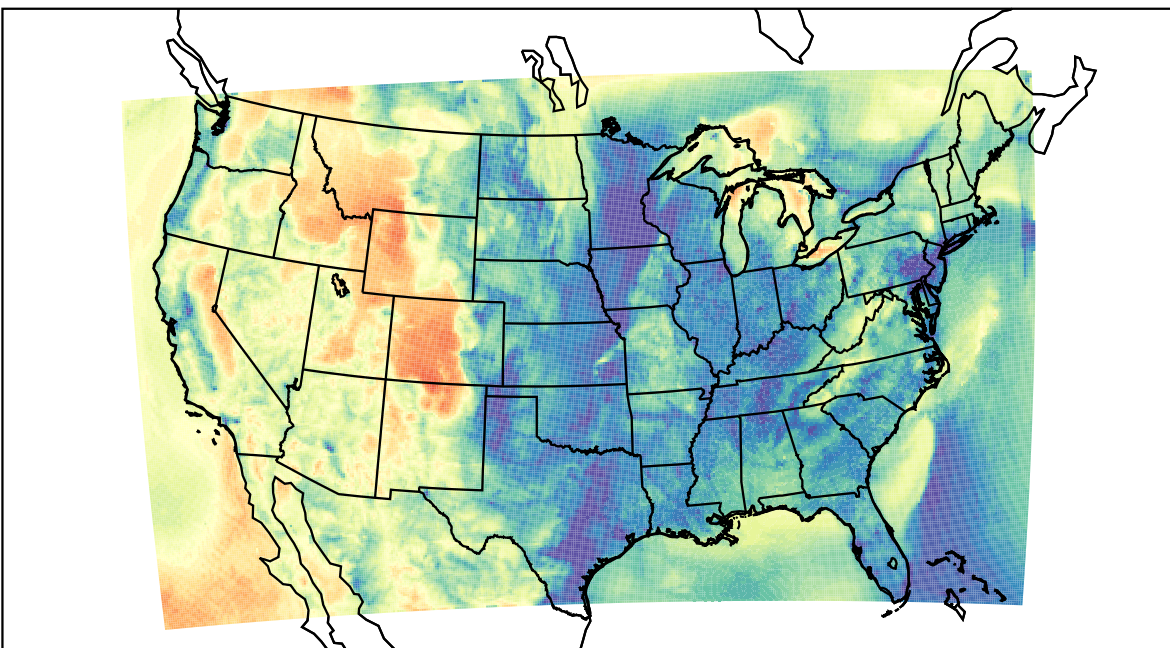
WRF (2023-04-15_13:00:00)
