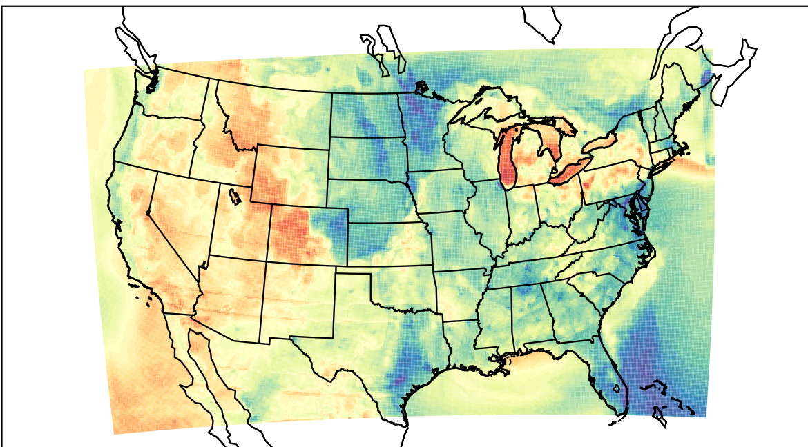
WRF (2023-04-15_02:00:00)
