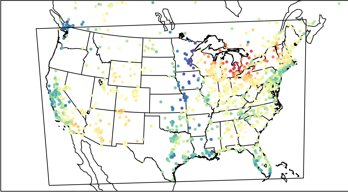
AirNOW (2023-04-15_17:00:00)
