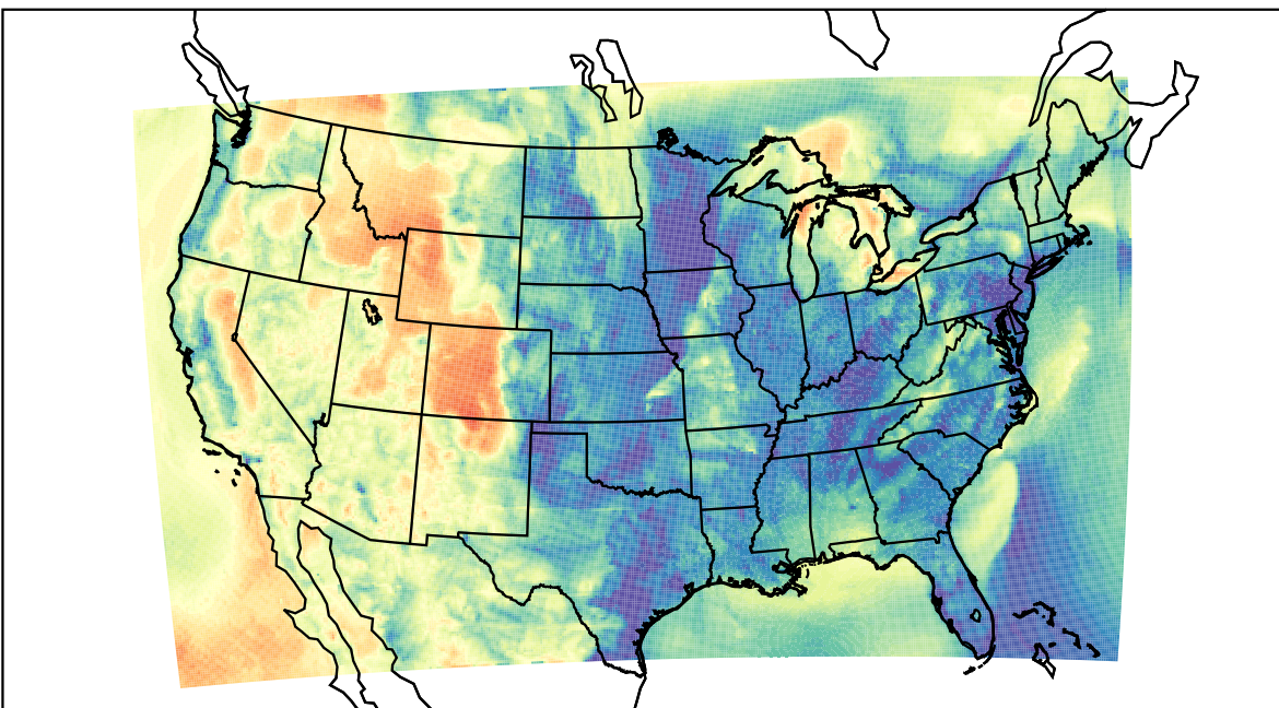
WRF (2023-04-15_12:00:00)
