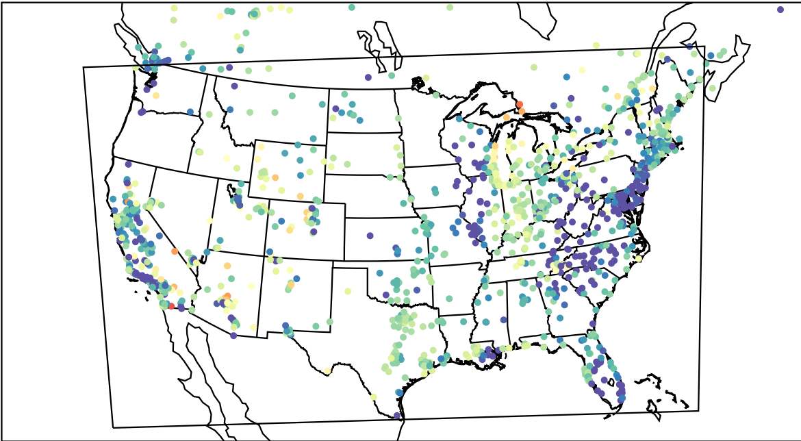
AirNOW (2023-04-16_06:00:00)
