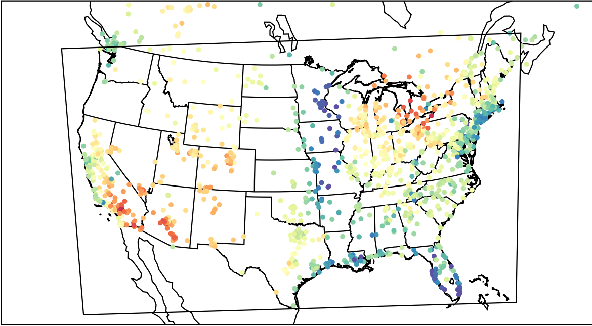
AirNOW (2023-04-15_23:00:00)
