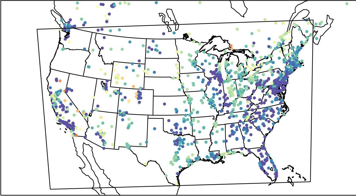
AirNOW (2023-04-16_12:00:00)
