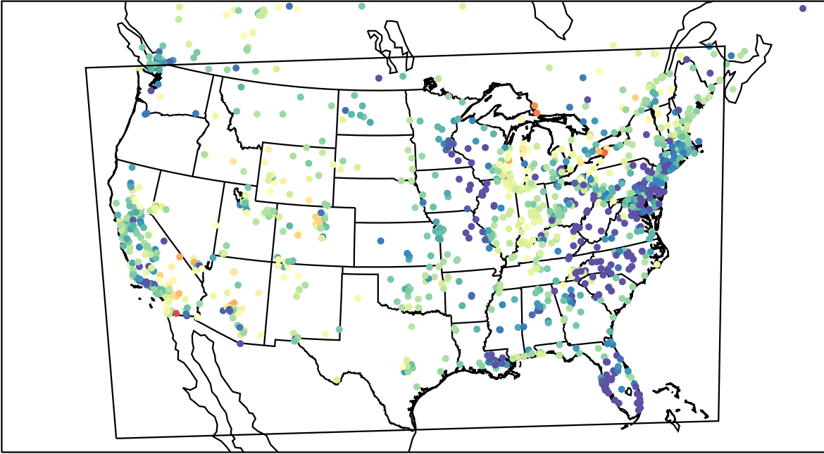
AirNOW (2023-04-16_04:00:00)
