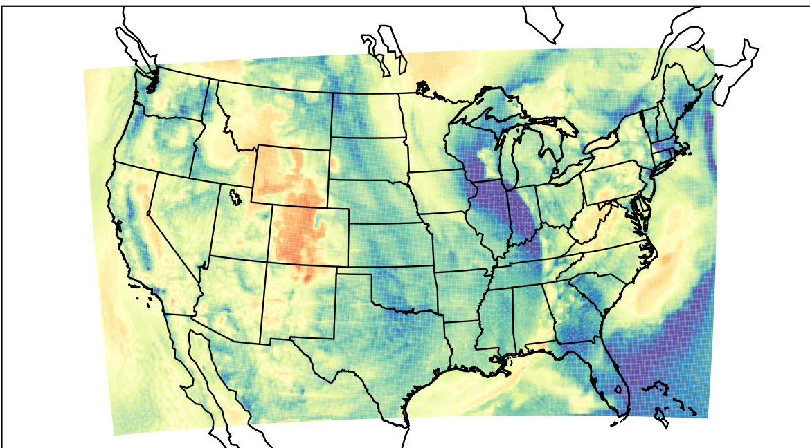
WRF (2023-04-16_14:00:00)
