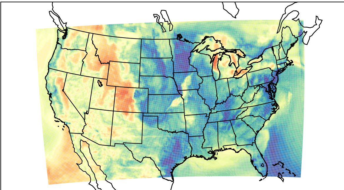
WRF (2023-04-15_08:00:00)
