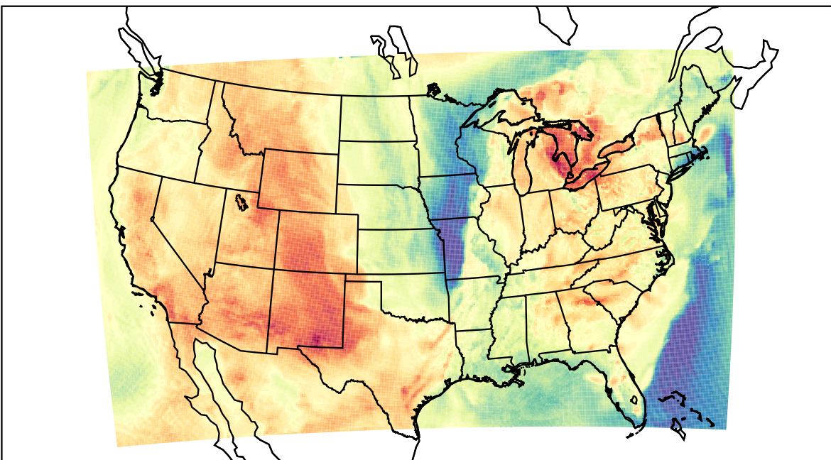
WRF (2023-04-15_22:00:00)
