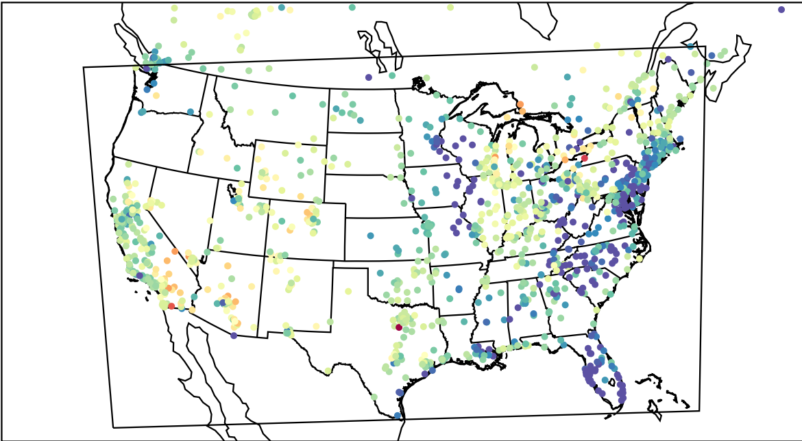
AirNOW (2023-04-16_03:00:00)
