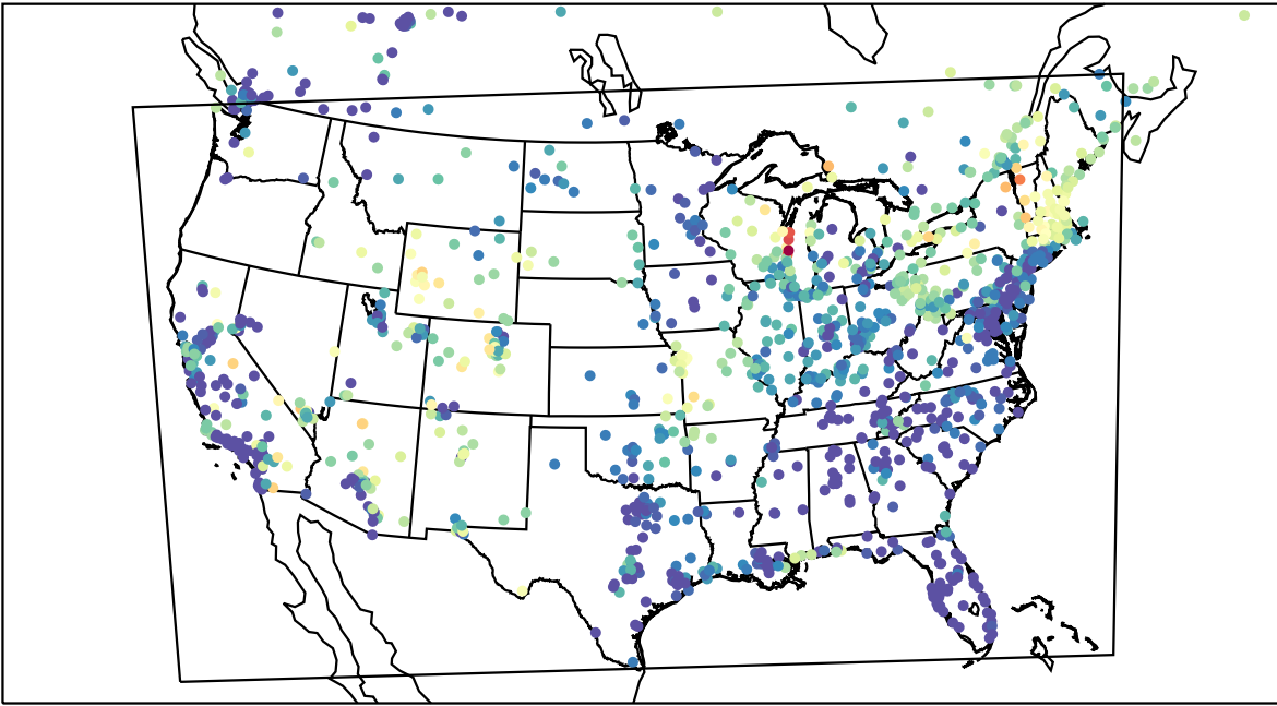
AirNOW (2023-04-15_12:00:00)
