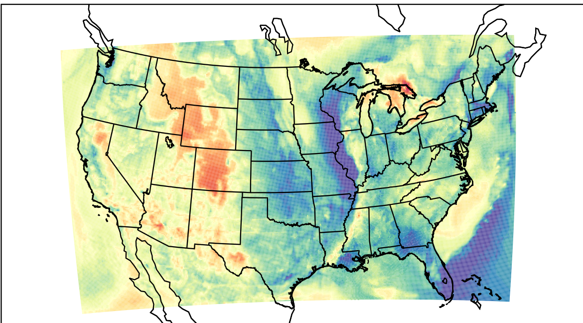
WRF (2023-04-16_06:00:00)
