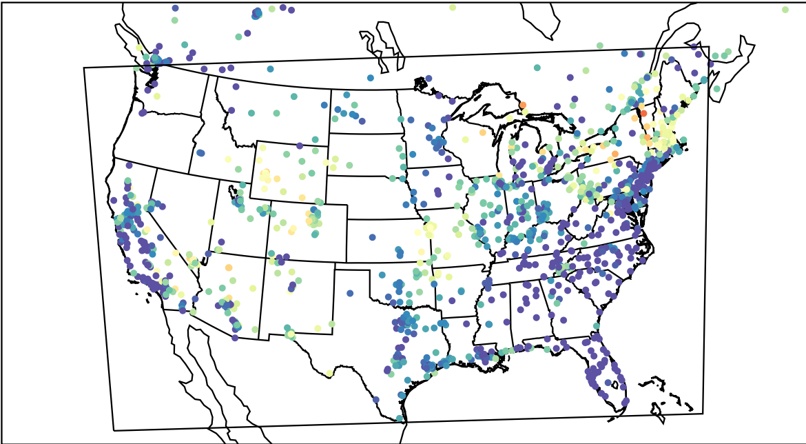
AirNOW (2023-04-15_10:00:00)
