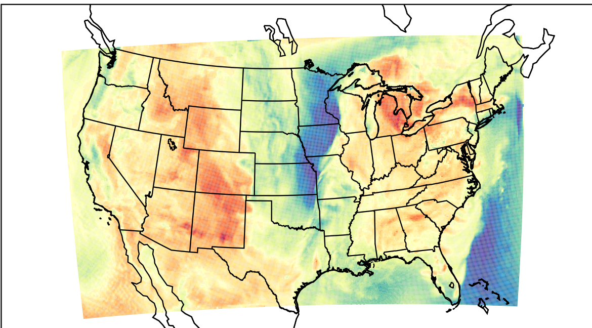
WRF (2023-04-15_18:00:00)
