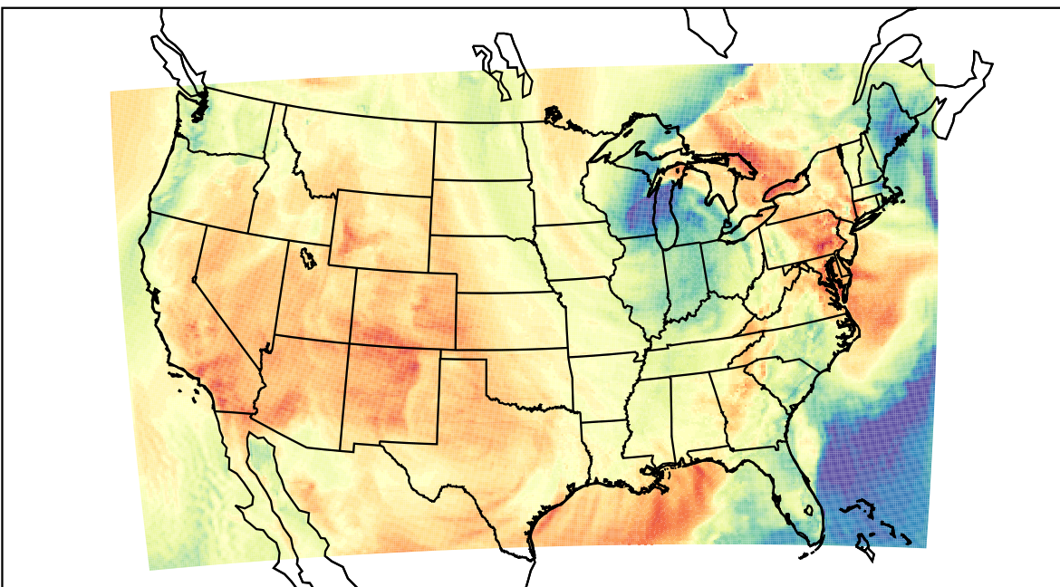
WRF (2023-04-16_22:00:00)
