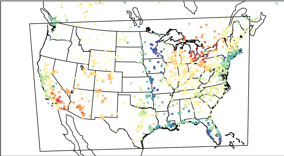
AirNOW (2023-04-15_22:00:00)
