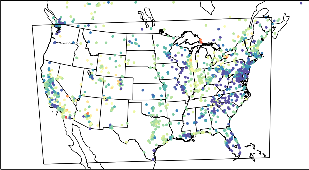
AirNOW (2023-04-16_05:00:00)
