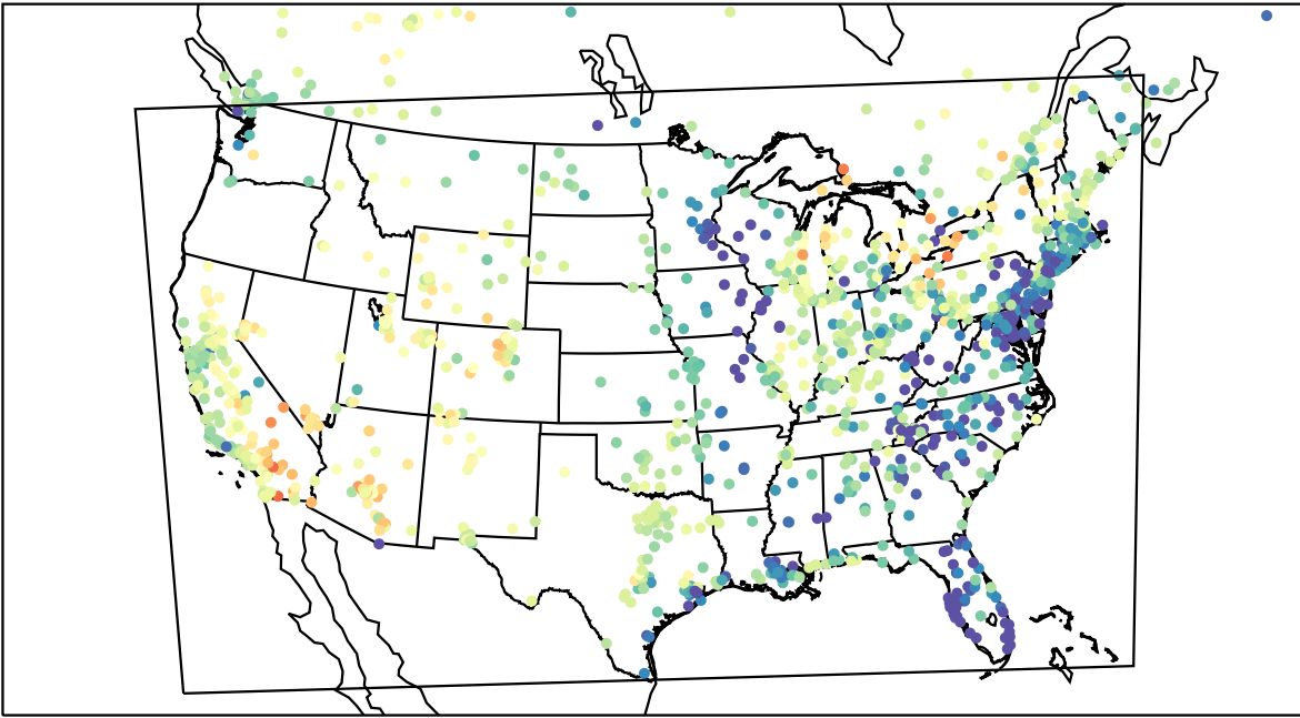
AirNOW (2023-04-16_02:00:00)
