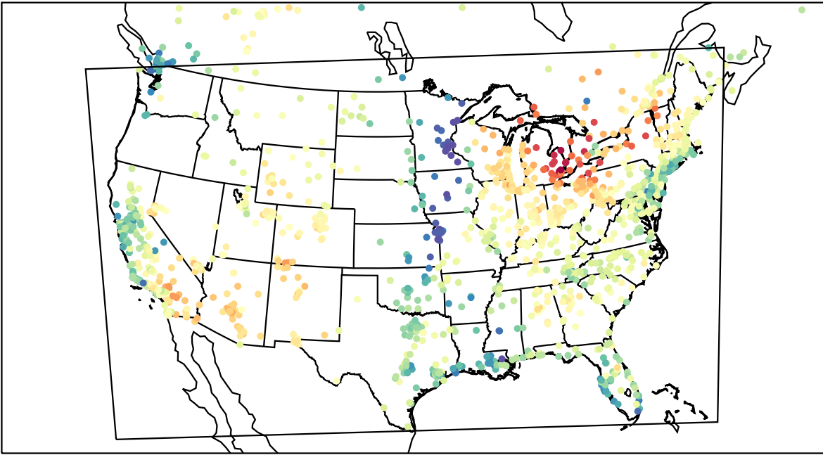
AirNOW (2023-04-15_18:00:00)
