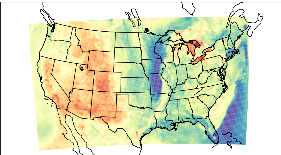
WRF (2023-04-16_01:00:00)
