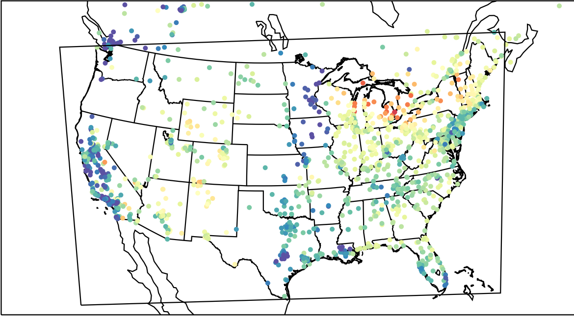
AirNOW (2023-04-15_15:00:00)
