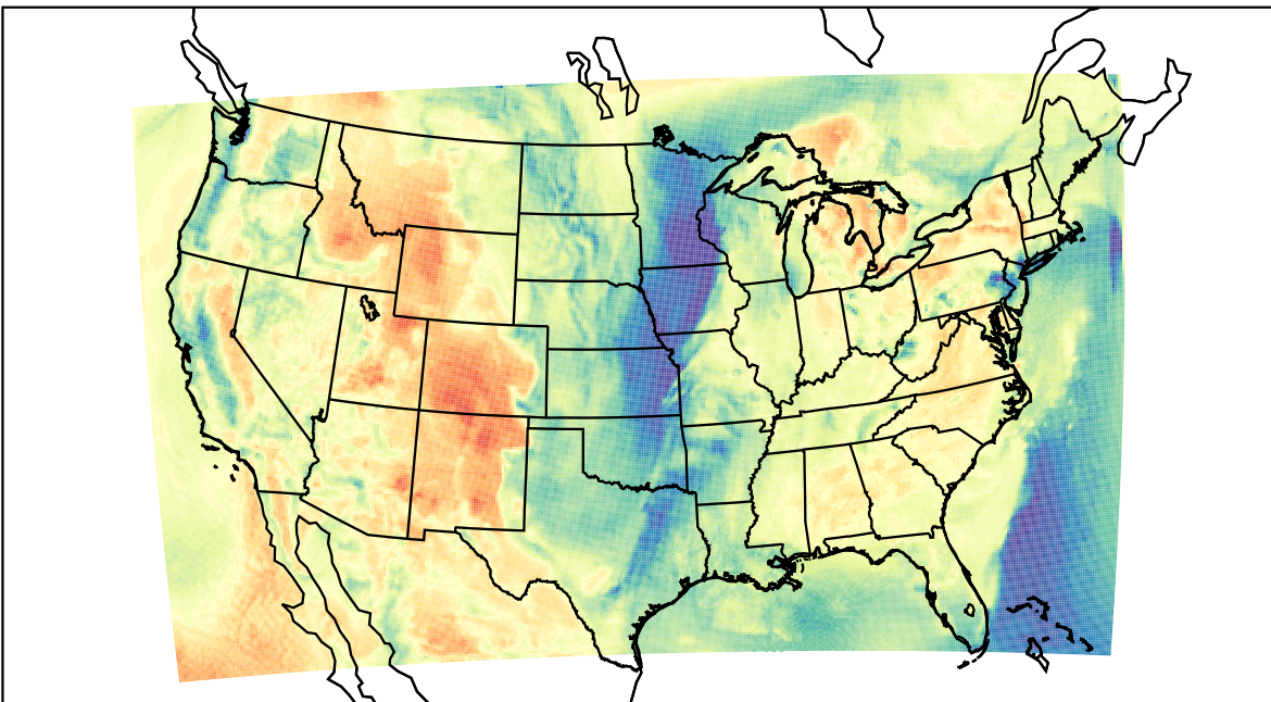
WRF (2023-04-15_16:00:00)
