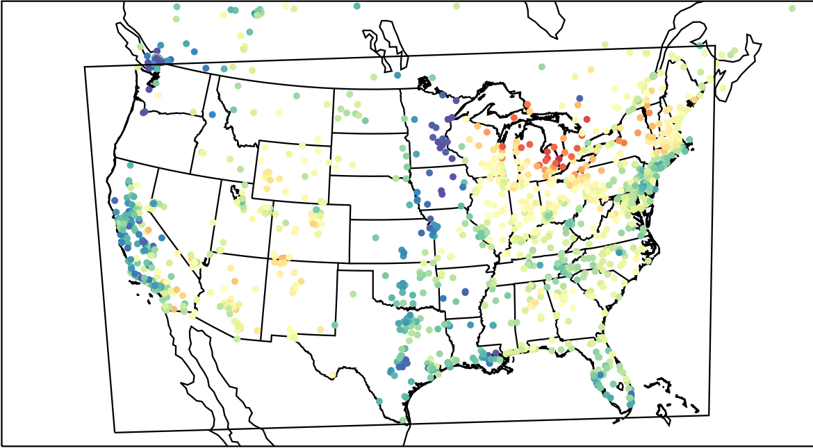
AirNOW (2023-04-15_16:00:00)
