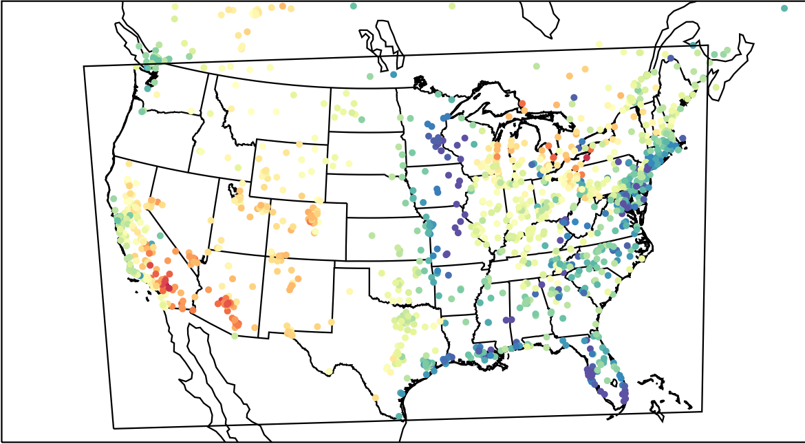
AirNOW (2023-04-16_00:00:00)
