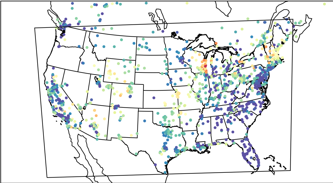
AirNOW (2023-04-15_07:00:00)
