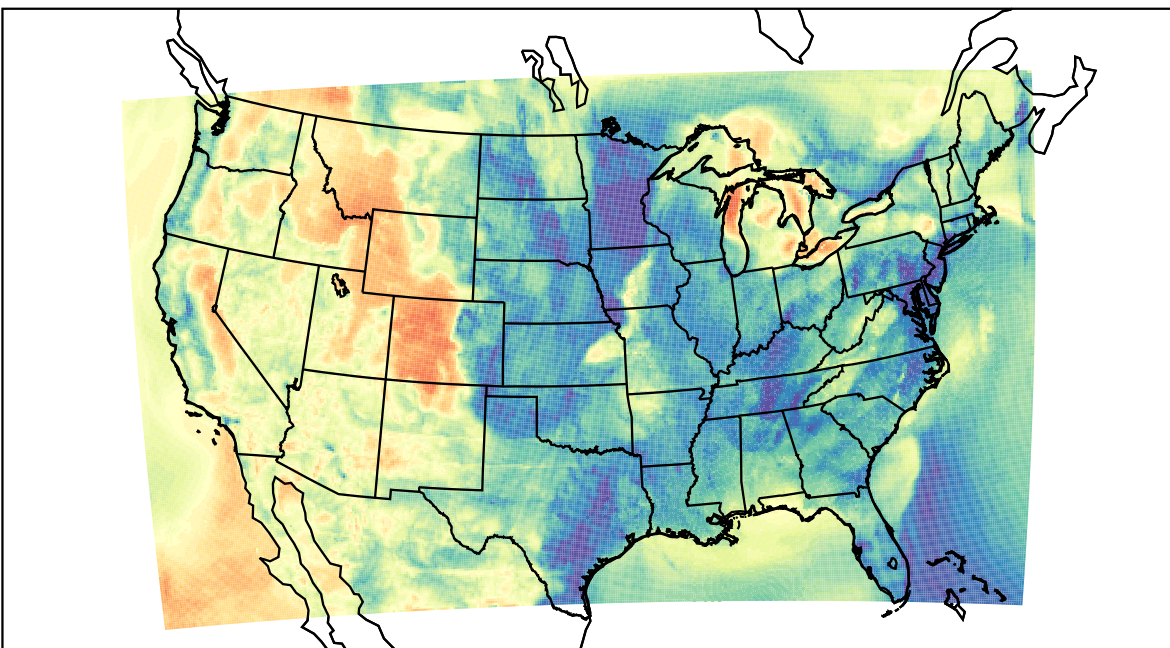
WRF (2023-04-15_09:00:00)
