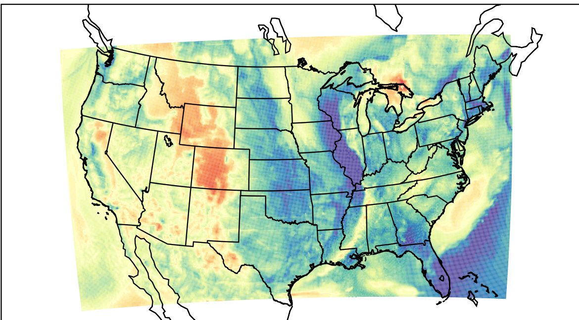
WRF (2023-04-16_08:00:00)
