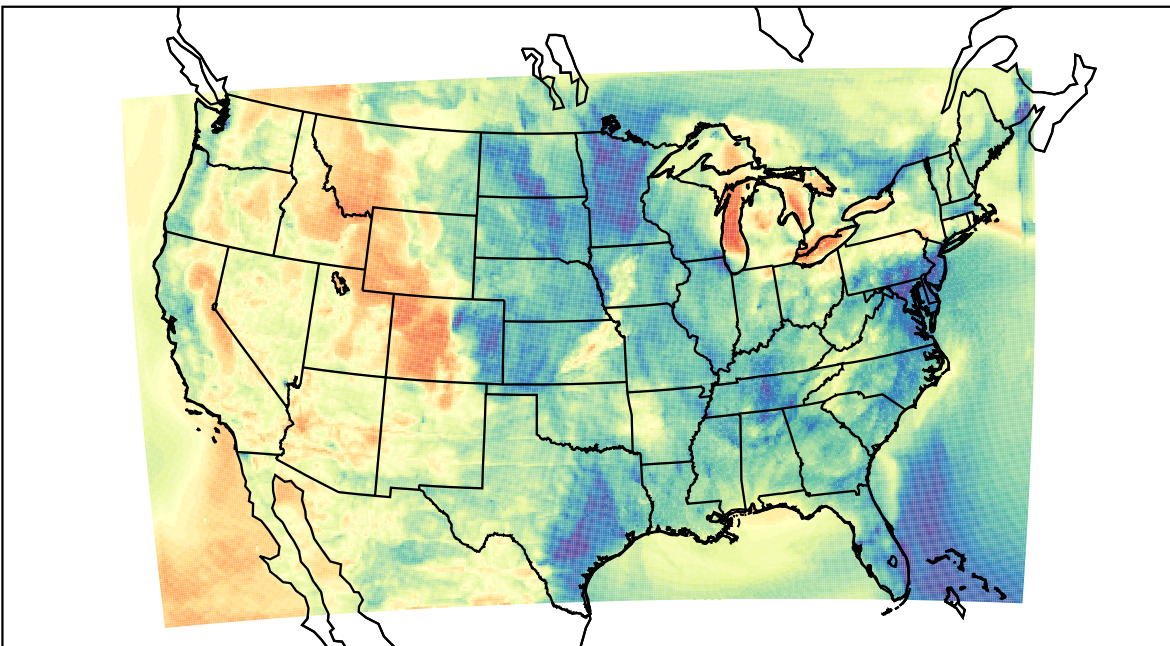
WRF (2023-04-15_05:00:00)
