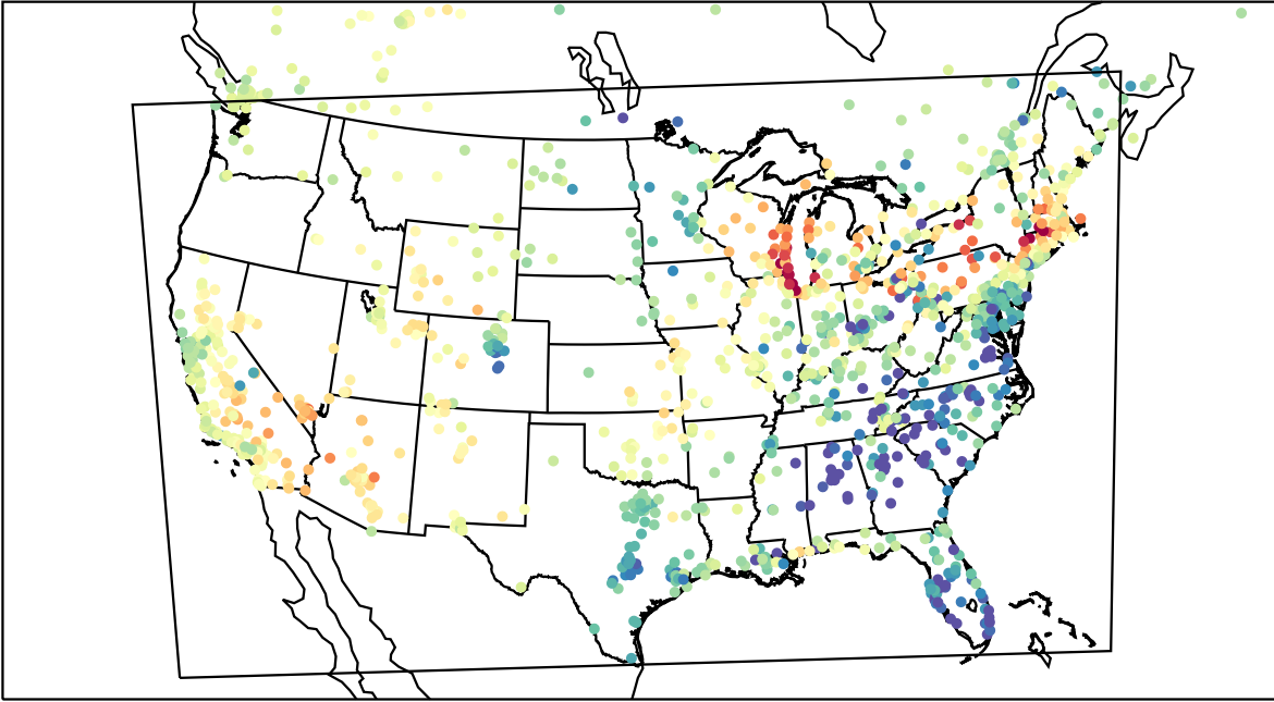
AirNOW (2023-04-15_01:00:00)
