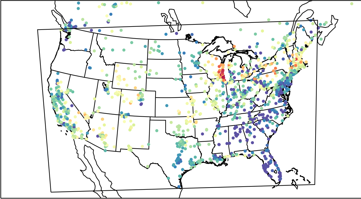
AirNOW (2023-04-15_04:00:00)
