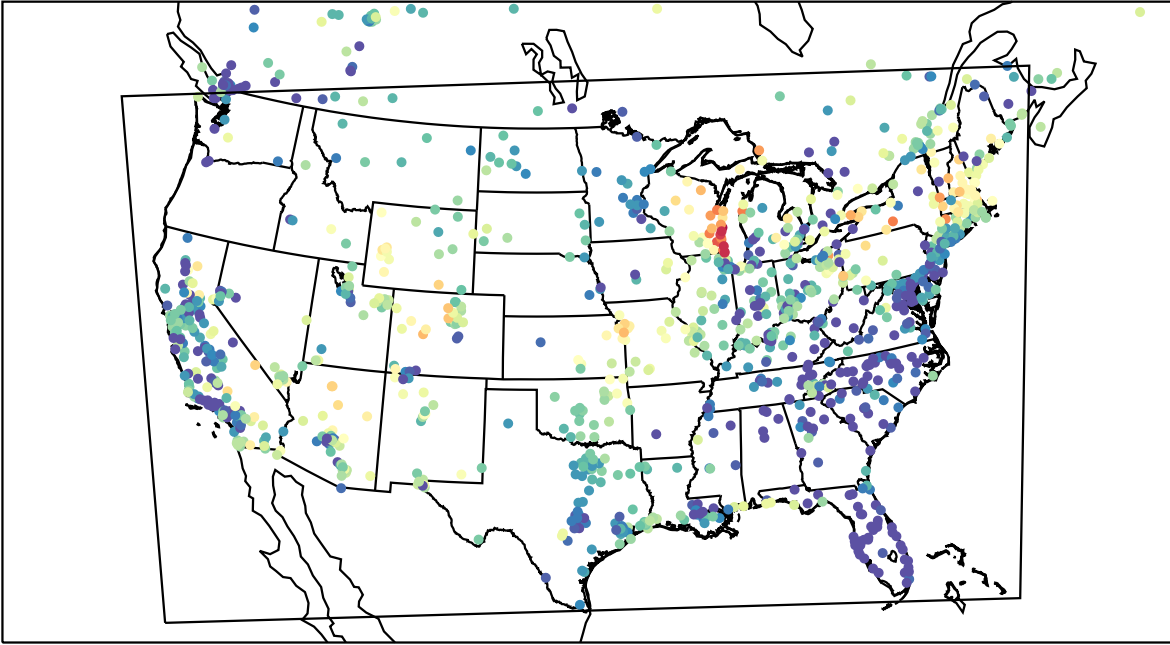
AirNOW (2023-04-15_06:00:00)
