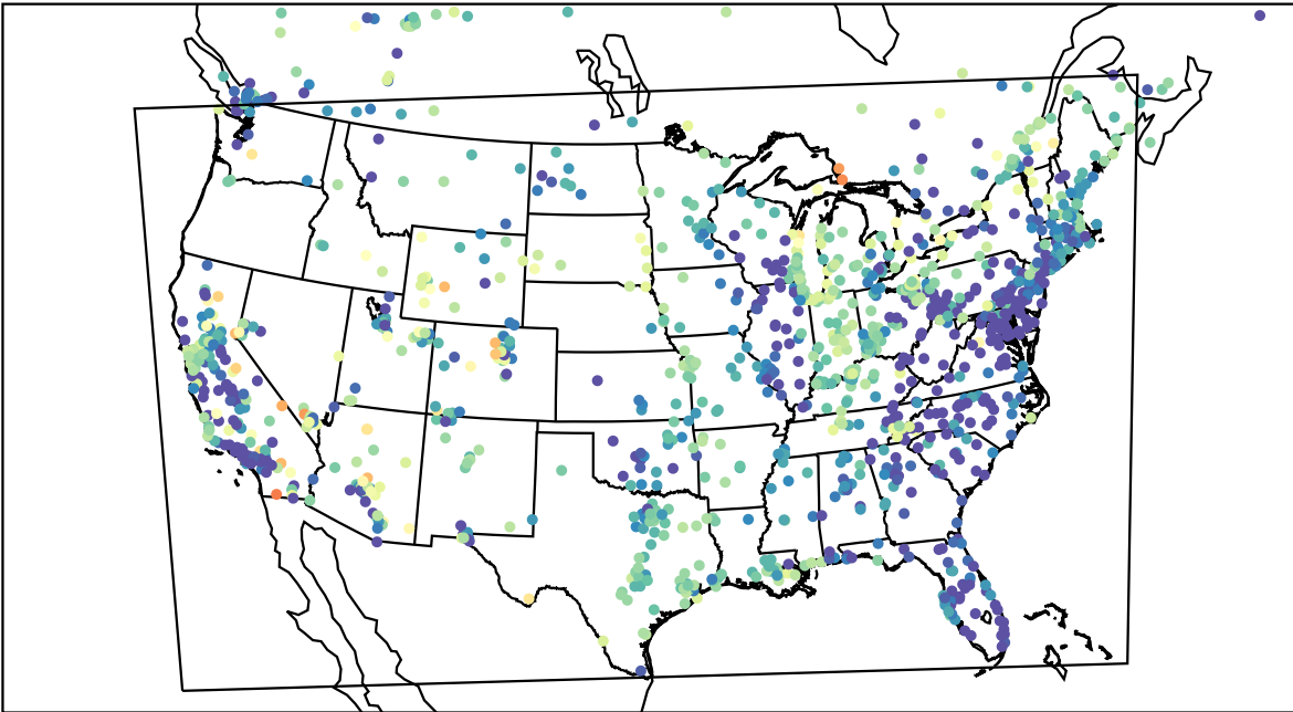
AirNOW (2023-04-16_09:00:00)
