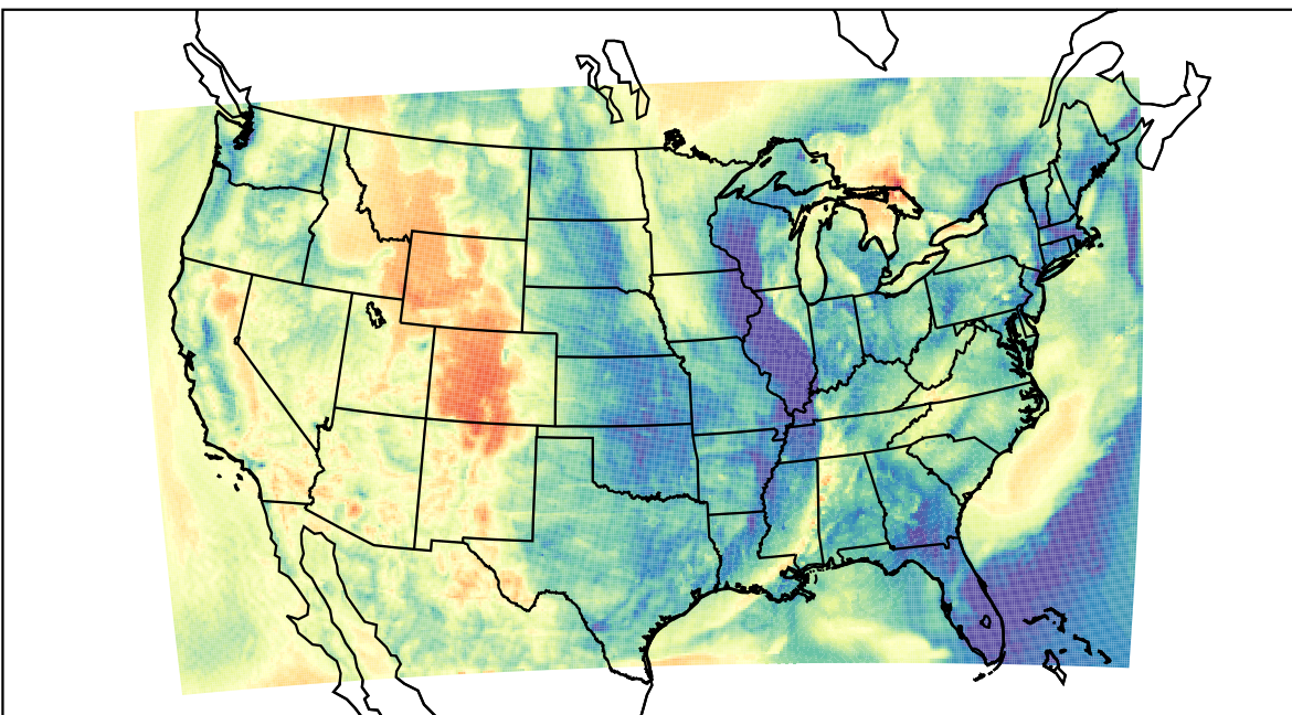
WRF (2023-04-16_09:00:00)
