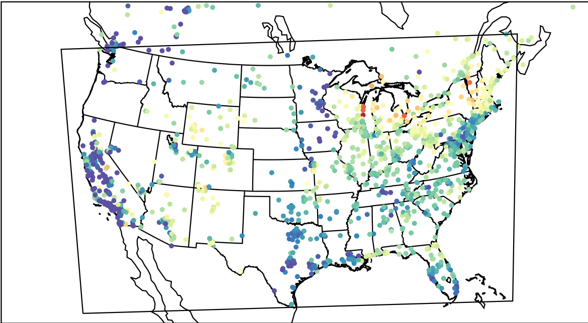
AirNOW (2023-04-15_14:00:00)
