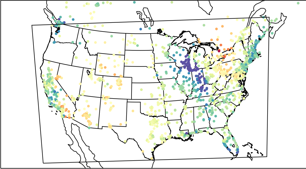
AirNOW (2023-04-16_17:00:00)
