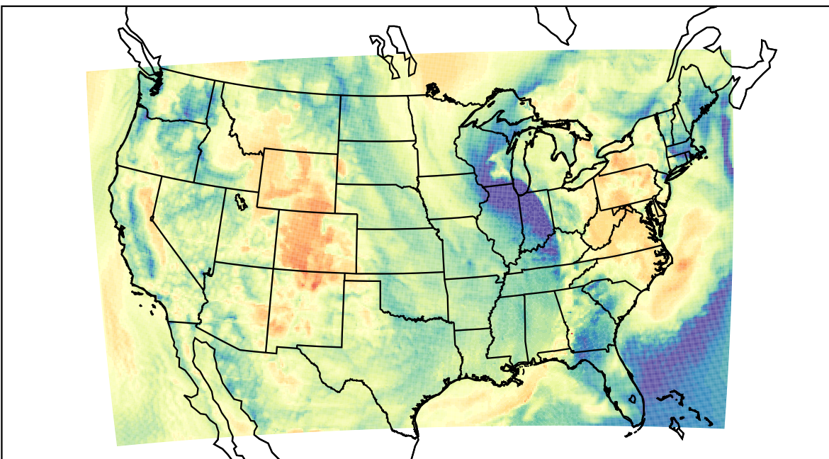
WRF (2023-04-16_15:00:00)
