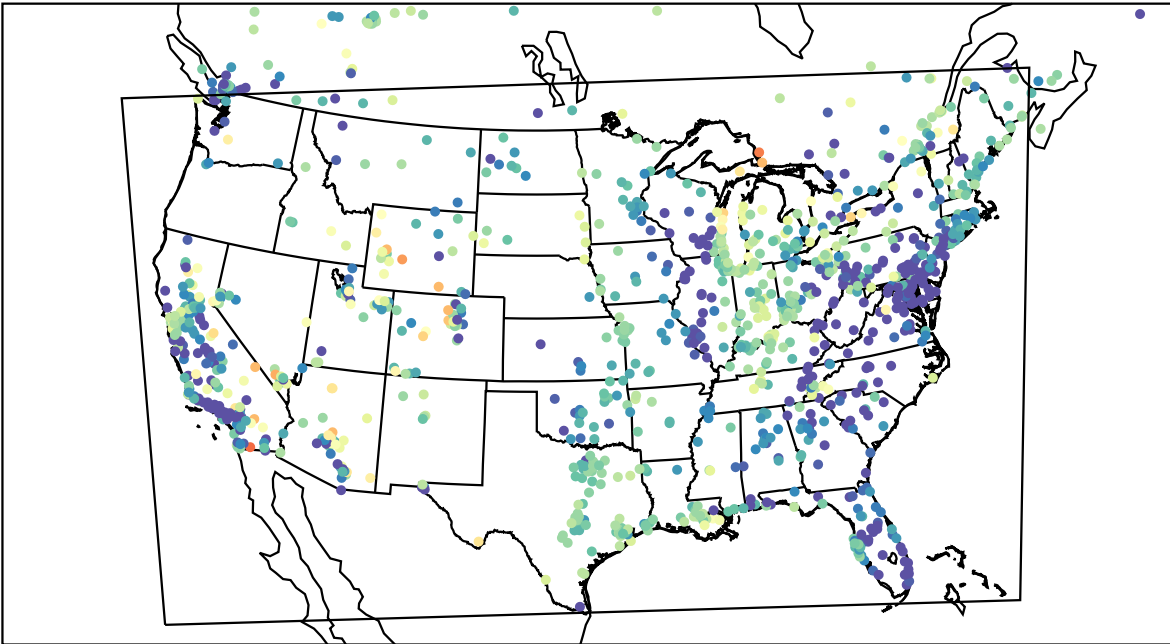
AirNOW (2023-04-16_08:00:00)
