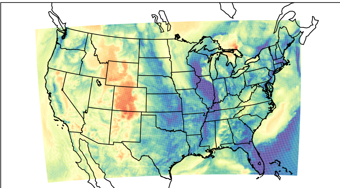
WRF (2023-04-16_11:00:00)
