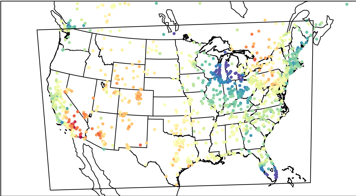
AirNOW (2023-04-16_21:00:00)
