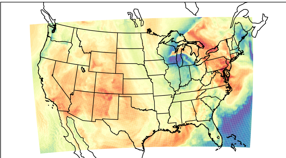
WRF (2023-04-16_20:00:00)
