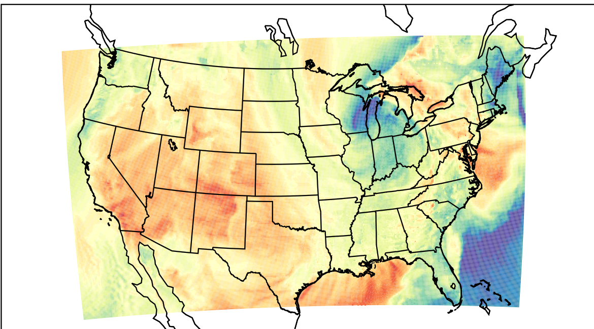
WRF (2023-04-16_23:00:00)
