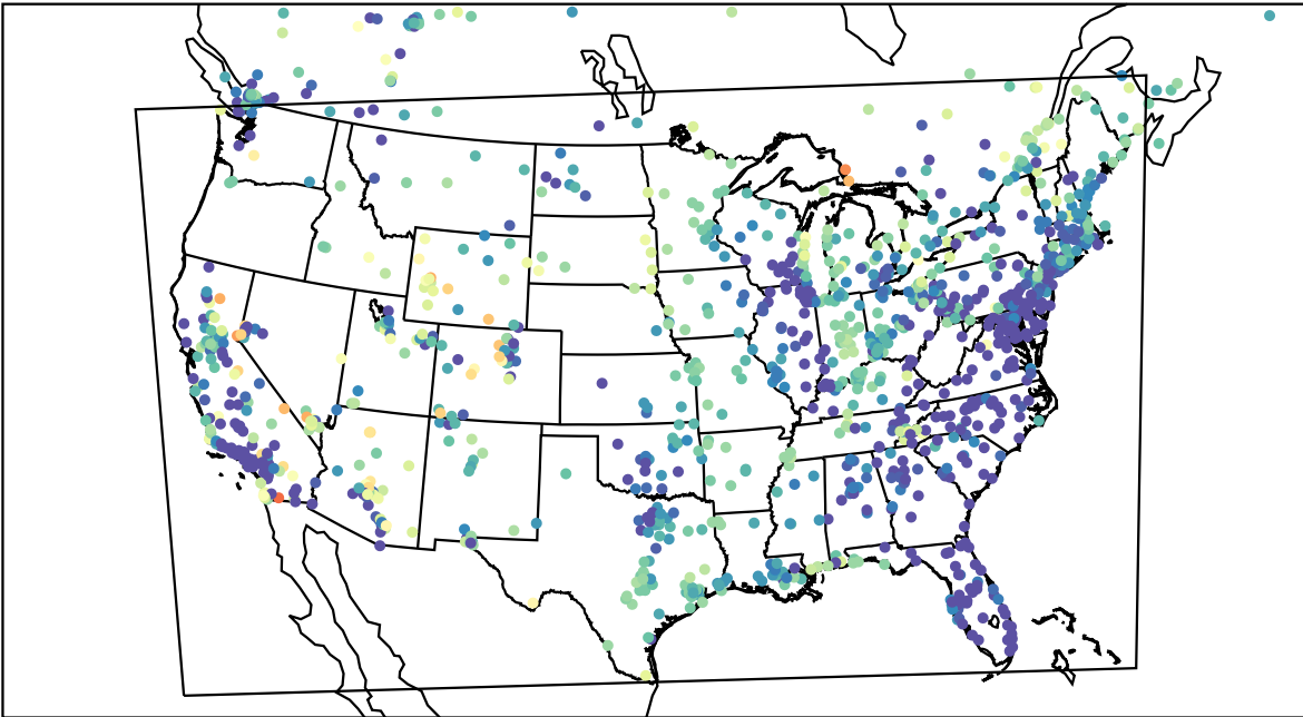
AirNOW (2023-04-16_11:00:00)
