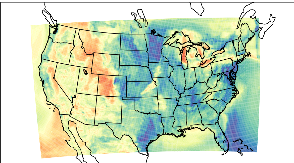
WRF (2023-04-15_06:00:00)
