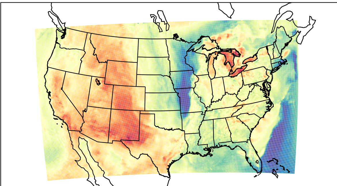
WRF (2023-04-15_23:00:00)
