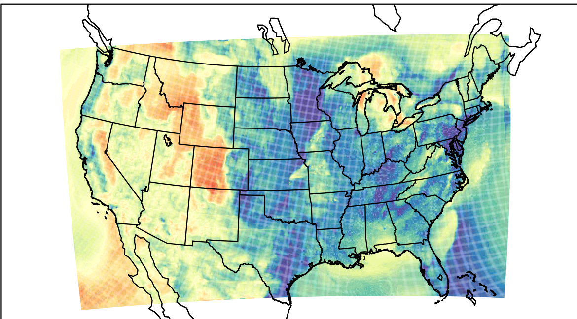
WRF (2023-04-15_11:00:00)
