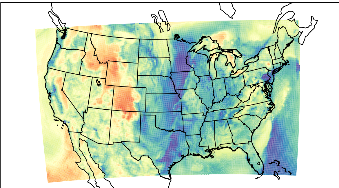
WRF (2023-04-15_14:00:00)
