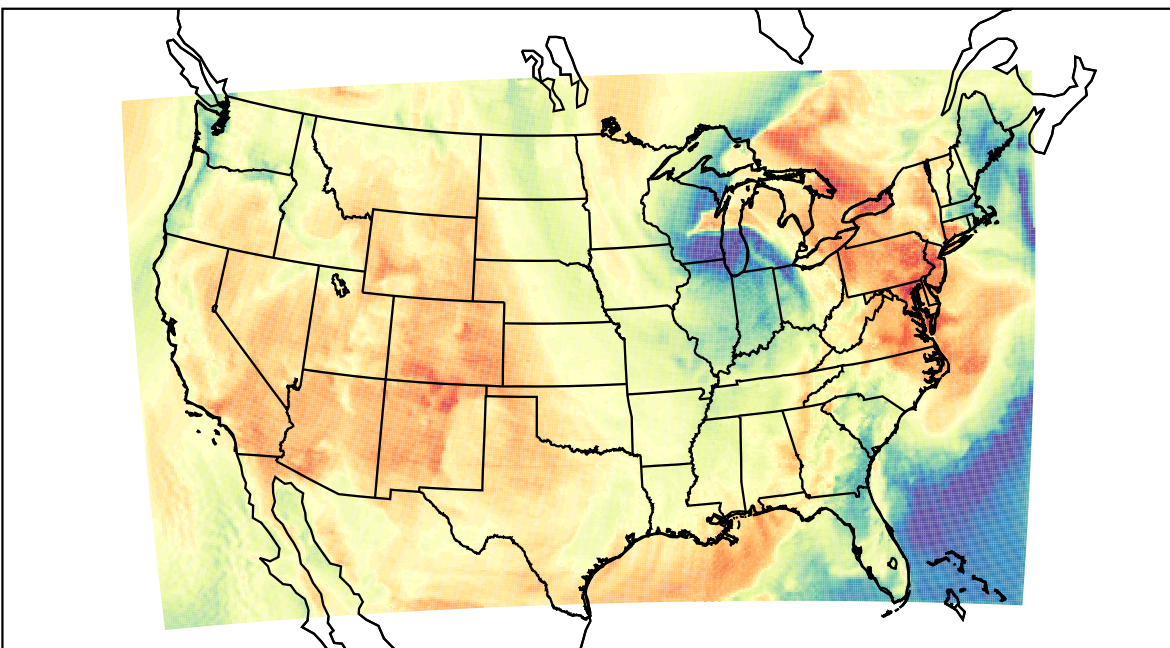
WRF (2023-04-16_19:00:00)
