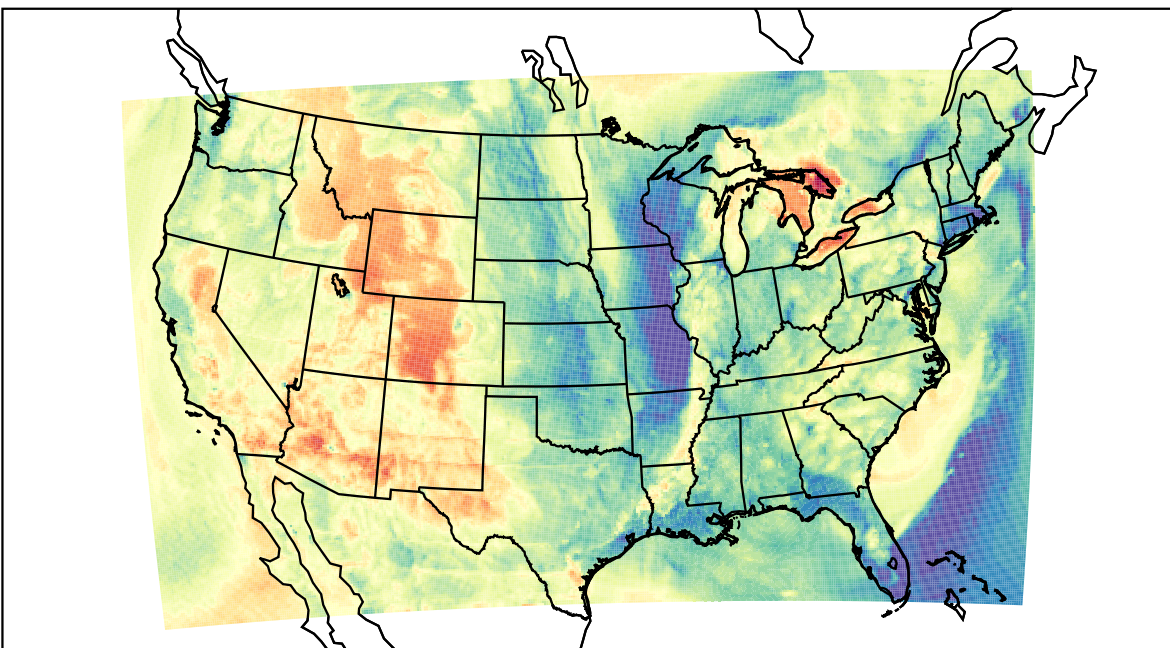
WRF (2023-04-16_03:00:00)
