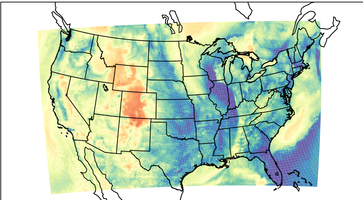
WRF (2023-04-16_12:00:00)
