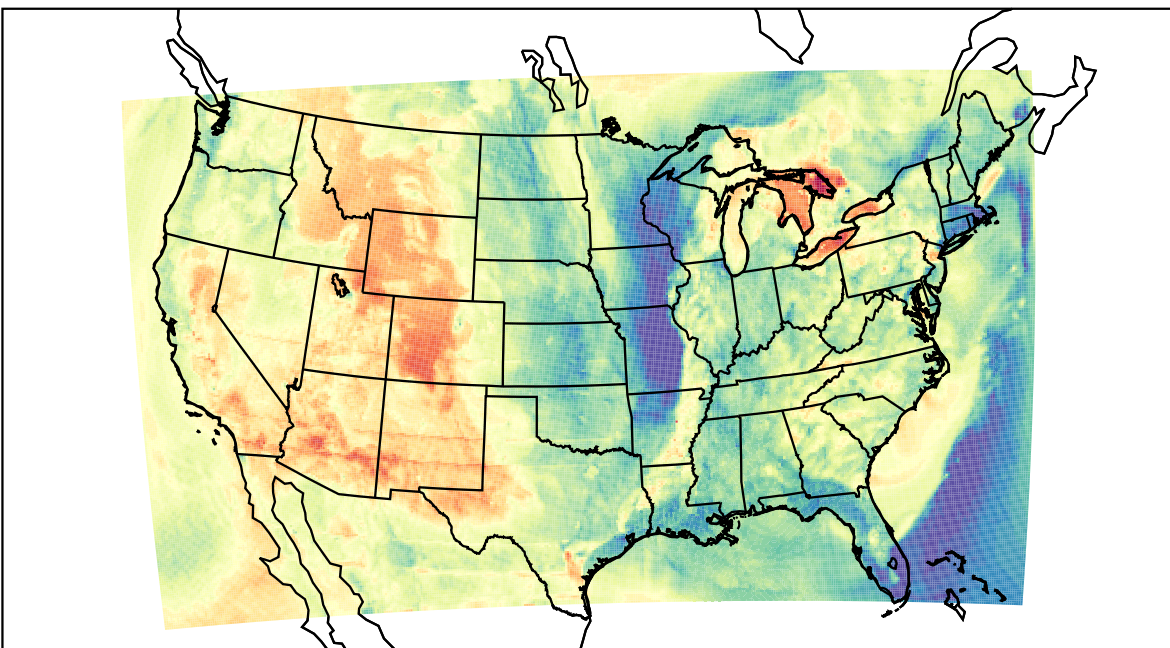
WRF (2023-04-16_02:00:00)
