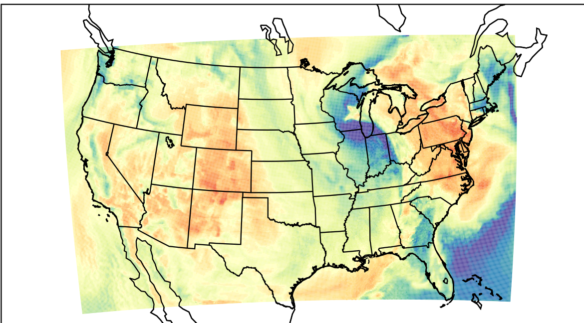
WRF (2023-04-16_17:00:00)
