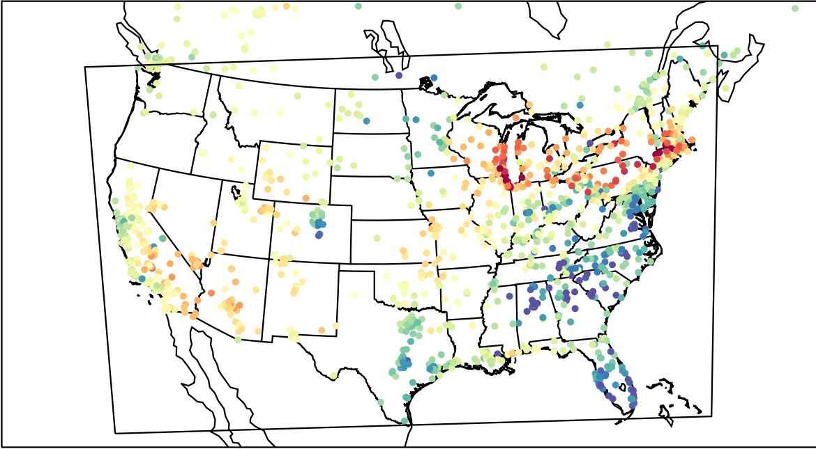
AirNOW (2023-04-15_00:00:00)
