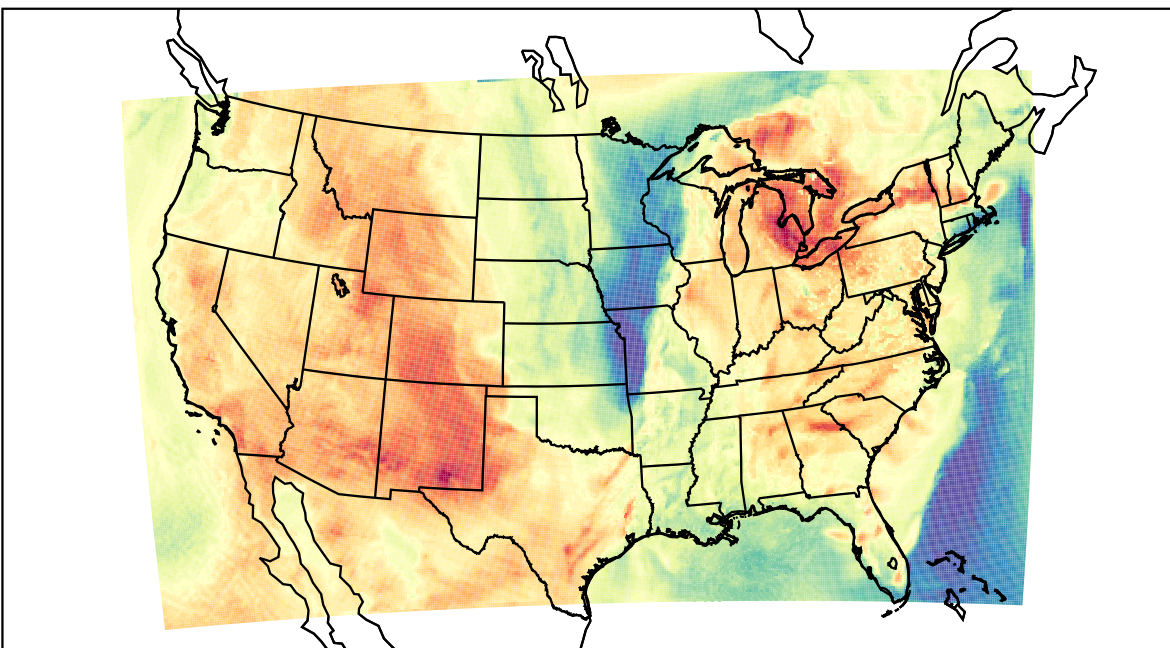
WRF (2023-04-15_21:00:00)
