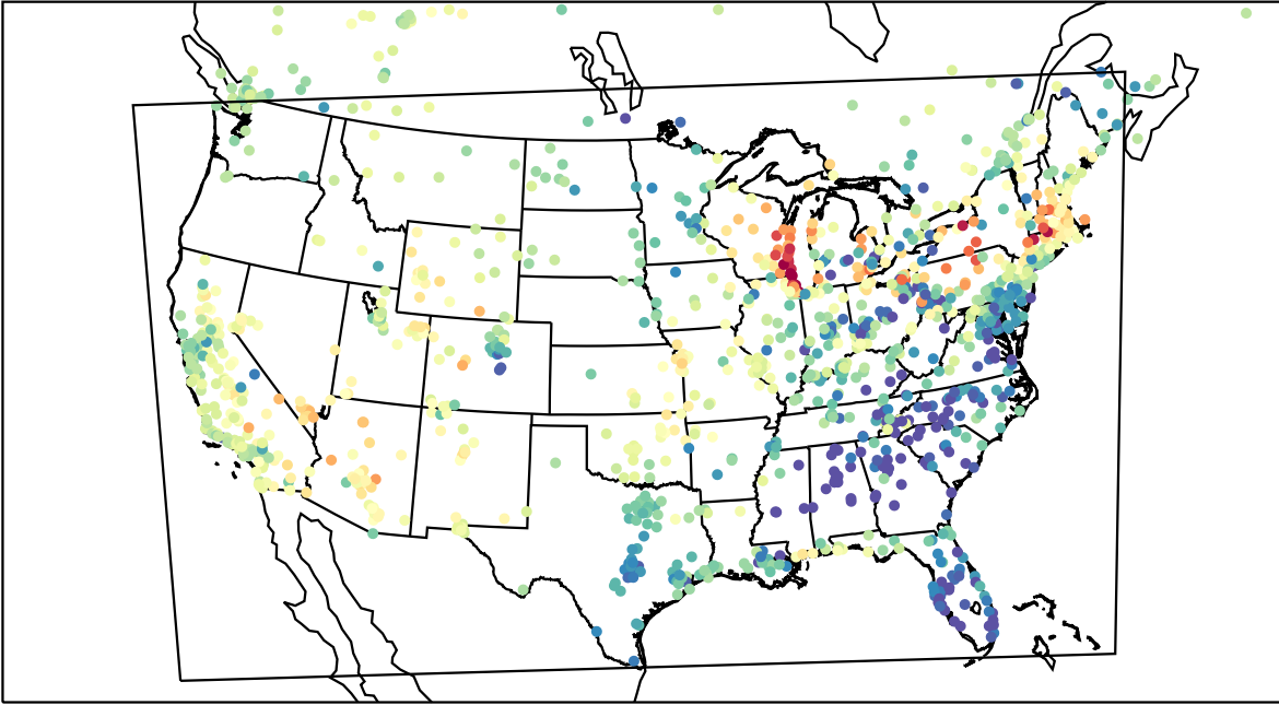
AirNOW (2023-04-15_02:00:00)
