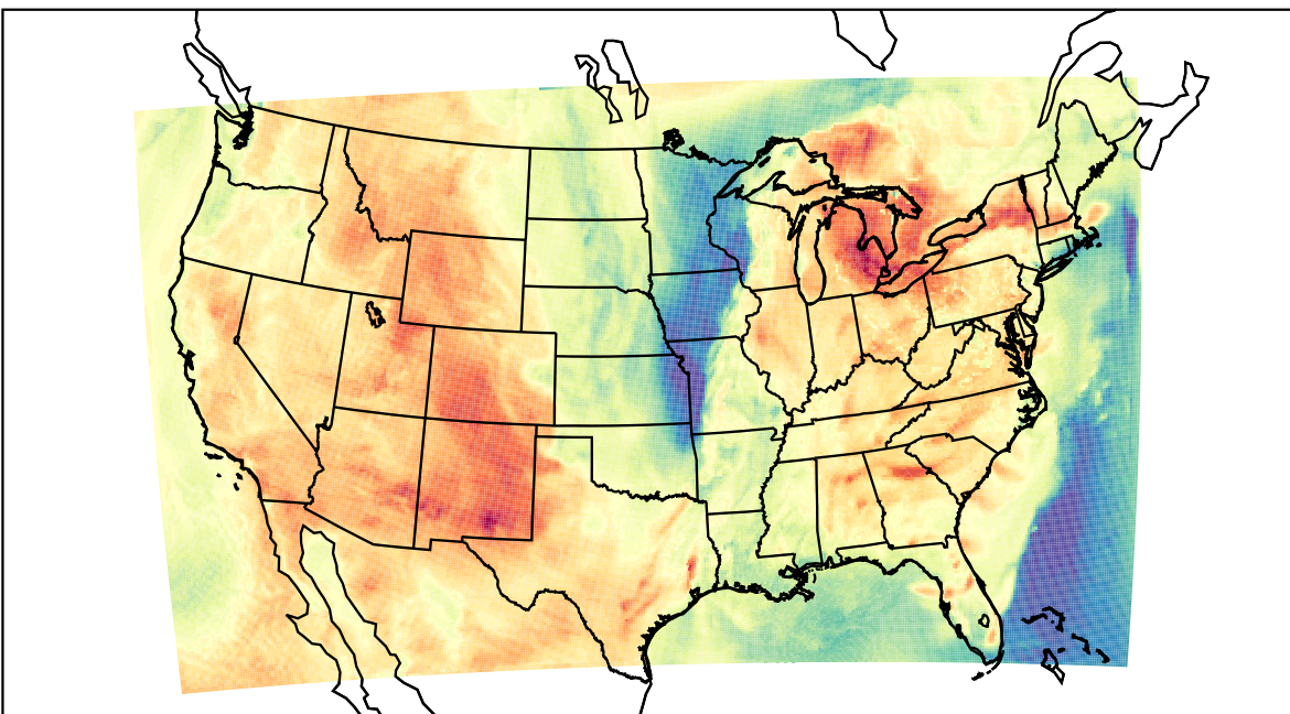
WRF (2023-04-15_20:00:00)
