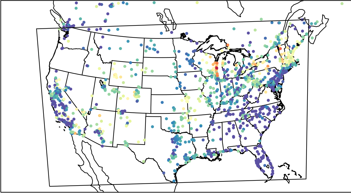
AirNOW (2023-04-15_09:00:00)
