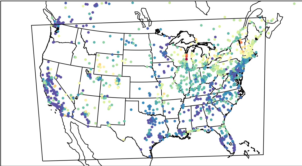
AirNOW (2023-04-15_13:00:00)
