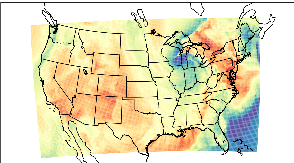
WRF (2023-04-16_21:00:00)
