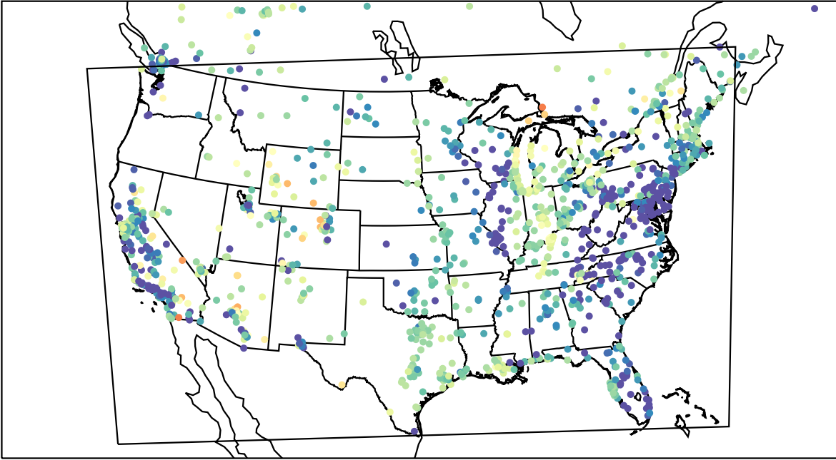
AirNOW (2023-04-16_07:00:00)
