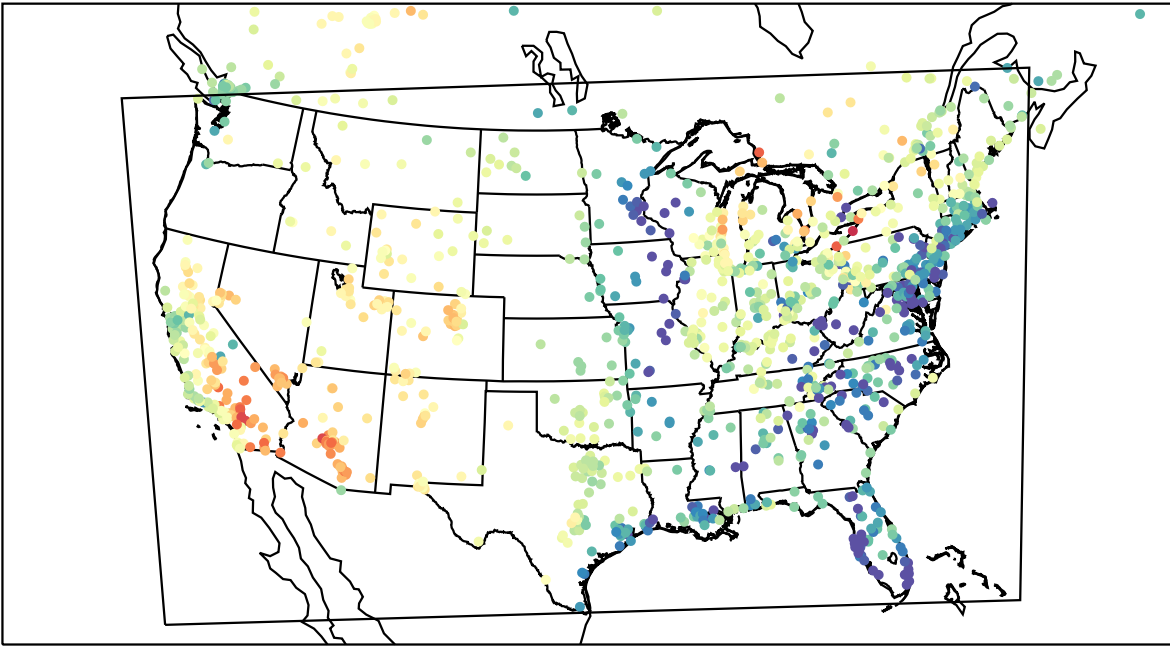
AirNOW (2023-04-16_01:00:00)
