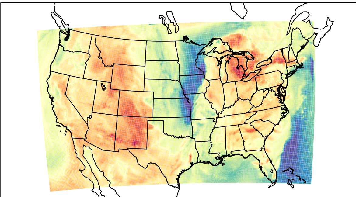
WRF (2023-04-15_19:00:00)
