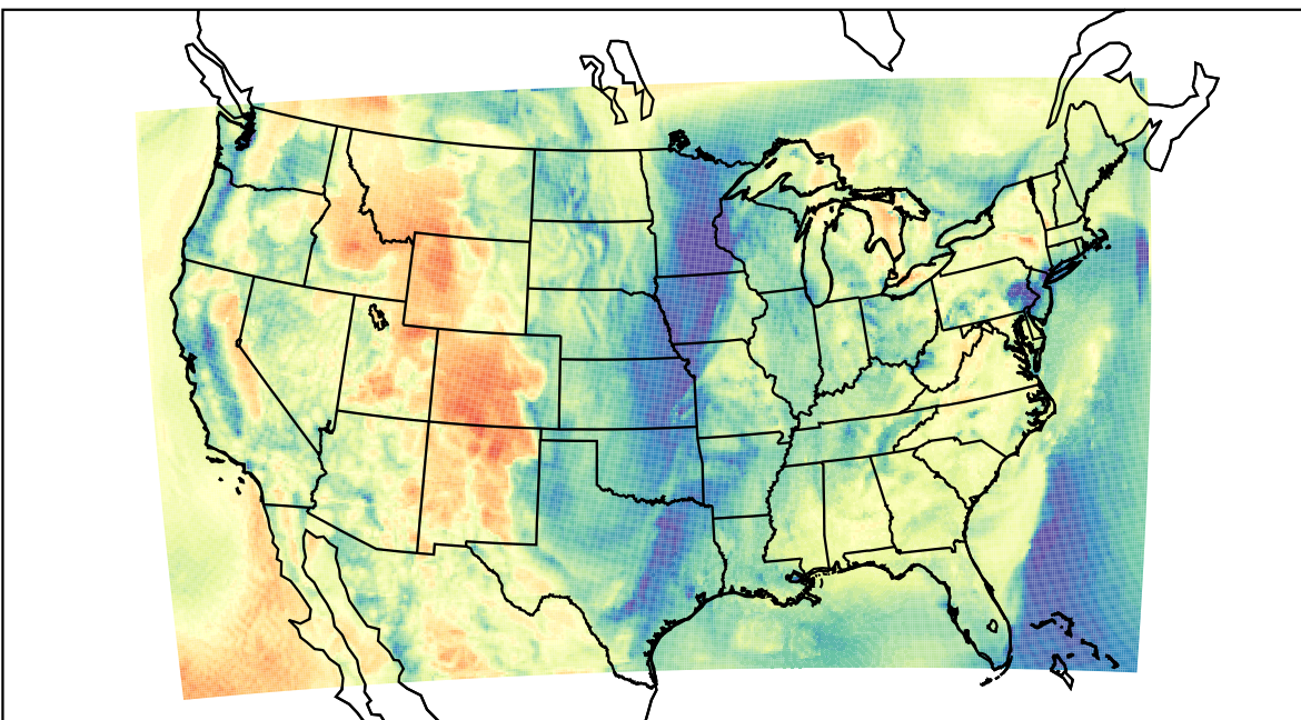
WRF (2023-04-15_15:00:00)
