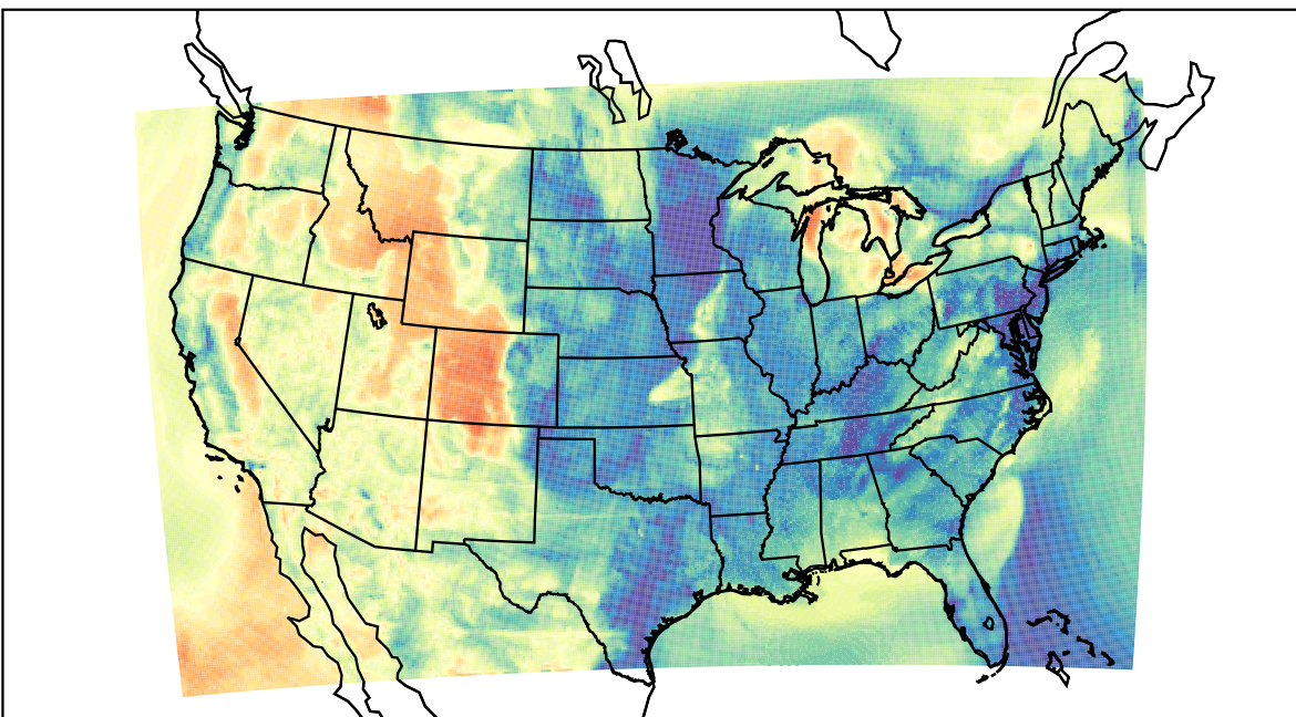
WRF (2023-04-15_10:00:00)
