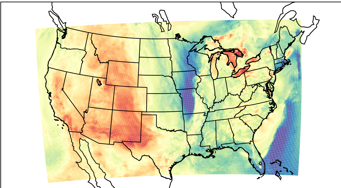
WRF (2023-04-16_00:00:00)
