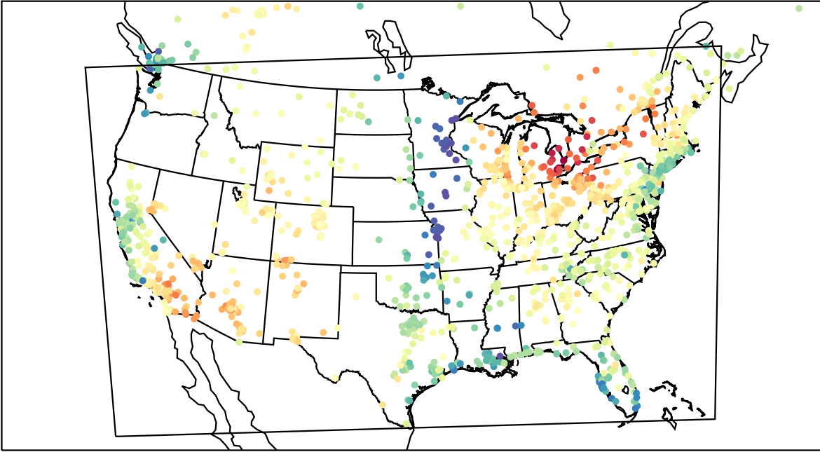
AirNOW (2023-04-15_19:00:00)
