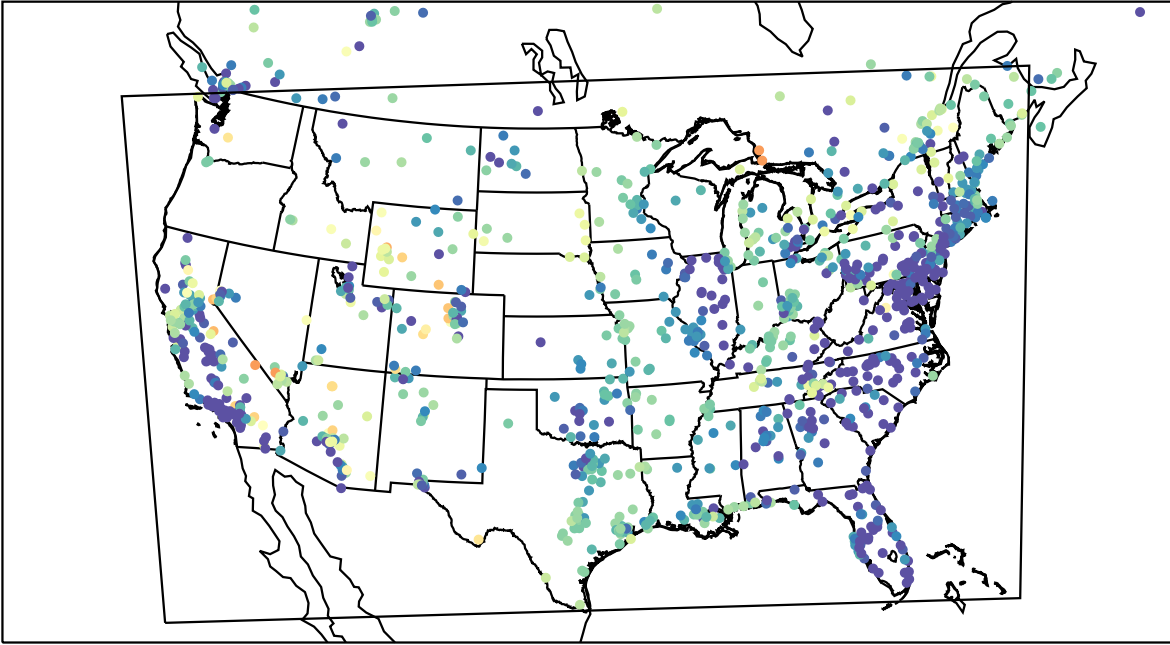
AirNOW (2023-04-16_10:00:00)
