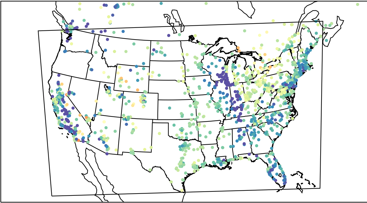
AirNOW (2023-04-16_14:00:00)
