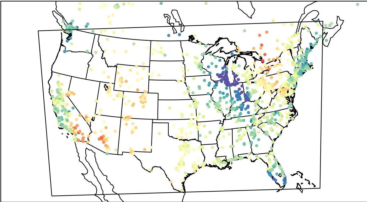
AirNOW (2023-04-16_18:00:00)
