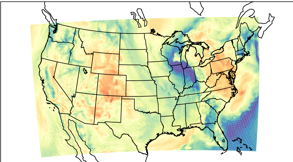
WRF (2023-04-16_16:00:00)
