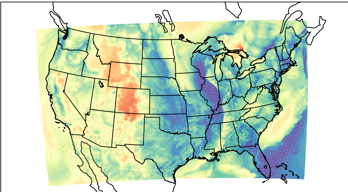
WRF (2023-04-16_10:00:00)
