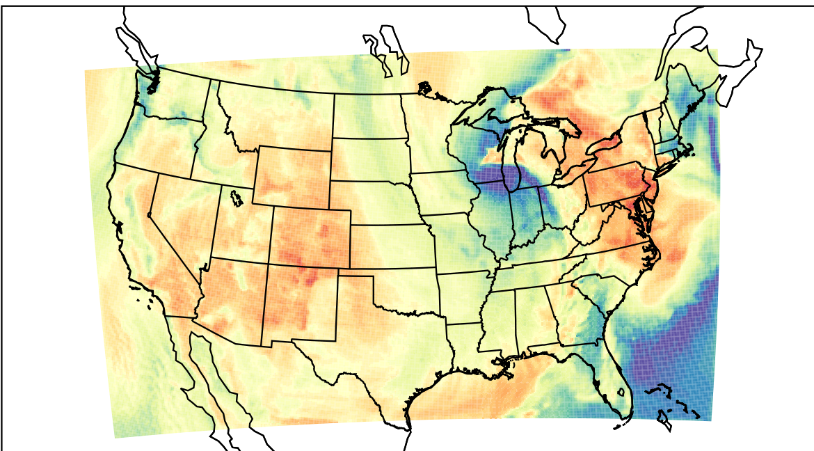
WRF (2023-04-16_18:00:00)
