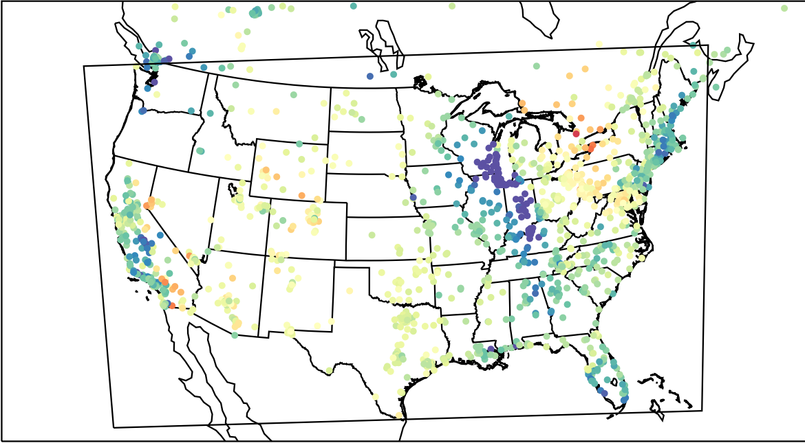
AirNOW (2023-04-16_16:00:00)
