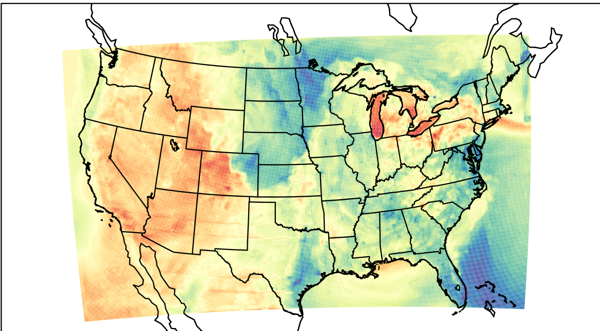
WRF (2023-04-15_01:00:00)
