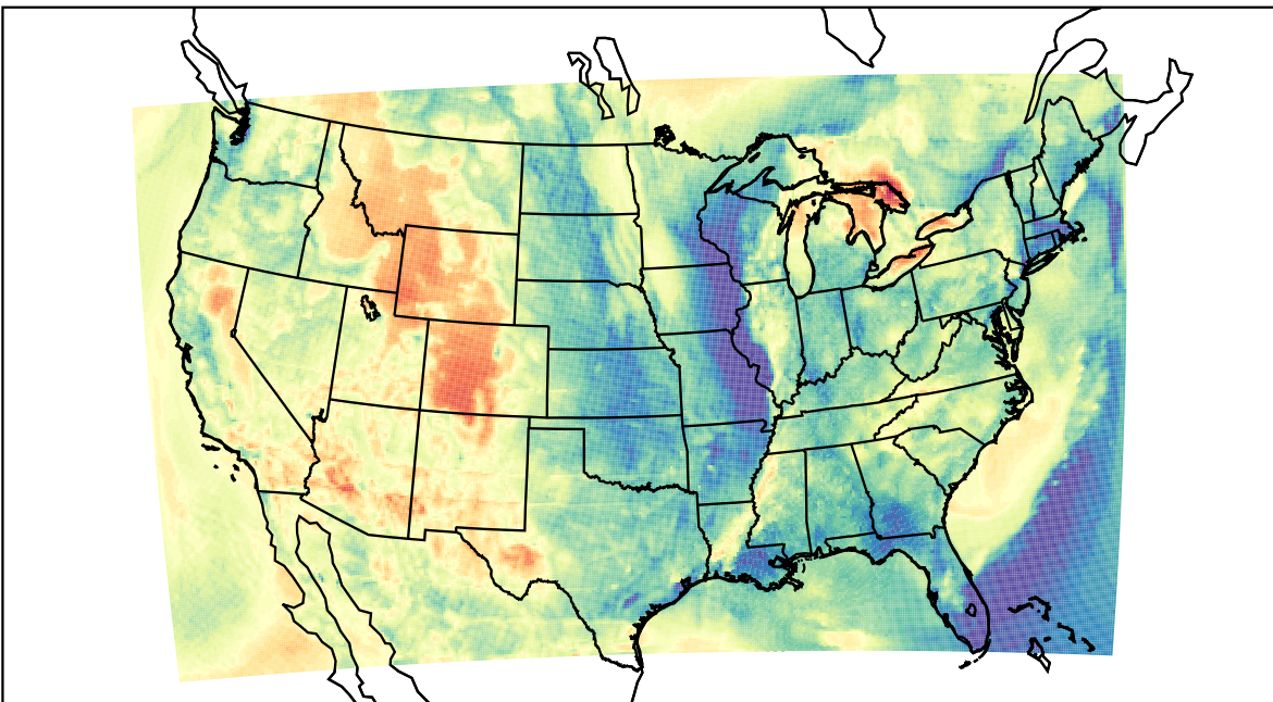
WRF (2023-04-16_05:00:00)
