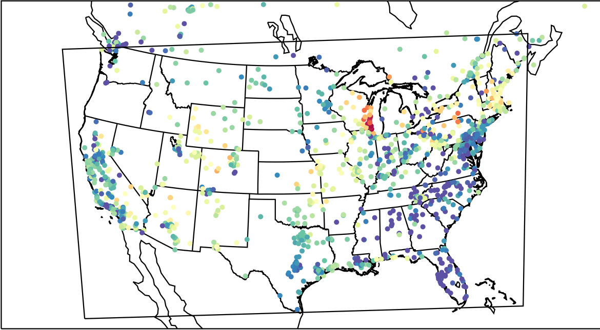
AirNOW (2023-04-15_05:00:00)
