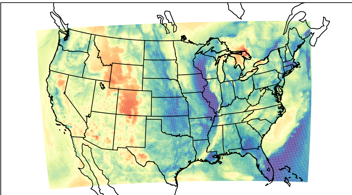
WRF (2023-04-16_07:00:00)
