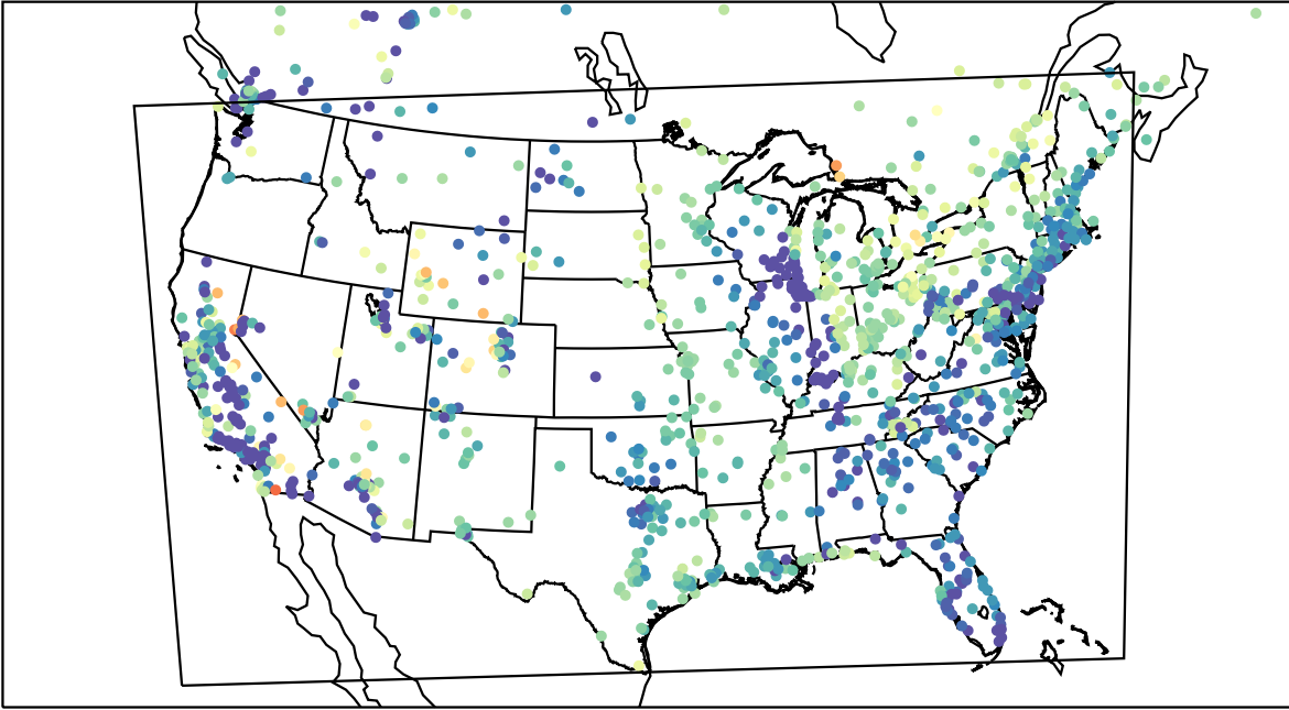
AirNOW (2023-04-16_13:00:00)
