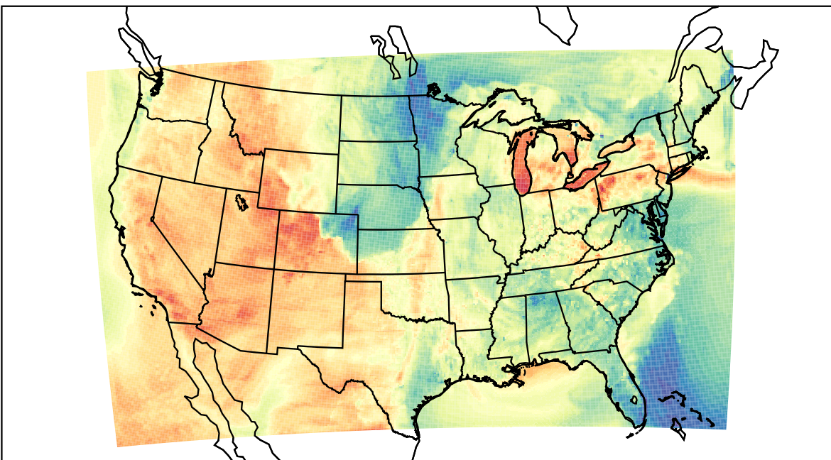
WRF (2023-04-15_00:00:00)
