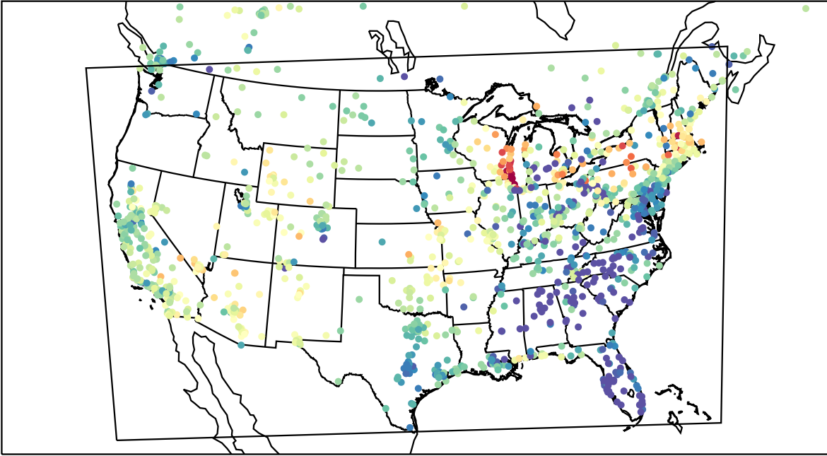
AirNOW (2023-04-15_03:00:00)
