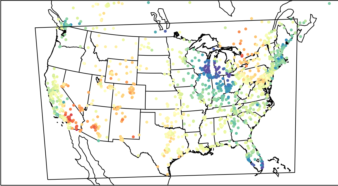
AirNOW (2023-04-16_20:00:00)
