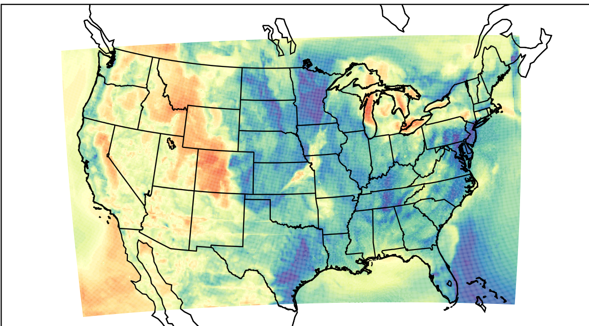
WRF (2023-04-15_07:00:00)
