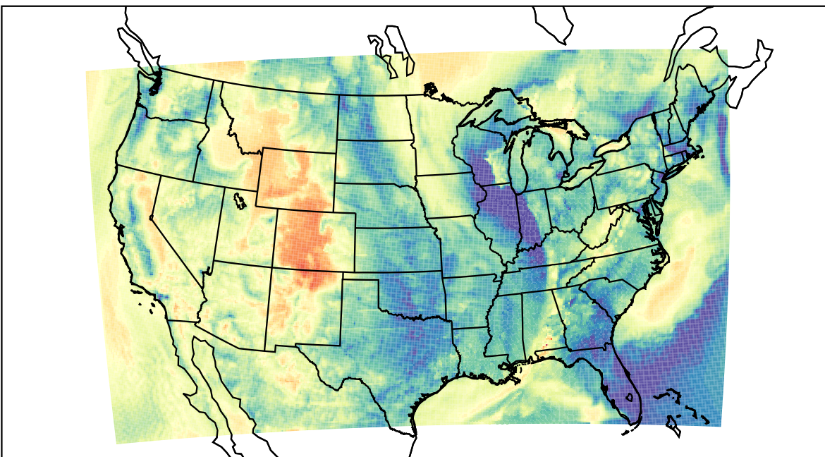
WRF (2023-04-16_13:00:00)
