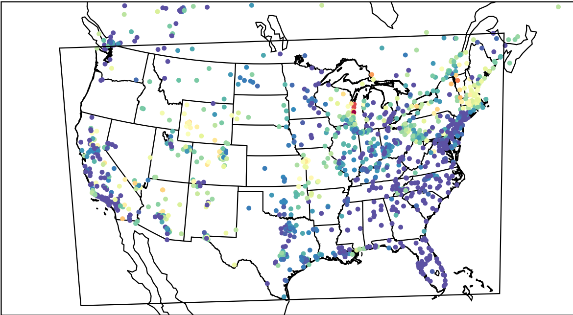
AirNOW (2023-04-15_11:00:00)
