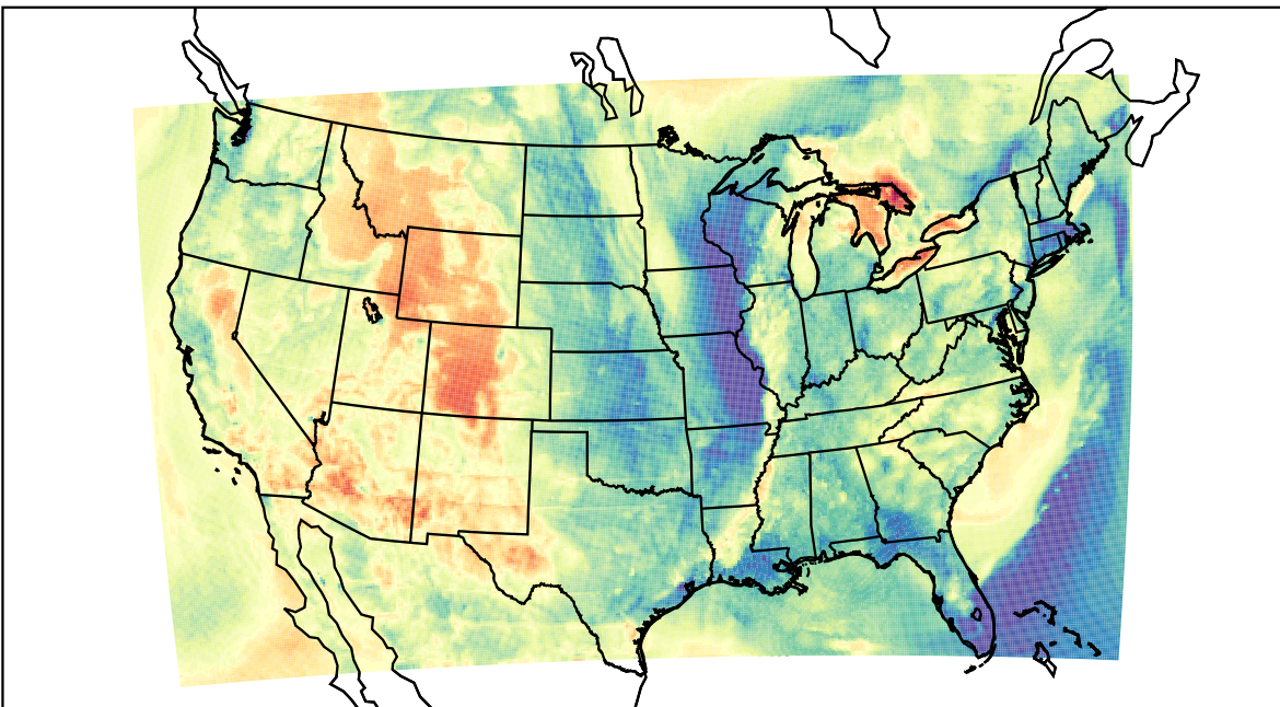
WRF (2023-04-16_04:00:00)
