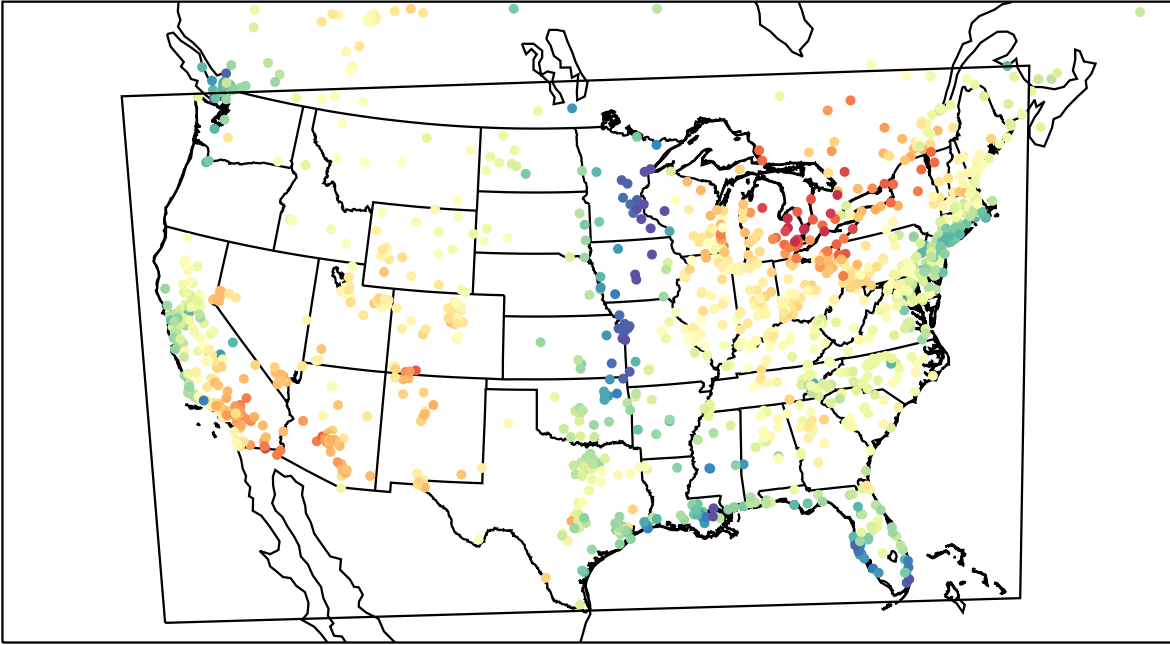
AirNOW (2023-04-15_20:00:00)
