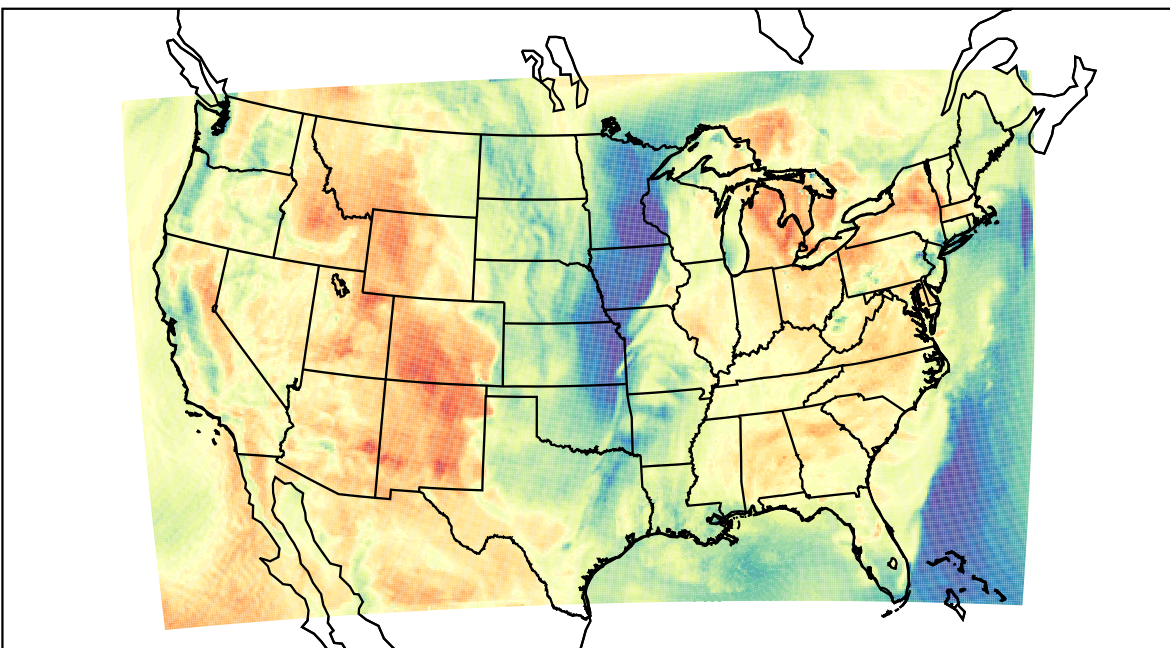
WRF (2023-04-15_17:00:00)
