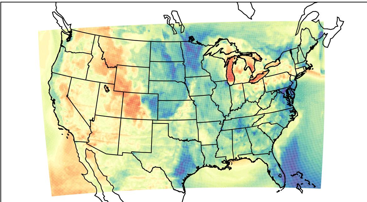
WRF (2023-04-15_03:00:00)
