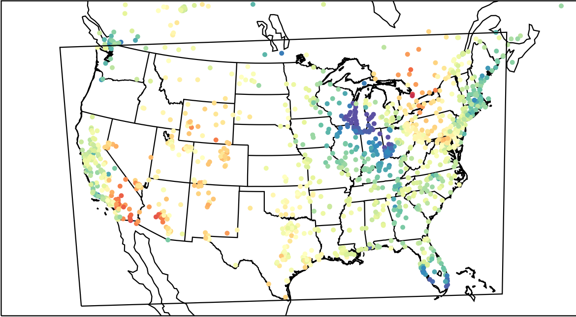
AirNOW (2023-04-16_19:00:00)
