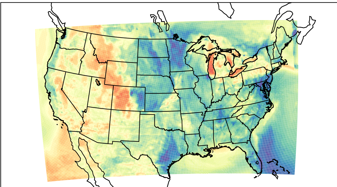
WRF (2023-04-15_04:00:00)
