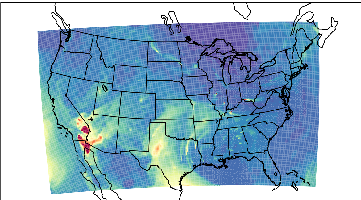
WRF 2023-04-18_15:00:00
