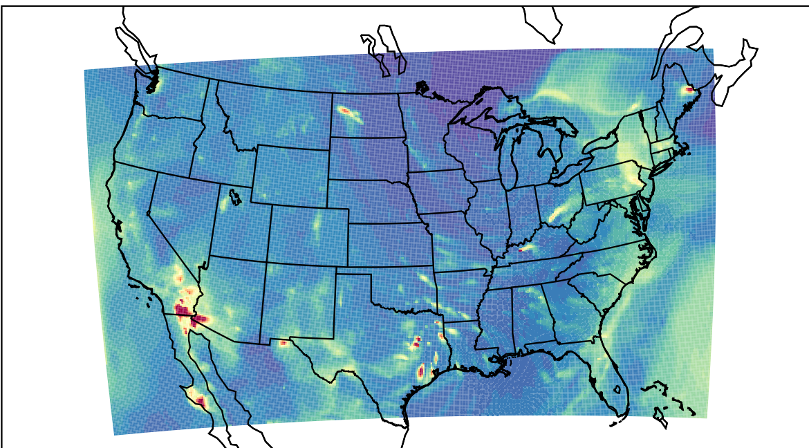
WRF 2023-04-17_05:00:00
