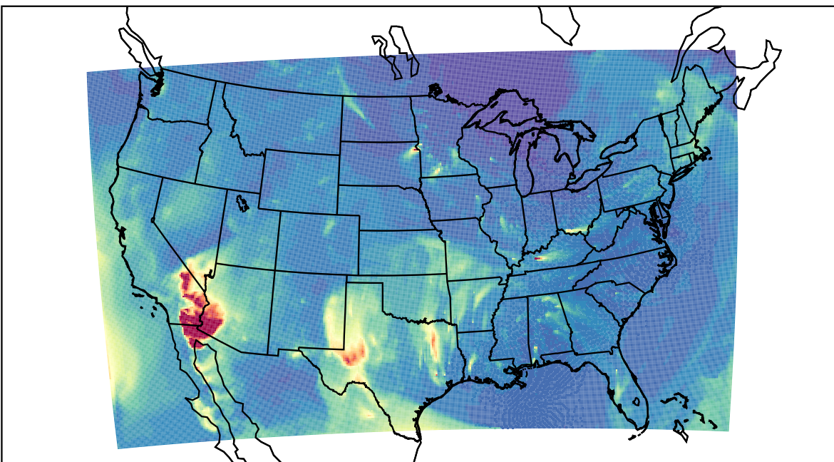
WRF 2023-04-18_07:00:00
