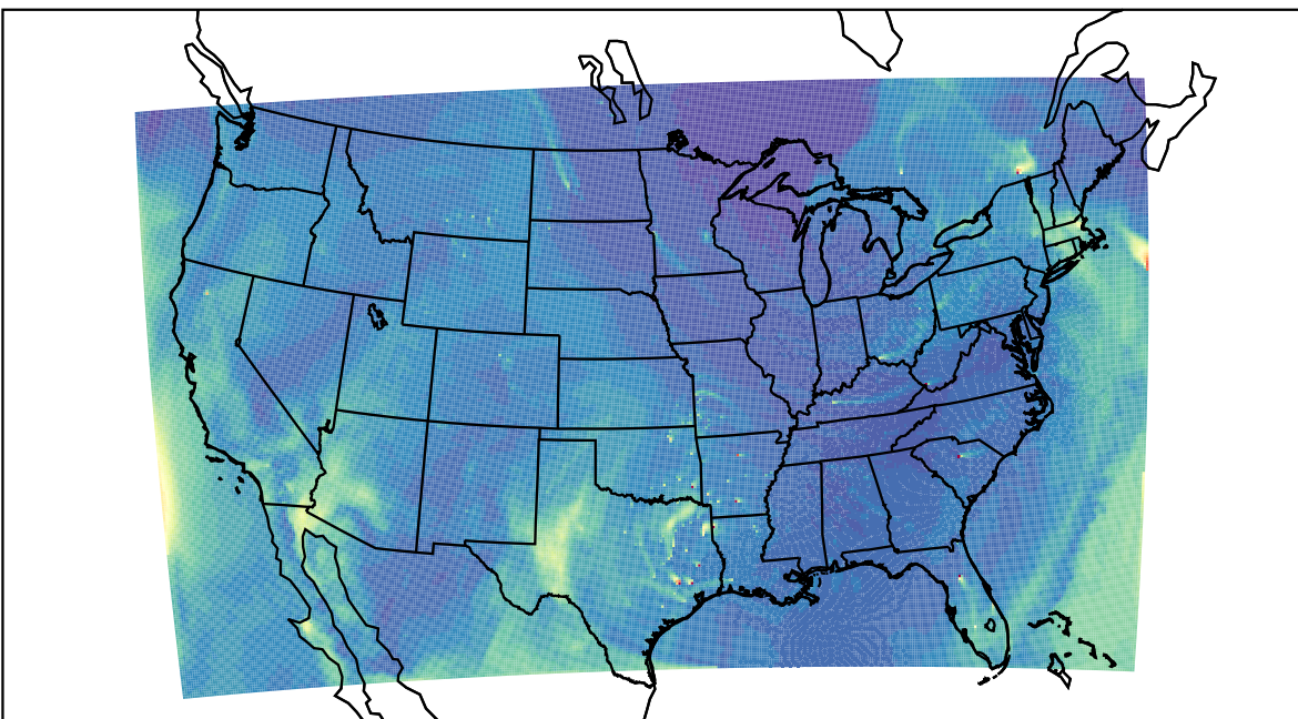
WRF 2023-04-17_20:00:00
