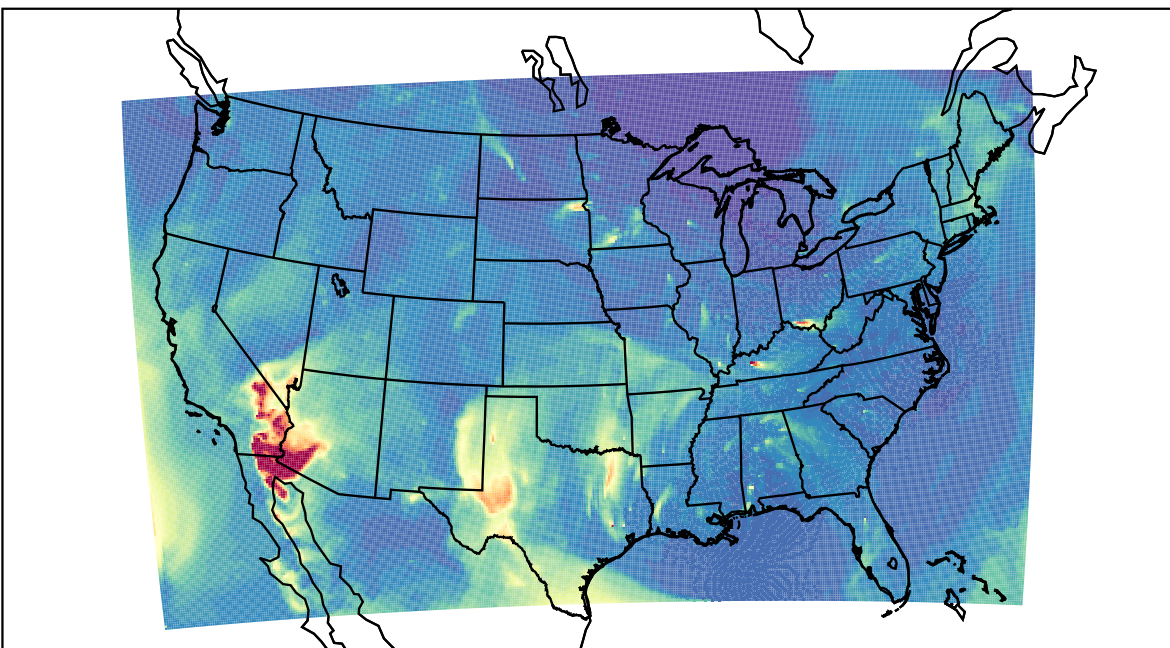
WRF 2023-04-18_09:00:00
