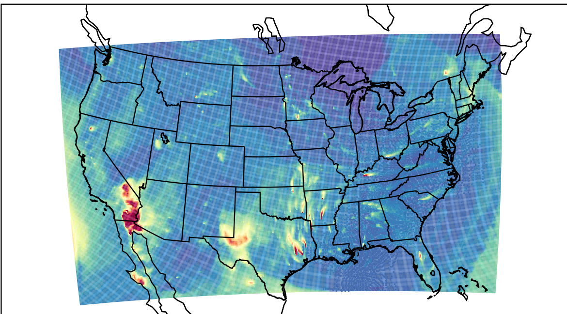
WRF 2023-04-18_03:00:00
