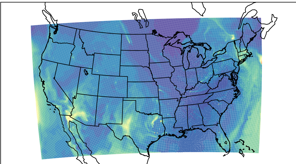
WRF 2023-04-17_18:00:00
