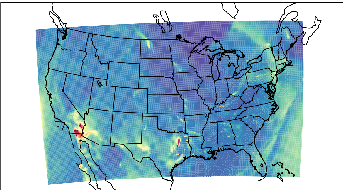
WRF 2023-04-17_12:00:00
