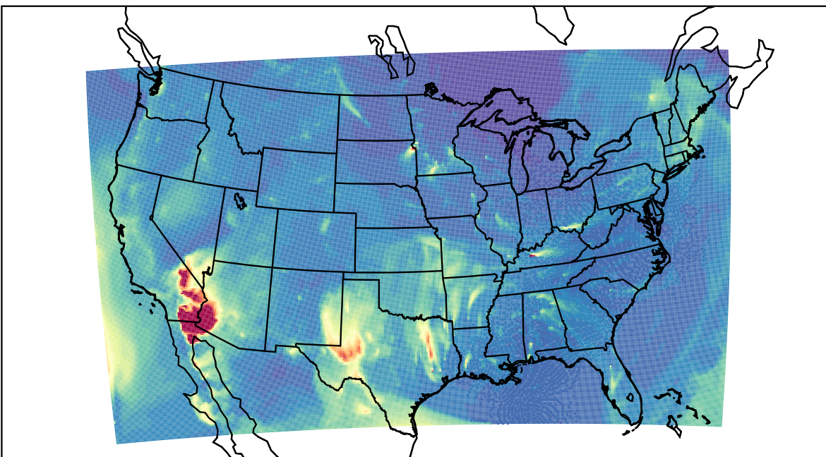
WRF 2023-04-18_06:00:00
