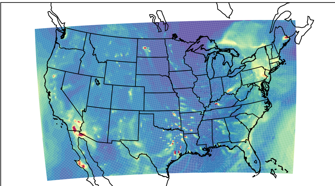
WRF 2023-04-17_03:00:00
