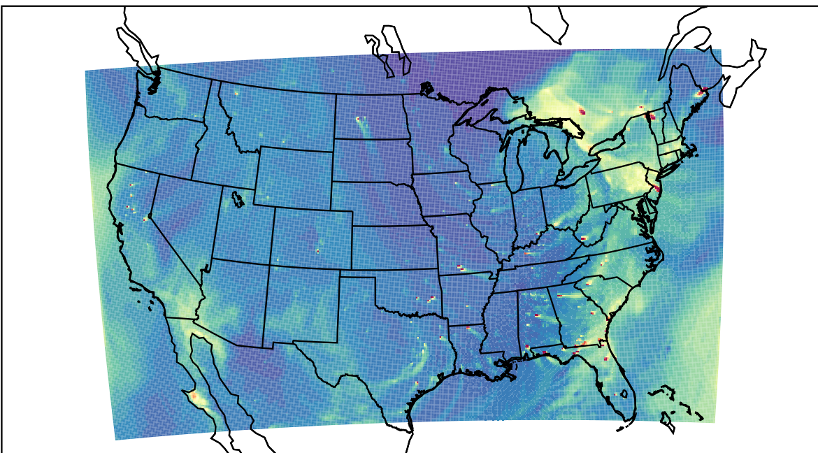
WRF 2023-04-17_00:00:00
