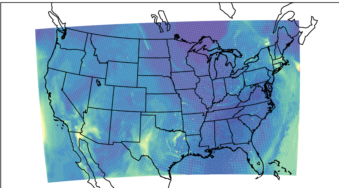
WRF 2023-04-17_19:00:00
