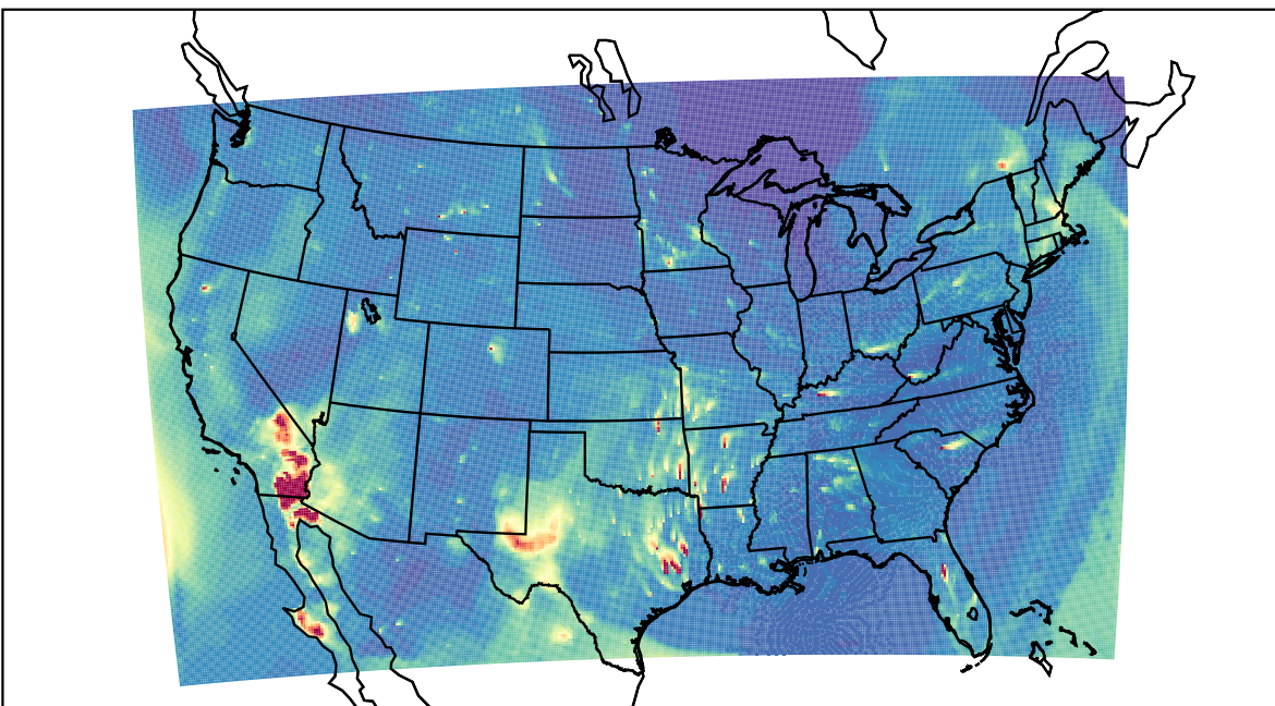
WRF 2023-04-18_02:00:00
