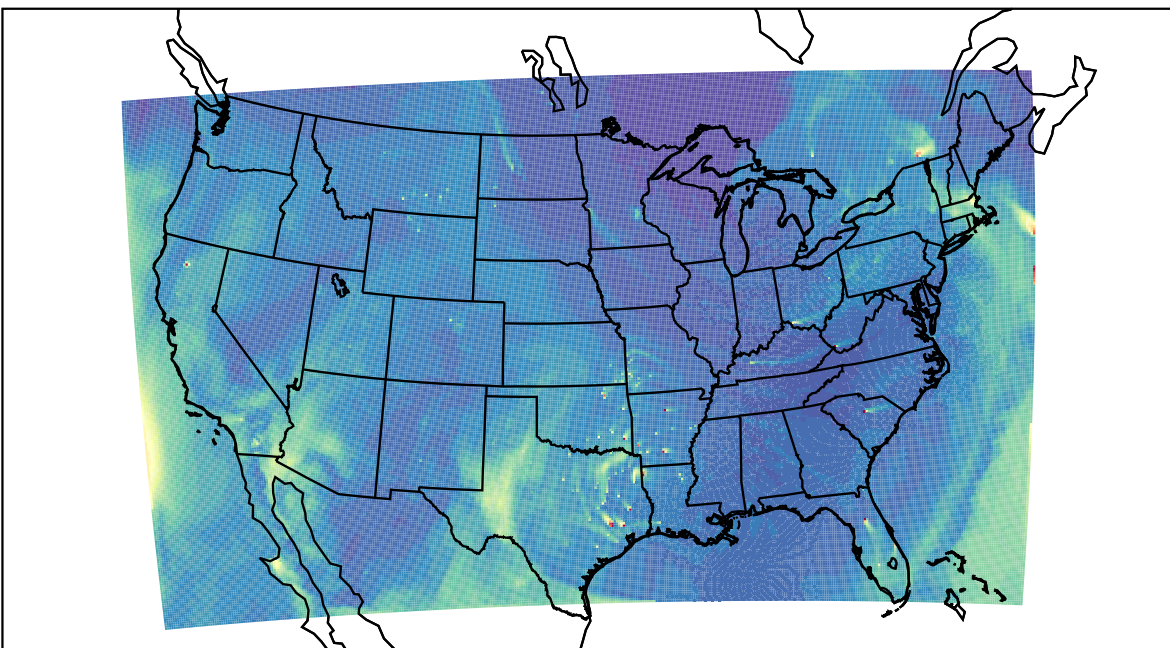
WRF 2023-04-17_21:00:00
