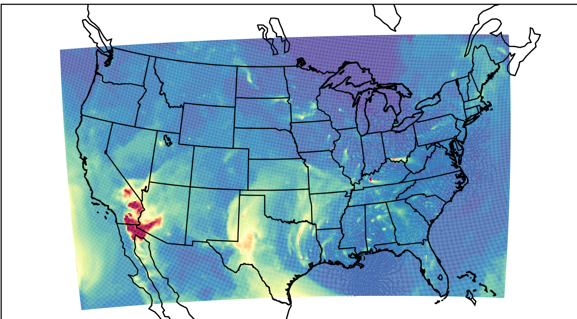
WRF 2023-04-18_12:00:00
