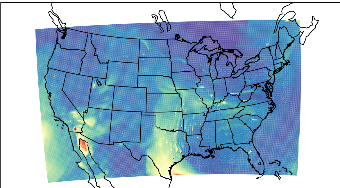
WRF 2023-04-18_22:00:00
