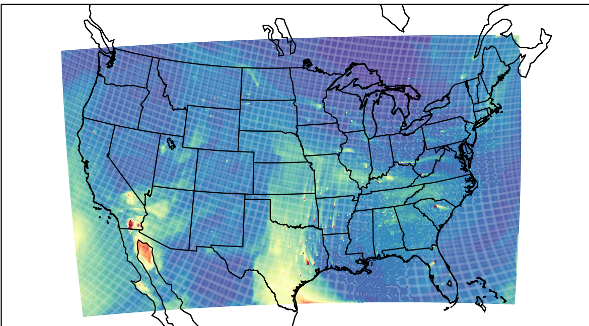
WRF 2023-04-18_23:00:00
