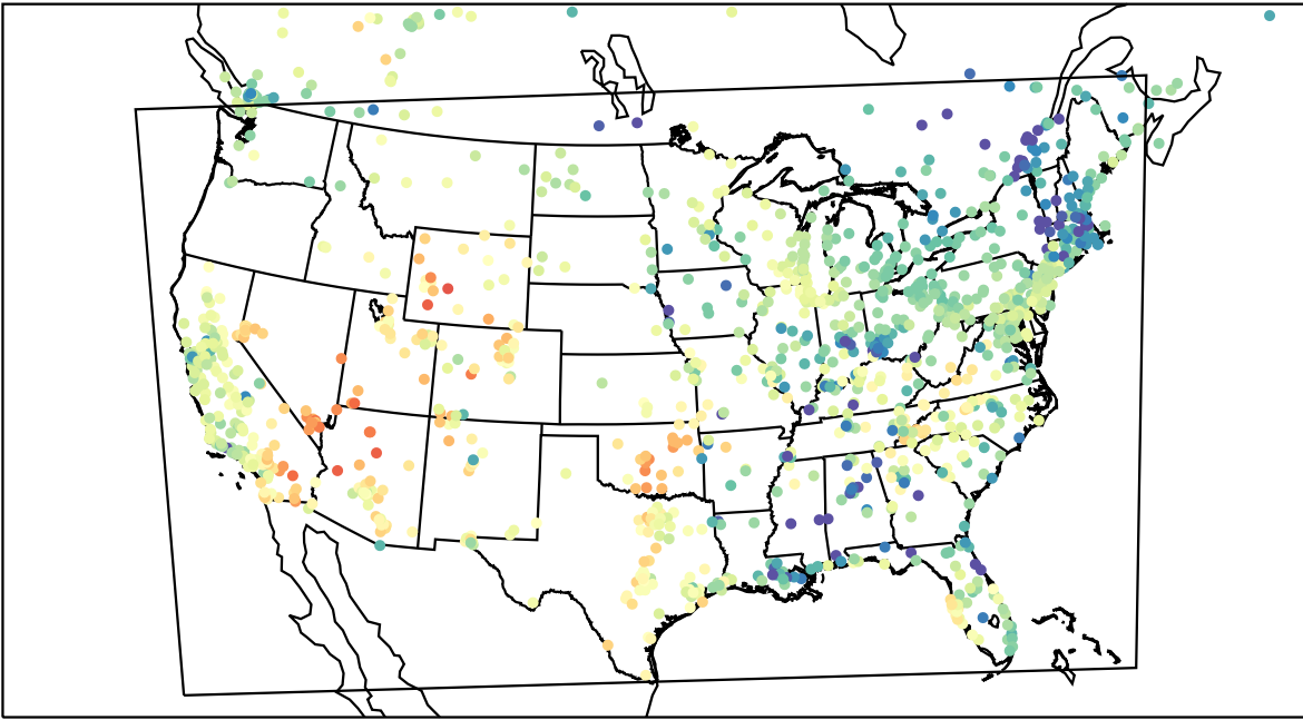
AirNOW (2023-04-18_02:00:00)
