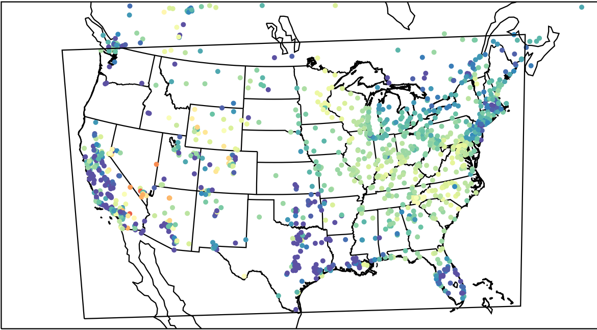
AirNOW (2023-04-17_13:00:00)
