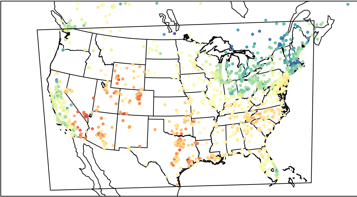
AirNOW (2023-04-17_20:00:00)
