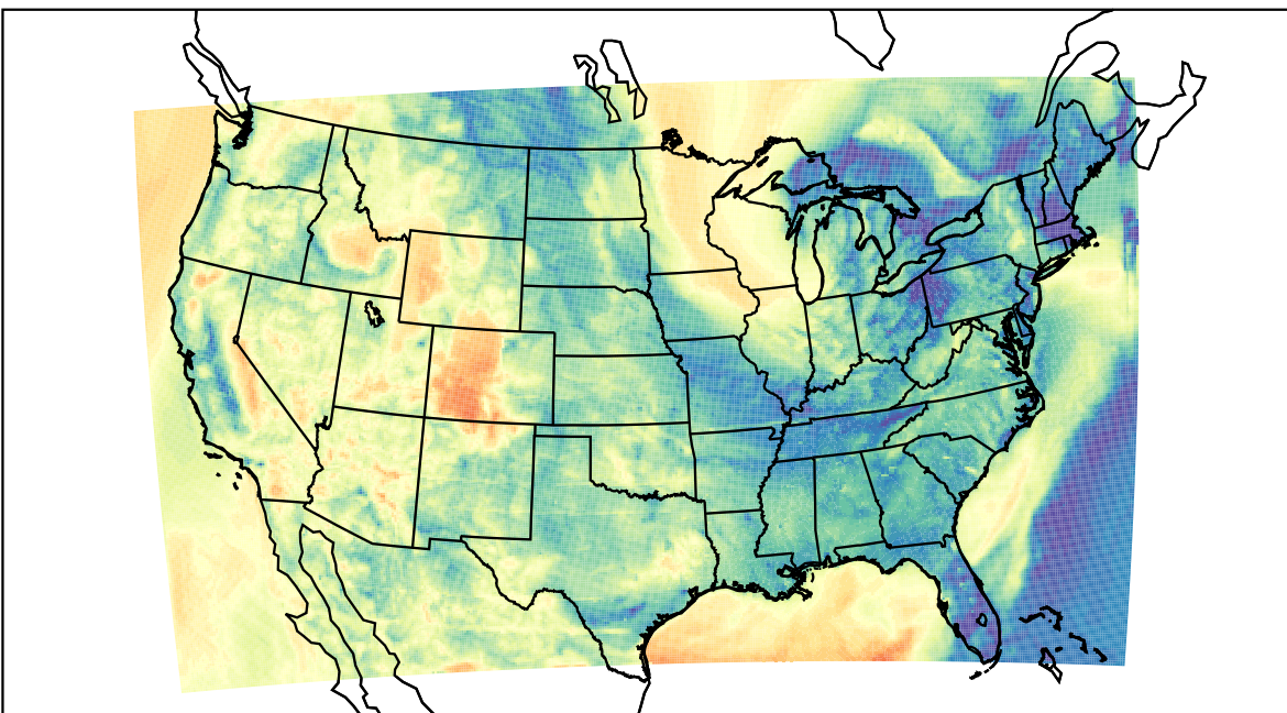
WRF (2023-04-17_10:00:00)
