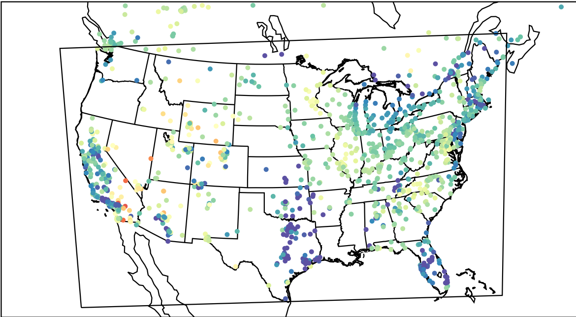
AirNOW (2023-04-17_07:00:00)
