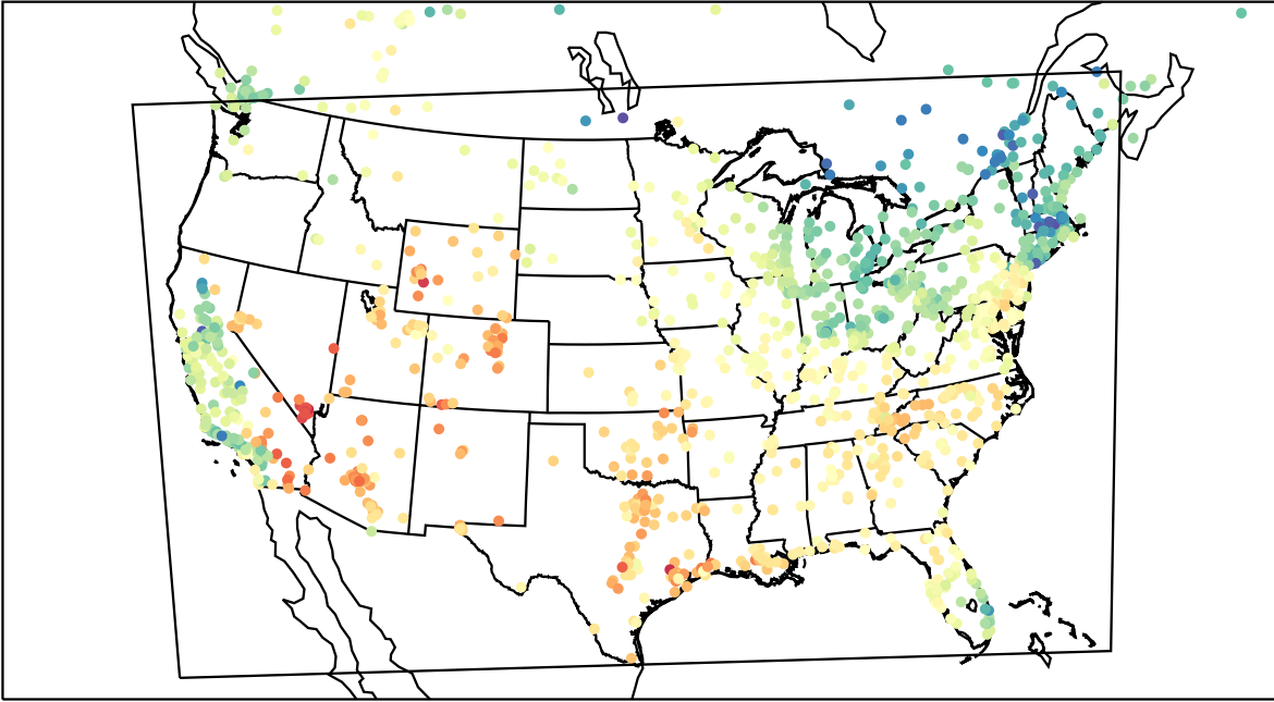
AirNOW (2023-04-17_19:00:00)
