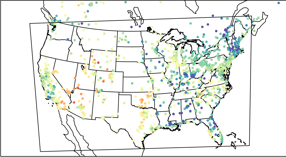
AirNOW (2023-04-18_03:00:00)
