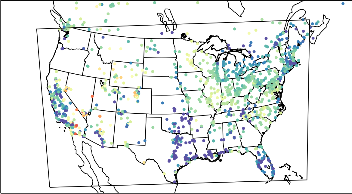
AirNOW (2023-04-17_09:00:00)
