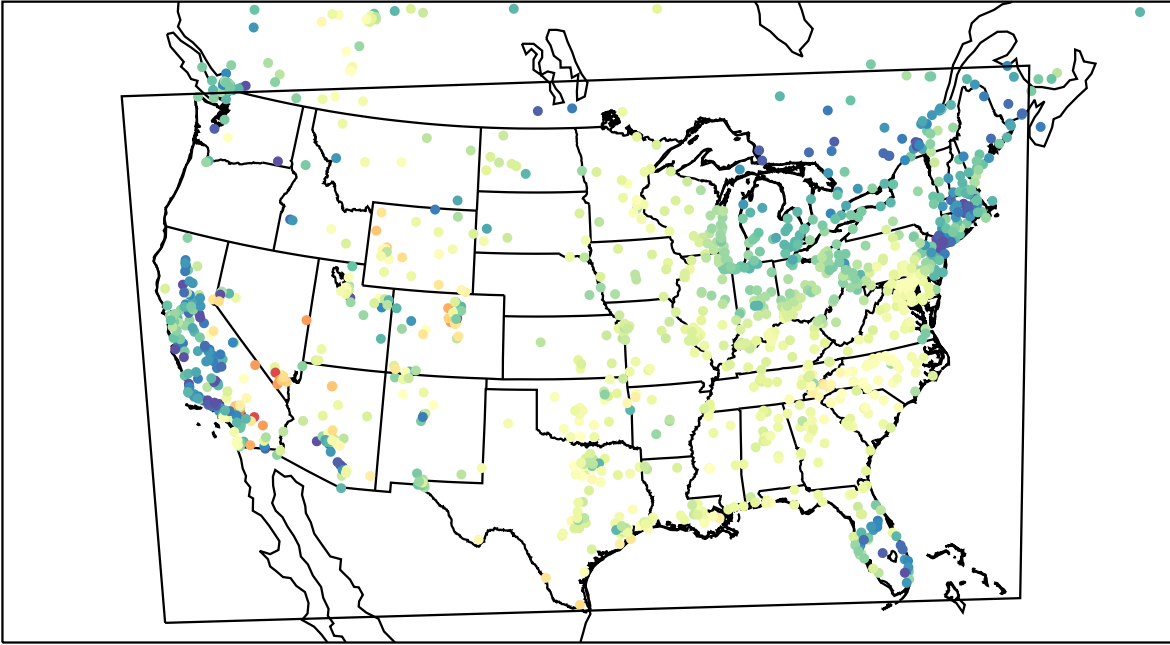
AirNOW (2023-04-17_15:00:00)
