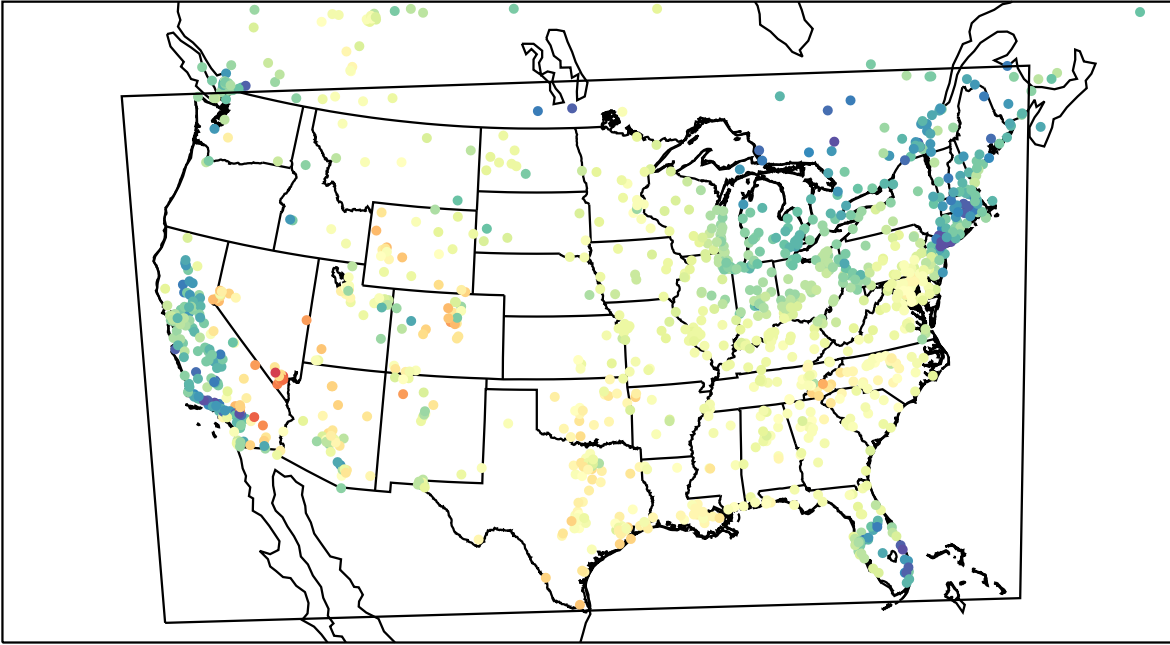
AirNOW (2023-04-17_16:00:00)
