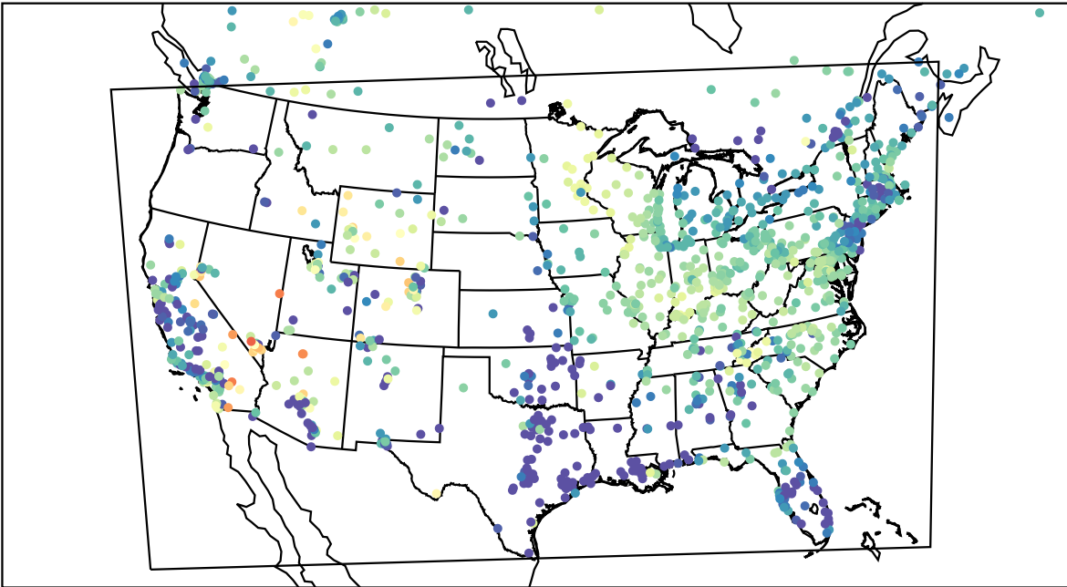
AirNOW (2023-04-17_12:00:00)
