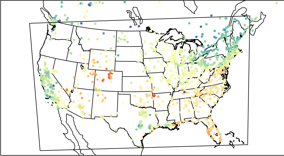
AirNOW (2023-04-18_16:00:00)
