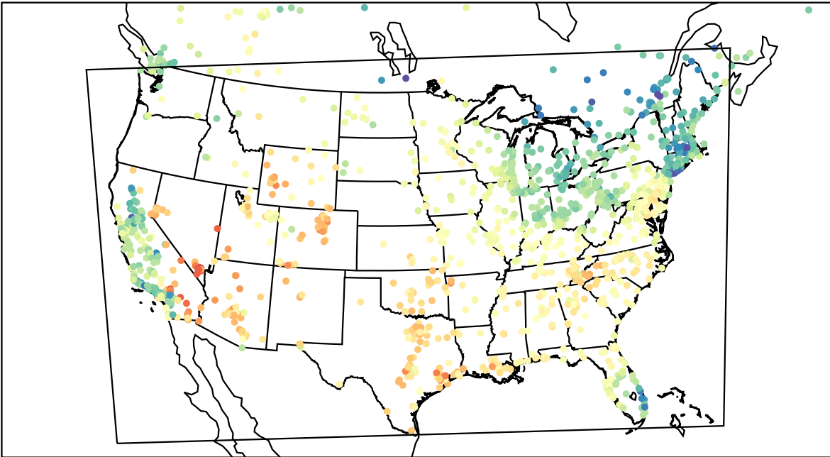
AirNOW (2023-04-17_18:00:00)
