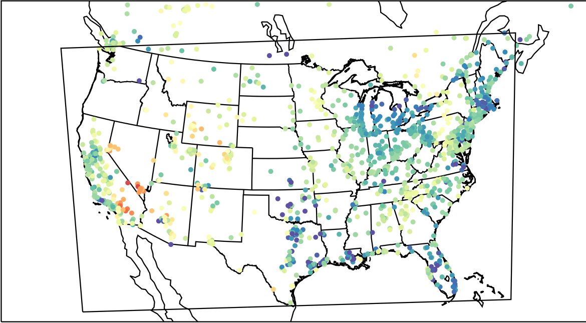
AirNOW (2023-04-17_03:00:00)
