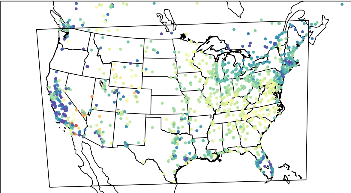
AirNOW (2023-04-17_14:00:00)
