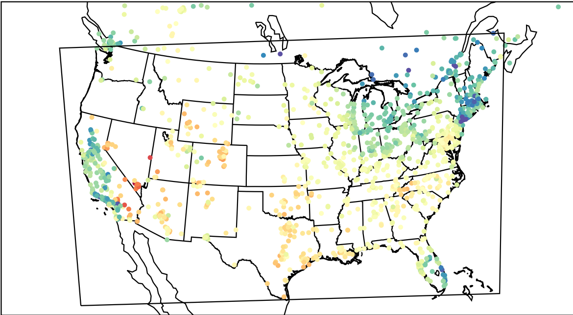
AirNOW (2023-04-17_17:00:00)
