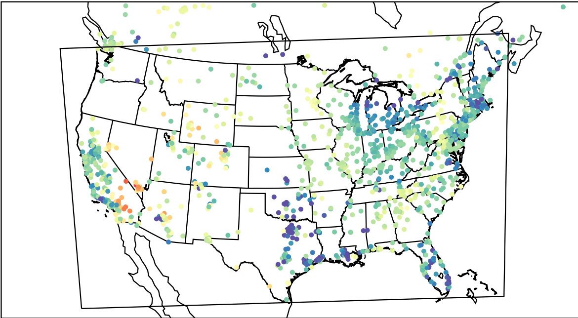
AirNOW (2023-04-17_04:00:00)
