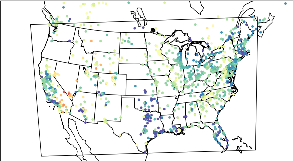
AirNOW (2023-04-17_05:00:00)
