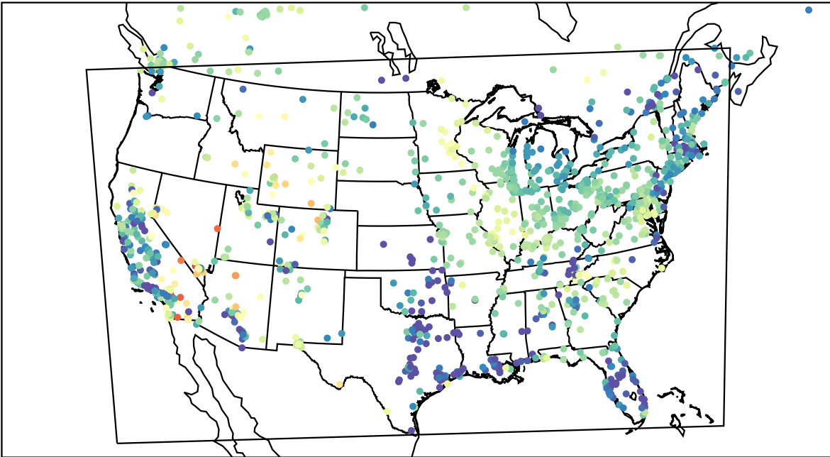
AirNOW (2023-04-17_08:00:00)
