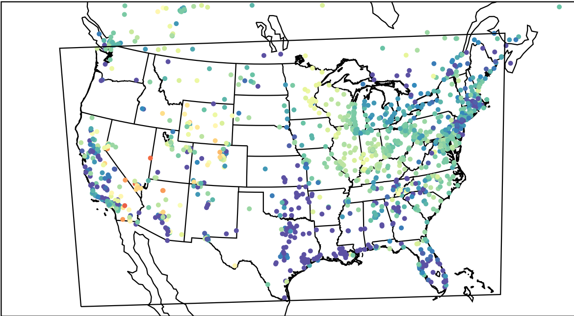
AirNOW (2023-04-17_11:00:00)
