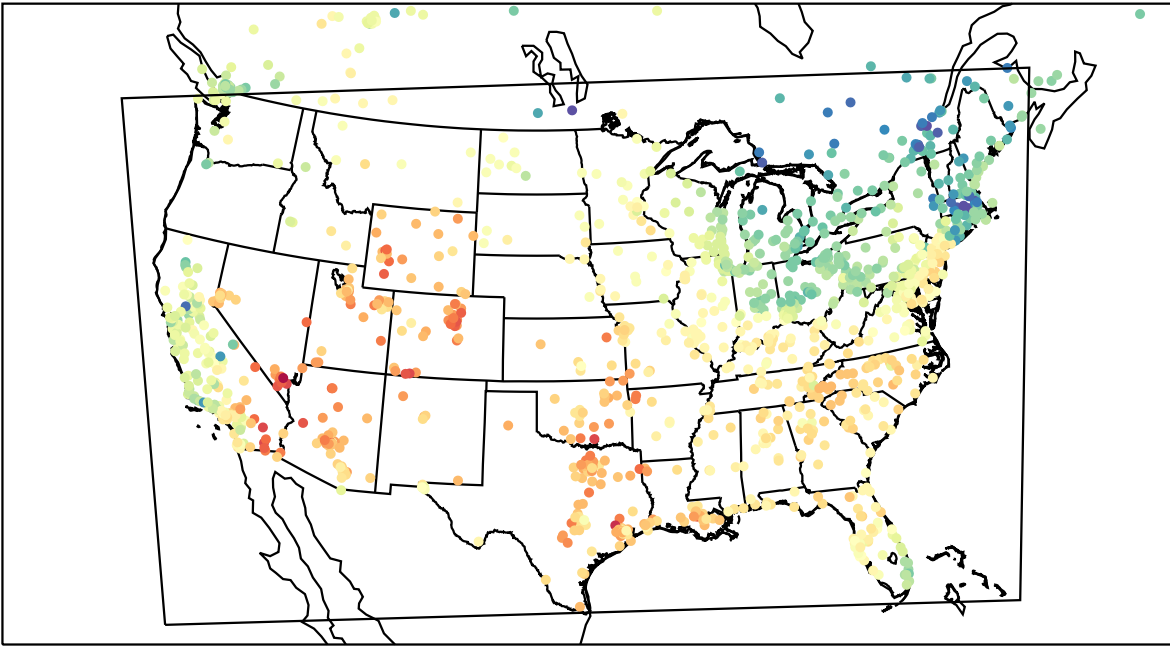
AirNOW (2023-04-17_21:00:00)
