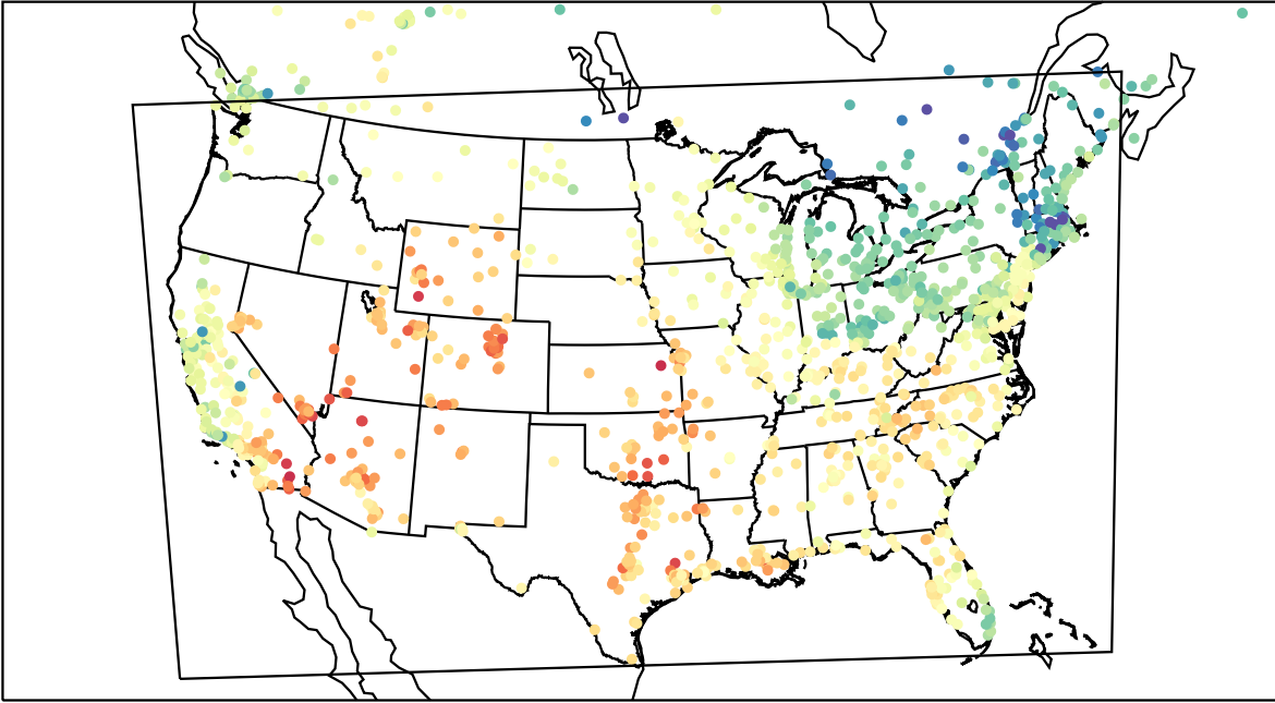
AirNOW (2023-04-17_23:00:00)
