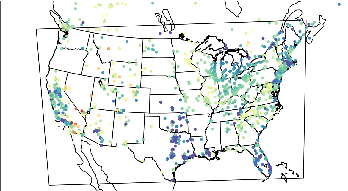
AirNOW (2023-04-17_06:00:00)
