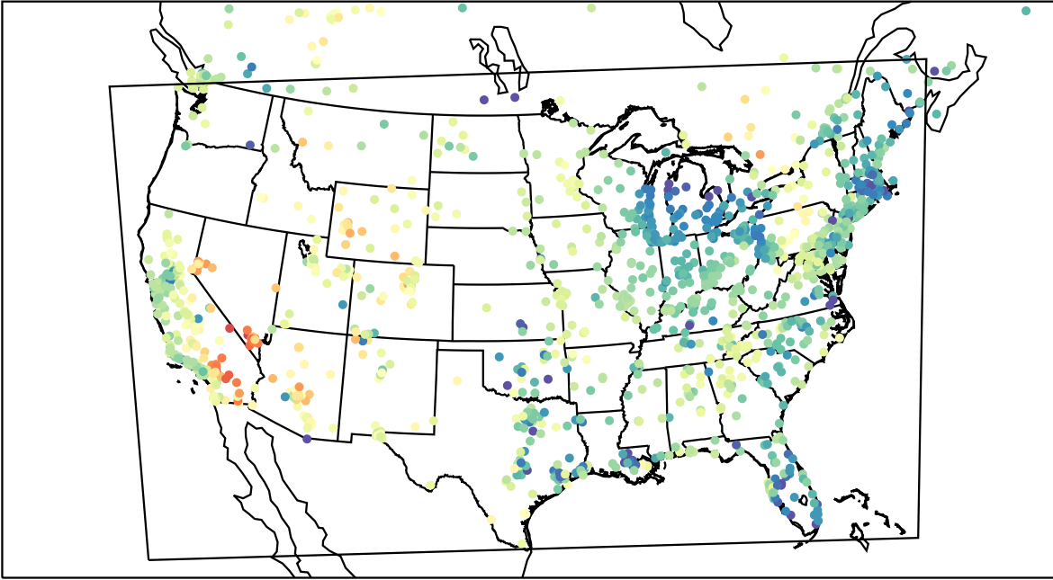
AirNOW (2023-04-17_02:00:00)
