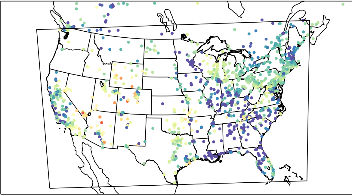
AirNOW (2023-04-18_11:00:00)
