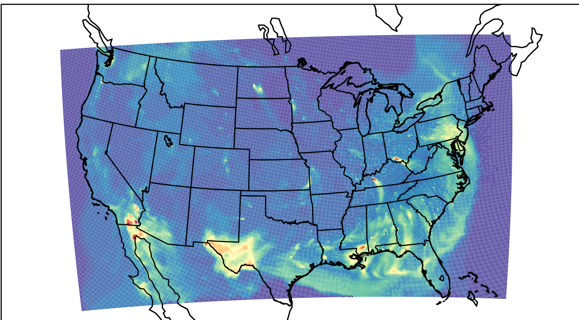
WRF 2023-04-23_08:00:00
