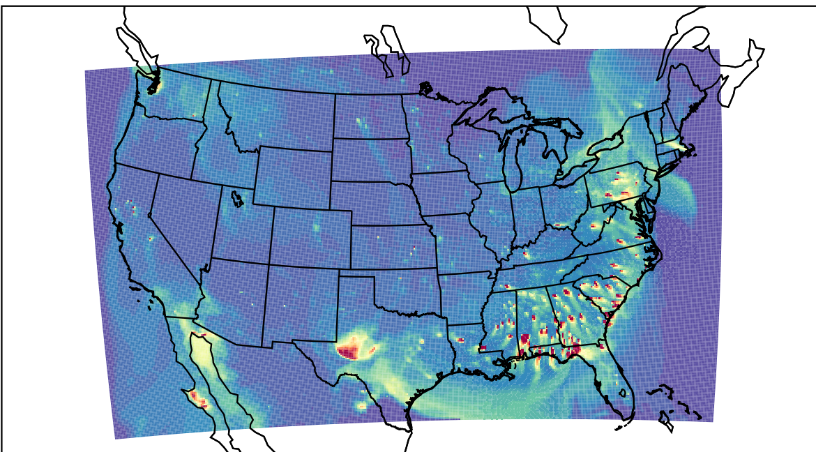
WRF 2023-04-23_01:00:00
