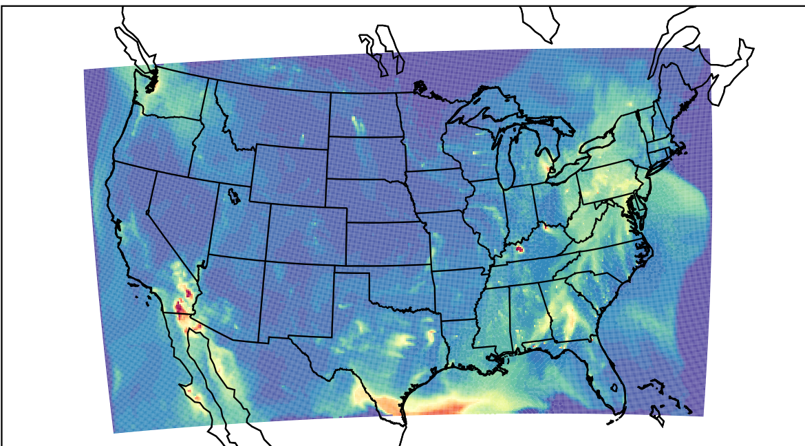
WRF 2023-04-22_09:00:00
