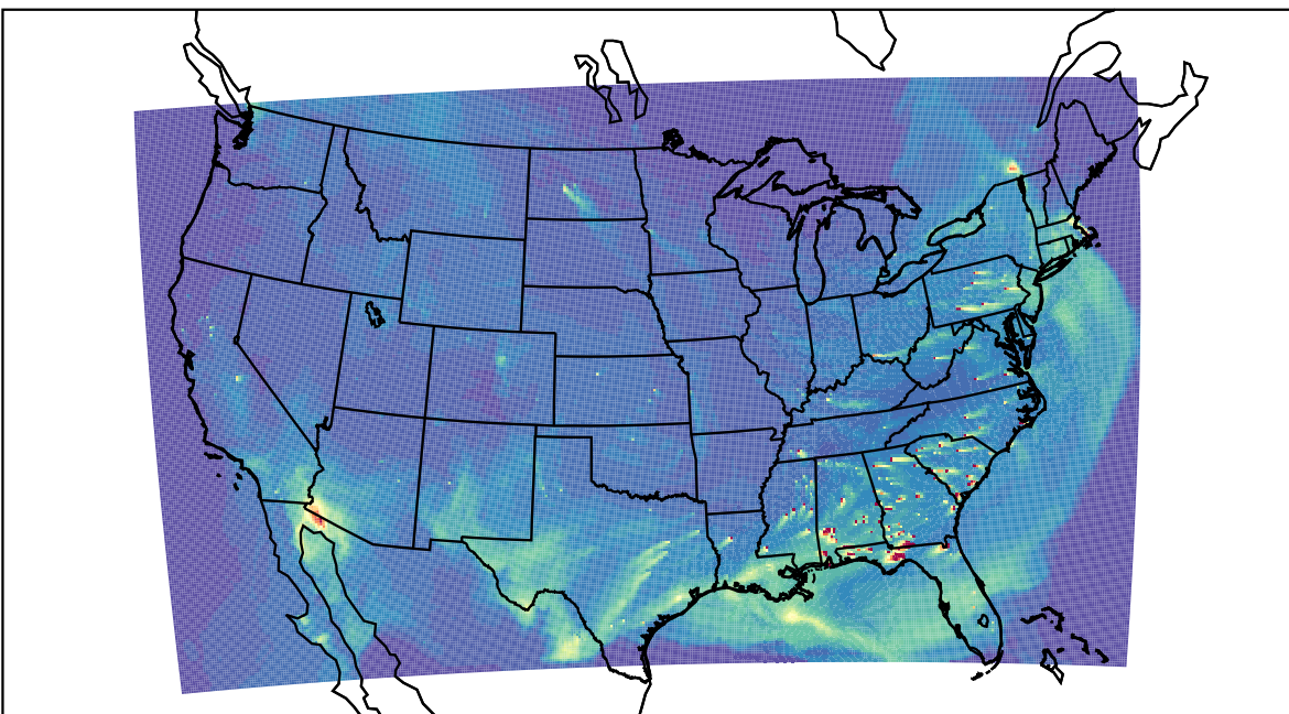
WRF 2023-04-23_22:00:00
