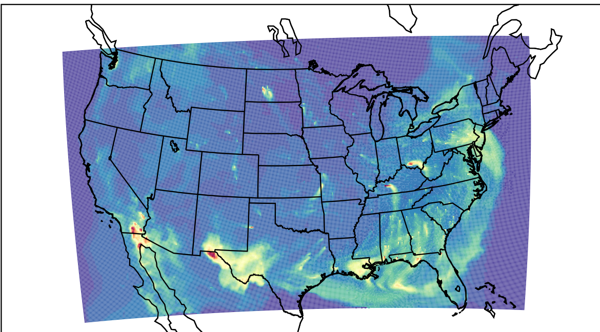
WRF 2023-04-23_11:00:00
