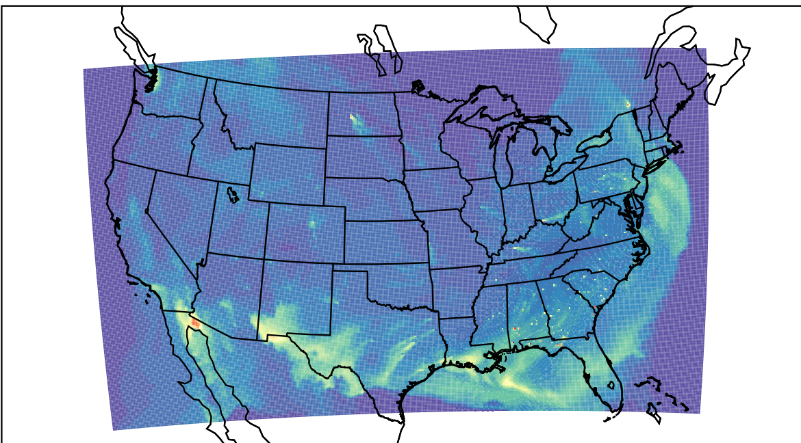
WRF 2023-04-23_17:00:00
