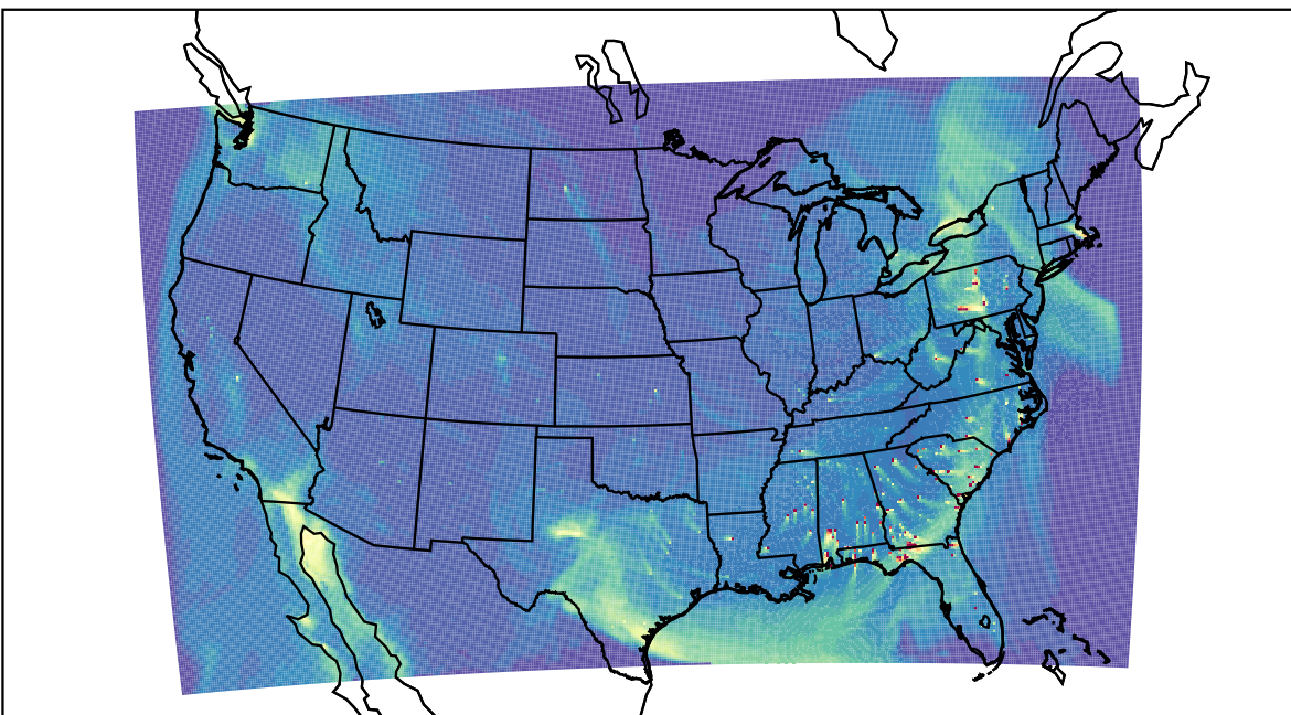
WRF 2023-04-22_21:00:00
