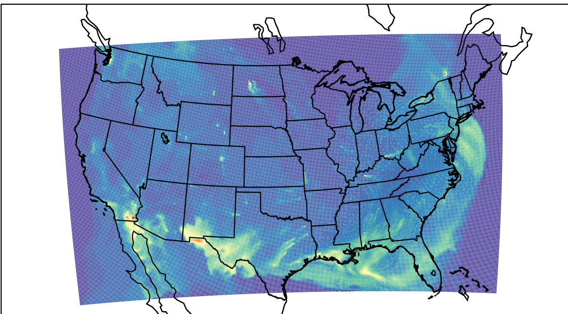
WRF 2023-04-23_15:00:00
