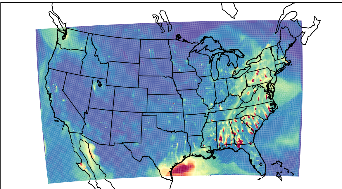
WRF 2023-04-22_01:00:00
