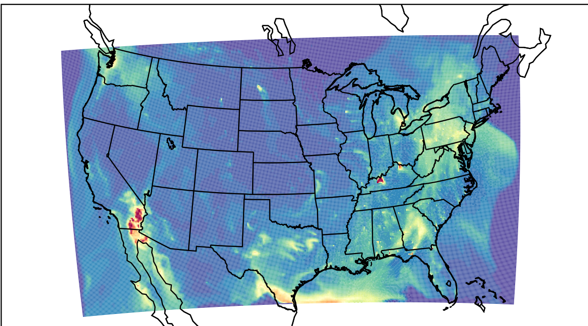
WRF 2023-04-22_11:00:00
