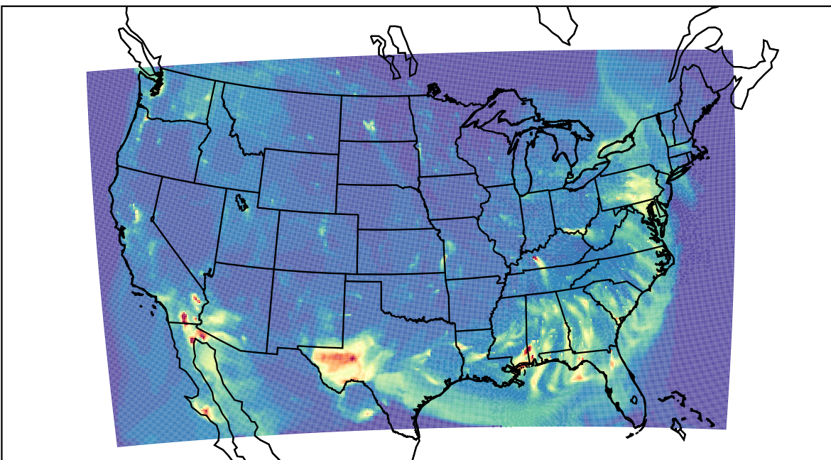
WRF 2023-04-23_05:00:00
