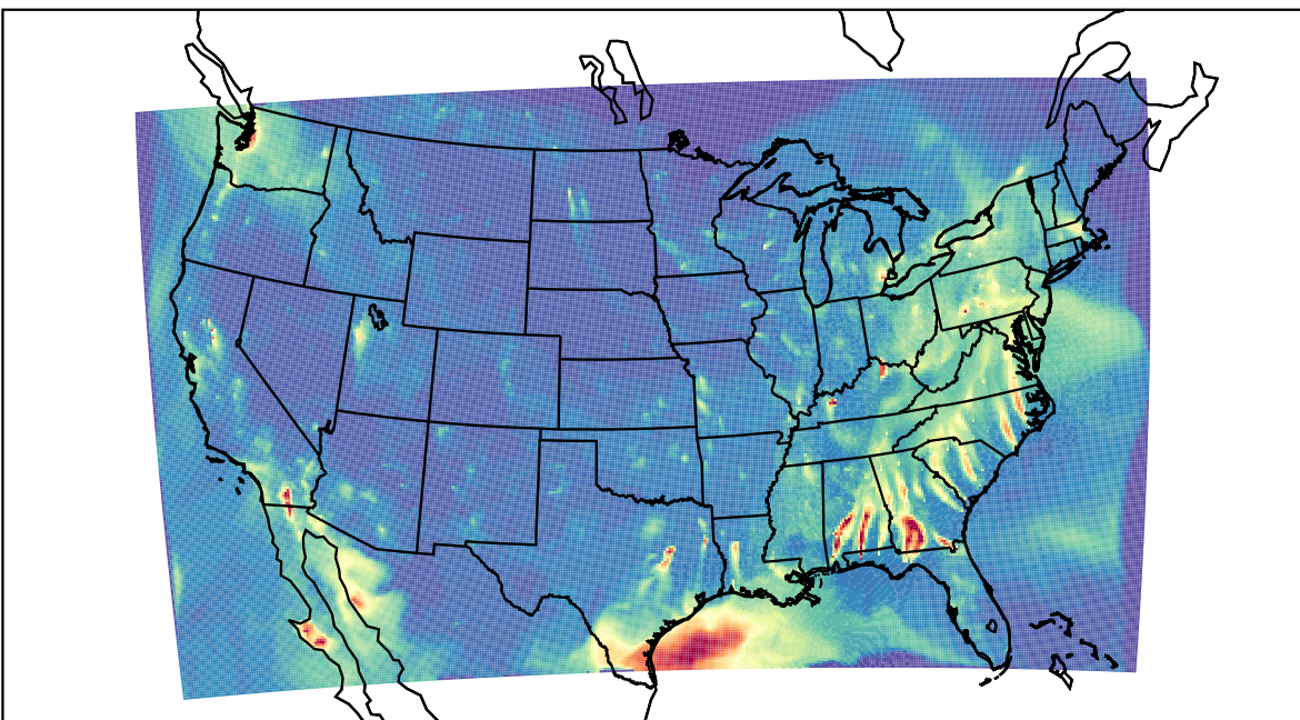
WRF 2023-04-22_04:00:00
