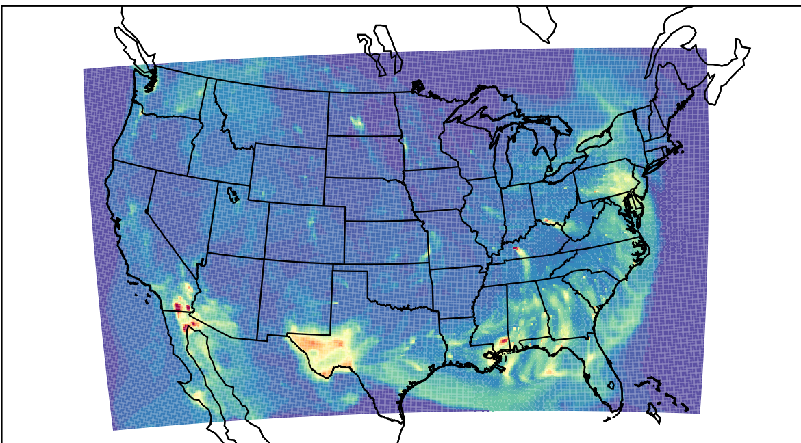
WRF 2023-04-23_07:00:00
