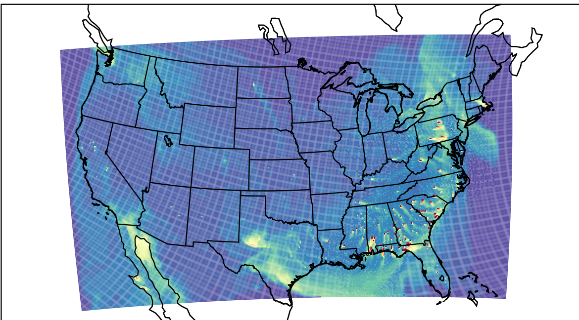
WRF 2023-04-22_23:00:00
