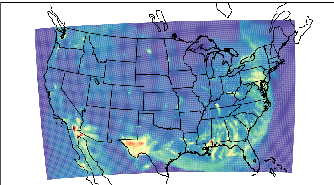
WRF 2023-04-23_06:00:00
