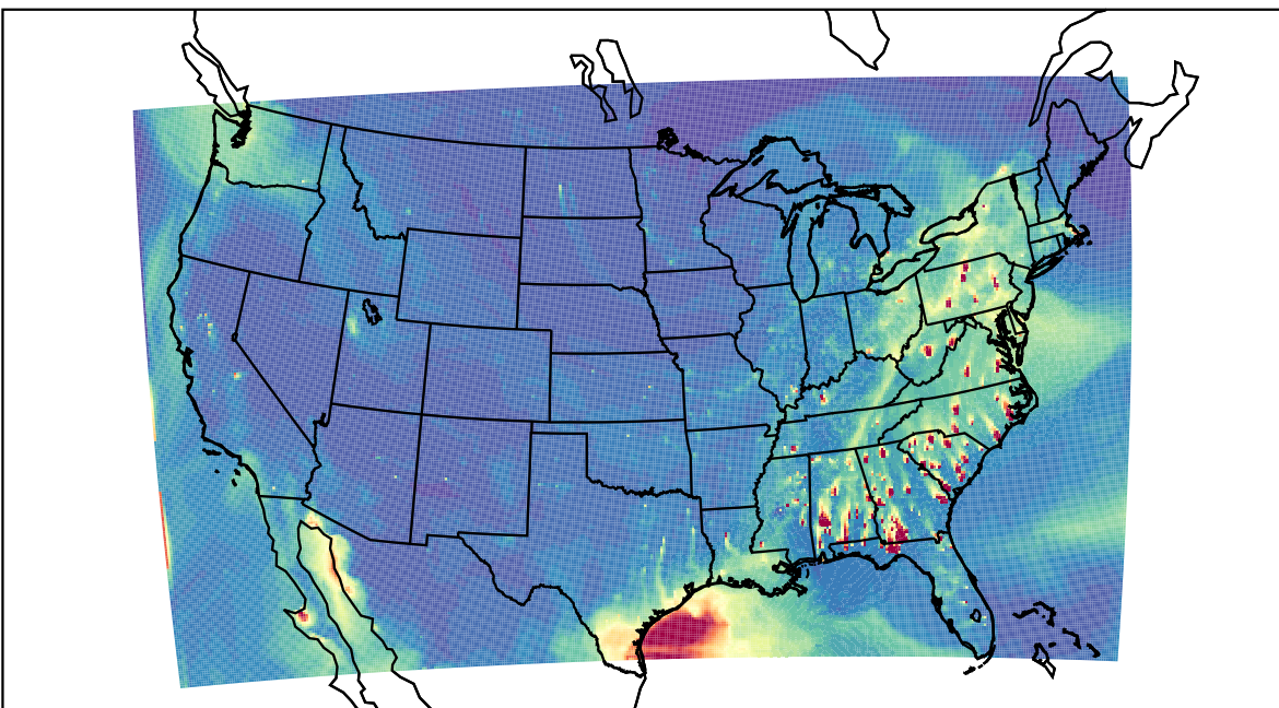
WRF 2023-04-22_00:00:00
