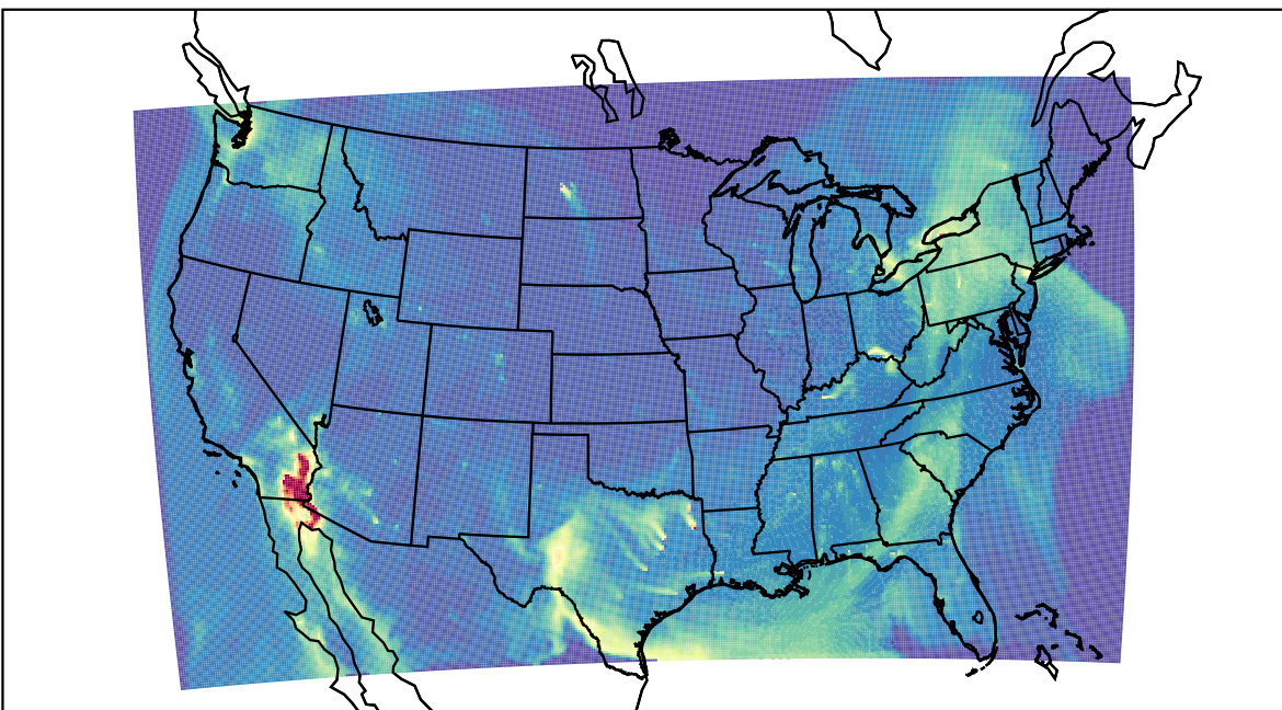
WRF 2023-04-22_15:00:00
