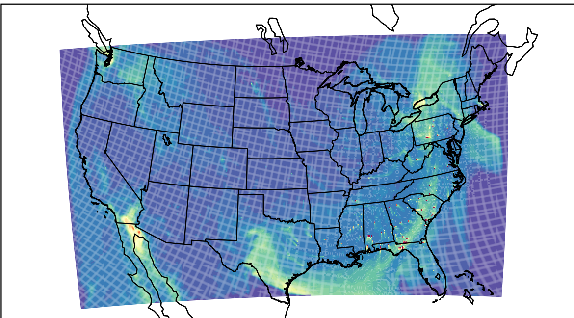
WRF 2023-04-22_19:00:00
