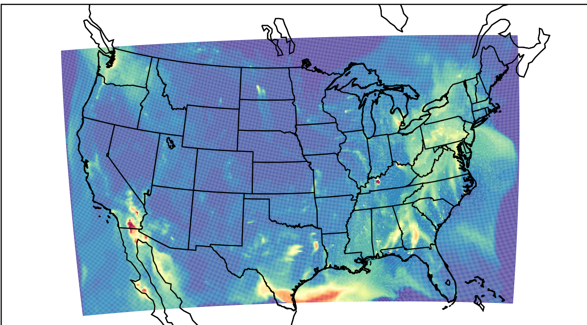
WRF 2023-04-22_08:00:00
