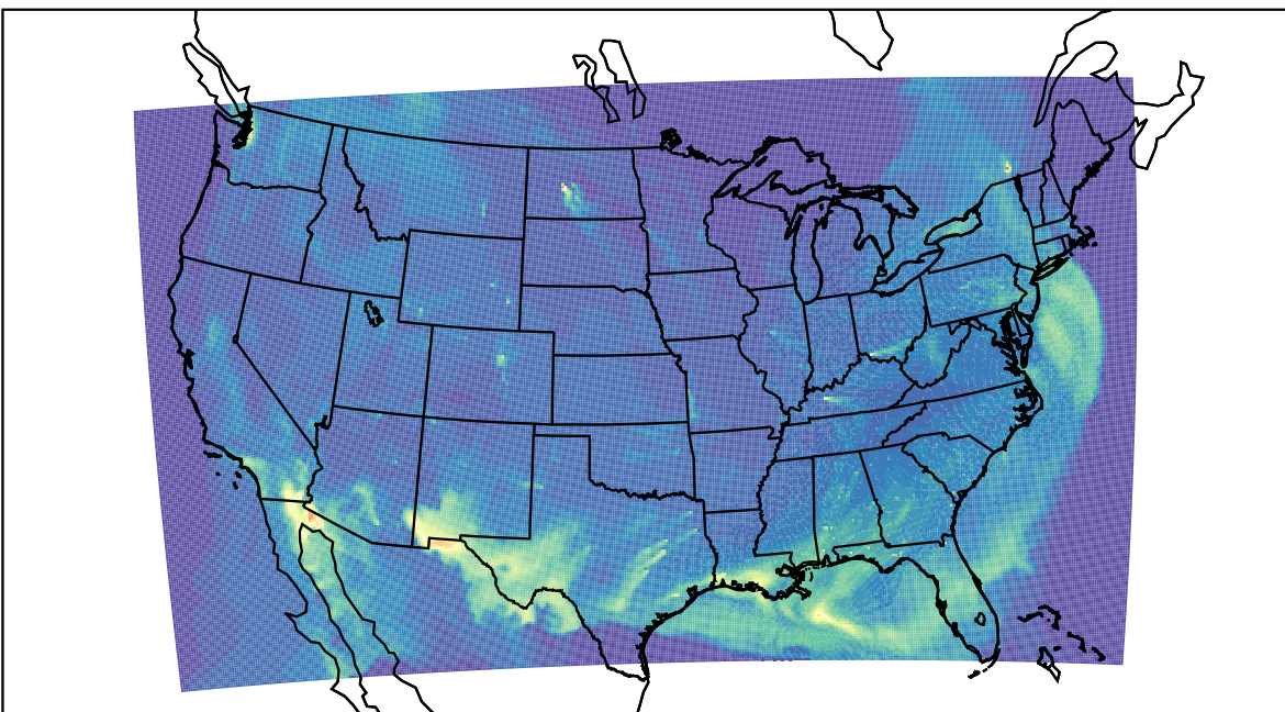
WRF 2023-04-23_16:00:00
