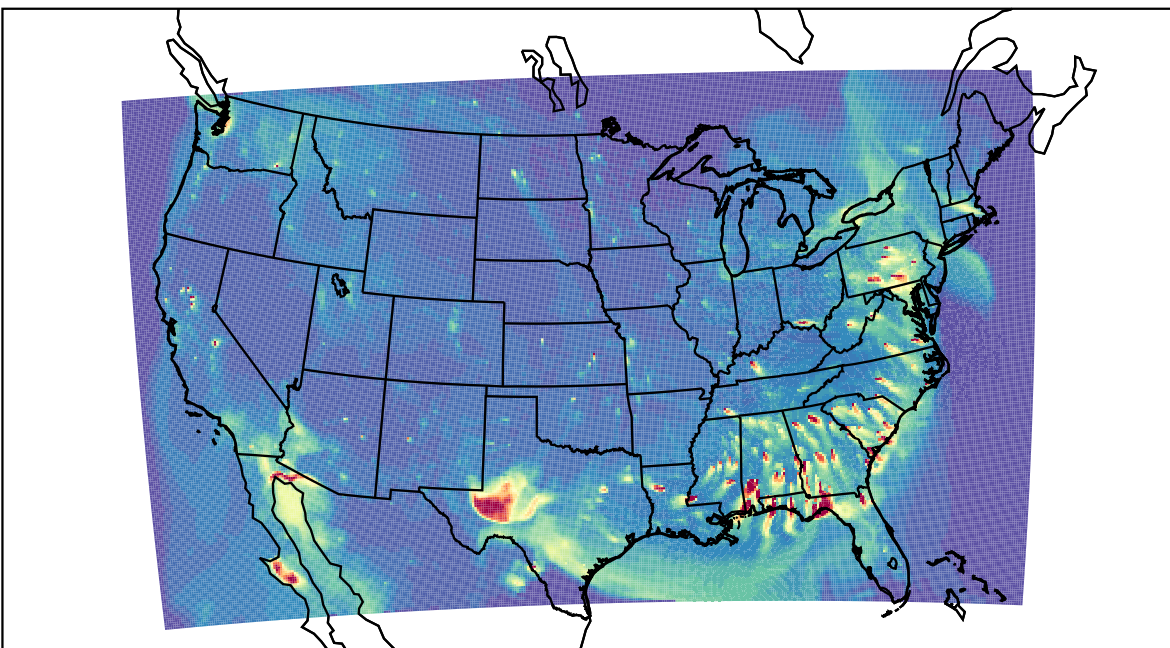
WRF 2023-04-23_02:00:00
