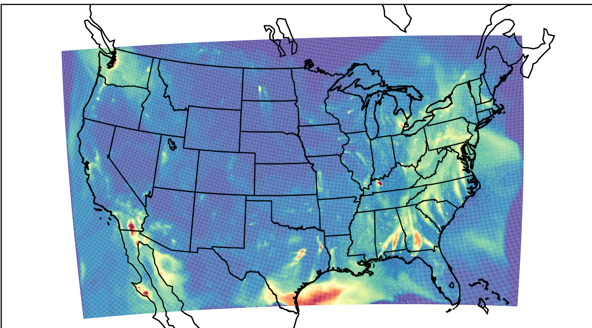
WRF 2023-04-22_06:00:00
