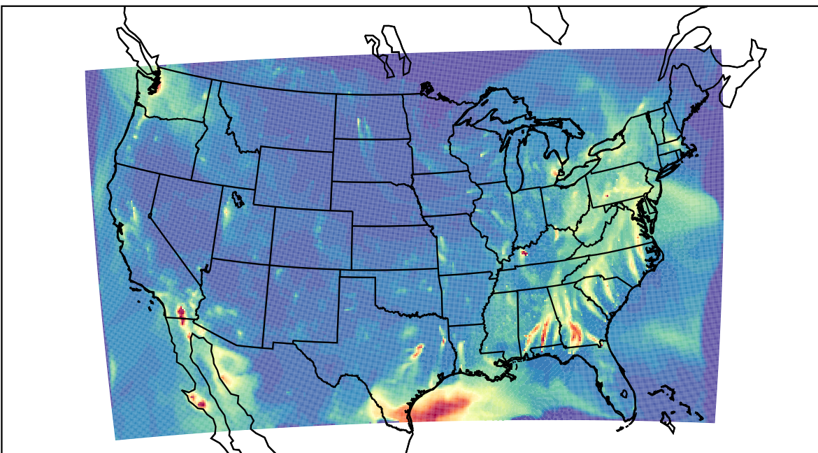
WRF 2023-04-22_05:00:00
