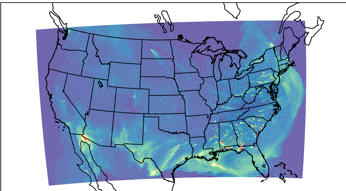
WRF 2023-04-23_21:00:00
