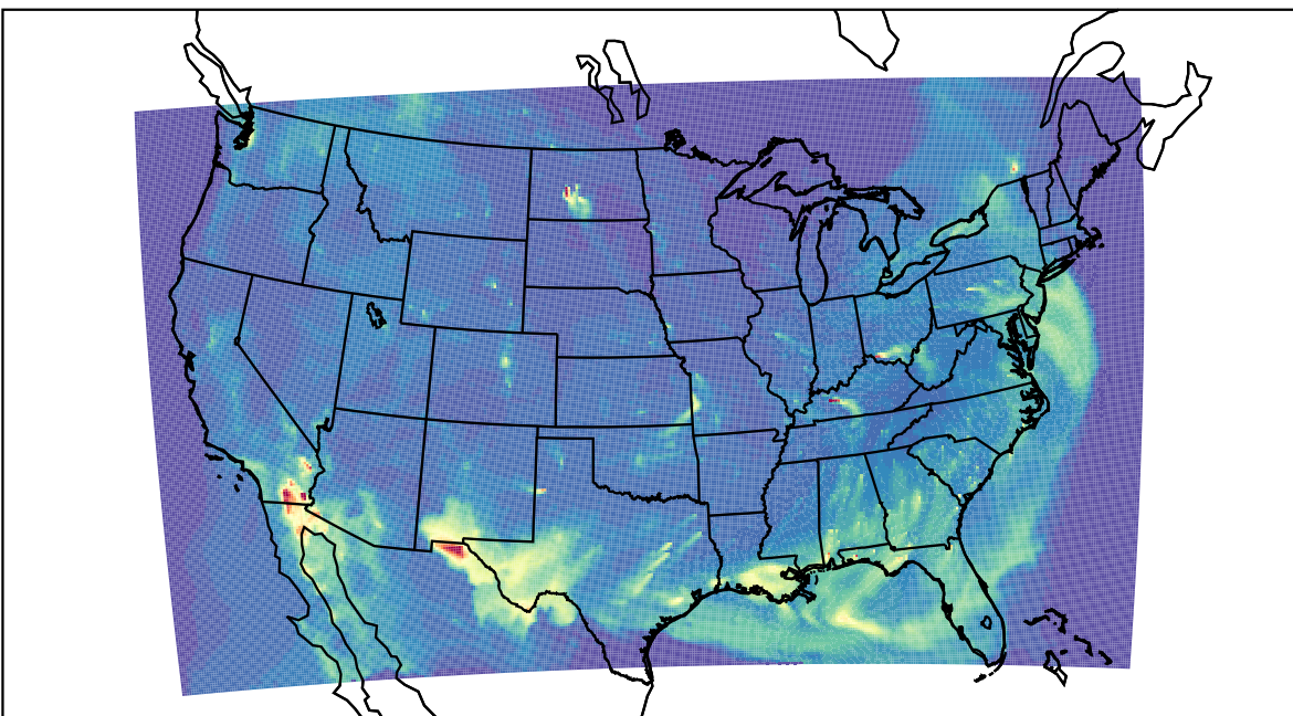
WRF 2023-04-23_13:00:00
