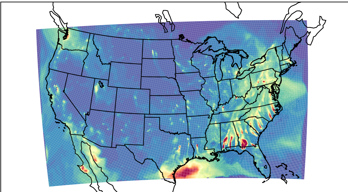
WRF 2023-04-22_03:00:00
