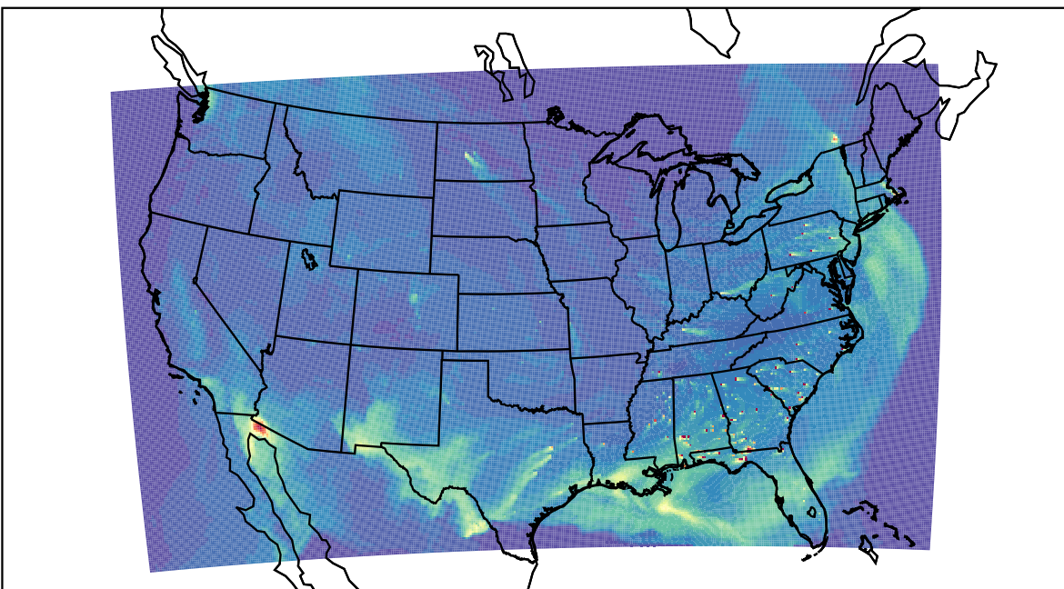
WRF 2023-04-23_19:00:00
