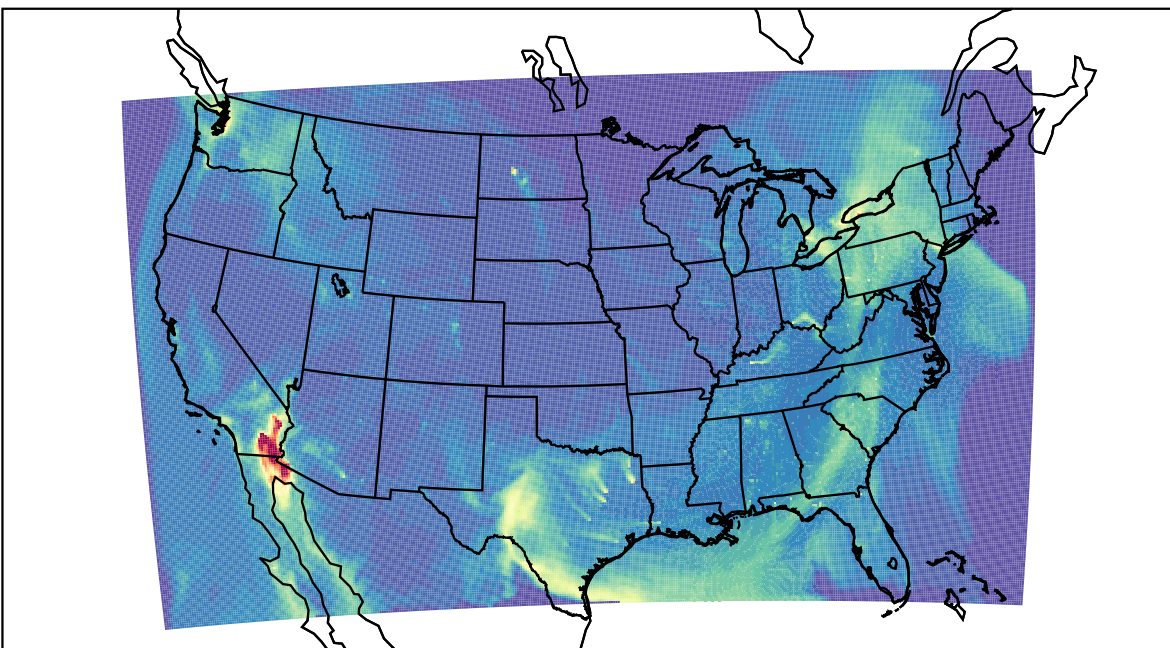
WRF 2023-04-22_16:00:00
