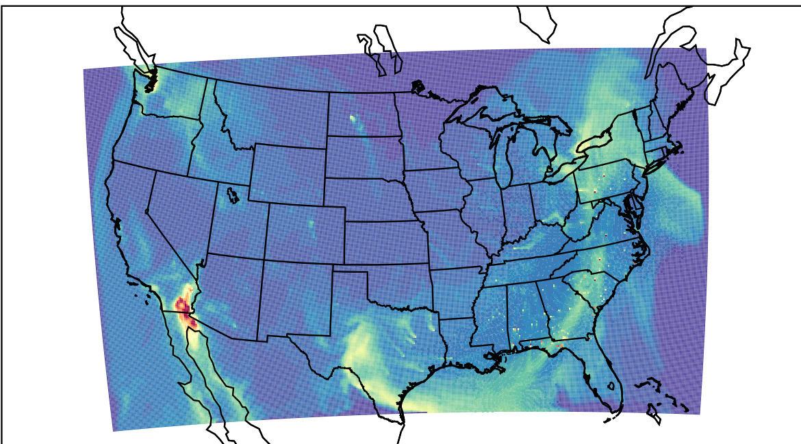
WRF 2023-04-22_17:00:00
