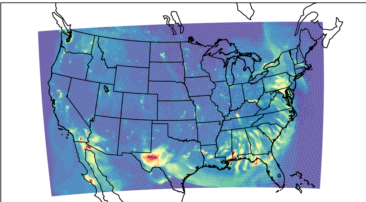
WRF 2023-04-23_04:00:00
