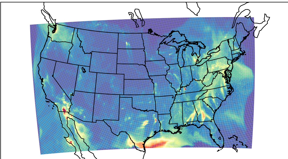
WRF 2023-04-22_07:00:00
