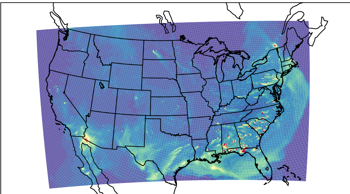
WRF 2023-04-23_23:00:00
