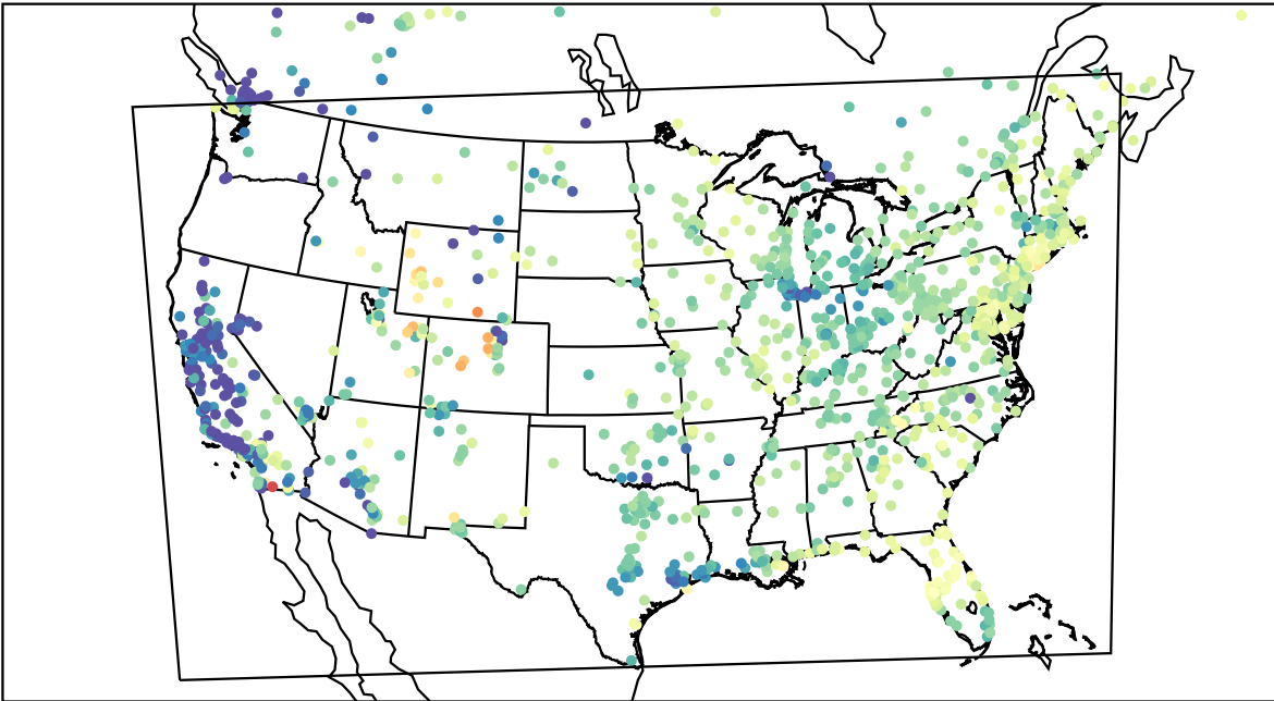
AirNOW (2023-04-23_14:00:00)
