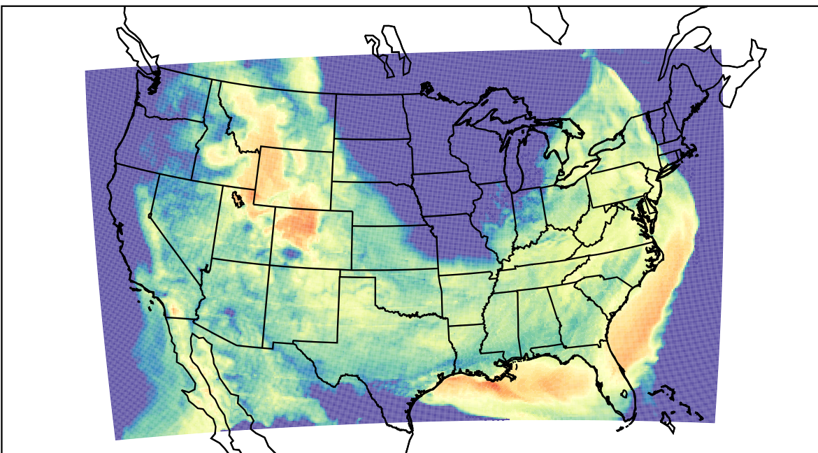
WRF (2023-04-23_14:00:00)
