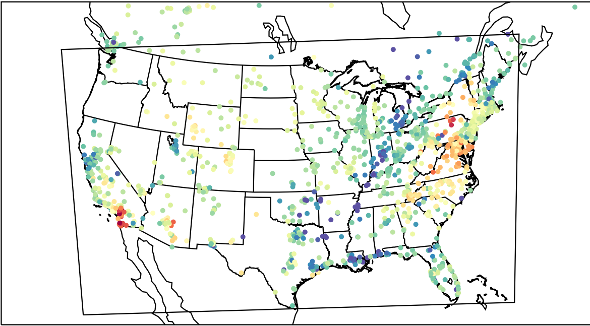
AirNOW (2023-04-22_02:00:00)
