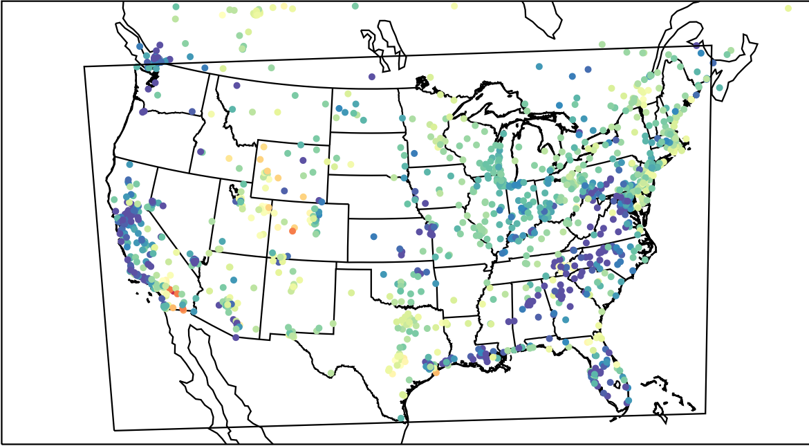
AirNOW (2023-04-23_05:00:00)
