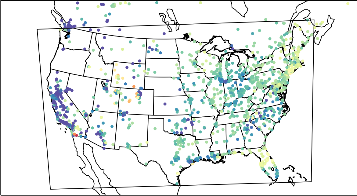
AirNOW (2023-04-23_13:00:00)
