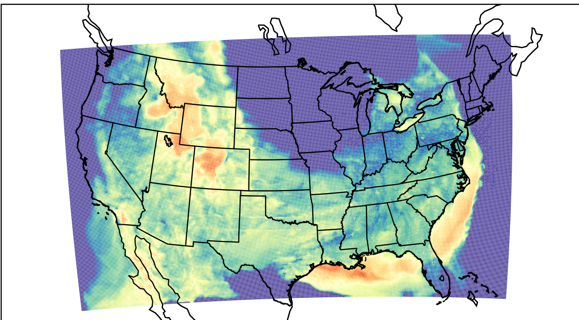
WRF (2023-04-23_09:00:00)
