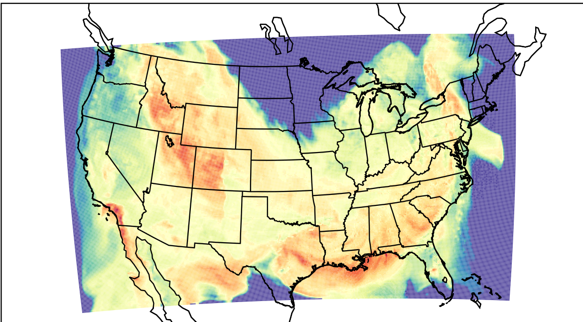
WRF (2023-04-22_22:00:00)
