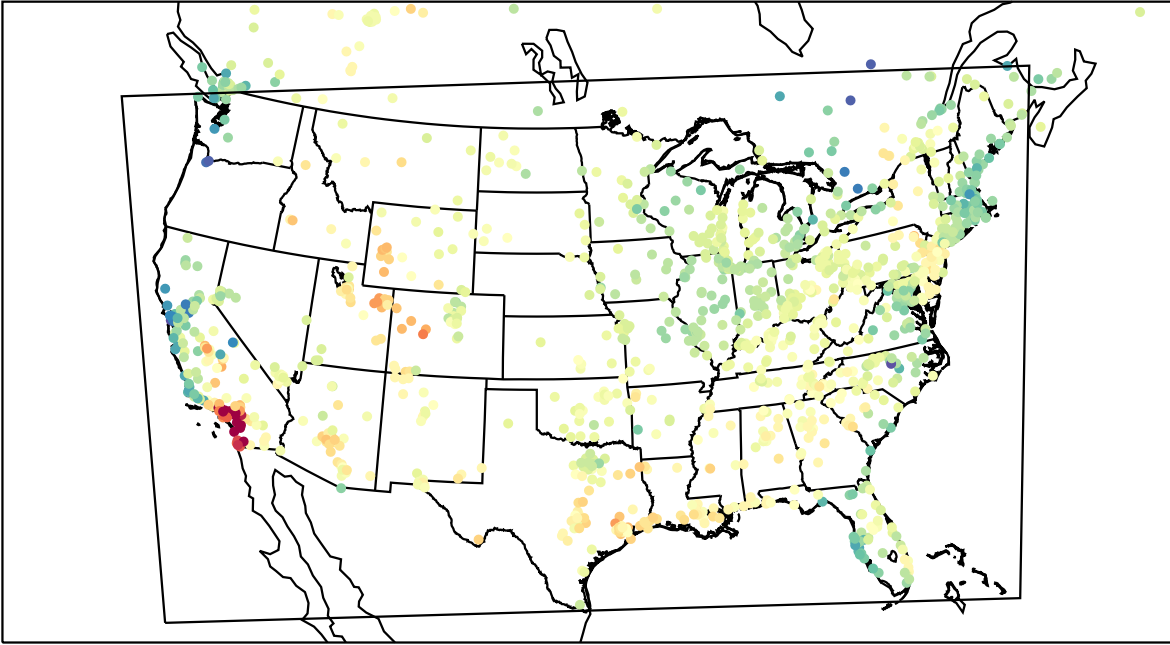
AirNOW (2023-04-22_21:00:00)
