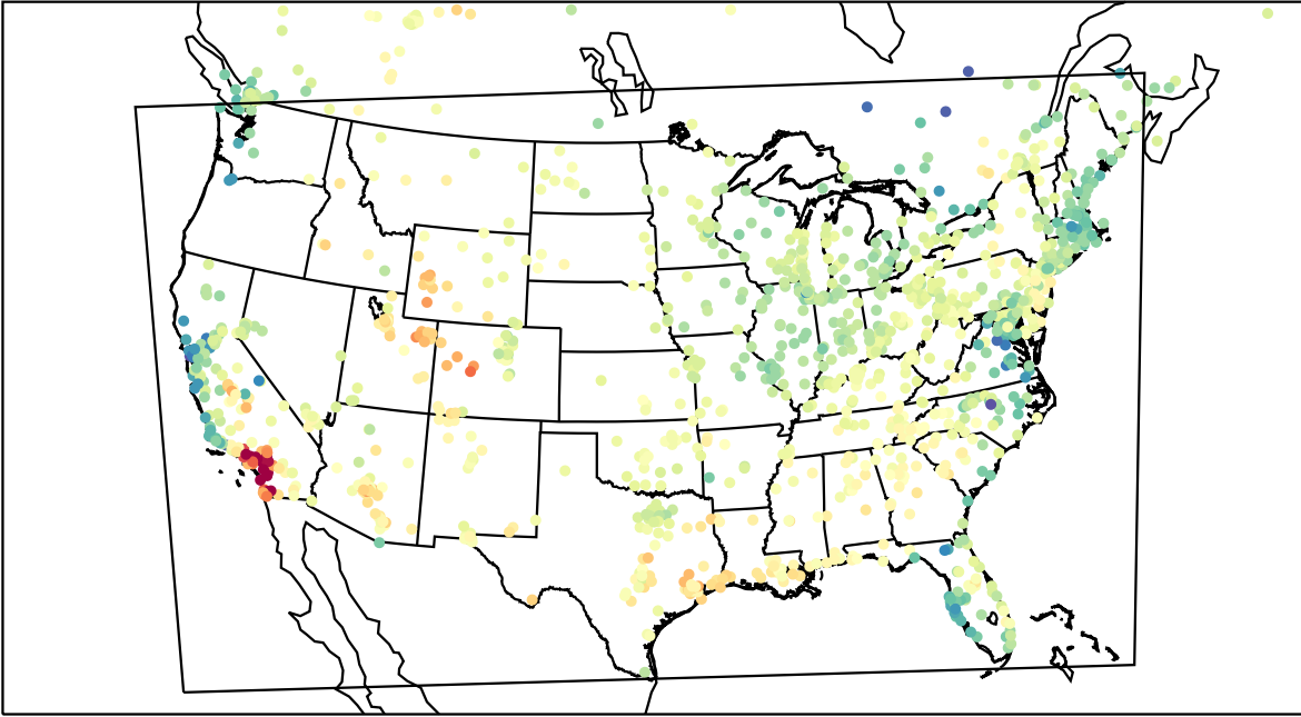
AirNOW (2023-04-22_22:00:00)
