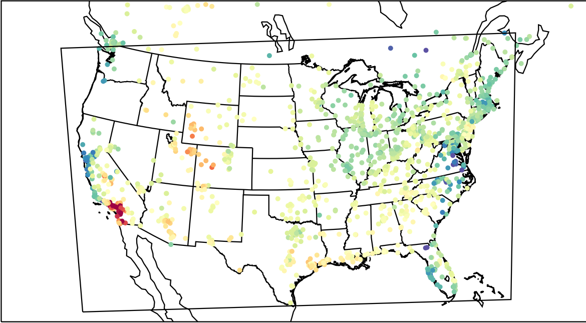
AirNOW (2023-04-22_23:00:00)
