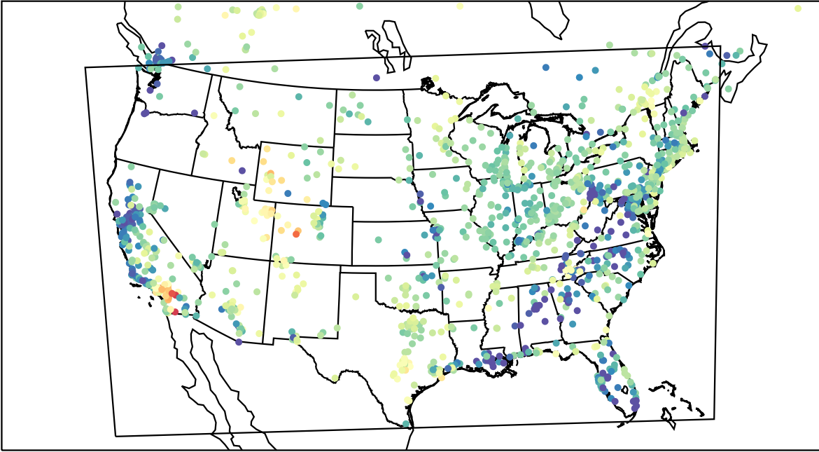
AirNOW (2023-04-23_03:00:00)
