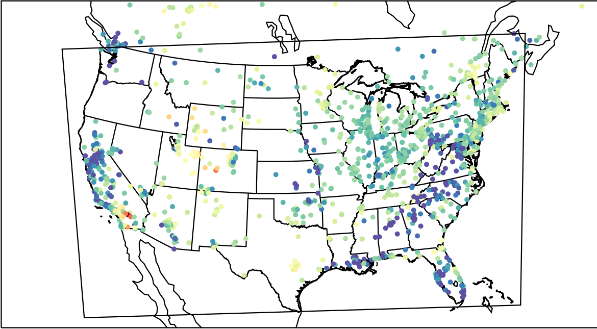
AirNOW (2023-04-23_04:00:00)
