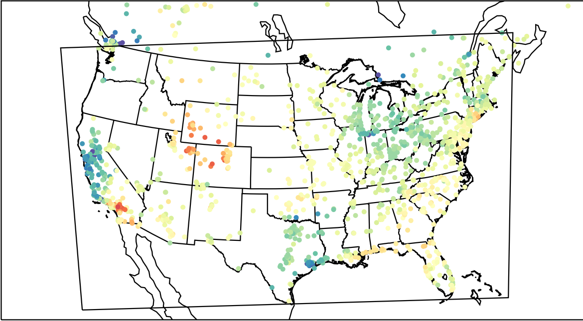
AirNOW (2023-04-23_18:00:00)
