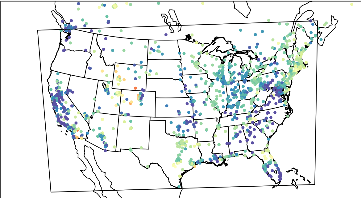
AirNOW (2023-04-23_08:00:00)
