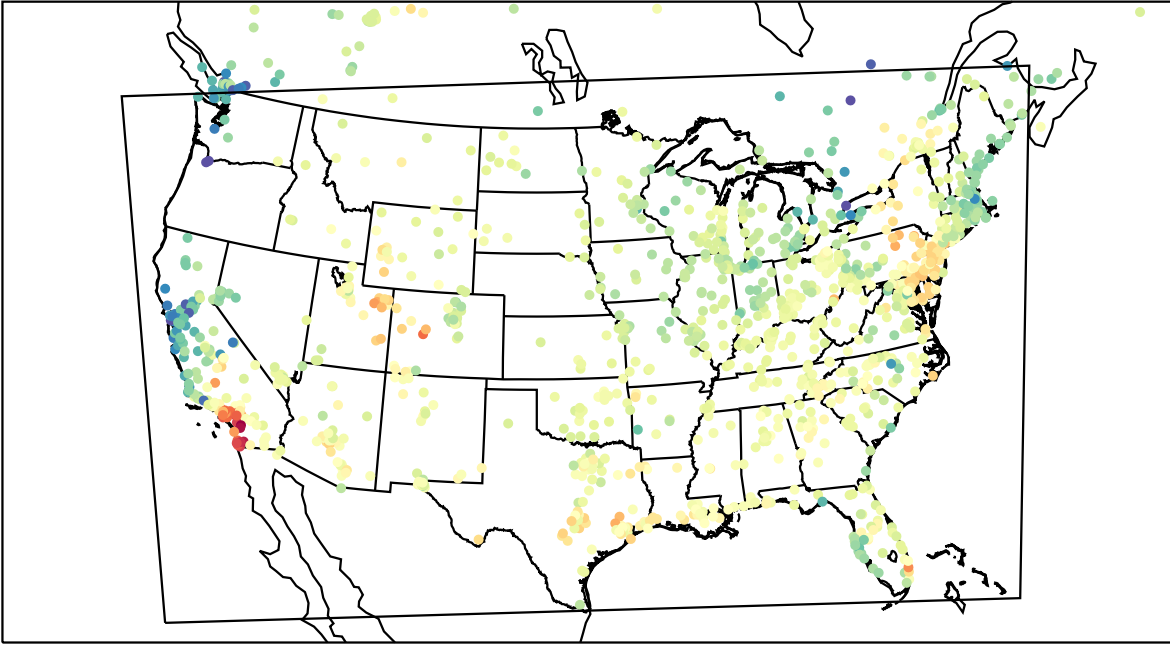
AirNOW (2023-04-22_18:00:00)
