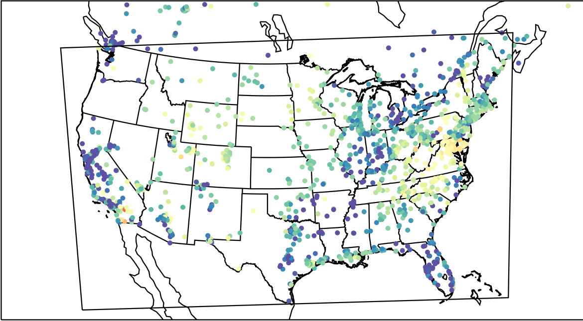
AirNOW (2023-04-22_09:00:00)
