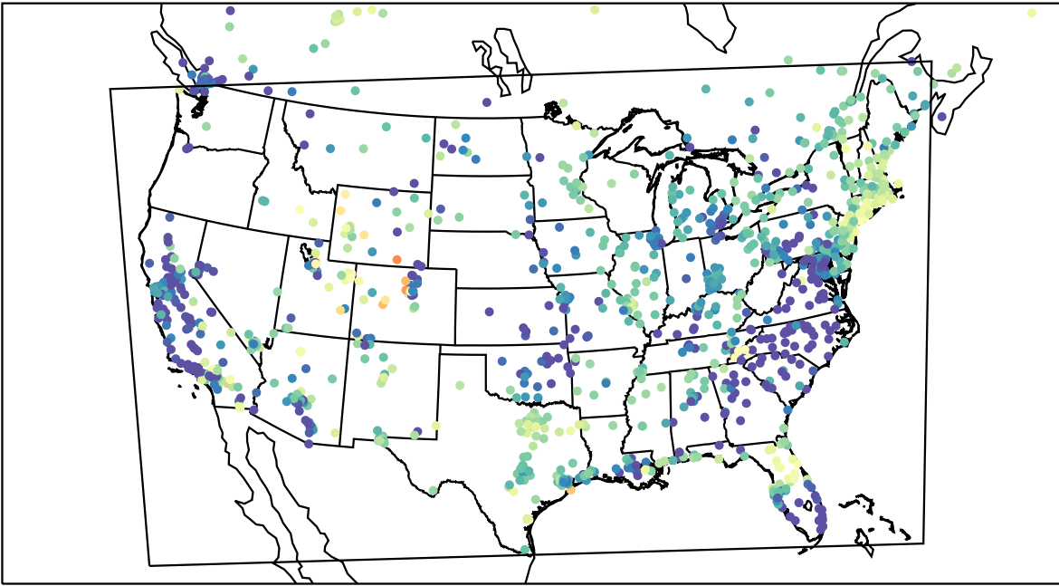
AirNOW (2023-04-23_10:00:00)
