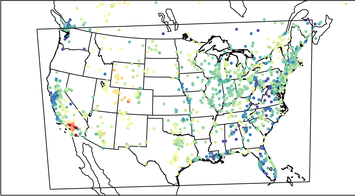
AirNOW (2023-04-23_02:00:00)
