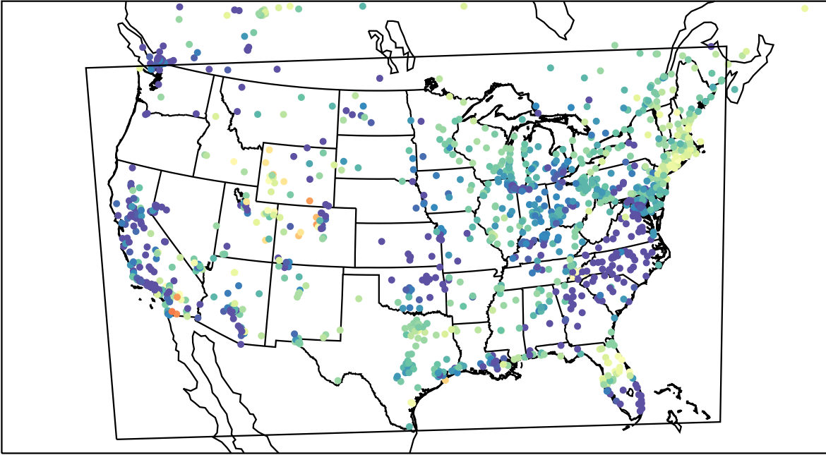
AirNOW (2023-04-23_11:00:00)
