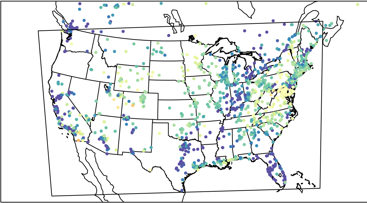
AirNOW (2023-04-22_11:00:00)
