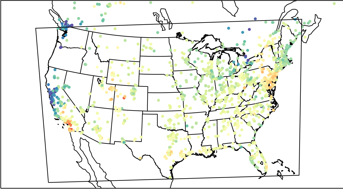
AirNOW (2023-04-22_17:00:00)
