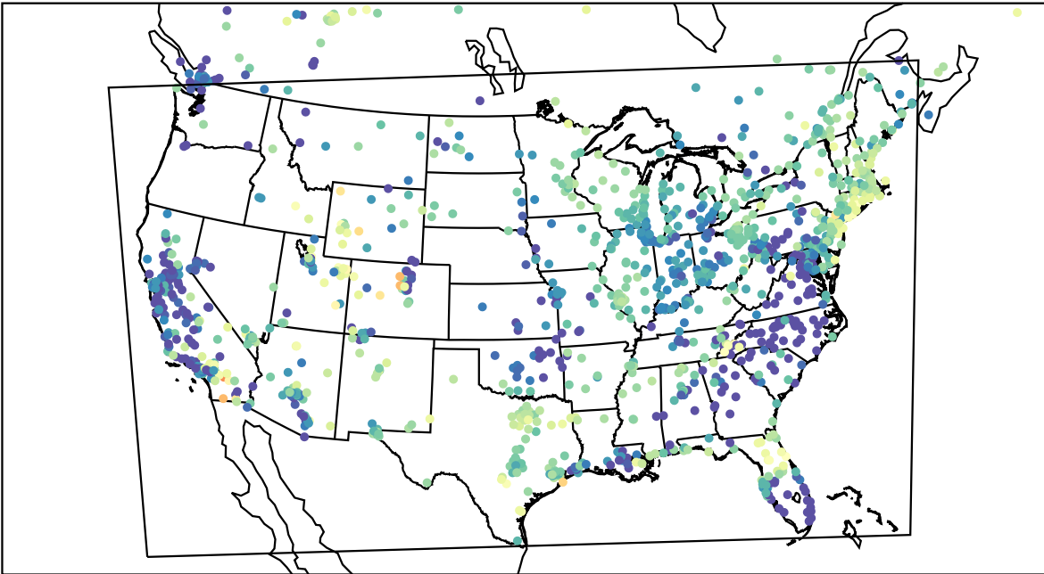
AirNOW (2023-04-23_09:00:00)
