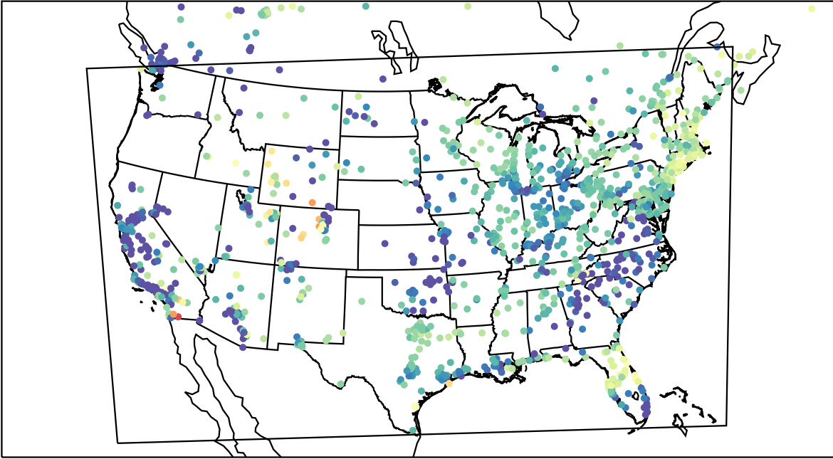
AirNOW (2023-04-23_12:00:00)
