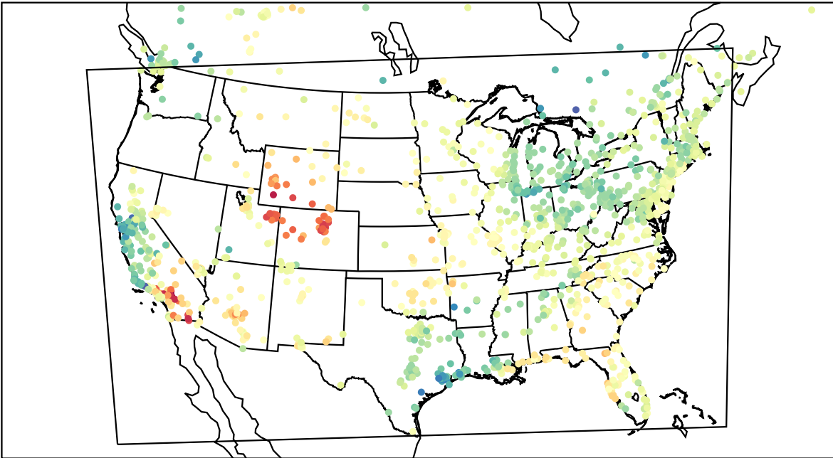
AirNOW (2023-04-23_22:00:00)
