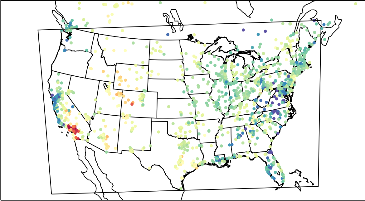
AirNOW (2023-04-23_01:00:00)
