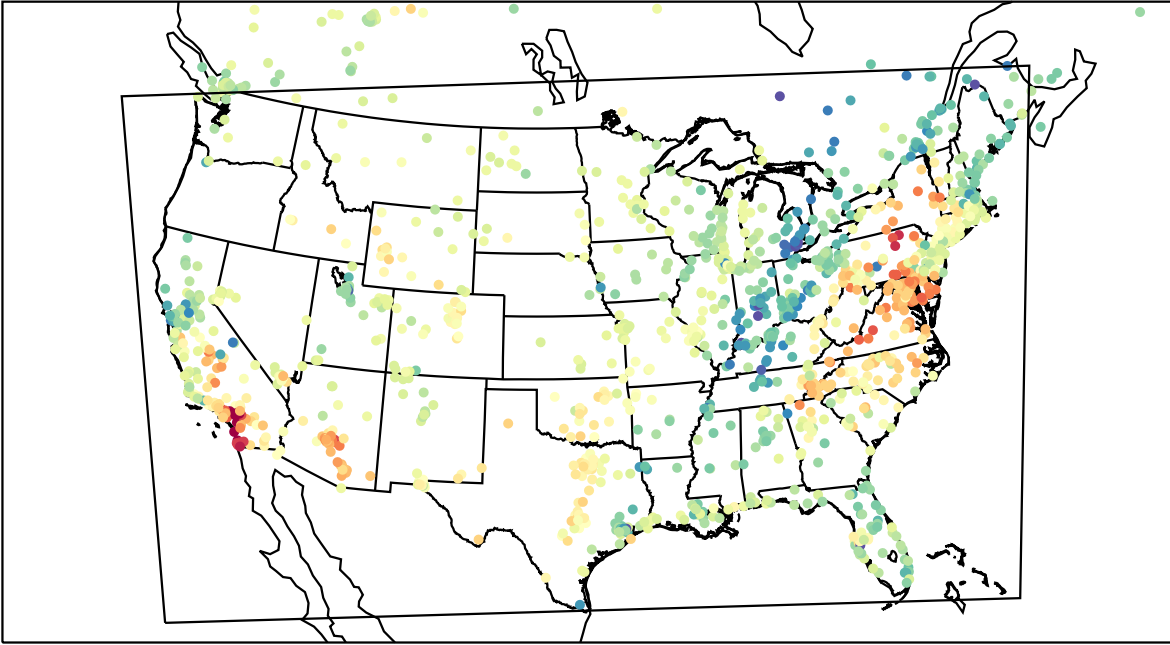
AirNOW (2023-04-22_00:00:00)
