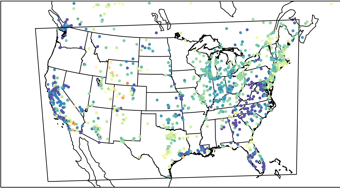
AirNOW (2023-04-23_06:00:00)
