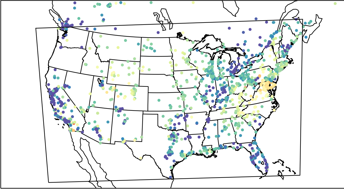
AirNOW (2023-04-22_08:00:00)
