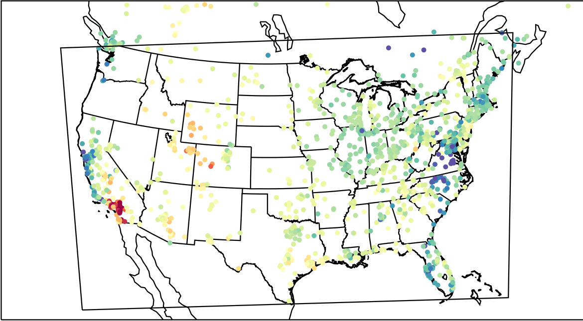
AirNOW (2023-04-23_00:00:00)
