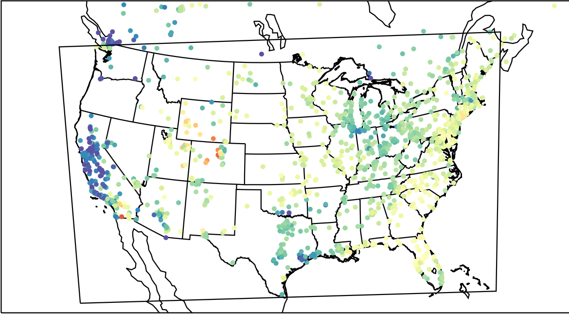
AirNOW (2023-04-23_15:00:00)
