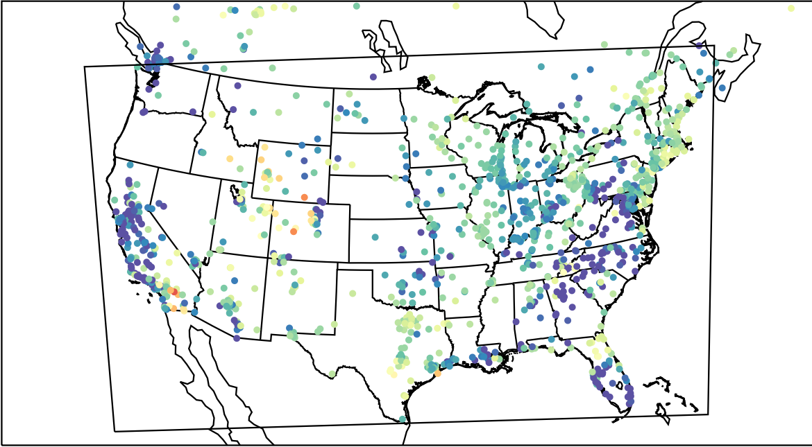
AirNOW (2023-04-23_07:00:00)
