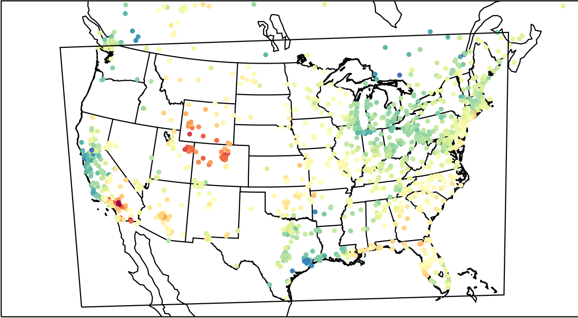
AirNOW (2023-04-23_21:00:00)
