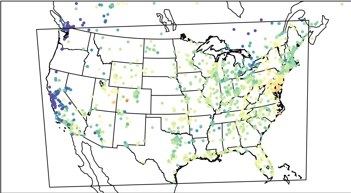
AirNOW (2023-04-22_15:00:00)
