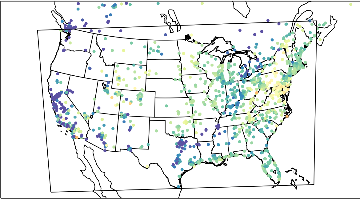
AirNOW (2023-04-22_13:00:00)
