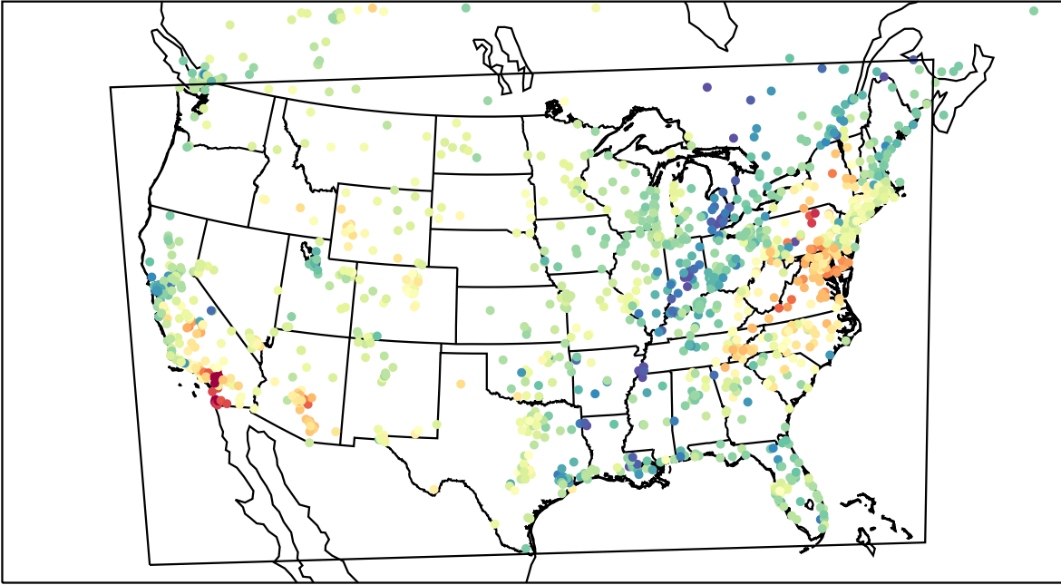
AirNOW (2023-04-22_01:00:00)
