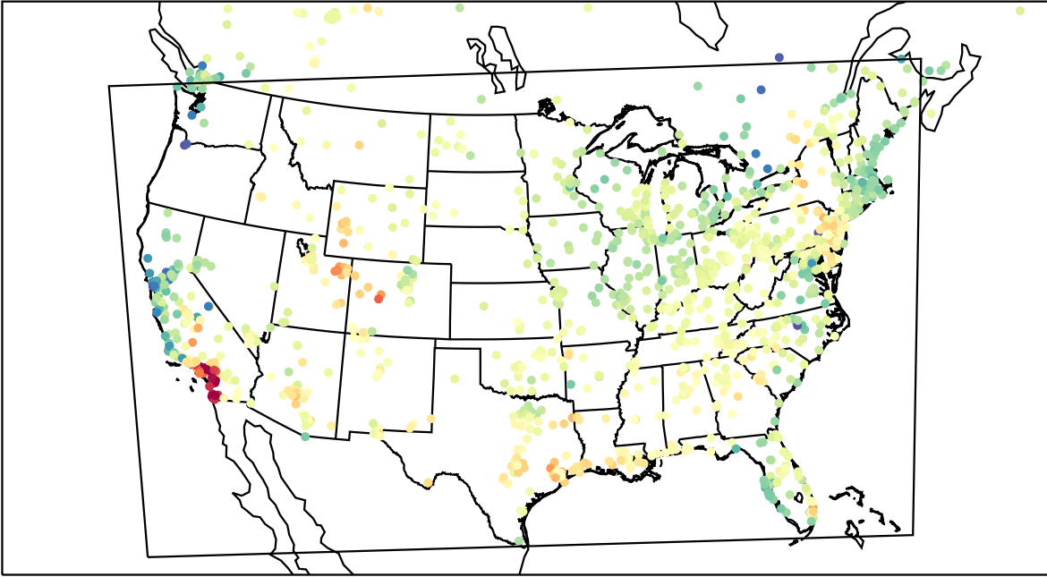
AirNOW (2023-04-22_20:00:00)
