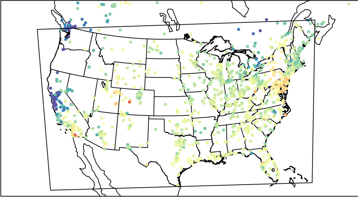
AirNOW (2023-04-22_16:00:00)
