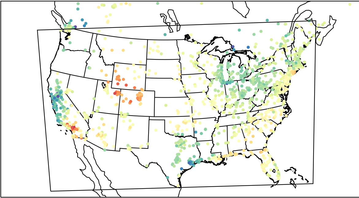
AirNOW (2023-04-23_19:00:00)
