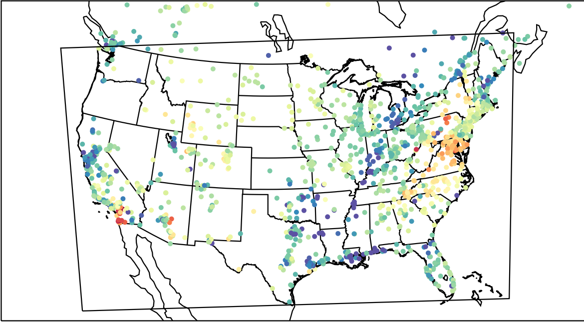
AirNOW (2023-04-22_03:00:00)
