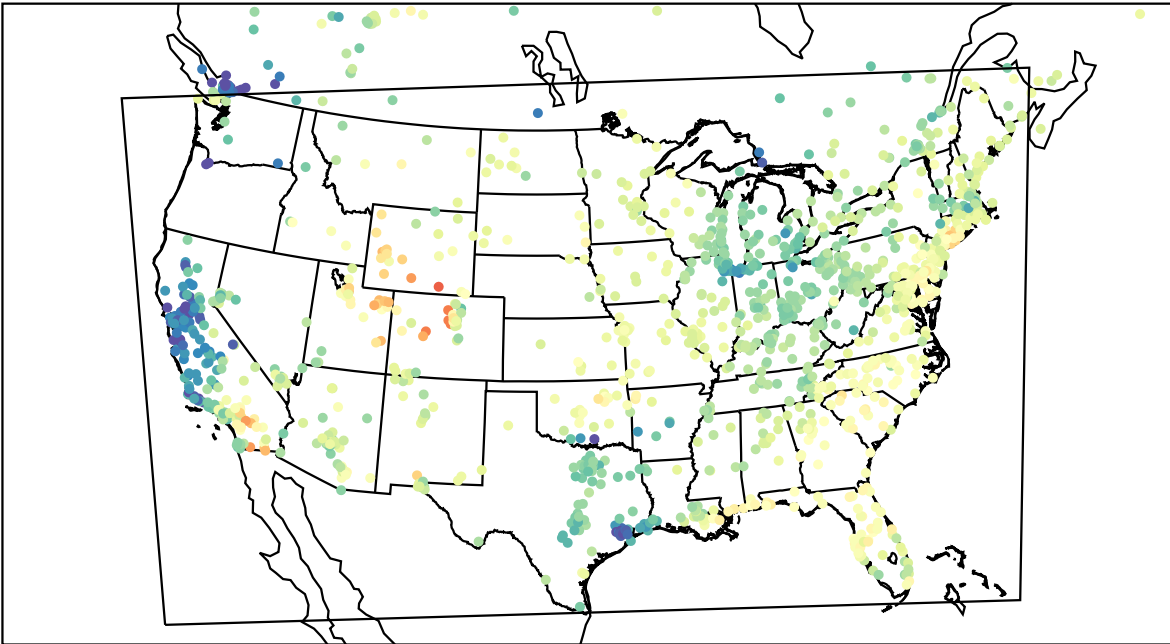
AirNOW (2023-04-23_16:00:00)
