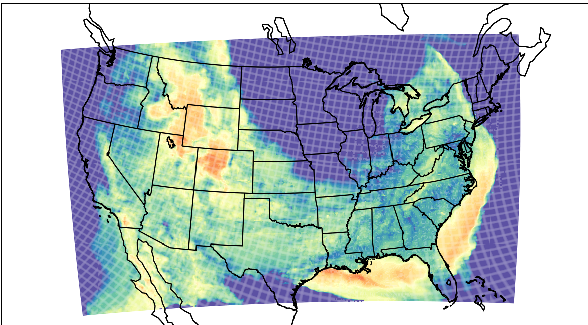
WRF (2023-04-23_12:00:00)
