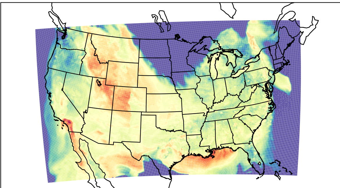
WRF (2023-04-23_00:00:00)
