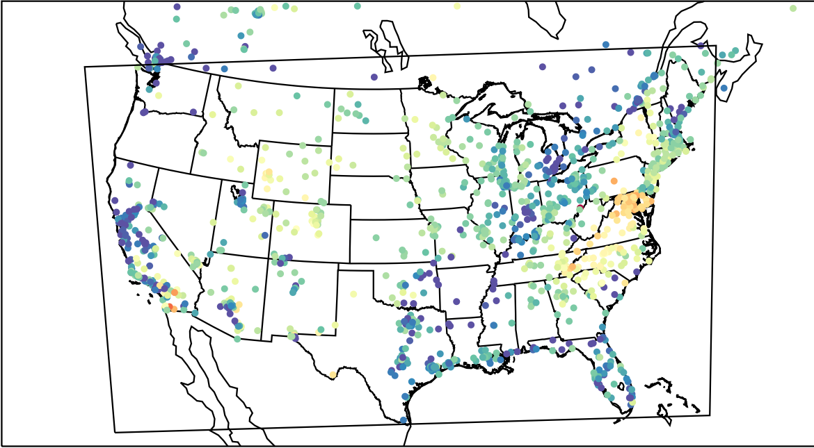
AirNOW (2023-04-22_06:00:00)
