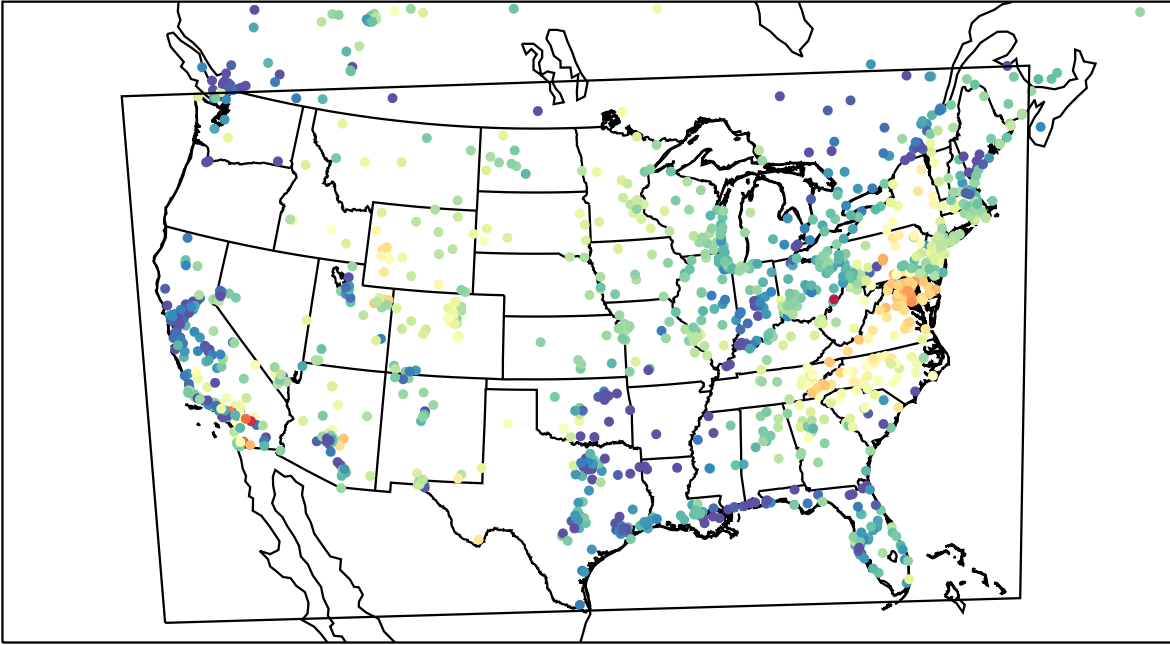
AirNOW (2023-04-22_05:00:00)
