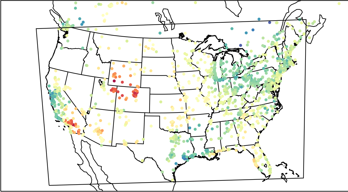
AirNOW (2023-04-23_23:00:00)
