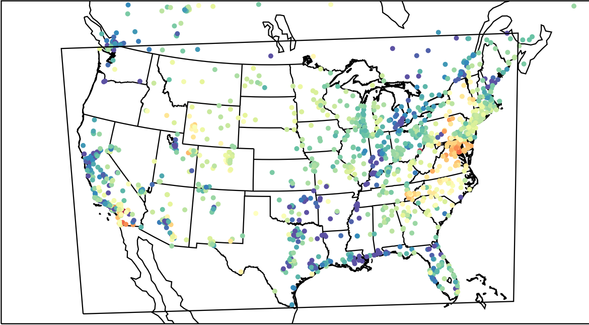
AirNOW (2023-04-22_04:00:00)
