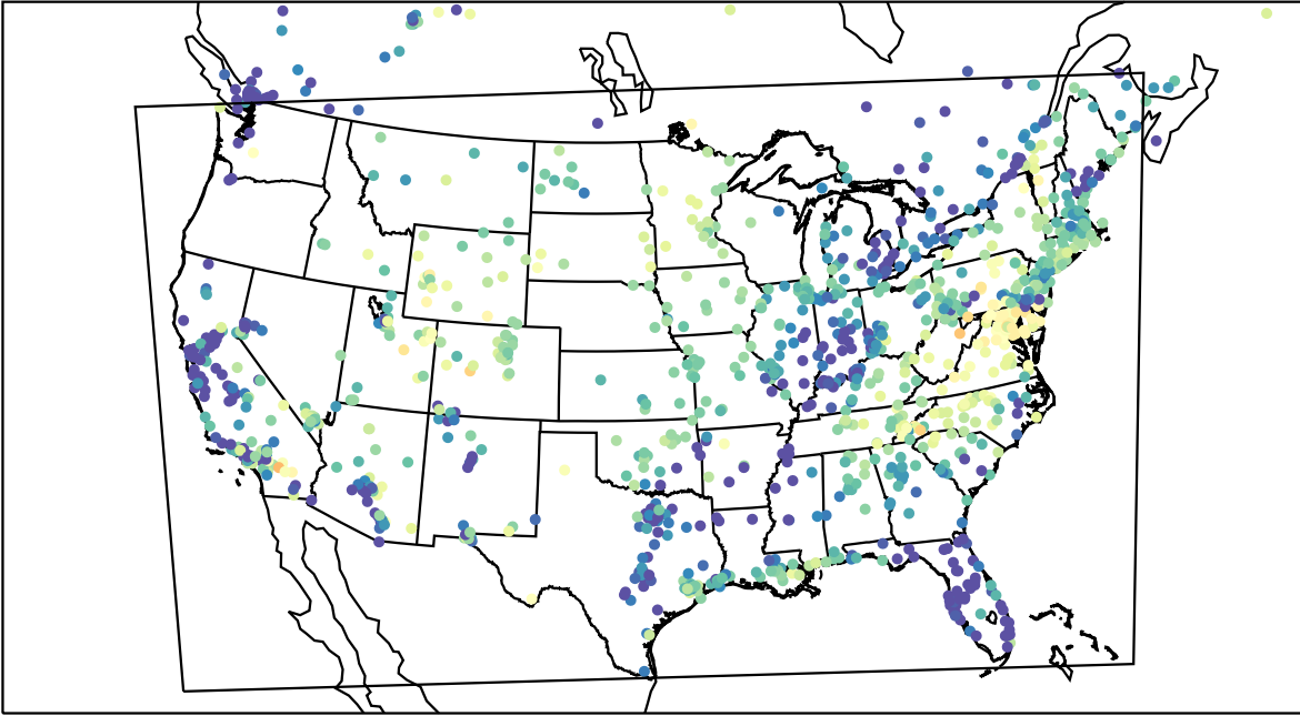
AirNOW (2023-04-22_10:00:00)
