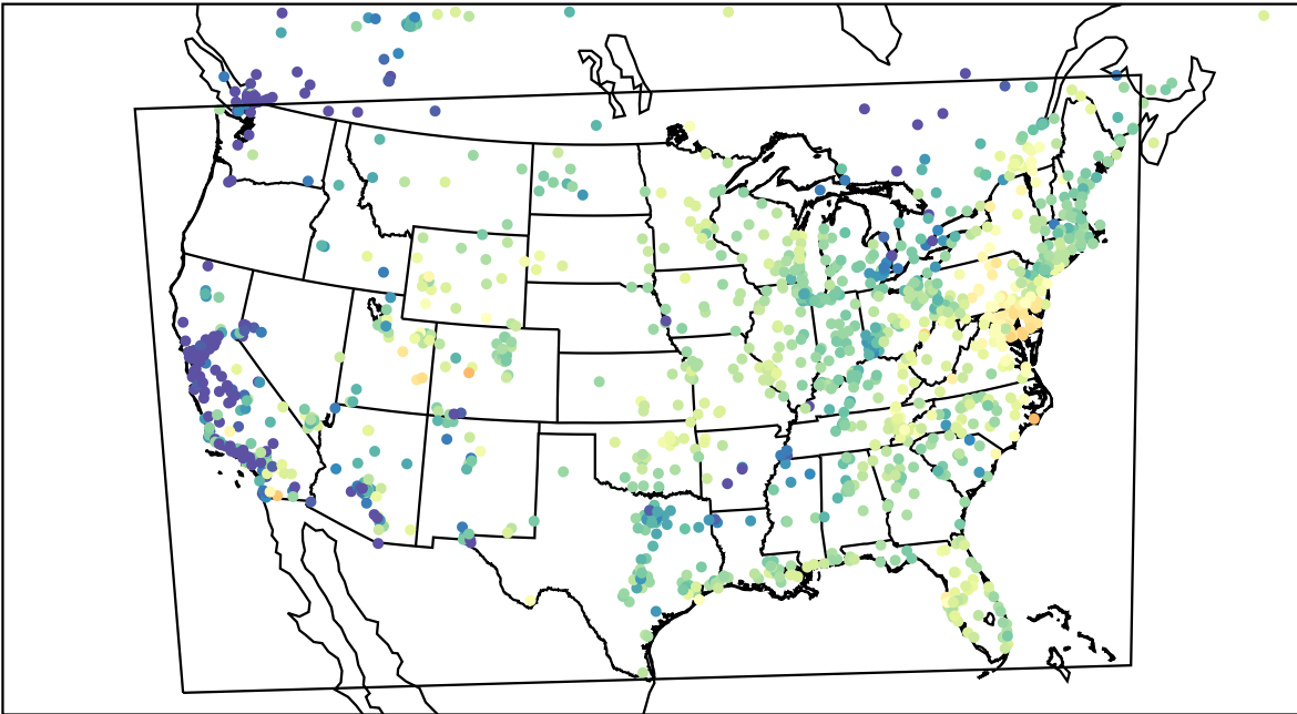
AirNOW (2023-04-22_14:00:00)
