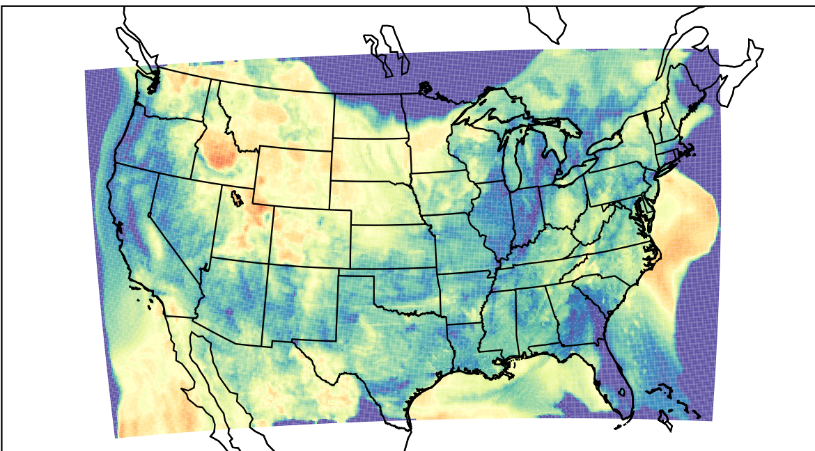
WRF (2023-04-22_12:00:00)
