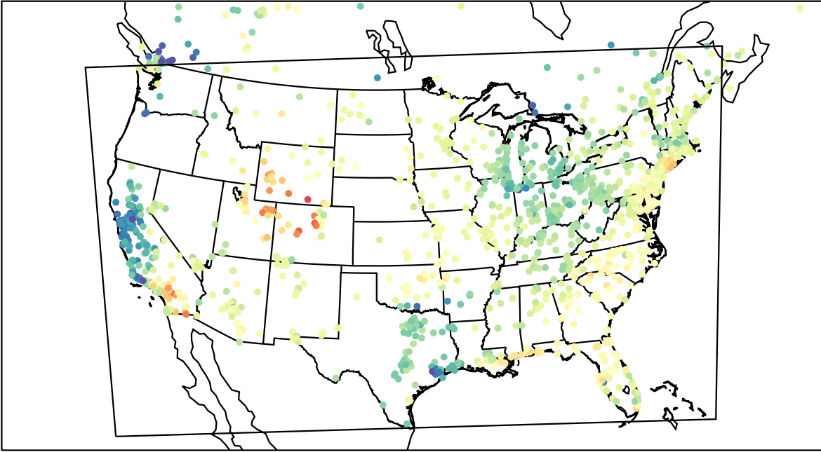
AirNOW (2023-04-23_17:00:00)
