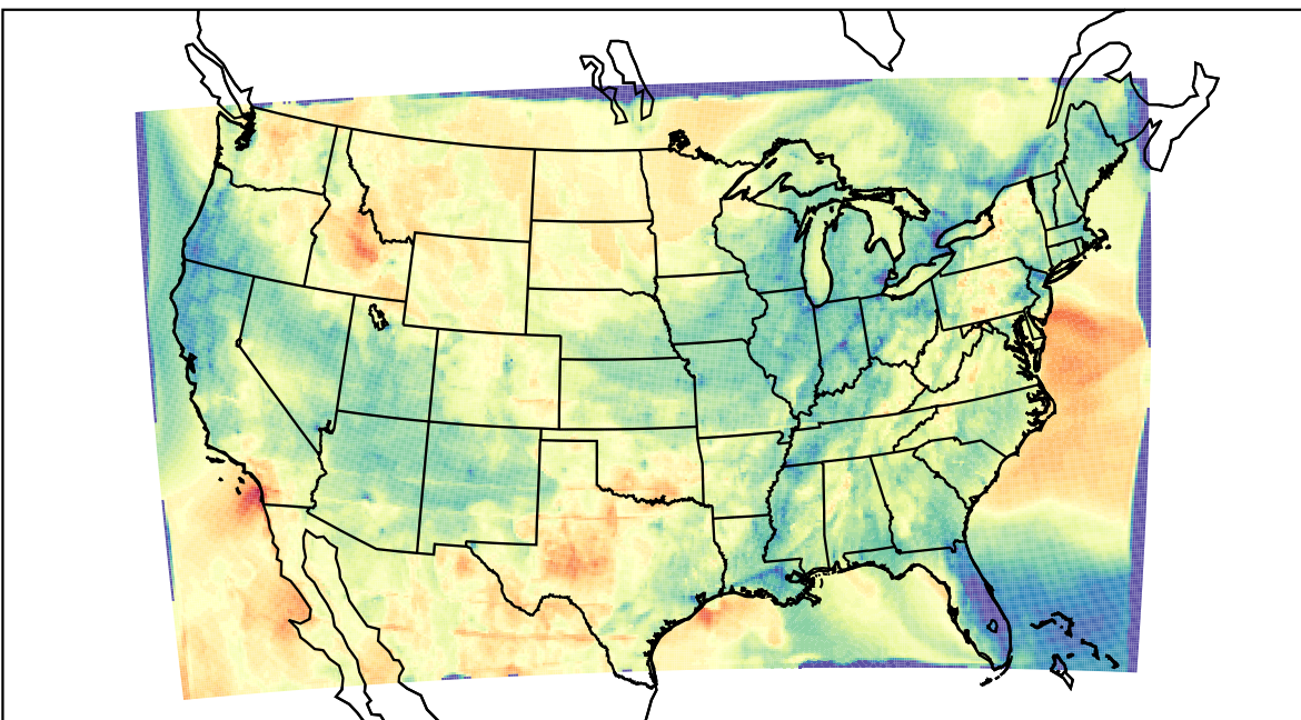
WRF (2023-04-22_02:00:00)
