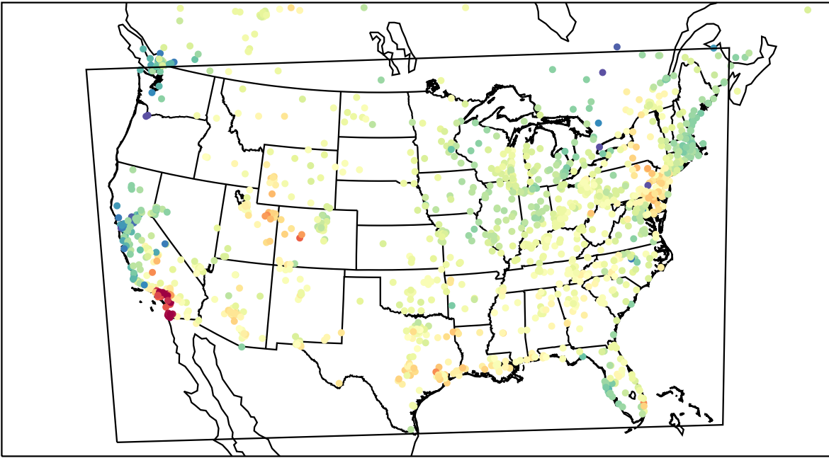
AirNOW (2023-04-22_19:00:00)
