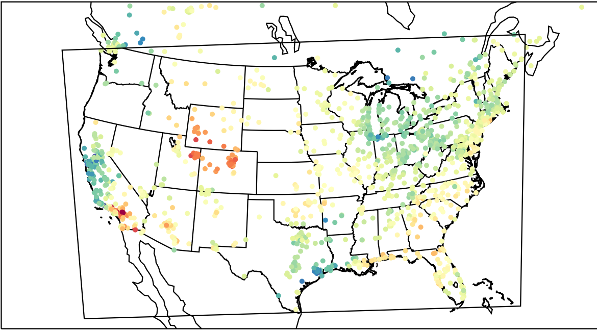
AirNOW (2023-04-23_20:00:00)
