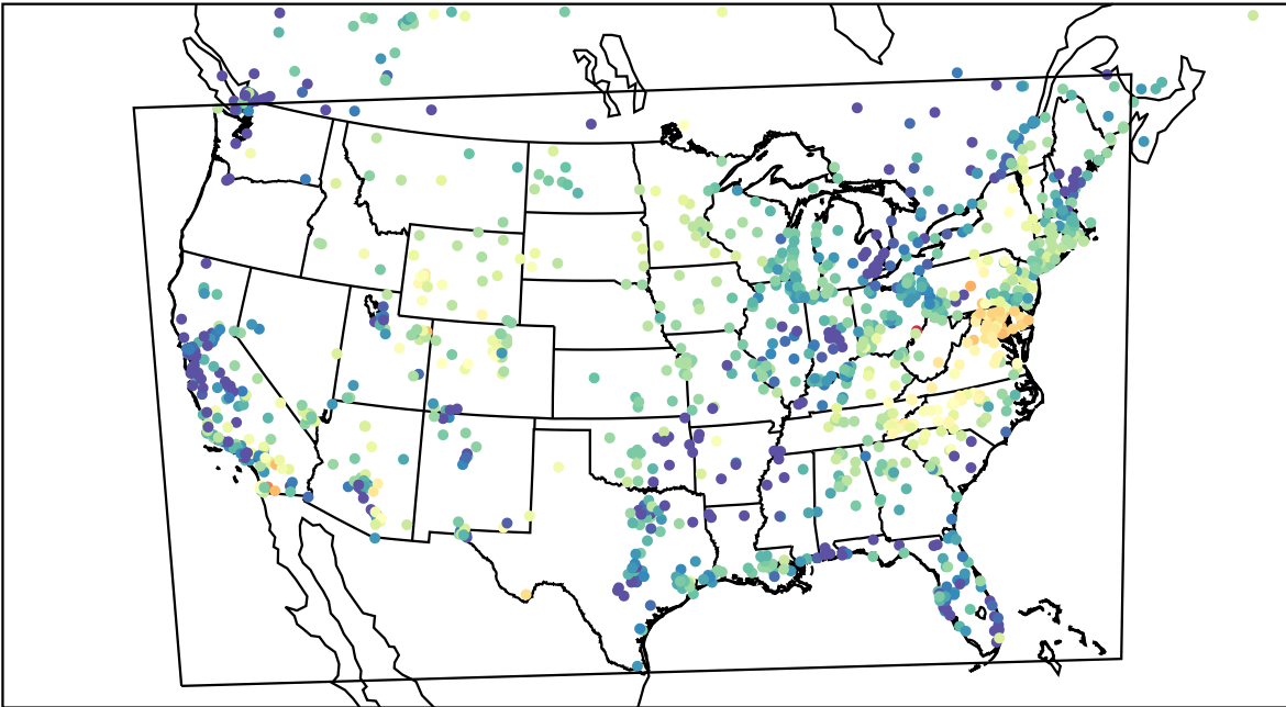
AirNOW (2023-04-22_07:00:00)
