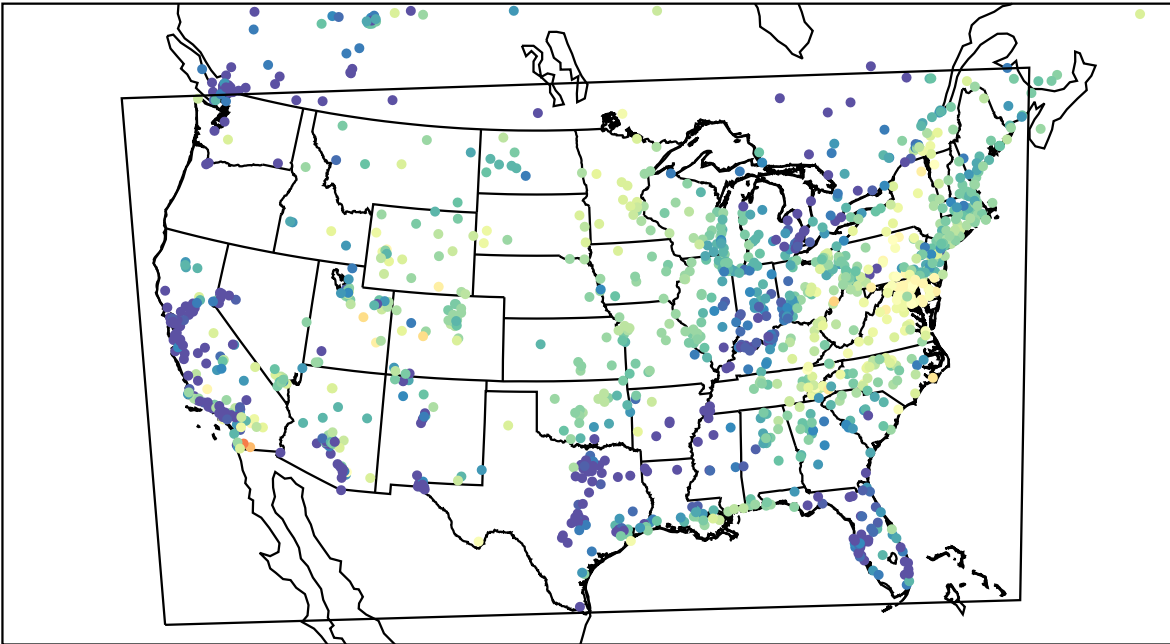
AirNOW (2023-04-22_12:00:00)
