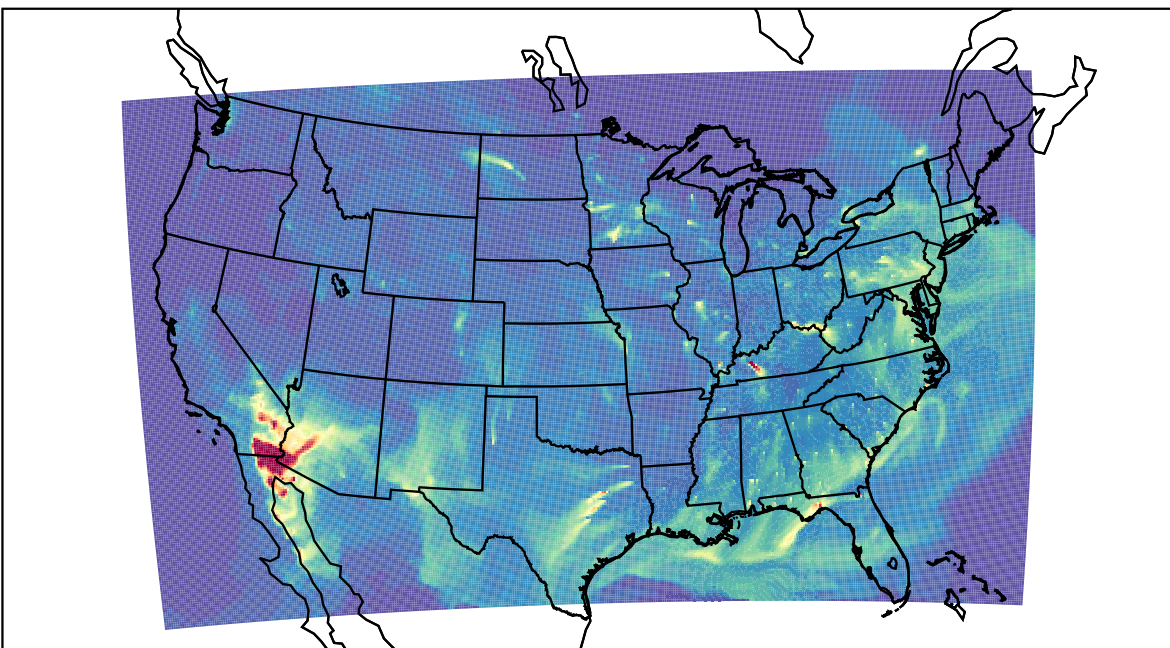
WRF 2023-04-24_10:00:00
