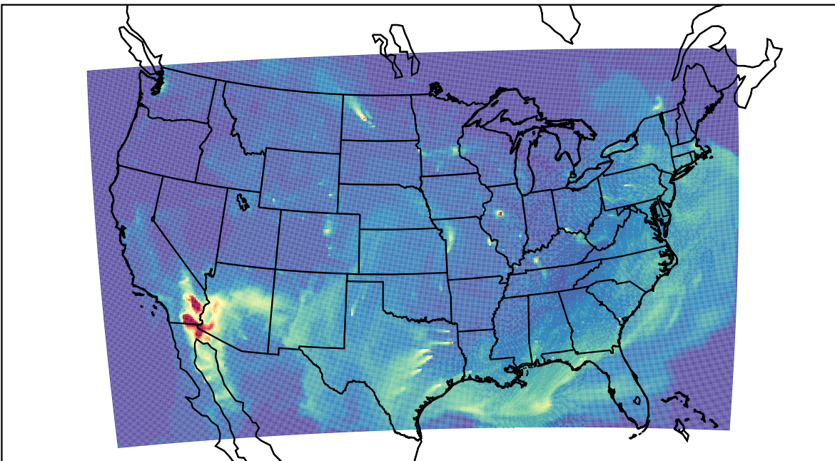
WRF 2023-04-24_15:00:00
