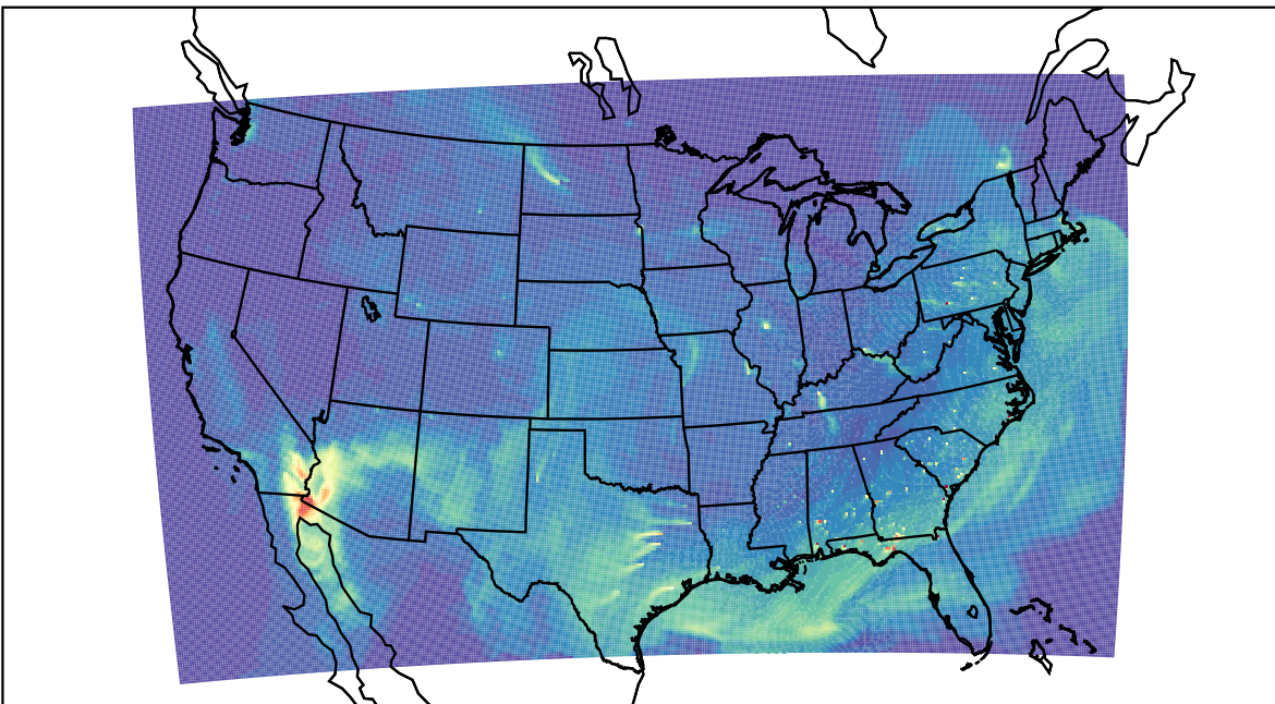
WRF 2023-04-24_17:00:00
