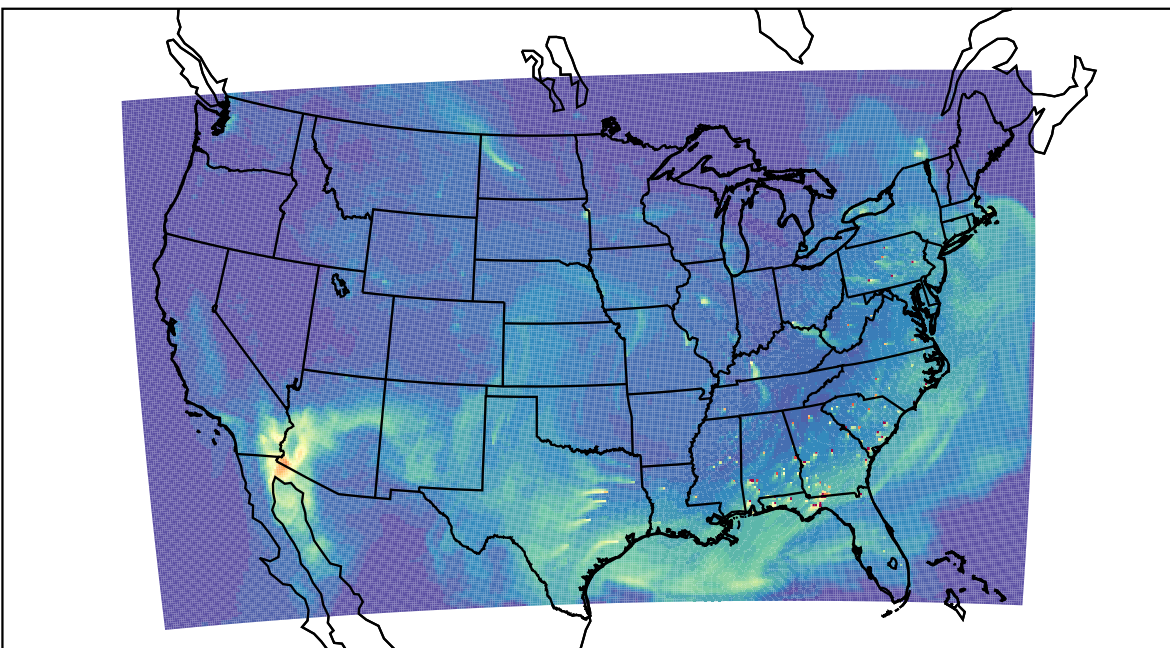
WRF 2023-04-24_18:00:00
