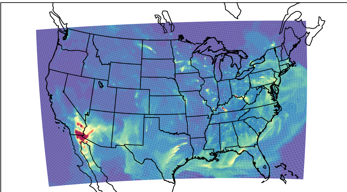
WRF 2023-04-24_11:00:00
