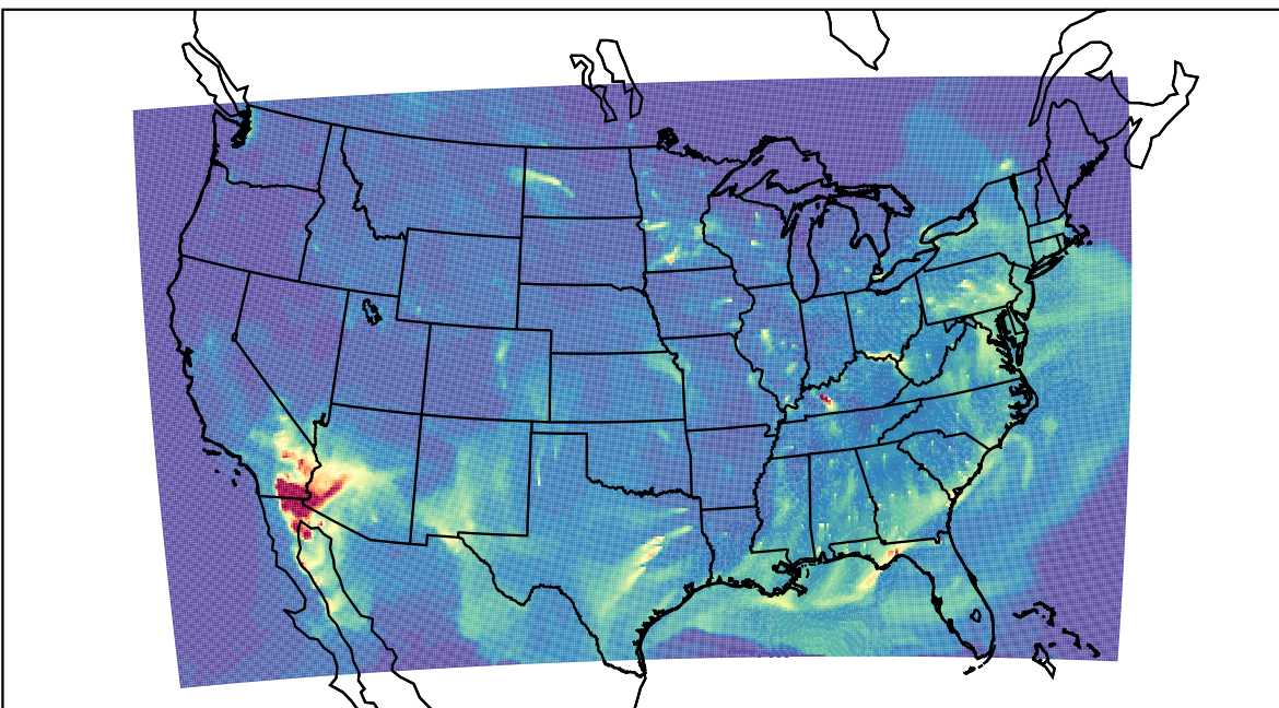
WRF 2023-04-24_09:00:00
