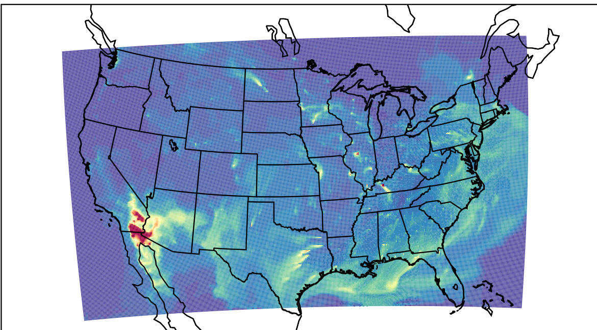
WRF 2023-04-24_13:00:00
