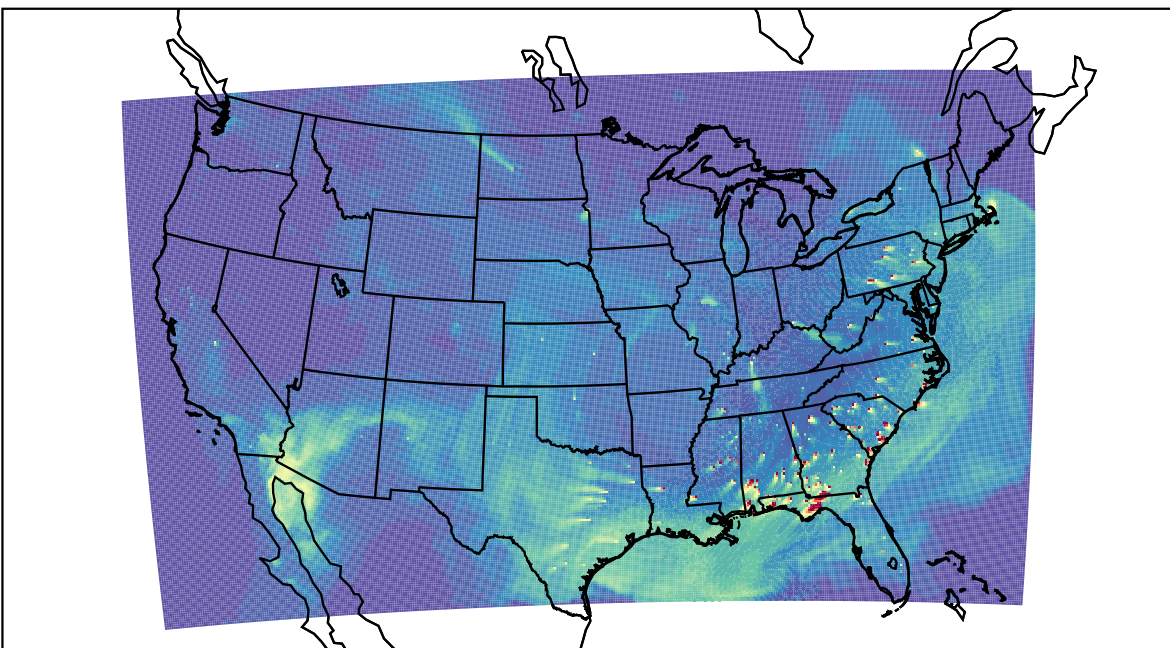
WRF 2023-04-24_21:00:00
