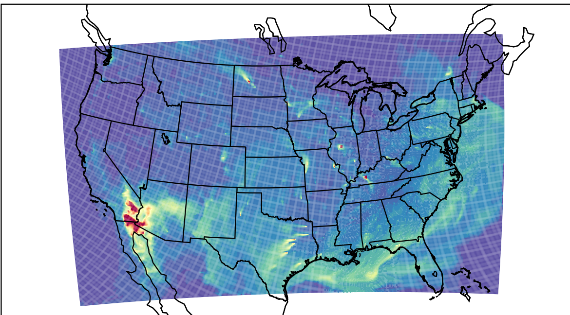
WRF 2023-04-24_14:00:00
