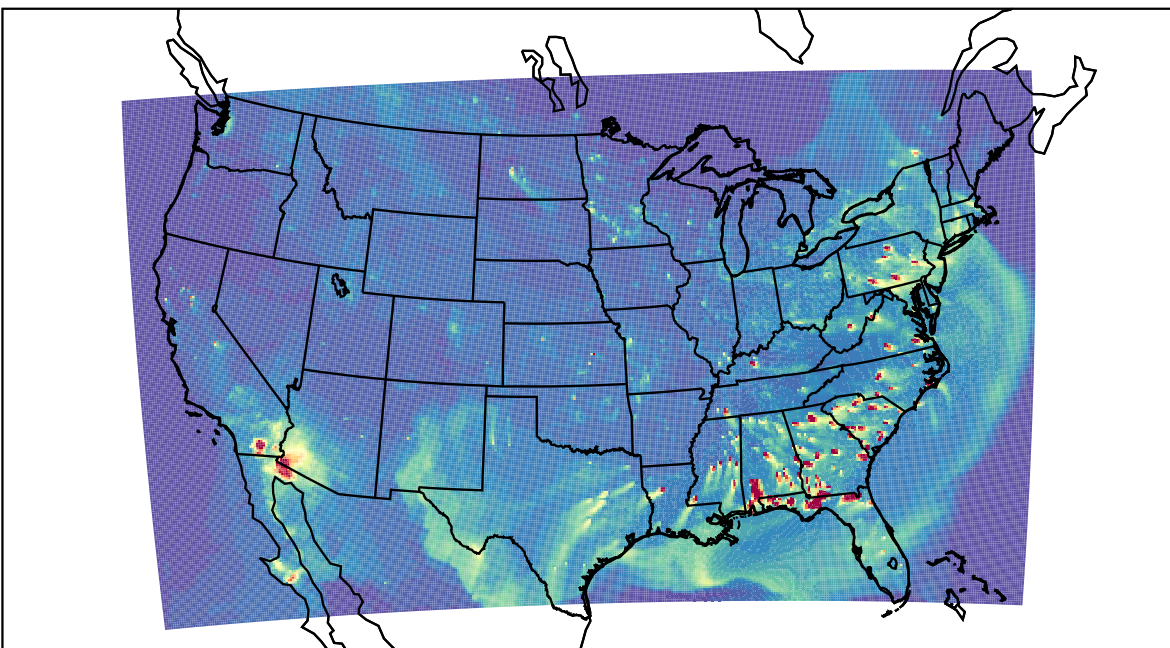
WRF 2023-04-24_01:00:00
