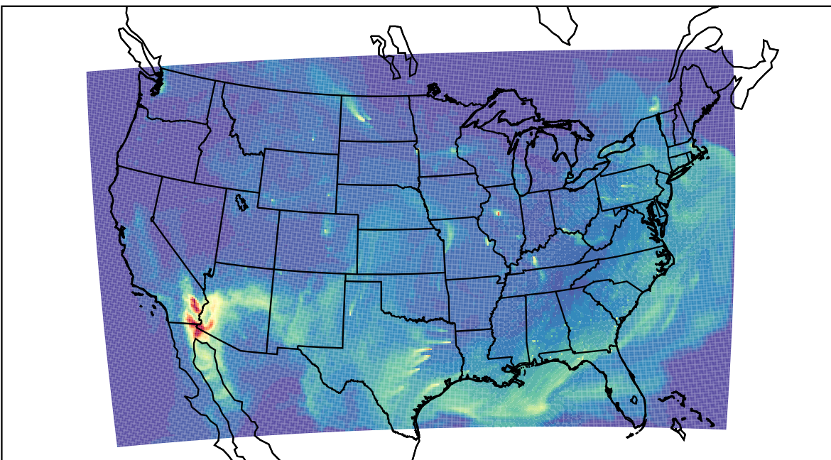
WRF 2023-04-24_16:00:00
