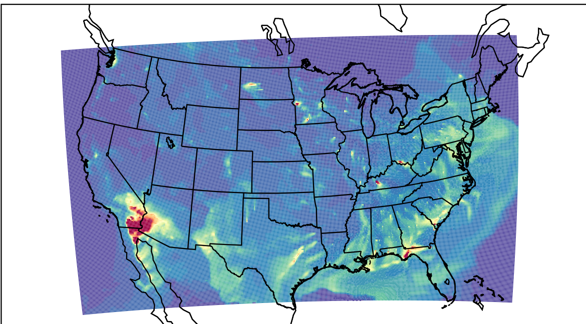
WRF 2023-04-24_06:00:00
