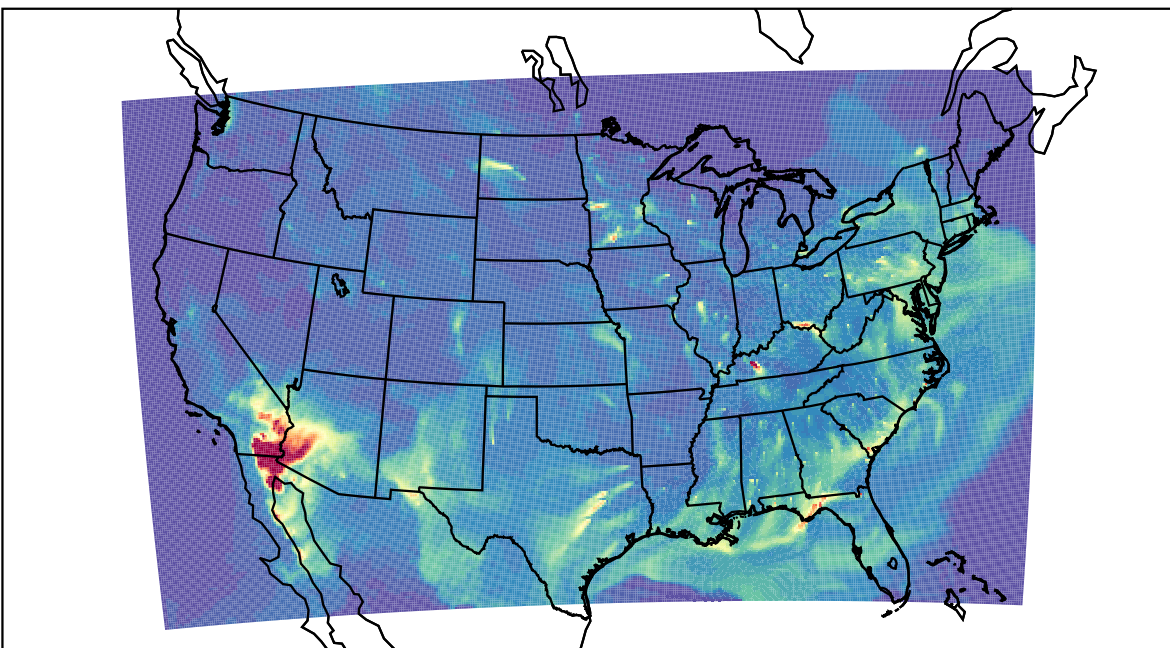
WRF 2023-04-24_08:00:00
