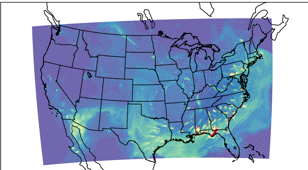
WRF 2023-04-24_23:00:00
