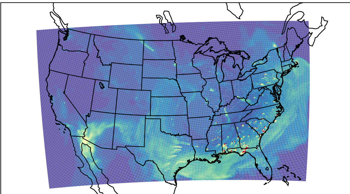
WRF 2023-04-24_20:00:00
