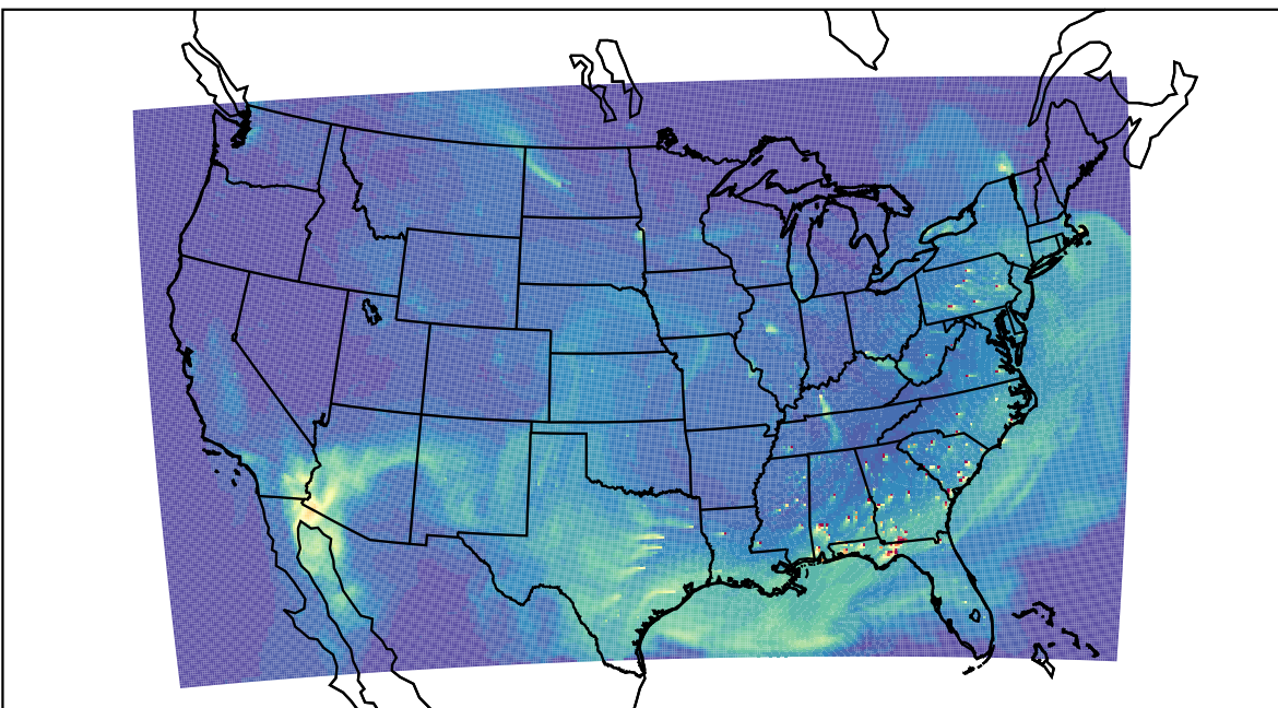
WRF 2023-04-24_19:00:00
