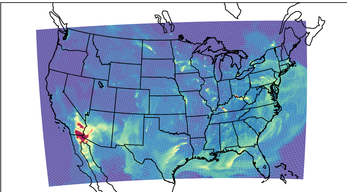
WRF 2023-04-24_12:00:00
