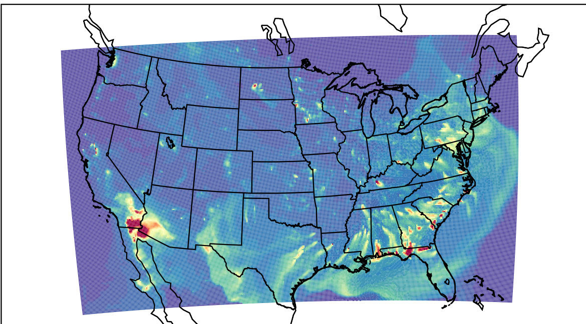
WRF 2023-04-24_03:00:00
