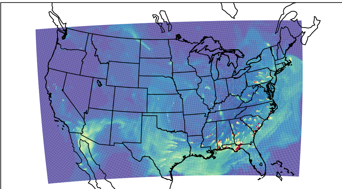
WRF 2023-04-24_22:00:00
