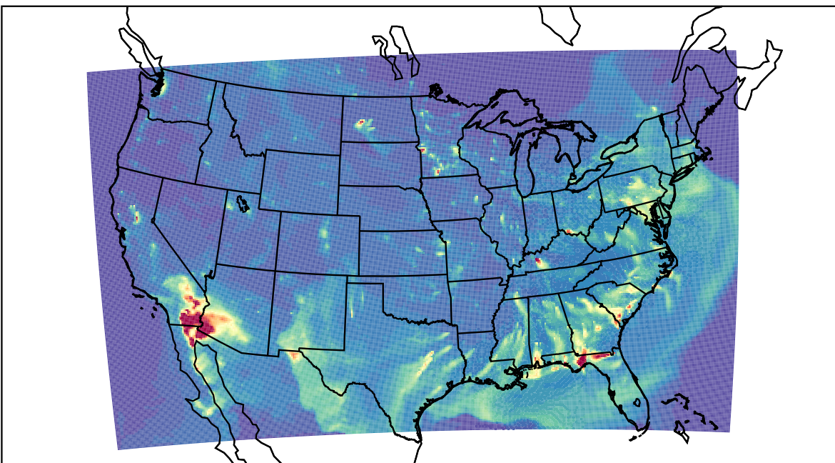
WRF 2023-04-24_04:00:00
