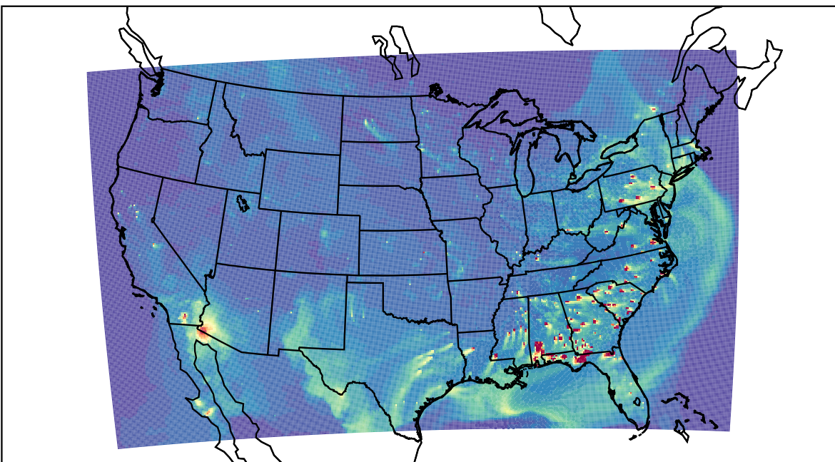
WRF 2023-04-24_00:00:00
