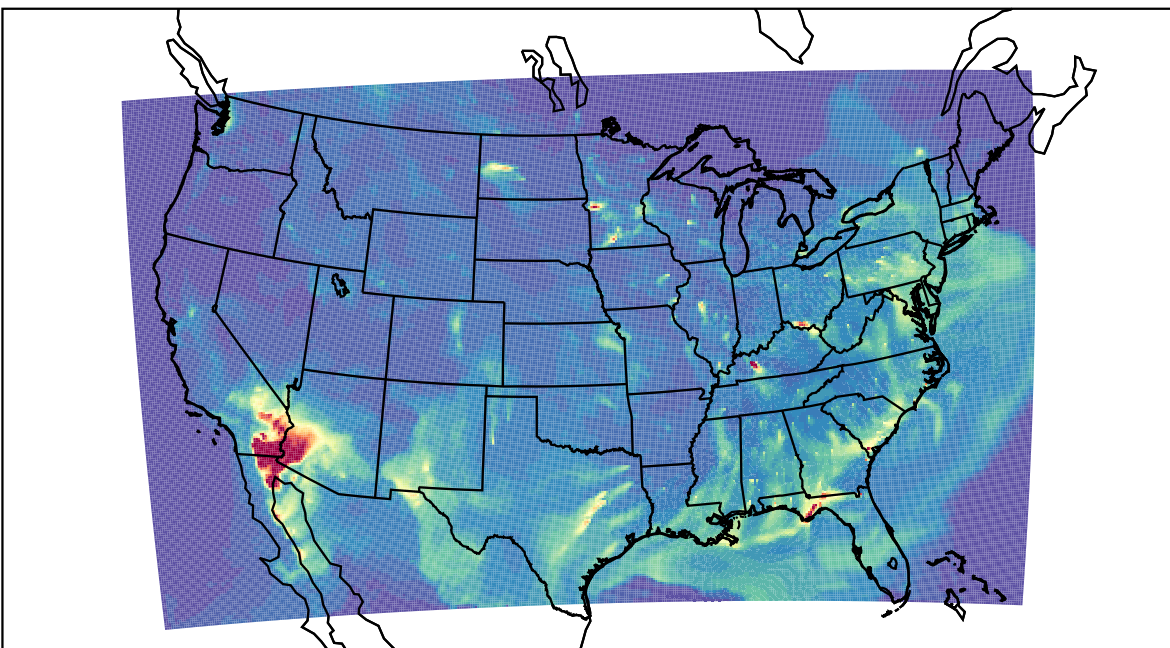
WRF 2023-04-24_07:00:00
