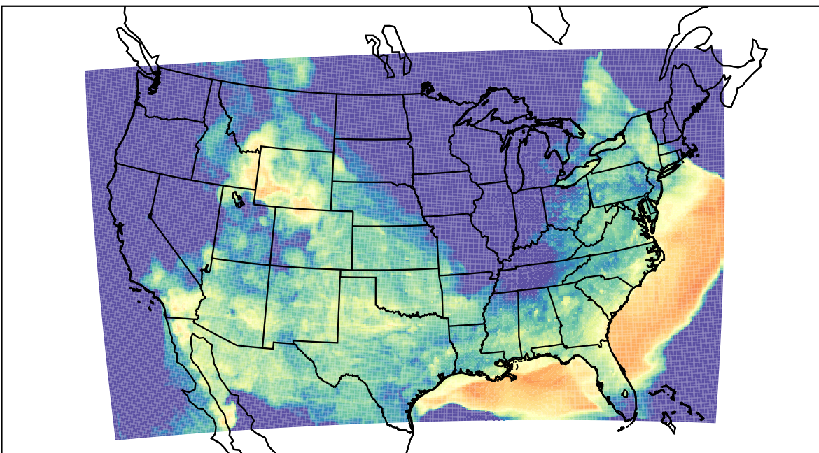
WRF (2023-04-24_05:00:00)
