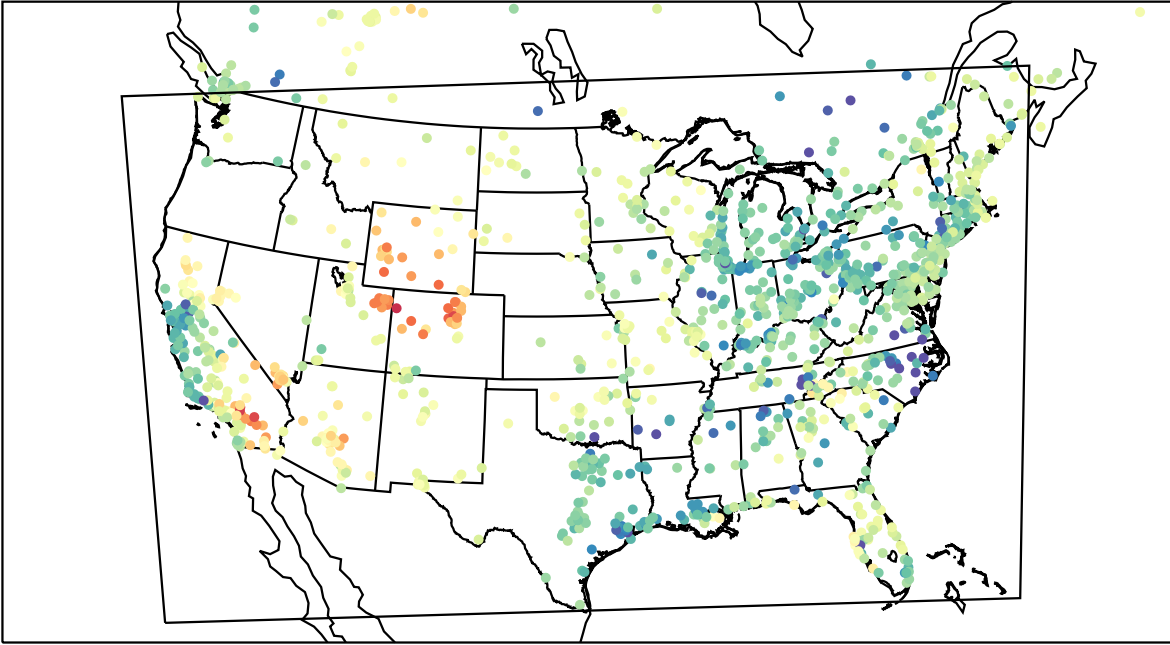
AirNOW (2023-04-24_01:00:00)
