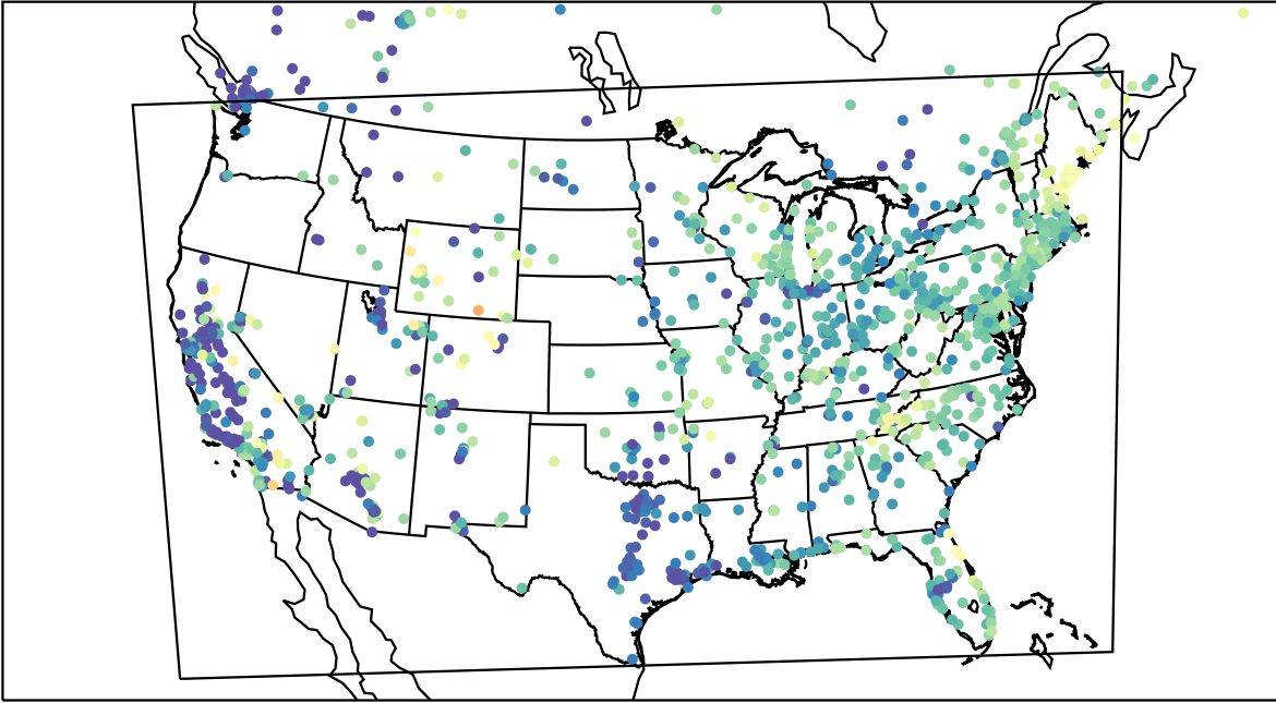
AirNOW (2023-04-24_13:00:00)
