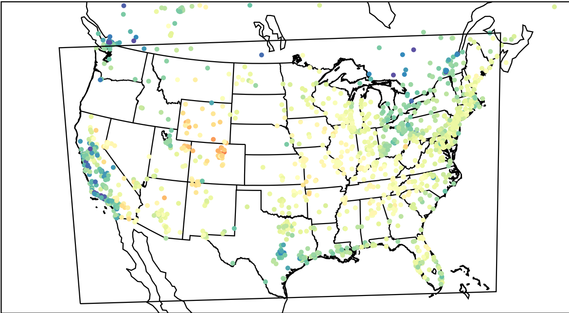
AirNOW (2023-04-24_17:00:00)
