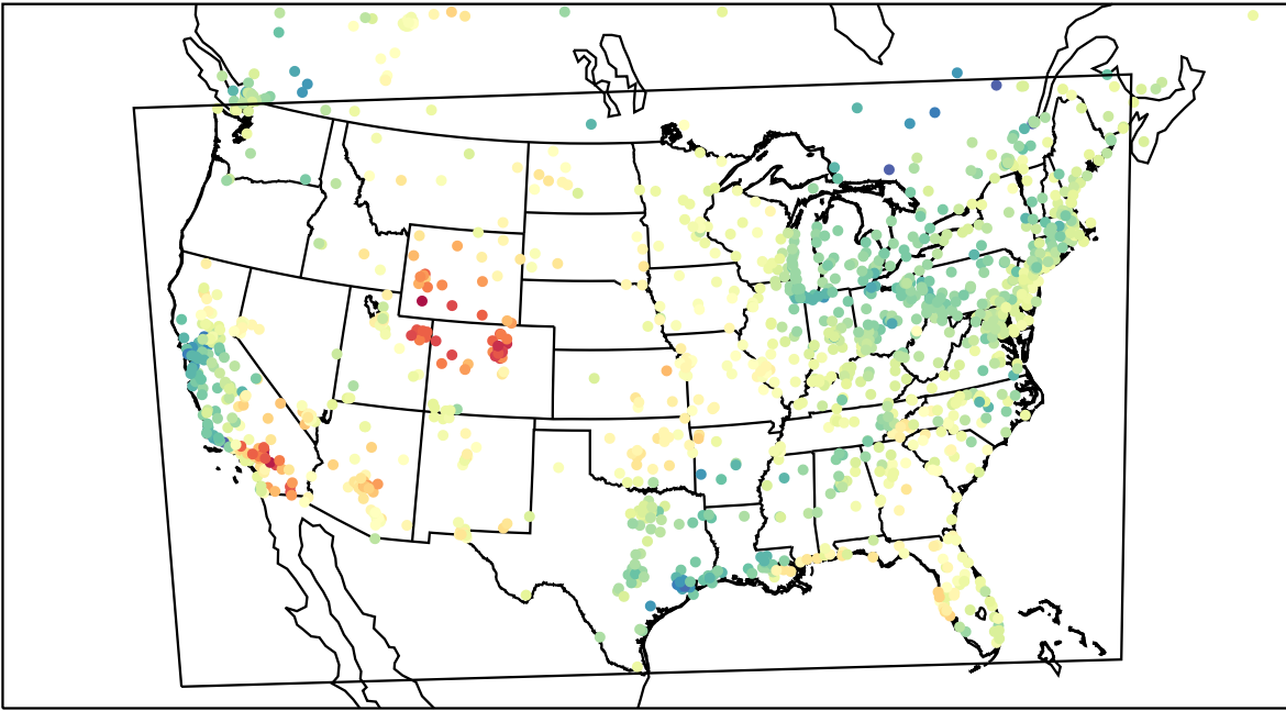
AirNOW (2023-04-23_23:00:00)
