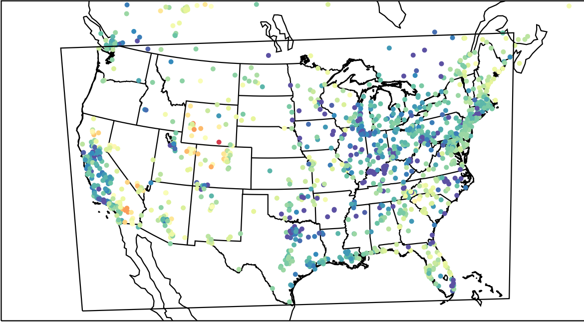
AirNOW (2023-04-24_04:00:00)
