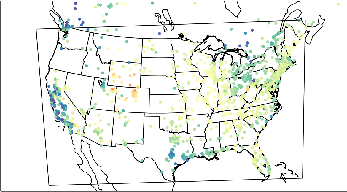
AirNOW (2023-04-24_16:00:00)
