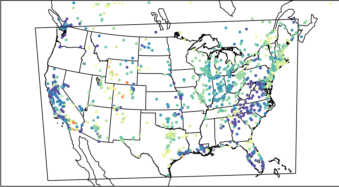
AirNOW (2023-04-23_06:00:00)
