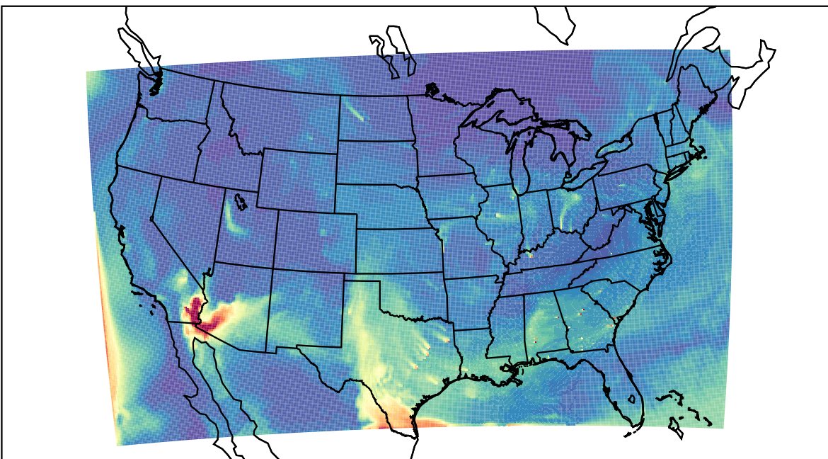
WRF 2023-04-25_17:00:00
