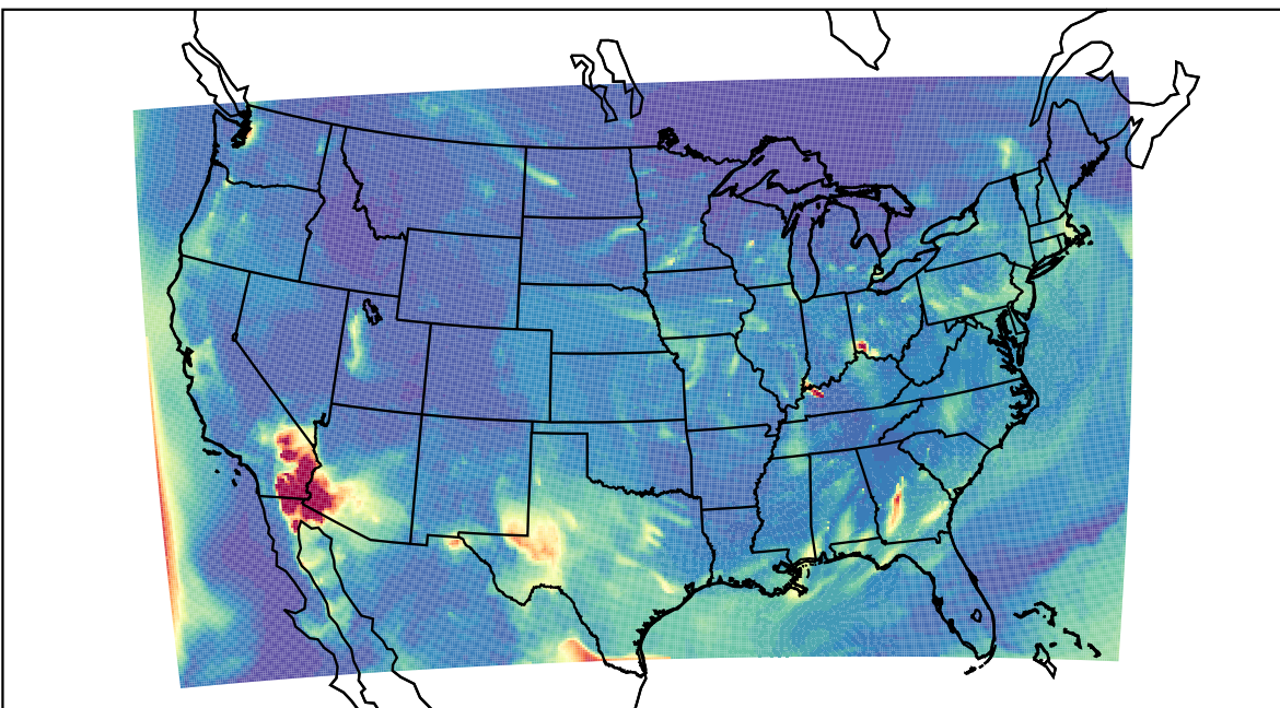
WRF 2023-04-25_06:00:00
