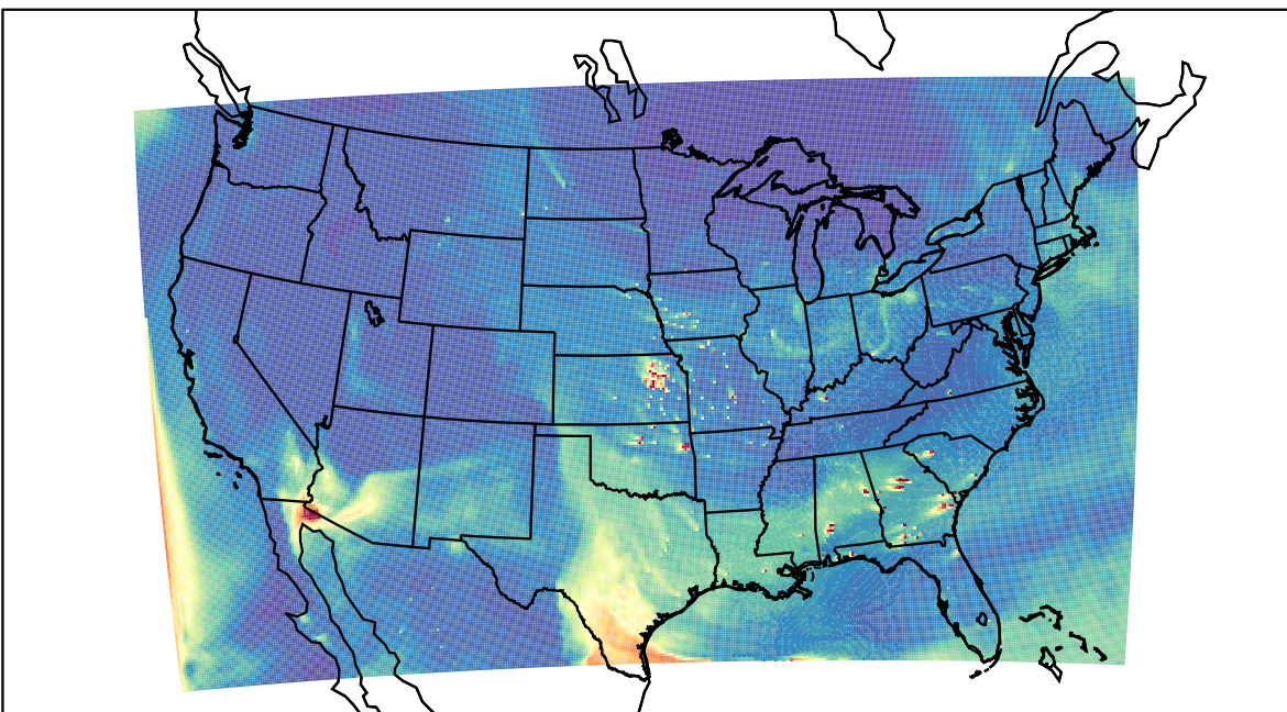
WRF 2023-04-25_22:00:00
