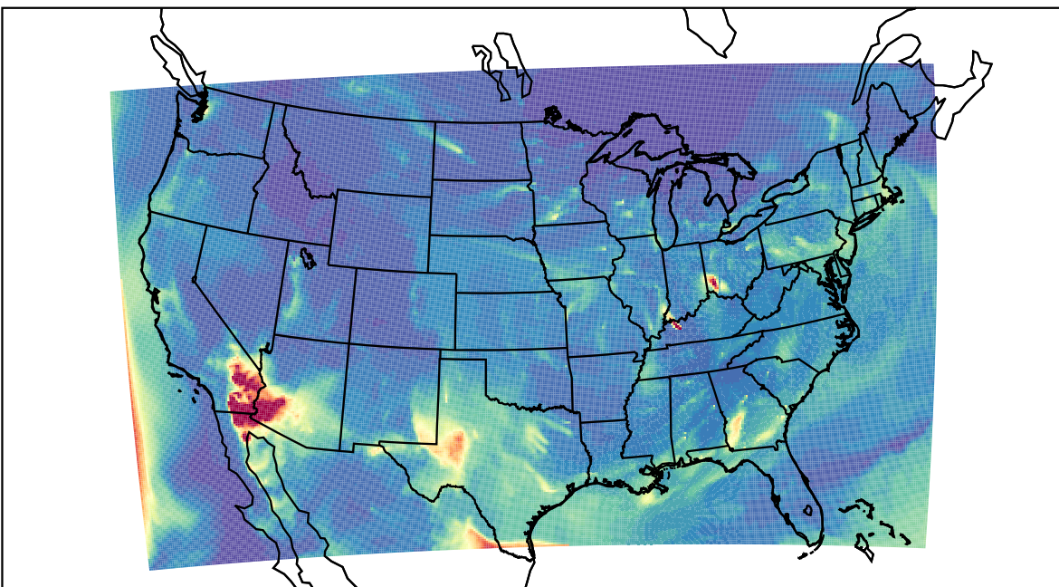
WRF 2023-04-25_08:00:00
