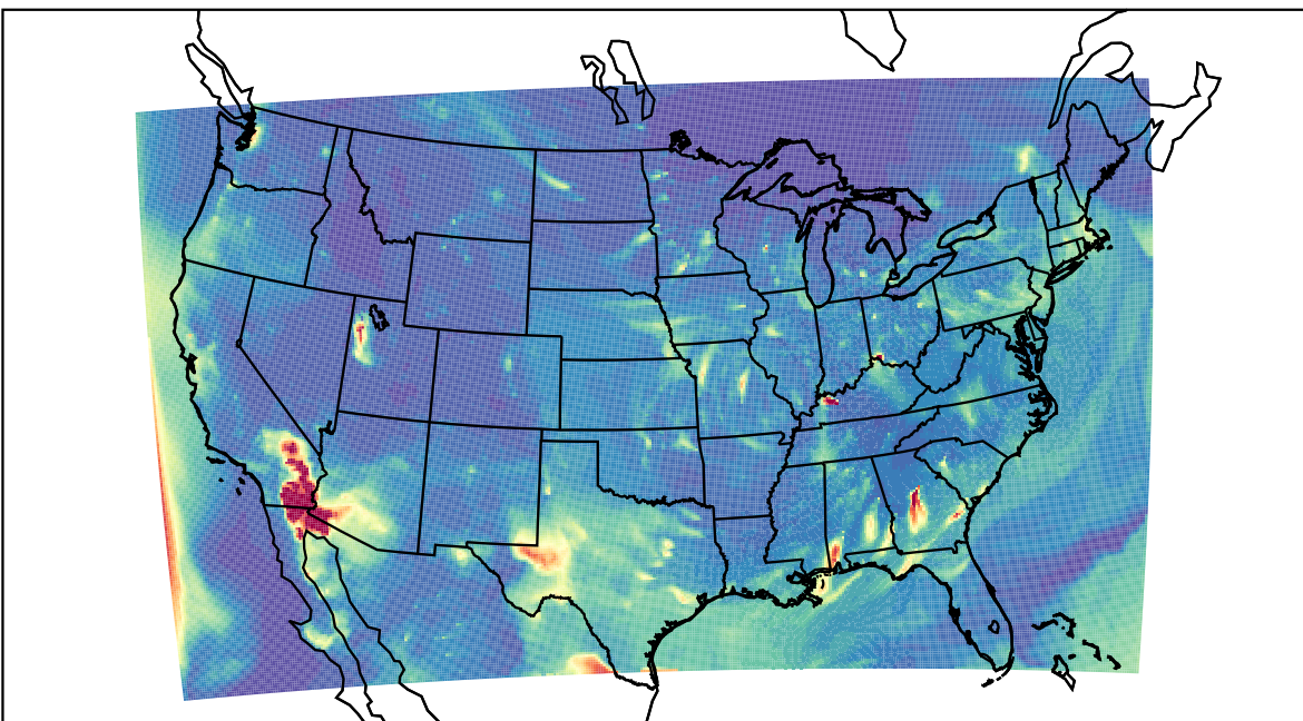
WRF 2023-04-25_04:00:00
