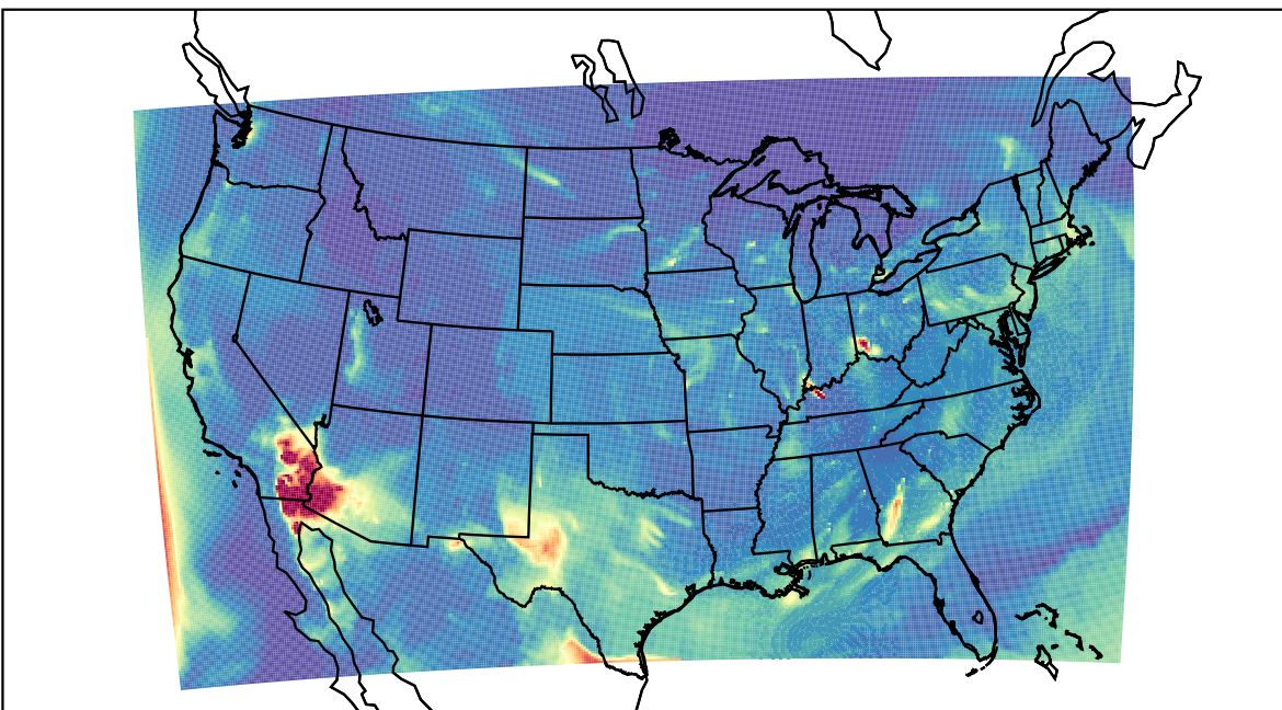
WRF 2023-04-25_07:00:00
