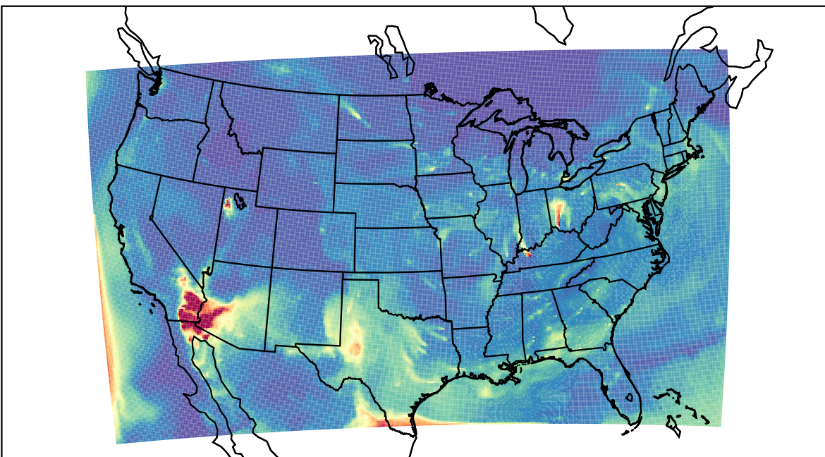
WRF 2023-04-25_12:00:00
