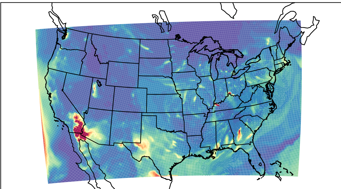
WRF 2023-04-25_05:00:00
