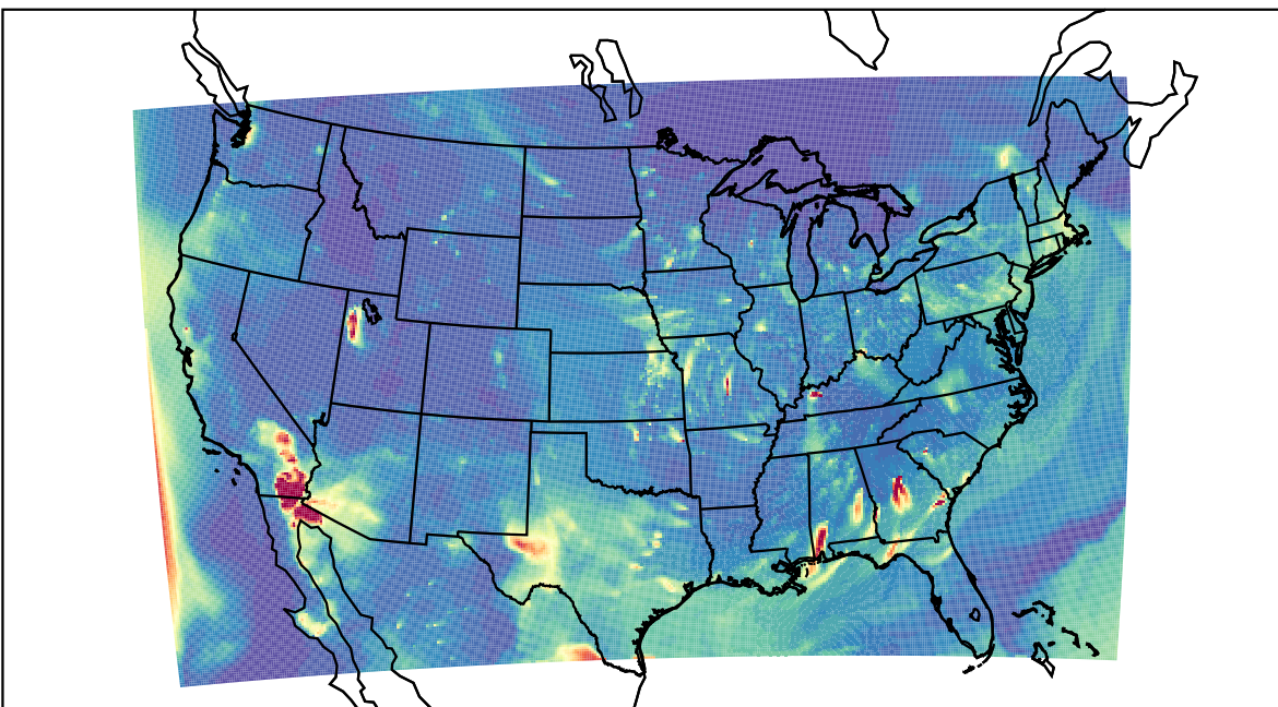
WRF 2023-04-25_03:00:00
