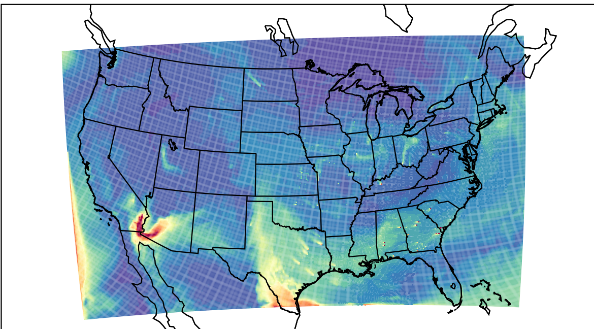
WRF 2023-04-25_18:00:00
