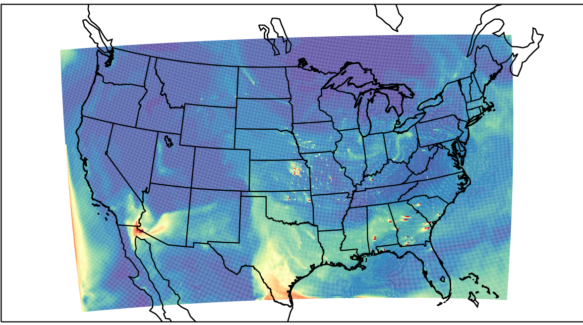
WRF 2023-04-25_21:00:00
