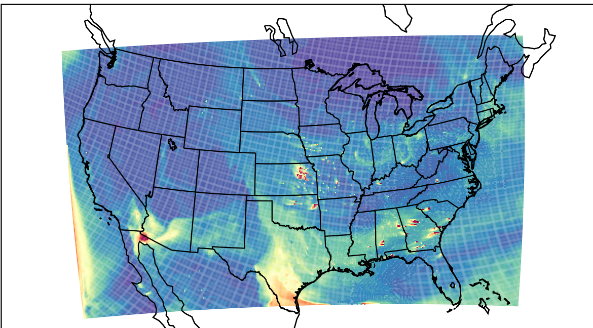
WRF 2023-04-25_23:00:00
