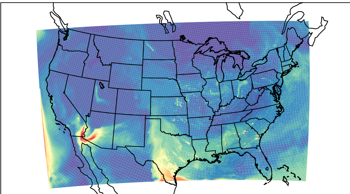
WRF 2023-04-25_19:00:00
