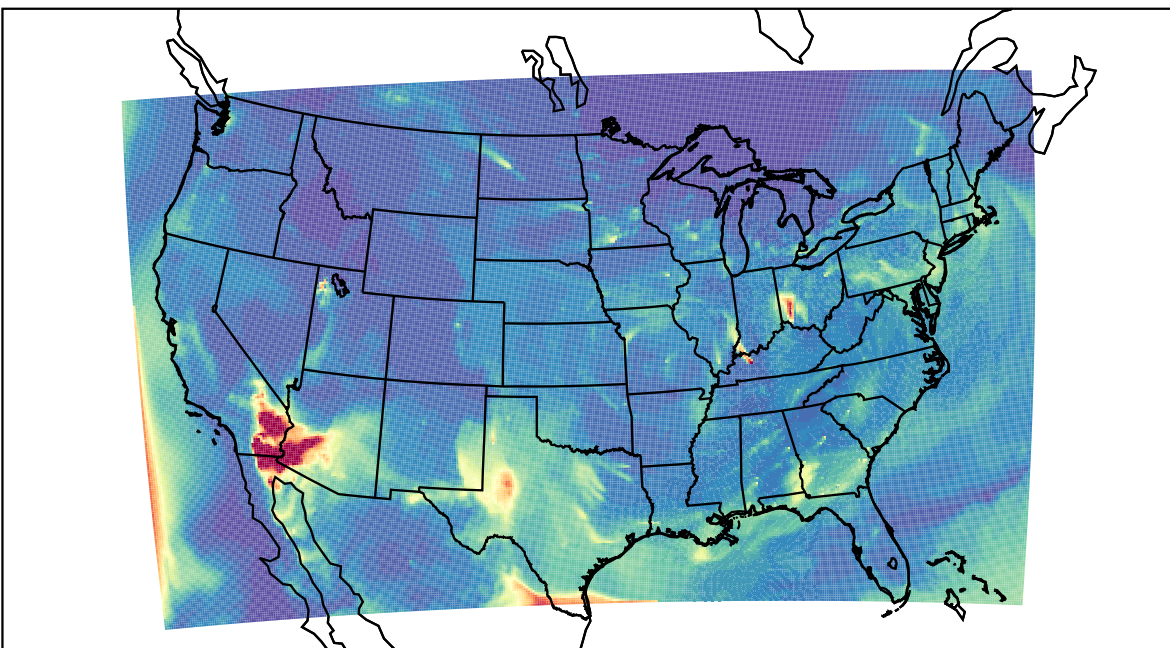
WRF 2023-04-25_10:00:00
