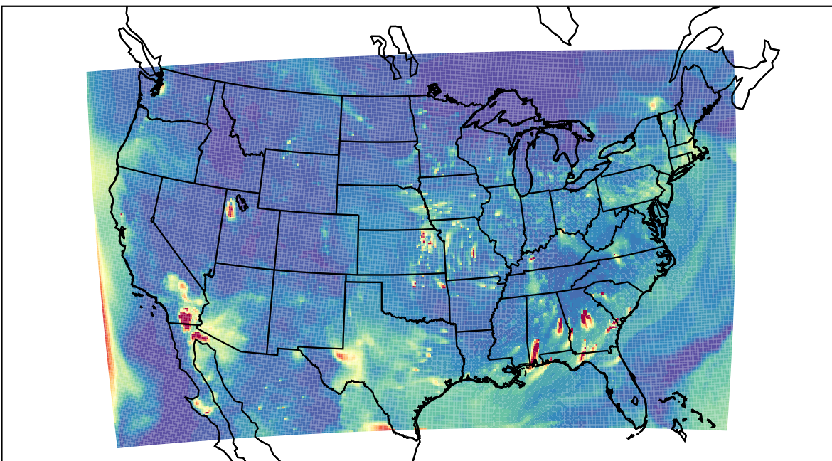
WRF 2023-04-25_02:00:00
