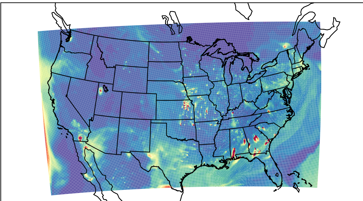
WRF 2023-04-25_01:00:00
