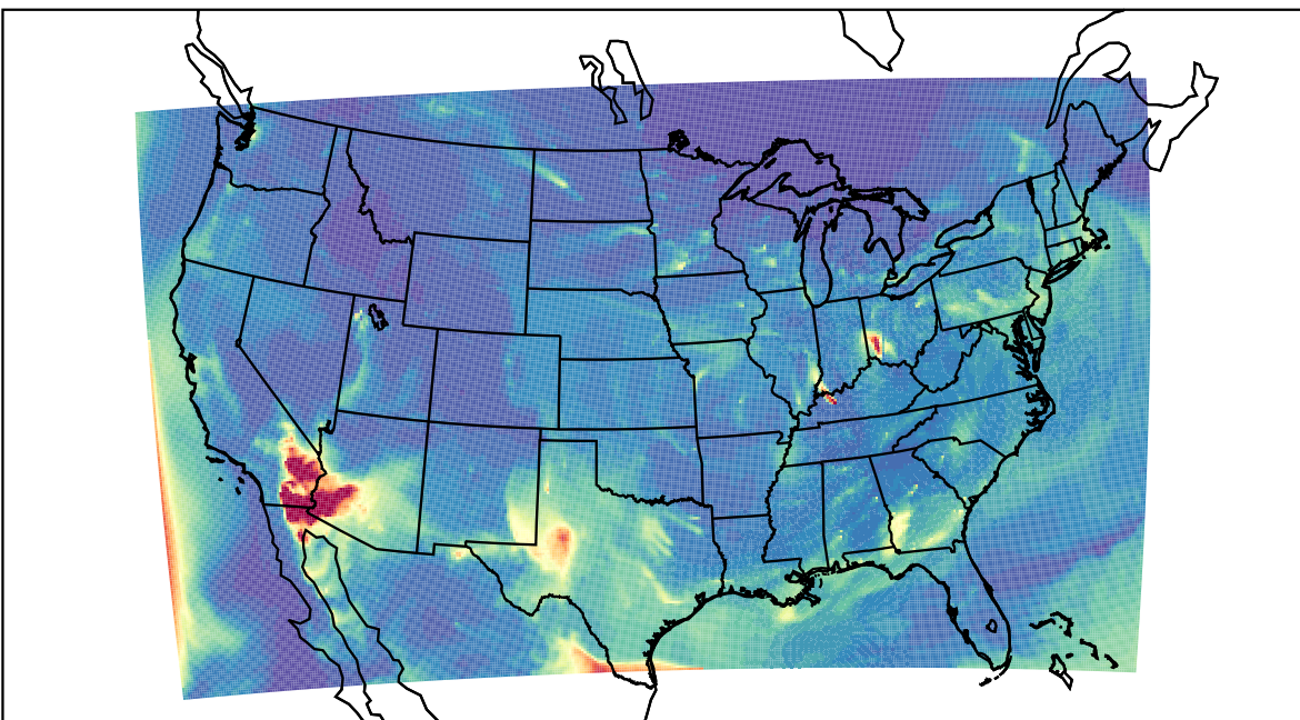
WRF 2023-04-25_09:00:00
