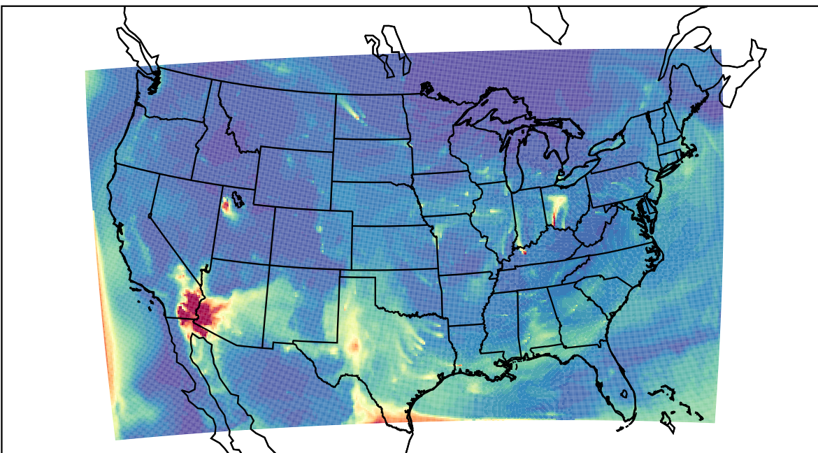
WRF 2023-04-25_14:00:00
