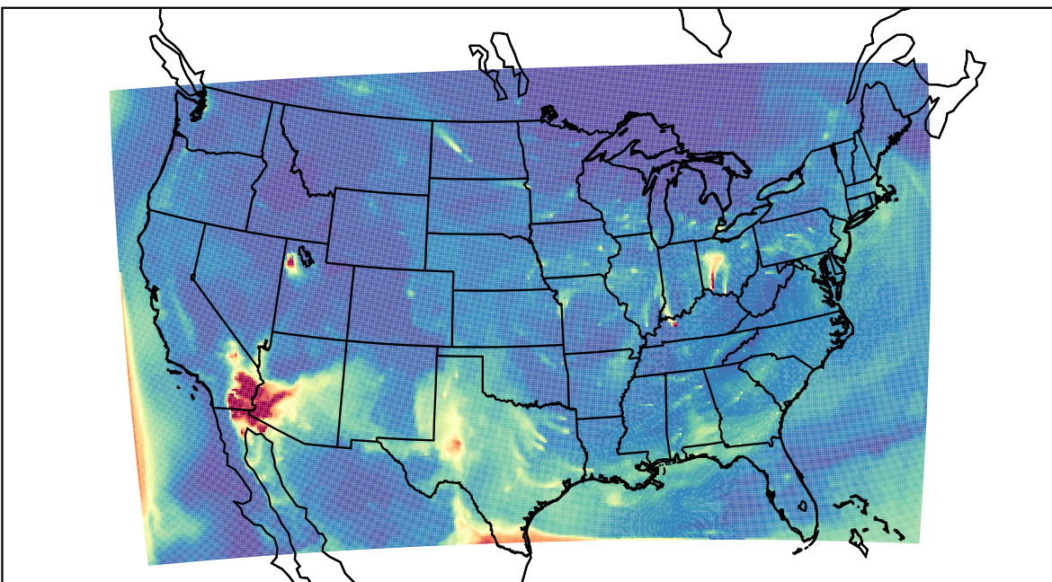
WRF 2023-04-25_13:00:00
