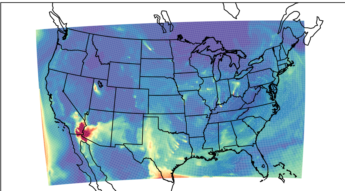
WRF 2023-04-25_15:00:00
