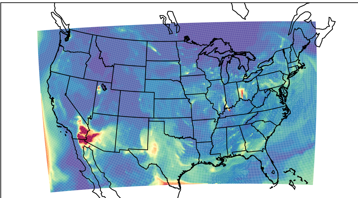
WRF 2023-04-25_11:00:00
