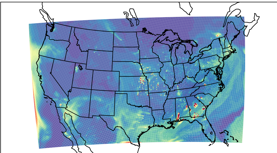
WRF 2023-04-25_00:00:00
