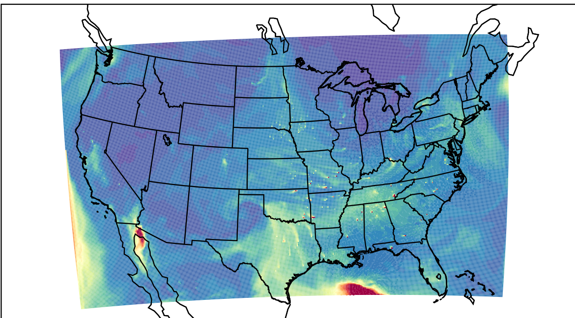
WRF 2023-04-26_20:00:00
