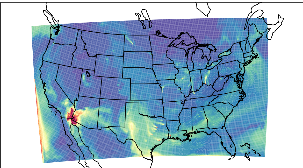
WRF 2023-04-25_16:00:00
