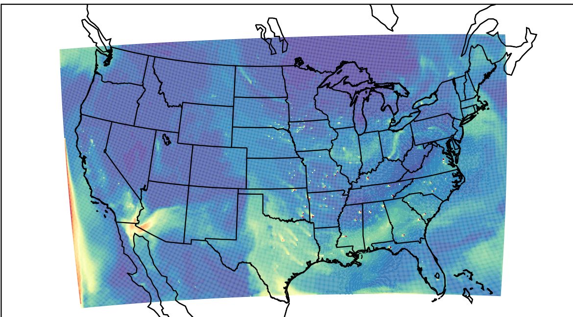
WRF 2023-04-25_21:00:00
